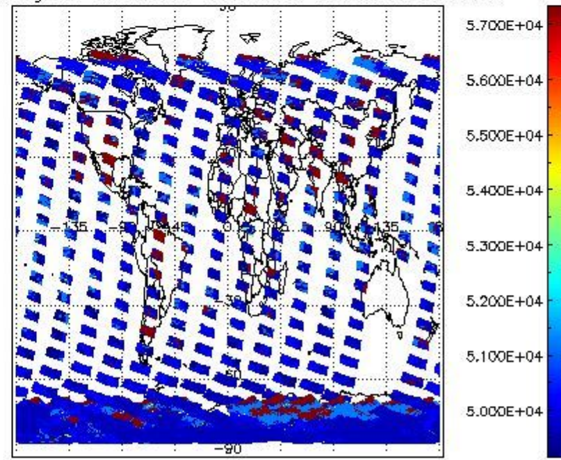
cloud_flags for 21NOV2002 00:00:00 to 22NOV2002 00:00:00
