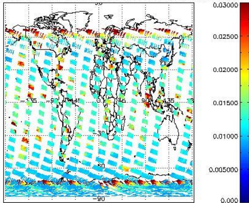
SCIOL2P_NADUV003_vcd_err for 21NOV2002 00:00:00 to 22NOV2002 00:00:00
