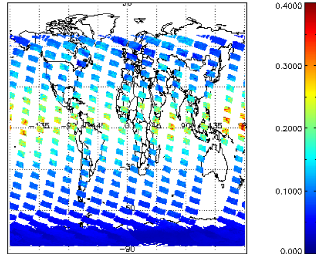
SCIOL2P_NADUV1NO2_vcd_err for 21NOV2002 00:00:00 to 22NOV2002 00:00:00
