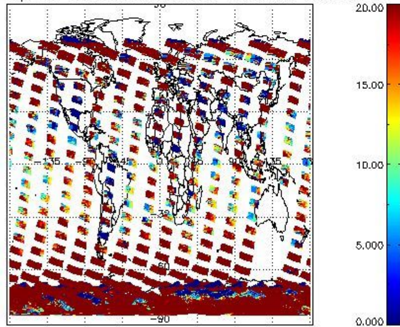
cLopt_depth for 21NOV2002 00:00:00 to 22NOV2002 00:00:00
