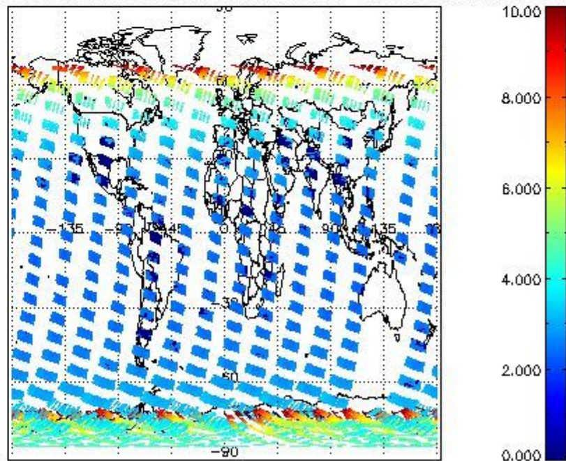
SCIOL2P_NADUV003_amf_cl for 21NOV2002 00:00:00 to 22NOV2002 00:00:00
