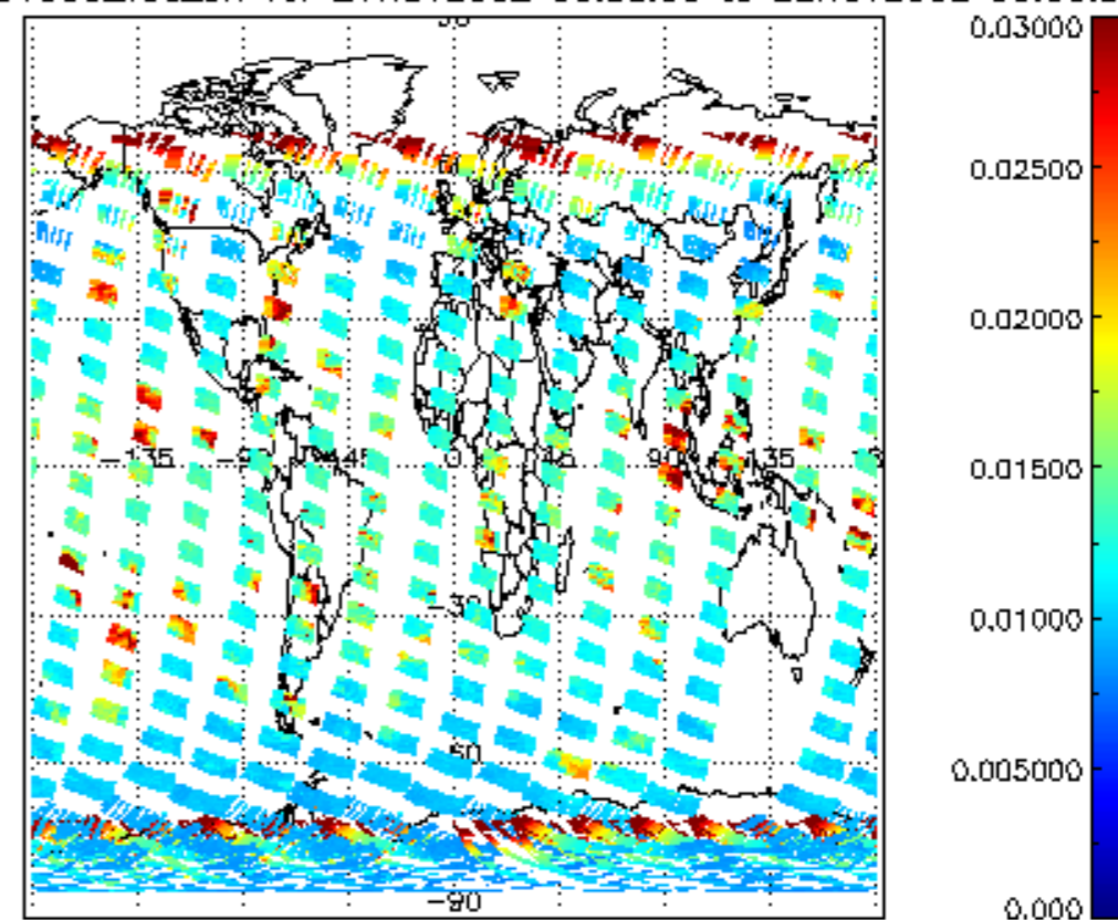
SCIOL2P_NADUV003_vcd_err for 21NOV2002 00:00:00 to 22NOV2002 00:00:00
