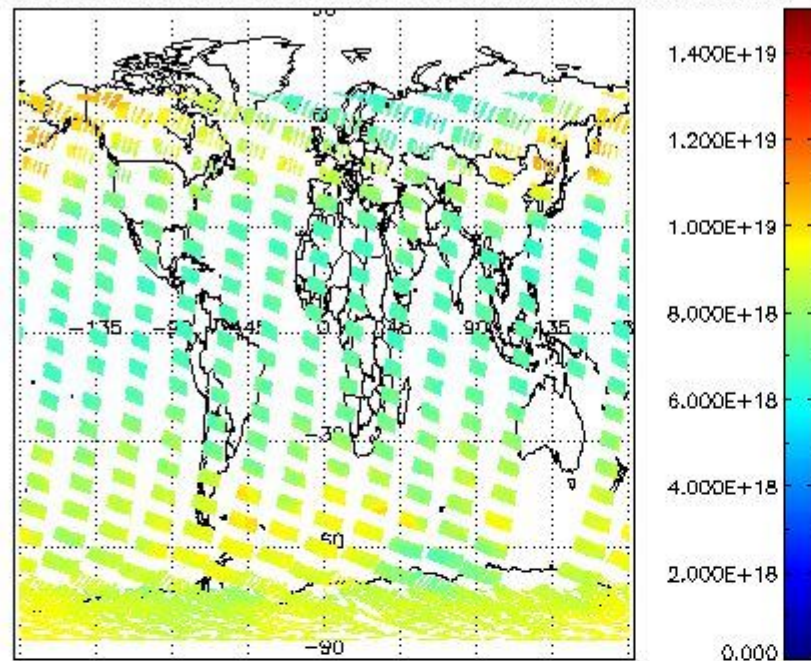
SCIOL2P_NADUV003_vcd for 21NOV2002 00:00:00 to 22NOV2002 00:00:00
