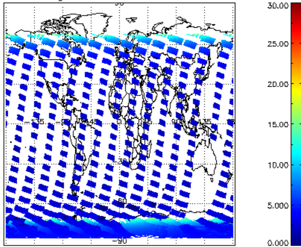
SCIOL2P_NADUV1NO2_amf_gr for 21NOV2002 00:00:00 to 22NOV2002 00:00:00
