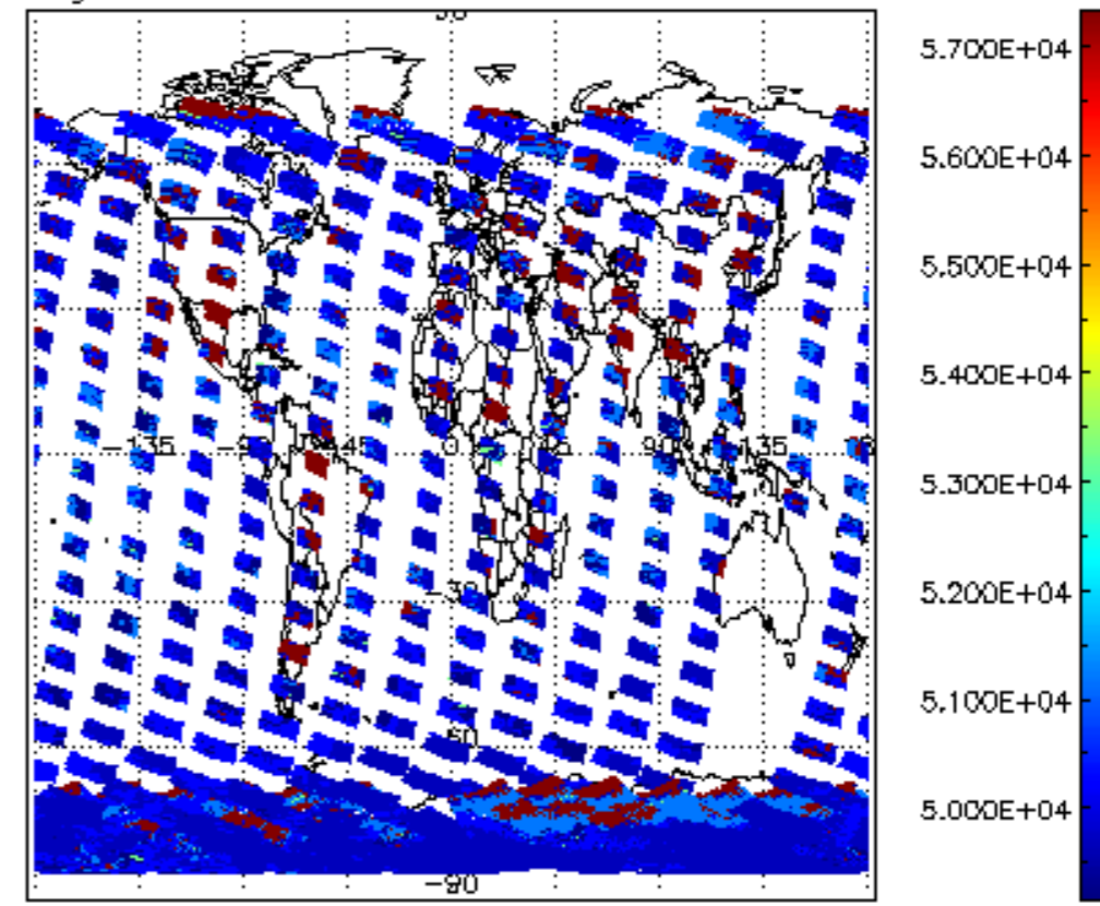
cloud_flags for 21NOV2002 00:00:00 to 22NOV2002 00:00:00
