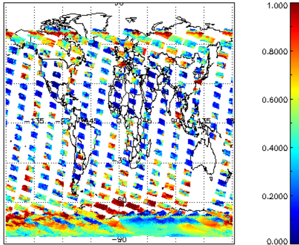
cLfrac for 21NOV2002 00:00:00 to 22NOV2002 00:00:00
