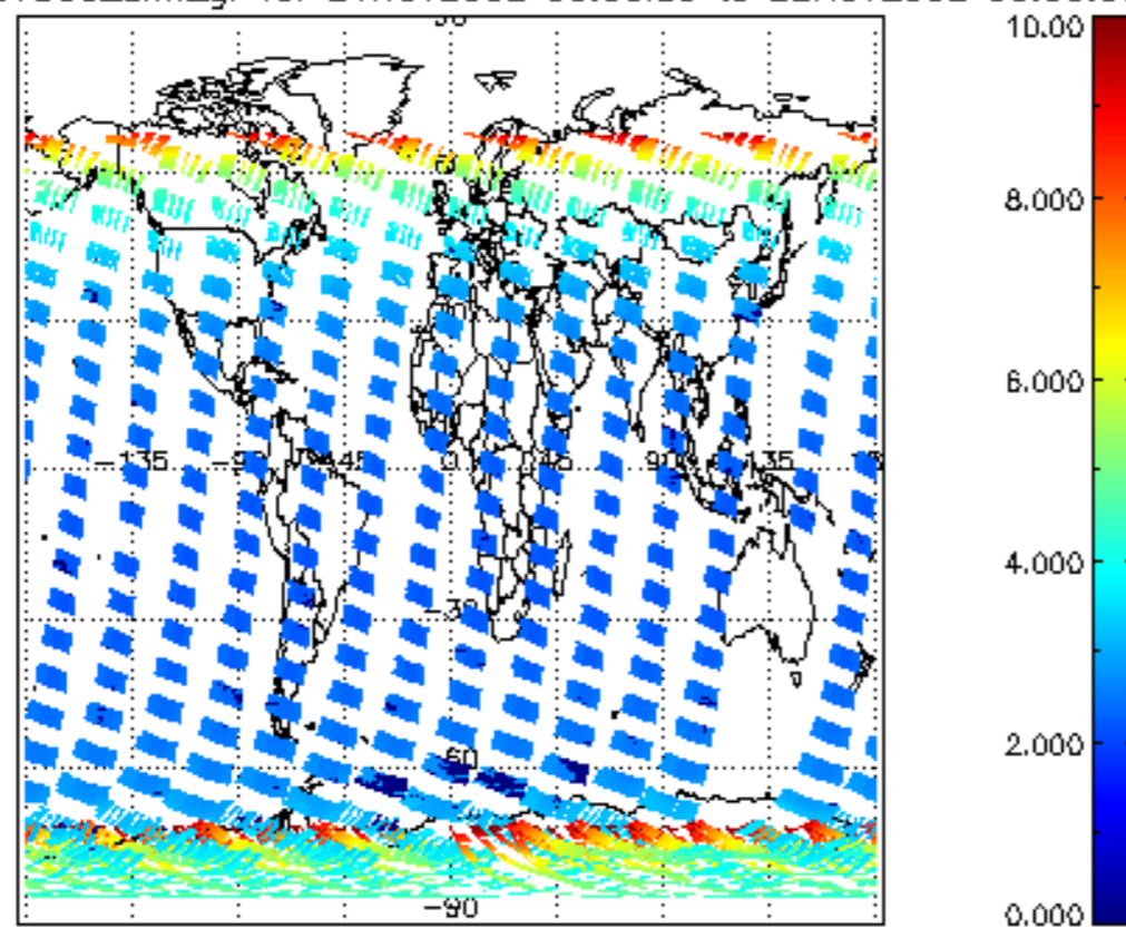
SCIOL2P_NADUV003_amf_gr for 21NOV2002 00:00:00 to 22NOV2002 00:00:00
