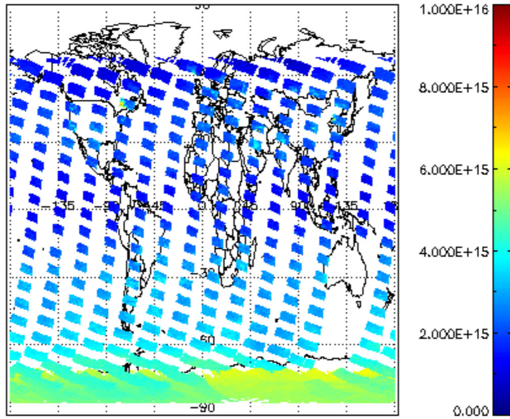
SCIOL2P_NADUV1NO2_vcd for 21NOV2002 00:00:00 to 22NOV2002 00:00:00
