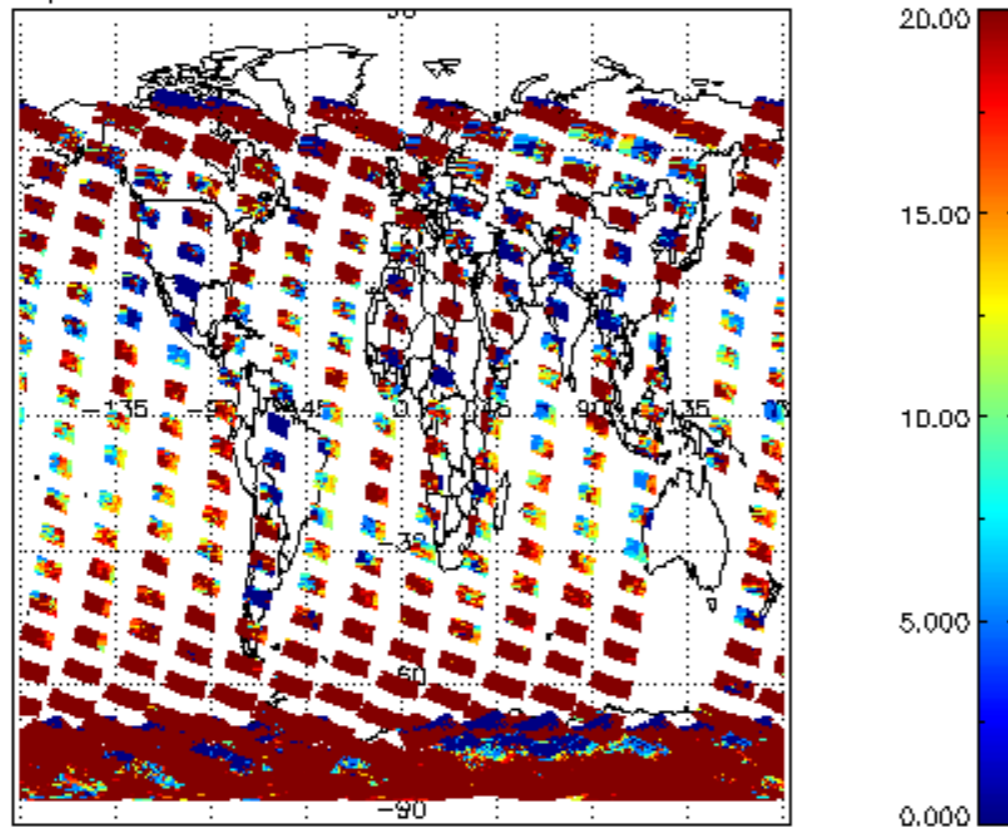
cL_opt_depth for 21NOV2002 00:00:00 to 22NOV2002 00:00:00
