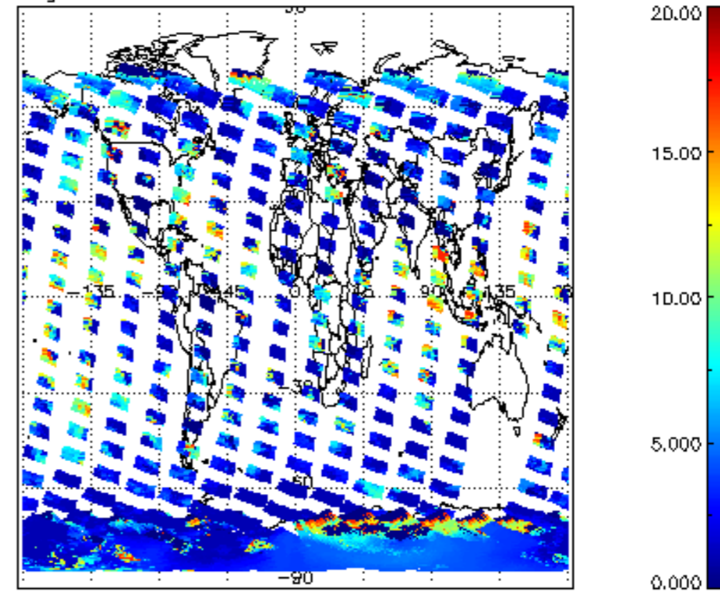
cL_top_height for 21NOV2002 00:00:00 to 22NOV2002 00:00:00
