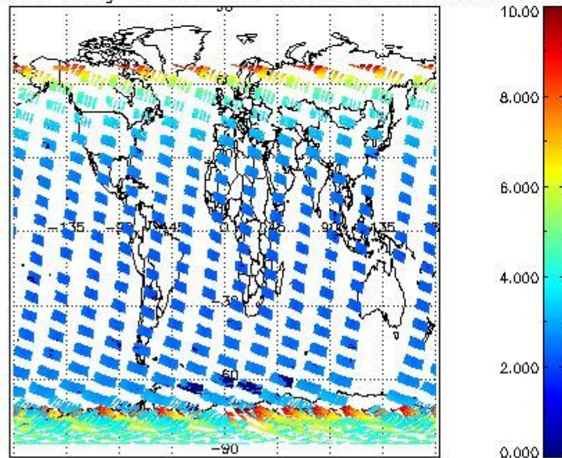
SCIOL2P_NADUV003_amf_gr for 21NOV2002 00:00:00 to 22NOV2002 00:00:00
