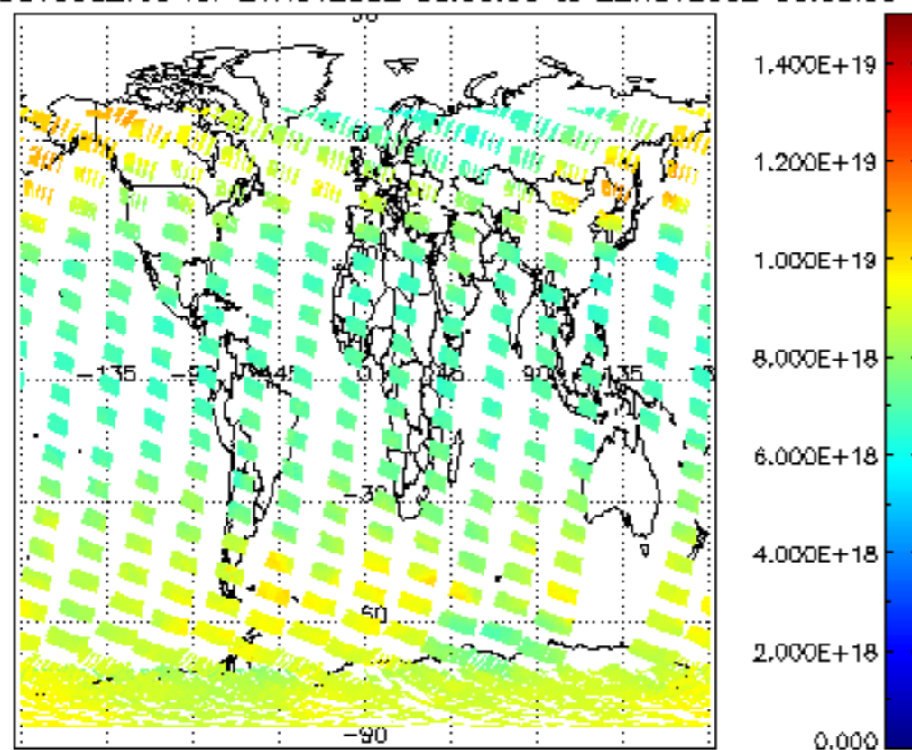
SCIOL2P_NADUV003_vcd for 21NOV2002 00:00:00 to 22NOV2002 00:00:00
