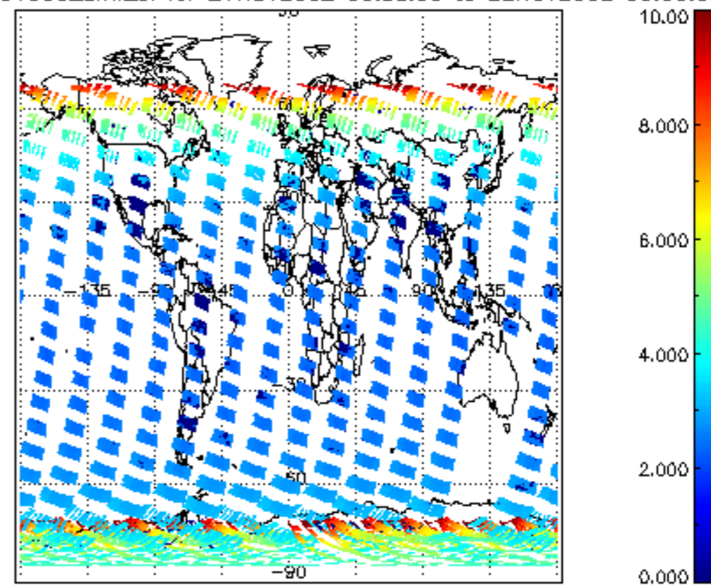
SCIOL2P_NADUV003_amf_cl for 21NOV2002 00:00:00 to 22NOV2002 00:00:00
