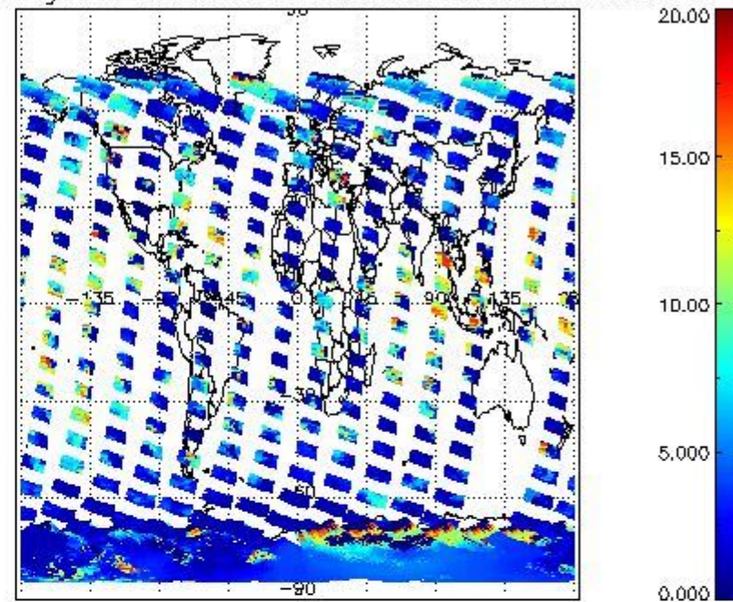
cL_top_height for 21NOV2002 00:00:00 to 22NOV2002 00:00:00
