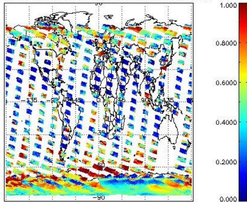
cLfrac for 21NOV2002 00:00:00 to 22NOV2002 00:00:00
