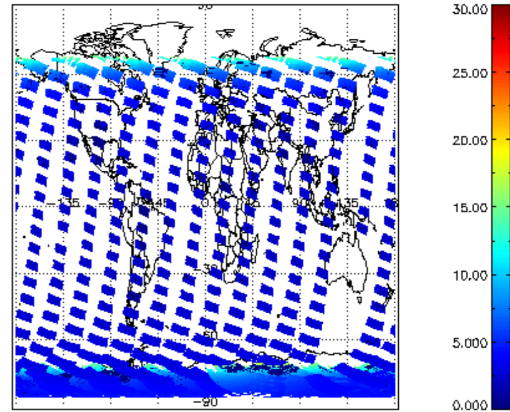
SCIOL2P_NADUV1NO2_amf_cl for 21NOV2002 00:00:00 to 22NOV2002 00:00:00
