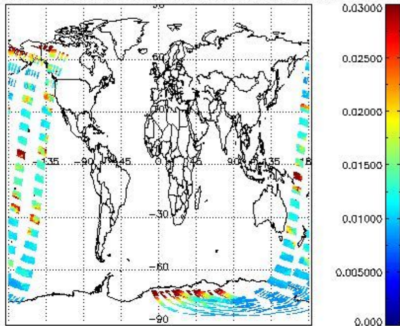
SCIOL2P_NADUV003_vcd_err for 20NOV2002 00:00:00 to 21NOV2002 00:00:00
