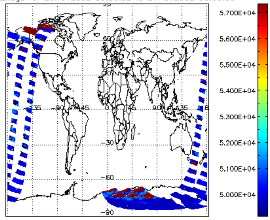
cloud_flags for 20NOV2002 00:00:00 to 21NOV2002 00:00:00
