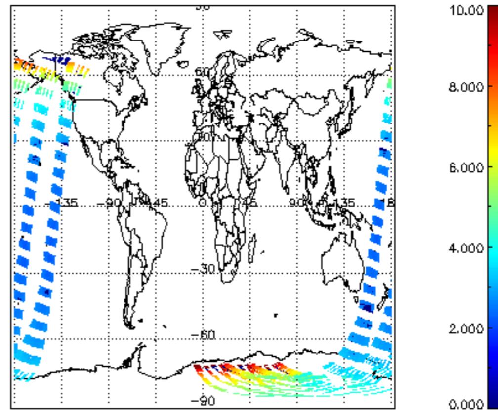
SCIOL2P_NADUV003_amf_cl for 20NOV2002 00:00:00 to 21NOV2002 00:00:00
