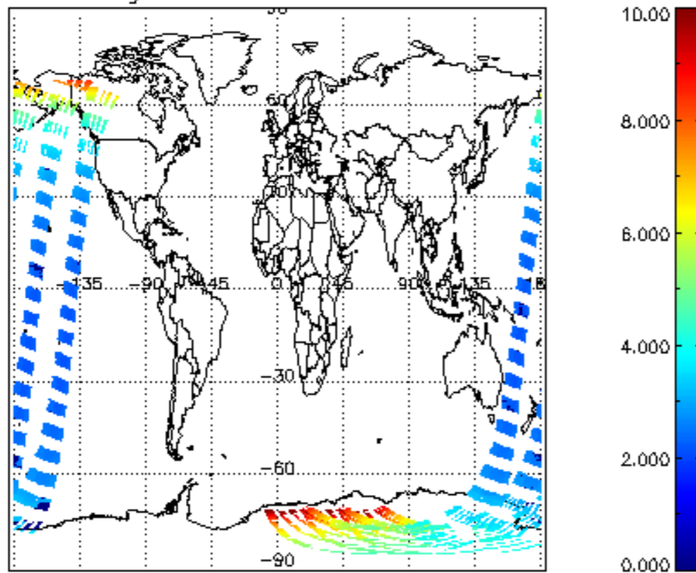
SCIOL2P_NADUV003_amf_gr for 20NOV2002 00:00:00 to 21NOV2002 00:00:00
