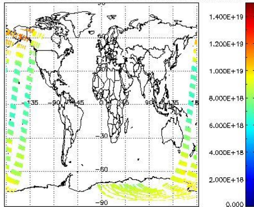
SCIOL2P_NADUV003_vcd for 20NOV2002 00:00:00 to 21NOV2002 00:00:00
