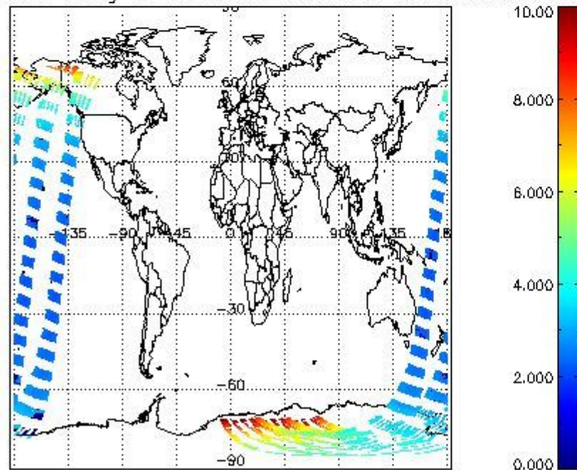
SCIOL2P_NADUV003_amf_gr for 20NOV2002 00:00:00 to 21NOV2002 00:00:00
