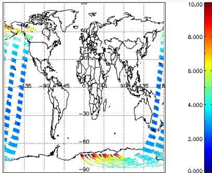
SCIOL2P_NADUV003_amf_cl for 20NOV2002 00:00:00 to 21NOV2002 00:00:00
