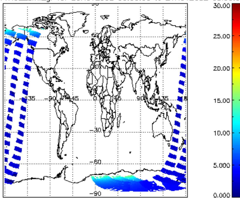
SCIOL2P_NADUV1NO2_amf_gr for 20NOV2002 00:00:00 to 21NOV2002 00:00:00
