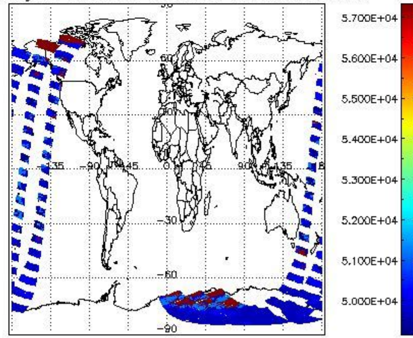
cloud_flags for 20NOV2002 00:00:00 to 21NOV2002 00:00:00
