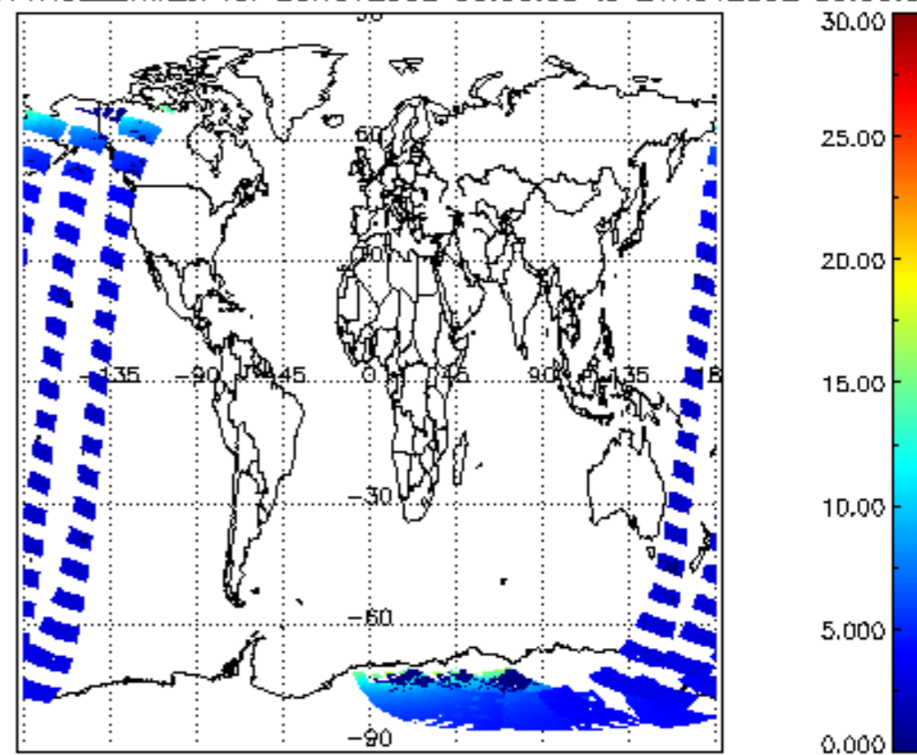
SCIOL2P_NADUV1NO2_amf_cl for 20NOV2002 00:00:00 to 21NOV2002 00:00:00
