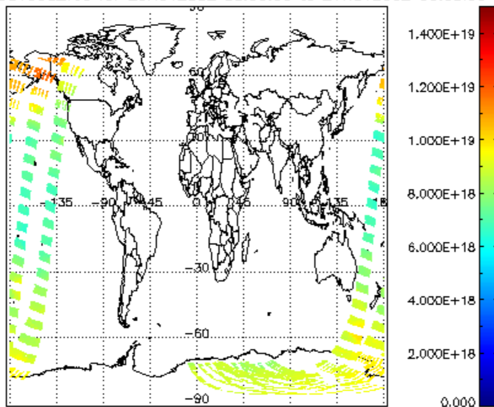
SCIOL2P_NADUV003_vcd for 20NOV2002 00:00:00 to 21NOV2002 00:00:00
