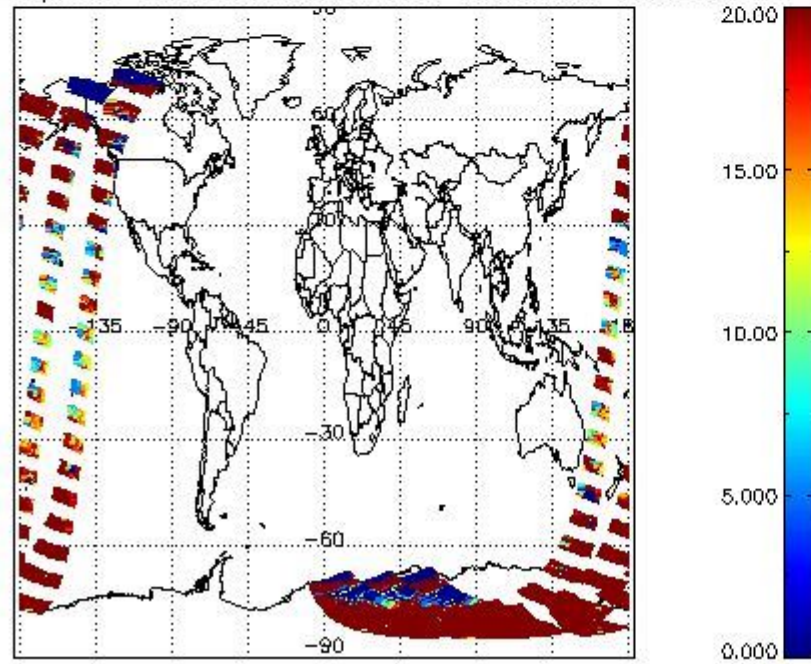
cLopt_depth for 20NOV2002 00:00:00 to 21NOV2002 00:00:00
