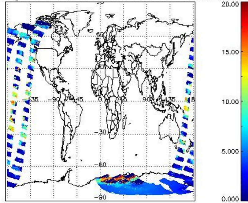
cL_top_height for 20NOV2002 00:00:00 to 21NOV2002 00:00:00
