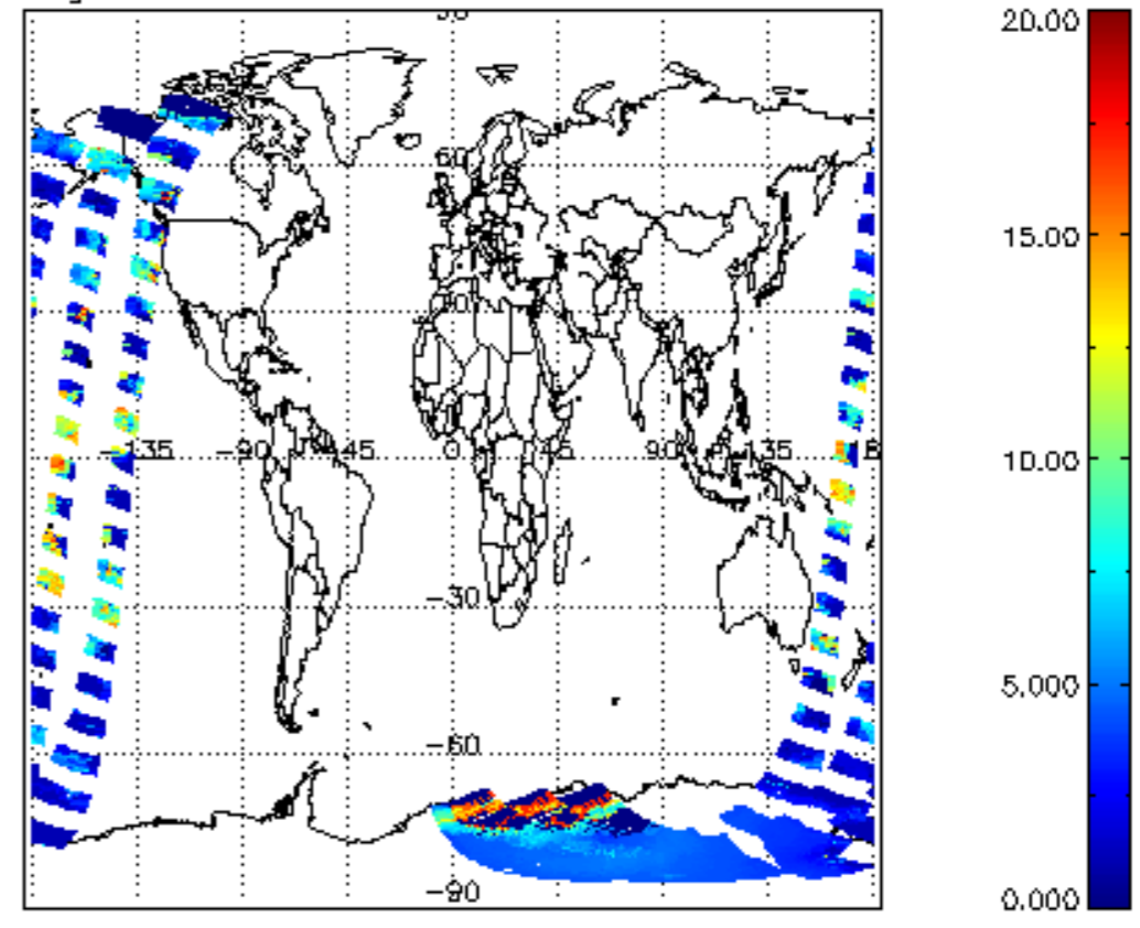
cL_top_height for 20NOV2002 00:00:00 to 21NOV2002 00:00:00
