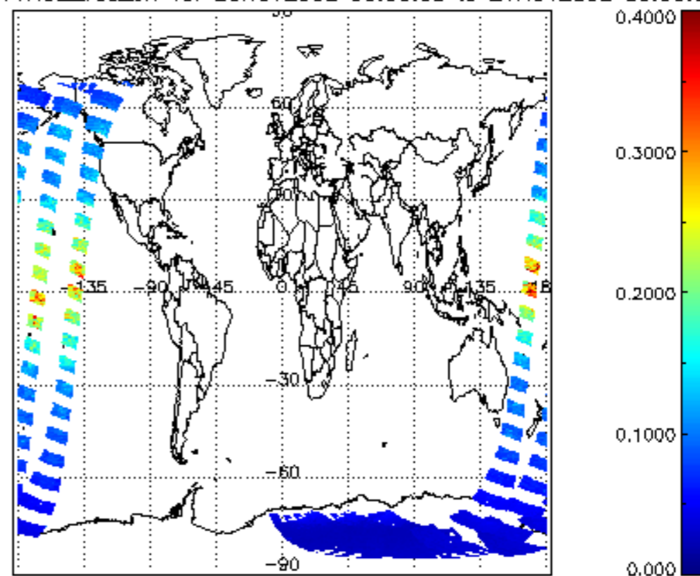
SCIOL2P_NADUV1NO2_vcd_err for 20NOV2002 00:00:00 to 21NOV2002 00:00:00
