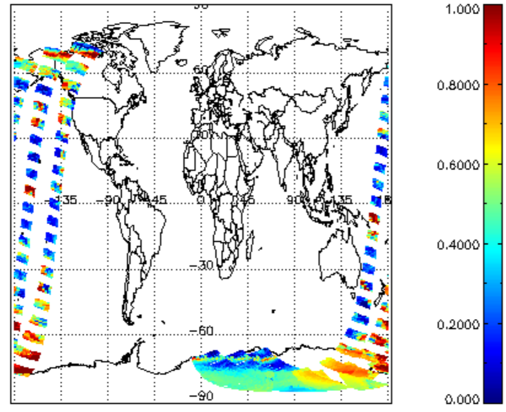
cLfrac for 20NOV2002 00:00:00 to 21NOV2002 00:00:00
