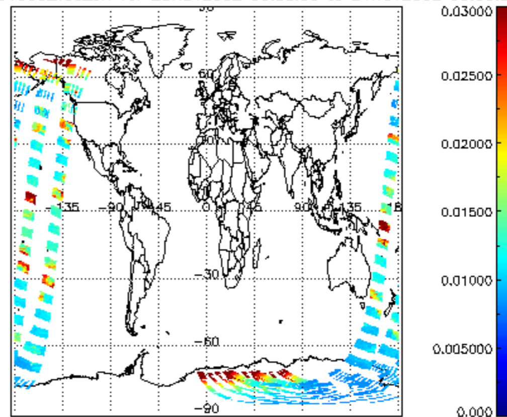
SCIOL2P_NADUV003_vcd_err for 20NOV2002 00:00:00 to 21NOV2002 00:00:00
