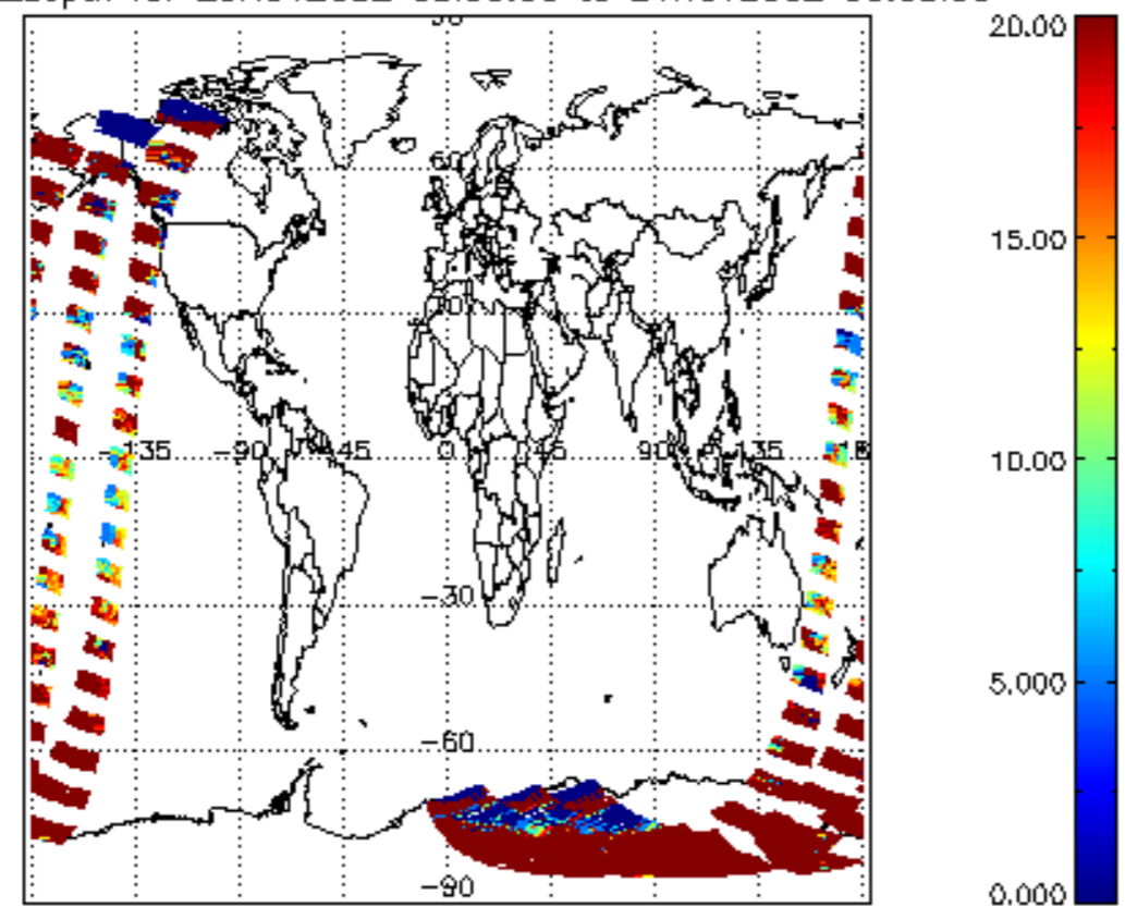
cL_opt_depth for 20NOV2002 00:00:00 to 21NOV2002 00:00:00
