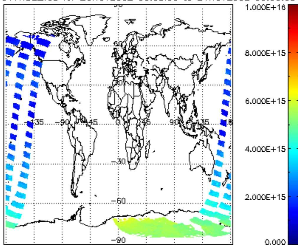
SCIOL2P_NADUV1NO2_vcd for 20NOV2002 00:00:00 to 21NOV2002 00:00:00
