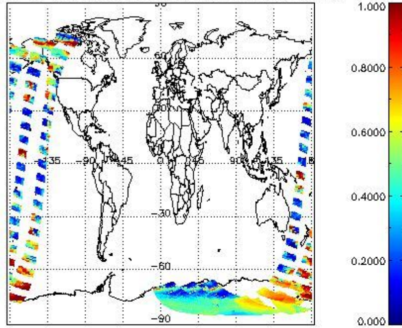
cLfrac for 20NOV2002 00:00:00 to 21NOV2002 00:00:00
