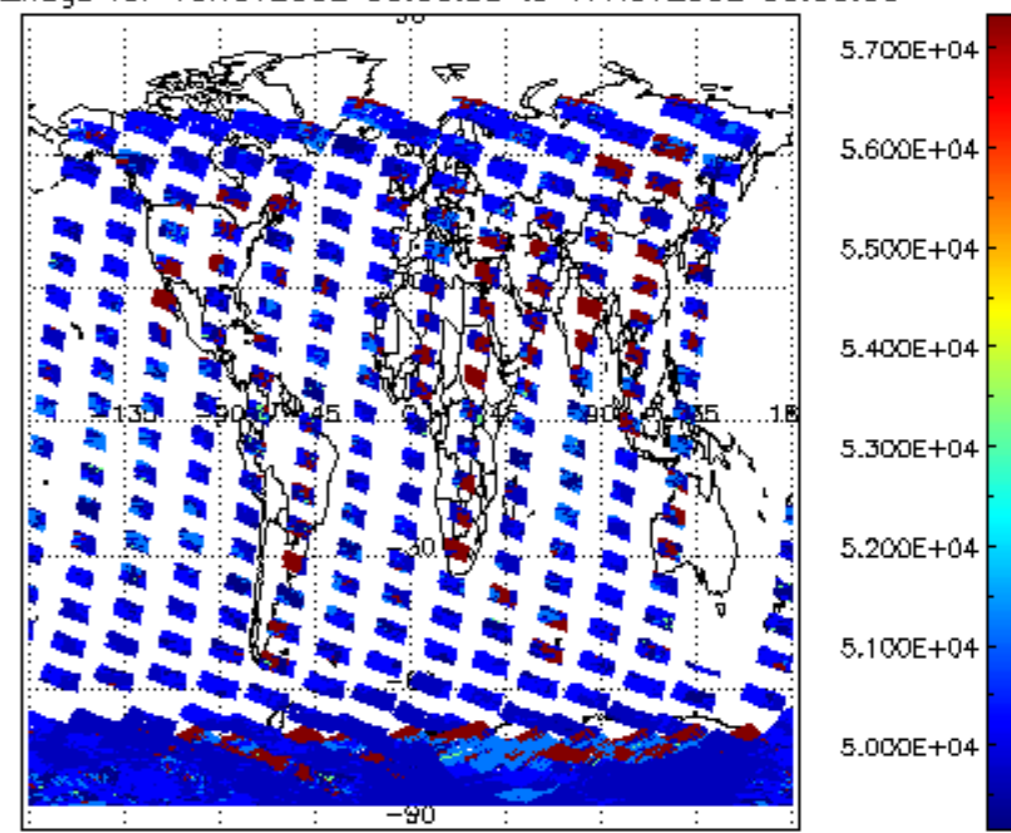
cloud_flags for 16NOV2002 00:00:00 to 17NOV2002 00:00:00
