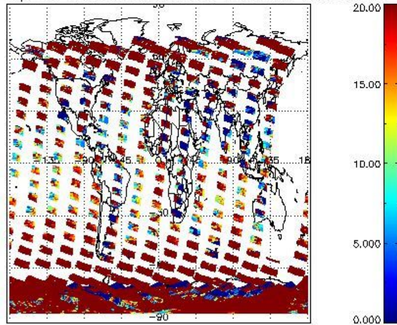
cL_opt_depth for 16NOV2002 00:00:00 to 17NOV2002 00:00:00
