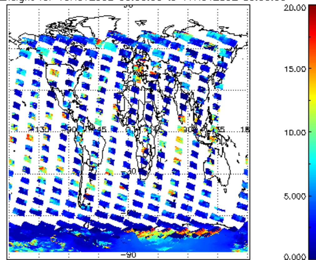
cL_top_height for 16NOV2002 00:00:00 to 17NOV2002 00:00:00
