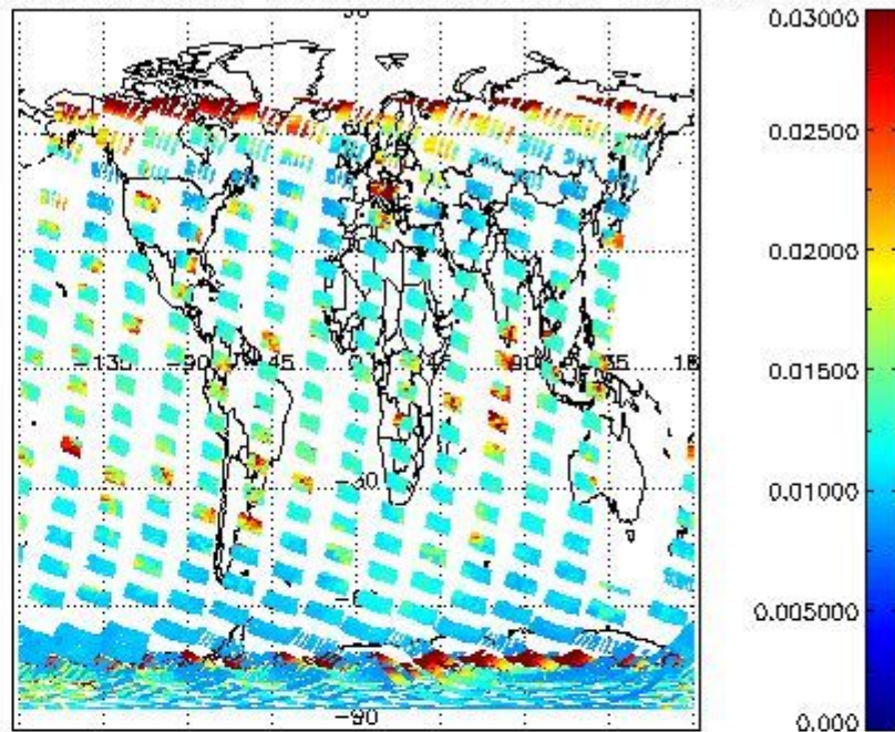
SCIOL2P_NADUV003_vcd_err for 16NOV2002 00:00:00 to 17NOV2002 00:00:00
