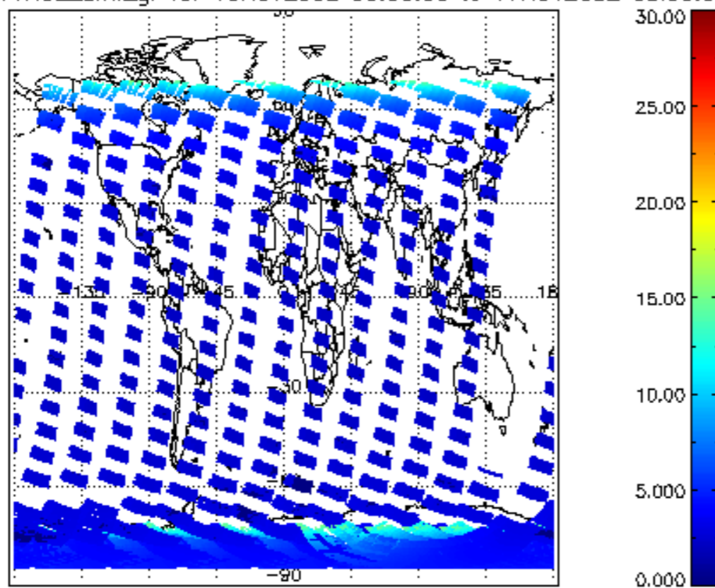
SCIOL2P_NADUV1NO2_amf_gr for 16NOV2002 00:00:00 to 17NOV2002 00:00:00
