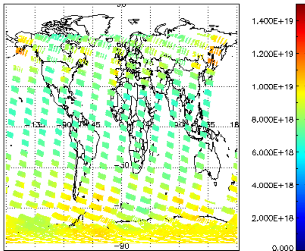
SCIOL2P_NADUV003_vcd for 16NOV2002 00:00:00 to 17NOV2002 00:00:00
