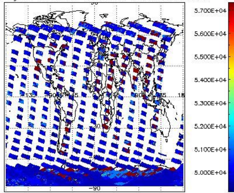
cloud_flags for 16NOV2002 00:00:00 to 17NOV2002 00:00:00
