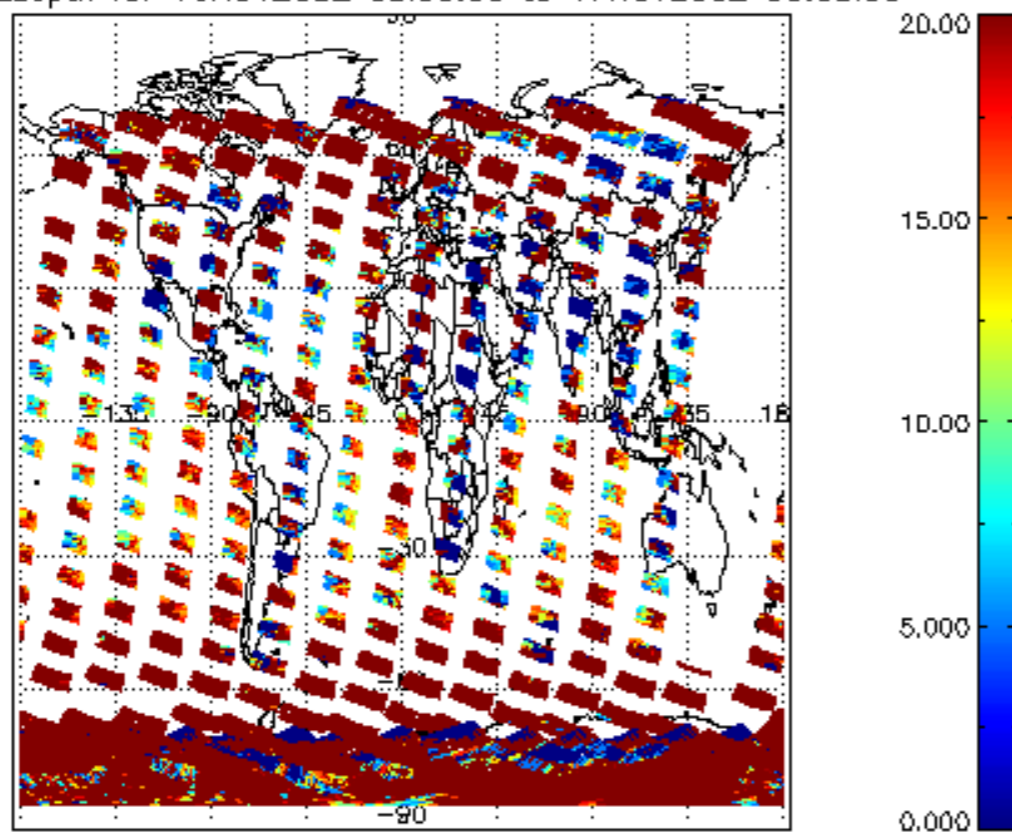
cL_opt_depth for 16NOV2002 00:00:00 to 17NOV2002 00:00:00
