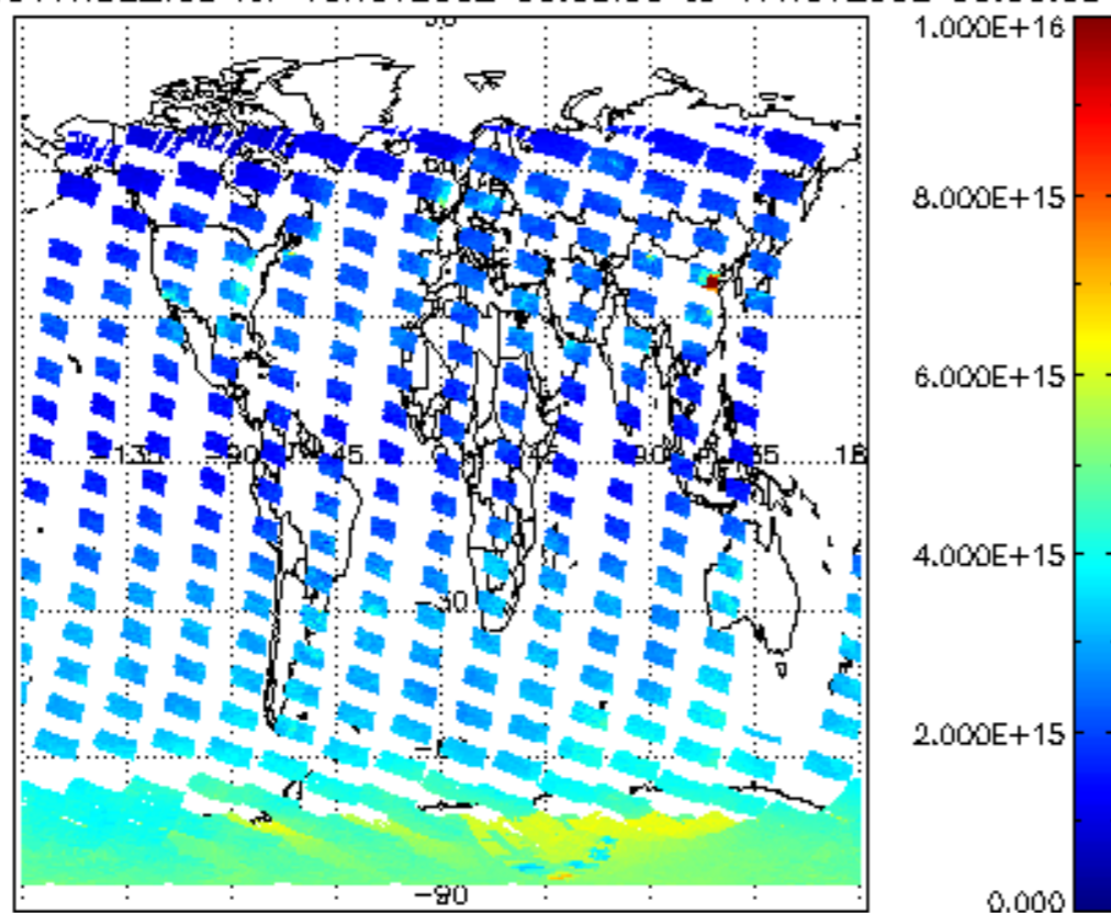
SCIOL2P_NADUV1NO2_vcd for 16NOV2002 00:00:00 to 17NOV2002 00:00:00
