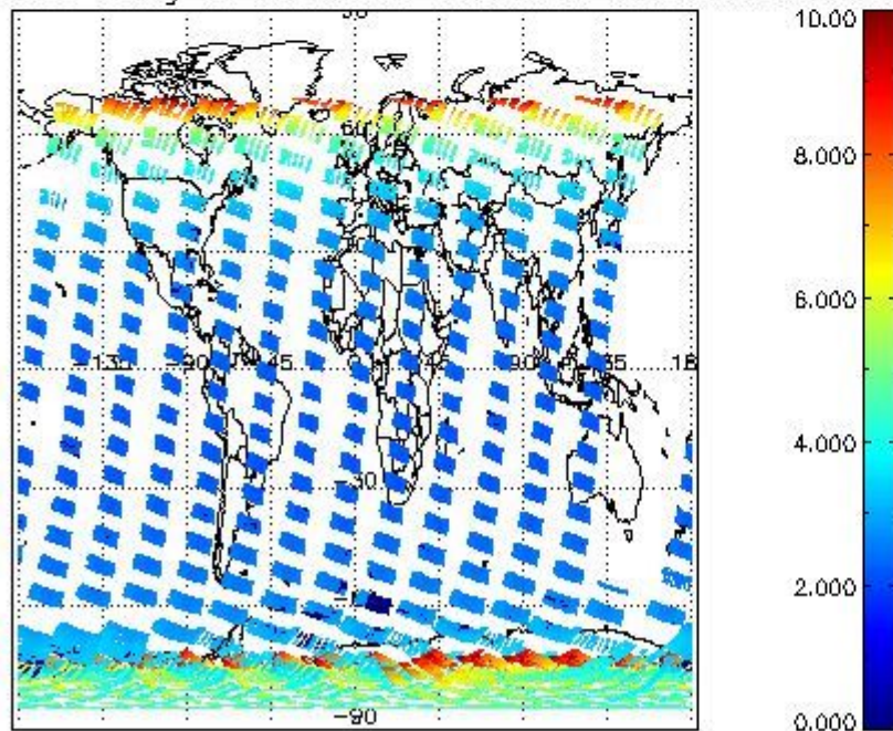
SCIOL2P_NADUV003_amf_gr for 16NOV2002 00:00:00 to 17NOV2002 00:00:00
