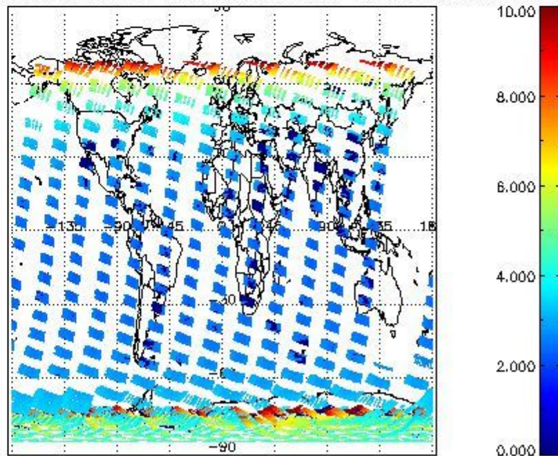
SCIOL2P_NADUV003_amf_cl for 16NOV2002 00:00:00 to 17NOV2002 00:00:00
