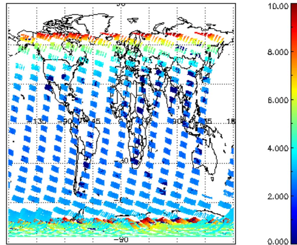
SCIOL2P_NADUV003_amf_cl for 16NOV2002 00:00:00 to 17NOV2002 00:00:00
