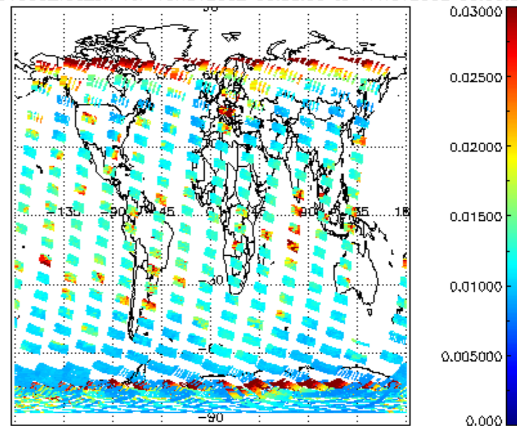
SCIOL2P_NADUV003_vcd_err for 16NOV2002 00:00:00 to 17NOV2002 00:00:00
