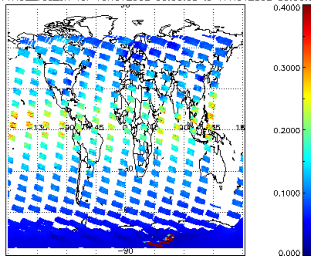
SCIOL2P_NADUV1NO2_vcd_err for 16NOV2002 00:00:00 to 17NOV2002 00:00:00
