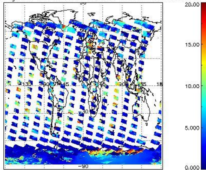
cL_top_height for 16NOV2002 00:00:00 to 17NOV2002 00:00:00
