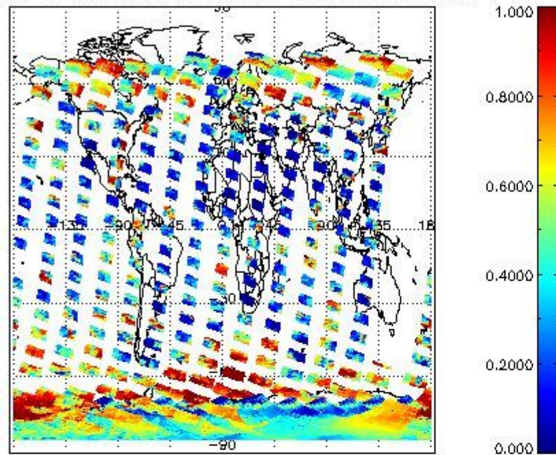
cLfrac for 16NOV2002 00:00:00 to 17NOV2002 00:00:00
