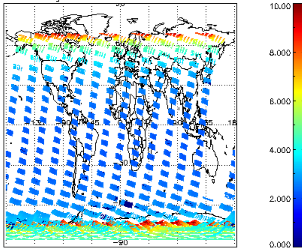
SCIOL2P_NADUV003_amf_gr for 16NOV2002 00:00:00 to 17NOV2002 00:00:00
