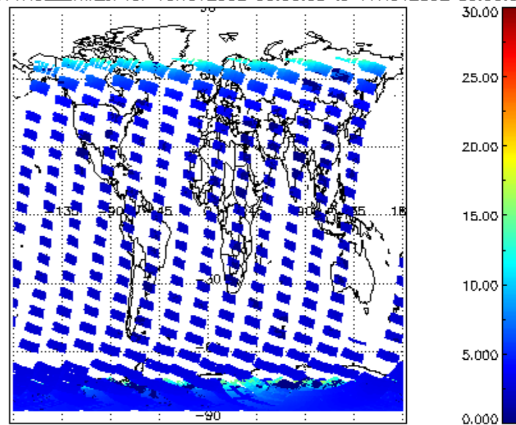
SCIOL2P_NADUV1NO2_amf_cl for 16NOV2002 00:00:00 to 17NOV2002 00:00:00
