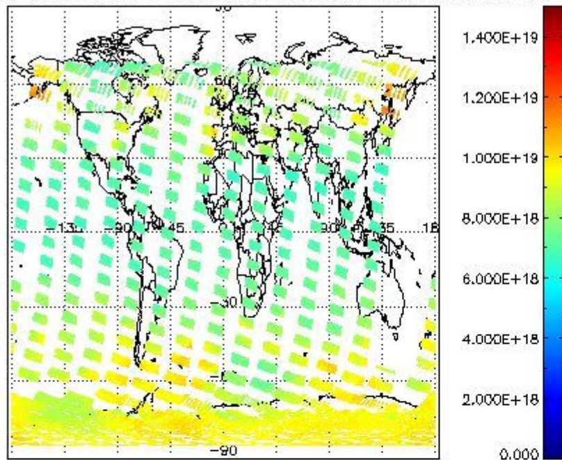
SCIOL2P_NADUV003_vcd for 16NOV2002 00:00:00 to 17NOV2002 00:00:00
