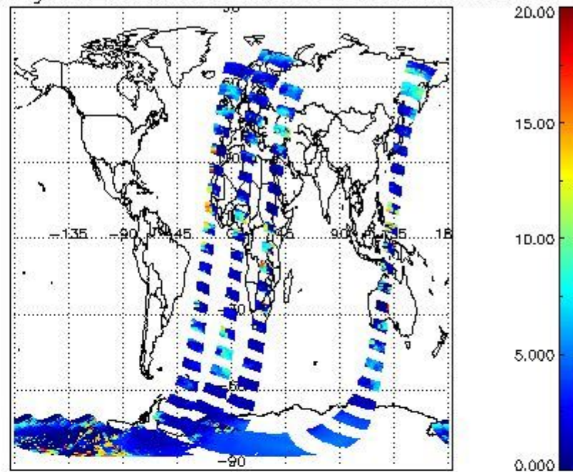
cL_top_height for 10NOV2002 00:00:00 to 11NOV2002 00:00:00
