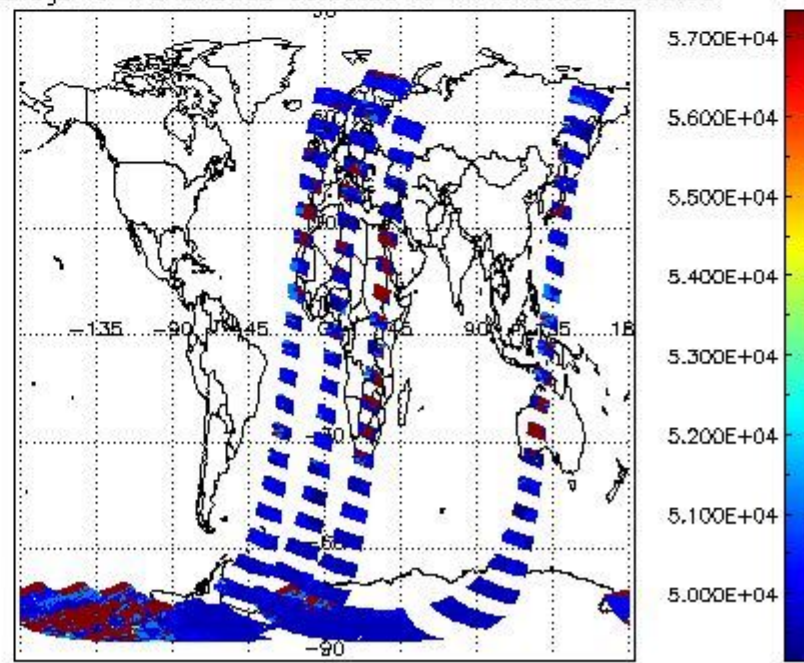
cloud_flags for 10NOV2002 00:00:00 to 11NOV2002 00:00:00
