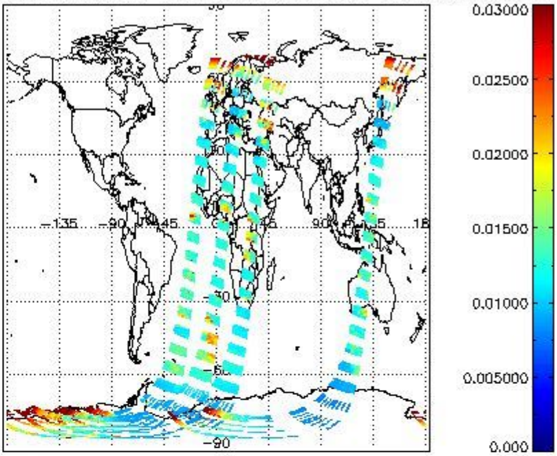
SCIOL2P_NADUV003_vcd_err for 10NOV2002 00:00:00 to 11NOV2002 00:00:00
