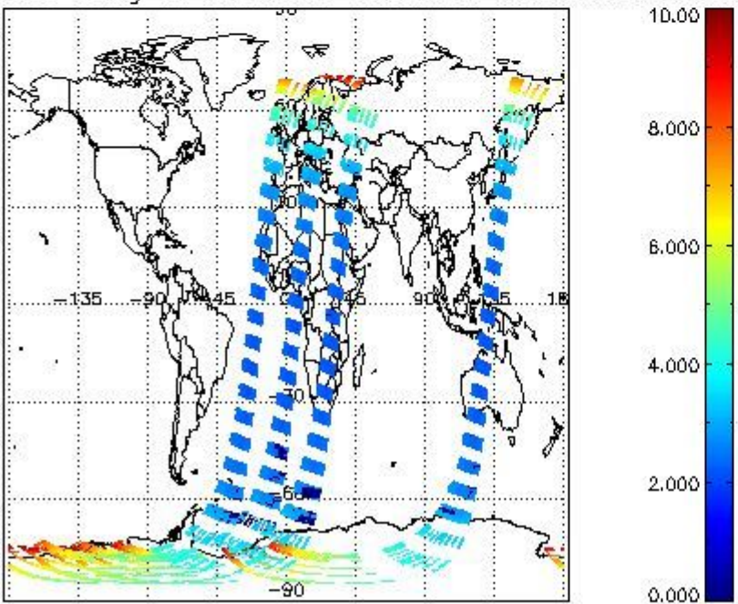
SCIOL2P_NADUV003_amf_gr for 10NOV2002 00:00:00 to 11NOV2002 00:00:00
