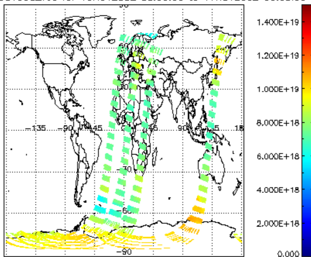
SCIOL2P_NADUV003_vcd for 10NOV2002 00:00:00 to 11NOV2002 00:00:00
