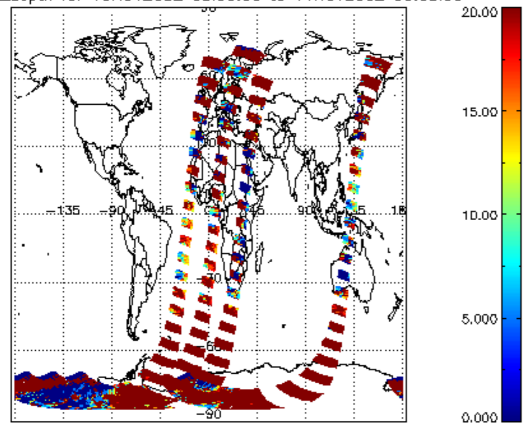
cl_opt_depth for 10NOV2002 00:00:00 to 11NOV2002 00:00:00
