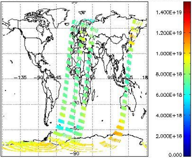
SCIOL2P_NADUV003_vcd for 10NOV2002 00:00:00 to 11NOV2002 00:00:00
