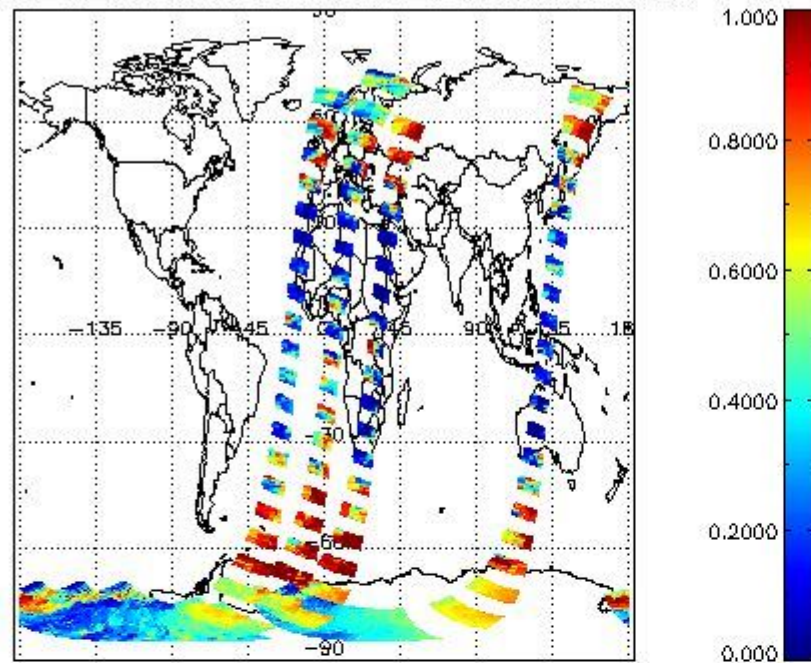
cLfrac for 10NOV2002 00:00:00 to 11NOV2002 00:00:00
