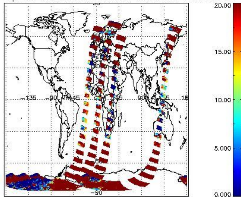
cL_opt_depth for 10NOV2002 00:00:00 to 11NOV2002 00:00:00
