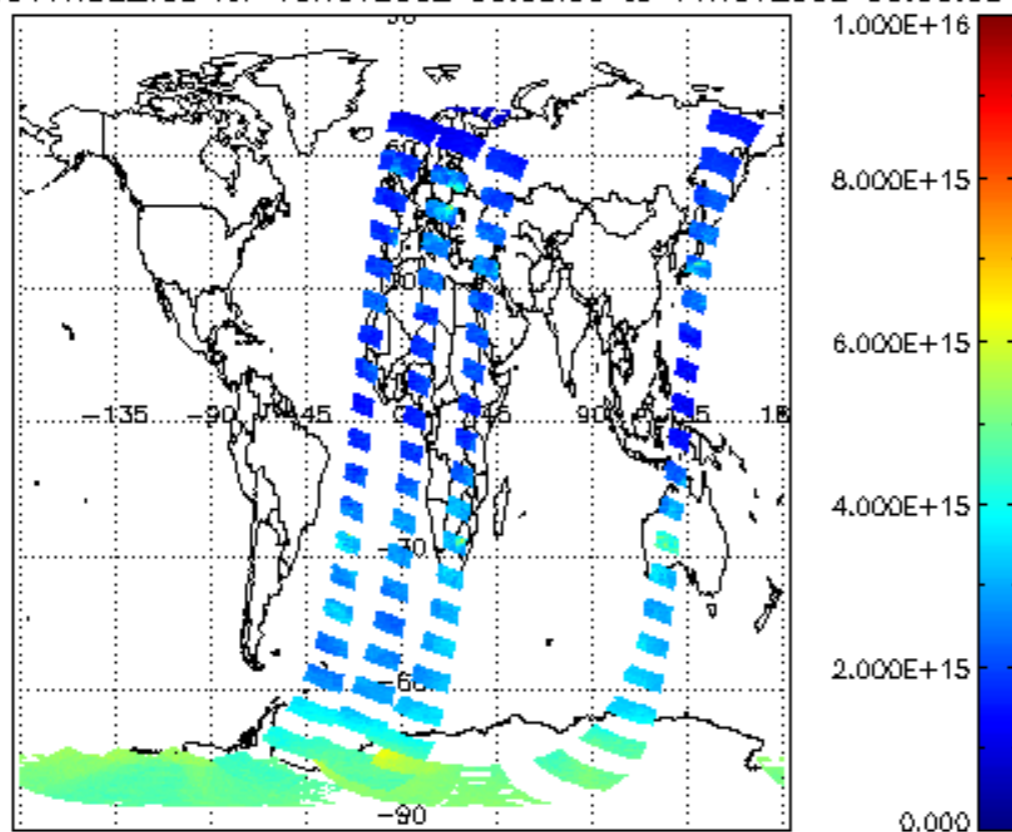
SCIOL2P_NADUV1NO2_vcd for 10NOV2002 00:00:00 to 11NOV2002 00:00:00
