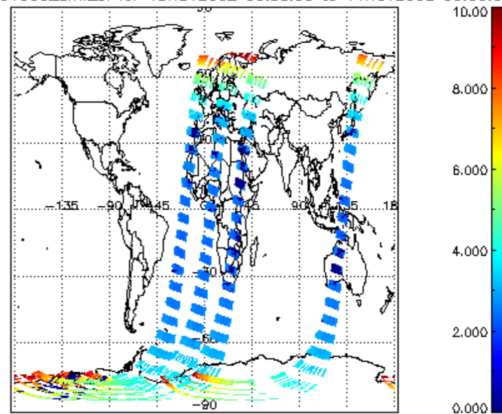
SCIOL2P_NADUV003_amf_cl for 10NOV2002 00:00:00 to 11NOV2002 00:00:00
