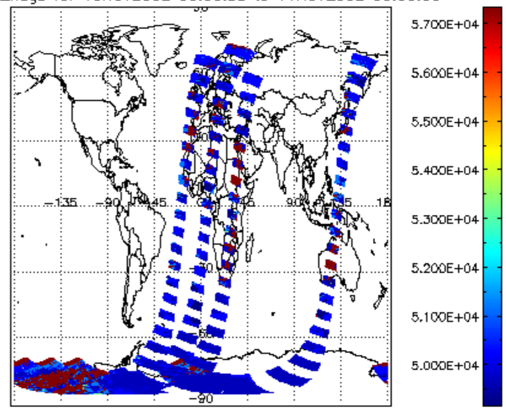
cloud_flags for 10NOV2002 00:00:00 to 11NOV2002 00:00:00
