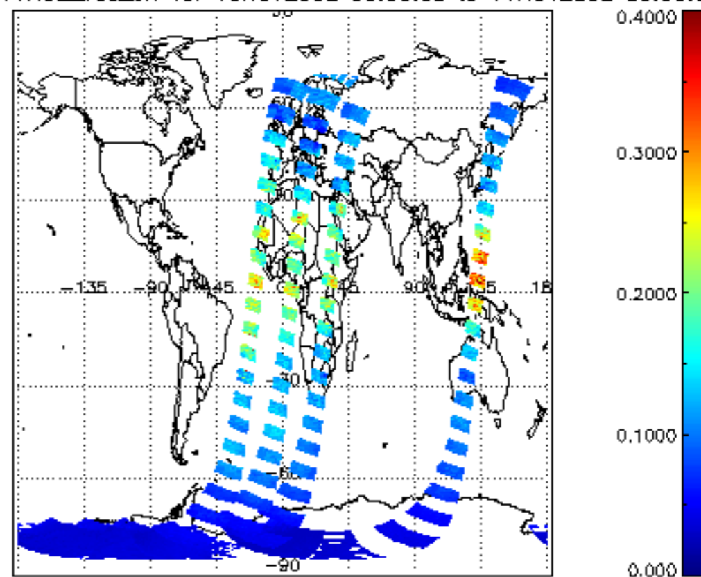
SCIOL2P_NADUV1NO2_vcd_err for 10NOV2002 00:00:00 to 11NOV2002 00:00:00
