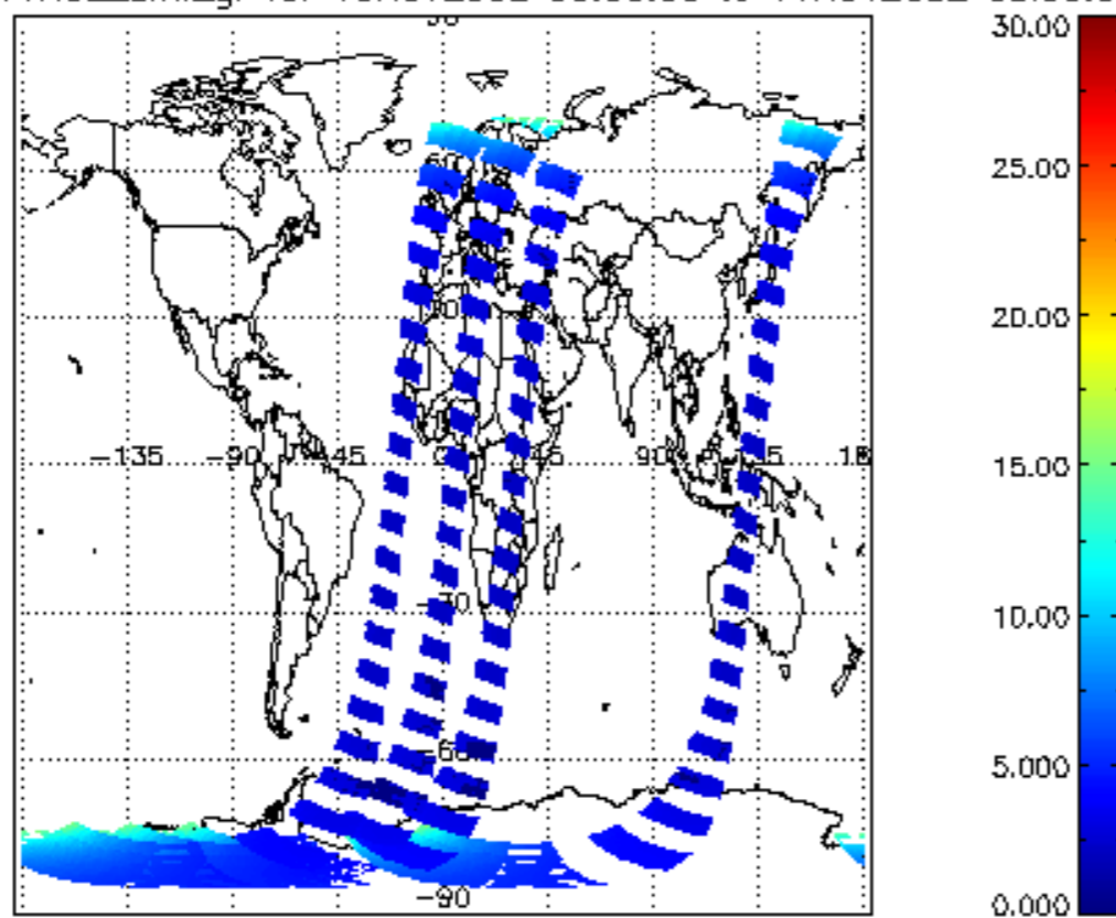
SCIOL2P_NADUV1NO2_amf_gr for 10NOV2002 00:00:00 to 11NOV2002 00:00:00
