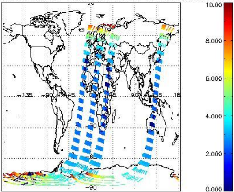
SCIOL2P_NADUV003_amf_cl for 10NOV2002 00:00:00 to 11NOV2002 00:00:00
