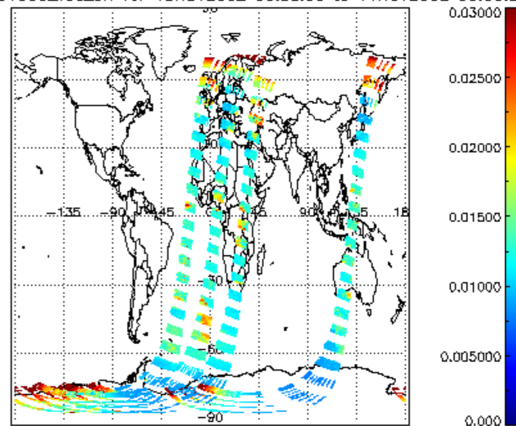
SCIOL2P_NADUV003_vcd_err for 10NOV2002 00:00:00 to 11NOV2002 00:00:00
