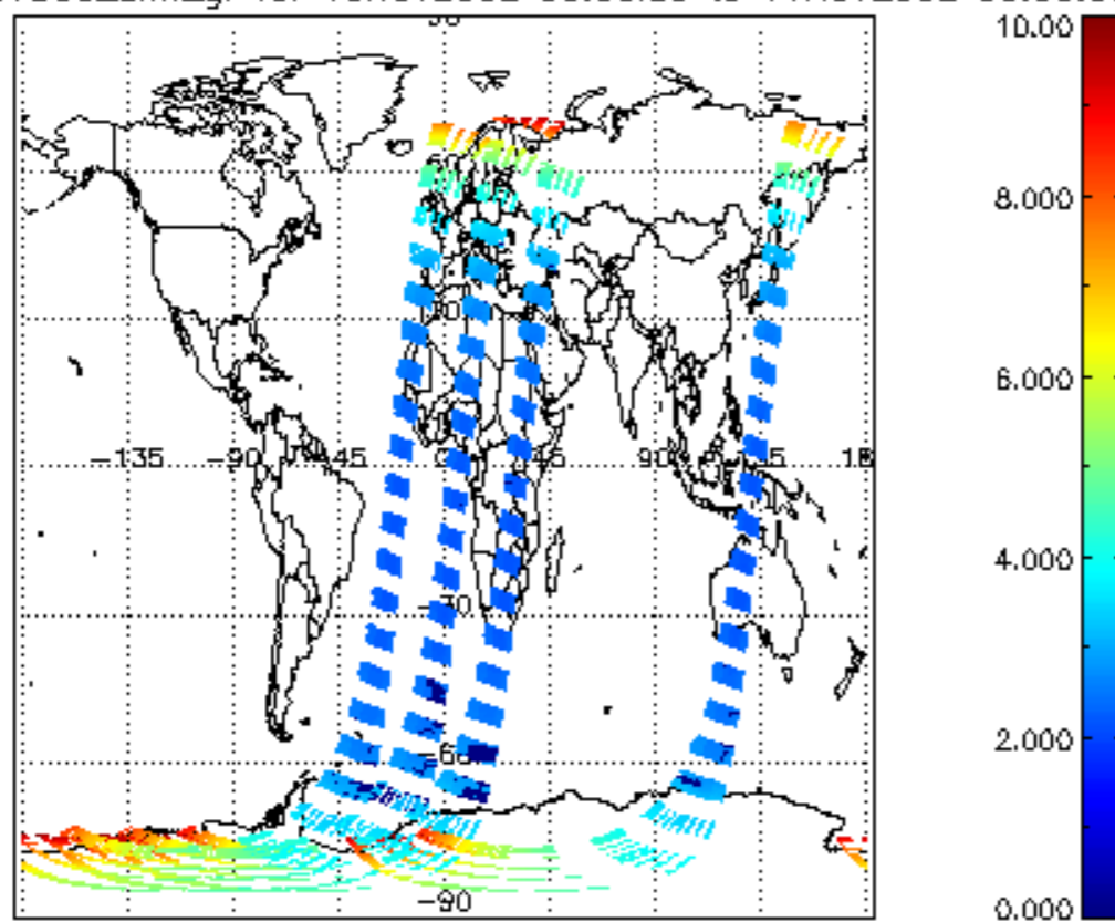
SCIOL2P_NADUV003_amf_gr for 10NOV2002 00:00:00 to 11NOV2002 00:00:00
