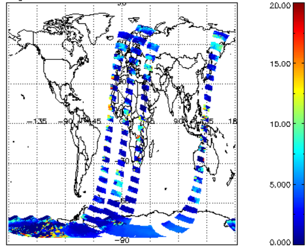
cl_top_height for 10NOV2002 00:00:00 to 11NOV2002 00:00:00
