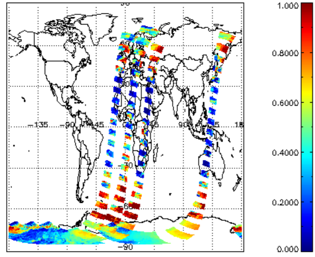
cLfrac for 10NOV2002 00:00:00 to 11NOV2002 00:00:00
