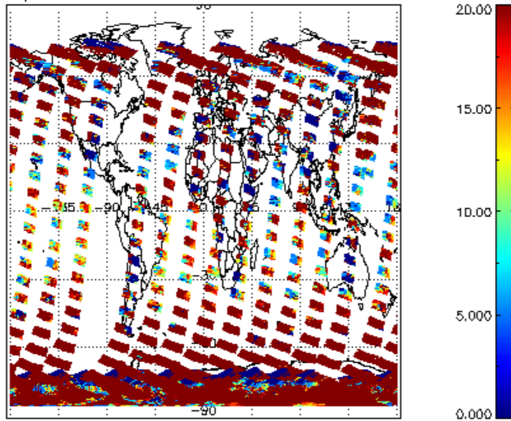
cL_opt_depth for 08NOV2002 00:00:00 to 09NOV2002 00:00:00
