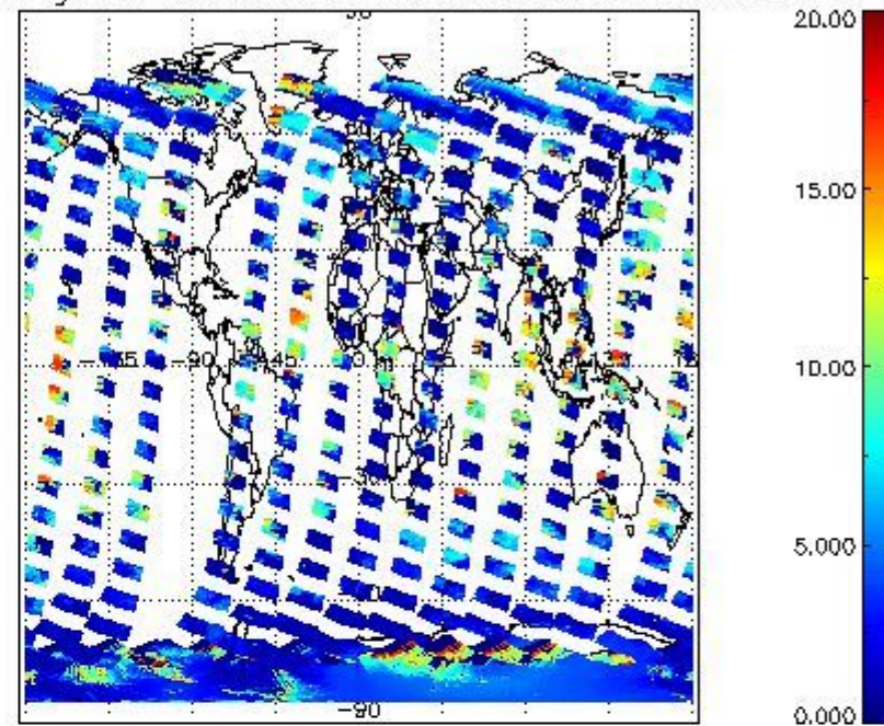
cL_top_height for 08NOV2002 00:00:00 to 09NOV2002 00:00:00
