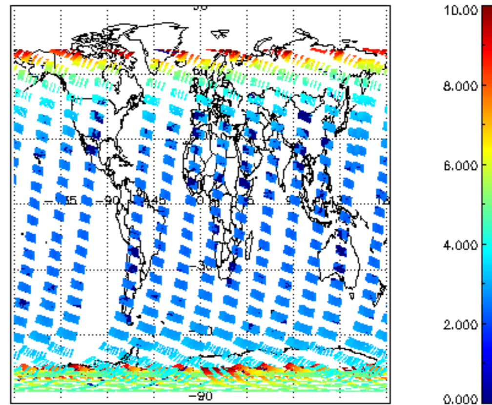
SCIOL2P_NADUV003_amf_cl for 08NOV2002 00:00:00 to 09NOV2002 00:00:00
