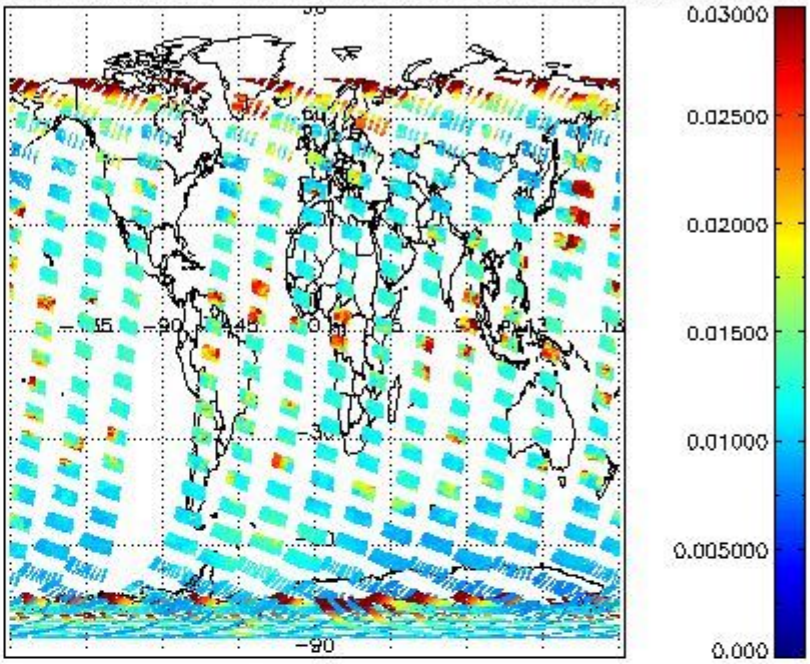
SCIOL2P_NADUV003_vcd_err for 08NOV2002 00:00:00 to 09NOV2002 00:00:00
