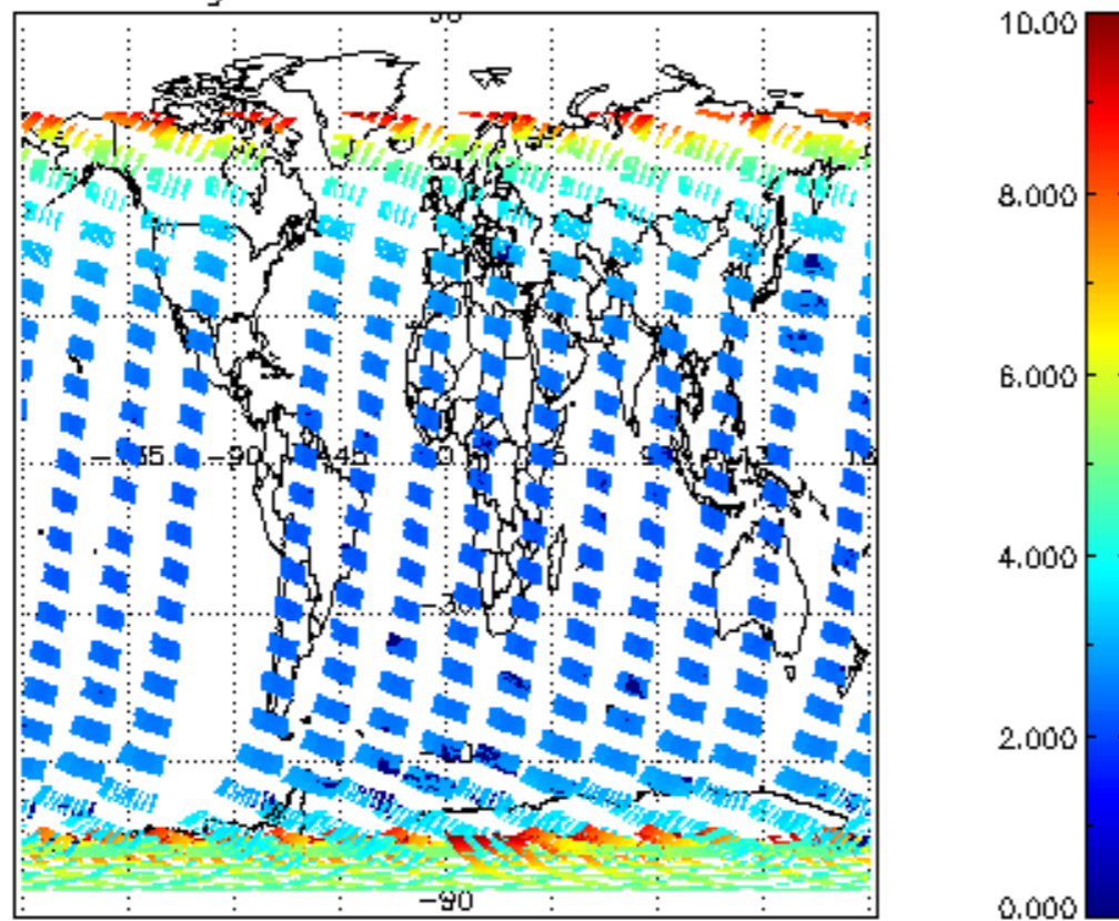
SCIOL2P_NADUV003_amf_gr for 08NOV2002 00:00:00 to 09NOV2002 00:00:00
