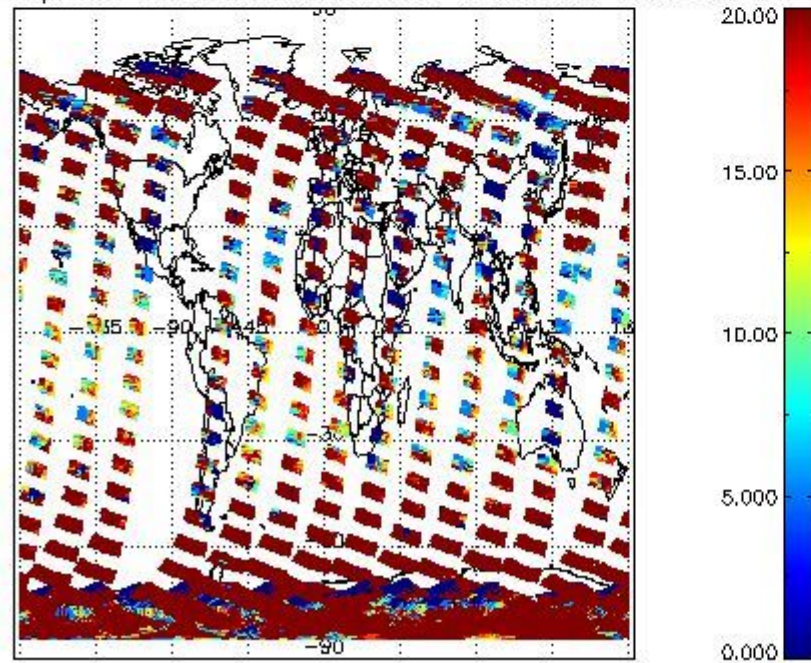
cL_opt_depth for 08NOV2002 00:00:00 to 09NOV2002 00:00:00
