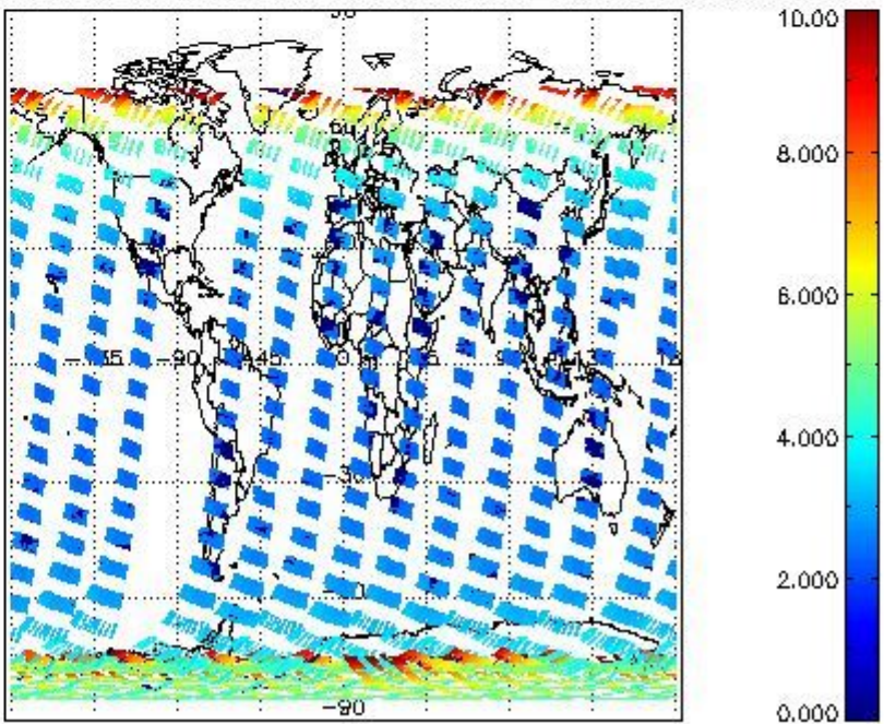
SCIOL2P_NADUV003_amf_err for 08NOV2002 00:00:00 to 09NOV2002 00:00:00
