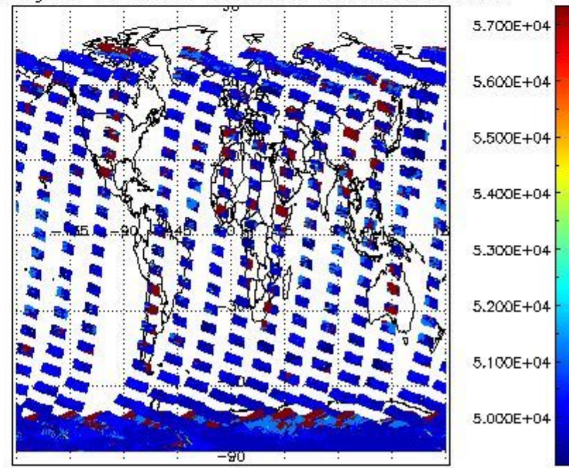
cloud_flags for 08NOV2002 00:00:00 to 09NOV2002 00:00:00
