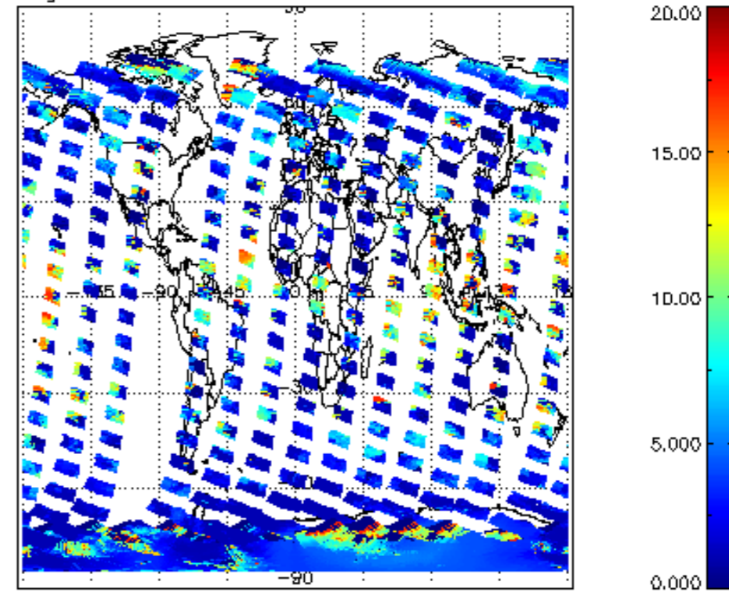
cL_top_height for 08NOV2002 00:00:00 to 09NOV2002 00:00:00
