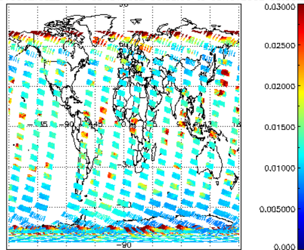
SCIOL2P_NADUV003_vcd_err for 08NOV2002 00:00:00 to 09NOV2002 00:00:00
