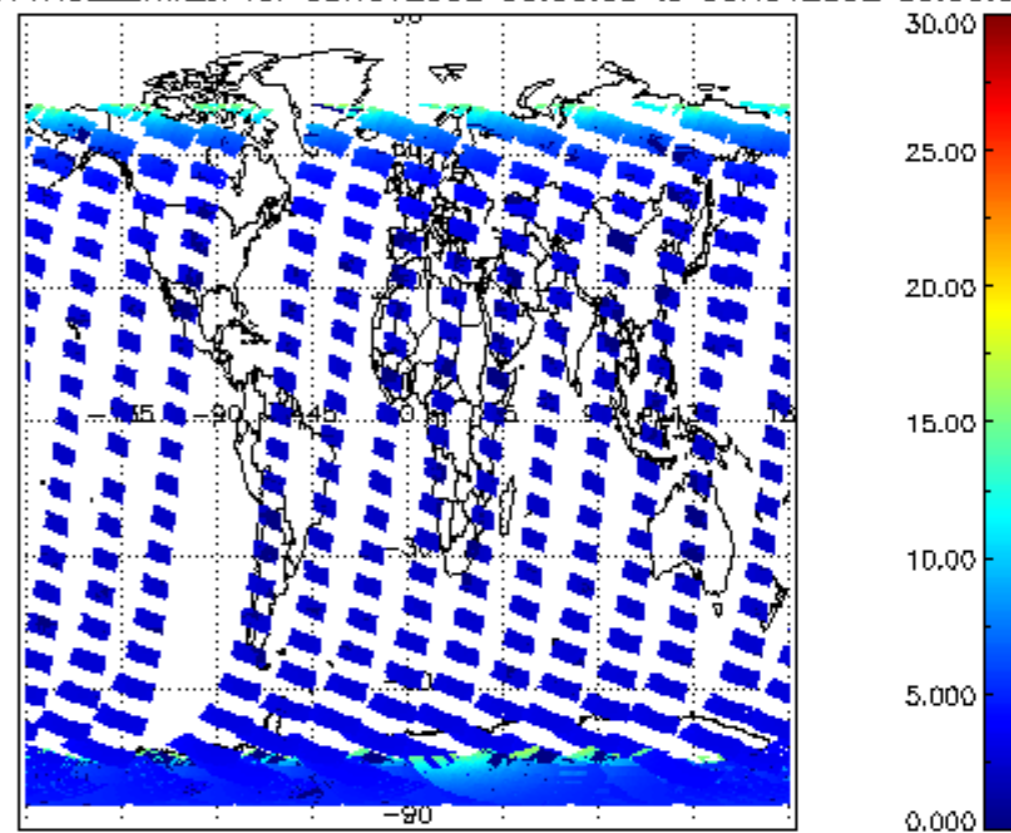
SCIOL2P_NADUV1NO2_amf_cl for 08NOV2002 00:00:00 to 09NOV2002 00:00:00
