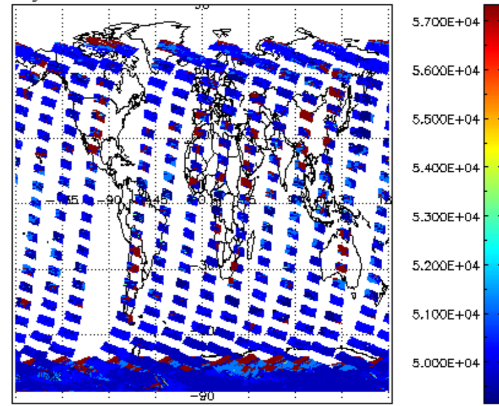
cloud_flags for 08NOV2002 00:00:00 to 09NOV2002 00:00:00
