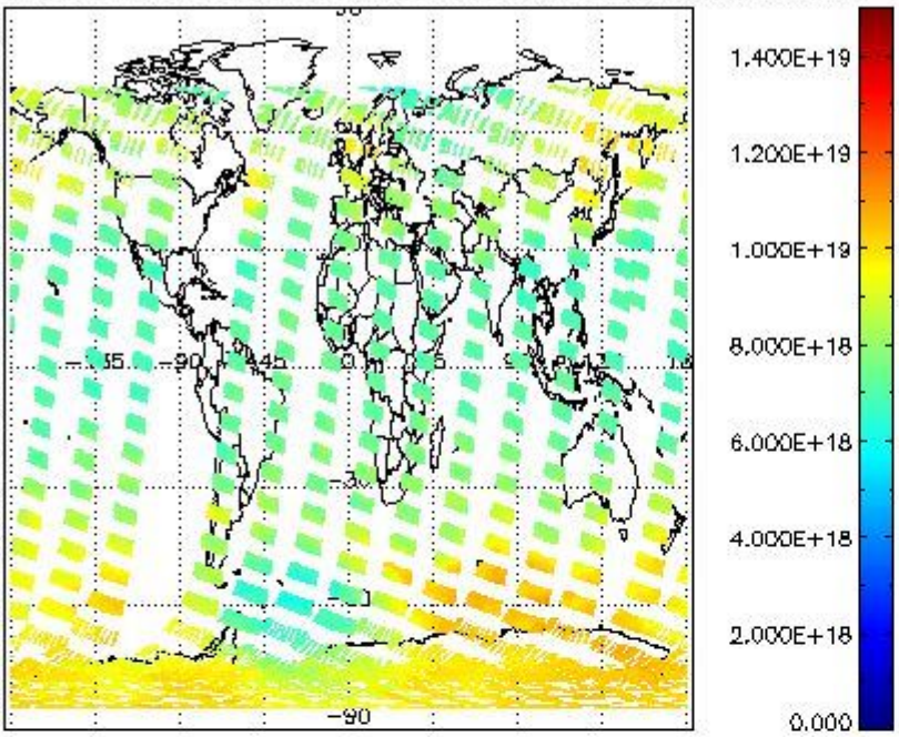
SCIOL2P_NADUV003_vcd for 08NOV2002 00:00:00 to 09NOV2002 00:00:00
