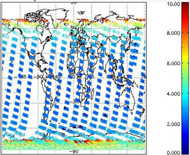
SCIOL2P_NADUV003_amf_gr for 08NOV2002 00:00:00 to 09NOV2002 00:00:00
