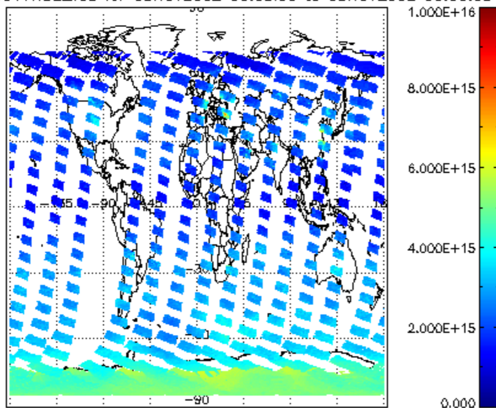
SCIOL2P_NADUV1NO2_vcd for 08NOV2002 00:00:00 to 09NOV2002 00:00:00
