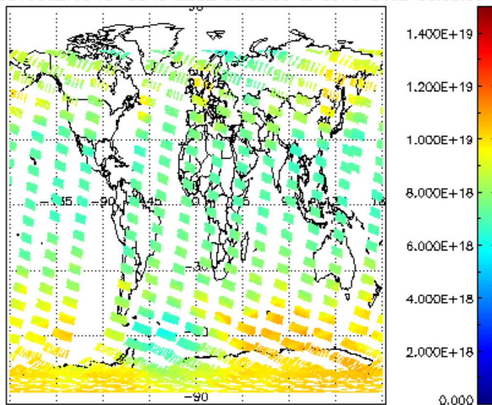
SCIOL2P_NADUV003_vcd for 08NOV2002 00:00:00 to 09NOV2002 00:00:00
