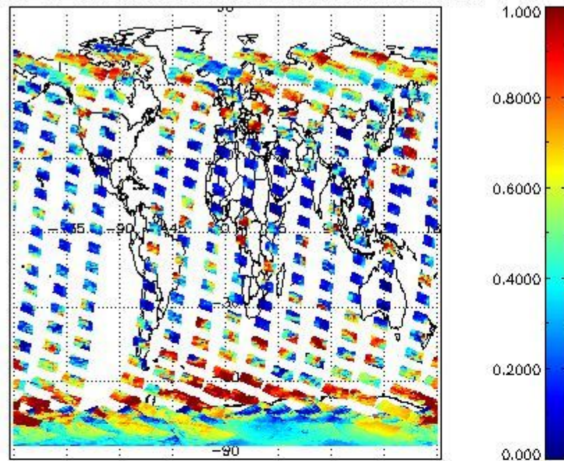
cLfrac for 08NOV2002 00:00:00 to 09NOV2002 00:00:00
