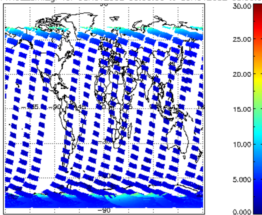
SCIOL2P_NADUV1NO2_amf_gr for 08NOV2002 00:00:00 to 09NOV2002 00:00:00
