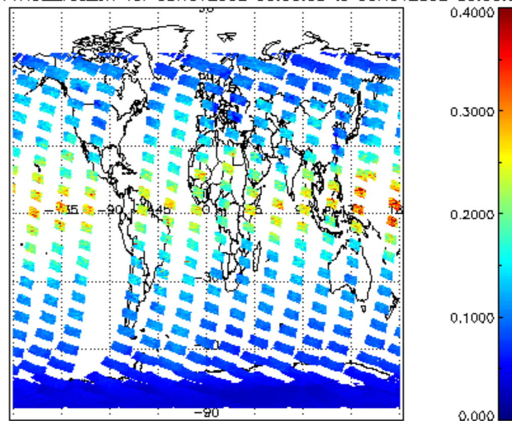
SCIOL2P_NADUV1NO2_vcd_err for 08NOV2002 00:00:00 to 09NOV2002 00:00:00
