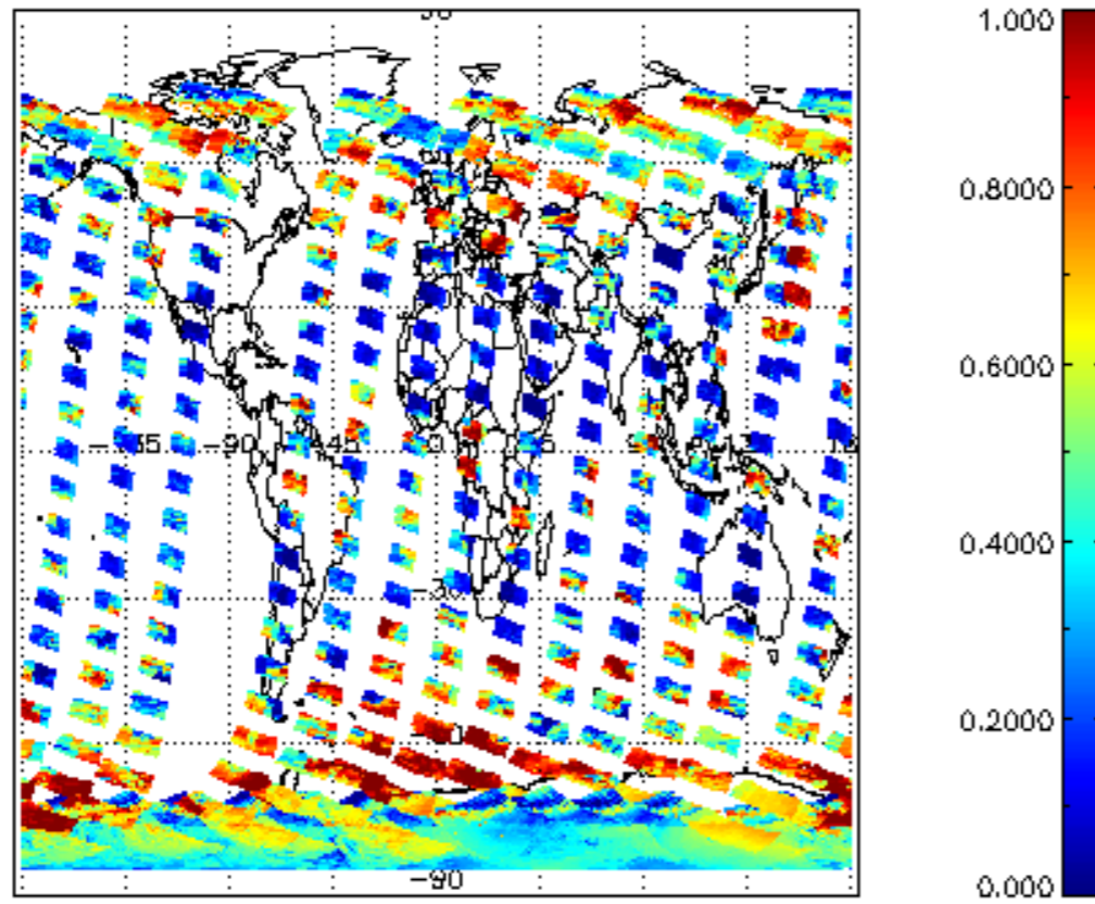
cLfrac for 08NOV2002 00:00:00 to 09NOV2002 00:00:00
