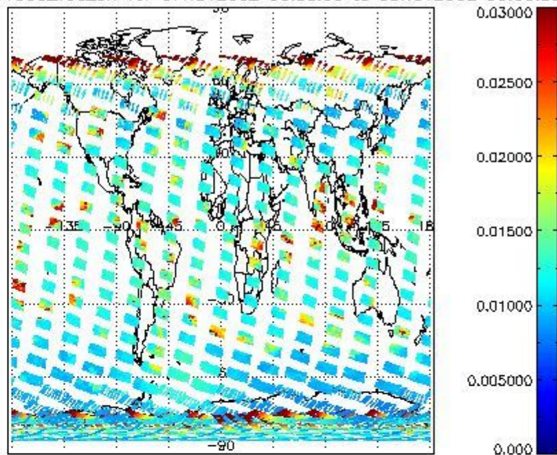
SCIOL2P_NADUV003_vcd_err for 07NOV2002 00:00:00 to 08NOV2002 00:00:00
