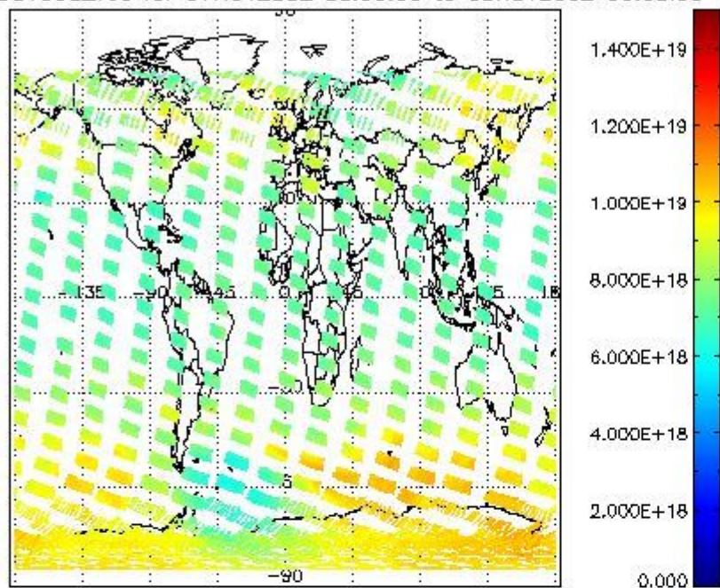
SCIOL2P_NADUV003_vcd for 07NOV2002 00:00:00 to 08NOV2002 00:00:00
