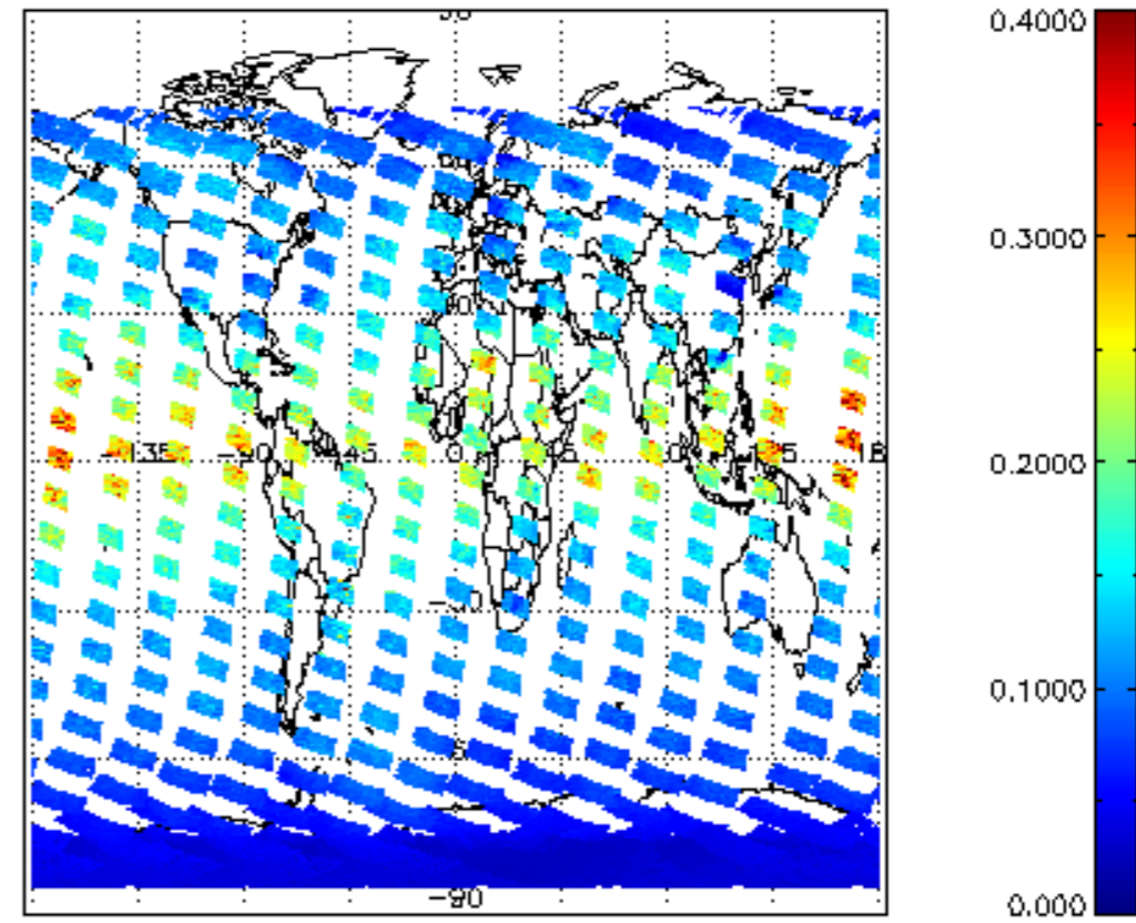
SCIOL2P_NADUV1NO2_vcd_err for 07NOV2002 00:00:00 to 08NOV2002 00:00:00
