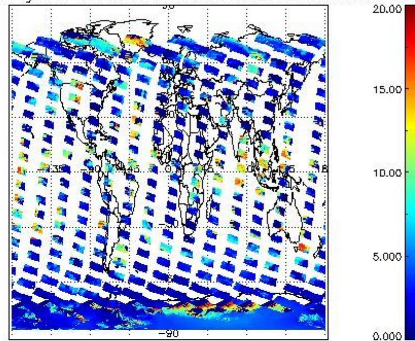
cL_top_height for 07NOV2002 00:00:00 to 08NOV2002 00:00:00
