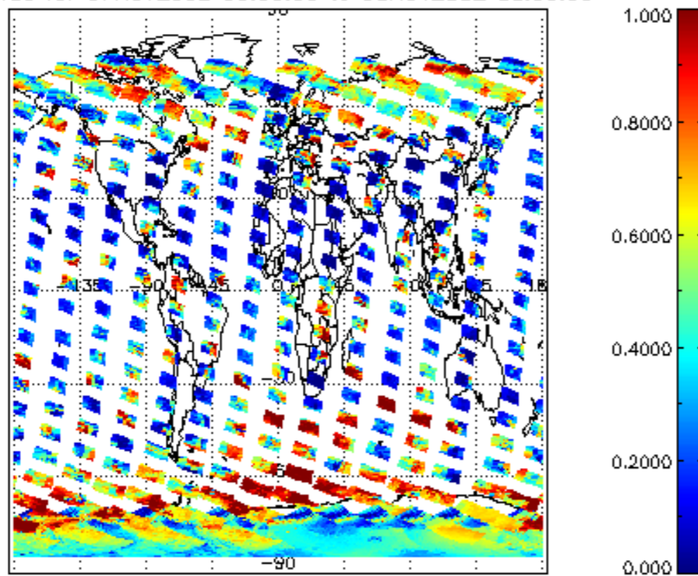
cLfrac for 07NOV2002 00:00:00 to 08NOV2002 00:00:00
