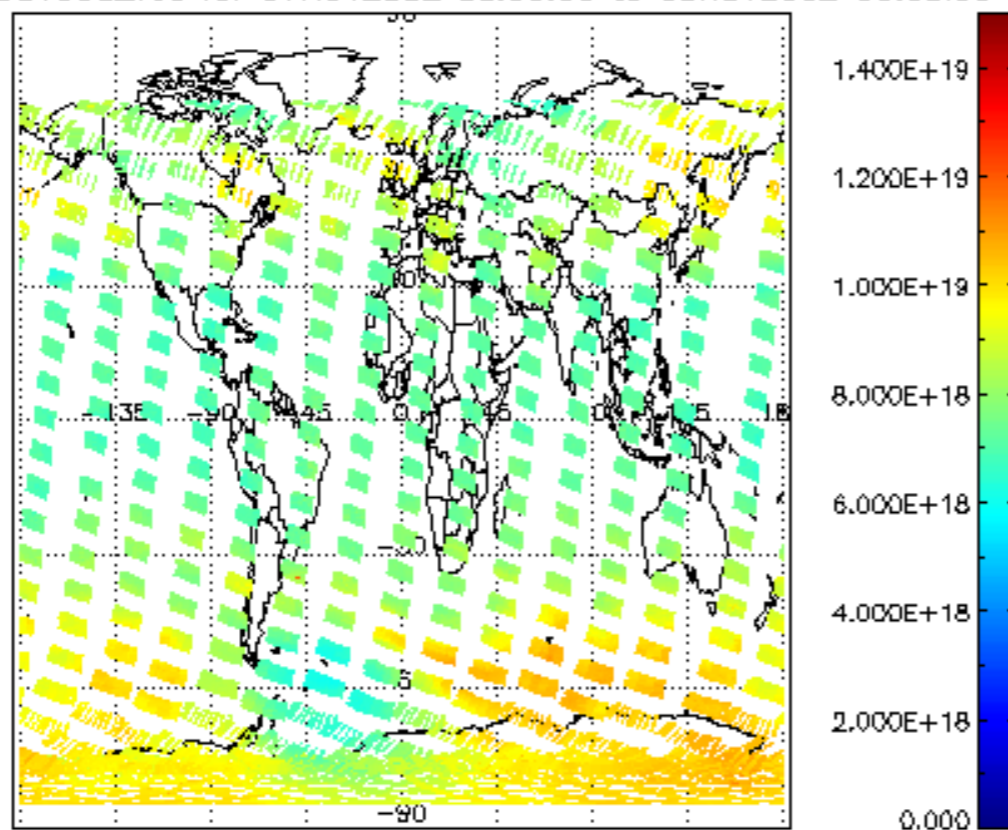
SCIOL2P_NADUV003_vcd for 07NOV2002 00:00:00 to 08NOV2002 00:00:00
