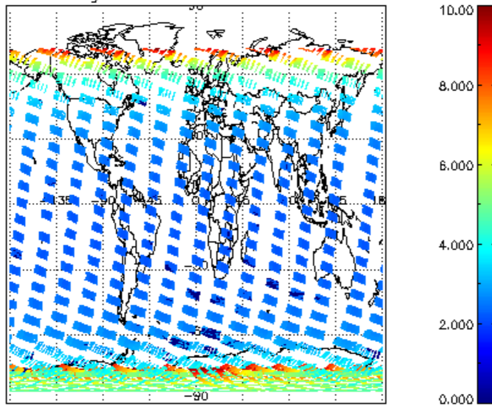
SCIOL2P_NADUV003_amf_gr for 07NOV2002 00:00:00 to 08NOV2002 00:00:00
