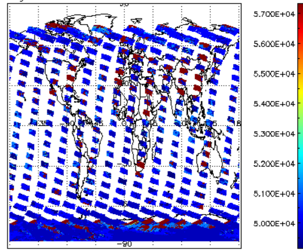
cloud_flags for 07NOV2002 00:00:00 to 08NOV2002 00:00:00
