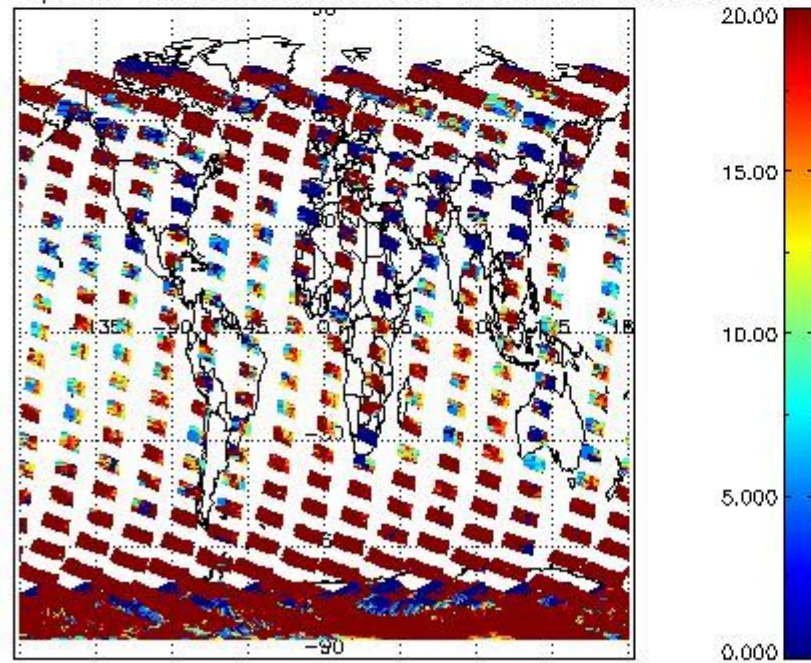
cL_opt_depth for 07NOV2002 00:00:00 to 08NOV2002 00:00:00
