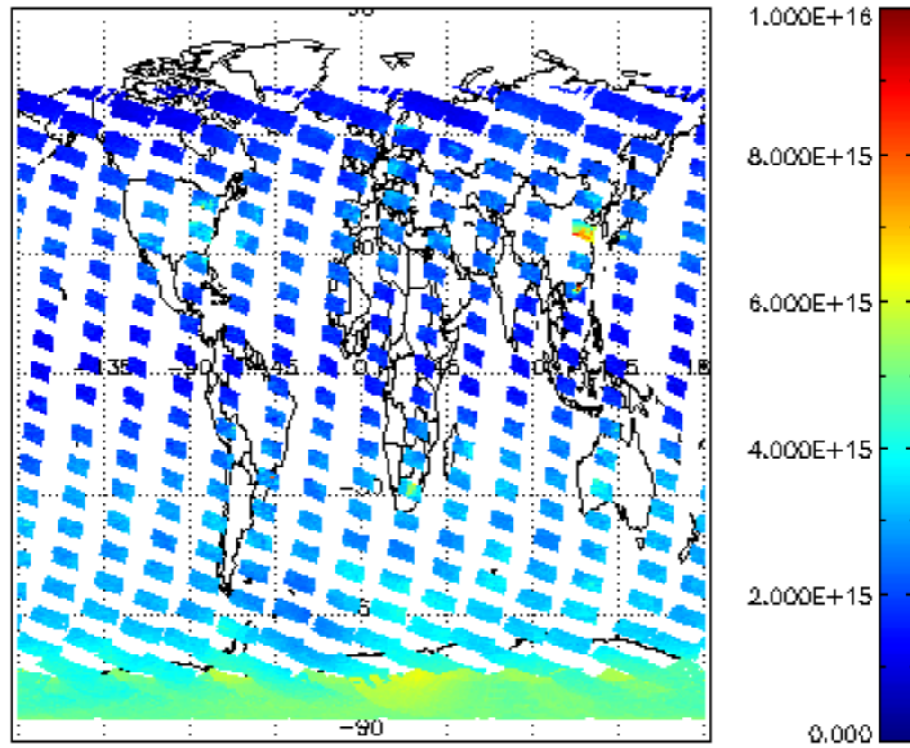
SCIOL2P_NADUV1NO2_vcd for 07NOV2002 00:00:00 to 08NOV2002 00:00:00
