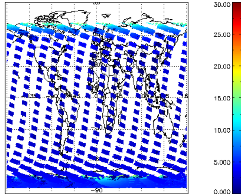
SCIOL2P_NADUV1NO2_amf_cl for 07NOV2002 00:00:00 to 08NOV2002 00:00:00
