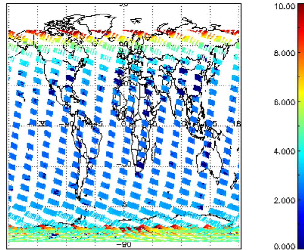
SCIOL2P_NADUV003_amf_cl for 07NOV2002 00:00:00 to 08NOV2002 00:00:00
