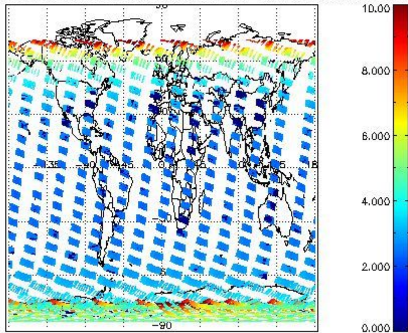
SCIOL2P_NADUV003_amf_cl for 07NOV2002 00:00:00 to 08NOV2002 00:00:00
