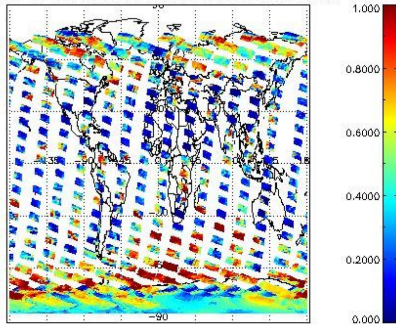
cLfrac for 07NOV2002 00:00:00 to 08NOV2002 00:00:00
