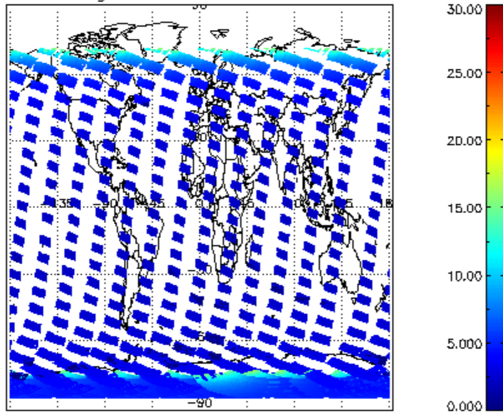
SCIOL2P_NADUV1NO2_amf_gr for 07NOV2002 00:00:00 to 08NOV2002 00:00:00
