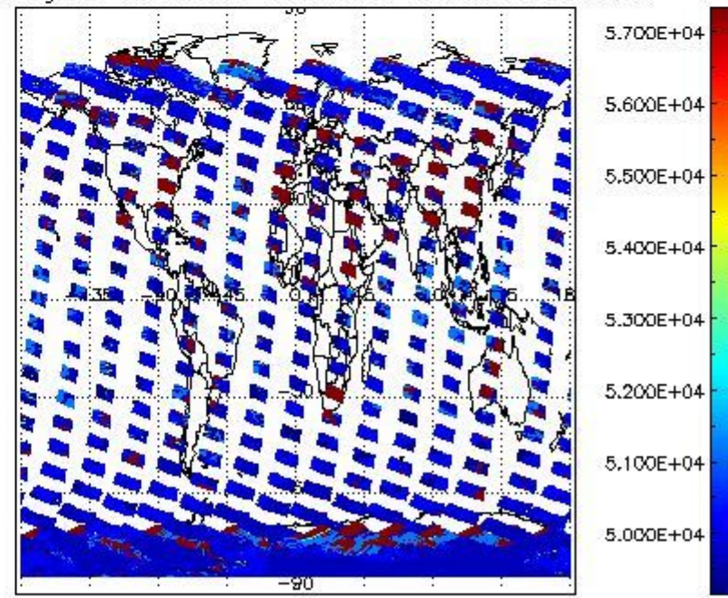
cloud_flags for 07NOV2002 00:00:00 to 08NOV2002 00:00:00
