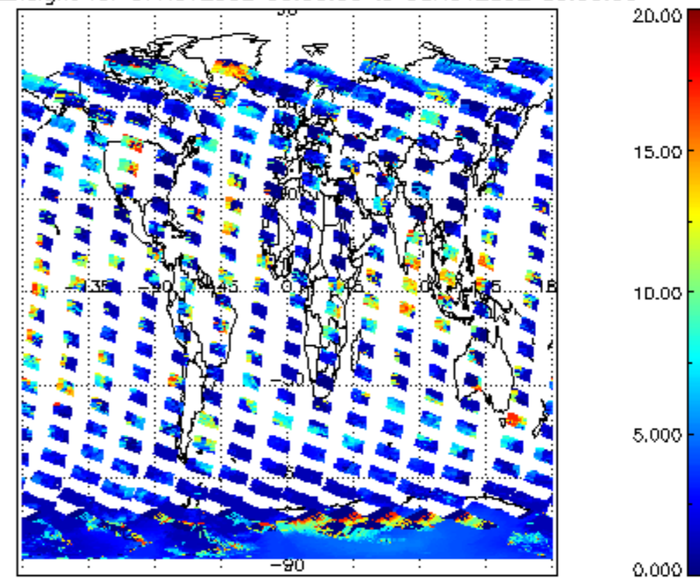
cL_top_height for 07NOV2002 00:00:00 to 08NOV2002 00:00:00
