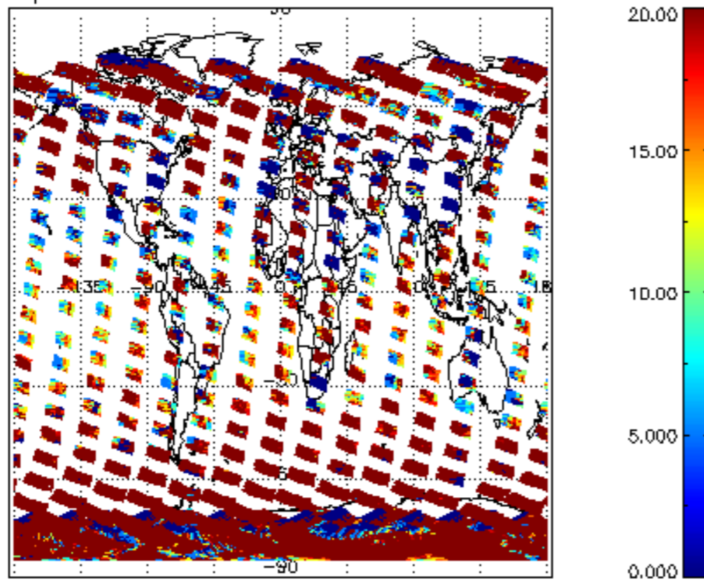
cL_opt_depth for 07NOV2002 00:00:00 to 08NOV2002 00:00:00
