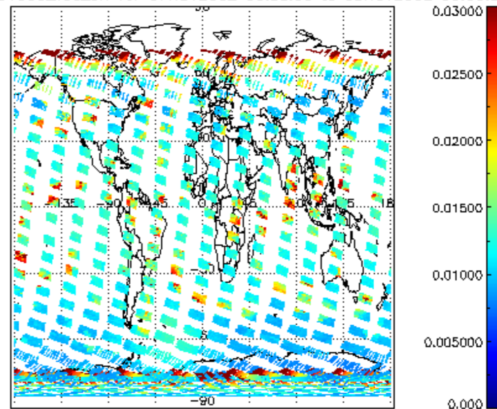
SCIOL2P_NADUV003_vcd_err for 07NOV2002 00:00:00 to 08NOV2002 00:00:00
