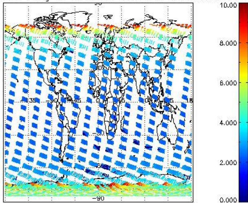
SCIOL2P_NADUV003_amf_gr for 07NOV2002 00:00:00 to 08NOV2002 00:00:00
