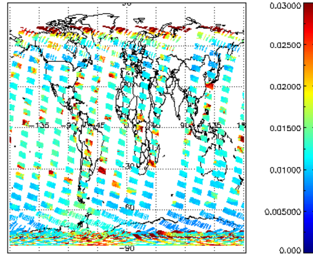
SCIOL2P_NADUV003_vcd_err for 30OCT2002 00:00:00 to 31OCT2002 00:00:00
