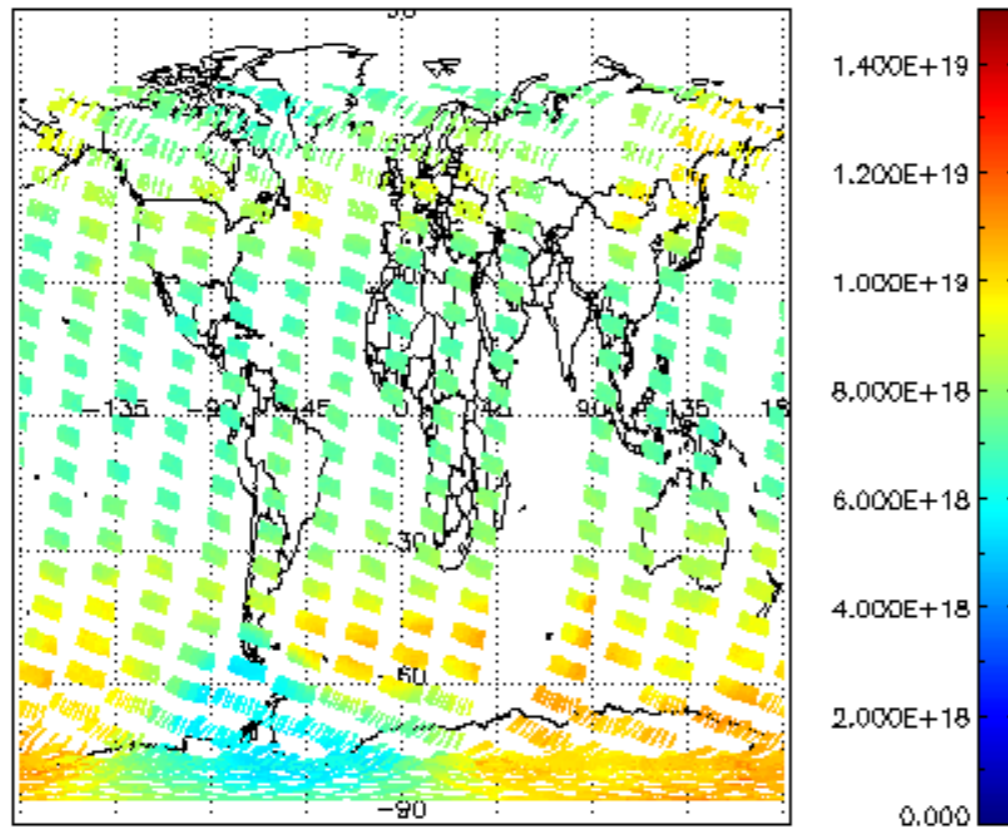
SCIOL2P_NADUV003_vcd for 30OCT2002 00:00:00 to 31OCT2002 00:00:00
