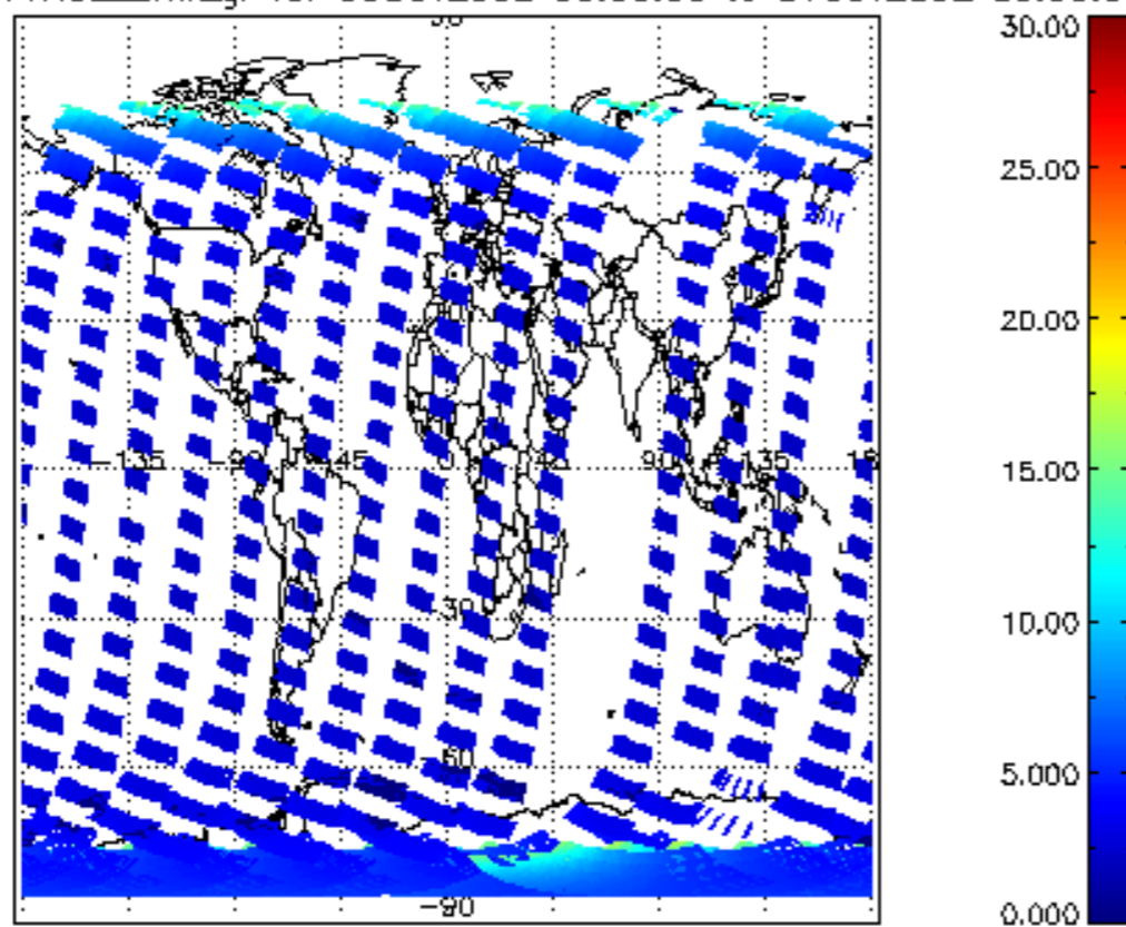
ICIOL2P_NADUV1NO2_amf_gr for 30OCT2002 00:00:00 to 31OCT2002 00:00:00
