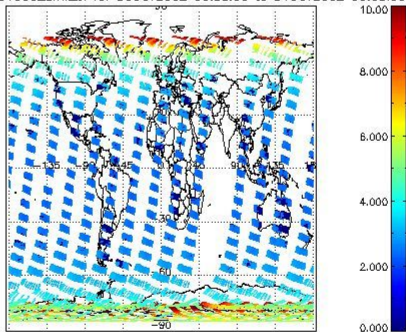
SCIOL2P_NADUV003_amf_sl for 30OCT2002 00:00:00 to 31OCT2002 00:00:00
