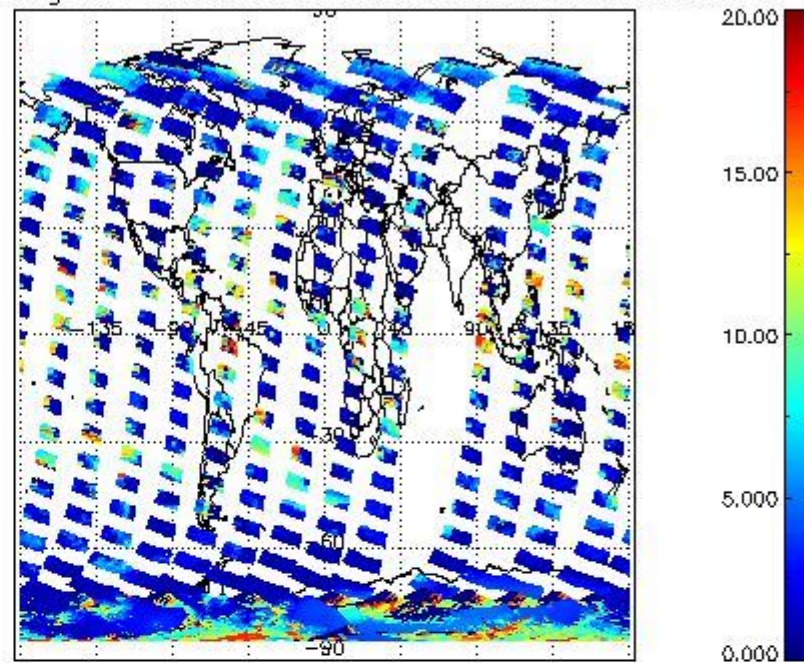
cL_top_height for 30OCT2002 00:00:00 to 31OCT2002 00:00:00
