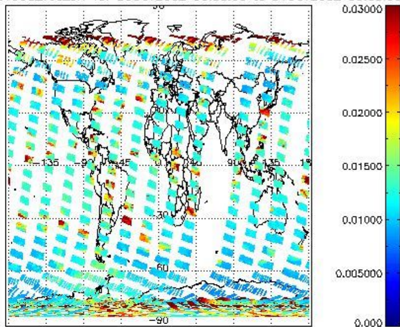
SCIOL2P_NADUV003_vcd_err for 30OCT2002 00:00:00 to 31OCT2002 00:00:00
