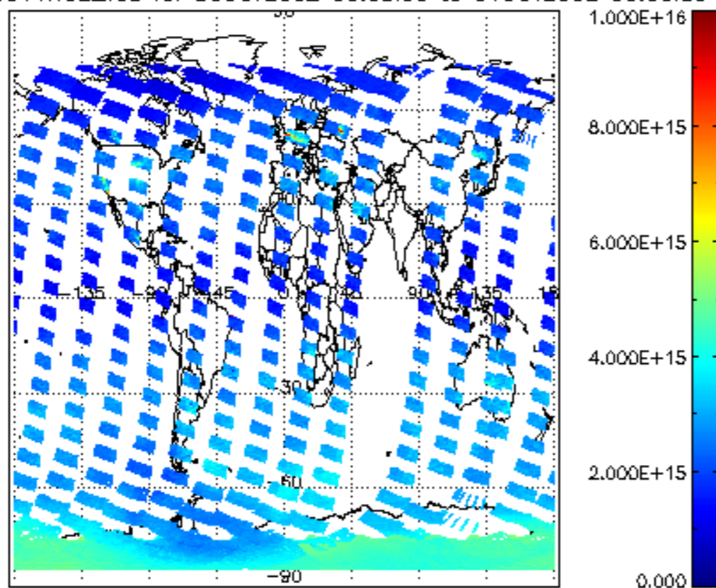
SCIOL2P_NADUV1NO2_vcd for 30OCT2002 00:00:00 to 31OCT2002 00:00:00
