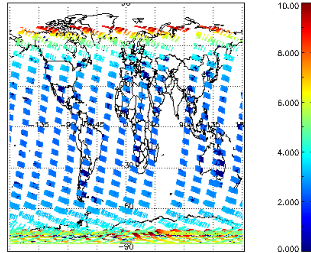
SCIOL2P_NADUV003_amf_el for 30OCT2002 00:00:00 to 31OCT2002 00:00:00
