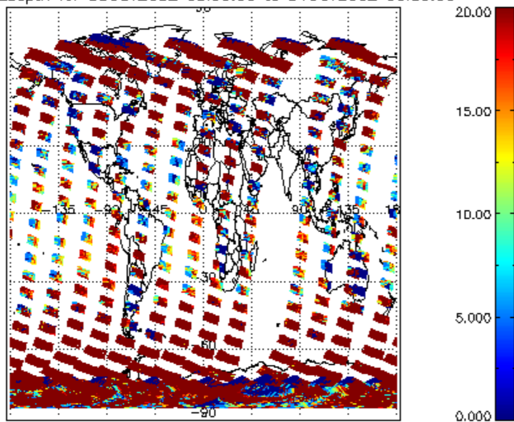
cl_opt_depth for 30OCT2002 00:00:00 to 31OCT2002 00:00:00
