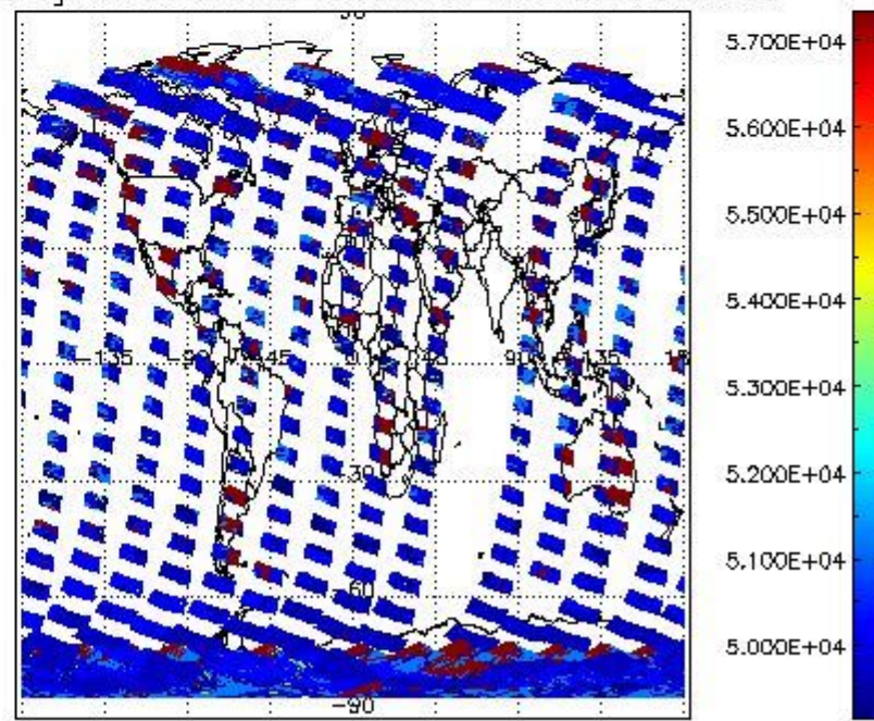
cloud_flags for 30OCT2002 00:00:00 to 31OCT2002 00:00:00
