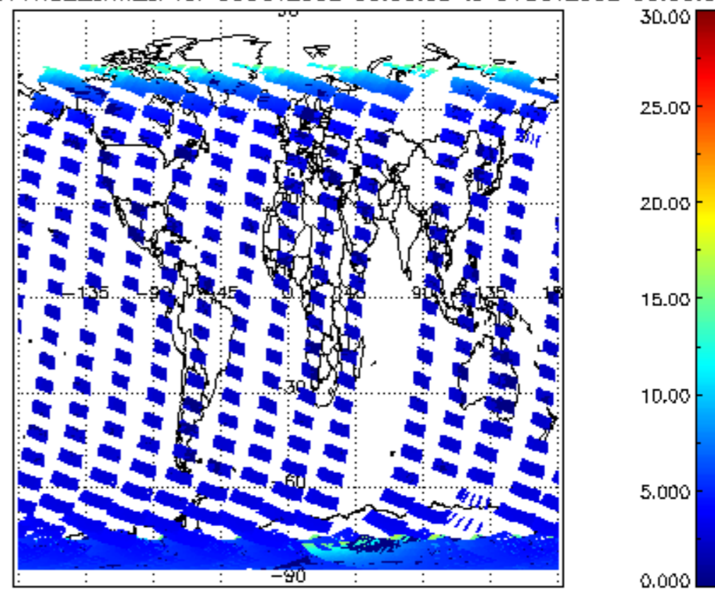
ICIOL2P_NADUV1NO2_amf_cl for 30OCT2002 00:00:00 to 31OCT2002 00:00:00
