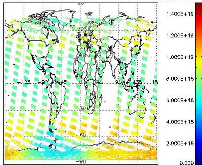
SCIOL2P_NADUV003_vcd for 30OCT2002 00:00:00 to 31OCT2002 00:00:00
