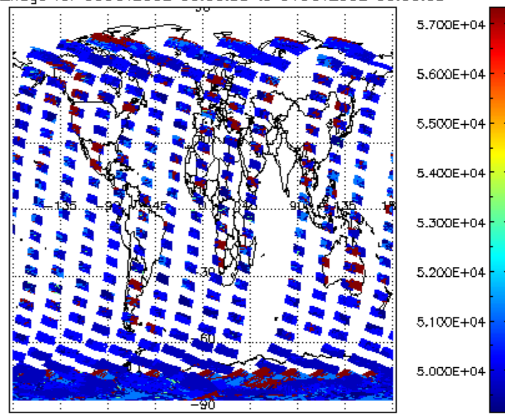
cloud_flags for 30OCT2002 00:00:00 to 31OCT2002 00:00:00
