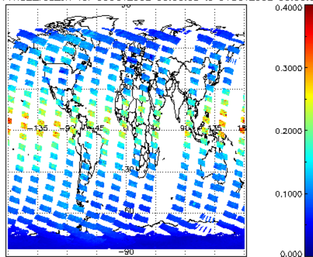
ICIOL2P_NADUV1NO2_vcd_err for 30OCT2002 00:00:00 to 31OCT2002 00:00:00
