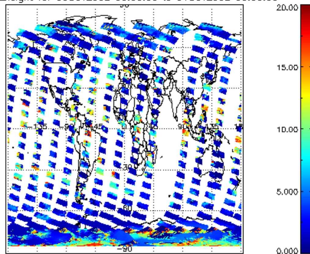
cl_top_height for 30OCT2002 00:00:00 to 31OCT2002 00:00:00
