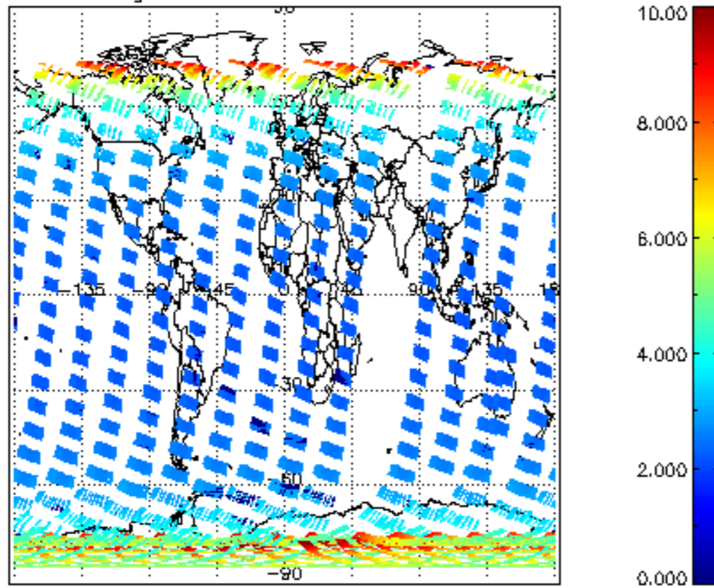
SCIOL2P_NADUV003_amf_gr for 30OCT2002 00:00:00 to 31OCT2002 00:00:00
