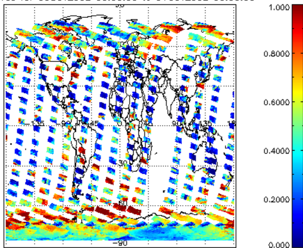
cl_frac for 30OCT2002 00:00:00 to 31OCT2002 00:00:00
