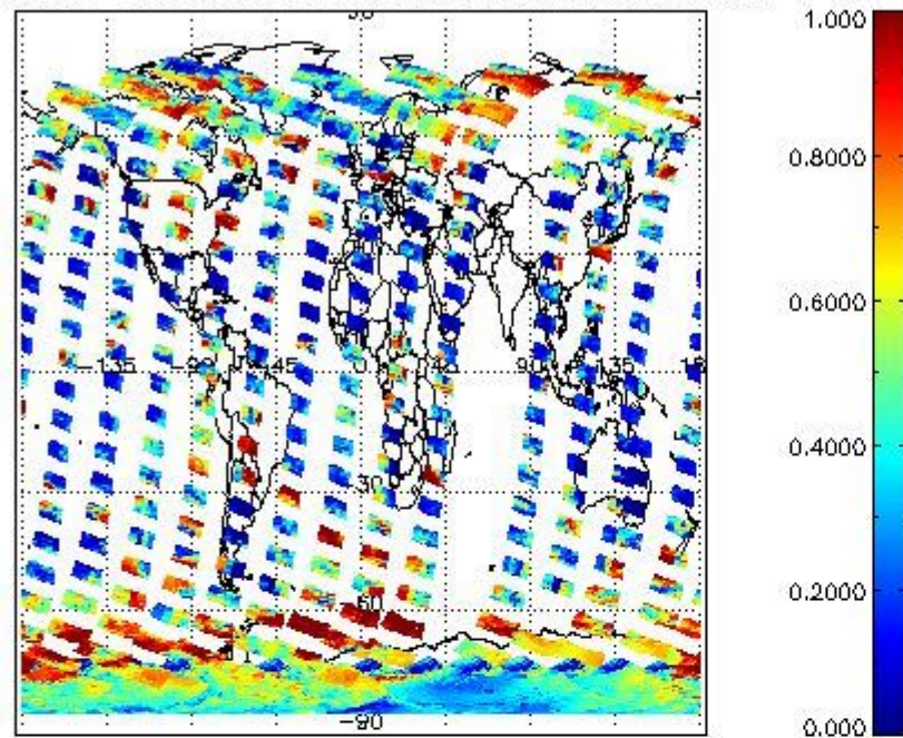
cLfrac for 30OCT2002 00:00:00 to 31OCT2002 00:00:00
