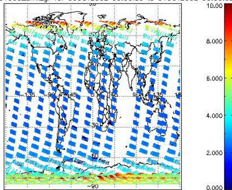
SCIOL2P_NADUV003_amf_gr for 30OCT2002 00:00:00 to 31OCT2002 00:00:00
