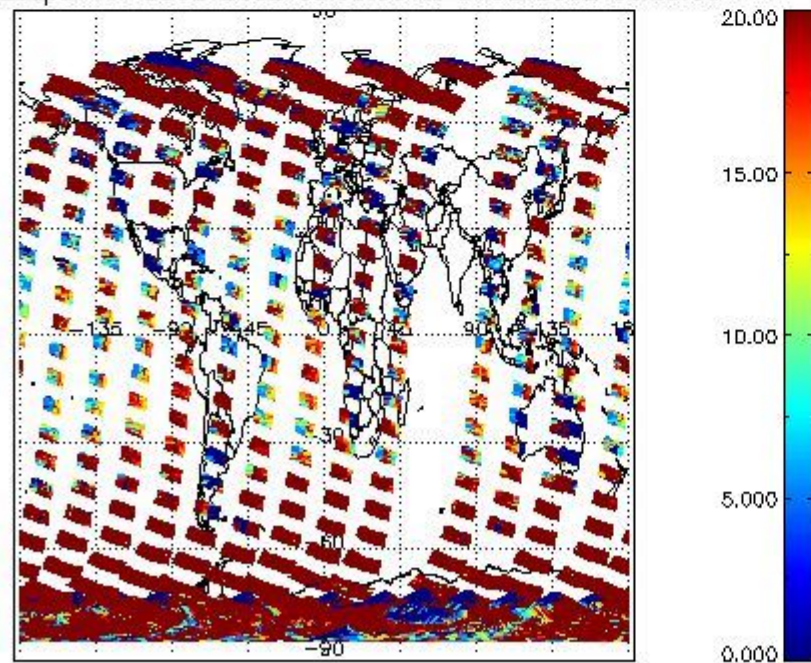
cLopt_depth for 30OCT2002 00:00:00 to 31OCT2002 00:00:00
