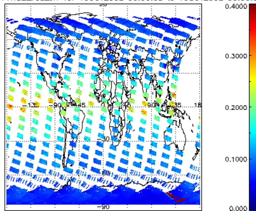
ICIOL2P_NADUV1NO2_vcd_err for 15OCT2002 00:00:00 to 16OCT2002 00:00:00
