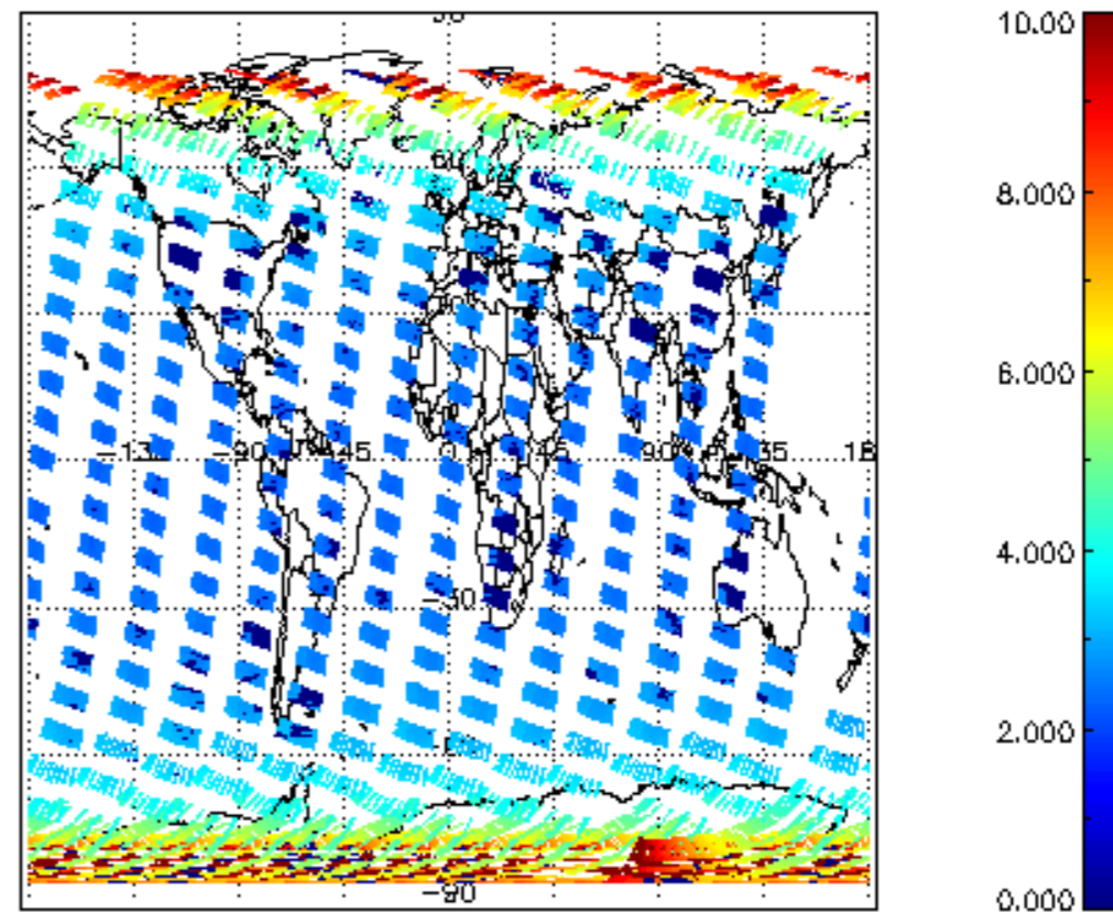
SCIOL2P_NADUV003_amf_el for 15OCT2002 00:00:00 to 16OCT2002 00:00:00
