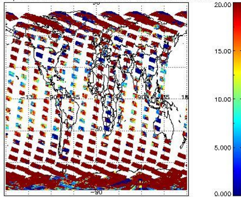
cLopt_depth for 15OCT2002 00:00:00 to 16OCT2002 00:00:00
