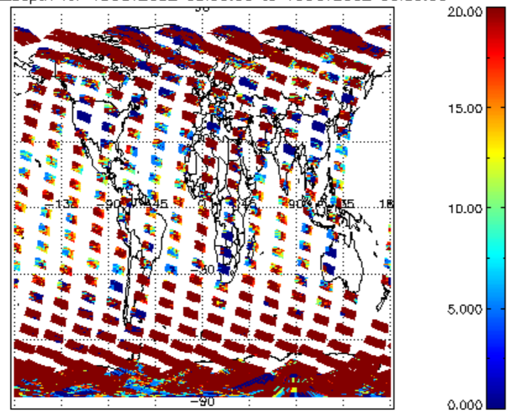
cl_opt_depth for 15OCT2002 00:00:00 to 16OCT2002 00:00:00
