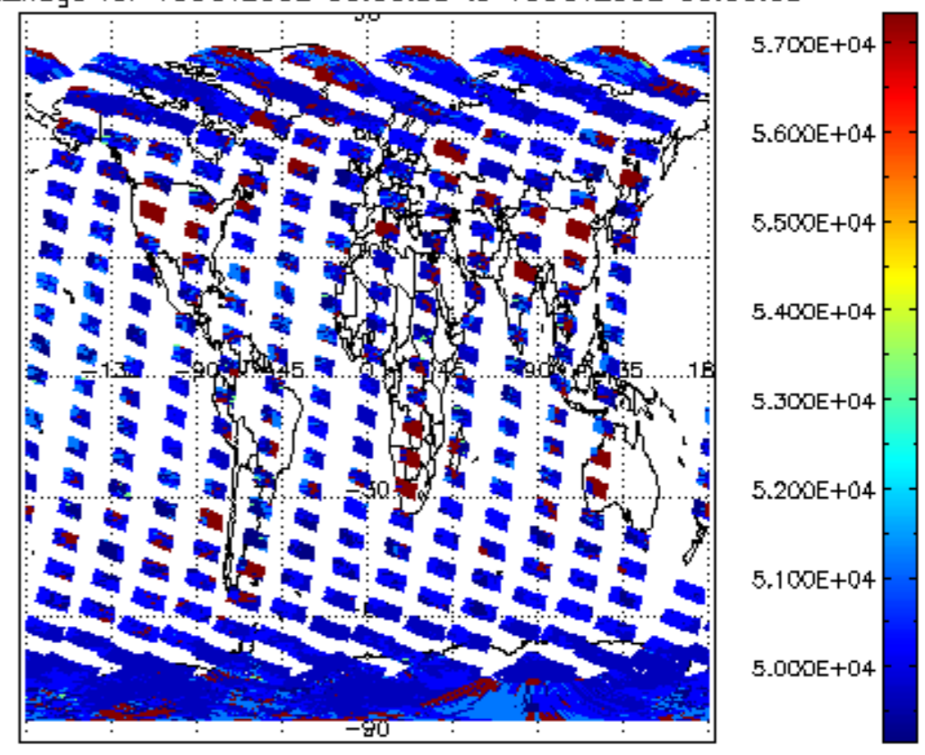
cloud_flags for 15OCT2002 00:00:00 to 16OCT2002 00:00:00
