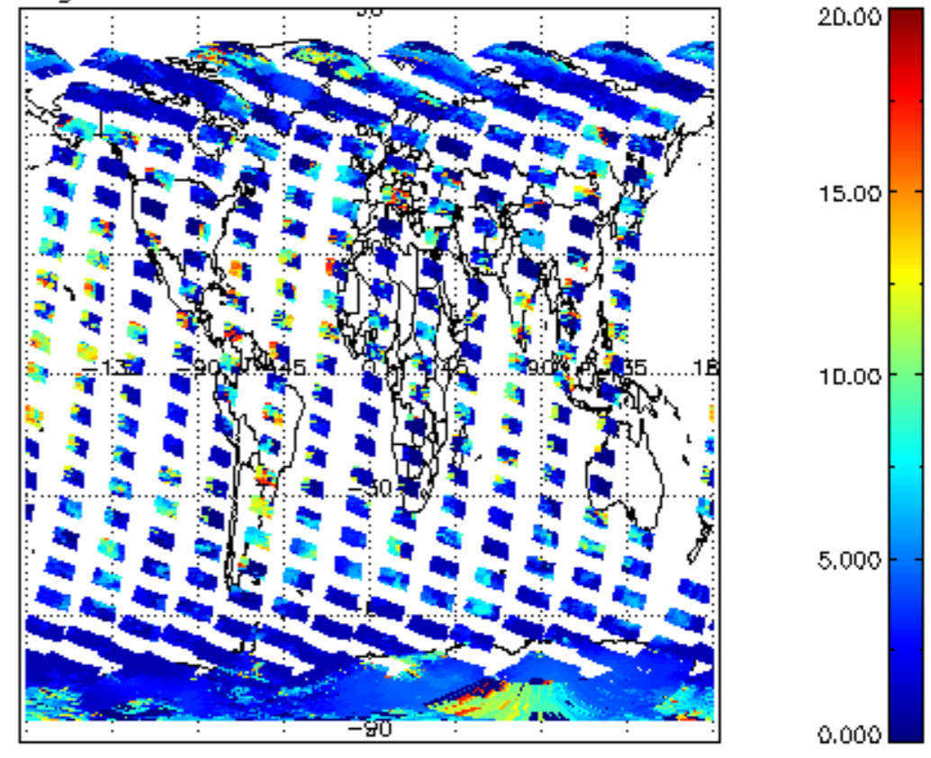
cl_top_height for 15OCT2002 00:00:00 to 16OCT2002 00:00:00
