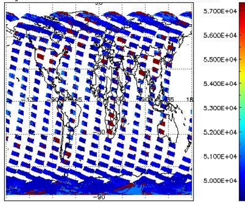
cloud_flags for 15OCT2002 00:00:00 to 16OCT2002 00:00:00
