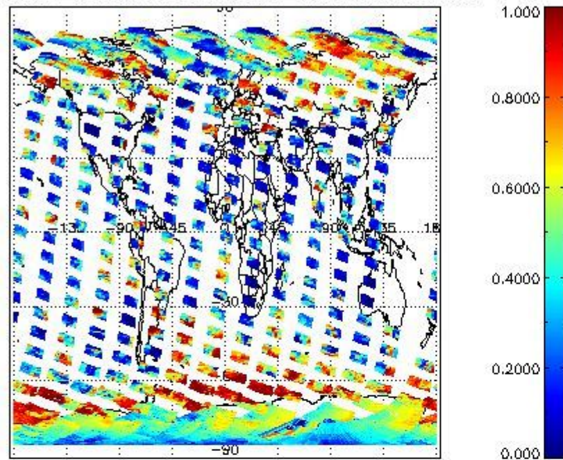
cLfrac for 15OCT2002 00:00:00 to 16OCT2002 00:00:00
