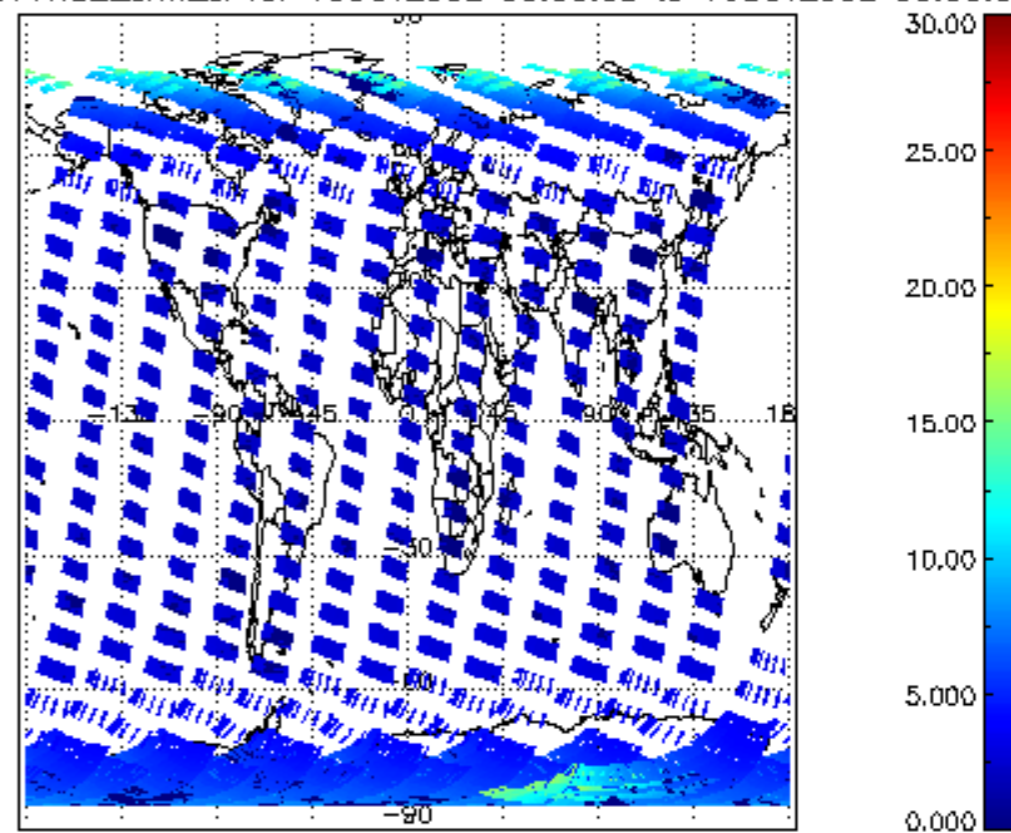
ICIOL2P_NADUV1NO2_amf_cl for 15OCT2002 00:00:00 to 16OCT2002 00:00:00
