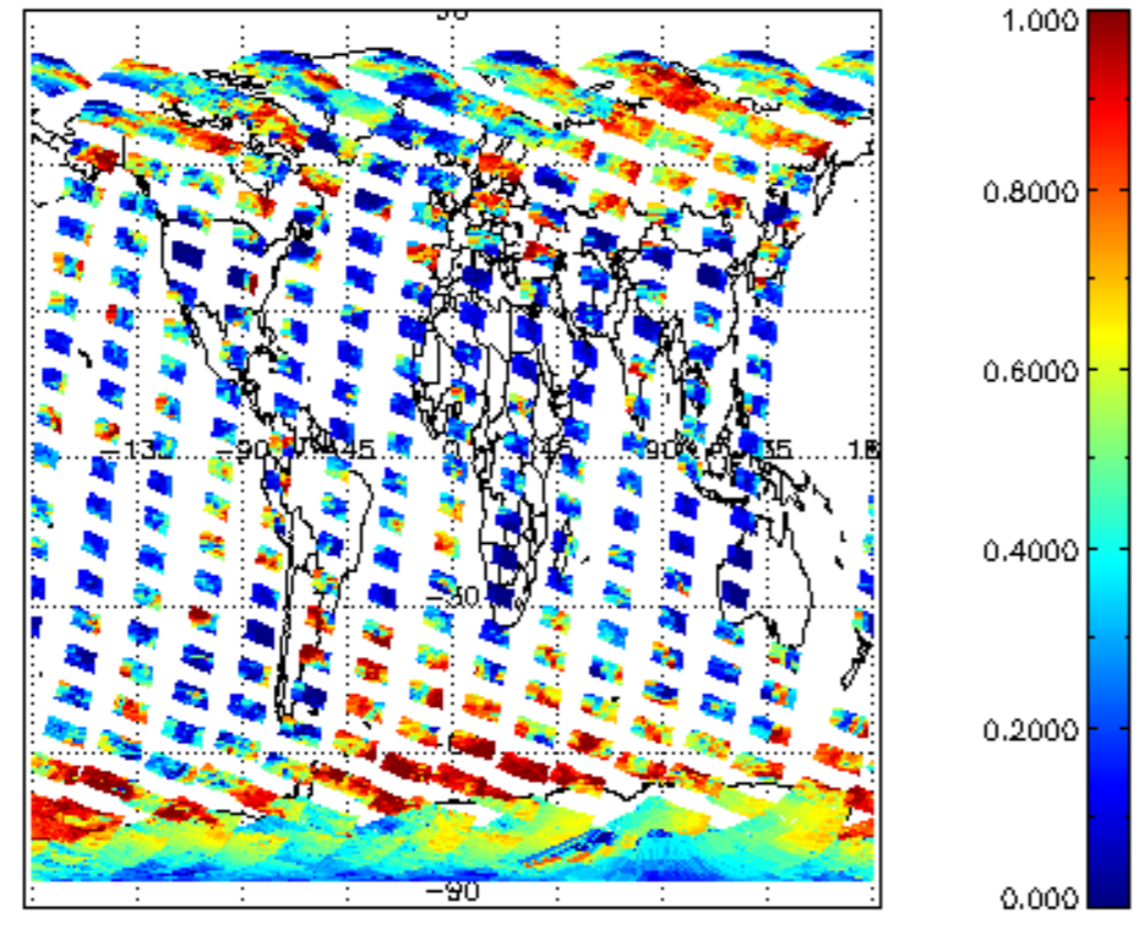
cl_frac for 15OCT2002 00:00:00 to 16OCT2002 00:00:00
