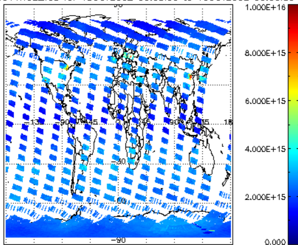
SCIOL2P_NADUV1NO2_vcd for 15OCT2002 00:00:00 to 16OCT2002 00:00:00
