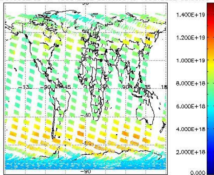
SCIOL2P_NADUV003_vcd for 15OCT2002 00:00:00 to 16OCT2002 00:00:00
