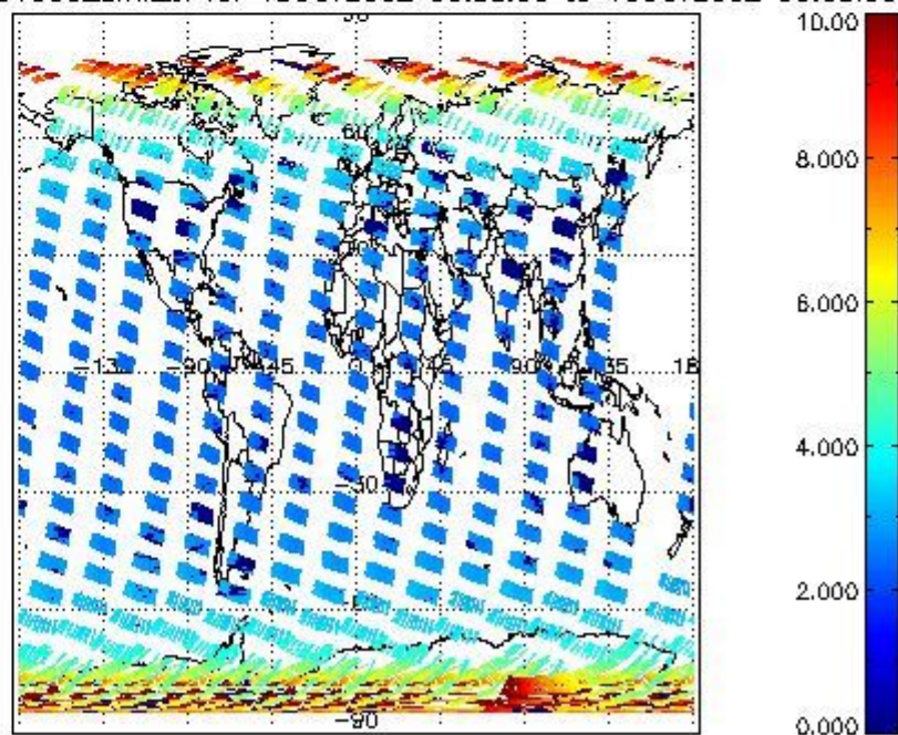
SCIOL2P_NADUV003_amf_sl for 15OCT2002 00:00:00 to 16OCT2002 00:00:00
