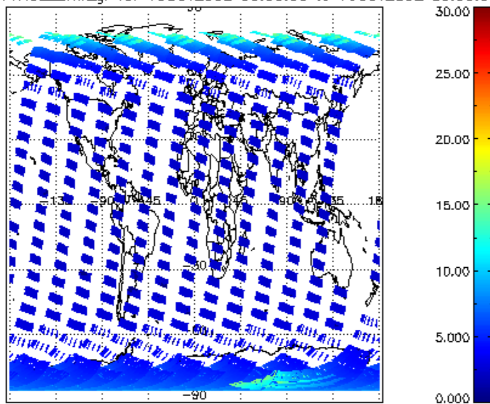
ICIOL2P_NADUV1NO2_amf_gr for 15OCT2002 00:00:00 to 16OCT2002 00:00:00
