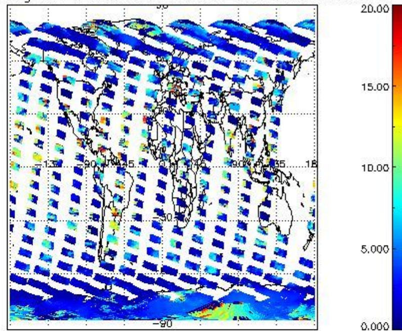
cL_top_height for 15OCT2002 00:00:00 to 16OCT2002 00:00:00
