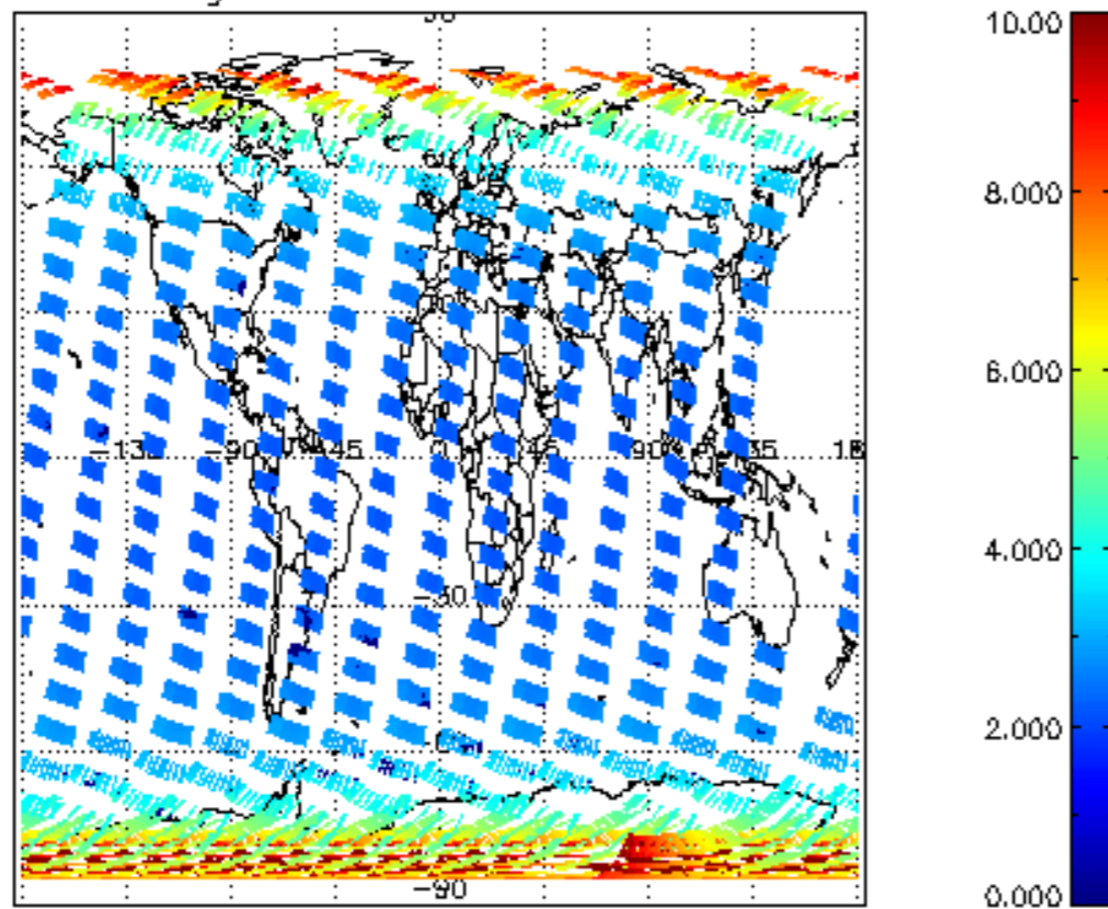
SCIOL2P_NADUV003_amf_gr for 15OCT2002 00:00:00 to 16OCT2002 00:00:00
