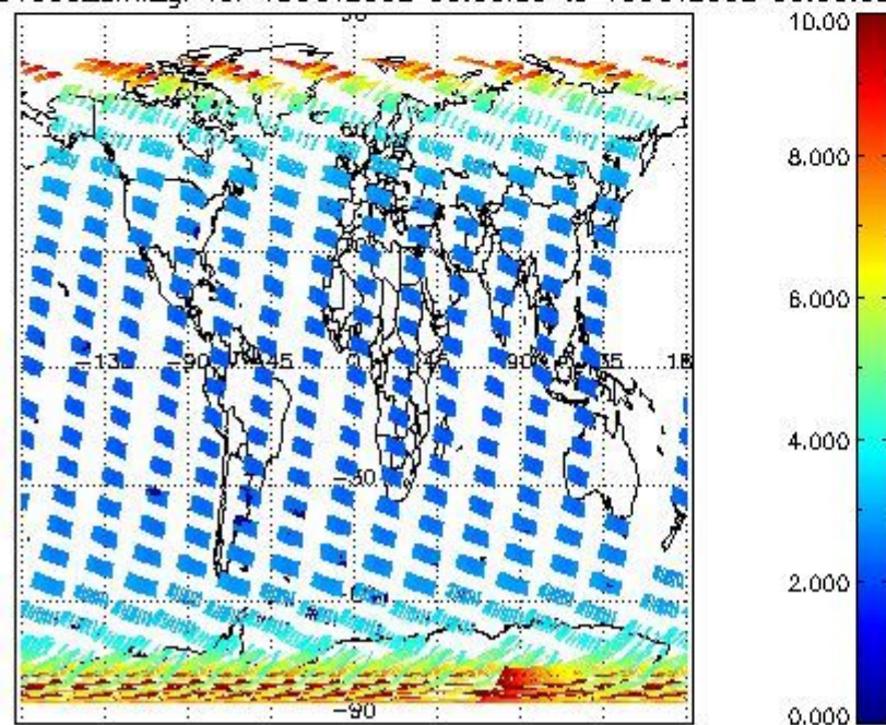
SCIOL2P_NADUV003_amf_gr for 15OCT2002 00:00:00 to 16OCT2002 00:00:00
