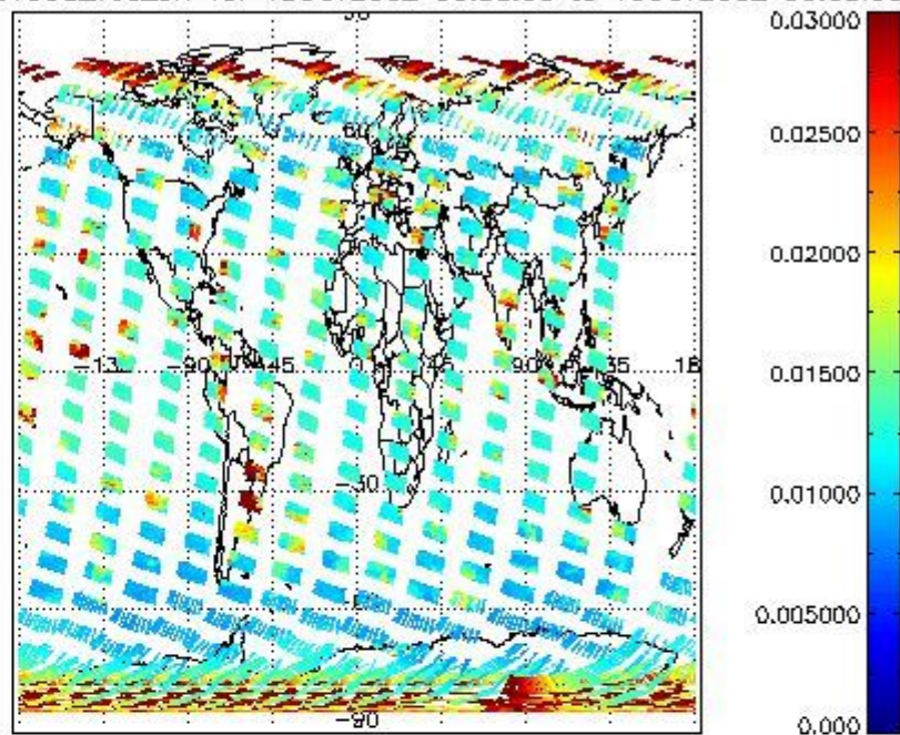
SCIOL2P_NADUV003_vcd_err for 15OCT2002 00:00:00 to 16OCT2002 00:00:00
