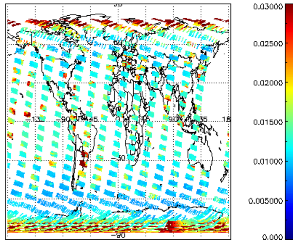
SCIOL2P_NADUV003_vcd_err for 15OCT2002 00:00:00 to 16OCT2002 00:00:00
