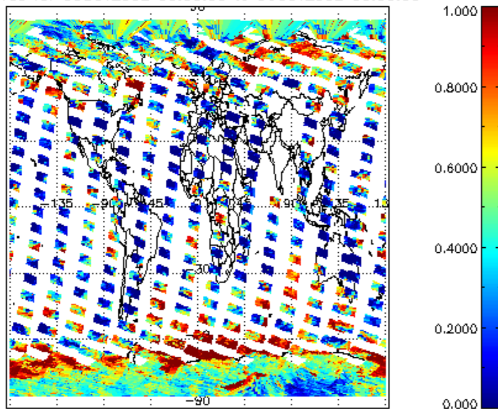
cl_frac for 05OCT2002 00:00:00 to 06OCT2002 00:00:00
