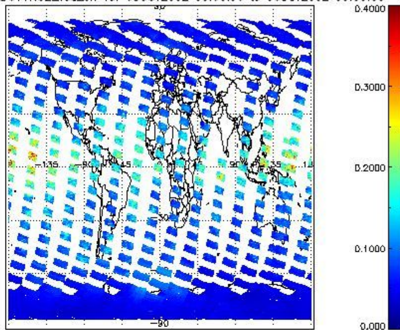
SCIOL2P_NADUV1N02_vcd_err for 05OCT2002 00:00:00 to 06OCT2002 00:00:00
