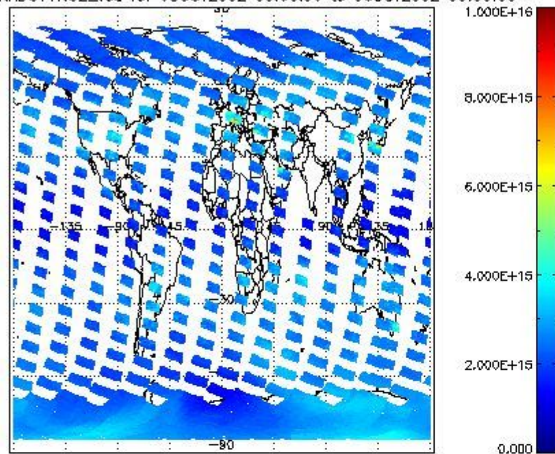
SCIOL2P_NADUV1N02_vcd for 05OCT2002 00:00:00 to 06OCT2002 00:00:00
