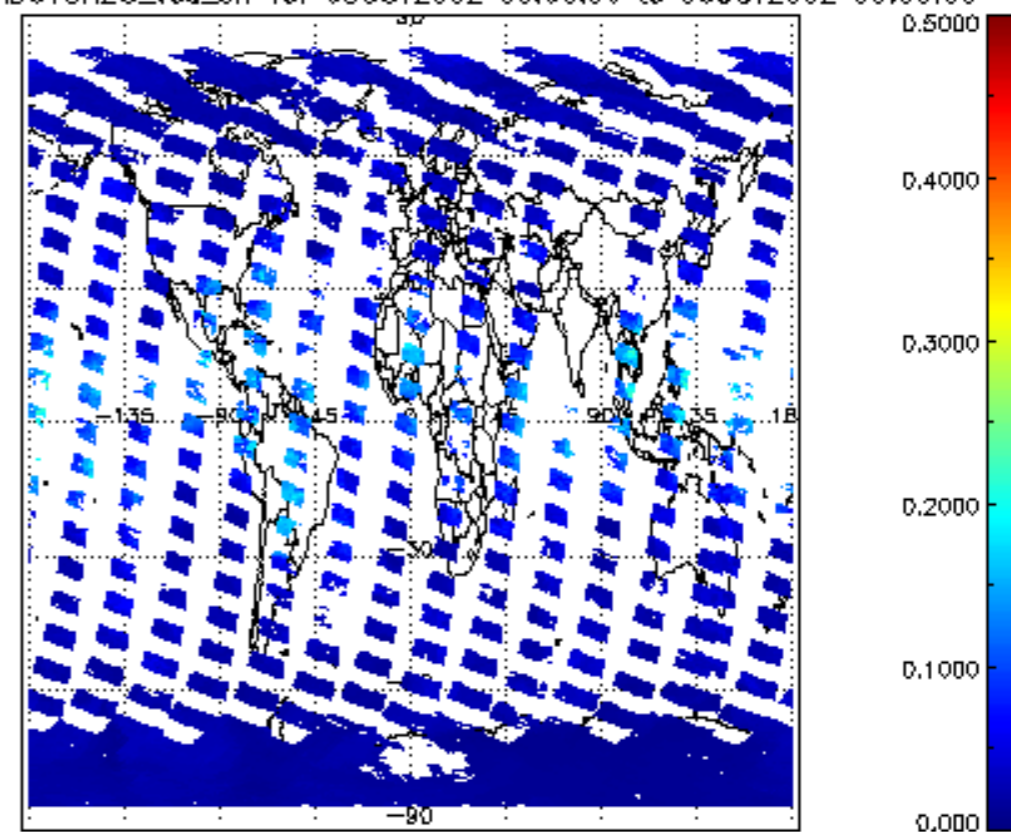
SCIOL2P_NADUV8H20_vcd_err for 05OCT2002 00:00:00 to 06OCT2002 00:00:00
