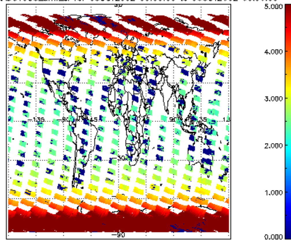
SCIOL2P_NADUV003_amf_cl for 05OCT2002 00:00:00 to 06OCT2002 00:00:00
