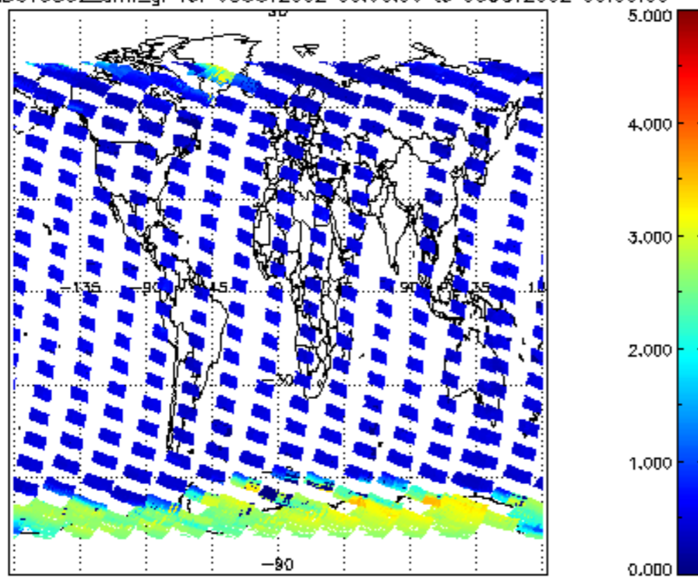
SCIOL2P_NADUV5S02_amf_gr for 05OCT2002 00:00:00 to 06OCT2002 00:00:00
