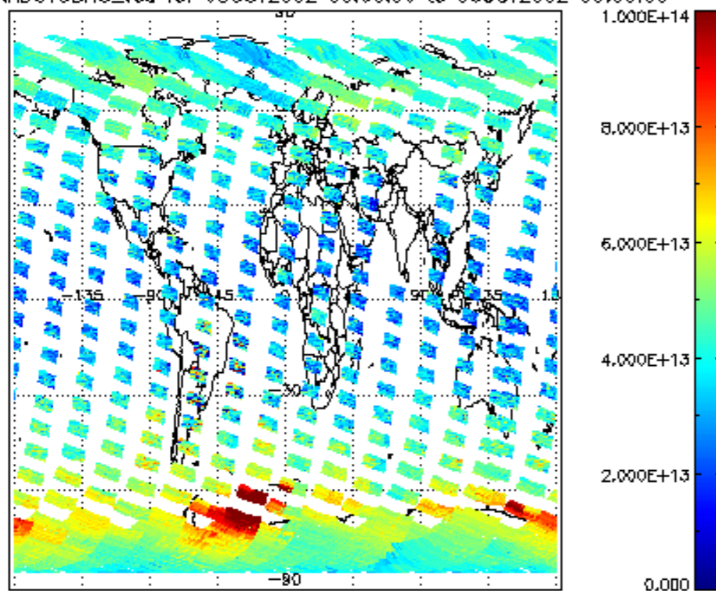
SCIOL2P_NADUV3BRO_vcd for 05OCT2002 00:00:00 to 06OCT2002 00:00:00
