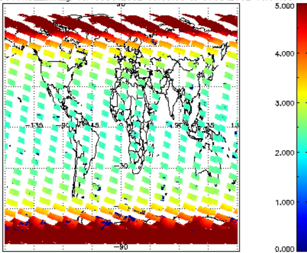
SCIOL2P_NADUV1NO2_amf_gr for 05OCT2002 00:00:00 to 06OCT2002 00:00:00
