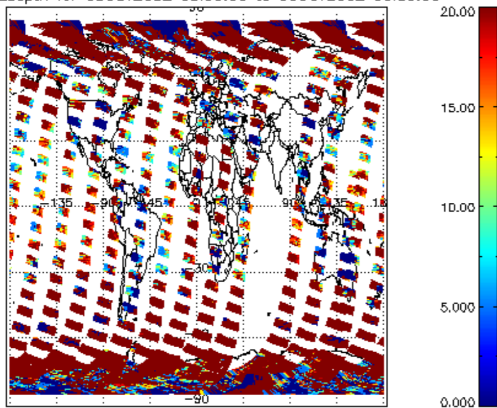
cl_opt_depth for 05OCT2002 00:00:00 to 06OCT2002 00:00:00
