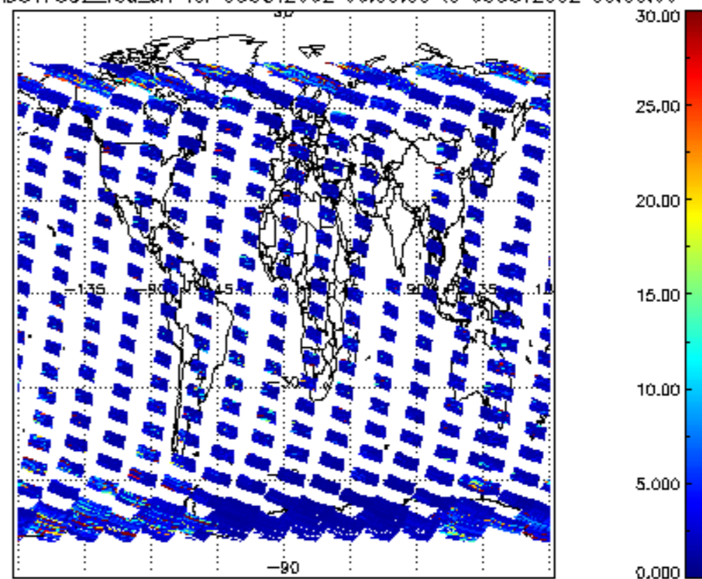
SCIOL2P_NADUV7S02_vcd_err for 05OCT2002 00:00:00 to 06OCT2002 00:00:00
