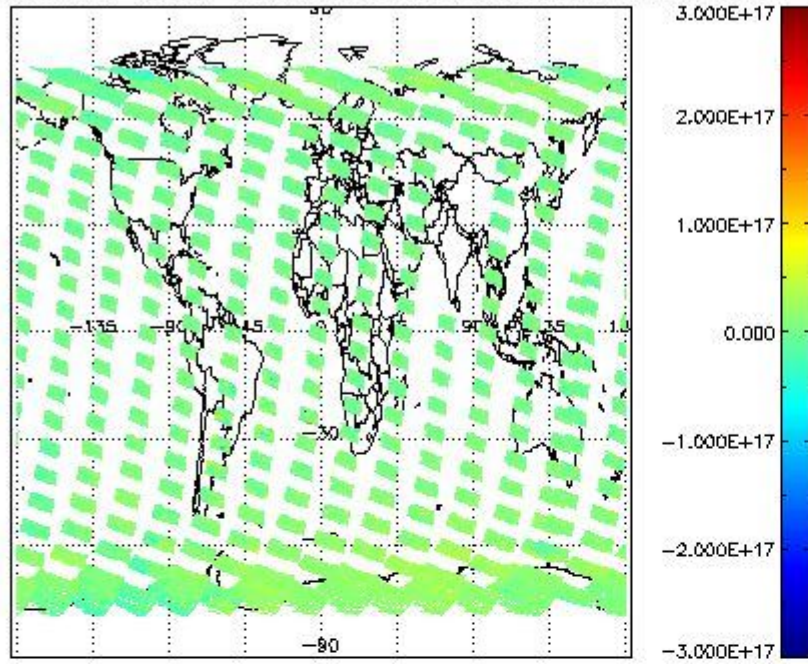
SCIOL2P_NADUV7S02_vcd for 05OCT2002 00:00:00 to 06OCT2002 00:00:00
