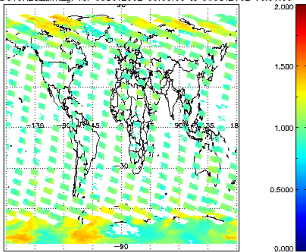
SCIOL2P_NADUV8H20_amf_gr for 05OCT2002 00:00:00 to 06OCT2002 00:00:00
