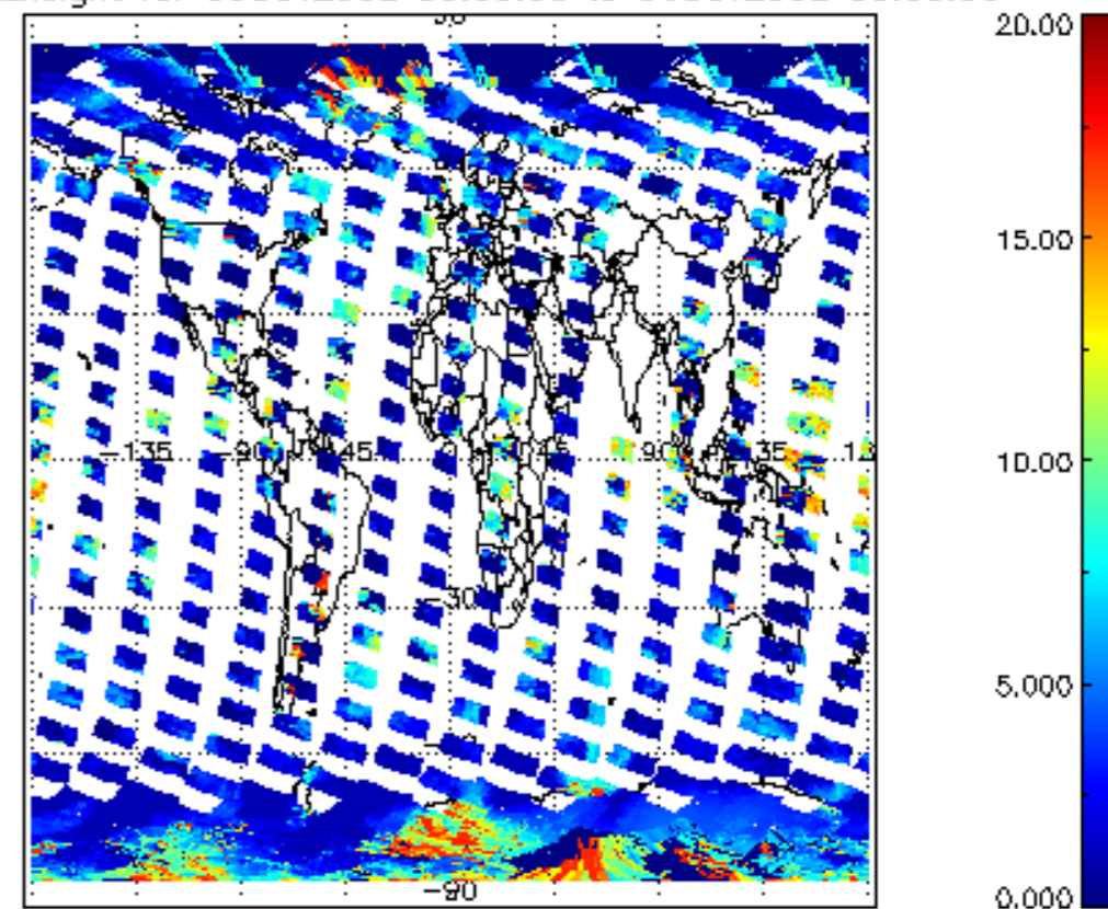
cl_top_height for 05OCT2002 00:00:00 to 06OCT2002 00:00:00
