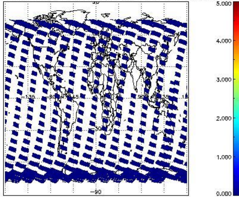
SCIOL2P_NADUV7S02_amf_cl for 05OCT2002 00:00:00 to 06OCT2002 00:00:00
