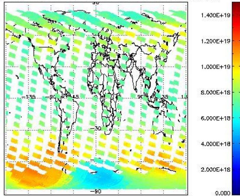
SCIOL2P_NADUV003_vcd for 05OCT2002 00:00:00 to 06OCT2002 00:00:00
