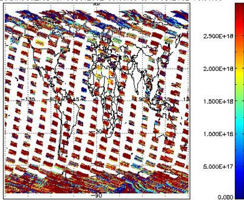
SCIDL2P_NADIR3CO_vcd for 05OCT2002 00:00:00 to 06OCT2002 00:00:00
