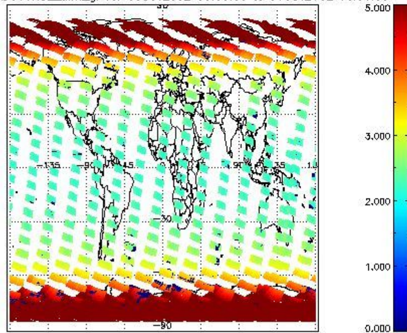
SCIOL2P_NADUV1N02_amf_gr for 05OCT2002 00:00:00 to 06OCT2002 00:00:00
