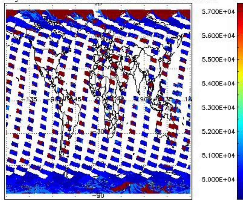
cloud_flags for 05OCT2002 00:00:00 to 06OCT2002 00:00:00
