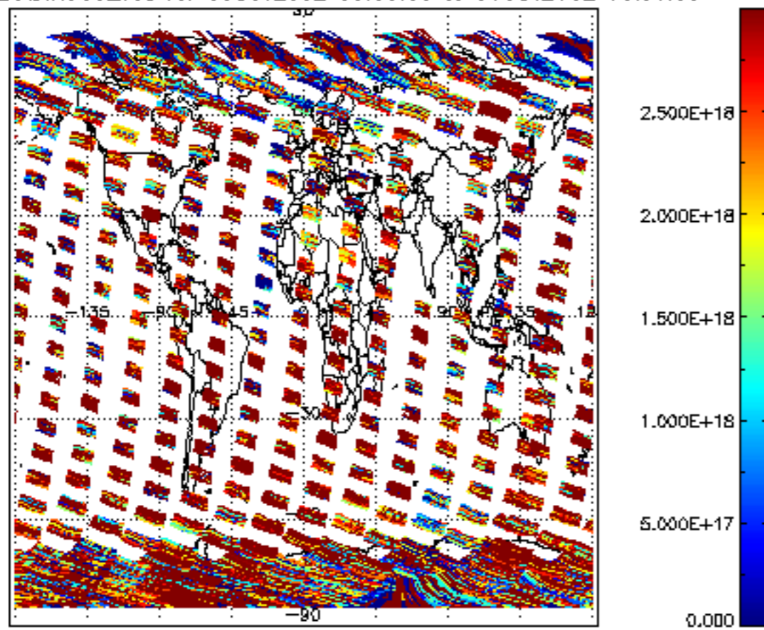
SCIOL2P_NADIR3CO_vcd for 05OCT2002 00:00:00 to 06OCT2002 00:00:00
