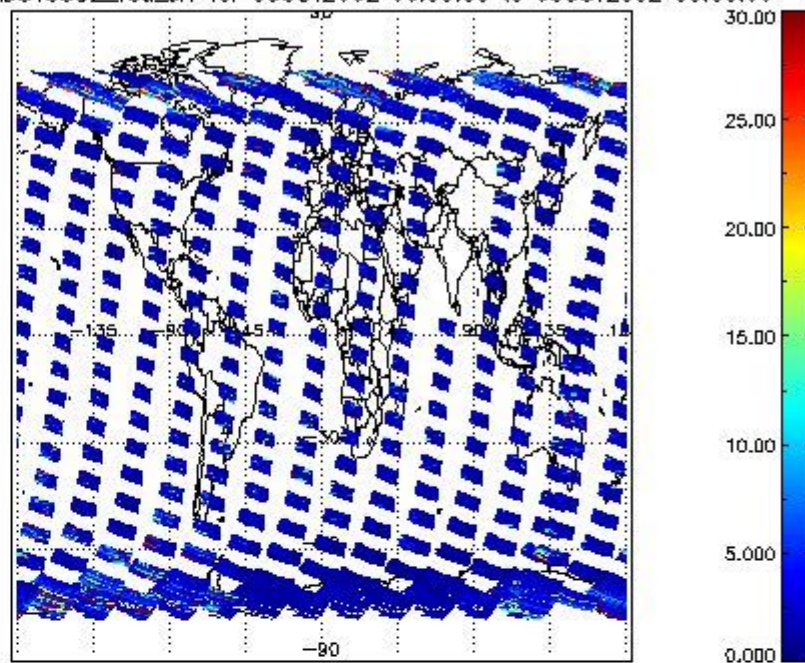
SCIOL2P_NADUV5S02_vcd_err for 05OCT2002 00:00:00 to 06OCT2002 00:00:00
