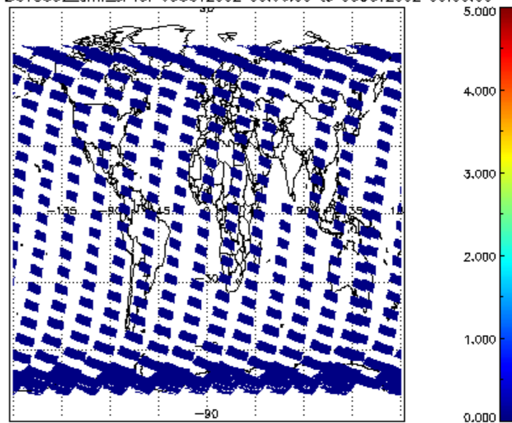
SCIOL2P_NADUV5S02_amf_cl for 05OCT2002 00:00:00 to 06OCT2002 00:00:00
