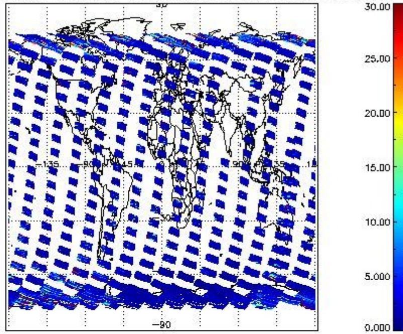
SCIOL2P_NADUV7S02_vcd_err for 05OCT2002 00:00:00 to 06OCT2002 00:00:00
