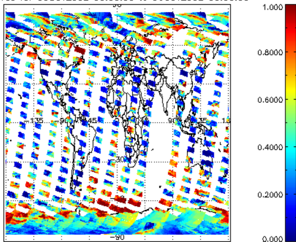
cl_frac for 05OCT2002 00:00:00 to 06OCT2002 00:00:00
