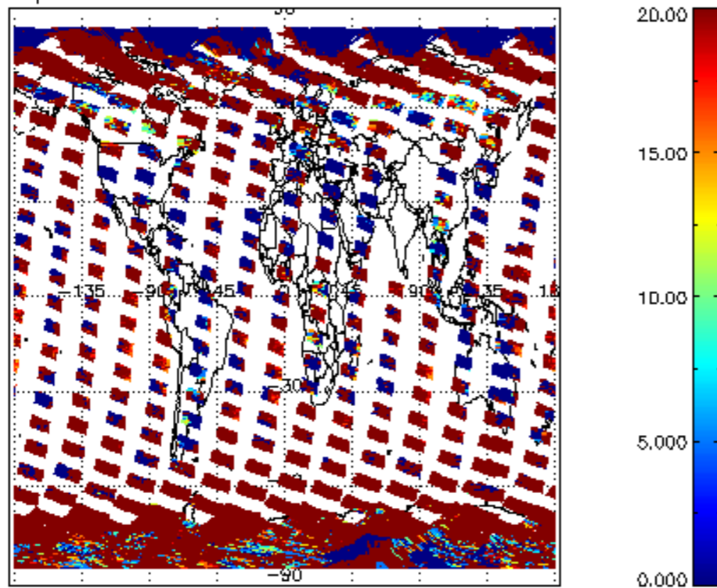
cl_opt_depth for 05OCT2002 00:00:00 to 06OCT2002 00:00:00
