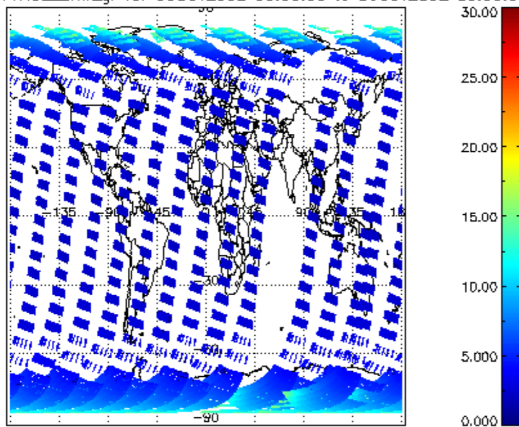
iCIOL2P_NADUV1NO2_amf_gr for 05OCT2002 00:00:00 to 06OCT2002 00:00:00
