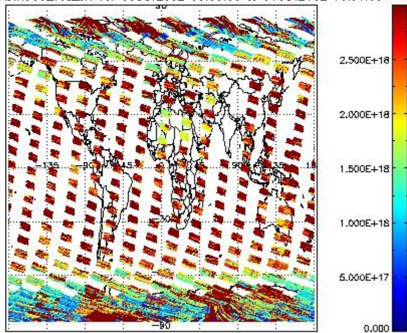
SCIDL2P_NADIR3CO_vcd_err for 05OCT2002 00:00:00 to 06OCT2002 00:00:00
