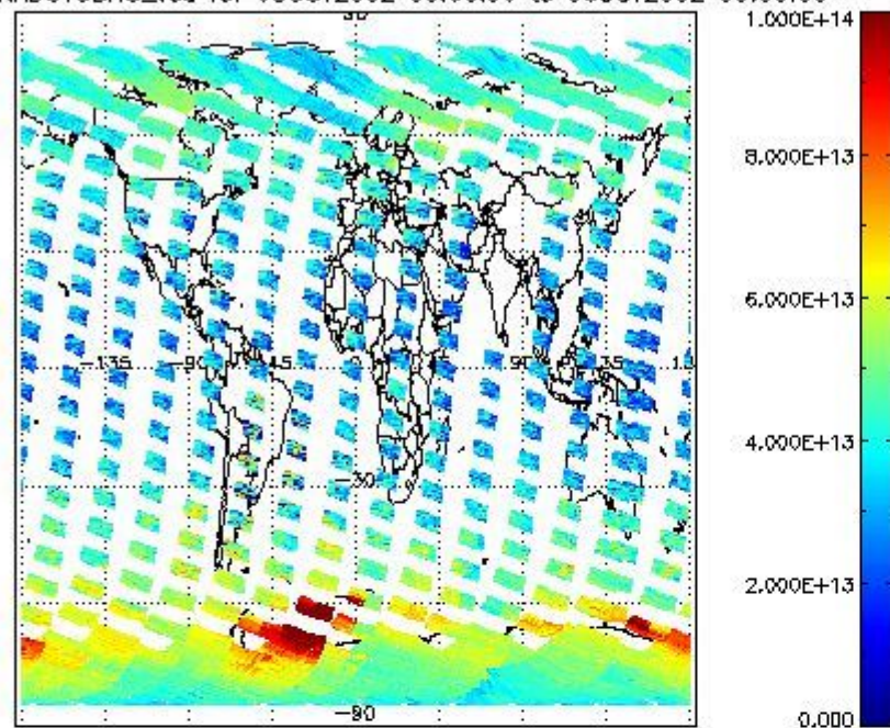
SCIOL2P_NADUV3BRO_vcd for 05OCT2002 00:00:00 to 06OCT2002 00:00:00
