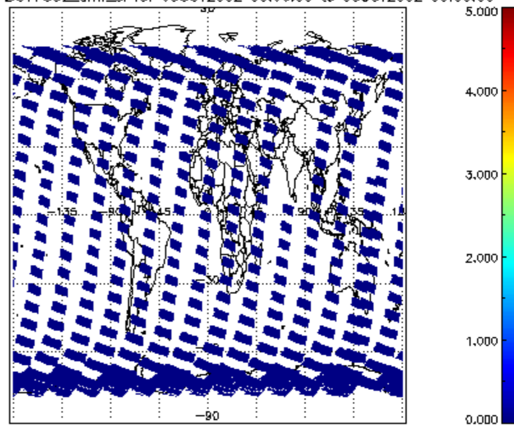
SCIOL2P_NADUV7S02_amf_sl for 05OCT2002 00:00:00 to 06OCT2002 00:00:00
