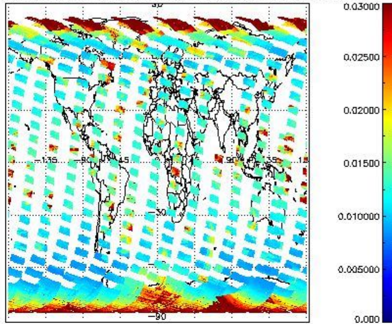
SCIOL2P_NADUV003_vcd_err for 05OCT2002 00:00:00 to 06OCT2002 00:00:00
