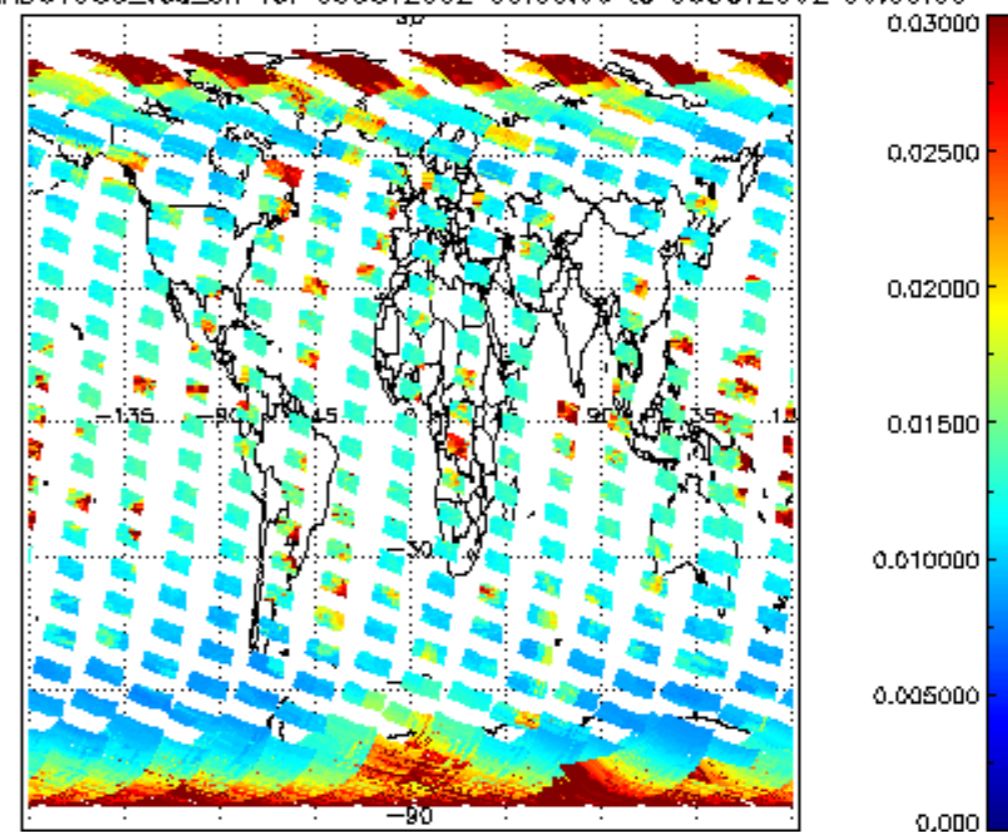
SCIOL2P_NADUV003_vcd_err for 05OCT2002 00:00:00 to 06OCT2002 00:00:00
