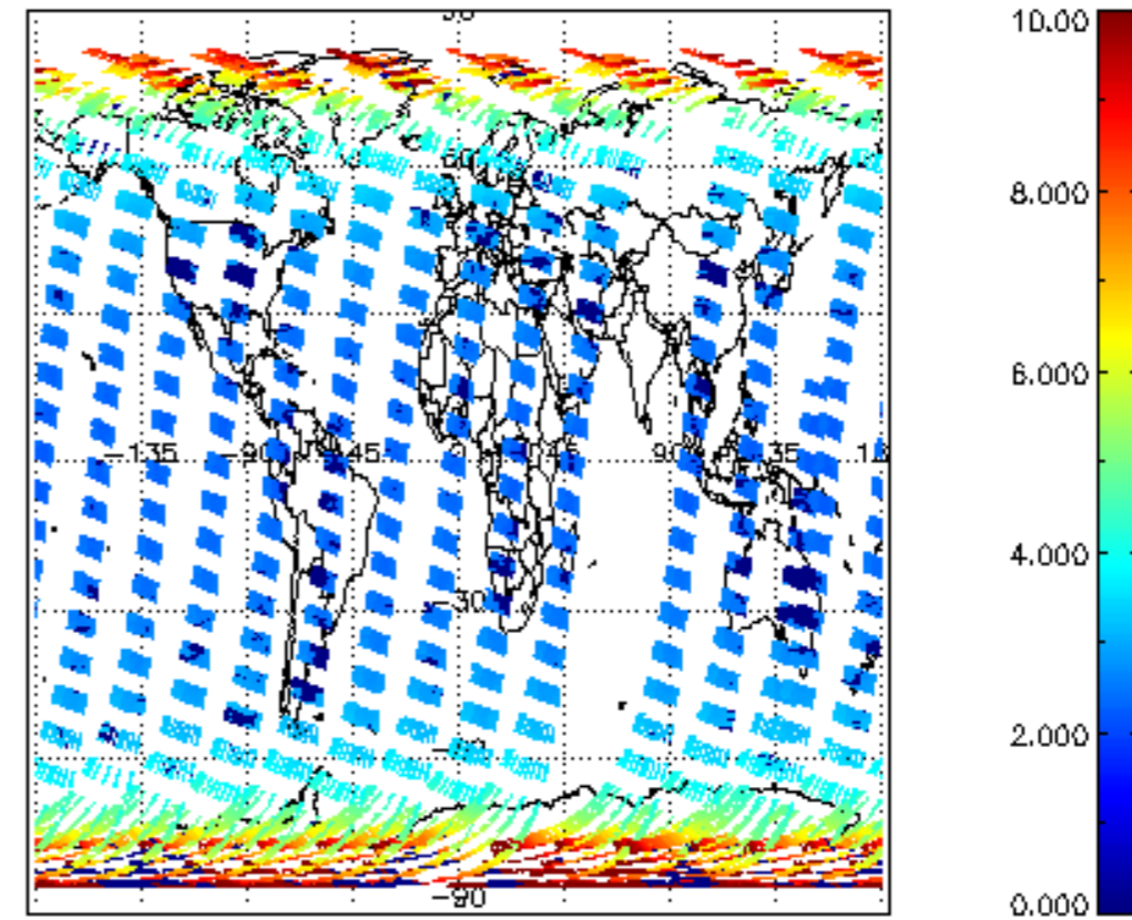
SCIOL2P_NADUV003_amf_el for 05OCT2002 00:00:00 to 06OCT2002 00:00:00
