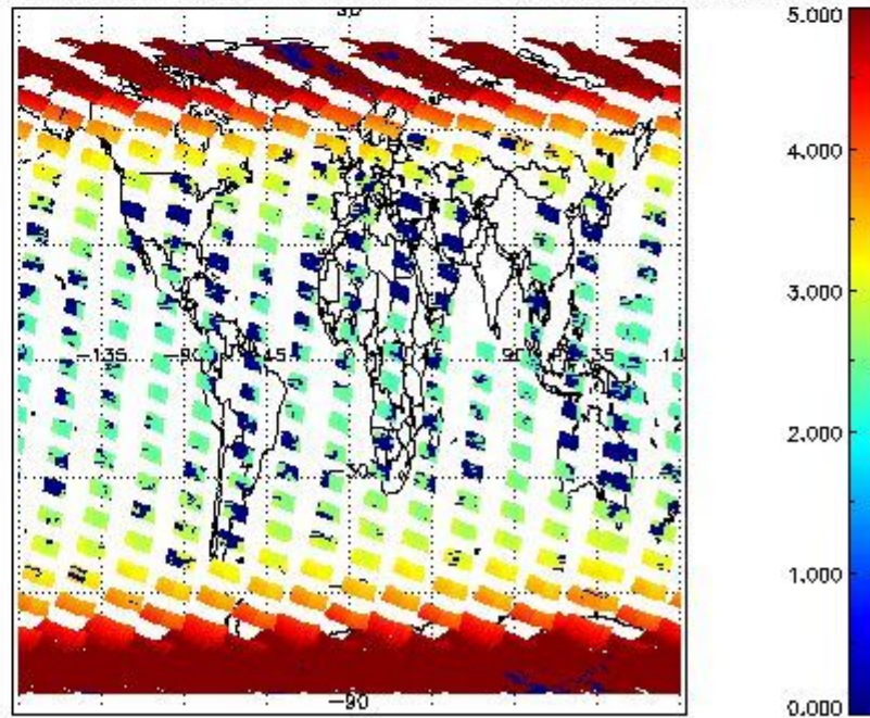
SCIOL2P_NADUV003_amf_cl for 05OCT2002 00:00:00 to 06OCT2002 00:00:00
