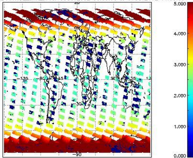
SCIOL2P_NADUV1N02_amf_cl for 05OCT2002 00:00:00 to 06OCT2002 00:00:00
