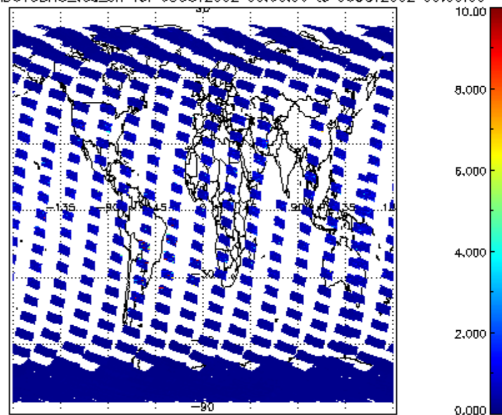
SCIOL2P_NADUV3BRO_vcd_err for 05OCT2002 00:00:00 to 06OCT2002 00:00:00
