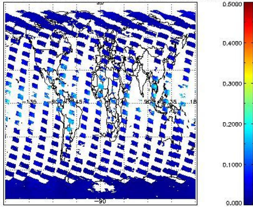
SCIOL2P_NADUV8H20_vcd_err for 05OCT2002 00:00:00 to 06OCT2002 00:00:00
