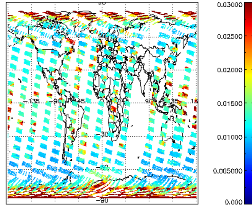
SCIOL2P_NADUV003_vcd_err for 05OCT2002 00:00:00 to 06OCT2002 00:00:00
