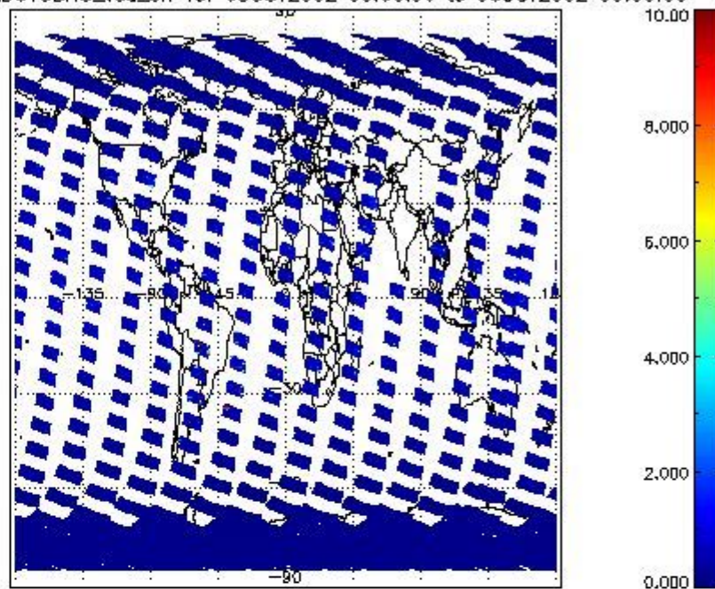
SCIOL2P_NADUV3BRO_vcd_err for 05OCT2002 00:00:00 to 06OCT2002 00:00:00
