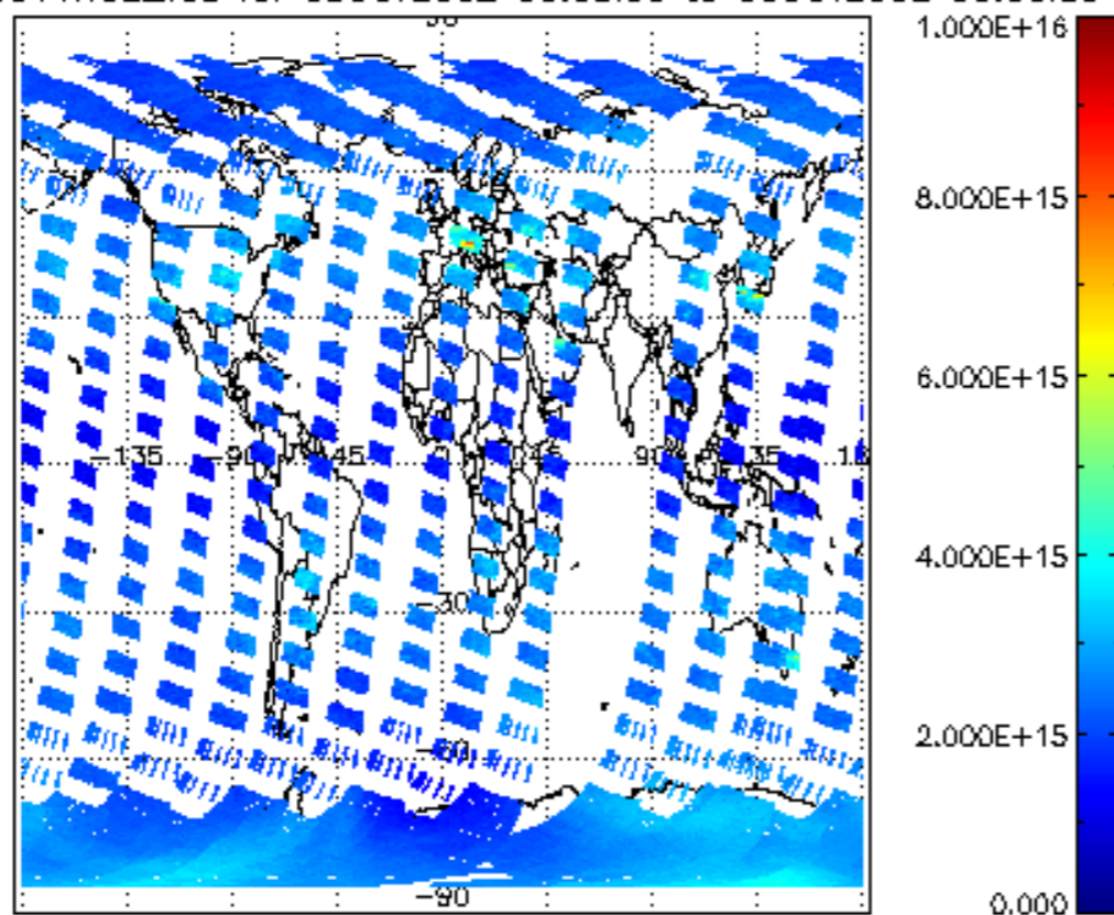
SCIOL2P_NADUV1NO2_vcd for 05OCT2002 00:00:00 to 06OCT2002 00:00:00
