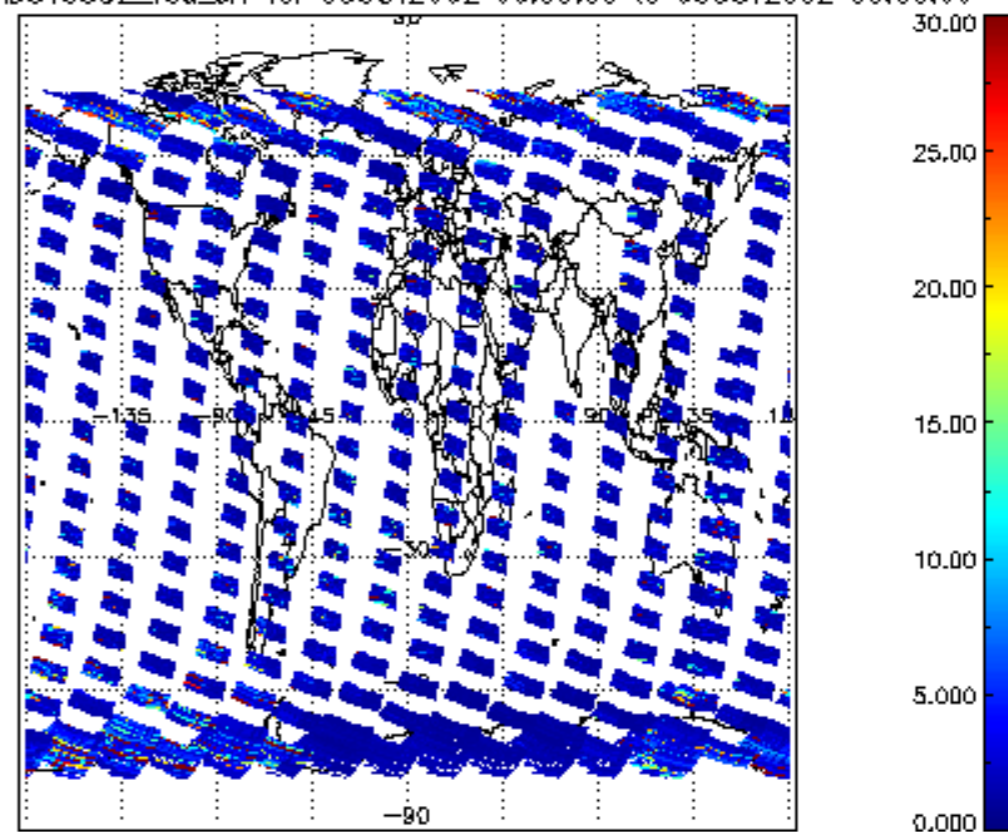
SCIOL2P_NADUV5S02_vcd_err for 05OCT2002 00:00:00 to 06OCT2002 00:00:00
