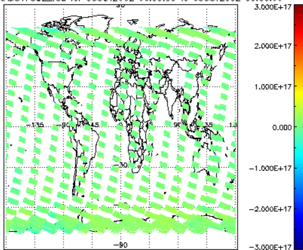
SCIOL2P_NADUV7S02_vcd for 05OCT2002 00:00:00 to 06OCT2002 00:00:00
