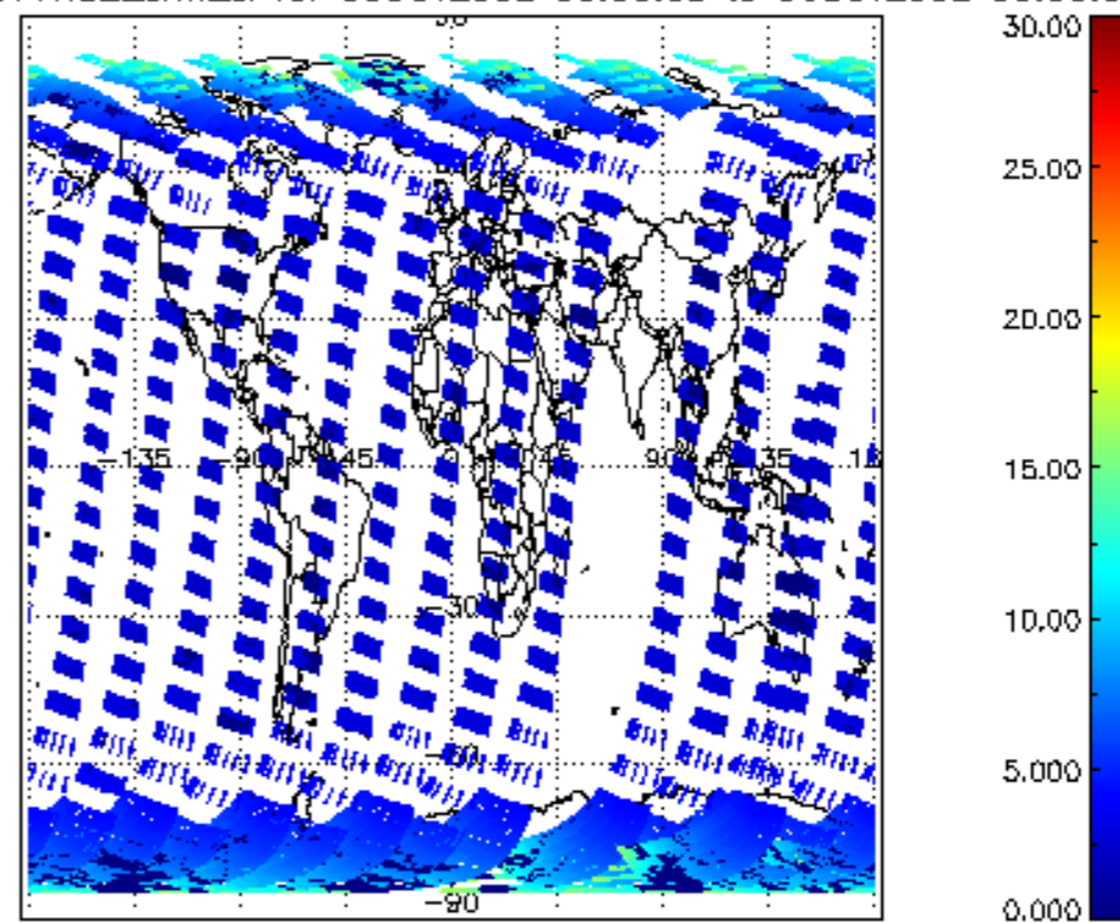
iCIOL2P_NADUV1NO2_amf_cl for 05OCT2002 00:00:00 to 06OCT2002 00:00:00
