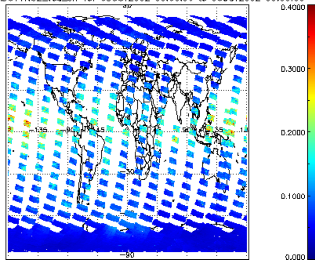
SCIOL2P_NADUV1NO2_vcd_err for 05OCT2002 00:00:00 to 06OCT2002 00:00:00
