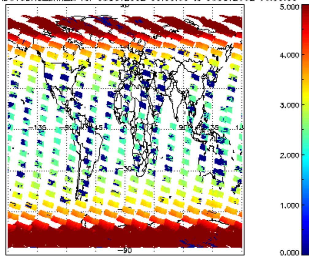
SCIOL2P_NADUV3BRO_amf_cl for 05OCT2002 00:00:00 to 06OCT2002 00:00:00
