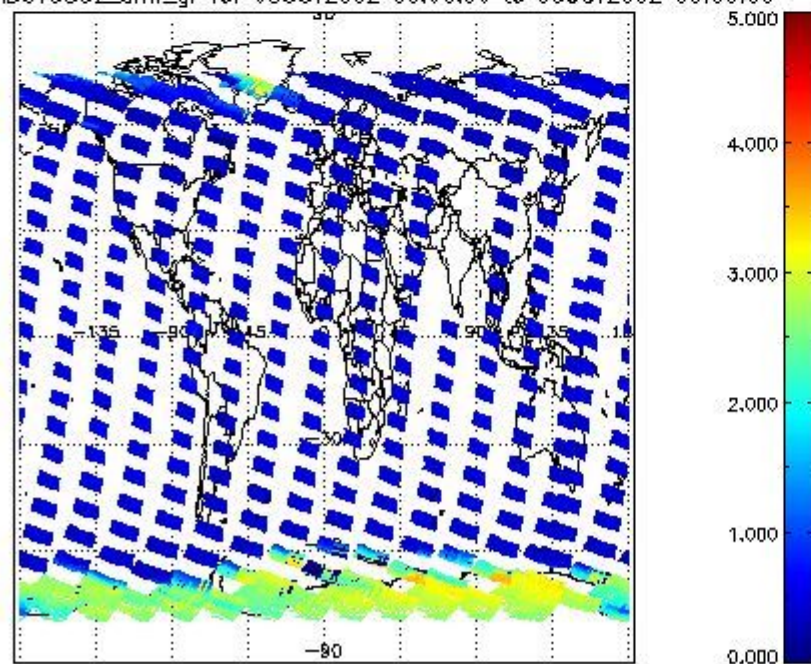
SCIOL2P_NADUV5S02_amf_gr for 05OCT2002 00:00:00 to 06OCT2002 00:00:00
