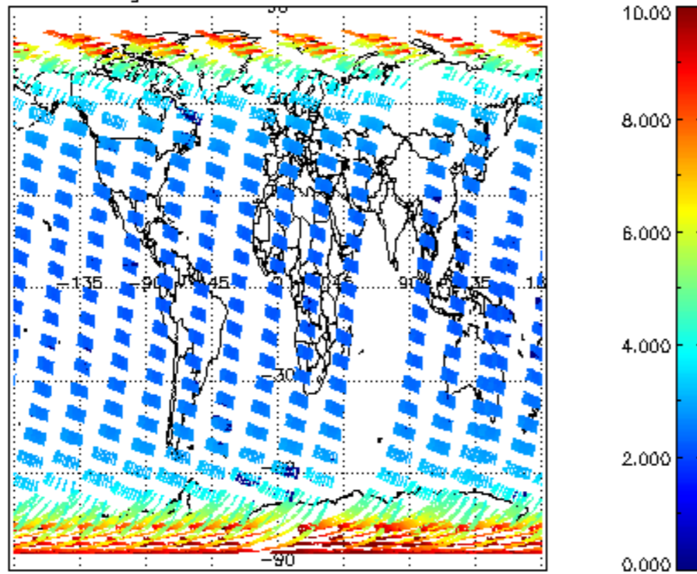
SCIOL2P_NADUV003_amf_gr for 05OCT2002 00:00:00 to 06OCT2002 00:00:00
