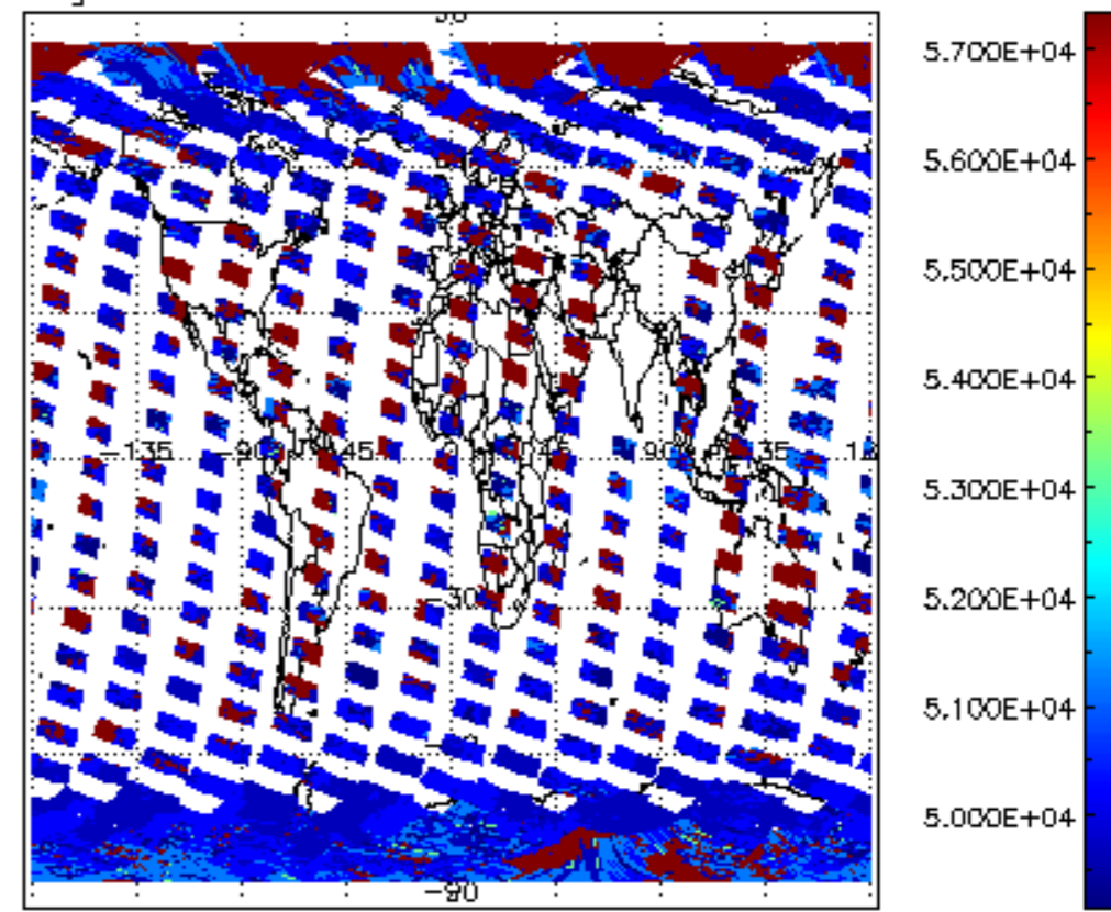
cloud_flags for 05OCT2002 00:00:00 to 06OCT2002 00:00:00
