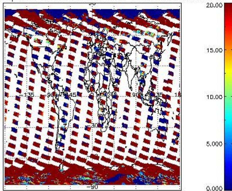
cL_opt_depth for 05OCT2002 00:00:00 to 06OCT2002 00:00:00
