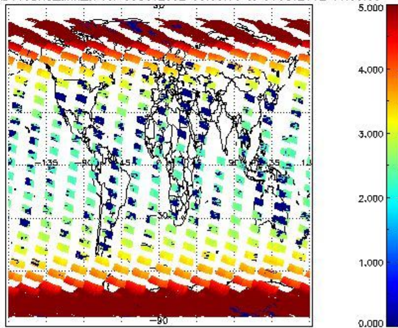
SCIOL2P_NADUV3BRO_amf_cl for 05OCT2002 00:00:00 to 06OCT2002 00:00:00
