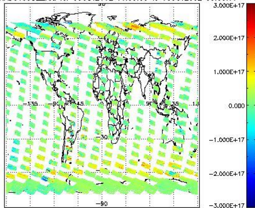
SCIOL2P_NADUV5S02_vcd for 05OCT2002 00:00:00 to 06OCT2002 00:00:00
