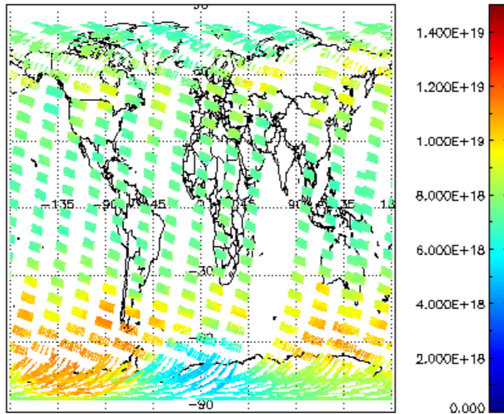
SCIOL2P_NADUV003_vcd for 05OCT2002 00:00:00 to 06OCT2002 00:00:00
