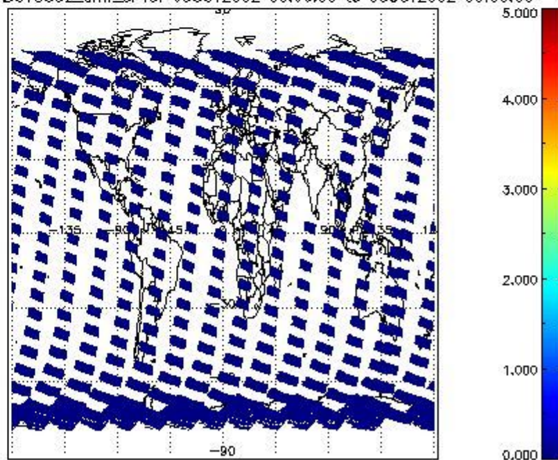
SCIOL2P_NADUV5S02_amf_cl for 05OCT2002 00:00:00 to 06OCT2002 00:00:00
