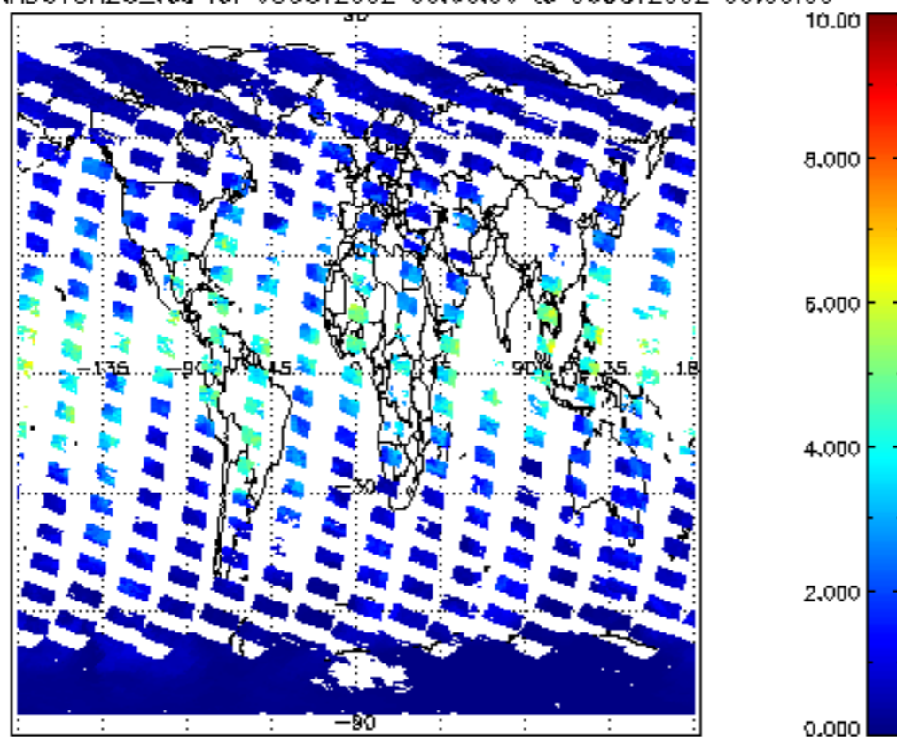
SCIOL2P_NADUV8H20_vcd for 05OCT2002 00:00:00 to 06OCT2002 00:00:00
