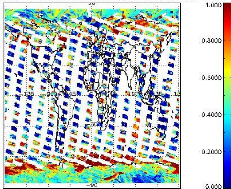
cLfrac for 05OCT2002 00:00:00 to 06OCT2002 00:00:00
