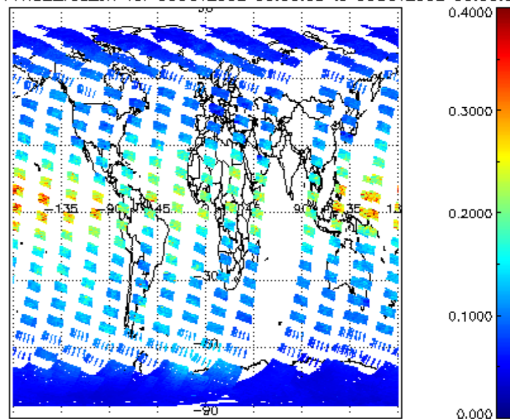
iCIOL2P_NADUV1NO2_vcd_err for 05OCT2002 00:00:00 to 06OCT2002 00:00:00
