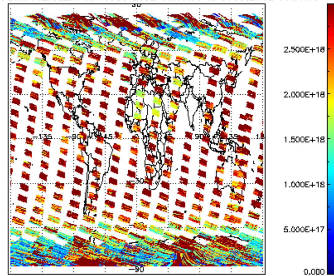
SCIOL2P_NADIR3CO_vcd_err for 05OCT2002 00:00:00 to 06OCT2002 00:00:00
