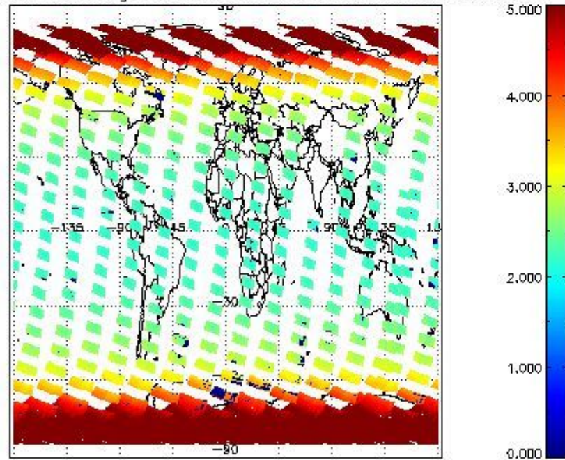
SCIOL2P_NADUV003_amf_gr for 05OCT2002 00:00:00 to 06OCT2002 00:00:00
