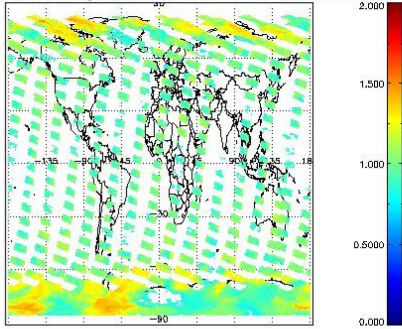
SCIOL2P_NADUV8H20_amf_gr for 05OCT2002 00:00:00 to 06OCT2002 00:00:00
