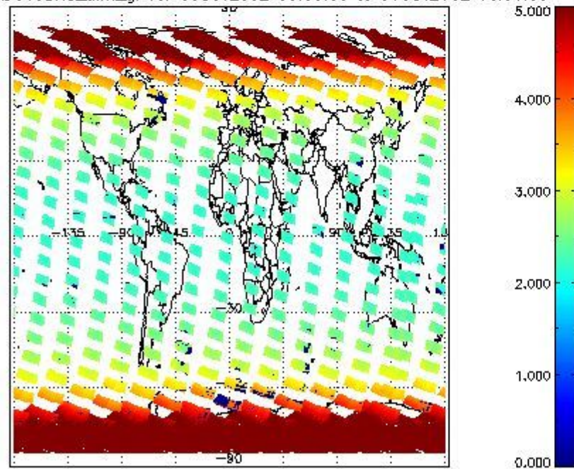
SCIOL2P_NADUV3BRO_amf_gr for 05OCT2002 00:00:00 to 06OCT2002 00:00:00
