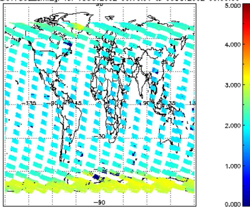
SCIOL2P_NADUV7S02_amf_gr for 05OCT2002 00:00:00 to 06OCT2002 00:00:00
