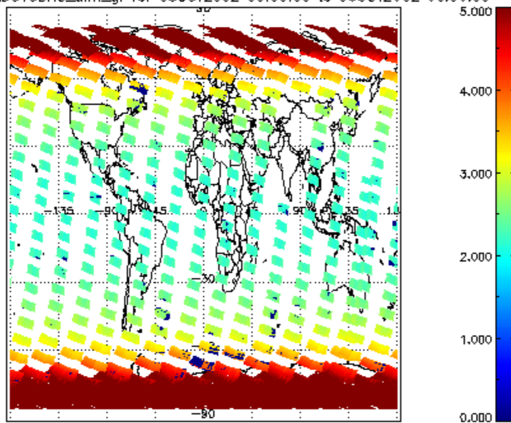
SCIOL2P_NADUV3BRO_amf_gr for 05OCT2002 00:00:00 to 06OCT2002 00:00:00
