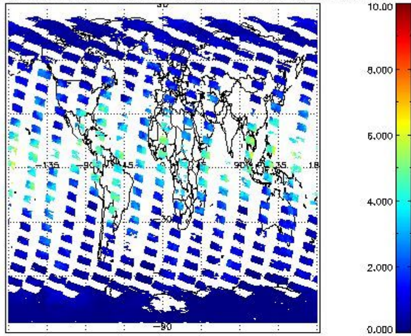
SCIOL2P_NADUV8H20_vcd for 05OCT2002 00:00:00 to 06OCT2002 00:00:00
