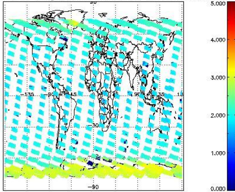
SCIOL2P_NADUV7S02_amf_gr for 05OCT2002 00:00:00 to 06OCT2002 00:00:00
