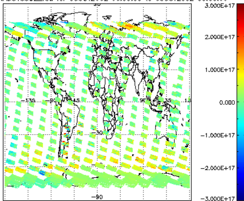
SCIOL2P_NADUV5S02_vcd for 05OCT2002 00:00:00 to 06OCT2002 00:00:00
