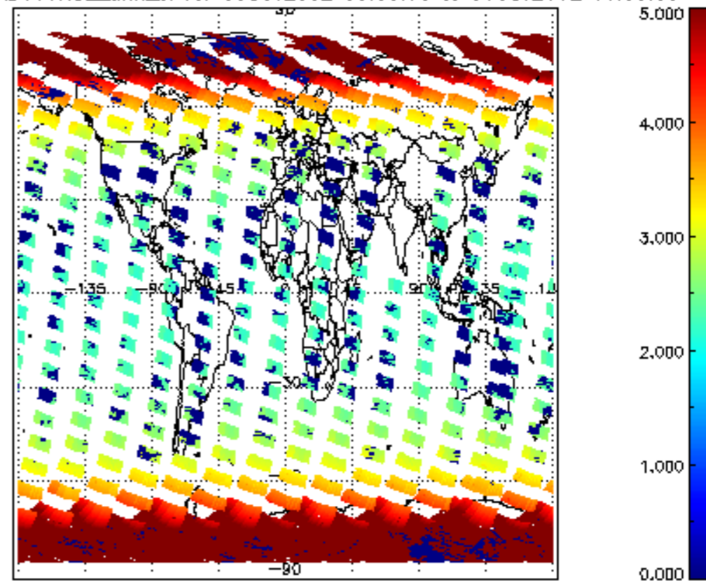
SCIOL2P_NADUV1NO2_amf_cl for 05OCT2002 00:00:00 to 06OCT2002 00:00:00
