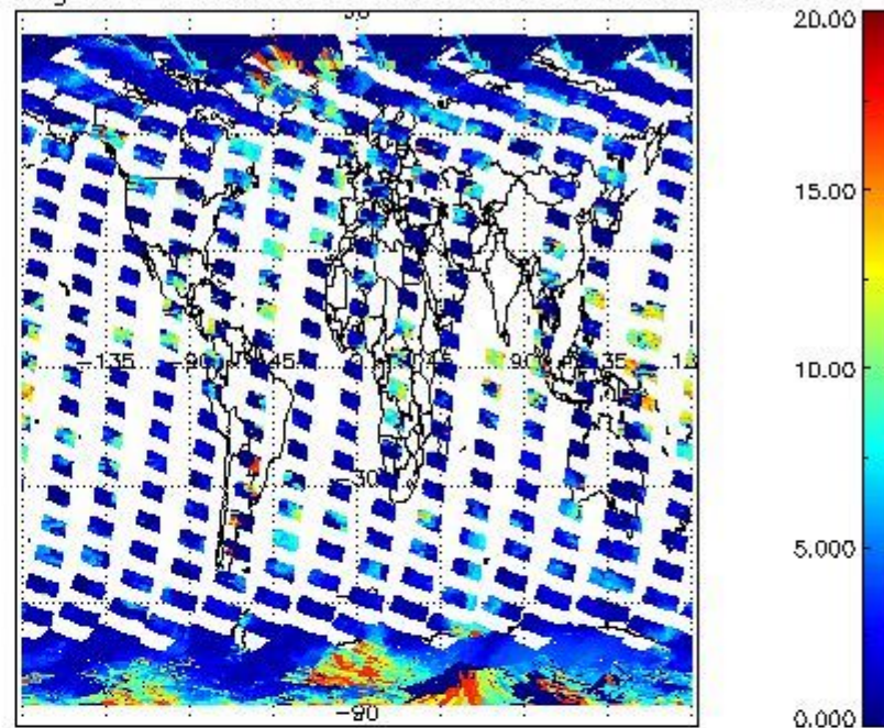
cL_top_height for 05OCT2002 00:00:00 to 06OCT2002 00:00:00
