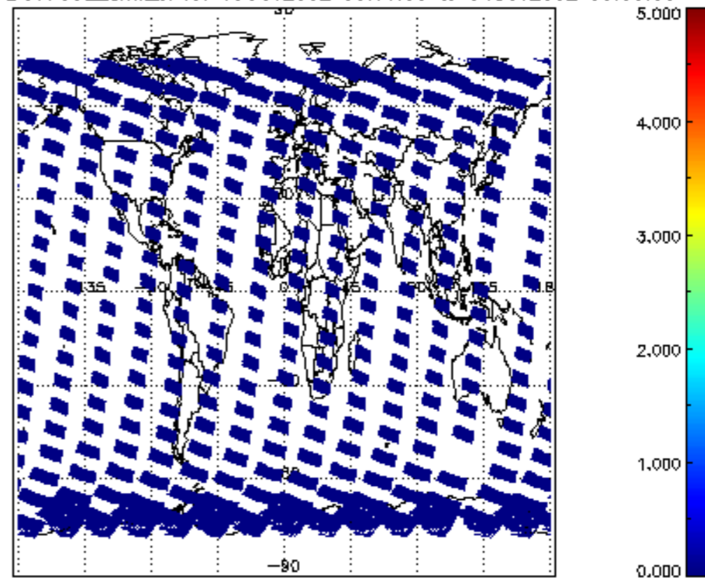
SCIOL2P_NADUV7S02_amf_cl for 03OCT2002 00:00:00 to 04OCT2002 00:00:00
