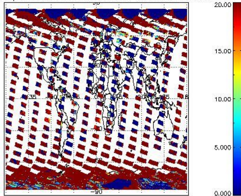
cL_opt_depth for 03OCT2002 00:00:00 to 04OCT2002 00:00:00
