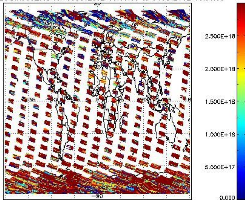
SCIO2P_NADIR3CO_vcd for 03OCT2002 00:00:00 to 04OCT2002 00:00:00
