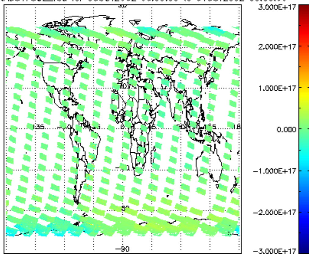
SCIOL2P_NADUV7S02_vcd for 03OCT2002 00:00:00 to 04OCT2002 00:00:00
