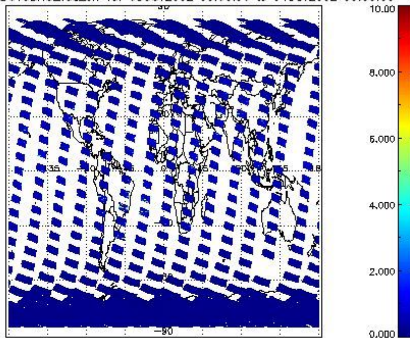
SCIOL2P_NADUV3BRO_vcd_err for 03OCT2002 00:00:00 to 04OCT2002 00:00:00
