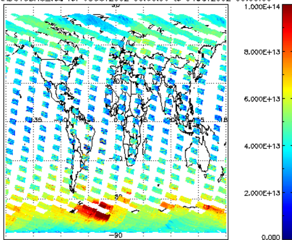
SCIOL2P_NADUV3BRO_vcd for 03OCT2002 00:00:00 to 04OCT2002 00:00:00
