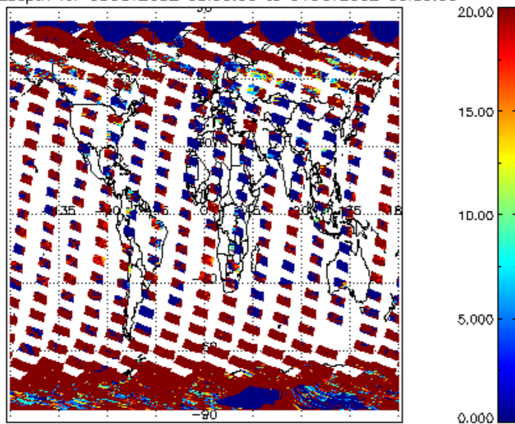
cl_opt_depth for 03OCT2002 00:00:00 to 04OCT2002 00:00:00
