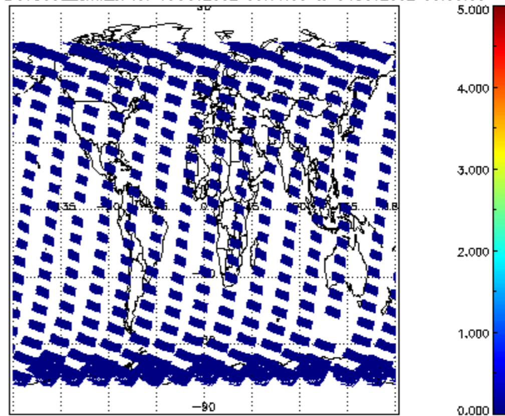
SCIOL2P_NADUV5S02_amf_cl for 03OCT2002 00:00:00 to 04OCT2002 00:00:00
