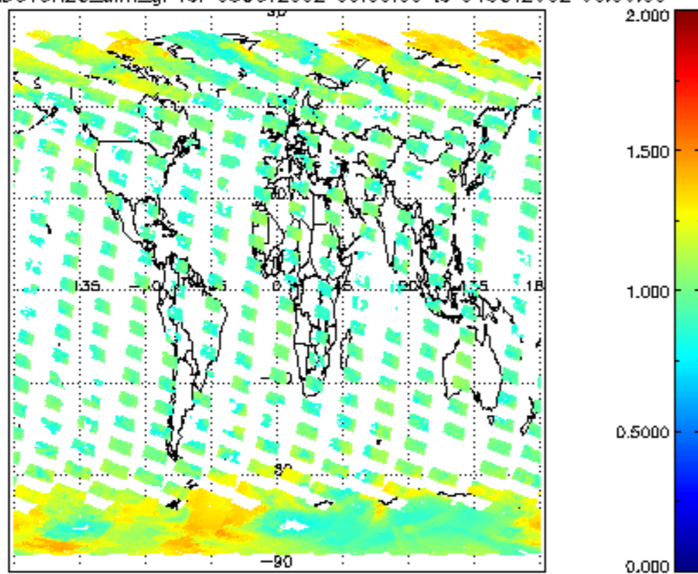
SCIOL2P_NADUV8H20_amf_gr for 03OCT2002 00:00:00 to 04OCT2002 00:00:00
