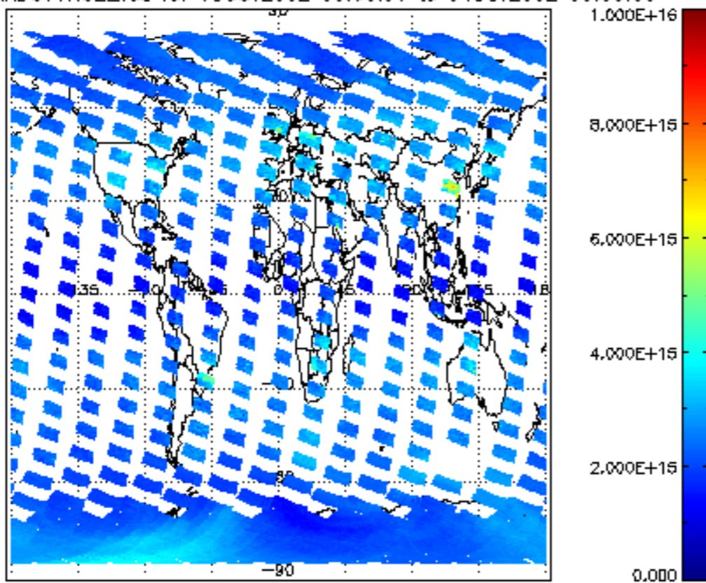
SCIOL2P_NADUV1NO2_vcd for 03OCT2002 00:00:00 to 04OCT2002 00:00:00
