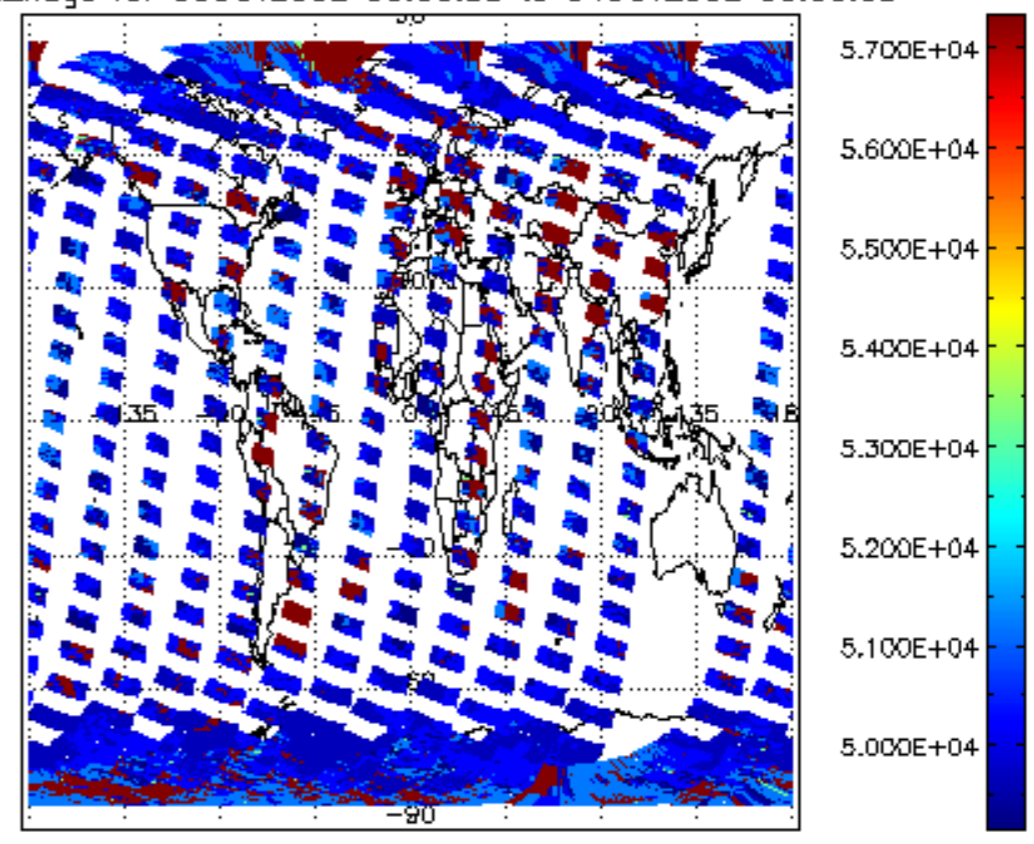
cloud_flags for 03OCT2002 00:00:00 to 04OCT2002 00:00:00
