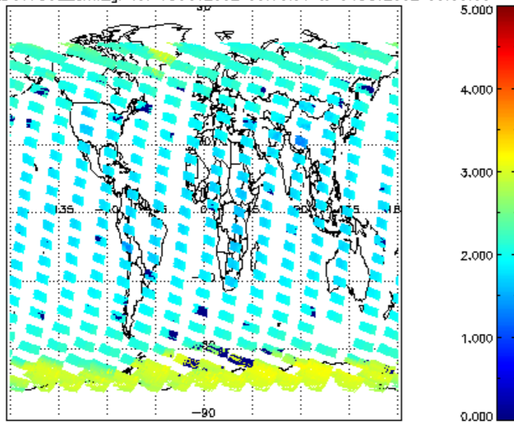
SCIOL2P_NADUV7S02_amf_gr for 03OCT2002 00:00:00 to 04OCT2002 00:00:00
