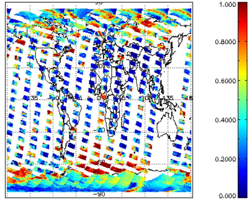
cl_frac for 03OCT2002 00:00:00 to 04OCT2002 00:00:00
