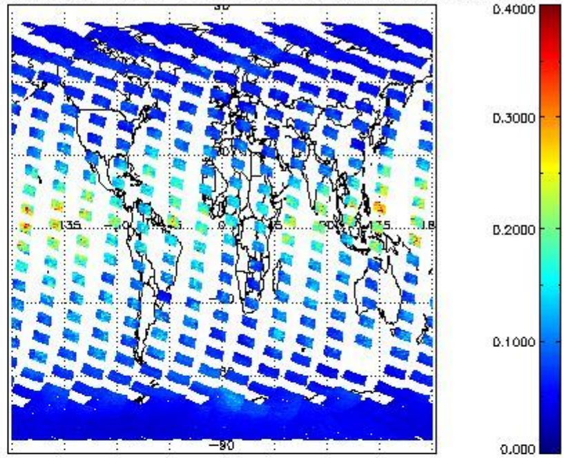
SCIOL2P_NADUV1N02_vcd_err for 03OCT2002 00:00:00 to 04OCT2002 00:00:00
