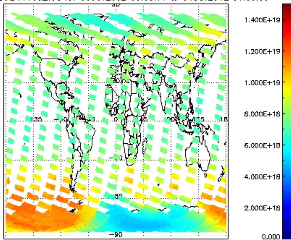
SCIOL2P_NADUV003_vcd for 03OCT2002 00:00:00 to 04OCT2002 00:00:00
