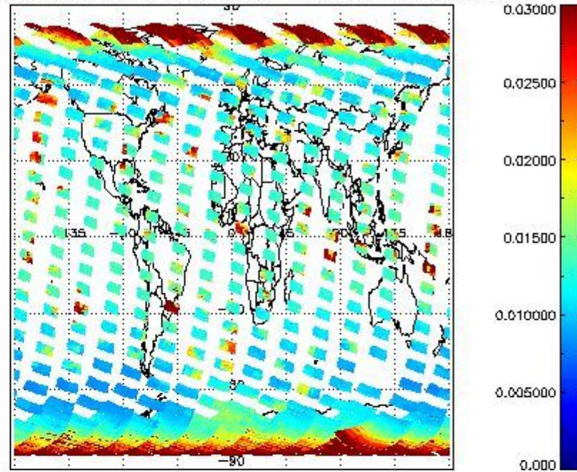
SCIOL2P_NADUV003_vcd_err for 03OCT2002 00:00:00 to 04OCT2002 00:00:00
