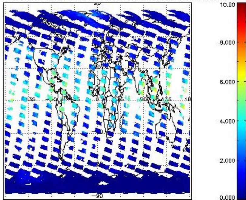
SCIOL2P_NADUV8H20_vcd for 03OCT2002 00:00:00 to 04OCT2002 00:00:00
