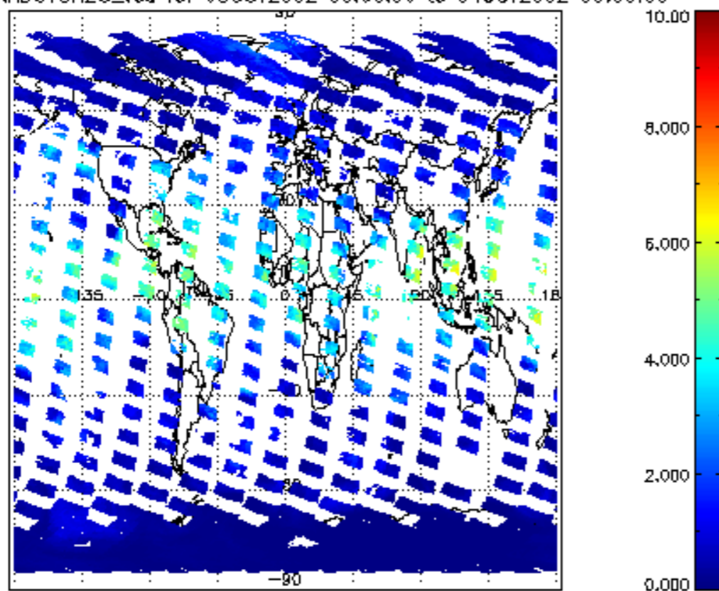
SCIOL2P_NADUV8H20_vcd for 03OCT2002 00:00:00 to 04OCT2002 00:00:00
