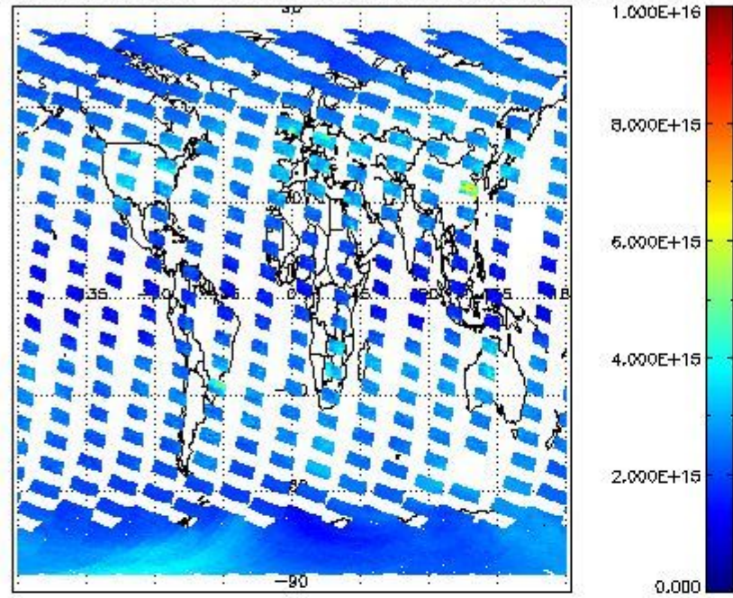
SCIOL2P_NADUV1N02_vcd for 03OCT2002 00:00:00 to 04OCT2002 00:00:00
