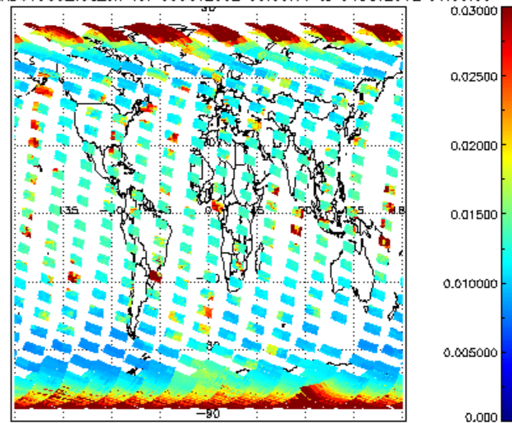
SCIOL2P_NADUV003_vcd_err for 03OCT2002 00:00:00 to 04OCT2002 00:00:00
