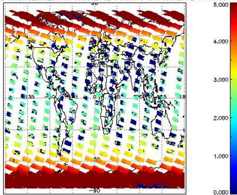
SCIOL2P_NADUV3BRO_amf_cl for 03OCT2002 00:00:00 to 04OCT2002 00:00:00
