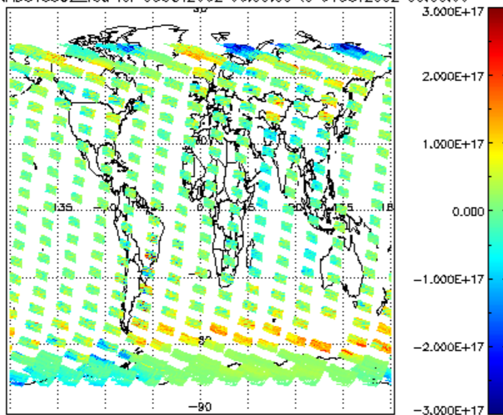
SCIOL2P_NADUV5S02_vcd for 03OCT2002 00:00:00 to 04OCT2002 00:00:00
