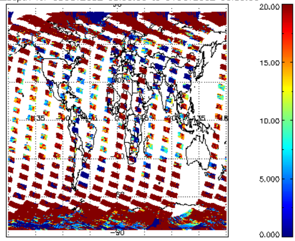
cl_opt_depth for 03OCT2002 00:00:00 to 04OCT2002 00:00:00
