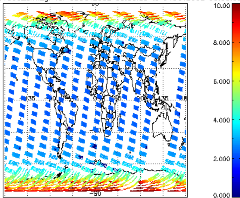
SCIOL2P_NADUV003_amf_gr for 03OCT2002 00:00:00 to 04OCT2002 00:00:00
