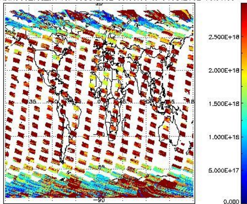
SCIO2P_NADIR3CO_vcd_err for 03OCT2002 00:00:00 to 04OCT2002 00:00:00
