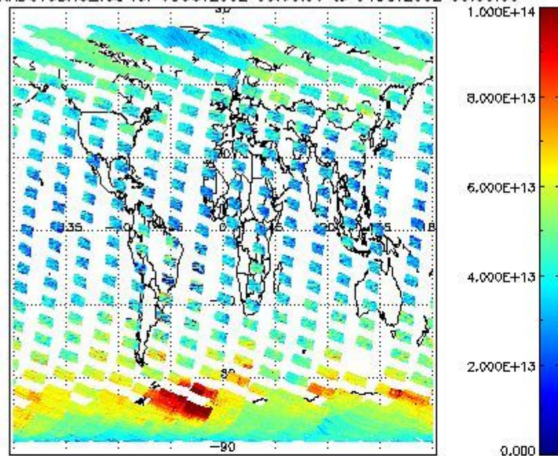
SCIOL2P_NADUV3BRO_vcd for 03OCT2002 00:00:00 to 04OCT2002 00:00:00
