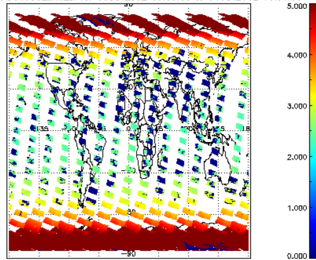
SCIOL2P_NADUV003_amf_cl for 03OCT2002 00:00:00 to 04OCT2002 00:00:00
