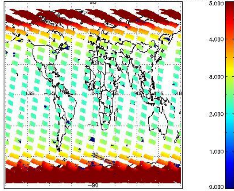
SCIOL2P_NADUV1N02_amf_gr for 03OCT2002 00:00:00 to 04OCT2002 00:00:00
