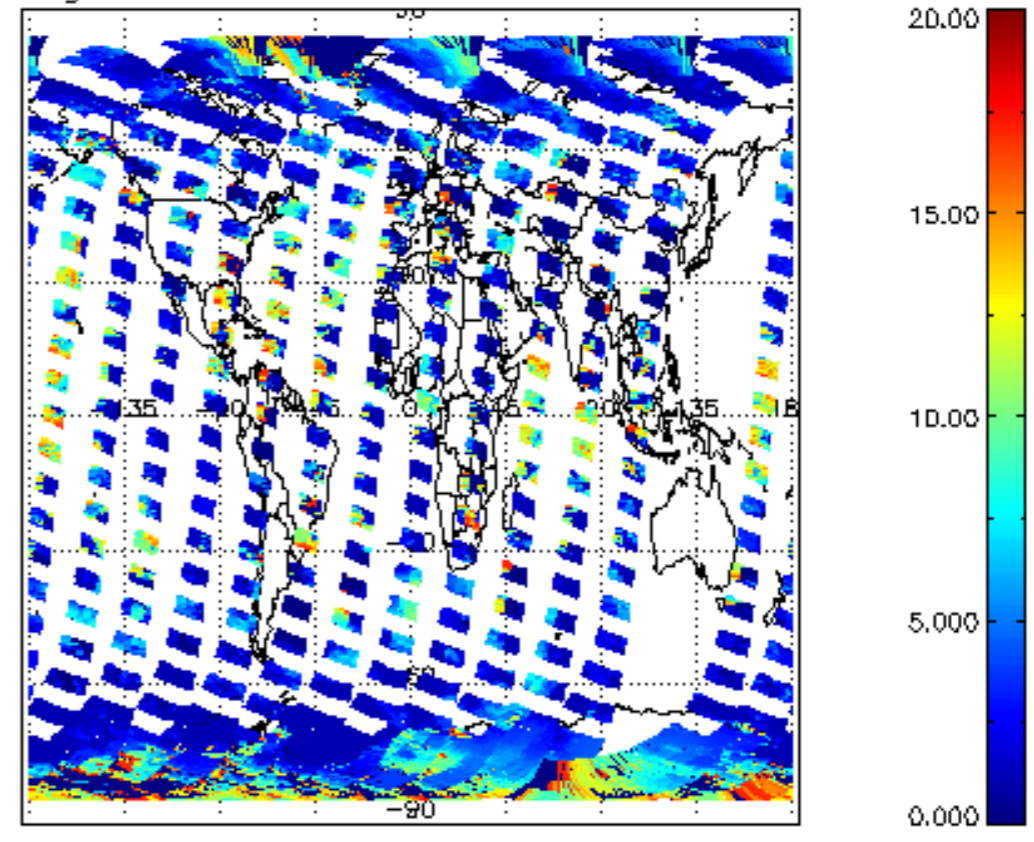
cl_top_height for 03OCT2002 00:00:00 to 04OCT2002 00:00:00
