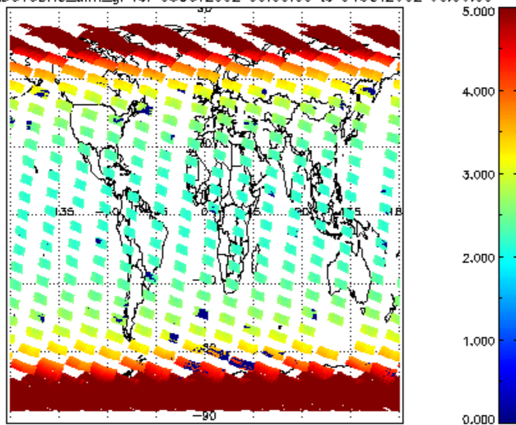
SCIOL2P_NADUV3BRO_amf_gr for 03OCT2002 00:00:00 to 04OCT2002 00:00:00
