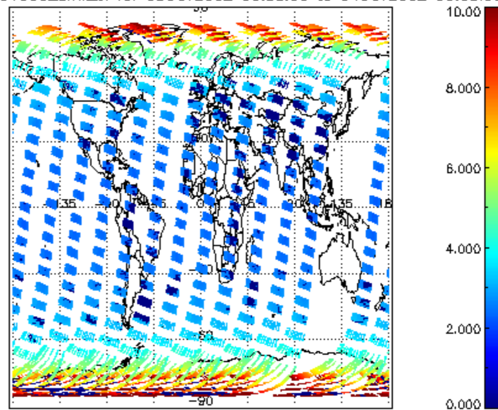
SCIOL2P_NADUV003_amf_sl for 03OCT2002 00:00:00 to 04OCT2002 00:00:00
