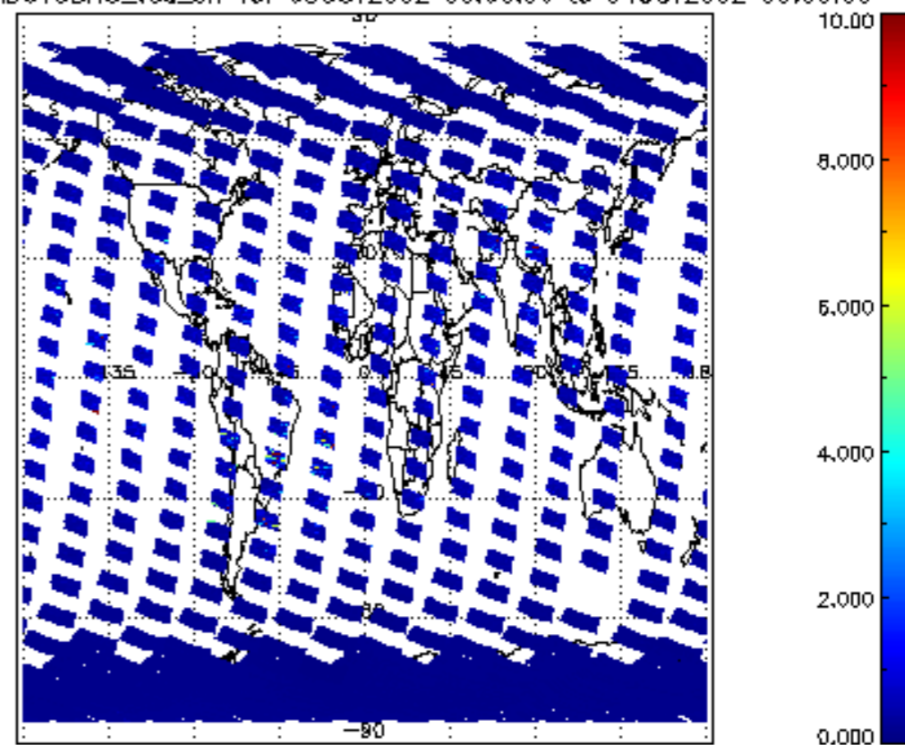
SCIOL2P_NADUV3BRO_vcd_err for 03OCT2002 00:00:00 to 04OCT2002 00:00:00
