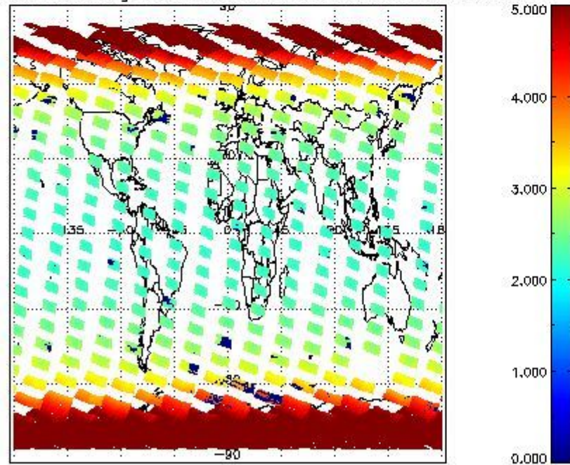
SCIOL2P_NADUV003_amf_gr for 03OCT2002 00:00:00 to 04OCT2002 00:00:00
