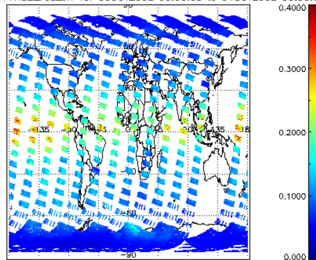
ICIOL2P_NADUV1NO2_vcd_err for 03OCT2002 00:00:00 to 04OCT2002 00:00:00
