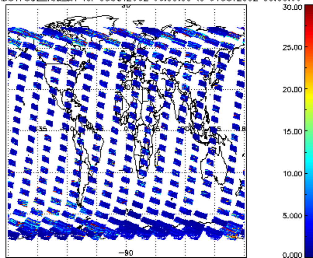
SCIOL2P_NADUV7S02_vcd_err for 03OCT2002 00:00:00 to 04OCT2002 00:00:00
