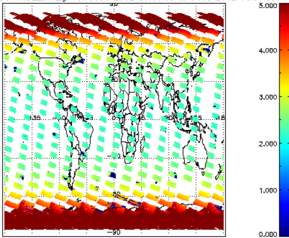
SCIOL2P_NADUV1NO2_amf_gr for 03OCT2002 00:00:00 to 04OCT2002 00:00:00
