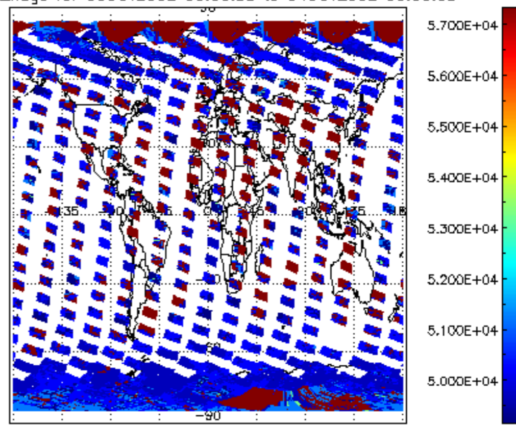
cloud_flags for 03OCT2002 00:00:00 to 04OCT2002 00:00:00
