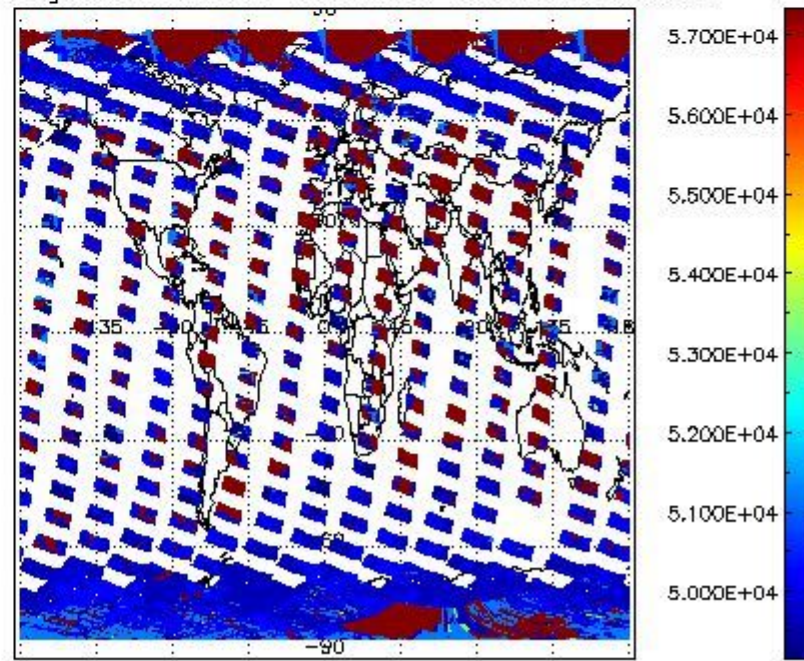
cloud_flags for 03OCT2002 00:00:00 to 04OCT2002 00:00:00
