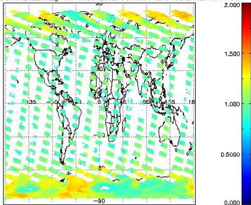
SCIOL2P_NADUV8H20_amf_gr for 03OCT2002 00:00:00 to 04OCT2002 00:00:00
