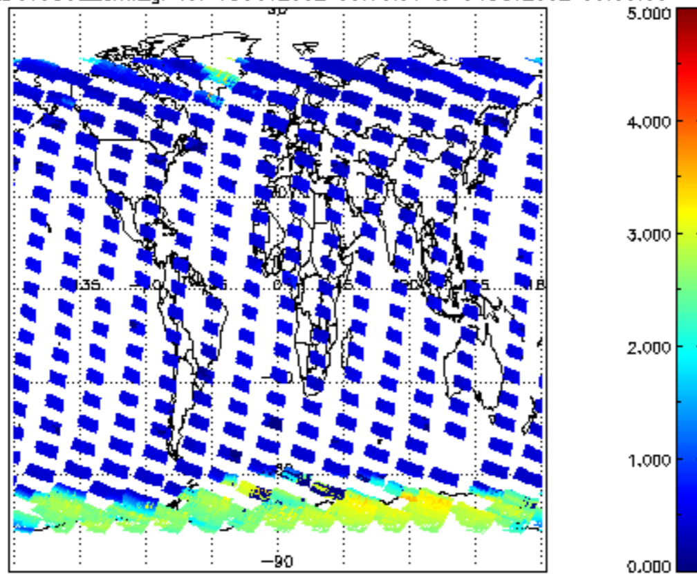
SCIOL2P_NADUV5S02_amf_gr for 03OCT2002 00:00:00 to 04OCT2002 00:00:00
