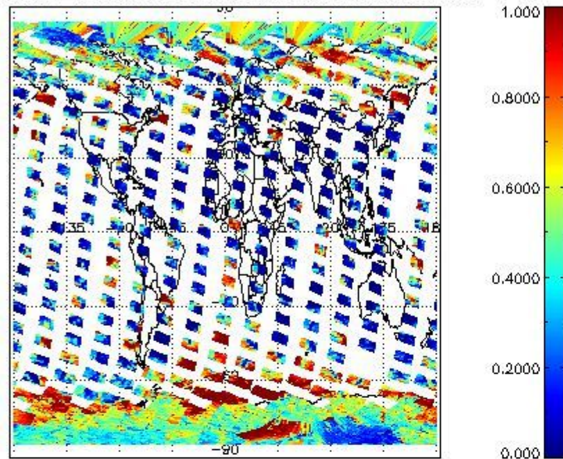
cLfrac for 03OCT2002 00:00:00 to 04OCT2002 00:00:00
