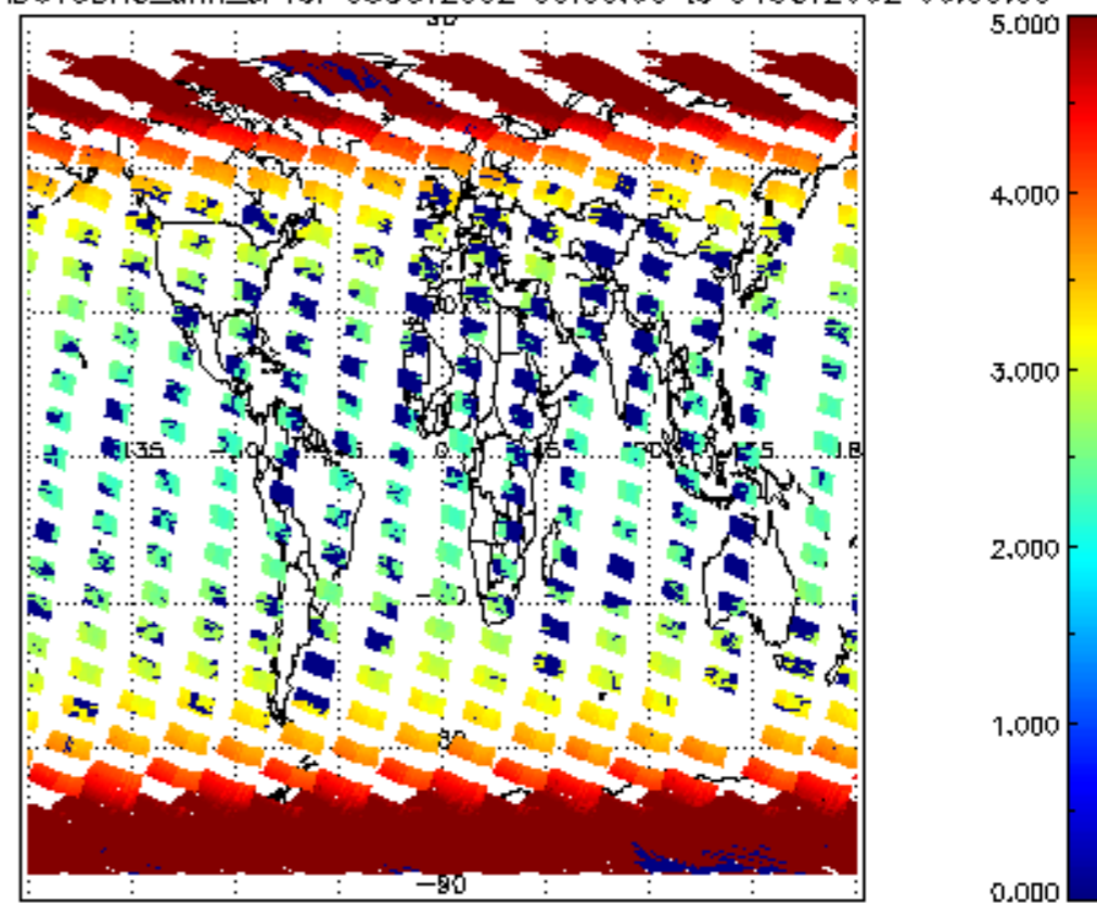
SCIOL2P_NADUV3BRO_amf_cl for 03OCT2002 00:00:00 to 04OCT2002 00:00:00
