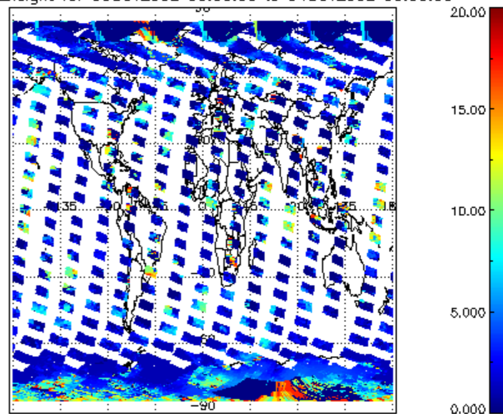
cl_top_height for 03OCT2002 00:00:00 to 04OCT2002 00:00:00
