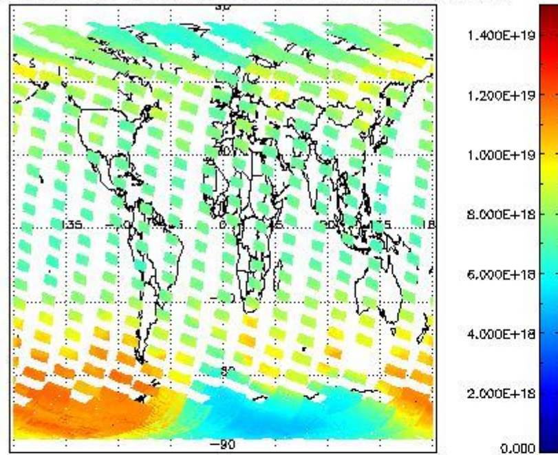
SCIOL2P_NADUV003_vcd for 03OCT2002 00:00:00 to 04OCT2002 00:00:00
