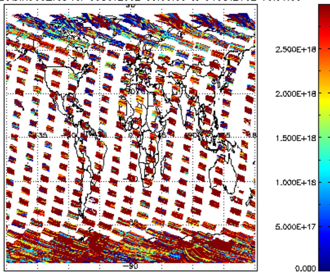
SCIOL2P_NADIR3CO_vcd for 03OCT2002 00:00:00 to 04OCT2002 00:00:00
