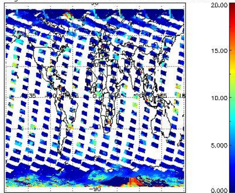
cL_top_height for 03OCT2002 00:00:00 to 04OCT2002 00:00:00
