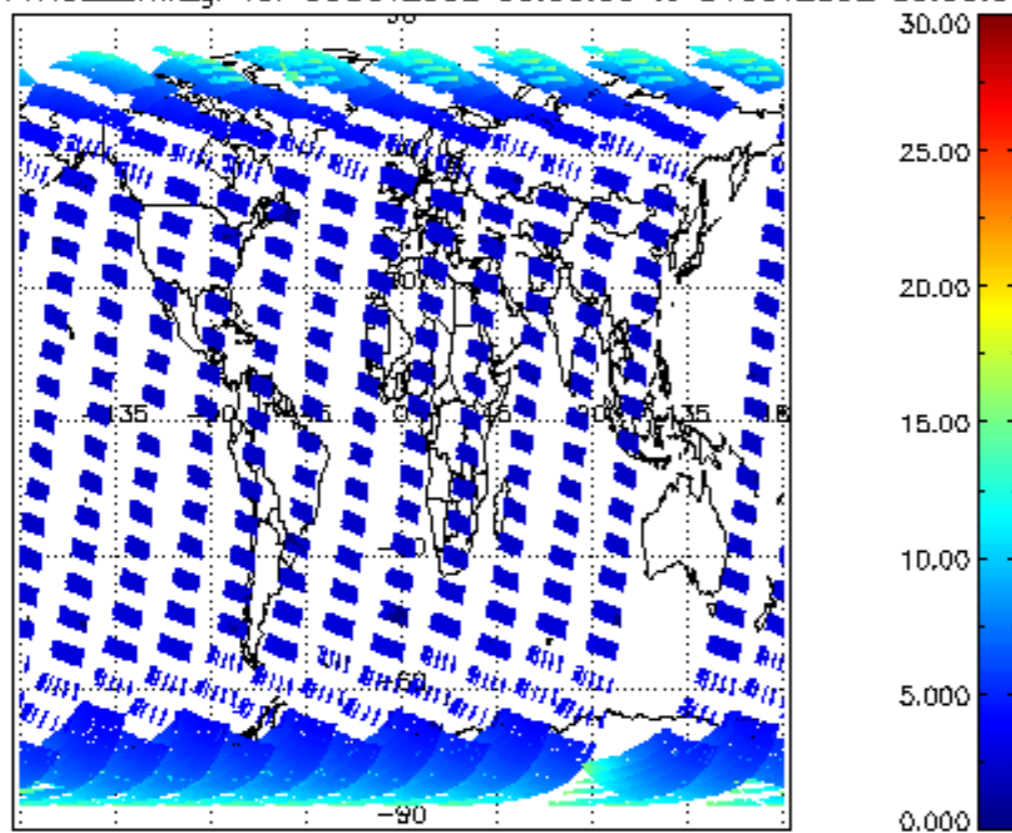
ICIOL2P_NADUV1NO2_amf_gr for 03OCT2002 00:00:00 to 04OCT2002 00:00:00
