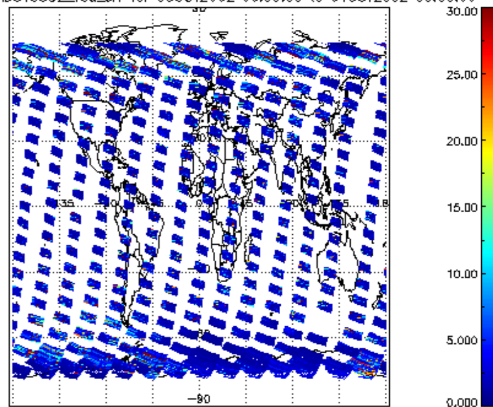
SCIOL2P_NADUV5S02_vcd_err for 03OCT2002 00:00:00 to 04OCT2002 00:00:00
