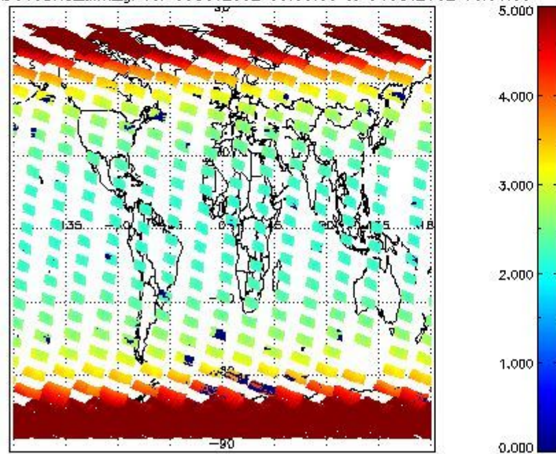
SCIOL2P_NADUV3BRO_amf_gr for 03OCT2002 00:00:00 to 04OCT2002 00:00:00
