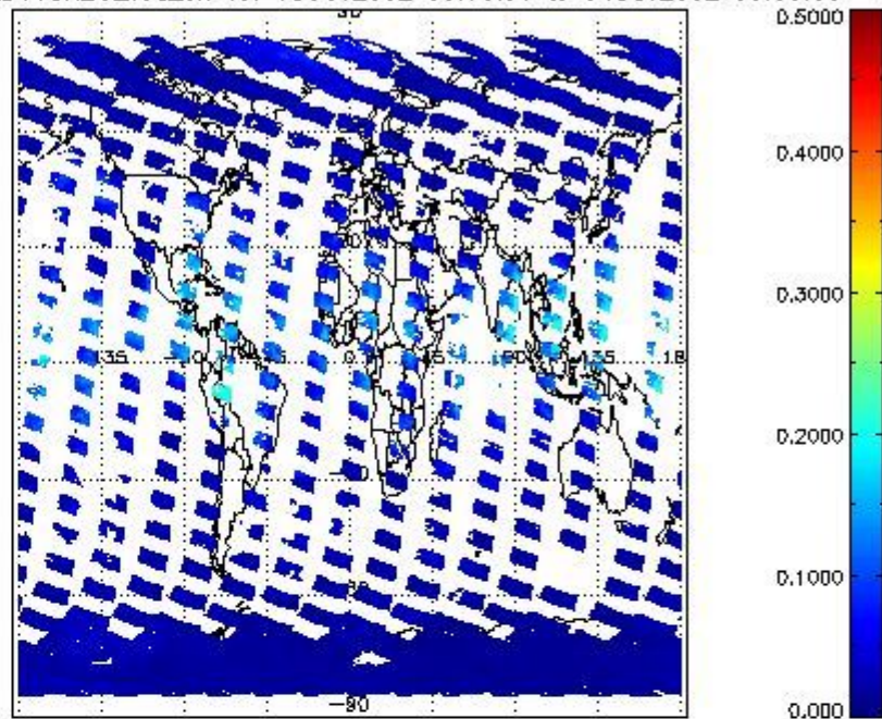
SCIOL2P_NADUV8H20_vcd_err for 03OCT2002 00:00:00 to 04OCT2002 00:00:00
