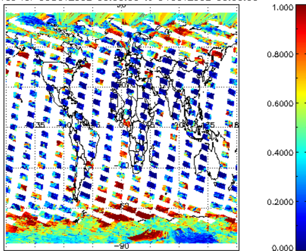
cl_frac for 03OCT2002 00:00:00 to 04OCT2002 00:00:00
