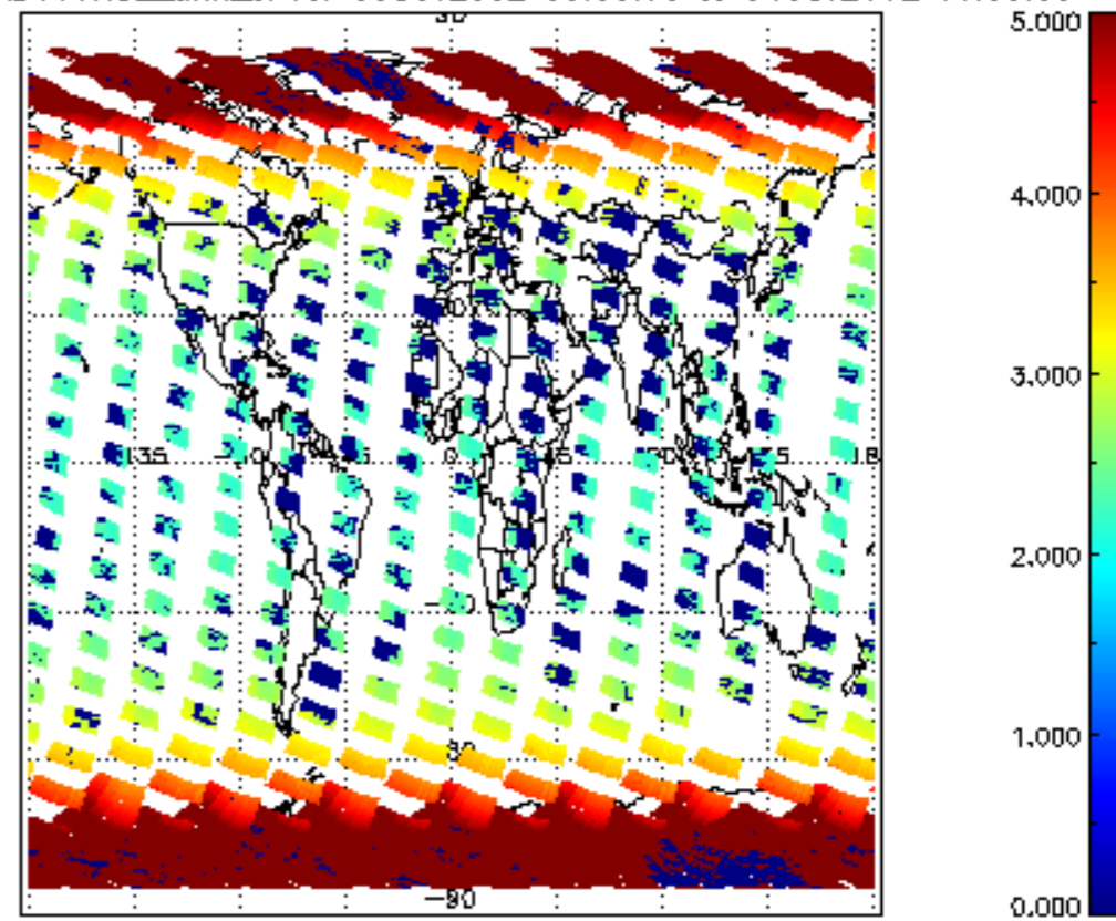
SCIOL2P_NADUV1NO2_amf_cl for 03OCT2002 00:00:00 to 04OCT2002 00:00:00
