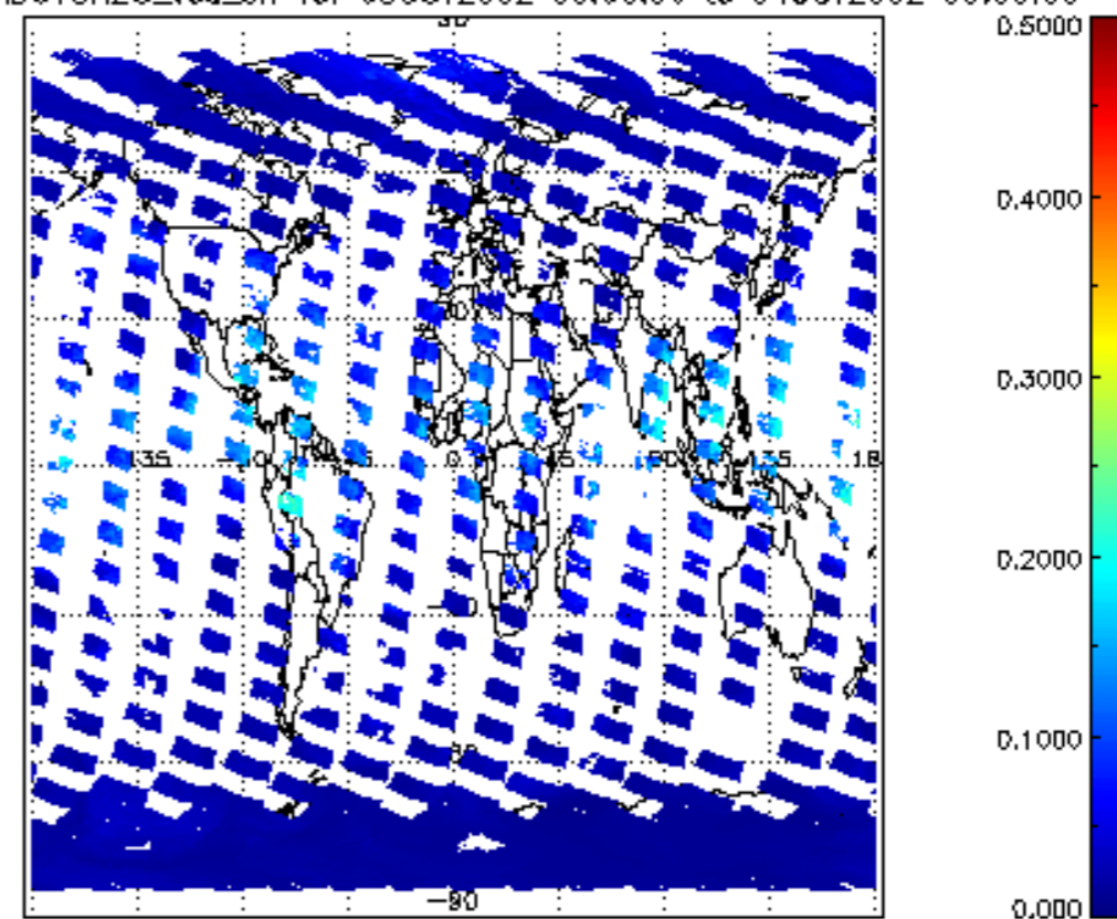
SCIOL2P_NADUV8H20_vcd_err for 03OCT2002 00:00:00 to 04OCT2002 00:00:00
