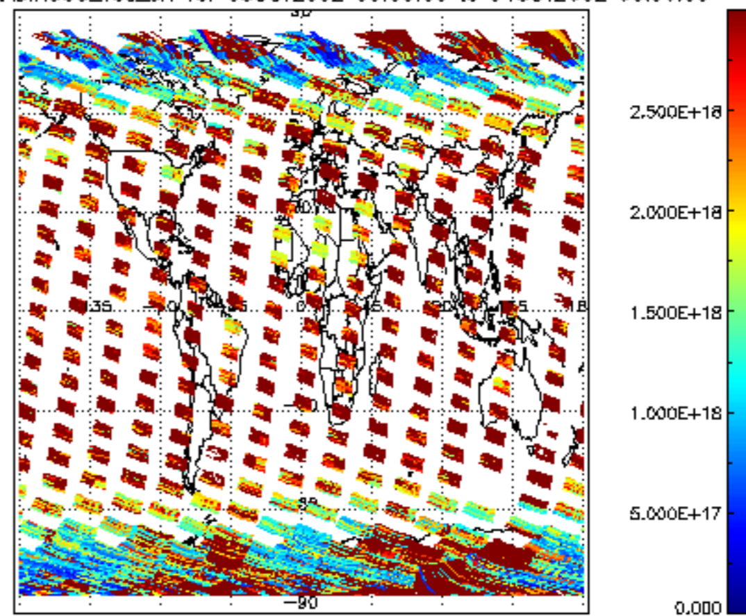
SCIOL2P_NADIR3CO_vcd_err for 03OCT2002 00:00:00 to 04OCT2002 00:00:00
