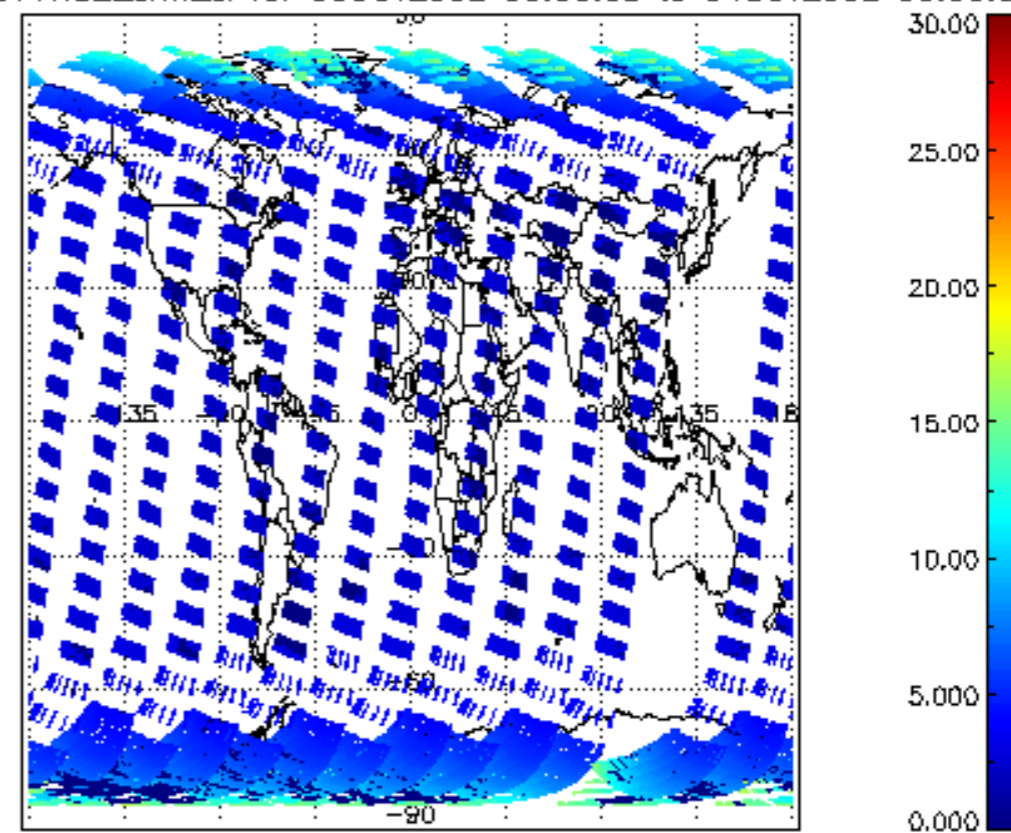
ICIOL2P_NADUV1NO2_amf_cl for 03OCT2002 00:00:00 to 04OCT2002 00:00:00
