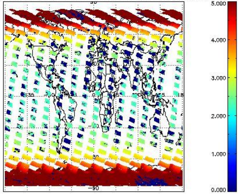
SCIOL2P_NADUV1N02_amf_cl for 03OCT2002 00:00:00 to 04OCT2002 00:00:00
