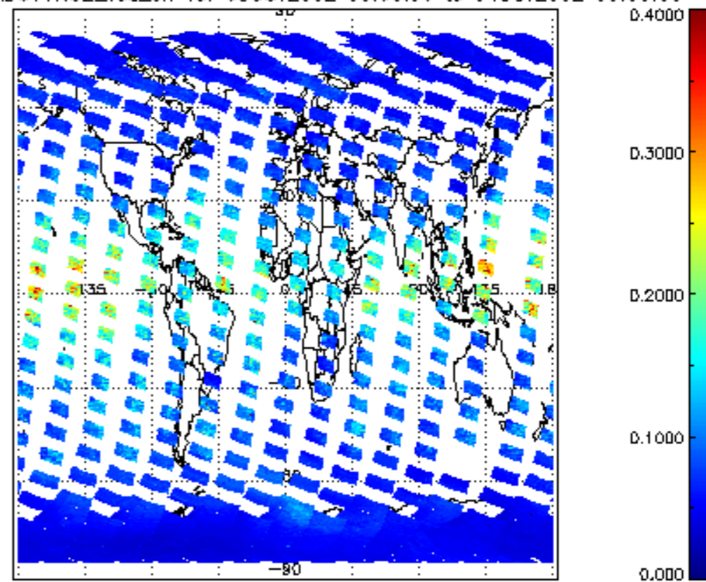
SCIOL2P_NADUV1NO2_vcd_err for 03OCT2002 00:00:00 to 04OCT2002 00:00:00
