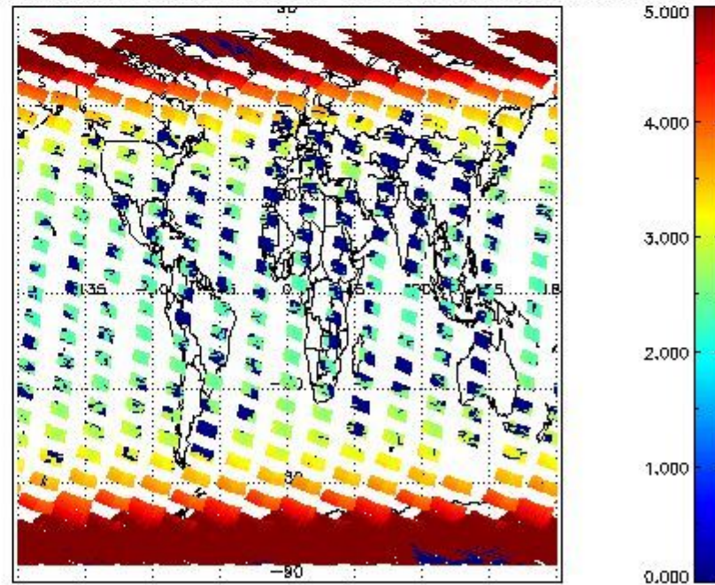
SCIOL2P_NADUV003_amf_cl for 03OCT2002 00:00:00 to 04OCT2002 00:00:00
