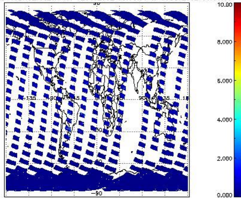
SCIOL2P_NADUV3BRO_vcd_err for 02OCT2002 00:00:00 to 03OCT2002 00:00:00
