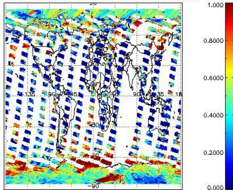
cLfrac for 02OCT2002 00:00:00 to 03OCT2002 00:00:00
