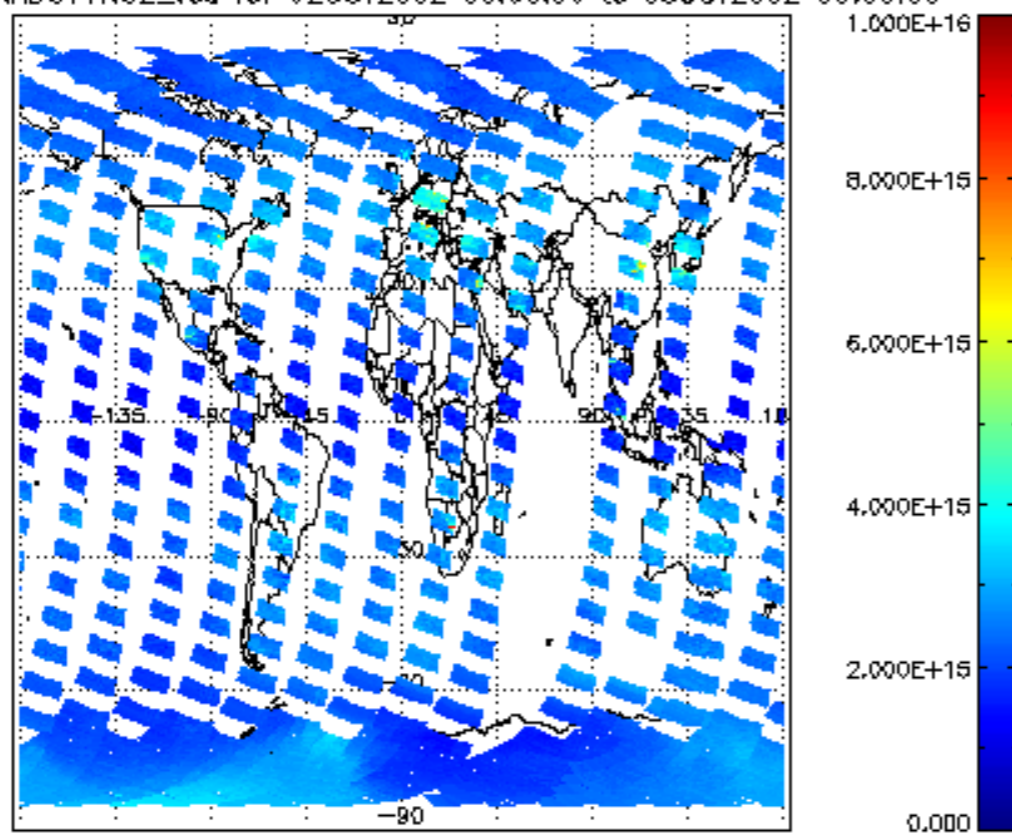
SCIOL2P_NADUV1N02_vcd for 02OCT2002 00:00:00 to 03OCT2002 00:00:00
