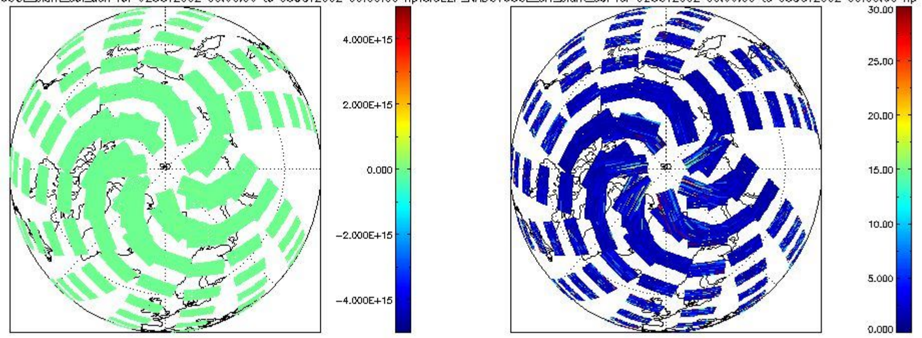
CIOL2P_NADUV60CL_slant_col_den for 02OCT2002 00:00:00 to 03OCT2002 00:00:00 np CIOL2P_NADUV60CL_err_slant_col for 02OCT2002 00:00:00 to 03OCT2002 00:00:00 np
