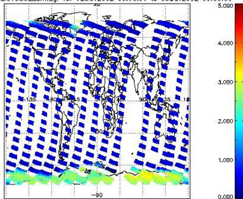
SCIOL2P_NADUV5S02_amf_gr for 02OCT2002 00:00:00 to 03OCT2002 00:00:00
