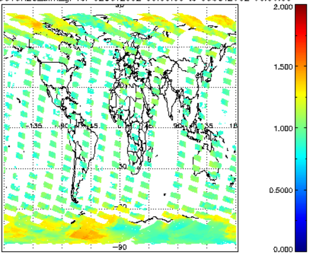
SCIOL2P_NADUV8H20_amf_gr for 02OCT2002 00:00:00 to 03OCT2002 00:00:00
