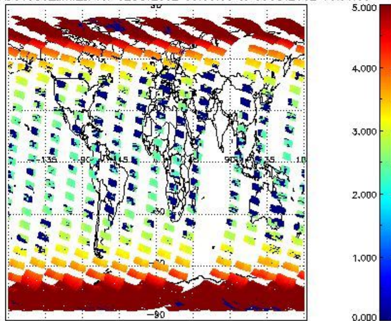
SCIOL2P_NADUV003_amf_cl for 02OCT2002 00:00:00 to 03OCT2002 00:00:00
