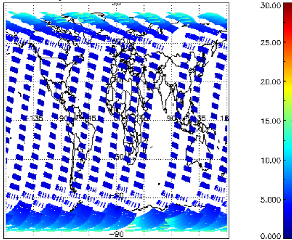
iCIOL2P_NADUV1NO2_amf_gr for 02OCT2002 00:00:00 to 03OCT2002 00:00:00
