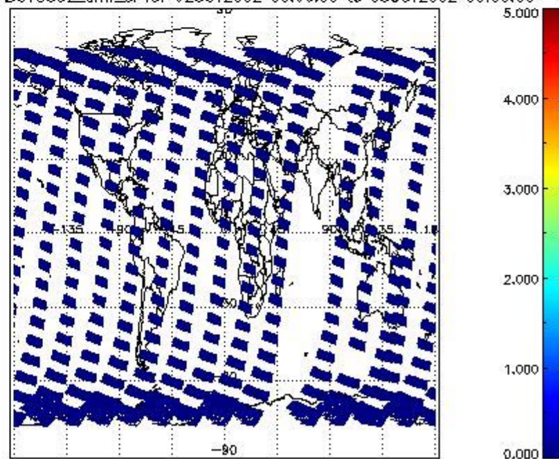
SCIOL2P_NADUV5S02_amf_cl for 02OCT2002 00:00:00 to 03OCT2002 00:00:00
