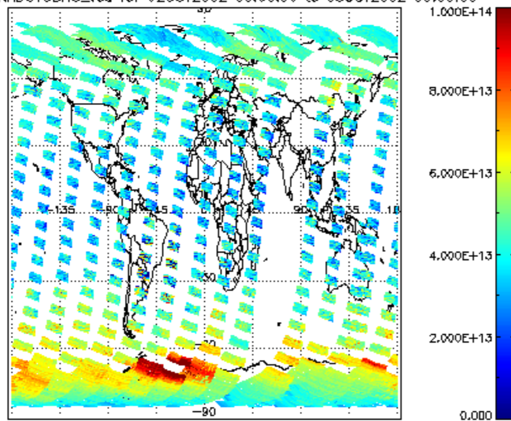
SCIOL2P_NADUV3BRO_vcd for 02OCT2002 00:00:00 to 03OCT2002 00:00:00
