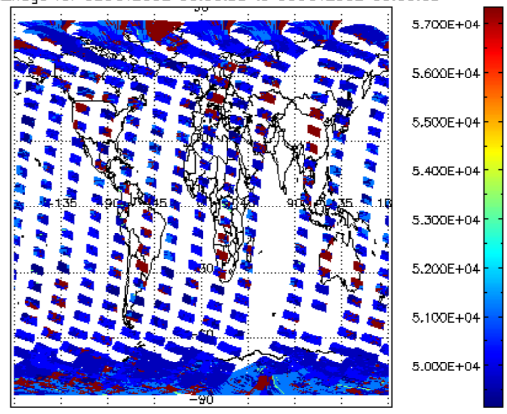
cloud_flags for 02OCT2002 00:00:00 to 03OCT2002 00:00:00
