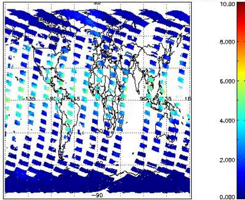
SCIOL2P_NADUV8H20_vcd for 02OCT2002 00:00:00 to 03OCT2002 00:00:00
