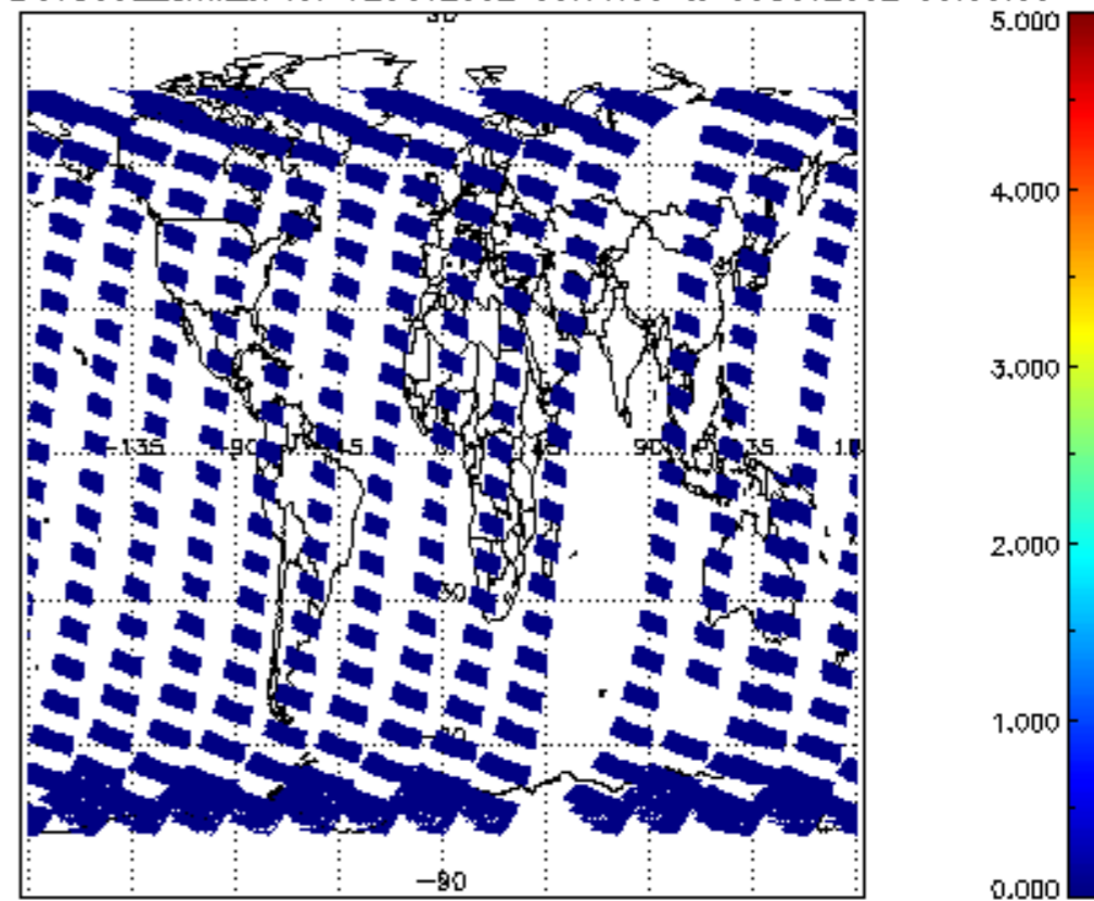
SCIOL2P_NADUV5S02_amf_sl for 02OCT2002 00:00:00 to 03OCT2002 00:00:00
