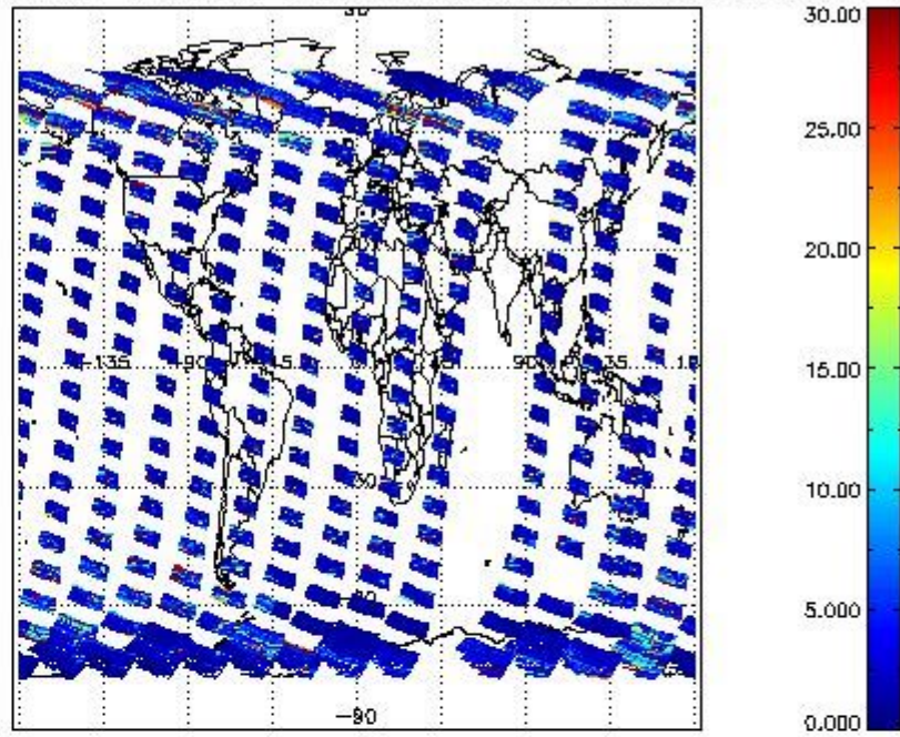
SCIOL2P_NADUV7S02_vcd_err for 02OCT2002 00:00:00 to 03OCT2002 00:00:00
