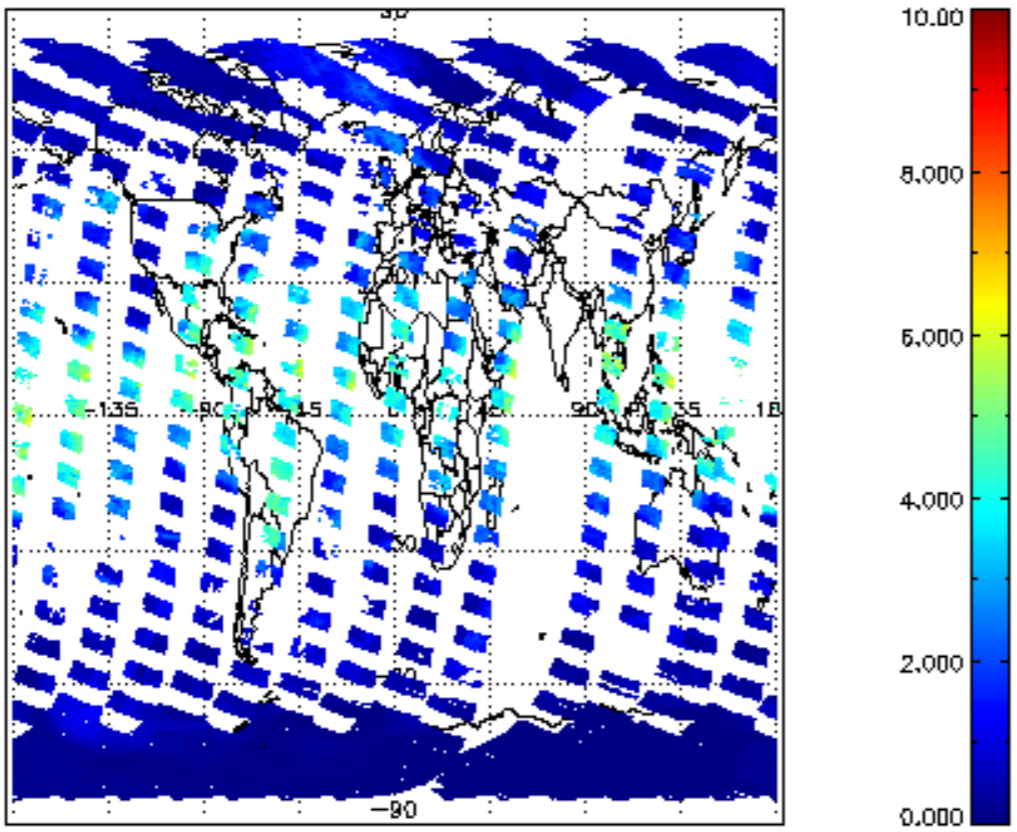
SCIOL2P_NADUV8H20_vcd for 02OCT2002 00:00:00 to 03OCT2002 00:00:00
