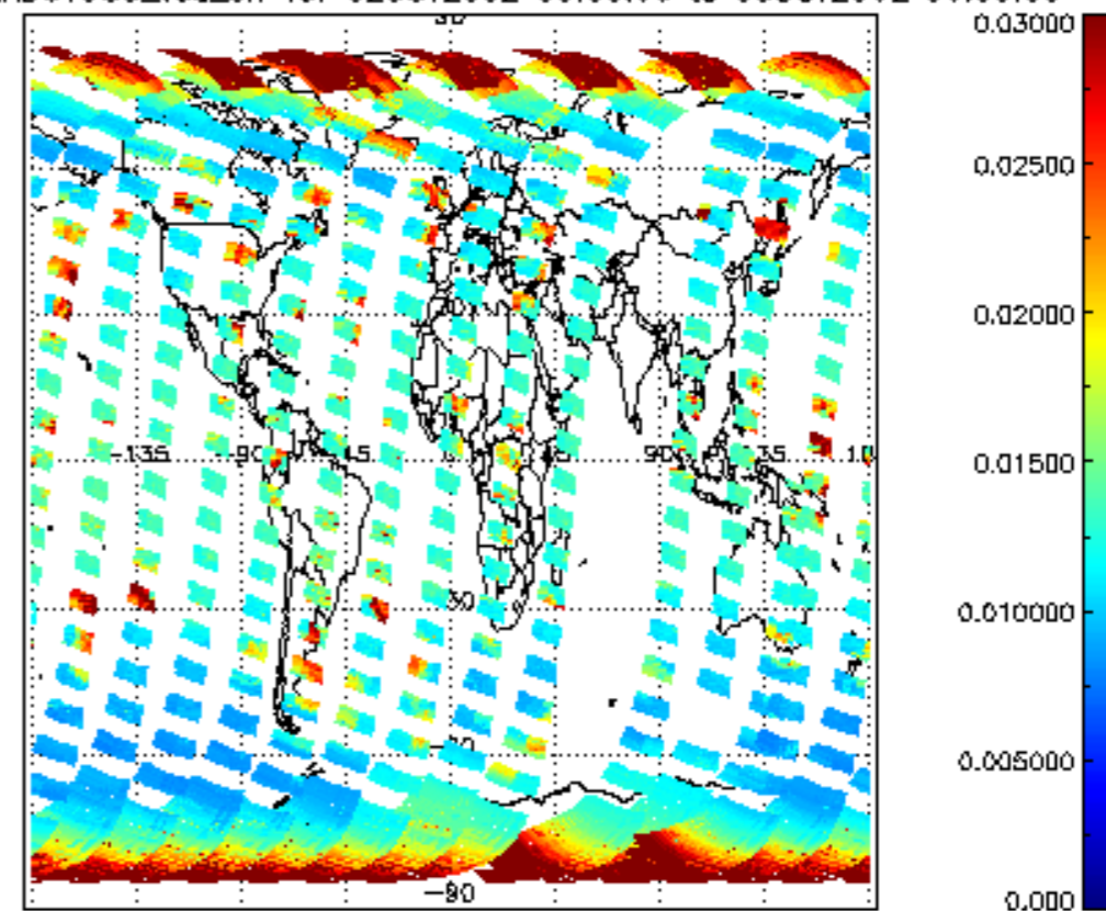
SCIOL2P_NADUV003_vcd_err for 02OCT2002 00:00:00 to 03OCT2002 00:00:00
