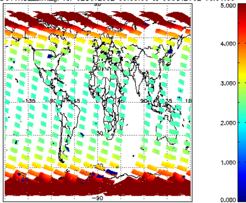
SCIOL2P_NADUV1N02_amf_gr for 02OCT2002 00:00:00 to 03OCT2002 00:00:00
