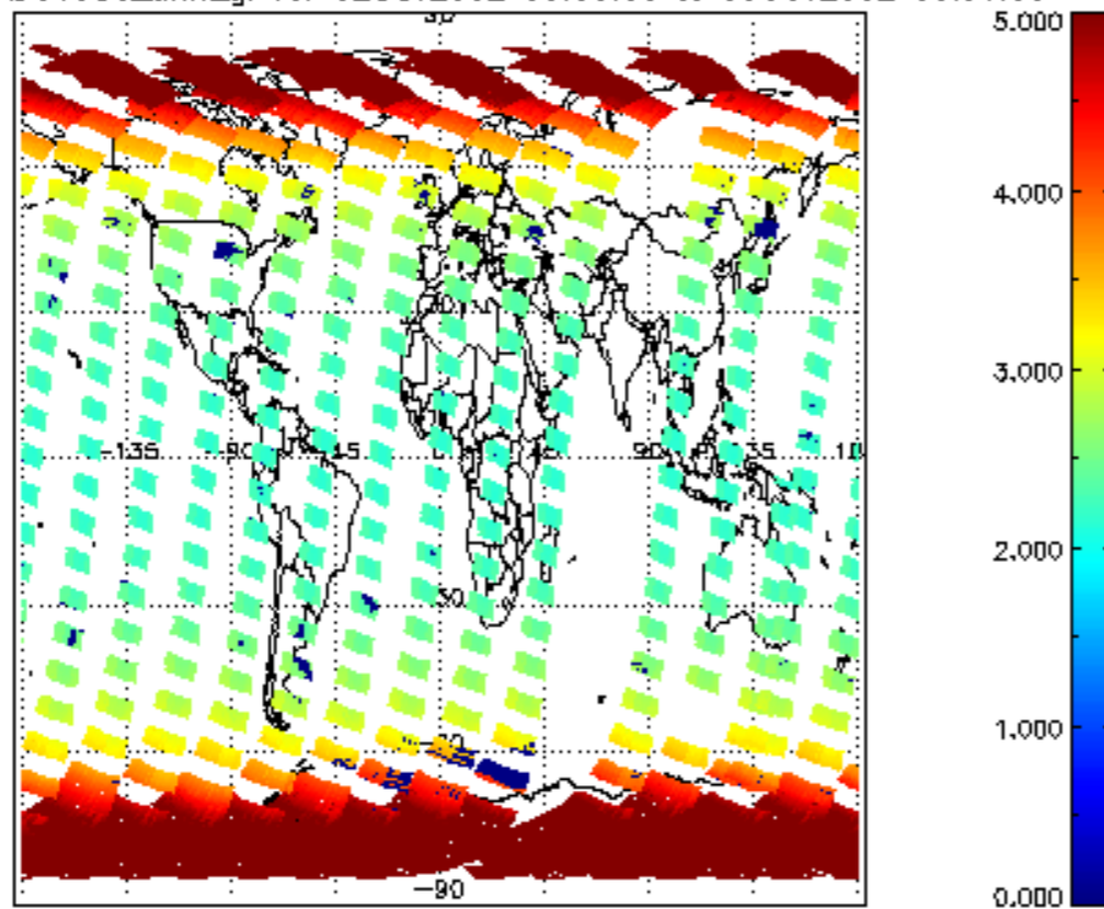
SCIOL2P_NADUV003_amf_gr for 02OCT2002 00:00:00 to 03OCT2002 00:00:00
