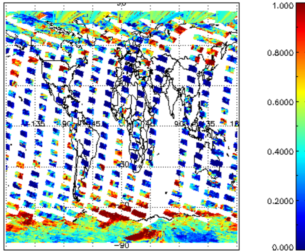
cl_frac for 02OCT2002 00:00:00 to 03OCT2002 00:00:00
