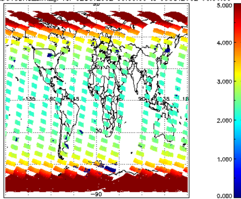
SCIOL2P_NADUV3BRO_amf_gr for 02OCT2002 00:00:00 to 03OCT2002 00:00:00
