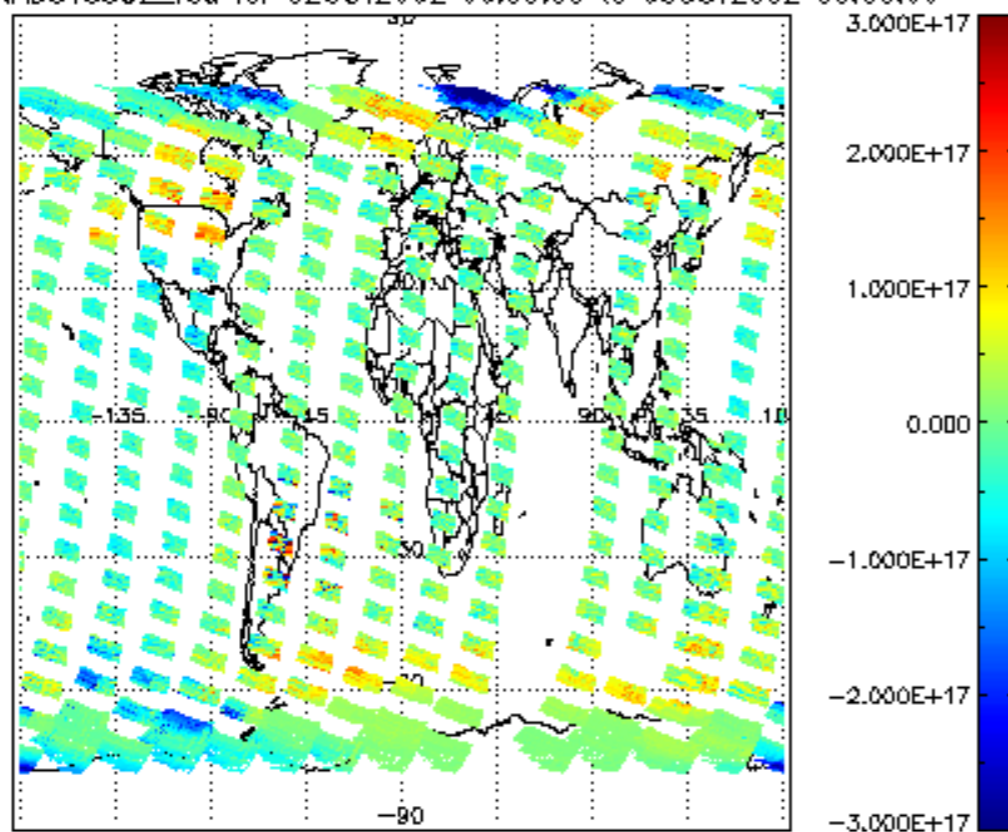
SCIOL2P_NADUV5S02_vcd for 02OCT2002 00:00:00 to 03OCT2002 00:00:00
