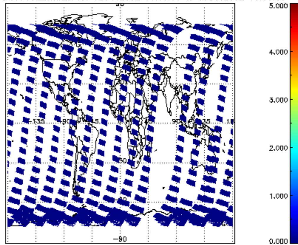
SCIOL2P_NADUV7S02_amf_sl for 02OCT2002 00:00:00 to 03OCT2002 00:00:00
