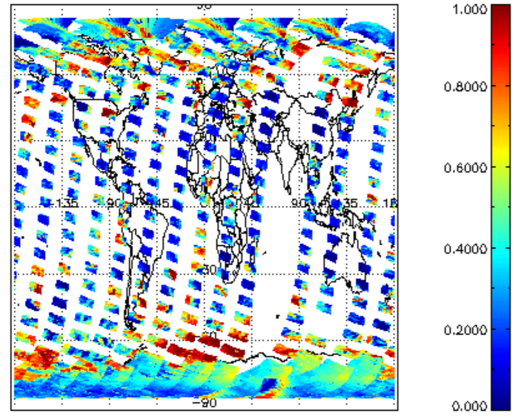
cl_frac for 02OCT2002 00:00:00 to 03OCT2002 00:00:00
