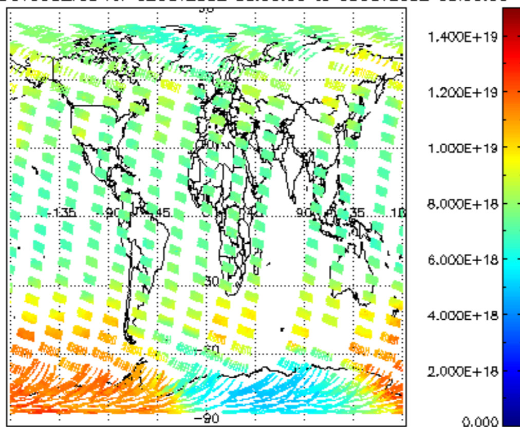
SCIOL2P_NADUV003_vcd for 02OCT2002 00:00:00 to 03OCT2002 00:00:00
