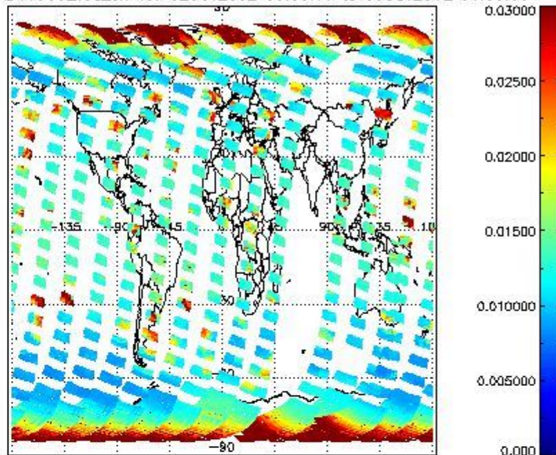
SCIOL2P_NADUV003_vcd_err for 02OCT2002 00:00:00 to 03OCT2002 00:00:00
