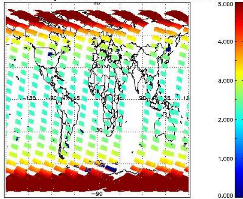
SCIOL2P_NADUV3BRO_amf_gr for 02OCT2002 00:00:00 to 03OCT2002 00:00:00
