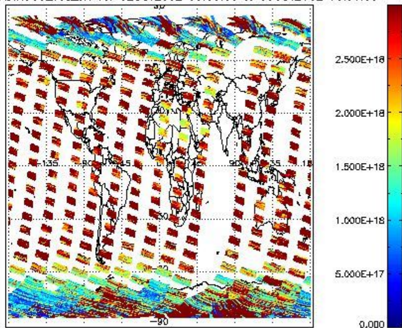
SCIDL2P_NADIR3CO_vcd_err for 02OCT2002 00:00:00 to 03OCT2002 00:00:00
