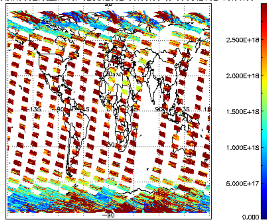
SCIOL2P_NADIR3CO_vcd_err for 02OCT2002 00:00:00 to 03OCT2002 00:00:00
