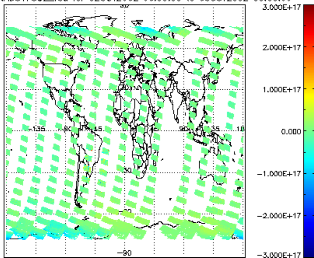
SCIOL2P_NADUV7S02_vcd for 02OCT2002 00:00:00 to 03OCT2002 00:00:00
