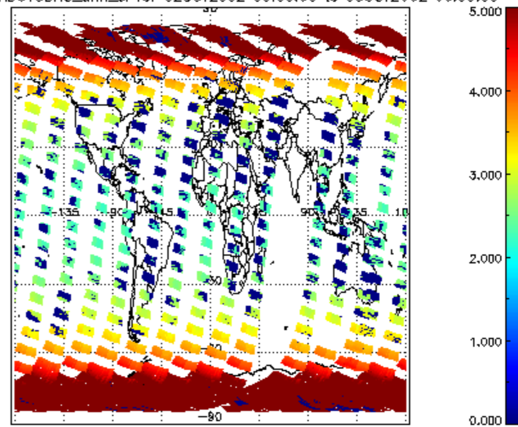
SCIOL2P_NADUV3BRO_amf_cl for 02OCT2002 00:00:00 to 03OCT2002 00:00:00
