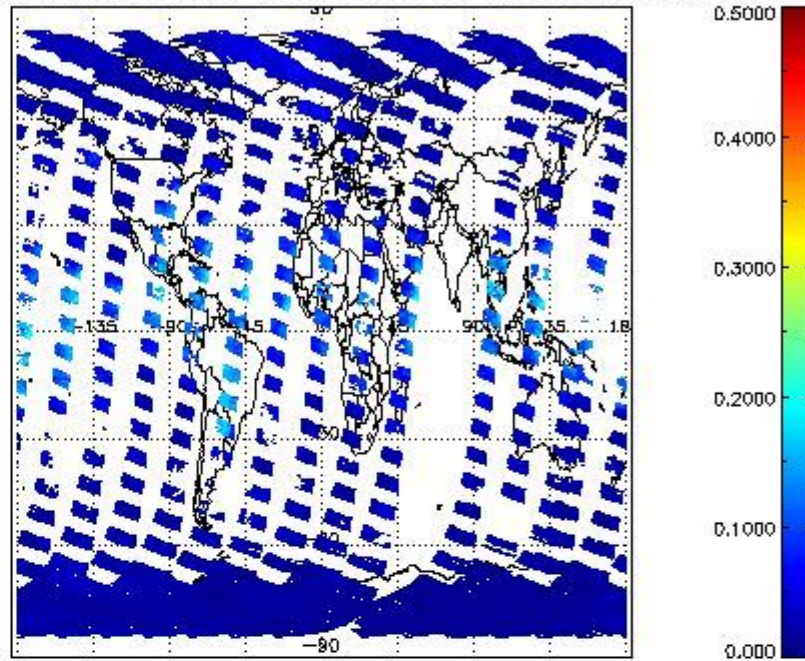
SCIOL2P_NADUV8H20_vcd_err for 02OCT2002 00:00:00 to 03OCT2002 00:00:00
