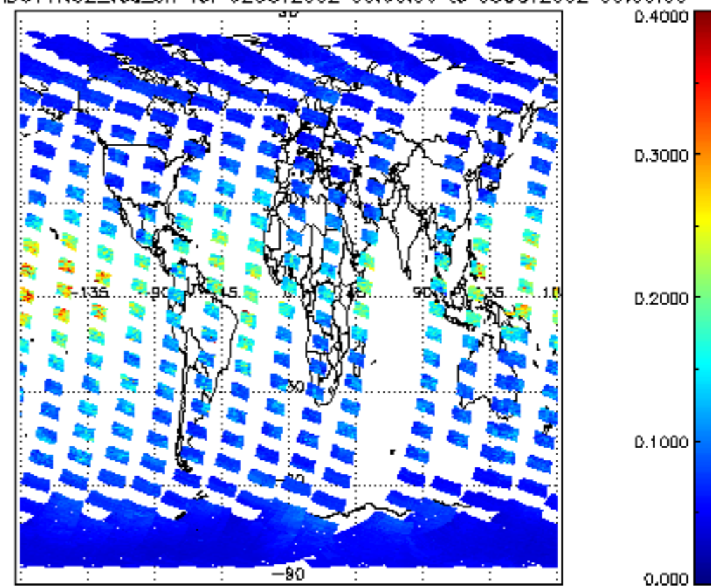
SCIOL2P_NADUV1N02_vcd_err for 02OCT2002 00:00:00 to 03OCT2002 00:00:00
