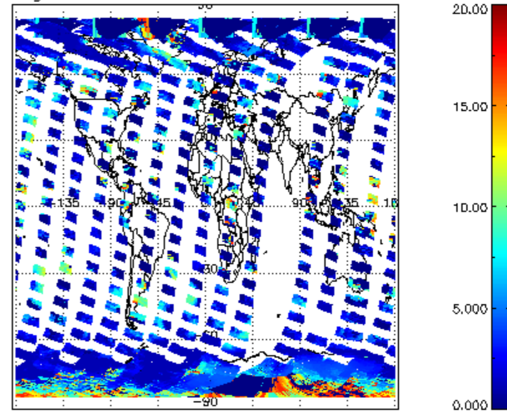
cl_top_height for 02OCT2002 00:00:00 to 03OCT2002 00:00:00
