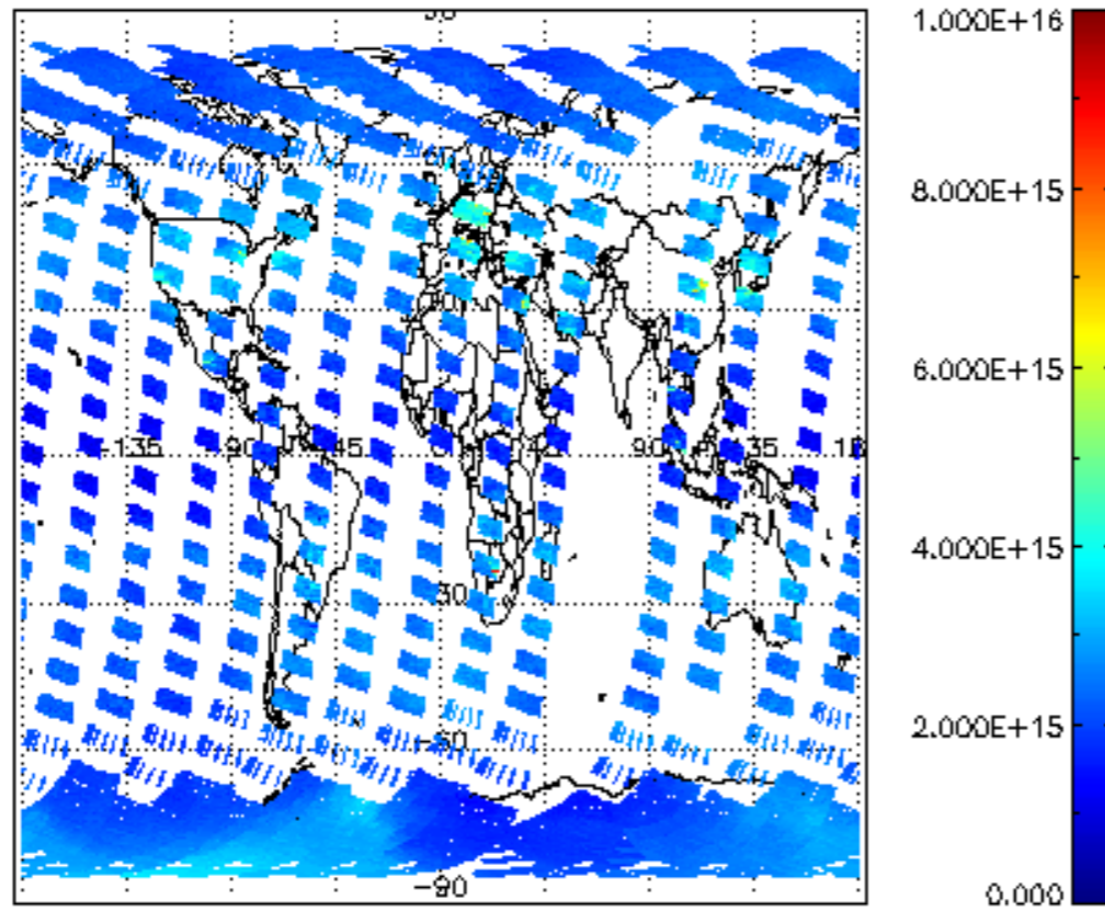
SCIOL2P_NADUV1NO2_vcd for 02OCT2002 00:00:00 to 03OCT2002 00:00:00
