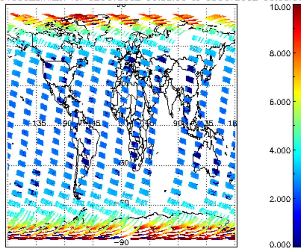
SCIOL2P_NADUV003_amf_sl for 02OCT2002 00:00:00 to 03OCT2002 00:00:00
