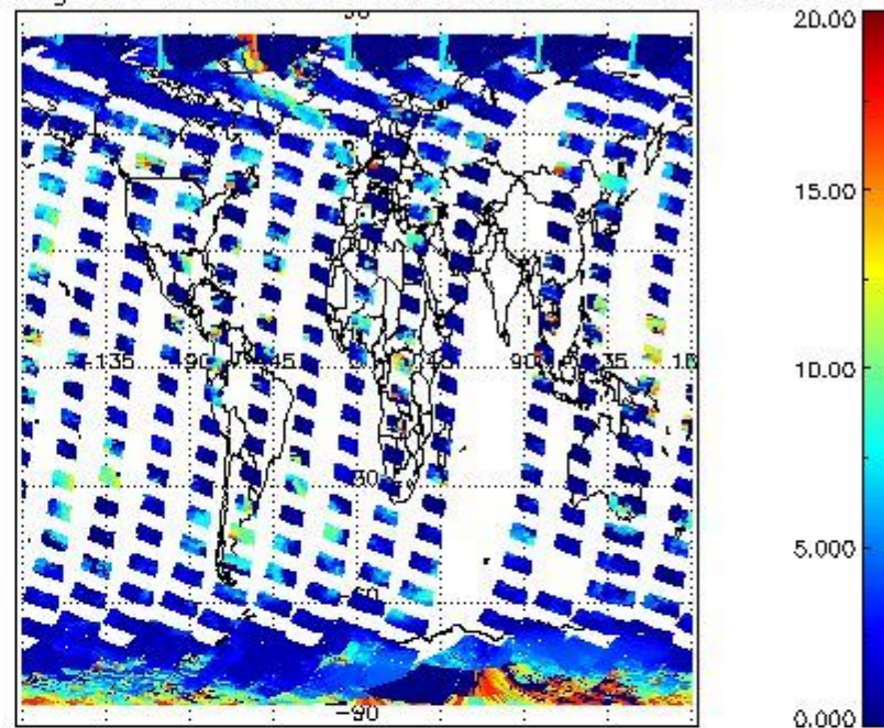
cL_top_height for 02OCT2002 00:00:00 to 03OCT2002 00:00:00
