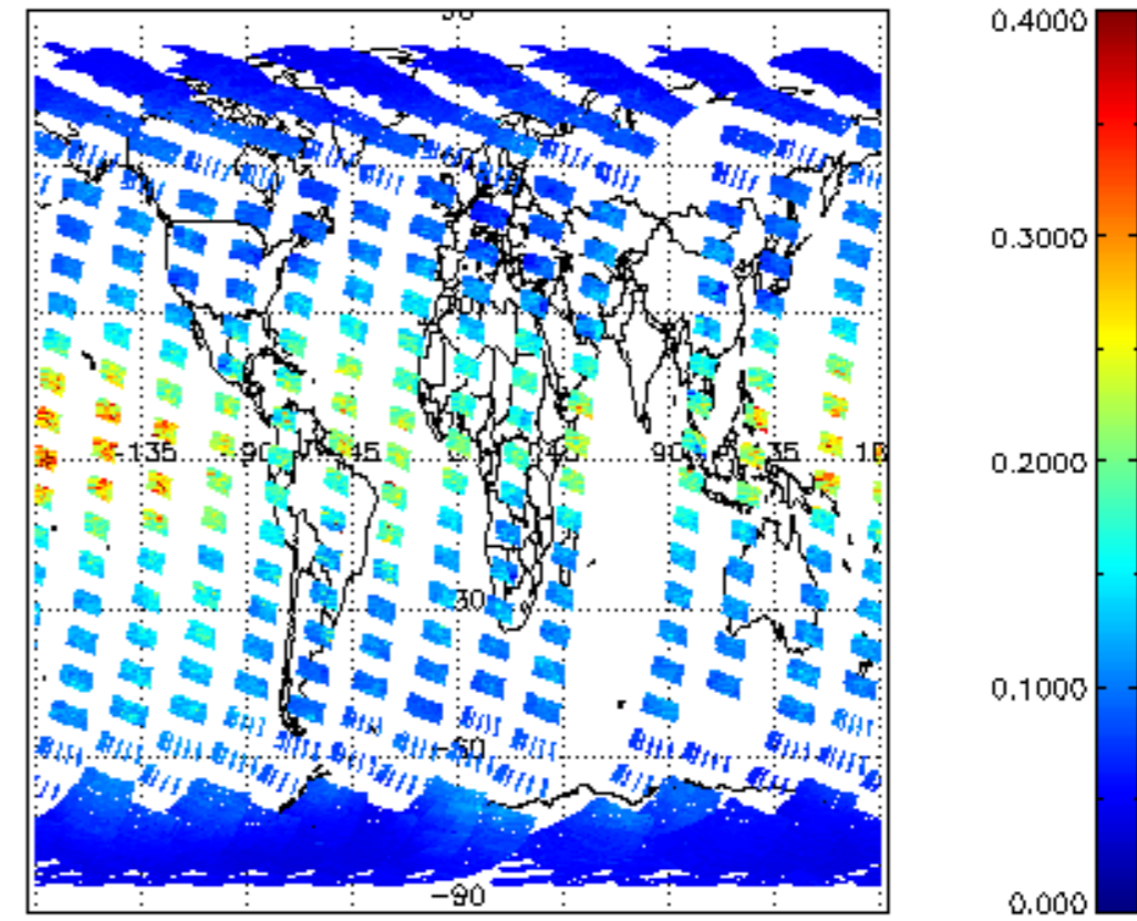
iCIOL2P_NADUV1NO2_vcd_err for 02OCT2002 00:00:00 to 03OCT2002 00:00:00
