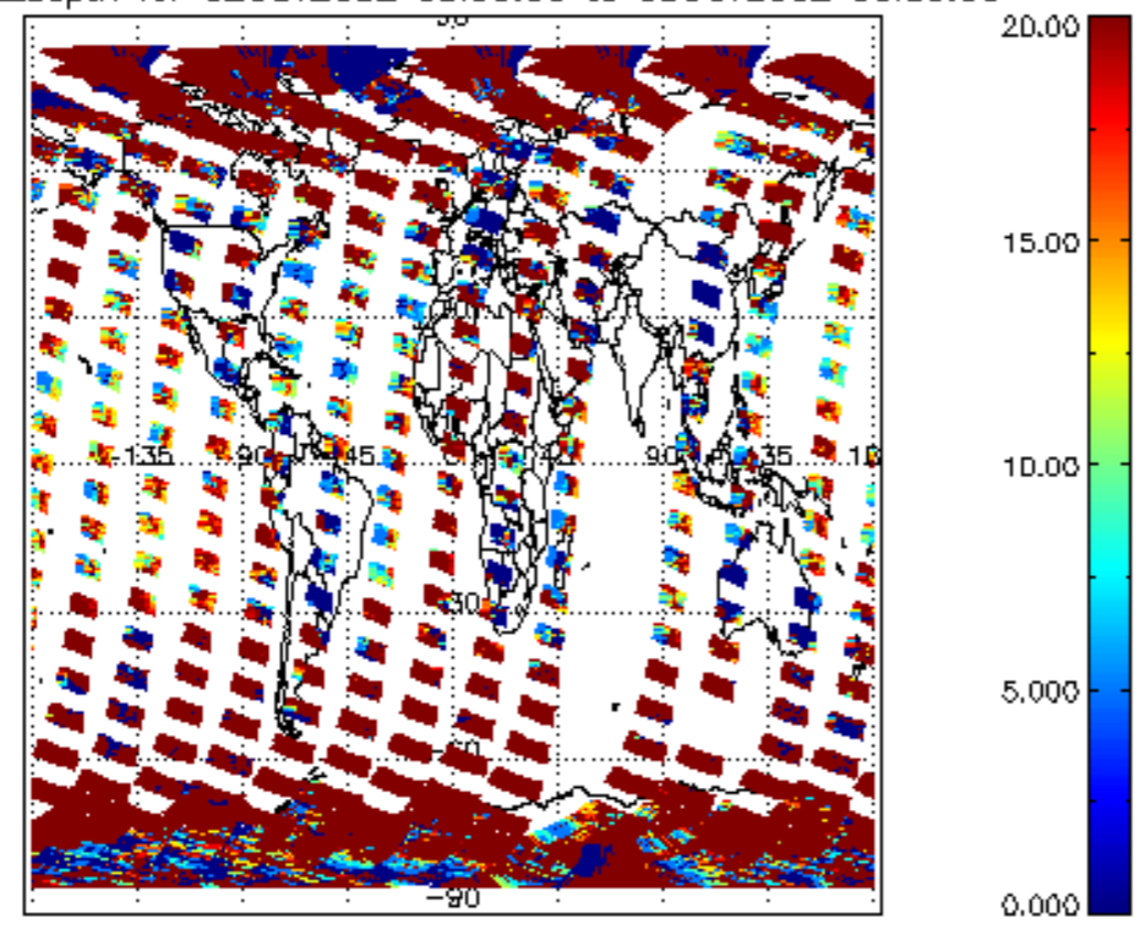
cl_opt_depth for 02OCT2002 00:00:00 to 03OCT2002 00:00:00
