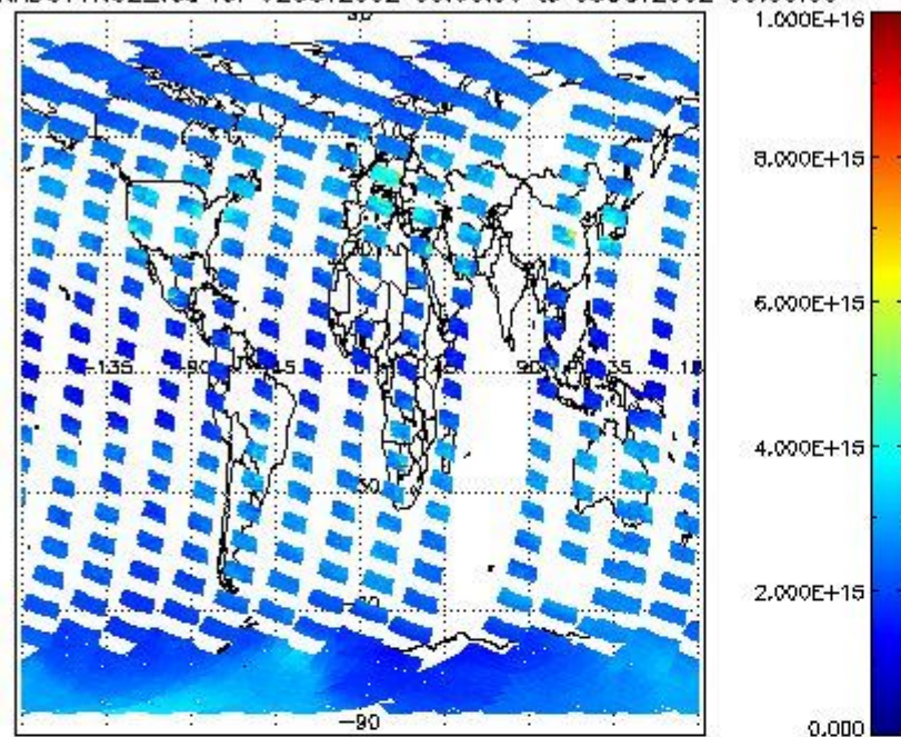
SCIOL2P_NADUV1N02_vcd for 02OCT2002 00:00:00 to 03OCT2002 00:00:00
