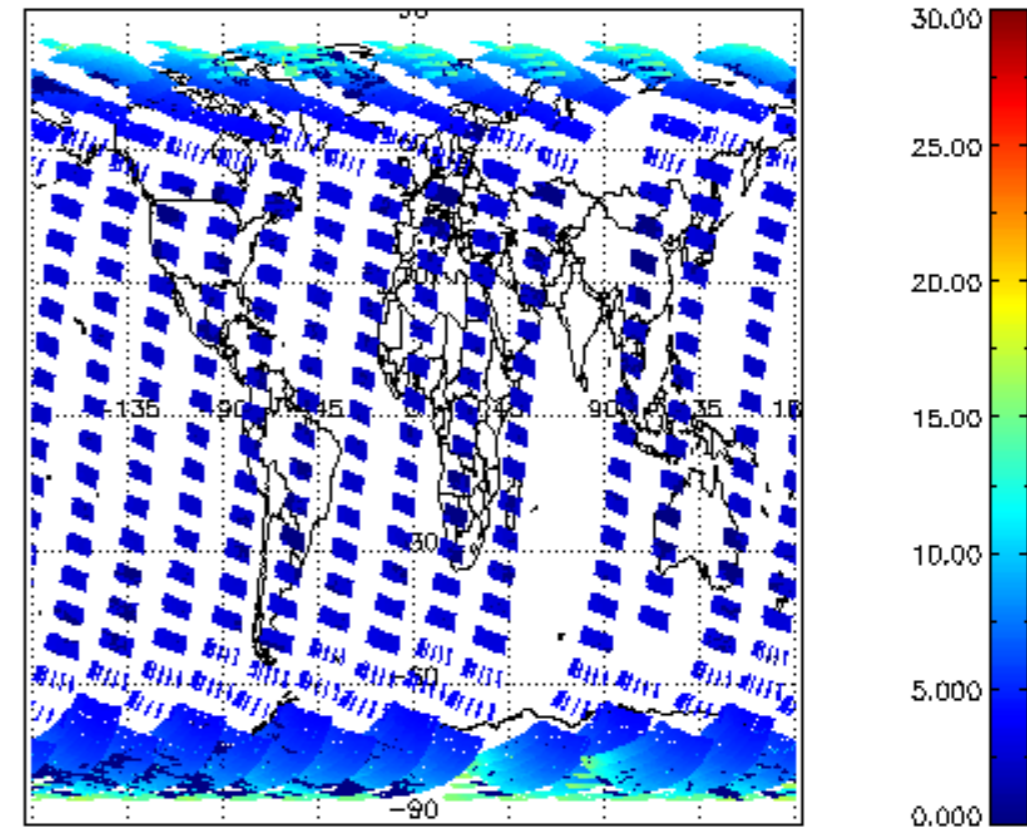
iCIOL2P_NADUV1NO2_amf_cl for 02OCT2002 00:00:00 to 03OCT2002 00:00:00
