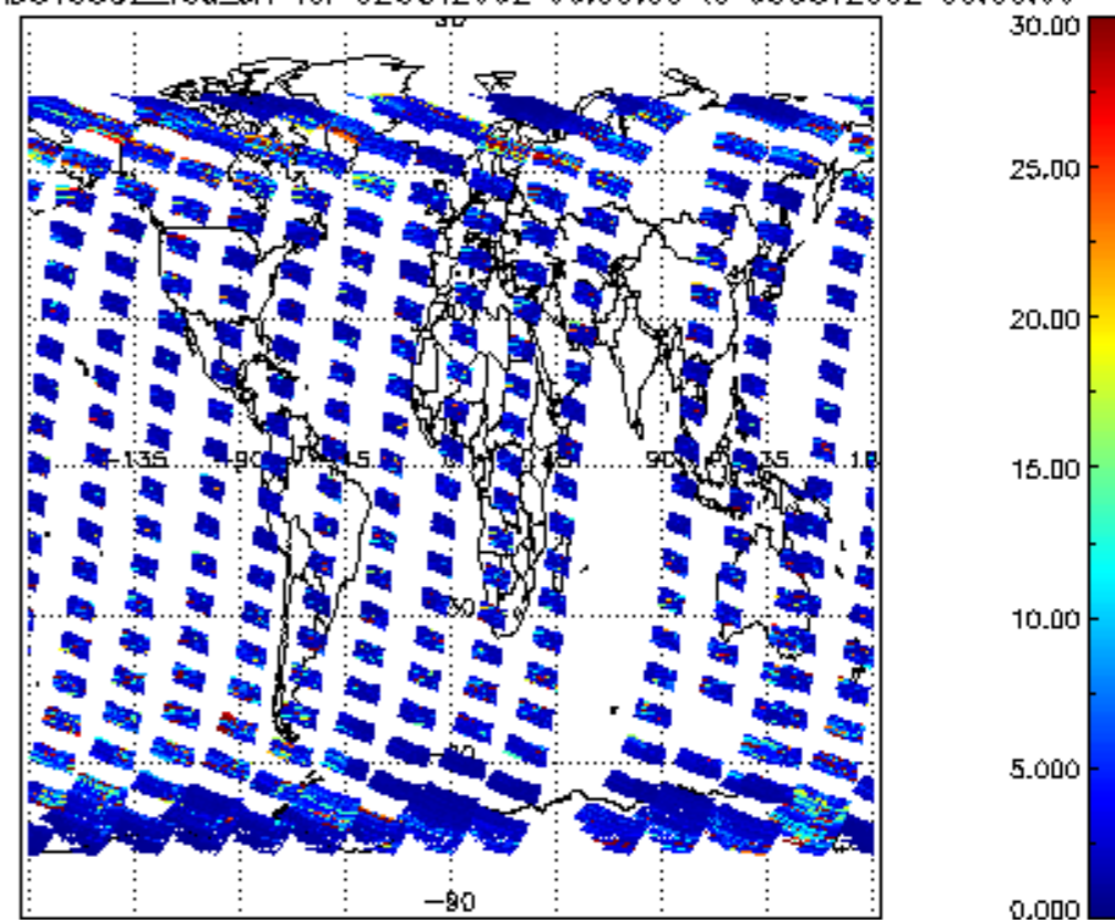
SCIOL2P_NADUV5S02_vcd_err for 02OCT2002 00:00:00 to 03OCT2002 00:00:00
