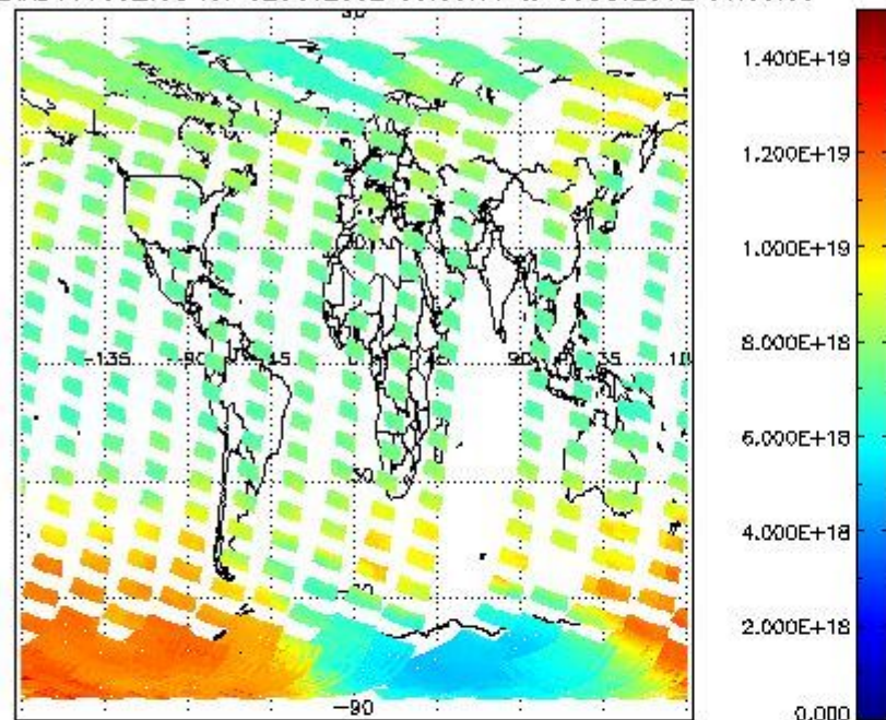
SCIOL2P_NADUV003_vcd for 02OCT2002 00:00:00 to 03OCT2002 00:00:00
