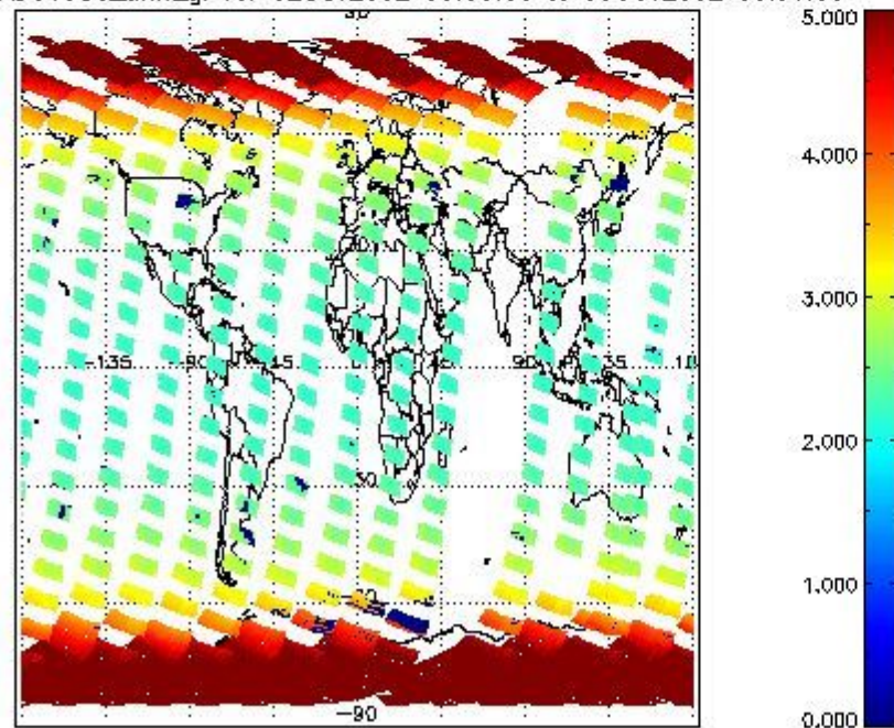
SCIOL2P_NADUV003_amf_gr for 02OCT2002 00:00:00 to 03OCT2002 00:00:00
