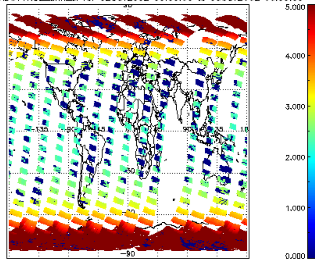
SCIOL2P_NADUV1N02_amf_cl for 02OCT2002 00:00:00 to 03OCT2002 00:00:00
