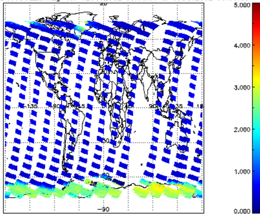
SCIOL2P_NADUV5S02_amf_gr for 02OCT2002 00:00:00 to 03OCT2002 00:00:00
