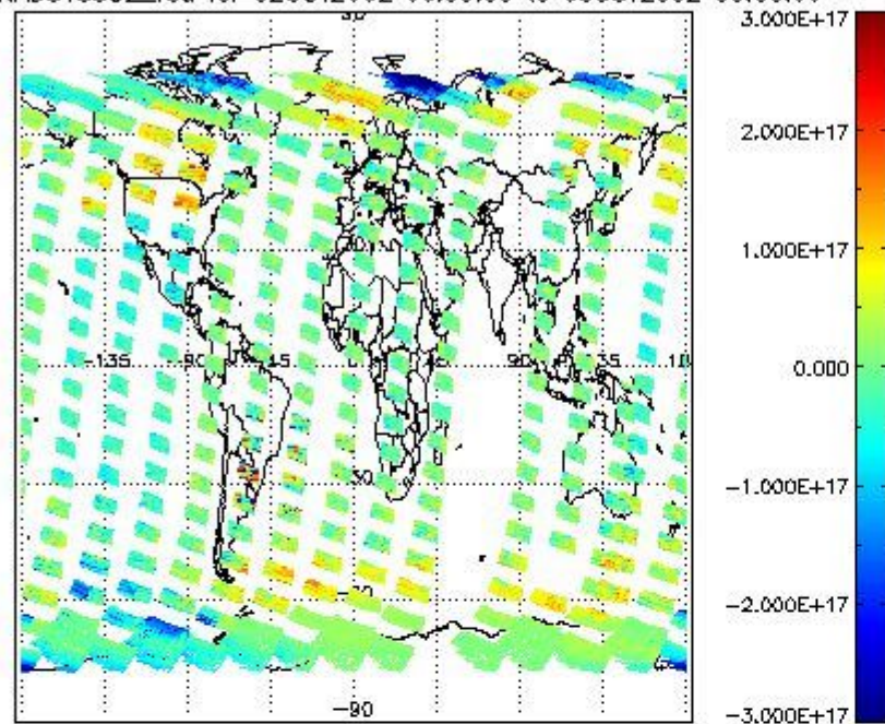
SCIOL2P_NADUV5S02_vcd for 02OCT2002 00:00:00 to 03OCT2002 00:00:00
