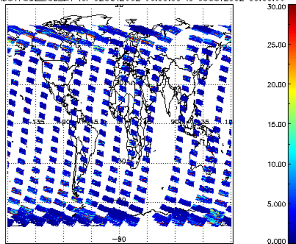
SCIOL2P_NADUV7S02_vcd_err for 02OCT2002 00:00:00 to 03OCT2002 00:00:00
