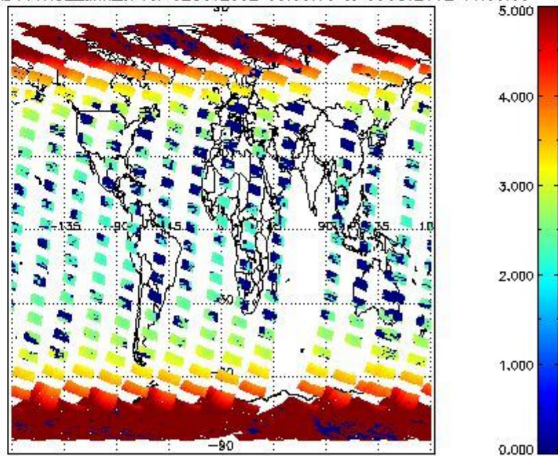
SCIOL2P_NADUV1N02_amf_cl for 02OCT2002 00:00:00 to 03OCT2002 00:00:00
