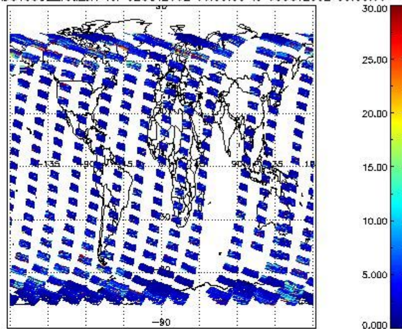
SCIOL2P_NADUV5S02_vcd_err for 02OCT2002 00:00:00 to 03OCT2002 00:00:00
