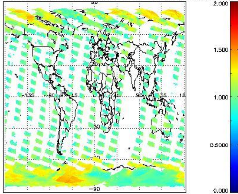
SCIOL2P_NADUV8H20_amf_gr for 02OCT2002 00:00:00 to 03OCT2002 00:00:00
