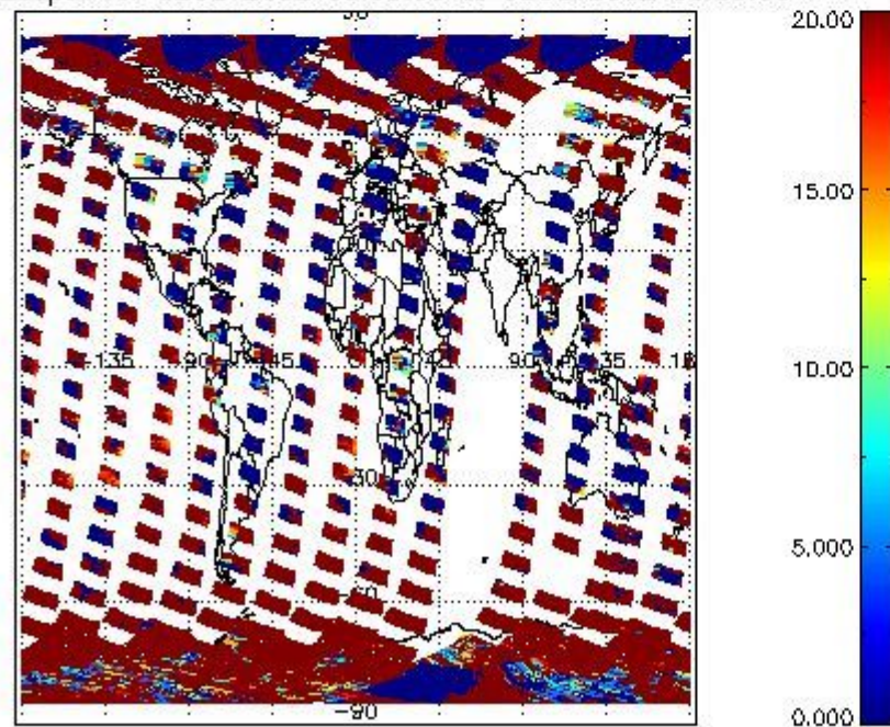
cL_opt_depth for 02OCT2002 00:00:00 to 03OCT2002 00:00:00
