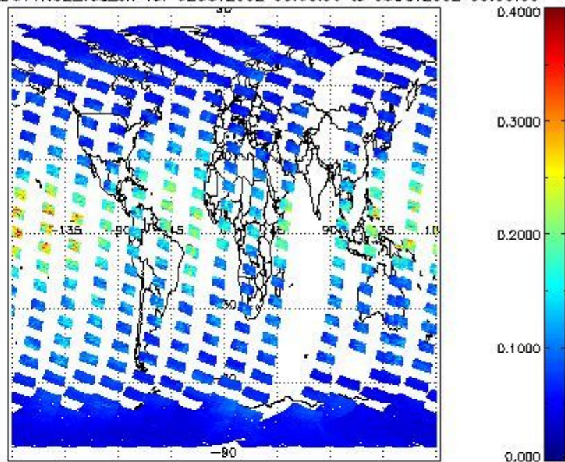
SCIOL2P_NADUV1N02_vcd_err for 02OCT2002 00:00:00 to 03OCT2002 00:00:00
