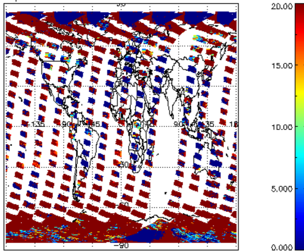
cl_opt_depth for 02OCT2002 00:00:00 to 03OCT2002 00:00:00
