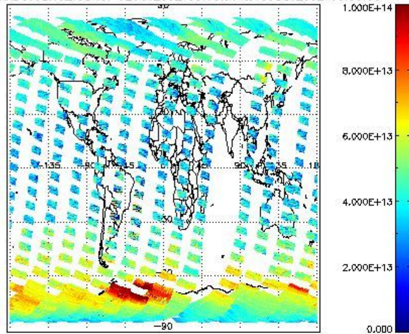
SCIOL2P_NADUV3BRO_vcd for 02OCT2002 00:00:00 to 03OCT2002 00:00:00
