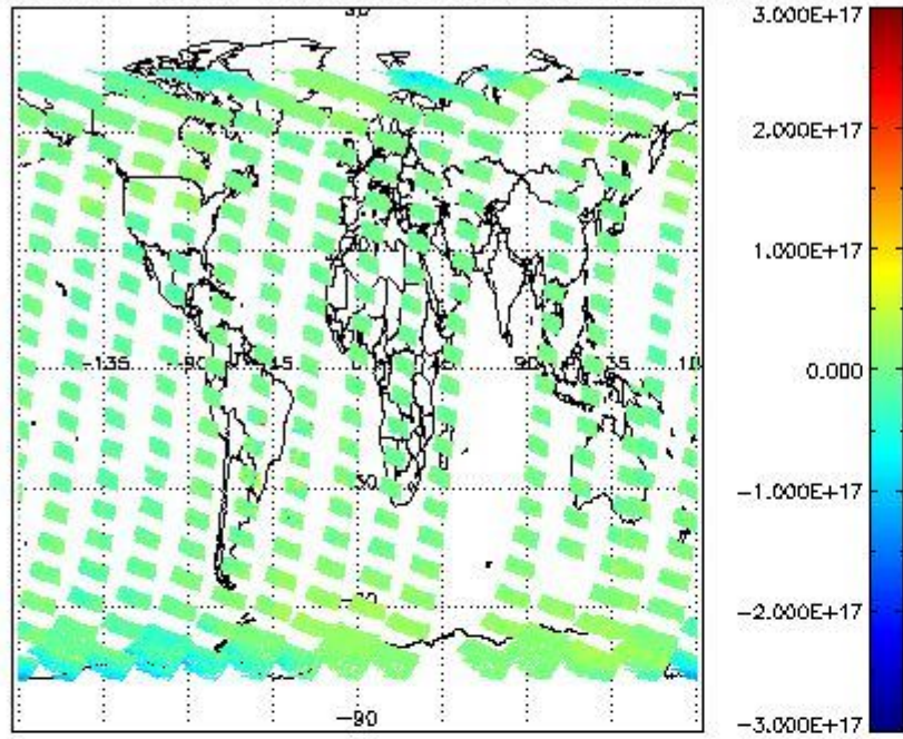
SCIOL2P_NADUV7S02_vcd for 02OCT2002 00:00:00 to 03OCT2002 00:00:00
