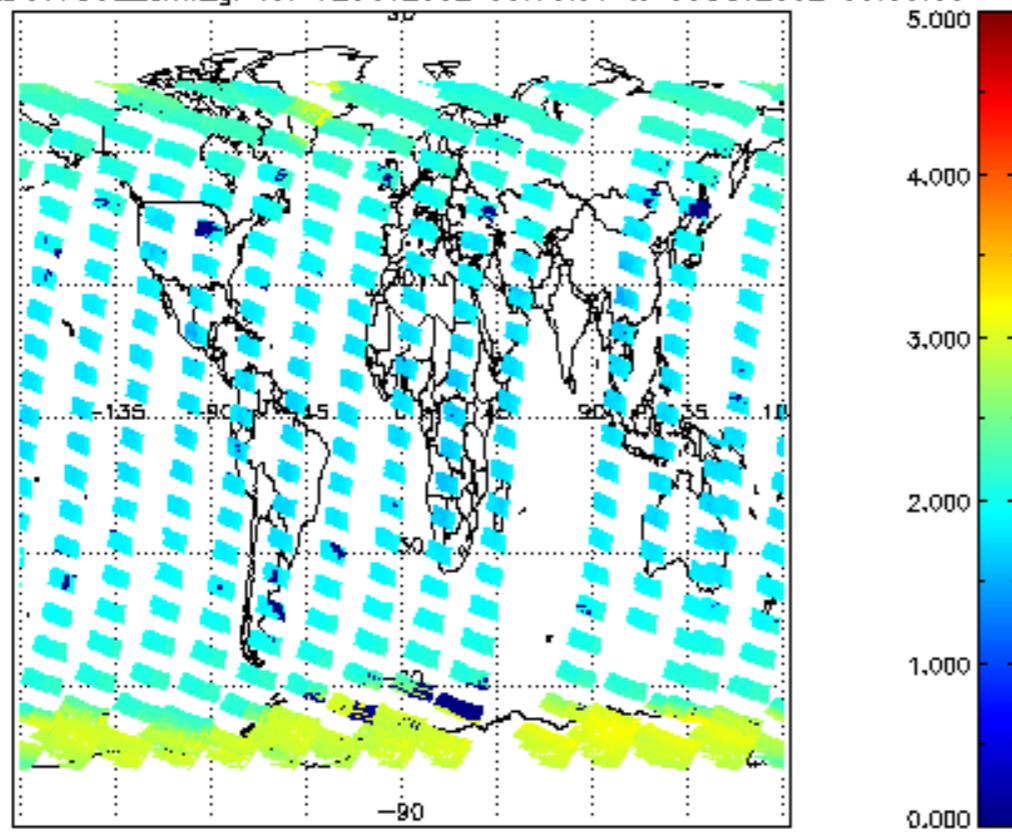
SCIOL2P_NADUV7S02_amf_gr for 02OCT2002 00:00:00 to 03OCT2002 00:00:00
