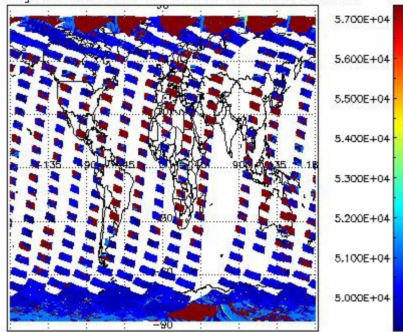
cloud_flags for 02OCT2002 00:00:00 to 03OCT2002 00:00:00
