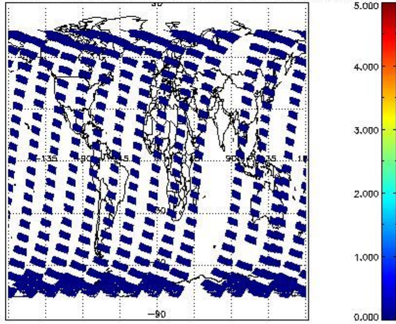
SCIOL2P_NADUV7S02_amf_cl for 02OCT2002 00:00:00 to 03OCT2002 00:00:00
