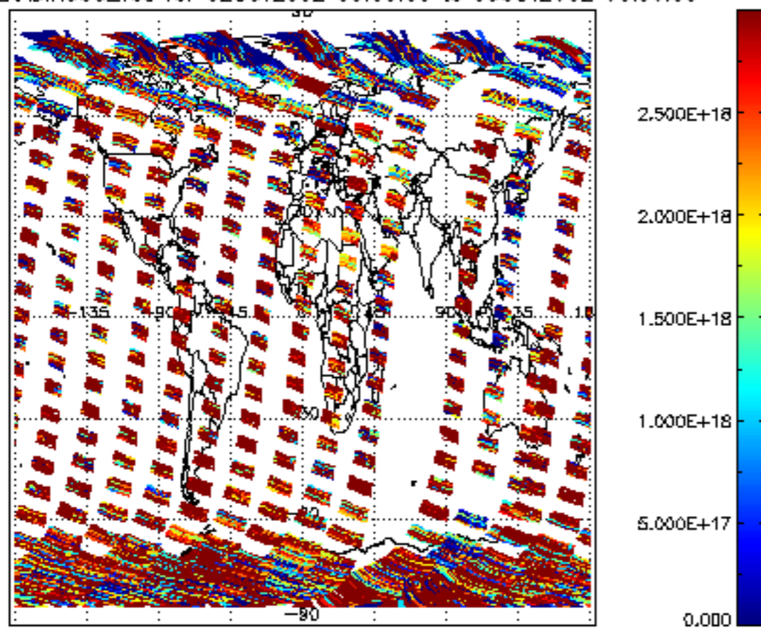
SCIOL2P_NADIR3CO_vcd for 02OCT2002 00:00:00 to 03OCT2002 00:00:00
