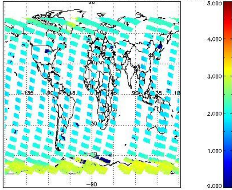
SCIOL2P_NADUV7S02_amf_gr for 02OCT2002 00:00:00 to 03OCT2002 00:00:00
