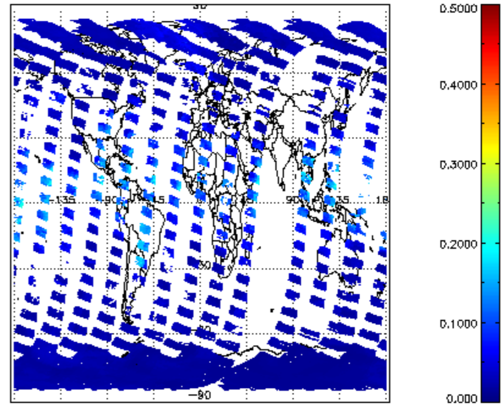
SCIOL2P_NADUV8H20_vcd_err for 02OCT2002 00:00:00 to 03OCT2002 00:00:00
