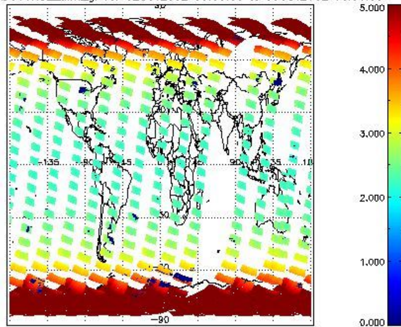
SCIOL2P_NADUV1N02_amf_gr for 02OCT2002 00:00:00 to 03OCT2002 00:00:00
