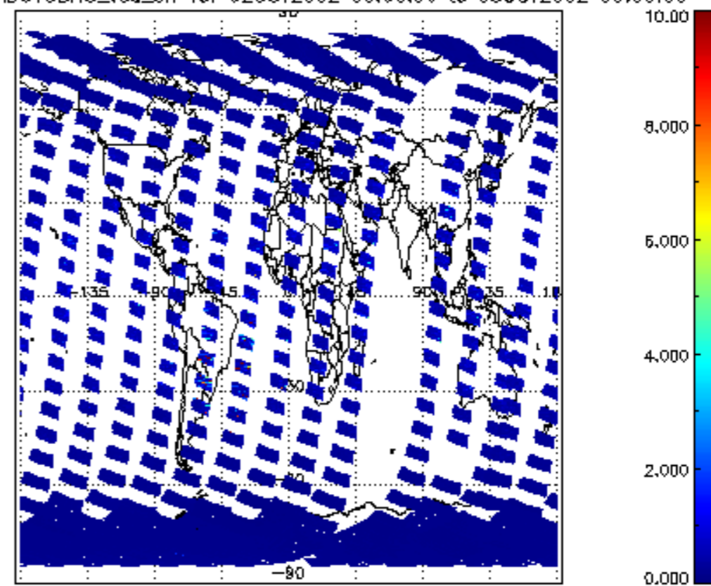
SCIOL2P_NADUV3BRO_vcd_err for 02OCT2002 00:00:00 to 03OCT2002 00:00:00
