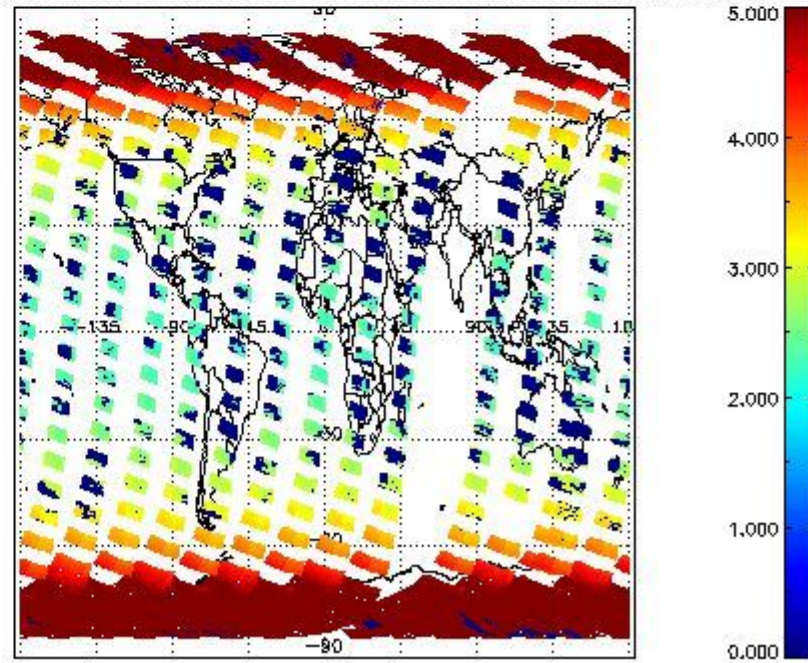
SCIOL2P_NADUV3BRO_amf_cl for 02OCT2002 00:00:00 to 03OCT2002 00:00:00
