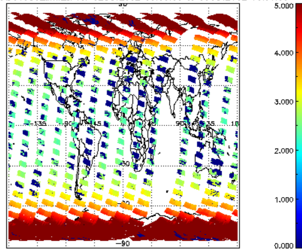
SCIOL2P_NADUV003_amf_cl for 02OCT2002 00:00:00 to 03OCT2002 00:00:00
