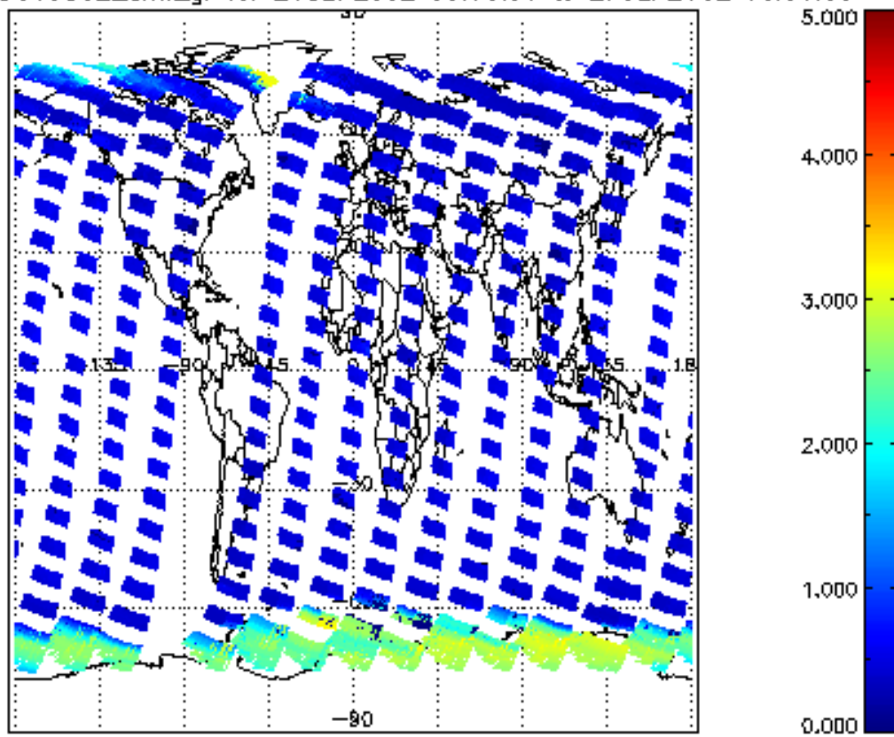
SCIOL2P_NADUV5S02_amf_gr for 26SEP2002 00:00:00 to 27SEP2002 00:00:00
