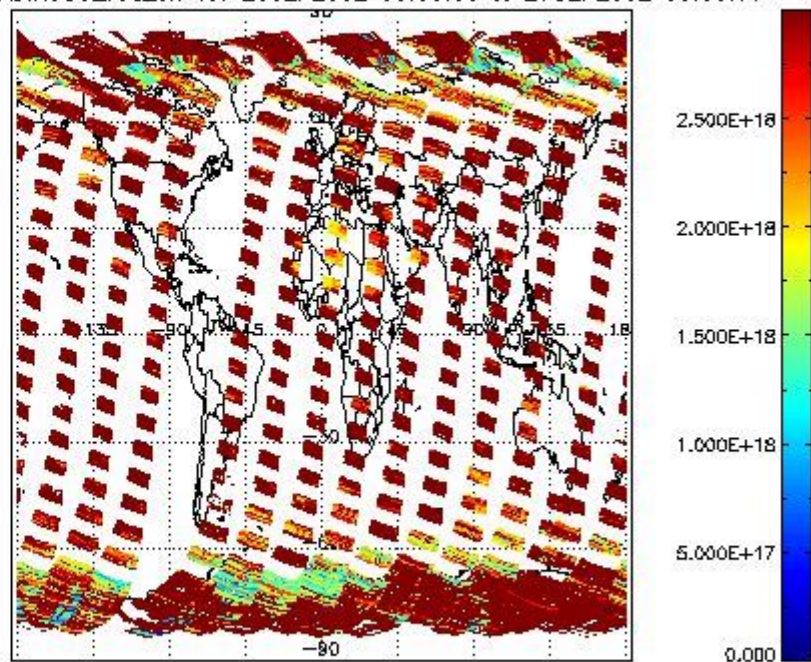
SCIDL2P_NADIR3CO_vcd_err for 26SEP2002 00:00:00 to 27SEP2002 00:00:00
