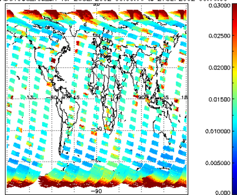
SCIOL2P_NADUV003_vcd_err for 26SEP2002 00:00:00 to 27SEP2002 00:00:00
