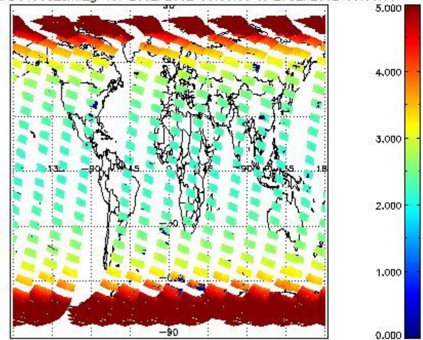
SCIOL2P_NADUV003_amf_gr for 26SEP2002 00:00:00 to 27SEP2002 00:00:00
