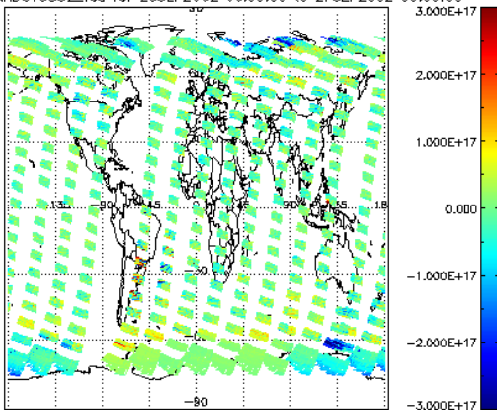
SCIOL2P_NADUV5S02_vcd for 26SEP2002 00:00:00 to 27SEP2002 00:00:00
