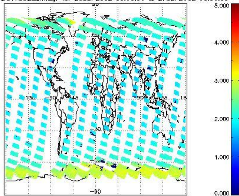
SCIOL2P_NADUV7S02_amf_gr for 26SEP2002 00:00:00 to 27SEP2002 00:00:00
