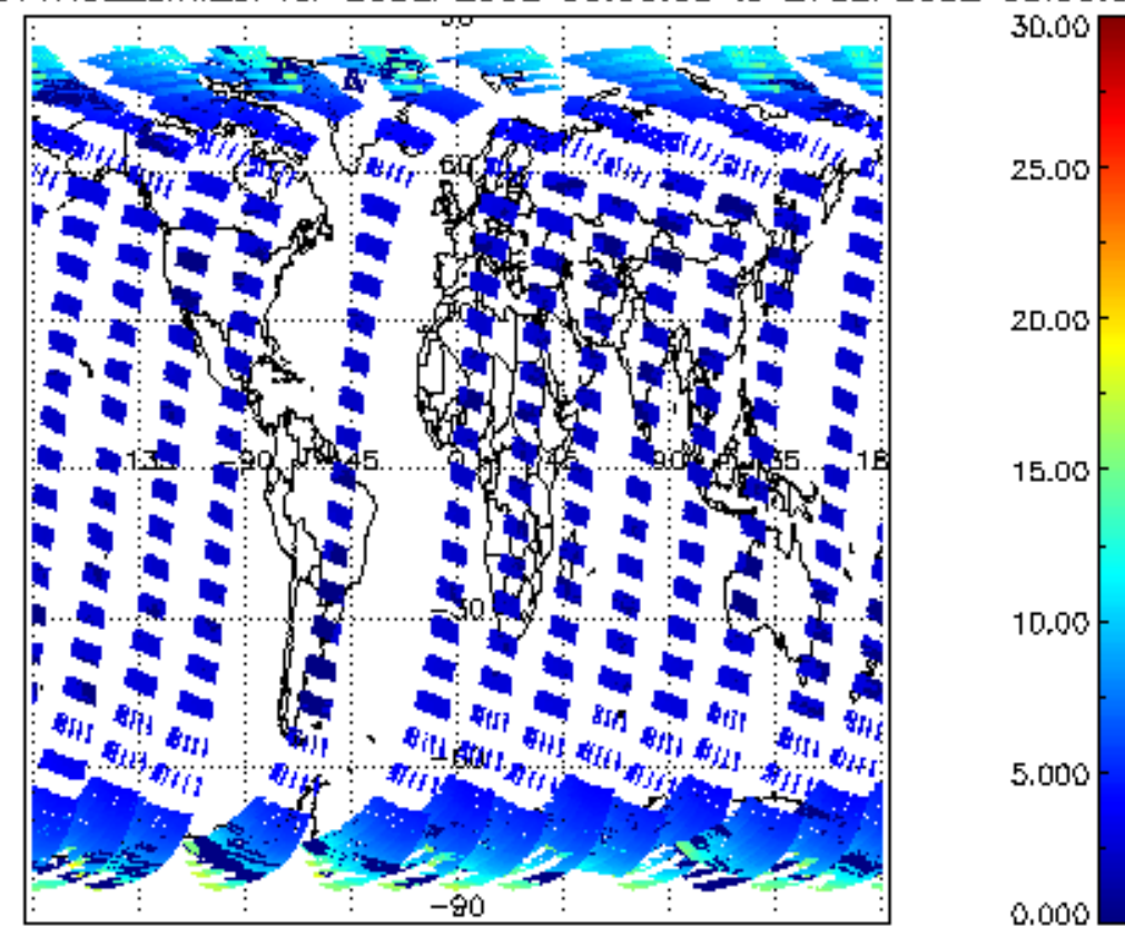
iCIOL2P_NADUV1NO2_amf_cl for 26SEP2002 00:00:00 to 27SEP2002 00:00:00
