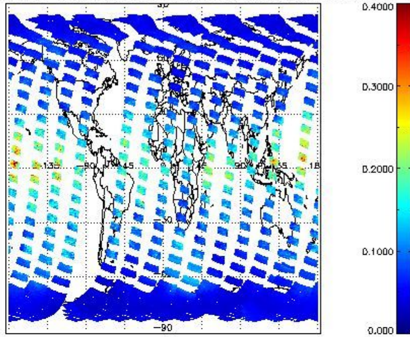
SCIOL2P_NADUV1N02_vcd_err for 26SEP2002 00:00:00 to 27SEP2002 00:00:00
