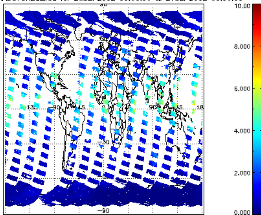
SCIOL2P_NADUV8H20_vcd for 26SEP2002 00:00:00 to 27SEP2002 00:00:00
