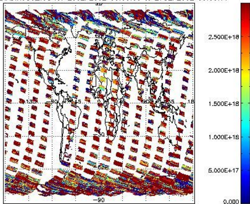
SCIDL2P_NADIR3CO_vcd for 26SEP2002 00:00:00 to 27SEP2002 00:00:00
