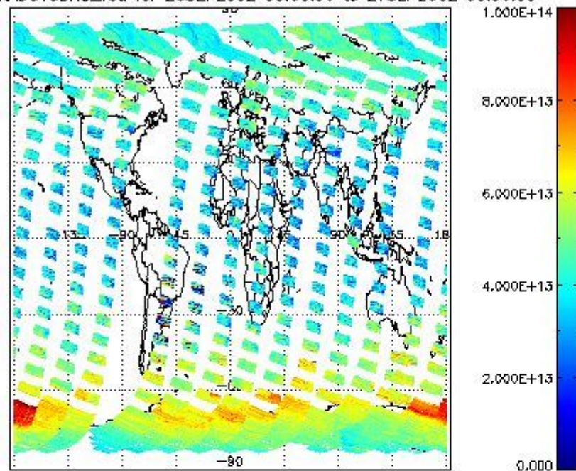
SCIOL2P_NADUV3BRO_vcd for 26SEP2002 00:00:00 to 27SEP2002 00:00:00
