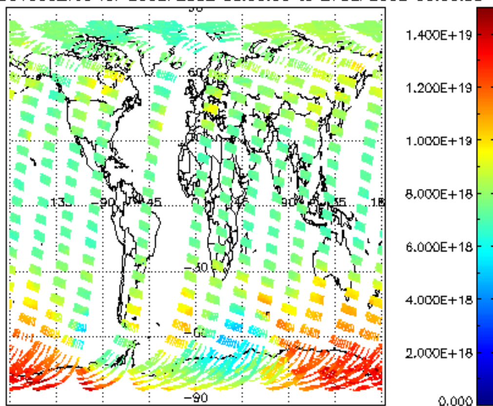
SCIOL2P_NADUV003_vcd for 26SEP2002 00:00:00 to 27SEP2002 00:00:00
