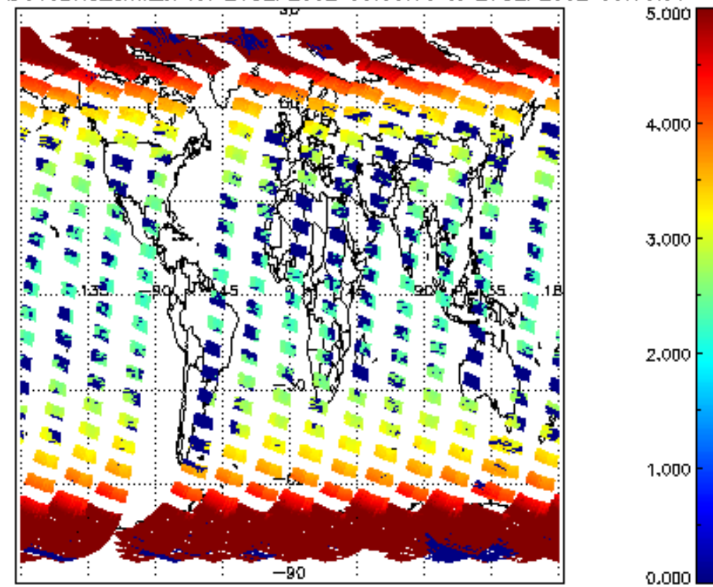
SCIOL2P_NADUV3BRO_amf_sl for 26SEP2002 00:00:00 to 27SEP2002 00:00:00
