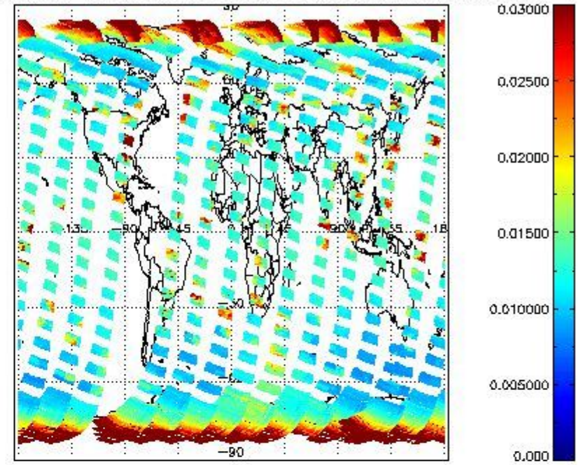
SCIOL2P_NADUV003_vcd_err for 26SEP2002 00:00:00 to 27SEP2002 00:00:00
