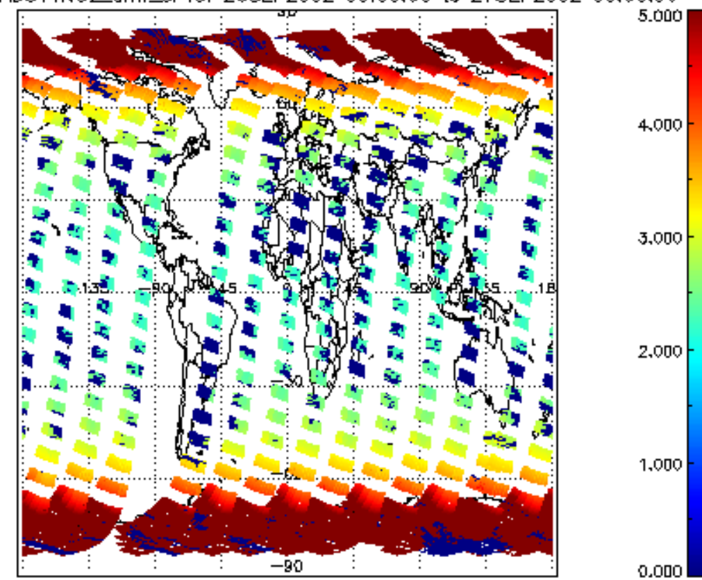
SCIOL2P_NADUV1N02_amf_cl for 26SEP2002 00:00:00 to 27SEP2002 00:00:00
