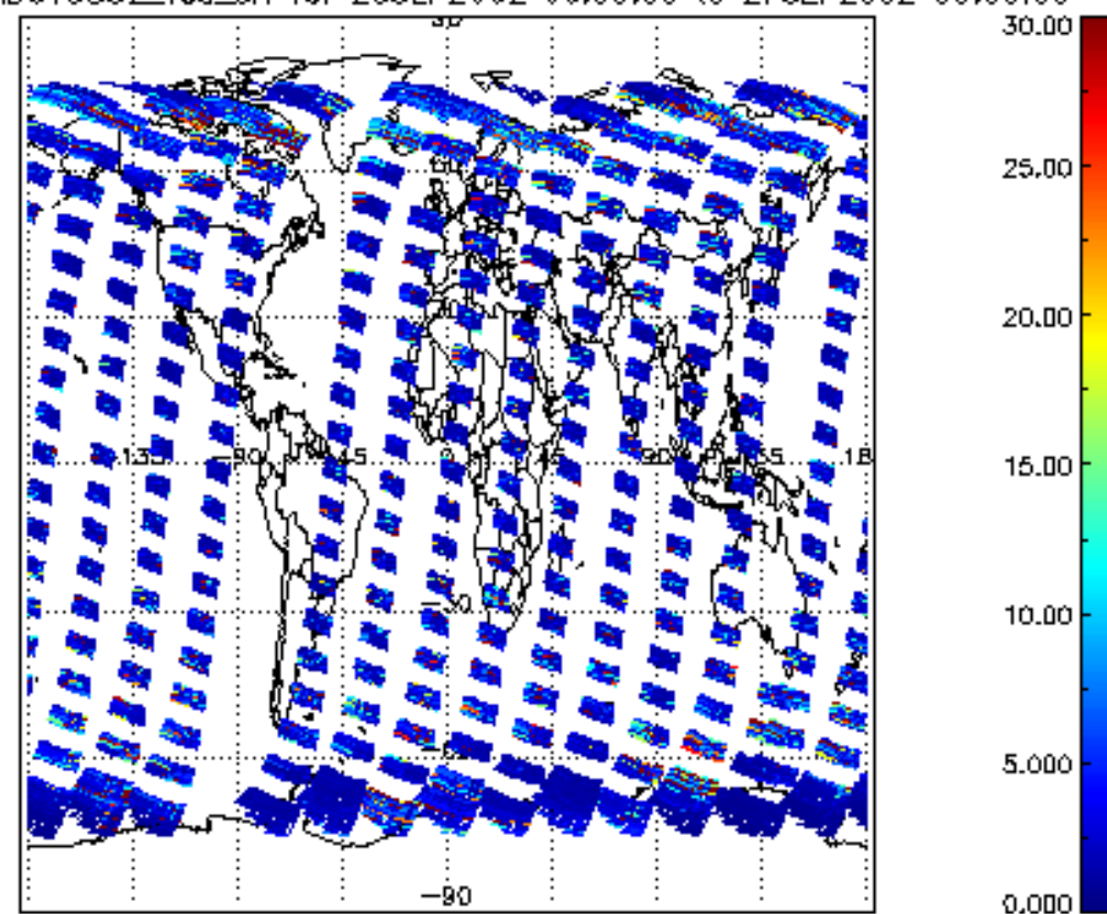
SCIOL2P_NADUV5S02_vcd_err for 26SEP2002 00:00:00 to 27SEP2002 00:00:00
