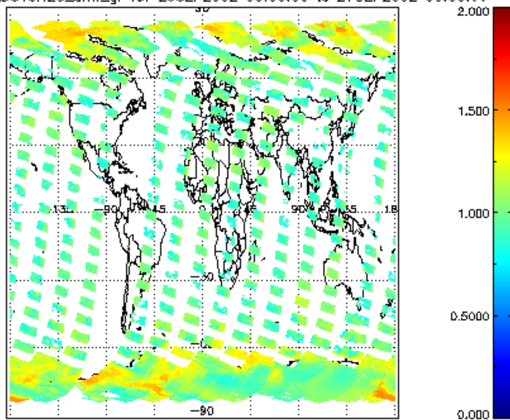
SCIOL2P_NADUV8H20_amf_gr for 26SEP2002 00:00:00 to 27SEP2002 00:00:00
