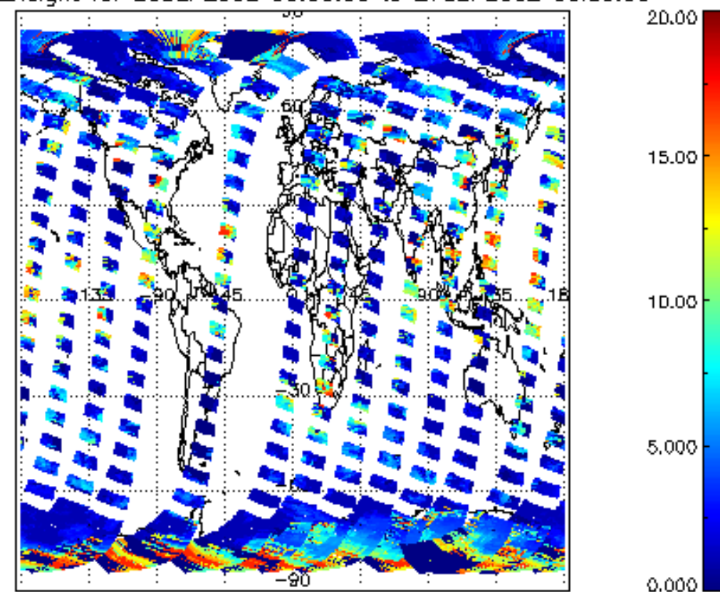
cl_top_height for 26SEP2002 00:00:00 to 27SEP2002 00:00:00
