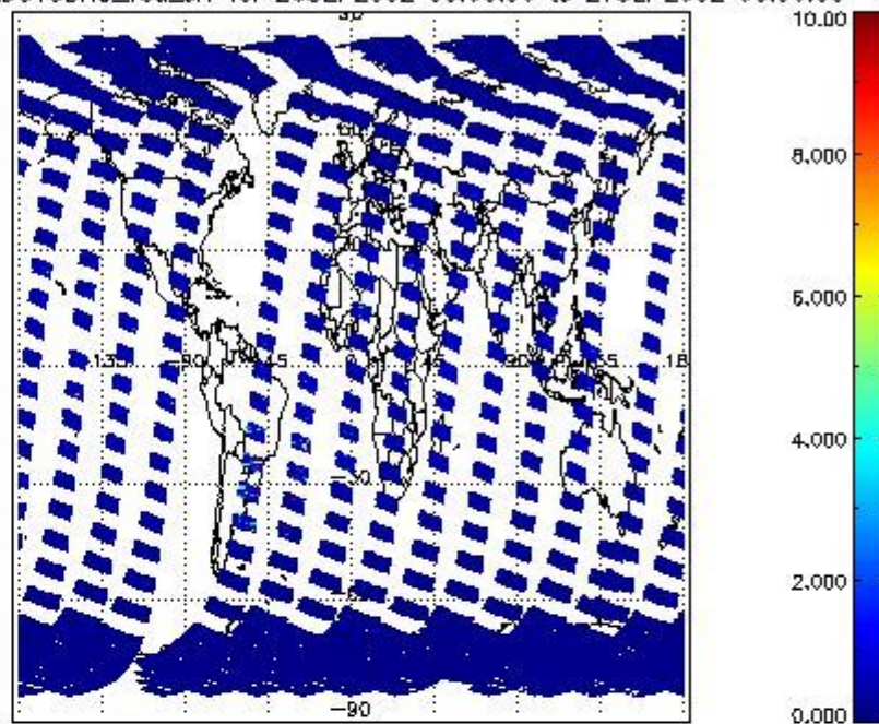
SCIOL2P_NADUV3BRO_vcd_err for 26SEP2002 00:00:00 to 27SEP2002 00:00:00
