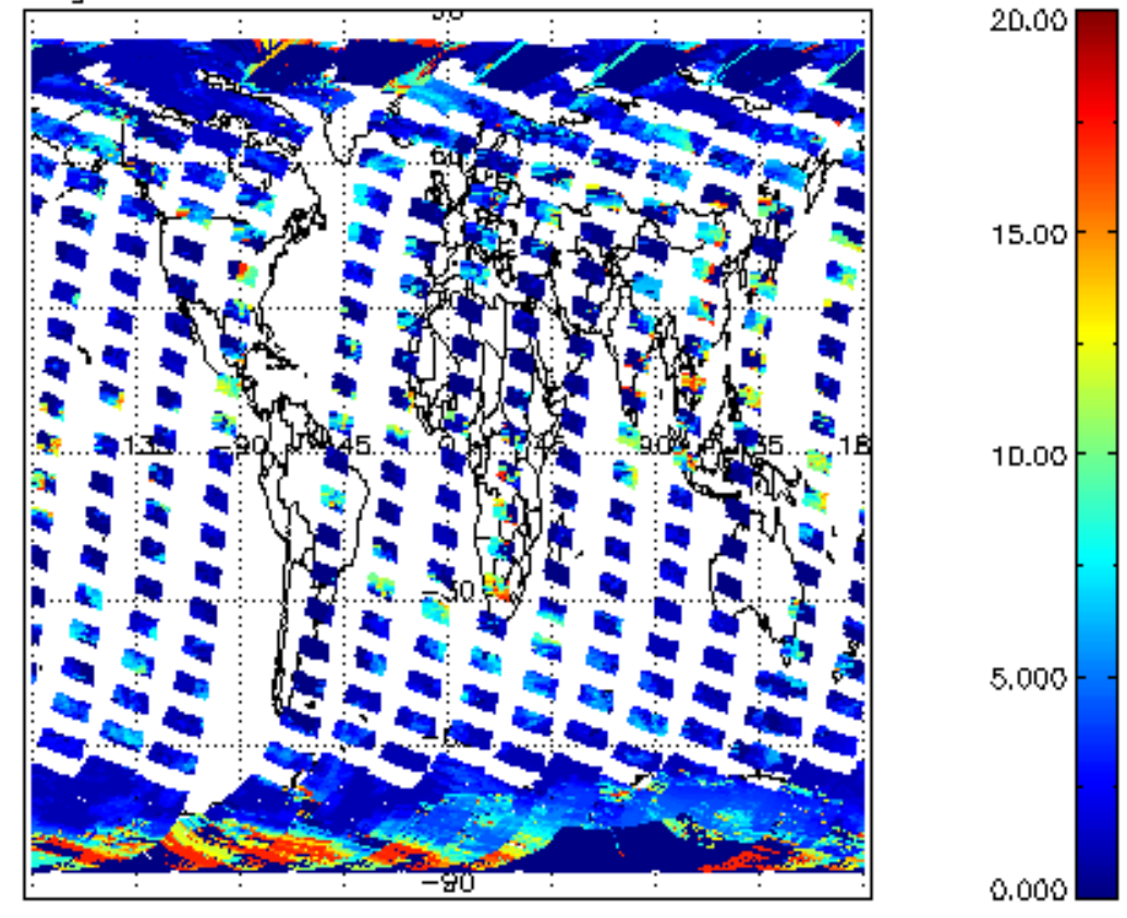
cl_top_height for 26SEP2002 00:00:00 to 27SEP2002 00:00:00
