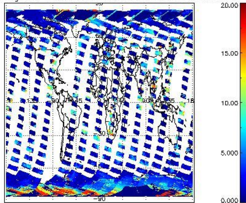
cL_top_height for 26SEP2002 00:00:00 to 27SEP2002 00:00:00
