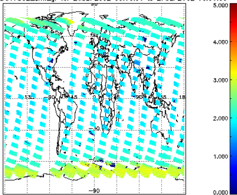
SCIOL2P_NADUV7S02_amf_gr for 26SEP2002 00:00:00 to 27SEP2002 00:00:00
