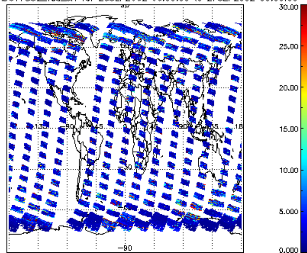
SCIOL2P_NADUV7S02_vcd_err for 26SEP2002 00:00:00 to 27SEP2002 00:00:00
