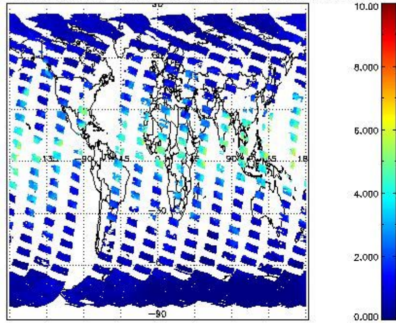
SCIOL2P_NADUV8H2O_vcd for 26SEP2002 00:00:00 to 27SEP2002 00:00:00
