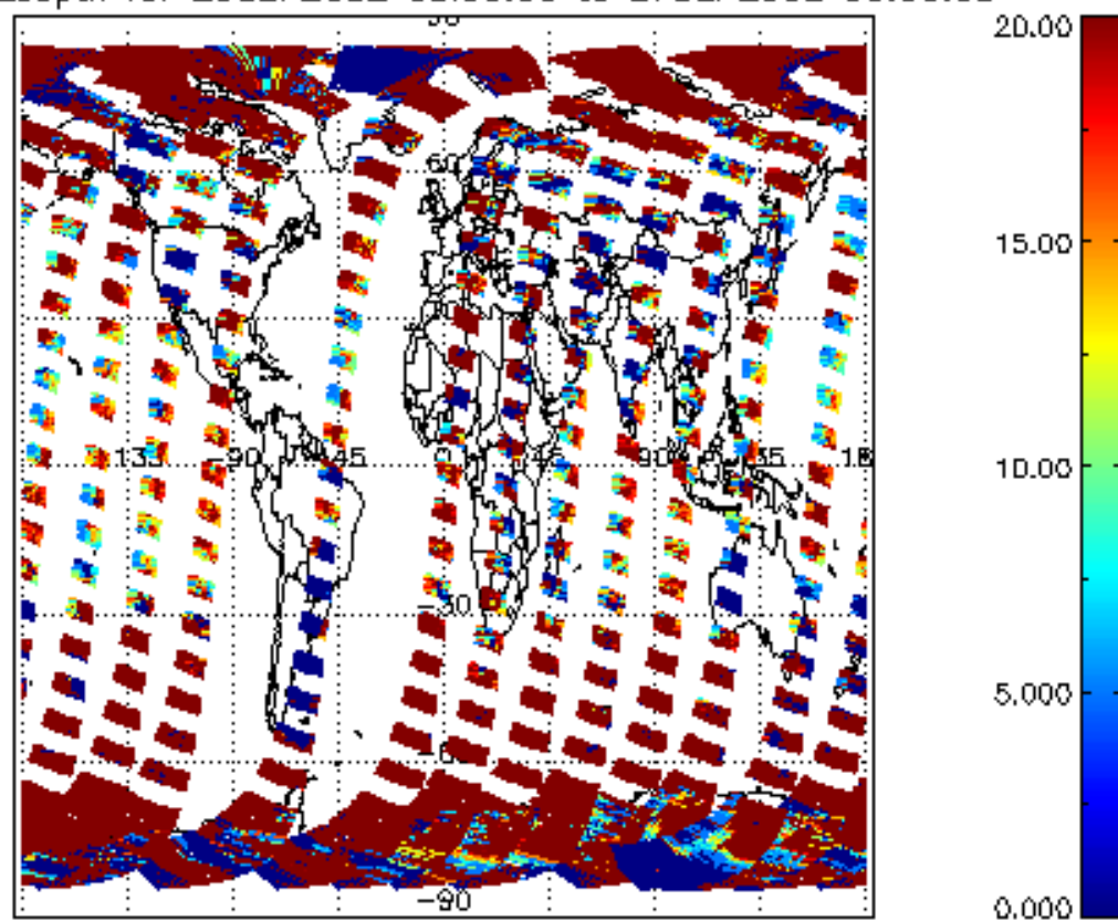
cl_opt_depth for 26SEP2002 00:00:00 to 27SEP2002 00:00:00
