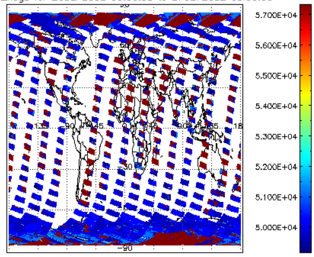
cloud_flags for 26SEP2002 00:00:00 to 27SEP2002 00:00:00
