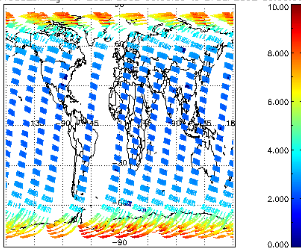
SCIOL2P_NADUV003_amf_gr for 26SEP2002 00:00:00 to 27SEP2002 00:00:00
