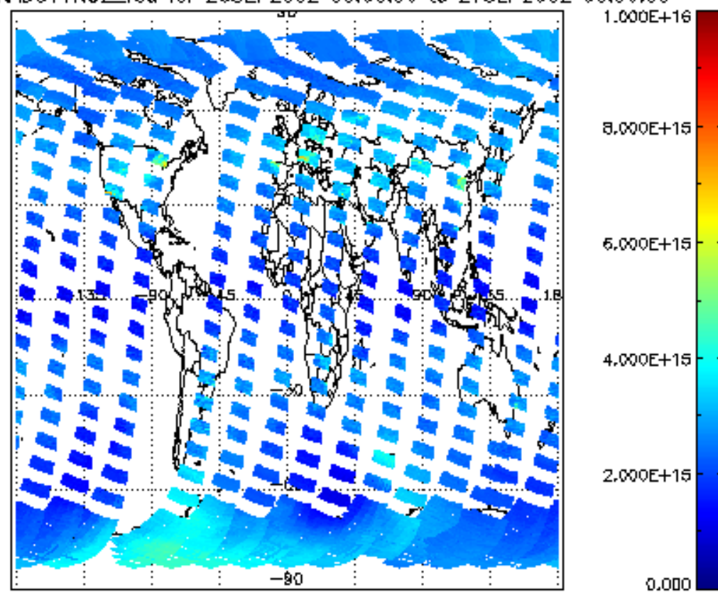
SCIOL2P_NADUV1N02_vcd for 26SEP2002 00:00:00 to 27SEP2002 00:00:00
