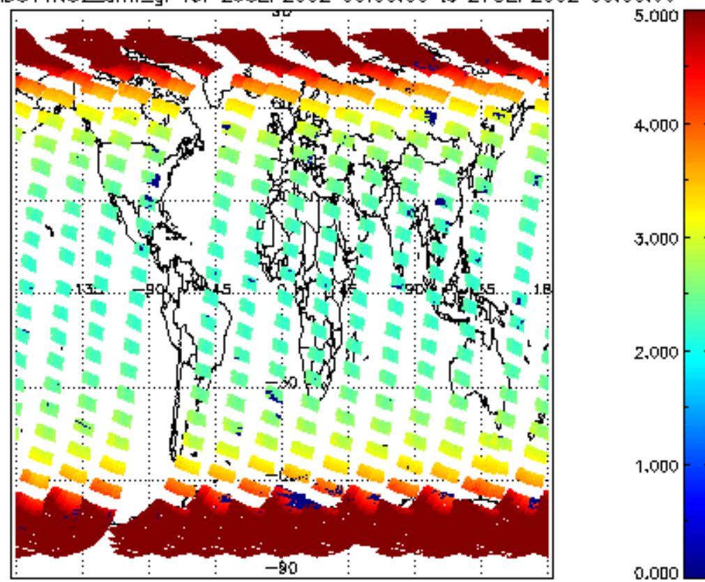
SCIOL2P_NADUV1N02_amf_gr for 26SEP2002 00:00:00 to 27SEP2002 00:00:00
