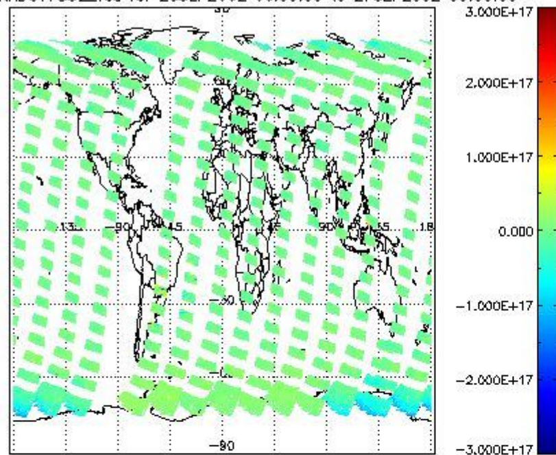
SCIOL2P_NADUV7S02_vcd for 26SEP2002 00:00:00 to 27SEP2002 00:00:00
