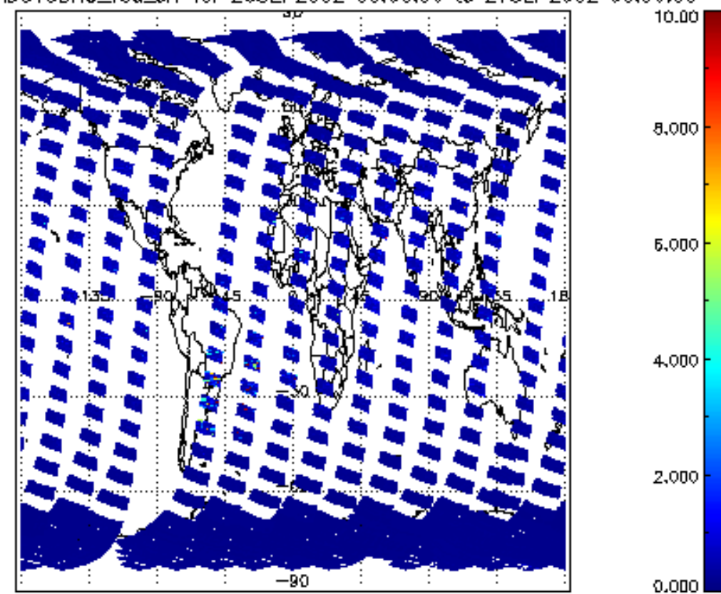
SCIOL2P_NADUV3BRO_vcd_err for 26SEP2002 00:00:00 to 27SEP2002 00:00:00
