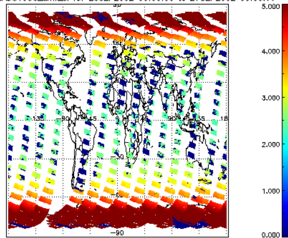
SCIOL2P_NADUV003_amf_cl for 26SEP2002 00:00:00 to 27SEP2002 00:00:00
