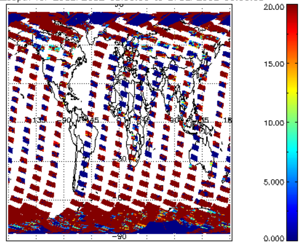
cl_opt_depth for 26SEP2002 00:00:00 to 27SEP2002 00:00:00
