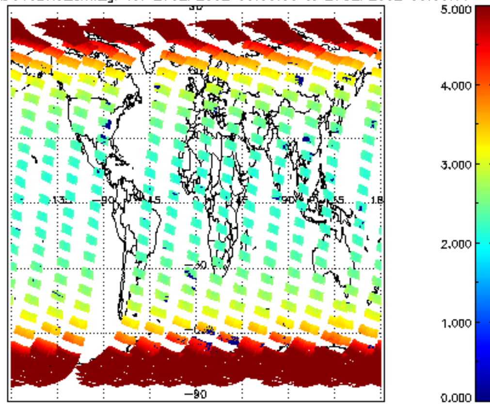
SCIOL2P_NADUV3BRO_amf_gr for 26SEP2002 00:00:00 to 27SEP2002 00:00:00
