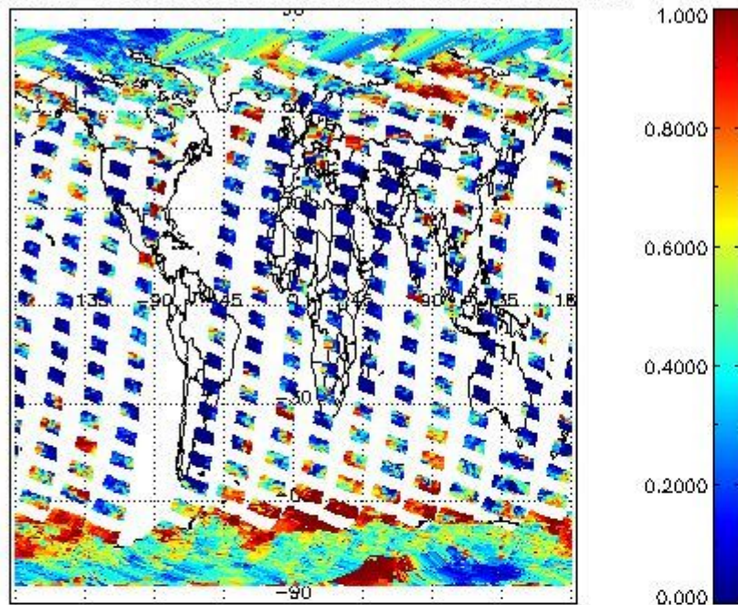
cL_frac for 26SEP2002 00:00:00 to 27SEP2002 00:00:00
