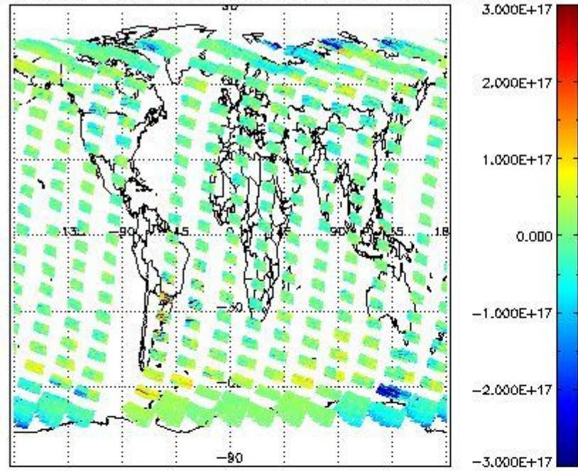
SCIOL2P_NADUV5S02_vcd for 26SEP2002 00:00:00 to 27SEP2002 00:00:00
