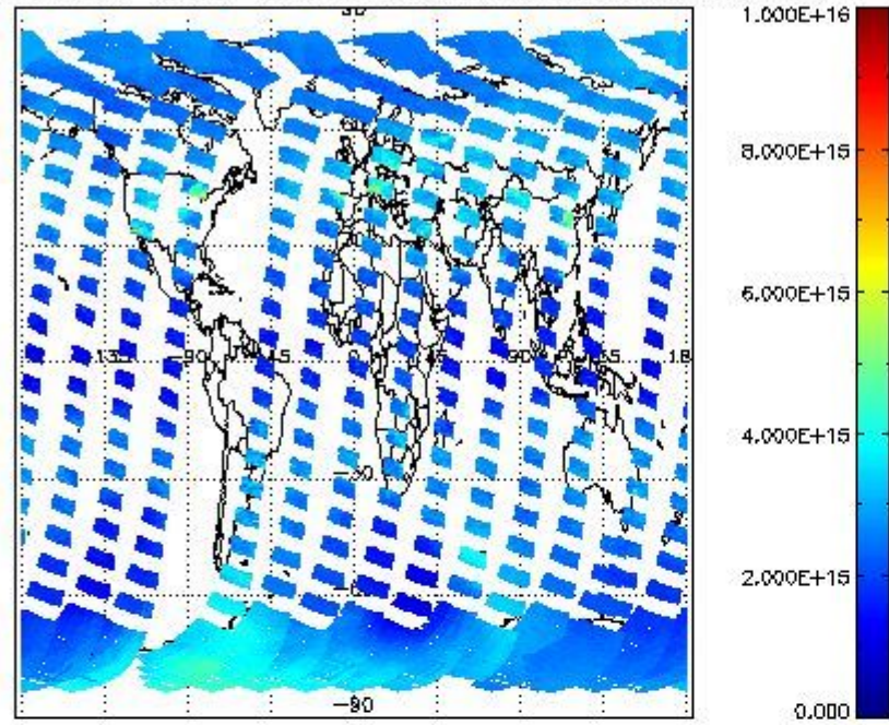
SCIOL2P_NADUV1N02_vcd for 26SEP2002 00:00:00 to 27SEP2002 00:00:00
