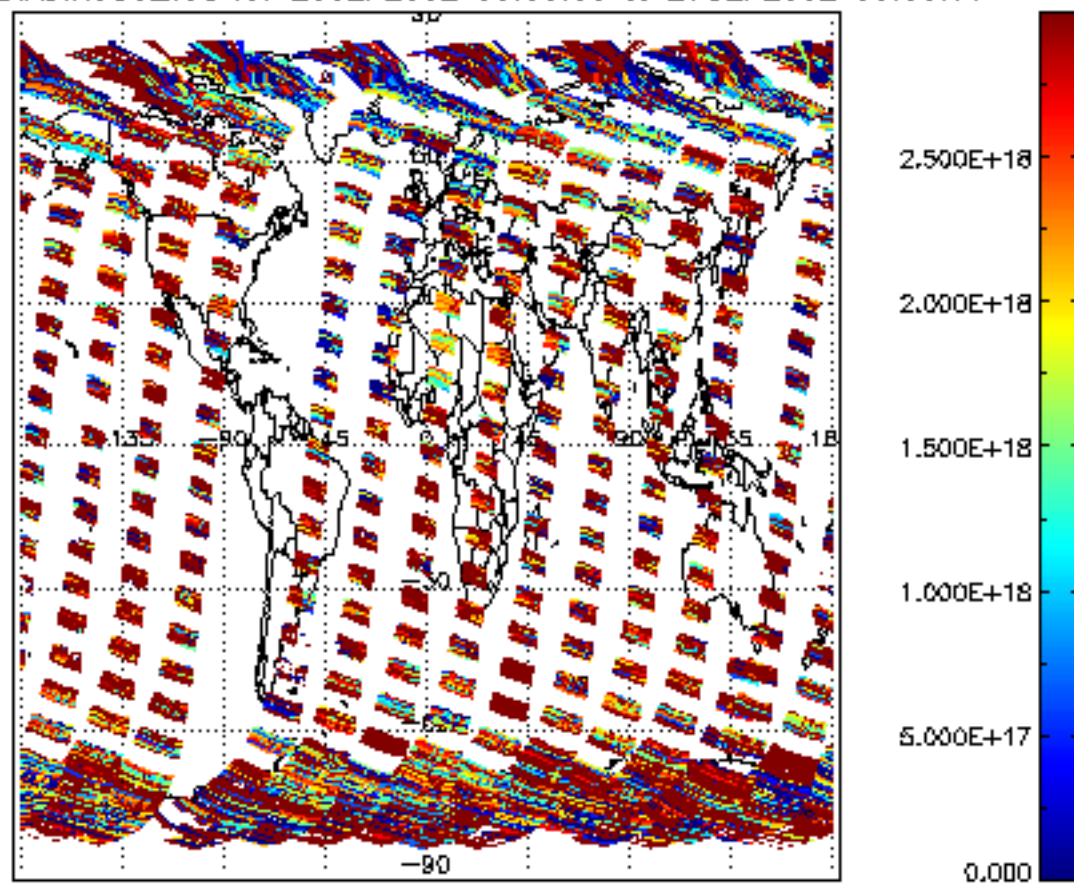
SCIOL2P_NADIR3CO_vcd for 26SEP2002 00:00:00 to 27SEP2002 00:00:00
