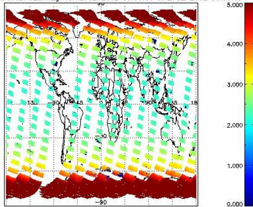
SCIOL2P_NADUV3BRO_amf_gr for 26SEP2002 00:00:00 to 27SEP2002 00:00:00
