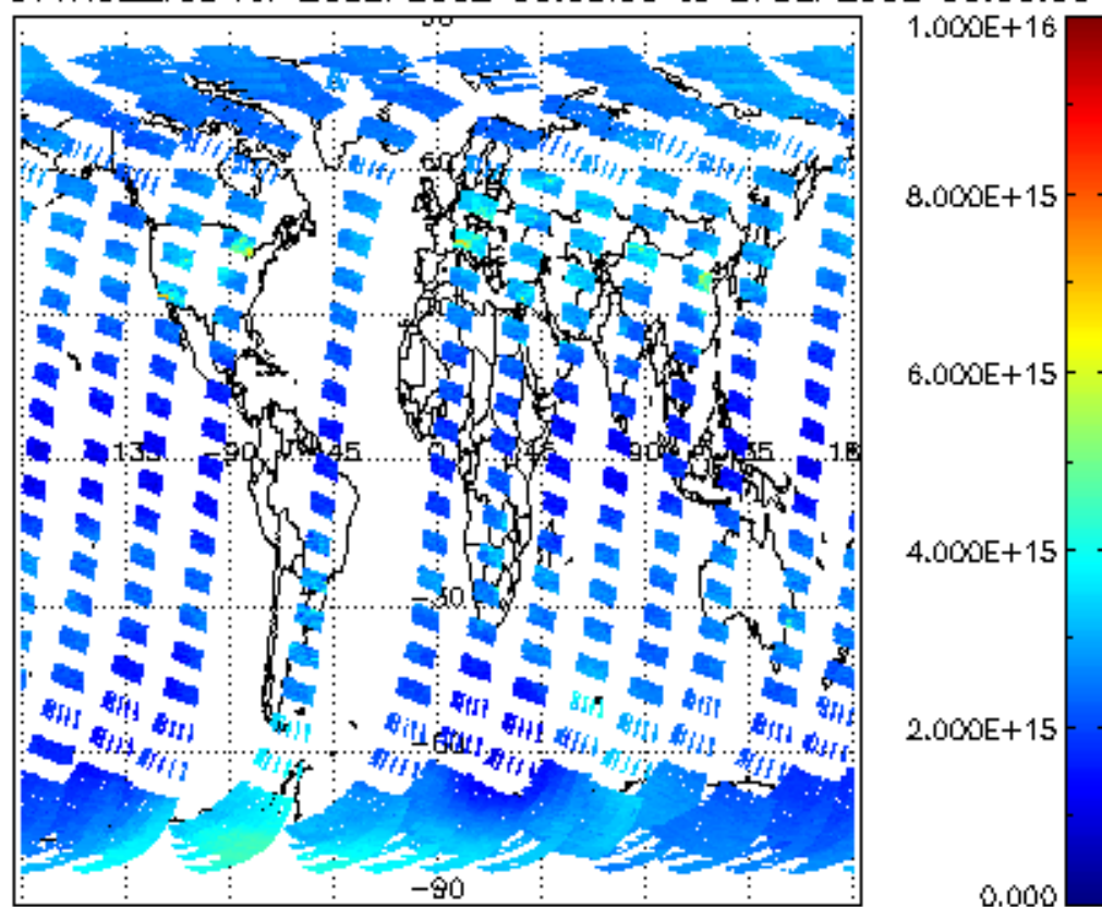
SCIOL2P_NADUV1NO2_vcd for 26SEP2002 00:00:00 to 27SEP2002 00:00:00
