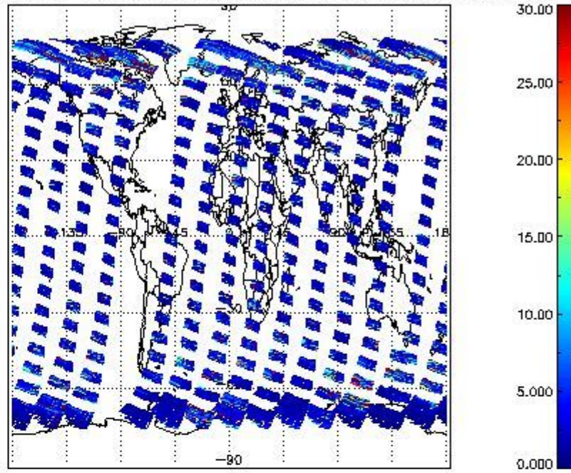
SCIOL2P_NADUV5S02_vcd_err for 26SEP2002 00:00:00 to 27SEP2002 00:00:00
