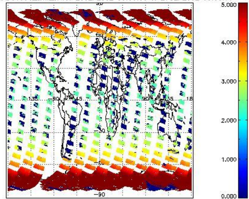
SCIOL2P_NADUV003_amf_cl for 26SEP2002 00:00:00 to 27SEP2002 00:00:00
