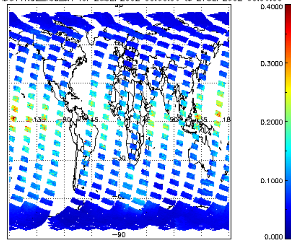
SCIOL2P_NADUV1N02_vcd_err for 26SEP2002 00:00:00 to 27SEP2002 00:00:00
