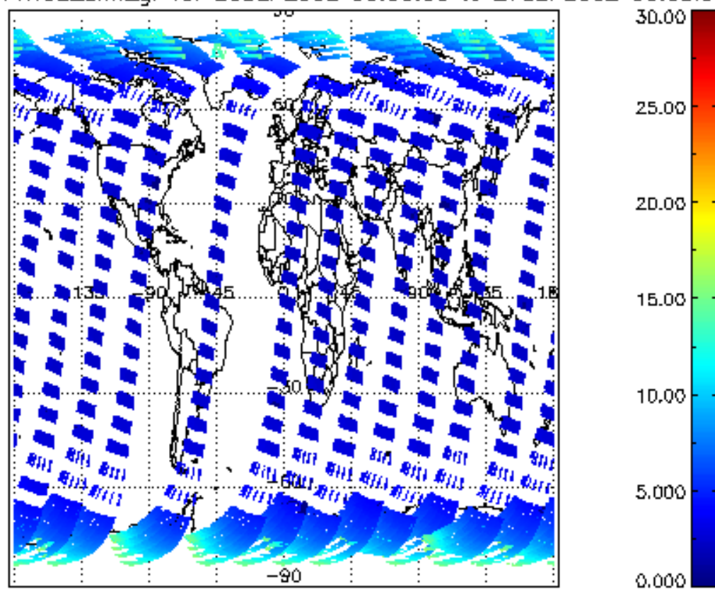
iCIOL2P_NADUV1NO2_amf_gr for 26SEP2002 00:00:00 to 27SEP2002 00:00:00
