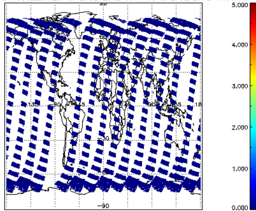
SCIOL2P_NADUV5S02_amf_cl for 26SEP2002 00:00:00 to 27SEP2002 00:00:00
