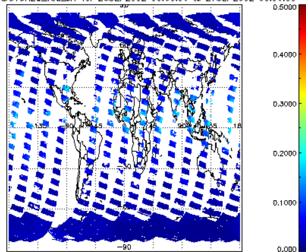
SCIOL2P_NADUV8H20_vcd_err for 26SEP2002 00:00:00 to 27SEP2002 00:00:00
