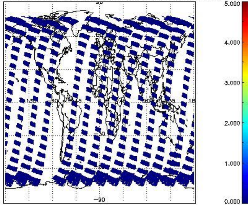
SCIOL2P_NADUV5S02_amf_cl for 26SEP2002 00:00:00 to 27SEP2002 00:00:00
