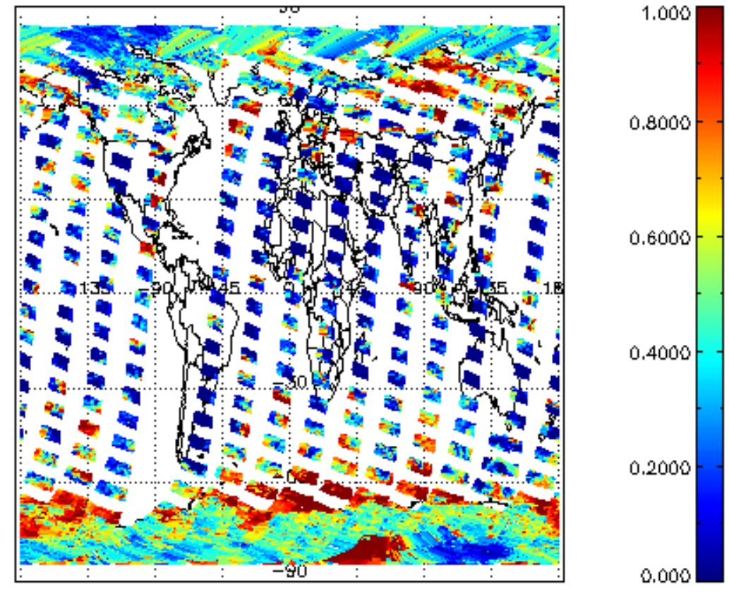
cl_frac for 26SEP2002 00:00:00 to 27SEP2002 00:00:00
