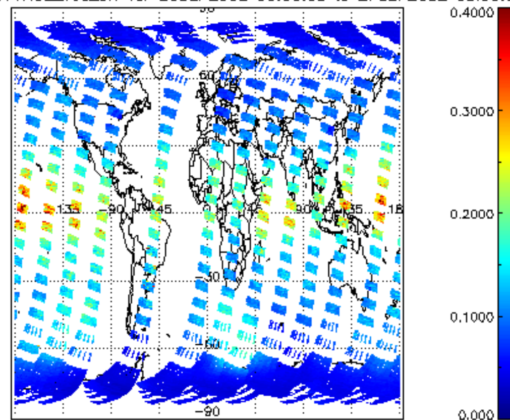
iCIOL2P_NADUV1NO2_vcd_err for 26SEP2002 00:00:00 to 27SEP2002 00:00:00
