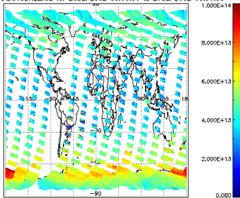
SCIOL2P_NADUV3BRO_vcd for 26SEP2002 00:00:00 to 27SEP2002 00:00:00
