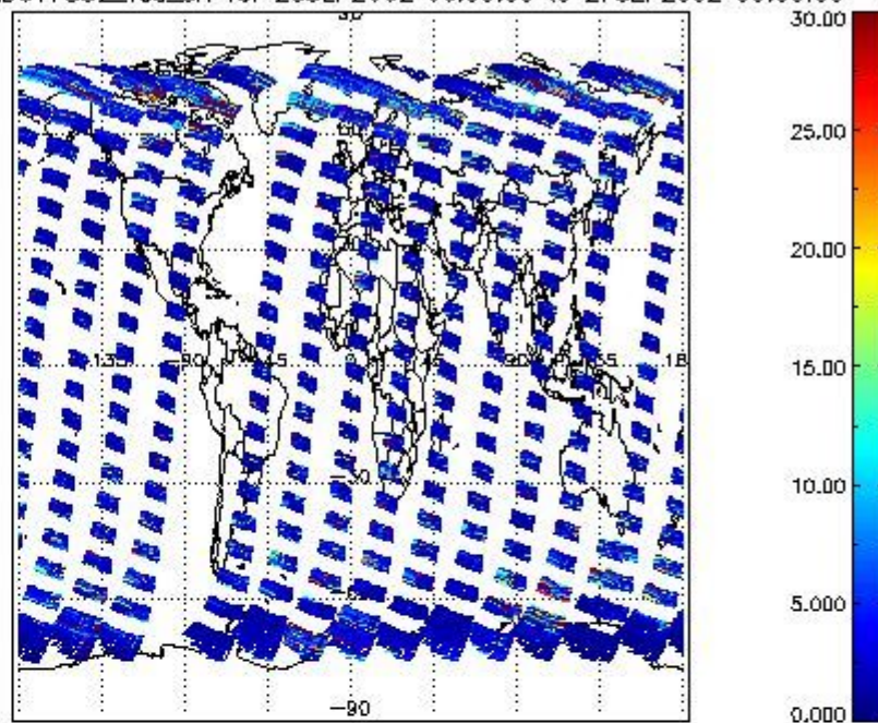
SCIOL2P_NADUV7S02_vcd_err for 26SEP2002 00:00:00 to 27SEP2002 00:00:00
