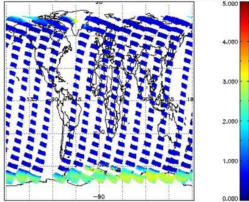
SCIOL2P_NADUV5S02_amf_gr for 26SEP2002 00:00:00 to 27SEP2002 00:00:00
