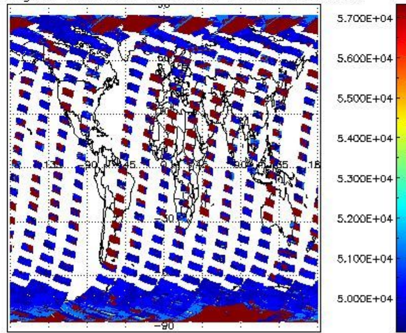
cloud_flags for 26SEP2002 00:00:00 to 27SEP2002 00:00:00
