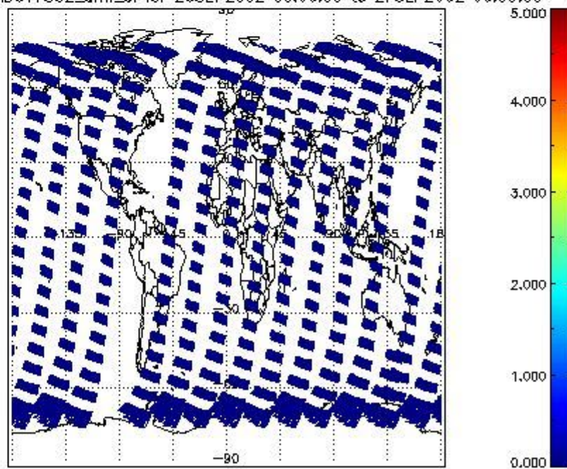
SCIOL2P_NADUV7S02_amf_cl for 26SEP2002 00:00:00 to 27SEP2002 00:00:00
