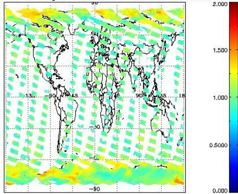
SCIOL2P_NADUV8H2O_arnf_gr for 26SEP2002 00:00:00 to 27SEP2002 00:00:00
