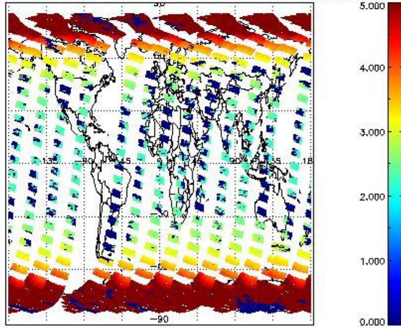
SCIOL2P_NADUV1N02_amf_cl for 26SEP2002 00:00:00 to 27SEP2002 00:00:00
