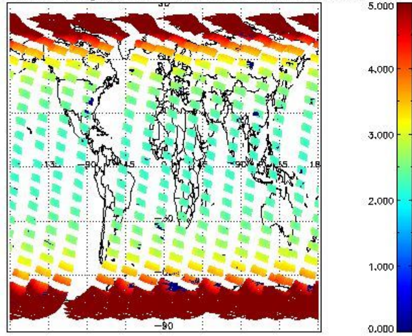
SCIOL2P_NADUV1N02_amf_gr for 26SEP2002 00:00:00 to 27SEP2002 00:00:00
