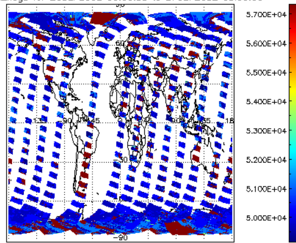
cloud_flags for 26SEP2002 00:00:00 to 27SEP2002 00:00:00
