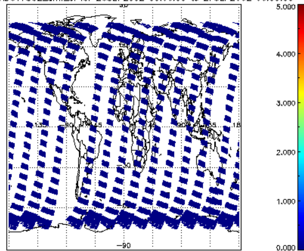
SCIOL2P_NADUV7S02_amf_cl for 26SEP2002 00:00:00 to 27SEP2002 00:00:00
