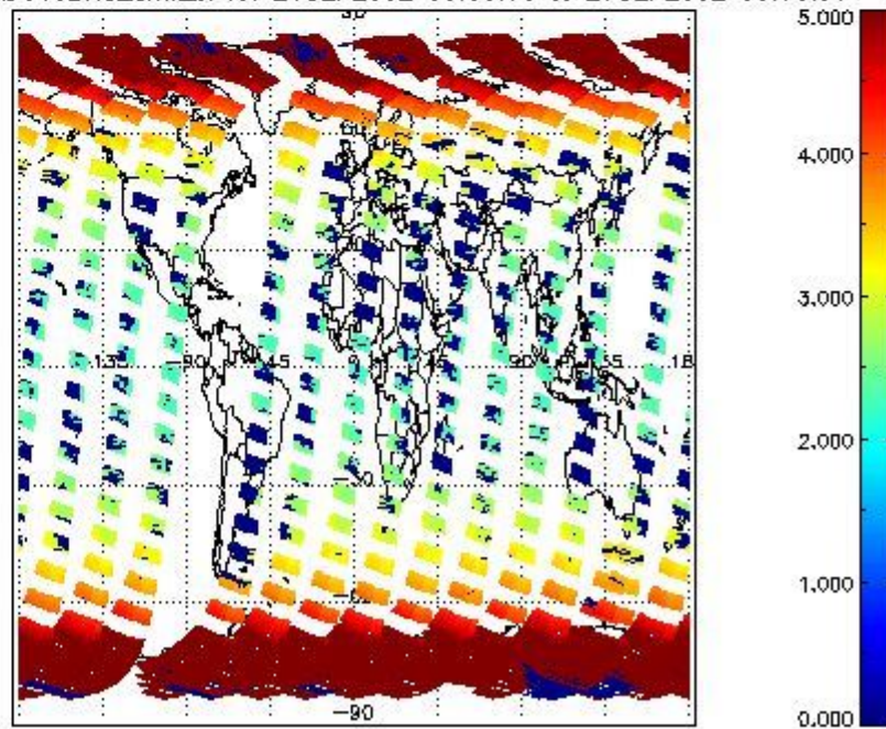
SCIOL2P_NADUV3BRO_amf_cl for 26SEP2002 00:00:00 to 27SEP2002 00:00:00
