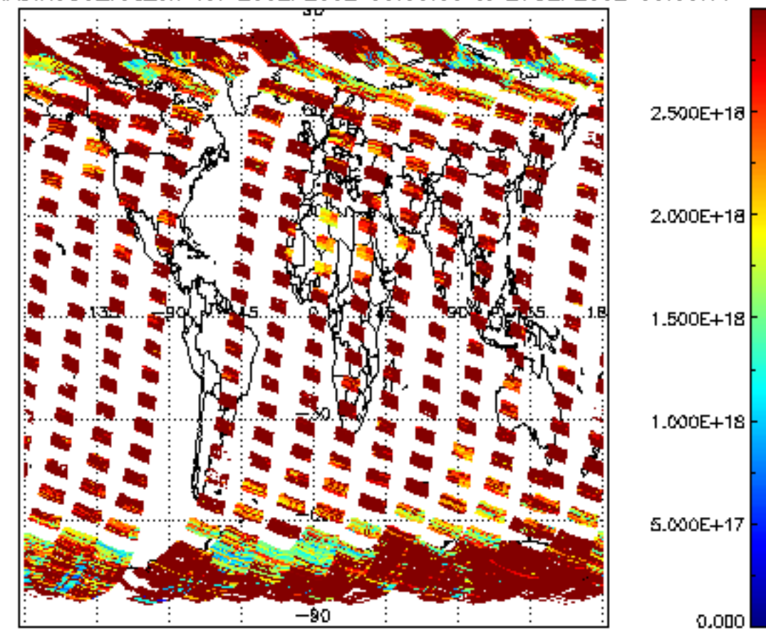
SCIOL2P_NADIR3CO_vcd_err for 26SEP2002 00:00:00 to 27SEP2002 00:00:00
