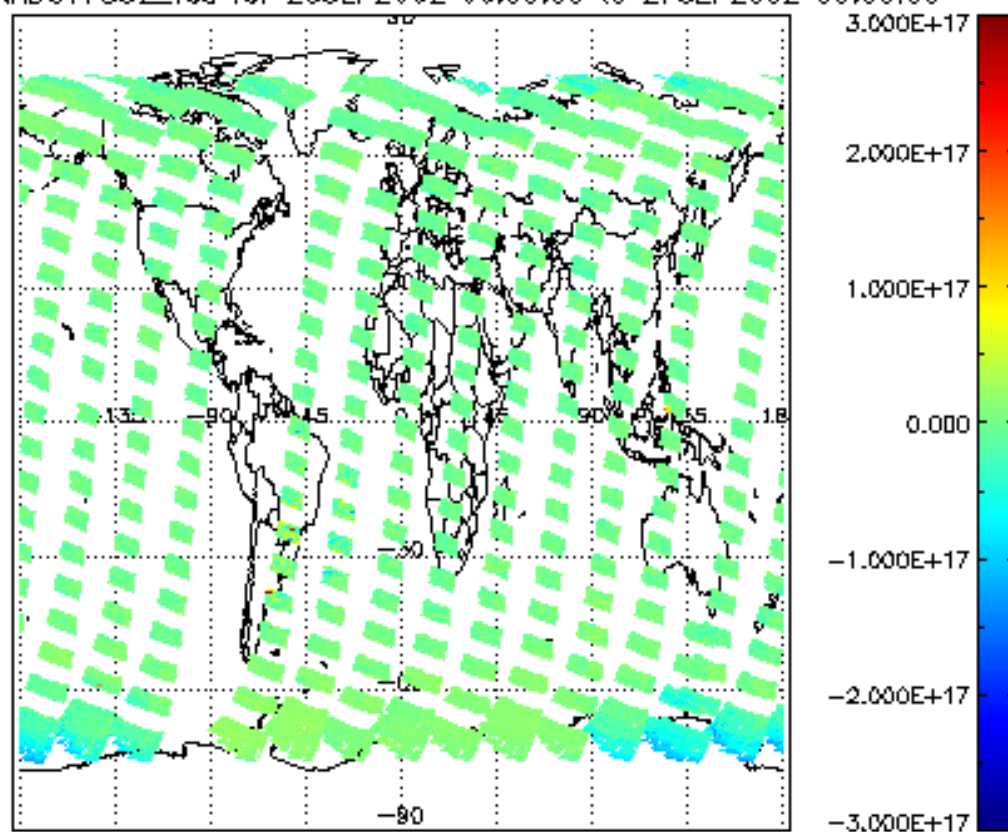
SCIOL2P_NADUV7S02_vcd for 26SEP2002 00:00:00 to 27SEP2002 00:00:00
