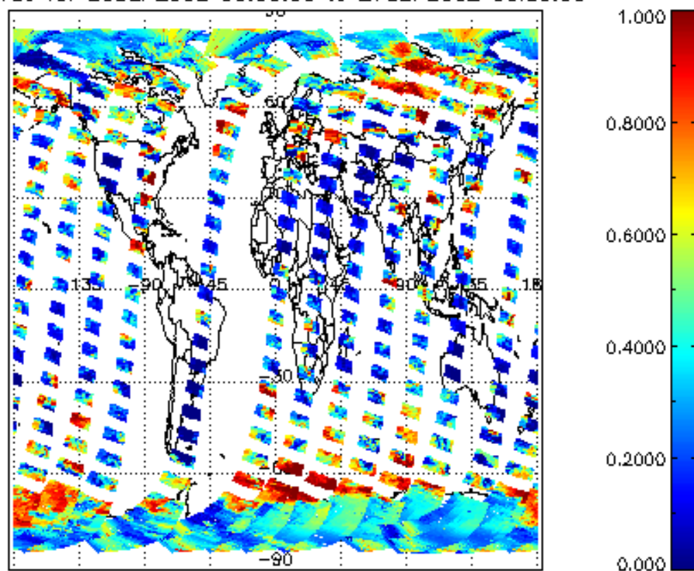
cl_frac for 26SEP2002 00:00:00 to 27SEP2002 00:00:00
