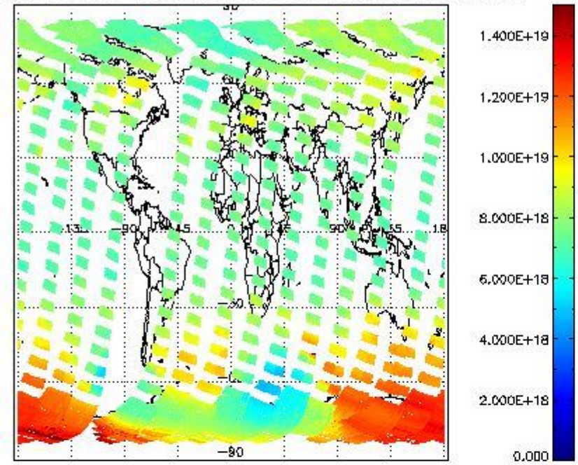
SCIOL2P_NADUV003_vcd for 26SEP2002 00:00:00 to 27SEP2002 00:00:00
