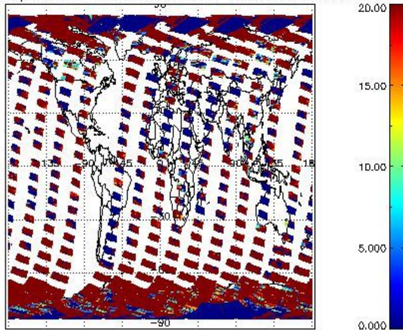
cL_opt_depth for 26SEP2002 00:00:00 to 27SEP2002 00:00:00
