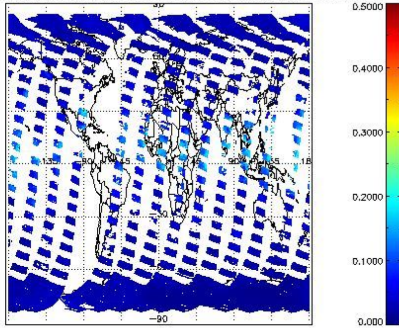
SCIOL2P_NADUV8H2O_vcd_err for 26SEP2002 00:00:00 to 27SEP2002 00:00:00
