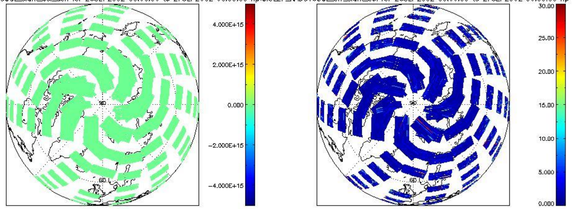
CIOL2P_NADUV60CLslant_col_den for 26SEP2002 00:00:00 to 27SEP2002 00:00:00 np; CIOL2P_NADUV60CLerr_slant_col for 26SEP2002 00:00:00 to 27SEP2002 00:00:00 np
