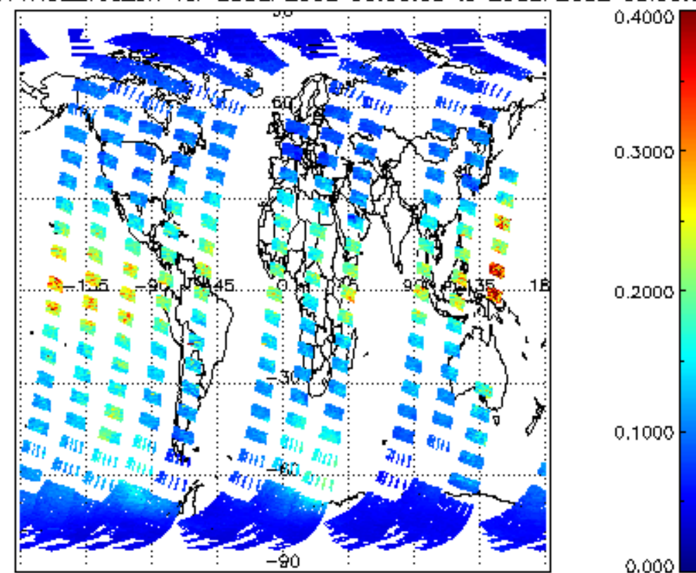
iCIOL2P_NADUV1NO2_vcd_err for 25SEP2002 00:00:00 to 26SEP2002 00:00:00
