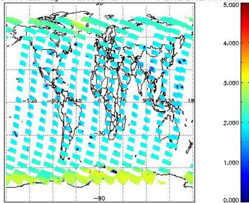
SCIOL2P_NADUV7S02_amf_gr for 25SEP2002 00:00:00 to 26SEP2002 00:00:00
