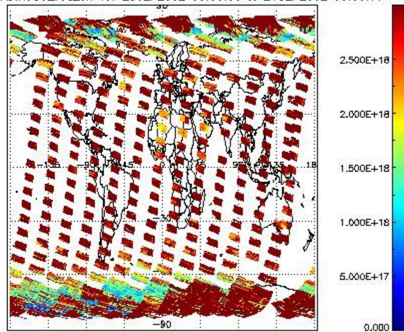
SCIO2P_NADIR3CO_vcd_err for 25SEP2002 00:00:00 to 26SEP2002 00:00:00
