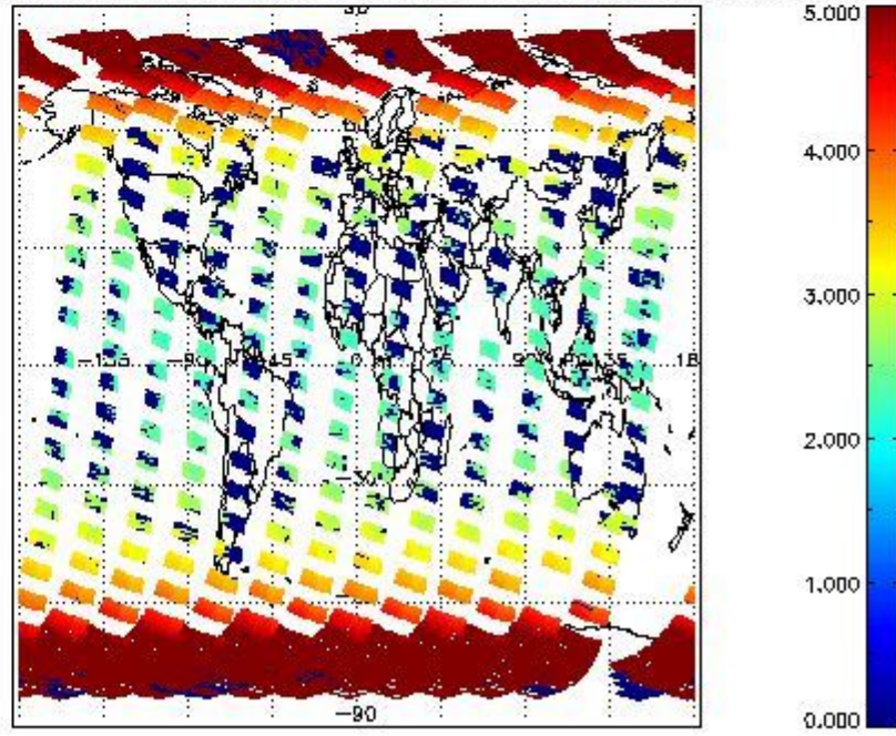
SCIOL2P_NADUV3BRO_amf_cl for 25SEP2002 00:00:00 to 26SEP2002 00:00:00
