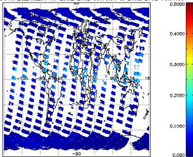
SCIOL2P_NADUV8H2O_vcd_err for 25SEP2002 00:00:00 to 26SEP2002 00:00:00
