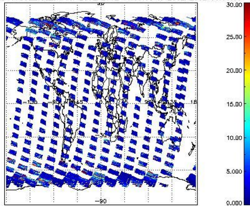
SCIOL2P_NADUV7S02_vcd_err for 25SEP2002 00:00:00 to 26SEP2002 00:00:00
