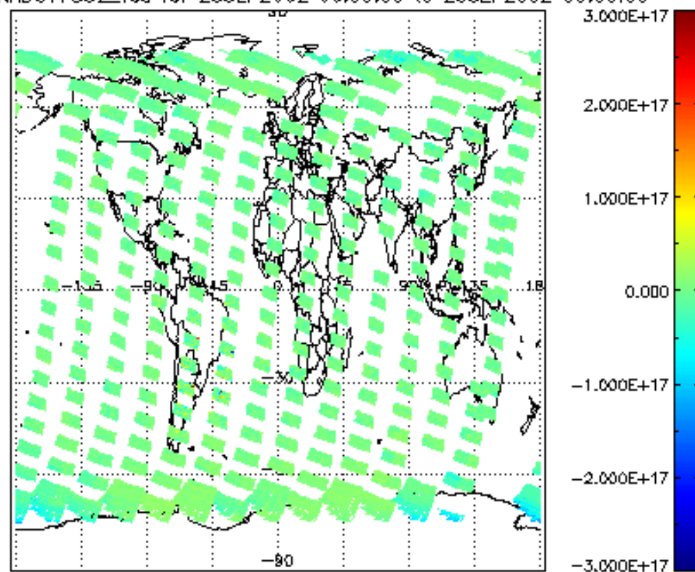
SCIOL2P_NADUV7S02_vcd for 25SEP2002 00:00:00 to 26SEP2002 00:00:00
