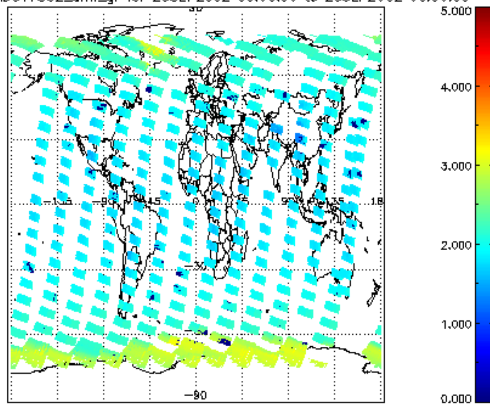
SCIOL2P_NADUV7S02_amf_gr for 25SEP2002 00:00:00 to 26SEP2002 00:00:00
