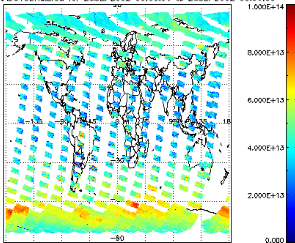
SCIOL2P_NADUV3BRO_vcd for 25SEP2002 00:00:00 to 26SEP2002 00:00:00
