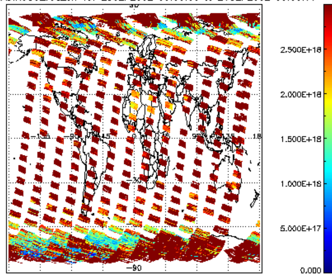
SCIOL2P_NADIR3CO_vcd_err for 25SEP2002 00:00:00 to 26SEP2002 00:00:00
