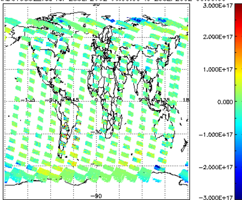
SCIOL2P_NADUV5S02_vcd for 25SEP2002 00:00:00 to 26SEP2002 00:00:00
