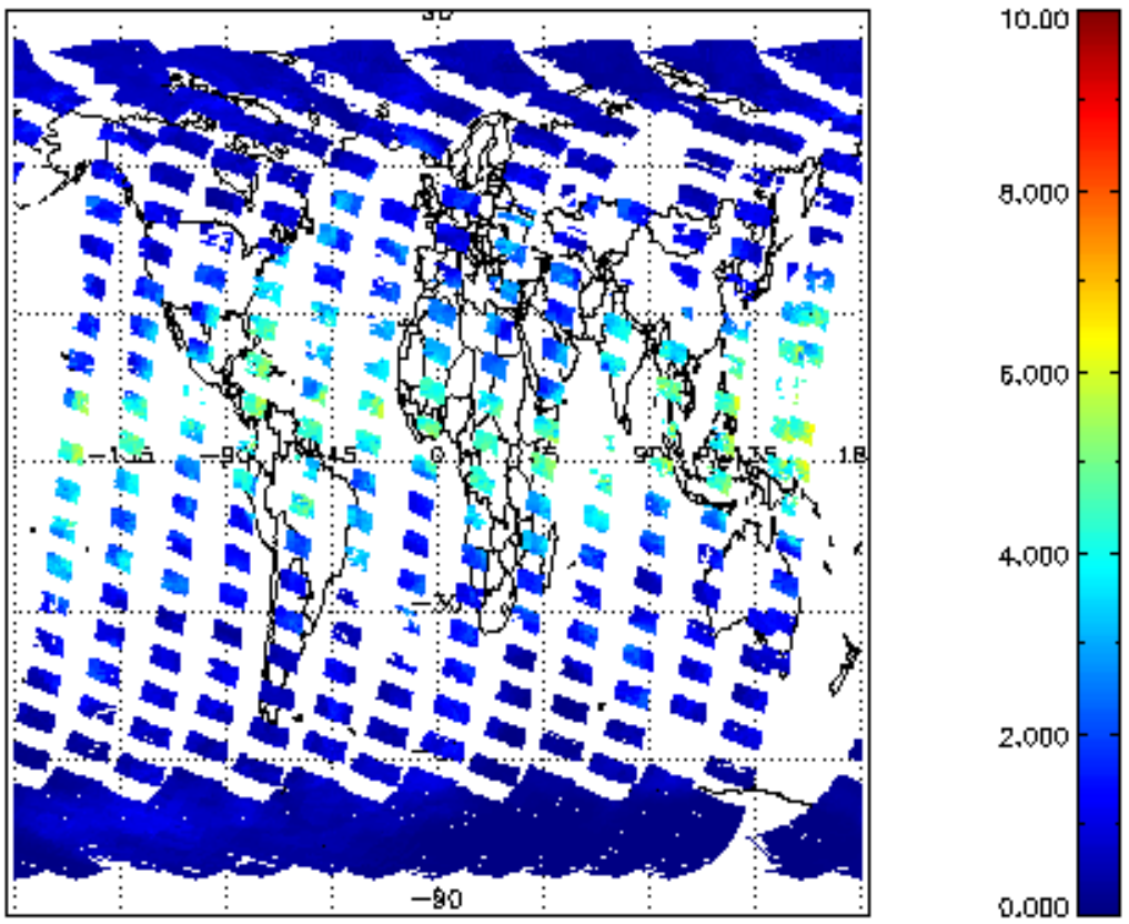
SCIOL2P_NADUV8H20_vcd for 25SEP2002 00:00:00 to 26SEP2002 00:00:00
