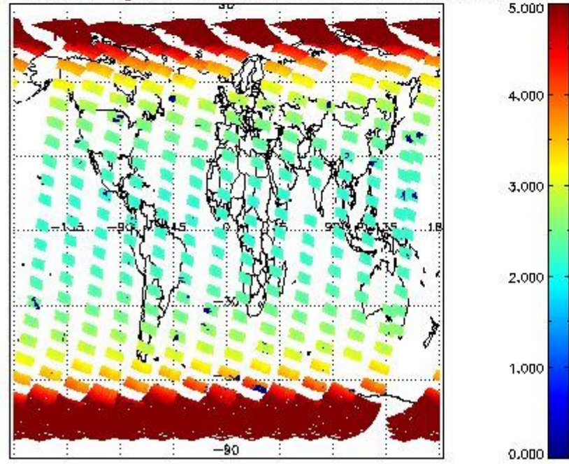
SCIOL2P_NADUV3BRO_amf_gr for 25SEP2002 00:00:00 to 26SEP2002 00:00:00
