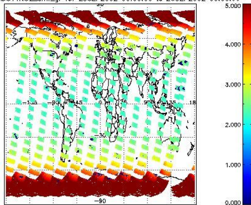
SCIOL2P_NADUV1NO2_amf_gr for 25SEP2002 00:00:00 to 26SEP2002 00:00:00
