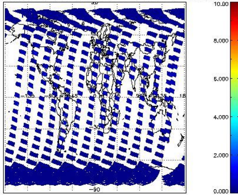
SCIOL2P_NADUV3BRO_vcd_err for 25SEP2002 00:00:00 to 26SEP2002 00:00:00
