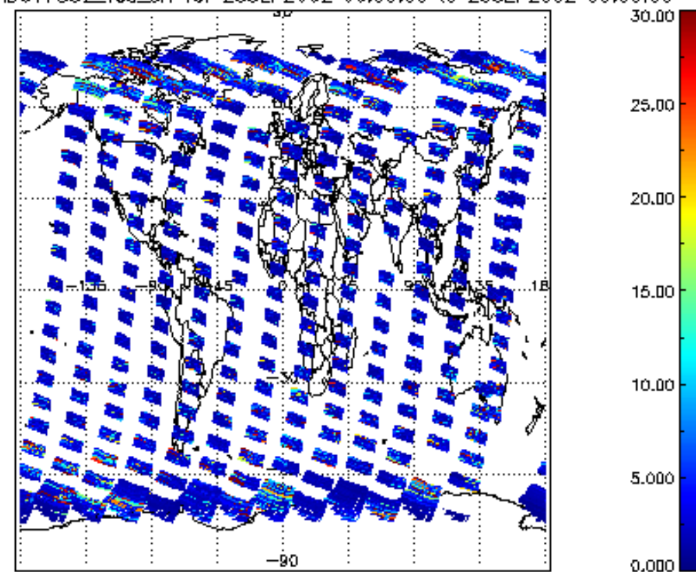
SCIOL2P_NADUV7S02_vcd_err for 25SEP2002 00:00:00 to 26SEP2002 00:00:00
