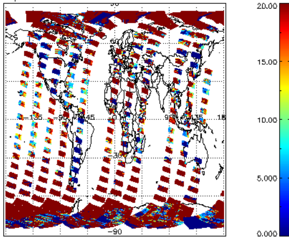
cl_opt_depth for 25SEP2002 00:00:00 to 26SEP2002 00:00:00
