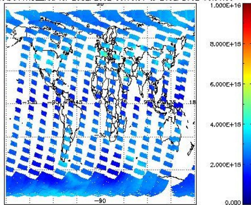
SCIOL2P_NADUV1NO2_vcd for 25SEP2002 00:00:00 to 26SEP2002 00:00:00
