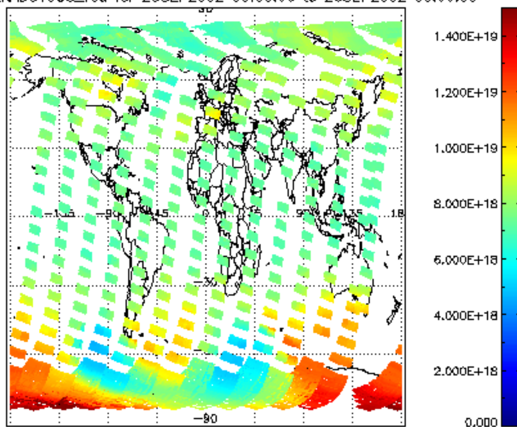
SCIOL2P_NADUV003_vcd for 25SEP2002 00:00:00 to 26SEP2002 00:00:00
