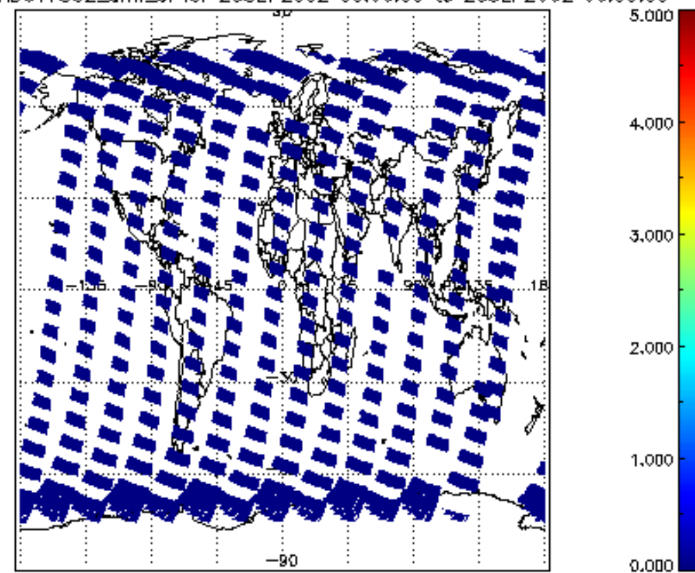
SCIOL2P_NADUV7S02_amf_cl for 25SEP2002 00:00:00 to 26SEP2002 00:00:00
