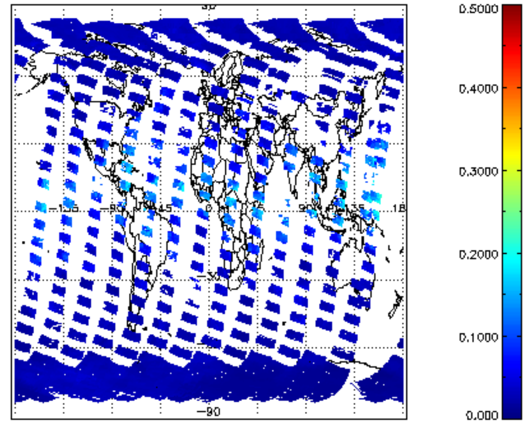
SCIOL2P_NADUV8H20_vcd_err for 25SEP2002 00:00:00 to 26SEP2002 00:00:00
