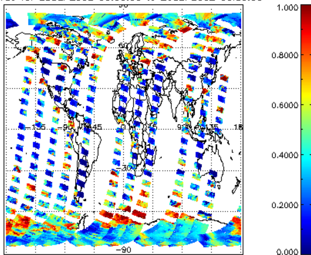
cl_frac for 25SEP2002 00:00:00 to 26SEP2002 00:00:00
