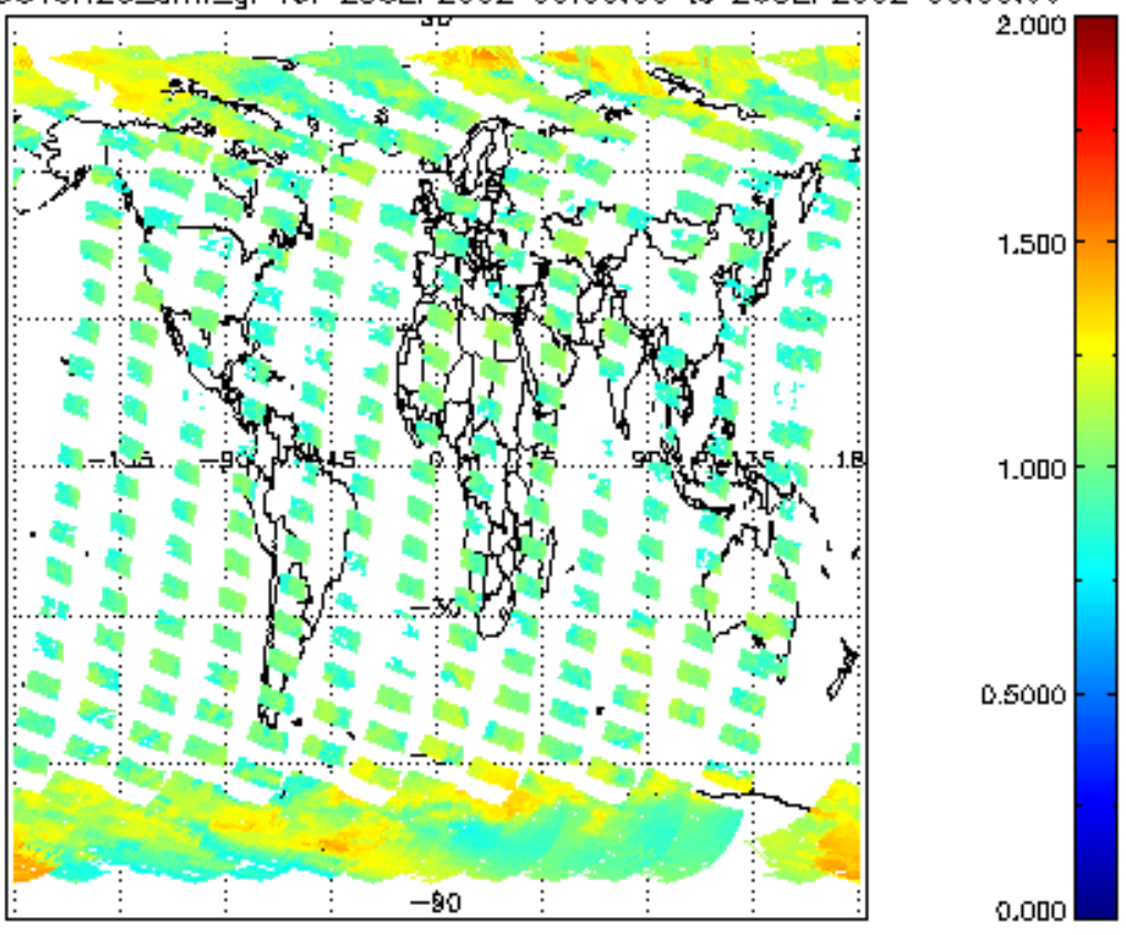
SCIOL2P_NADUV8H20_amf_gr for 25SEP2002 00:00:00 to 26SEP2002 00:00:00
