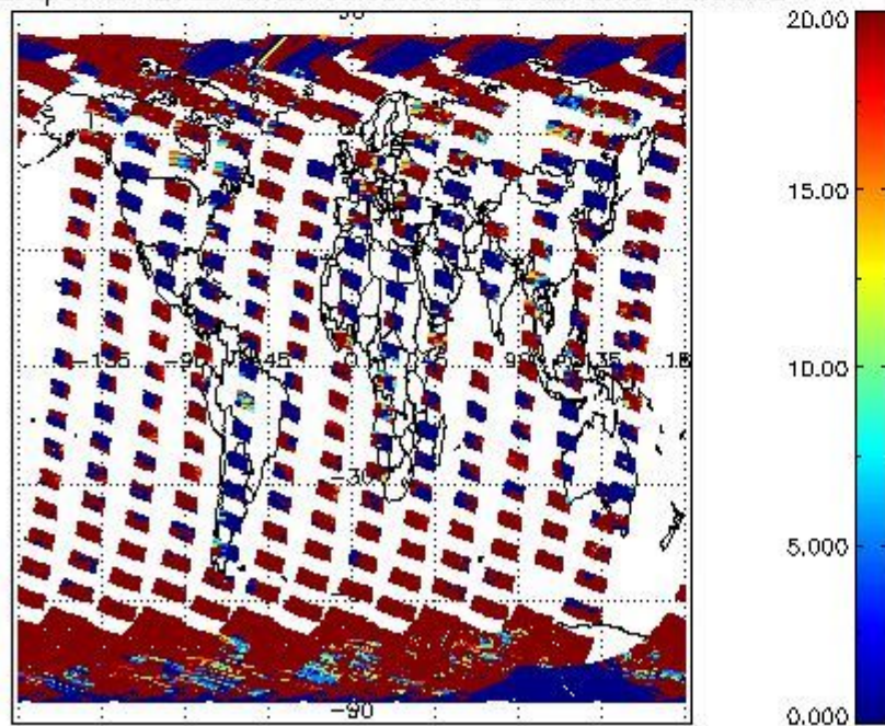
cL_opt_depth for 25SEP2002 00:00:00 to 26SEP2002 00:00:00
