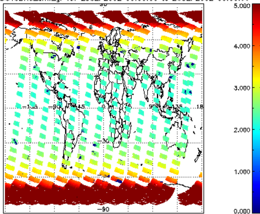
SCIOL2P_NADUV3BRO_amf_gr for 25SEP2002 00:00:00 to 26SEP2002 00:00:00
