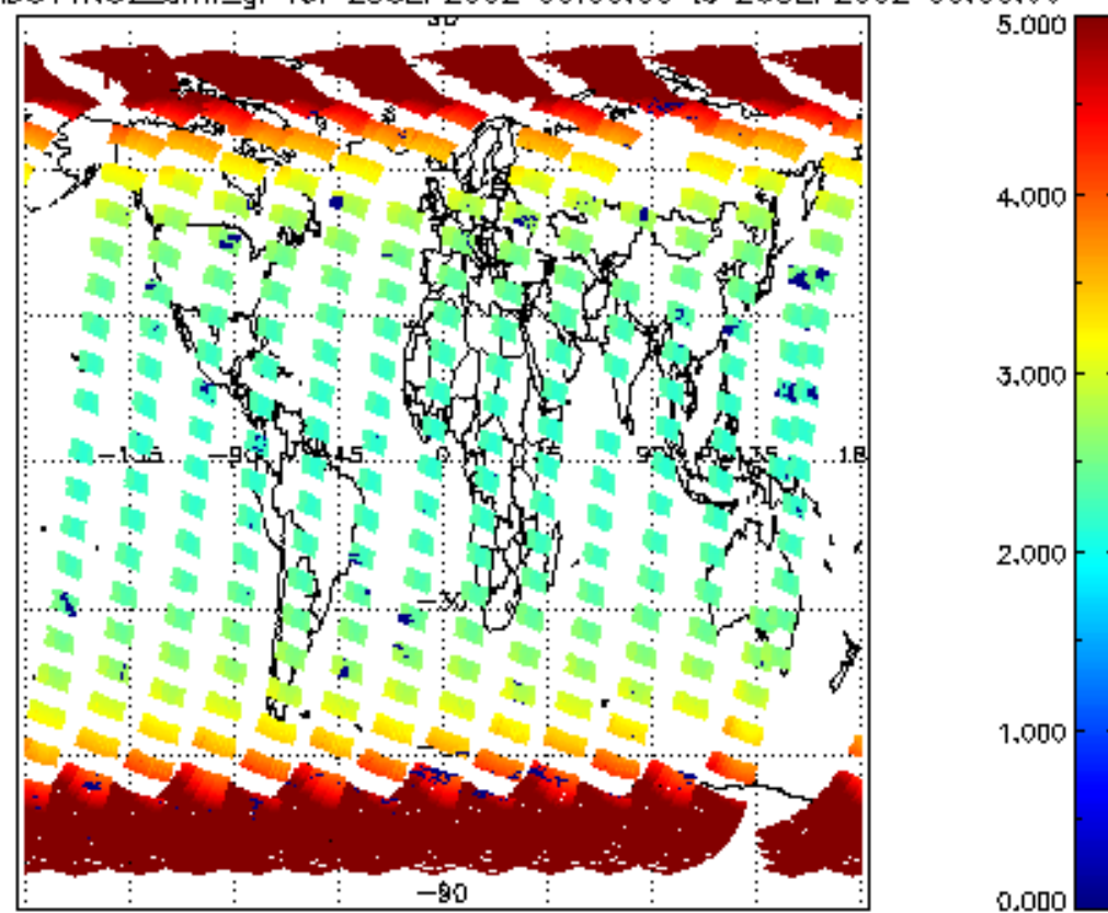
SCIOL2P_NADUV1NO2_amf_gr for 25SEP2002 00:00:00 to 26SEP2002 00:00:00
