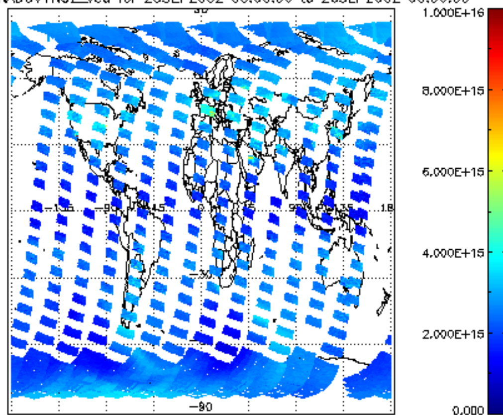
SCIOL2P_NADUV1NO2_vcd for 25SEP2002 00:00:00 to 26SEP2002 00:00:00
