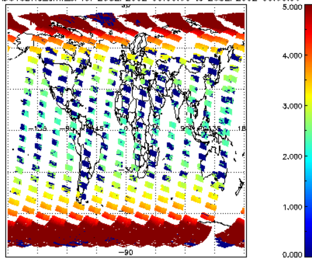
SCIOL2P_NADUV3BRO_amf_cl for 25SEP2002 00:00:00 to 26SEP2002 00:00:00
