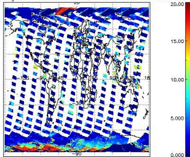
cL_top_height for 25SEP2002 00:00:00 to 26SEP2002 00:00:00
