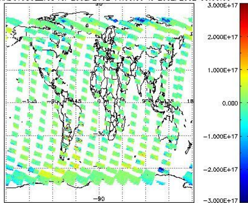
SCIOL2P_NADUV5S02_vcd for 25SEP2002 00:00:00 to 26SEP2002 00:00:00
