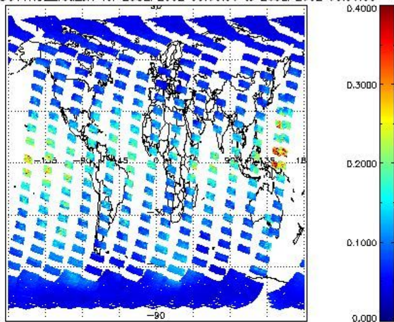
SCIOL2P_NADUV1NO2_vcd_err for 25SEP2002 00:00:00 to 26SEP2002 00:00:00
