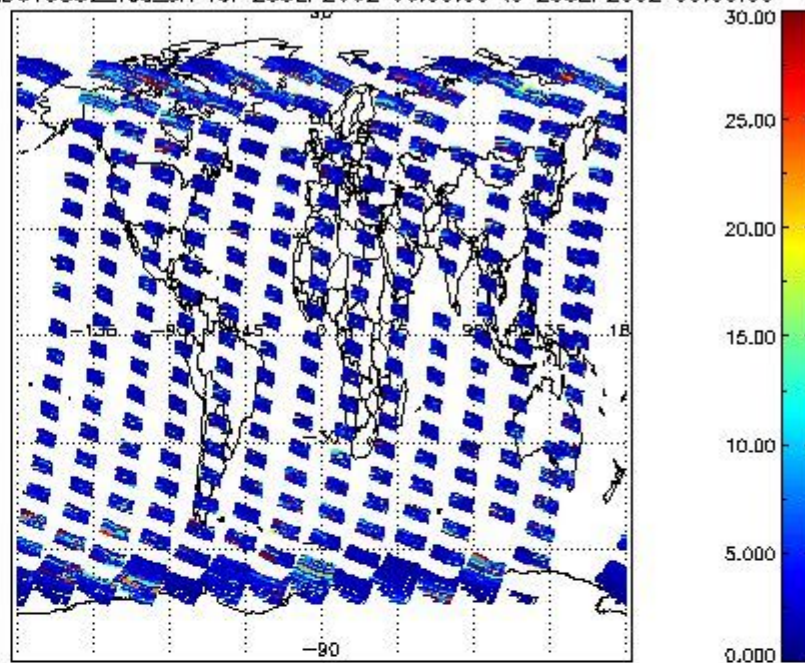
SCIOL2P_NADUV5S02_vcd_err for 25SEP2002 00:00:00 to 26SEP2002 00:00:00
