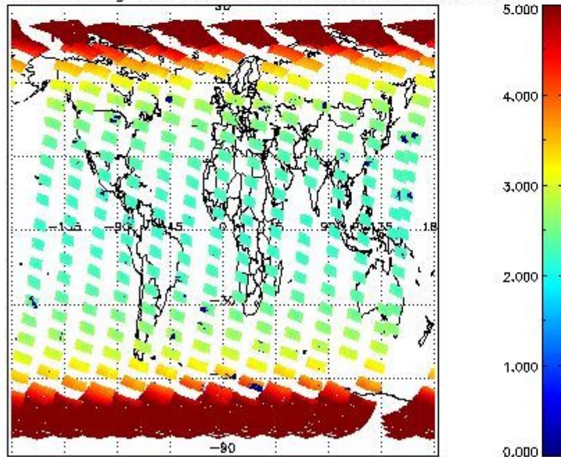
SCIOL2P_NADUV003_amf_gr for 25SEP2002 00:00:00 to 26SEP2002 00:00:00
