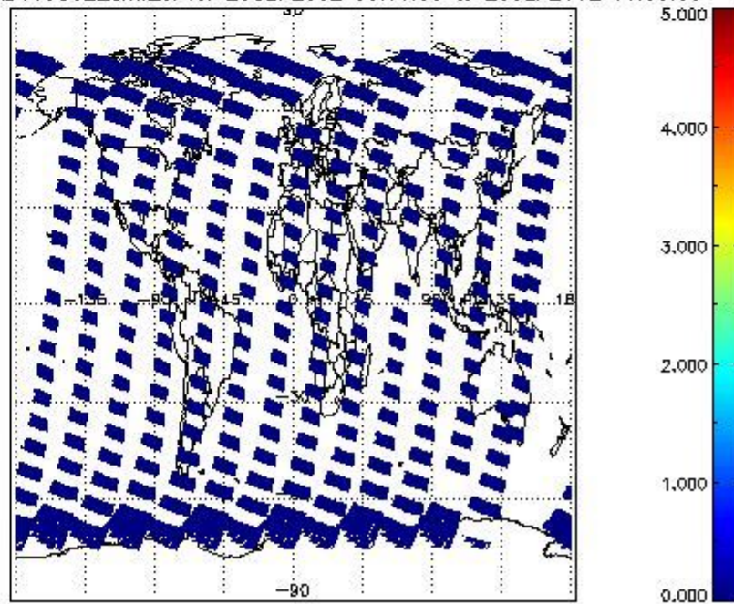
SCIOL2P_NADUV5S02_amf_cl for 25SEP2002 00:00:00 to 26SEP2002 00:00:00
