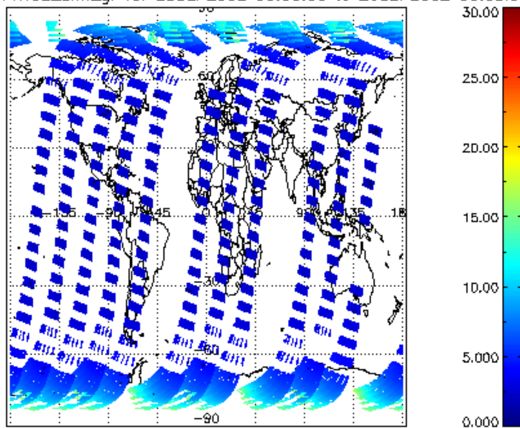
iCIOL2P_NADUV1NO2_amf_gr for 25SEP2002 00:00:00 to 26SEP2002 00:00:00
