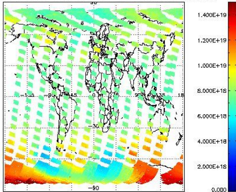
SCIOL2P_NADUV003_vcd for 25SEP2002 00:00:00 to 26SEP2002 00:00:00
