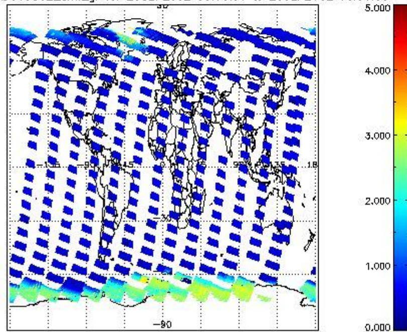
SCIOL2P_NADUV5S02_amf_gr for 25SEP2002 00:00:00 to 26SEP2002 00:00:00
