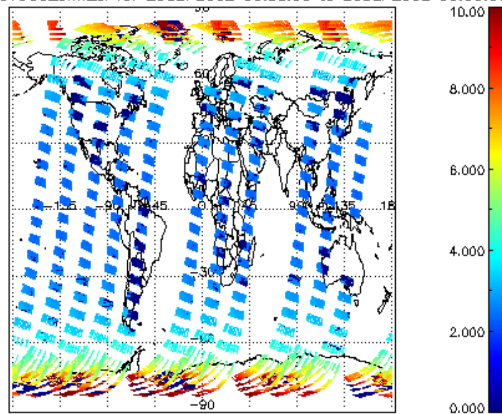
SCIOL2P_NADUV003_amf_cl for 25SEP2002 00:00:00 to 26SEP2002 00:00:00
