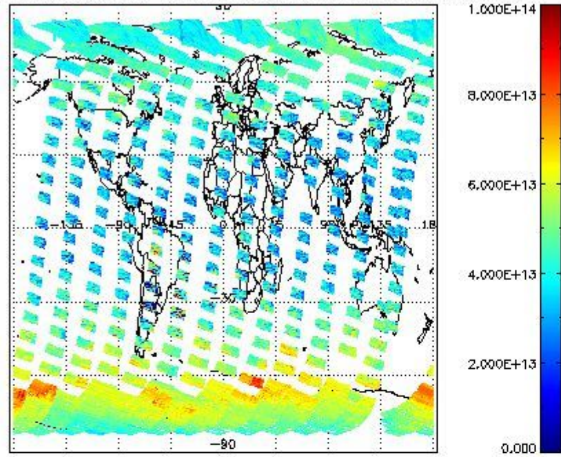
SCIOL2P_NADUV3BRO_vcd for 25SEP2002 00:00:00 to 26SEP2002 00:00:00
