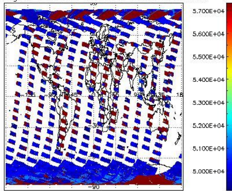
cloud_flags for 25SEP2002 00:00:00 to 26SEP2002 00:00:00
