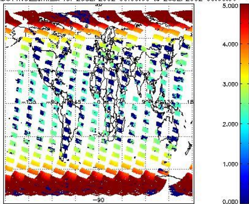
SCIOL2P_NADUV1NO2_amf_cl for 25SEP2002 00:00:00 to 26SEP2002 00:00:00
