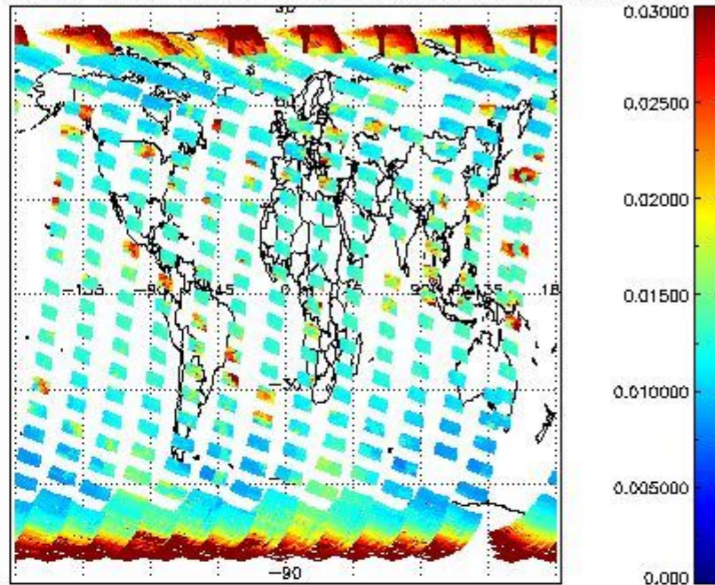
SCIOL2P_NADUV003_vcd_err for 25SEP2002 00:00:00 to 26SEP2002 00:00:00
