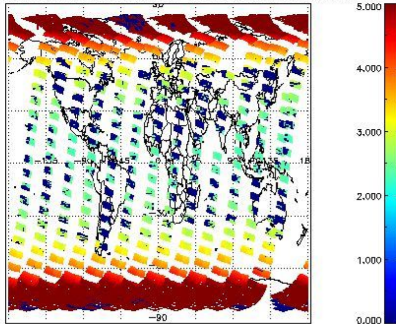
SCIOL2P_NADUV003_amf_cl for 25SEP2002 00:00:00 to 26SEP2002 00:00:00
