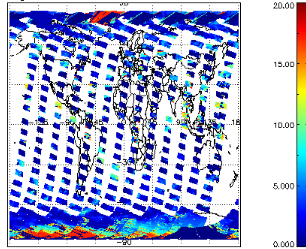
cl_top_height for 25SEP2002 00:00:00 to 26SEP2002 00:00:00
