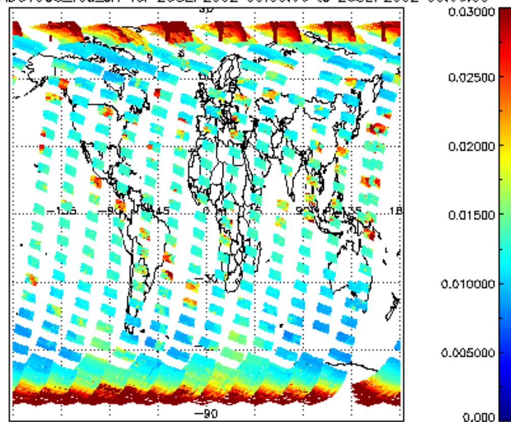
SCIOL2P_NADUV003_vcd_err for 25SEP2002 00:00:00 to 26SEP2002 00:00:00
