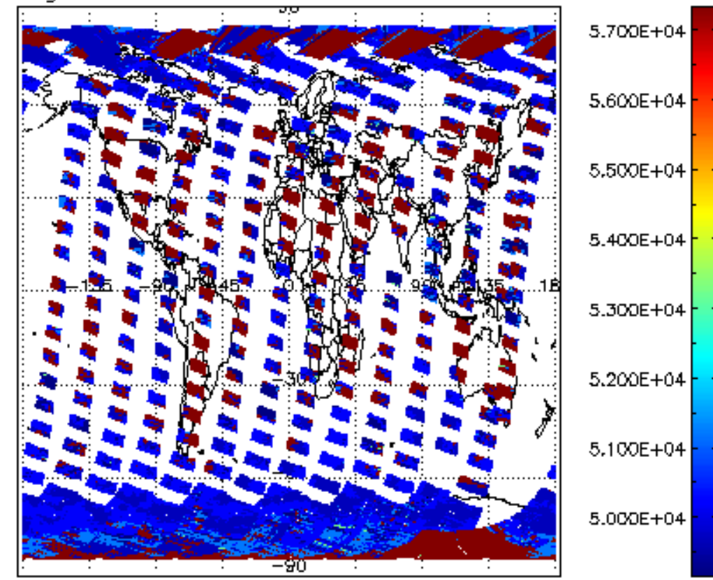
cloud_flags for 25SEP2002 00:00:00 to 26SEP2002 00:00:00
