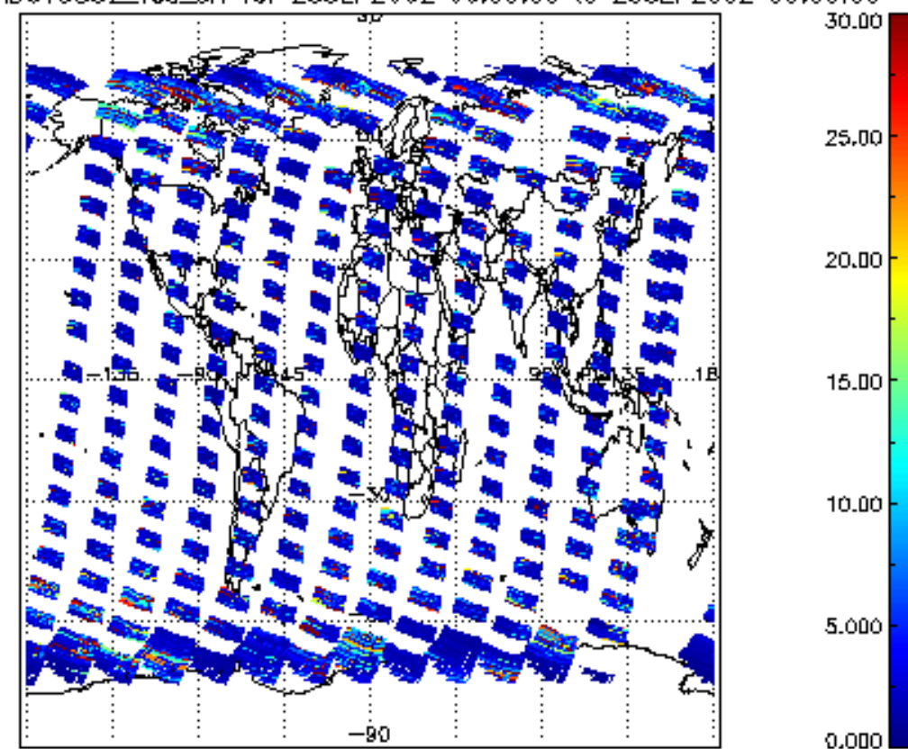
SCIOL2P_NADUV5S02_vcd_err for 25SEP2002 00:00:00 to 26SEP2002 00:00:00
