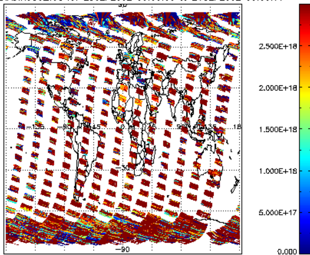
SCIOL2P_NADIR3CO_vcd for 25SEP2002 00:00:00 to 26SEP2002 00:00:00
