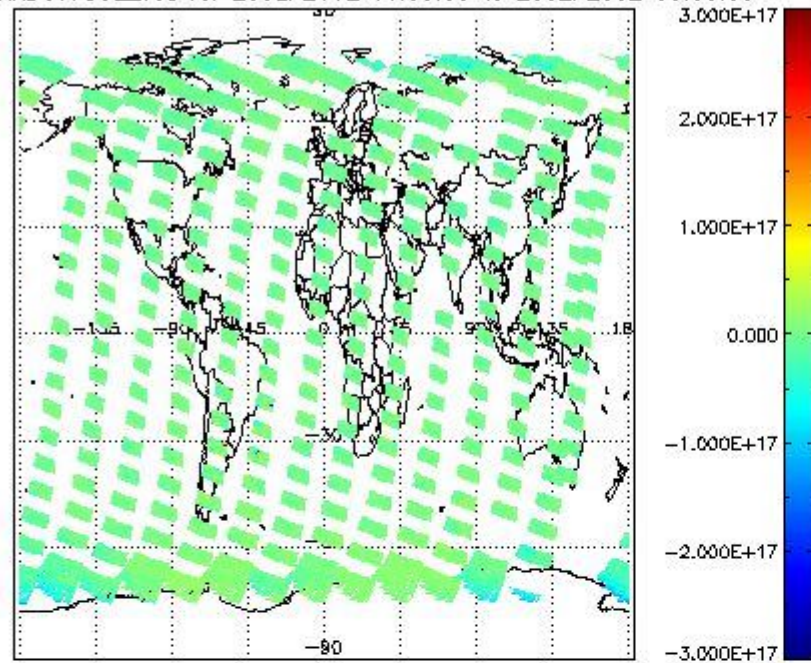
SCIOL2P_NADUV7S02_vcd for 25SEP2002 00:00:00 to 26SEP2002 00:00:00
