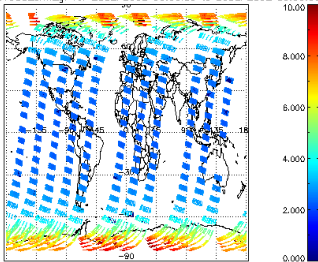
SCIOL2P_NADUV003_amf_gr for 25SEP2002 00:00:00 to 26SEP2002 00:00:00
