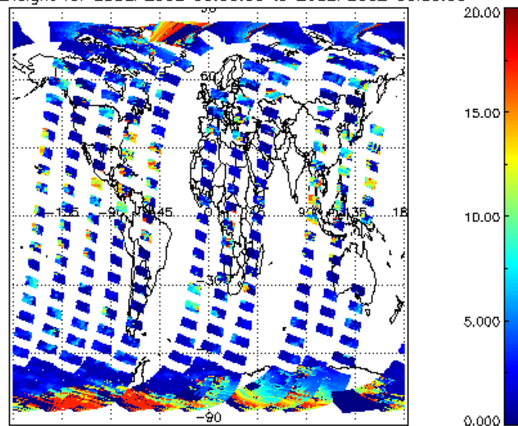
cl_top_height for 25SEP2002 00:00:00 to 26SEP2002 00:00:00
