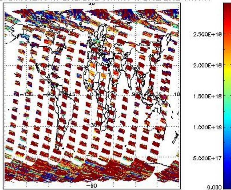
SCIO2P_NADIR3CO_vcd for 25SEP2002 00:00:00 to 26SEP2002 00:00:00
