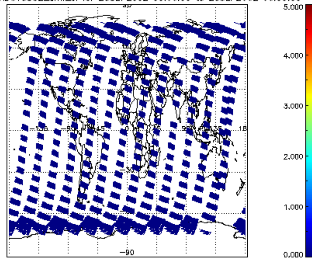
SCIOL2P_NADUV5S02_amf_cl for 25SEP2002 00:00:00 to 26SEP2002 00:00:00
