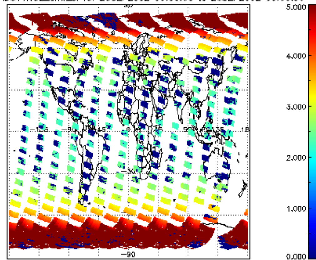
SCIOL2P_NADUV1NO2_amf_cl for 25SEP2002 00:00:00 to 26SEP2002 00:00:00
