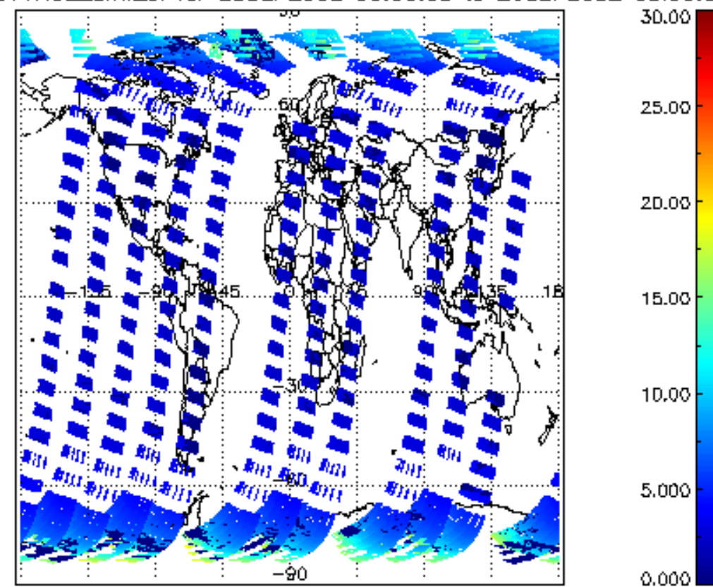
iCIOL2P_NADUV1NO2_amf_cl for 25SEP2002 00:00:00 to 26SEP2002 00:00:00
