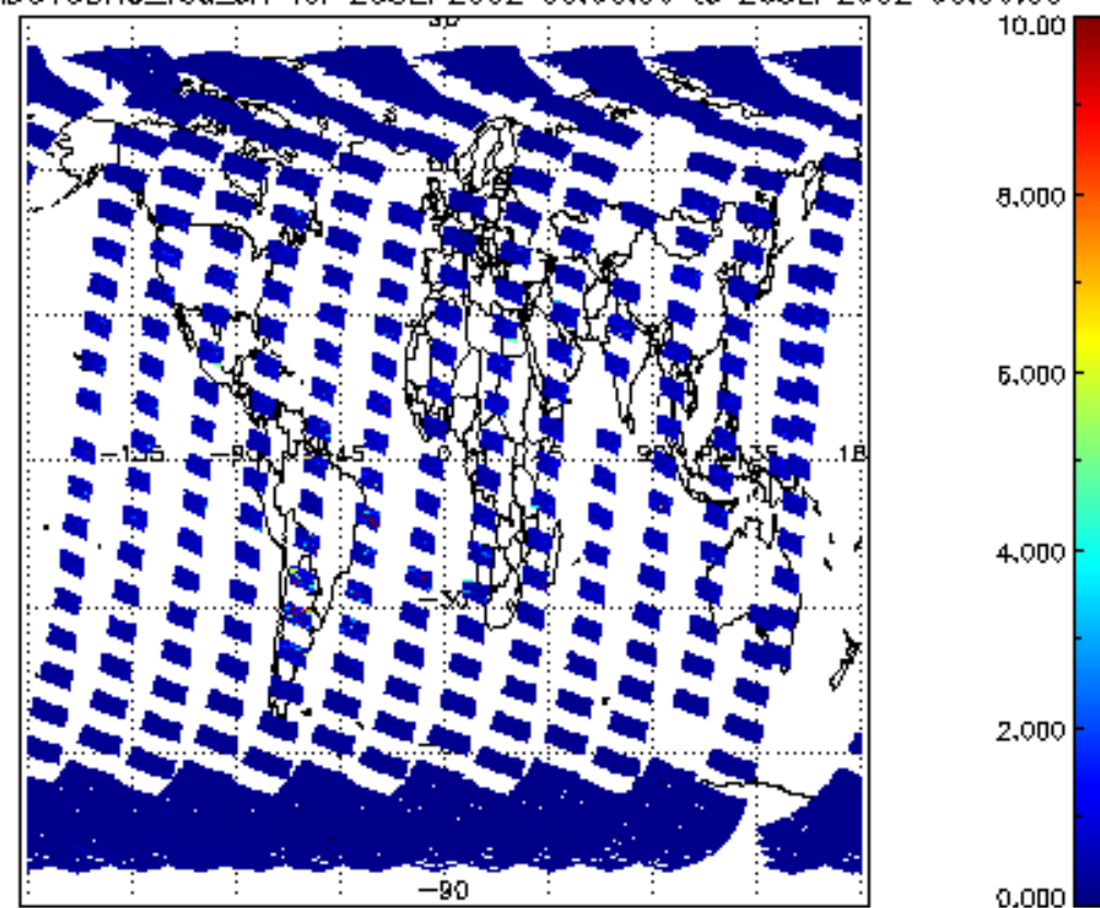
SCIOL2P_NADUV3BRO_vcd_err for 25SEP2002 00:00:00 to 26SEP2002 00:00:00
