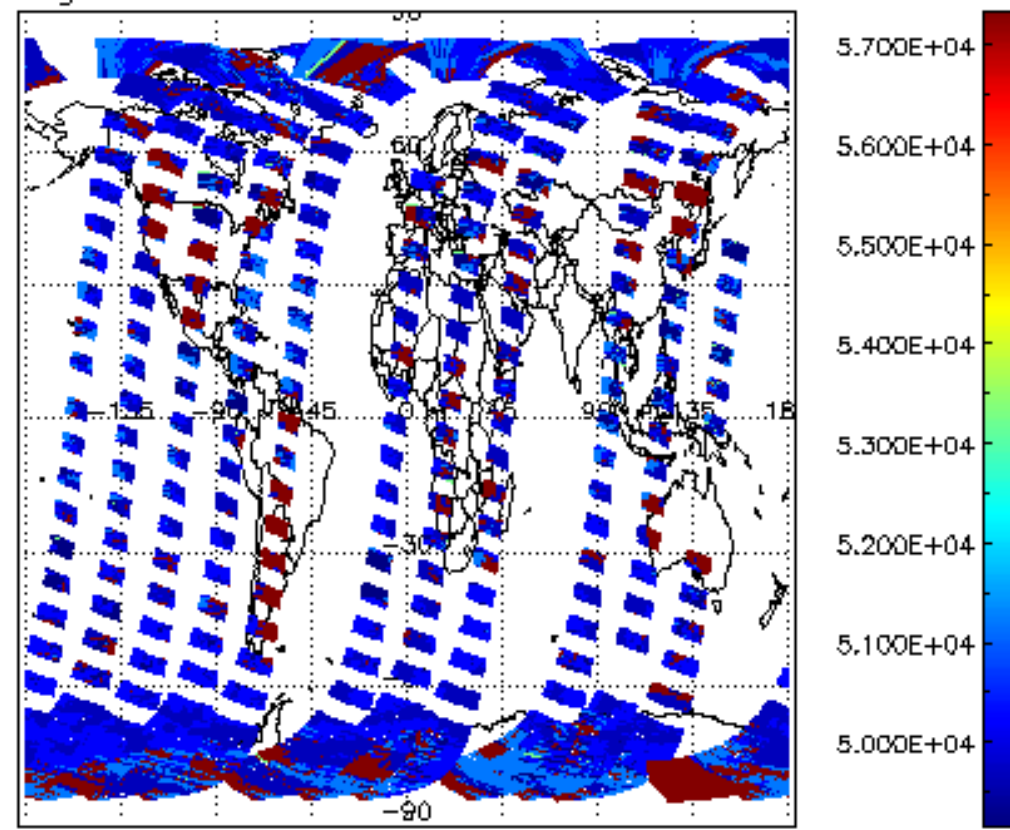
cloud_flags for 25SEP2002 00:00:00 to 26SEP2002 00:00:00
