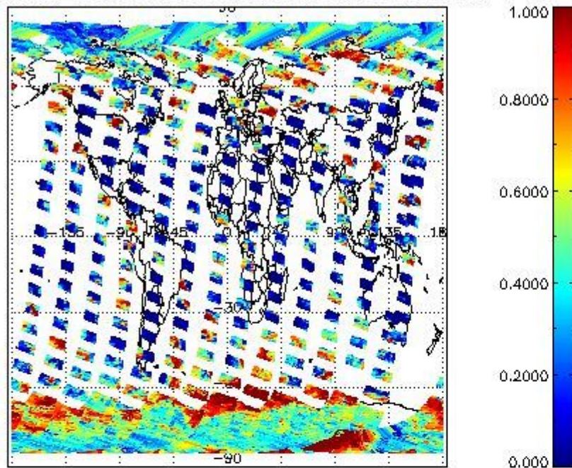
cL_frac for 25SEP2002 00:00:00 to 26SEP2002 00:00:00
