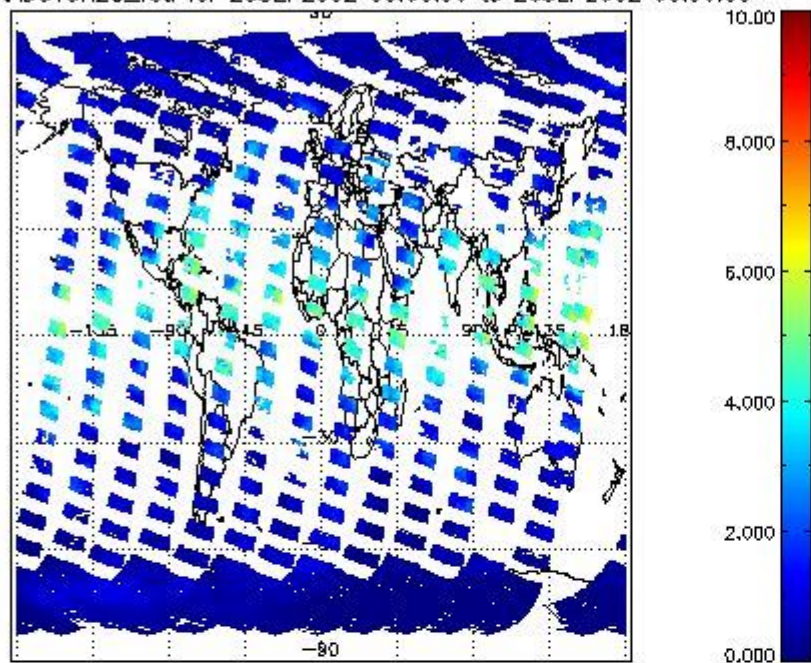
SCIOL2P_NADUV8H2O_vcd for 25SEP2002 00:00:00 to 26SEP2002 00:00:00
