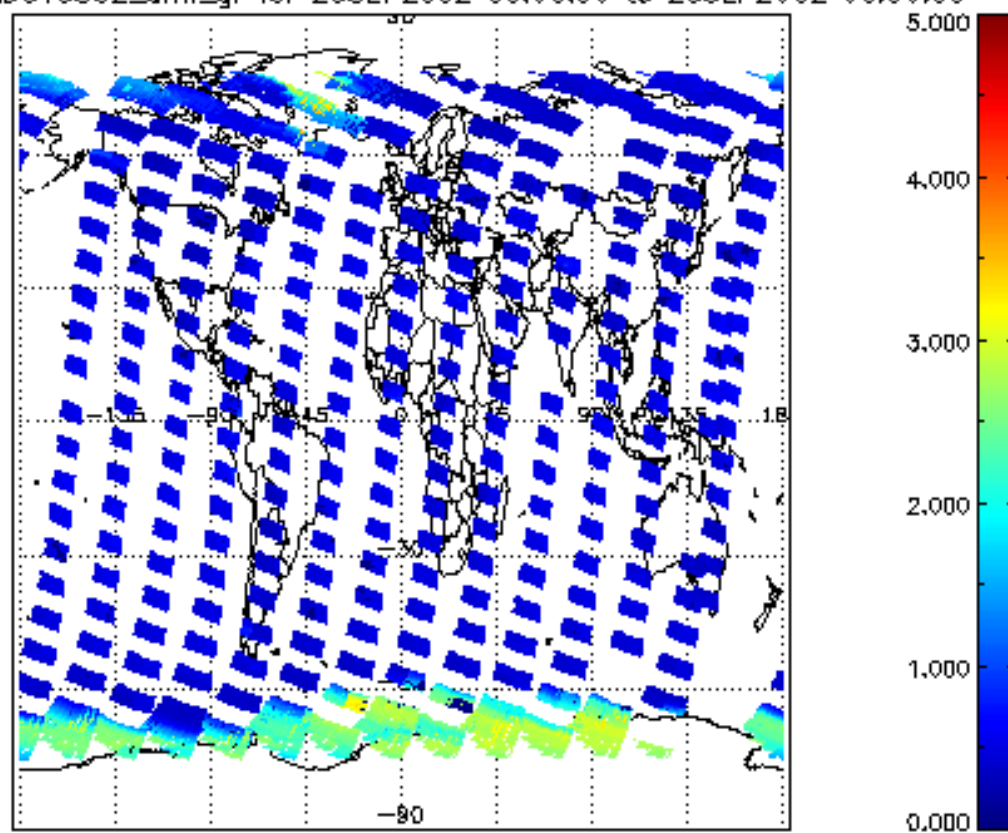
SCIOL2P_NADUV5S02_amf_gr for 25SEP2002 00:00:00 to 26SEP2002 00:00:00
