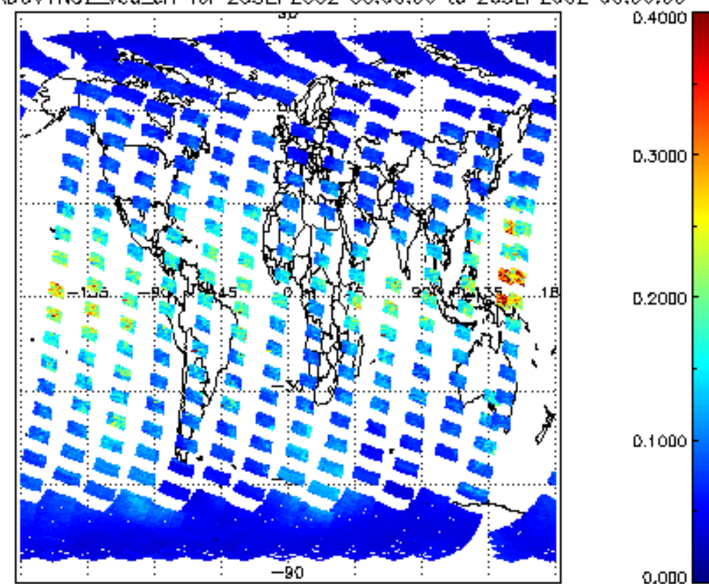
SCIOL2P_NADUV1NO2_vcd_err for 25SEP2002 00:00:00 to 26SEP2002 00:00:00
