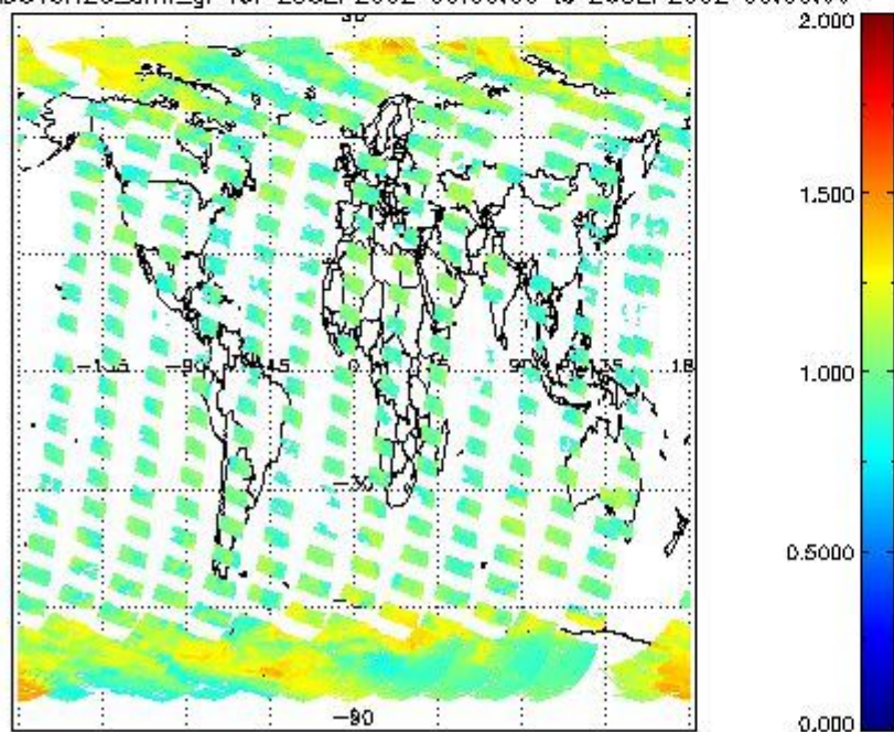
SCIOL2P_NADUV8H2O_arnf_gr for 25SEP2002 00:00:00 to 26SEP2002 00:00:00
