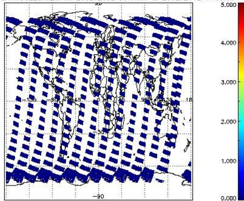
SCIOL2P_NADUV7S02_amf_cl for 25SEP2002 00:00:00 to 26SEP2002 00:00:00
