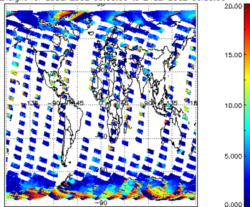
cl_top_height for 23SEP2002 00:00:00 to 24SEP2002 00:00:00
