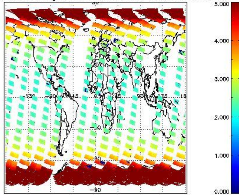
SCIOL2P_NADUV3BRO_amf_gr for 23SEP2002 00:00:00 to 24SEP2002 00:00:00
