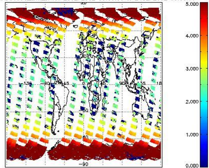
SCIOL2P_NADUV003_amf_cl for 23SEP2002 00:00:00 to 24SEP2002 00:00:00
