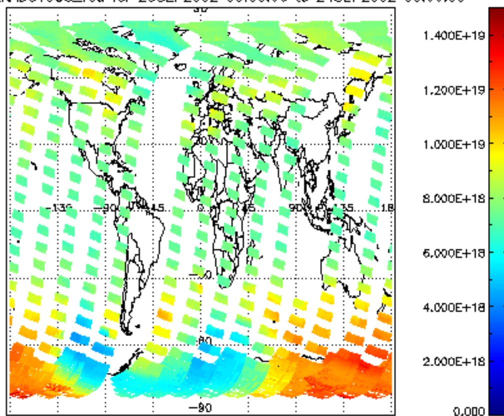
SCIOL2P_NADUV003_vcd for 23SEP2002 00:00:00 to 24SEP2002 00:00:00
