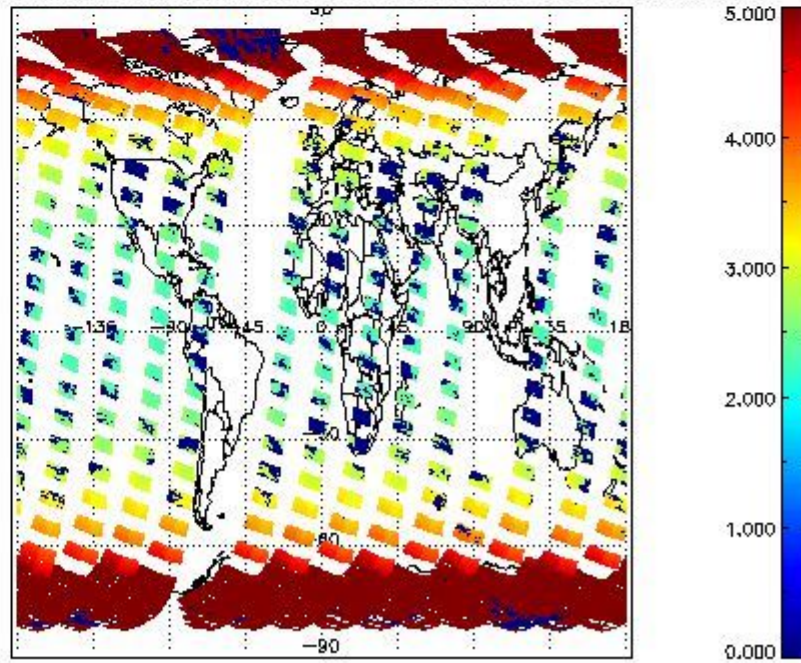
SCIOL2P_NADUV3BRO_amf_cl for 23SEP2002 00:00:00 to 24SEP2002 00:00:00
