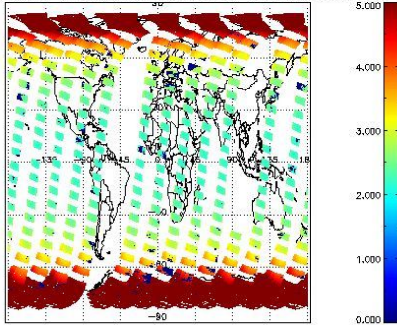
SCIOL2P_NADUV1N02_amf_gr for 23SEP2002 00:00:00 to 24SEP2002 00:00:00
