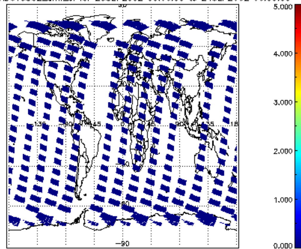
SCIOL2P_NADUV5S02_amf_cl for 23SEP2002 00:00:00 to 24SEP2002 00:00:00
