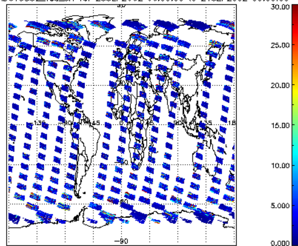
SCIOL2P_NADUV5S02_vcd_err for 23SEP2002 00:00:00 to 24SEP2002 00:00:00
