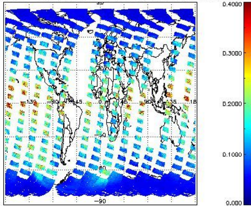
SCIOL2P_NADUV1N02_vcd_err for 23SEP2002 00:00:00 to 24SEP2002 00:00:00
