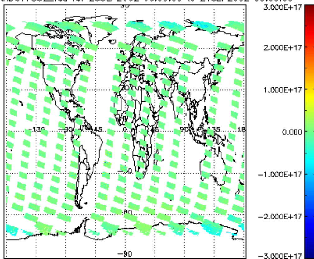
SCIOL2P_NADUV7S02_vcd for 23SEP2002 00:00:00 to 24SEP2002 00:00:00
