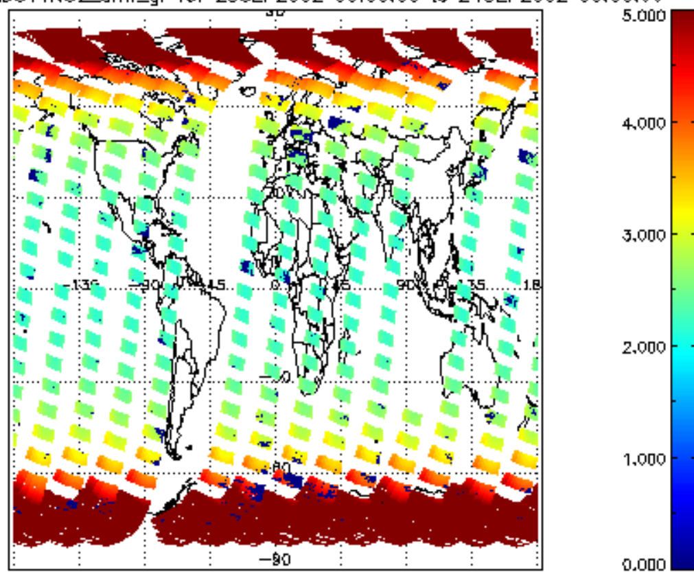
SCIOL2P_NADUV1NO2_amf_gr for 23SEP2002 00:00:00 to 24SEP2002 00:00:00
