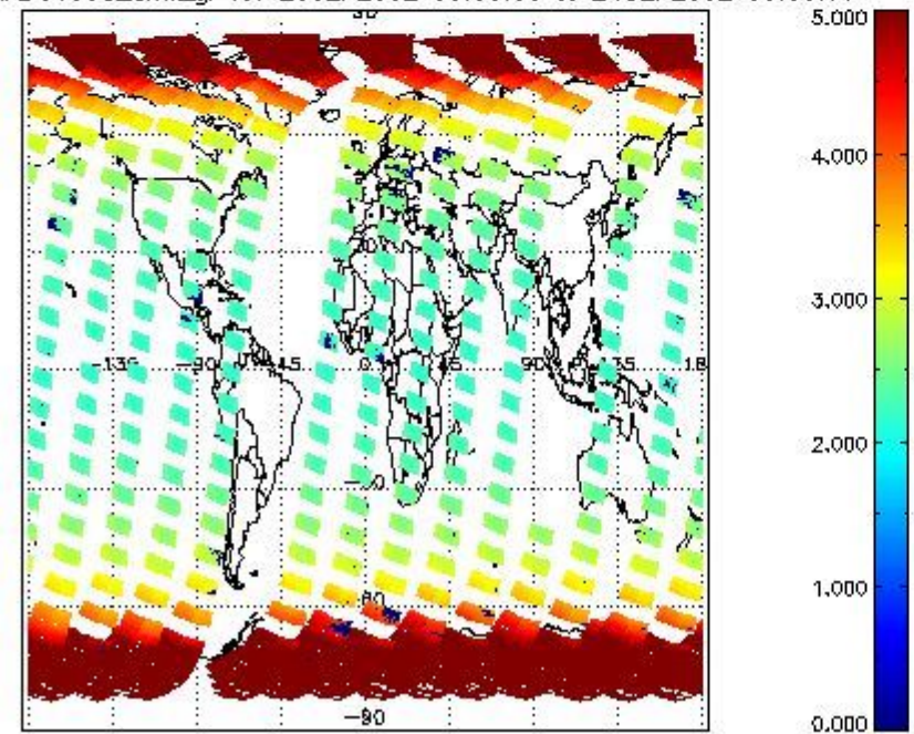
SCIOL2P_NADUV003_amf_gr for 23SEP2002 00:00:00 to 24SEP2002 00:00:00
