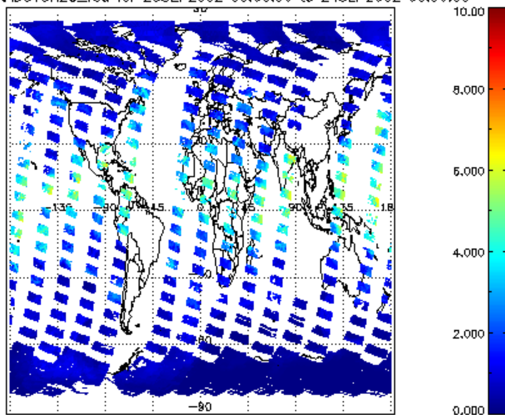
SCIOL2P_NADUV8H20_vcd for 23SEP2002 00:00:00 to 24SEP2002 00:00:00
