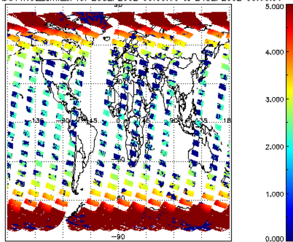
SCIOL2P_NADUV1NO2_amf_cl for 23SEP2002 00:00:00 to 24SEP2002 00:00:00
