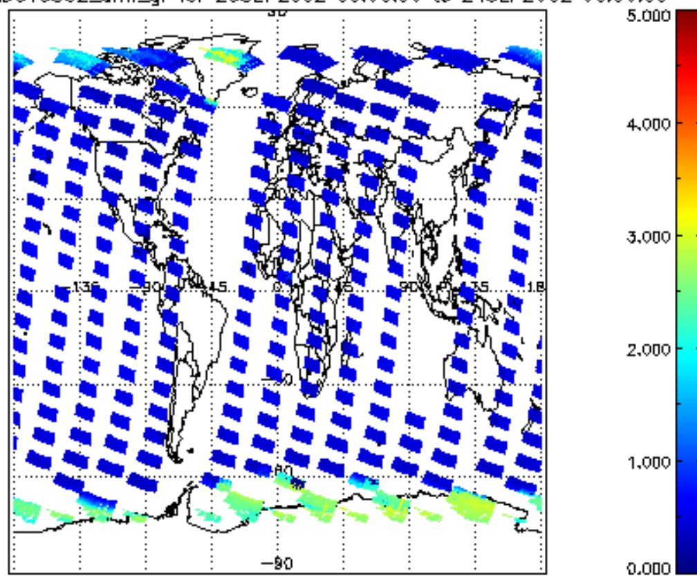
SCIOL2P_NADUV5S02_amf_gr for 23SEP2002 00:00:00 to 24SEP2002 00:00:00
