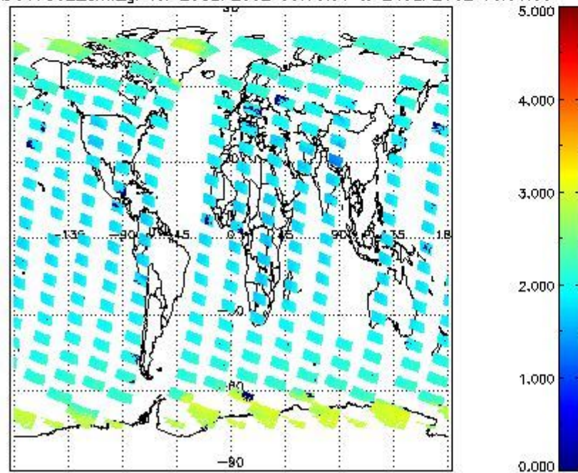
SCIOL2P_NADUV7S02_amf_gr for 23SEP2002 00:00:00 to 24SEP2002 00:00:00
