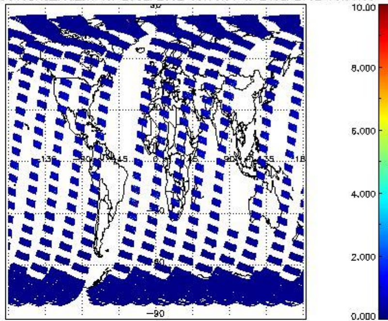
SCIOL2P_NADUV3BRO_vcd_err for 23SEP2002 00:00:00 to 24SEP2002 00:00:00
