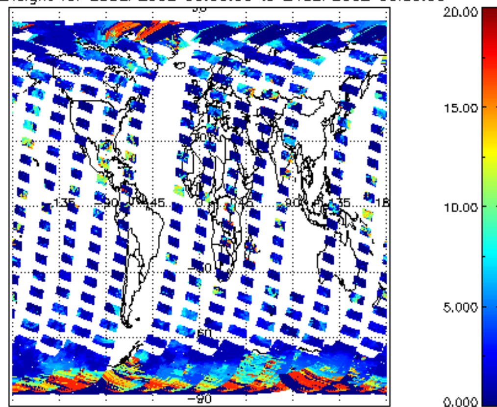
cl_top_height for 23SEP2002 00:00:00 to 24SEP2002 00:00:00
