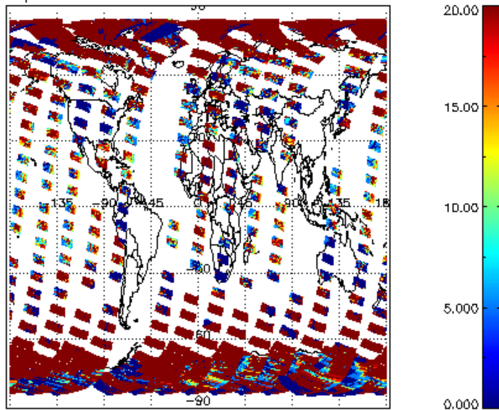
cl_opt_depth for 23SEP2002 00:00:00 to 24SEP2002 00:00:00
