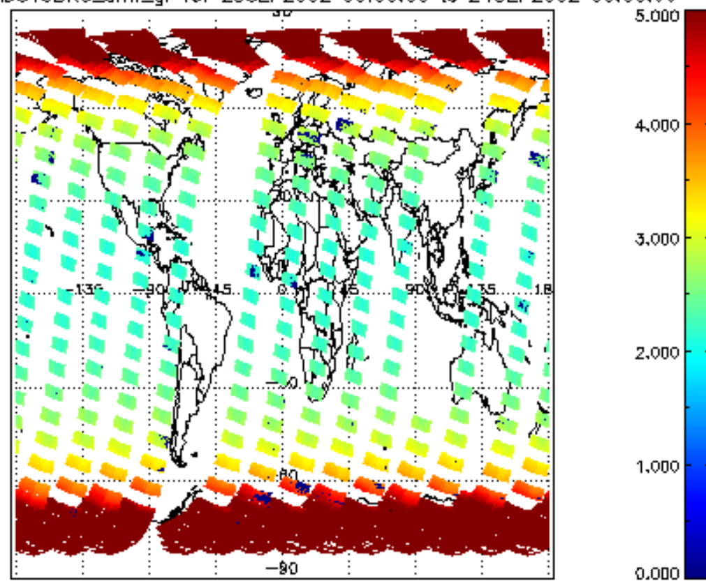
SCIOL2P_NADUV3BRO_amf_gr for 23SEP2002 00:00:00 to 24SEP2002 00:00:00
