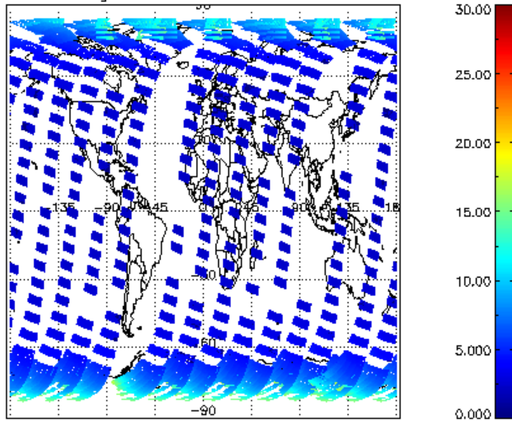
iCIOL2P_NADUV1NO2_amf_gr for 23SEP2002 00:00:00 to 24SEP2002 00:00:00
