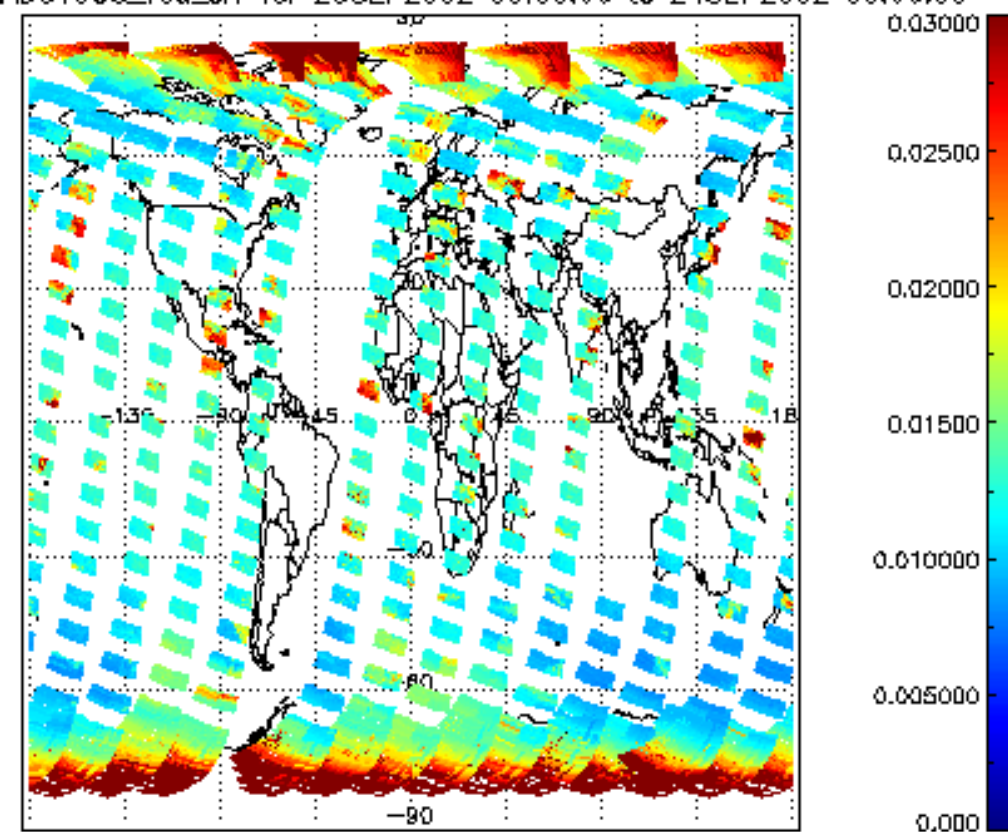
SCIOL2P_NADUV003_vcd_err for 23SEP2002 00:00:00 to 24SEP2002 00:00:00
