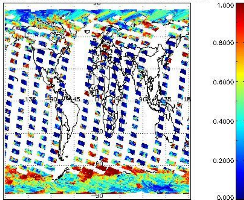
cL_frac for 23SEP2002 00:00:00 to 24SEP2002 00:00:00
