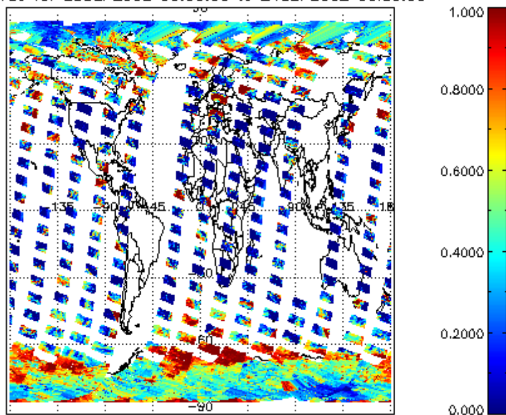
cl_frac for 23SEP2002 00:00:00 to 24SEP2002 00:00:00
