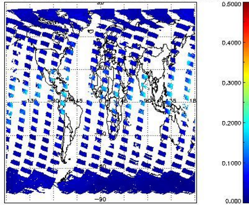
SCIOL2P_NADUV8H2O_vcd_err for 23SEP2002 00:00:00 to 24SEP2002 00:00:00
