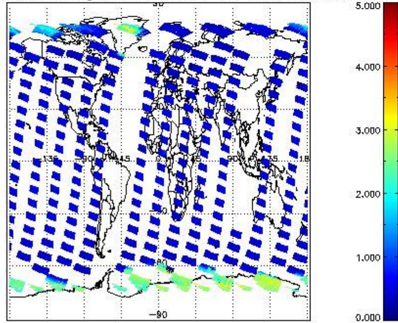
SCIOL2P_NADUV5S02_amf_gr for 23SEP2002 00:00:00 to 24SEP2002 00:00:00
