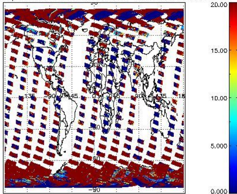
cL_opt_depth for 23SEP2002 00:00:00 to 24SEP2002 00:00:00
