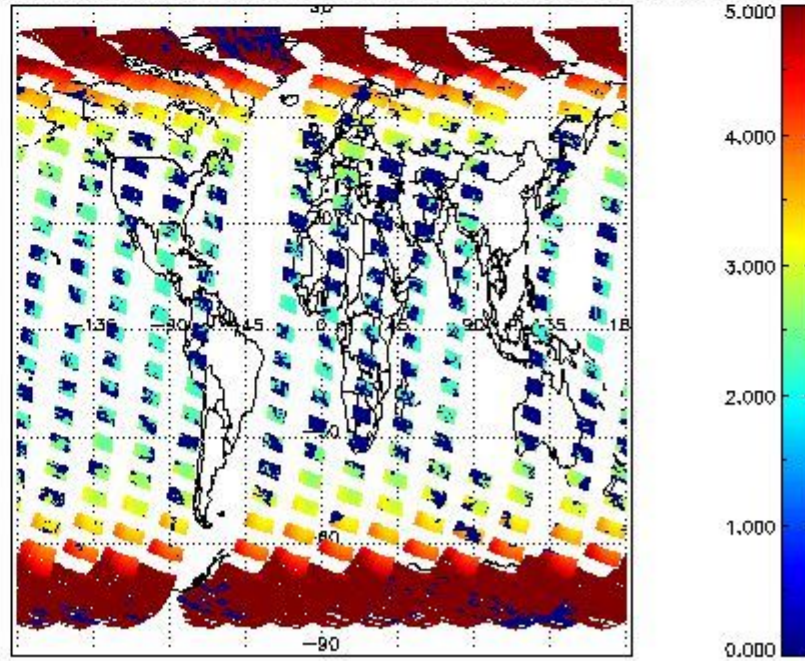
SCIOL2P_NADUV1N02_amf_cl for 23SEP2002 00:00:00 to 24SEP2002 00:00:00
