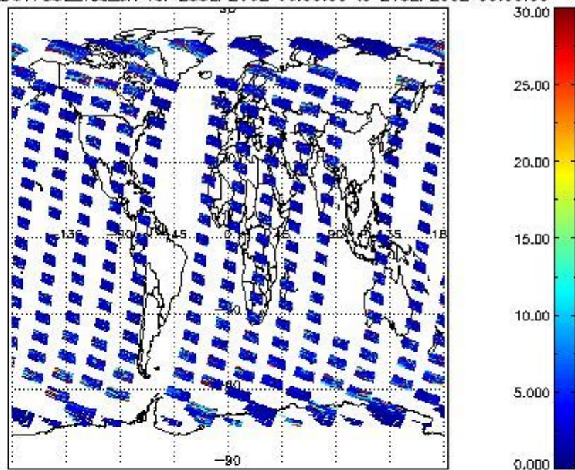
SCIOL2P_NADUV7S02_vcd_err for 23SEP2002 00:00:00 to 24SEP2002 00:00:00
