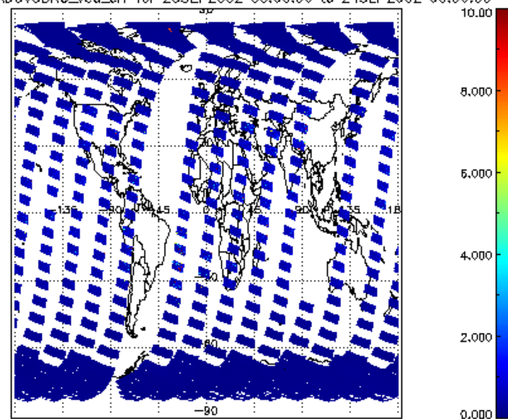
SCIOL2P_NADUV3BRO_vcd_err for 23SEP2002 00:00:00 to 24SEP2002 00:00:00
