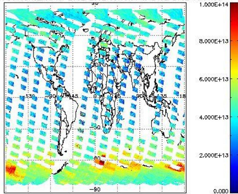
SCIOL2P_NADUV3BRO_vcd for 23SEP2002 00:00:00 to 24SEP2002 00:00:00
