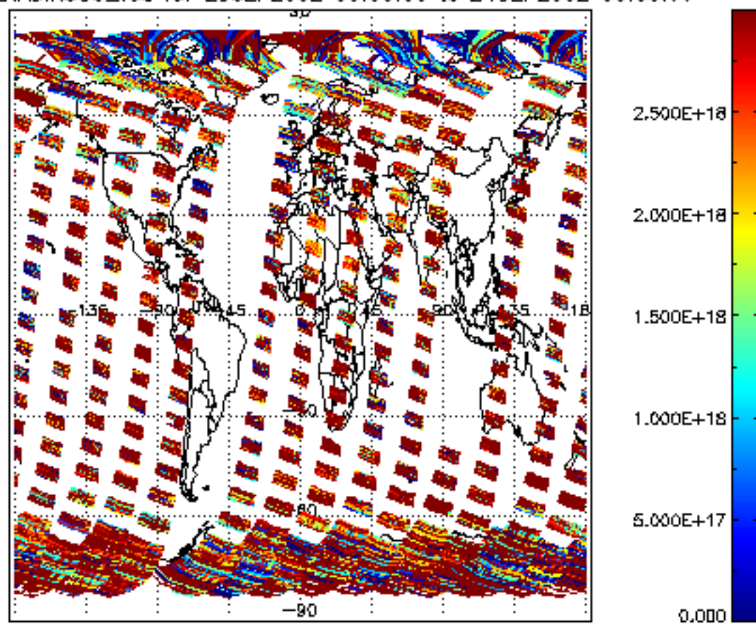
SCIOL2P_NADIR3CO_vcd for 23SEP2002 00:00:00 to 24SEP2002 00:00:00
