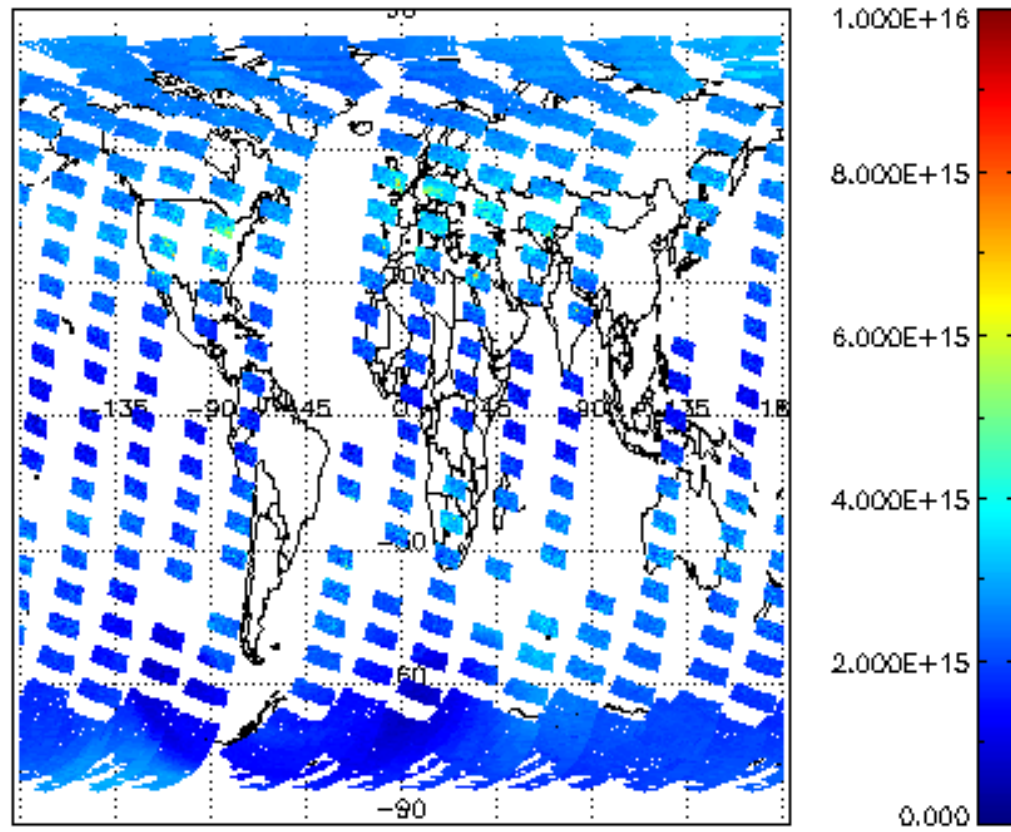
SCIOL2P_NADUV1NO2_vcd for 23SEP2002 00:00:00 to 24SEP2002 00:00:00
