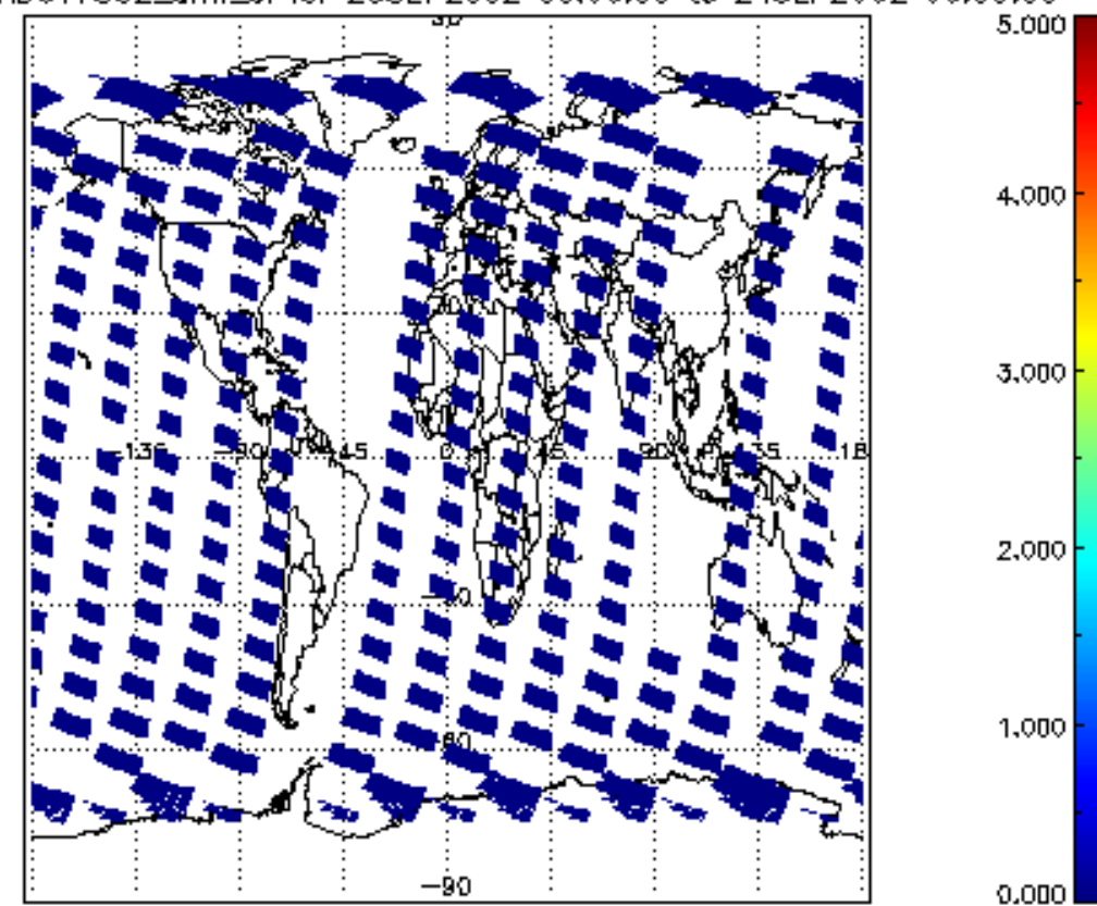
SCIOL2P_NADUV7S02_amf_cl for 23SEP2002 00:00:00 to 24SEP2002 00:00:00
