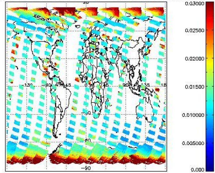
SCIOL2P_NADUV003_vcd_err for 23SEP2002 00:00:00 to 24SEP2002 00:00:00
