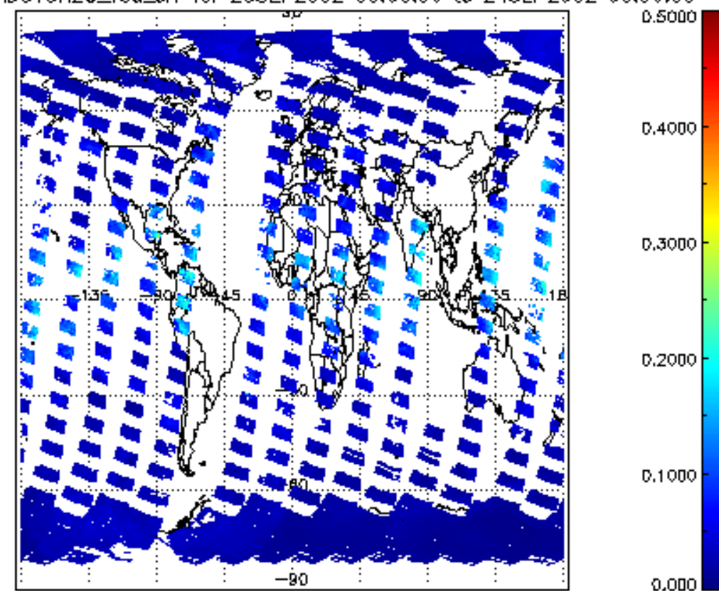
SCIOL2P_NADUV8H20_vcd_err for 23SEP2002 00:00:00 to 24SEP2002 00:00:00
