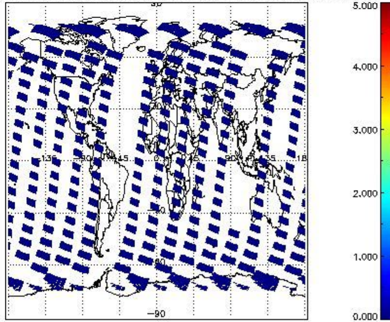
SCIOL2P_NADUV5S02_amf_cl for 23SEP2002 00:00:00 to 24SEP2002 00:00:00
