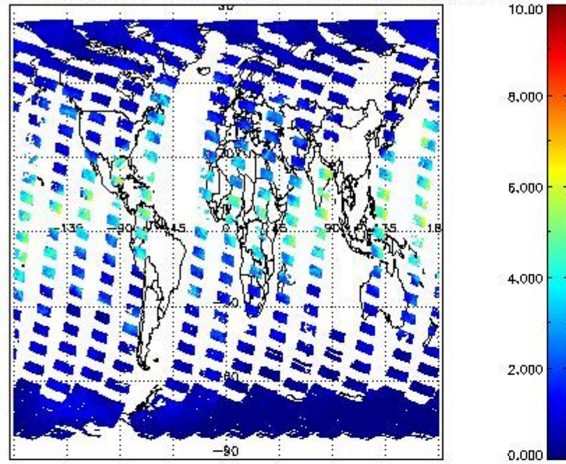
SCIOL2P_NADUV8H2O_vcd for 23SEP2002 00:00:00 to 24SEP2002 00:00:00
