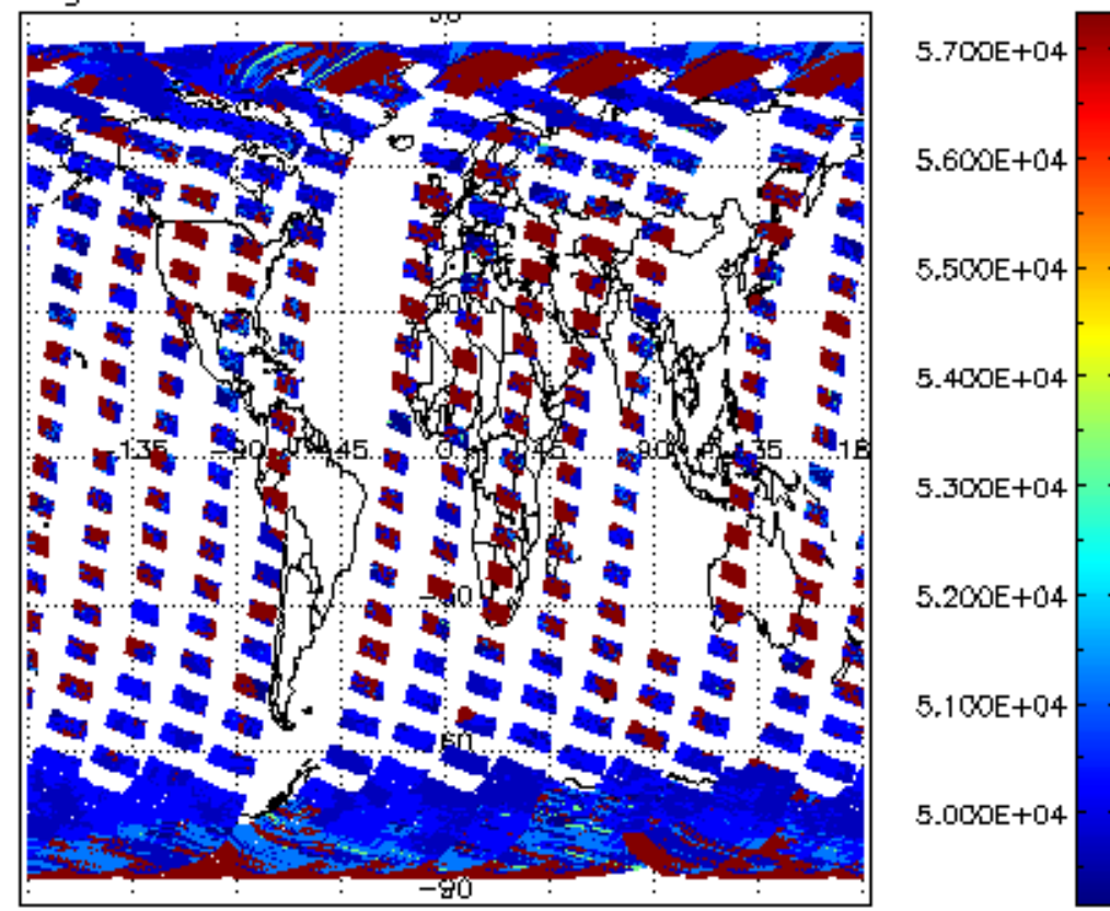
cloud_flags for 23SEP2002 00:00:00 to 24SEP2002 00:00:00
