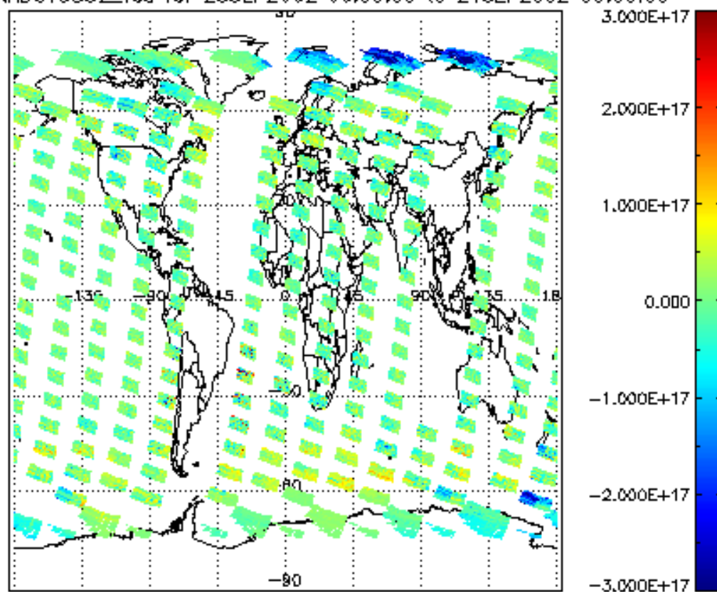
SCIOL2P_NADUV5S02_vcd for 23SEP2002 00:00:00 to 24SEP2002 00:00:00
