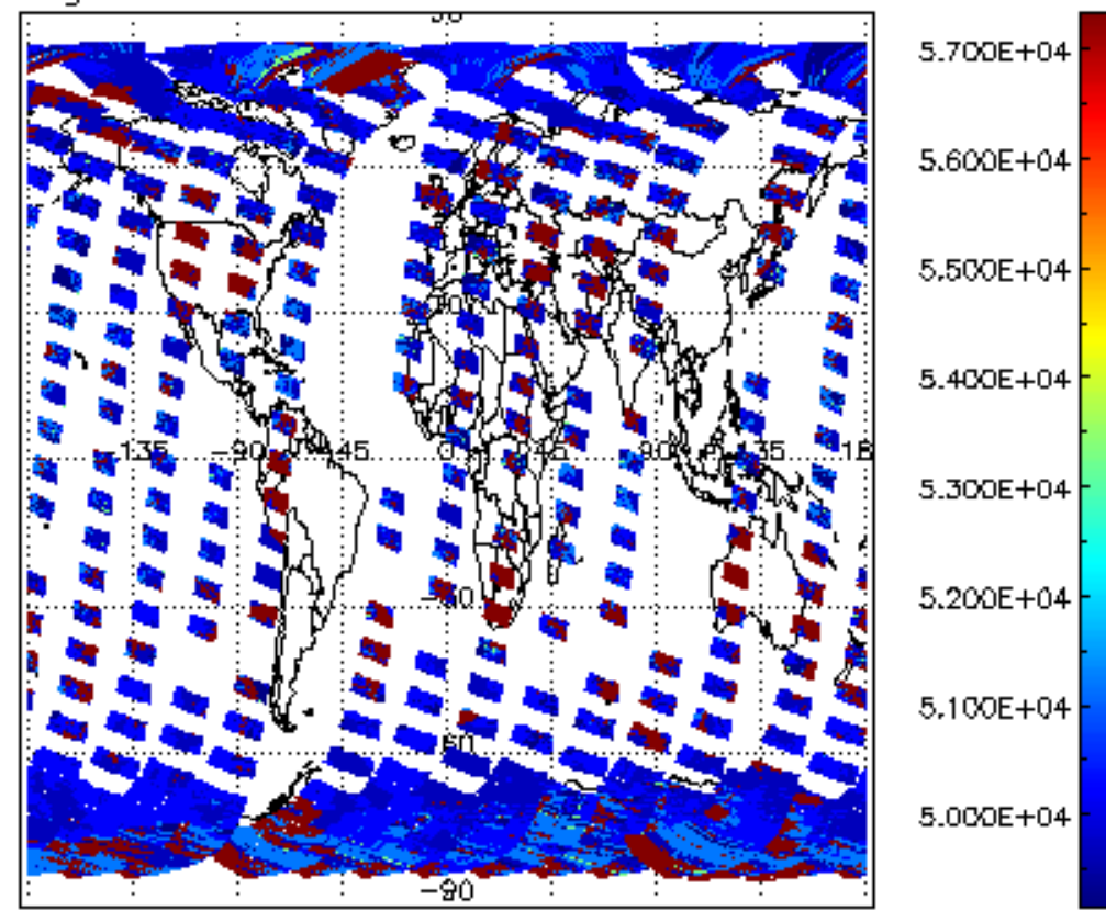
cloud_flags for 23SEP2002 00:00:00 to 24SEP2002 00:00:00
