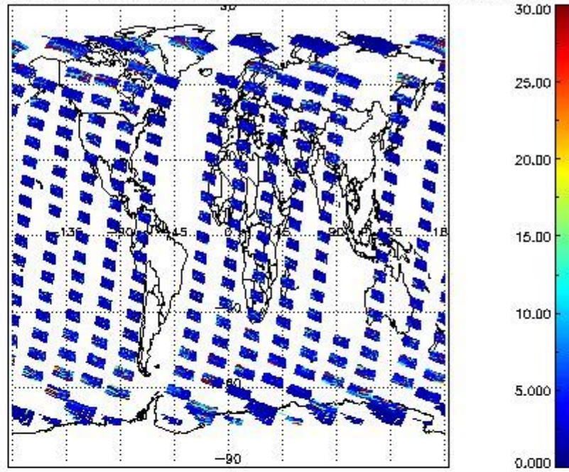
SCIOL2P_NADUV5S02_vcd_err for 23SEP2002 00:00:00 to 24SEP2002 00:00:00
