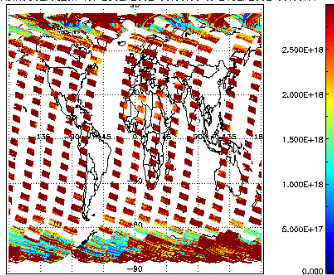
SCIOL2P_NADIR3CO_vcd_err for 23SEP2002 00:00:00 to 24SEP2002 00:00:00
