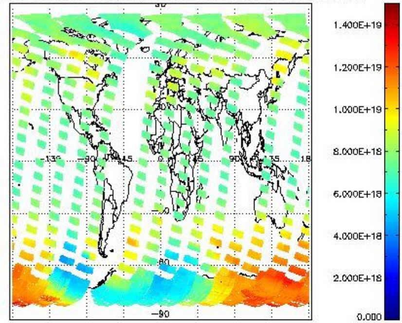
SCIOL2P_NADUV003_vcd for 23SEP2002 00:00:00 to 24SEP2002 00:00:00
