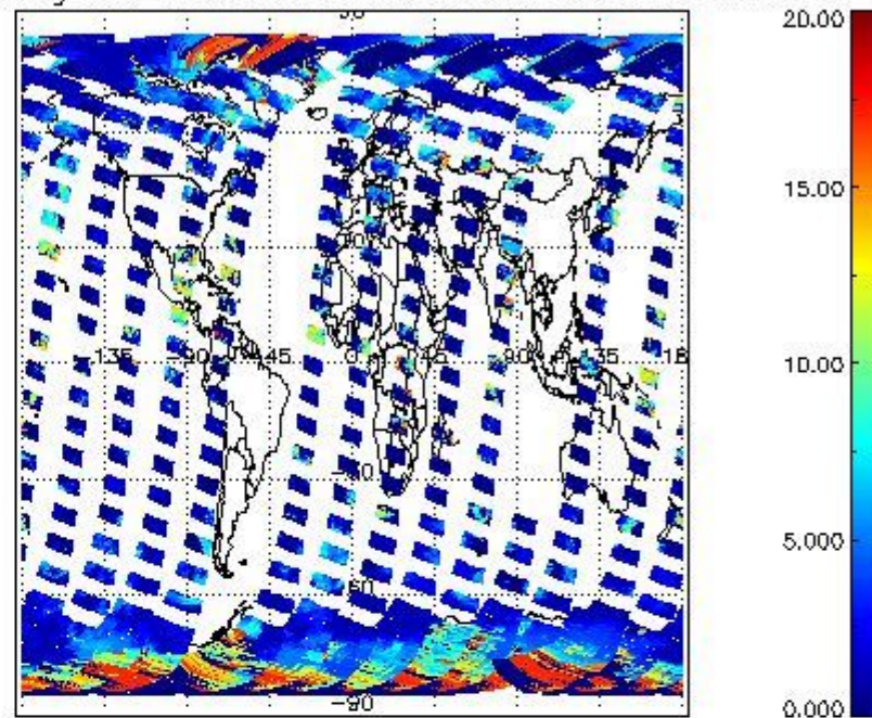
cL_top_height for 23SEP2002 00:00:00 to 24SEP2002 00:00:00
