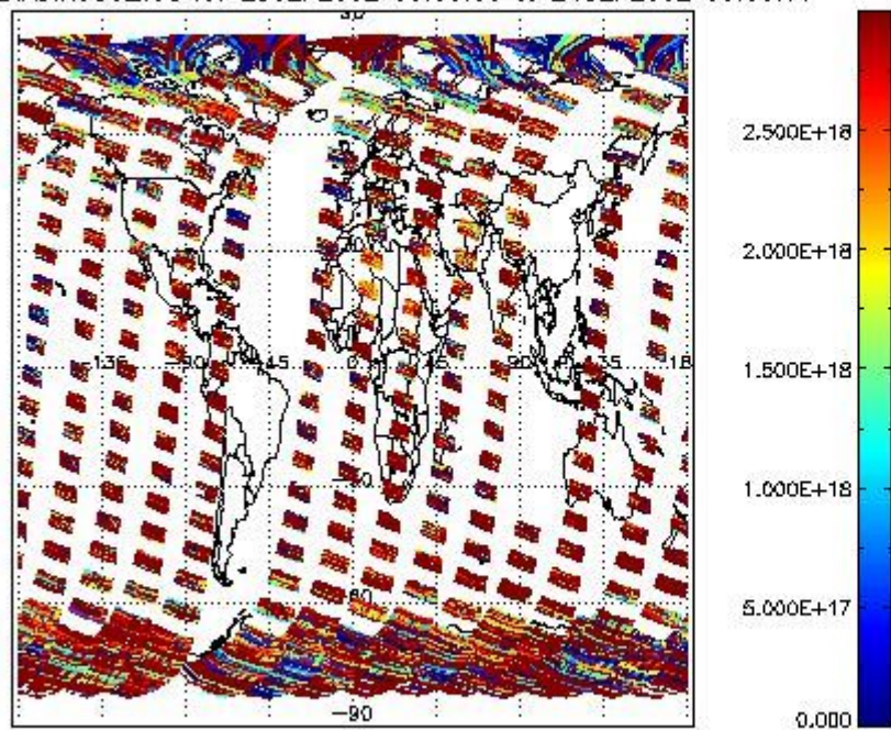
SCIO2P_NADIR3CO_vcd for 23SEP2002 00:00:00 to 24SEP2002 00:00:00
