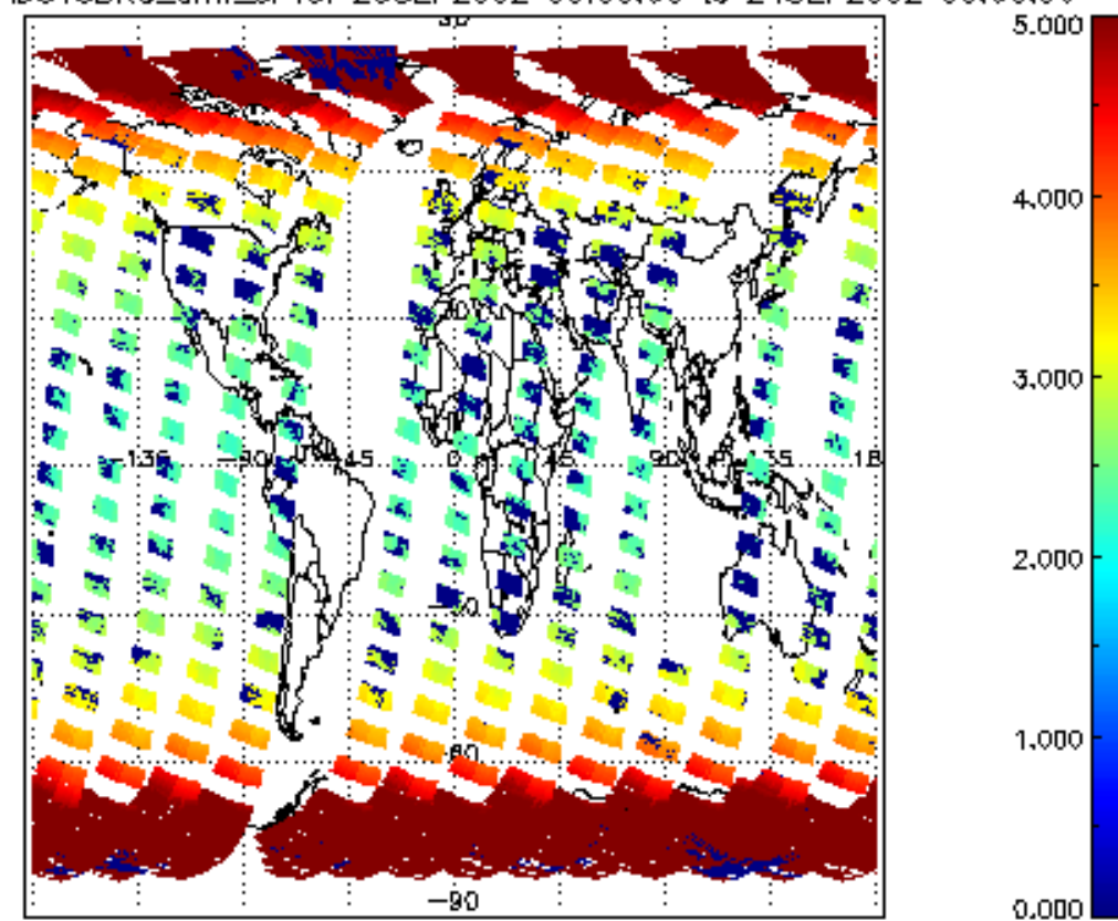
SCIOL2P_NADUV3BRO_amf_sl for 23SEP2002 00:00:00 to 24SEP2002 00:00:00
