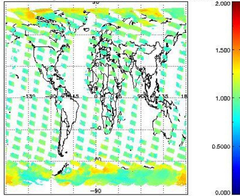
SCIOL2P_NADUV8H2O_arnf_gr for 23SEP2002 00:00:00 to 24SEP2002 00:00:00
