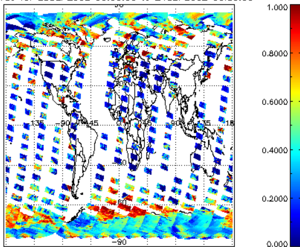
cl_frac for 23SEP2002 00:00:00 to 24SEP2002 00:00:00
