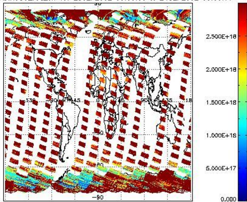
SCIO2P_NADIR3CO_vcd_err for 23SEP2002 00:00:00 to 24SEP2002 00:00:00
