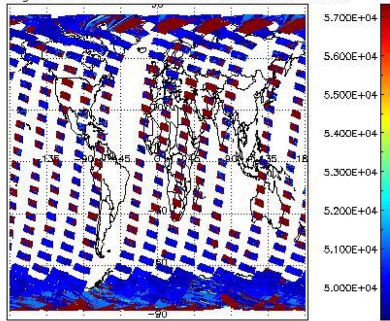
cloud_flags for 23SEP2002 00:00:00 to 24SEP2002 00:00:00
