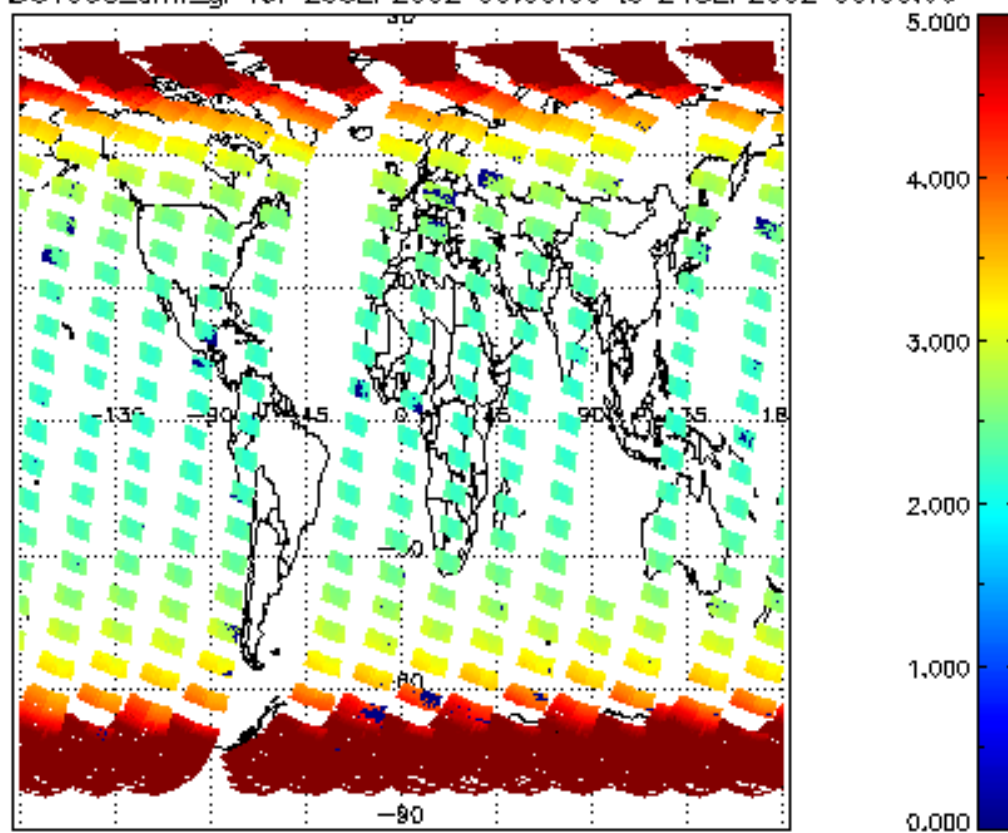
SCIOL2P_NADUV003_amf_gr for 23SEP2002 00:00:00 to 24SEP2002 00:00:00
