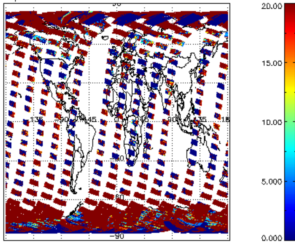
cl_opt_depth for 23SEP2002 00:00:00 to 24SEP2002 00:00:00
