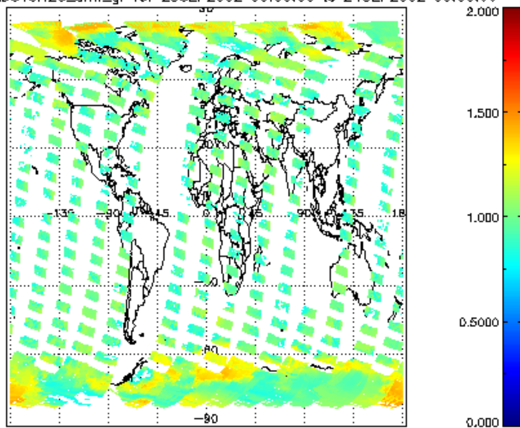
SCIOL2P_NADUV8H20_amf_gr for 23SEP2002 00:00:00 to 24SEP2002 00:00:00
