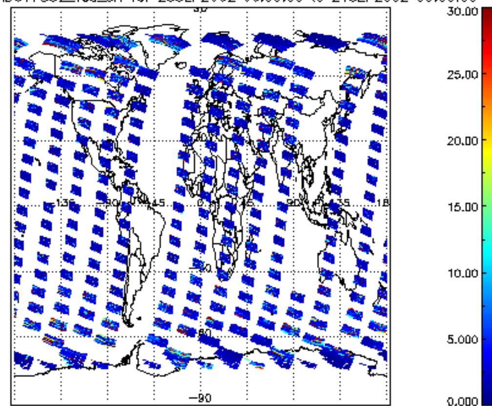
SCIOL2P_NADUV7S02_vcd_err for 23SEP2002 00:00:00 to 24SEP2002 00:00:00
