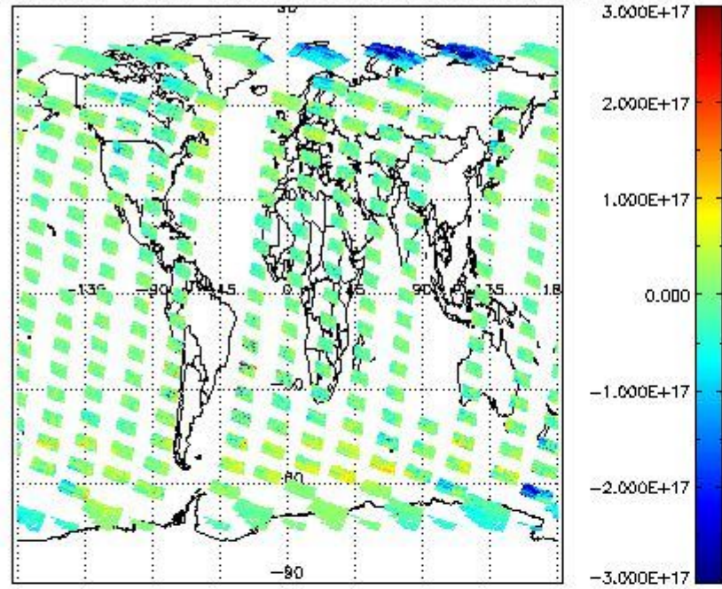
SCIOL2P_NADUV5S02_vcd for 23SEP2002 00:00:00 to 24SEP2002 00:00:00
