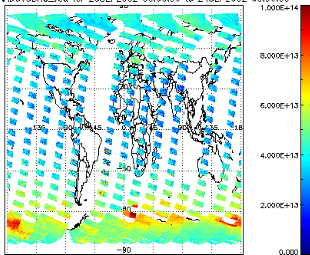
SCIOL2P_NADUV3BRO_vcd for 23SEP2002 00:00:00 to 24SEP2002 00:00:00
