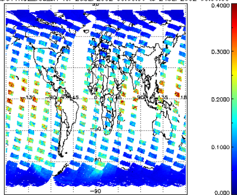
SCIOL2P_NADUV1NO2_vcd_err for 23SEP2002 00:00:00 to 24SEP2002 00:00:00
