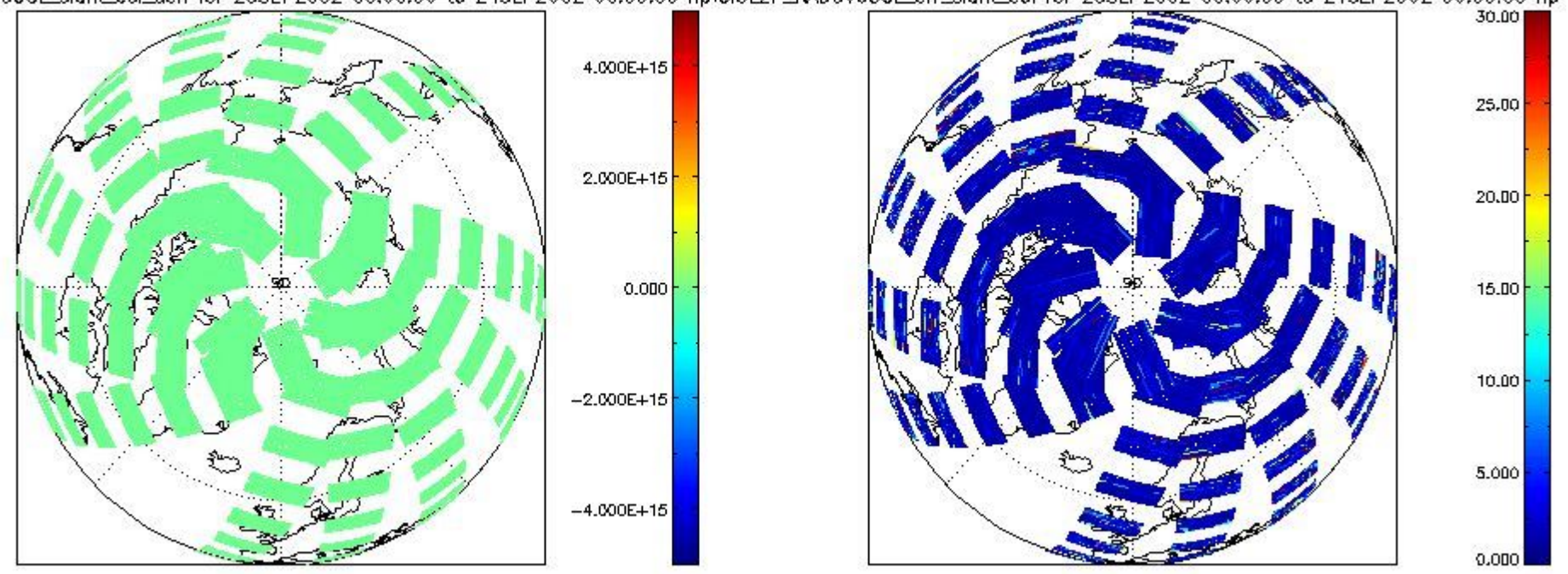
CIOL2P_NADUV60CLslant_col_den for 23SEP2002 00:00:00 to 24SEP2002 00:00:00 np | CIOL2P_NADUV60CLerr_slant_col for 23SEP2002 00:00:00 to 24SEP2002 00:00:00 np
