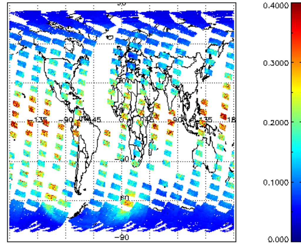
iCIOL2P_NADUV1NO2_vcd_err for 23SEP2002 00:00:00 to 24SEP2002 00:00:00
