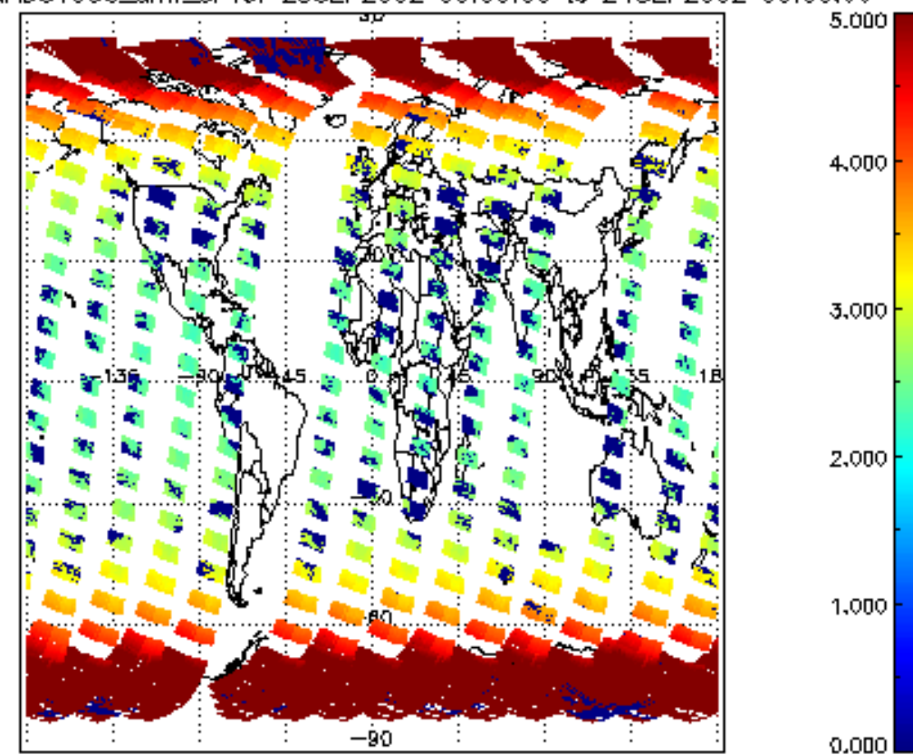
SCIOL2P_NADUV003_amf_cl for 23SEP2002 00:00:00 to 24SEP2002 00:00:00
