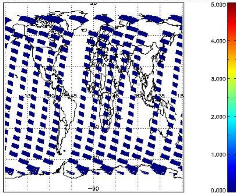
SCIOL2P_NADUV7S02_amf_cl for 23SEP2002 00:00:00 to 24SEP2002 00:00:00
