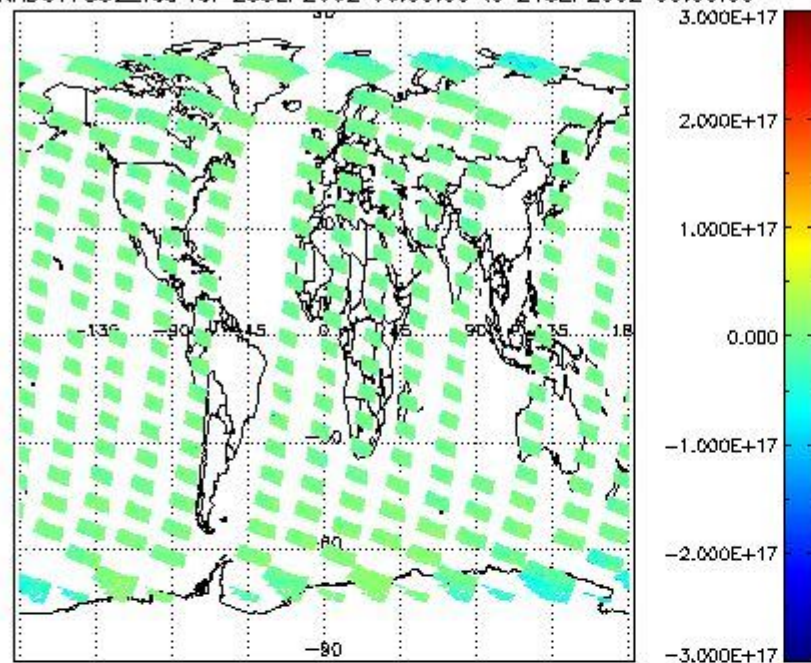
SCIOL2P_NADUV7S02_vcd for 23SEP2002 00:00:00 to 24SEP2002 00:00:00
