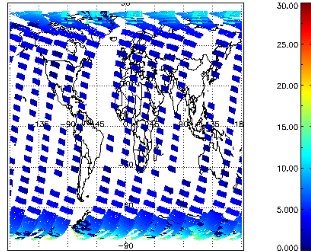
iCIOL2P_NADUV1NO2_amf_cl for 23SEP2002 00:00:00 to 24SEP2002 00:00:00
