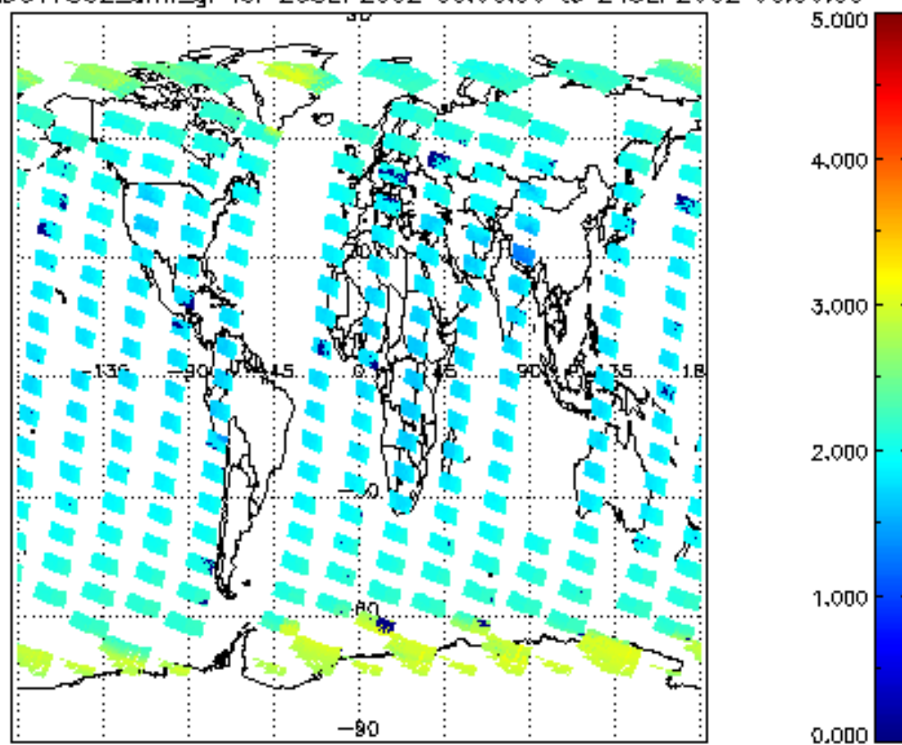
SCIOL2P_NADUV7S02_amf_gr for 23SEP2002 00:00:00 to 24SEP2002 00:00:00
