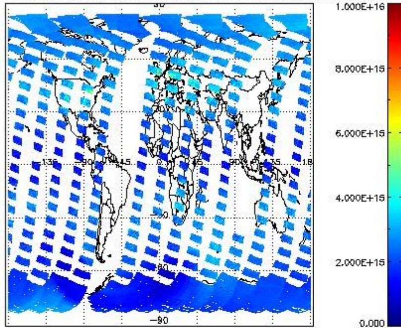
SCIOL2P_NADUV1N02_vcd for 23SEP2002 00:00:00 to 24SEP2002 00:00:00
