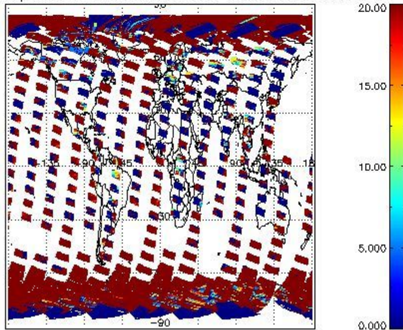
cL_opt_depth for 16SEP2002 00:00:00 to 17SEP2002 00:00:00
