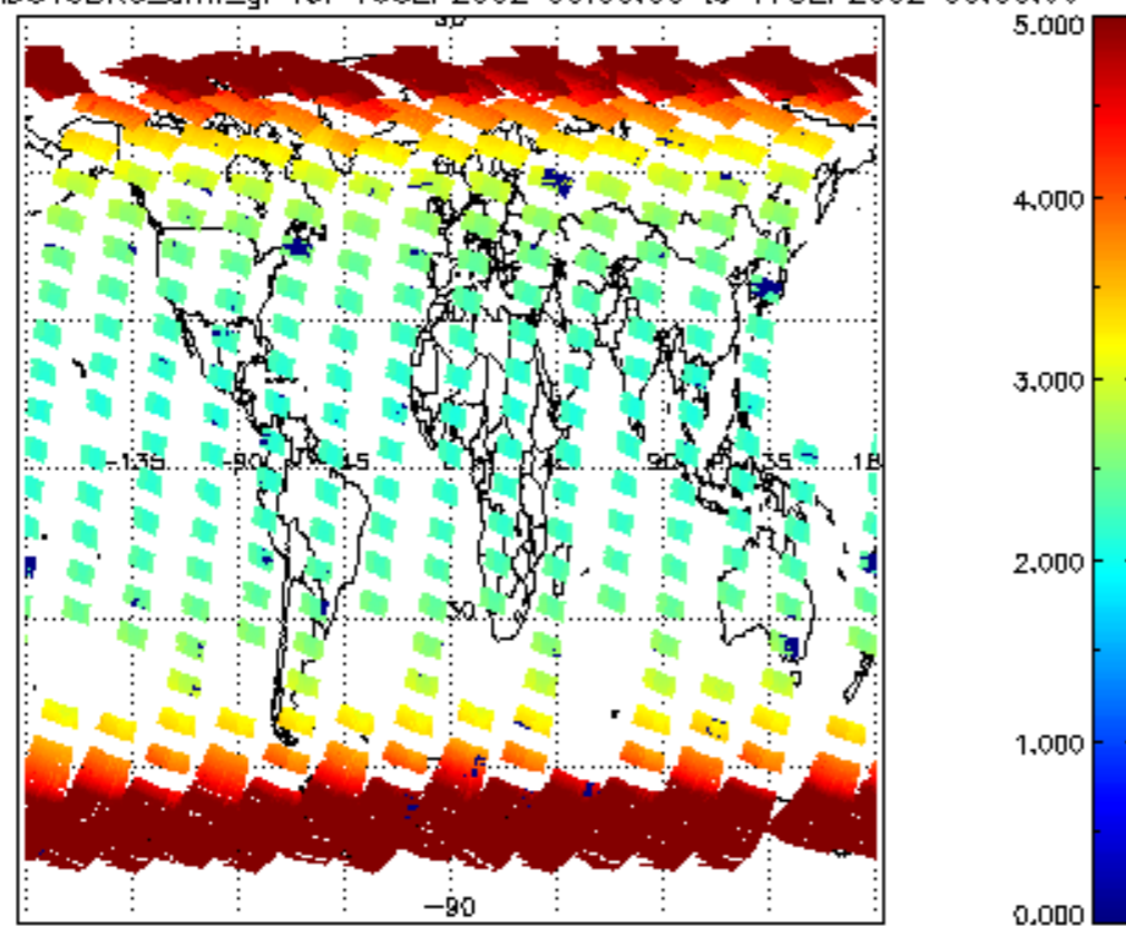
SCIOL2P_NADUV3BRO_amf_gr for 16SEP2002 00:00:00 to 17SEP2002 00:00:00
