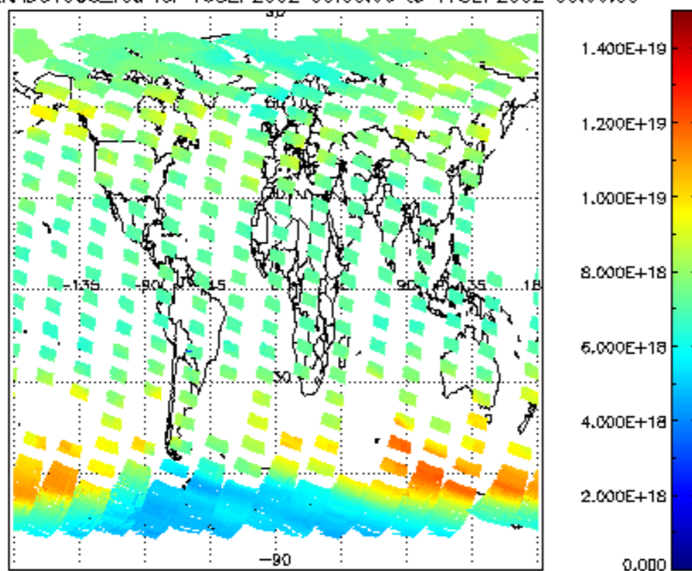
SCIOL2P_NADUV003_vcd for 16SEP2002 00:00:00 to 17SEP2002 00:00:00
