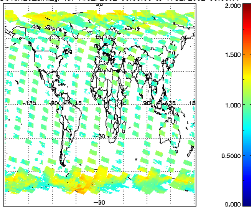
SCIOL2P_NADUV8H20_amf_gr for 16SEP2002 00:00:00 to 17SEP2002 00:00:00
