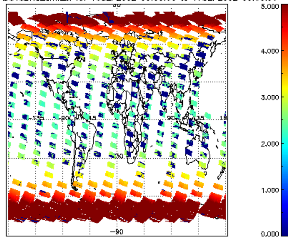
SCIOL2P_NADUV3BRO_amf_cl for 16SEP2002 00:00:00 to 17SEP2002 00:00:00
