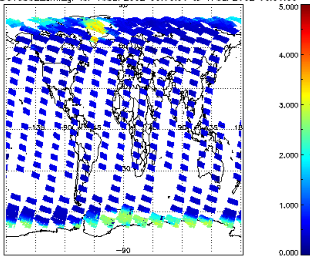
SCIOL2P_NADUV5S02_amf_gr for 16SEP2002 00:00:00 to 17SEP2002 00:00:00
