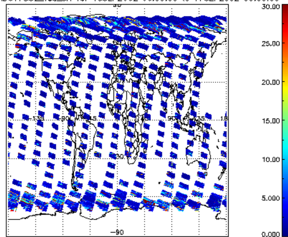
SCIOL2P_NADUV7S02_vcd_err for 16SEP2002 00:00:00 to 17SEP2002 00:00:00
