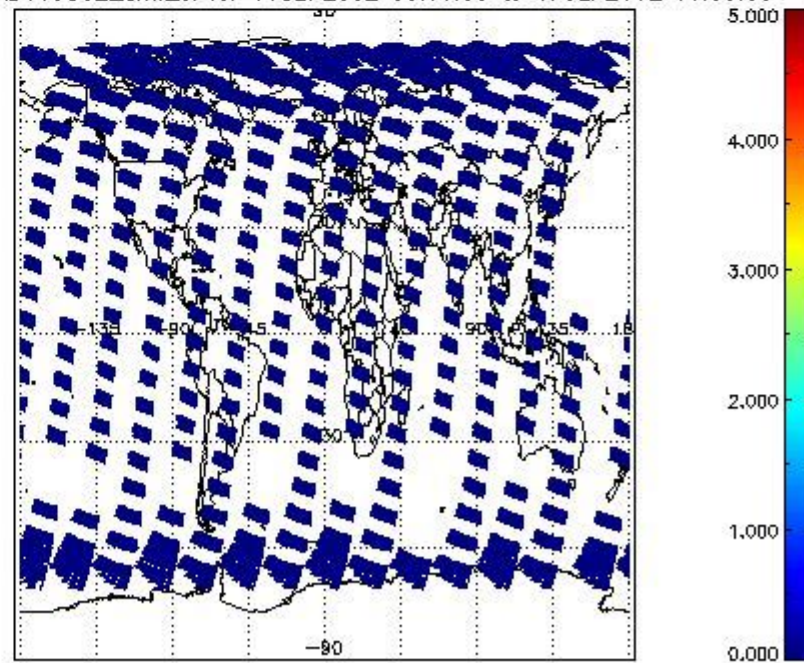
SCIOL2P_NADUV5S02_amf_cl for 16SEP2002 00:00:00 to 17SEP2002 00:00:00
