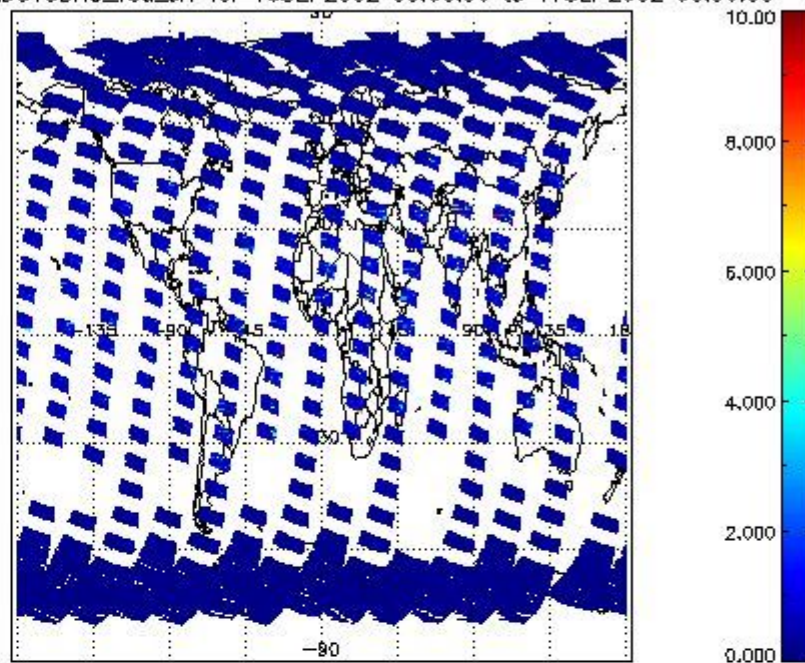
SCIOL2P_NADUV3BRO_vcd_err for 16SEP2002 00:00:00 to 17SEP2002 00:00:00
