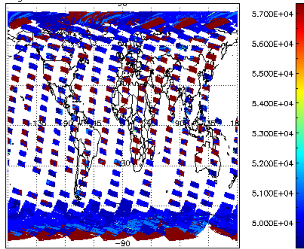
cloud_flags for 16SEP2002 00:00:00 to 17SEP2002 00:00:00
