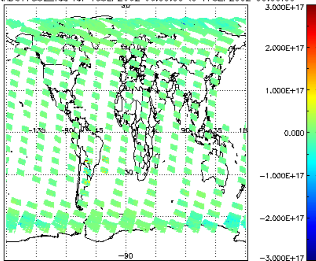
SCIOL2P_NADUV7S02_vcd for 16SEP2002 00:00:00 to 17SEP2002 00:00:00
