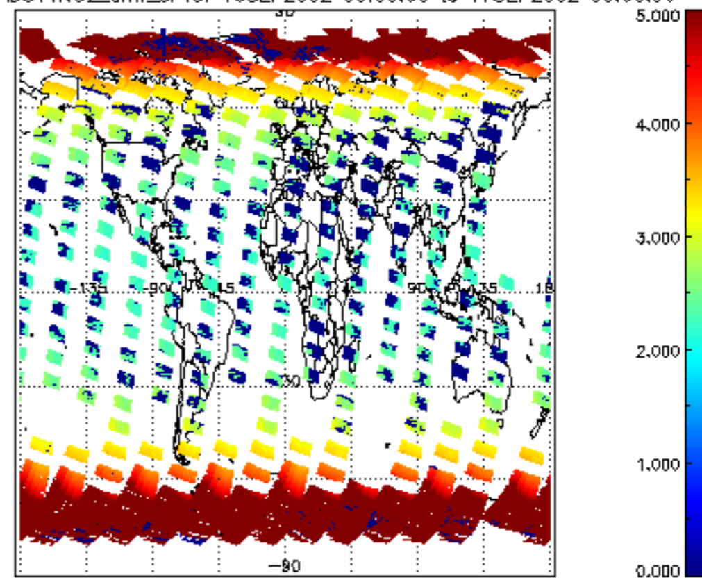
SCIOL2P_NADUV1NO2_amf_sl for 16SEP2002 00:00:00 to 17SEP2002 00:00:00
