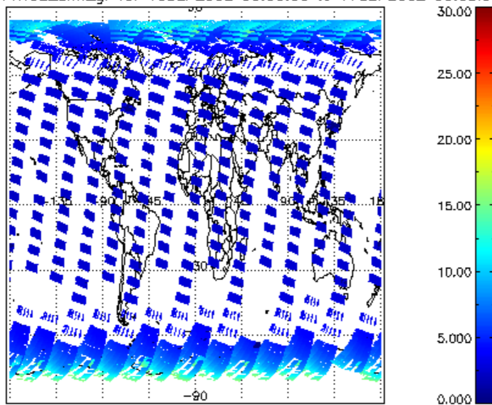
iCIOL2P_NADUV1NO2_amf_gr for 16SEP2002 00:00:00 to 17SEP2002 00:00:00
