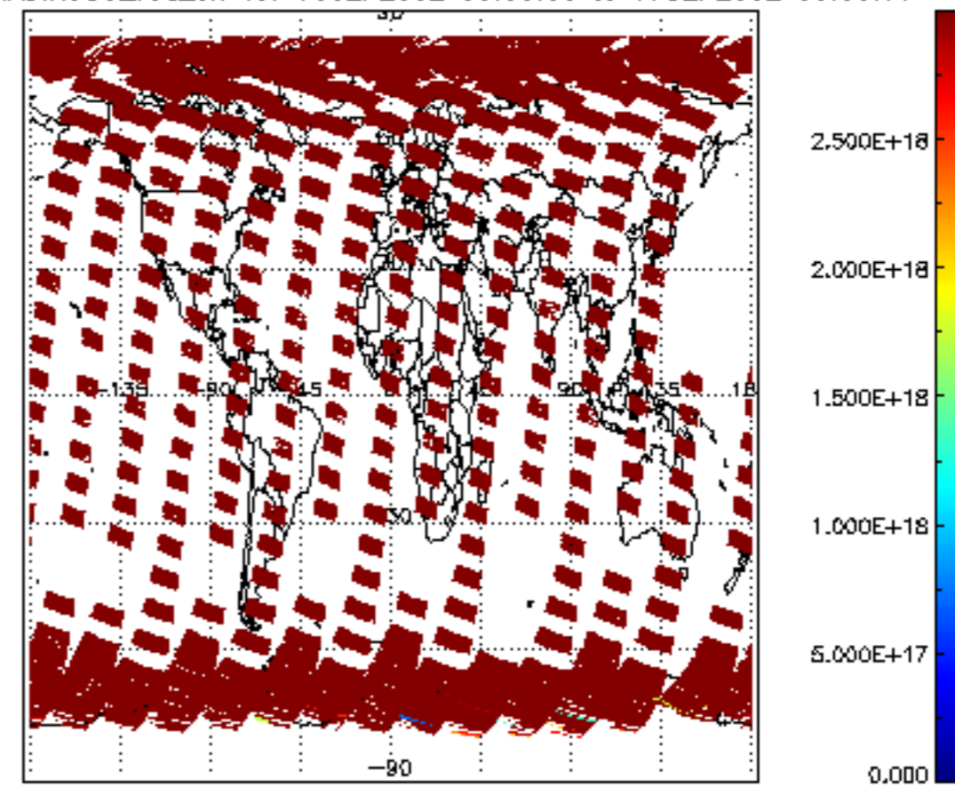
SCIOL2P_NADIR3CO_vcd_err for 16SEP2002 00:00:00 to 17SEP2002 00:00:00
