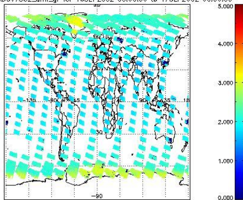
SCIOL2P_NADUV7S02_amf_gr for 16SEP2002 00:00:00 to 17SEP2002 00:00:00
