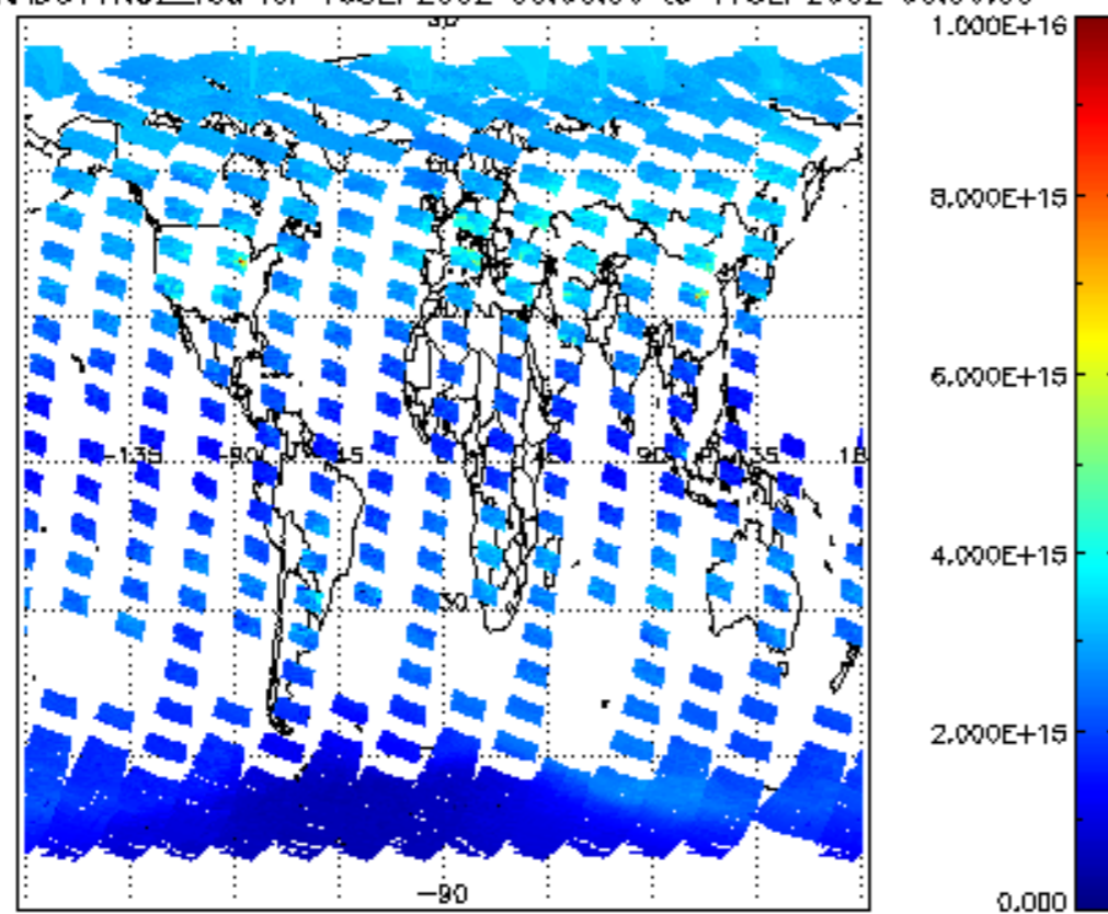
SCIOL2P_NADUV1NO2_vcd for 16SEP2002 00:00:00 to 17SEP2002 00:00:00
