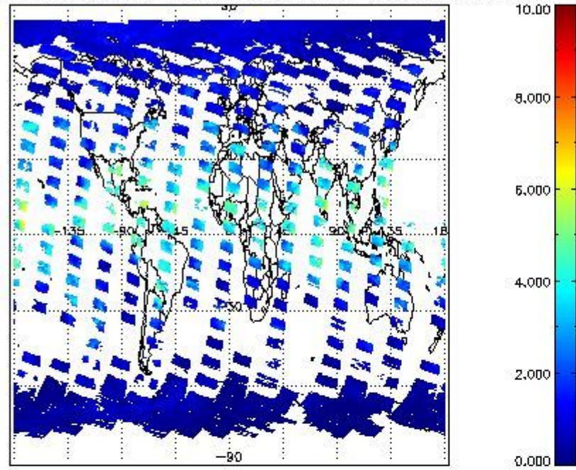
SCIOL2P_NADUV8H2O_vcd for 16SEP2002 00:00:00 to 17SEP2002 00:00:00
