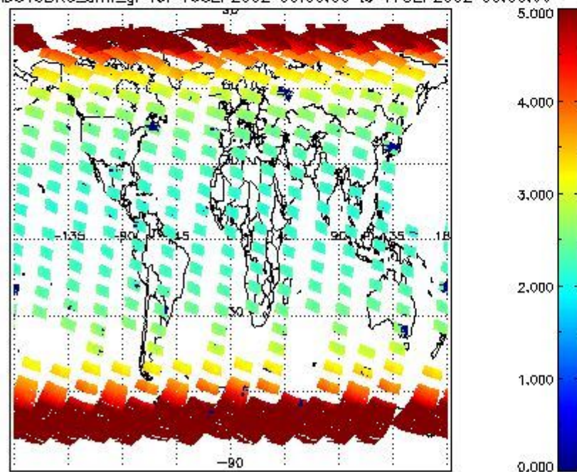
SCIOL2P_NADUV3BRO_amf_gr for 16SEP2002 00:00:00 to 17SEP2002 00:00:00
