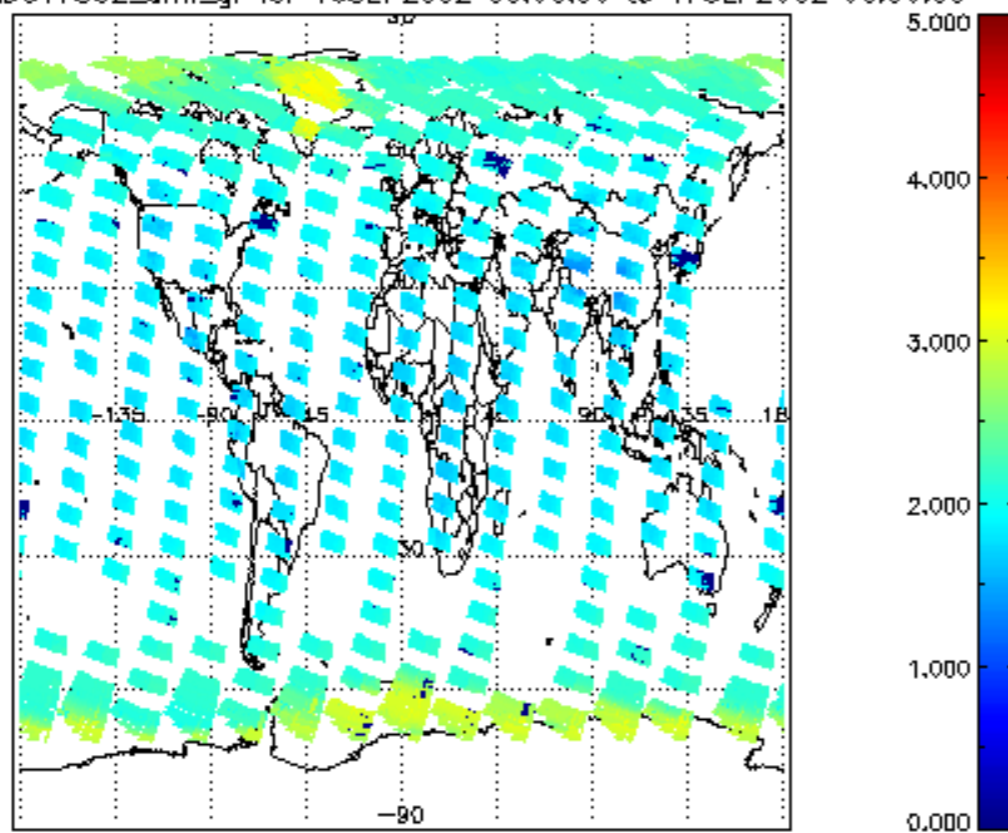
SCIOL2P_NADUV7S02_amf_gr for 16SEP2002 00:00:00 to 17SEP2002 00:00:00
