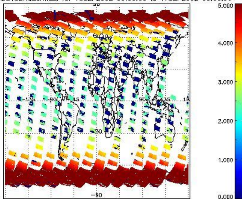
SCIOL2P_NADUV3BRO_amf_cl for 16SEP2002 00:00:00 to 17SEP2002 00:00:00
