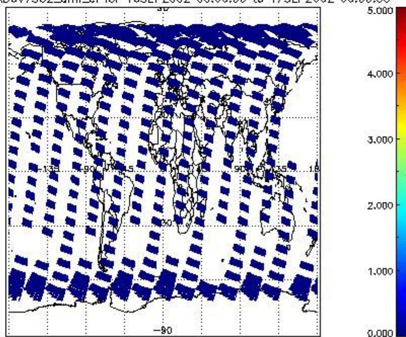
SCIOL2P_NADUV7S02_amf_cl for 16SEP2002 00:00:00 to 17SEP2002 00:00:00
