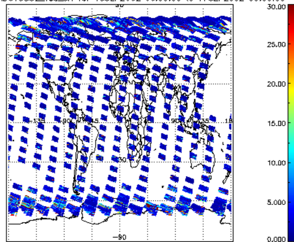
SCIOL2P_NADUV5S02_vcd_err for 16SEP2002 00:00:00 to 17SEP2002 00:00:00
