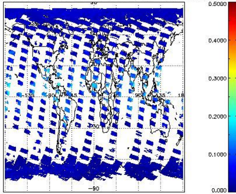
SCIOL2P_NADUV8H2O_vcd_err for 16SEP2002 00:00:00 to 17SEP2002 00:00:00
