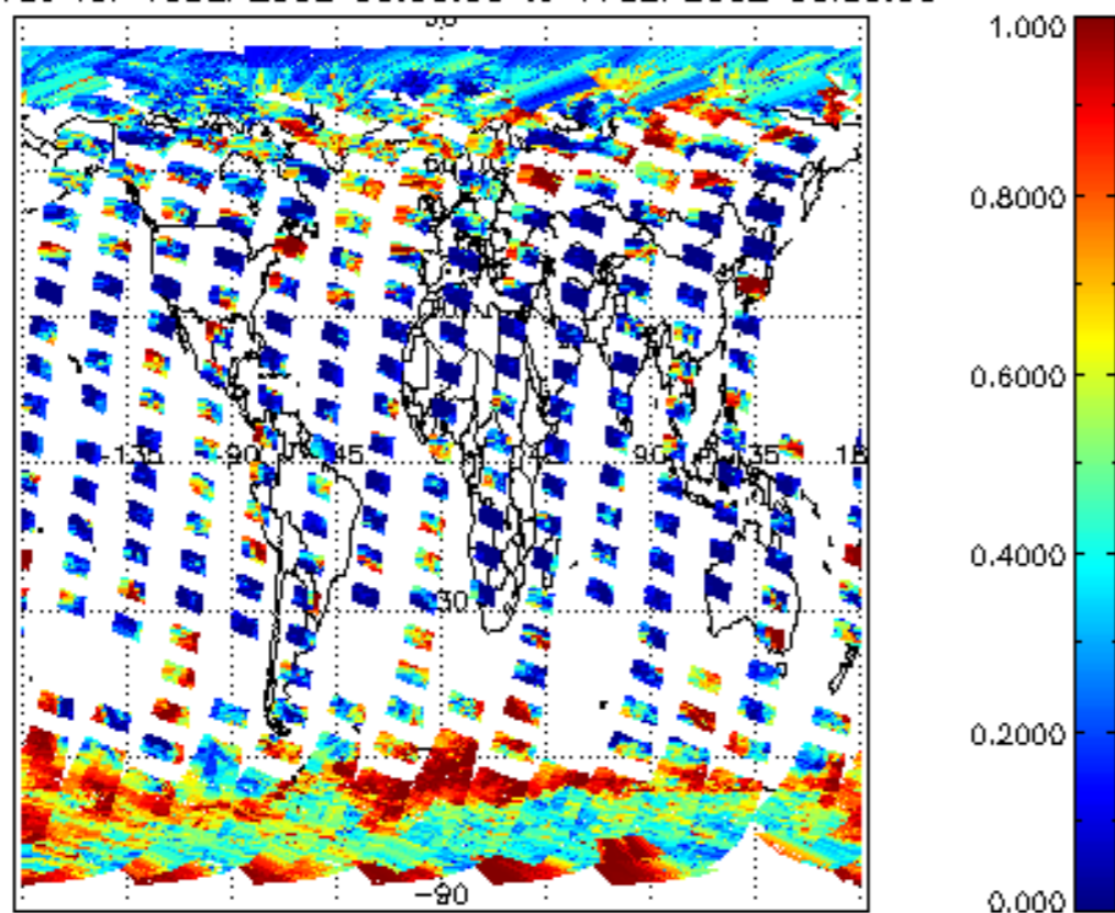
cl_frac for 16SEP2002 00:00:00 to 17SEP2002 00:00:00
