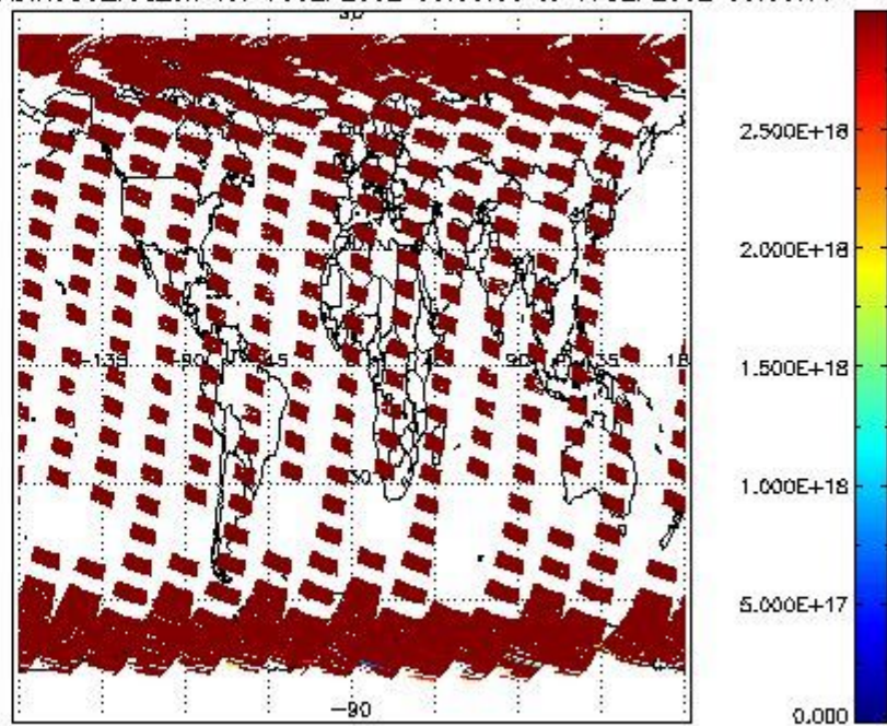
SCIDL2P_NADIR3CO_vcd_err for 16SEP2002 00:00:00 to 17SEP2002 00:00:00
