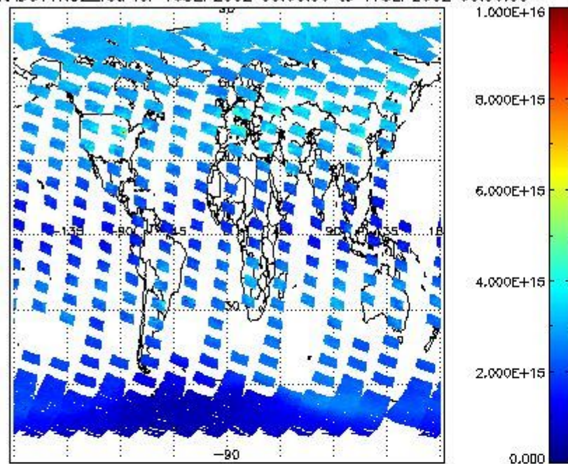
SCIOL2P_NADUV1N02_vcd for 16SEP2002 00:00:00 to 17SEP2002 00:00:00
