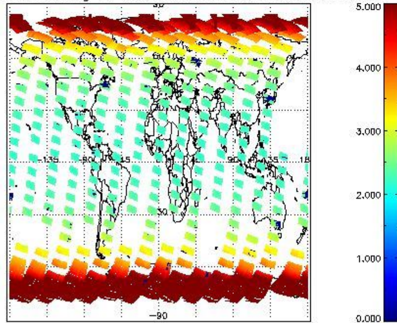
SCIOL2P_NADUV003_amf_gr for 16SEP2002 00:00:00 to 17SEP2002 00:00:00
