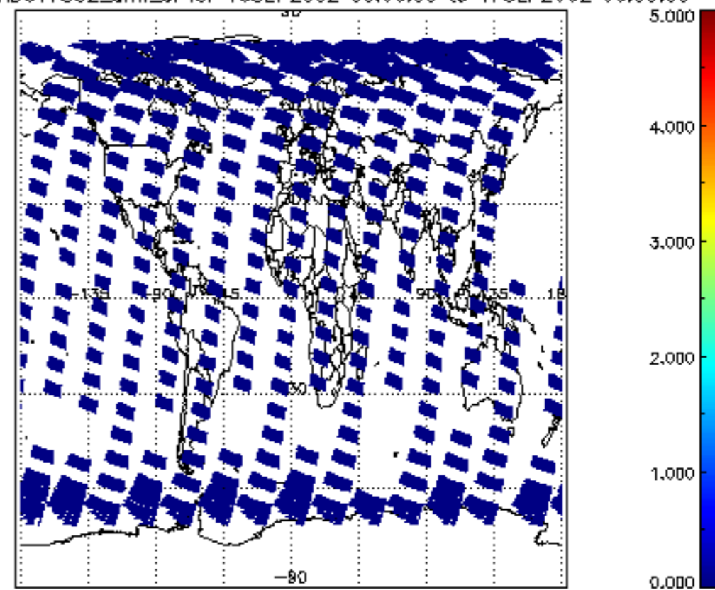
SCIOL2P_NADUV7S02_amf_cl for 16SEP2002 00:00:00 to 17SEP2002 00:00:00
