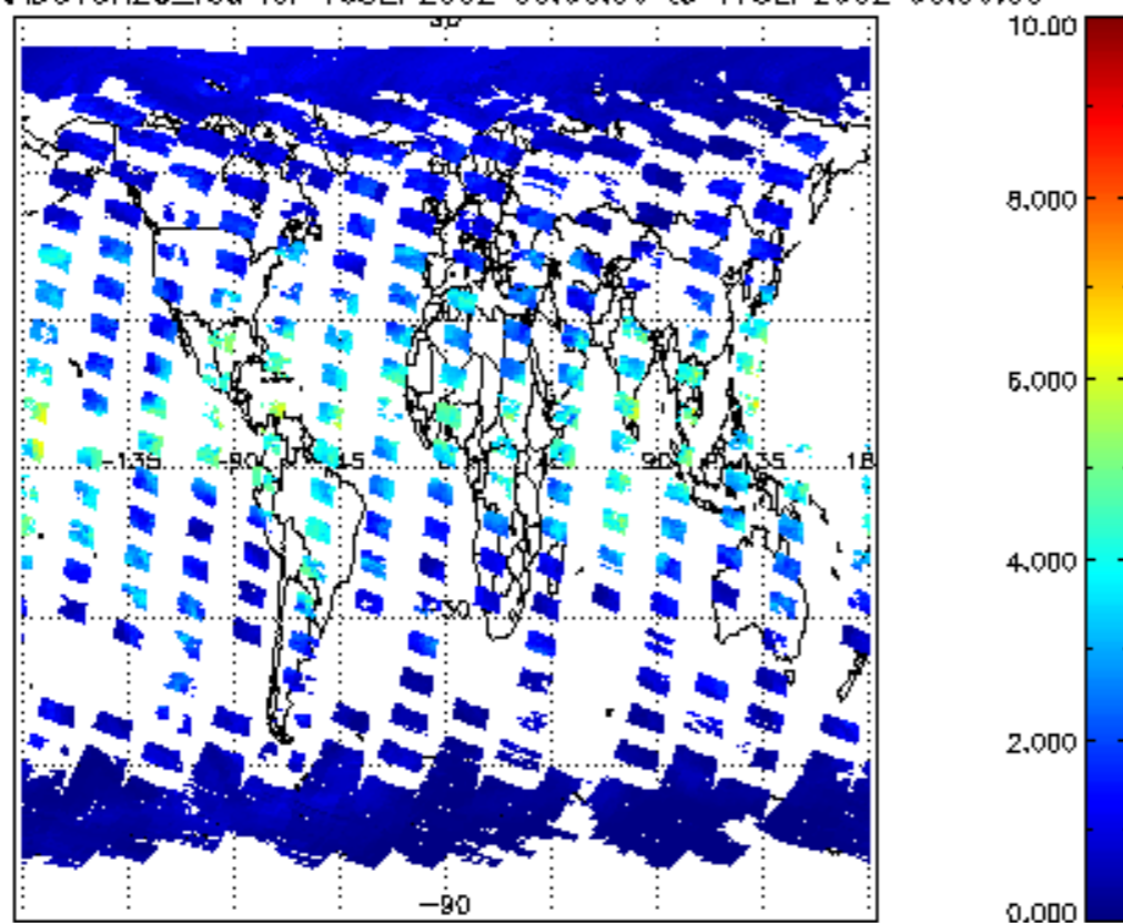
SCIOL2P_NADUV8H20_vcd for 16SEP2002 00:00:00 to 17SEP2002 00:00:00
