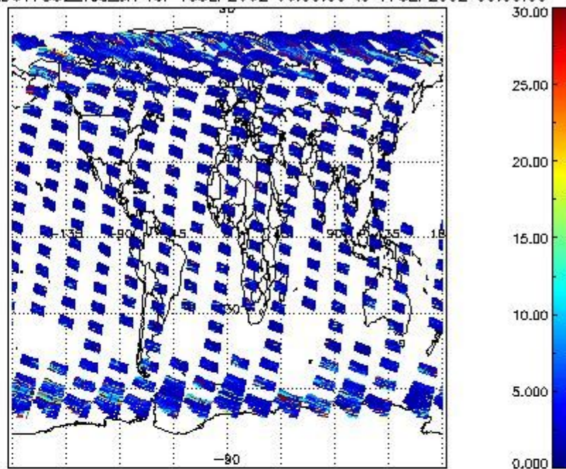
SCIOL2P_NADUV7S02_vcd_err for 16SEP2002 00:00:00 to 17SEP2002 00:00:00
