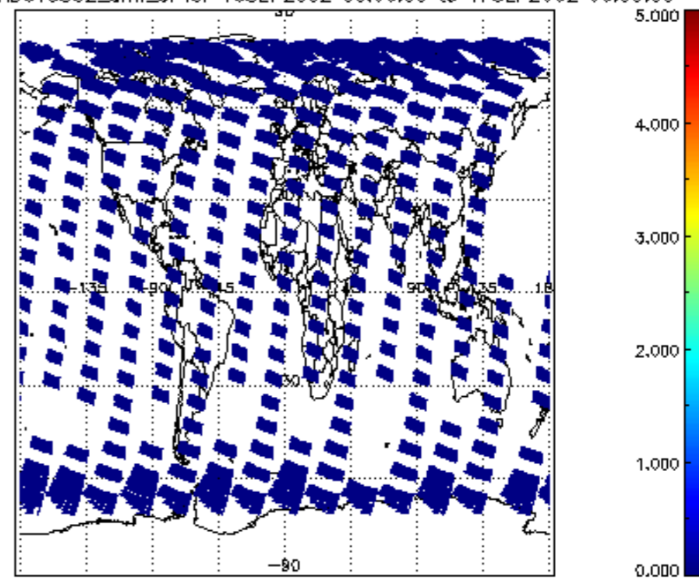
SCIOL2P_NADUV5S02_amf_cl for 16SEP2002 00:00:00 to 17SEP2002 00:00:00
