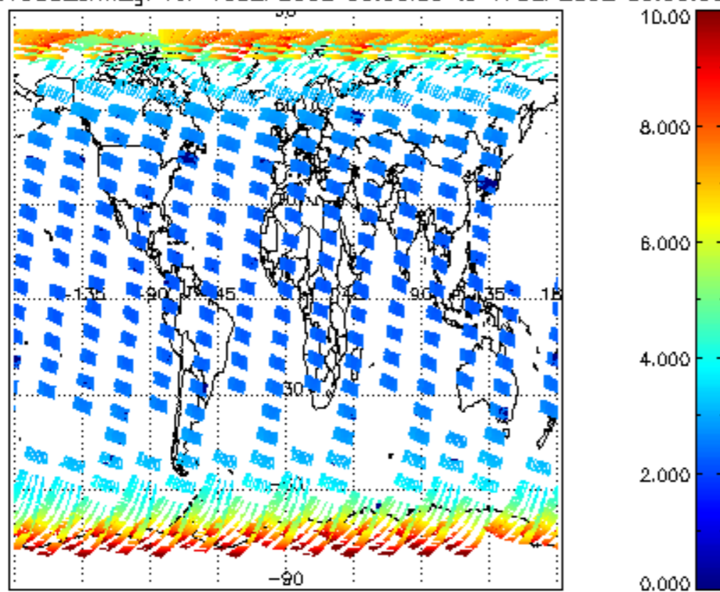
SCIOL2P_NADUV003_amf_gr for 16SEP2002 00:00:00 to 17SEP2002 00:00:00
