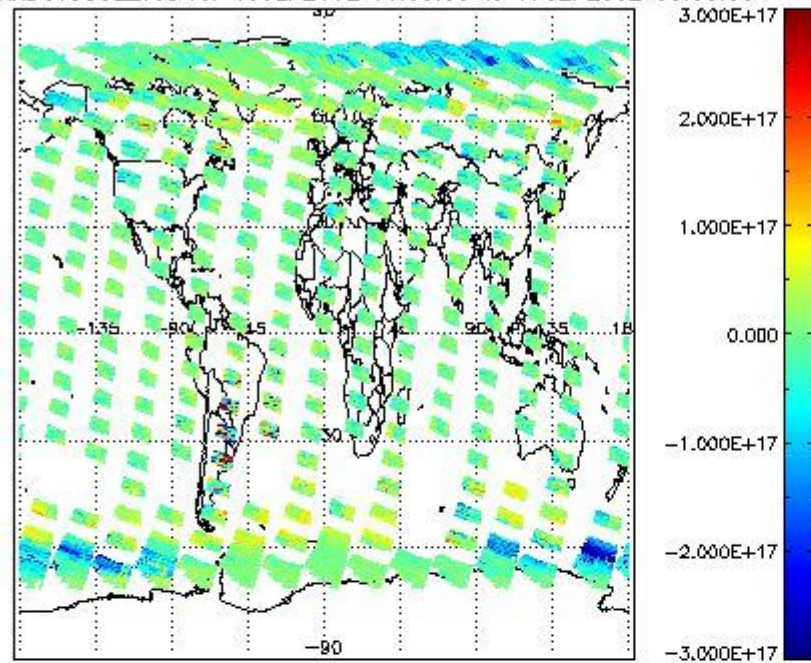
SCIOL2P_NADUV5S02_vcd for 16SEP2002 00:00:00 to 17SEP2002 00:00:00
