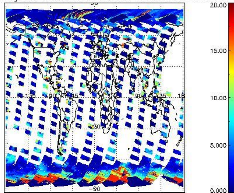
cL_top_height for 16SEP2002 00:00:00 to 17SEP2002 00:00:00
