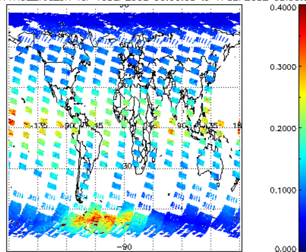
iCIOL2P_NADUV1NO2_vcd_err for 16SEP2002 00:00:00 to 17SEP2002 00:00:00
