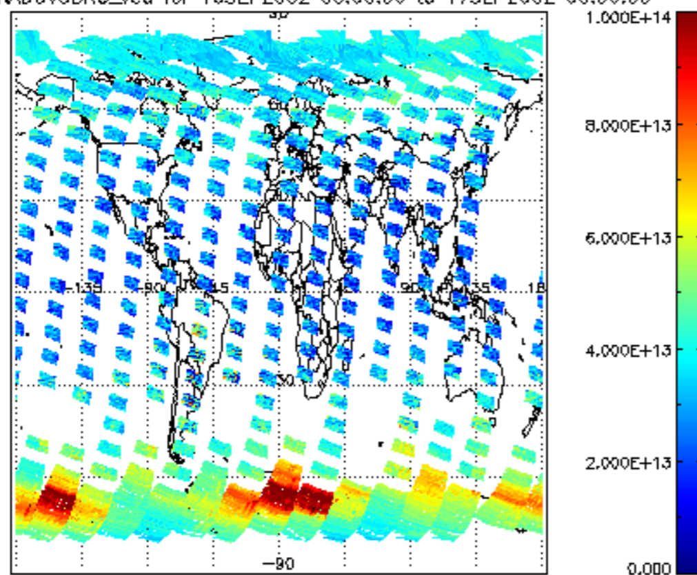
SCIOL2P_NADUV3BRO_vcd for 16SEP2002 00:00:00 to 17SEP2002 00:00:00
