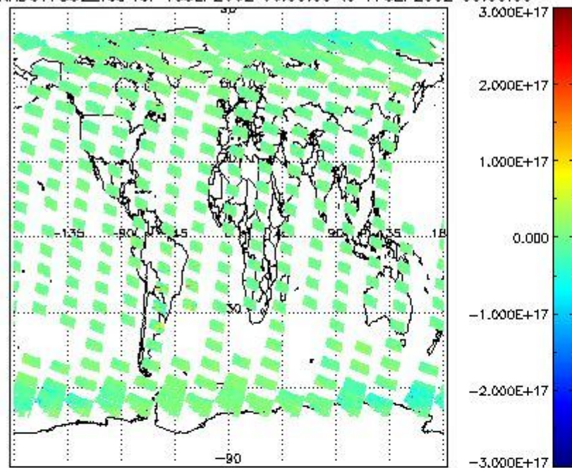
SCIOL2P_NADUV7S02_vcd for 16SEP2002 00:00:00 to 17SEP2002 00:00:00
