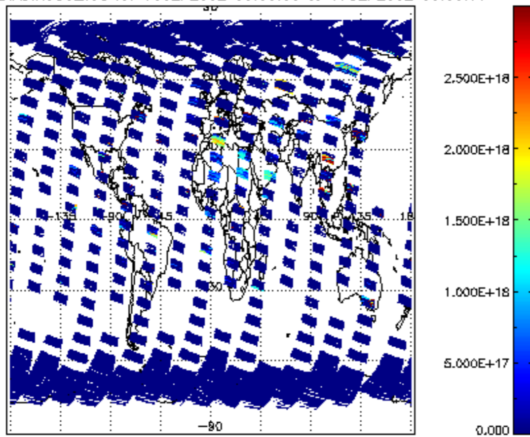
SCIOL2P_NADIR3CO_vcd for 16SEP2002 00:00:00 to 17SEP2002 00:00:00
