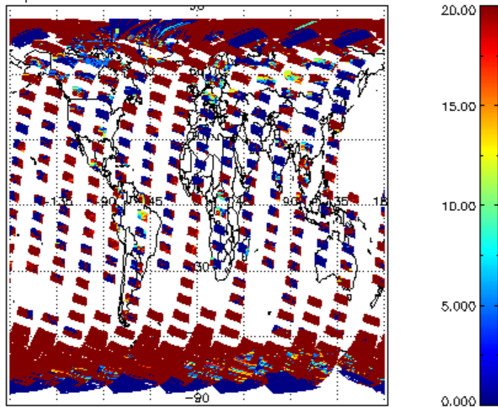
cl_opt_depth for 16SEP2002 00:00:00 to 17SEP2002 00:00:00
