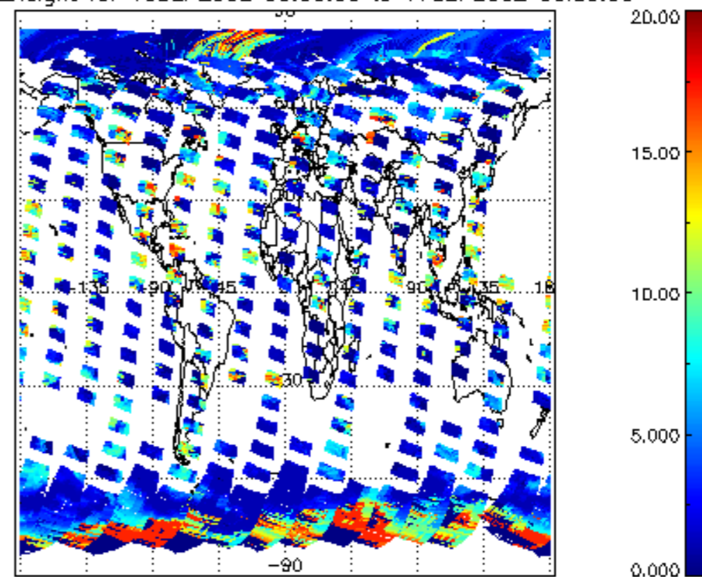
cl_top_height for 16SEP2002 00:00:00 to 17SEP2002 00:00:00
