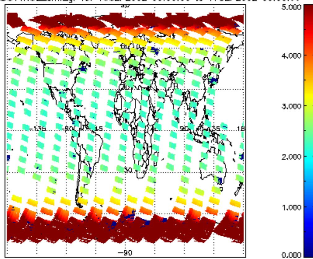
SCIOL2P_NADUV1NO2_amf_gr for 16SEP2002 00:00:00 to 17SEP2002 00:00:00
