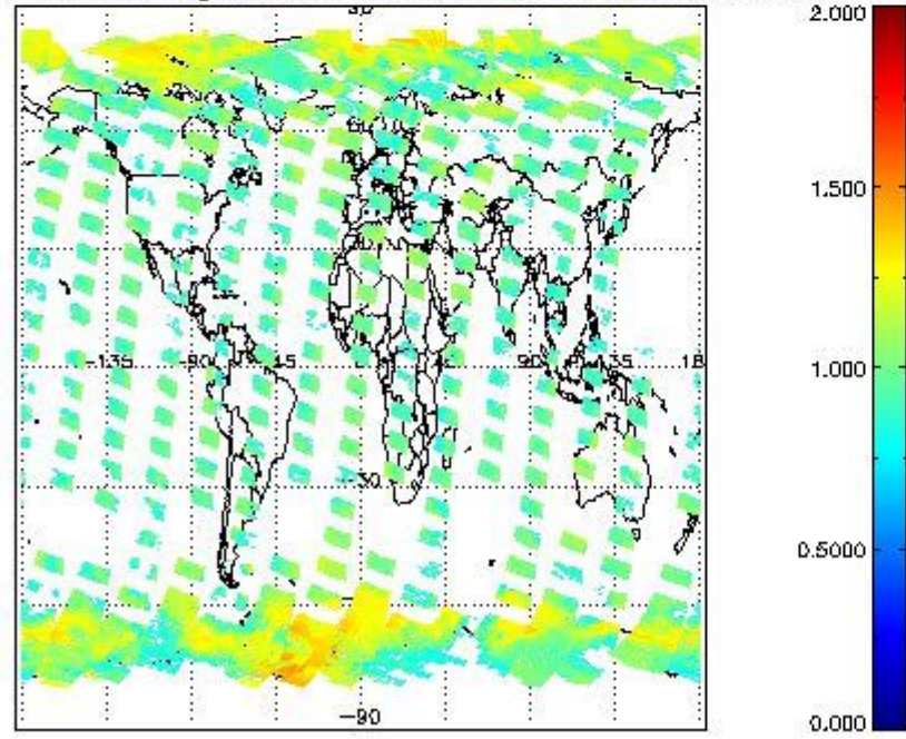
SCIOL2P_NADUV8H2O_arnf_gr for 16SEP2002 00:00:00 to 17SEP2002 00:00:00
