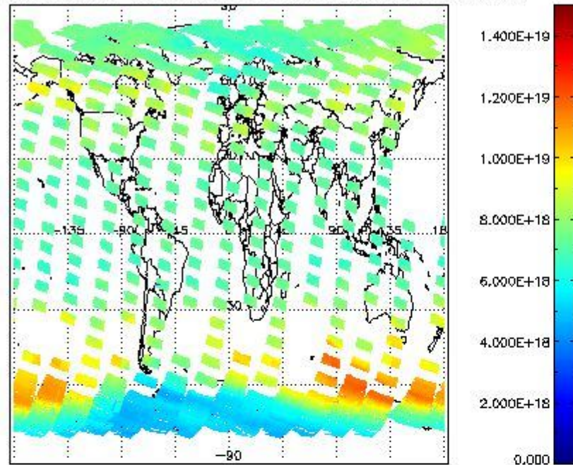
SCIOL2P_NADUV003_vcd for 16SEP2002 00:00:00 to 17SEP2002 00:00:00
