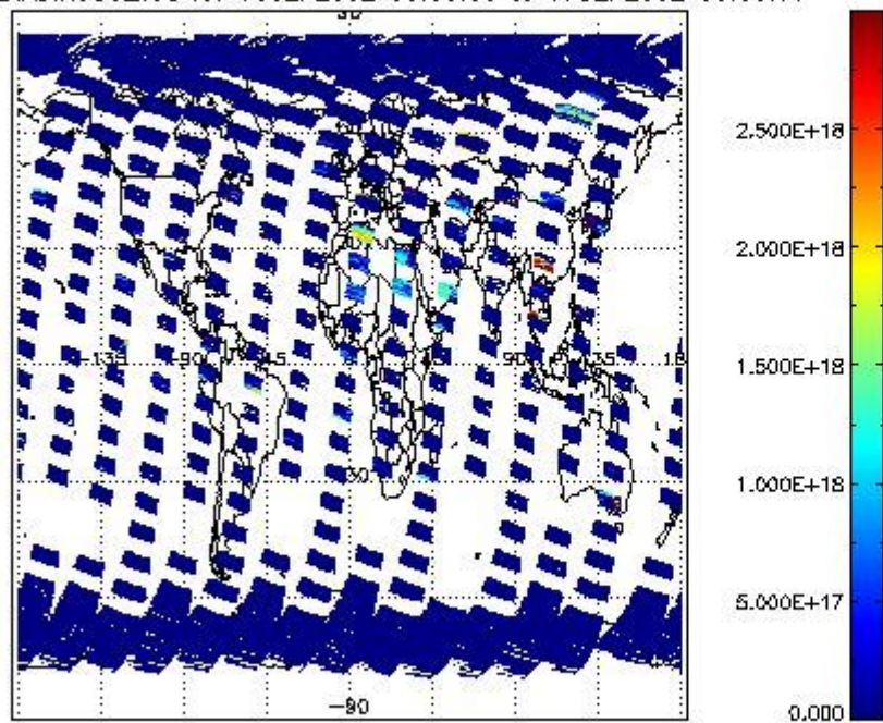
SCIDL2P_NADIR3CO_vcd for 16SEP2002 00:00:00 to 17SEP2002 00:00:00
