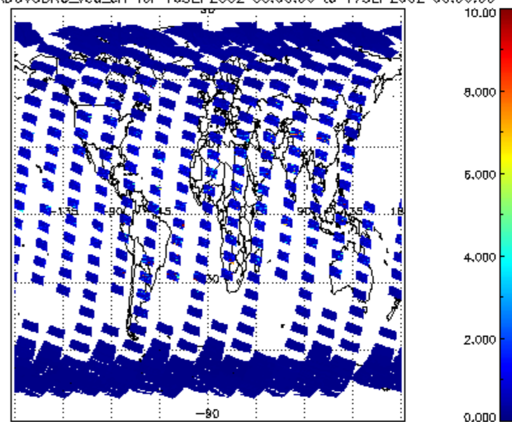
SCIOL2P_NADUV3BRO_vcd_err for 16SEP2002 00:00:00 to 17SEP2002 00:00:00
