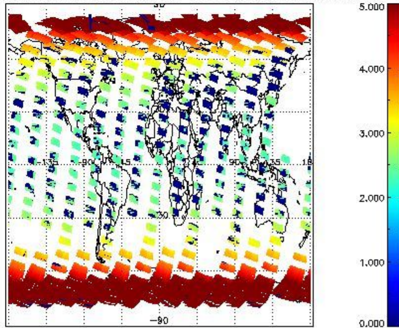
SCIOL2P_NADUV003_amf_cl for 16SEP2002 00:00:00 to 17SEP2002 00:00:00
