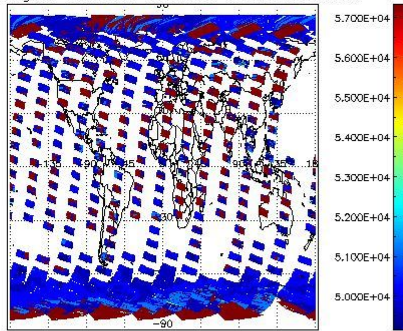
cloud_flags for 16SEP2002 00:00:00 to 17SEP2002 00:00:00
