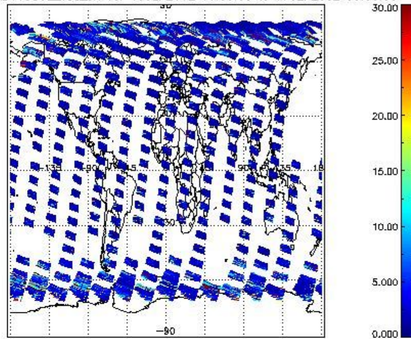
SCIOL2P_NADUV5S02_vcd_err for 16SEP2002 00:00:00 to 17SEP2002 00:00:00
