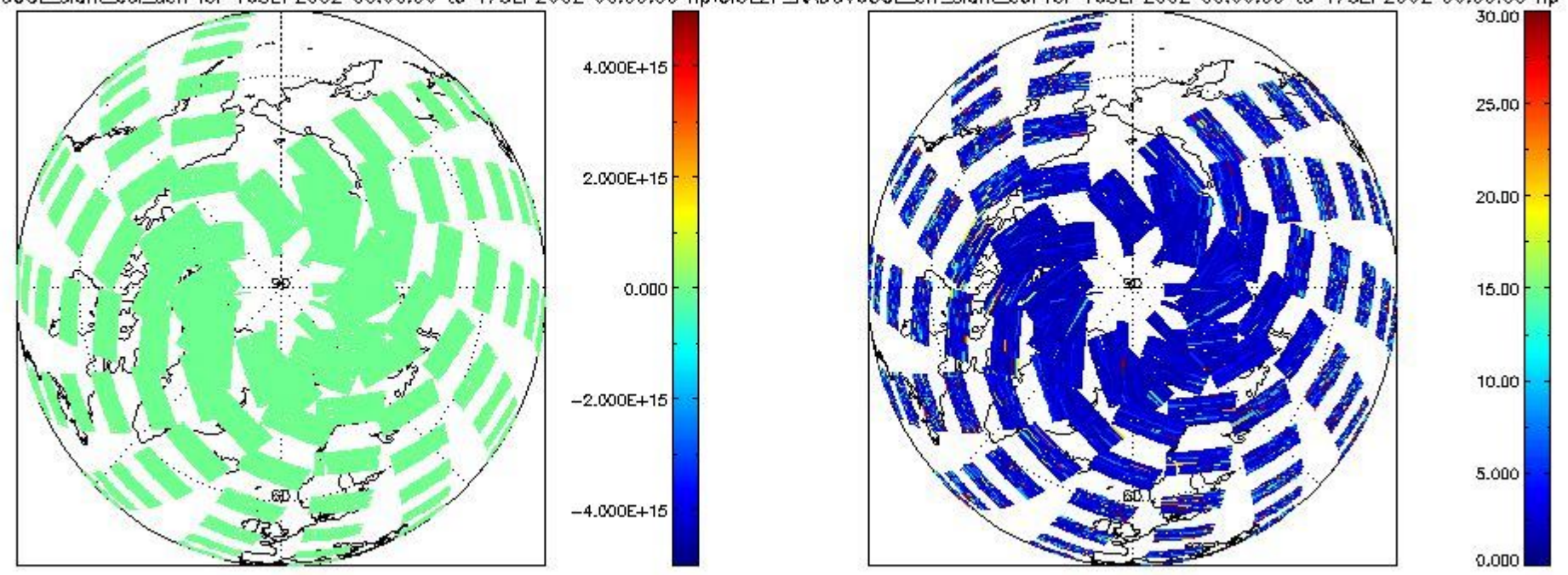
CIOL2P_NADUV60CLslant_col_den for 16SEP2002 00:00:00 to 17SEP2002 00:00:00 np; CIOL2P_NADUV60CLerr_slant_col for 16SEP2002 00:00:00 to 17SEP2002 00:00:00 np
