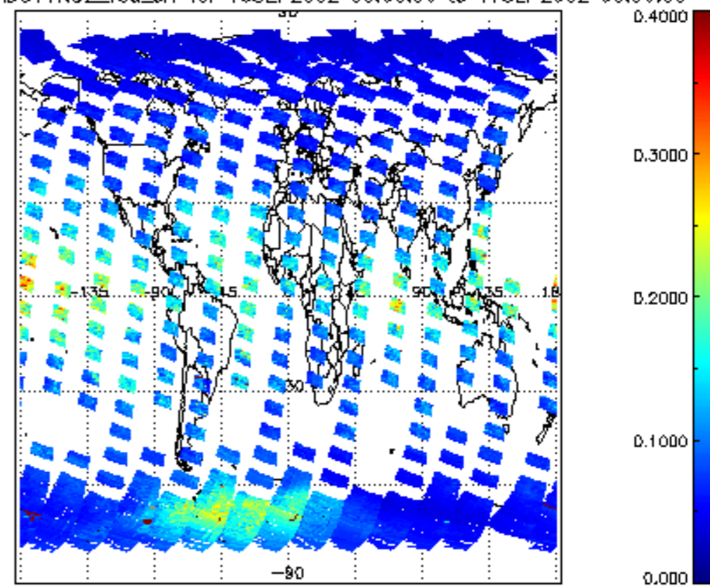
SCIOL2P_NADUV1NO2_vcd_err for 16SEP2002 00:00:00 to 17SEP2002 00:00:00
