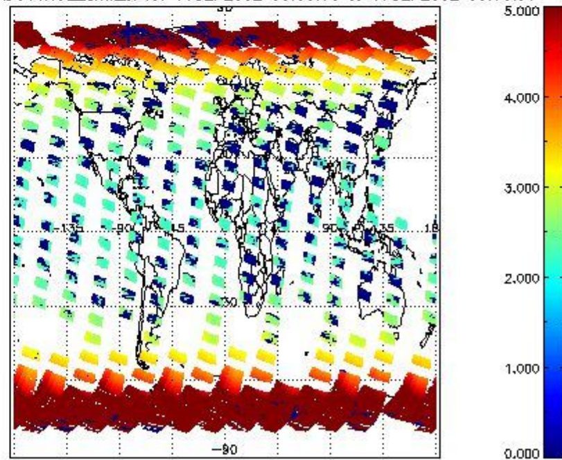
SCIOL2P_NADUV1N02_amf_cl for 16SEP2002 00:00:00 to 17SEP2002 00:00:00
