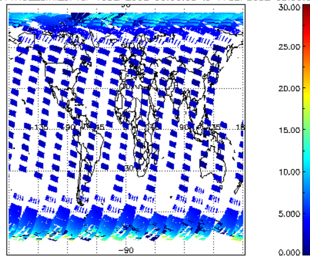
iCIOL2P_NADUV1NO2_amf_cl for 16SEP2002 00:00:00 to 17SEP2002 00:00:00
