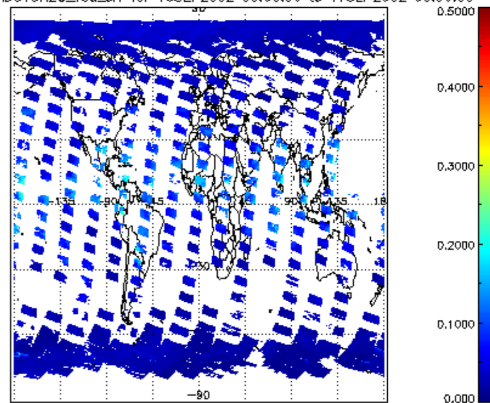
SCIOL2P_NADUV8H20_vcd_err for 16SEP2002 00:00:00 to 17SEP2002 00:00:00
