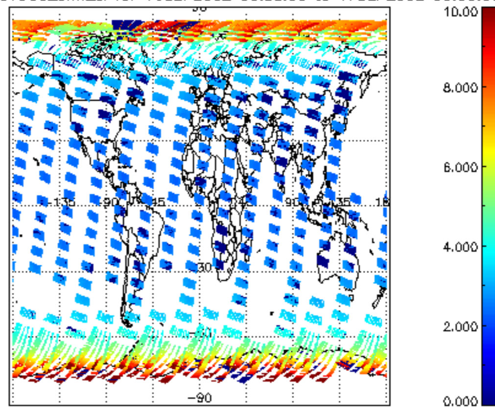
SCIOL2P_NADUV003_amf_cl for 16SEP2002 00:00:00 to 17SEP2002 00:00:00
