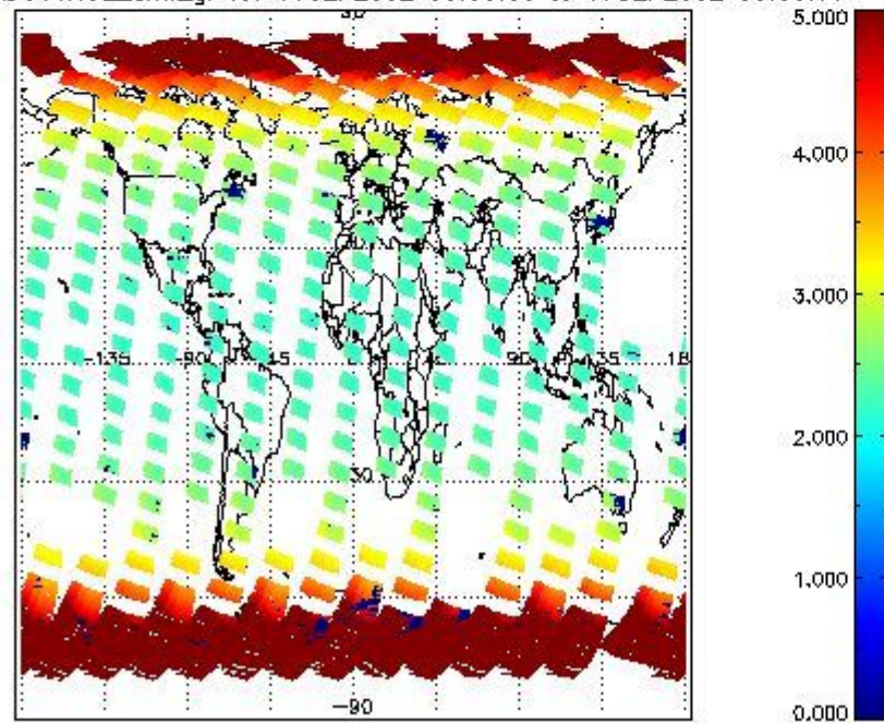
SCIOL2P_NADUV1N02_amf_gr for 16SEP2002 00:00:00 to 17SEP2002 00:00:00
