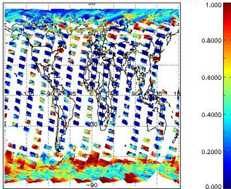
cL_frac for 16SEP2002 00:00:00 to 17SEP2002 00:00:00
