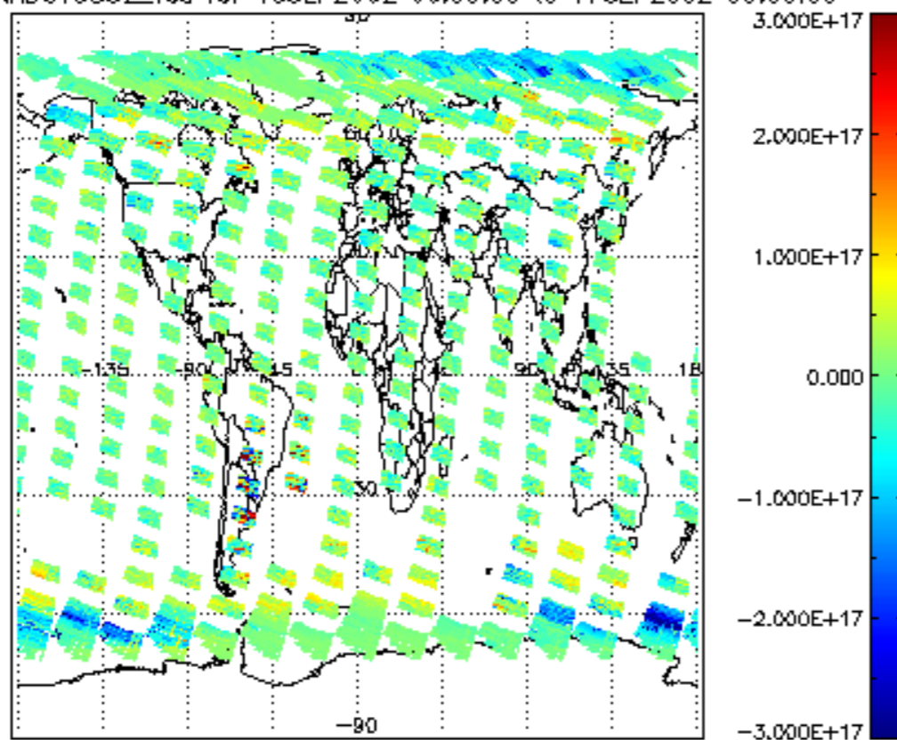
SCIOL2P_NADUV5S02_vcd for 16SEP2002 00:00:00 to 17SEP2002 00:00:00
