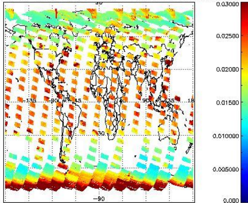
SCIOL2P_NADUV003_vcd_err for 16SEP2002 00:00:00 to 17SEP2002 00:00:00
