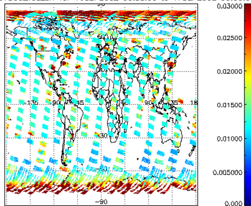
SCIOL2P_NADUV003_vcd_err for 16SEP2002 00:00:00 to 17SEP2002 00:00:00
