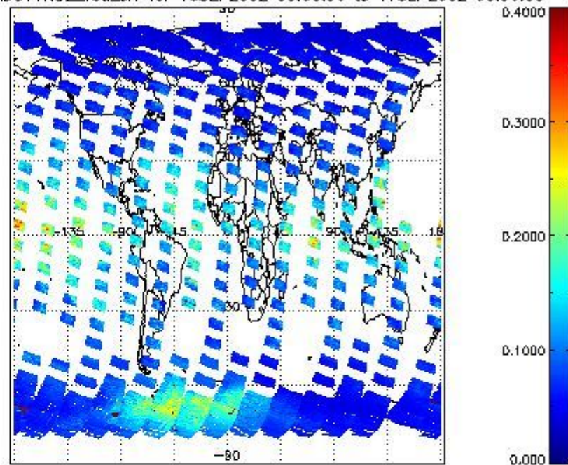
SCIOL2P_NADUV1N02_vcd_err for 16SEP2002 00:00:00 to 17SEP2002 00:00:00
