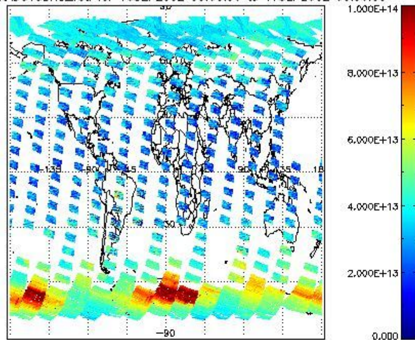
SCIOL2P_NADUV3BRO_vcd for 16SEP2002 00:00:00 to 17SEP2002 00:00:00
