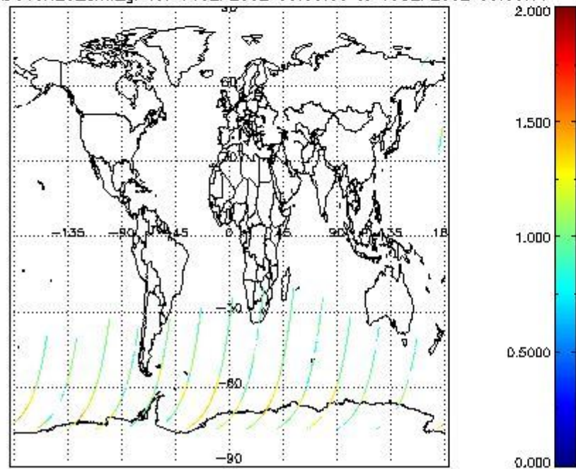
SCIOL2P_NADUV8H2O_arnf_gr for 14SEP2002 00:00:00 to 15SEP2002 00:00:00
