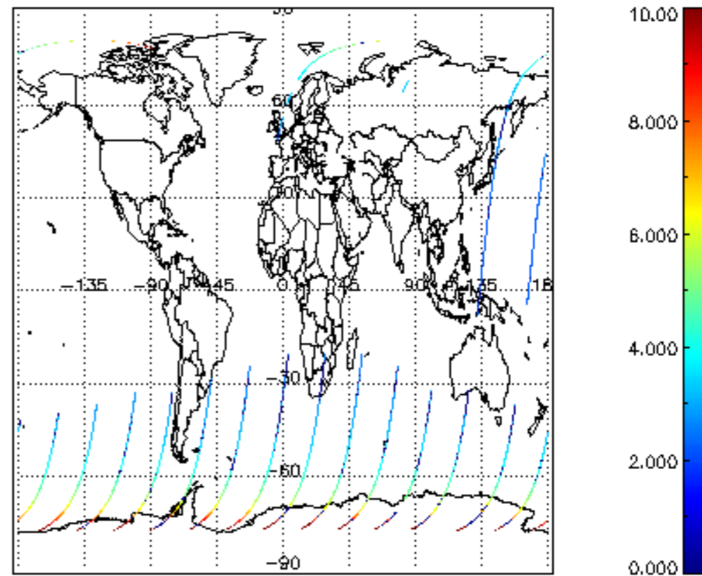
SCIOL2P_NADUV003_amf_cl for 14SEP2002 00:00:00 to 15SEP2002 00:00:00
