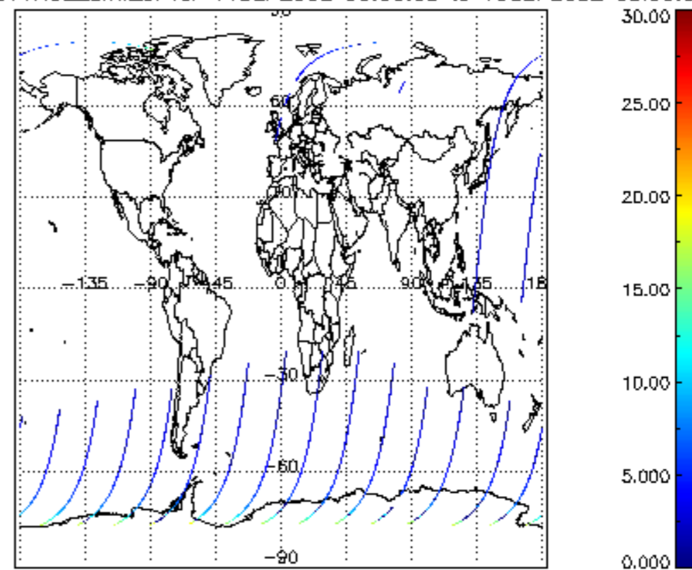
iCIOL2P_NADUV1NO2_amf_cl for 14SEP2002 00:00:00 to 15SEP2002 00:00:00
