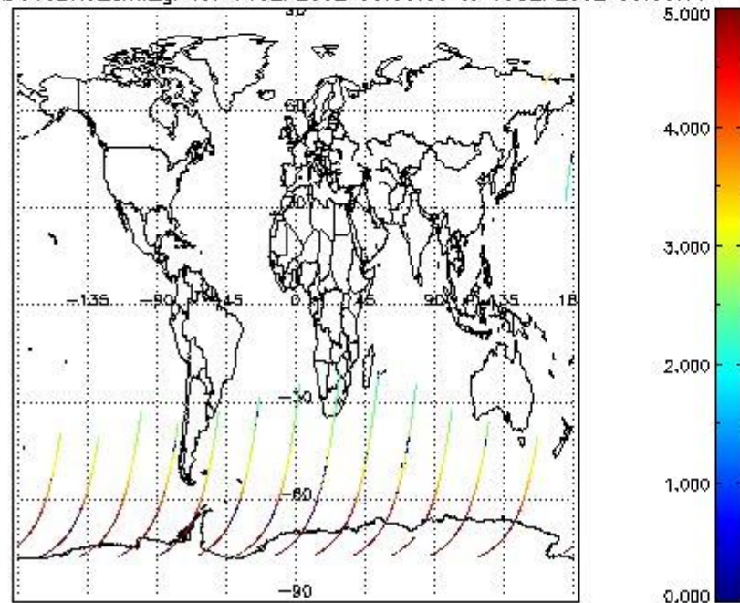
SCIOL2P_NADUV3BRO_amf_gr for 14SEP2002 00:00:00 to 15SEP2002 00:00:00
