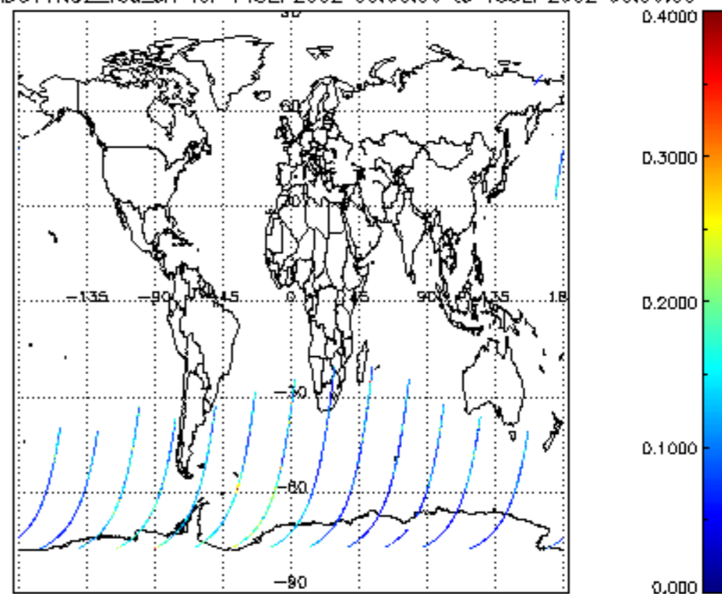
SCIOL2P_NADUV1NO2_vcd_err for 14SEP2002 00:00:00 to 15SEP2002 00:00:00
