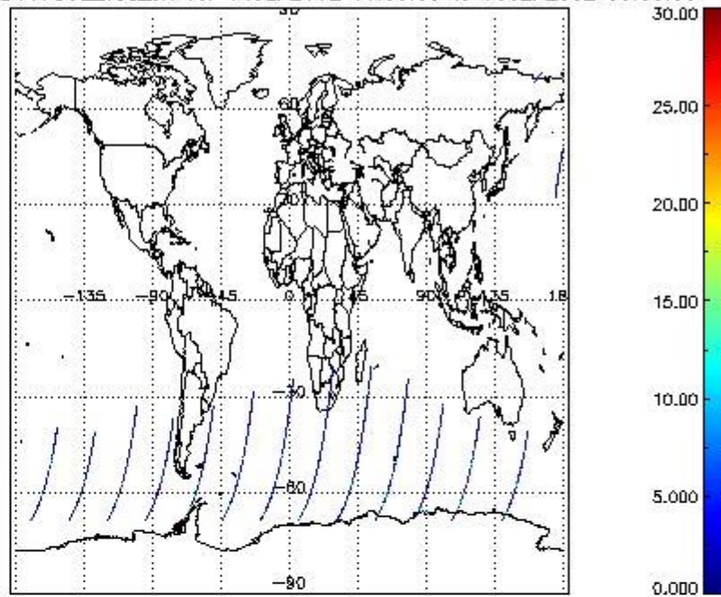
SCIOL2P_NADUV7S02_vcd_err for 14SEP2002 00:00:00 to 15SEP2002 00:00:00
