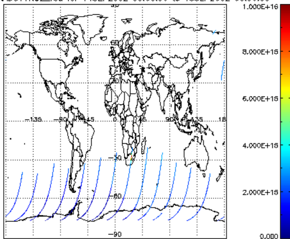
SCIOL2P_NADUV1NO2_vcd for 14SEP2002 00:00:00 to 15SEP2002 00:00:00
