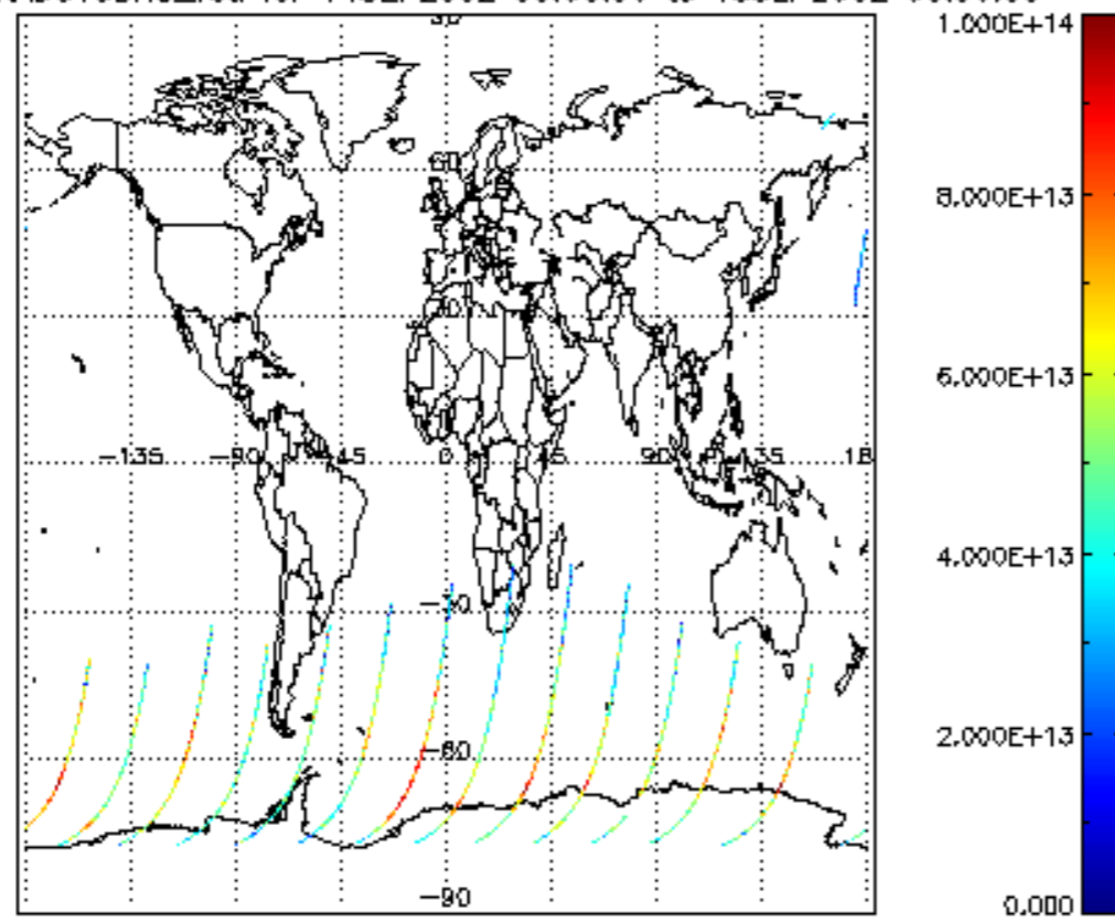
SCIOL2P_NADUV3BRO_vcd for 14SEP2002 00:00:00 to 15SEP2002 00:00:00
