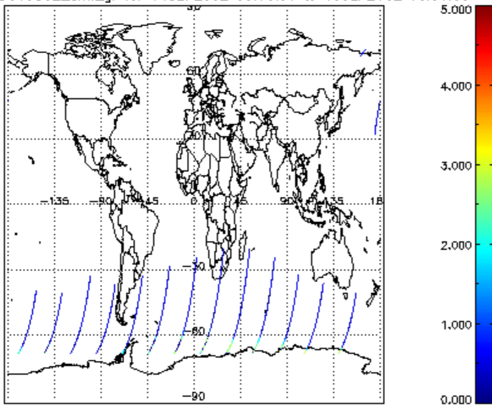
SCIOL2P_NADUV5S02_amf_gr for 14SEP2002 00:00:00 to 15SEP2002 00:00:00
