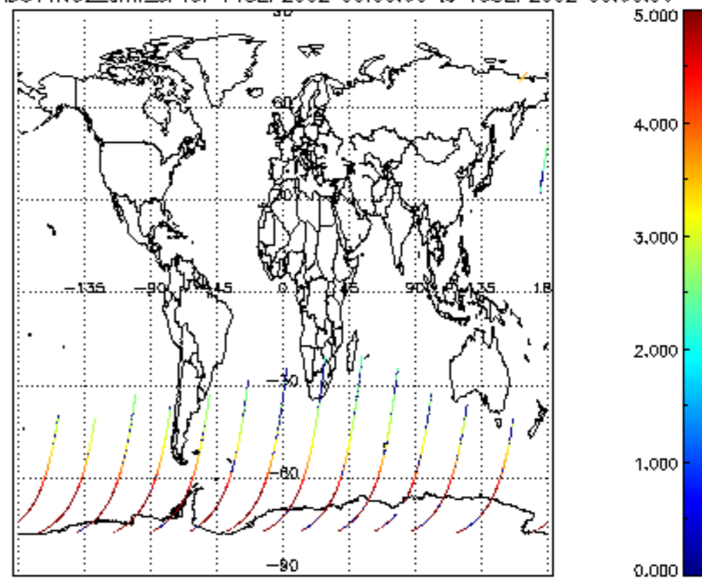
SCIOL2P_NADUV1NO2_amf_cl for 14SEP2002 00:00:00 to 15SEP2002 00:00:00
