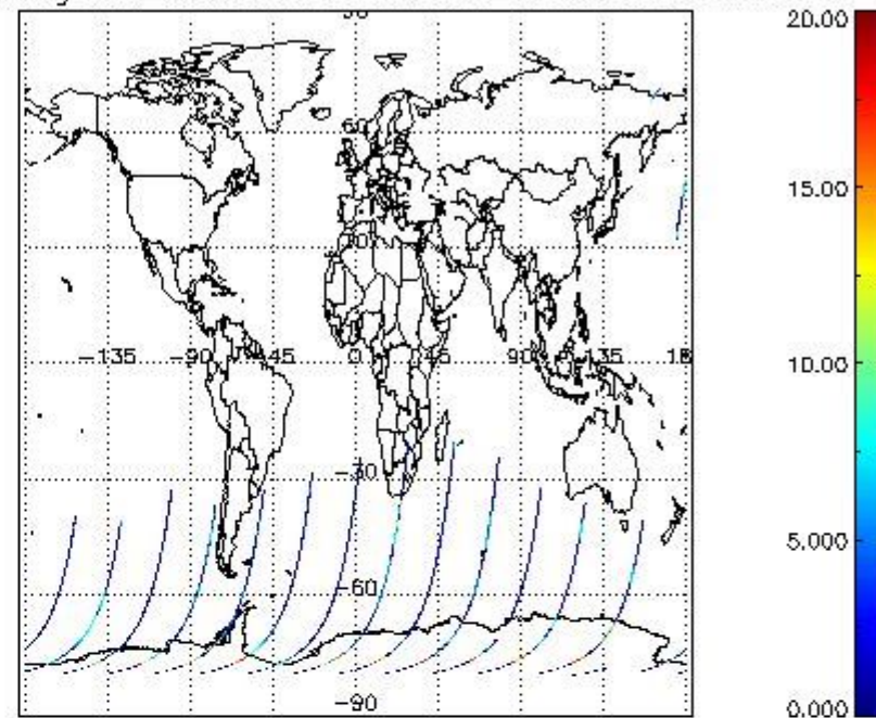
cL_top_height for 14SEP2002 00:00:00 to 15SEP2002 00:00:00
