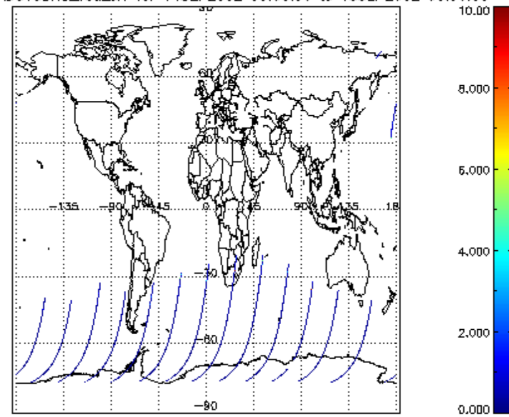
SCIOL2P_NADUV3BRO_vcd_err for 14SEP2002 00:00:00 to 15SEP2002 00:00:00
