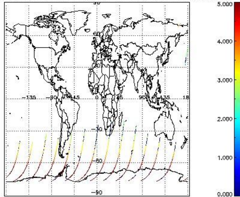
SCIOL2P_NADUV003_amf_cl for 14SEP2002 00:00:00 to 15SEP2002 00:00:00
