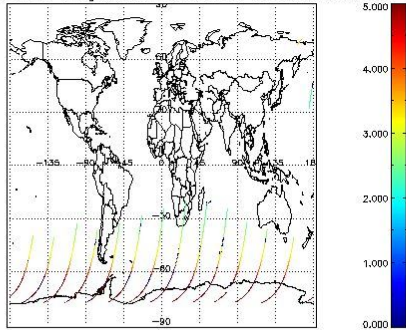
SCIOL2P_NADUV1NO2_amf_gr for 14SEP2002 00:00:00 to 15SEP2002 00:00:00
