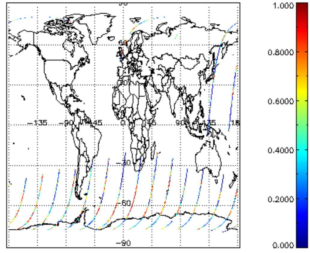
cl_frac for 14SEP2002 00:00:00 to 15SEP2002 00:00:00
