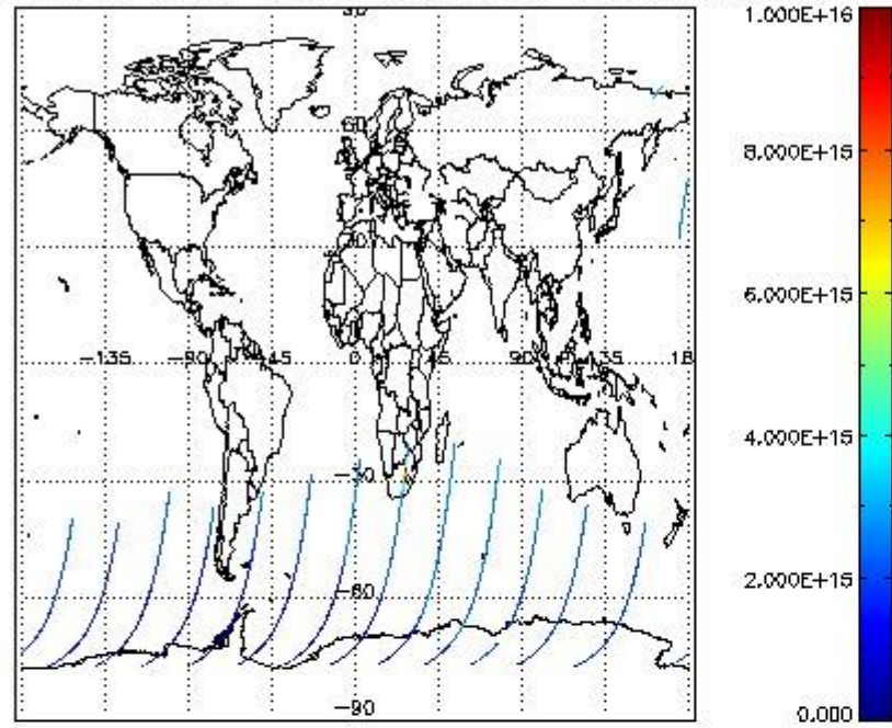
SCIOL2P_NADUV1NO2_vcd for 14SEP2002 00:00:00 to 15SEP2002 00:00:00
