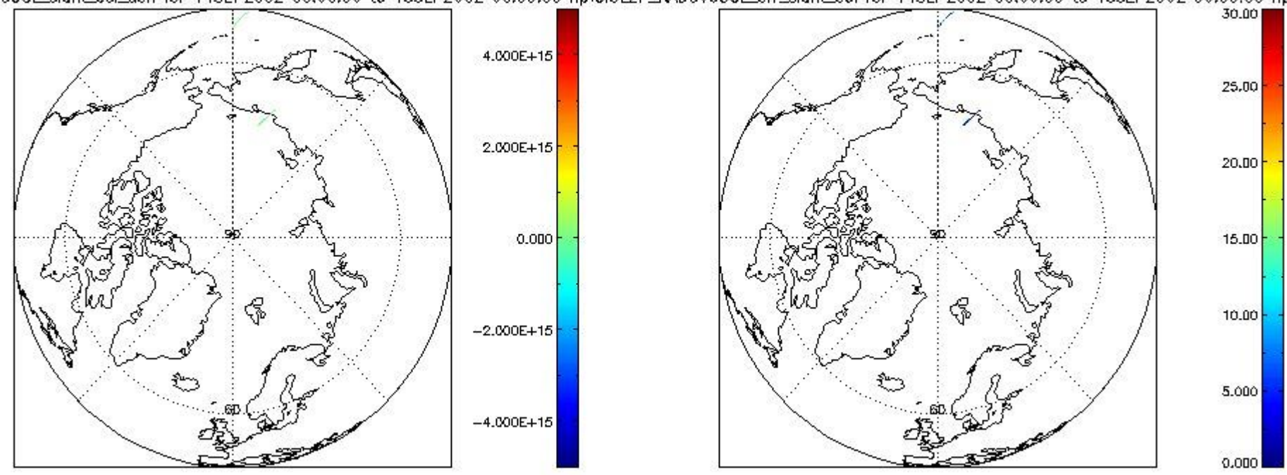
CIOL2P_NADUV60CLslant_col_den for 14SEP2002 00:00:00 to 15SEP2002 00:00:00 np; CIOL2P_NADUV60CLarr_slant_col for 14SEP2002 00:00:00 to 15SEP2002 00:00:00 np
