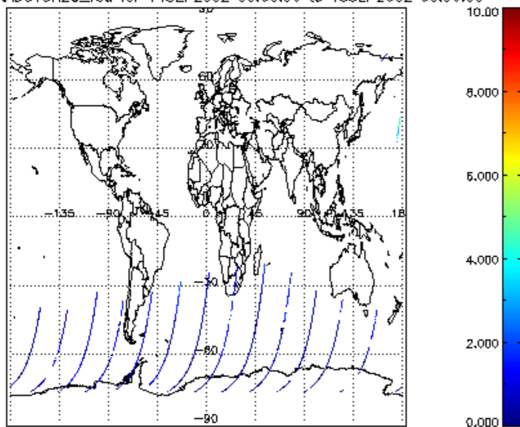
SCIOL2P_NADUV8H2O_vcd for 14SEP2002 00:00:00 to 15SEP2002 00:00:00
