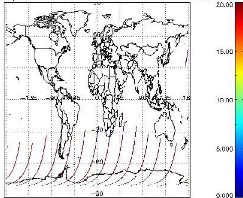
cL_opt_depth for 14SEP2002 00:00:00 to 15SEP2002 00:00:00
