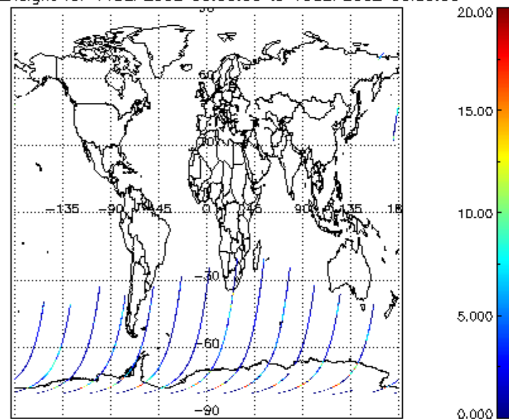
cl_top_height for 14SEP2002 00:00:00 to 15SEP2002 00:00:00
