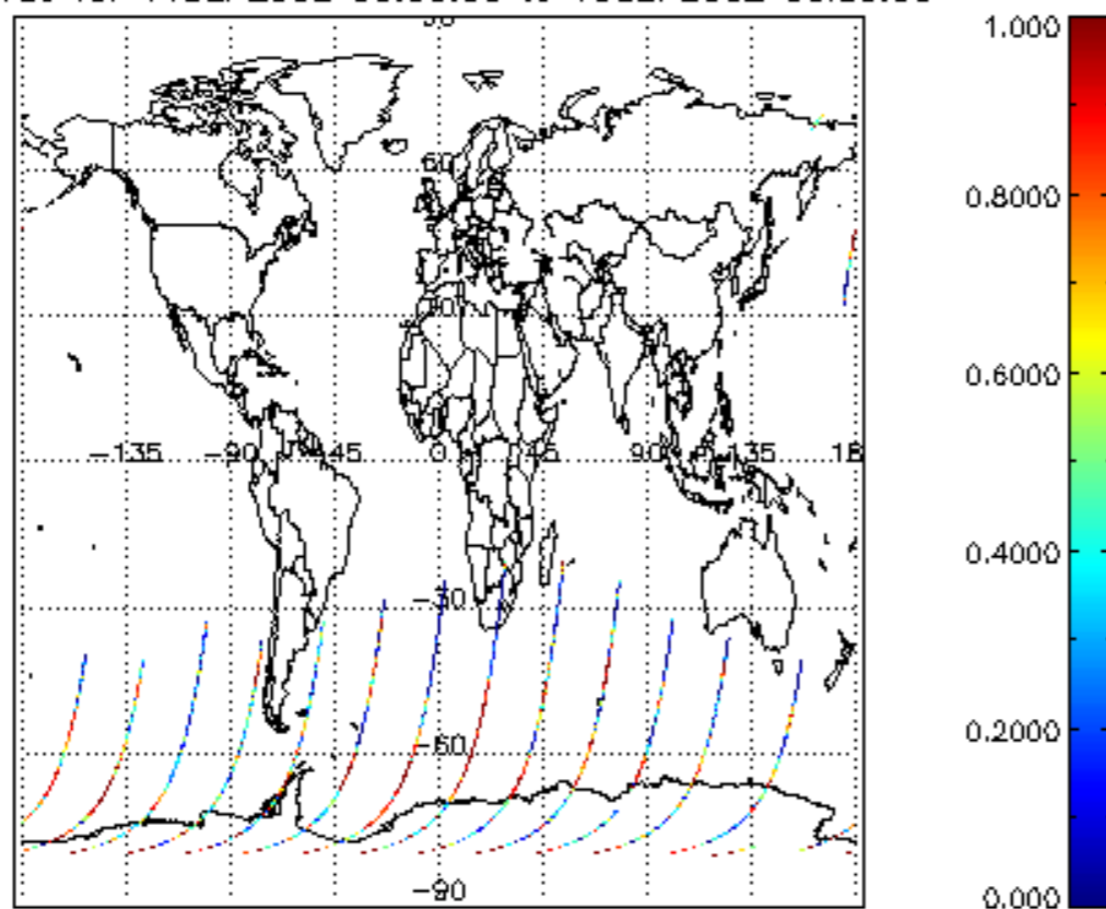
cl_frac for 14SEP2002 00:00:00 to 15SEP2002 00:00:00
