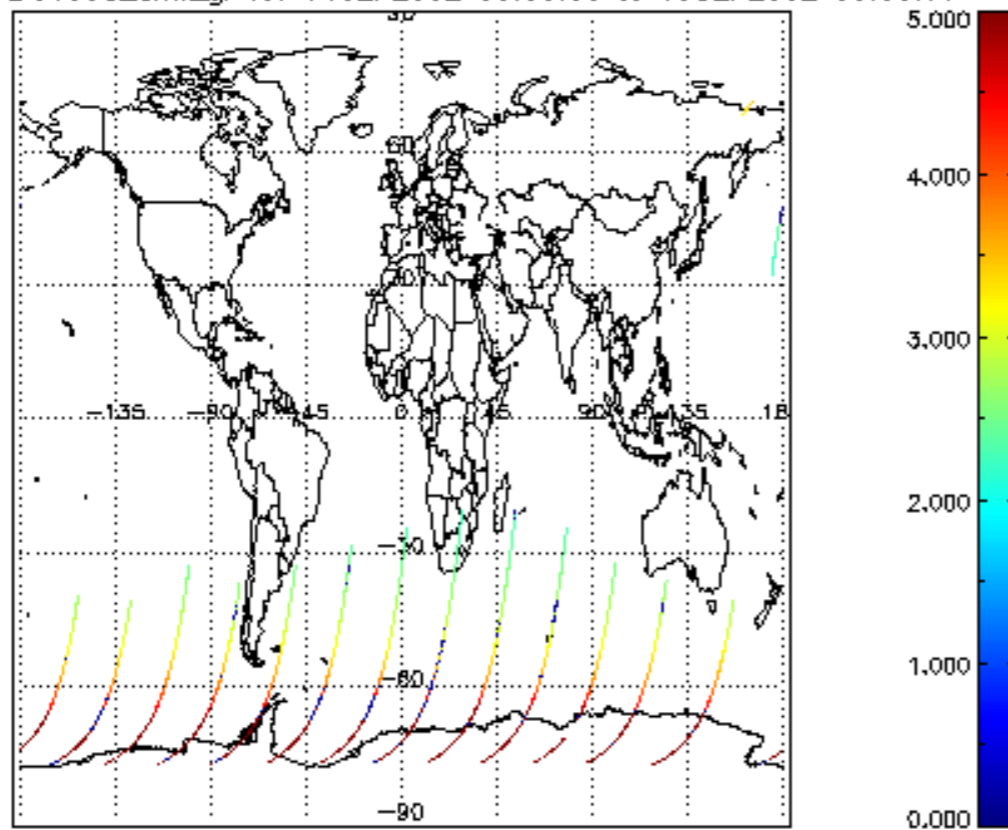
SCIOL2P_NADUV003_amf_gr for 14SEP2002 00:00:00 to 15SEP2002 00:00:00
