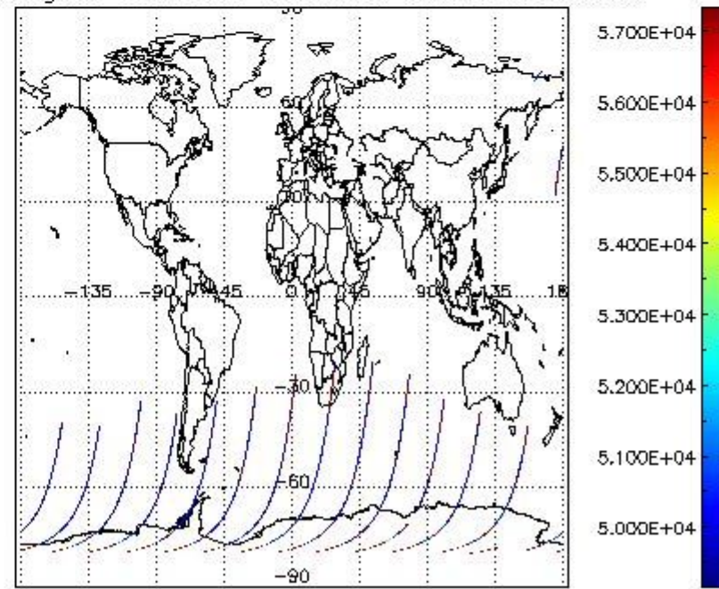
cloud_flags for 14SEP2002 00:00:00 to 15SEP2002 00:00:00
