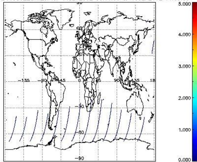
SCIOL2P_NADUV5S02_amf_cl for 14SEP2002 00:00:00 to 15SEP2002 00:00:00
