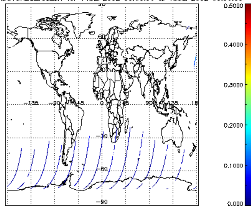
SCIOL2P_NADUV8H2O_vcd_err for 14SEP2002 00:00:00 to 15SEP2002 00:00:00
