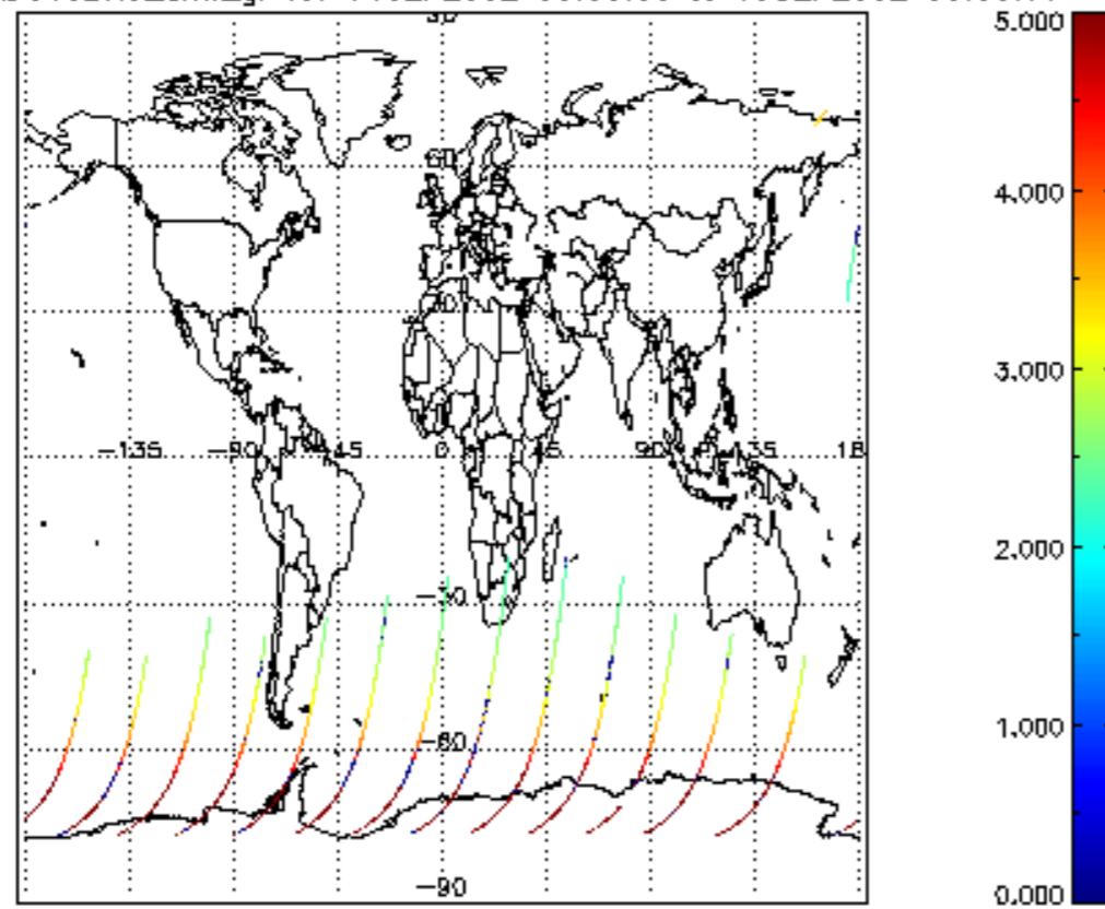
SCIOL2P_NADUV3BRO_amf_gr for 14SEP2002 00:00:00 to 15SEP2002 00:00:00
