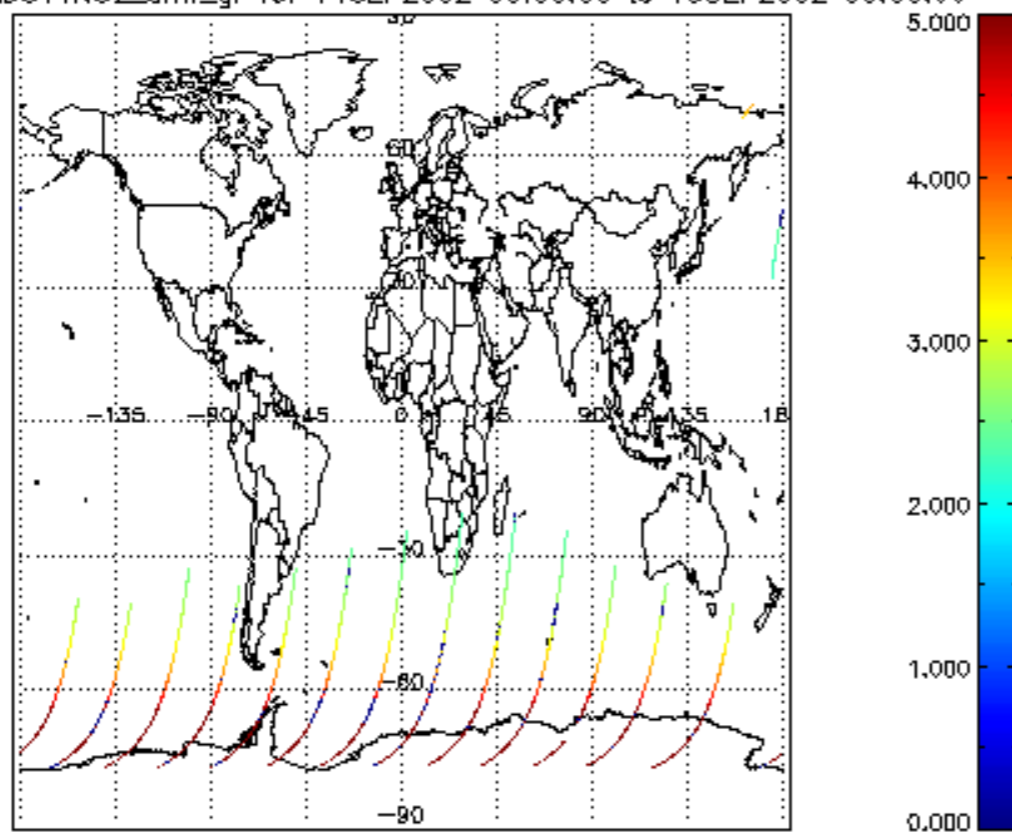
SCIOL2P_NADUV1NO2_amf_gr for 14SEP2002 00:00:00 to 15SEP2002 00:00:00
