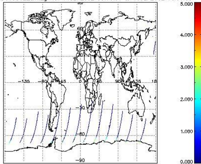
SCIOL2P_NADUV5S02_amf_gr for 14SEP2002 00:00:00 to 15SEP2002 00:00:00
