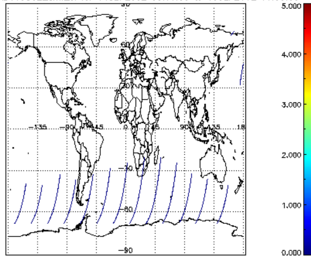
SCIOL2P_NADUV5S02_amf_cl for 14SEP2002 00:00:00 to 15SEP2002 00:00:00
