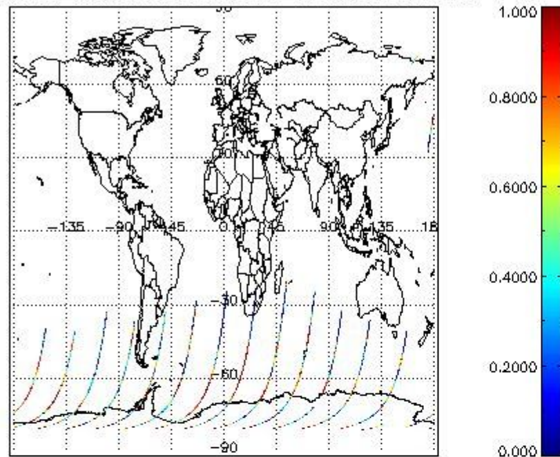
cL_frac for 14SEP2002 00:00:00 to 15SEP2002 00:00:00
