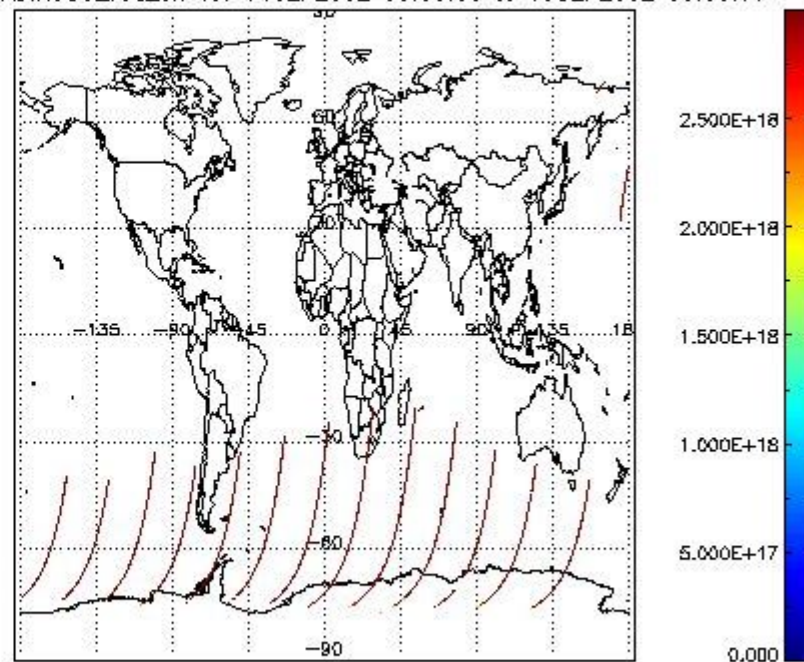
SCIDL2P_NADIR3CO_vcd_err for 14SEP2002 00:00:00 to 15SEP2002 00:00:00
