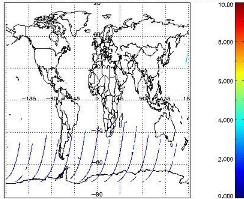
SCIOL2P_NADUV8H2O_vcd for 14SEP2002 00:00:00 to 15SEP2002 00:00:00
