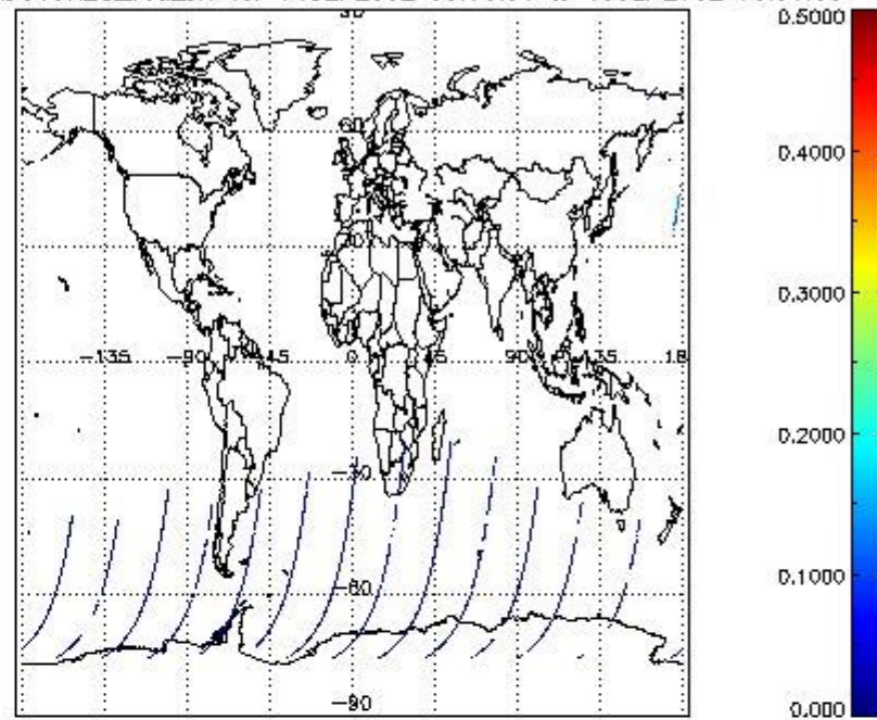
SCIOL2P_NADUV8H2O_vcd_err for 14SEP2002 00:00:00 to 15SEP2002 00:00:00
