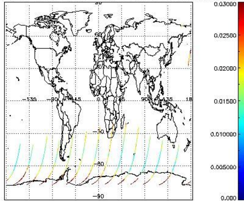
SCIOL2P_NADUV003_vcd_err for 14SEP2002 00:00:00 to 15SEP2002 00:00:00
