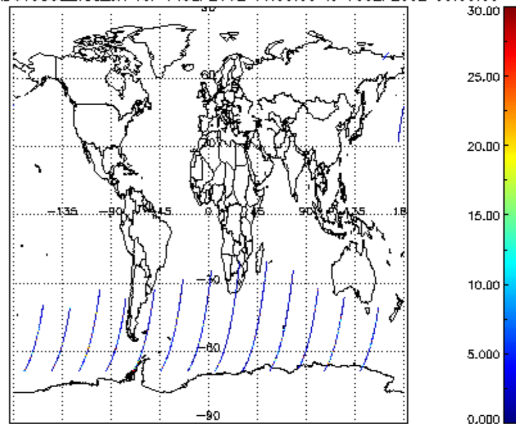
SCIOL2P_NADUV5S02_vcd_err for 14SEP2002 00:00:00 to 15SEP2002 00:00:00
