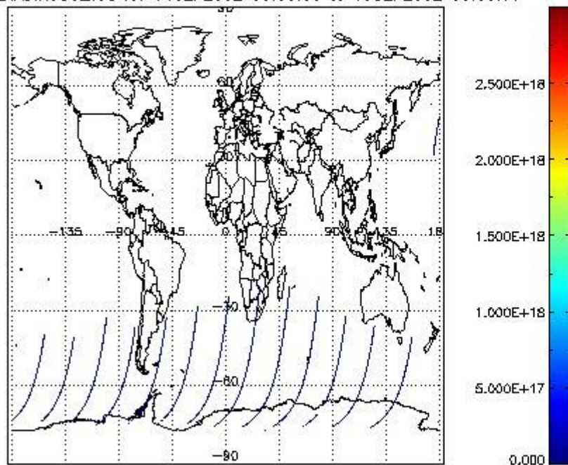
SCIDL2P_NADIR3CO_vcd for 14SEP2002 00:00:00 to 15SEP2002 00:00:00
