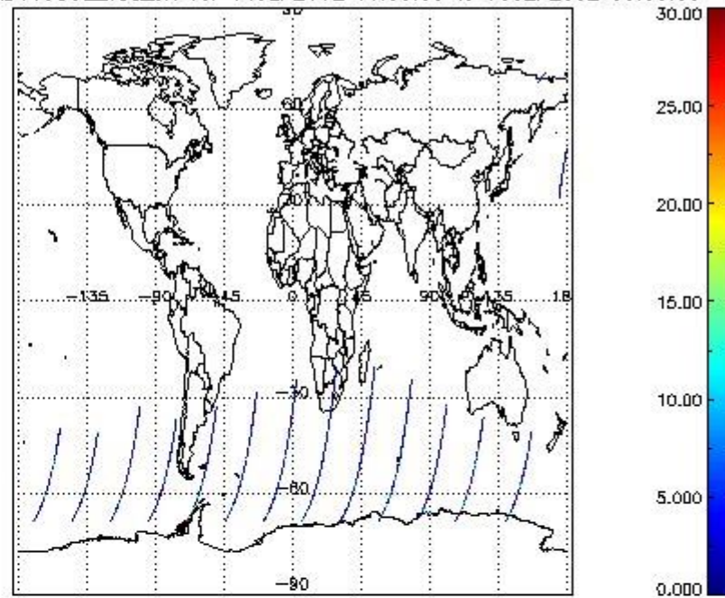
SCIOL2P_NADUV5S02_vcd_err for 14SEP2002 00:00:00 to 15SEP2002 00:00:00
