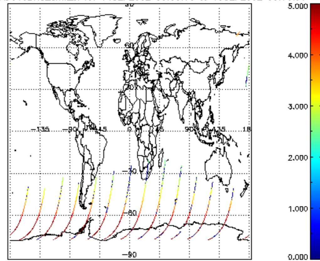
SCIOL2P_NADUV3BRO_amf_cl for 14SEP2002 00:00:00 to 15SEP2002 00:00:00
