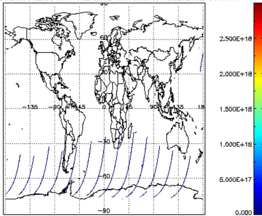
SCIOL2P_NADIR3CO_vcd for 14SEP2002 00:00:00 to 15SEP2002 00:00:00
