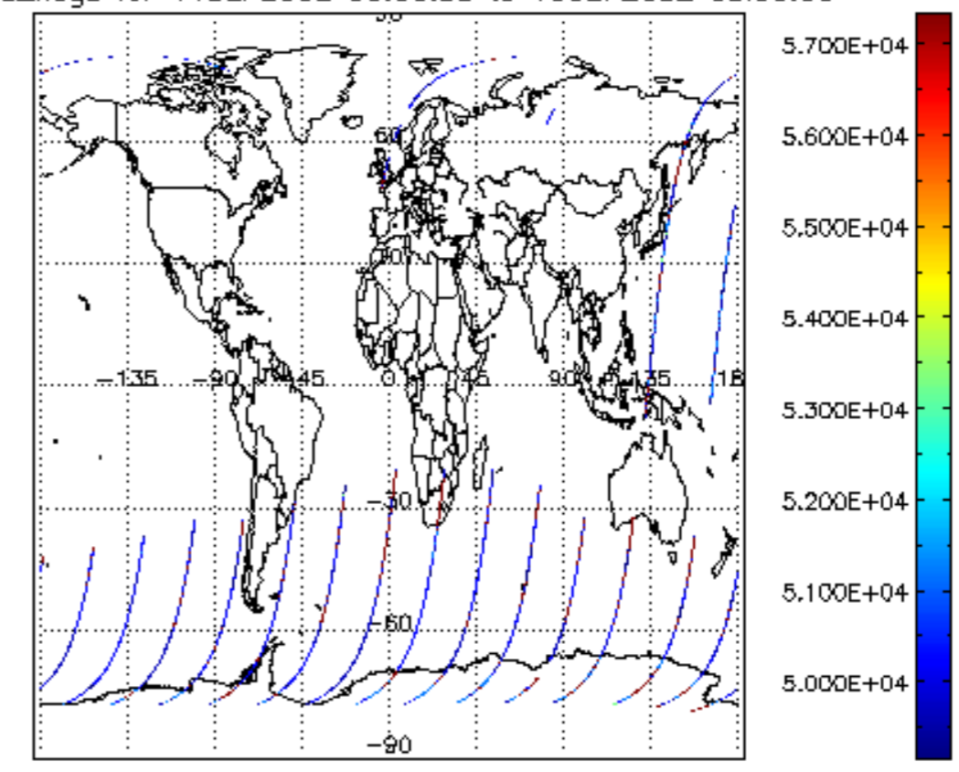
cloud_flags for 14SEP2002 00:00:00 to 15SEP2002 00:00:00
