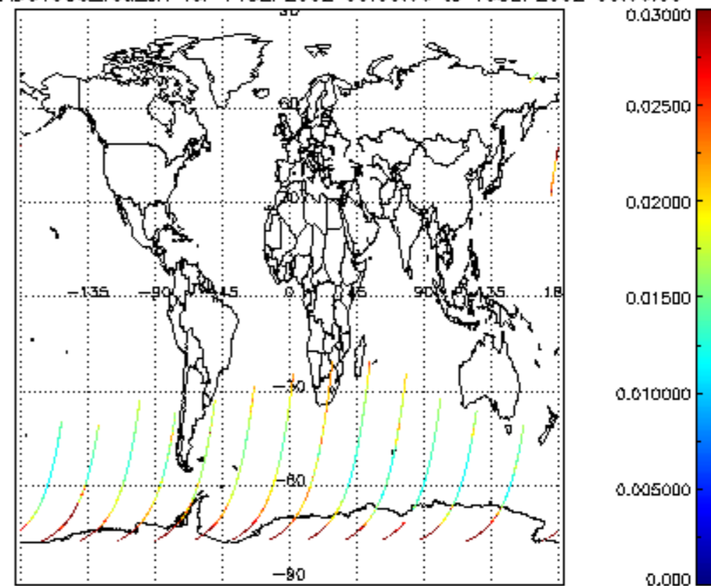
SCIOL2P_NADUV003_vcd_err for 14SEP2002 00:00:00 to 15SEP2002 00:00:00
