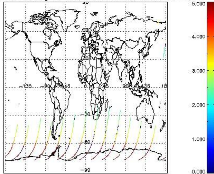
SCIOL2P_NADUV003_amf_gr for 14SEP2002 00:00:00 to 15SEP2002 00:00:00
