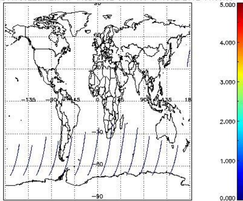
SCIOL2P_NADUV7S02_amf_cl for 14SEP2002 00:00:00 to 15SEP2002 00:00:00
