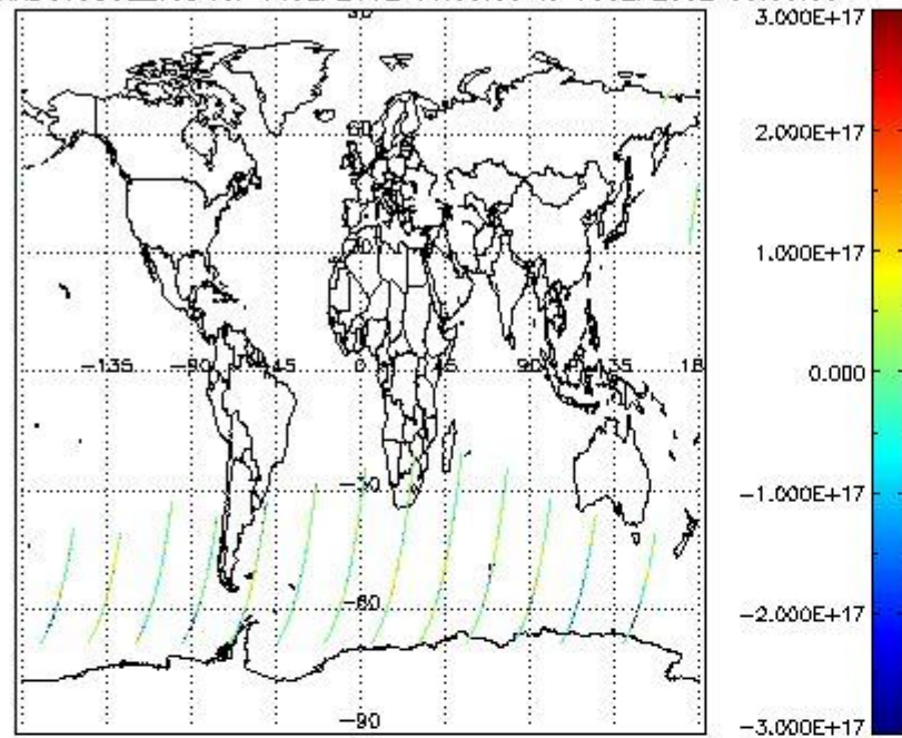
SCIOL2P_NADUV5S02_vcd for 14SEP2002 00:00:00 to 15SEP2002 00:00:00
