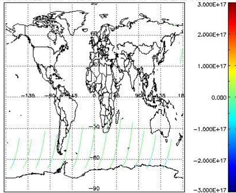
SCIOL2P_NADUV7S02_vcd for 14SEP2002 00:00:00 to 15SEP2002 00:00:00
