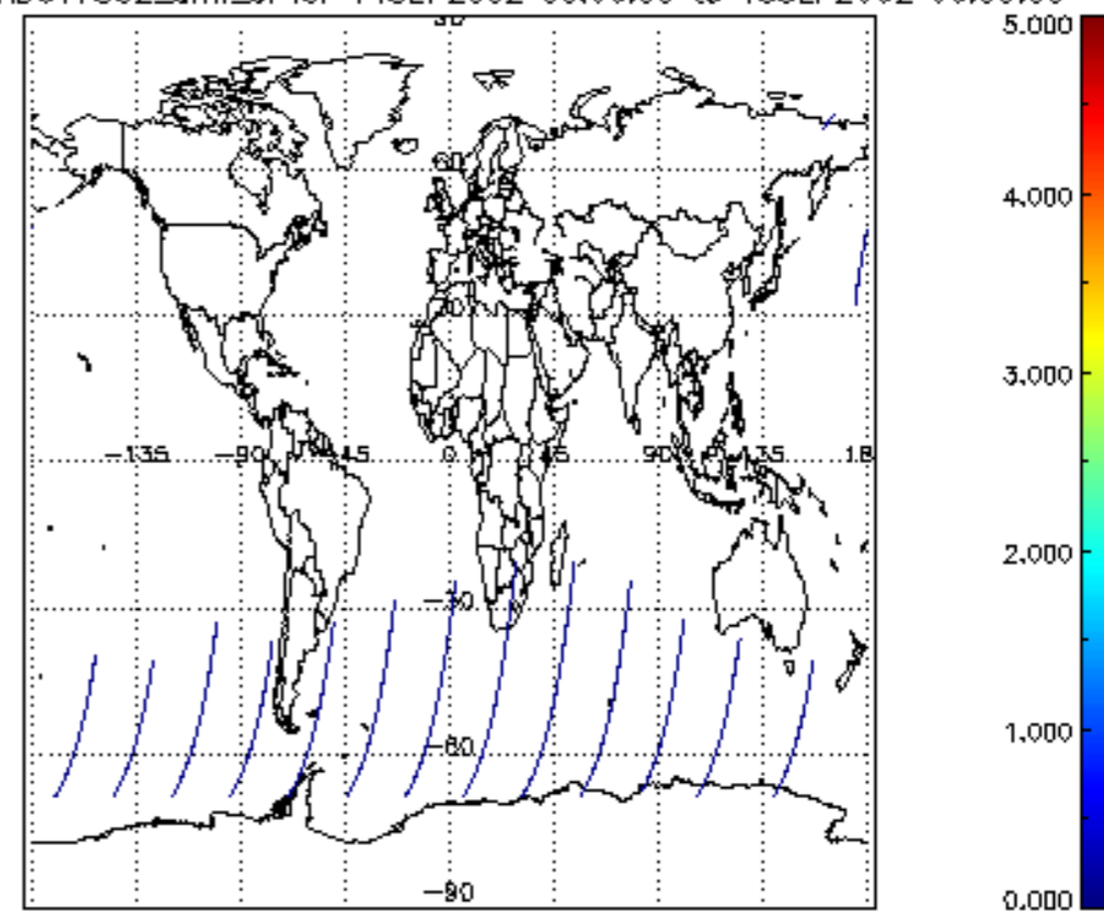
SCIOL2P_NADUV7S02_amf_cl for 14SEP2002 00:00:00 to 15SEP2002 00:00:00
