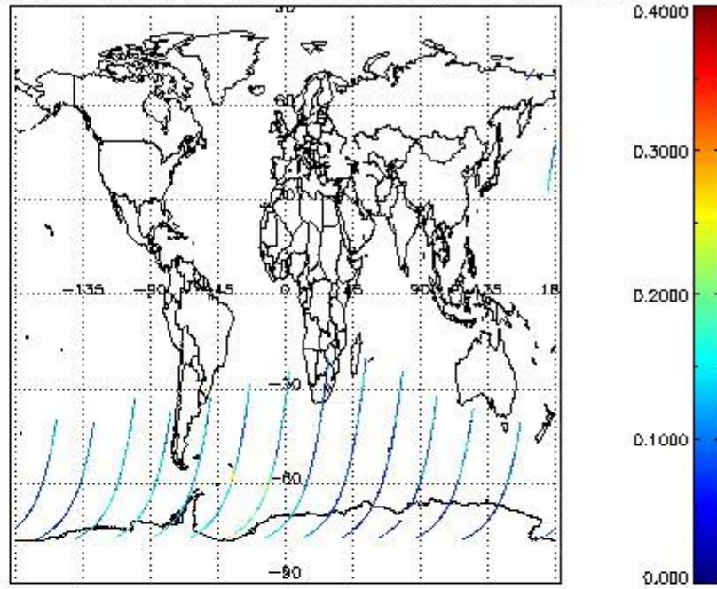
SCIOL2P_NADUV1NO2_vcd_err for 14SEP2002 00:00:00 to 15SEP2002 00:00:00
