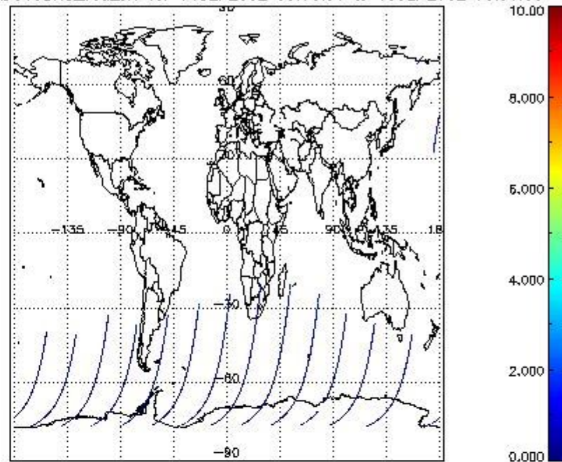
SCIOL2P_NADUV3BRO_vcd_err for 14SEP2002 00:00:00 to 15SEP2002 00:00:00
