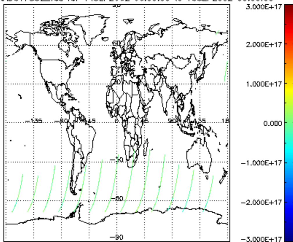
SCIOL2P_NADUV7S02_vcd for 14SEP2002 00:00:00 to 15SEP2002 00:00:00
