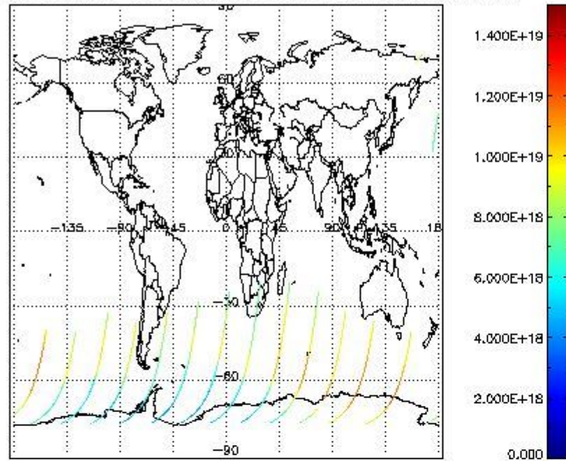
SCIOL2P_NADUV003_vcd for 14SEP2002 00:00:00 to 15SEP2002 00:00:00
