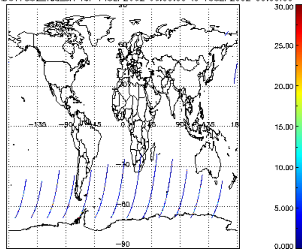
SCIOL2P_NADUV7S02_vcd_err for 14SEP2002 00:00:00 to 15SEP2002 00:00:00
