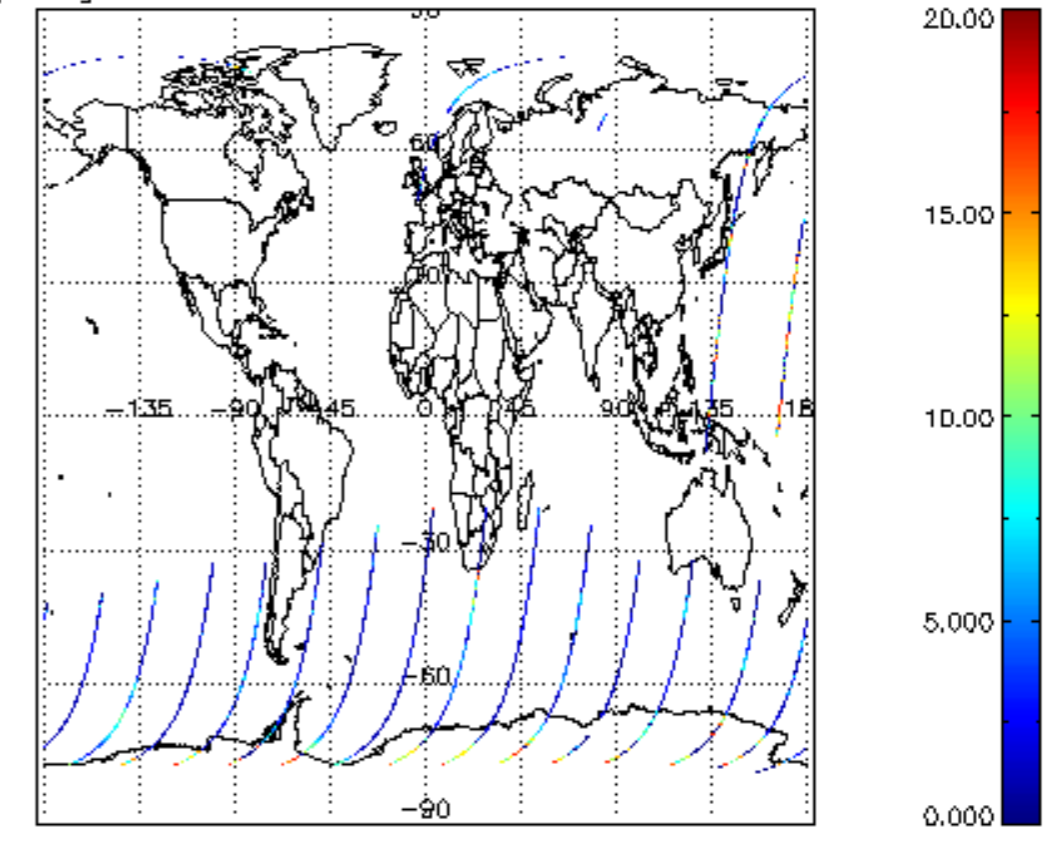
cl_top_height for 14SEP2002 00:00:00 to 15SEP2002 00:00:00
