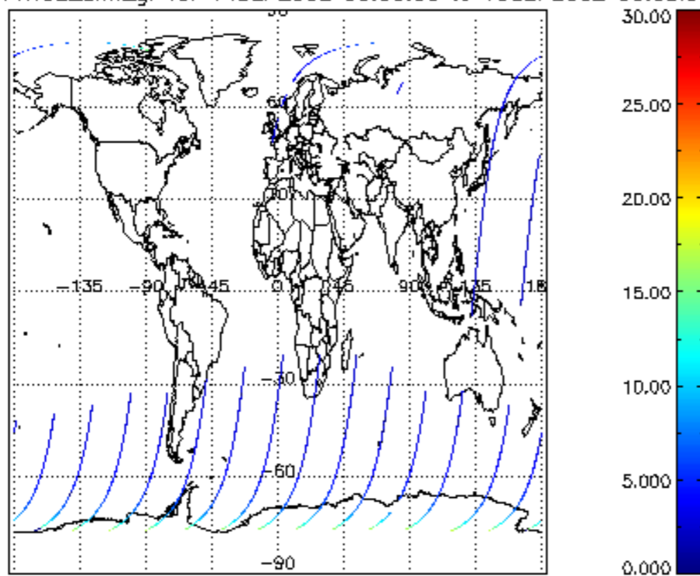
iCIOL2P_NADUV1NO2_amf_gr for 14SEP2002 00:00:00 to 15SEP2002 00:00:00
