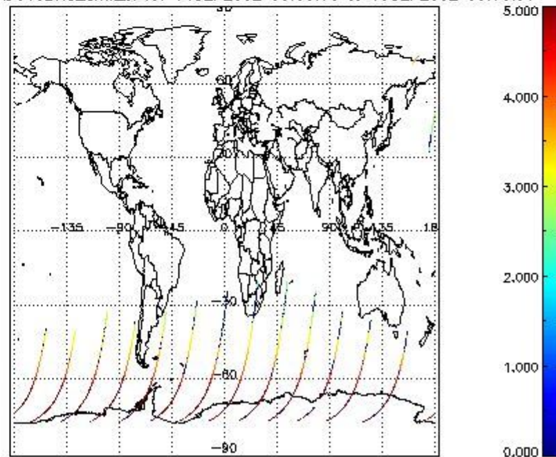
SCIOL2P_NADUV3BRO_amf_cl for 14SEP2002 00:00:00 to 15SEP2002 00:00:00
