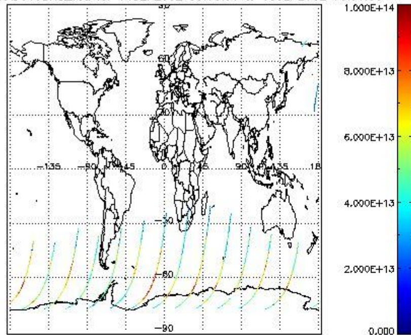
SCIOL2P_NADUV3BRO_vcd for 14SEP2002 00:00:00 to 15SEP2002 00:00:00
