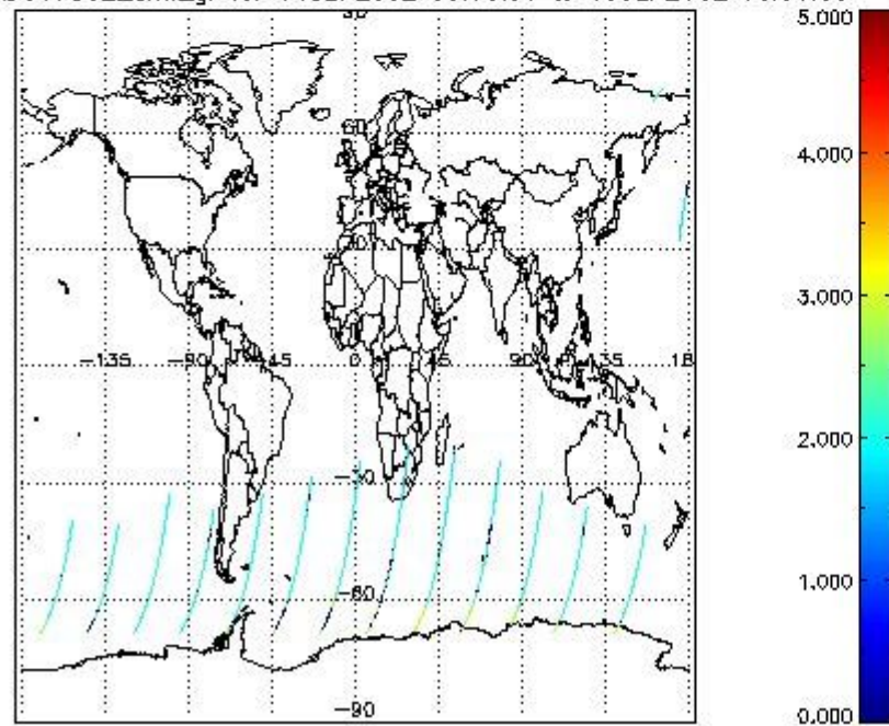
SCIOL2P_NADUV7S02_amf_gr for 14SEP2002 00:00:00 to 15SEP2002 00:00:00
