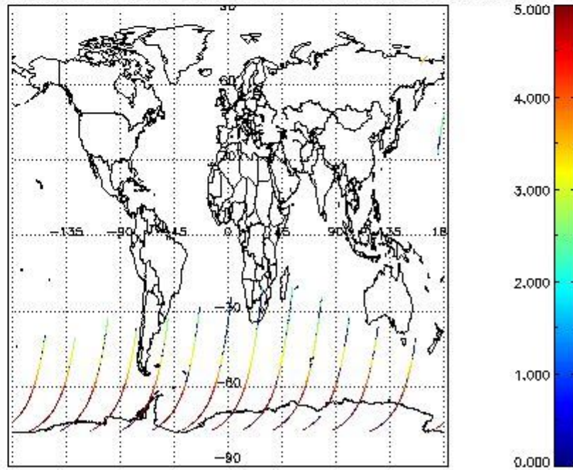
SCIOL2P_NADUV1NO2_amf_cl for 14SEP2002 00:00:00 to 15SEP2002 00:00:00
