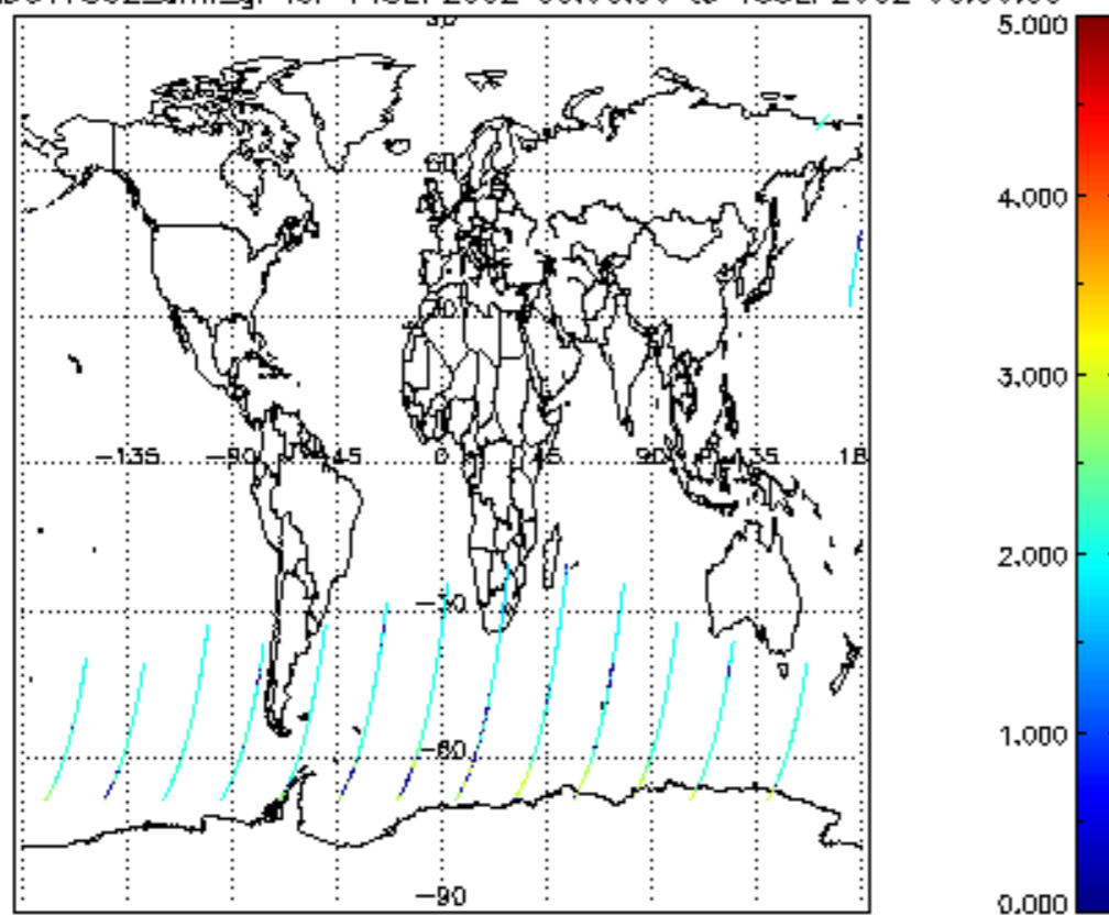
SCIOL2P_NADUV7S02_amf_gr for 14SEP2002 00:00:00 to 15SEP2002 00:00:00
