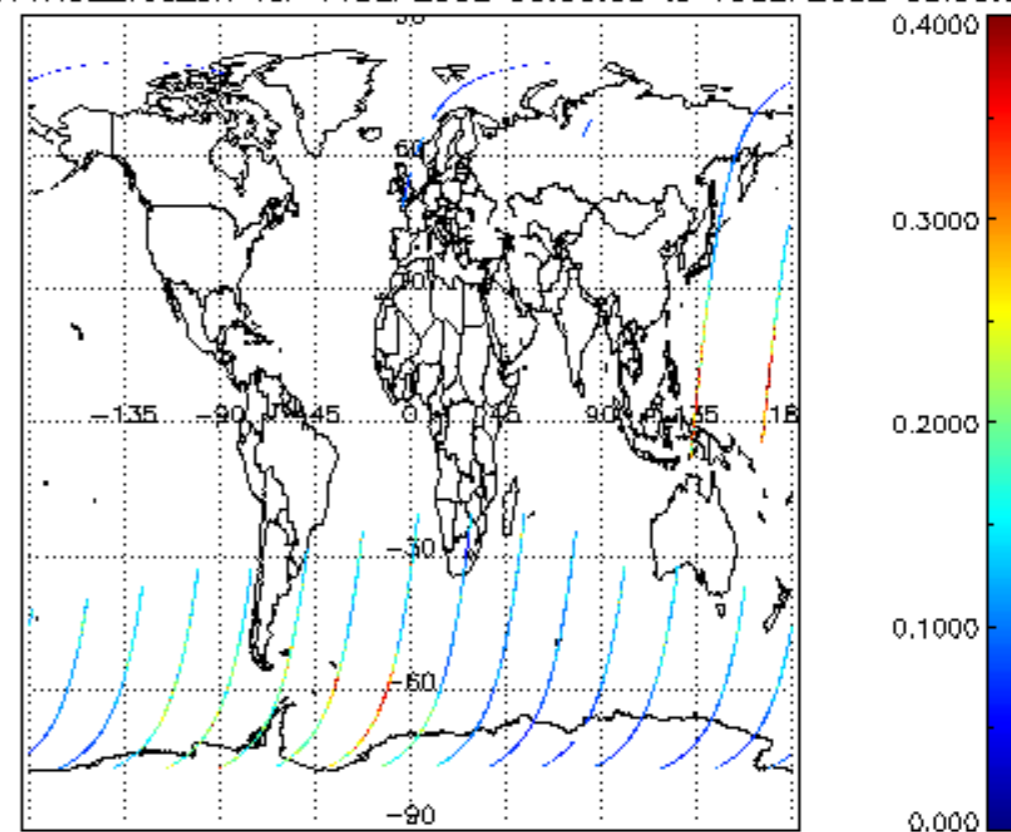
iCIOL2P_NADUV1NO2_vcd_err for 14SEP2002 00:00:00 to 15SEP2002 00:00:00
