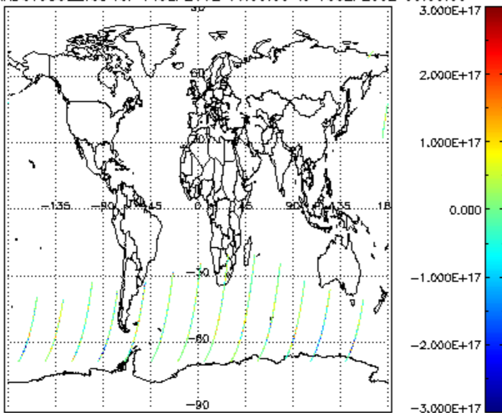
SCIOL2P_NADUV5S02_vcd for 14SEP2002 00:00:00 to 15SEP2002 00:00:00
