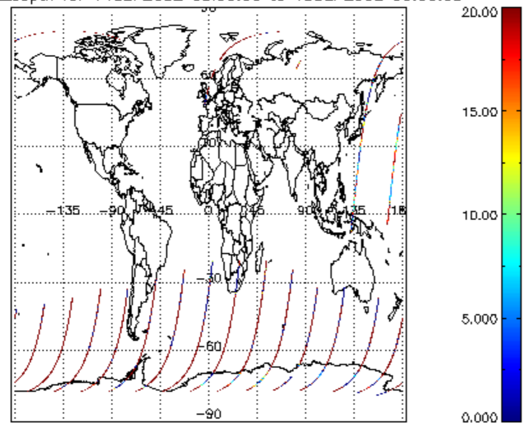
cl_opt_depth for 14SEP2002 00:00:00 to 15SEP2002 00:00:00
