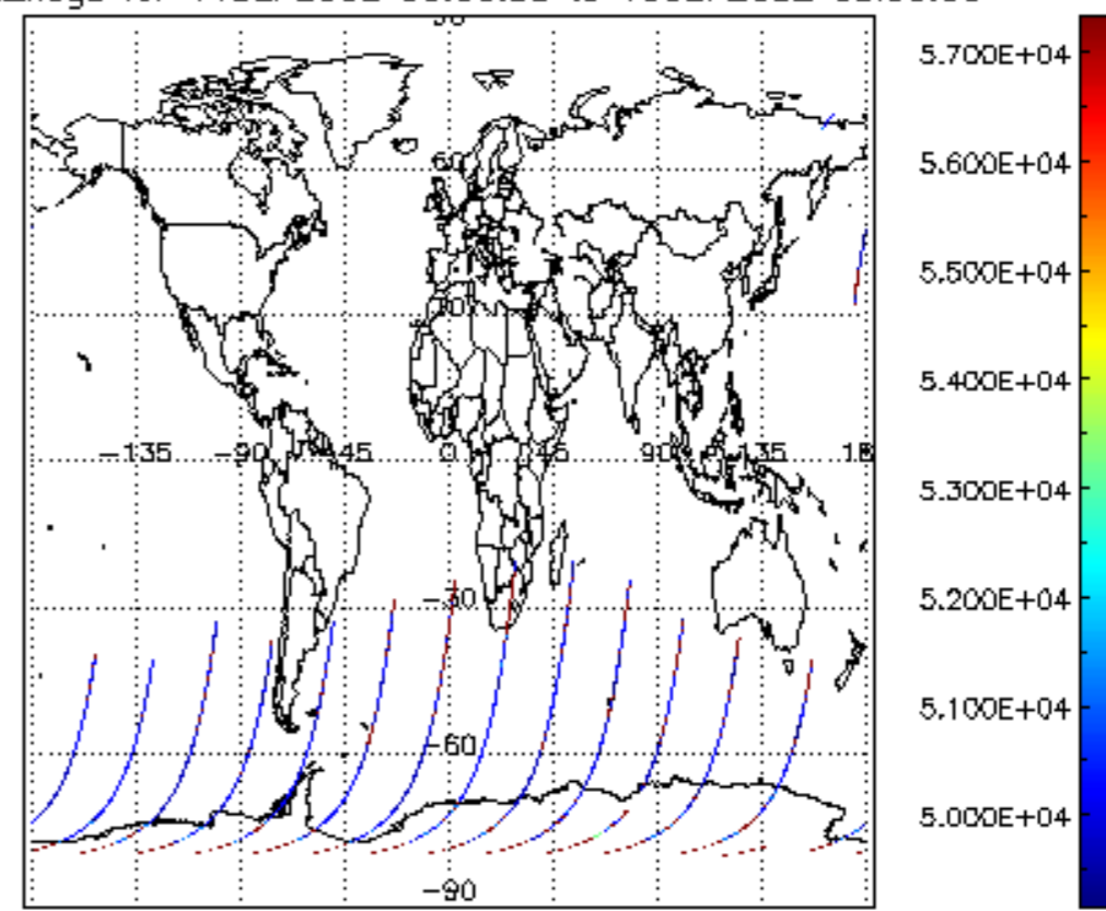
cloud_flags for 14SEP2002 00:00:00 to 15SEP2002 00:00:00
