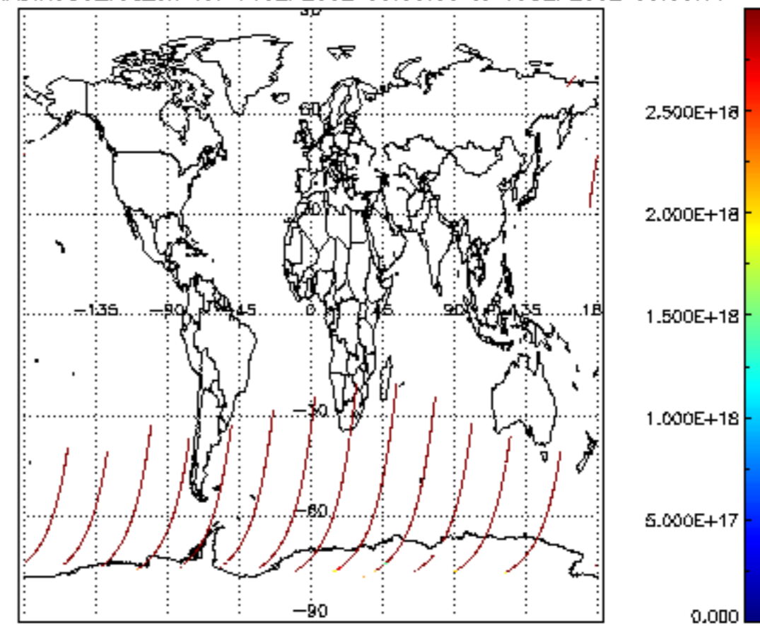
SCIOL2P_NADIR3CO_vcd_err for 14SEP2002 00:00:00 to 15SEP2002 00:00:00
