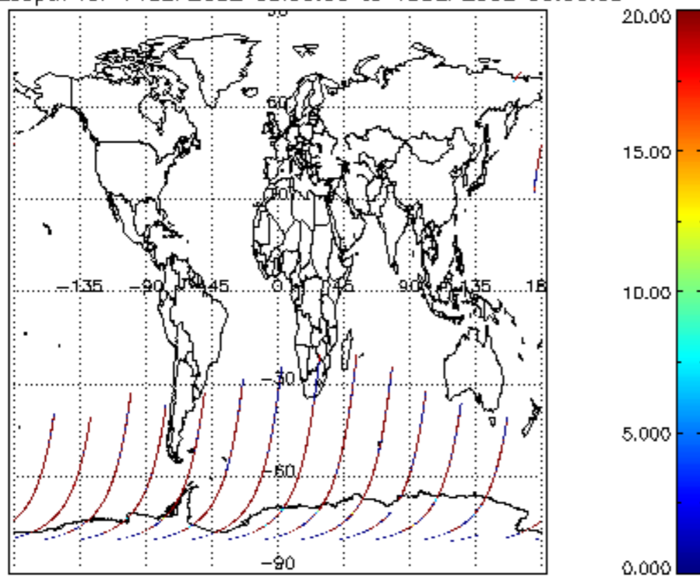
cl_opt_depth for 14SEP2002 00:00:00 to 15SEP2002 00:00:00
