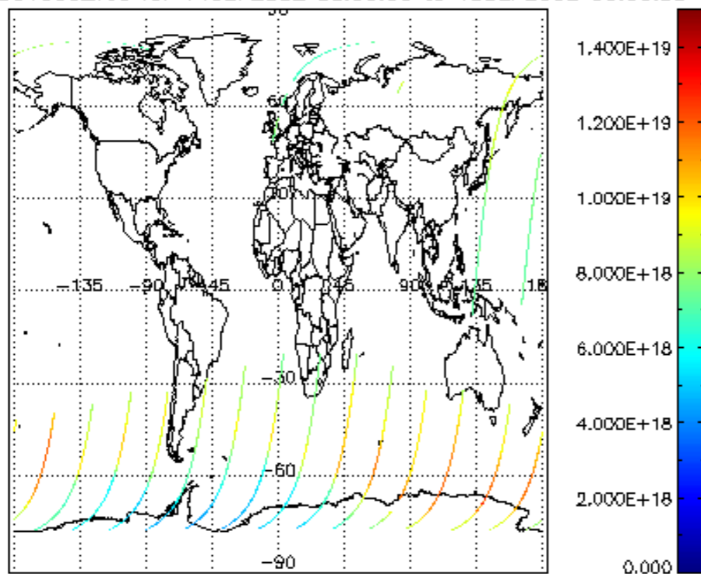
SCIOL2P_NADUV003_vcd for 14SEP2002 00:00:00 to 15SEP2002 00:00:00
