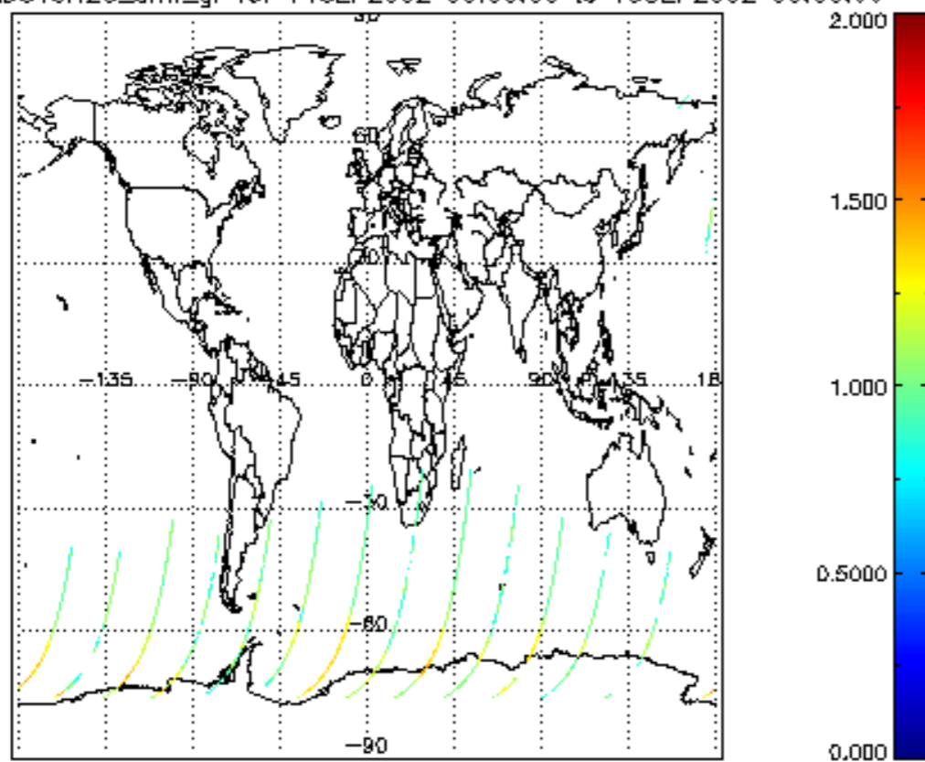
SCIOL2P_NADUV8H2O_amf_gr for 14SEP2002 00:00:00 to 15SEP2002 00:00:00
