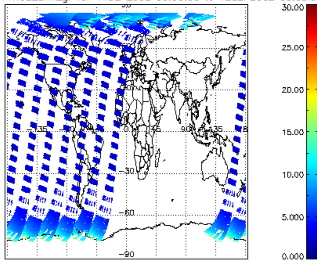
iCIOL2P_NADUV1NO2_amf_gr for 11SEP2002 00:00:00 to 12SEP2002 00:00:00
