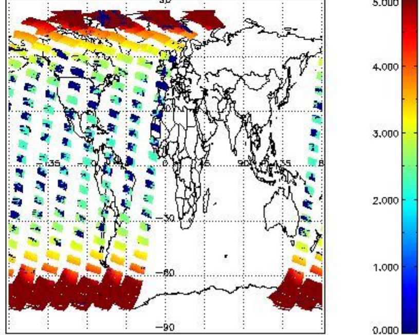
SCIOL2P_NADUV1N02_amf_cl for 11SEP2002 00:00:00 to 12SEP2002 00:00:00
