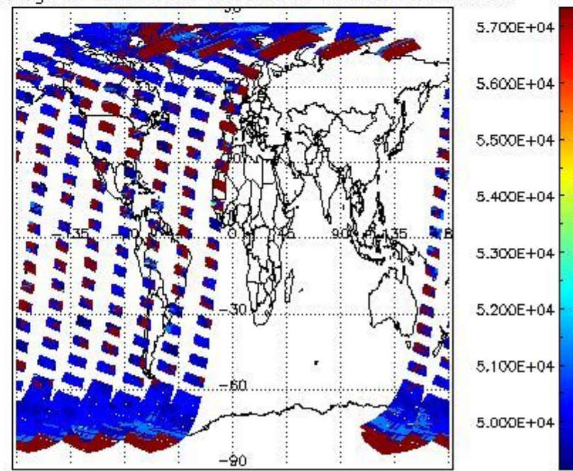
cloud_flags for 11SEP2002 00:00:00 to 12SEP2002 00:00:00
