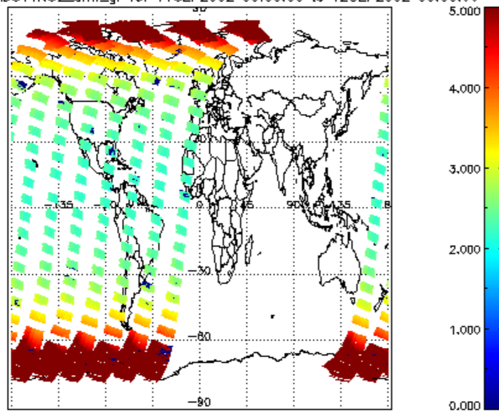
SCIOL2P_NADUV1N02_amf_gr for 11SEP2002 00:00:00 to 12SEP2002 00:00:00
