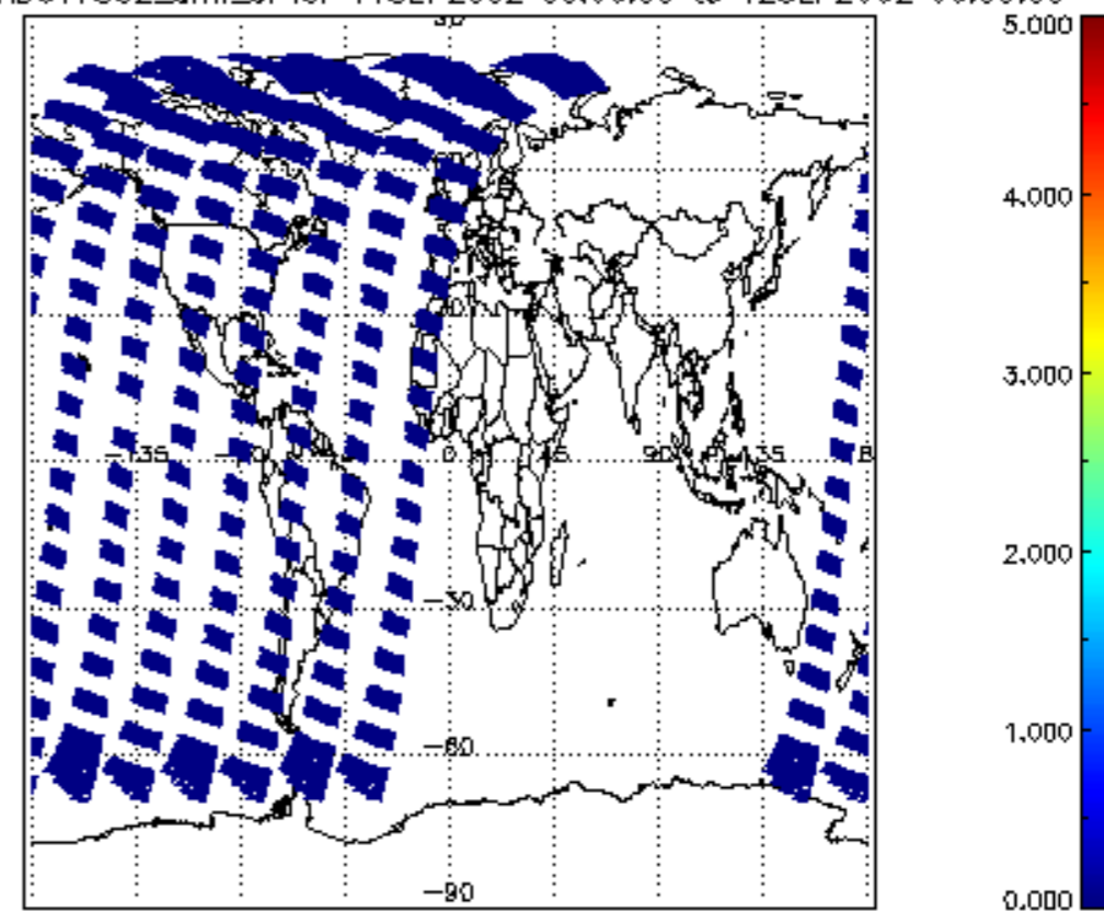
SCIOL2P_NADUV7S02_amf_cl for 11SEP2002 00:00:00 to 12SEP2002 00:00:00
