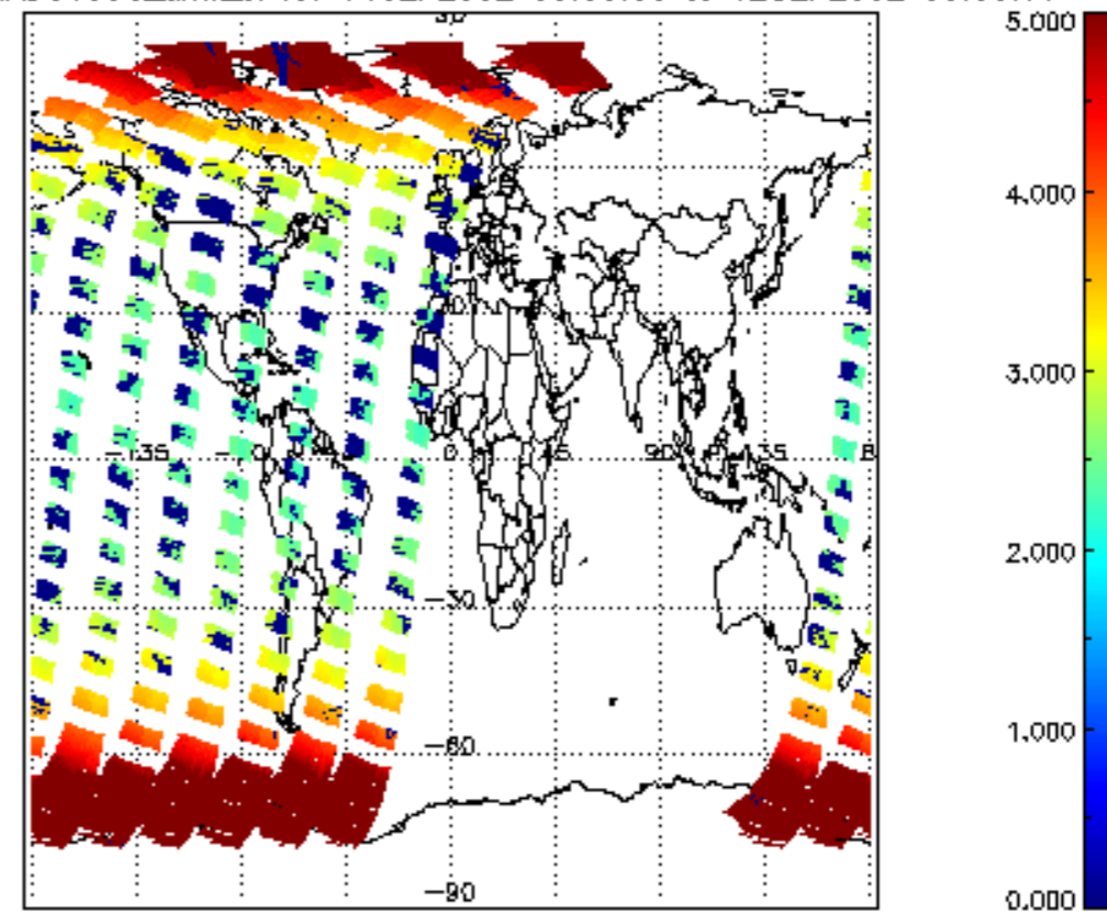
SCIOL2P_NADUV003_amf_cl for 11SEP2002 00:00:00 to 12SEP2002 00:00:00
