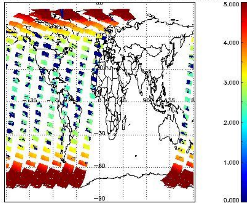
SCIOL2P_NADUV003_amf_cl for 11SEP2002 00:00:00 to 12SEP2002 00:00:00
