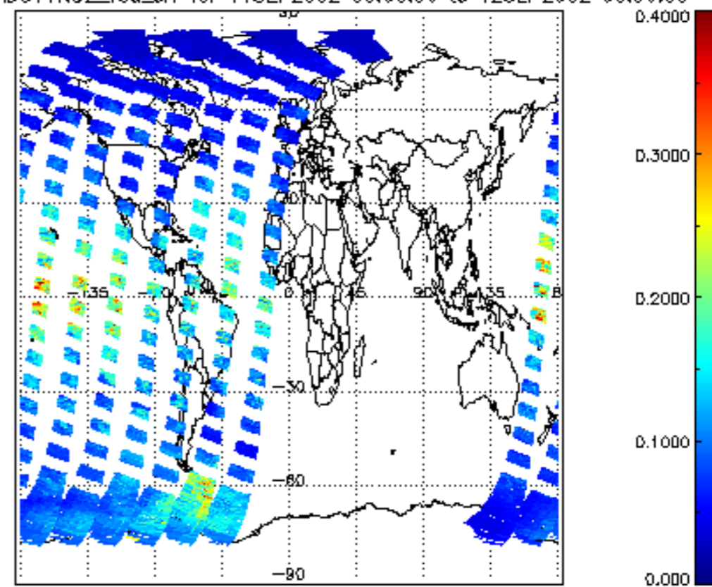
SCIOL2P_NADUV1N02_vcd_err for 11SEP2002 00:00:00 to 12SEP2002 00:00:00
