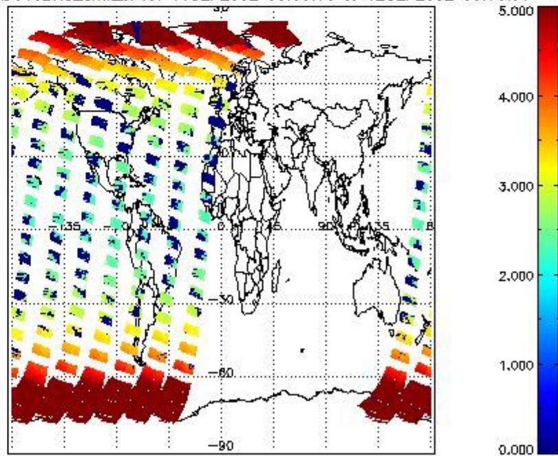
SCIOL2P_NADUV3BRO_amf_cl for 11SEP2002 00:00:00 to 12SEP2002 00:00:00
