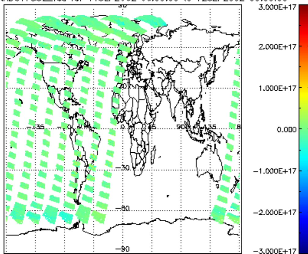
SCIOL2P_NADUV7S02_vcd for 11SEP2002 00:00:00 to 12SEP2002 00:00:00
