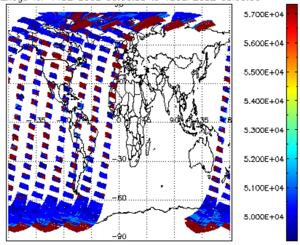
cloud_flags for 11SEP2002 00:00:00 to 12SEP2002 00:00:00
