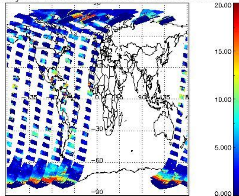
cL_top_height for 11SEP2002 00:00:00 to 12SEP2002 00:00:00
