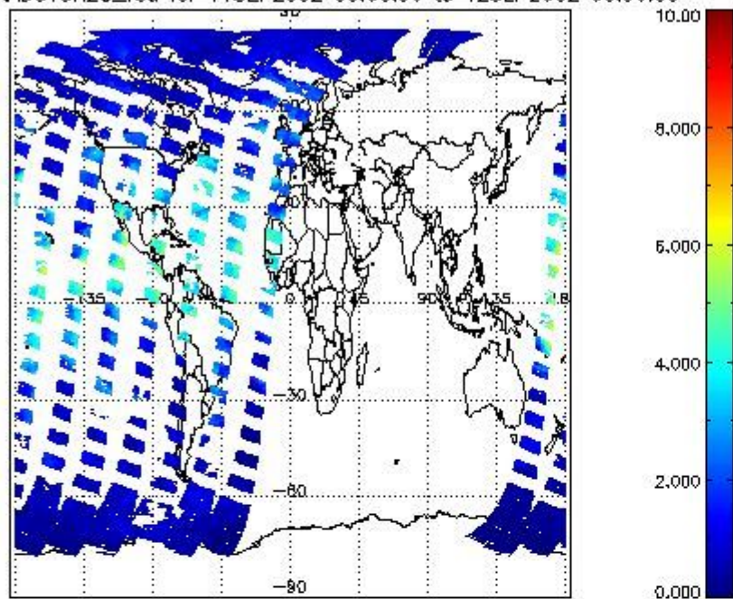
SCIOL2P_NADUV8H2O_vcd for 11SEP2002 00:00:00 to 12SEP2002 00:00:00
