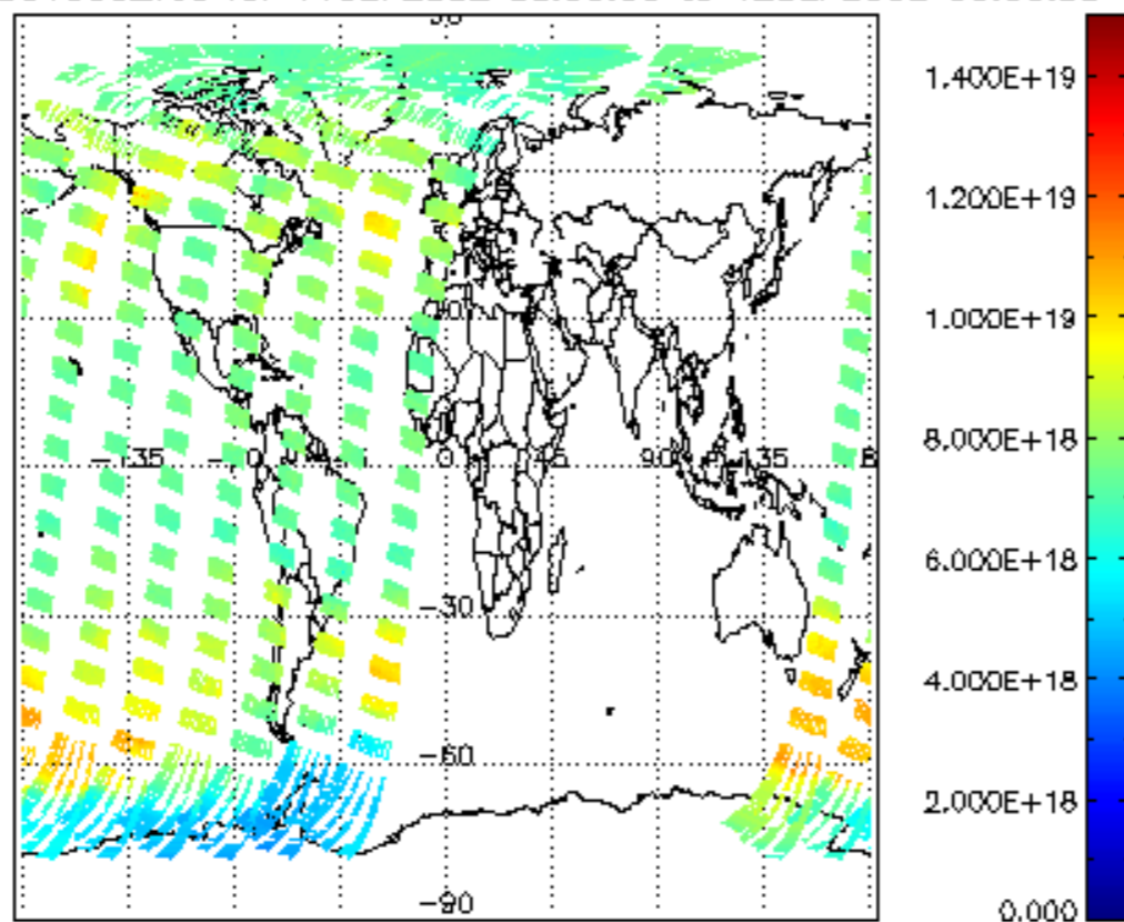
SCIOL2P_NADUV003_vcd for 11SEP2002 00:00:00 to 12SEP2002 00:00:00
