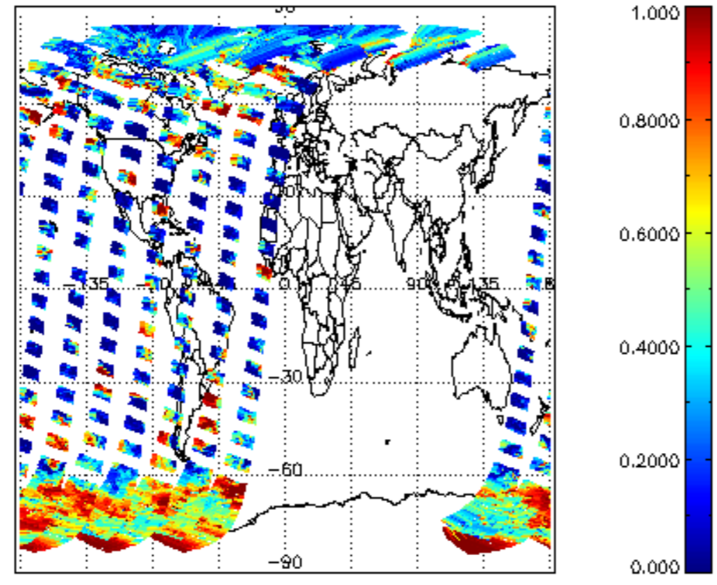
cl_frac for 11SEP2002 00:00:00 to 12SEP2002 00:00:00
