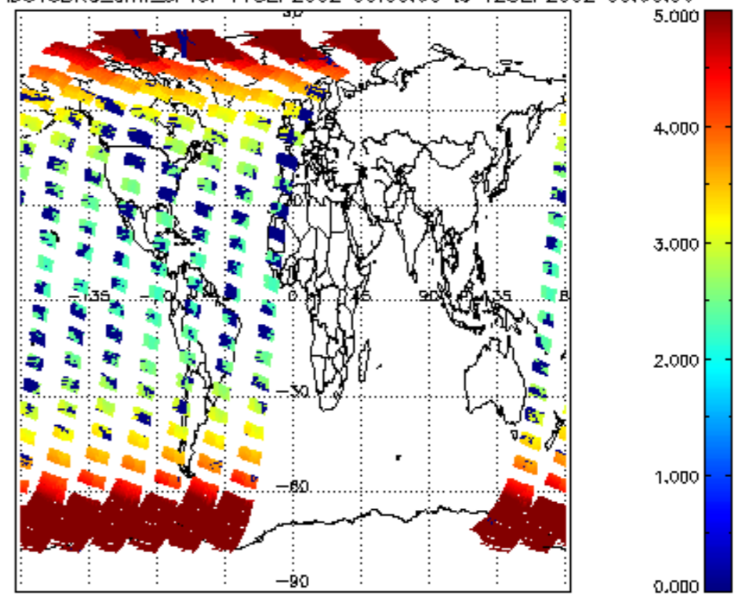
SCIOL2P_NADUV3BRO_amf_cl for 11SEP2002 00:00:00 to 12SEP2002 00:00:00
