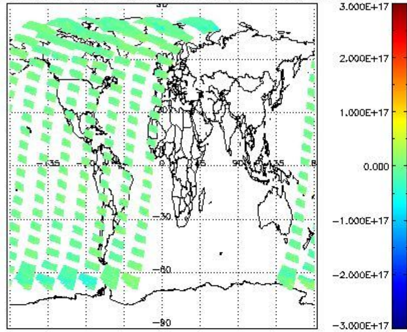
SCIOL2P_NADUV7S02_vcd for 11SEP2002 00:00:00 to 12SEP2002 00:00:00
