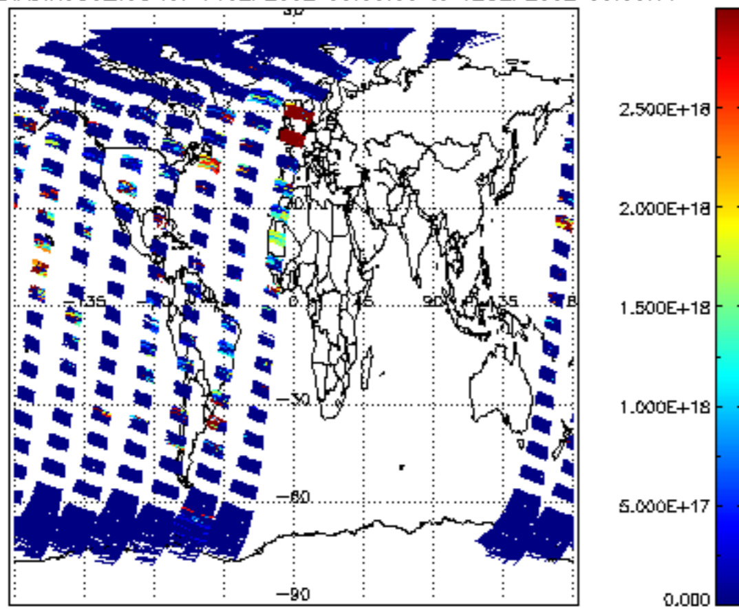
SCIOL2P_NADIR3CO_vcd for 11SEP2002 00:00:00 to 12SEP2002 00:00:00
