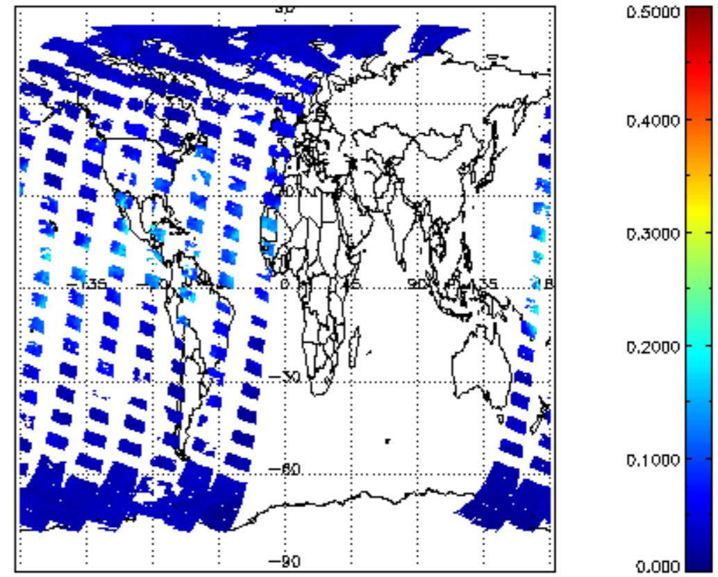
SCIOL2P_NADUV8H2O_vcd_err for 11SEP2002 00:00:00 to 12SEP2002 00:00:00
