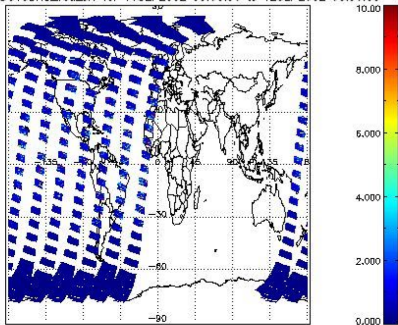
SCIOL2P_NADUV3BRO_vcd_err for 11SEP2002 00:00:00 to 12SEP2002 00:00:00
