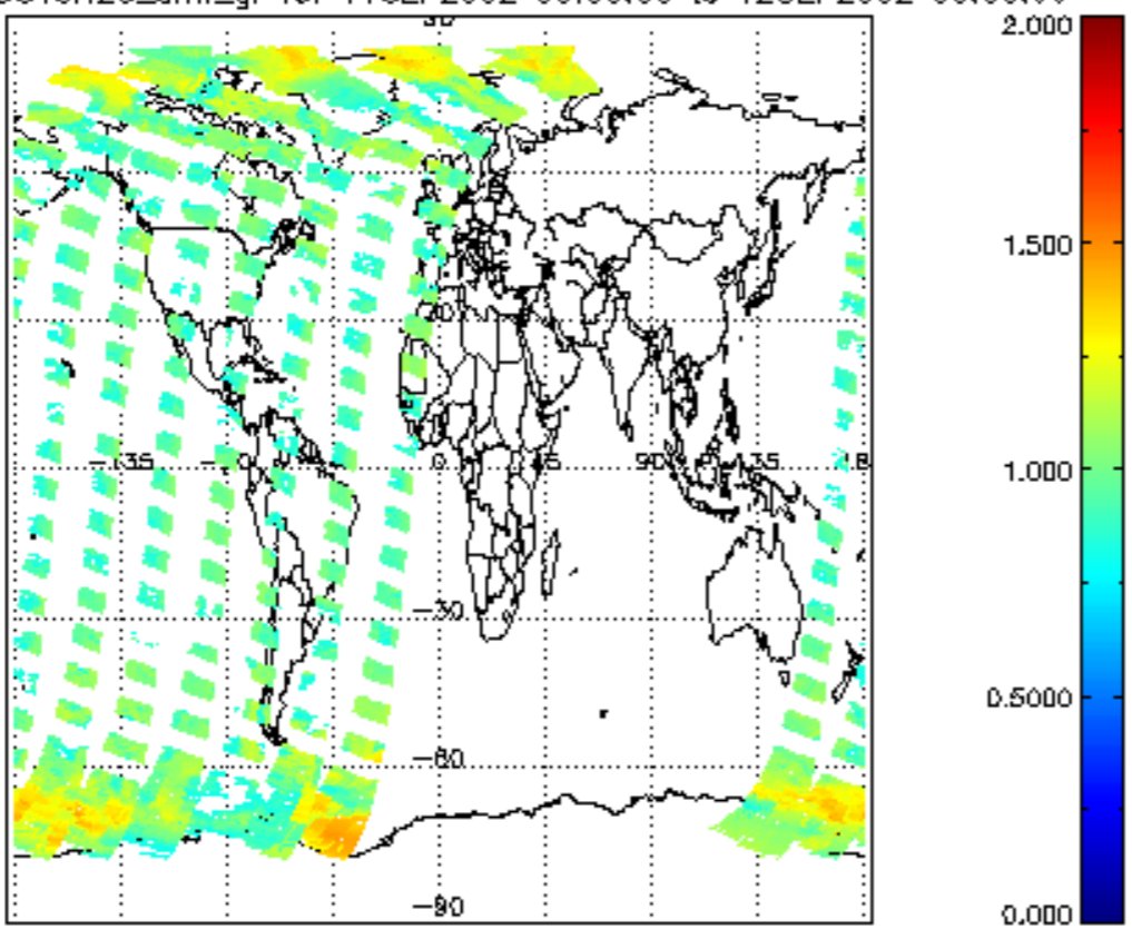
SCIOL2P_NADUV8H2O_amf_gr for 11SEP2002 00:00:00 to 12SEP2002 00:00:00
