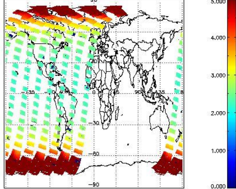
SCIOL2P_NADUV1N02_amf_gr for 11SEP2002 00:00:00 to 12SEP2002 00:00:00
