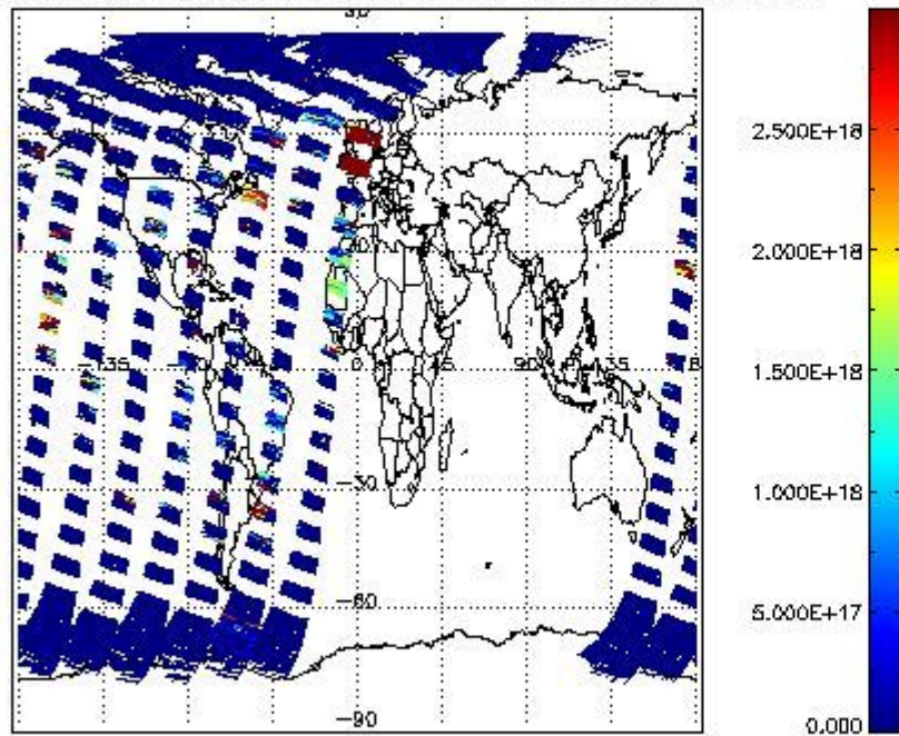
SCIO2P_NADIR3CO_vcd for 11SEP2002 00:00:00 to 12SEP2002 00:00:00
