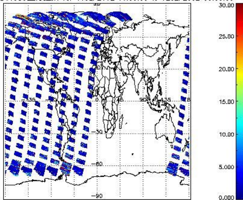
SCIOL2P_NADUV5S02_vcd_err for 11SEP2002 00:00:00 to 12SEP2002 00:00:00
