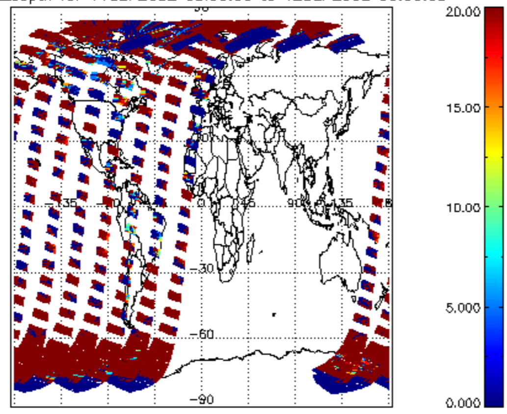
cl_opt_depth for 11SEP2002 00:00:00 to 12SEP2002 00:00:00
