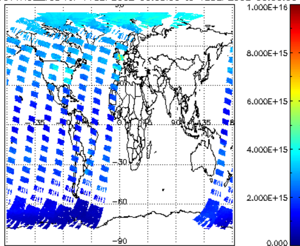
SCIOL2P_NADUV1NO2_vcd for 11SEP2002 00:00:00 to 12SEP2002 00:00:00
