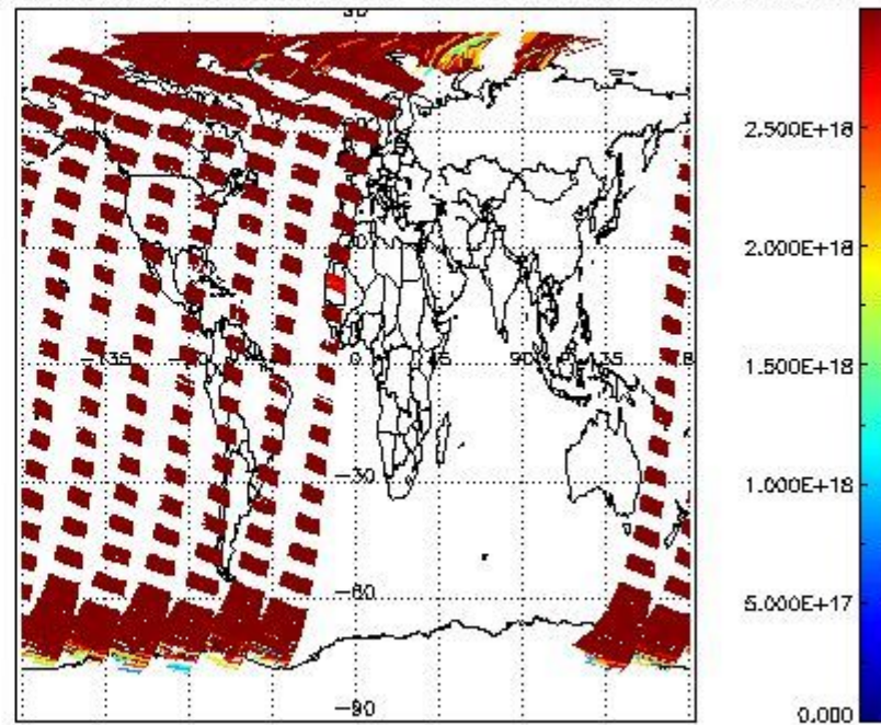
SCIO2P_NADIR3CO_vcd_err for 11SEP2002 00:00:00 to 12SEP2002 00:00:00
