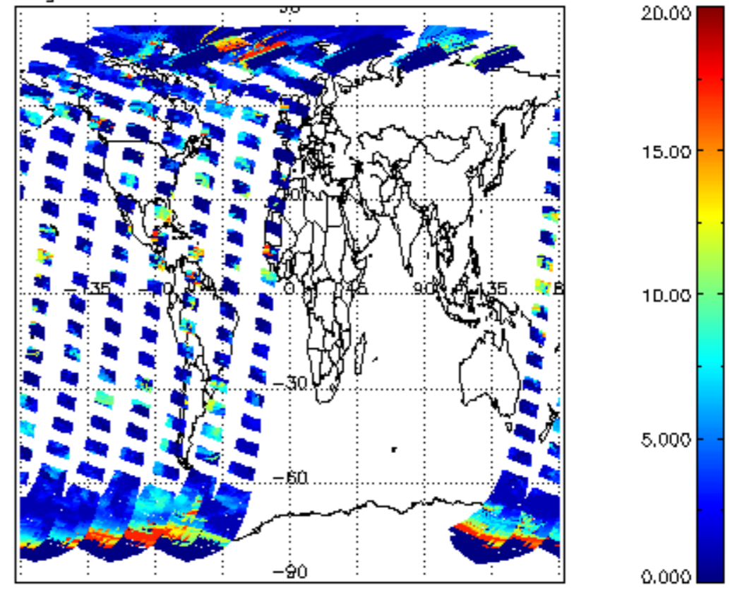
cl_top_height for 11SEP2002 00:00:00 to 12SEP2002 00:00:00
