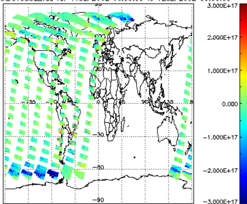
SCIOL2P_NADUV5S02_vcd for 11SEP2002 00:00:00 to 12SEP2002 00:00:00
