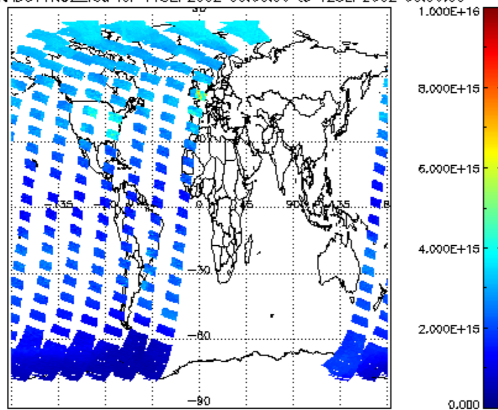
SCIOL2P_NADUV1N02_vcd for 11SEP2002 00:00:00 to 12SEP2002 00:00:00
