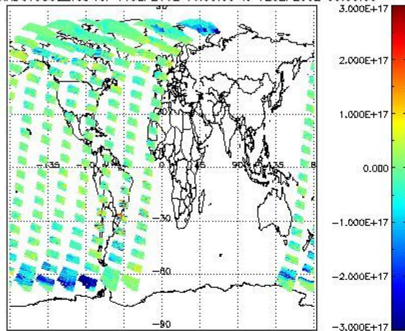
SCIOL2P_NADUV5S02_vcd for 11SEP2002 00:00:00 to 12SEP2002 00:00:00
