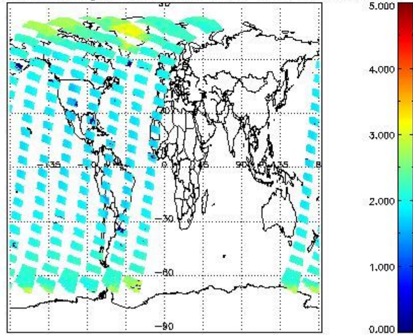
SCIOL2P_NADUV7S02_amf_gr for 11SEP2002 00:00:00 to 12SEP2002 00:00:00
