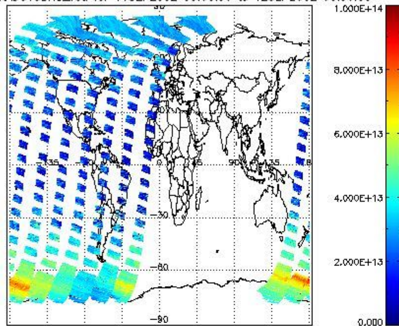
SCIOL2P_NADUV3BRO_vcd for 11SEP2002 00:00:00 to 12SEP2002 00:00:00
