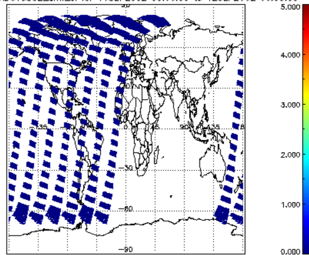
SCIOL2P_NADUV5S02_amf_cl for 11SEP2002 00:00:00 to 12SEP2002 00:00:00
