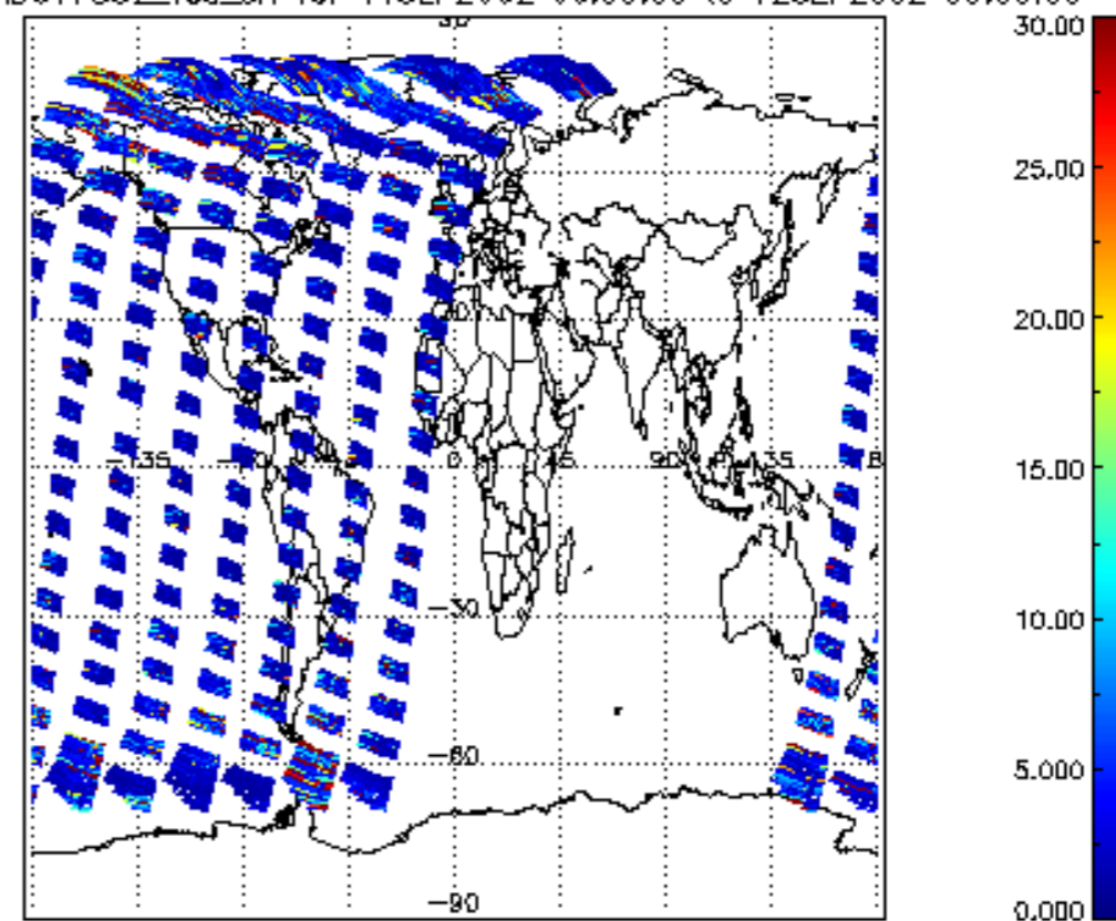
SCIOL2P_NADUV7S02_vcd_err for 11SEP2002 00:00:00 to 12SEP2002 00:00:00
