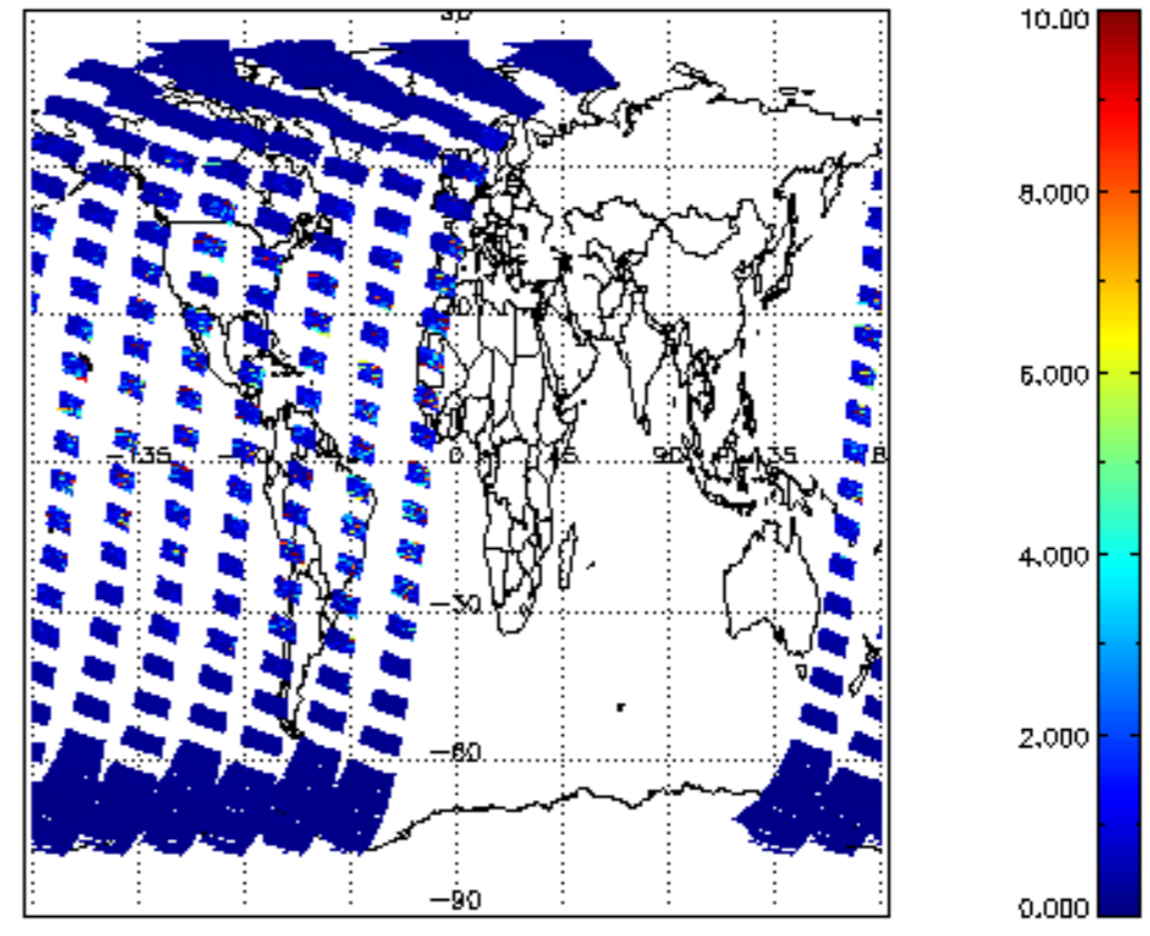
SCIOL2P_NADUV3BRO_vcd_err for 11SEP2002 00:00:00 to 12SEP2002 00:00:00
