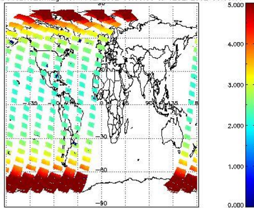
SCIOL2P_NADUV3BRO_amf_gr for 11SEP2002 00:00:00 to 12SEP2002 00:00:00
