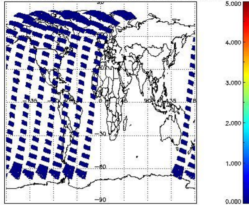
SCIOL2P_NADUV7S02_amf_cl for 11SEP2002 00:00:00 to 12SEP2002 00:00:00
