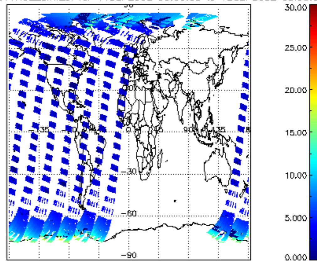
iCIOL2P_NADUV1NO2_amf_cl for 11SEP2002 00:00:00 to 12SEP2002 00:00:00
