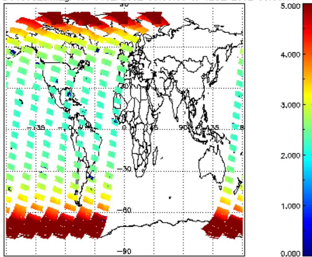
SCIOL2P_NADUV003_amf_gr for 11SEP2002 00:00:00 to 12SEP2002 00:00:00
