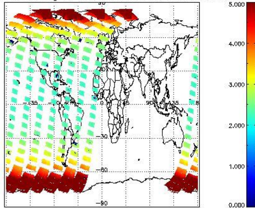
SCIOL2P_NADUV003_amf_gr for 11SEP2002 00:00:00 to 12SEP2002 00:00:00
