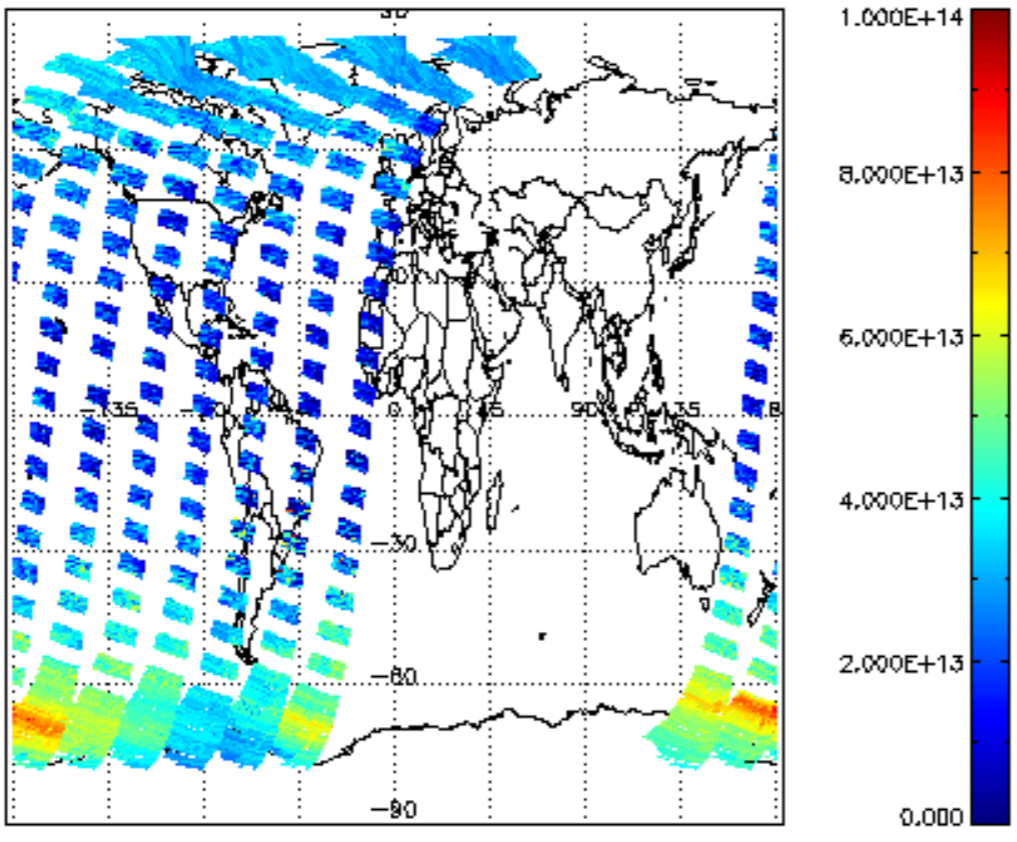
SCIOL2P_NADUV3BRO_vcd for 11SEP2002 00:00:00 to 12SEP2002 00:00:00
