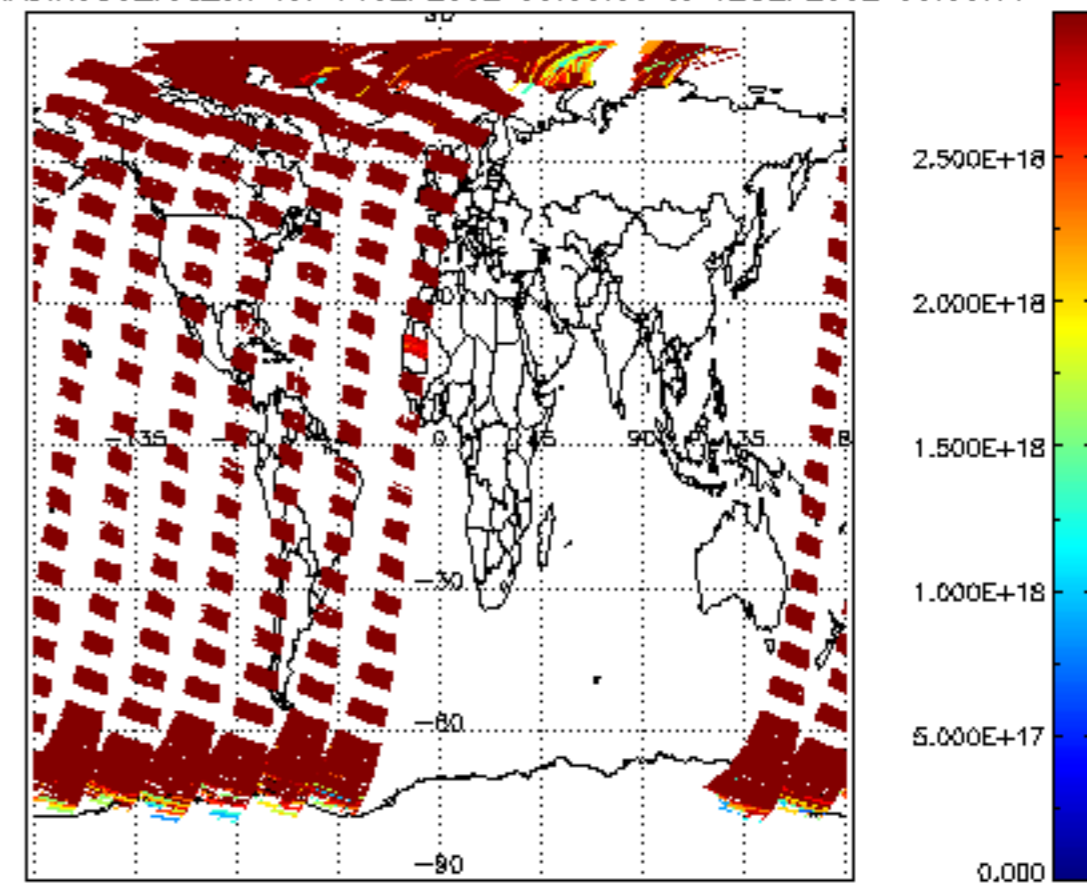
SCIOL2P_NADIR3CO_vcd_err for 11SEP2002 00:00:00 to 12SEP2002 00:00:00
