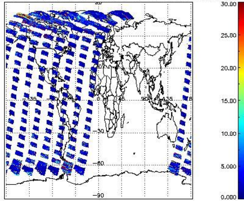
SCIOL2P_NADUV7S02_vcd_err for 11SEP2002 00:00:00 to 12SEP2002 00:00:00
