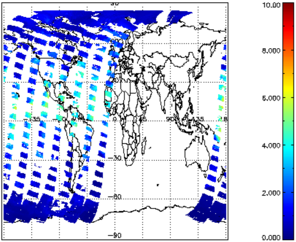
SCIOL2P_NADUV8H2O_vcd for 11SEP2002 00:00:00 to 12SEP2002 00:00:00
