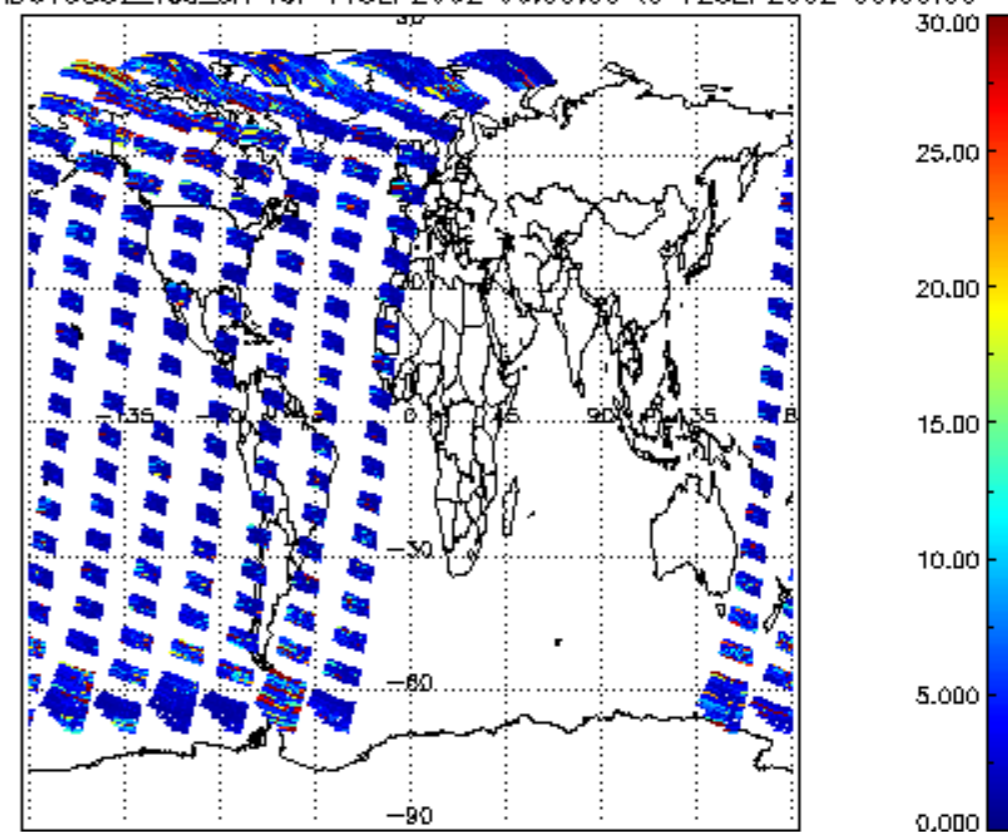
SCIOL2P_NADUV5S02_vcd_err for 11SEP2002 00:00:00 to 12SEP2002 00:00:00
