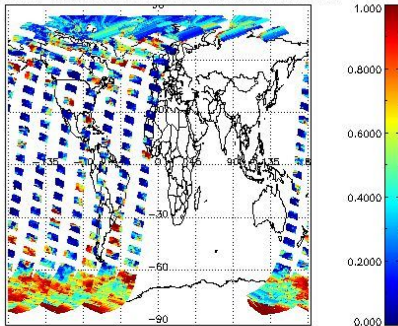
cL_frac for 11SEP2002 00:00:00 to 12SEP2002 00:00:00
