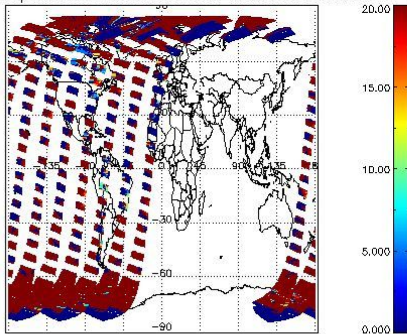
cL_opt_depth for 11SEP2002 00:00:00 to 12SEP2002 00:00:00
