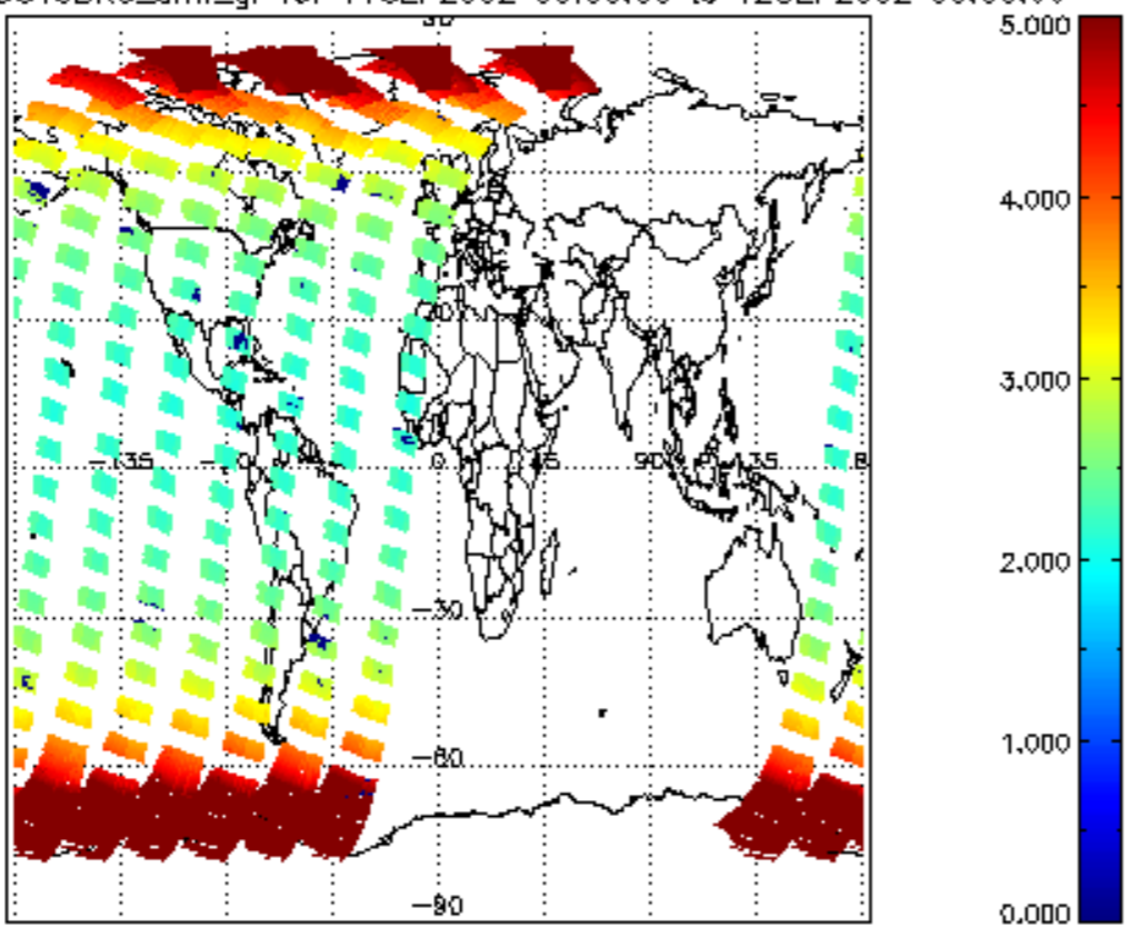
SCIOL2P_NADUV3BRO_amf_gr for 11SEP2002 00:00:00 to 12SEP2002 00:00:00
