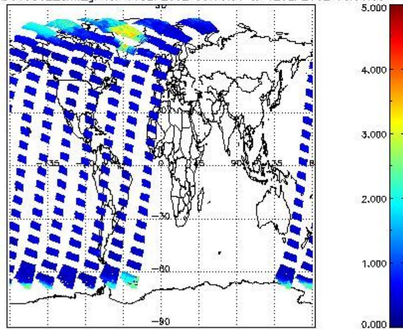
SCIOL2P_NADUV5S02_amf_gr for 11SEP2002 00:00:00 to 12SEP2002 00:00:00
