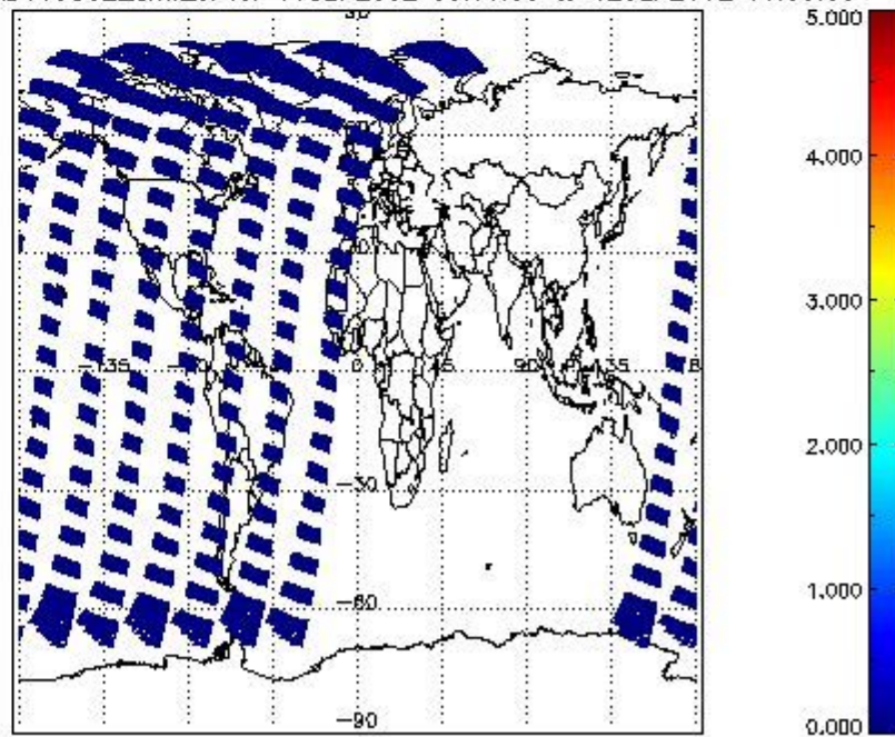
SCIOL2P_NADUV5S02_amf_cl for 11SEP2002 00:00:00 to 12SEP2002 00:00:00
