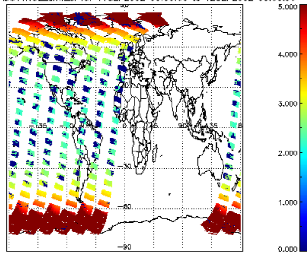
SCIOL2P_NADUV1N02_amf_sl for 11SEP2002 00:00:00 to 12SEP2002 00:00:00
