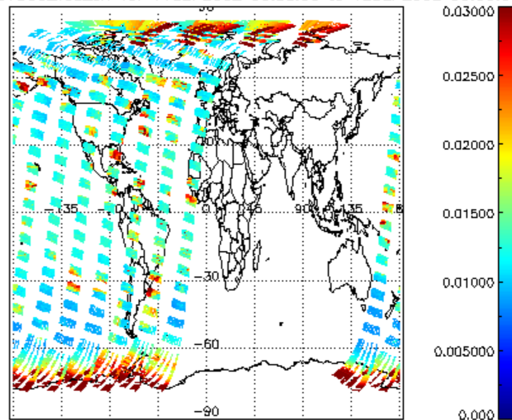
SCIOL2P_NADUV003_vcd_err for 11SEP2002 00:00:00 to 12SEP2002 00:00:00
