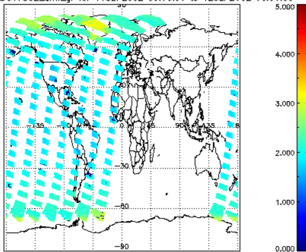
SCIOL2P_NADUV7S02_amf_gr for 11SEP2002 00:00:00 to 12SEP2002 00:00:00
