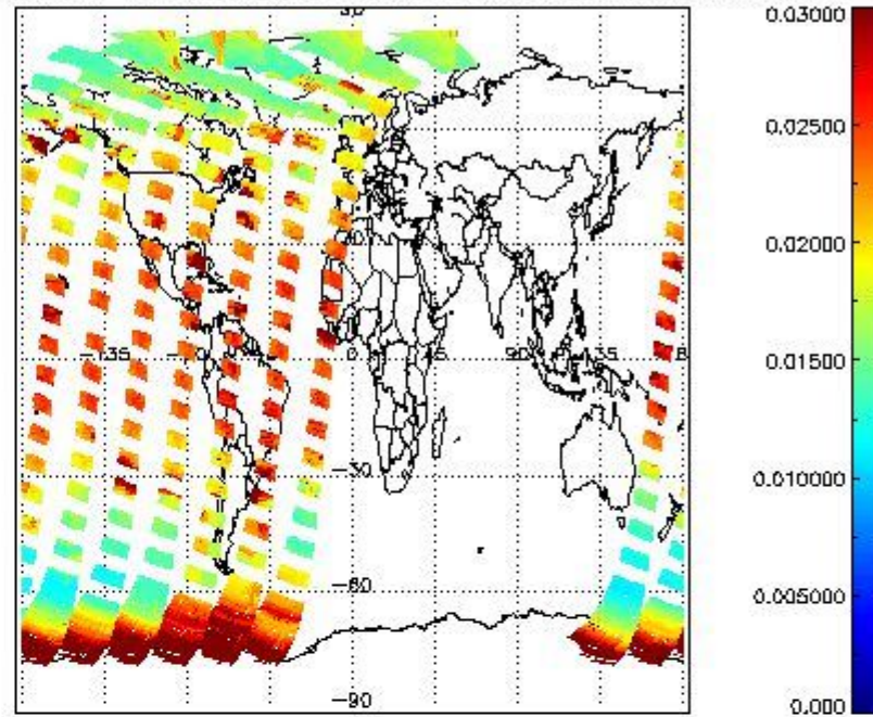
SCIOL2P_NADUV003_vcd_err for 11SEP2002 00:00:00 to 12SEP2002 00:00:00
