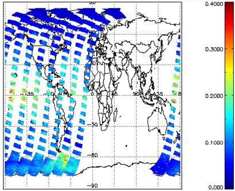
SCIOL2P_NADUV1N02_vcd_err for 11SEP2002 00:00:00 to 12SEP2002 00:00:00
