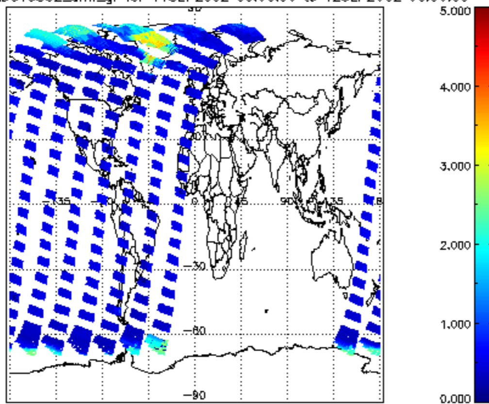
SCIOL2P_NADUV5S02_amf_gr for 11SEP2002 00:00:00 to 12SEP2002 00:00:00
