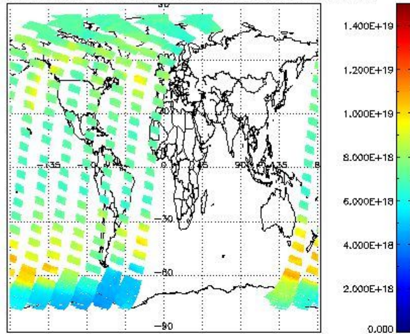
SCIOL2P_NADUV003_vcd for 11SEP2002 00:00:00 to 12SEP2002 00:00:00
