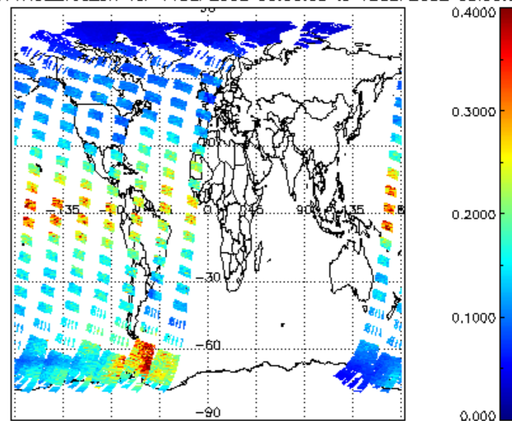
iCIOL2P_NADUV1NO2_vcd_err for 11SEP2002 00:00:00 to 12SEP2002 00:00:00
