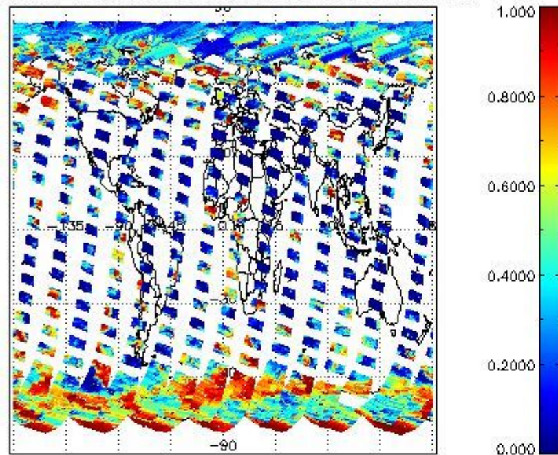
cL_frac for 05SEP2002 00:00:00 to 06SEP2002 00:00:00
