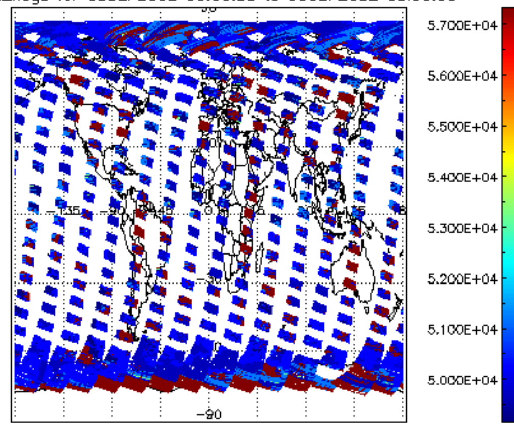
cloud_flags for 05SEP2002 00:00:00 to 06SEP2002 00:00:00
