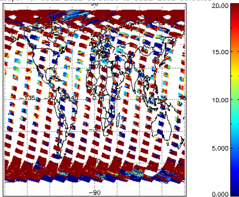
cl_opt_depth for 05SEP2002 00:00:00 to 06SEP2002 00:00:00
