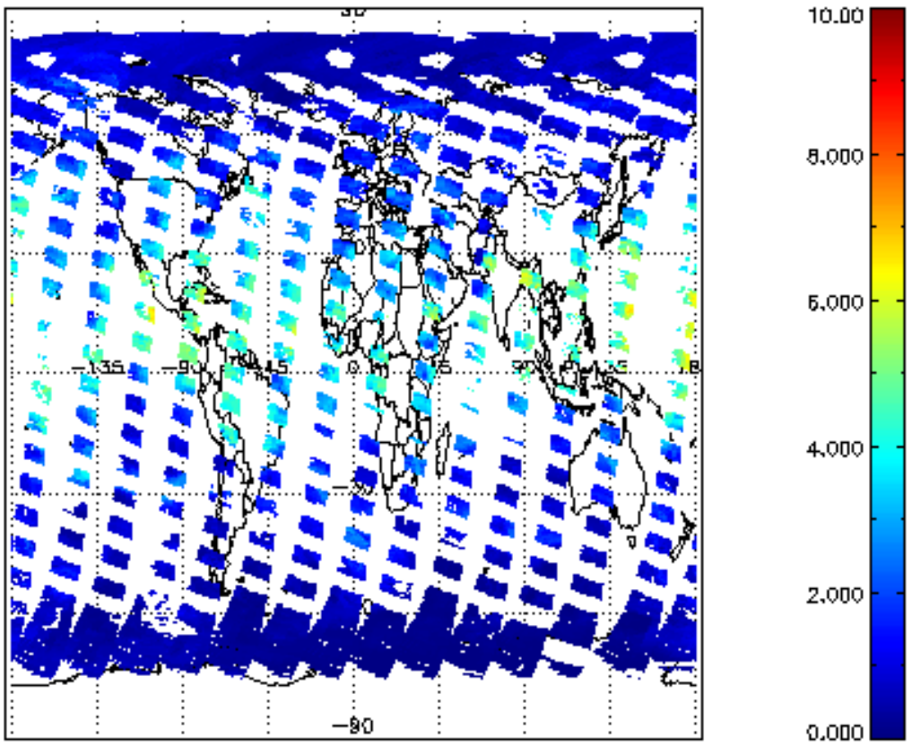
SCIOL2P_NADUV8H20_vcd for 05SEP2002 00:00:00 to 06SEP2002 00:00:00
