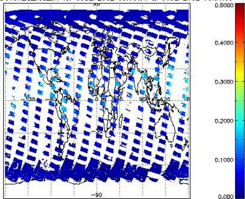
SCIOL2P_NADUV8H2O_vcd_err for 05SEP2002 00:00:00 to 06SEP2002 00:00:00
