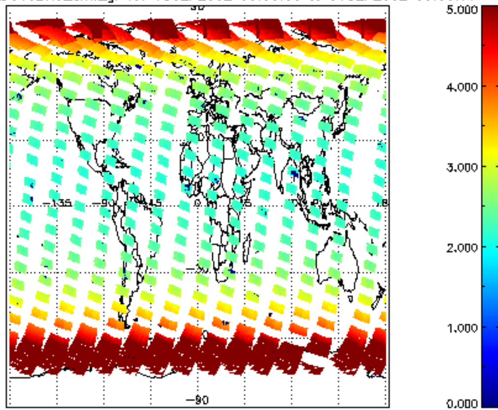
SCIOL2P_NADUV3BRO_amf_gr for 05SEP2002 00:00:00 to 06SEP2002 00:00:00
