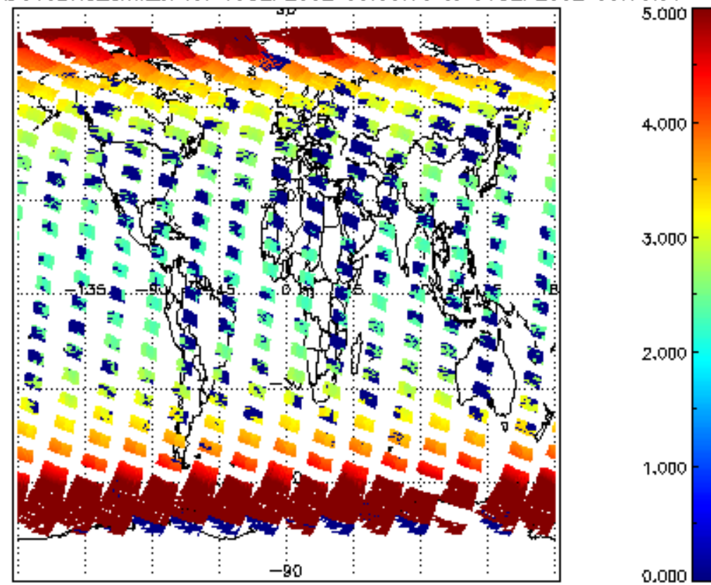
SCIOL2P_NADUV3BRO_amf_sl for 05SEP2002 00:00:00 to 06SEP2002 00:00:00
