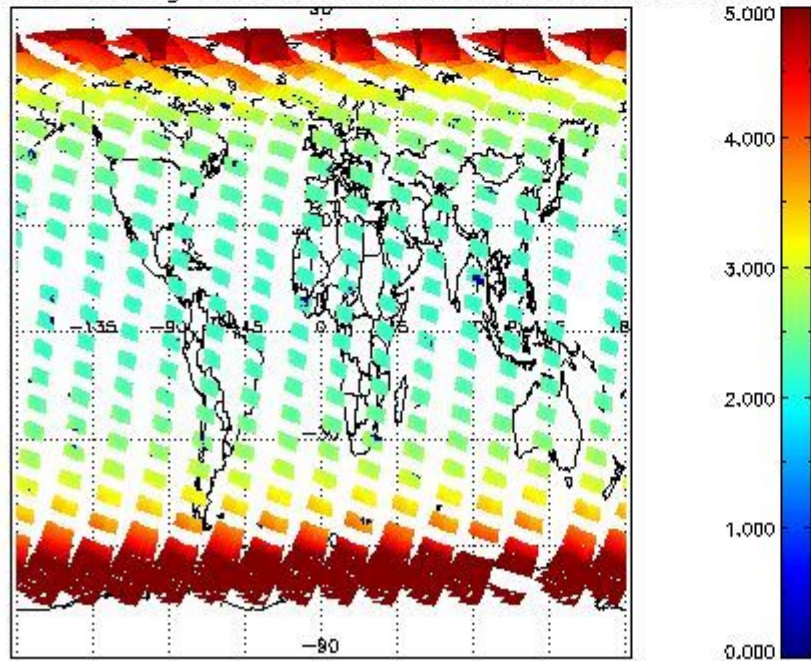
SCIOL2P_NADUV003_amf_gr for 05SEP2002 00:00:00 to 06SEP2002 00:00:00
