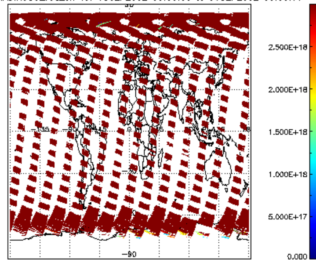
SCIOL2P_NADIR3CO_vcd_err for 05SEP2002 00:00:00 to 06SEP2002 00:00:00
