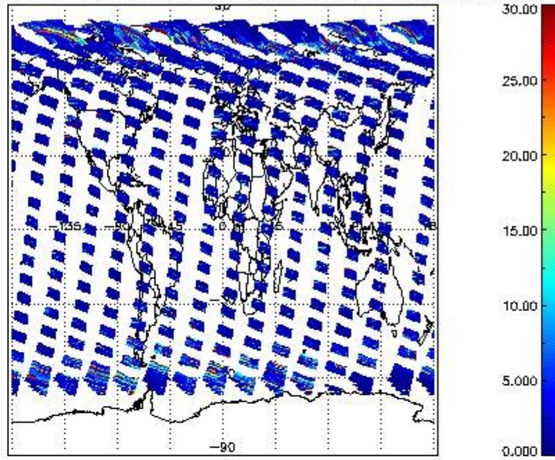
SCIOL2P_NADUV5S02_vcd_err for 05SEP2002 00:00:00 to 06SEP2002 00:00:00
