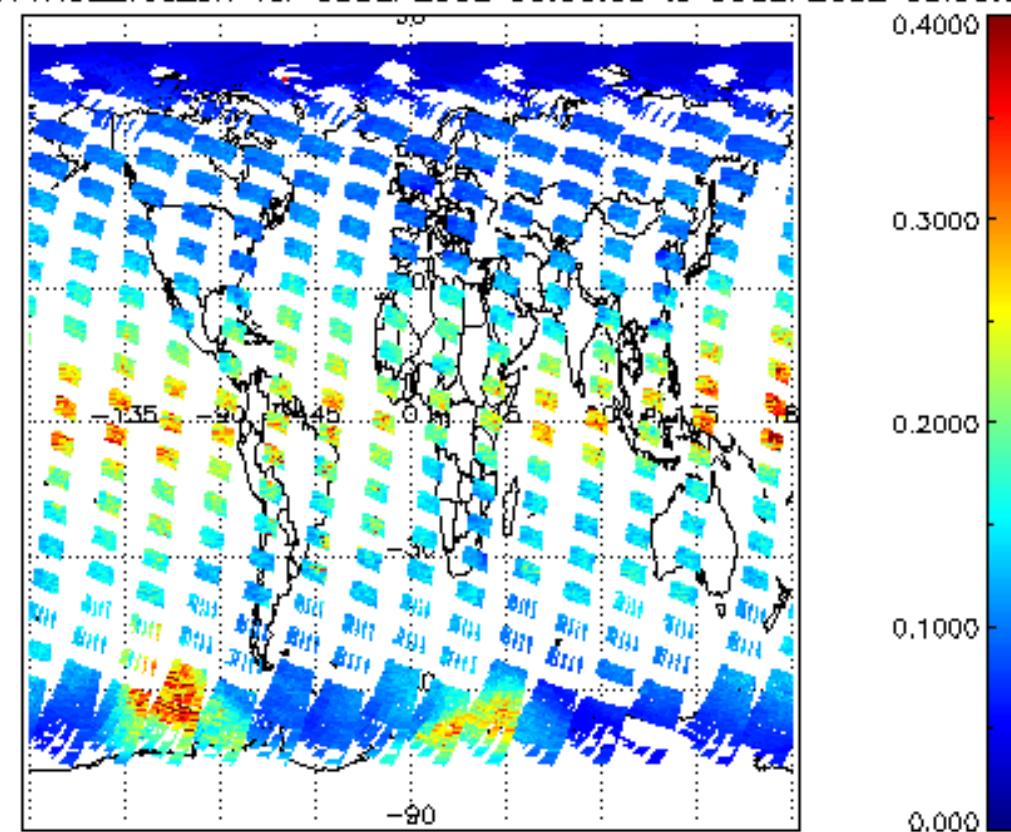
iCIOL2P_NADUV1NO2_vcd_err for 05SEP2002 00:00:00 to 06SEP2002 00:00:00
