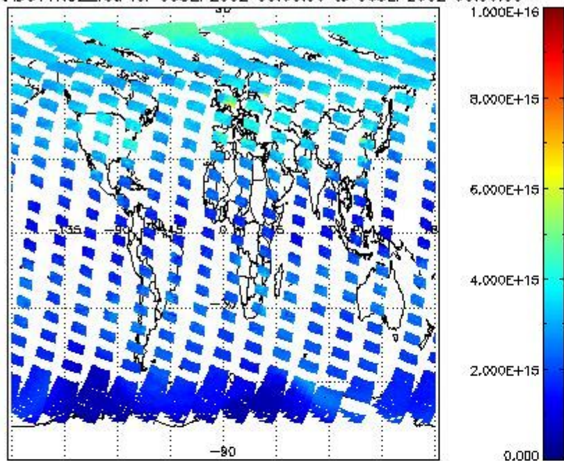
SCIOL2P_NADUV1N02_vcd for 05SEP2002 00:00:00 to 06SEP2002 00:00:00
