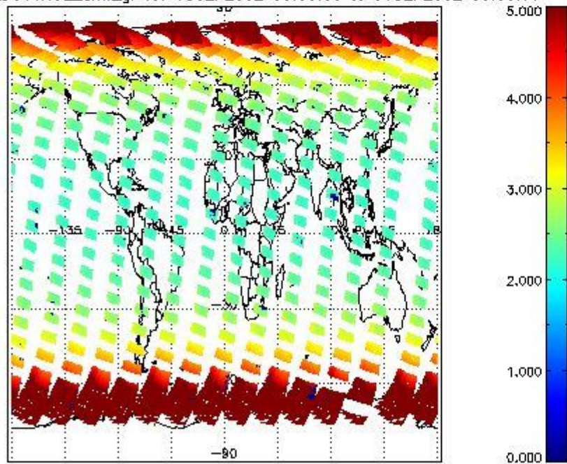
SCIOL2P_NADUV1N02_amf_gr for 05SEP2002 00:00:00 to 06SEP2002 00:00:00
