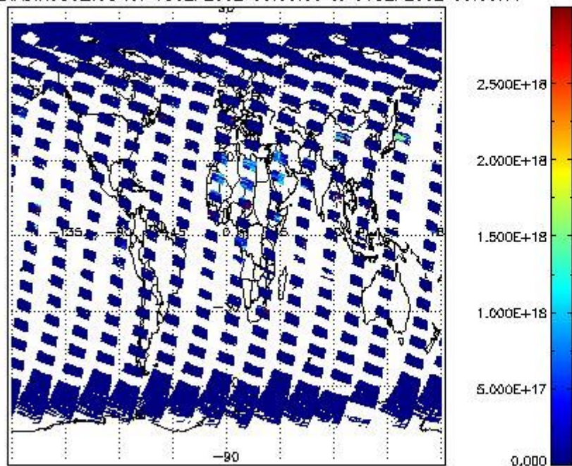
SCIDL2P_NADIR3CO_vcd for 05SEP2002 00:00:00 to 06SEP2002 00:00:00
