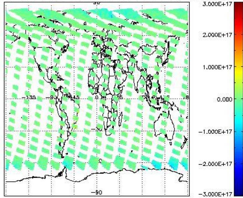
SCIOL2P_NADUV7S02_vcd for 05SEP2002 00:00:00 to 06SEP2002 00:00:00
