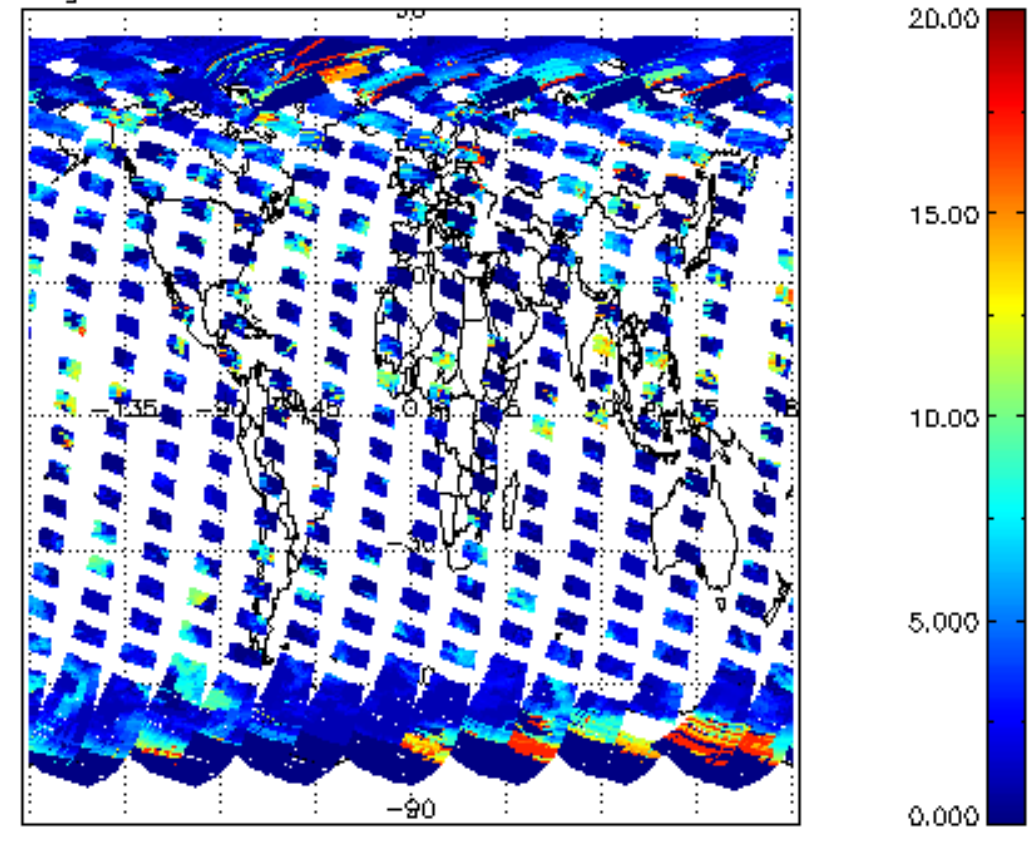
cl_top_height for 05SEP2002 00:00:00 to 06SEP2002 00:00:00
