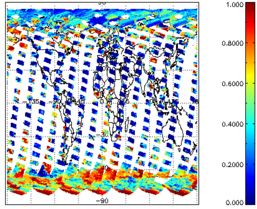
cl_frac for 05SEP2002 00:00:00 to 06SEP2002 00:00:00
