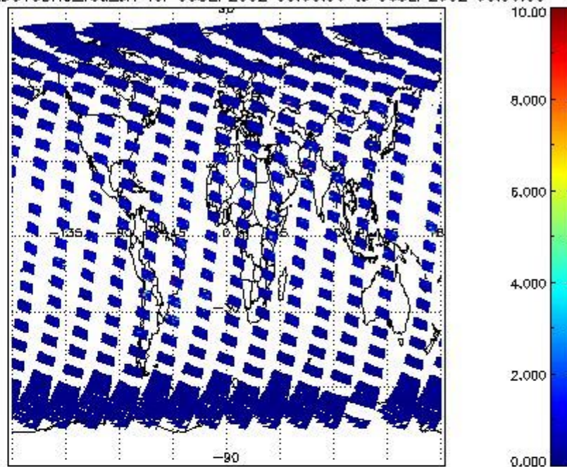
SCIOL2P_NADUV3BRO_vcd_err for 05SEP2002 00:00:00 to 06SEP2002 00:00:00
