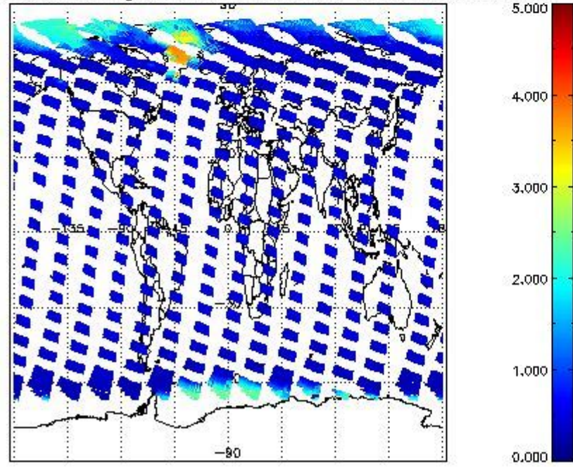
SCIOL2P_NADUV5S02_amf_gr for 05SEP2002 00:00:00 to 06SEP2002 00:00:00
