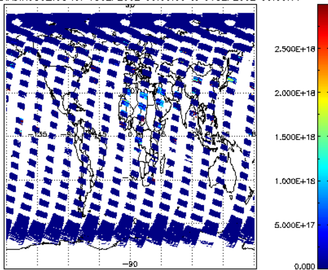
SCIOL2P_NADIR3CO_vcd for 05SEP2002 00:00:00 to 06SEP2002 00:00:00
