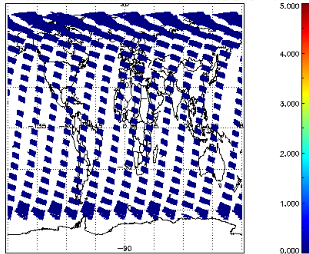
SCIOL2P_NADUV7S02_amf_cl for 05SEP2002 00:00:00 to 06SEP2002 00:00:00
