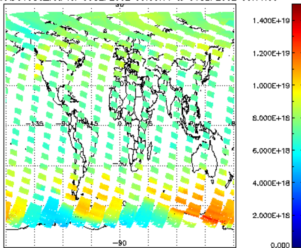
SCIOL2P_NADUV003_vcd for 05SEP2002 00:00:00 to 06SEP2002 00:00:00
