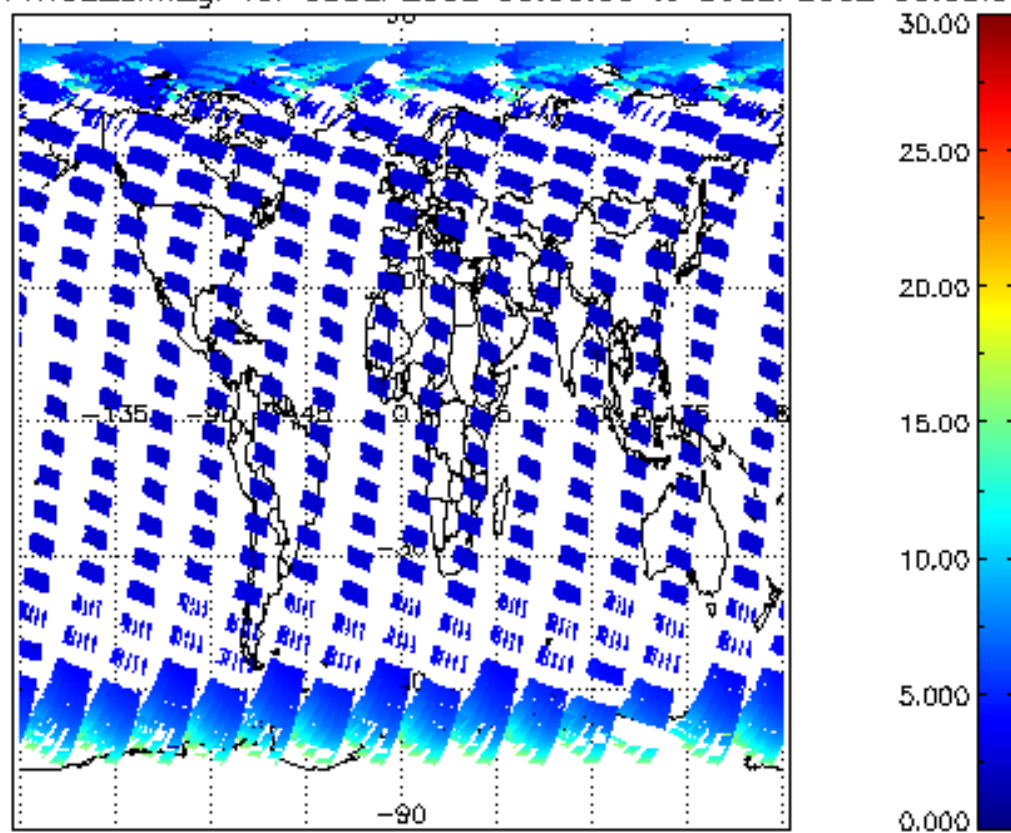
iCIOL2P_NADUV1NO2_amf_gr for 05SEP2002 00:00:00 to 06SEP2002 00:00:00
