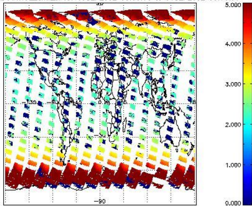
SCIOL2P_NADUV1N02_amf_cl for 05SEP2002 00:00:00 to 06SEP2002 00:00:00
