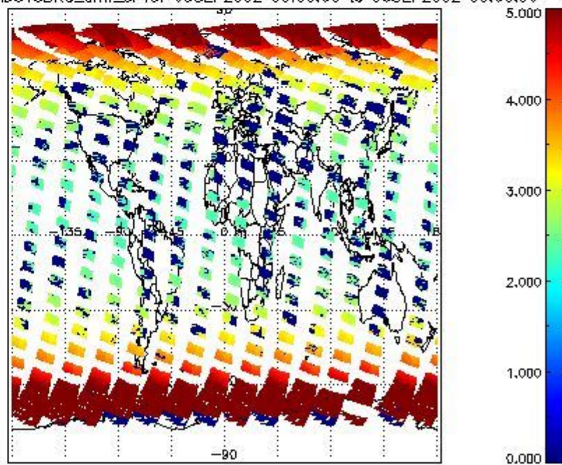
SCIOL2P_NADUV3BRO_amf_cl for 05SEP2002 00:00:00 to 06SEP2002 00:00:00
