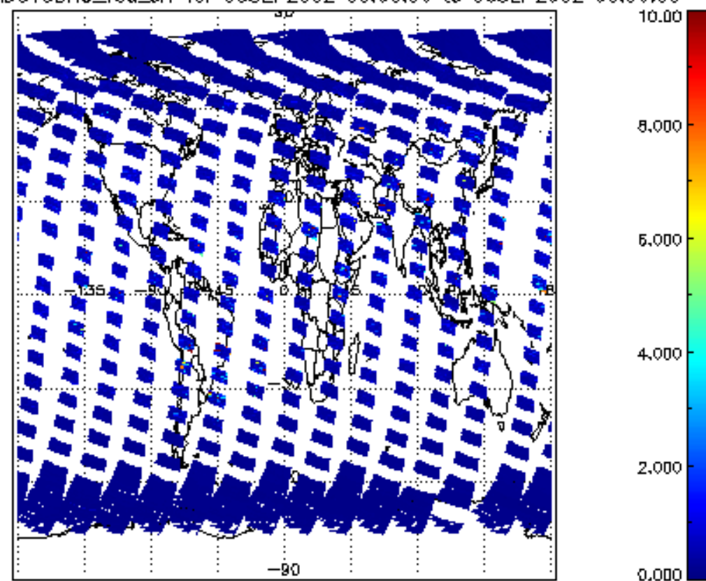
SCIOL2P_NADUV3BRO_vcd_err for 05SEP2002 00:00:00 to 06SEP2002 00:00:00
