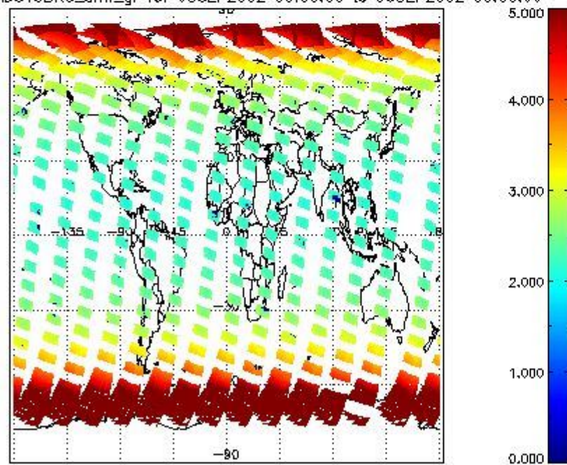
SCIOL2P_NADUV3BRO_amf_gr for 05SEP2002 00:00:00 to 06SEP2002 00:00:00
