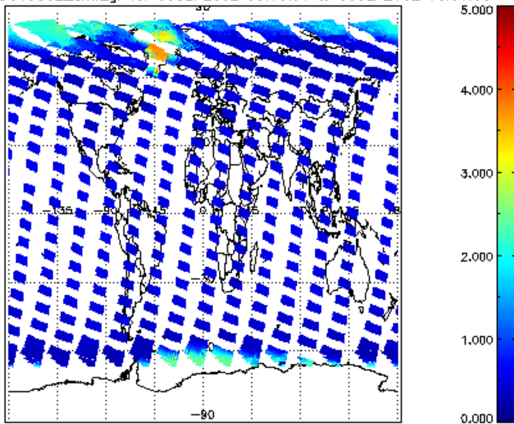
SCIOL2P_NADUV5S02_amf_gr for 05SEP2002 00:00:00 to 06SEP2002 00:00:00
