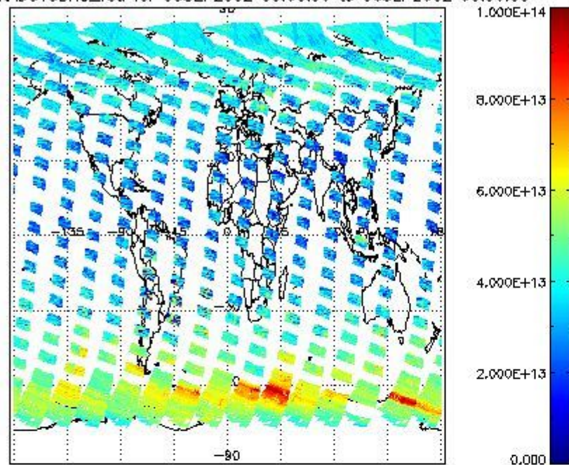
SCIOL2P_NADUV3BRO_vcd for 05SEP2002 00:00:00 to 06SEP2002 00:00:00
