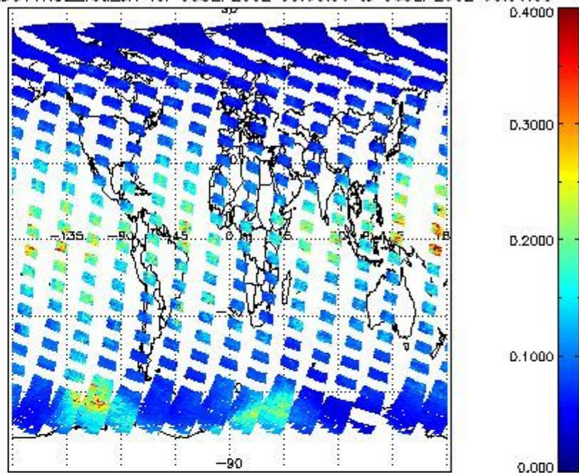
SCIOL2P_NADUV1N02_vcd_err for 05SEP2002 00:00:00 to 06SEP2002 00:00:00
