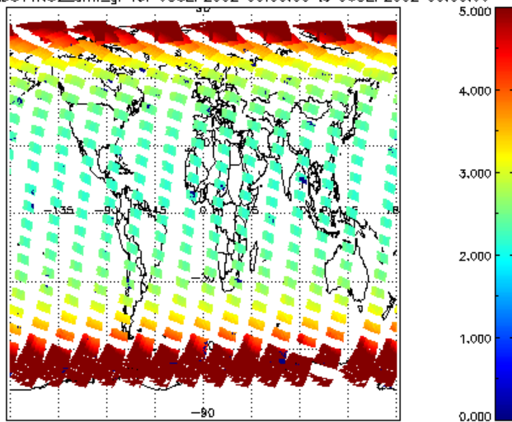
SCIOL2P_NADUV1N02_amf_gr for 05SEP2002 00:00:00 to 06SEP2002 00:00:00
