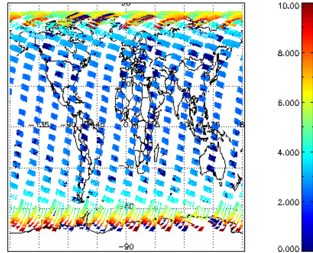
SCIOL2P_NADUV003_amf_cl for 05SEP2002 00:00:00 to 06SEP2002 00:00:00
