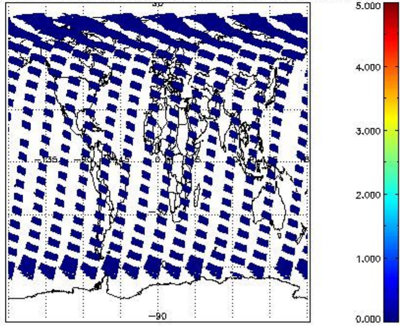
SCIOL2P_NADUV7S02_amf_cl for 05SEP2002 00:00:00 to 06SEP2002 00:00:00
