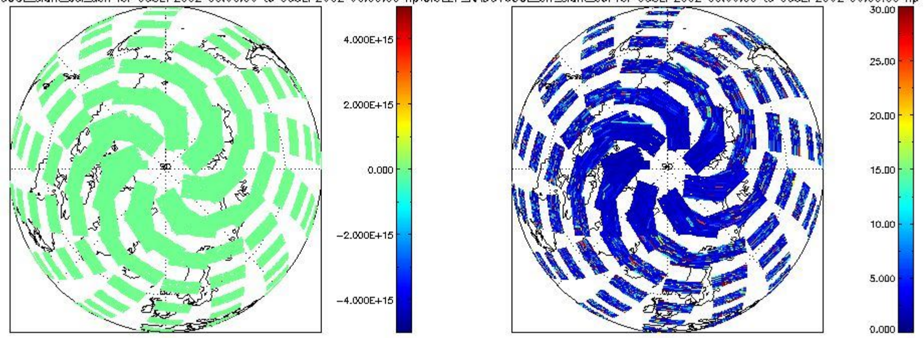
CIOL2P_NADUV60CLslant_col_den for 05SEP2002 00:00:00 to 06SEP2002 00:00:00 np; CIOL2P_NADUV60CLarr_slant_col for 05SEP2002 00:00:00 to 06SEP2002 00:00:00 np
