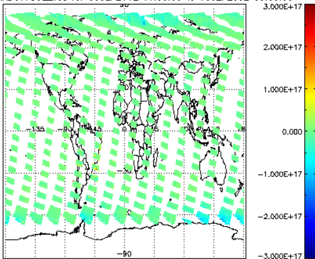
SCIOL2P_NADUV7S02_vcd for 05SEP2002 00:00:00 to 06SEP2002 00:00:00
