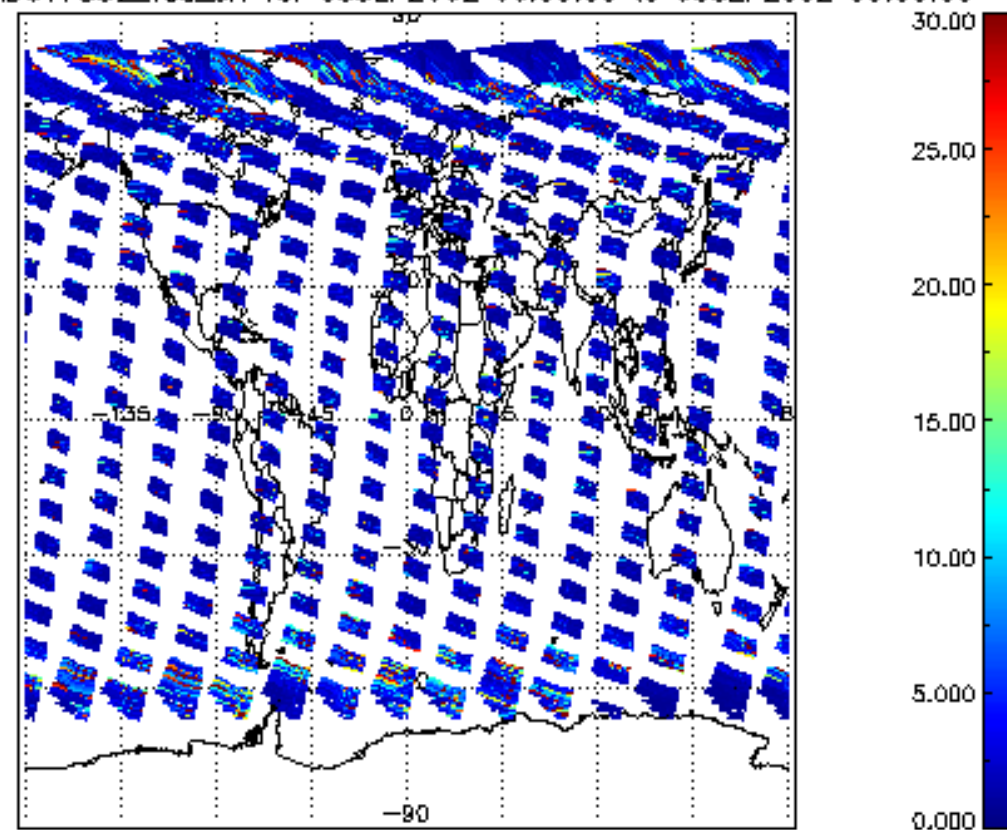
SCIOL2P_NADUV7S02_vcd_err for 05SEP2002 00:00:00 to 06SEP2002 00:00:00
