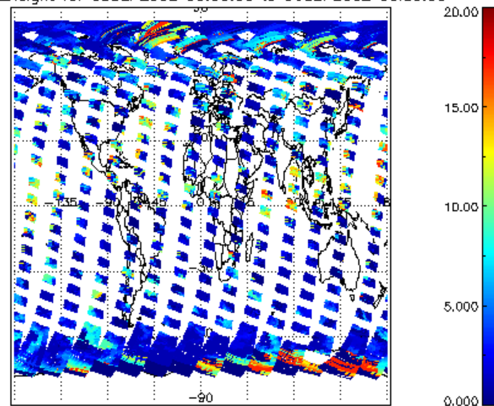
cl_top_height for 05SEP2002 00:00:00 to 06SEP2002 00:00:00
