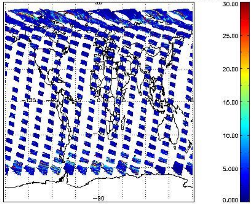
SCIOL2P_NADUV7S02_vcd_err for 05SEP2002 00:00:00 to 06SEP2002 00:00:00
