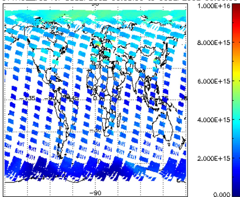
SCIOL2P_NADUV1NO2_vcd for 05SEP2002 00:00:00 to 06SEP2002 00:00:00
