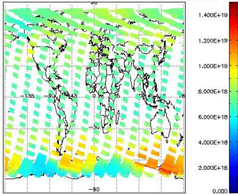
SCIOL2P_NADUV003_vcd for 05SEP2002 00:00:00 to 06SEP2002 00:00:00
