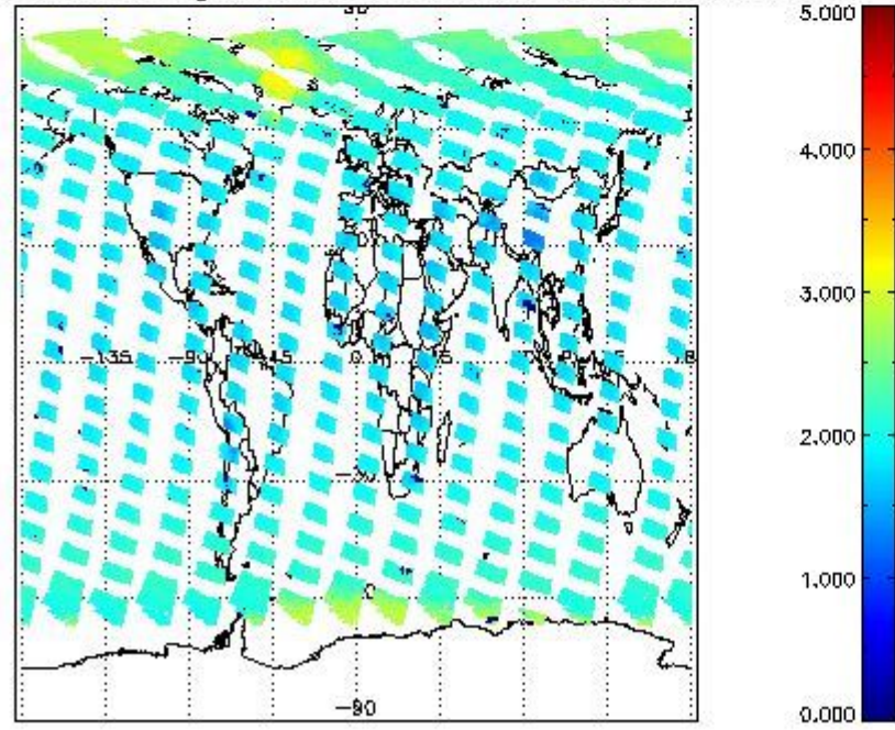
SCIOL2P_NADUV7S02_amf_gr for 05SEP2002 00:00:00 to 06SEP2002 00:00:00
