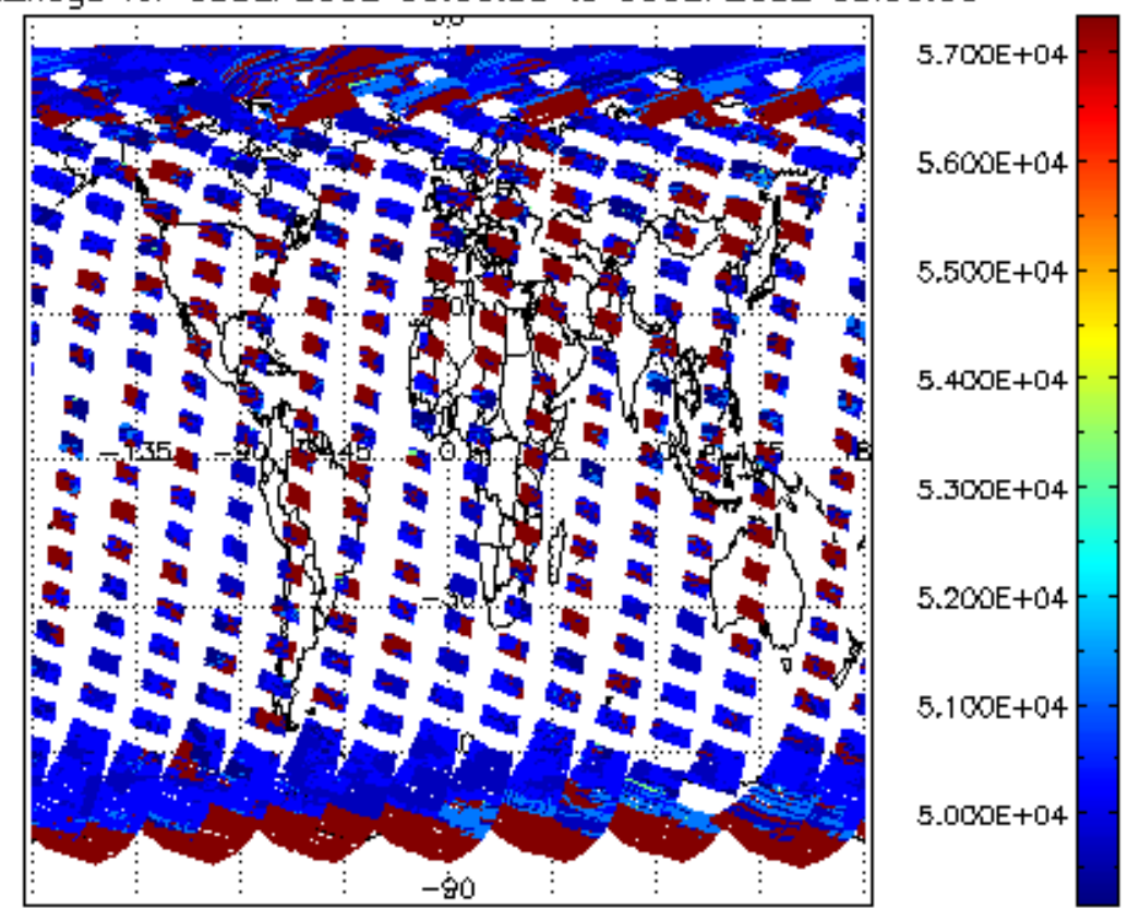
cloud_flags for 05SEP2002 00:00:00 to 06SEP2002 00:00:00
