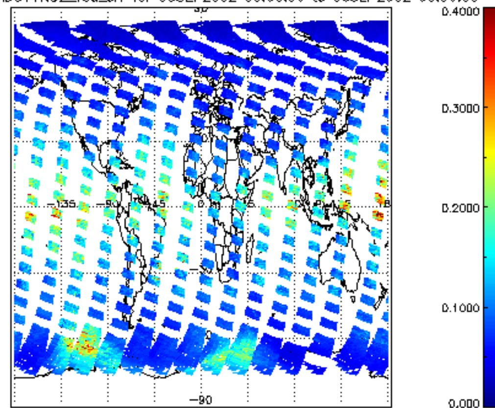
SCIOL2P_NADUV1N02_vcd_err for 05SEP2002 00:00:00 to 06SEP2002 00:00:00
