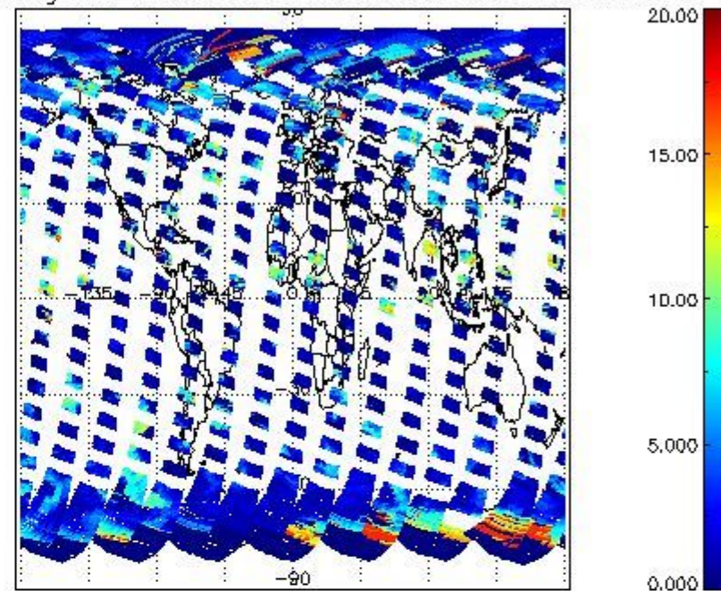
cL_top_height for 05SEP2002 00:00:00 to 06SEP2002 00:00:00
