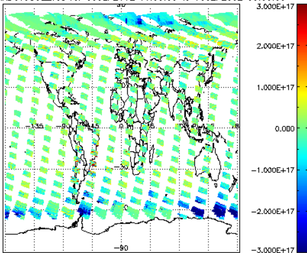
SCIOL2P_NADUV5S02_vcd for 05SEP2002 00:00:00 to 06SEP2002 00:00:00
