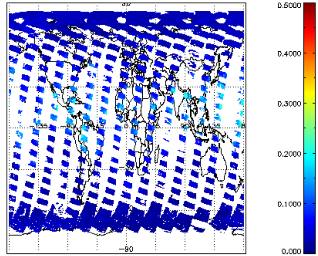
SCIOL2P_NADUV8H20_vcd_err for 05SEP2002 00:00:00 to 06SEP2002 00:00:00
