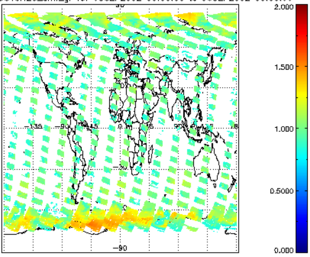
SCIOL2P_NADUV8H20_amf_gr for 05SEP2002 00:00:00 to 06SEP2002 00:00:00
