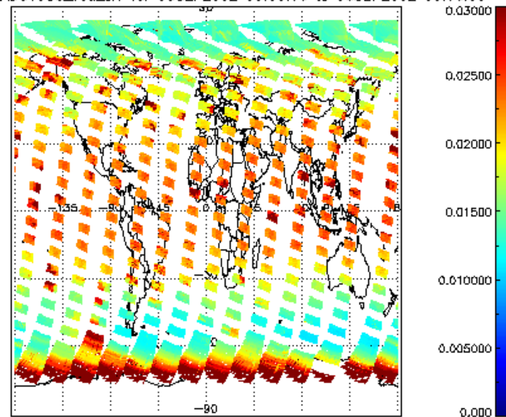
SCIOL2P_NADUV003_vcd_err for 05SEP2002 00:00:00 to 06SEP2002 00:00:00
