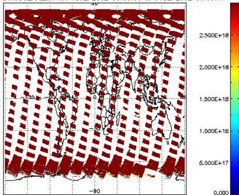
SCIDL2P_NADIR3CO_vcd_err for 05SEP2002 00:00:00 to 06SEP2002 00:00:00
