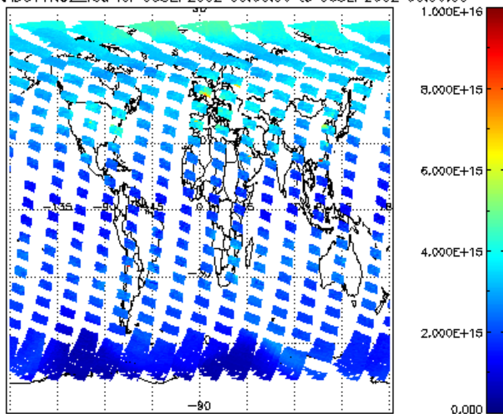
SCIOL2P_NADUV1N02_vcd for 05SEP2002 00:00:00 to 06SEP2002 00:00:00
