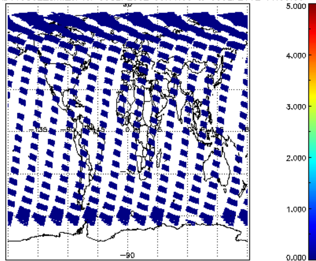
SCIOL2P_NADUV5S02_amf_cl for 05SEP2002 00:00:00 to 06SEP2002 00:00:00
