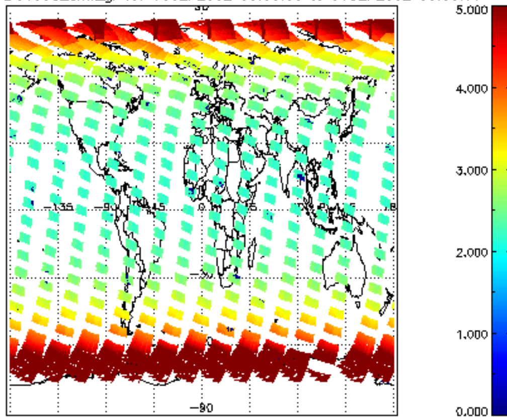
SCIOL2P_NADUV003_amf_gr for 05SEP2002 00:00:00 to 06SEP2002 00:00:00
