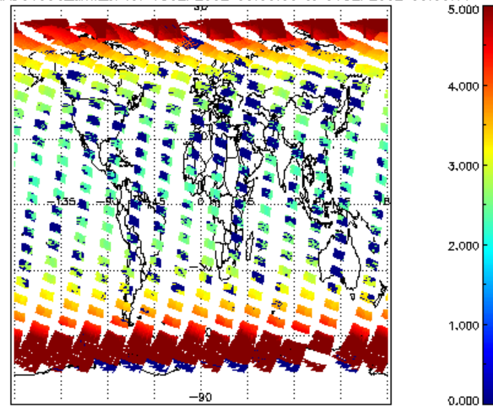
SCIOL2P_NADUV003_amf_cl for 05SEP2002 00:00:00 to 06SEP2002 00:00:00
