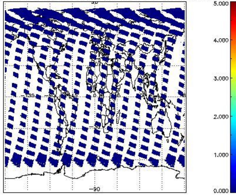
SCIOL2P_NADUV5S02_amf_cl for 05SEP2002 00:00:00 to 06SEP2002 00:00:00
