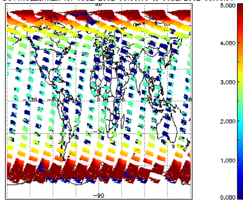
SCIOL2P_NADUV1N02_amf_sl for 05SEP2002 00:00:00 to 06SEP2002 00:00:00
