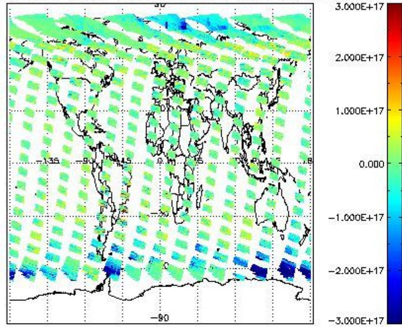
SCIOL2P_NADUV5S02_vcd for 05SEP2002 00:00:00 to 06SEP2002 00:00:00
