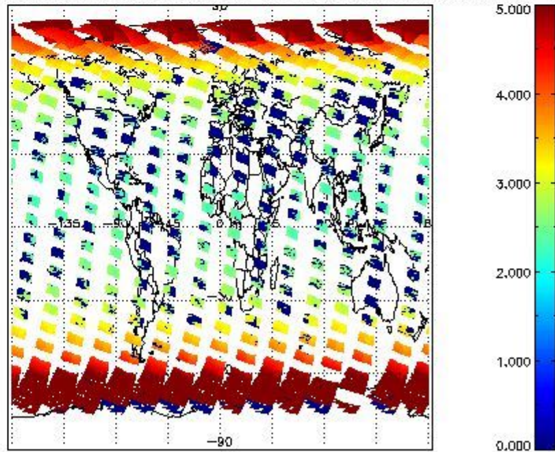
SCIOL2P_NADUV003_amf_cl for 05SEP2002 00:00:00 to 06SEP2002 00:00:00
