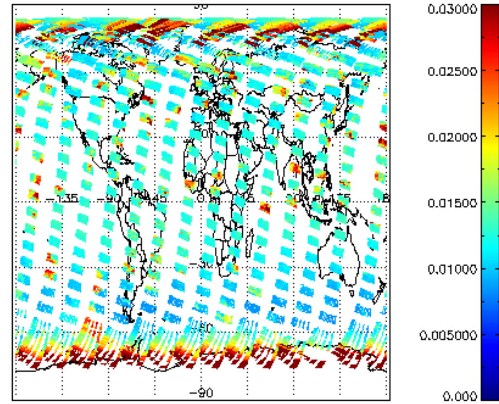
SCIOL2P_NADUV003_vcd_err for 05SEP2002 00:00:00 to 06SEP2002 00:00:00
