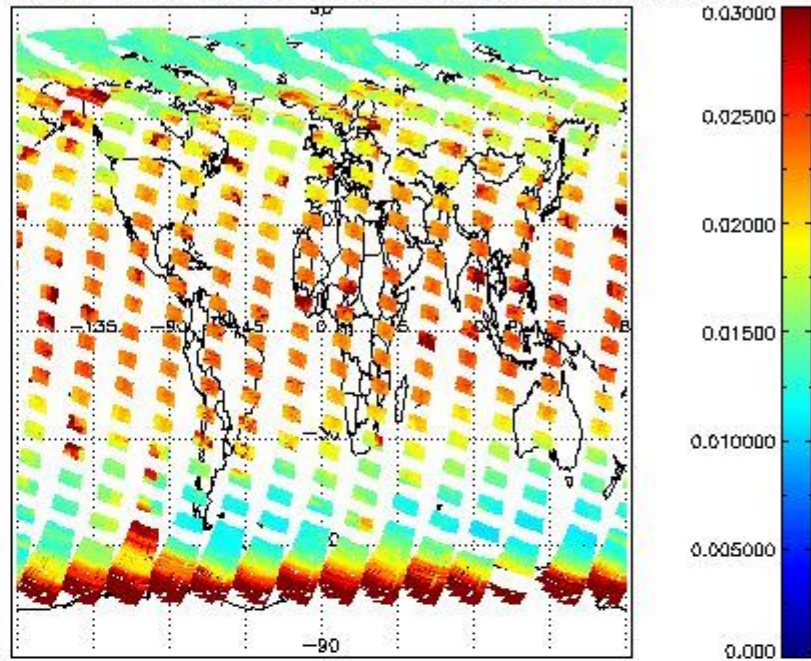
SCIOL2P_NADUV003_vcd_err for 05SEP2002 00:00:00 to 06SEP2002 00:00:00
