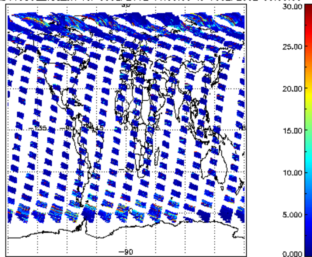
SCIOL2P_NADUV5S02_vcd_err for 05SEP2002 00:00:00 to 06SEP2002 00:00:00
