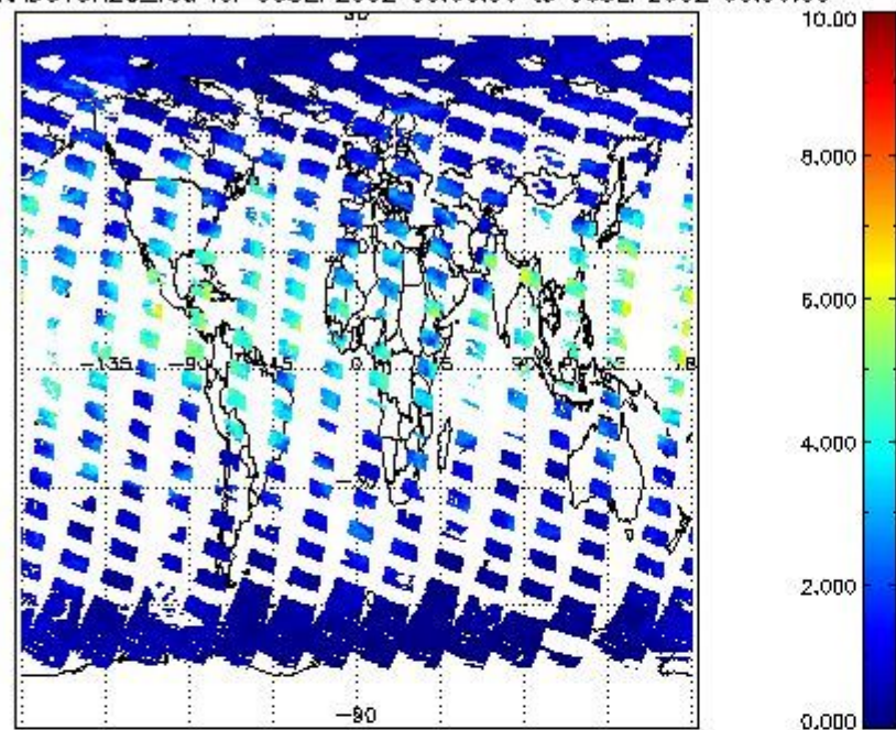
SCIOL2P_NADUV8H2O_vcd for 05SEP2002 00:00:00 to 06SEP2002 00:00:00
