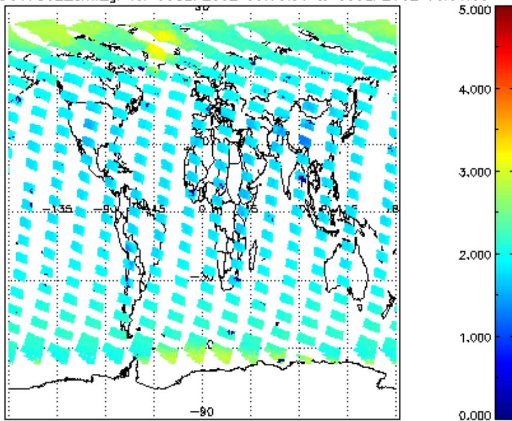
SCIOL2P_NADUV7S02_amf_gr for 05SEP2002 00:00:00 to 06SEP2002 00:00:00
