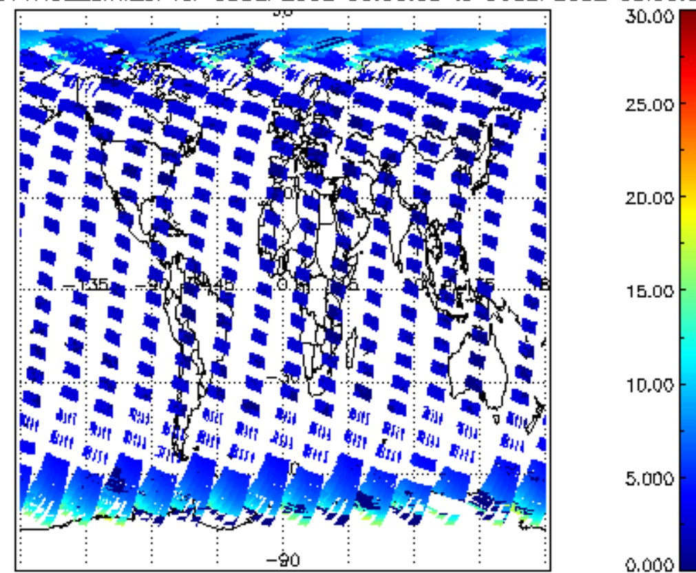
iCIOL2P_NADUV1NO2_amf_cl for 05SEP2002 00:00:00 to 06SEP2002 00:00:00
