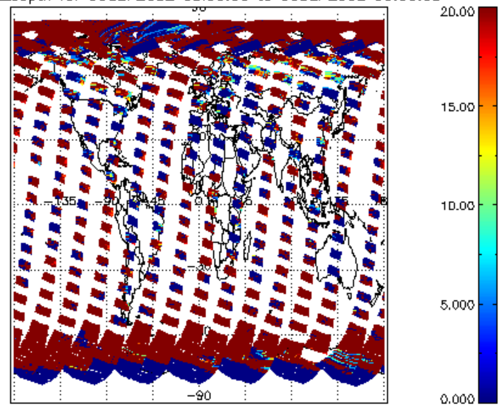
cl_lopt_depth for 05SEP2002 00:00:00 to 06SEP2002 00:00:00
