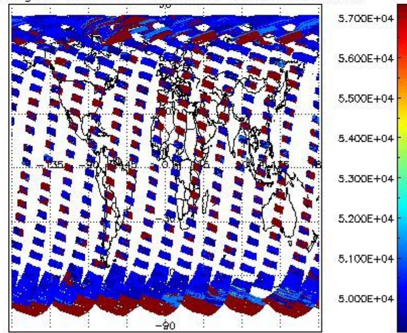
cloud_flags for 05SEP2002 00:00:00 to 06SEP2002 00:00:00
