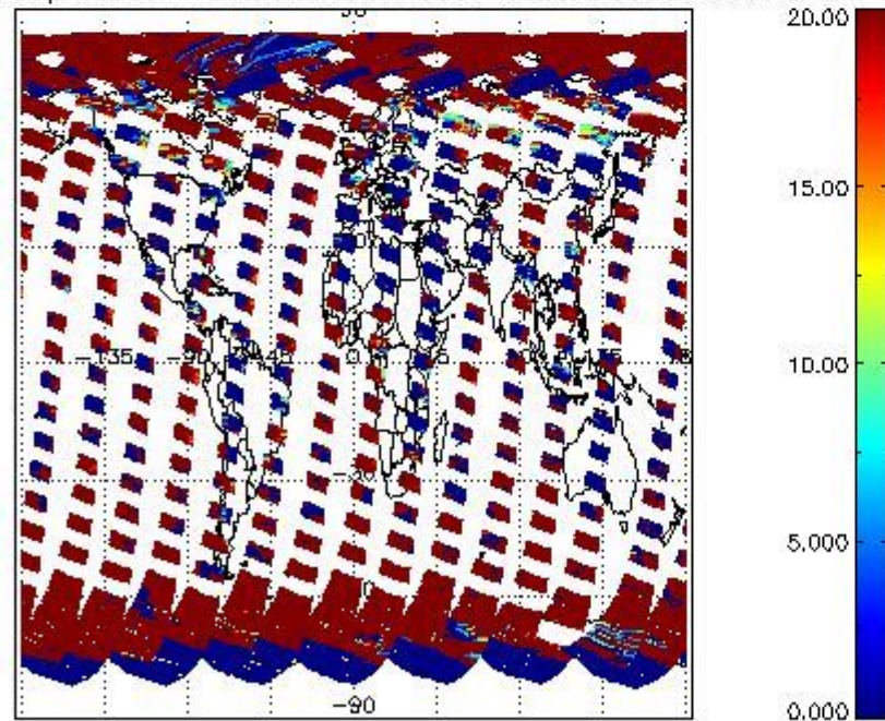
cL_opt_depth for 05SEP2002 00:00:00 to 06SEP2002 00:00:00
