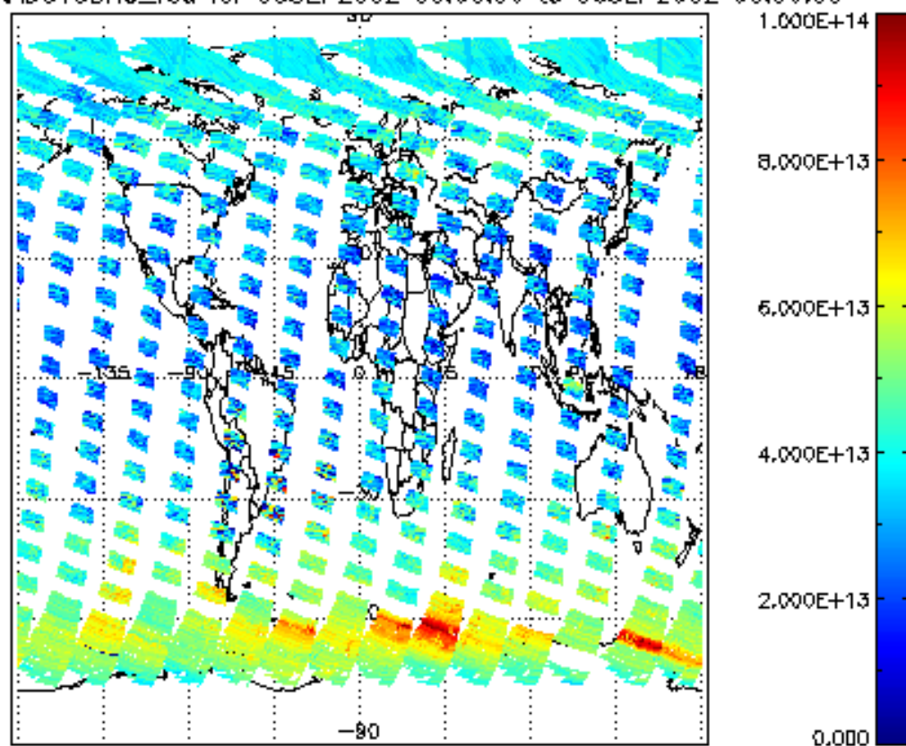
SCIOL2P_NADUV3BRO_vcd for 05SEP2002 00:00:00 to 06SEP2002 00:00:00
