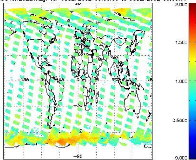
SCIOL2P_NADUV8H2O_arnf_gr for 05SEP2002 00:00:00 to 06SEP2002 00:00:00
