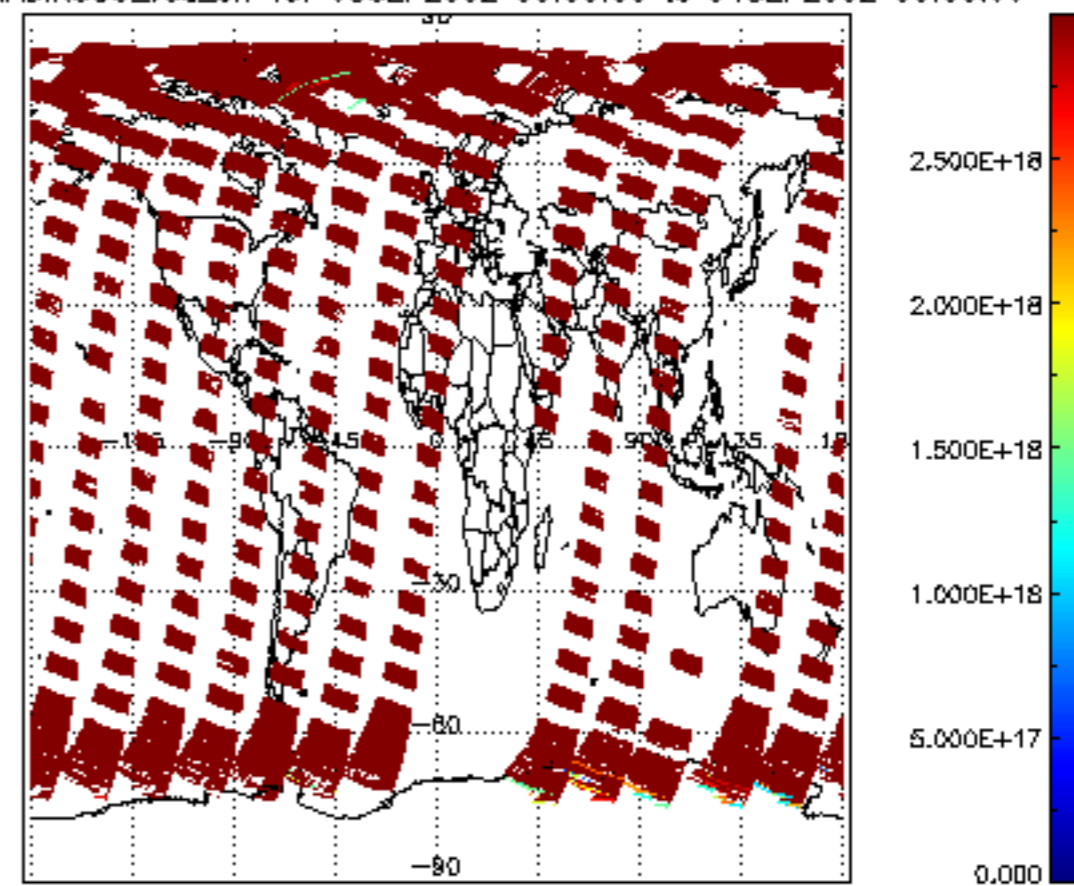
SCIOL2P_NADIR3CO_vcd_err for 03SEP2002 00:00:00 to 04SEP2002 00:00:00
