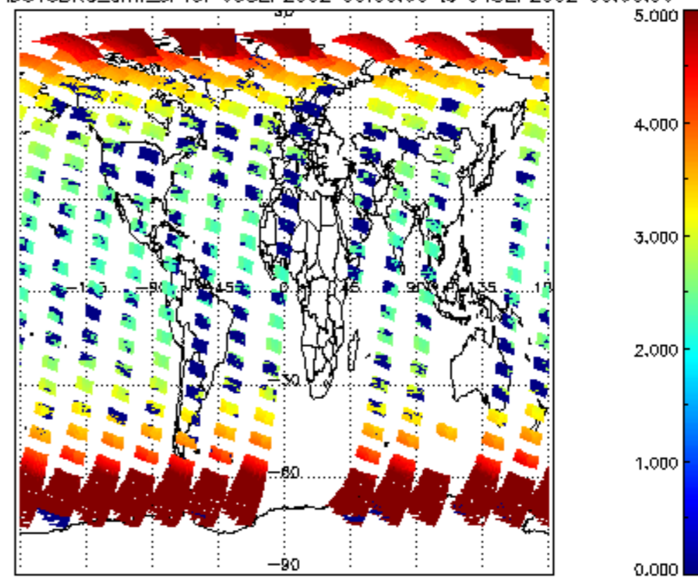
SCIOL2P_NADUV3BRO_amf_cl for 03SEP2002 00:00:00 to 04SEP2002 00:00:00
