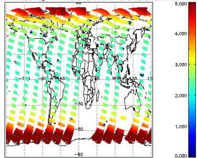
SCIOL2P_NADUV003_amf_gr for 03SEP2002 00:00:00 to 04SEP2002 00:00:00
