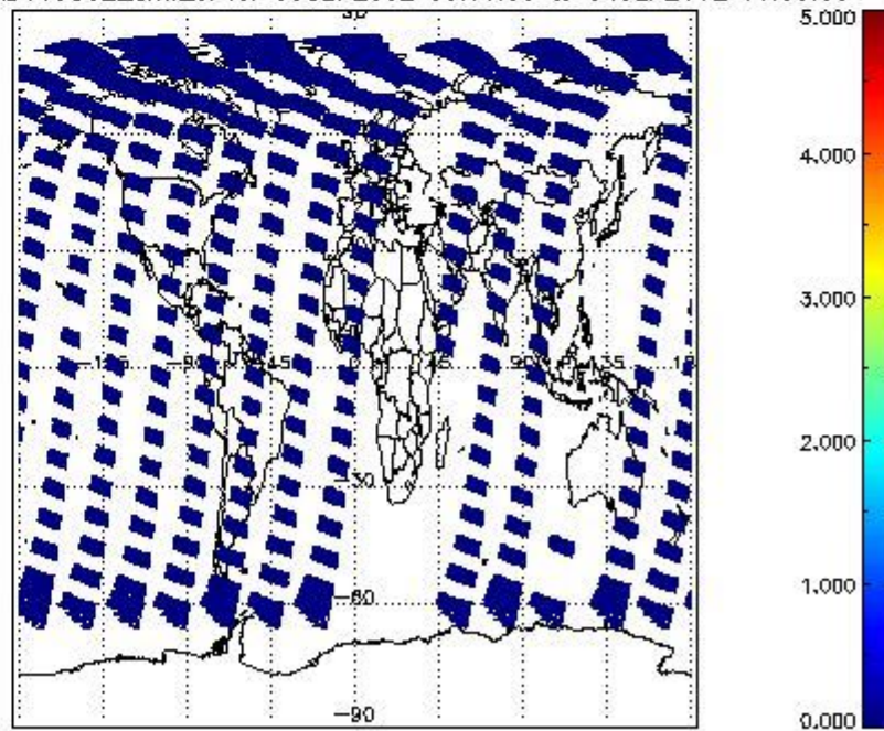
SCIOL2P_NADUV5S02_amf_cl for 03SEP2002 00:00:00 to 04SEP2002 00:00:00
