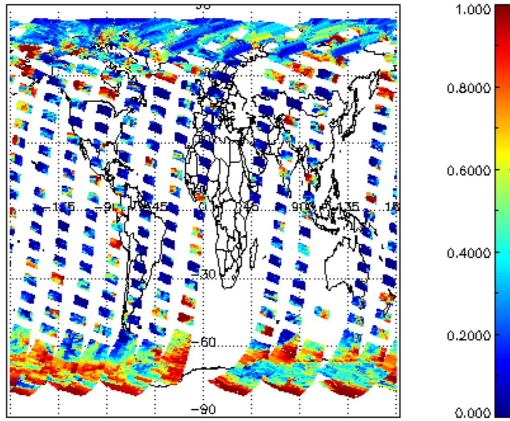
cl_frac for 03SEP2002 00:00:00 to 04SEP2002 00:00:00
