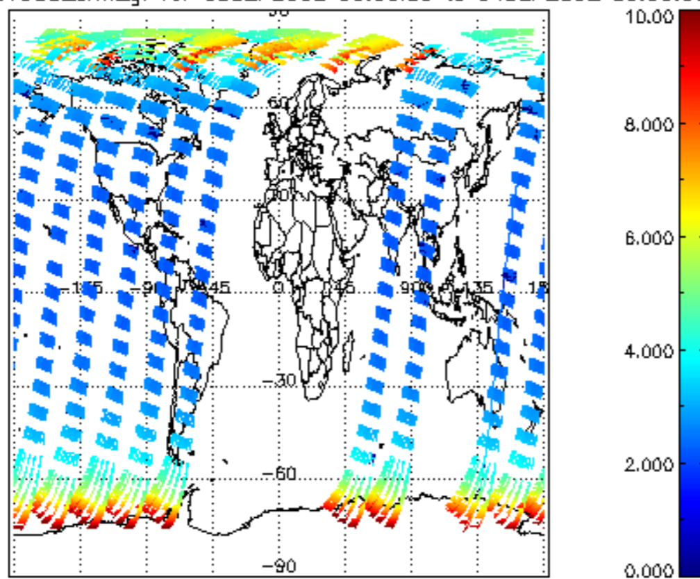
SCIOL2P_NADUV003_amf_gr for 03SEP2002 00:00:00 to 04SEP2002 00:00:00
