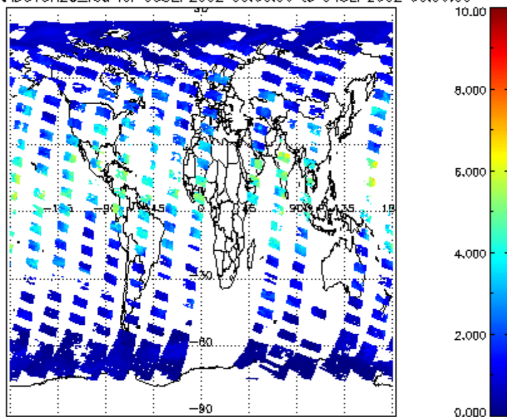
SCIOL2P_NADUV8H2O_vcd for 03SEP2002 00:00:00 to 04SEP2002 00:00:00
