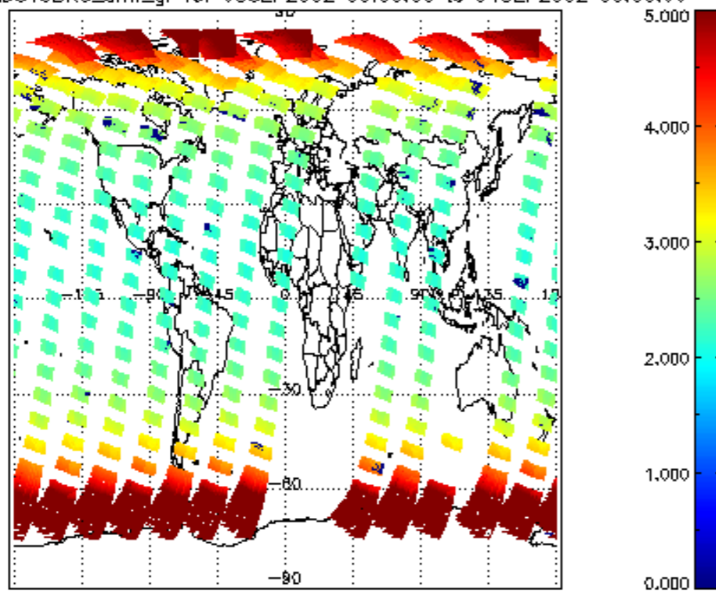
SCIOL2P_NADUV3BRO_amf_gr for 03SEP2002 00:00:00 to 04SEP2002 00:00:00
