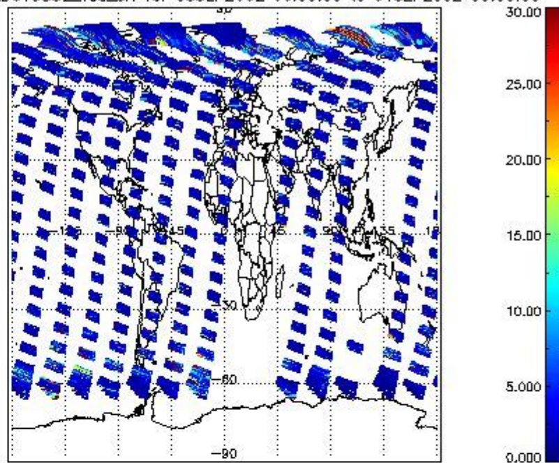
SCIOL2P_NADUV5S02_vcd_err for 03SEP2002 00:00:00 to 04SEP2002 00:00:00
