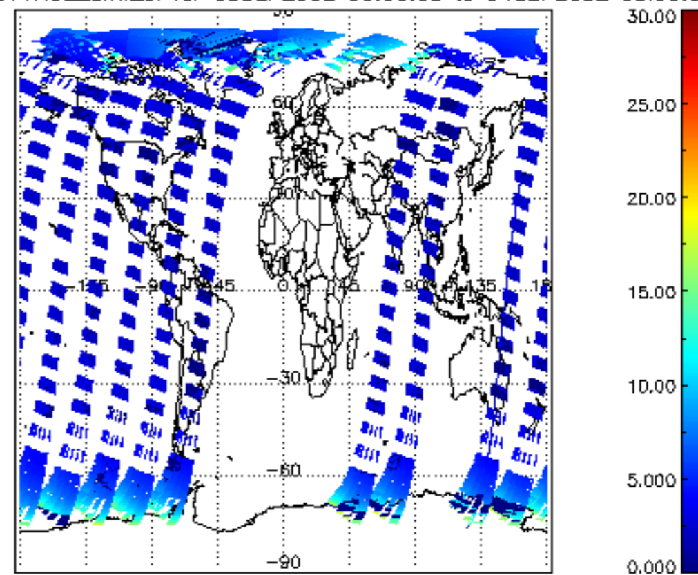
iCIOL2P_NADUV1NO2_amf_cl for 03SEP2002 00:00:00 to 04SEP2002 00:00:00
