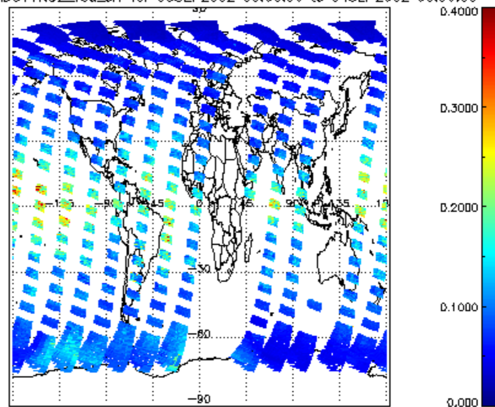
SCIOL2P_NADUV1NO2_vcd_err for 03SEP2002 00:00:00 to 04SEP2002 00:00:00
