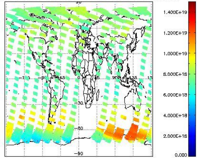
SCIOL2P_NADUV003_vcd for 03SEP2002 00:00:00 to 04SEP2002 00:00:00
