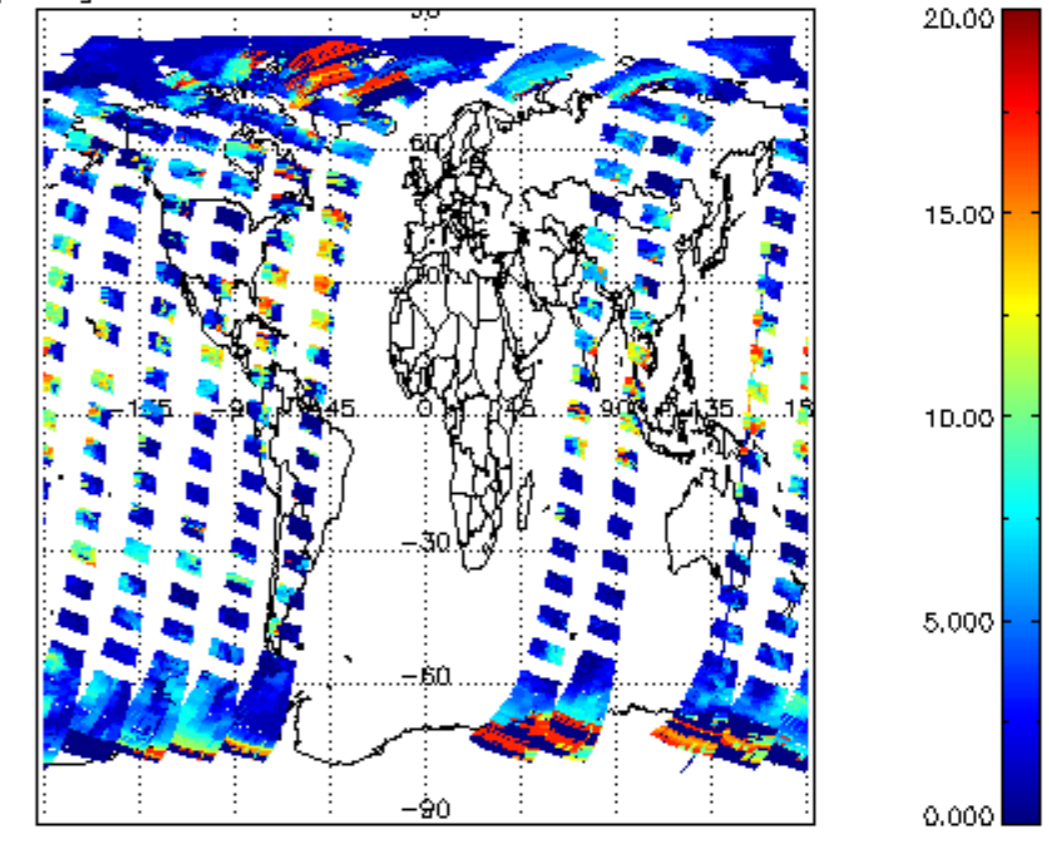
cl_top_height for 03SEP2002 00:00:00 to 04SEP2002 00:00:00
