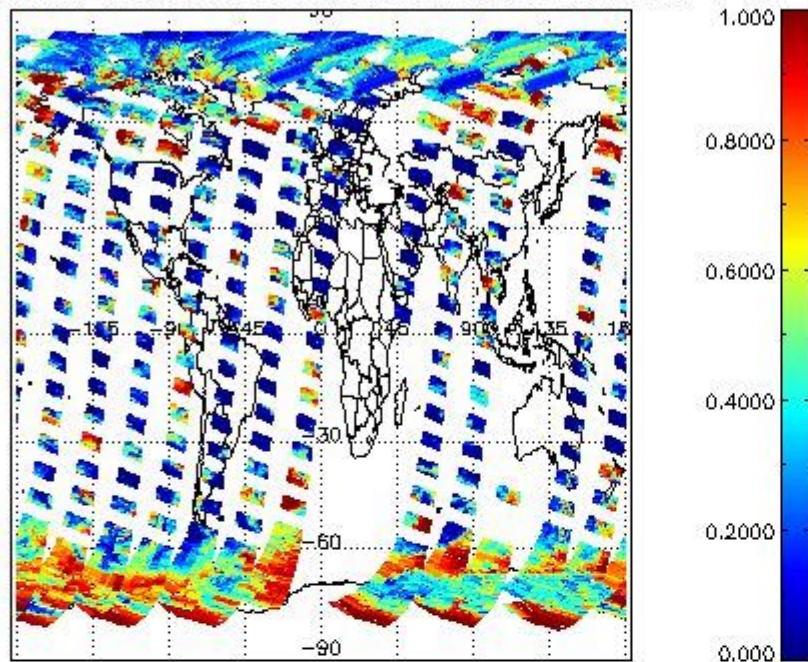
cL_frac for 03SEP2002 00:00:00 to 04SEP2002 00:00:00
