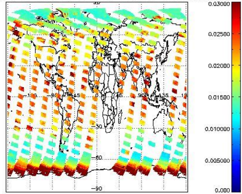
SCIOL2P_NADUV003_vcd_err for 03SEP2002 00:00:00 to 04SEP2002 00:00:00
