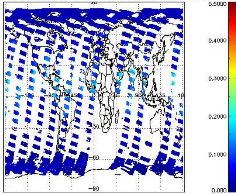
SCIOL2P_NADUV8H2O_vcd_err for 03SEP2002 00:00:00 to 04SEP2002 00:00:00
