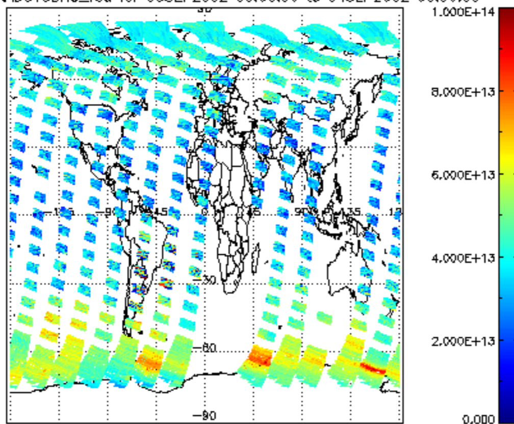
SCIOL2P_NADUV3BRO_vcd for 03SEP2002 00:00:00 to 04SEP2002 00:00:00
