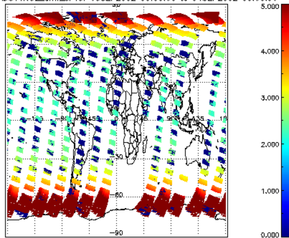
SCIOL2P_NADUV1NO2_amf_sl for 03SEP2002 00:00:00 to 04SEP2002 00:00:00
