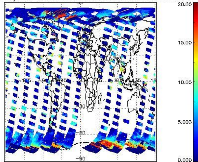
cL_top_height for 03SEP2002 00:00:00 to 04SEP2002 00:00:00
