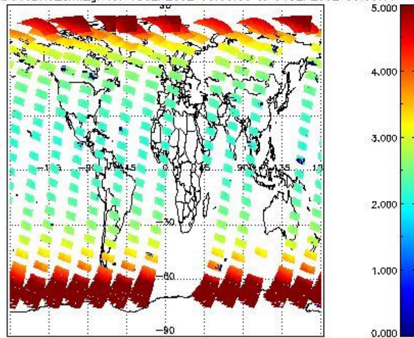
SCIOL2P_NADUV3BRO_amf_gr for 03SEP2002 00:00:00 to 04SEP2002 00:00:00
