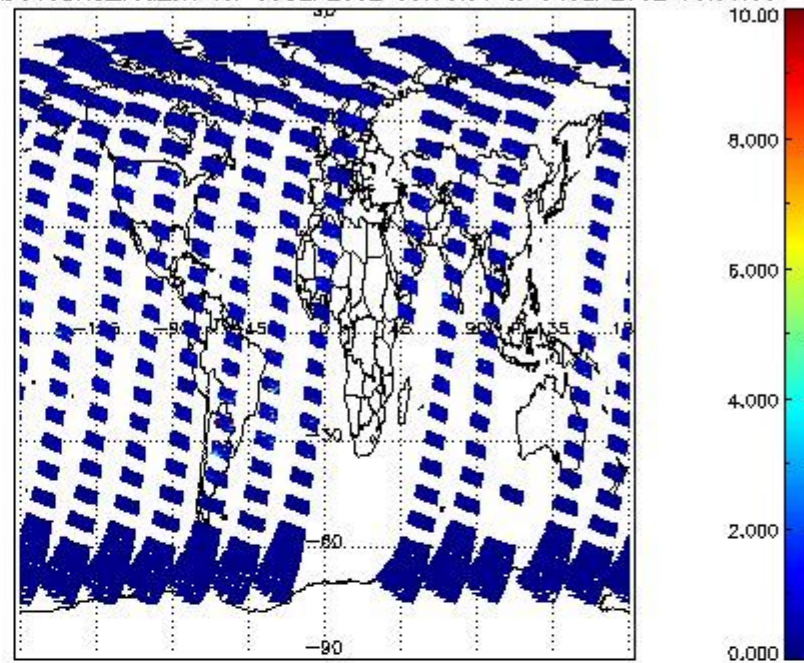
SCIOL2P_NADUV3BRO_vcd_err for 03SEP2002 00:00:00 to 04SEP2002 00:00:00
