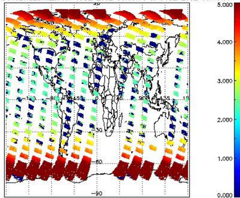
SCIOL2P_NADUV3BRO_amf_cl for 03SEP2002 00:00:00 to 04SEP2002 00:00:00
