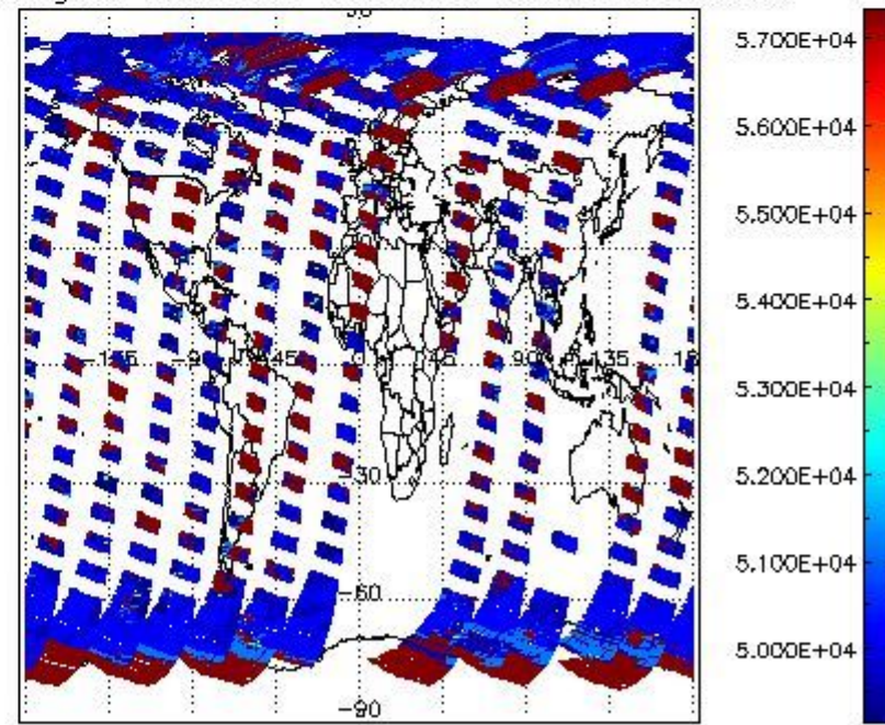
cloud_flags for 03SEP2002 00:00:00 to 04SEP2002 00:00:00
