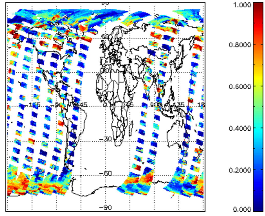
cl_frac for 03SEP2002 00:00:00 to 04SEP2002 00:00:00
