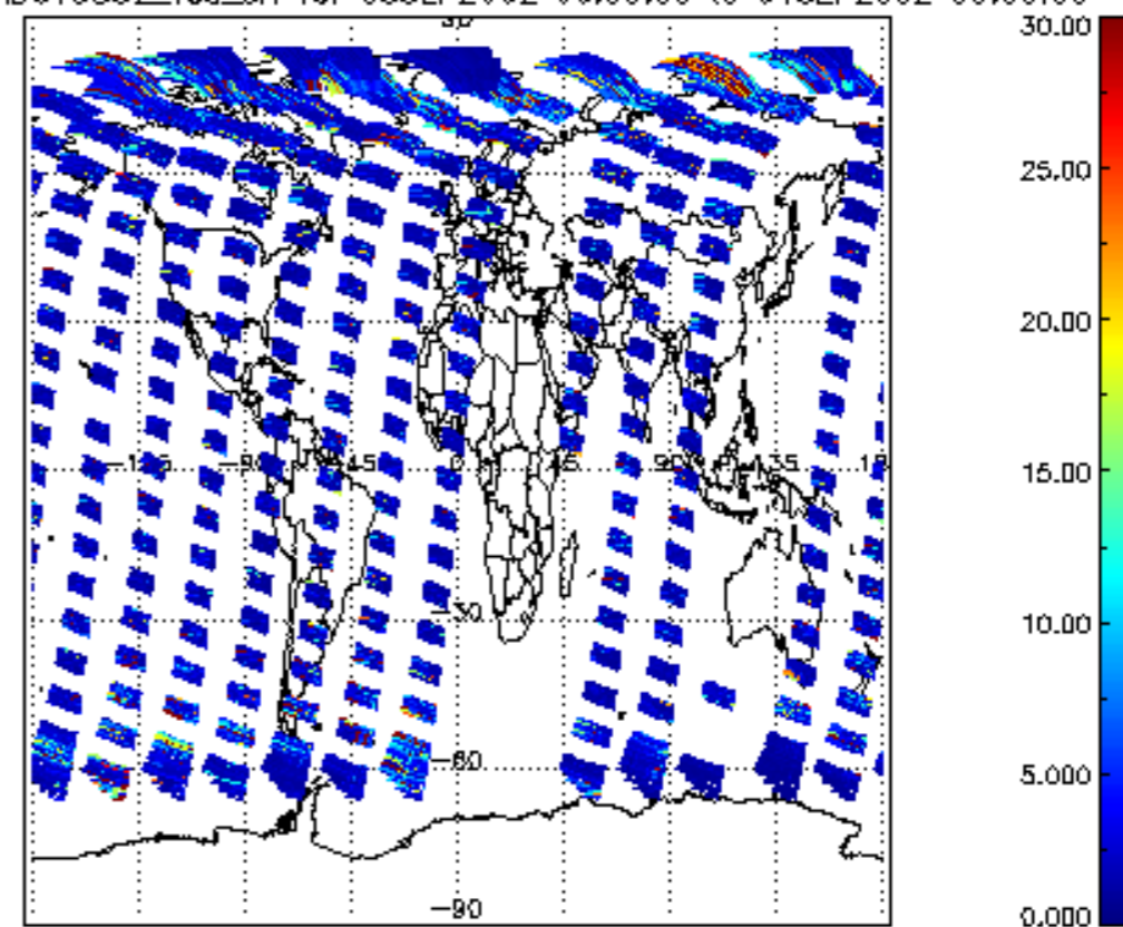
SCIOL2P_NADUV5S02_vcd_err for 03SEP2002 00:00:00 to 04SEP2002 00:00:00
