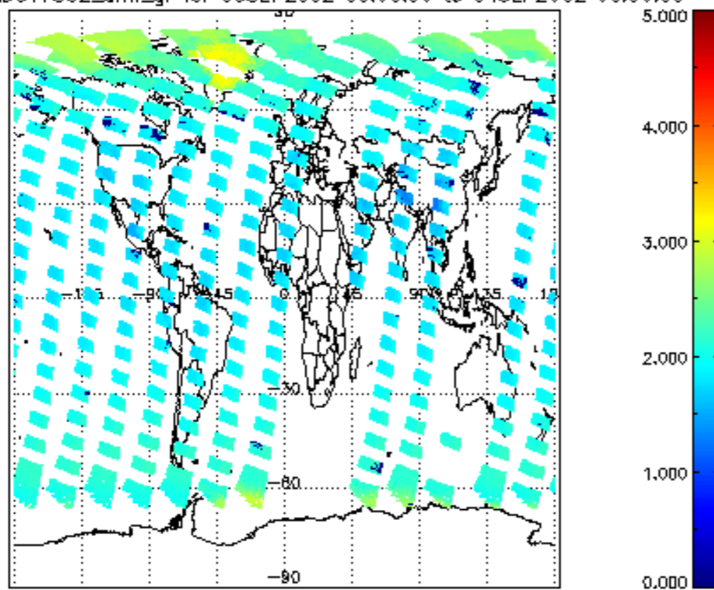
SCIOL2P_NADUV7S02_amf_gr for 03SEP2002 00:00:00 to 04SEP2002 00:00:00
