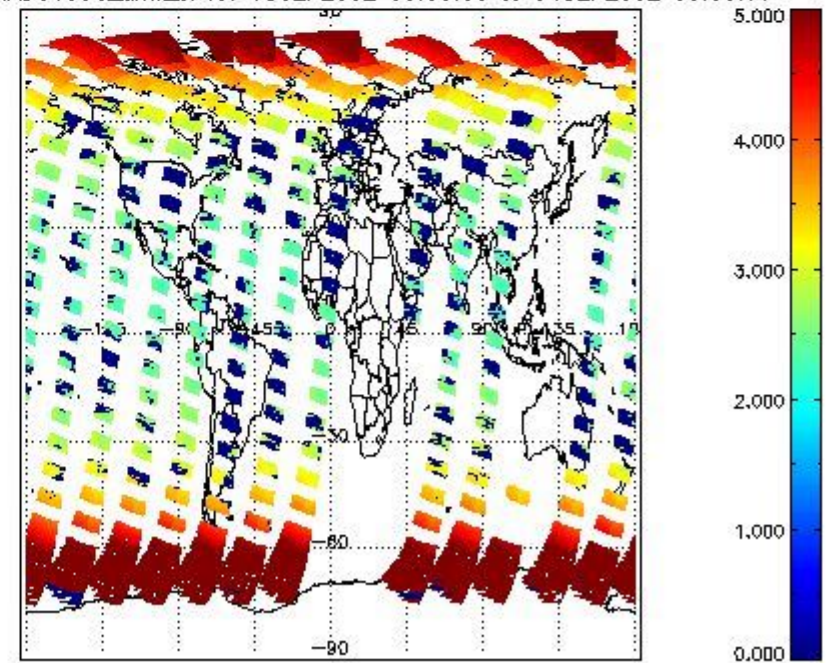
SCIOL2P_NADUV003_amf_cl for 03SEP2002 00:00:00 to 04SEP2002 00:00:00
