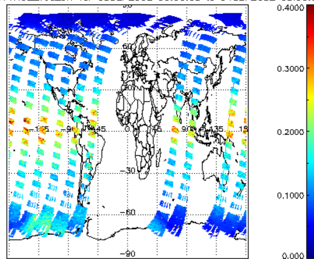
iCIOL2P_NADUV1NO2_vcd_err for 03SEP2002 00:00:00 to 04SEP2002 00:00:00
