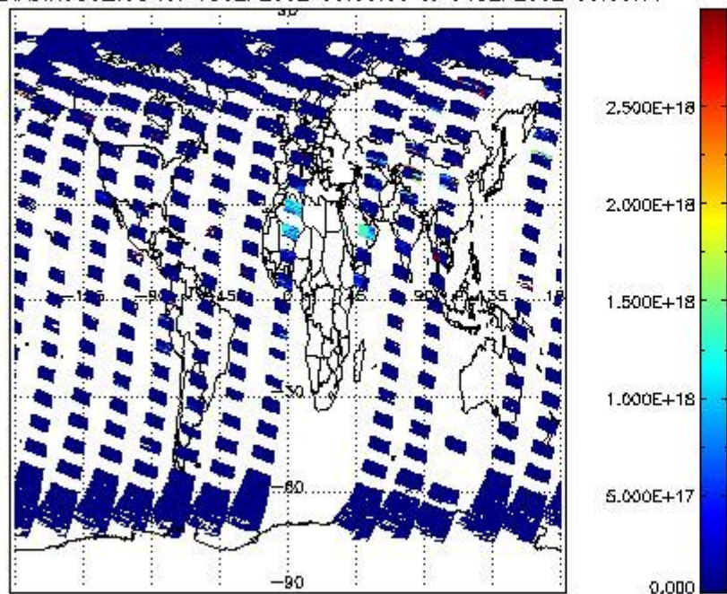
SCIDL2P_NADIR3CO_vcd for 03SEP2002 00:00:00 to 04SEP2002 00:00:00
