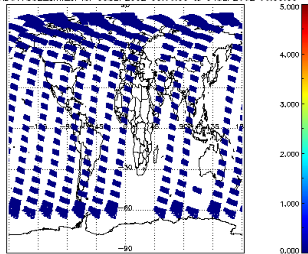
SCIOL2P_NADUV7S02_amf_cl for 03SEP2002 00:00:00 to 04SEP2002 00:00:00
