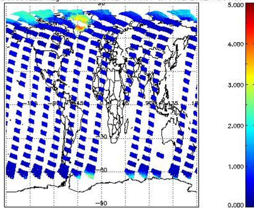
SCIOL2P_NADUV5S02_amf_gr for 03SEP2002 00:00:00 to 04SEP2002 00:00:00
