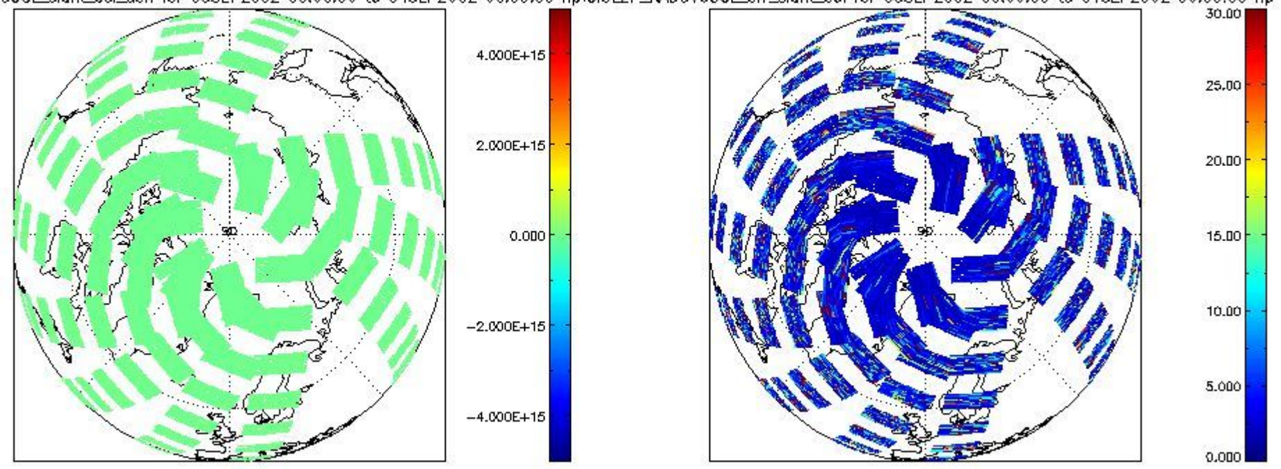
CIOL2P_NADUV60CLslant_col_den for 03SEP2002 00:00:00 to 04SEP2002 00:00:00 np; CIOL2P_NADUV60CLerr_slant_col for 03SEP2002 00:00:00 to 04SEP2002 00:00:00 np
