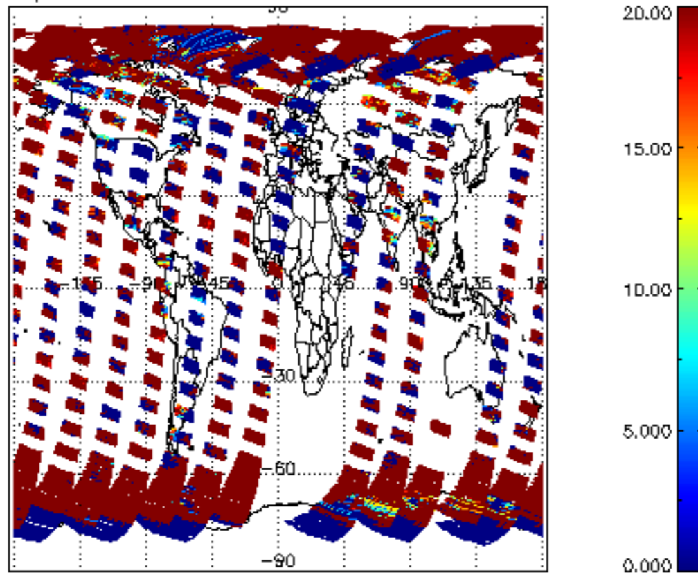
cl_opt_depth for 03SEP2002 00:00:00 to 04SEP2002 00:00:00
