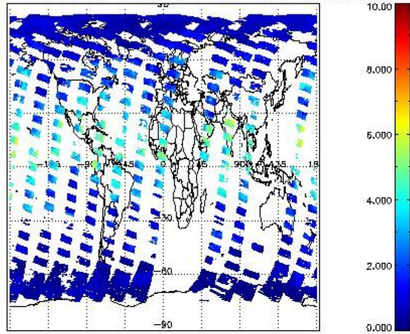
SCIOL2P_NADUV8H2O_vcd for 03SEP2002 00:00:00 to 04SEP2002 00:00:00
