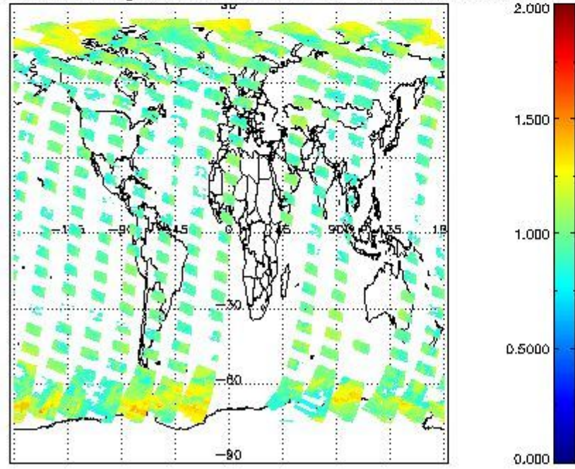
SCIOL2P_NADUV8H2O_arnf_gr for 03SEP2002 00:00:00 to 04SEP2002 00:00:00
