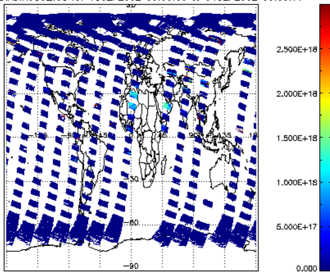
SCIOL2P_NADIR3CO_vcd for 03SEP2002 00:00:00 to 04SEP2002 00:00:00
