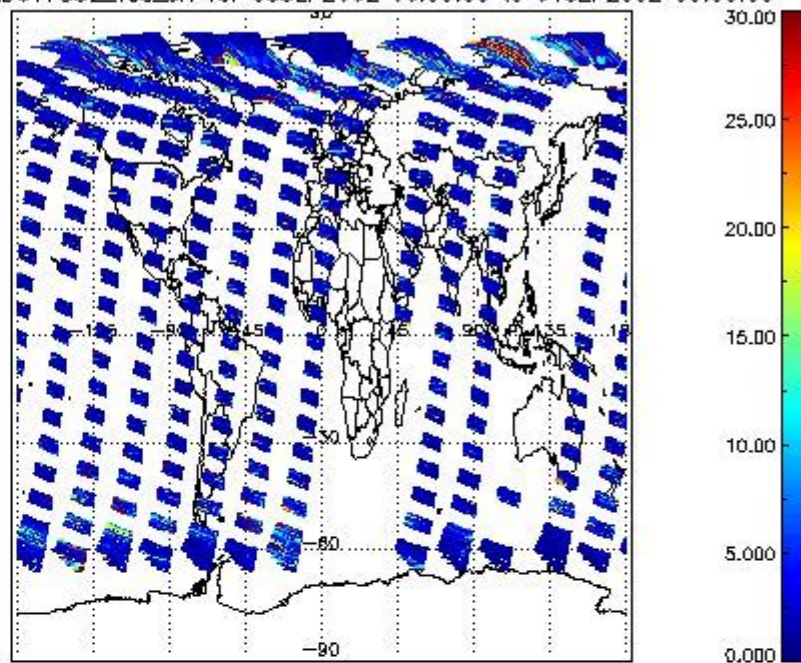
SCIOL2P_NADUV7S02_vcd_err for 03SEP2002 00:00:00 to 04SEP2002 00:00:00
