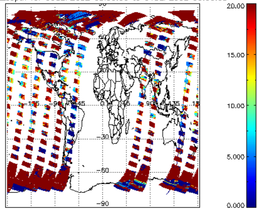
cl_opt_depth for 03SEP2002 00:00:00 to 04SEP2002 00:00:00
