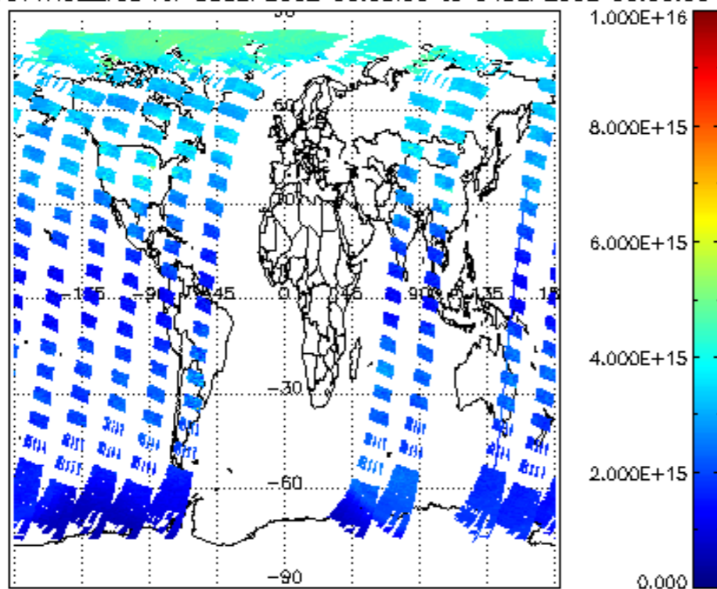
SCIOL2P_NADUV1NO2_vcd for 03SEP2002 00:00:00 to 04SEP2002 00:00:00
