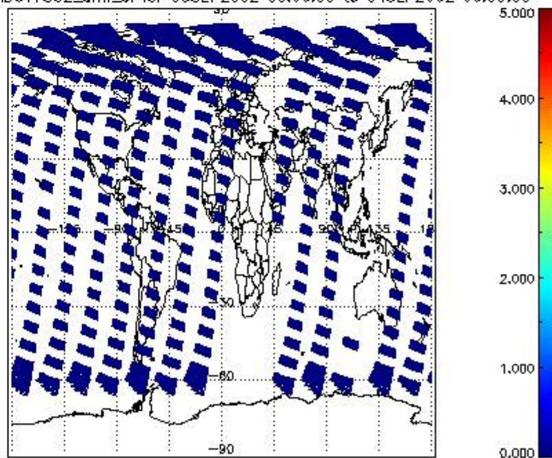
SCIOL2P_NADUV7S02_amf_cl for 03SEP2002 00:00:00 to 04SEP2002 00:00:00
