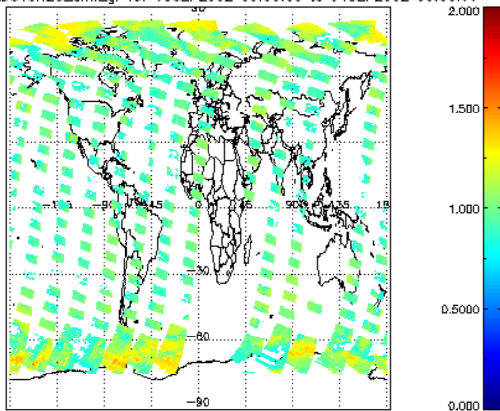
SCIOL2P_NADUV8H2O_amf_gr for 03SEP2002 00:00:00 to 04SEP2002 00:00:00
