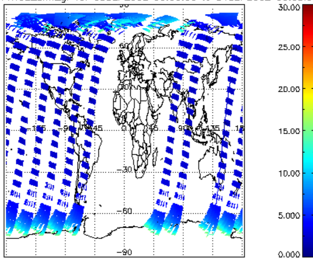
iCIOL2P_NADUV1NO2_amf_gr for 03SEP2002 00:00:00 to 04SEP2002 00:00:00
