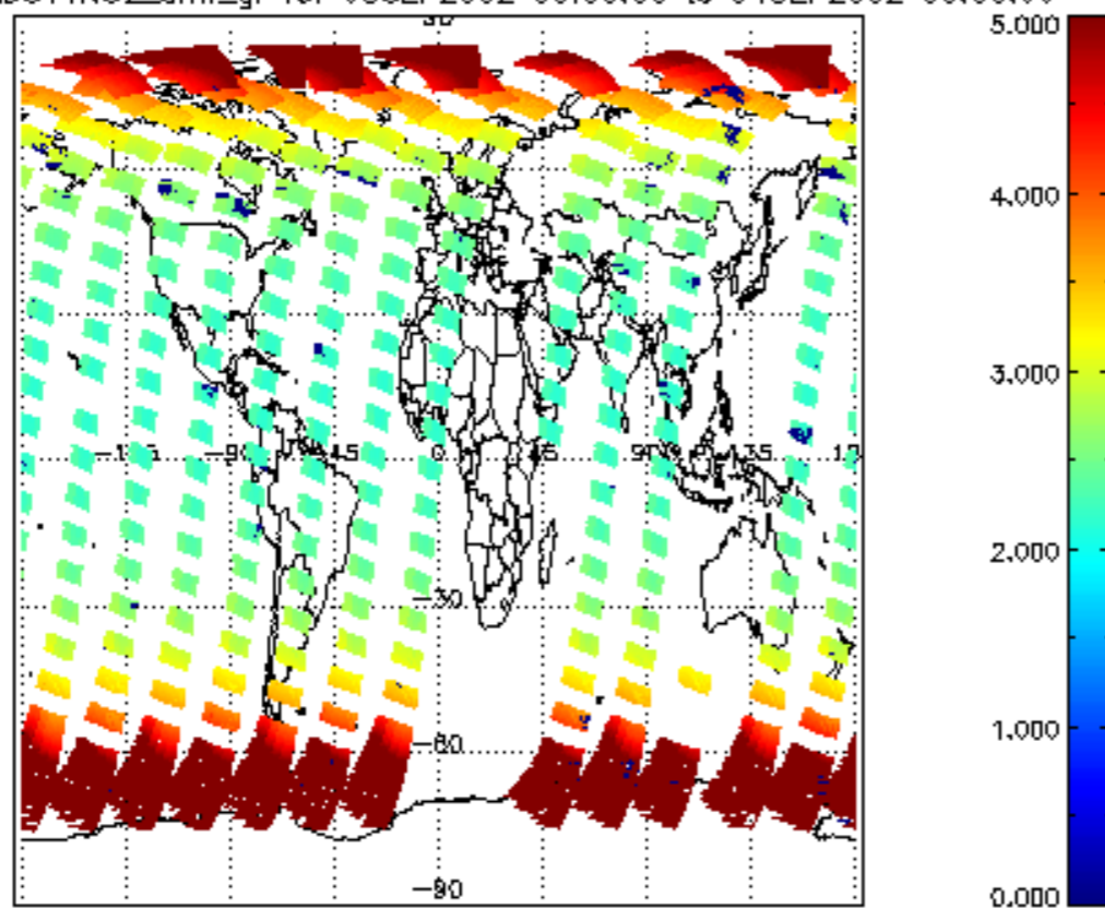
SCIOL2P_NADUV1NO2_amf_gr for 03SEP2002 00:00:00 to 04SEP2002 00:00:00
