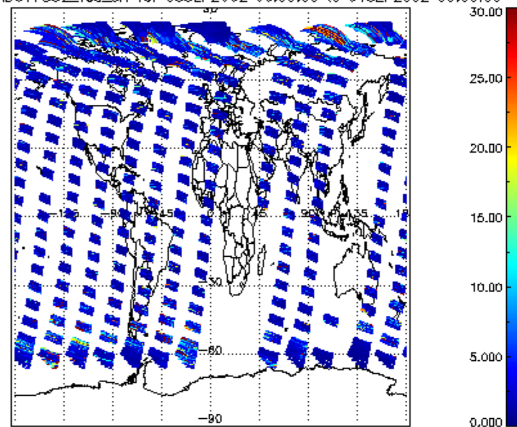
SCIOL2P_NADUV7S02_vcd_err for 03SEP2002 00:00:00 to 04SEP2002 00:00:00
