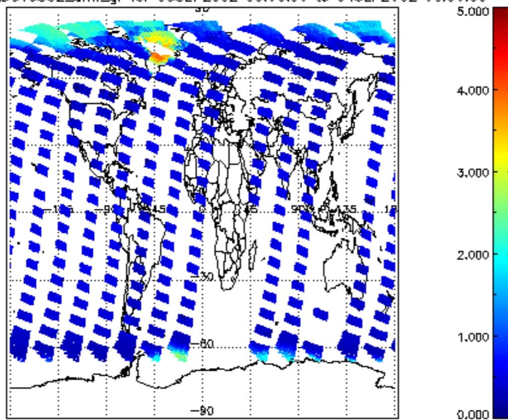
SCIOL2P_NADUV5S02_amf_gr for 03SEP2002 00:00:00 to 04SEP2002 00:00:00
