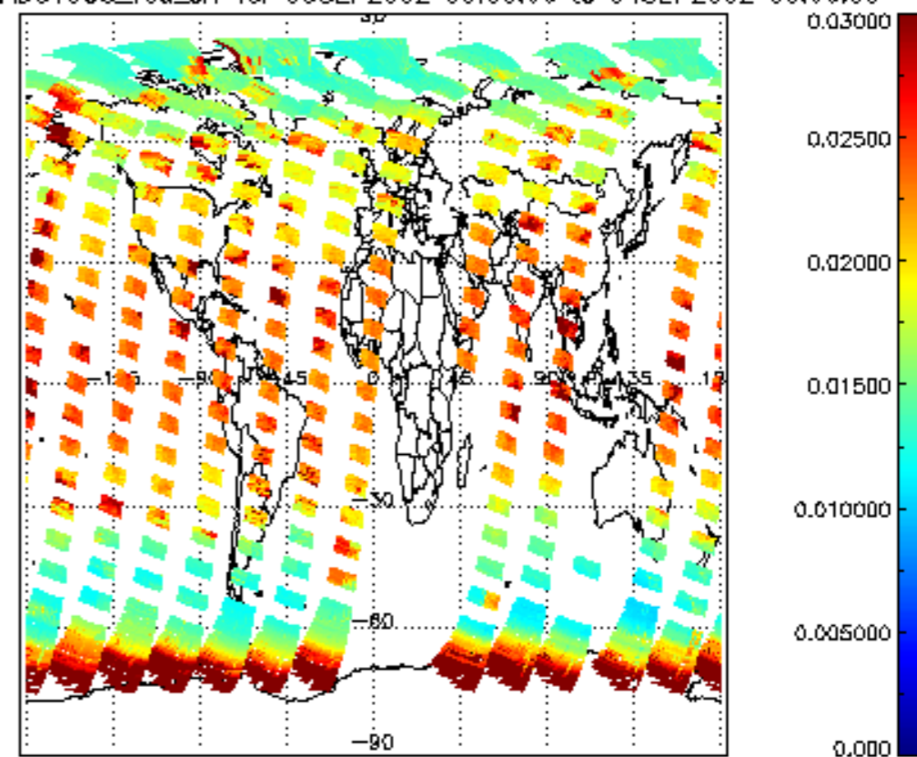
SCIOL2P_NADUV003_vcd_err for 03SEP2002 00:00:00 to 04SEP2002 00:00:00
