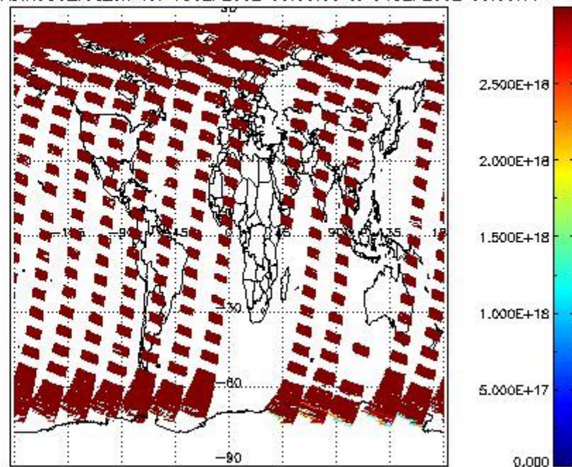
SCIDL2P_NADIR3CO_vcd_err for 03SEP2002 00:00:00 to 04SEP2002 00:00:00
