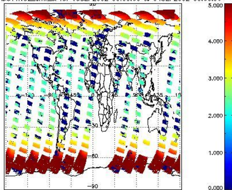
SCIOL2P_NADUV1N02_amf_cl for 03SEP2002 00:00:00 to 04SEP2002 00:00:00
