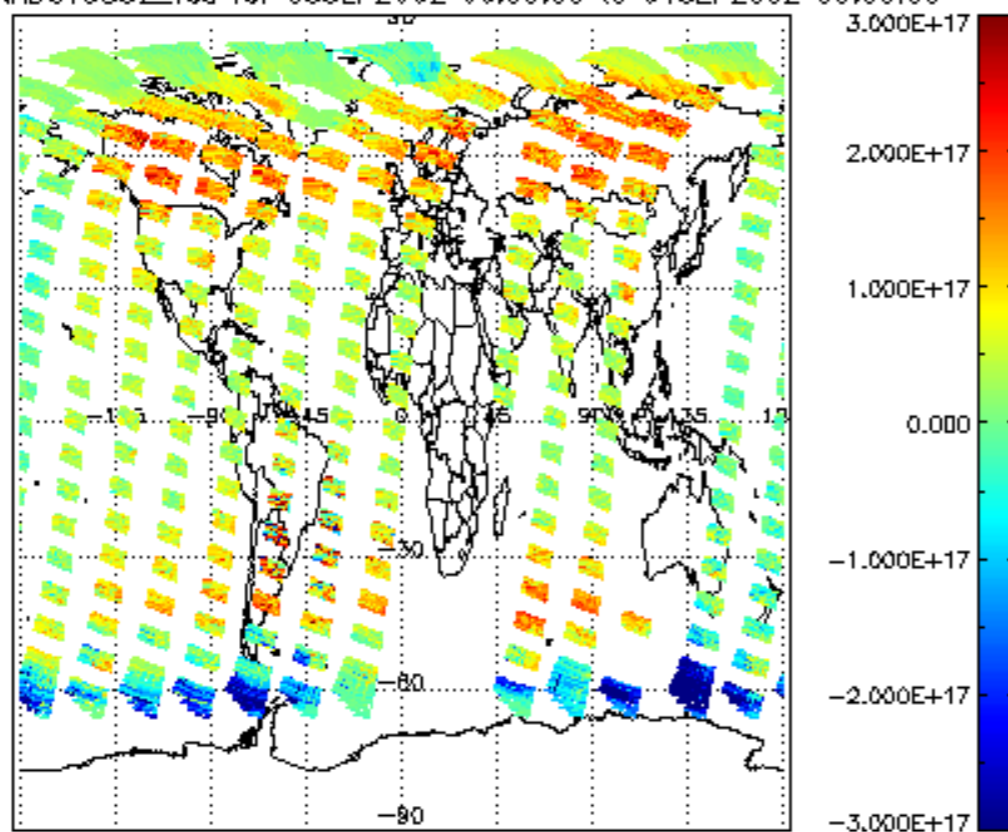
SCIOL2P_NADUV5S02_vcd for 03SEP2002 00:00:00 to 04SEP2002 00:00:00
