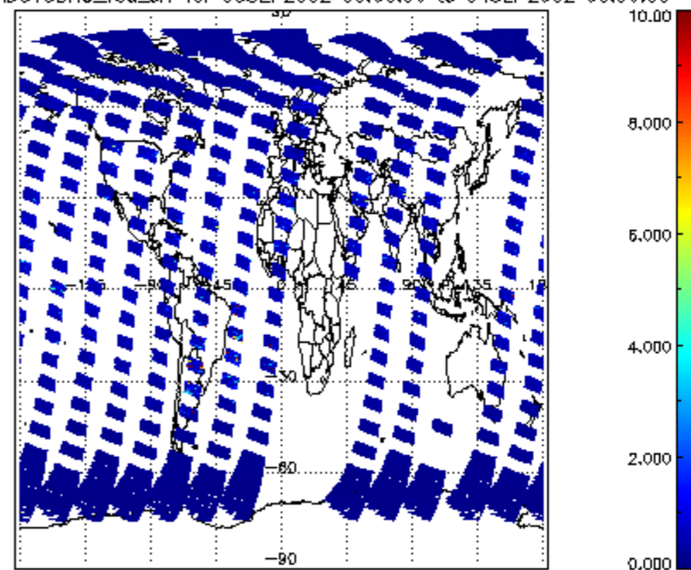
SCIOL2P_NADUV3BRO_vcd_err for 03SEP2002 00:00:00 to 04SEP2002 00:00:00
