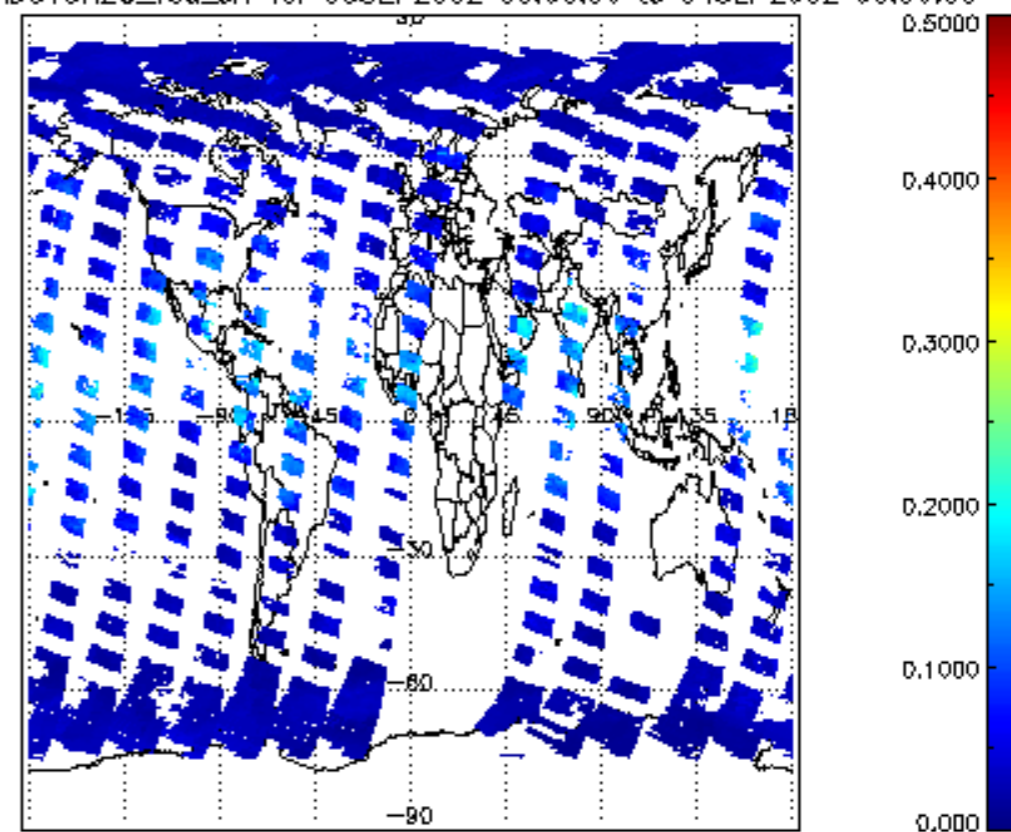
SCIOL2P_NADUV8H2O_vcd_err for 03SEP2002 00:00:00 to 04SEP2002 00:00:00
