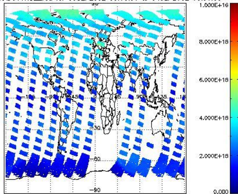
SCIOL2P_NADUV1N02_vcd for 03SEP2002 00:00:00 to 04SEP2002 00:00:00
