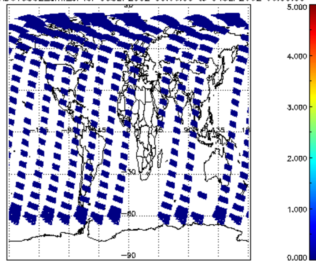
SCIOL2P_NADUV5S02_amf_cl for 03SEP2002 00:00:00 to 04SEP2002 00:00:00
