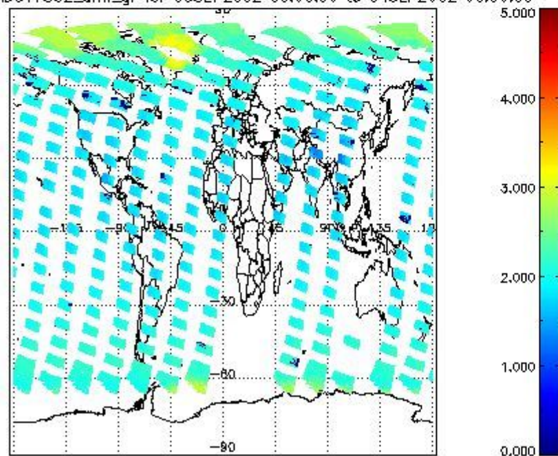
SCIOL2P_NADUV7S02_amf_gr for 03SEP2002 00:00:00 to 04SEP2002 00:00:00
