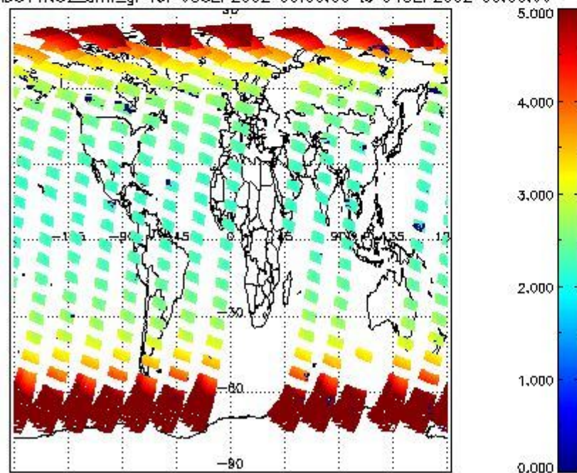
SCIOL2P_NADUV1N02_amf_gr for 03SEP2002 00:00:00 to 04SEP2002 00:00:00
