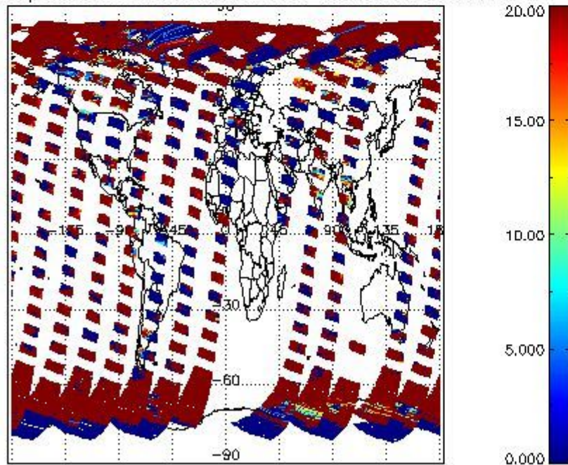
cL_opt_depth for 03SEP2002 00:00:00 to 04SEP2002 00:00:00
