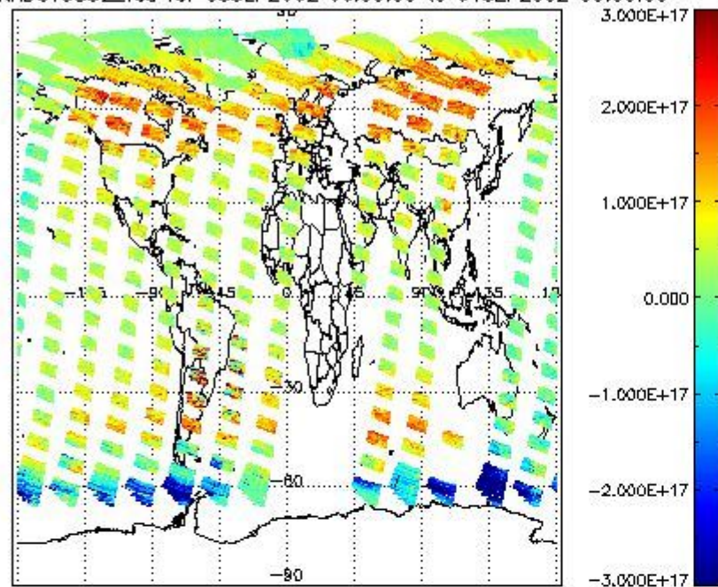
SCIOL2P_NADUV5S02_vcd for 03SEP2002 00:00:00 to 04SEP2002 00:00:00
