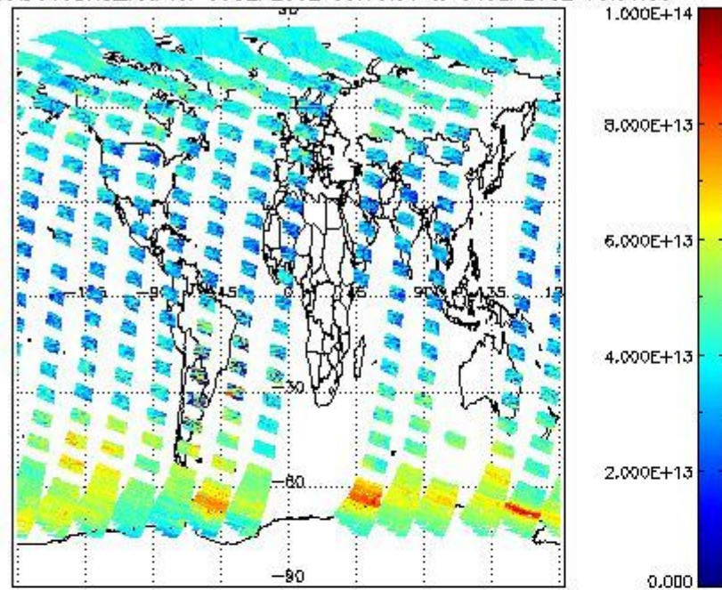
SCIOL2P_NADUV3BRO_vcd for 03SEP2002 00:00:00 to 04SEP2002 00:00:00
