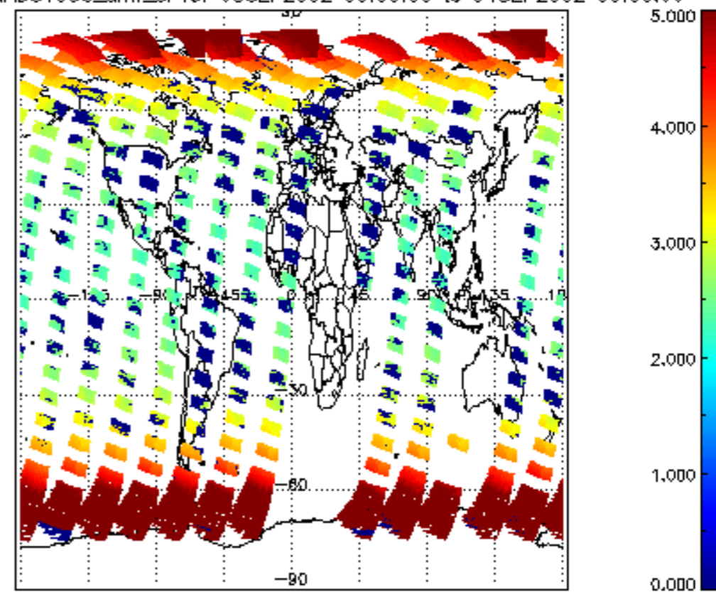
SCIOL2P_NADUV003_amf_cl for 03SEP2002 00:00:00 to 04SEP2002 00:00:00
