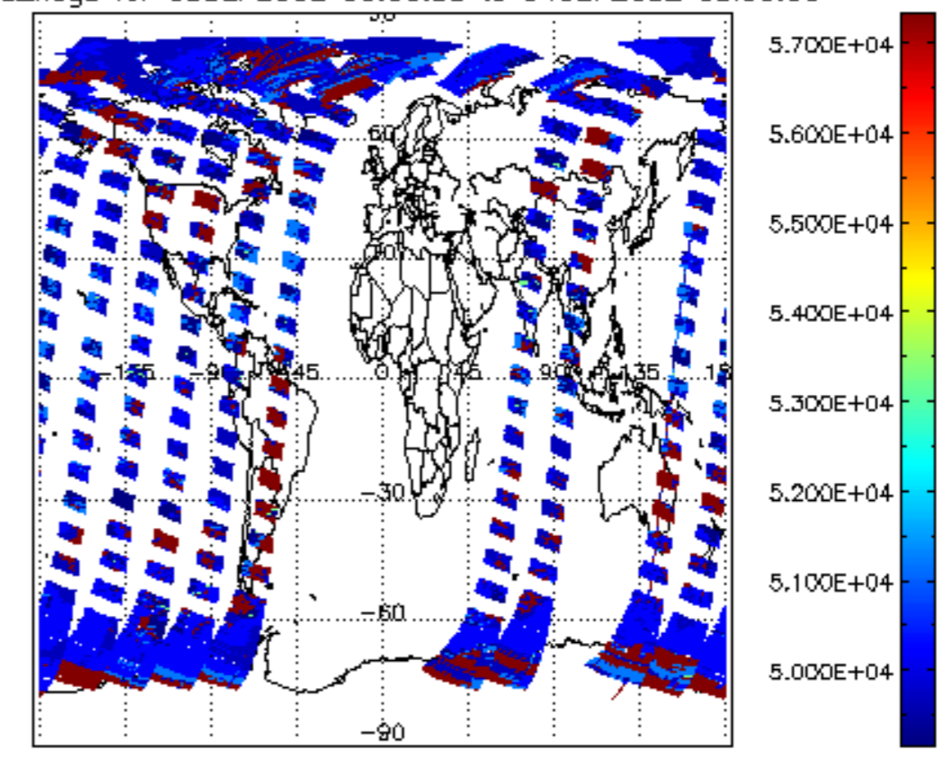
cloud_flags for 03SEP2002 00:00:00 to 04SEP2002 00:00:00
