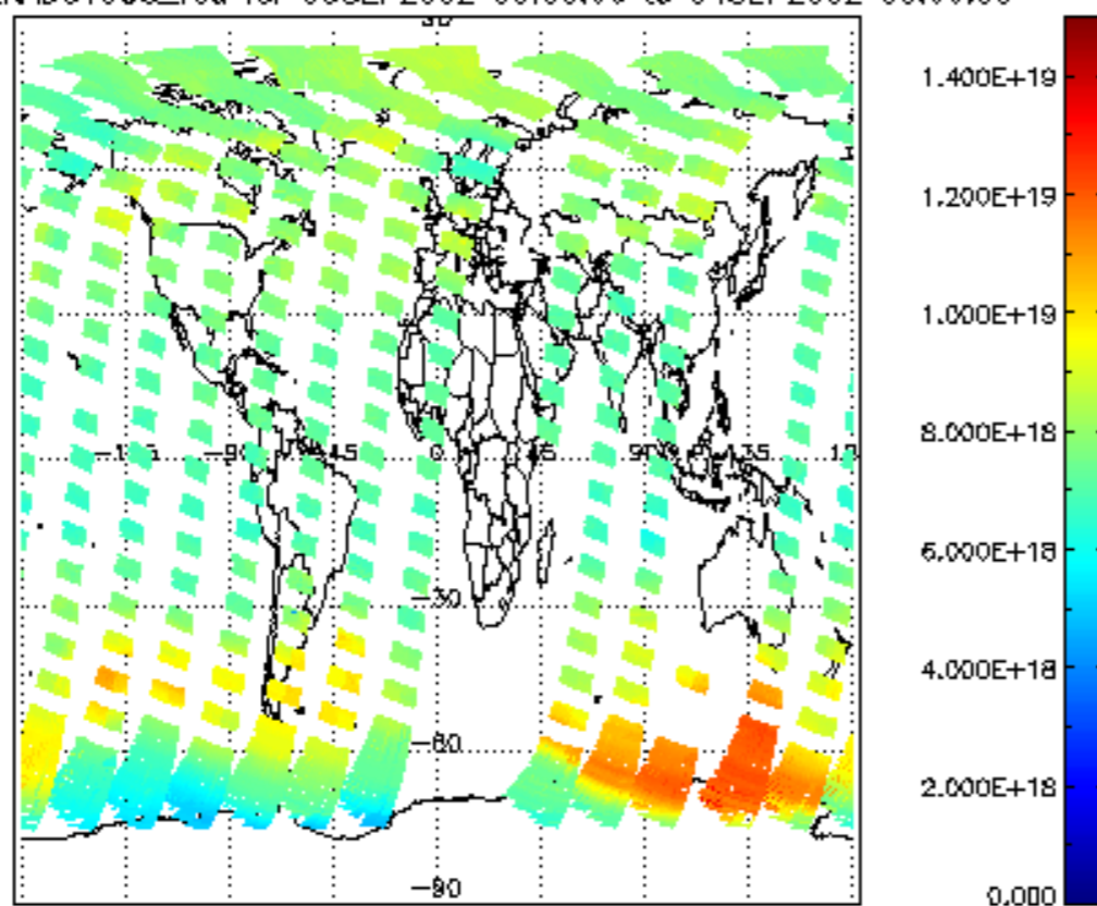
SCIOL2P_NADUV003_vcd for 03SEP2002 00:00:00 to 04SEP2002 00:00:00
