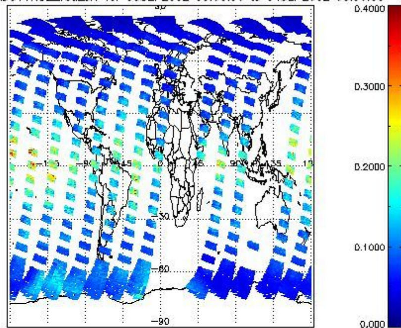
SCIOL2P_NADUV1N02_vcd_err for 03SEP2002 00:00:00 to 04SEP2002 00:00:00
