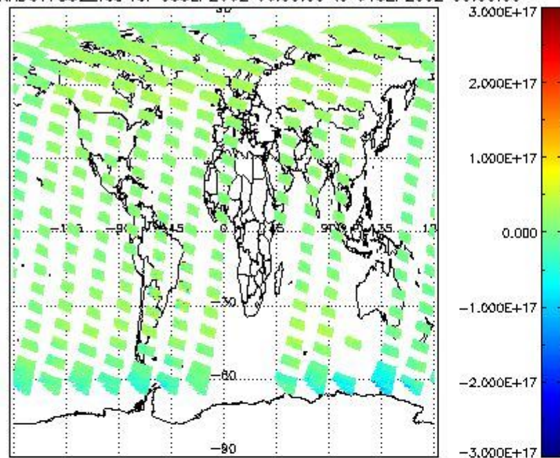
SCIOL2P_NADUV7S02_vcd for 03SEP2002 00:00:00 to 04SEP2002 00:00:00
