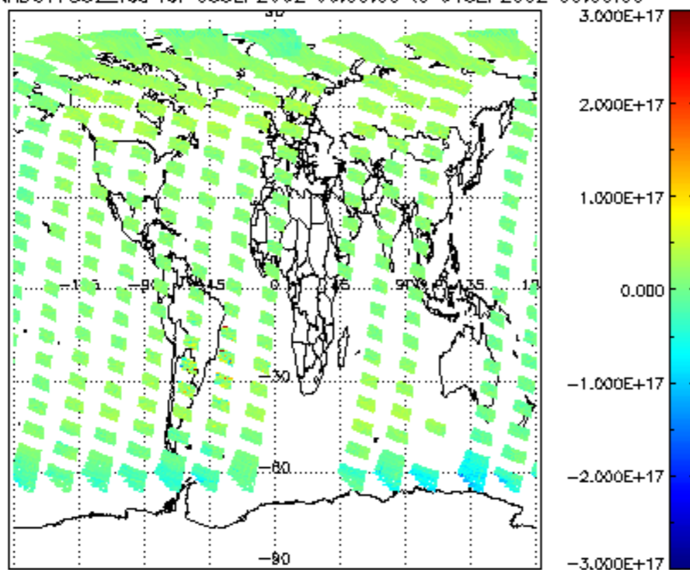
SCIOL2P_NADUV7S02_vcd for 03SEP2002 00:00:00 to 04SEP2002 00:00:00
