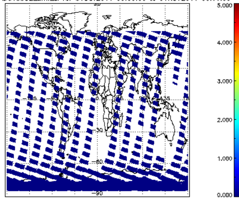
SCIOL2P_NADUV5S02_amf_cl for 31OCT2011 00:00:00 to 01NOV2011 00:00:00
