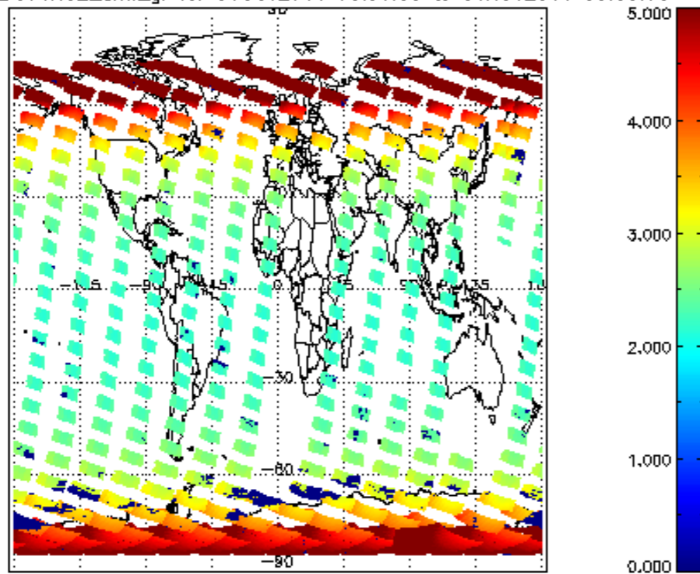
SCIOL2P_NADUV1NO2_amf_gr for 31OCT2011 00:00:00 to 01NOV2011 00:00:00
