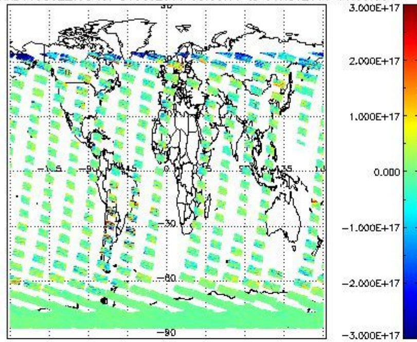
SCIOL2P_NADUV5S02_vcd for 31OCT2011 00:00:00 to 01NOV2011 00:00:00
