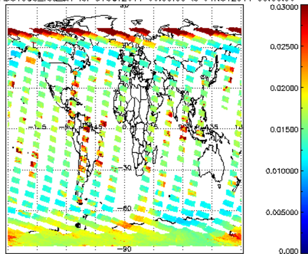
SCIOL2P_NADUV003_vcd_Lerr for 31OCT2011 00:00:00 to 01NOV2011 00:00:00
