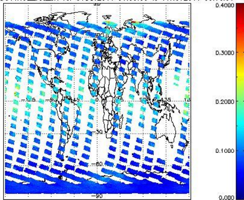
SCIOL2P_NADUV1N02_vcd_err for 31OCT2011 00:00:00 to 01NOV2011 00:00:00
