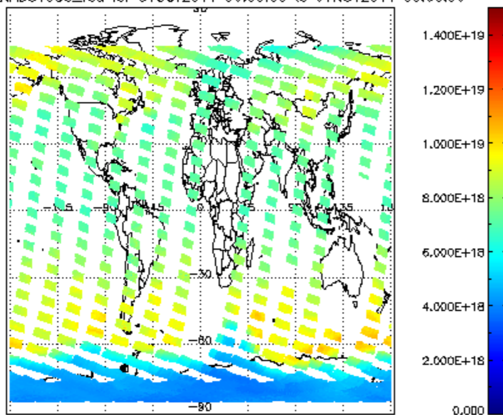
SCIOL2P_NADUV003_vcd for 31OCT2011 00:00:00 to 01NOV2011 00:00:00
