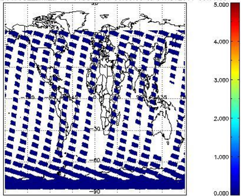
SCIOL2P_NADUV7S02_amf_cl for 31OCT2011 00:00:00 to 01NOV2011 00:00:00
