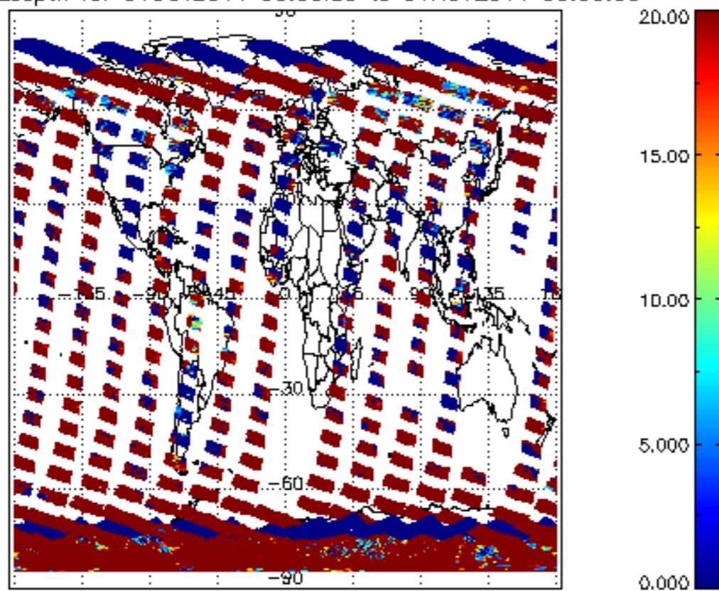
cL_opt_depth for 31OCT2011 00:00:00 to 01NOV2011 00:00:00
