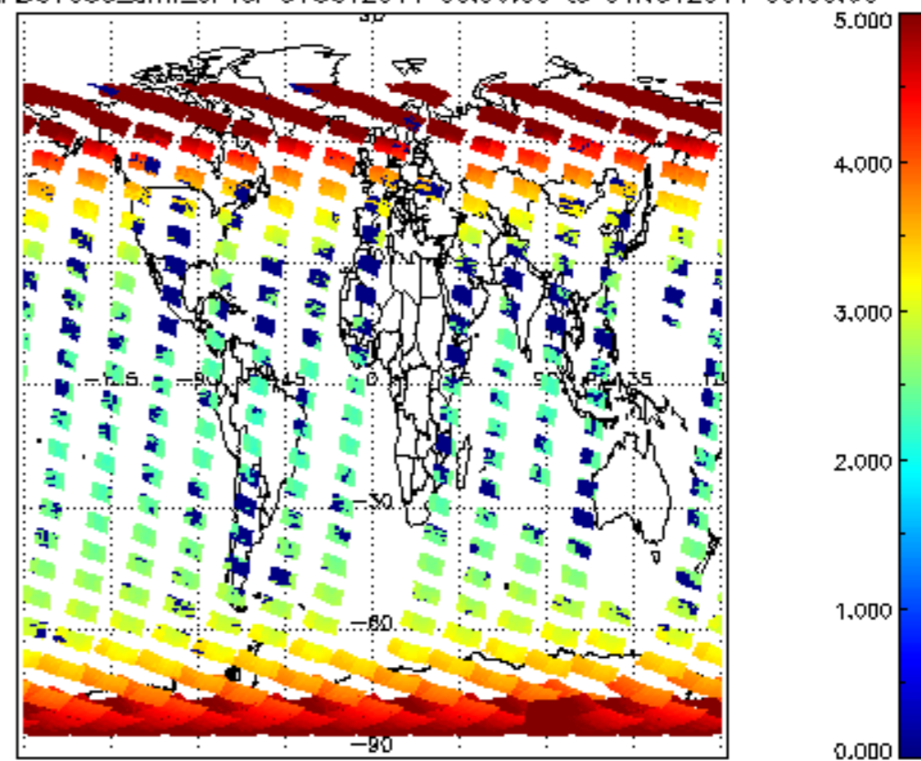
SCIOL2P_NADUV003_amf_cl for 31OCT2011 00:00:00 to 01NOV2011 00:00:00
