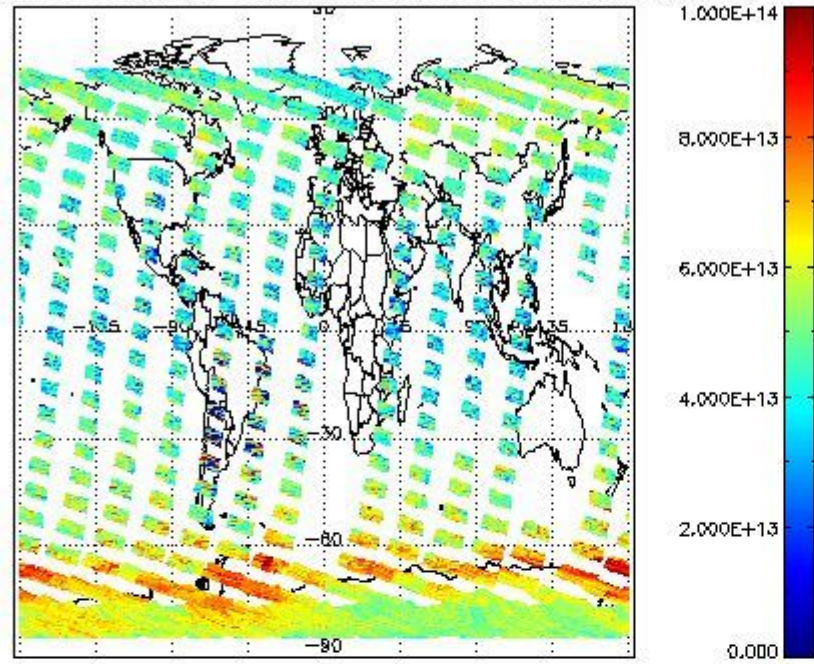
SCIOL2P_NADUV3BRO_vcd for 31OCT2011 00:00:00 to 01NOV2011 00:00:00
