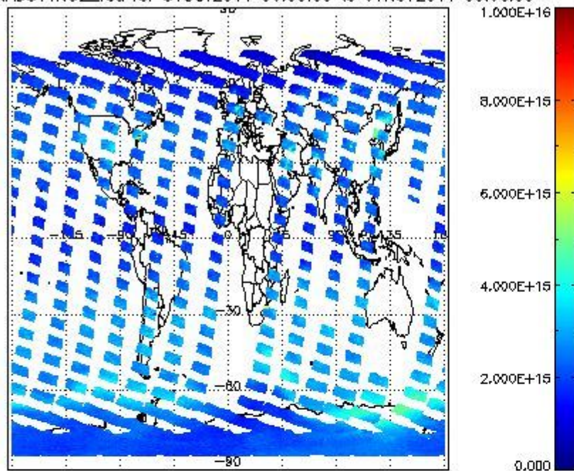
SCIOL2P_NADUV1N02_vcd for 31OCT2011 00:00:00 to 01NOV2011 00:00:00
