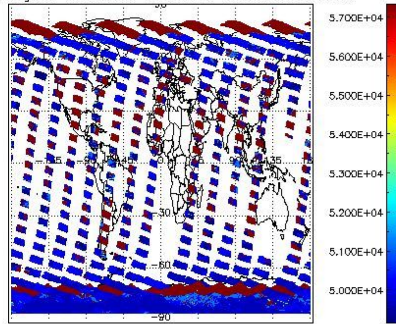
cloud_flags for 31OCT2011 00:00:00 to 01NOV2011 00:00:00
