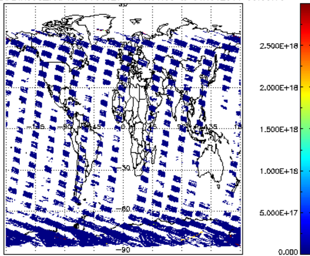
SCIOL2P_NADIR3CO_vcd for 31OCT2011 00:00:00 to 01NOV2011 00:00:00
