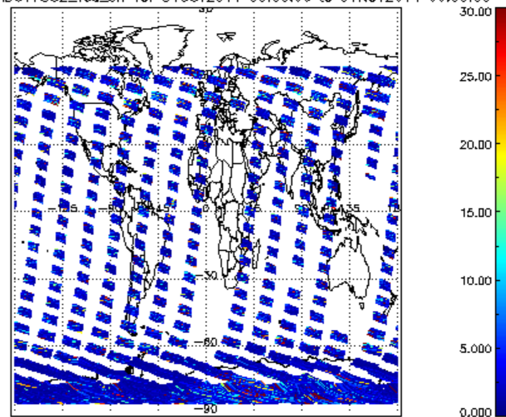
SCIOL2P_NADUV7S02_vcd_err for 31OCT2011 00:00:00 to 01NOV2011 00:00:00
