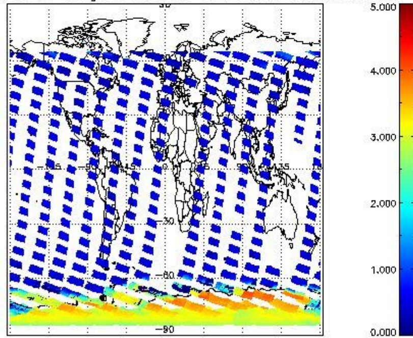
SCIOL2P_NADUV5S02_amf_gr for 31OCT2011 00:00:00 to 01NOV2011 00:00:00
