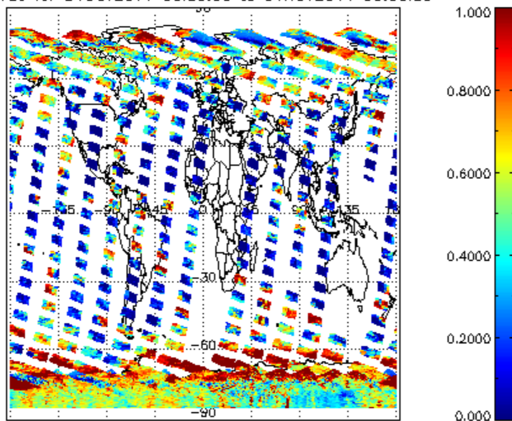
cL_frac for 31OCT2011 00:00:00 to 01NOV2011 00:00:00
