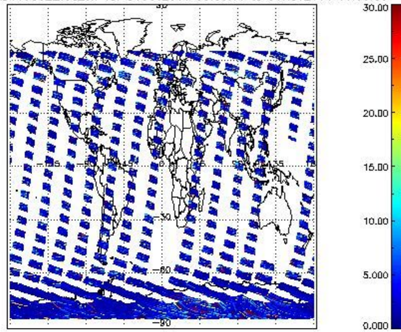
SCIOL2P_NADUV5S02_vcd_err for 31OCT2011 00:00:00 to 01NOV2011 00:00:00
