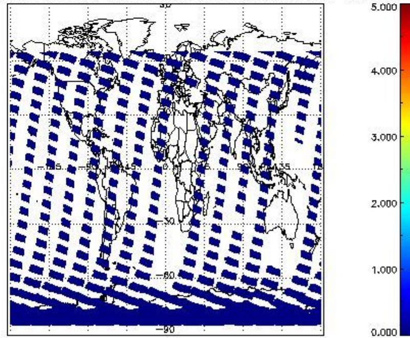
SCIOL2P_NADUV5S02_amf_cl for 31OCT2011 00:00:00 to 01NOV2011 00:00:00
