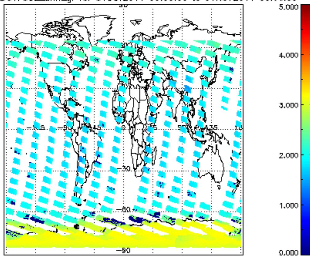
SCIOL2P_NADUV7S02_amf_gr for 31OCT2011 00:00:00 to 01NOV2011 00:00:00
