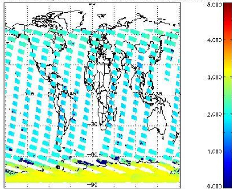
SCIOL2P_NADUV7S02_amf_gr for 31OCT2011 00:00:00 to 01NOV2011 00:00:00
