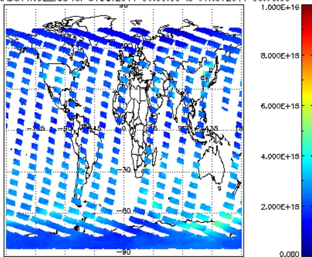
SCIOL2P_NADUV1NO2_vcd for 31OCT2011 00:00:00 to 01NOV2011 00:00:00
