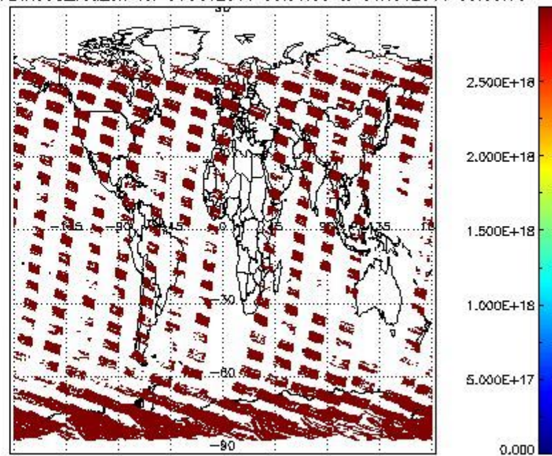
SCIDL2P_NADIR3CO_vcd_err for 31OCT2011 00:00:00 to 01NOV2011 00:00:00
