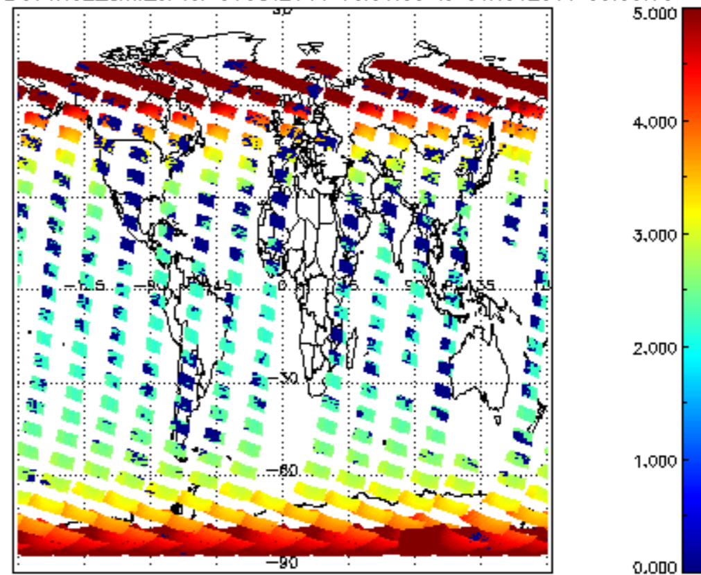
SCIOL2P_NADUV1NO2_amf_cl for 31OCT2011 00:00:00 to 01NOV2011 00:00:00
