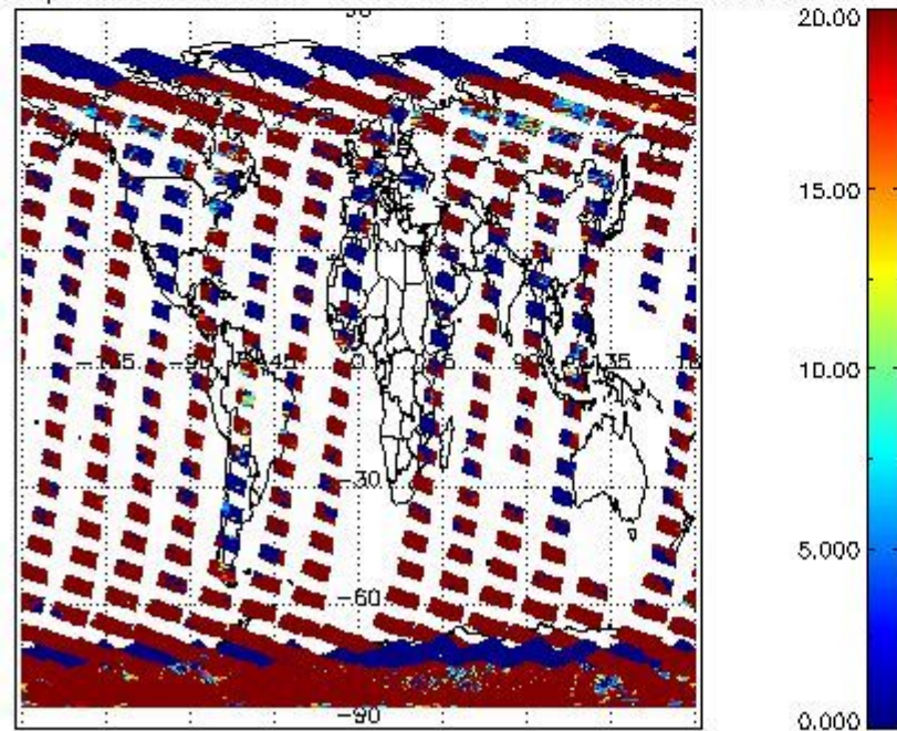
cL_opt_depth for 31OCT2011 00:00:00 to 01NOV2011 00:00:00
