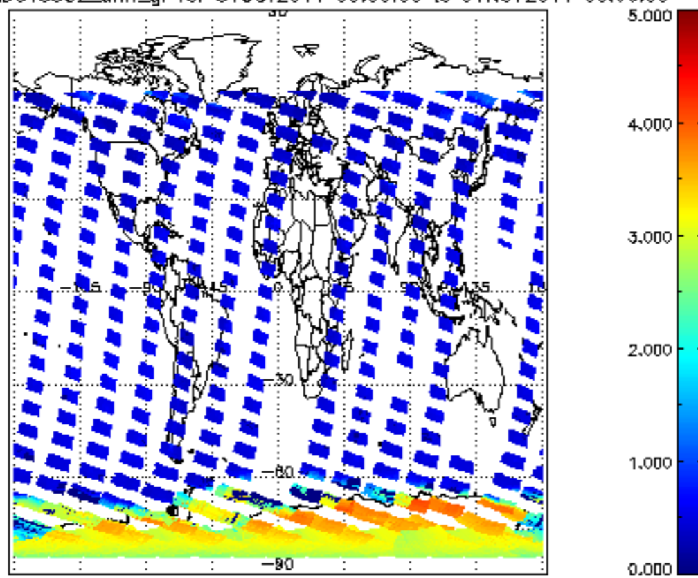
SCIOL2P_NADUV5S02_amf_gr for 31OCT2011 00:00:00 to 01NOV2011 00:00:00
