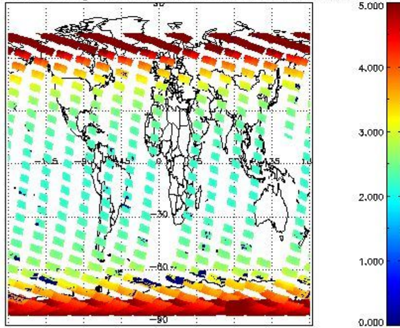
SCIOL2P_NADUV003_amf_gr for 31OCT2011 00:00:00 to 01NOV2011 00:00:00
