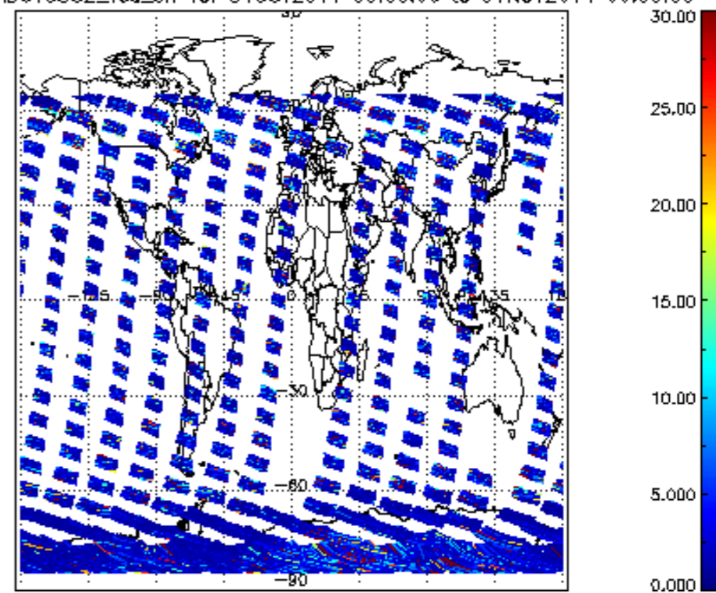
SCIOL2P_NADUV5S02_vcd_err for 31OCT2011 00:00:00 to 01NOV2011 00:00:00
