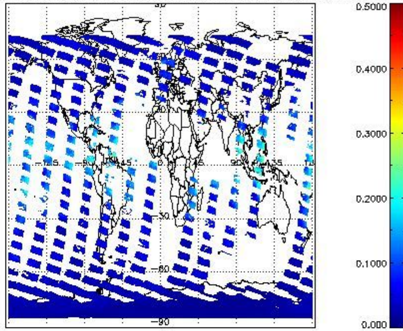
SCIOL2P_NADUV8H2O_vcd_err for 31OCT2011 00:00:00 to 01NOV2011 00:00:00
