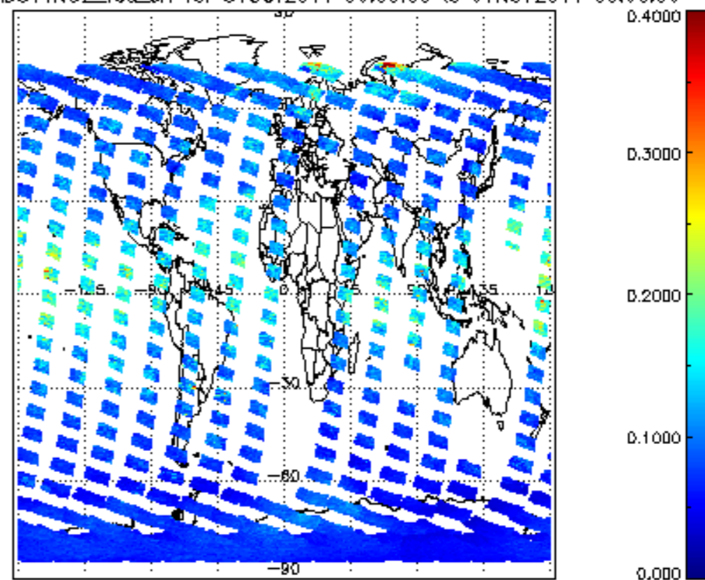
SCIOL2P_NADUV1NO2_vcd_err for 31OCT2011 00:00:00 to 01NOV2011 00:00:00
