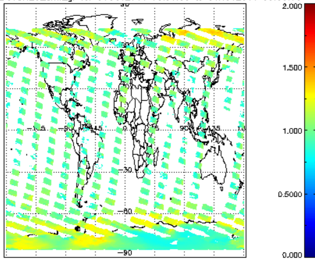
SCIOL2P_NADUV8H20_amf_gr for 31OCT2011 00:00:00 to 01NOV2011 00:00:00
