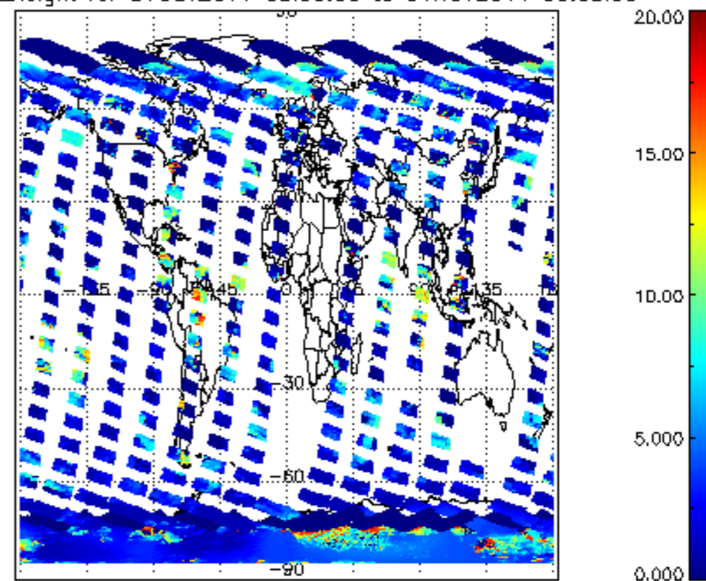
cL_top_height for 31OCT2011 00:00:00 to 01NOV2011 00:00:00
