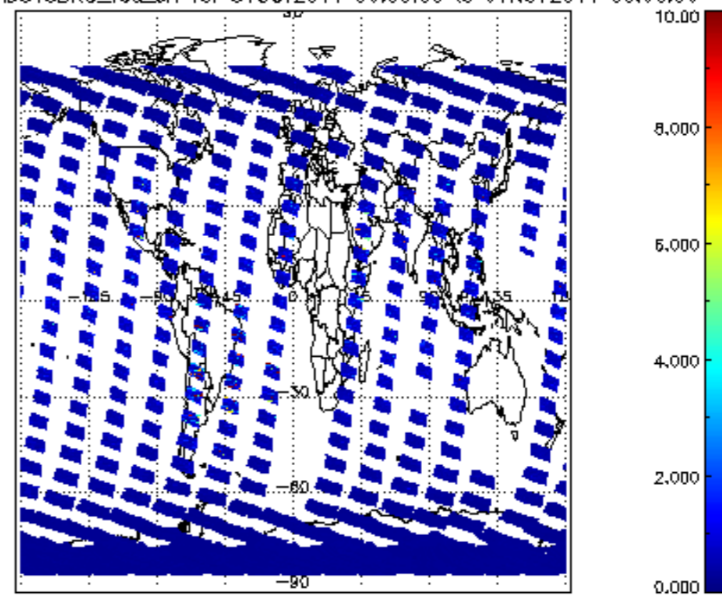
SCIOL2P_NADUV3BRO_vcd_err for 31OCT2011 00:00:00 to 01NOV2011 00:00:00
