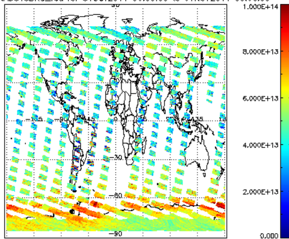
SCIOL2P_NADUV3BRO_vcd for 31OCT2011 00:00:00 to 01NOV2011 00:00:00
