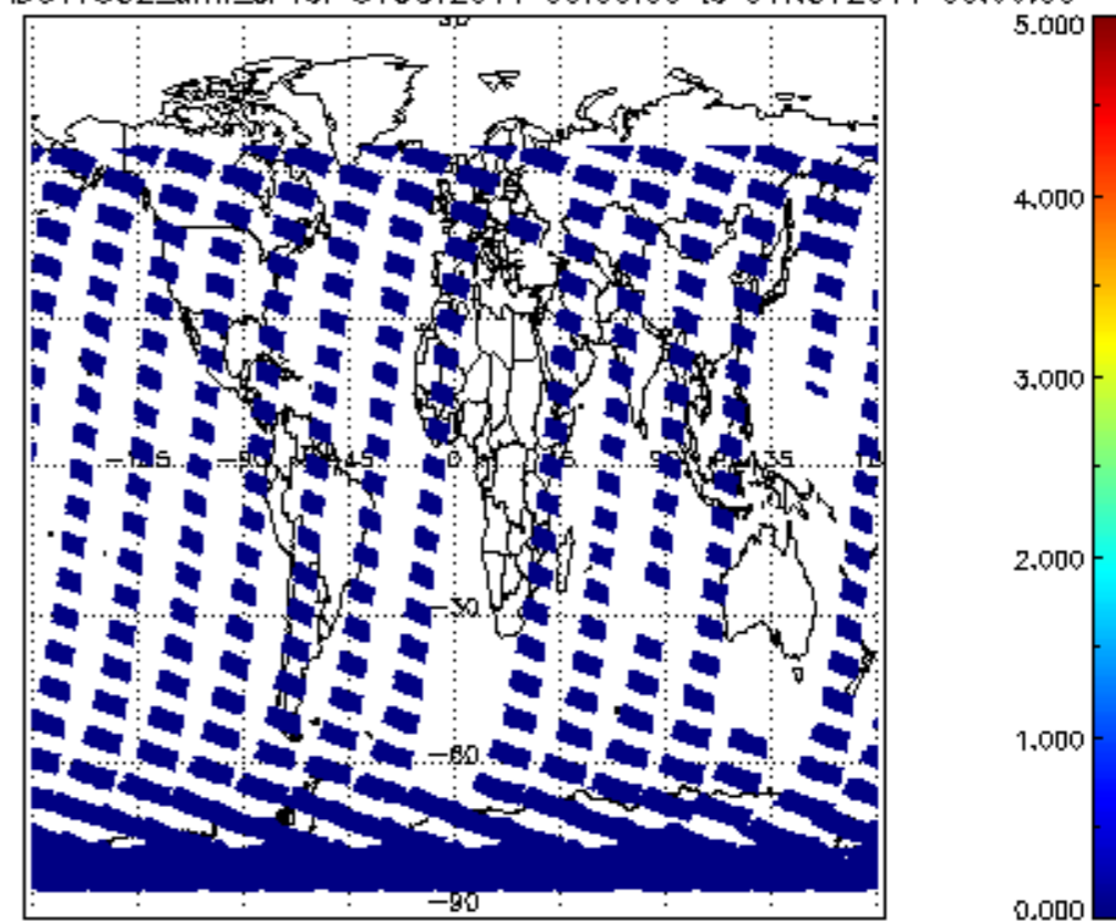
SCIOL2P_NADUV7S02_amf_cl for 31OCT2011 00:00:00 to 01NOV2011 00:00:00
