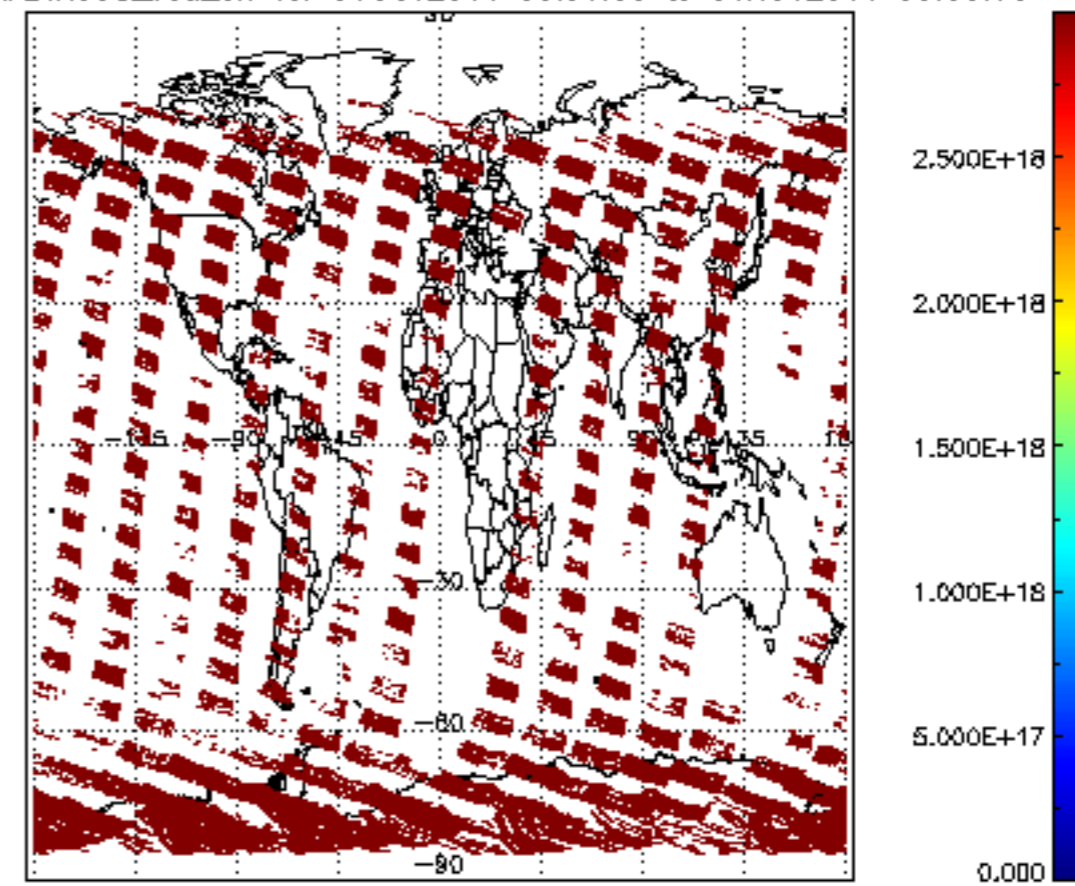
SCIOL2P_NADIR3CO_vcd_err for 31OCT2011 00:00:00 to 01NOV2011 00:00:00
