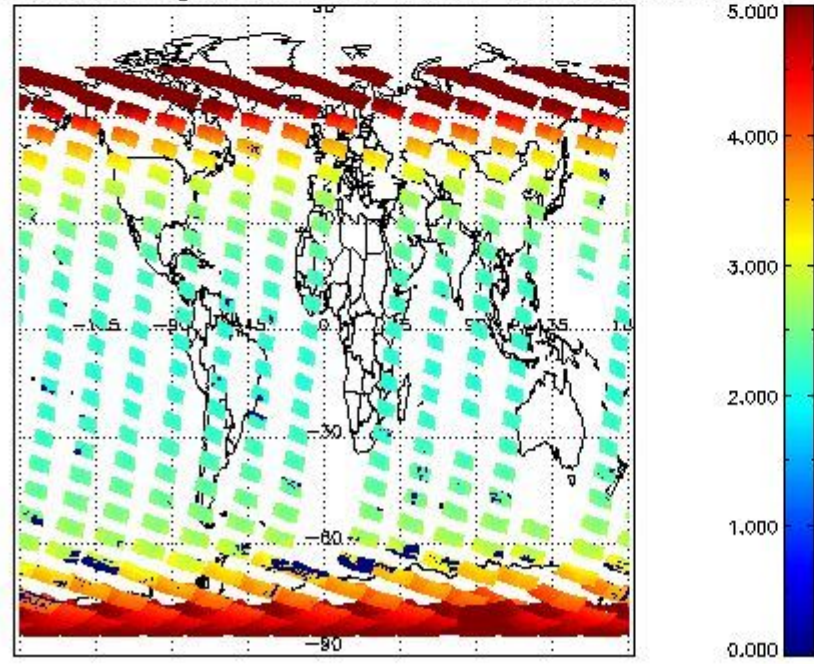
SCIOL2P_NADUV3BRO_amf_gr for 31OCT2011 00:00:00 to 01NOV2011 00:00:00
