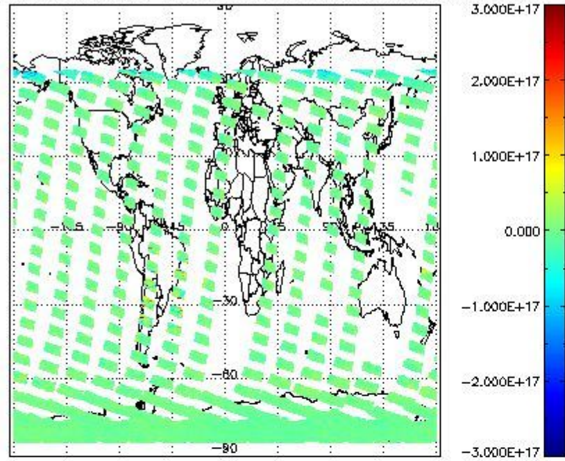
SCIOL2P_NADUV7S02_vcd for 31OCT2011 00:00:00 to 01NOV2011 00:00:00
