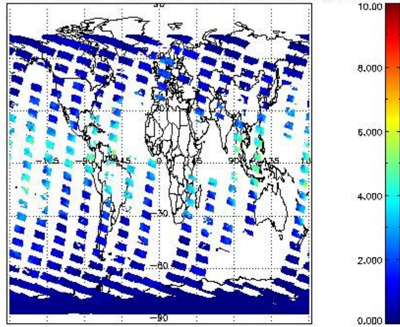
SCIOL2P_NADUV8H2O_vcd for 31OCT2011 00:00:00 to 01NOV2011 00:00:00
