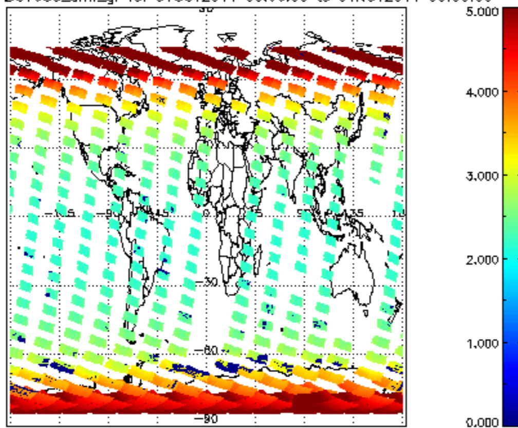
SCIOL2P_NADUV003_amf_gr for 31OCT2011 00:00:00 to 01NOV2011 00:00:00
