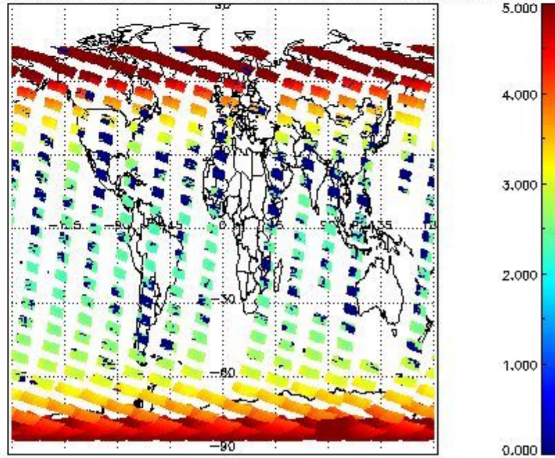
SCIOL2P_NADUV003_amf_cl for 31OCT2011 00:00:00 to 01NOV2011 00:00:00
