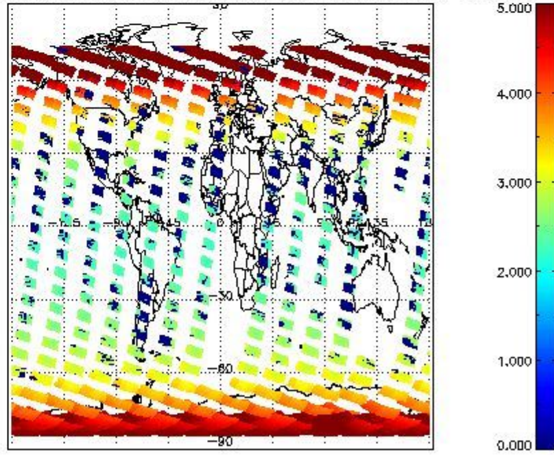
SCIOL2P_NADUV3BRO_amf_cl for 31OCT2011 00:00:00 to 01NOV2011 00:00:00
