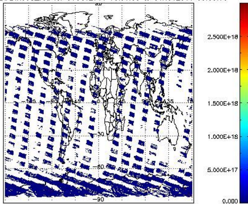
SCIDL2P_NADIR3CO_vcd for 31OCT2011 00:00:00 to 01NOV2011 00:00:00
