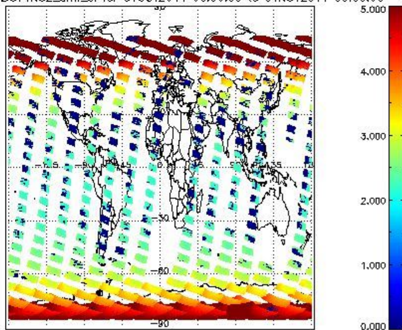
SCIOL2P_NADUV1N02_amf_cl for 31OCT2011 00:00:00 to 01NOV2011 00:00:00
