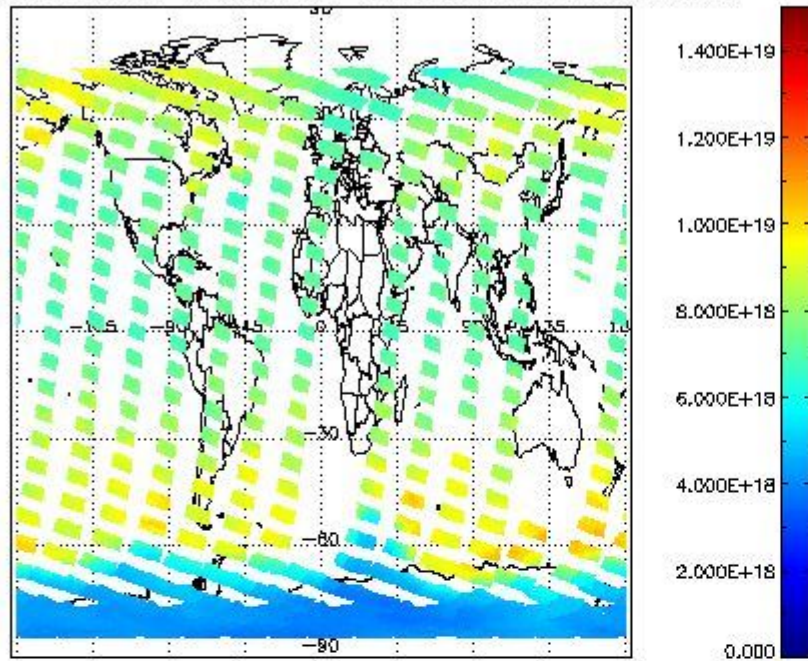
SCIOL2P_NADUV003_vcd for 31OCT2011 00:00:00 to 01NOV2011 00:00:00
