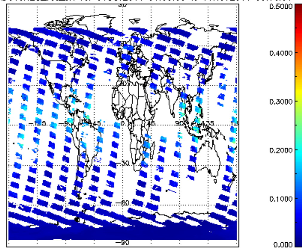
SCIOL2P_NADUV8H20_vcd_err for 31OCT2011 00:00:00 to 01NOV2011 00:00:00
