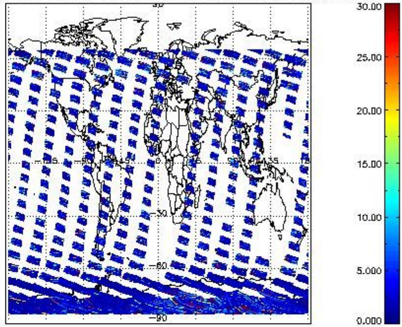
SCIOL2P_NADUV7S02_vcd_err for 31OCT2011 00:00:00 to 01NOV2011 00:00:00
