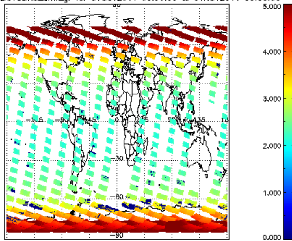
SCIOL2P_NADUV3BRO_amf_gr for 31OCT2011 00:00:00 to 01NOV2011 00:00:00
