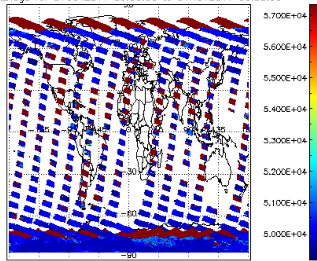
cloud_flags for 31OCT2011 00:00:00 to 01NOV2011 00:00:00
