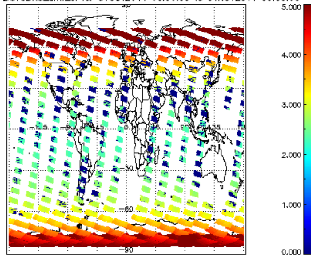
SCIOL2P_NADUV3BRO_amf_cl for 31OCT2011 00:00:00 to 01NOV2011 00:00:00
