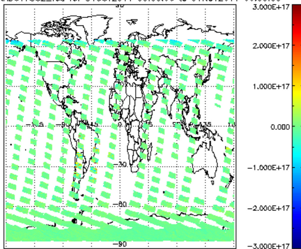
SCIOL2P_NADUV7S02_vcd for 31OCT2011 00:00:00 to 01NOV2011 00:00:00
