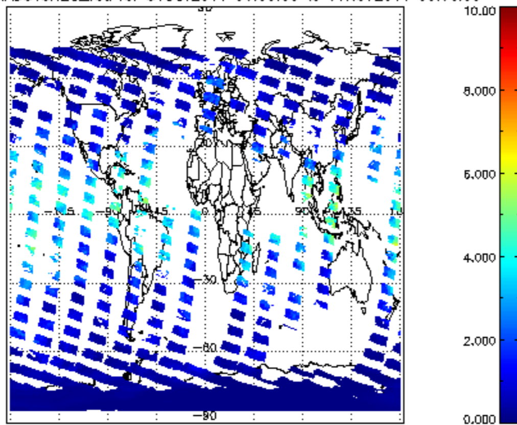
SCIOL2P_NADUV8H20_vcd for 31OCT2011 00:00:00 to 01NOV2011 00:00:00
