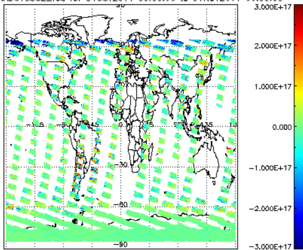
SCIOL2P_NADUV5S02_vcd for 31OCT2011 00:00:00 to 01NOV2011 00:00:00
