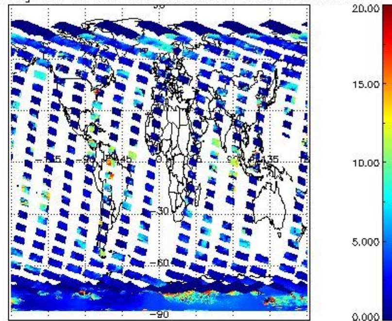
cL_top_height for 31OCT2011 00:00:00 to 01NOV2011 00:00:00
