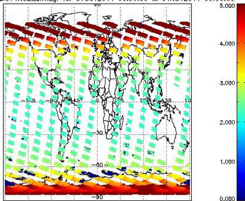
SCIOL2P_NADUV1N02_amf_gr for 31OCT2011 00:00:00 to 01NOV2011 00:00:00
