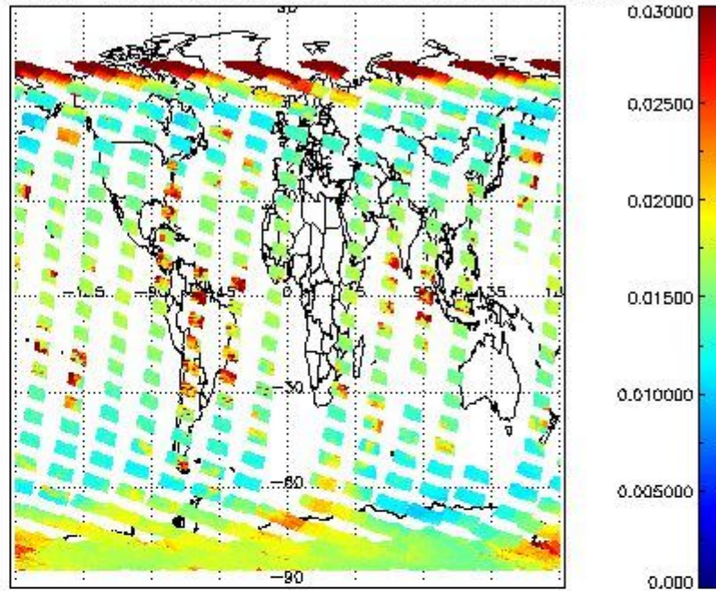
SCIOL2P_NADUV003_vcd_Lerr for 31OCT2011 00:00:00 to 01NOV2011 00:00:00
