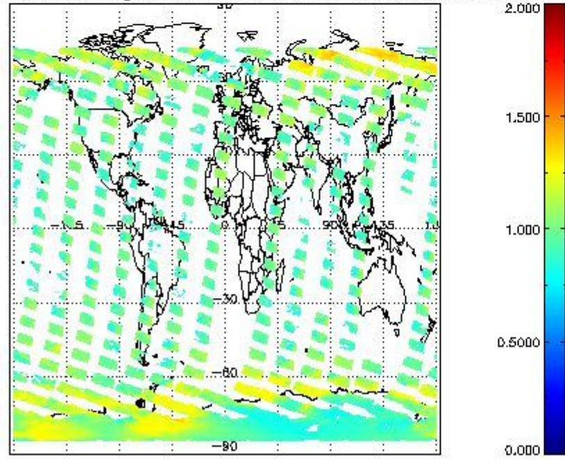
SCIOL2P_NADUV8H2O_amf_gr for 31OCT2011 00:00:00 to 01NOV2011 00:00:00
