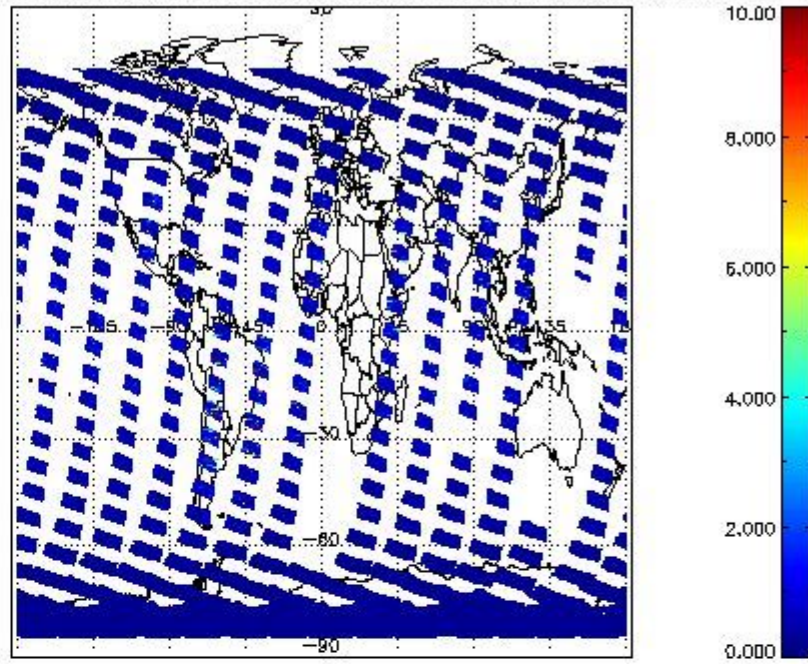
SCIOL2P_NADUV3BRO_vcd_err for 31OCT2011 00:00:00 to 01NOV2011 00:00:00
