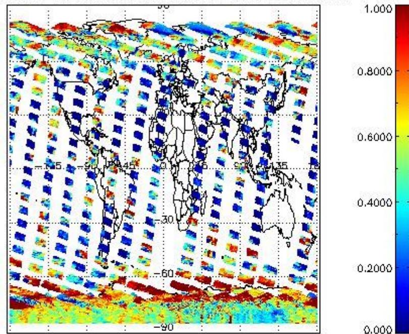
cL_frac for 31OCT2011 00:00:00 to 01NOV2011 00:00:00
