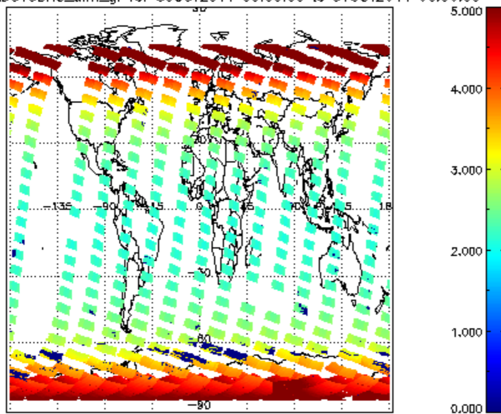
SCIOL2P_NADUV3BRO_amf_gr for 30OCT2011 00:00:00 to 31OCT2011 00:00:00
