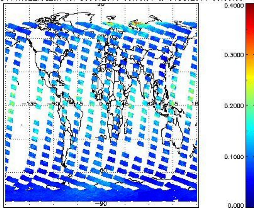
SCIOL2P_NADUV1NO2_vcd_err for 30OCT2011 00:00:00 to 31OCT2011 00:00:00
