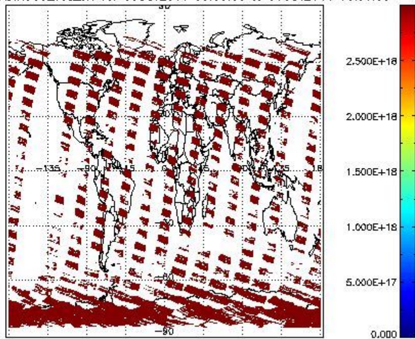
SCIDL2P_NADIR3CO_vcd_err for 30OCT2011 00:00:00 to 31OCT2011 00:00:00
