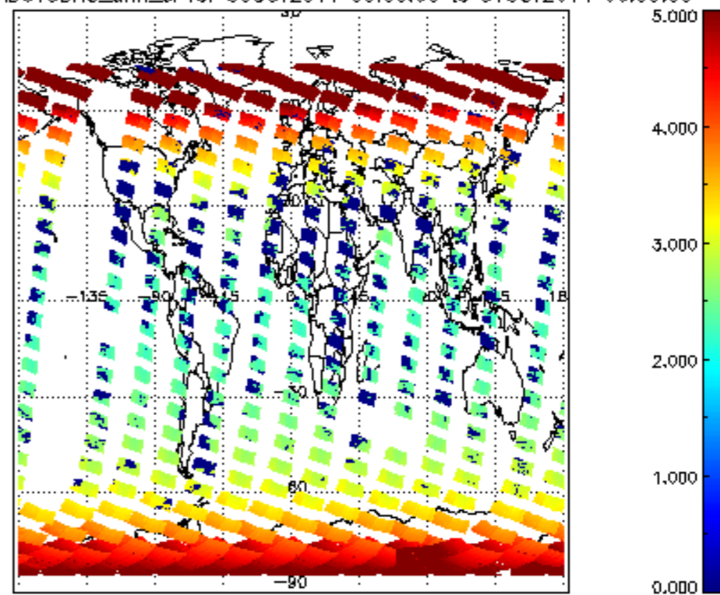
SCIOL2P_NADUV3BRO_amf_cl for 30OCT2011 00:00:00 to 31OCT2011 00:00:00
