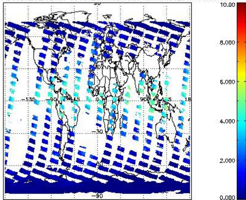
SCIOL2P_NADUV8H20_vcd for 30OCT2011 00:00:00 to 31OCT2011 00:00:00
