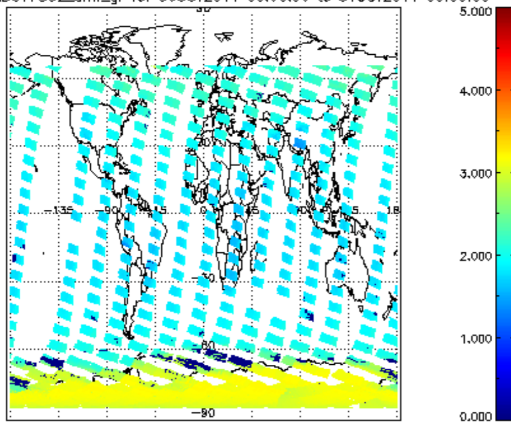
SCIOL2P_NADUV7S02_amf_gr for 30OCT2011 00:00:00 to 31OCT2011 00:00:00
