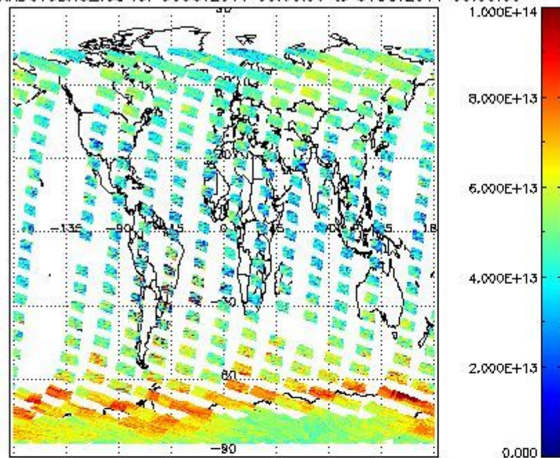
SCIOL2P_NADUV3BRO_vcd for 30OCT2011 00:00:00 to 31OCT2011 00:00:00
