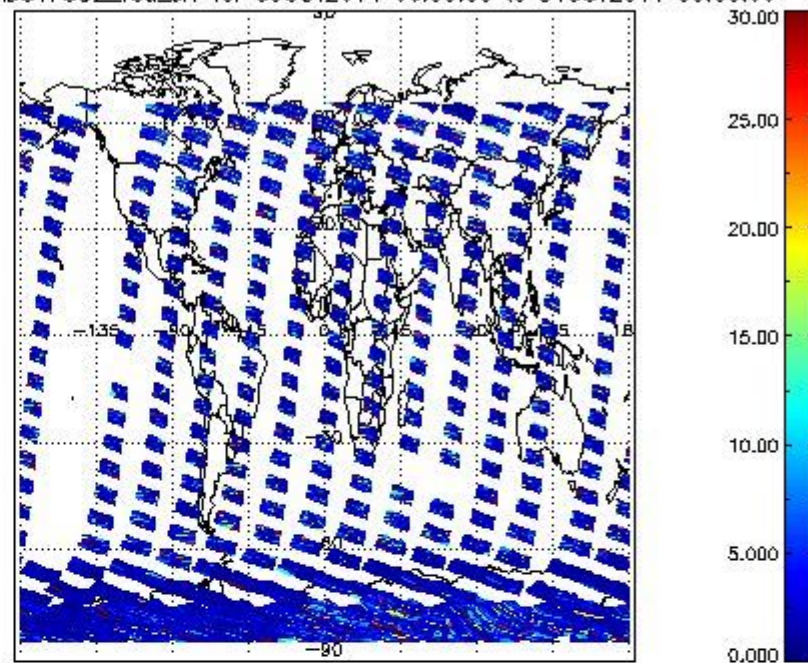
SCIOL2P_NADUV7S02_vcd_err for 30OCT2011 00:00:00 to 31OCT2011 00:00:00
