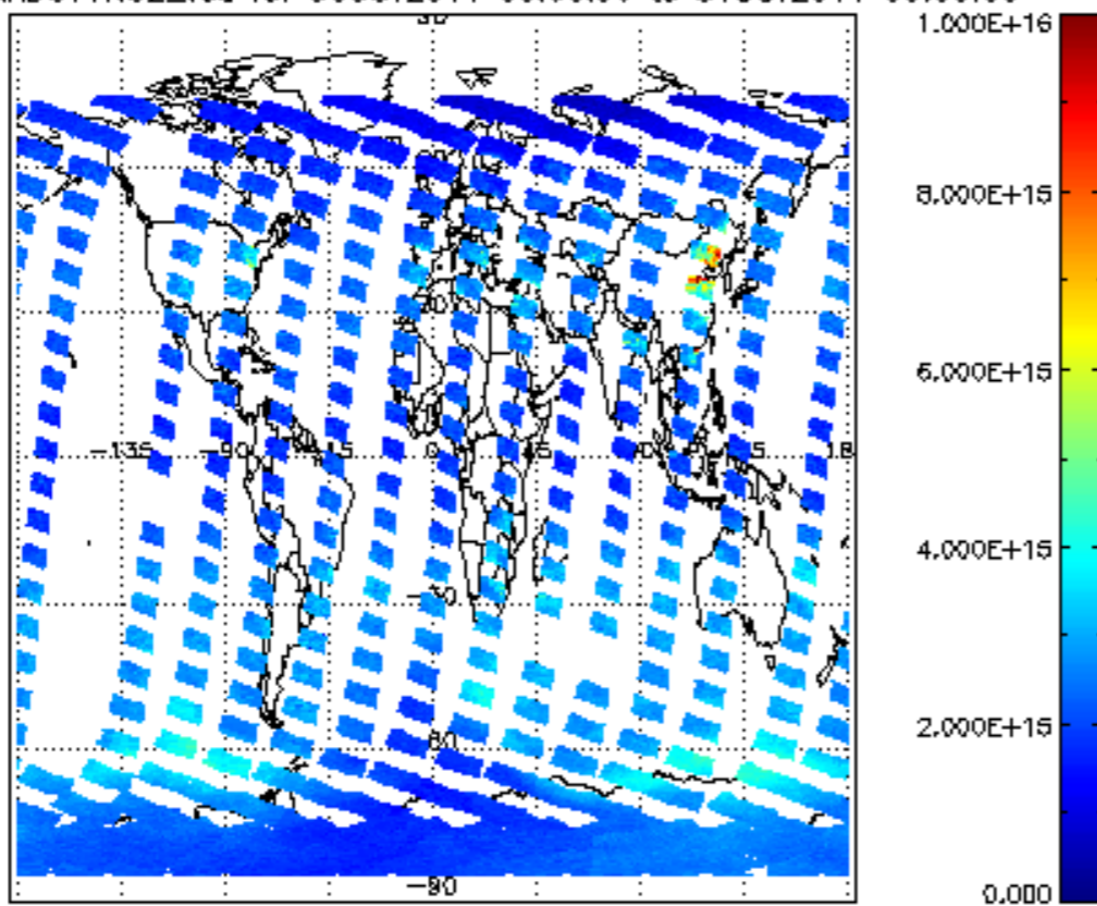
SCIOL2P_NADUV1NO2_vcd for 30OCT2011 00:00:00 to 31OCT2011 00:00:00
