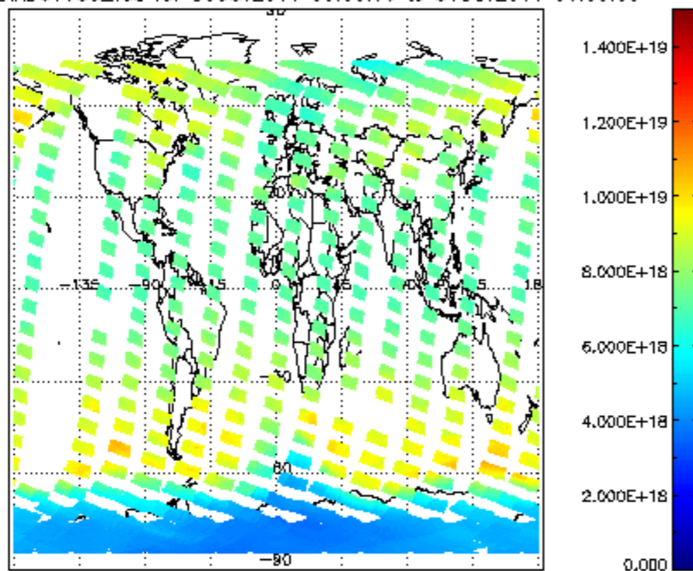
SCIOL2P_NADUV003_vcd for 30OCT2011 00:00:00 to 31OCT2011 00:00:00
