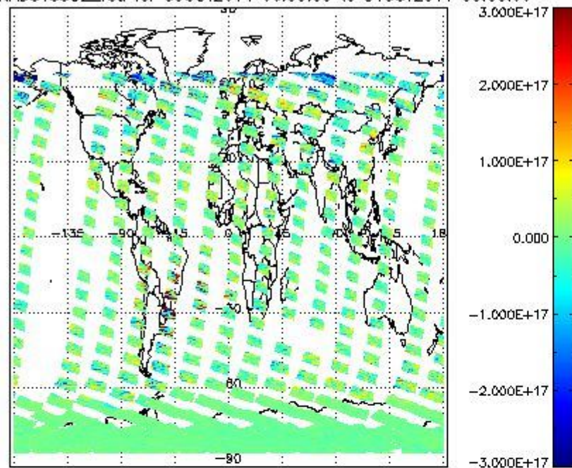
SCIOL2P_NADUV5SO2_vcd for 30OCT2011 00:00:00 to 31OCT2011 00:00:00
