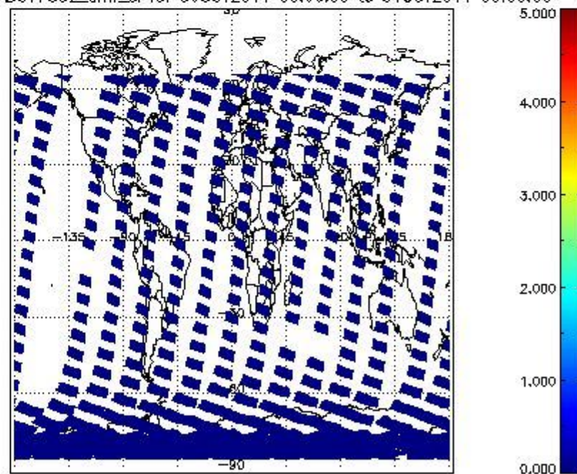
SCIOL2P_NADUV7S02_amf_cl for 30OCT2011 00:00:00 to 31OCT2011 00:00:00
