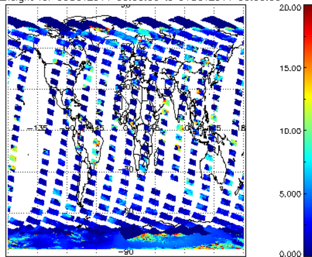
cl_top_height for 30OCT2011 00:00:00 to 31OCT2011 00:00:00
