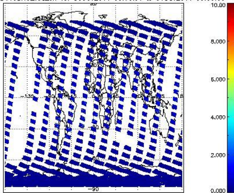
SCIOL2P_NADUV3BRO_vcd_err for 30OCT2011 00:00:00 to 31OCT2011 00:00:00
