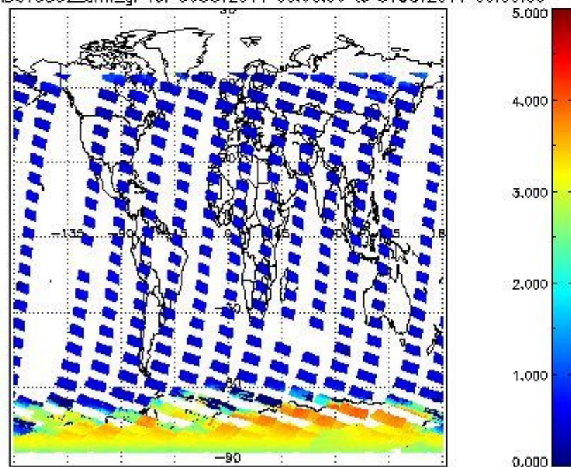
SCIOL2P_NADUV5SO2_amf_gr for 30OCT2011 00:00:00 to 31OCT2011 00:00:00
