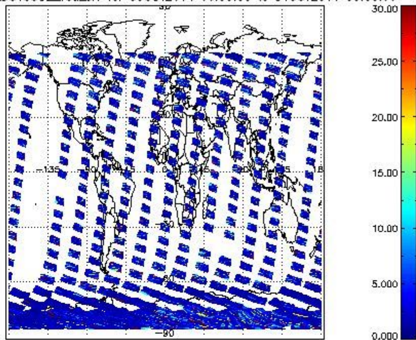
SCIOL2P_NADUV5SO2_vcd_err for 30OCT2011 00:00:00 to 31OCT2011 00:00:00
