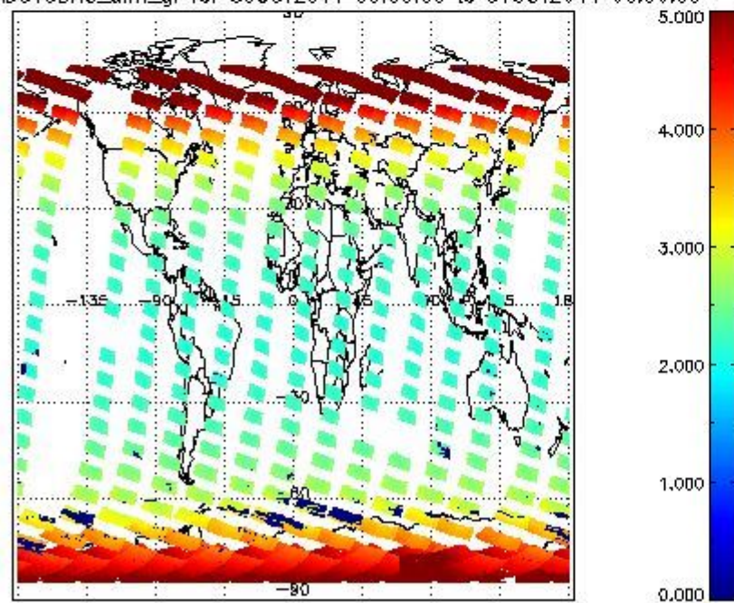
SCIOL2P_NADUV3BRO_amf_gr for 30OCT2011 00:00:00 to 31OCT2011 00:00:00
