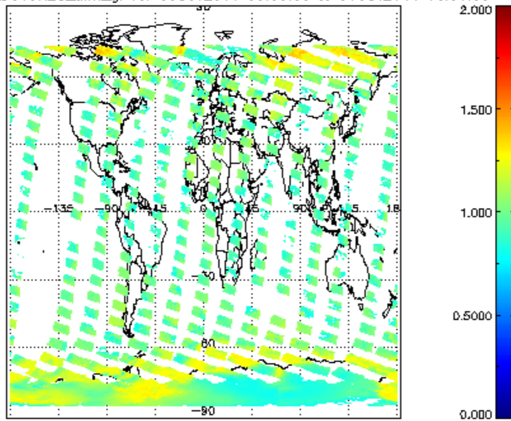
SCIOL2P_NADUV8H20_amf_gr for 30OCT2011 00:00:00 to 31OCT2011 00:00:00
