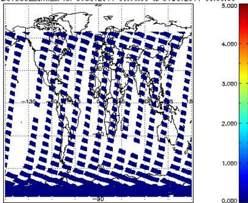
SCIOL2P_NADUV5SO2_amf_cl for 30OCT2011 00:00:00 to 31OCT2011 00:00:00
