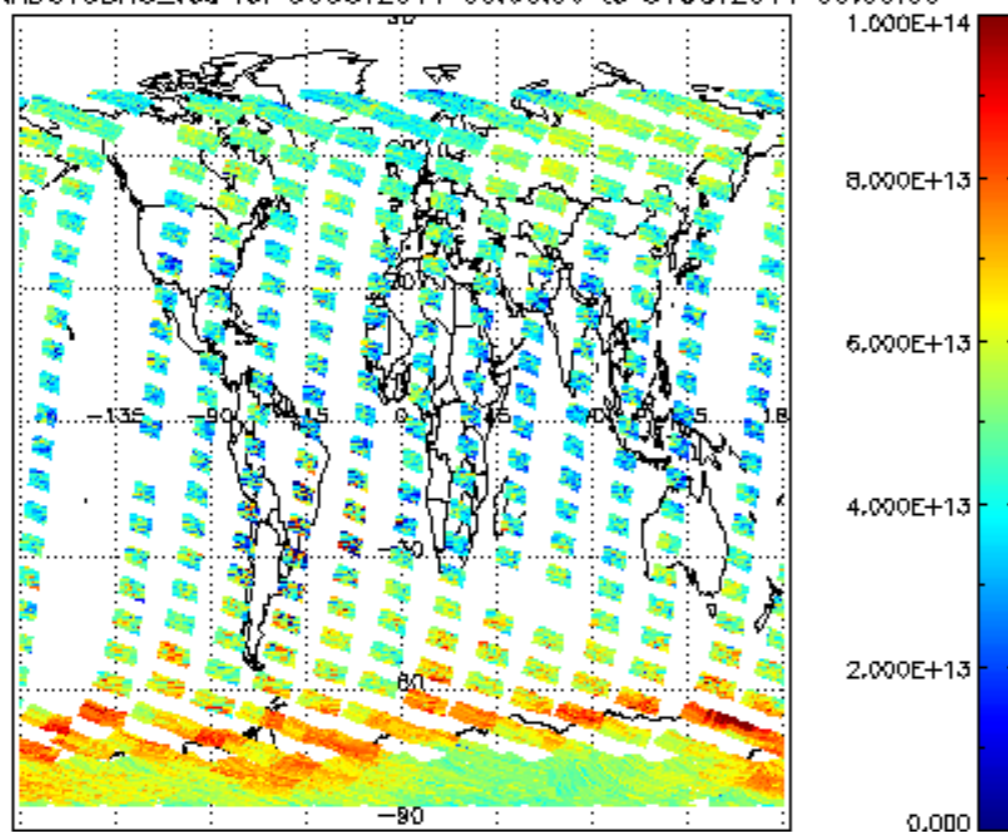
SCIOL2P_NADUV3BRO_vcd for 30OCT2011 00:00:00 to 31OCT2011 00:00:00
