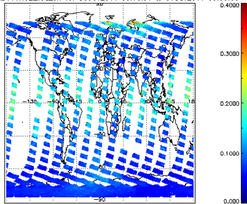
SCIOL2P_NADUV1NO2_vcd_err for 30OCT2011 00:00:00 to 31OCT2011 00:00:00
