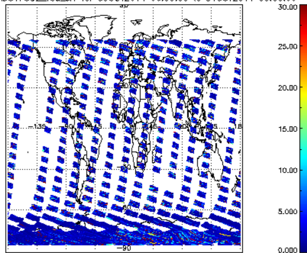
SCIOL2P_NADUV7S02_vcd_err for 30OCT2011 00:00:00 to 31OCT2011 00:00:00
