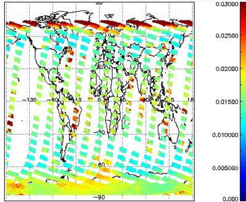
SCIOL2P_NADUV003_vcd_err for 30OCT2011 00:00:00 to 31OCT2011 00:00:00
