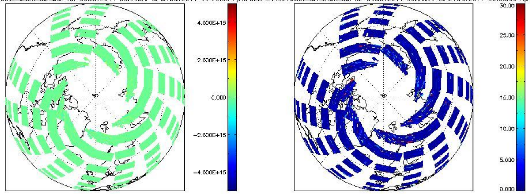
CIOL2P_NADUV60CL_slant_col_den for 30OCT2011 00:00:00 to 31OCT2011 00:00:00 np CIOL2P_NADUV60CL_err_slant_col for 30OCT2011 00:00:00 to 31OCT2011 00:00:00 np
