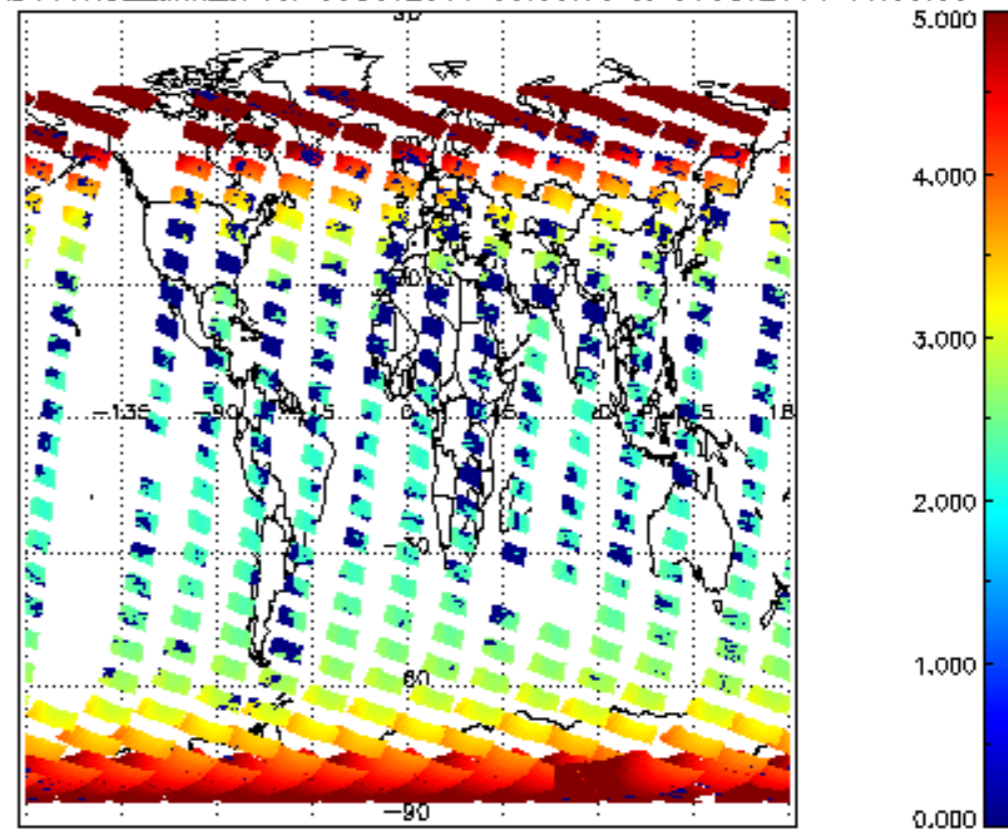
SCIOL2P_NADUV1NO2_amf_cl for 30OCT2011 00:00:00 to 31OCT2011 00:00:00
