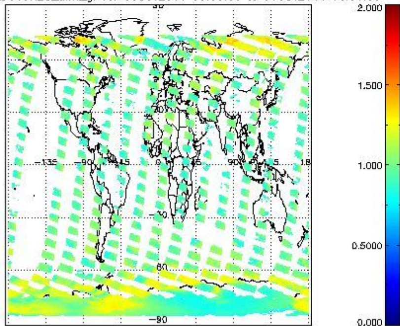
SCIOL2P_NADUV8H20_amf_gr for 30OCT2011 00:00:00 to 31OCT2011 00:00:00
