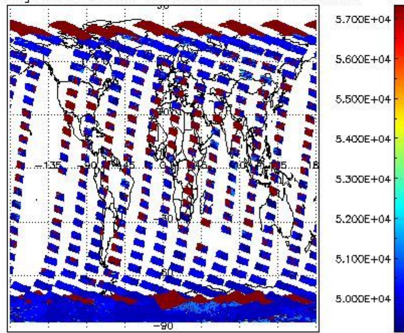
cloud_flags for 30OCT2011 00:00:00 to 31OCT2011 00:00:00
