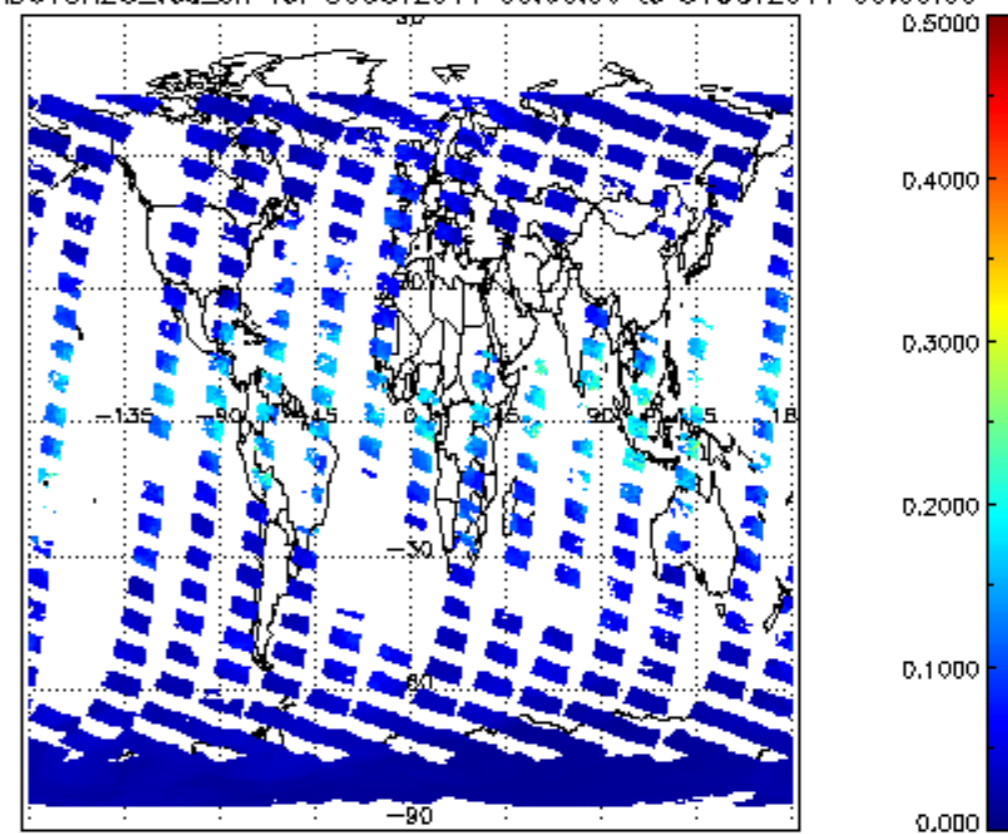
SCIOL2P_NADUV8H20_vcd_err for 30OCT2011 00:00:00 to 31OCT2011 00:00:00
