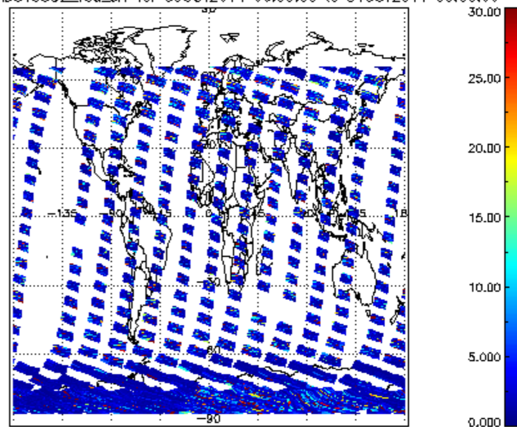
SCIOL2P_NADUV5S02_vcd_err for 30OCT2011 00:00:00 to 31OCT2011 00:00:00
