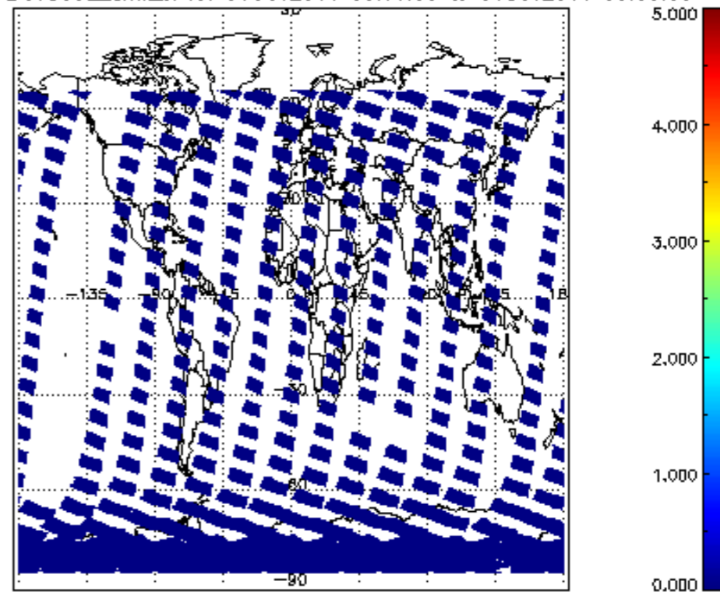
SCIOL2P_NADUV5S02_amf_cl for 30OCT2011 00:00:00 to 31OCT2011 00:00:00
