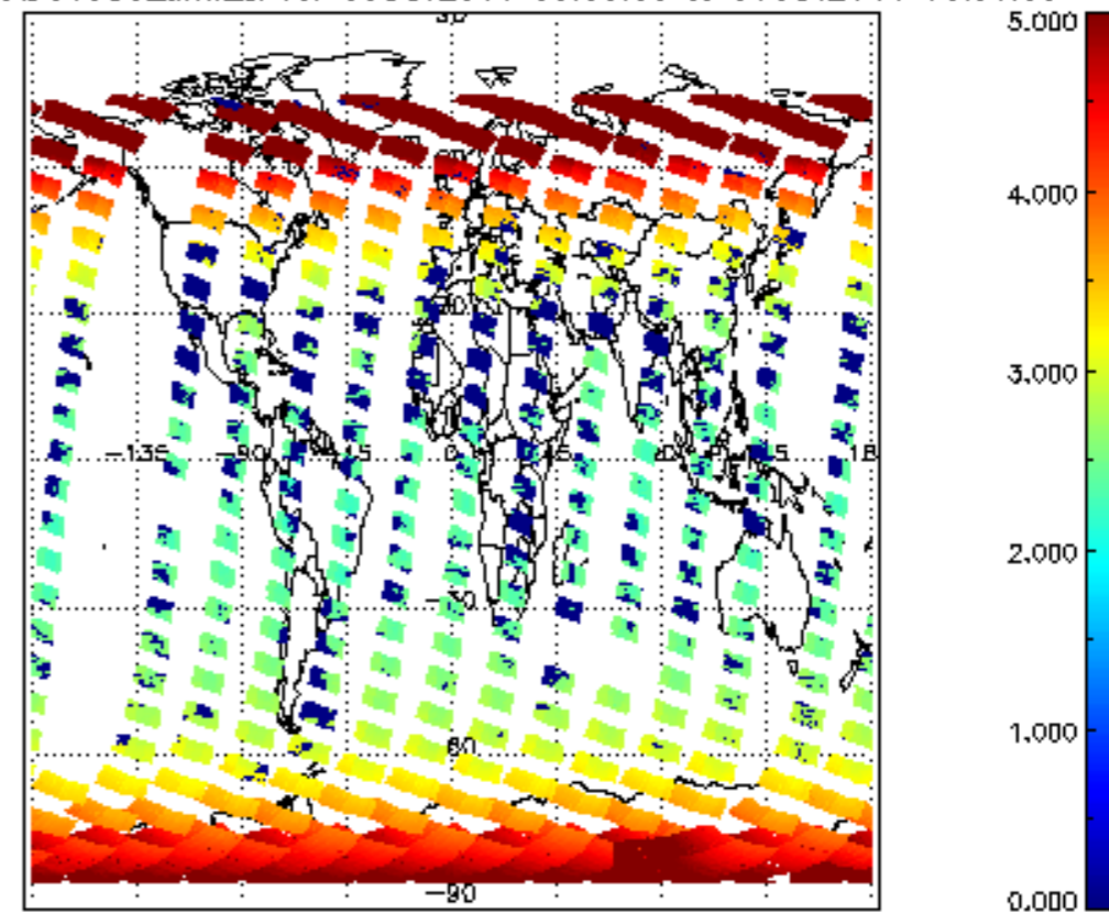
SCIOL2P_NADUV003_amf_cl for 30OCT2011 00:00:00 to 31OCT2011 00:00:00
