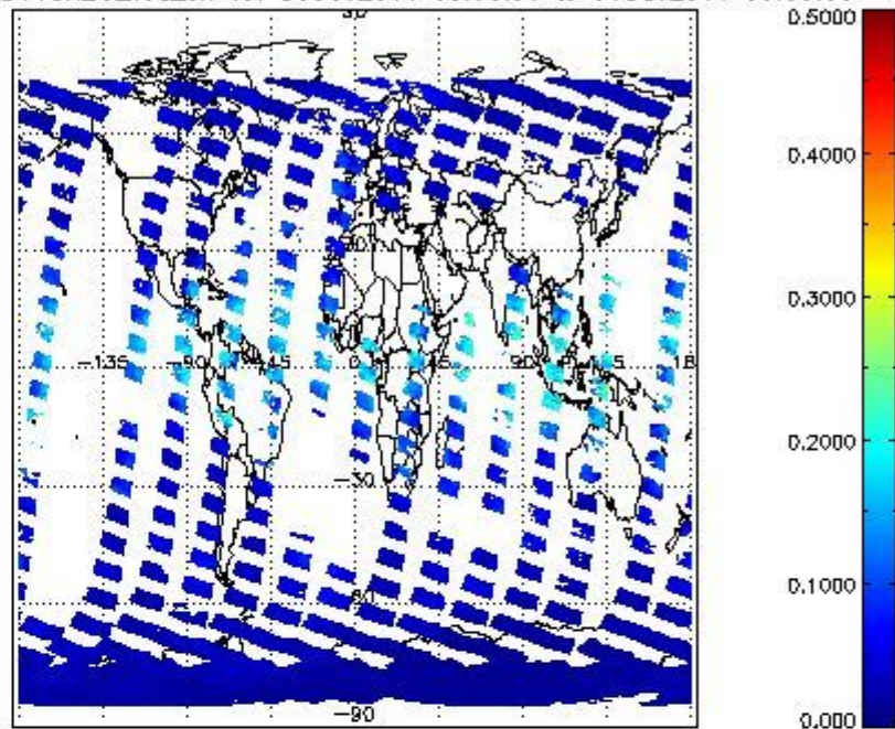
SCIOL2P_NADUV8H20_vcd_err for 30OCT2011 00:00:00 to 31OCT2011 00:00:00
