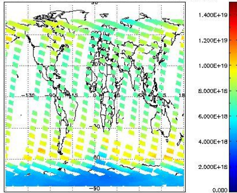
SCIOL2P_NADUV003_vcd for 30OCT2011 00:00:00 to 31OCT2011 00:00:00
