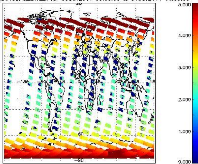
SCIOL2P_NADUV3BRO_amf_cl for 30OCT2011 00:00:00 to 31OCT2011 00:00:00
