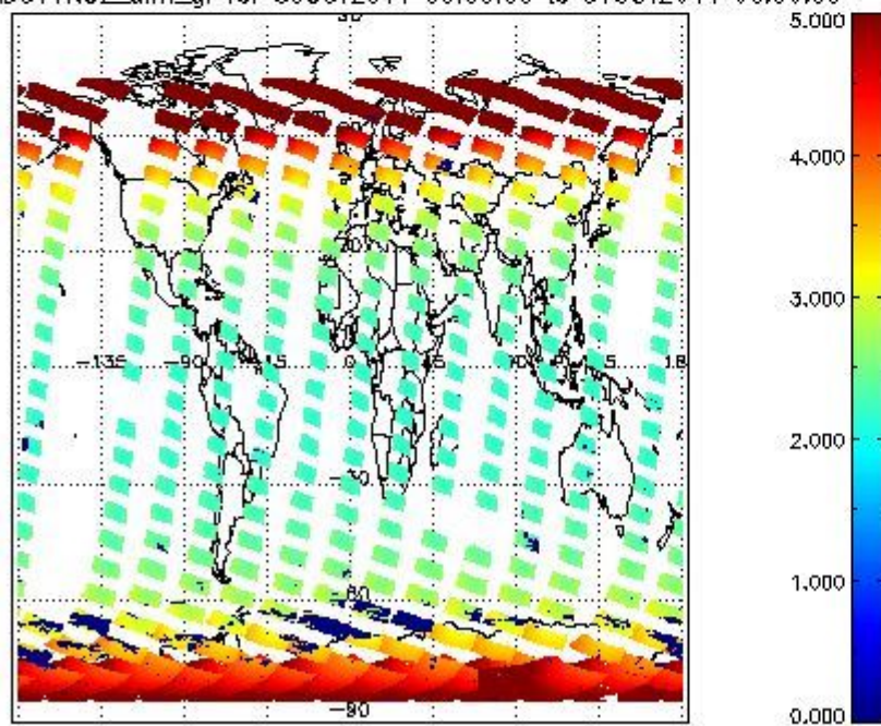
SCIOL2P_NADUV1NO2_amf_gr for 30OCT2011 00:00:00 to 31OCT2011 00:00:00
