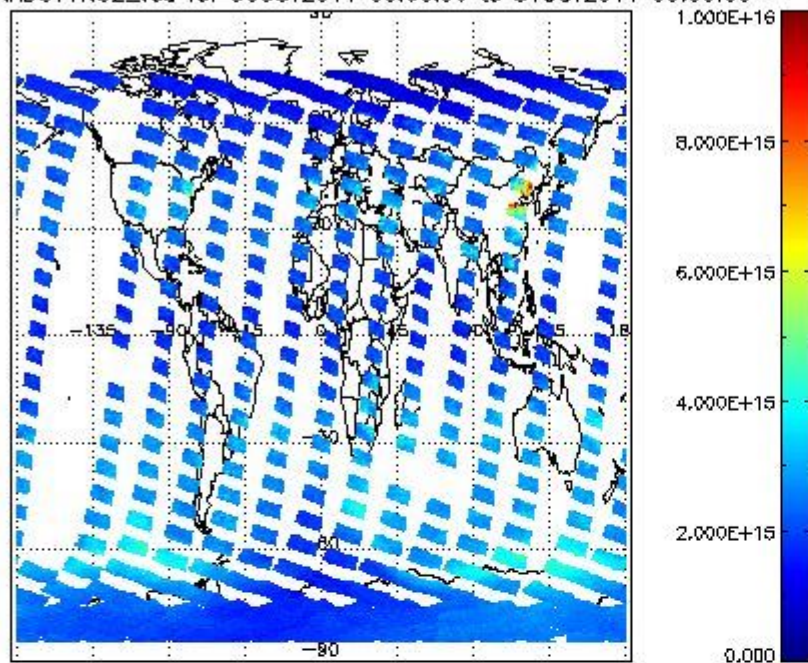
SCIOL2P_NADUV1NO2_vcd for 30OCT2011 00:00:00 to 31OCT2011 00:00:00
