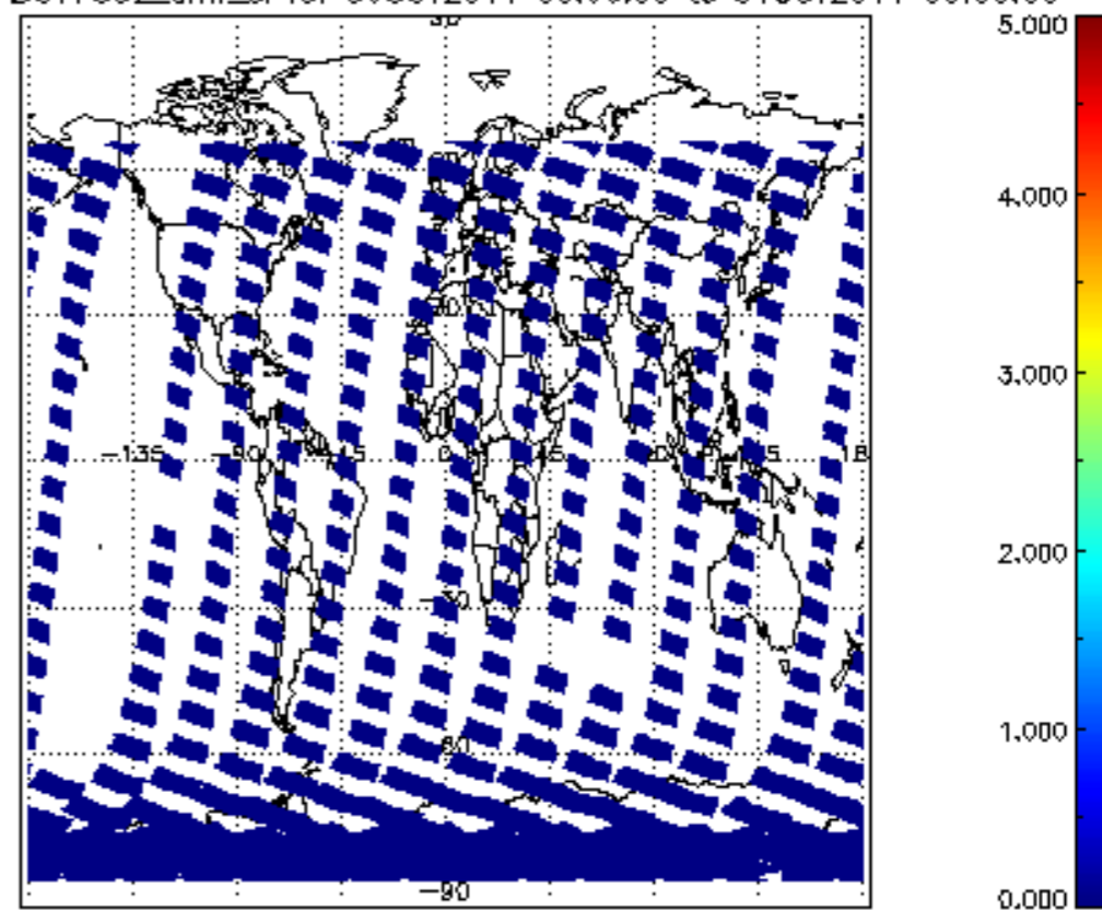
SCIOL2P_NADUV7S02_amf_cl for 30OCT2011 00:00:00 to 31OCT2011 00:00:00
