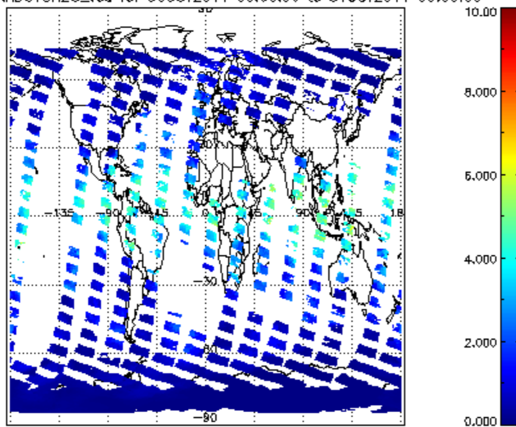
SCIOL2P_NADUV8H20_vcd for 30OCT2011 00:00:00 to 31OCT2011 00:00:00
