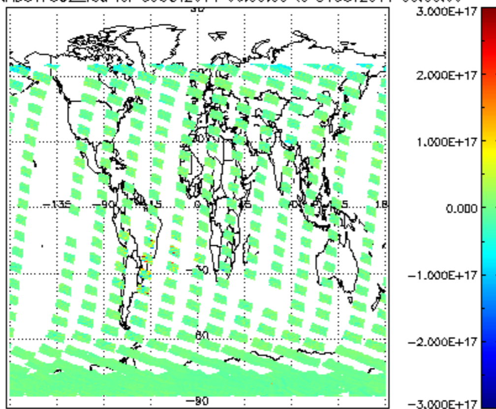
SCIOL2P_NADUV7S02_vcd for 30OCT2011 00:00:00 to 31OCT2011 00:00:00
