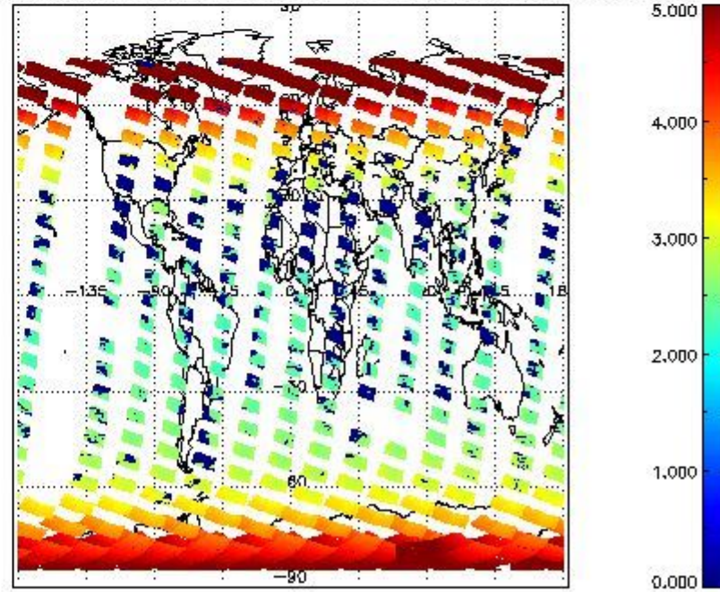
SCIOL2P_NADUV003_amf_cl for 30OCT2011 00:00:00 to 31OCT2011 00:00:00
