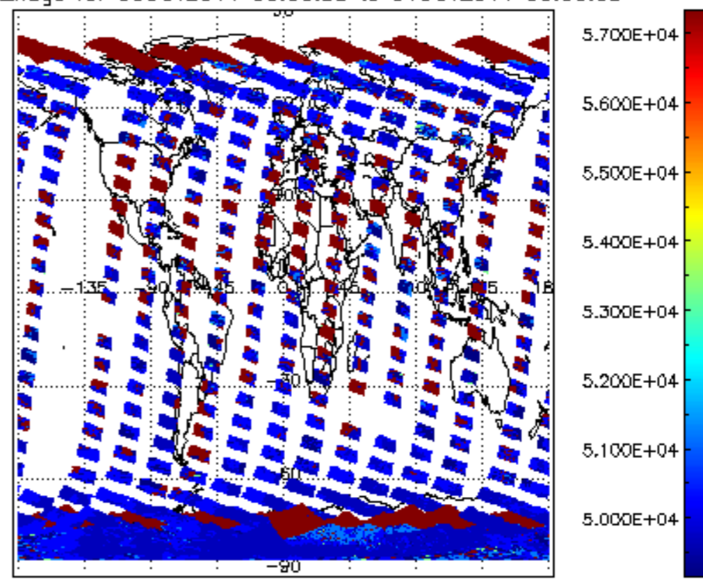
cloud_flags for 30OCT2011 00:00:00 to 31OCT2011 00:00:00
