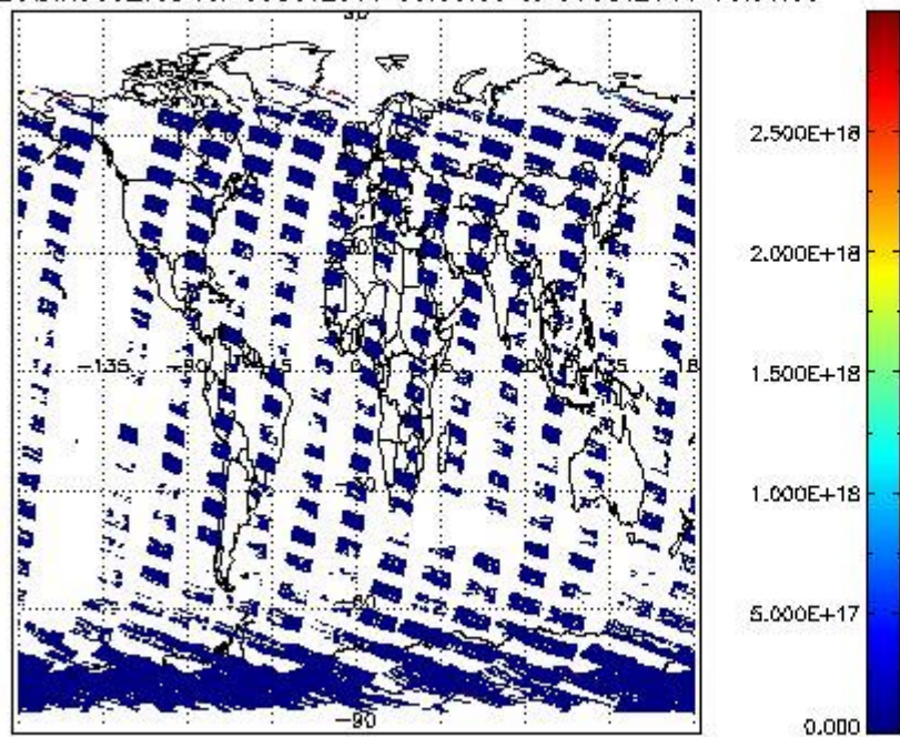
SCIDL2P_NADIR3CO_vcd for 30OCT2011 00:00:00 to 31OCT2011 00:00:00
