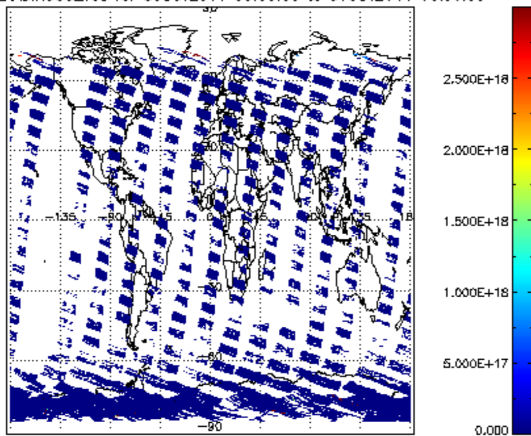
SCIOL2P_NADIR3CO_vcd for 30OCT2011 00:00:00 to 31OCT2011 00:00:00
