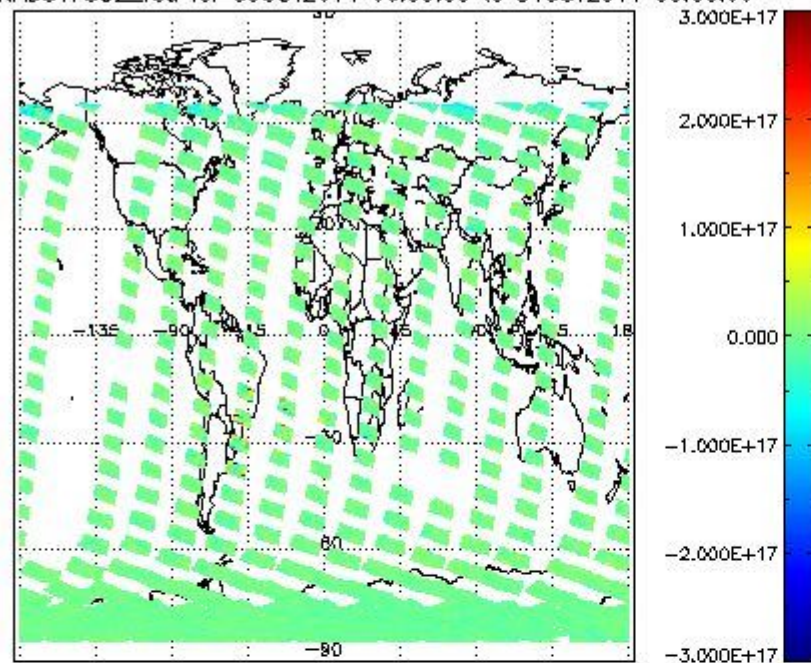
SCIOL2P_NADUV7S02_vcd for 30OCT2011 00:00:00 to 31OCT2011 00:00:00
