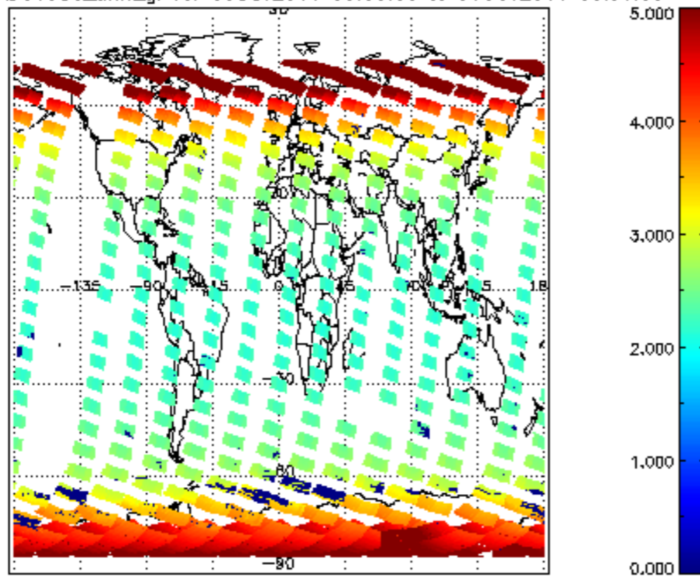
SCIOL2P_NADUV003_amf_gr for 30OCT2011 00:00:00 to 31OCT2011 00:00:00
