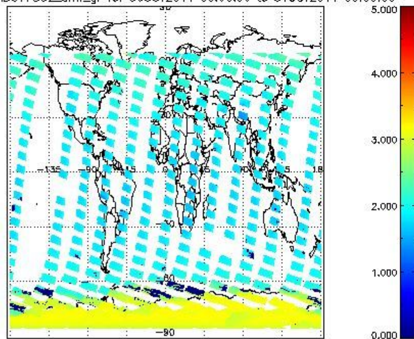
SCIOL2P_NADUV7S02_amf_gr for 30OCT2011 00:00:00 to 31OCT2011 00:00:00
