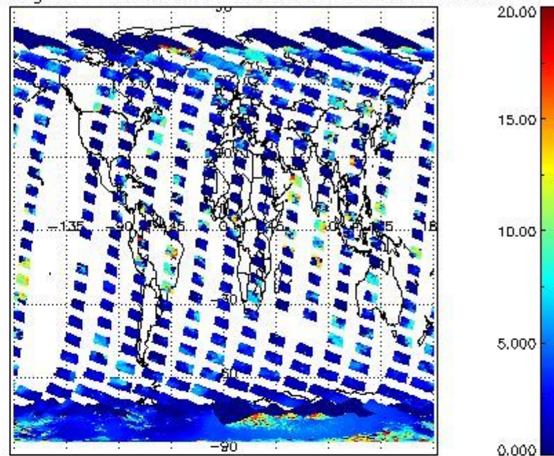
cL_top_height for 30OCT2011 00:00:00 to 31OCT2011 00:00:00
