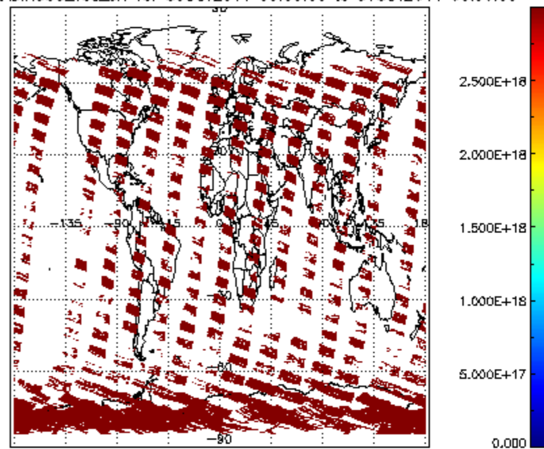
SCIOL2P_NADIR3CO_vcd_err for 30OCT2011 00:00:00 to 31OCT2011 00:00:00
