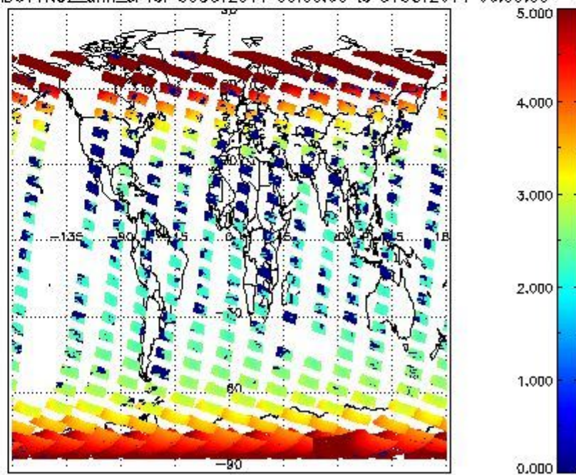
SCIOL2P_NADUV1NO2_amf_cl for 30OCT2011 00:00:00 to 31OCT2011 00:00:00
