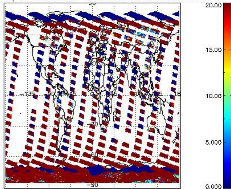
cL_opt_depth for 30OCT2011 00:00:00 to 31OCT2011 00:00:00
