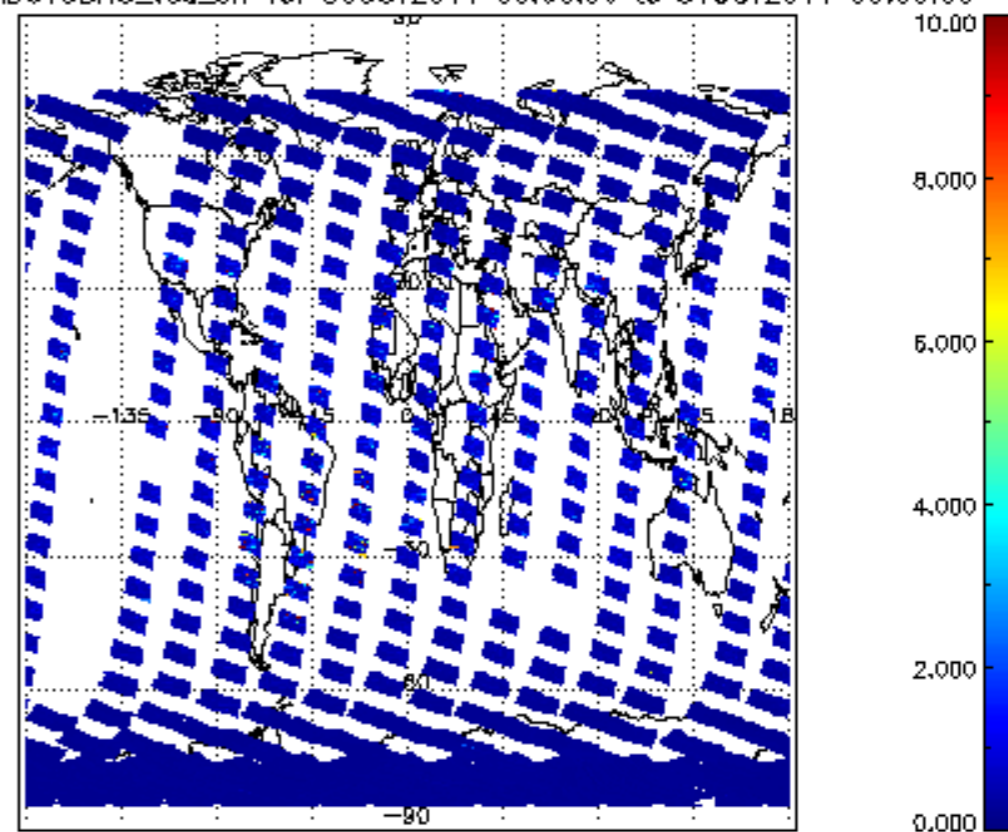
SCIOL2P_NADUV3BRO_vcd_err for 30OCT2011 00:00:00 to 31OCT2011 00:00:00
