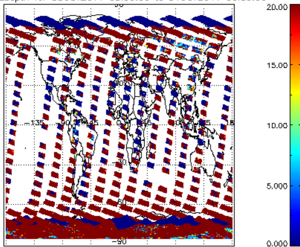
cl_opt_depth for 30OCT2011 00:00:00 to 31OCT2011 00:00:00
