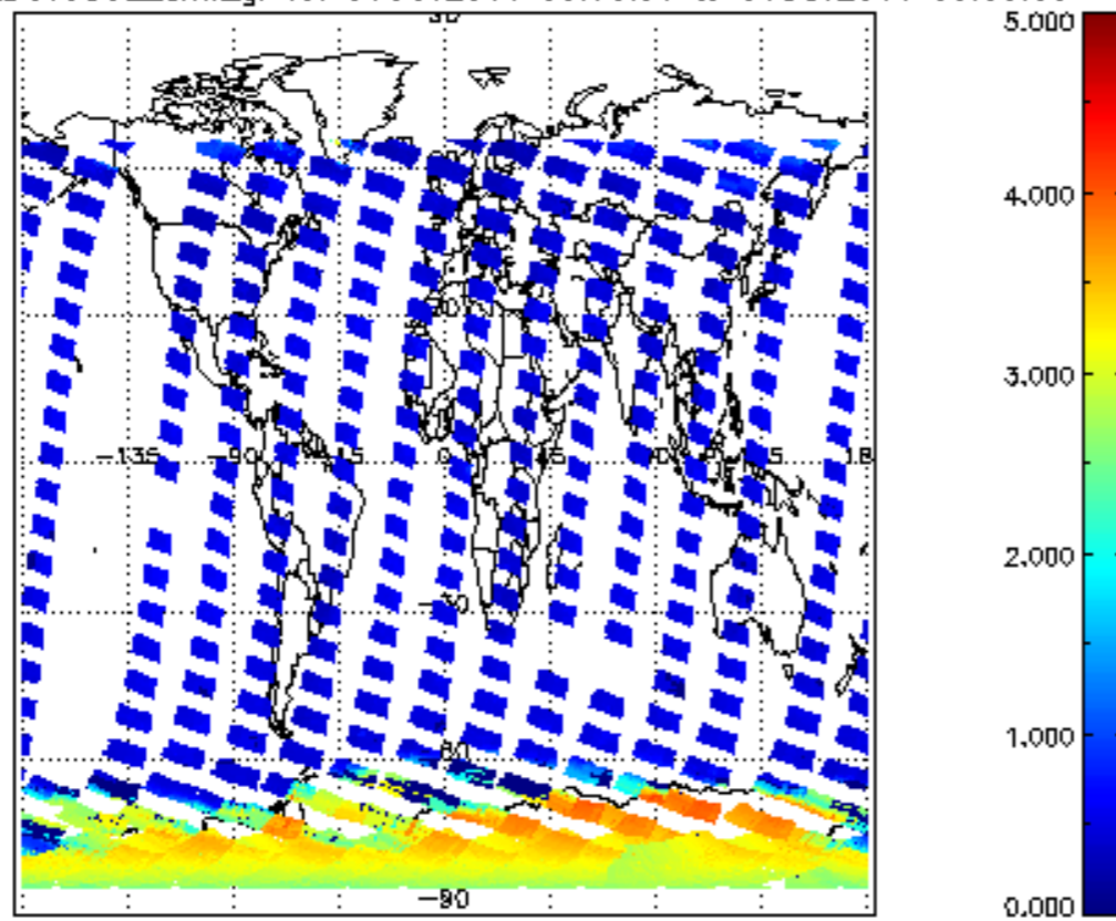
SCIOL2P_NADUV5S02_amf_gr for 30OCT2011 00:00:00 to 31OCT2011 00:00:00
