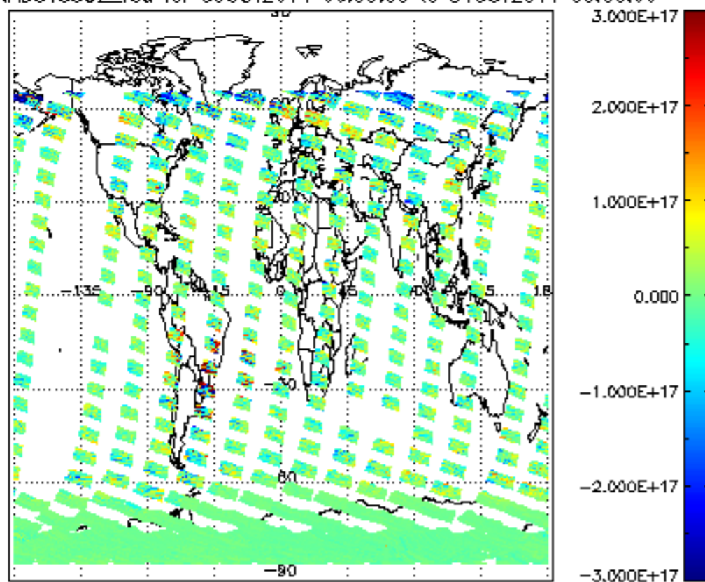
SCIOL2P_NADUV5S02_vcd for 30OCT2011 00:00:00 to 31OCT2011 00:00:00
