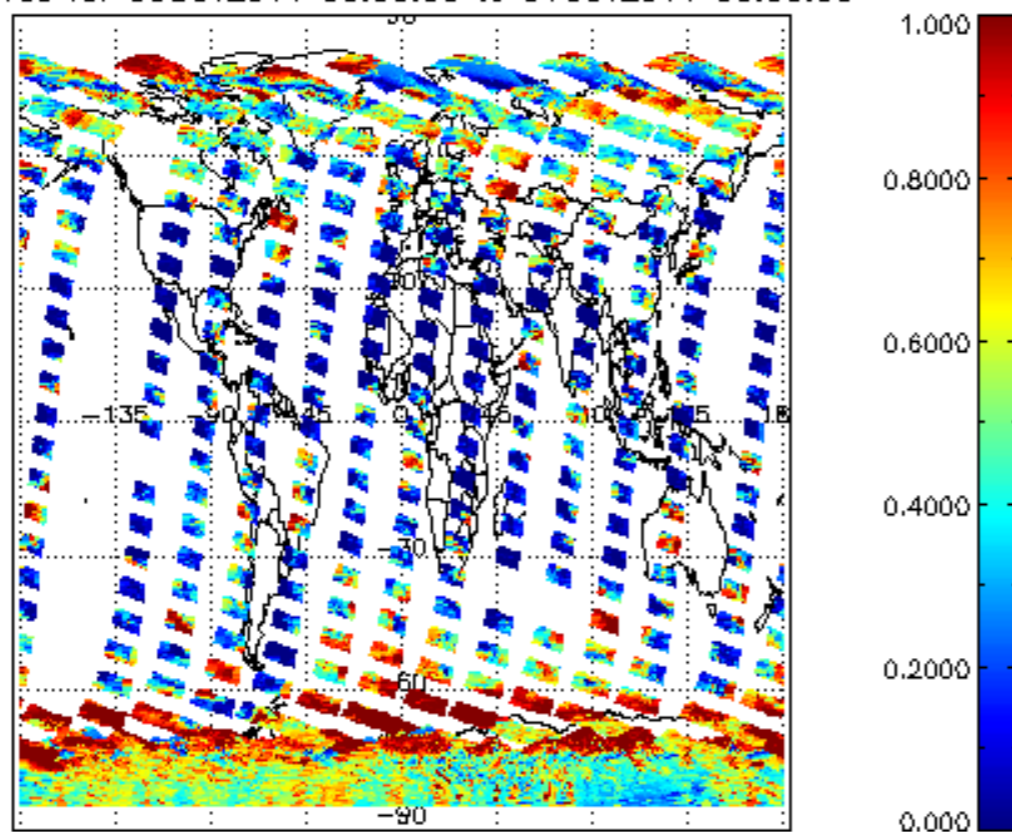
cl_frac for 30OCT2011 00:00:00 to 31OCT2011 00:00:00
