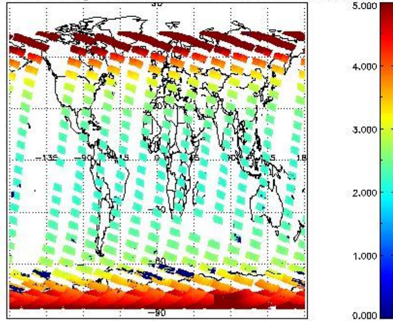
SCIOL2P_NADUV003_amf_gr for 30OCT2011 00:00:00 to 31OCT2011 00:00:00
