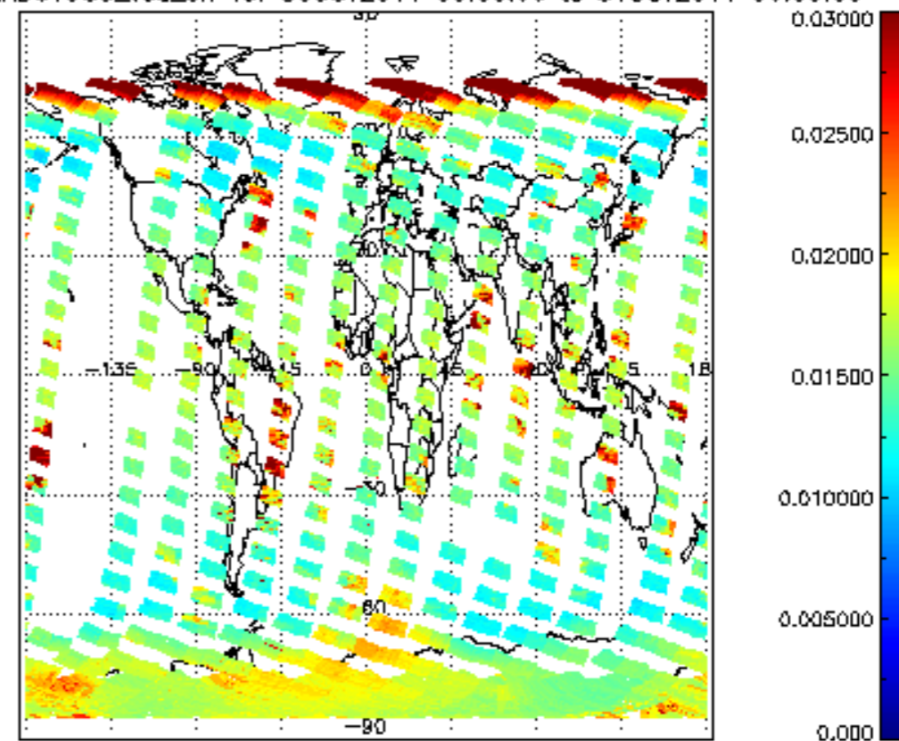
SCIOL2P_NADUV003_vcd_err for 30OCT2011 00:00:00 to 31OCT2011 00:00:00
