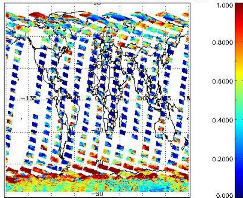
cLfrac for 30OCT2011 00:00:00 to 31OCT2011 00:00:00
