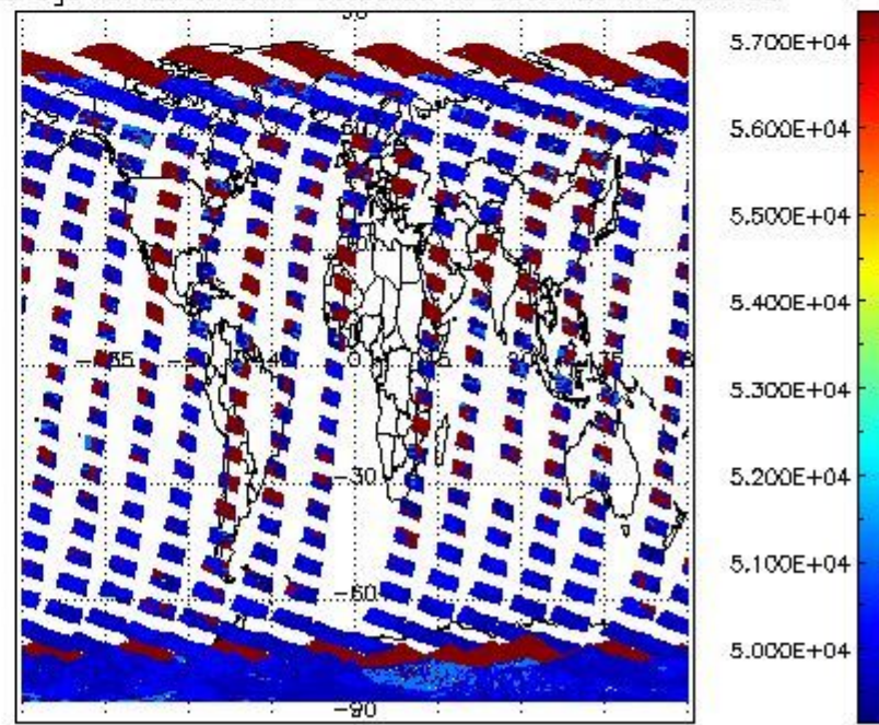
cloud_flags for 28OCT2011 00:00:00 to 29OCT2011 00:00:00
