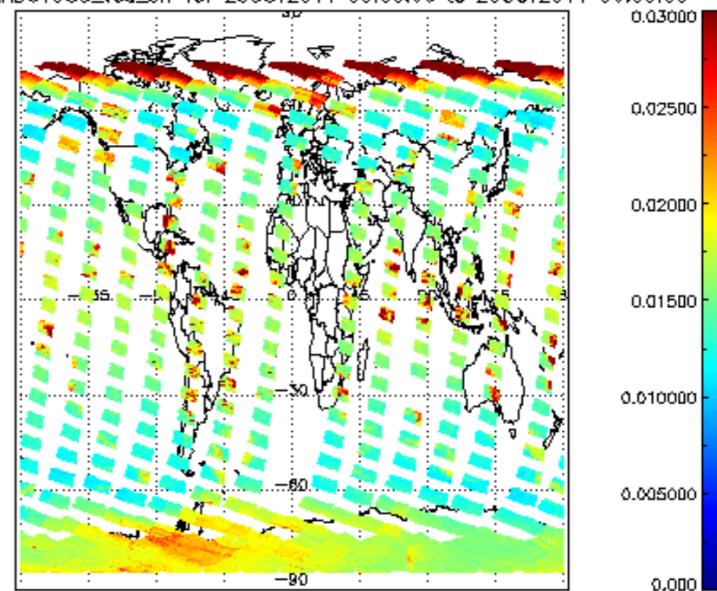
SCIOL2P_NADUV003_vcd_err for 28OCT2011 00:00:00 to 29OCT2011 00:00:00
