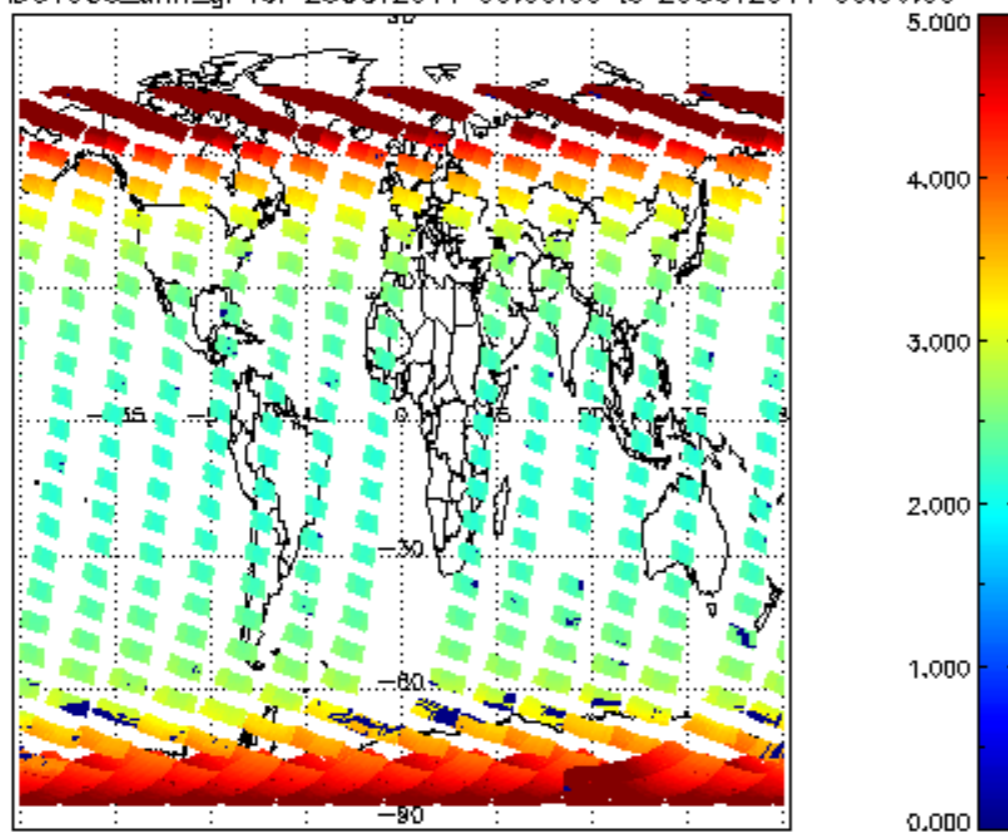
SCIOL2P_NADUV003_amf_gr for 28OCT2011 00:00:00 to 29OCT2011 00:00:00
