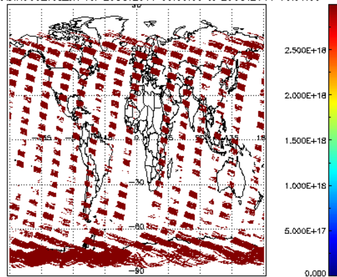
SCIOL2P_NADIR3CO_vcd_err for 28OCT2011 00:00:00 to 29OCT2011 00:00:00
