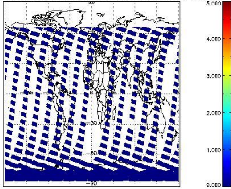
SCIOL2P_NADUV5SO2_amf_cl for 28OCT2011 00:00:00 to 29OCT2011 00:00:00
