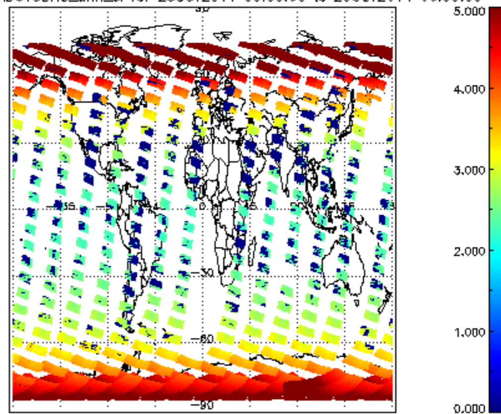
SCIOL2P_NADUV3BRO_amf_cl for 28OCT2011 00:00:00 to 29OCT2011 00:00:00
