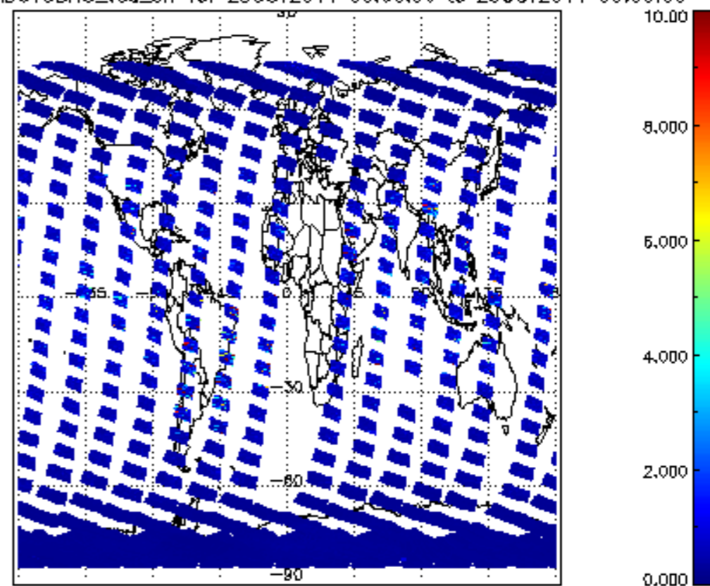
SCIOL2P_NADUV3BRO_vcd_err for 28OCT2011 00:00:00 to 29OCT2011 00:00:00
