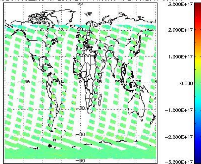
SCIOL2P_NADUV7S02_vcd for 28OCT2011 00:00:00 to 29OCT2011 00:00:00
