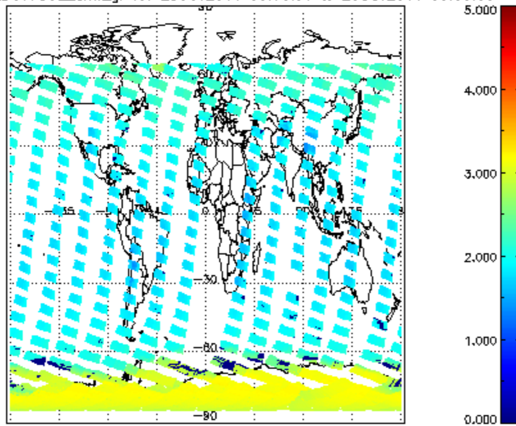
SCIOL2P_NADUV7S02_amf_gr for 28OCT2011 00:00:00 to 29OCT2011 00:00:00
