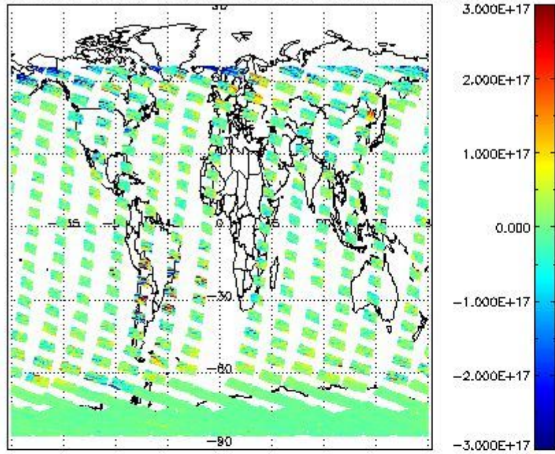
SCIOL2P_NADUV5SO2_vcd for 28OCT2011 00:00:00 to 29OCT2011 00:00:00
