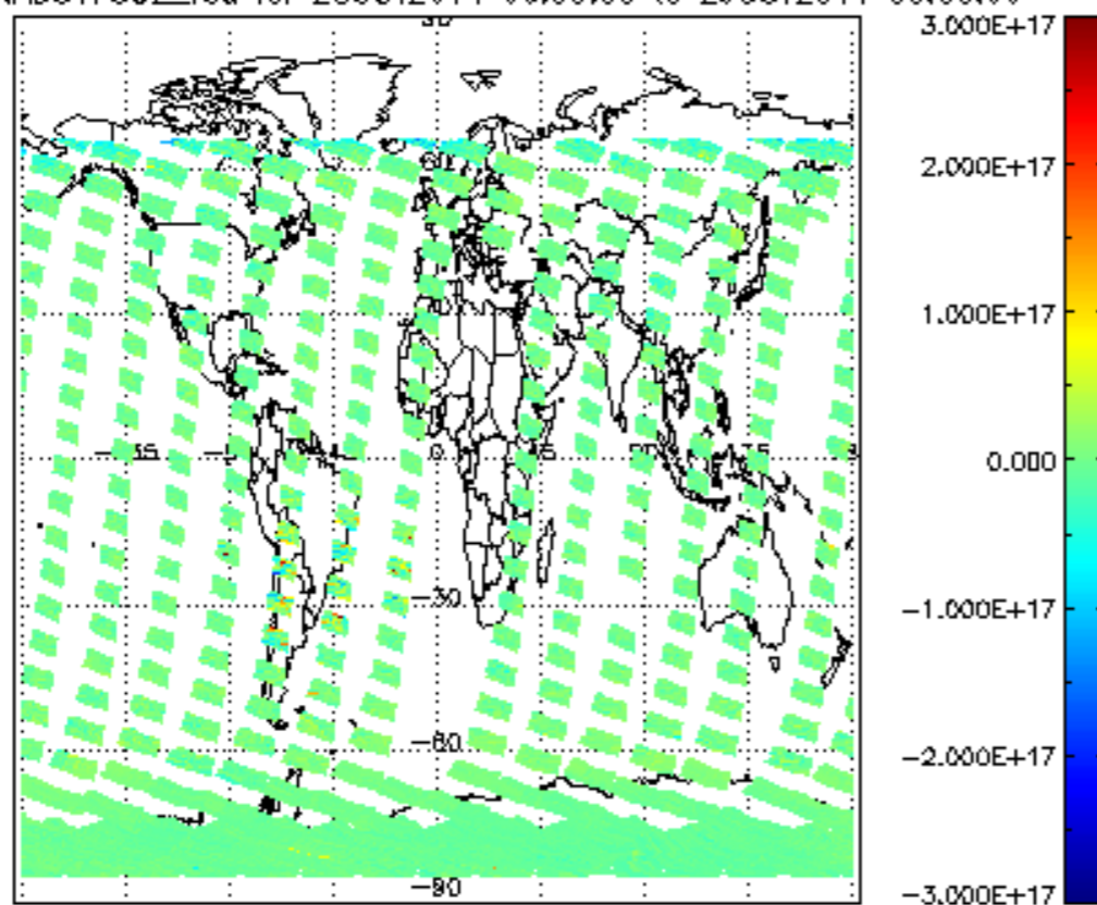
SCIOL2P_NADUV7S02_vcd for 28OCT2011 00:00:00 to 29OCT2011 00:00:00
