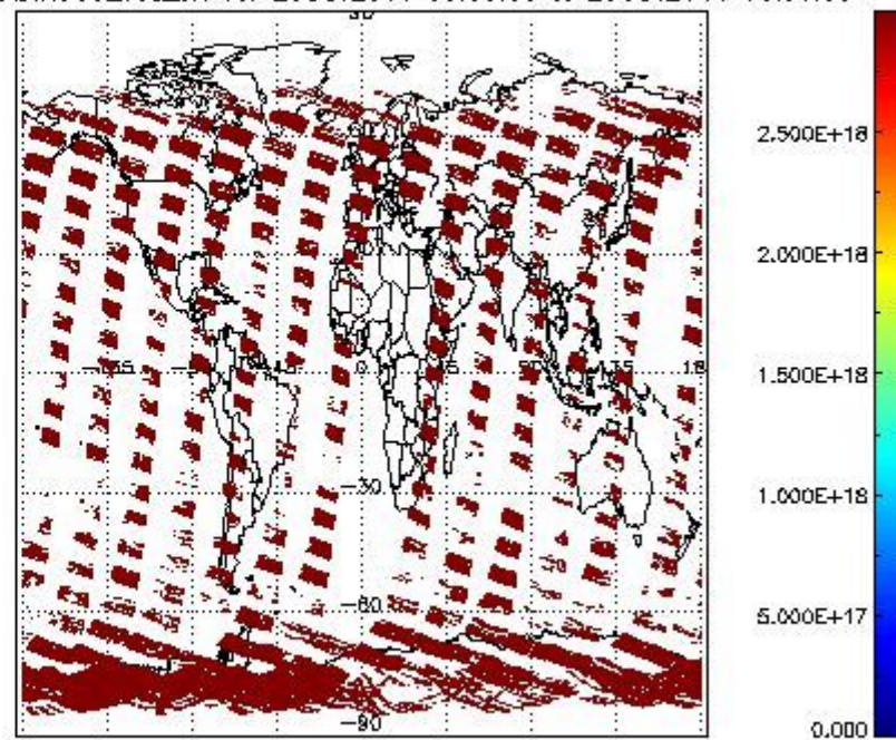
SCIDL2P_NADIR3CO_vcd_err for 28OCT2011 00:00:00 to 29OCT2011 00:00:00
