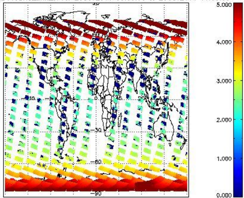
SCIOL2P_NADUV3BRO_amf_cl for 28OCT2011 00:00:00 to 29OCT2011 00:00:00
