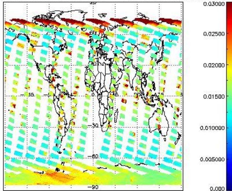
SCIOL2P_NADUV003_vcd_err for 28OCT2011 00:00:00 to 29OCT2011 00:00:00
