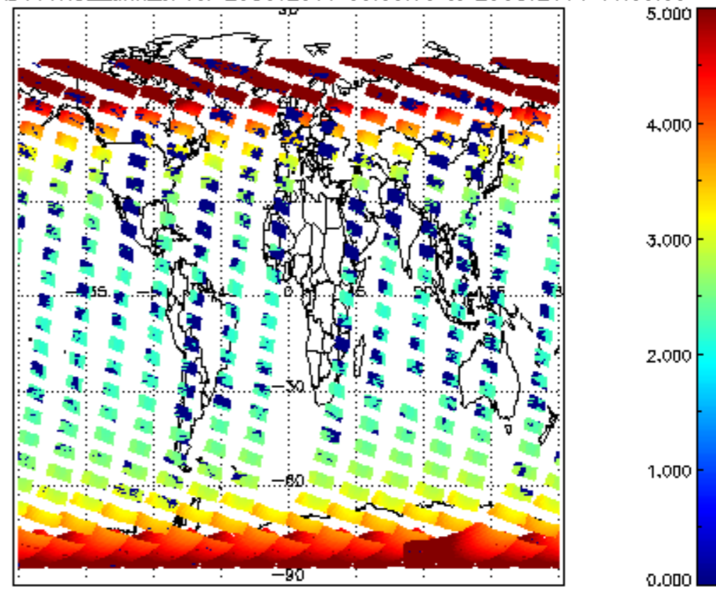
SCIOL2P_NADUV1NO2_amf_cl for 28OCT2011 00:00:00 to 29OCT2011 00:00:00
