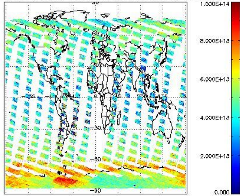
SCIOL2P_NADUV3BRO_vcd for 28OCT2011 00:00:00 to 29OCT2011 00:00:00
