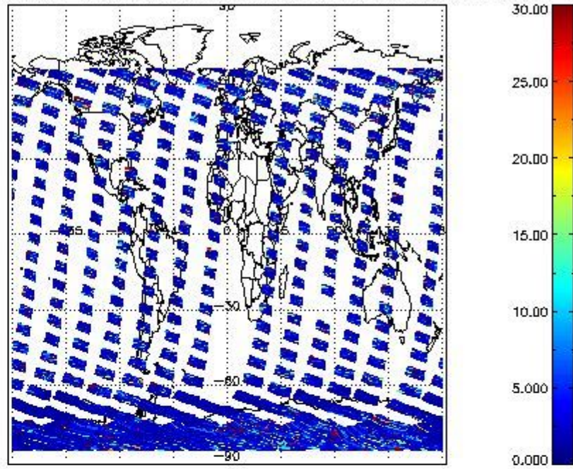
SCIOL2P_NADUV5SO2_vcd_err for 28OCT2011 00:00:00 to 29OCT2011 00:00:00
