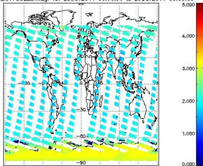
SCIOL2P_NADUV7S02_amf_gr for 28OCT2011 00:00:00 to 29OCT2011 00:00:00
