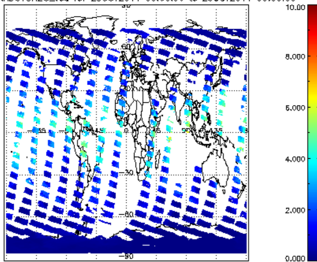
SCIOL2P_NADUV8H20_vcd for 28OCT2011 00:00:00 to 29OCT2011 00:00:00
