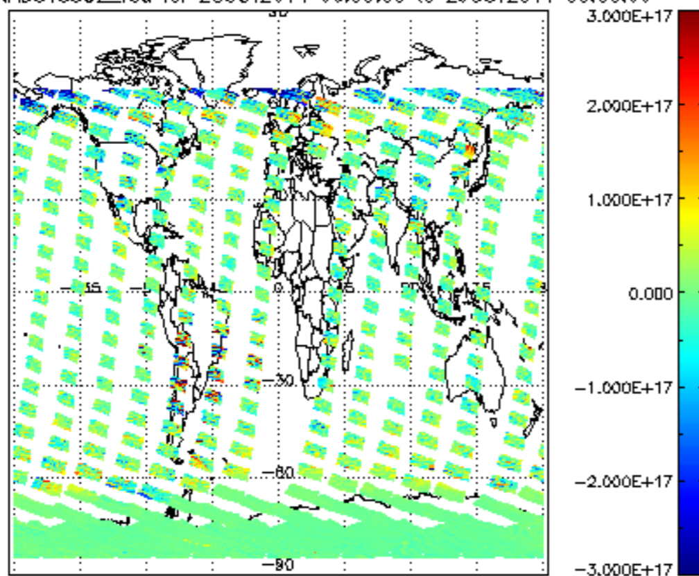
SCIOL2P_NADUV5S02_vcd for 28OCT2011 00:00:00 to 29OCT2011 00:00:00
