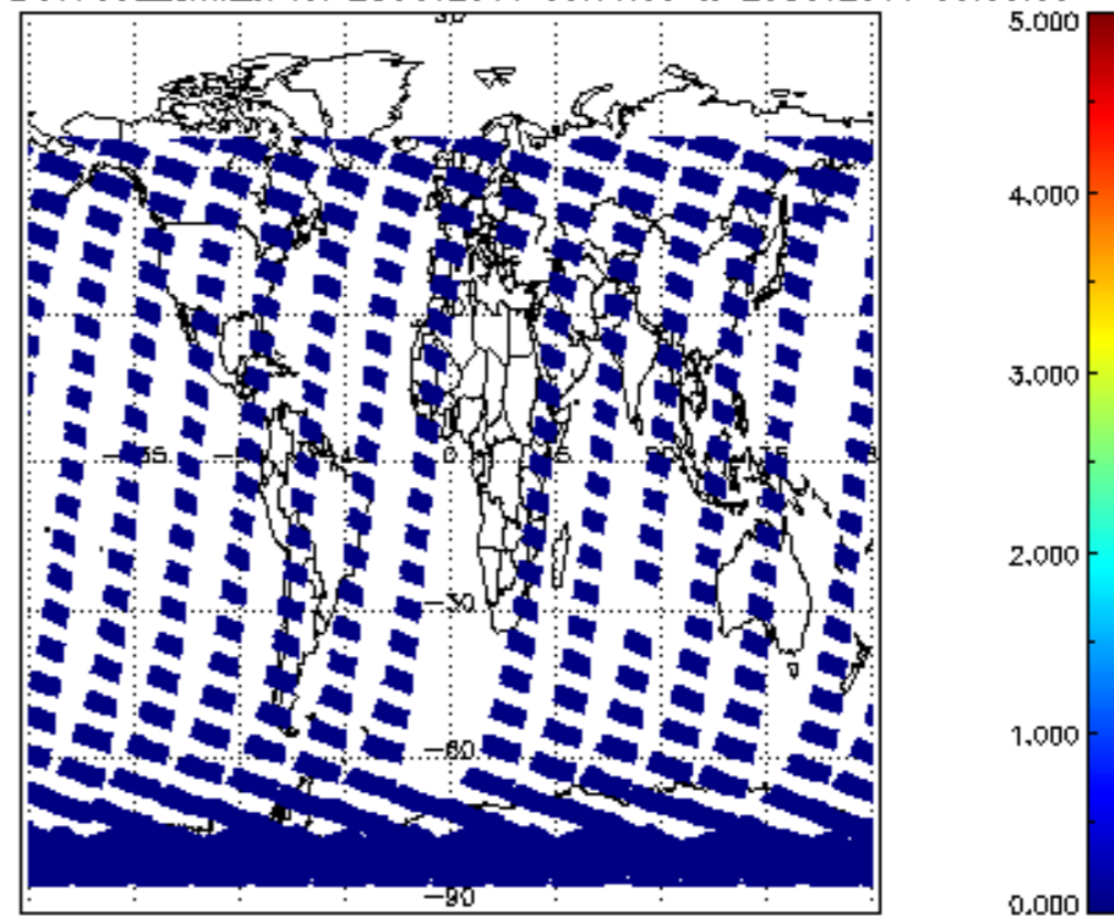
SCIOL2P_NADUV7S02_amf_sl for 28OCT2011 00:00:00 to 29OCT2011 00:00:00
