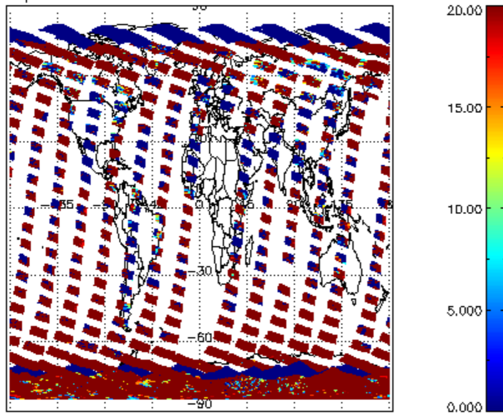
cl_opt_depth for 28OCT2011 00:00:00 to 29OCT2011 00:00:00
