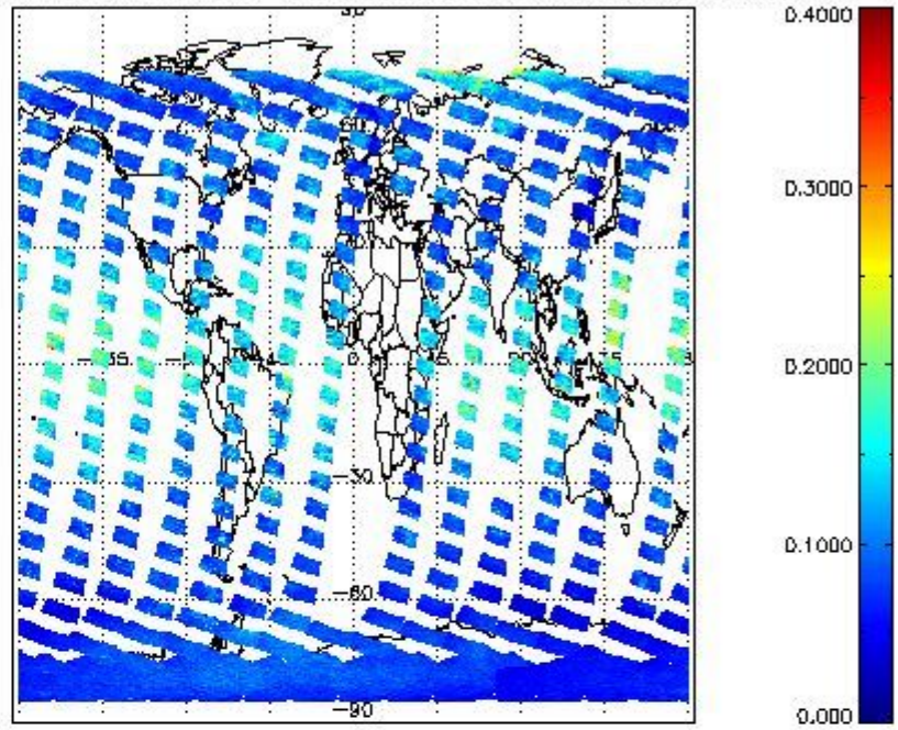
SCIOL2P_NADUV1NO2_vcd_err for 28OCT2011 00:00:00 to 29OCT2011 00:00:00
