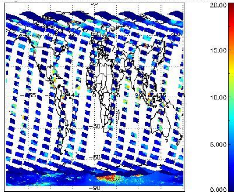
cL_top_height for 28OCT2011 00:00:00 to 29OCT2011 00:00:00
