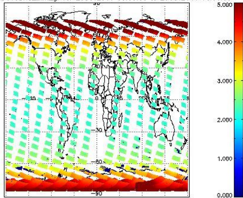
SCIOL2P_NADUV3BRO_amf_gr for 28OCT2011 00:00:00 to 29OCT2011 00:00:00
