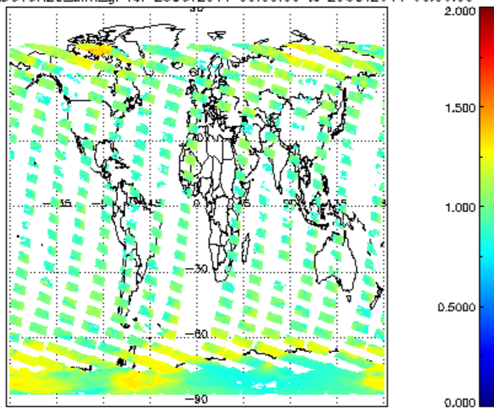
SCIOL2P_NADUV8H20_amf_gr for 28OCT2011 00:00:00 to 29OCT2011 00:00:00
