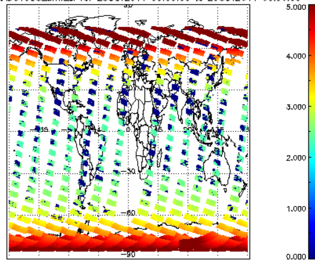
SCIOL2P_NADUV003_amf_cl for 28OCT2011 00:00:00 to 29OCT2011 00:00:00
