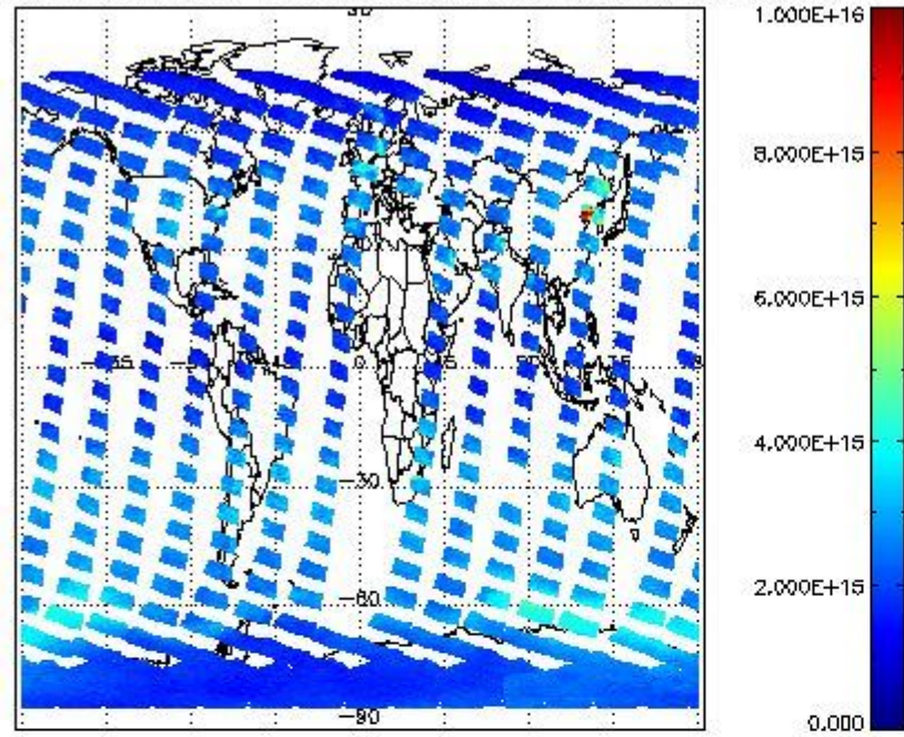
SCIOL2P_NADUV1NO2_vcd for 28OCT2011 00:00:00 to 29OCT2011 00:00:00
