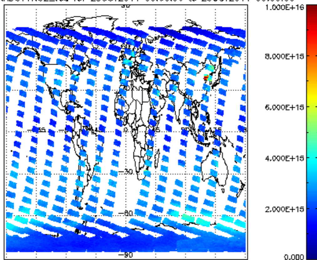
SCIOL2P_NADUV1NO2_vcd for 28OCT2011 00:00:00 to 29OCT2011 00:00:00
