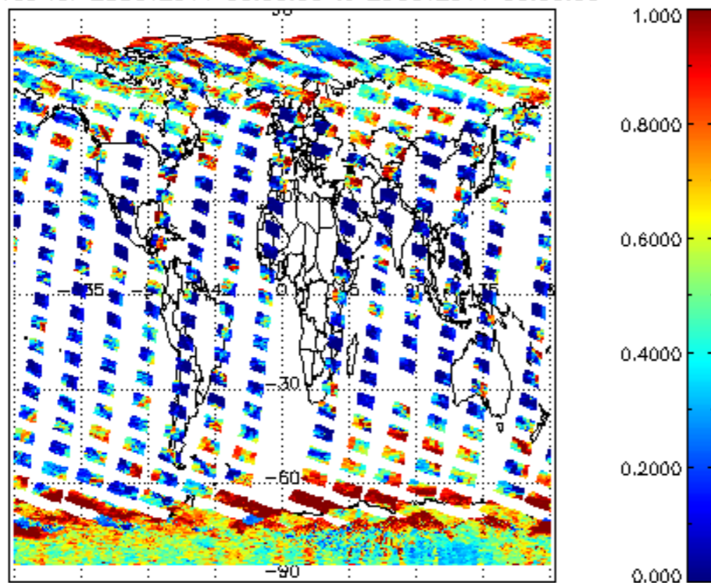
cl_frac for 28OCT2011 00:00:00 to 29OCT2011 00:00:00
