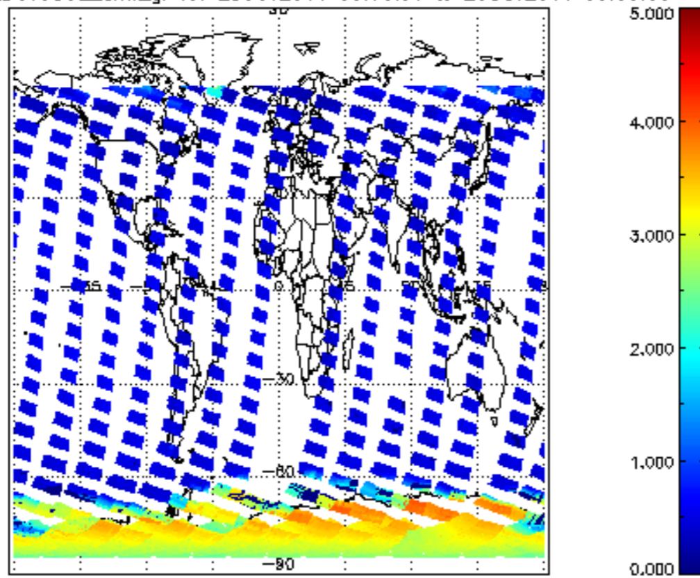
SCIOL2P_NADUV5S02_amf_gr for 28OCT2011 00:00:00 to 29OCT2011 00:00:00
