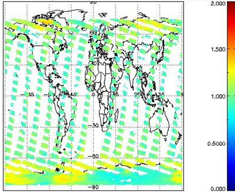
SCIOL2P_NADUV8H20_amf_gr for 28OCT2011 00:00:00 to 29OCT2011 00:00:00
