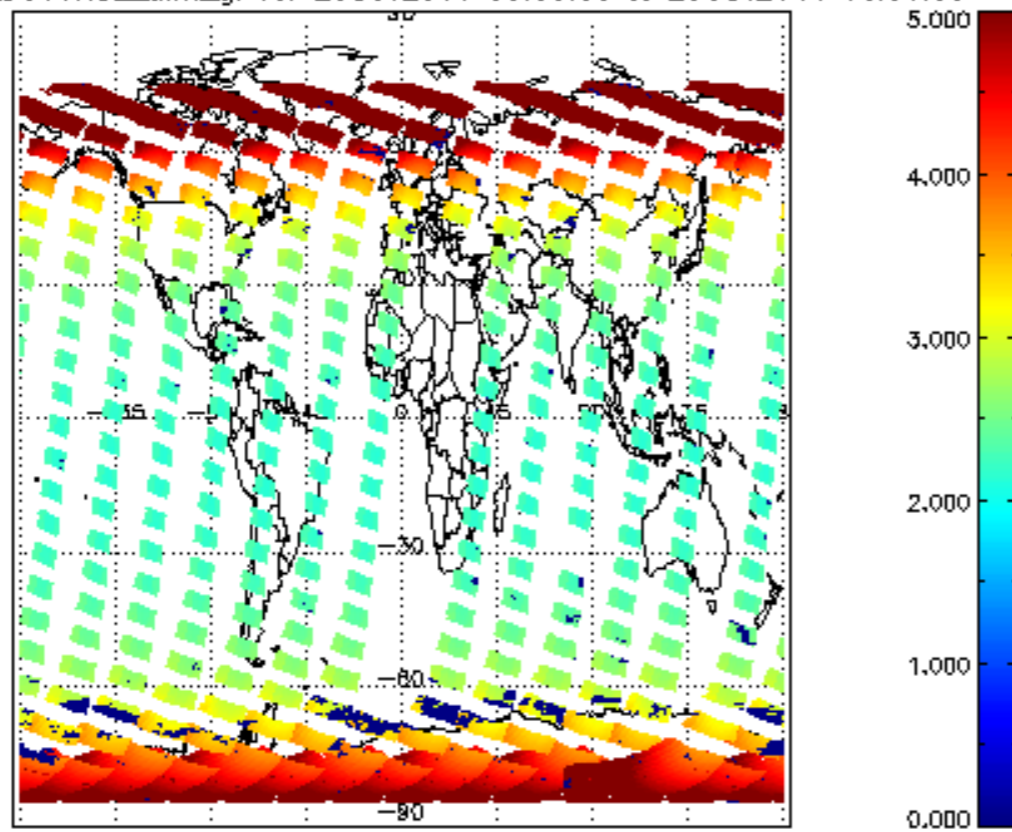
SCIOL2P_NADUV1NO2_amf_gr for 28OCT2011 00:00:00 to 29OCT2011 00:00:00
