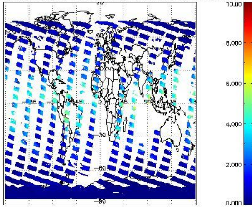
SCIOL2P_NADUV8H20_vcd for 28OCT2011 00:00:00 to 29OCT2011 00:00:00
