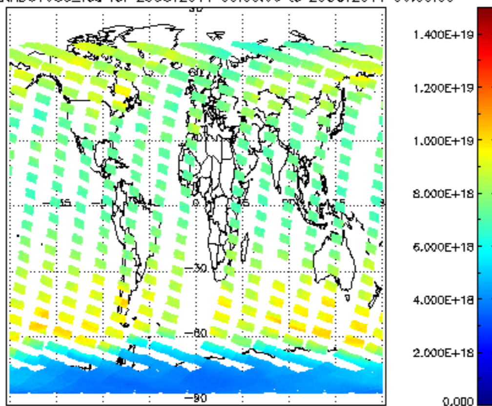
SCIOL2P_NADUV003_vcd for 28OCT2011 00:00:00 to 29OCT2011 00:00:00
