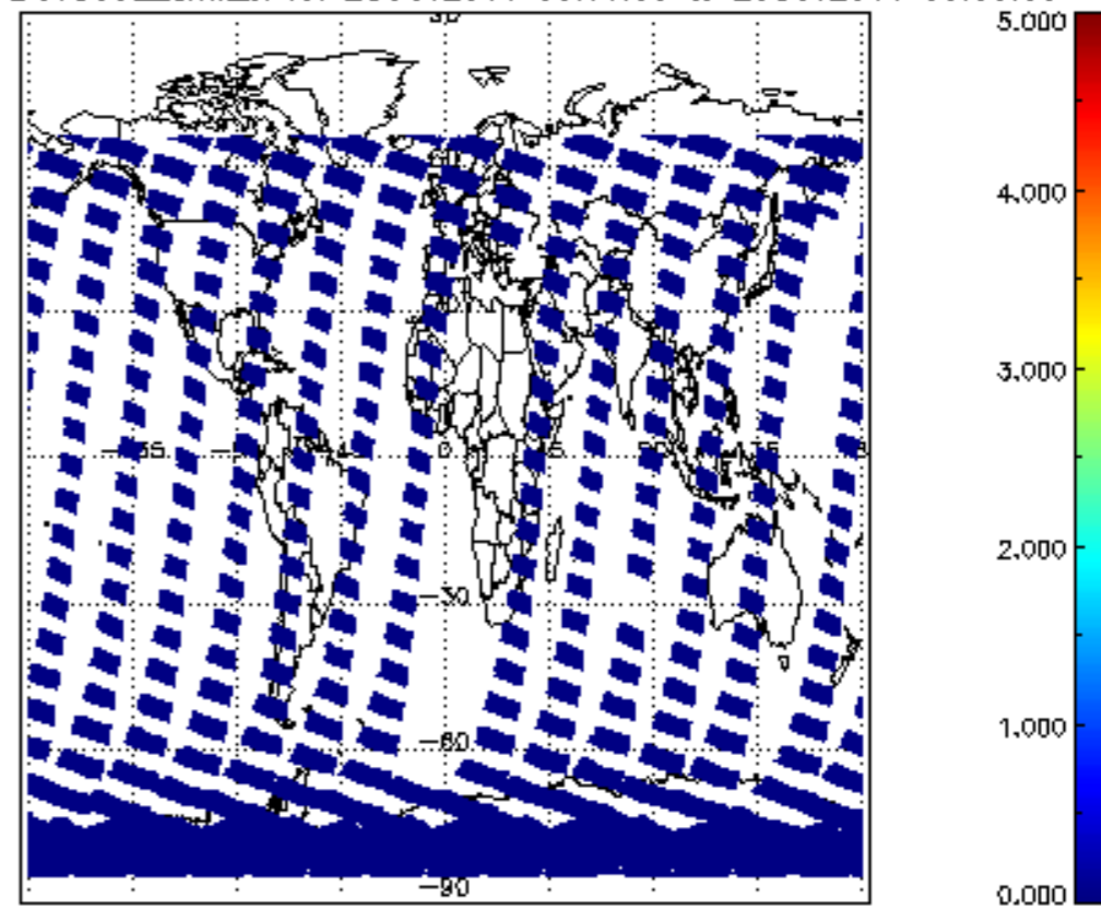
SCIOL2P_NADUV5S02_amf_cl for 28OCT2011 00:00:00 to 29OCT2011 00:00:00
