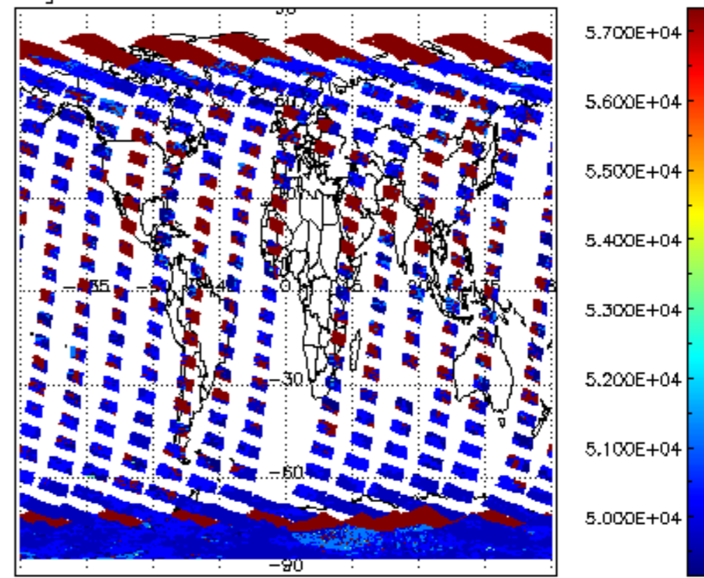
cloud_flags for 28OCT2011 00:00:00 to 29OCT2011 00:00:00
