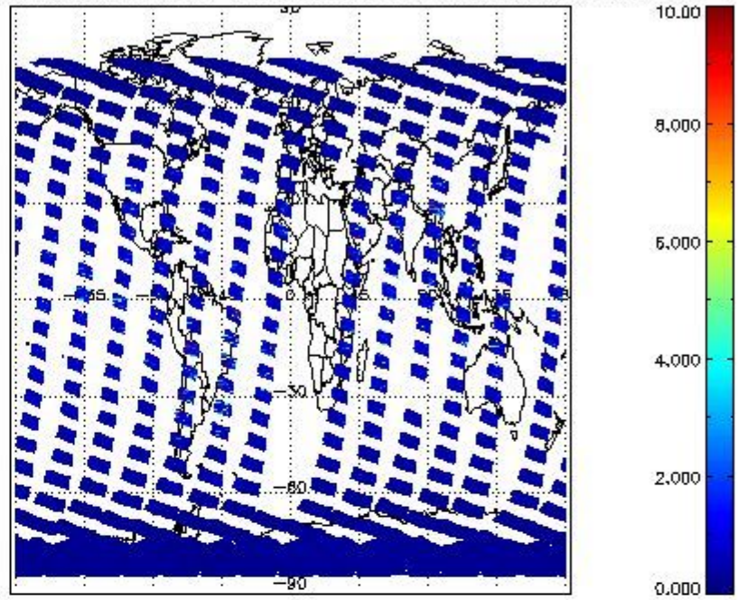
SCIOL2P_NADUV3BRO_vcd_err for 28OCT2011 00:00:00 to 29OCT2011 00:00:00
