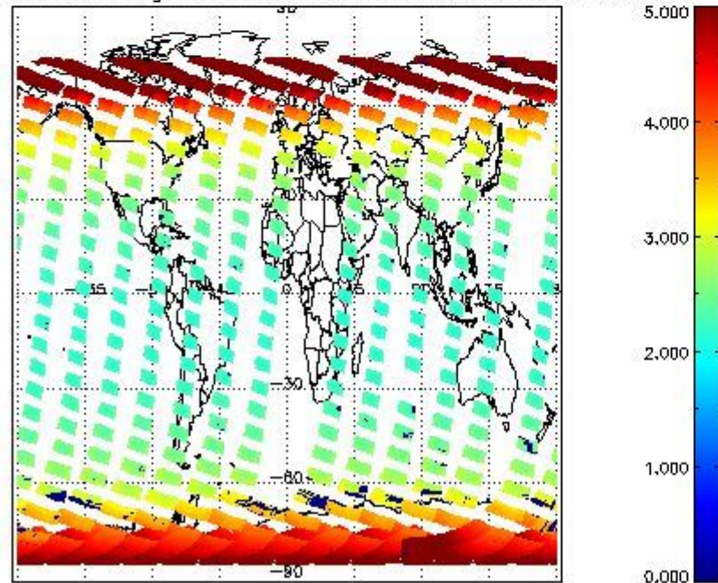
SCIOL2P_NADUV003_amf_gr for 28OCT2011 00:00:00 to 29OCT2011 00:00:00
