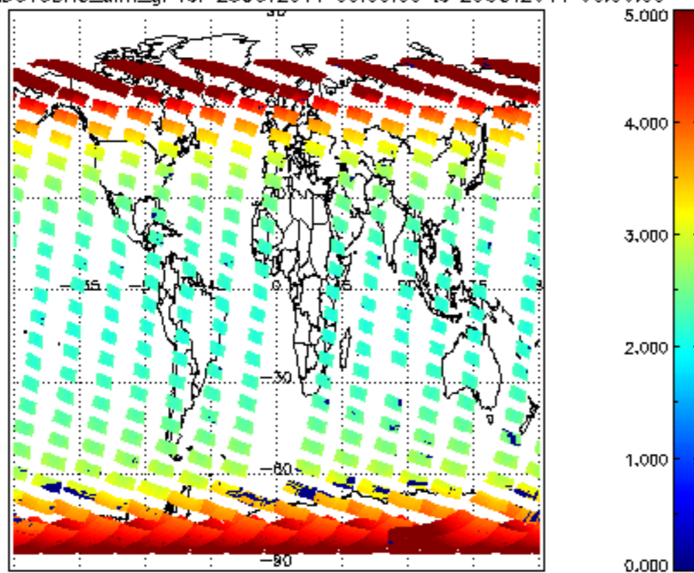
SCIOL2P_NADUV3BRO_amf_gr for 28OCT2011 00:00:00 to 29OCT2011 00:00:00
