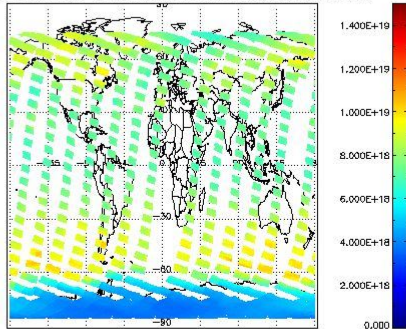
SCIOL2P_NADUV003_vcd for 28OCT2011 00:00:00 to 29OCT2011 00:00:00
