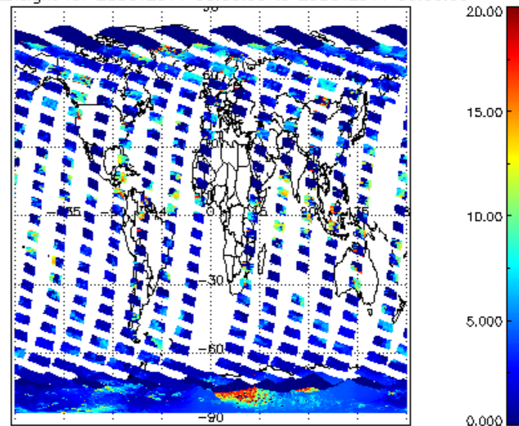
cl_top_height for 28OCT2011 00:00:00 to 29OCT2011 00:00:00
