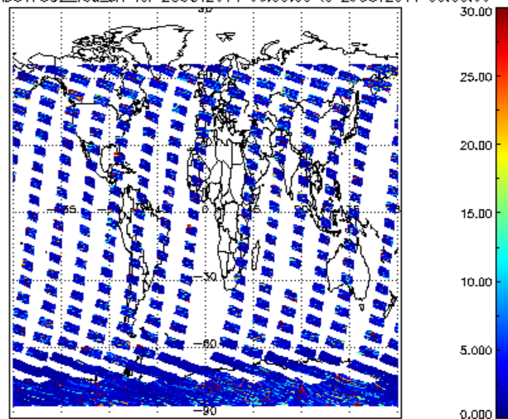
SCIOL2P_NADUV7S02_vcd_err for 28OCT2011 00:00:00 to 29OCT2011 00:00:00
