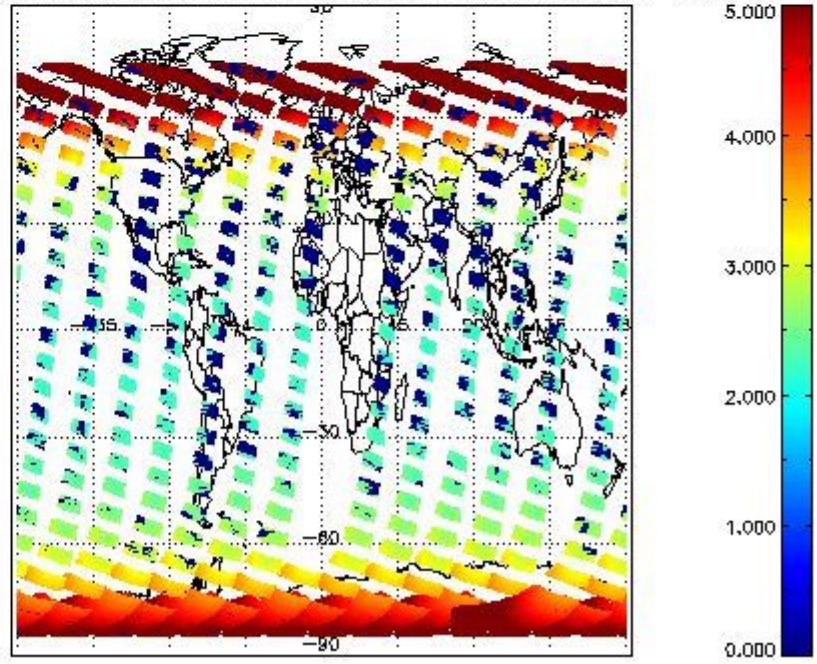
SCIOL2P_NADUV1NO2_amf_cl for 28OCT2011 00:00:00 to 29OCT2011 00:00:00
