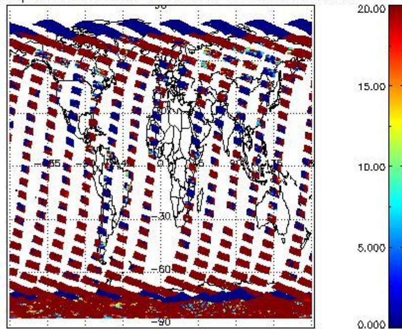
cL_opt_depth for 28OCT2011 00:00:00 to 29OCT2011 00:00:00
