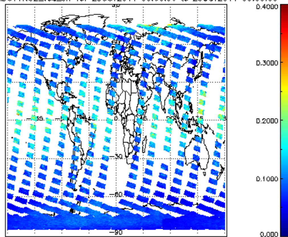
SCIOL2P_NADUV1NO2_vcd_err for 28OCT2011 00:00:00 to 29OCT2011 00:00:00
