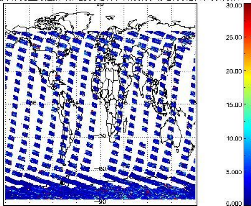
SCIOL2P_NADUV7S02_vcd_err for 28OCT2011 00:00:00 to 29OCT2011 00:00:00
