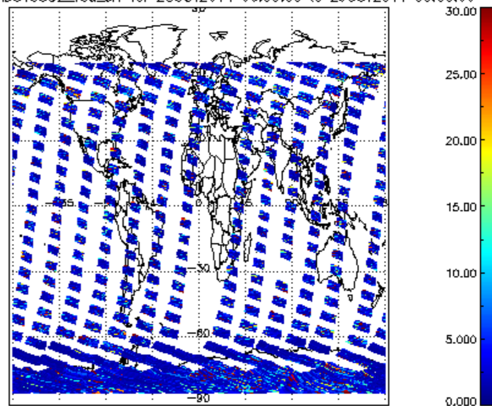
SCIOL2P_NADUV5S02_vcd_err for 28OCT2011 00:00:00 to 29OCT2011 00:00:00
