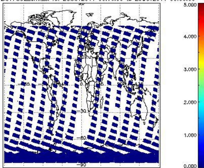
SCIOL2P_NADUV7S02_amf_cl for 28OCT2011 00:00:00 to 29OCT2011 00:00:00
