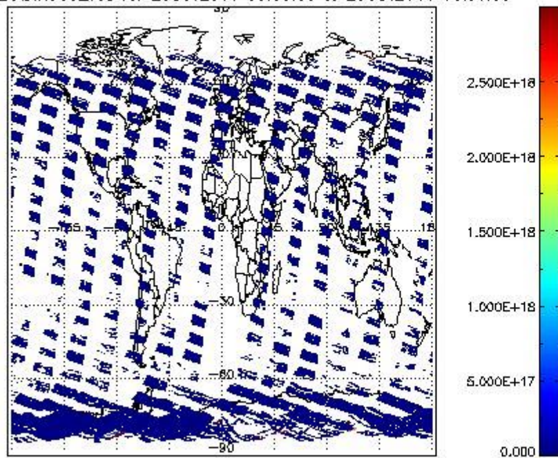
SCIDL2P_NADIR3CO_vcd for 28OCT2011 00:00:00 to 29OCT2011 00:00:00
