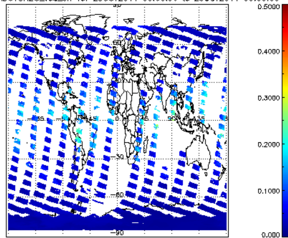
SCIOL2P_NADUV8H20_vcd_err for 28OCT2011 00:00:00 to 29OCT2011 00:00:00
