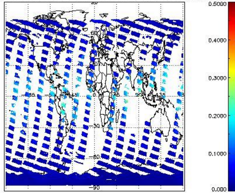
SCIOL2P_NADUV8H20_vcd_err for 28OCT2011 00:00:00 to 29OCT2011 00:00:00
