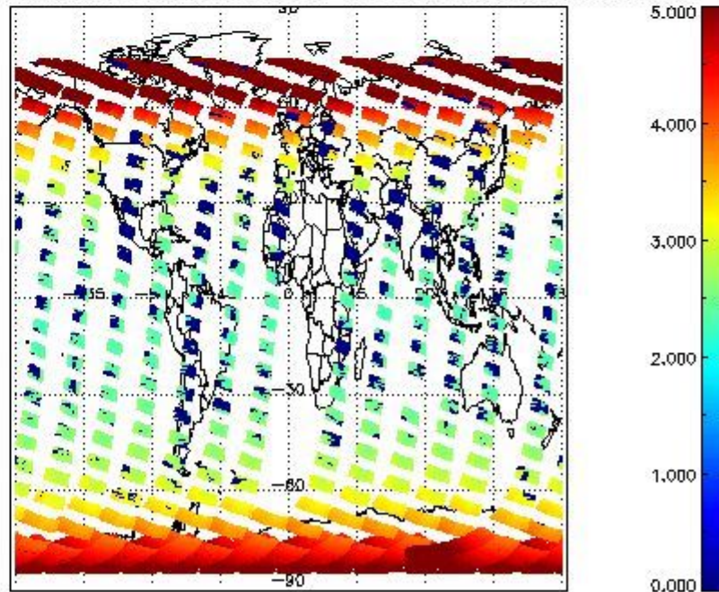
SCIOL2P_NADUV003_amf_cl for 28OCT2011 00:00:00 to 29OCT2011 00:00:00
