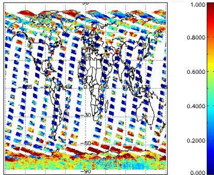
cLfrac for 28OCT2011 00:00:00 to 29OCT2011 00:00:00
