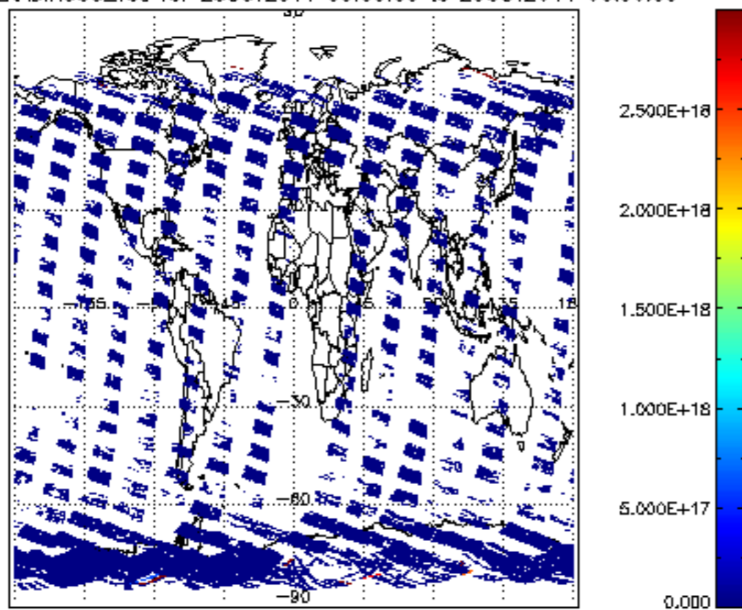
SCIOL2P_NADIR3CO_vcd for 28OCT2011 00:00:00 to 29OCT2011 00:00:00
