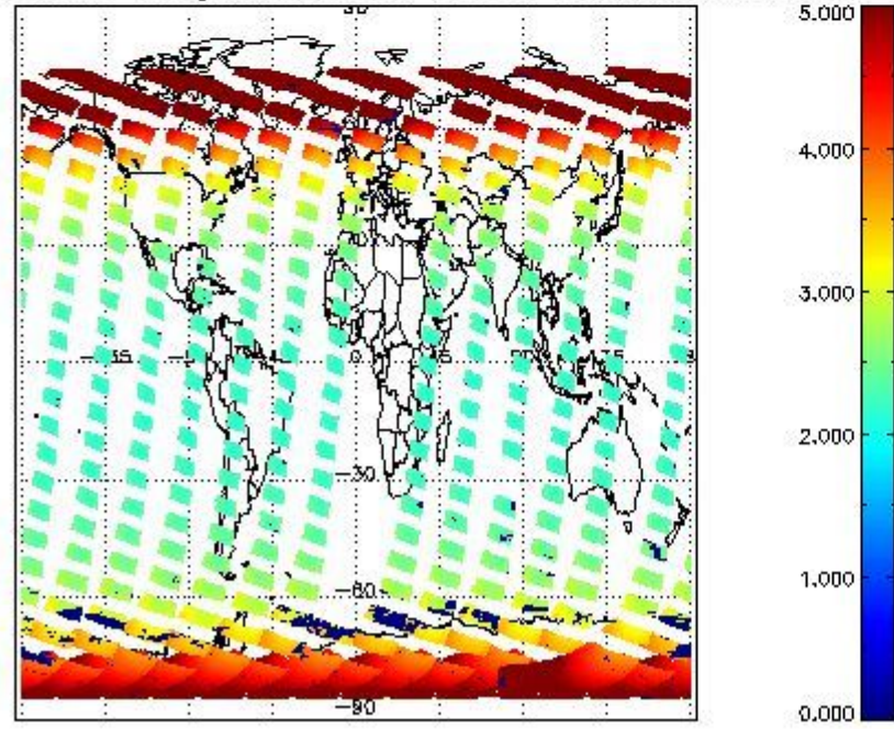
SCIOL2P_NADUV1NO2_amf_gr for 28OCT2011 00:00:00 to 29OCT2011 00:00:00
