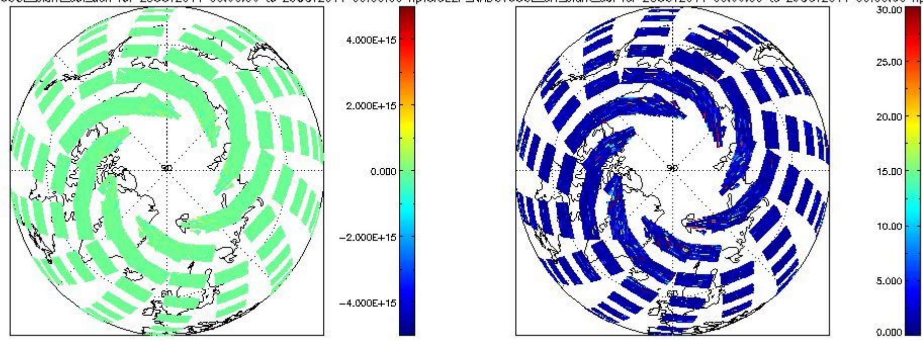
CIOL2P_NADUV60CL_slant_col_den for 28OCT2011 00:00:00 to 29OCT2011 00:00:00 np CIOL2P_NADUV60CL_err_slant_col for 28OCT2011 00:00:00 to 29OCT2011 00:00:00 np
