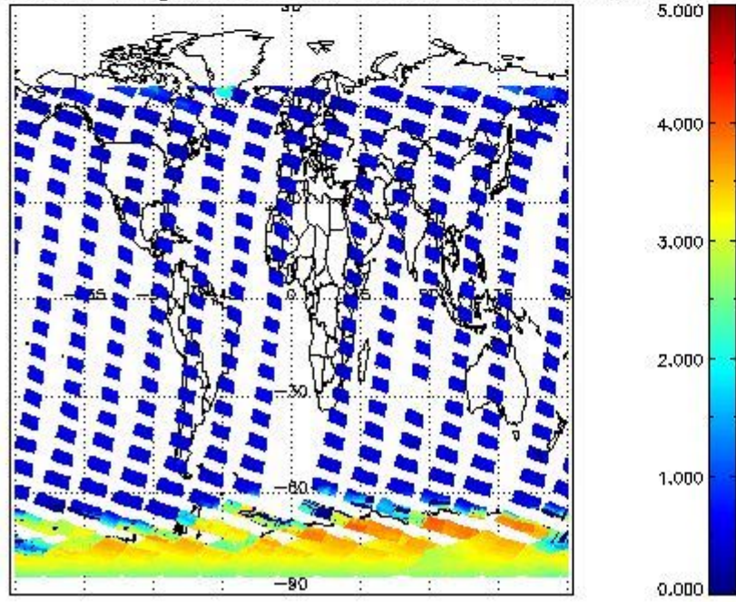
SCIOL2P_NADUV5SO2_amf_gr for 28OCT2011 00:00:00 to 29OCT2011 00:00:00
