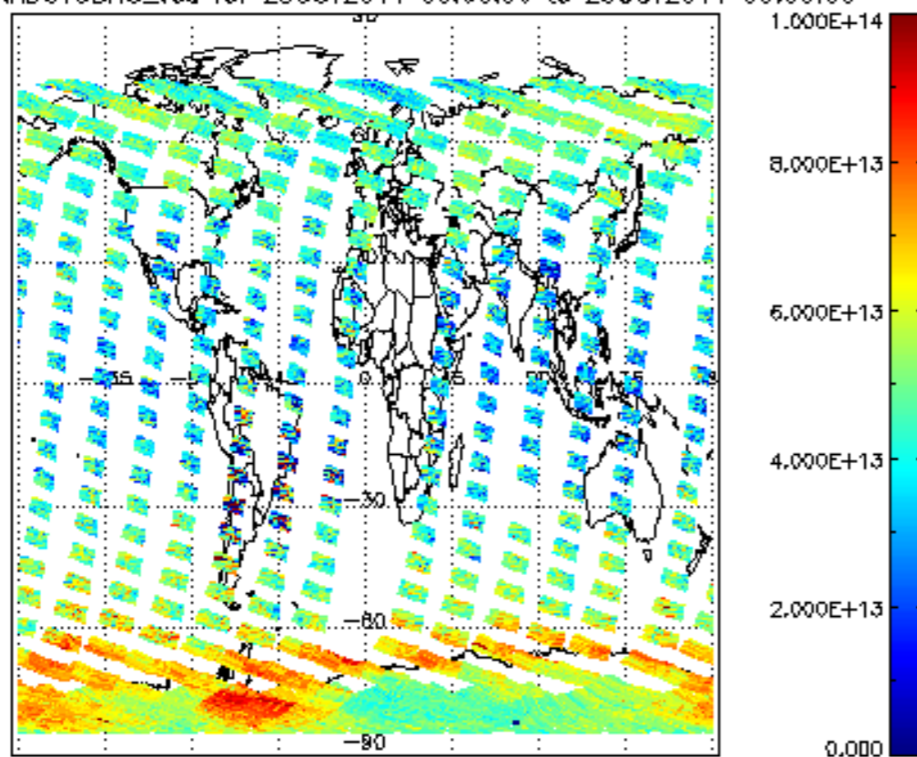
SCIOL2P_NADUV3BRO_vcd for 28OCT2011 00:00:00 to 29OCT2011 00:00:00
