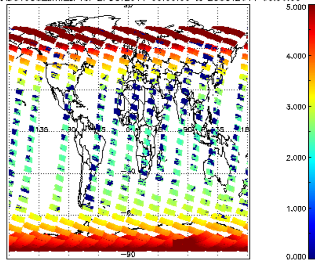
SCIOL2P_NADUV003_amf_cl for 27OCT2011 00:00:00 to 28OCT2011 00:00:00
