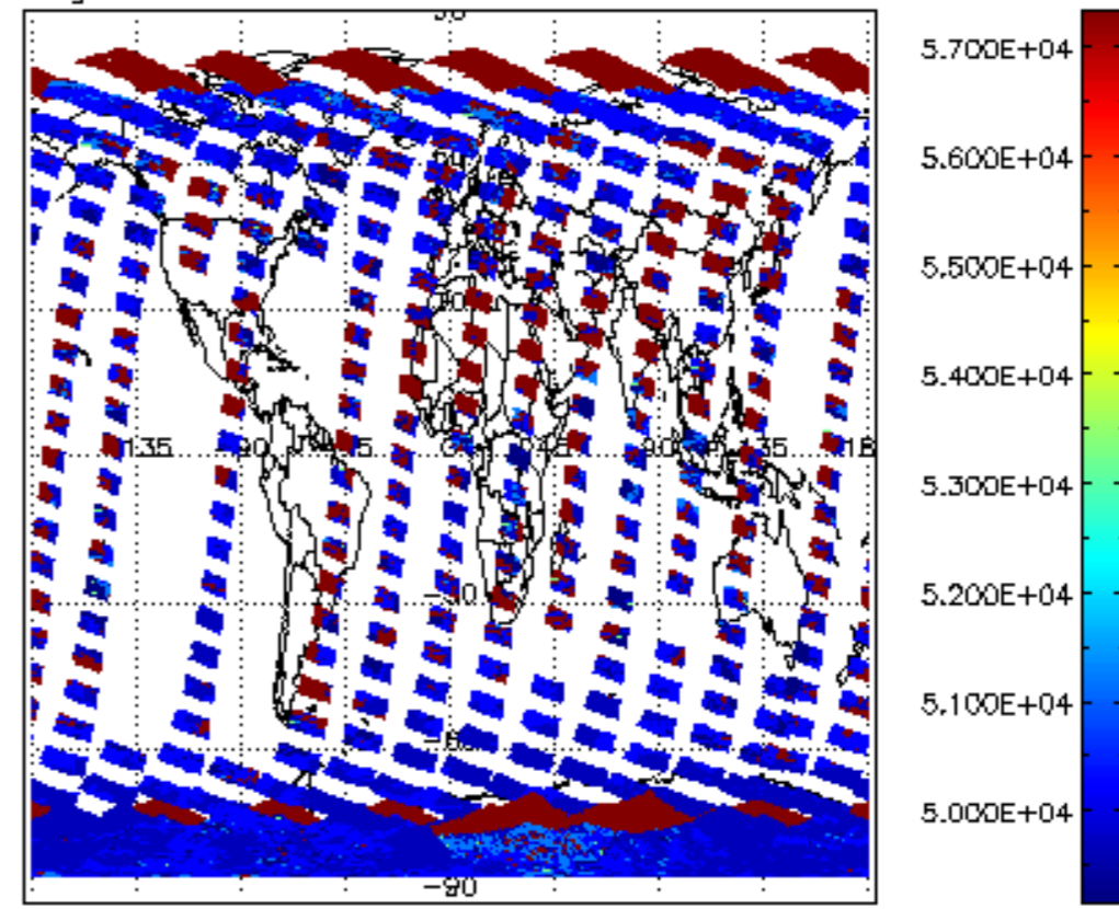
cloud_flags for 27OCT2011 00:00:00 to 28OCT2011 00:00:00
