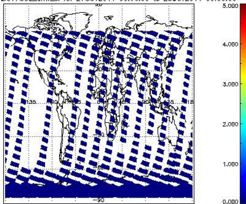
SCIOL2P_NADUV7S02_amf_cl for 27OCT2011 00:00:00 to 28OCT2011 00:00:00
