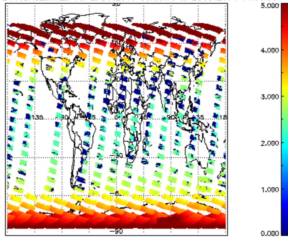
SCIOL2P_NADUV3BRO_amf_cl for 27OCT2011 00:00:00 to 28OCT2011 00:00:00
