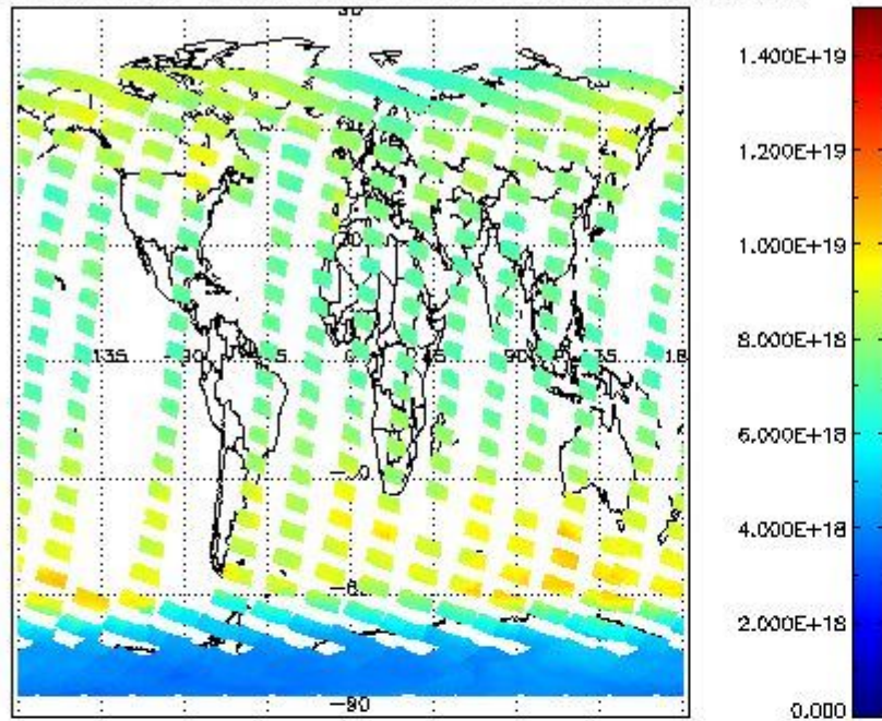
SCIOL2P_NADUV003_vcd for 27OCT2011 00:00:00 to 28OCT2011 00:00:00
