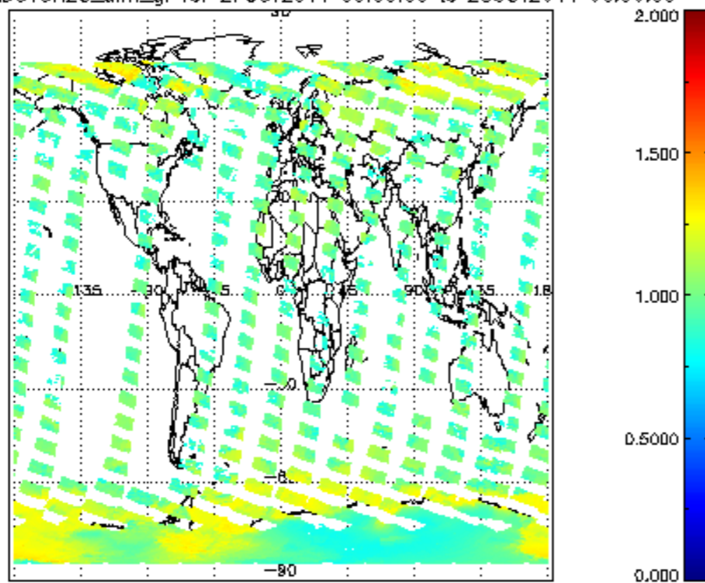
SCIOL2P_NADUV8H20_amf_gr for 27OCT2011 00:00:00 to 28OCT2011 00:00:00
