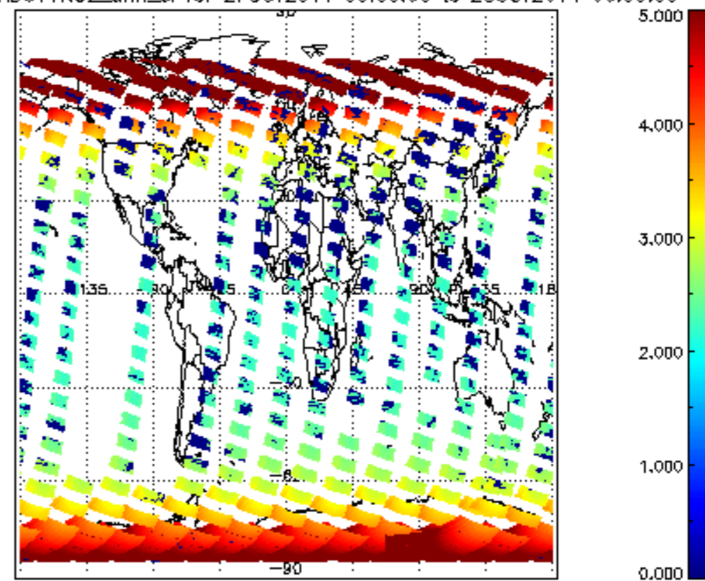
SCIOL2P_NADUV1NO2_amf_cl for 27OCT2011 00:00:00 to 28OCT2011 00:00:00
