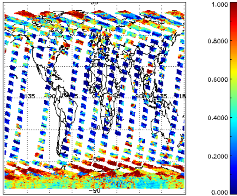
cl_frac for 27OCT2011 00:00:00 to 28OCT2011 00:00:00
