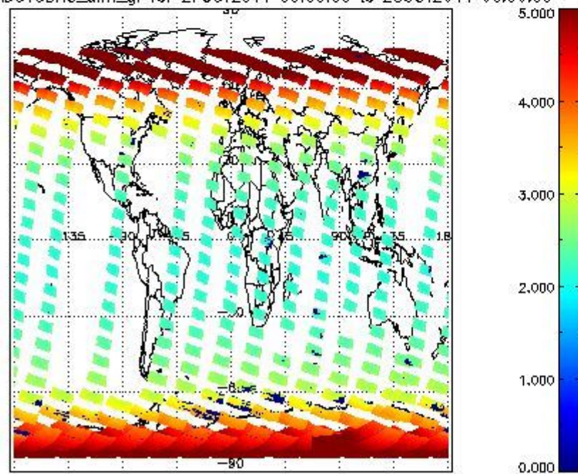
SCIOL2P_NADUV3BRO_amf_gr for 27OCT2011 00:00:00 to 28OCT2011 00:00:00
