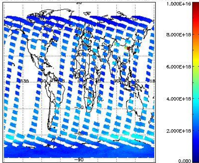
SCIOL2P_NADUV1NO2_vcd for 27OCT2011 00:00:00 to 28OCT2011 00:00:00
