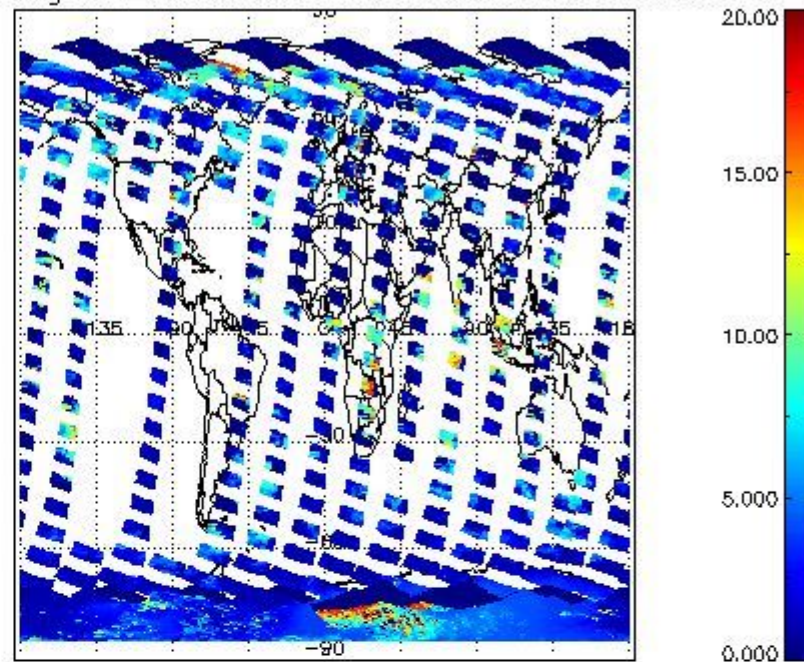
cL_top_height for 27OCT2011 00:00:00 to 28OCT2011 00:00:00
