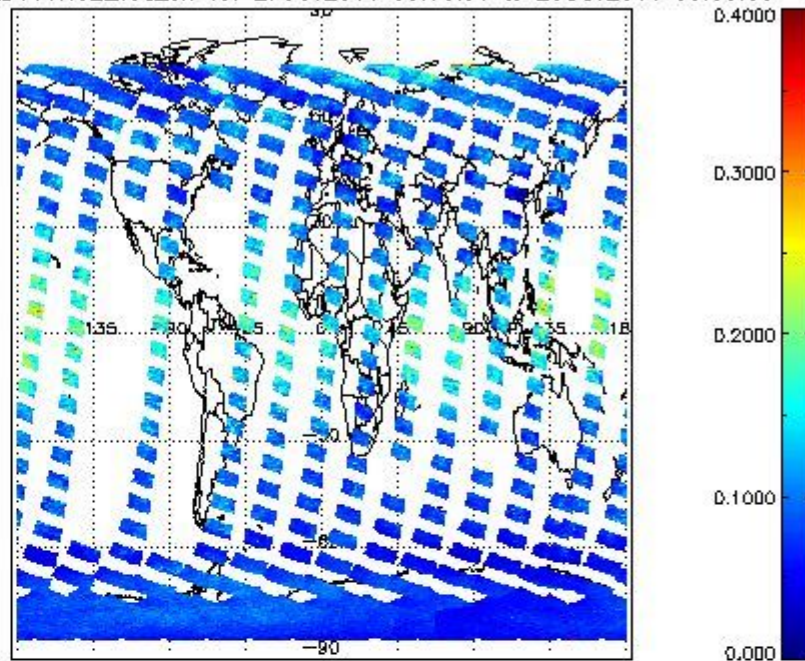
SCIOL2P_NADUV1NO2_vcd_err for 27OCT2011 00:00:00 to 28OCT2011 00:00:00
