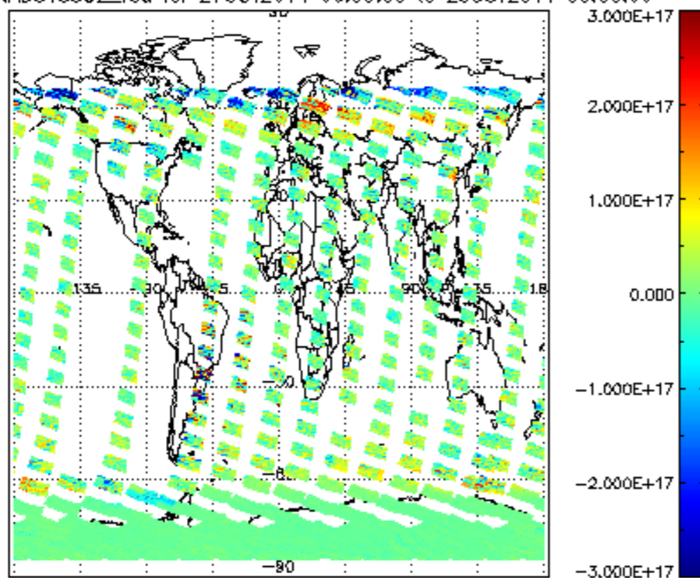
SCIOL2P_NADUV5S02_vcd for 27OCT2011 00:00:00 to 28OCT2011 00:00:00
