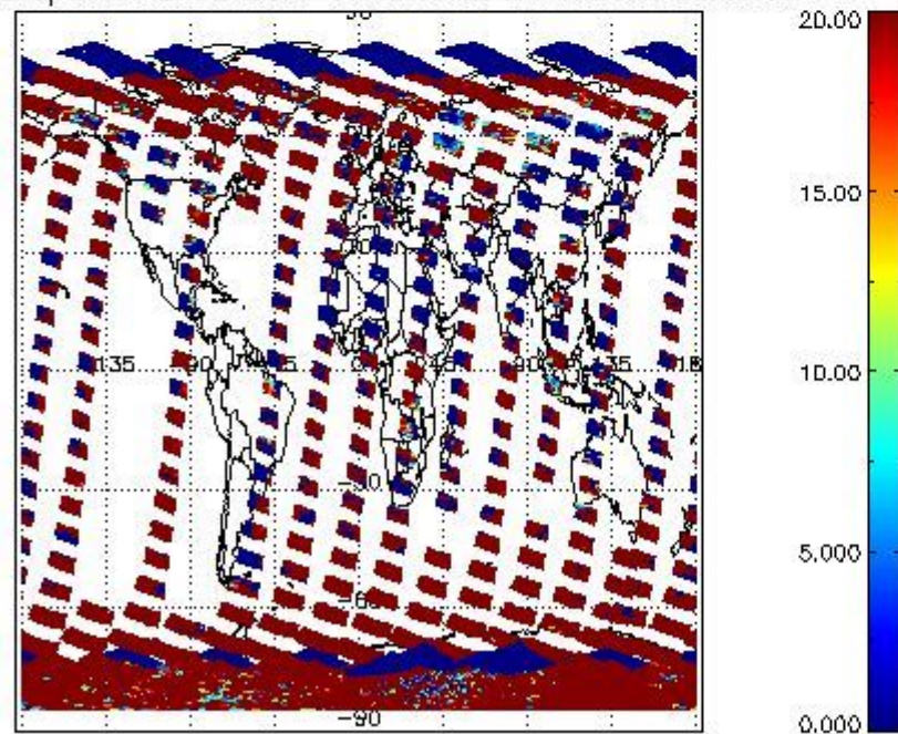
cL_opt_depth for 27OCT2011 00:00:00 to 28OCT2011 00:00:00
