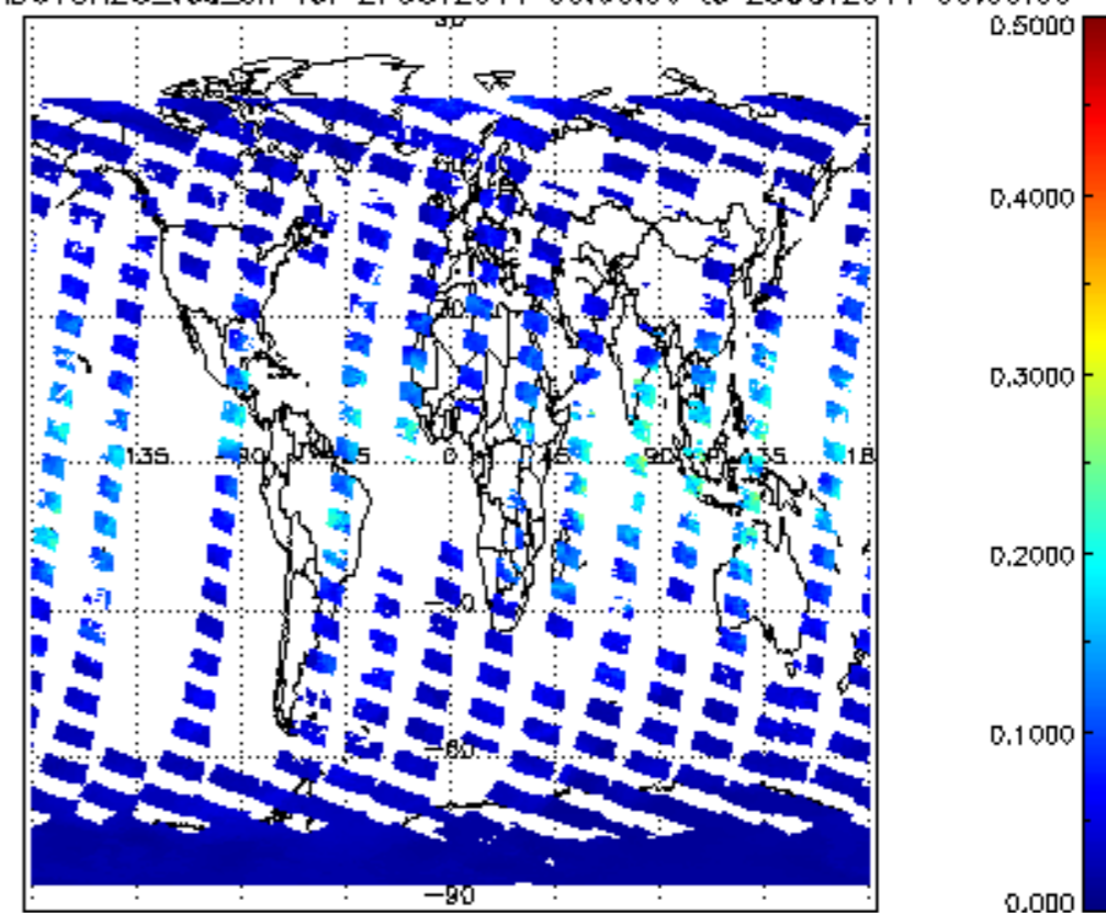
SCIOL2P_NADUV8H20_vcd_err for 27OCT2011 00:00:00 to 28OCT2011 00:00:00
