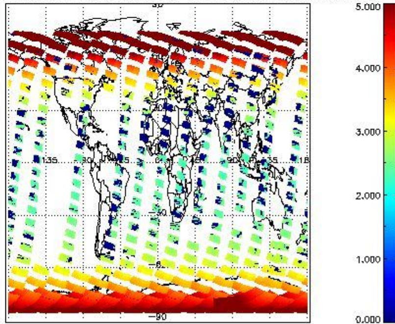
SCIOL2P_NADUV003_amf_cl for 27OCT2011 00:00:00 to 28OCT2011 00:00:00
