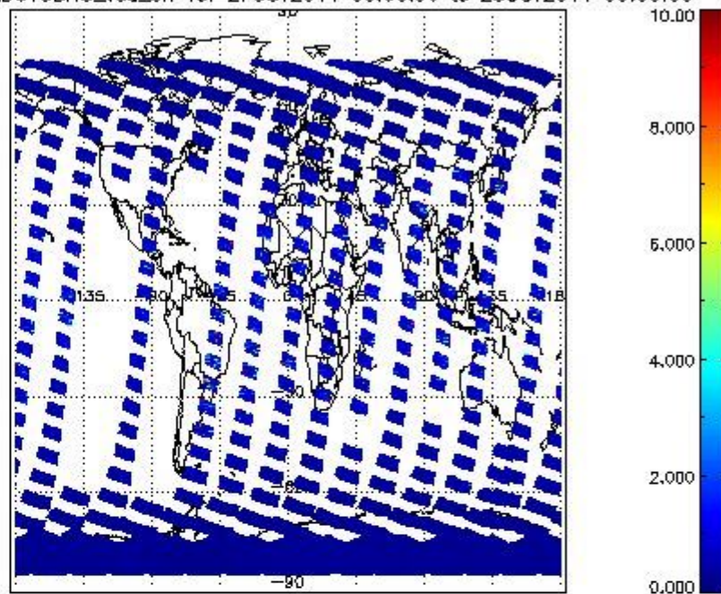
SCIOL2P_NADUV3BRO_vcd_err for 27OCT2011 00:00:00 to 28OCT2011 00:00:00
