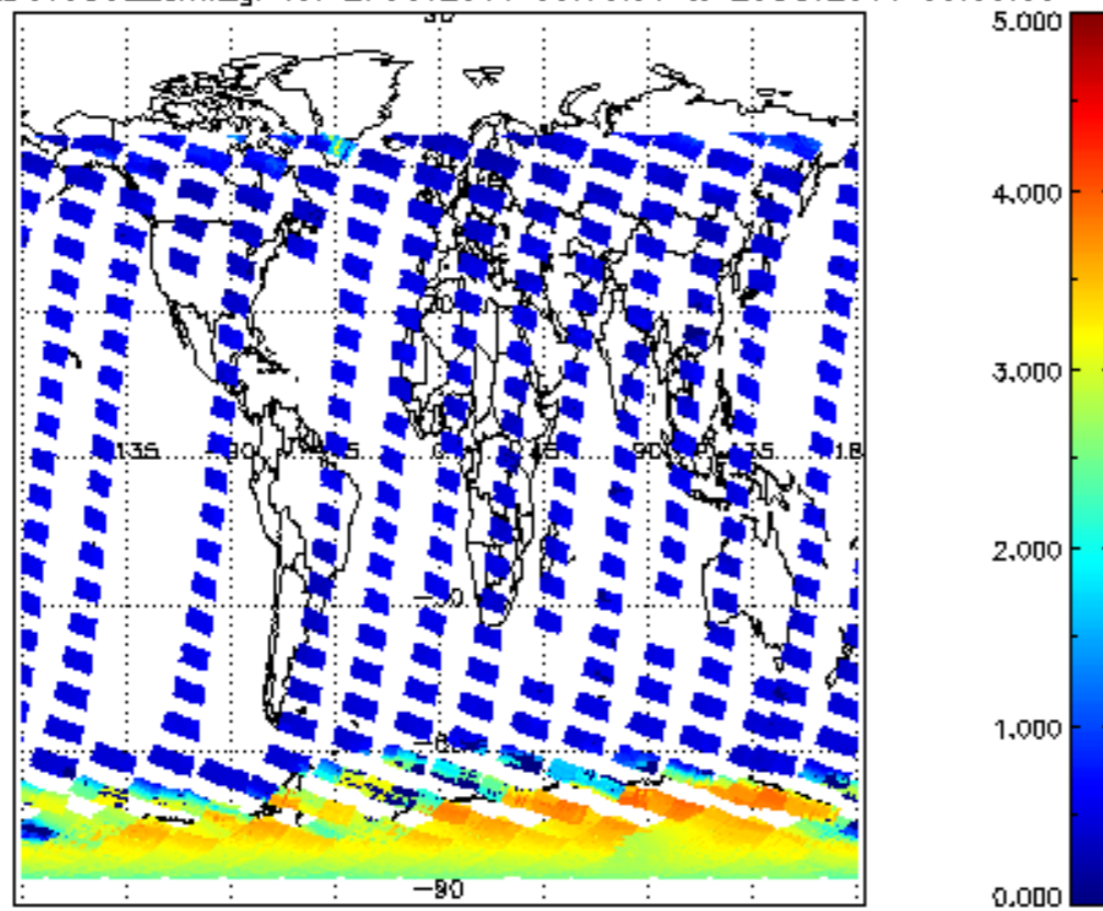
SCIOL2P_NADUV5S02_amf_gr for 27OCT2011 00:00:00 to 28OCT2011 00:00:00
