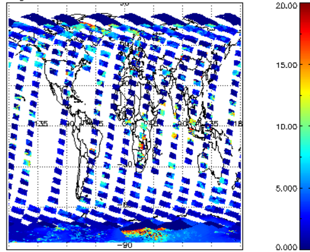
cl_top_height for 27OCT2011 00:00:00 to 28OCT2011 00:00:00
