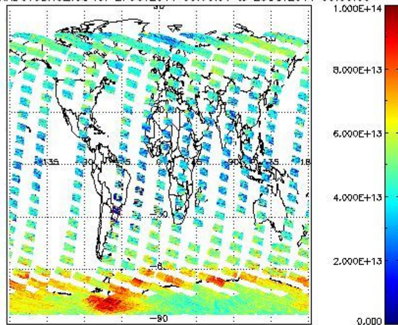
SCIOL2P_NADUV3BRO_vcd for 27OCT2011 00:00:00 to 28OCT2011 00:00:00
