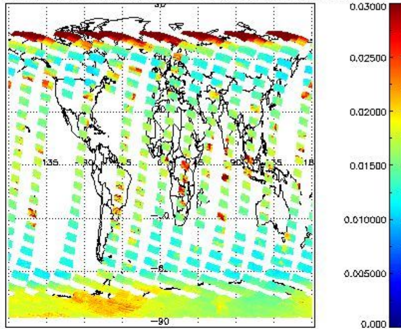
SCIOL2P_NADUV003_vcd_err for 27OCT2011 00:00:00 to 28OCT2011 00:00:00
