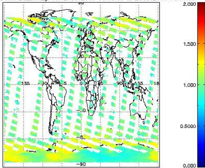
SCIOL2P_NADUV8H20_amf_gr for 27OCT2011 00:00:00 to 28OCT2011 00:00:00
