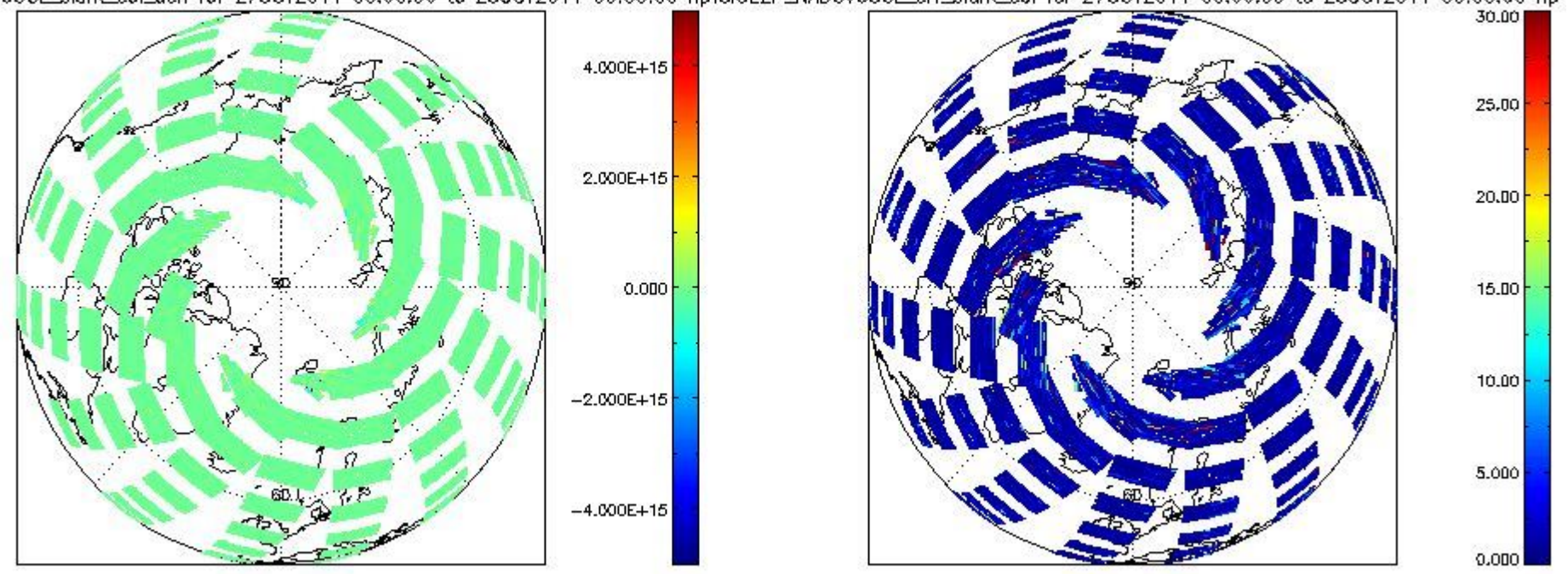
CIOL2P_NADUV60CL_slant_col_den for 27OCT2011 00:00:00 to 28OCT2011 00:00:00 np CIOL2P_NADUV60CL_err_slant_col for 27OCT2011 00:00:00 to 28OCT2011 00:00:00 np
