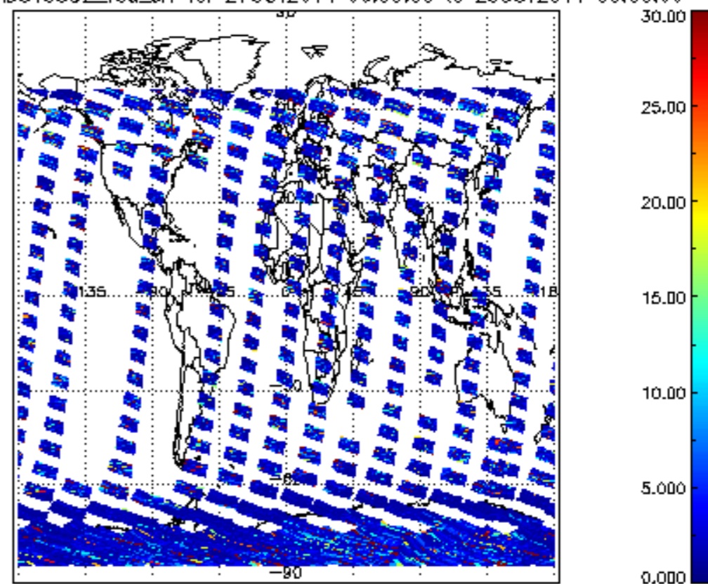
SCIOL2P_NADUV5S02_vcd_err for 27OCT2011 00:00:00 to 28OCT2011 00:00:00
