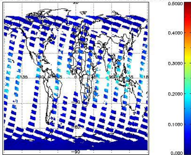
SCIOL2P_NADUV8H20_vcd_err for 27OCT2011 00:00:00 to 28OCT2011 00:00:00
