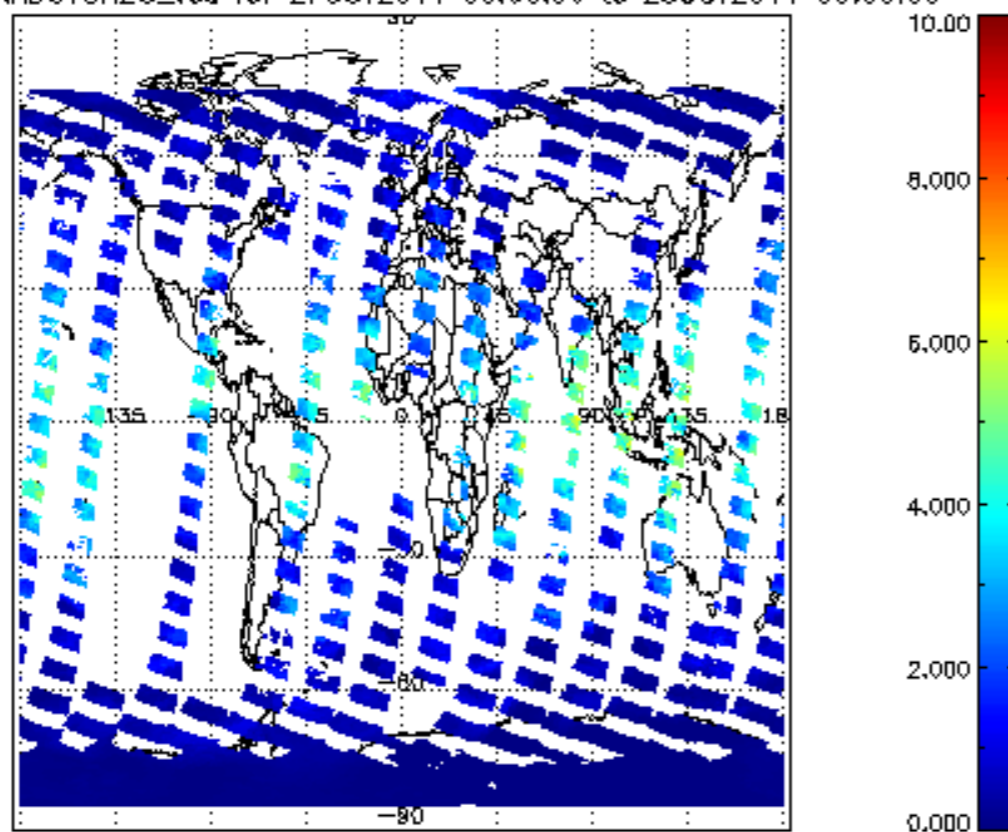
SCIOL2P_NADUV8H20_vcd for 27OCT2011 00:00:00 to 28OCT2011 00:00:00
