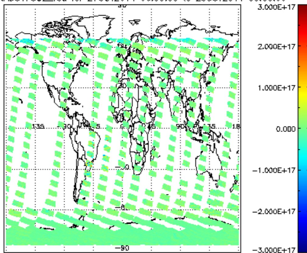
SCIOL2P_NADUV7S02_vcd for 27OCT2011 00:00:00 to 28OCT2011 00:00:00
