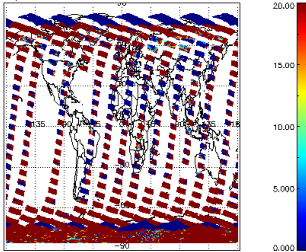
cl_opt_depth for 27OCT2011 00:00:00 to 28OCT2011 00:00:00
