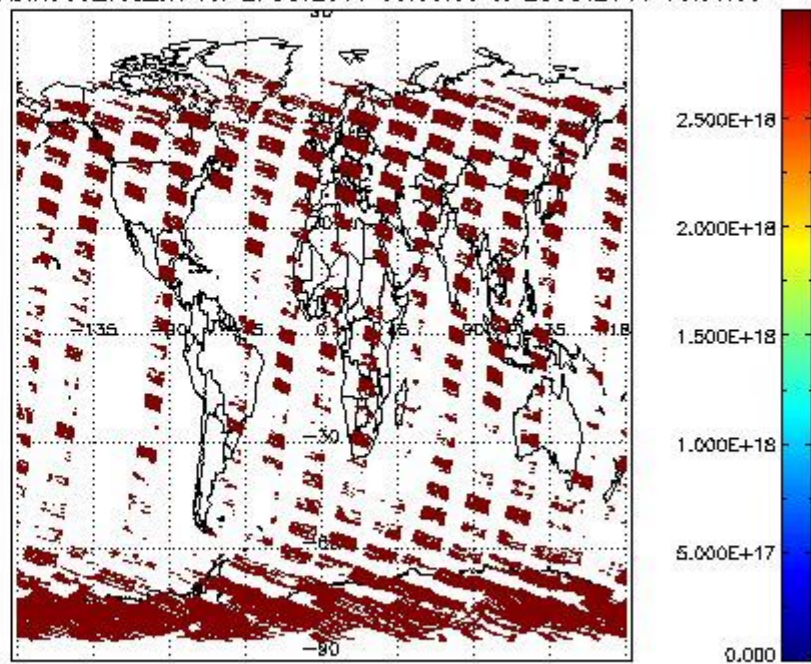
SCIDL2P_NADIR3CO_vcd_err for 27OCT2011 00:00:00 to 28OCT2011 00:00:00
