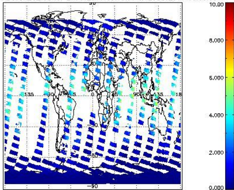
SCIOL2P_NADUV8H20_vcd for 27OCT2011 00:00:00 to 28OCT2011 00:00:00
