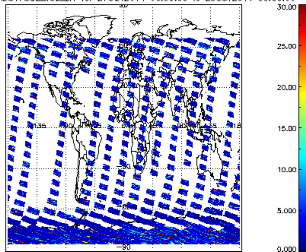
SCIOL2P_NADUV7S02_vcd_err for 27OCT2011 00:00:00 to 28OCT2011 00:00:00
