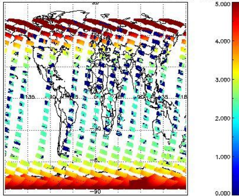
SCIOL2P_NADUV1NO2_amf_cl for 27OCT2011 00:00:00 to 28OCT2011 00:00:00
