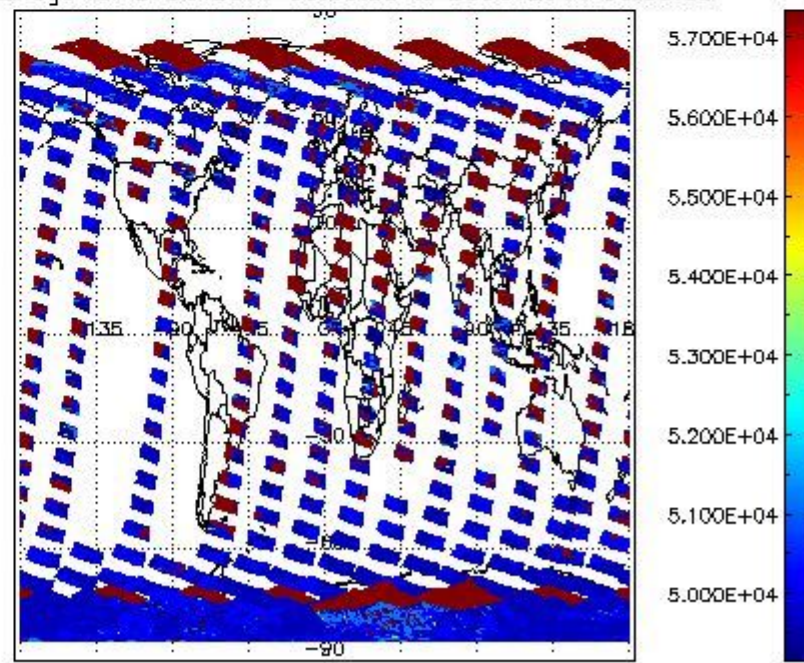
cloud_flags for 27OCT2011 00:00:00 to 28OCT2011 00:00:00
