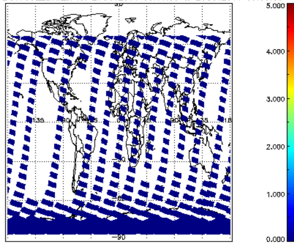
SCIOL2P_NADUV7S02_amf_sl for 27OCT2011 00:00:00 to 28OCT2011 00:00:00
