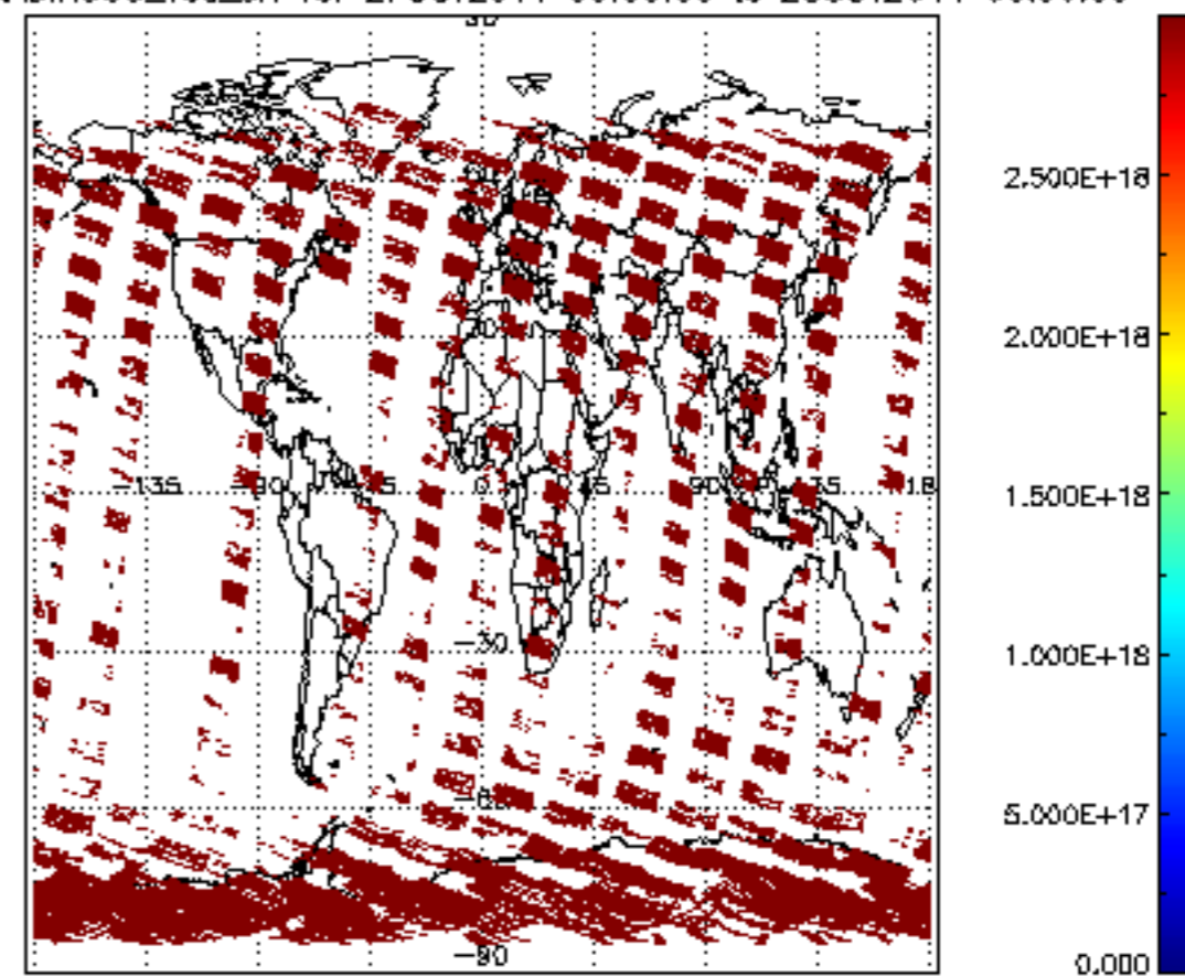
SCIOL2P_NADIR3CO_vcd_err for 27OCT2011 00:00:00 to 28OCT2011 00:00:00
