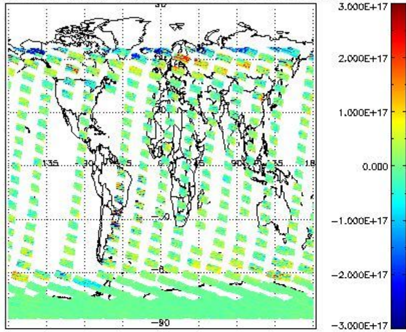
SCIOL2P_NADUV5S02_vcd for 27OCT2011 00:00:00 to 28OCT2011 00:00:00
