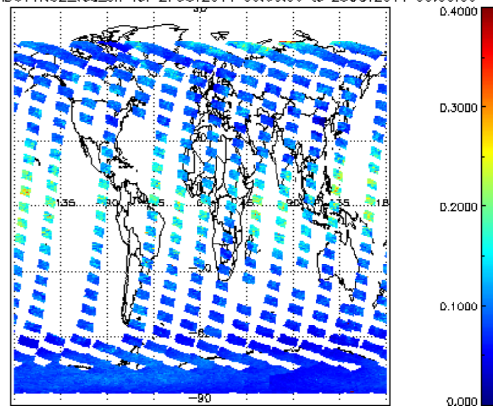
SCIOL2P_NADUV1NO2_vcd_err for 27OCT2011 00:00:00 to 28OCT2011 00:00:00
