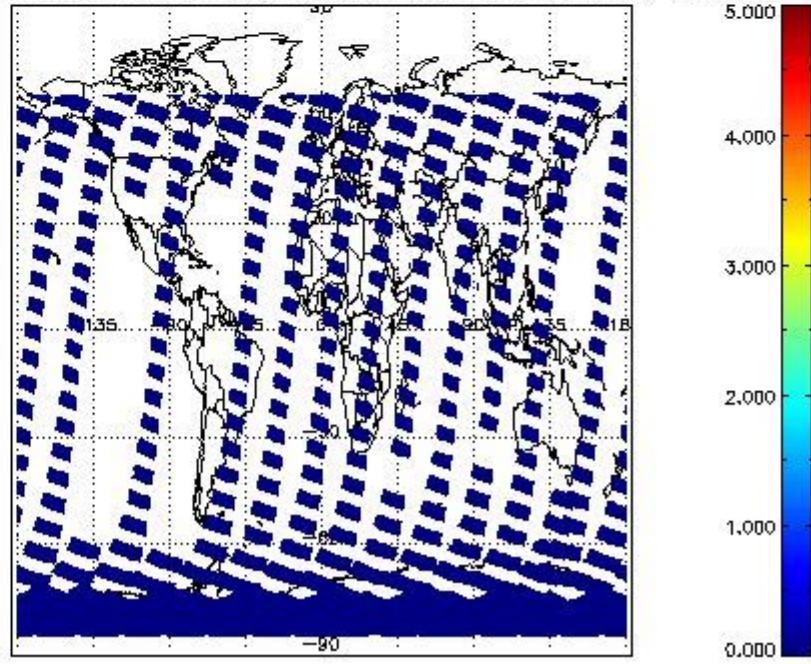
SCIOL2P_NADUV5S02_amf_cl for 27OCT2011 00:00:00 to 28OCT2011 00:00:00
