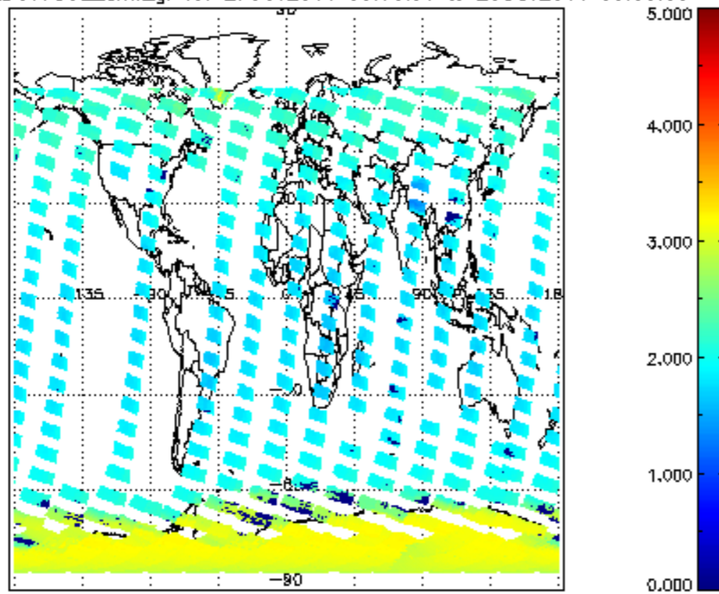
SCIOL2P_NADUV7S02_amf_gr for 27OCT2011 00:00:00 to 28OCT2011 00:00:00
