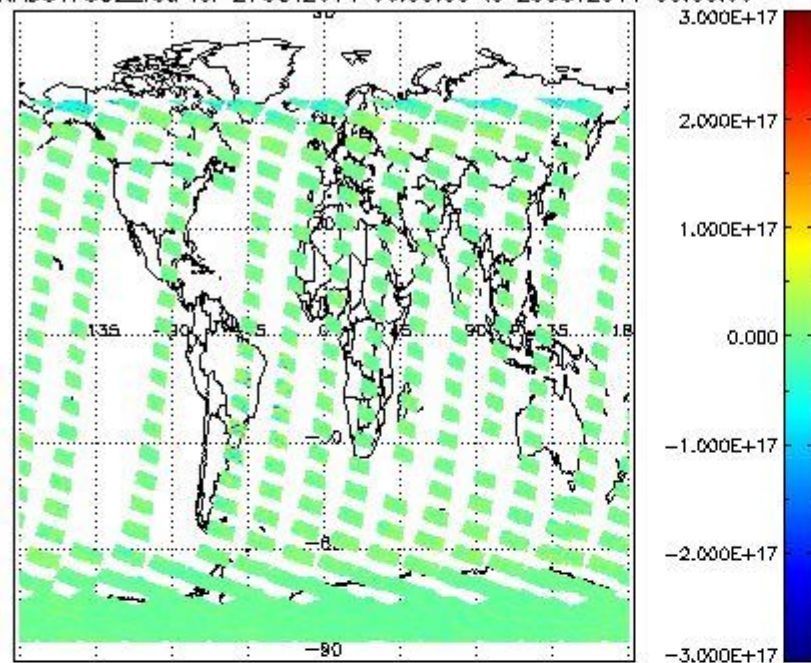
SCIOL2P_NADUV7S02_vcd for 27OCT2011 00:00:00 to 28OCT2011 00:00:00
