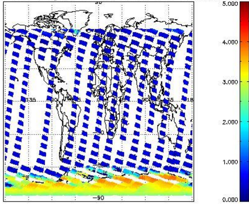
SCIOL2P_NADUV5S02_amf_gr for 27OCT2011 00:00:00 to 28OCT2011 00:00:00
