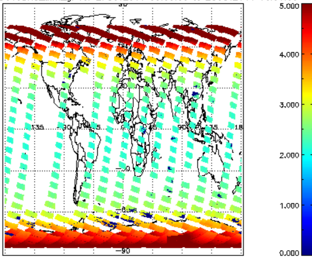
SCIOL2P_NADUV3BRO_amf_gr for 27OCT2011 00:00:00 to 28OCT2011 00:00:00
