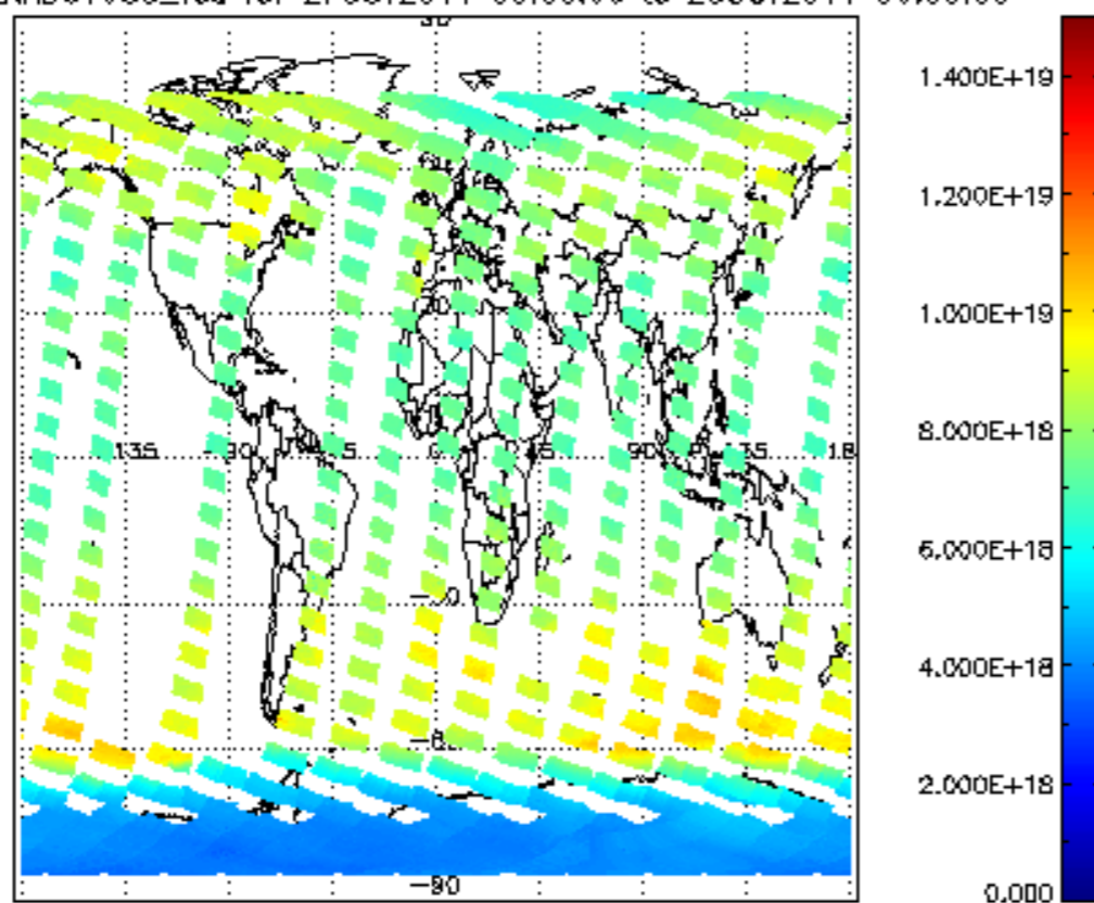
SCIOL2P_NADUV003_vcd for 27OCT2011 00:00:00 to 28OCT2011 00:00:00
