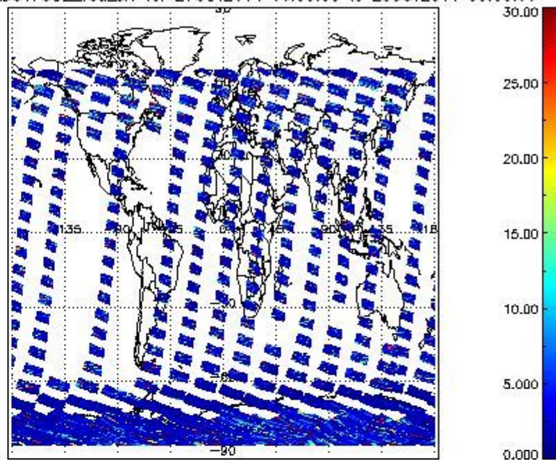
SCIOL2P_NADUV7S02_vcd_err for 27OCT2011 00:00:00 to 28OCT2011 00:00:00
