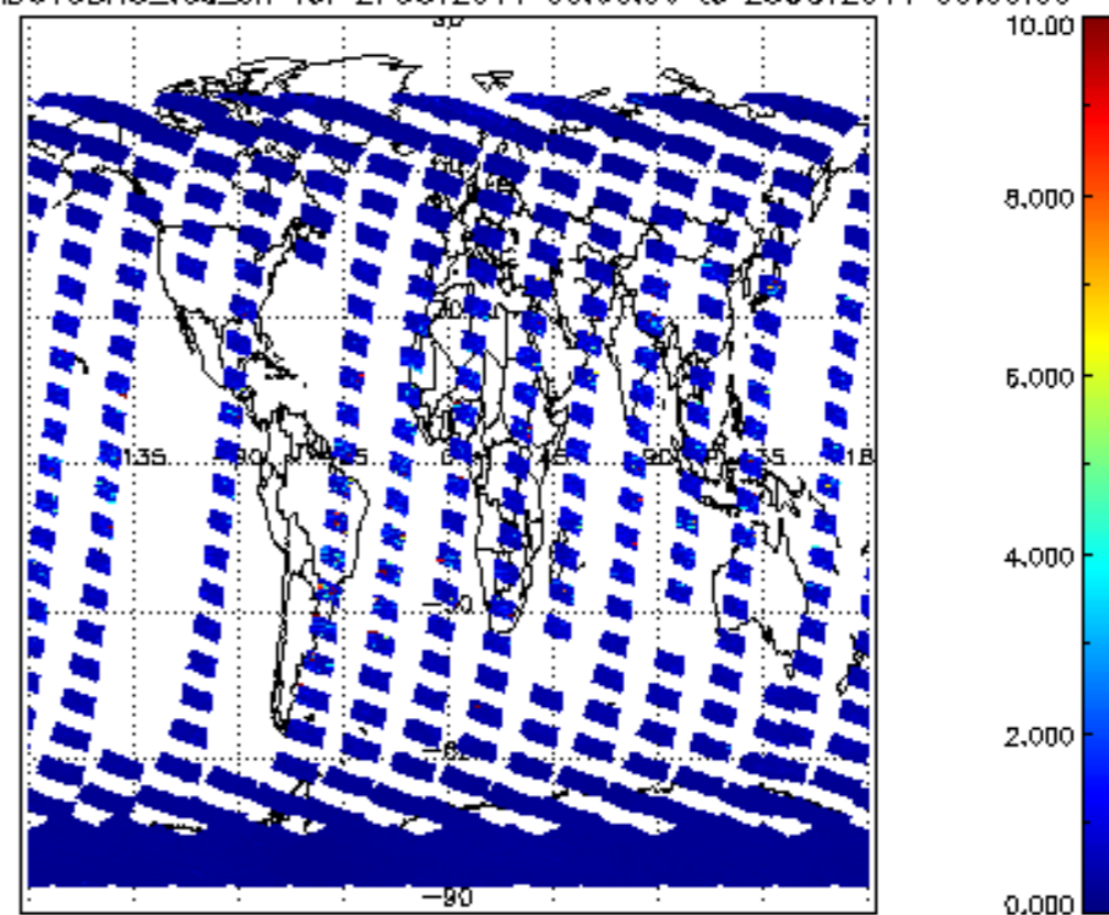
SCIOL2P_NADUV3BRO_vcd_err for 27OCT2011 00:00:00 to 28OCT2011 00:00:00
