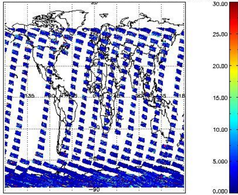
SCIOL2P_NADUV5S02_vcd_err for 27OCT2011 00:00:00 to 28OCT2011 00:00:00
