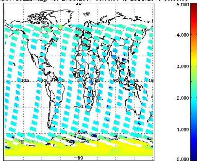
SCIOL2P_NADUV7S02_amf_gr for 27OCT2011 00:00:00 to 28OCT2011 00:00:00
