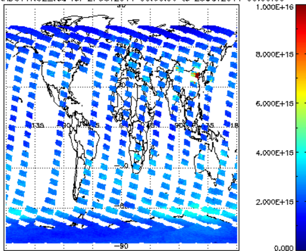
SCIOL2P_NADUV1NO2_vcd for 27OCT2011 00:00:00 to 28OCT2011 00:00:00
