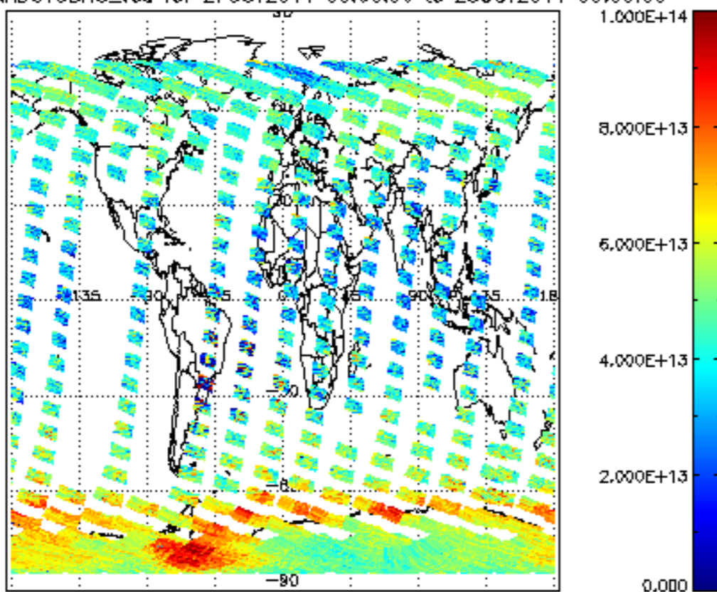
SCIOL2P_NADUV3BRO_vcd for 27OCT2011 00:00:00 to 28OCT2011 00:00:00
