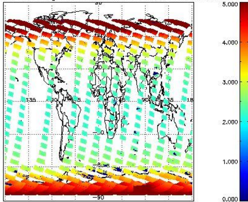
SCIOL2P_NADUV003_amf_gr for 27OCT2011 00:00:00 to 28OCT2011 00:00:00
