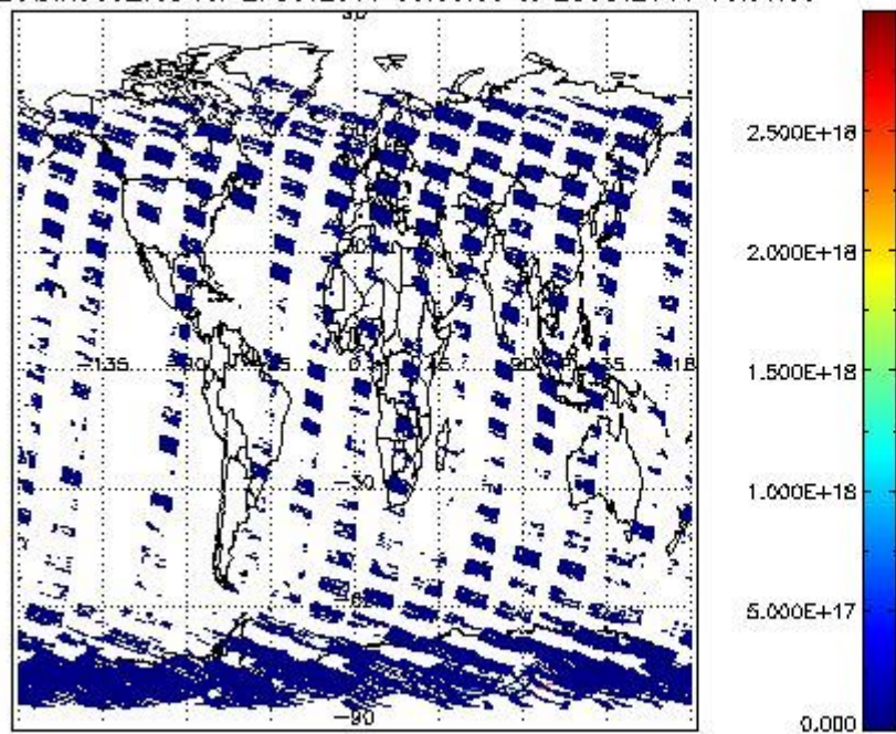
SCIDL2P_NADIR3CO_vcd for 27OCT2011 00:00:00 to 28OCT2011 00:00:00
