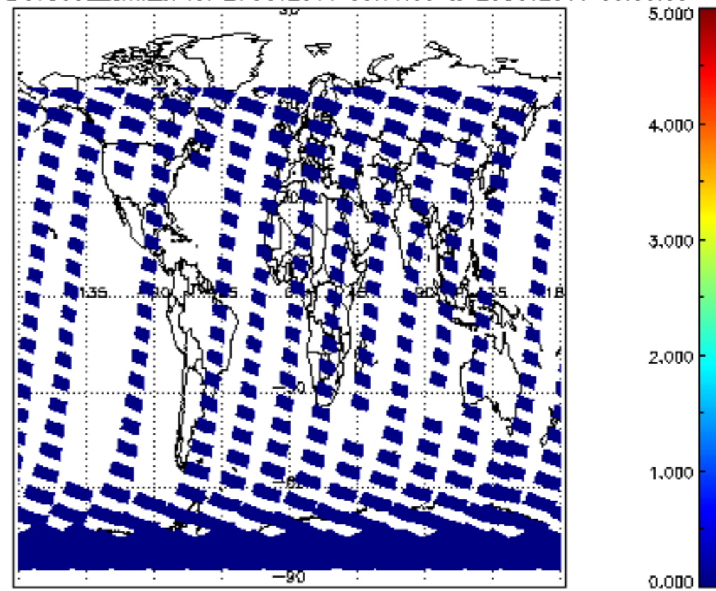
SCIOL2P_NADUV5S02_amf_sl for 27OCT2011 00:00:00 to 28OCT2011 00:00:00
