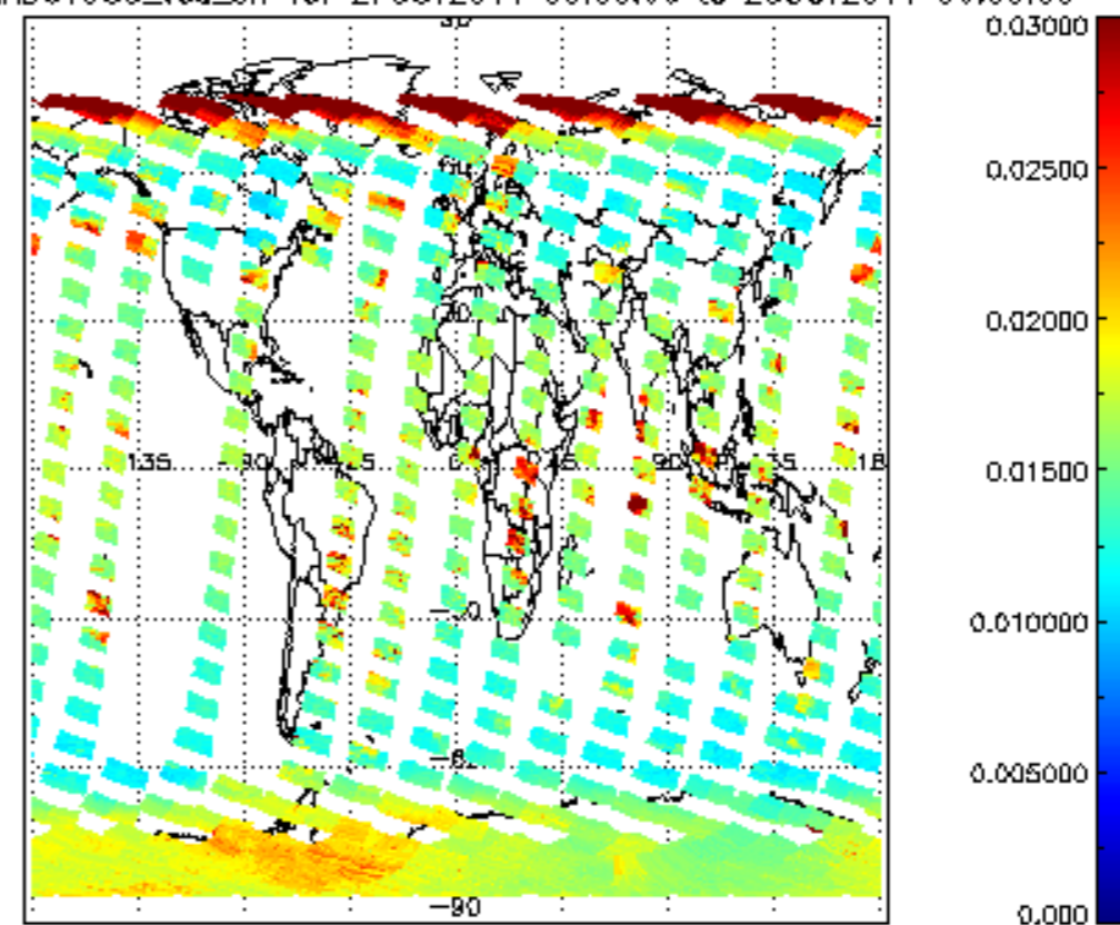
SCIOL2P_NADUV003_vcd_err for 27OCT2011 00:00:00 to 28OCT2011 00:00:00
