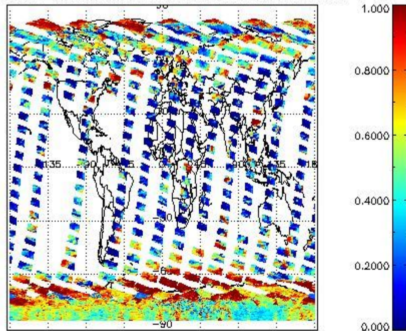
cLfrac for 27OCT2011 00:00:00 to 28OCT2011 00:00:00
