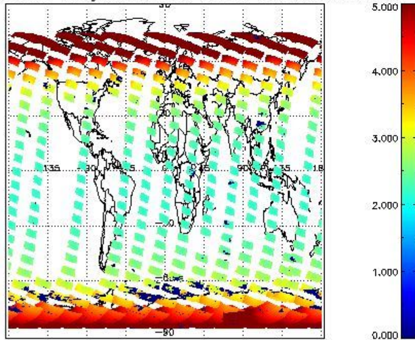
SCIOL2P_NADUV1NO2_amf_gr for 27OCT2011 00:00:00 to 28OCT2011 00:00:00
