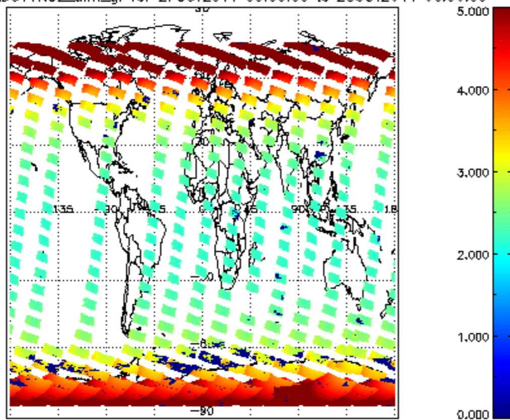
SCIOL2P_NADUV1NO2_amf_gr for 27OCT2011 00:00:00 to 28OCT2011 00:00:00
