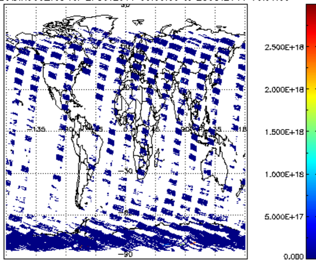
SCIOL2P_NADIR3CO_vcd for 27OCT2011 00:00:00 to 28OCT2011 00:00:00
