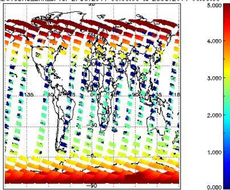
SCIOL2P_NADUV3BRO_amf_cl for 27OCT2011 00:00:00 to 28OCT2011 00:00:00
