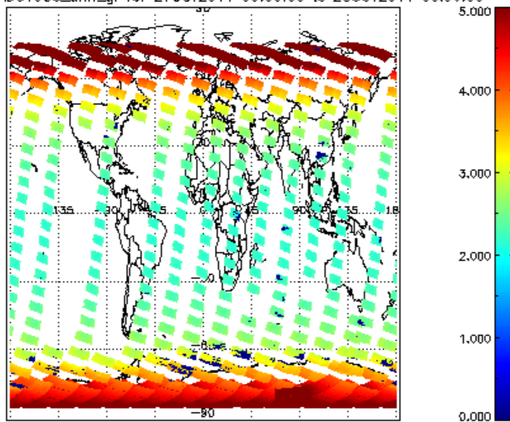
SCIOL2P_NADUV003_amf_gr for 27OCT2011 00:00:00 to 28OCT2011 00:00:00
