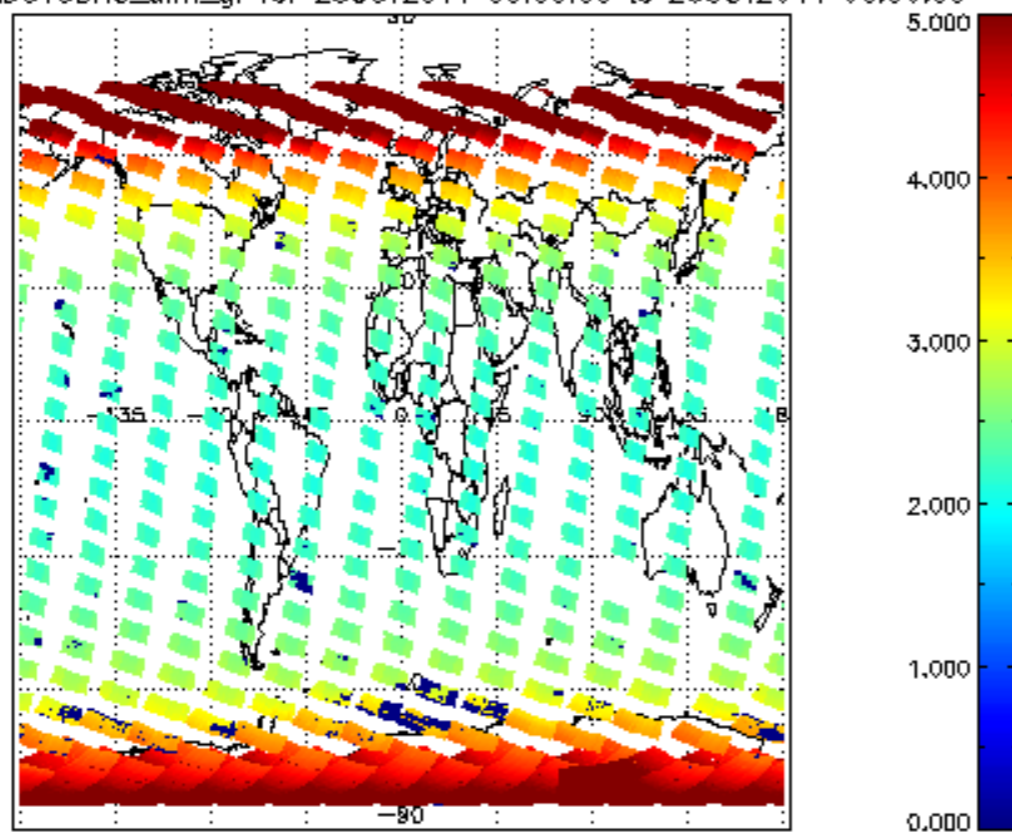
SCIOL2P_NADUV3BRO_amf_gr for 25OCT2011 00:00:00 to 26OCT2011 00:00:00
