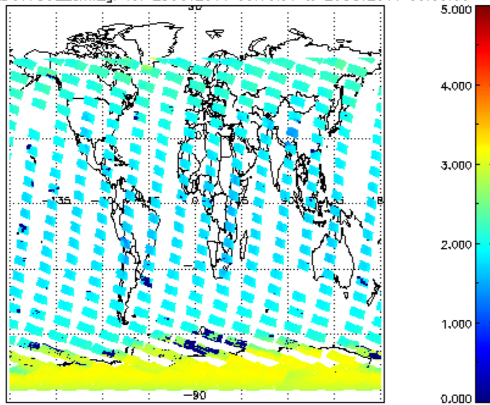
SCIOL2P_NADUV7S02_amf_gr for 25OCT2011 00:00:00 to 26OCT2011 00:00:00
