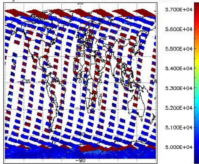
cloud_flags for 25OCT2011 00:00:00 to 26OCT2011 00:00:00
