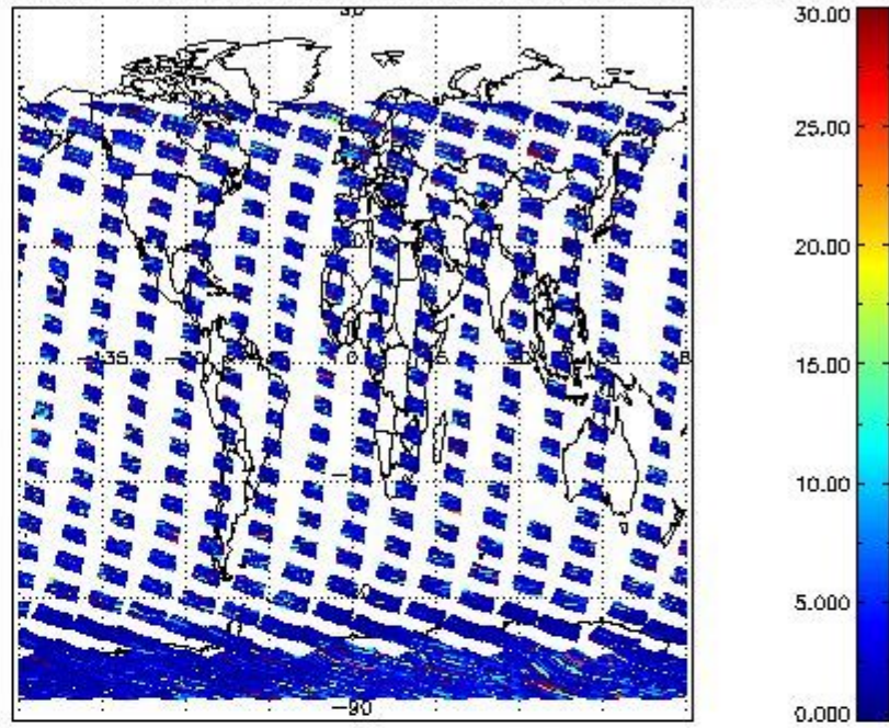
SCIOL2P_NADUV7S02_vcd_err for 25OCT2011 00:00:00 to 26OCT2011 00:00:00
