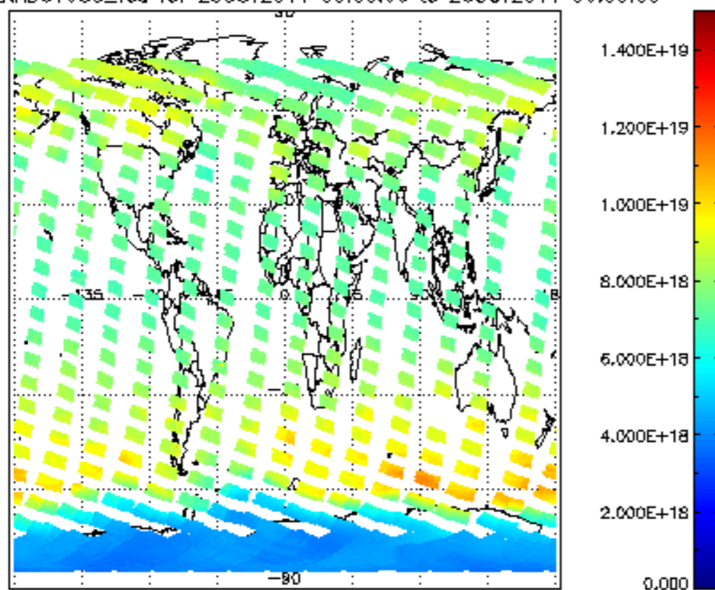
SCIOL2P_NADUV003_vcd for 25OCT2011 00:00:00 to 26OCT2011 00:00:00
