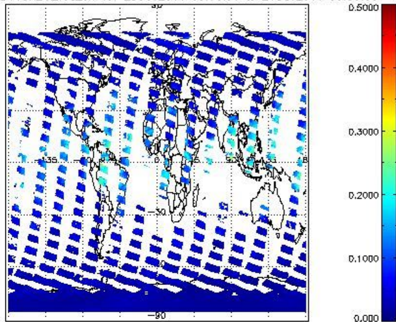
SCIOL2P_NADUV8H20_vcd_err for 25OCT2011 00:00:00 to 26OCT2011 00:00:00
