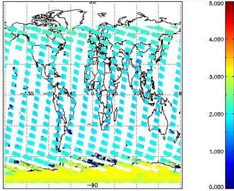
SCIOL2P_NADUV7S02_amf_gr for 25OCT2011 00:00:00 to 26OCT2011 00:00:00
