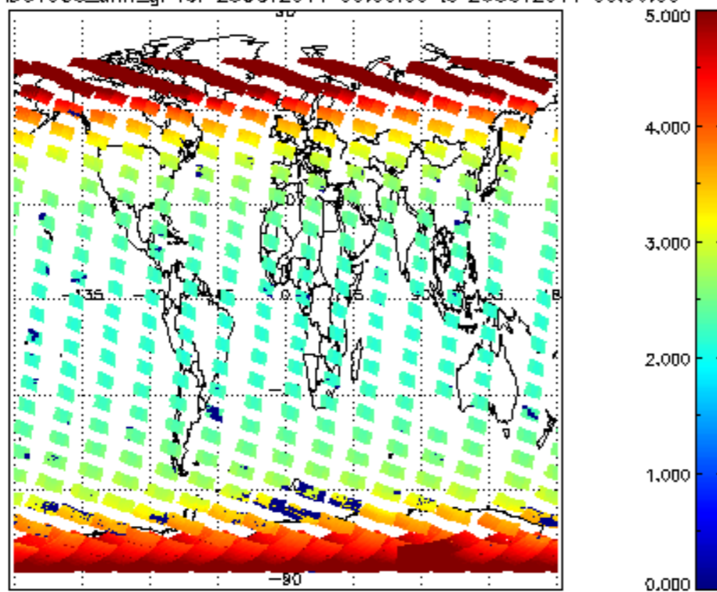
SCIOL2P_NADUV003_amf_gr for 25OCT2011 00:00:00 to 26OCT2011 00:00:00
