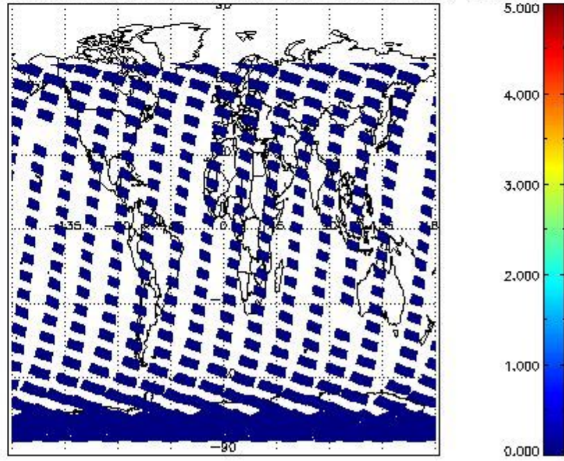
SCIOL2P_NADUV5S02_amf_cl for 25OCT2011 00:00:00 to 26OCT2011 00:00:00
