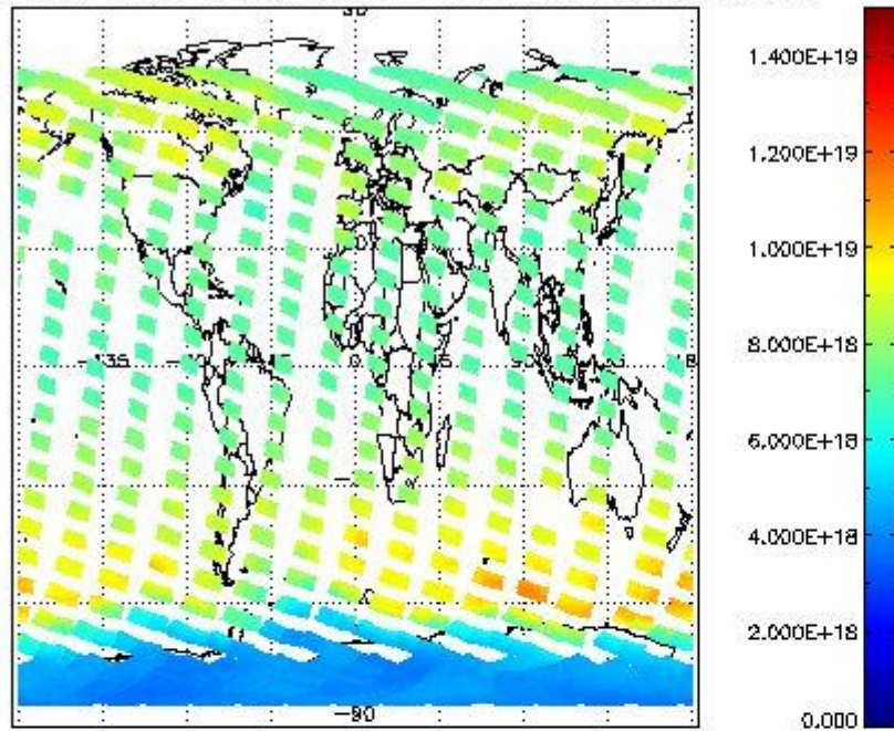
SCIOL2P_NADUV003_vcd for 25OCT2011 00:00:00 to 26OCT2011 00:00:00
