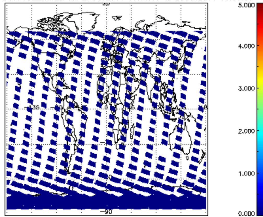
SCIOL2P_NADUV7S02_amf_sl for 25OCT2011 00:00:00 to 26OCT2011 00:00:00
