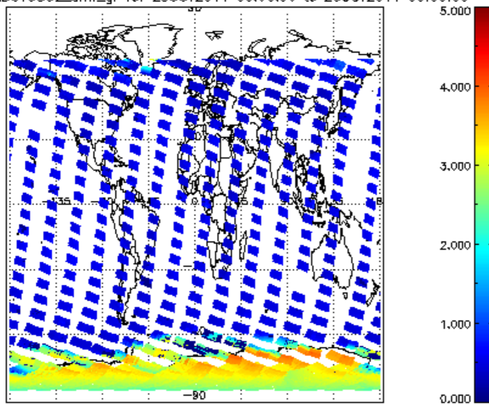
SCIOL2P_NADUV5S02_amf_gr for 25OCT2011 00:00:00 to 26OCT2011 00:00:00
