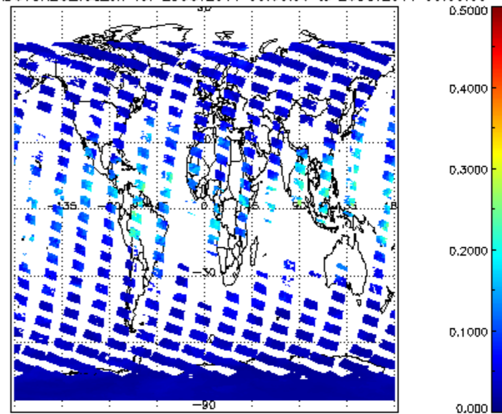
SCIOL2P_NADUV8H20_vcd_err for 25OCT2011 00:00:00 to 26OCT2011 00:00:00
