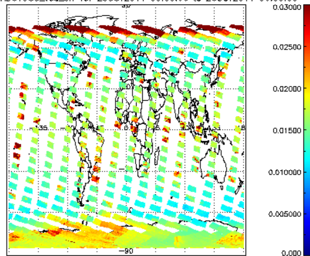
SCIOL2P_NADUV003_vcd_err for 25OCT2011 00:00:00 to 26OCT2011 00:00:00
