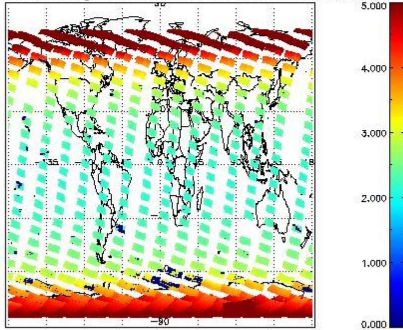
SCIOL2P_NADUV003_amf_gr for 25OCT2011 00:00:00 to 26OCT2011 00:00:00
