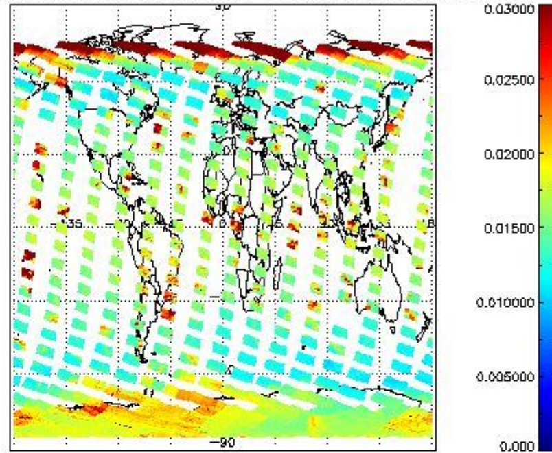
SCIOL2P_NADUV003_vcd_err for 25OCT2011 00:00:00 to 26OCT2011 00:00:00
