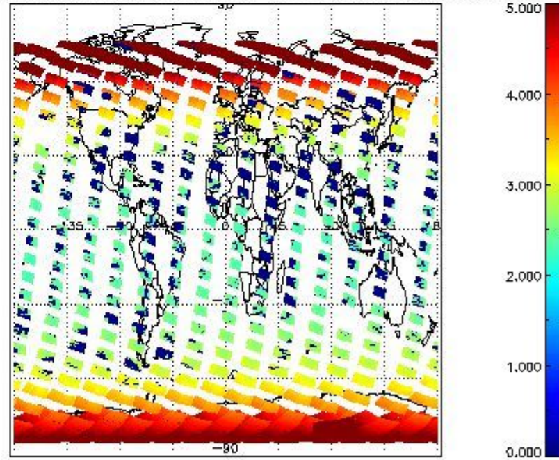
SCIOL2P_NADUV003_amf_cl for 25OCT2011 00:00:00 to 26OCT2011 00:00:00
