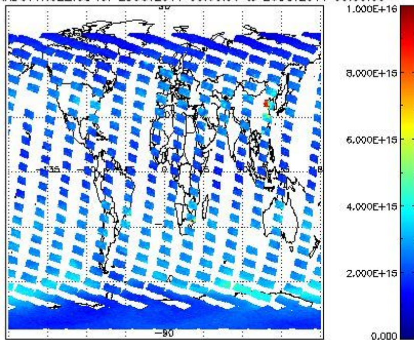
SCIOL2P_NADUV1NO2_vcd for 25OCT2011 00:00:00 to 26OCT2011 00:00:00
