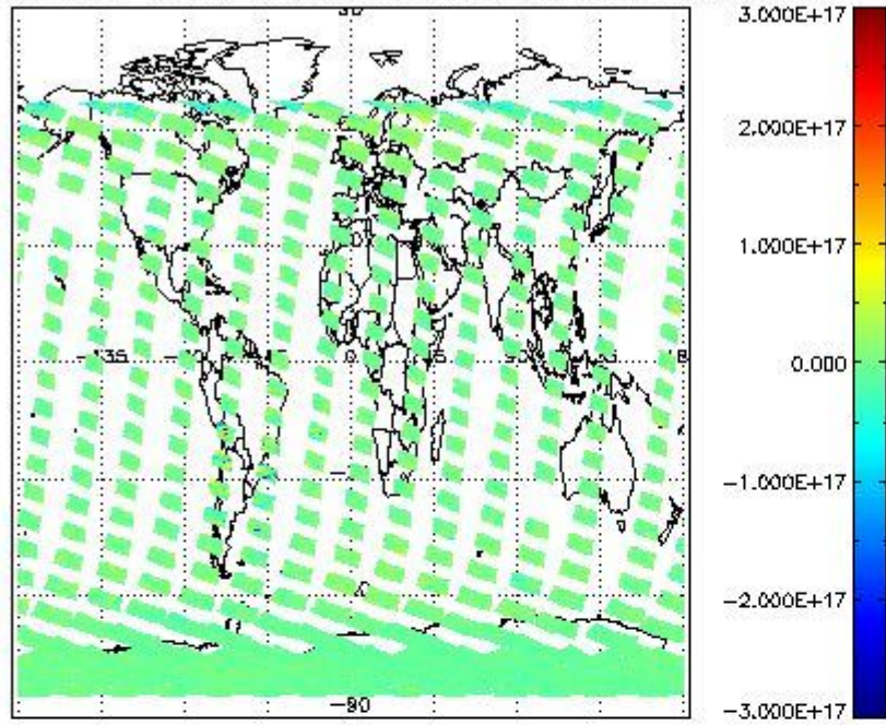
SCIOL2P_NADUV7S02_vcd for 25OCT2011 00:00:00 to 26OCT2011 00:00:00
