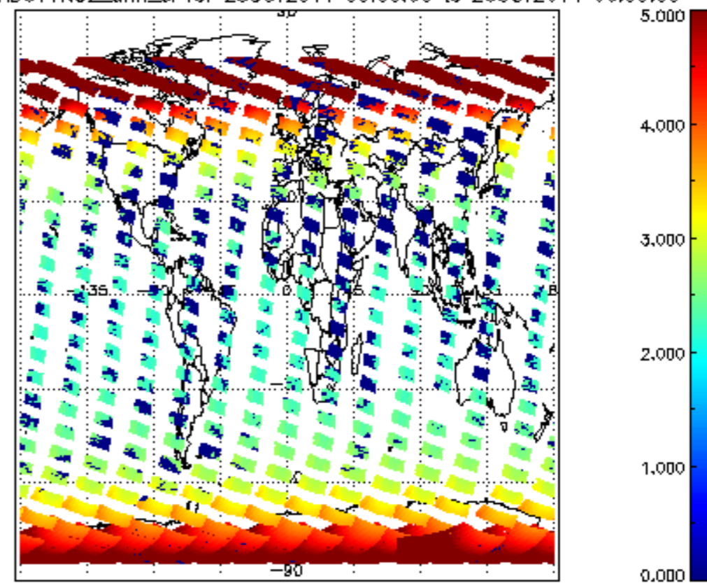
SCIOL2P_NADUV1NO2_amf_cl for 25OCT2011 00:00:00 to 26OCT2011 00:00:00
