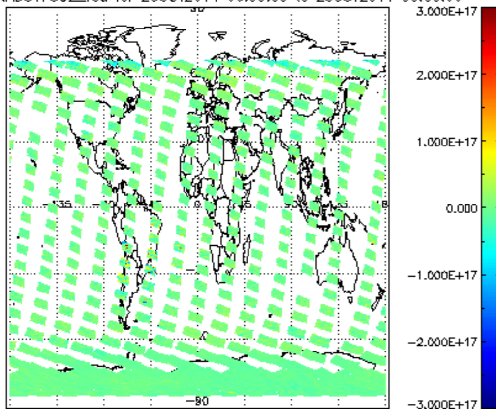
SCIOL2P_NADUV7S02_vcd for 25OCT2011 00:00:00 to 26OCT2011 00:00:00
