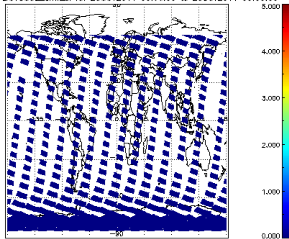
SCIOL2P_NADUV5S02_amf_cl for 25OCT2011 00:00:00 to 26OCT2011 00:00:00
