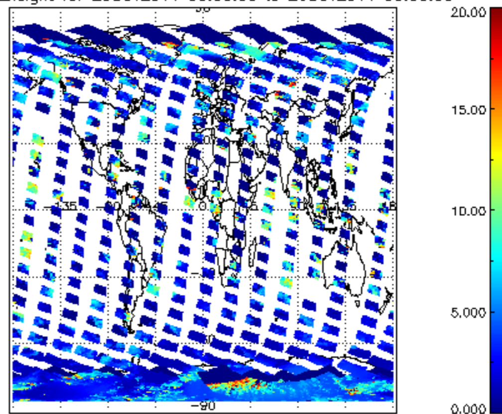
cl_top_height for 25OCT2011 00:00:00 to 26OCT2011 00:00:00
