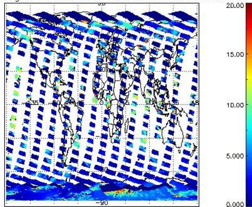
cL_top_height for 25OCT2011 00:00:00 to 26OCT2011 00:00:00
