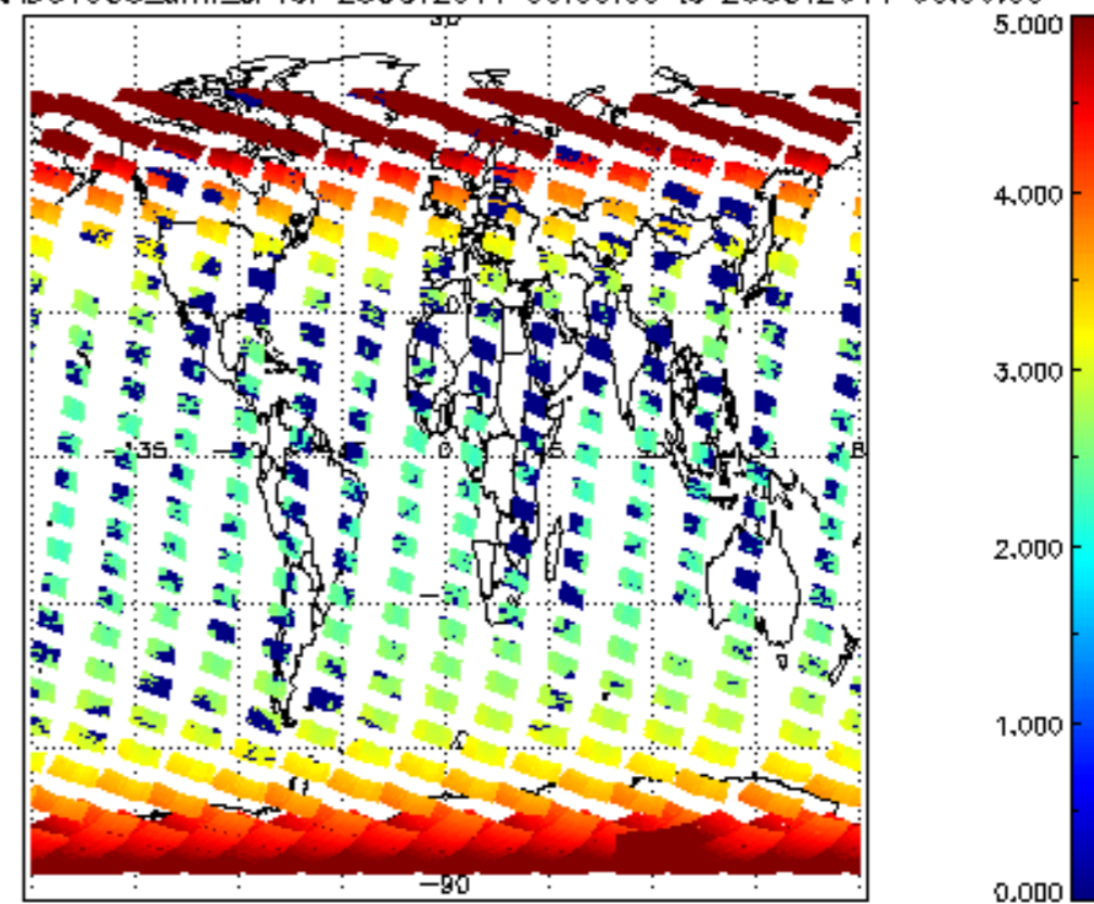
SCIOL2P_NADUV003_amf_cl for 25OCT2011 00:00:00 to 26OCT2011 00:00:00
