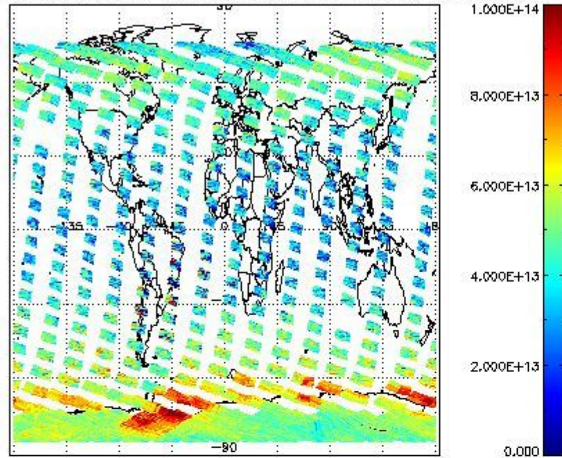
SCIOL2P_NADUV3BRO_vcd for 25OCT2011 00:00:00 to 26OCT2011 00:00:00
