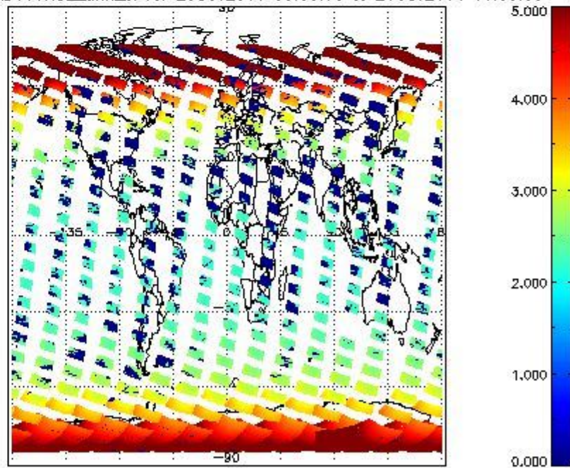
SCIOL2P_NADUV1NO2_amf_cl for 25OCT2011 00:00:00 to 26OCT2011 00:00:00
