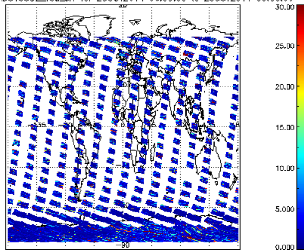
SCIOL2P_NADUV5S02_vcd_err for 25OCT2011 00:00:00 to 26OCT2011 00:00:00
