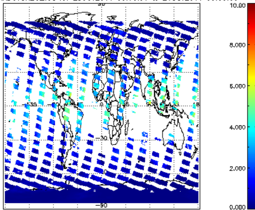
SCIOL2P_NADUV8H20_vcd for 25OCT2011 00:00:00 to 26OCT2011 00:00:00
