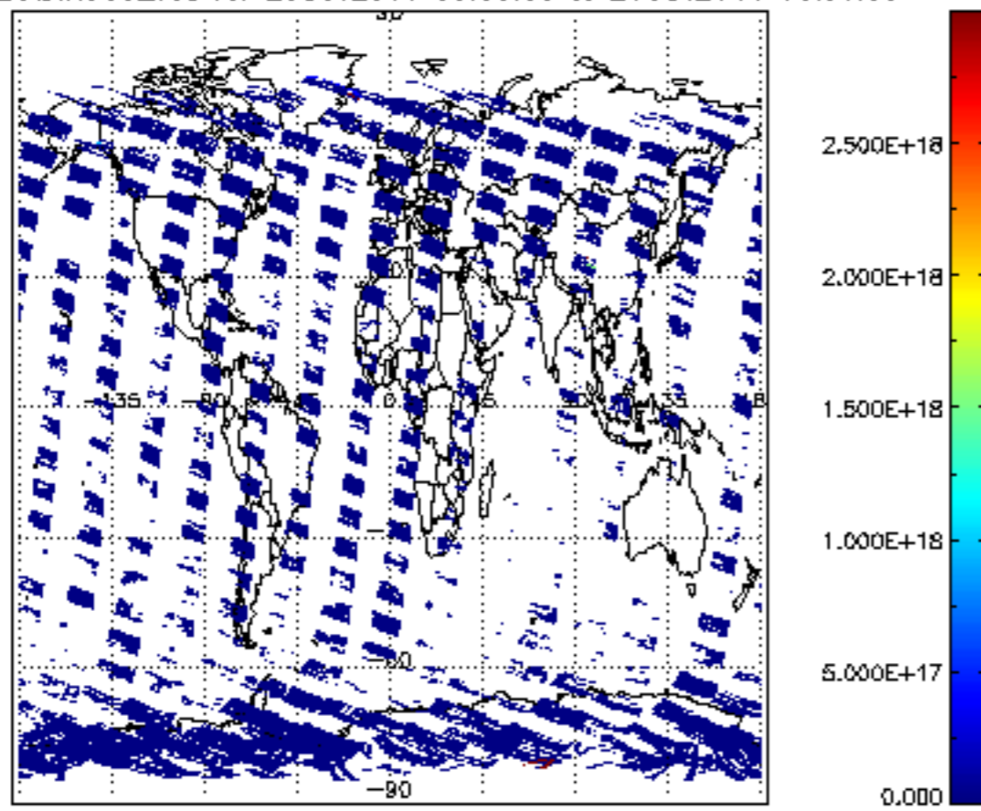
SCIOL2P_NADIR3CO_vcd for 25OCT2011 00:00:00 to 26OCT2011 00:00:00
