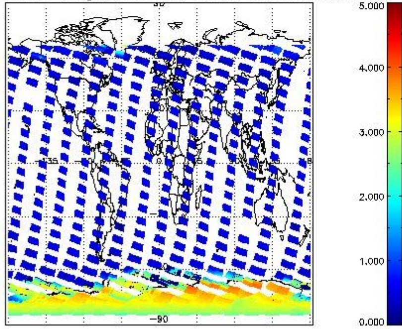
SCIOL2P_NADUV5S02_amf_gr for 25OCT2011 00:00:00 to 26OCT2011 00:00:00
