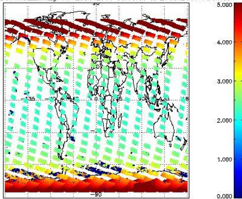
SCIOL2P_NADUV1NO2_amf_gr for 25OCT2011 00:00:00 to 26OCT2011 00:00:00
