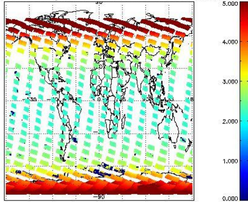
SCIOL2P_NADUV3BRO_amf_gr for 25OCT2011 00:00:00 to 26OCT2011 00:00:00
