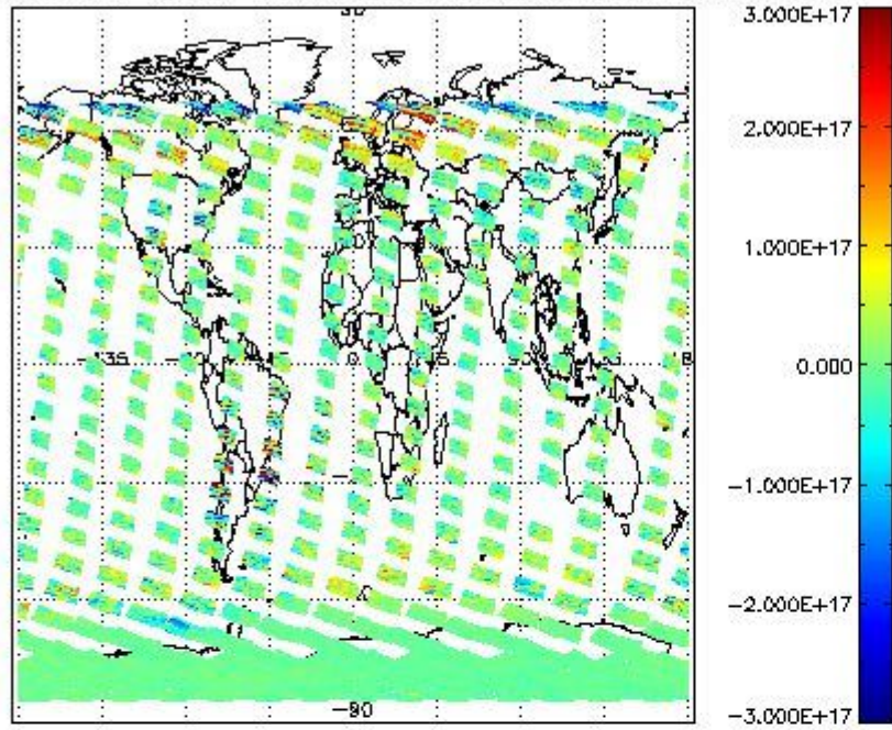
SCIOL2P_NADUV5S02_vcd for 25OCT2011 00:00:00 to 26OCT2011 00:00:00
