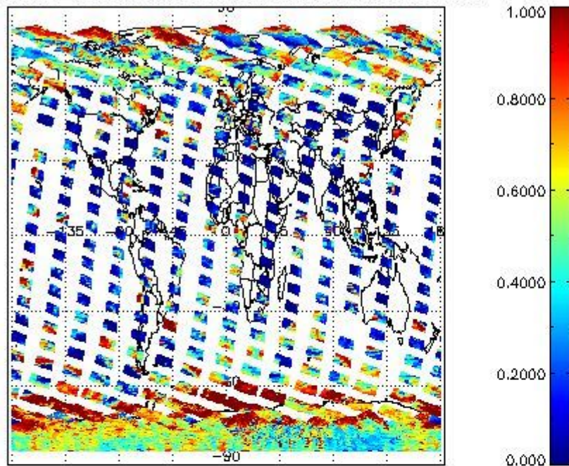
cLfrac for 25OCT2011 00:00:00 to 26OCT2011 00:00:00
