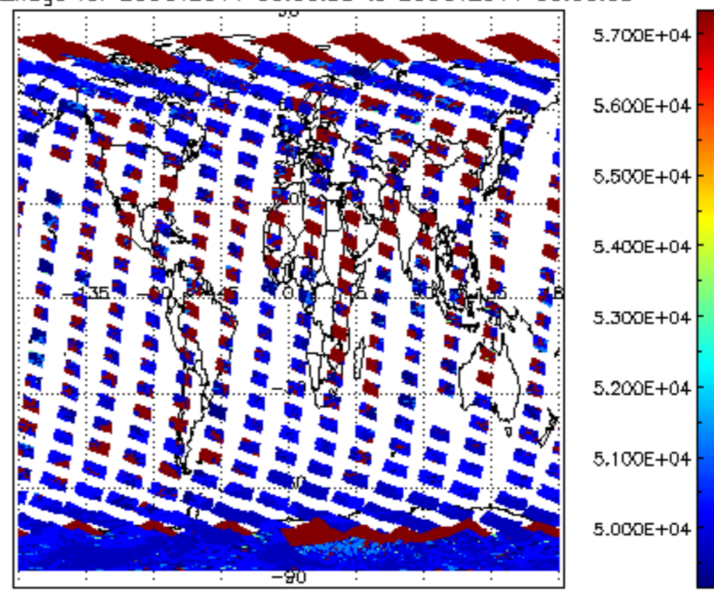
cloud_flags for 25OCT2011 00:00:00 to 26OCT2011 00:00:00
