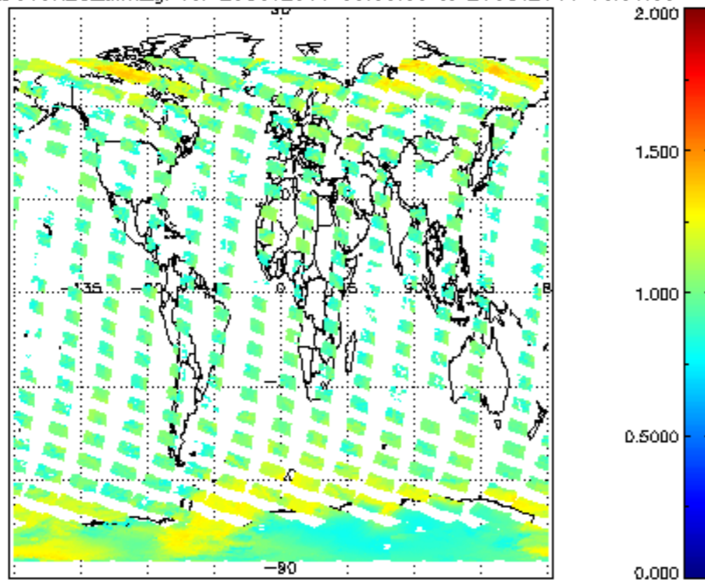
SCIOL2P_NADUV8H20_amf_gr for 25OCT2011 00:00:00 to 26OCT2011 00:00:00
