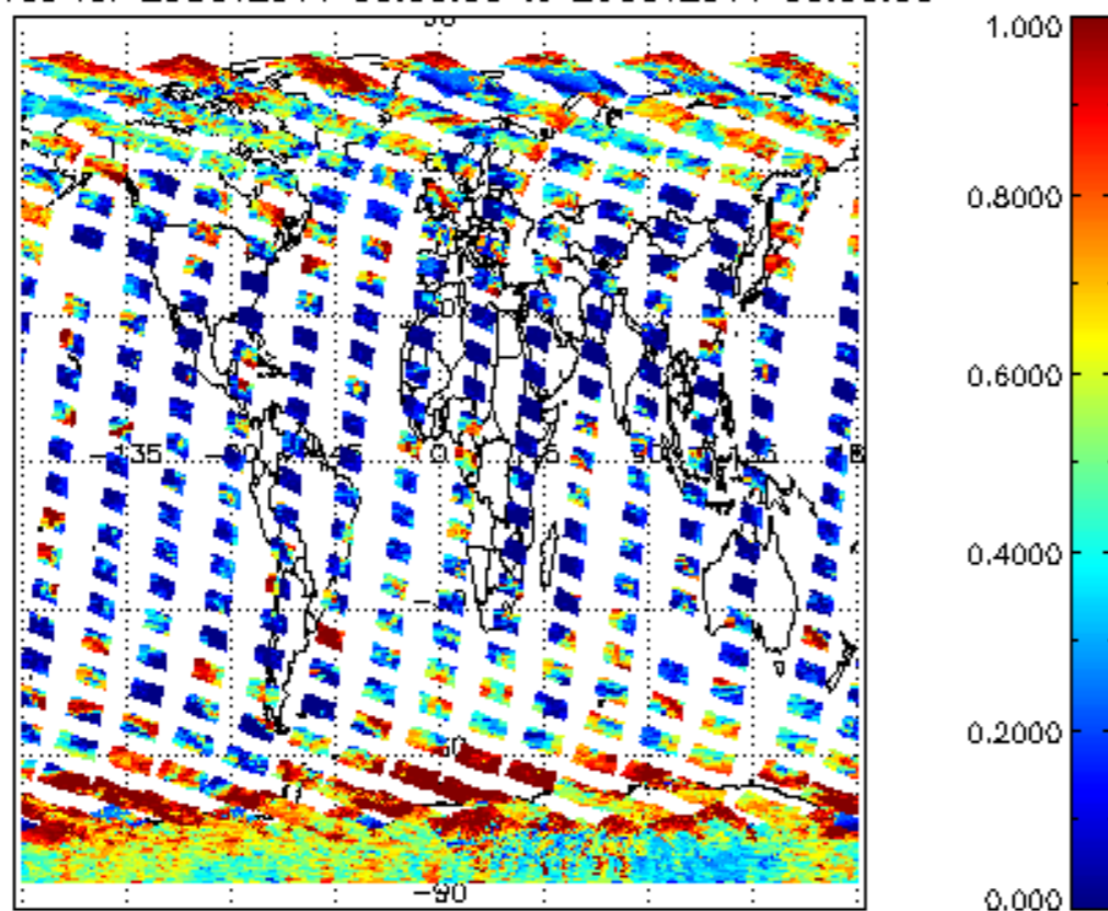
cl_frac for 25OCT2011 00:00:00 to 26OCT2011 00:00:00
