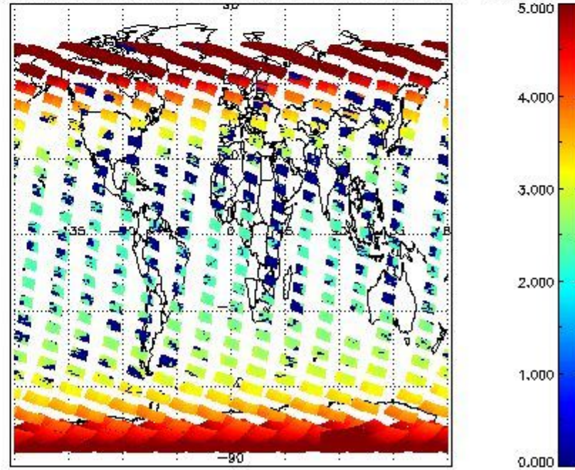
SCIOL2P_NADUV3BRO_amf_cl for 25OCT2011 00:00:00 to 26OCT2011 00:00:00
