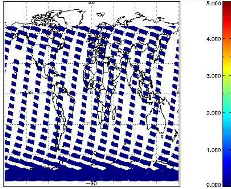
SCIOL2P_NADUV7S02_amf_cl for 25OCT2011 00:00:00 to 26OCT2011 00:00:00
