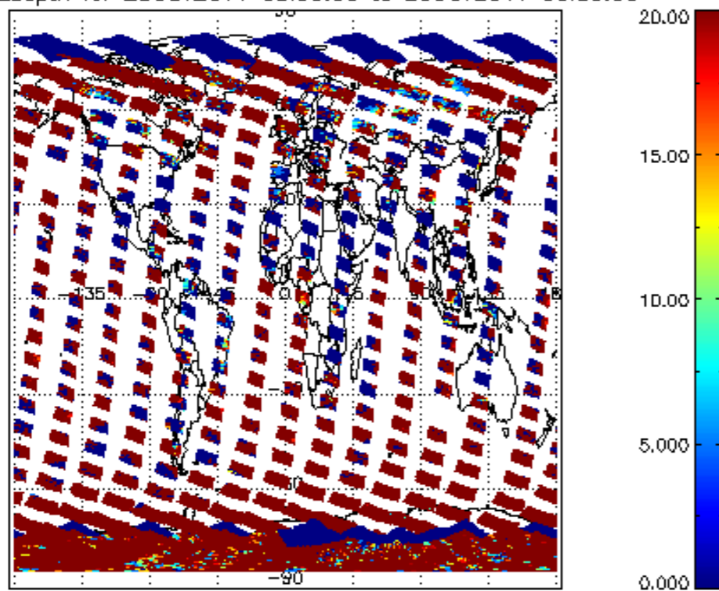
cl_opt_depth for 25OCT2011 00:00:00 to 26OCT2011 00:00:00
