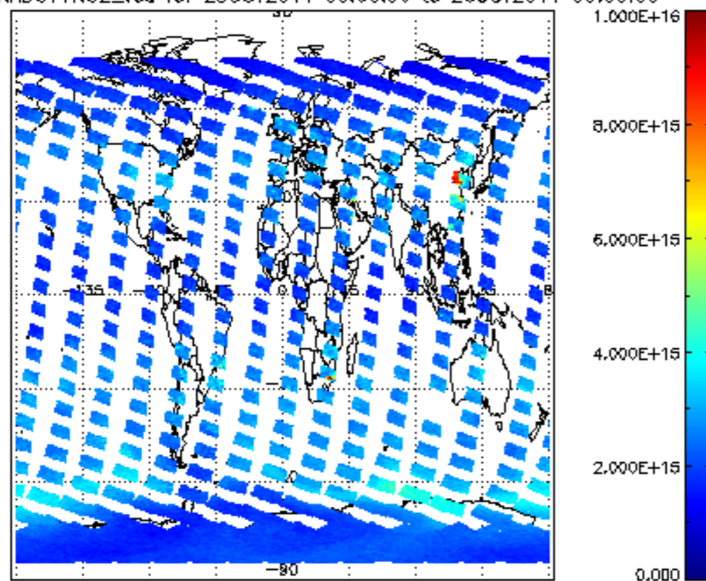
SCIOL2P_NADUV1NO2_vcd for 25OCT2011 00:00:00 to 26OCT2011 00:00:00
