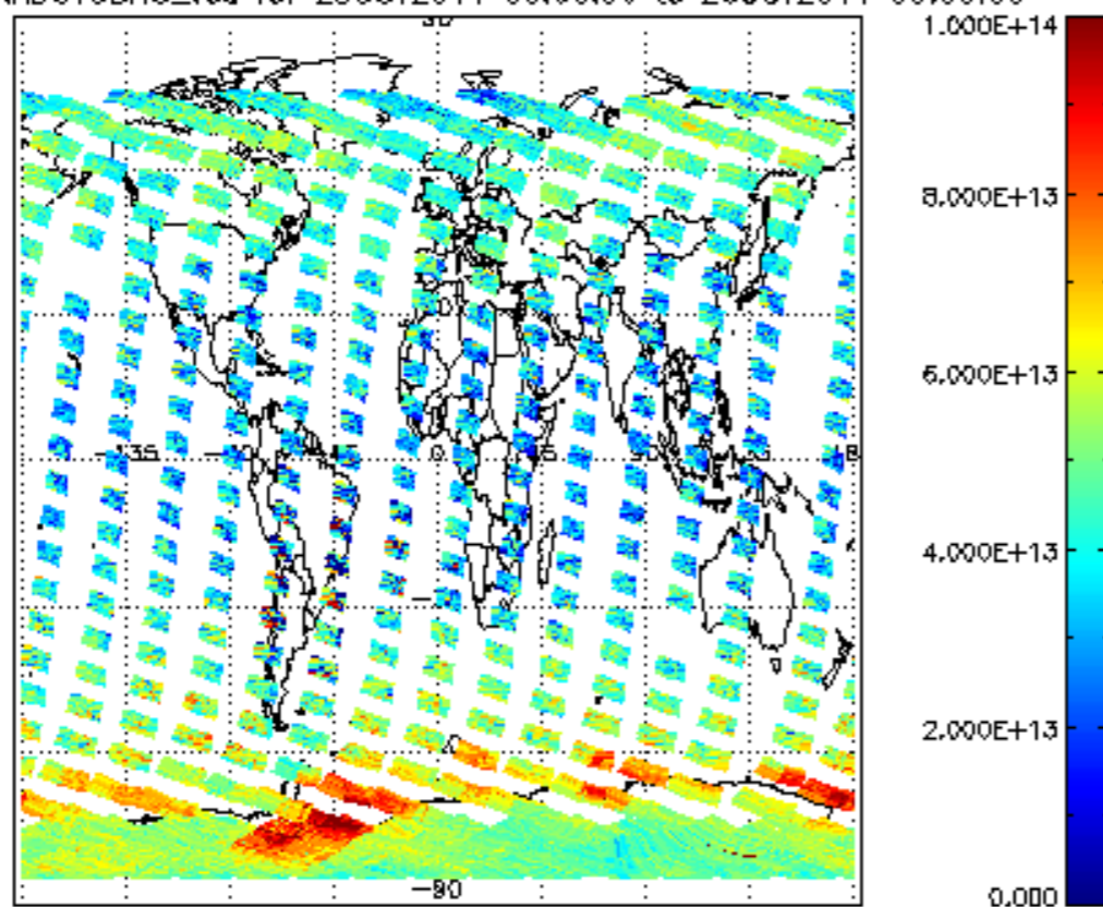
SCIOL2P_NADUV3BRO_vcd for 25OCT2011 00:00:00 to 26OCT2011 00:00:00
