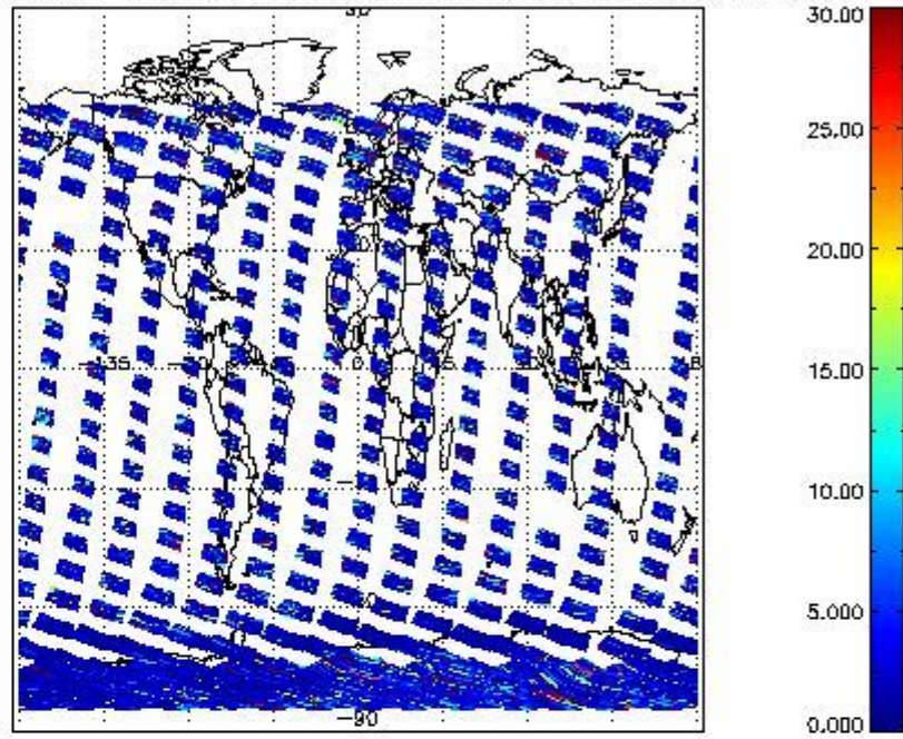
SCIOL2P_NADUV5S02_vcd_err for 25OCT2011 00:00:00 to 26OCT2011 00:00:00
