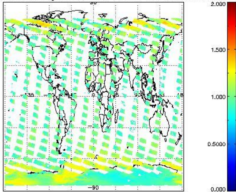
SCIOL2P_NADUV8H20_amf_gr for 25OCT2011 00:00:00 to 26OCT2011 00:00:00
