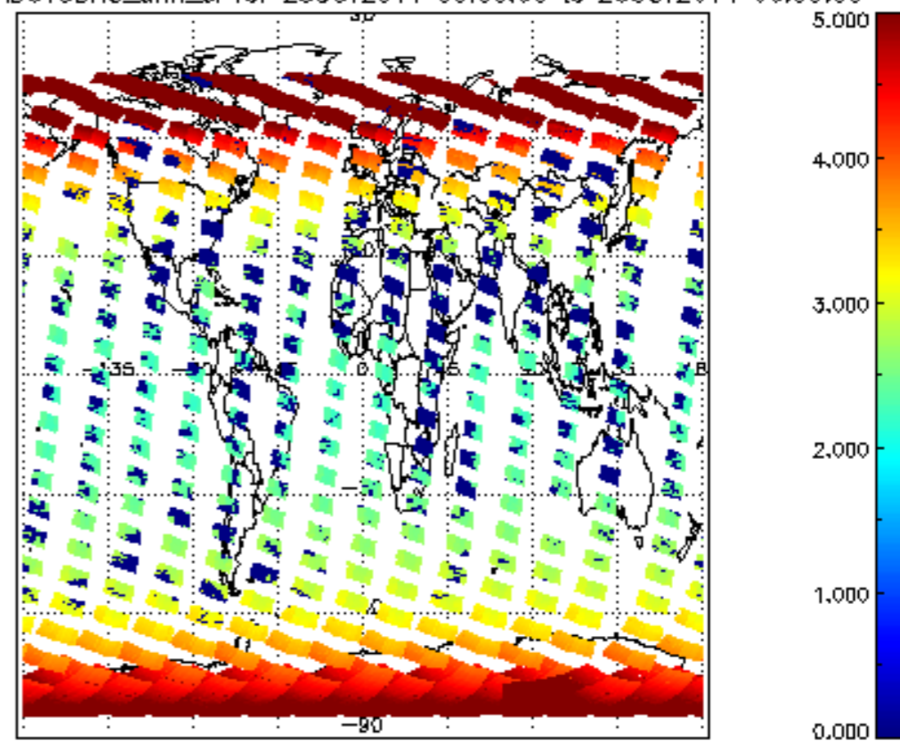
SCIOL2P_NADUV3BRO_amf_cl for 25OCT2011 00:00:00 to 26OCT2011 00:00:00
