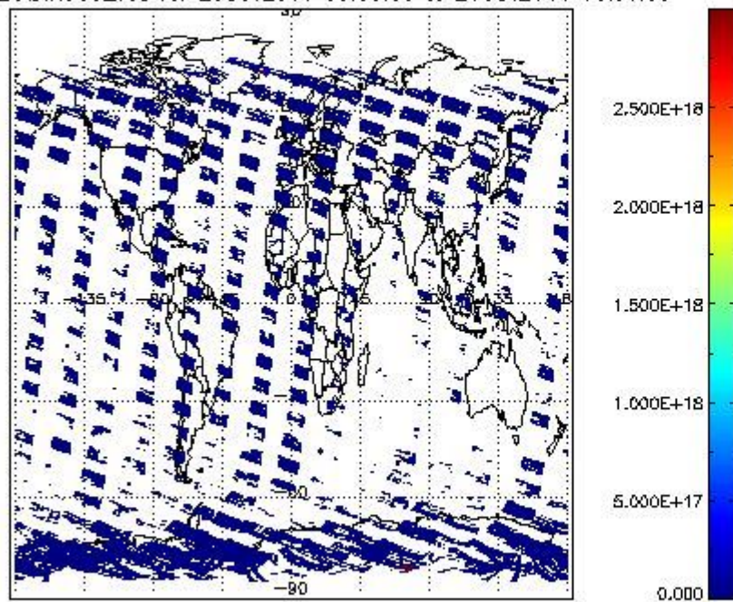
SCIOL2P_NADIR3CO_vcd for 25OCT2011 00:00:00 to 26OCT2011 00:00:00
