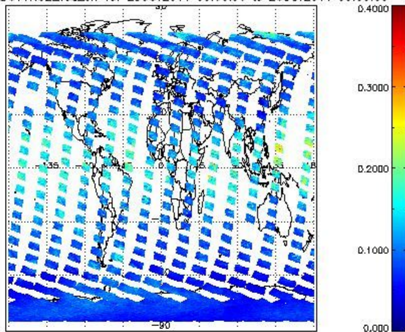
SCIOL2P_NADUV1NO2_vcd_err for 25OCT2011 00:00:00 to 26OCT2011 00:00:00
