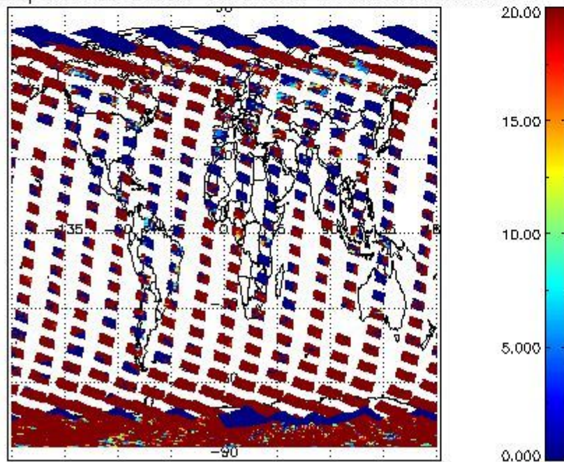
cL_opt_depth for 25OCT2011 00:00:00 to 26OCT2011 00:00:00
