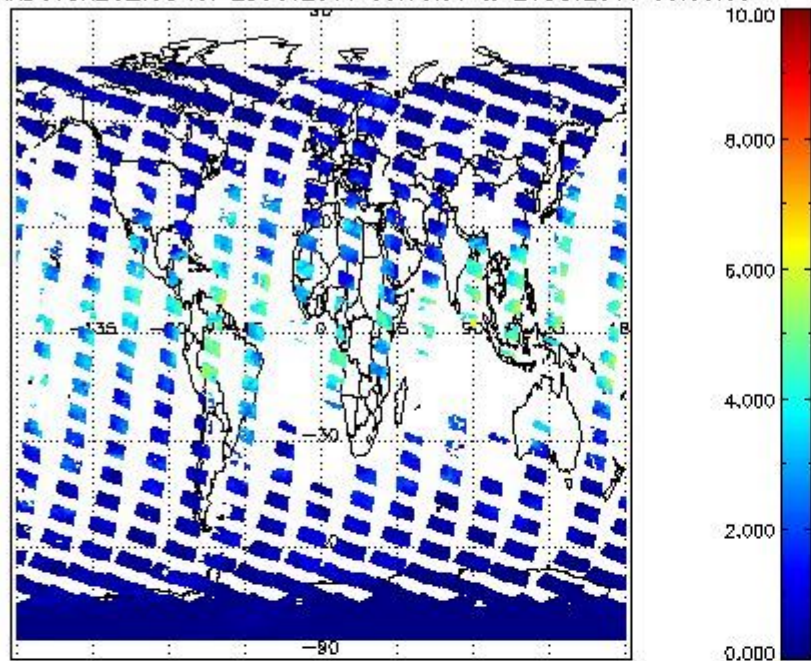
SCIOL2P_NADUV8H20_vcd for 25OCT2011 00:00:00 to 26OCT2011 00:00:00
