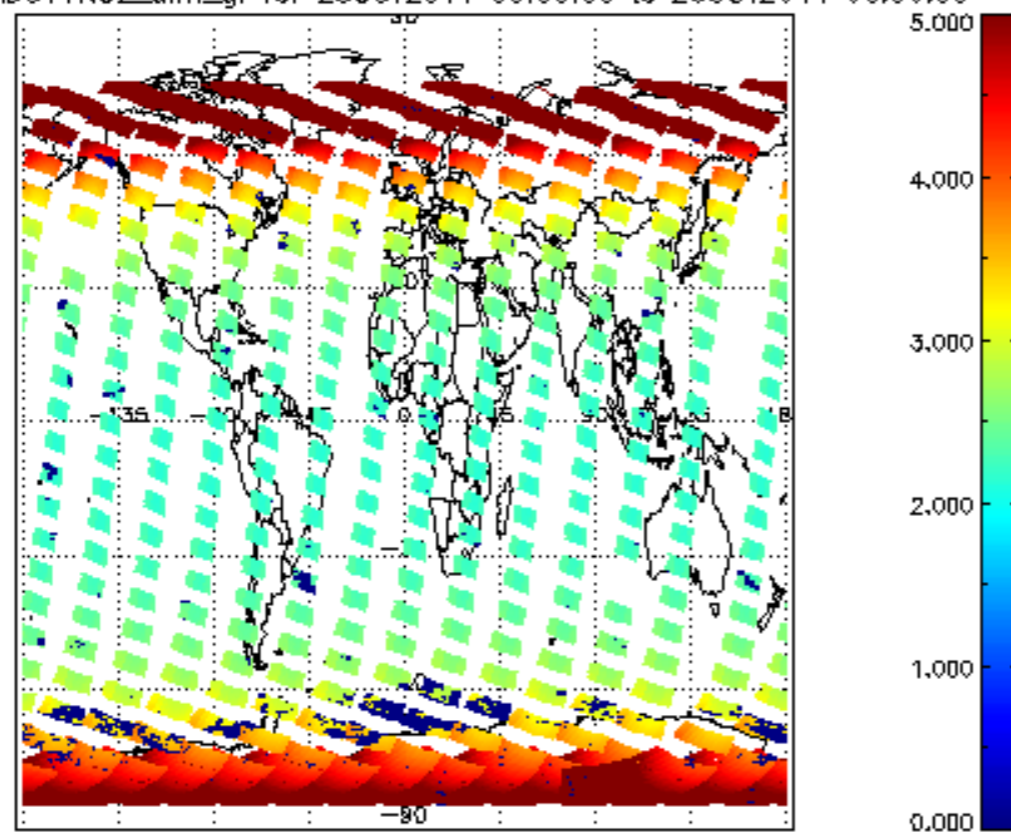
SCIOL2P_NADUV1NO2_amf_gr for 25OCT2011 00:00:00 to 26OCT2011 00:00:00
