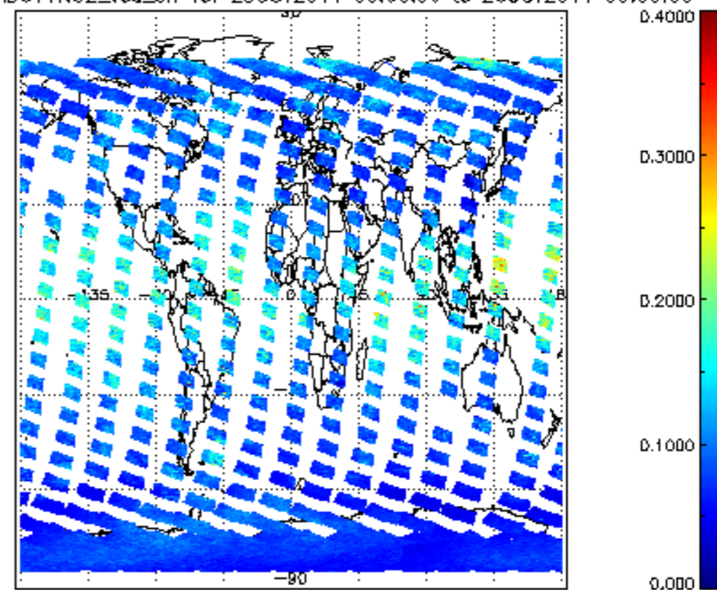
SCIOL2P_NADUV1NO2_vcd_err for 25OCT2011 00:00:00 to 26OCT2011 00:00:00
