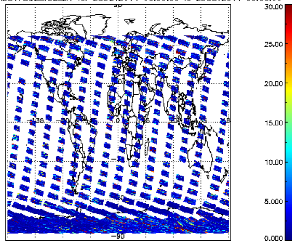
SCIOL2P_NADUV7S02_vcd_err for 25OCT2011 00:00:00 to 26OCT2011 00:00:00
