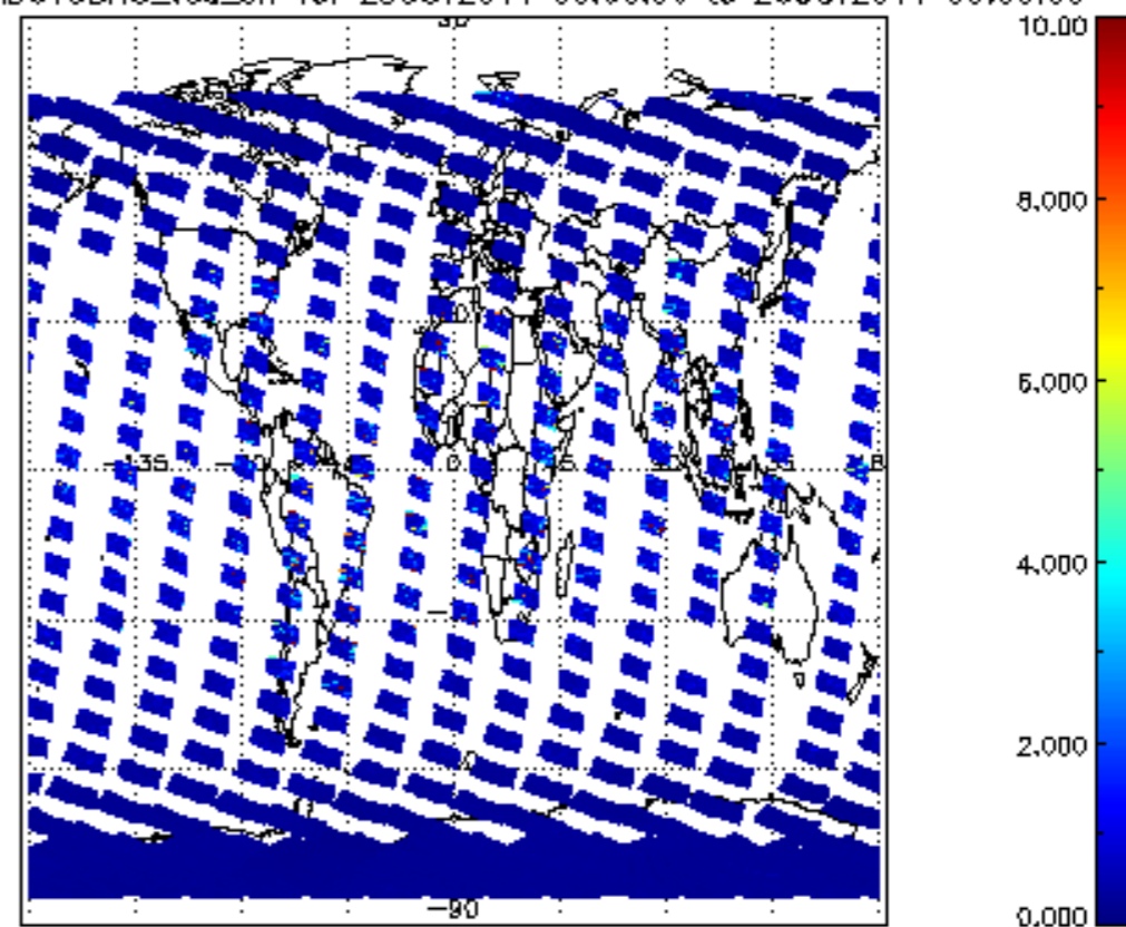
SCIOL2P_NADUV3BRO_vcd_err for 25OCT2011 00:00:00 to 26OCT2011 00:00:00
