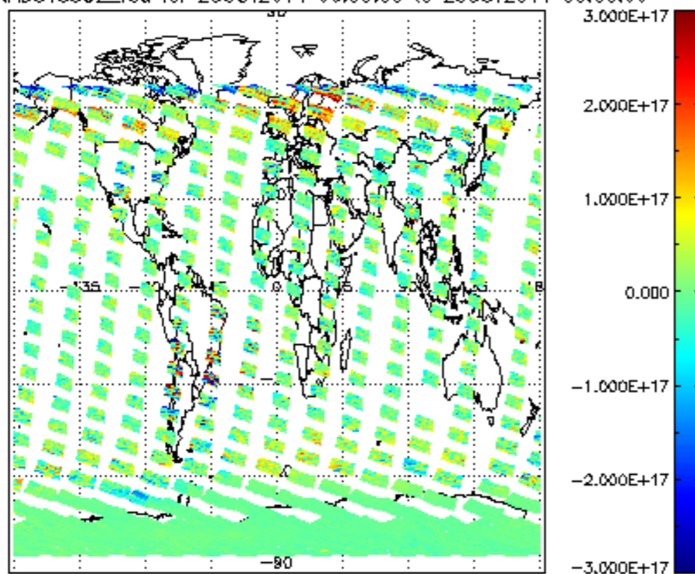
SCIOL2P_NADUV5S02_vcd for 25OCT2011 00:00:00 to 26OCT2011 00:00:00
