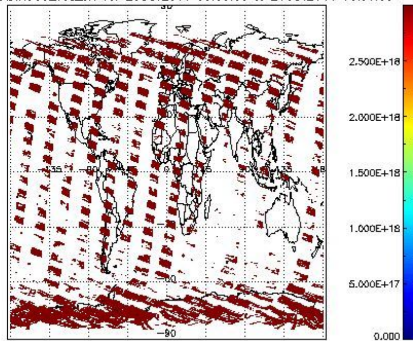
SCIOL2P_NADIR3CO_vcd_err for 25OCT2011 00:00:00 to 26OCT2011 00:00:00
