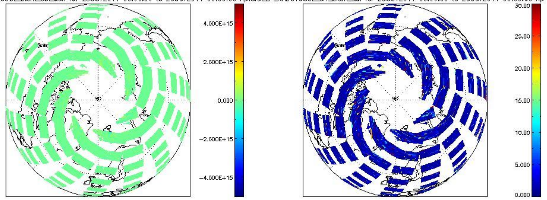
CIOL2P_NADUV60CLslant_col_den for 25OCT2011 00:00:00 to 26OCT2011 00:00:00 np CIOL2P_NADUV60CLarr_slant_col for 25OCT2011 00:00:00 to 26OCT2011 00:00:00 np
