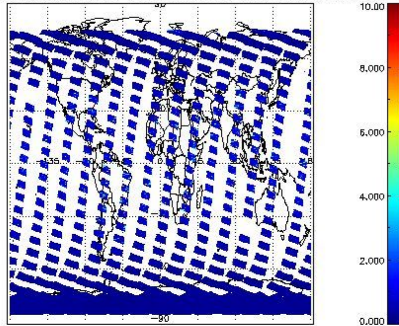
SCIOL2P_NADUV3BRO_vcd_err for 25OCT2011 00:00:00 to 26OCT2011 00:00:00
