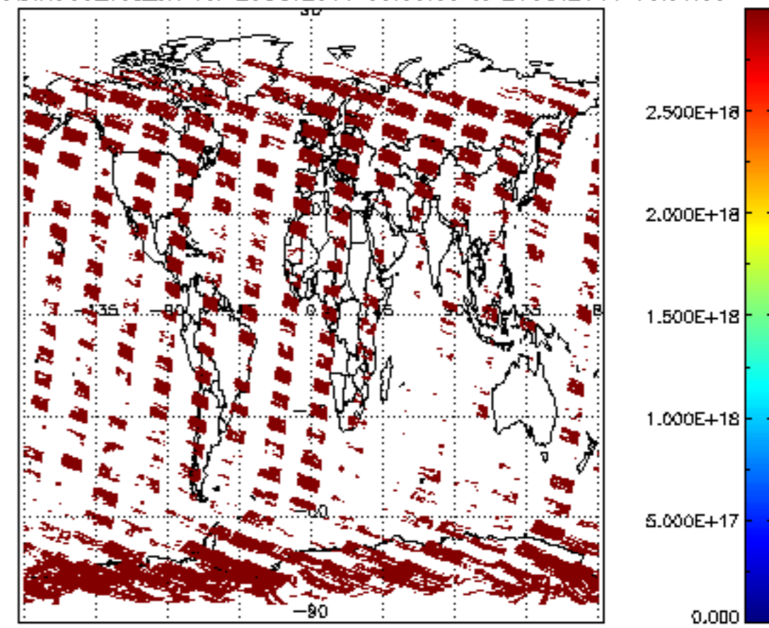
SCIOL2P_NADIR3CO_vcd_err for 25OCT2011 00:00:00 to 26OCT2011 00:00:00
