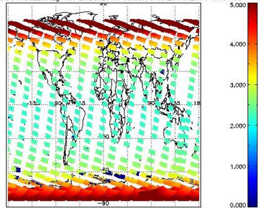
SCIOL2P_NADUV003_amf_gr for 24OCT2011 00:00:00 to 25OCT2011 00:00:00
