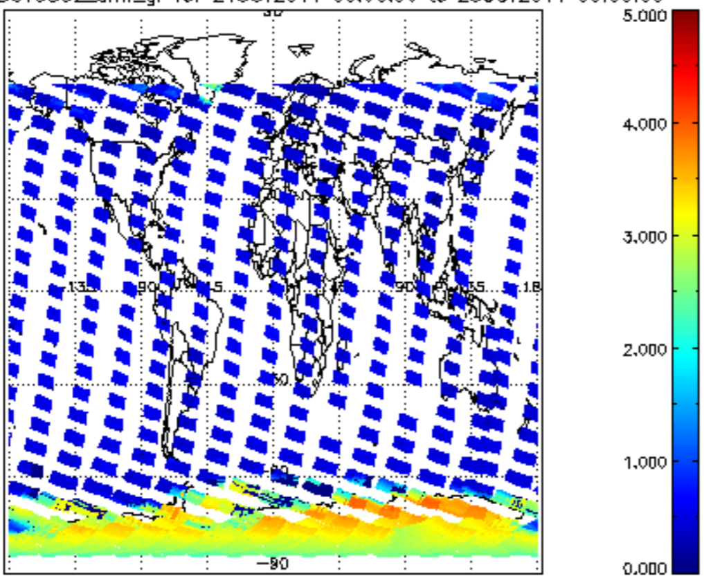
SCIOL2P_NADUV5S02_amf_gr for 24OCT2011 00:00:00 to 25OCT2011 00:00:00
