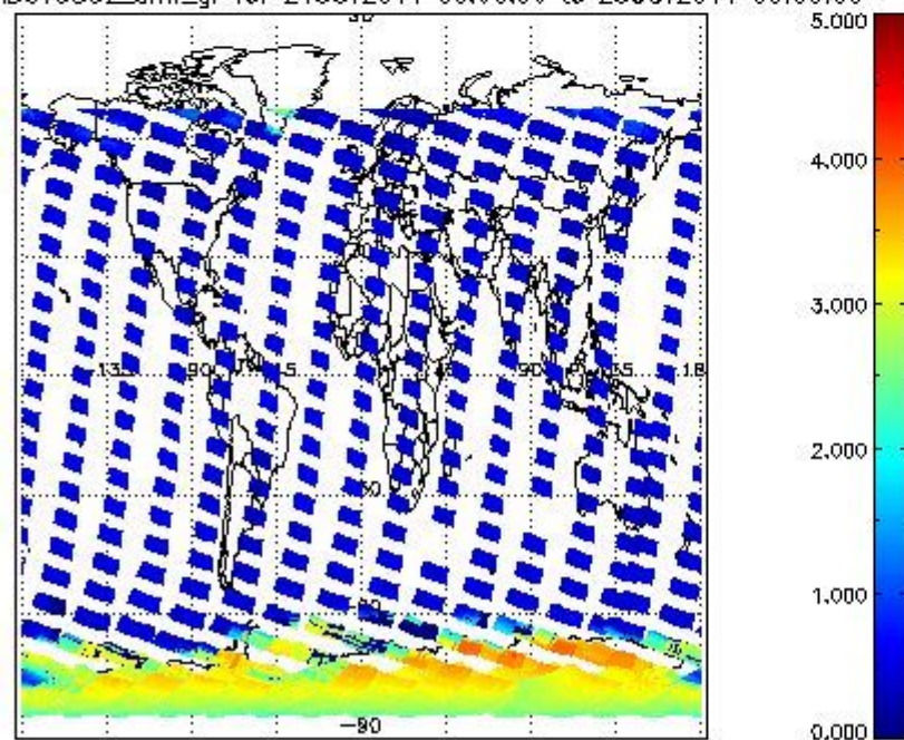
SCIOL2P_NADUV5S02_amf_gr for 24OCT2011 00:00:00 to 25OCT2011 00:00:00
