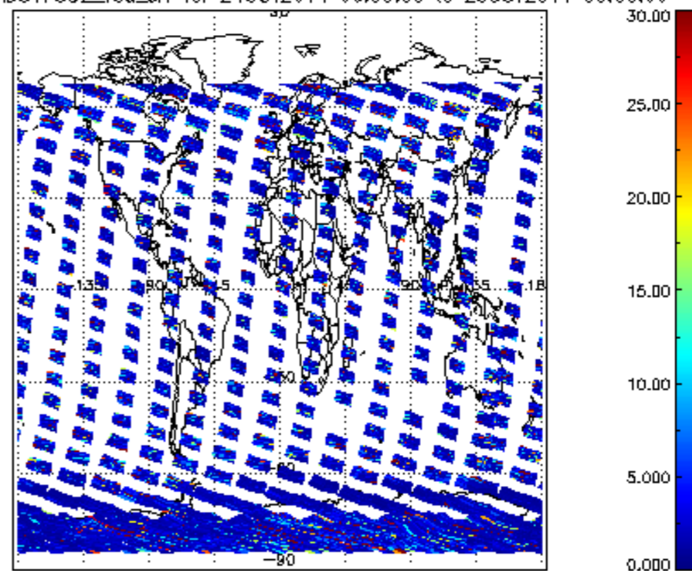
SCIOL2P_NADUV7S02_vcd_err for 24OCT2011 00:00:00 to 25OCT2011 00:00:00
