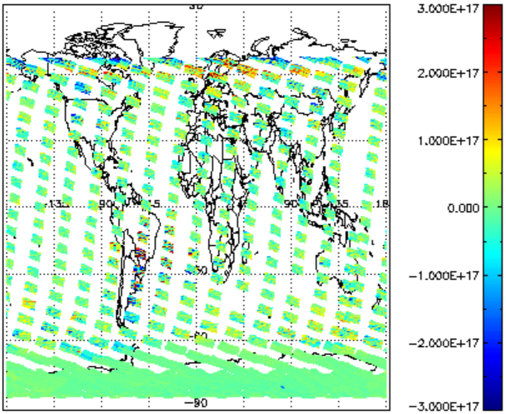
SCIOL2P_NADUV5S02_vcd for 24OCT2011 00:00:00 to 25OCT2011 00:00:00
