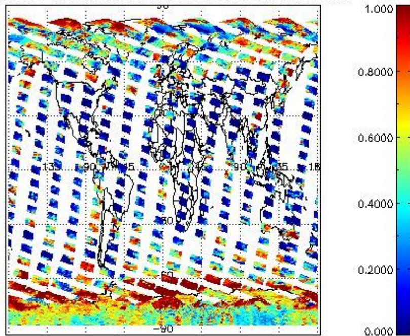
cLfrac for 24OCT2011 00:00:00 to 25OCT2011 00:00:00
