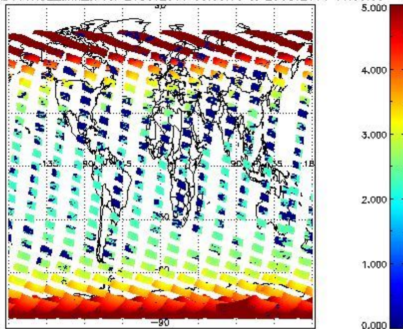
SCIOL2P_NADUV1N02_amf_cl for 24OCT2011 00:00:00 to 25OCT2011 00:00:00
