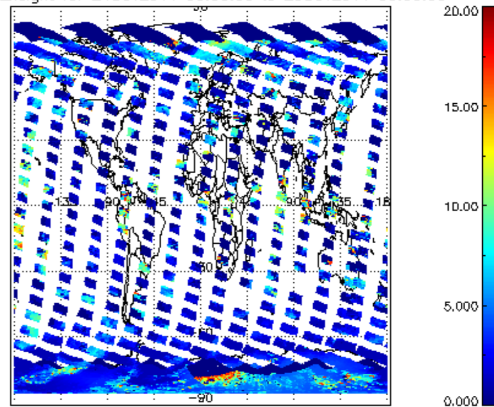
cl_top_height for 24OCT2011 00:00:00 to 25OCT2011 00:00:00
