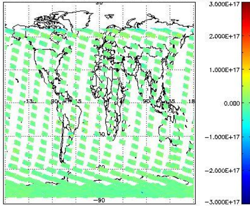
SCIOL2P_NADUV7S02_vcd for 24OCT2011 00:00:00 to 25OCT2011 00:00:00
