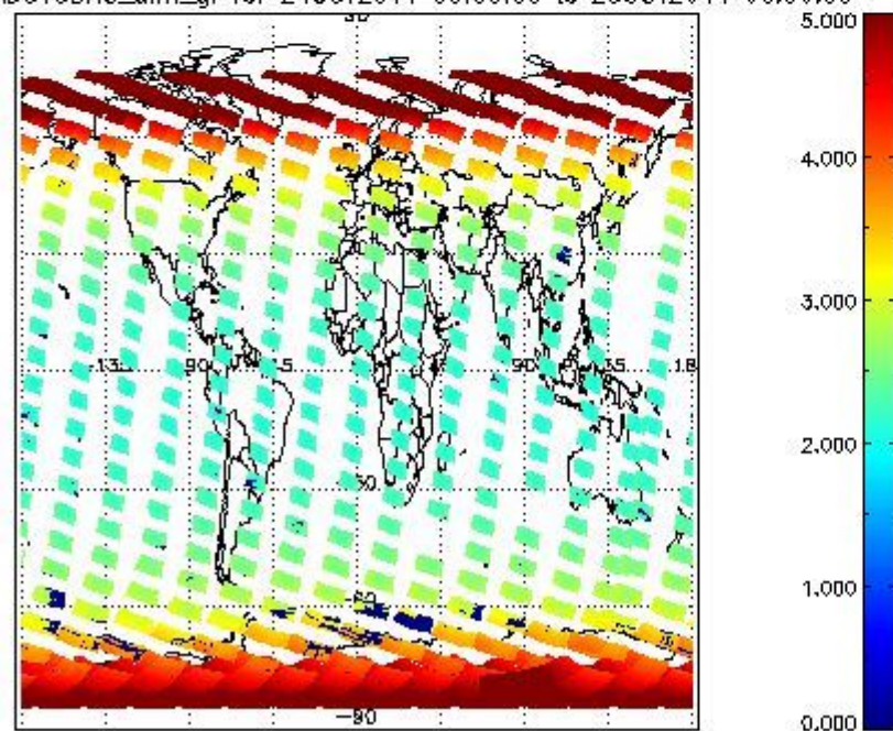
SCIOL2P_NADUV3BRO_amf_gr for 24OCT2011 00:00:00 to 25OCT2011 00:00:00
