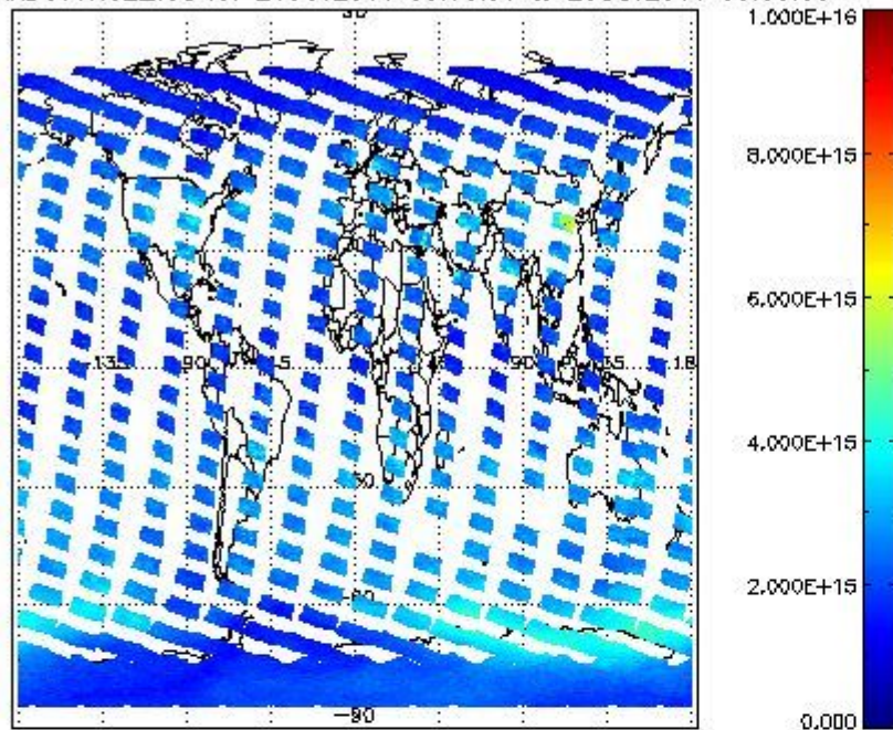
SCIOL2P_NADUV1N02_vcd for 24OCT2011 00:00:00 to 25OCT2011 00:00:00
