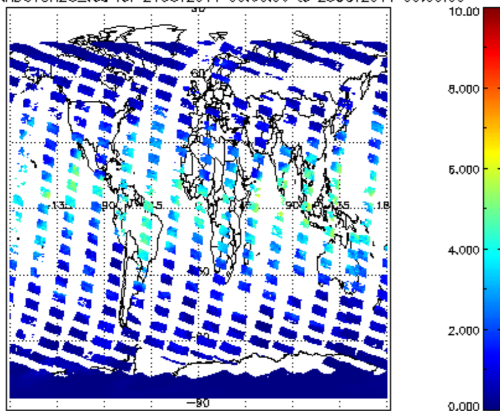
SCIOL2P_NADUV8H20_vcd for 24OCT2011 00:00:00 to 25OCT2011 00:00:00
