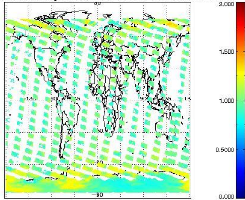
SCIOL2P_NADUV8H20_amf_gr for 24OCT2011 00:00:00 to 25OCT2011 00:00:00
