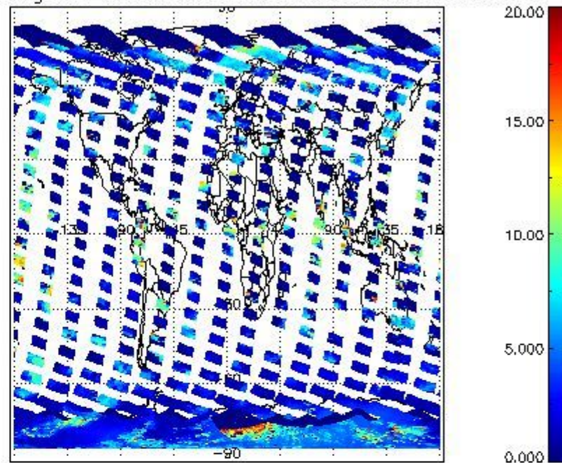
cL_top_height for 24OCT2011 00:00:00 to 25OCT2011 00:00:00
