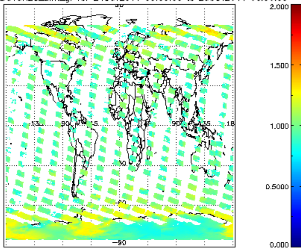
SCIOL2P_NADUV8H20_amf_gr for 24OCT2011 00:00:00 to 25OCT2011 00:00:00
