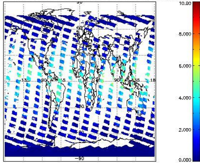
SCIOL2P_NADUV8H20_vcd for 24OCT2011 00:00:00 to 25OCT2011 00:00:00
