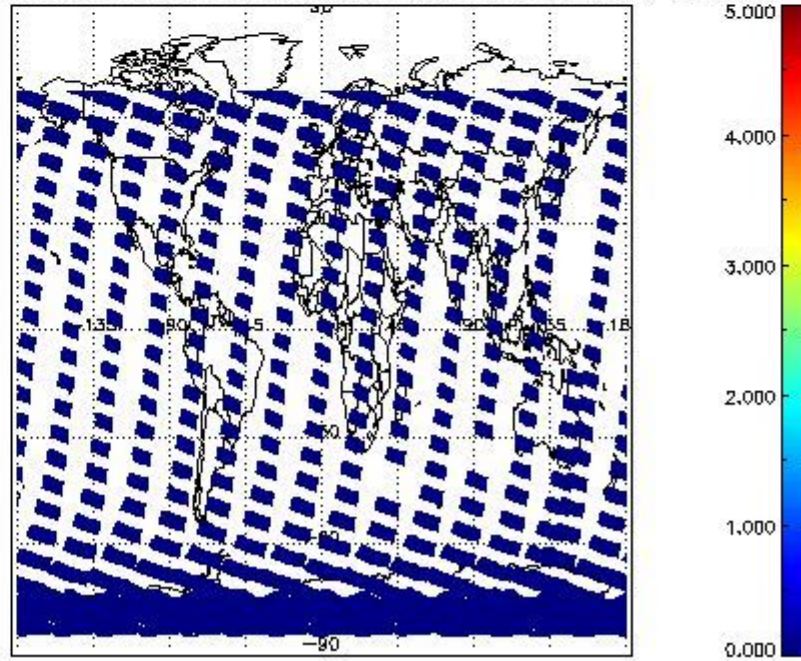
SCIOL2P_NADUV7S02_amf_cl for 24OCT2011 00:00:00 to 25OCT2011 00:00:00
