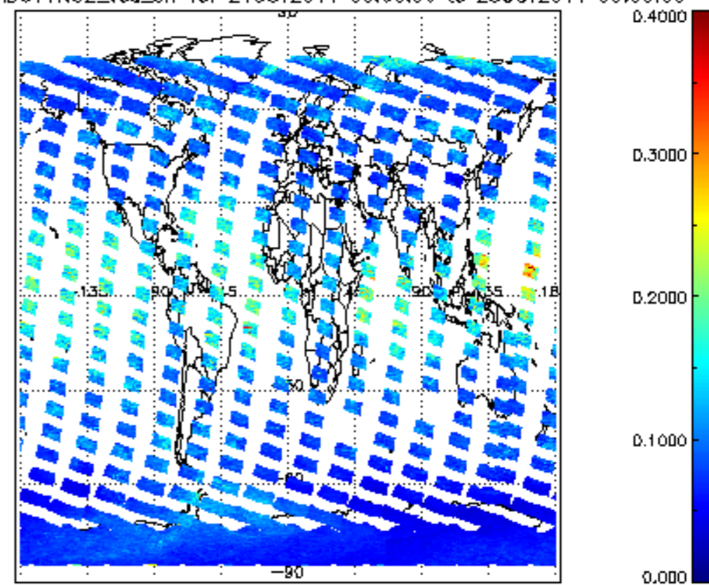
SCIOL2P_NADUV1NO2_vcd_err for 24OCT2011 00:00:00 to 25OCT2011 00:00:00
