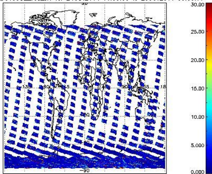
SCIOL2P_NADUV5S02_vcd_err for 24OCT2011 00:00:00 to 25OCT2011 00:00:00
