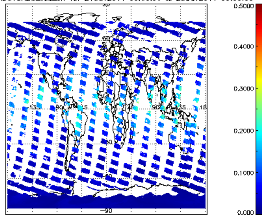
SCIOL2P_NADUV8H20_vcd_err for 24OCT2011 00:00:00 to 25OCT2011 00:00:00
