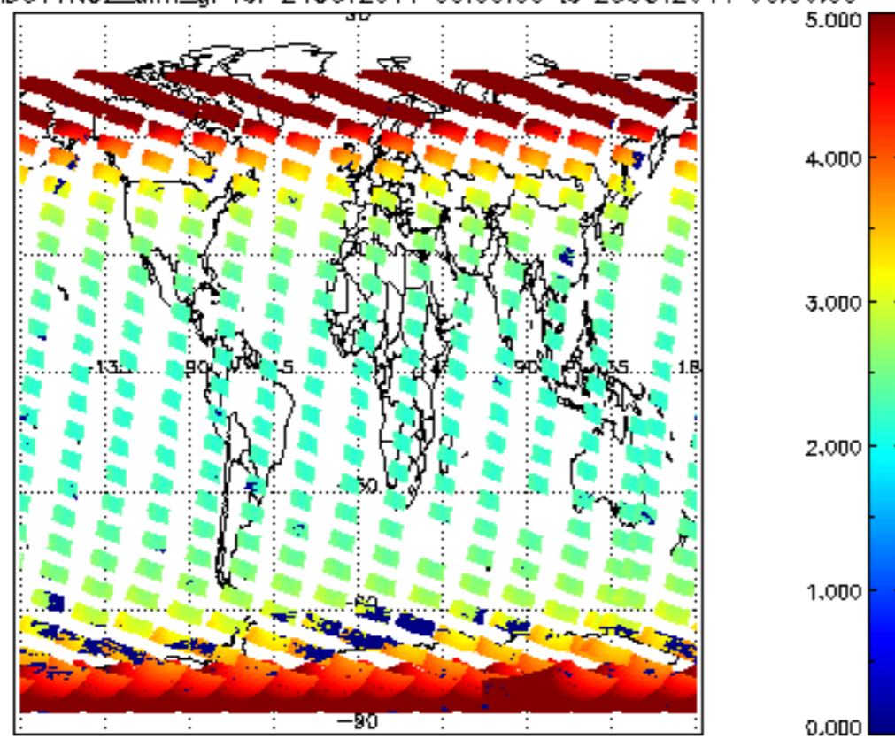
SCIOL2P_NADUV1NO2_amf_gr for 24OCT2011 00:00:00 to 25OCT2011 00:00:00
