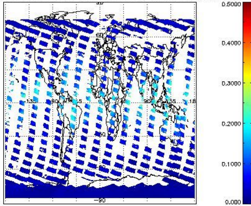
SCIOL2P_NADUV8H20_vcd_err for 24OCT2011 00:00:00 to 25OCT2011 00:00:00
