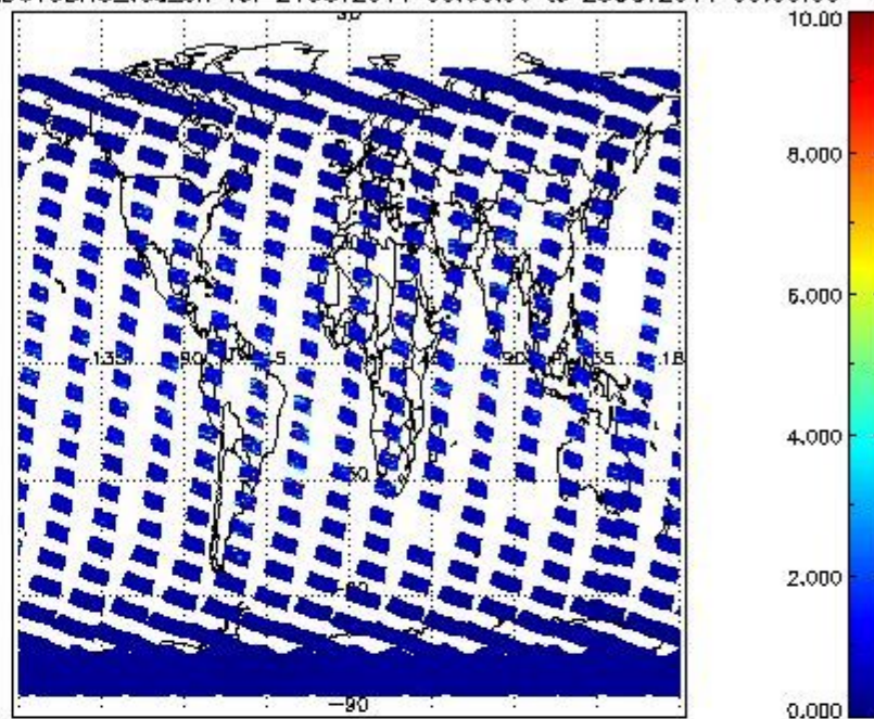
SCIOL2P_NADUV3BRO_vcd_err for 24OCT2011 00:00:00 to 25OCT2011 00:00:00
