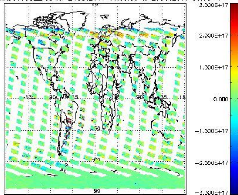
SCIOL2P_NADUV5S02_vcd for 24OCT2011 00:00:00 to 25OCT2011 00:00:00
