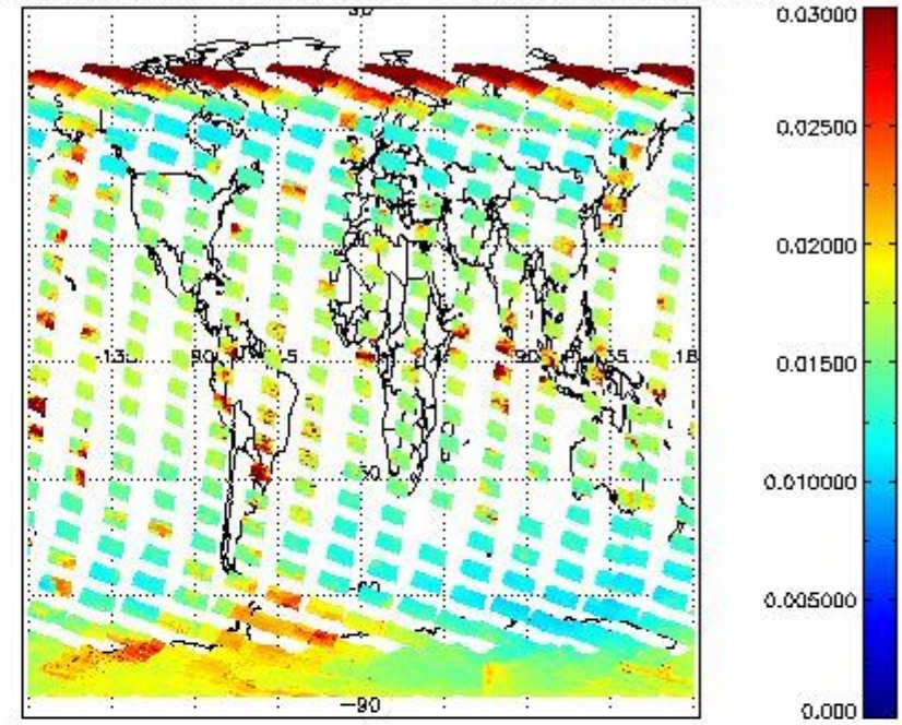
SCIOL2P_NADUV003_vcd_err for 24OCT2011 00:00:00 to 25OCT2011 00:00:00
