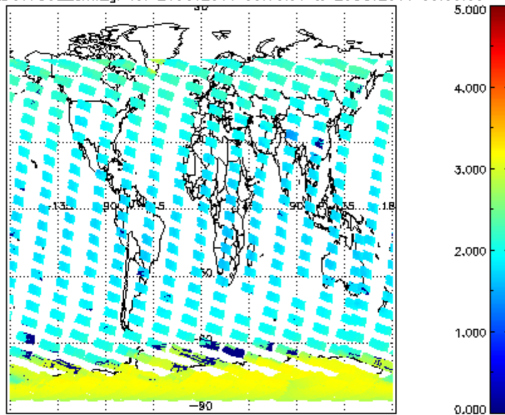
SCIOL2P_NADUV7S02_amf_gr for 24OCT2011 00:00:00 to 25OCT2011 00:00:00
