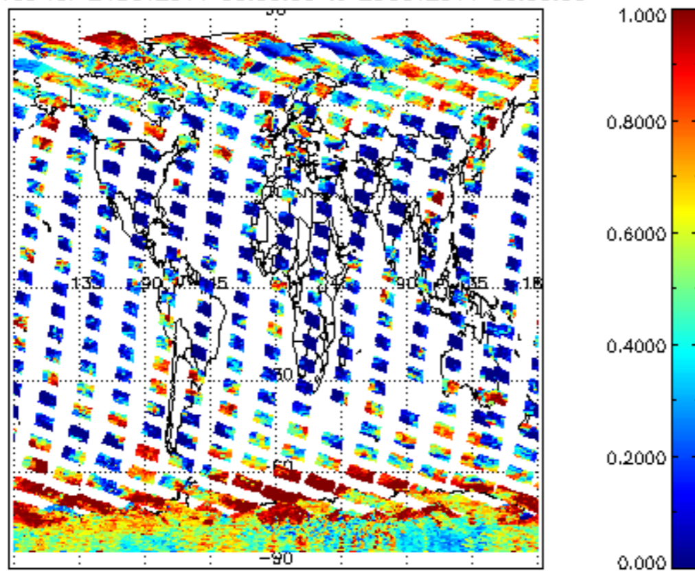
cl_frac for 24OCT2011 00:00:00 to 25OCT2011 00:00:00
