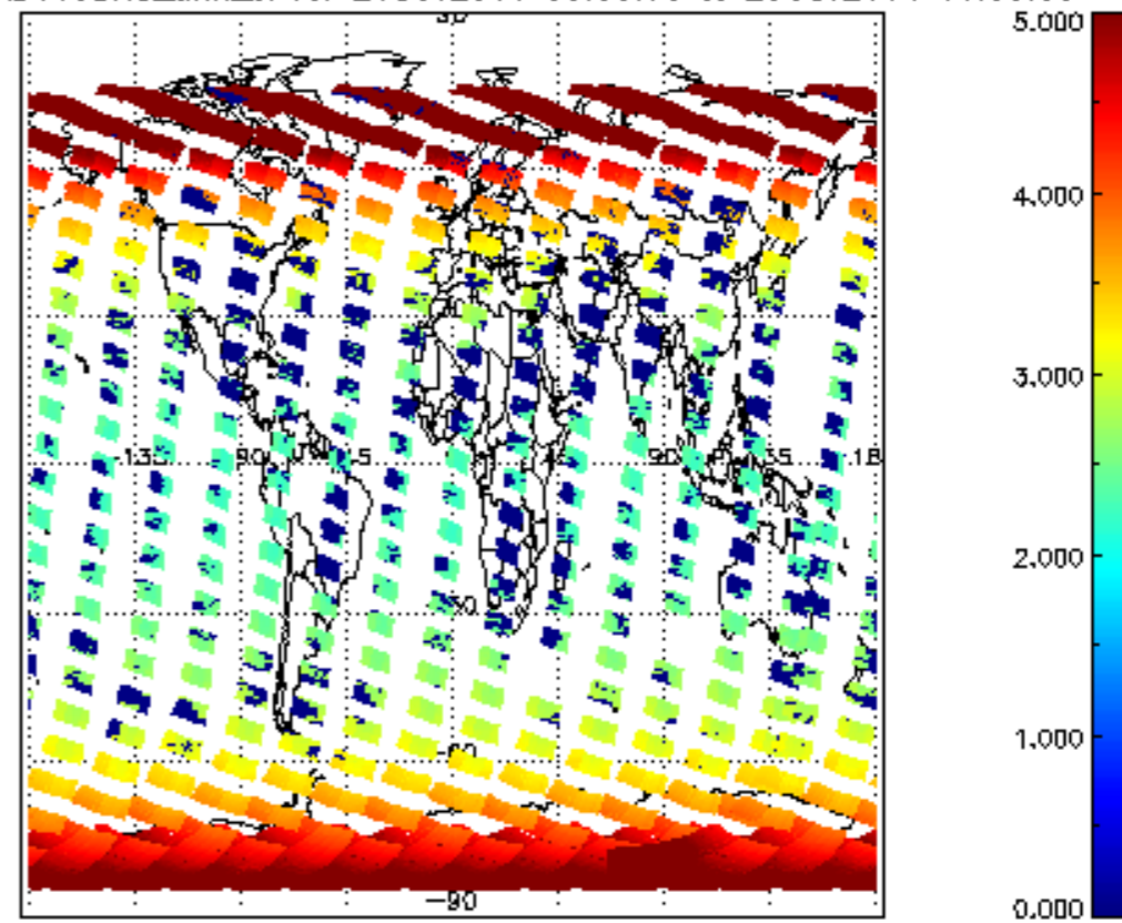
SCIOL2P_NADUV3BRO_amf_cl for 24OCT2011 00:00:00 to 25OCT2011 00:00:00
