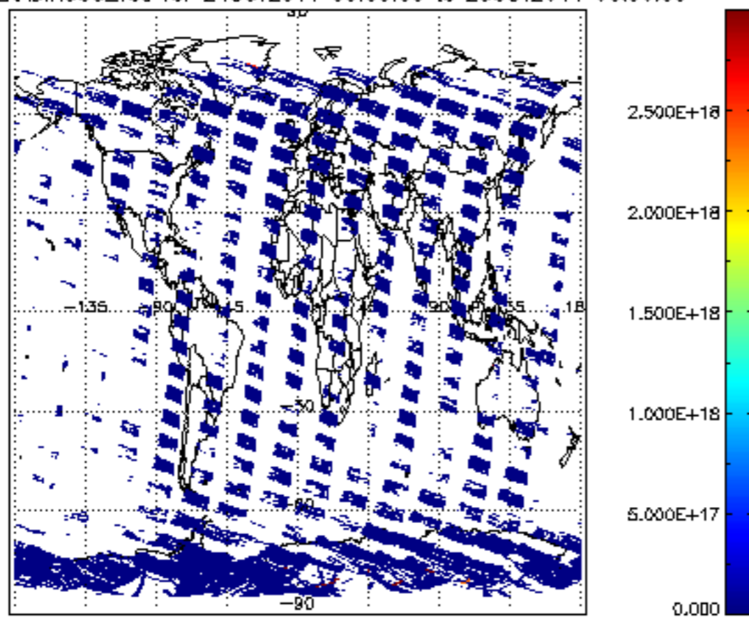
SCIOL2P_NADIR3CO_vcd for 24OCT2011 00:00:00 to 25OCT2011 00:00:00
