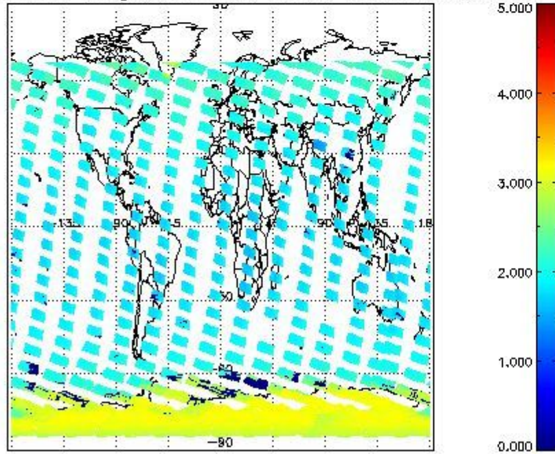
SCIOL2P_NADUV7S02_amf_gr for 24OCT2011 00:00:00 to 25OCT2011 00:00:00
