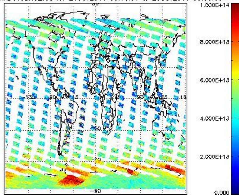
SCIOL2P_NADUV3BRO_vcd for 24OCT2011 00:00:00 to 25OCT2011 00:00:00
