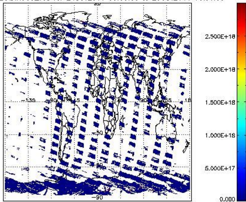
SCIO2P_NADIR3CO_vcd for 24OCT2011 00:00:00 to 25OCT2011 00:00:00
