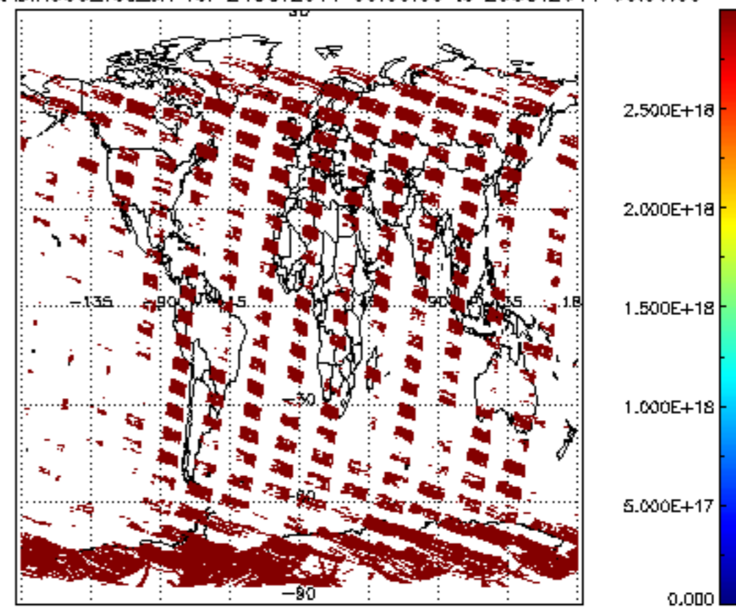
SCIOL2P_NADIR3CO_vcd_err for 24OCT2011 00:00:00 to 25OCT2011 00:00:00
