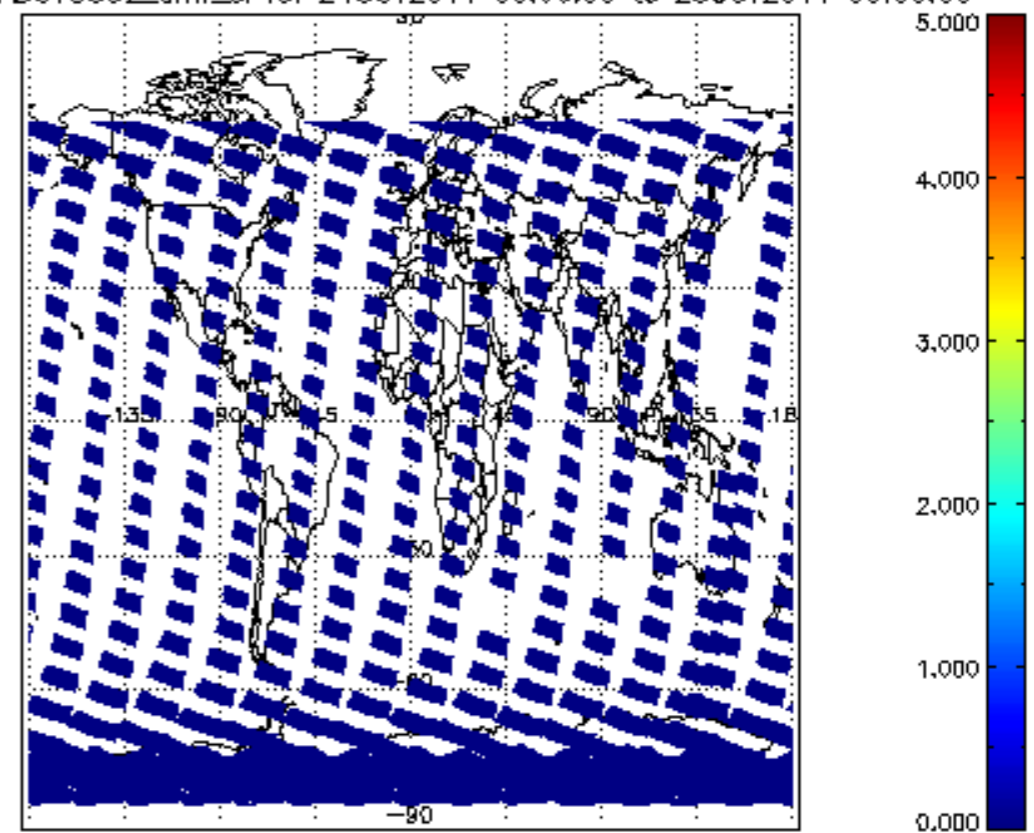
SCIOL2P_NADUV5S02_amf_cl for 24OCT2011 00:00:00 to 25OCT2011 00:00:00
