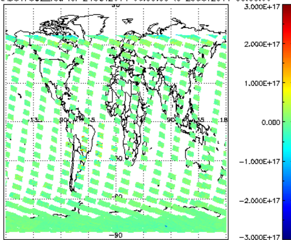
SCIOL2P_NADUV7S02_vcd for 24OCT2011 00:00:00 to 25OCT2011 00:00:00
