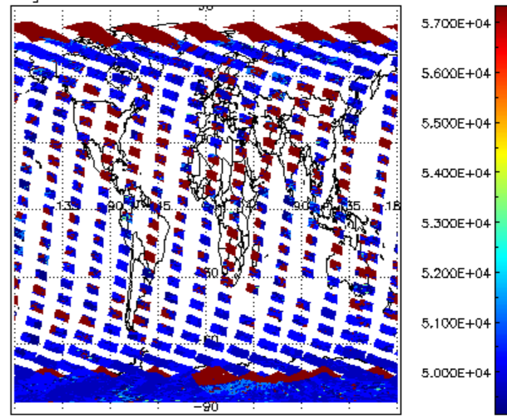
cloud_flags for 24OCT2011 00:00:00 to 25OCT2011 00:00:00
