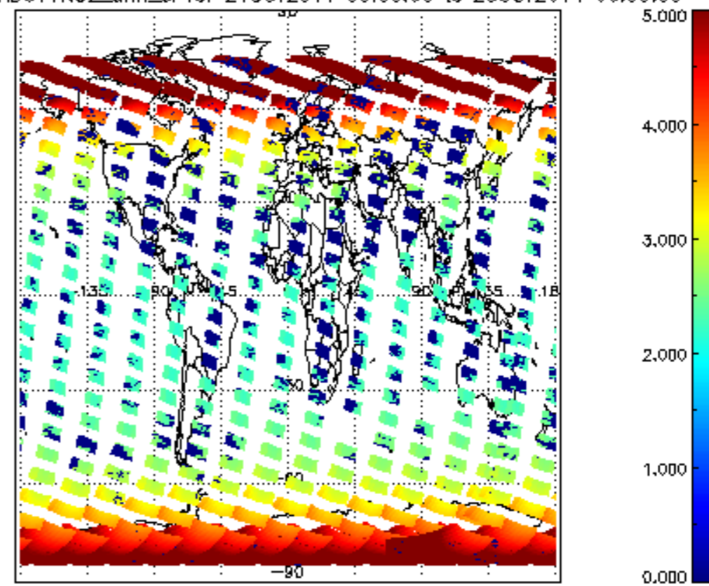
SCIOL2P_NADUV1NO2_amf_cl for 24OCT2011 00:00:00 to 25OCT2011 00:00:00
