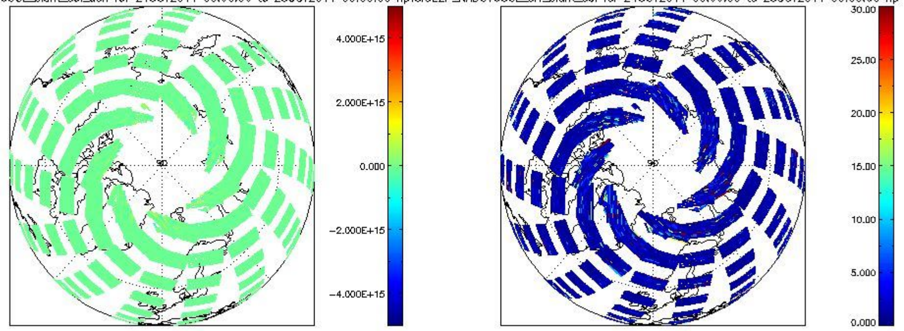
CIOL2P_NADUV60CL_slant_col_den for 24OCT2011 00:00:00 to 25OCT2011 00:00:00 npCIOL2P_NADUV60CL_err_slant_col for 24OCT2011 00:00:00 to 25OCT2011 00:00:00 np
