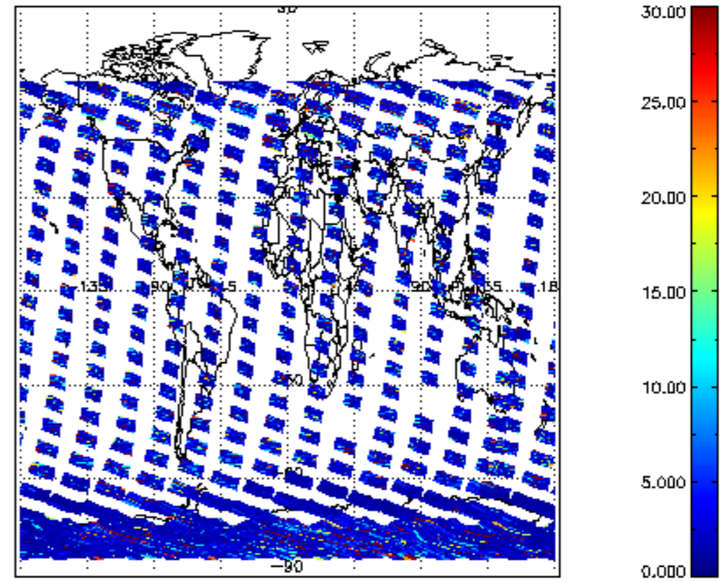
SCIOL2P_NADUV5S02_vcd_err for 24OCT2011 00:00:00 to 25OCT2011 00:00:00
