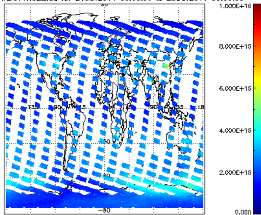
SCIOL2P_NADUV1NO2_vcd for 24OCT2011 00:00:00 to 25OCT2011 00:00:00
