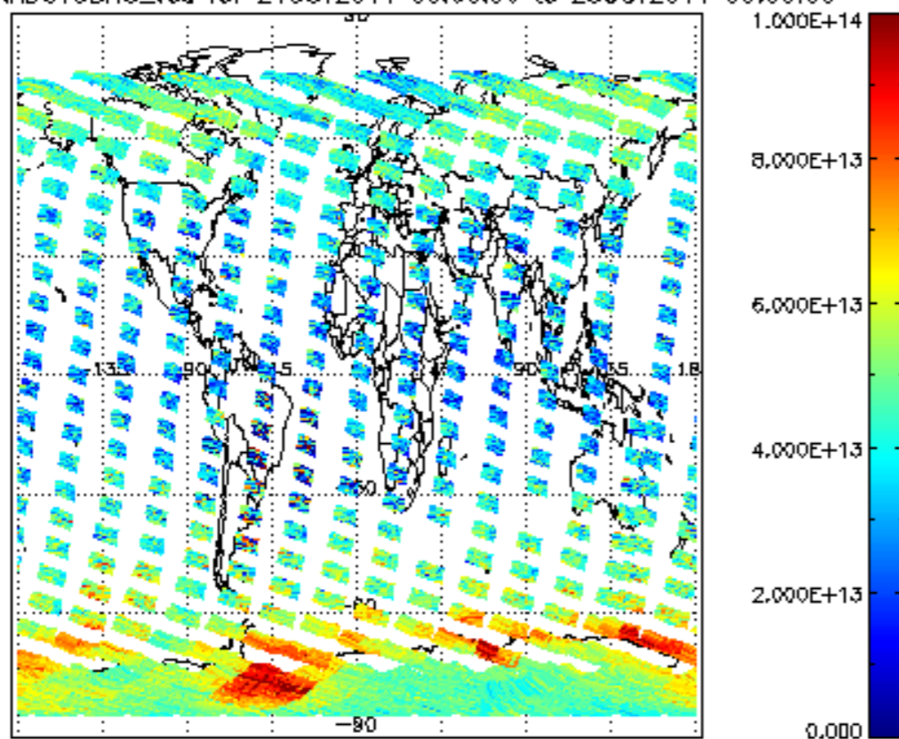
SCIOL2P_NADUV3BRO_vcd for 24OCT2011 00:00:00 to 25OCT2011 00:00:00
