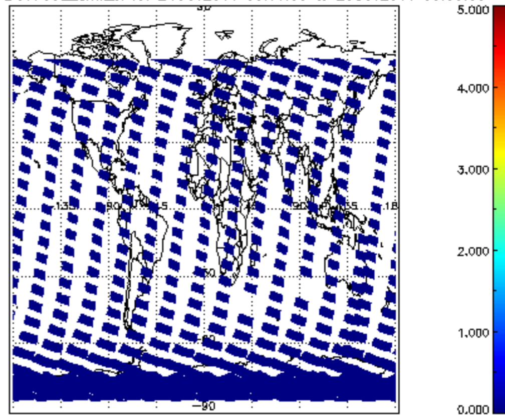
SCIOL2P_NADUV7S02_amf_cl for 24OCT2011 00:00:00 to 25OCT2011 00:00:00
