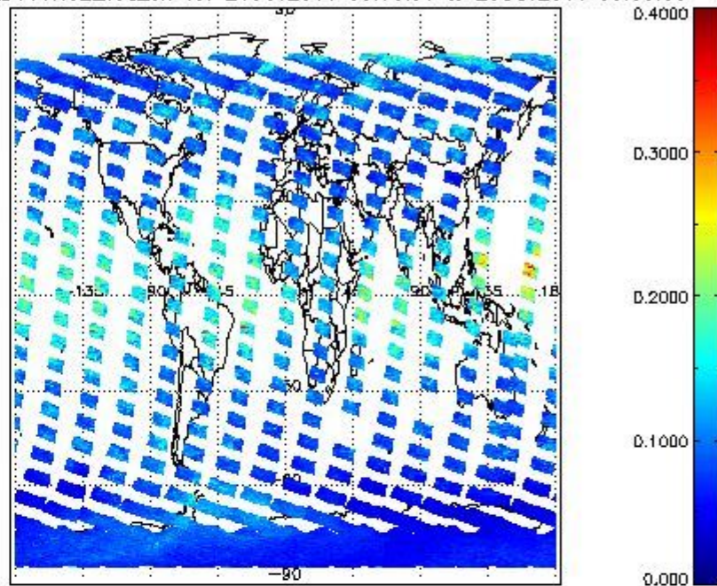
SCIOL2P_NADUV1N02_vcd_err for 24OCT2011 00:00:00 to 25OCT2011 00:00:00
