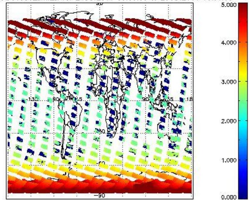
SCIOL2P_NADUV003_amf_cl for 24OCT2011 00:00:00 to 25OCT2011 00:00:00
