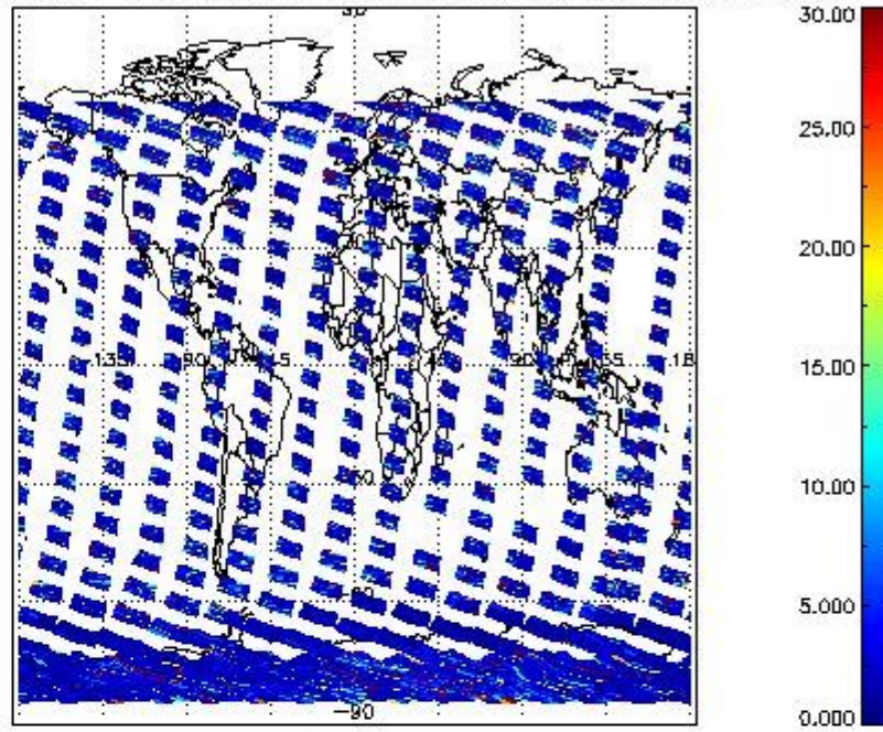
SCIOL2P_NADUV7S02_vcd_err for 24OCT2011 00:00:00 to 25OCT2011 00:00:00
