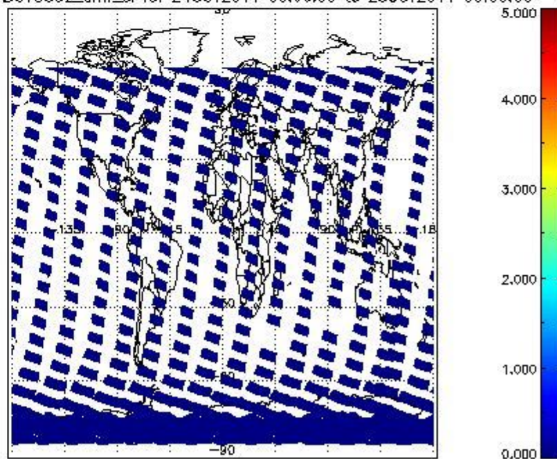
SCIOL2P_NADUV5S02_amf_cl for 24OCT2011 00:00:00 to 25OCT2011 00:00:00
