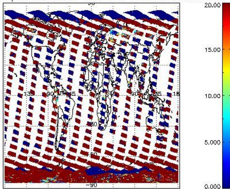
cL_opt_depth for 24OCT2011 00:00:00 to 25OCT2011 00:00:00
