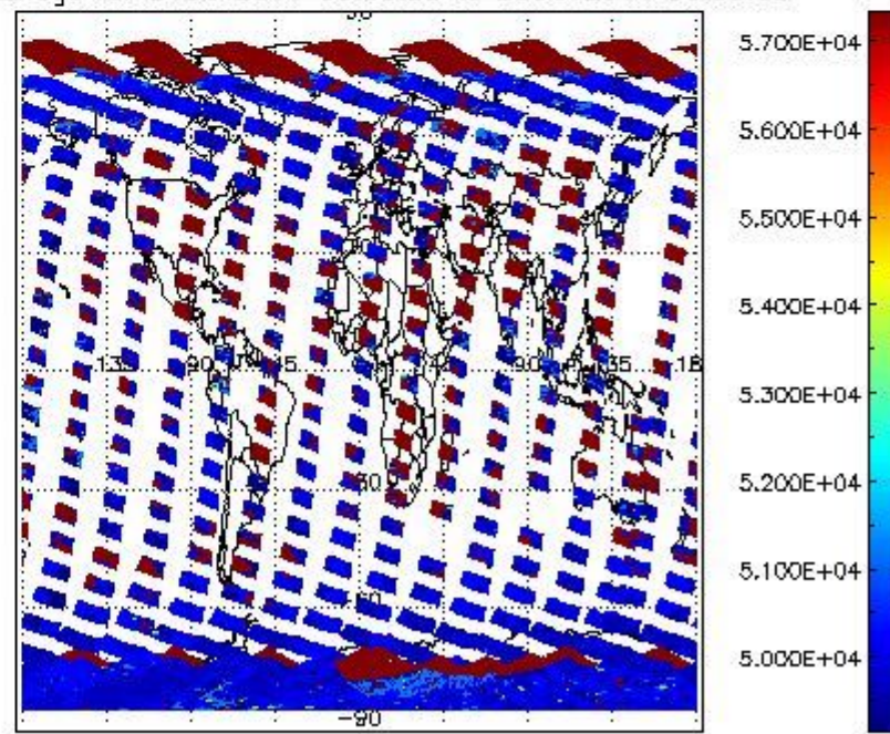
cloud_flags for 24OCT2011 00:00:00 to 25OCT2011 00:00:00
