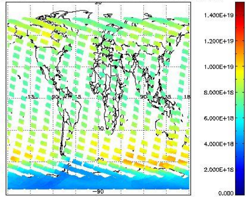
SCIOL2P_NADUV003_vcd for 24OCT2011 00:00:00 to 25OCT2011 00:00:00
