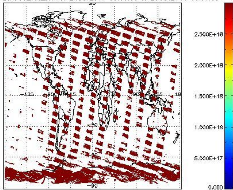
SCIO2P_NADIR3CO_vcd_err for 24OCT2011 00:00:00 to 25OCT2011 00:00:00
