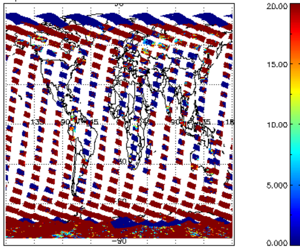
cl_opt_depth for 24OCT2011 00:00:00 to 25OCT2011 00:00:00
