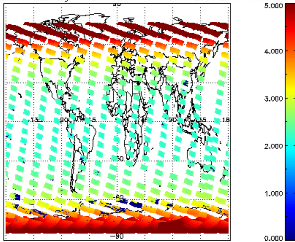
SCIOL2P_NADUV3BRO_amf_gr for 24OCT2011 00:00:00 to 25OCT2011 00:00:00
