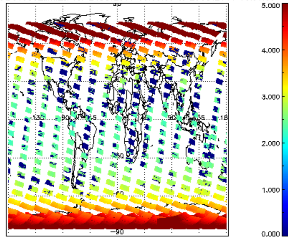
SCIOL2P_NADUV003_amf_cl for 24OCT2011 00:00:00 to 25OCT2011 00:00:00
