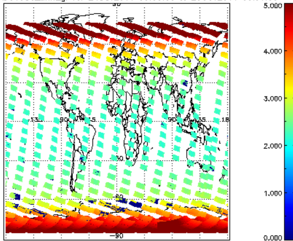
SCIOL2P_NADUV003_amf_gr for 24OCT2011 00:00:00 to 25OCT2011 00:00:00
