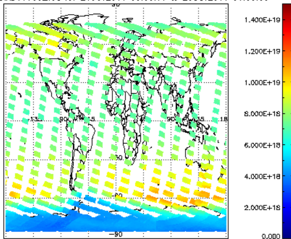
SCIOL2P_NADUV003_vcd for 24OCT2011 00:00:00 to 25OCT2011 00:00:00
