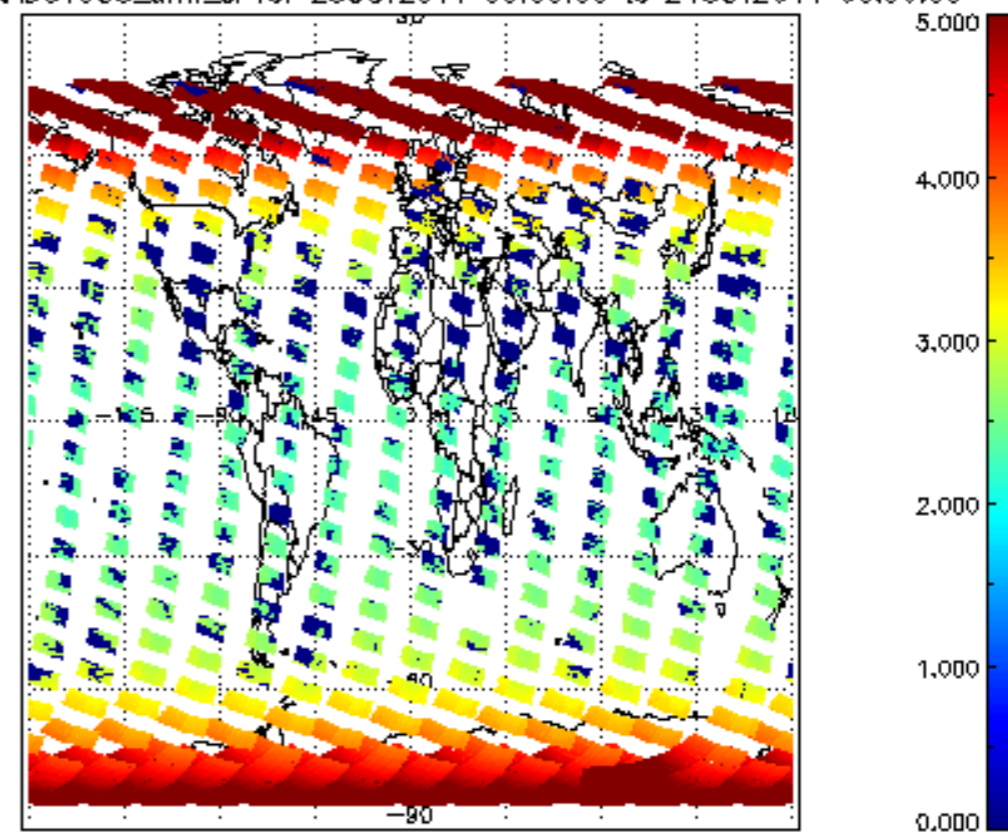
SCIOL2P_NADUV003_amf_cl for 23OCT2011 00:00:00 to 24OCT2011 00:00:00
