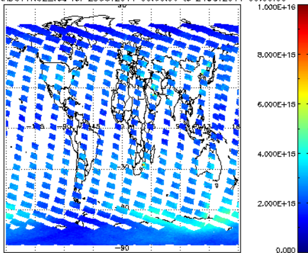
SCIOL2P_NADUV1NO2_vcd for 23OCT2011 00:00:00 to 24OCT2011 00:00:00
