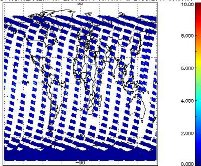
SCIOL2P_NADUV3BRO_vcd_err for 23OCT2011 00:00:00 to 24OCT2011 00:00:00
