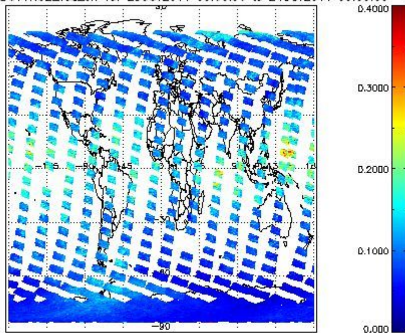
SCIOL2P_NADUV1NO2_vcd_err for 23OCT2011 00:00:00 to 24OCT2011 00:00:00
