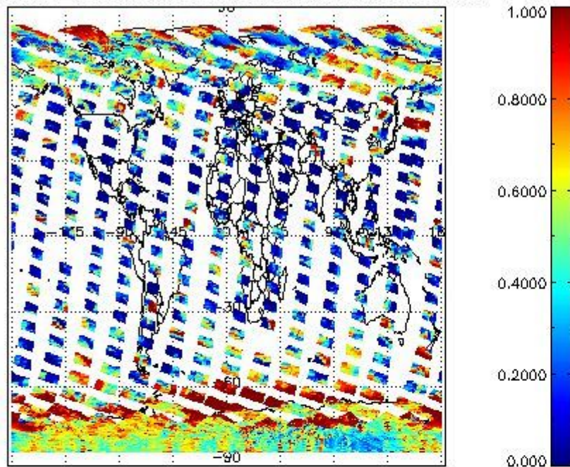
cLfrac for 23OCT2011 00:00:00 to 24OCT2011 00:00:00
