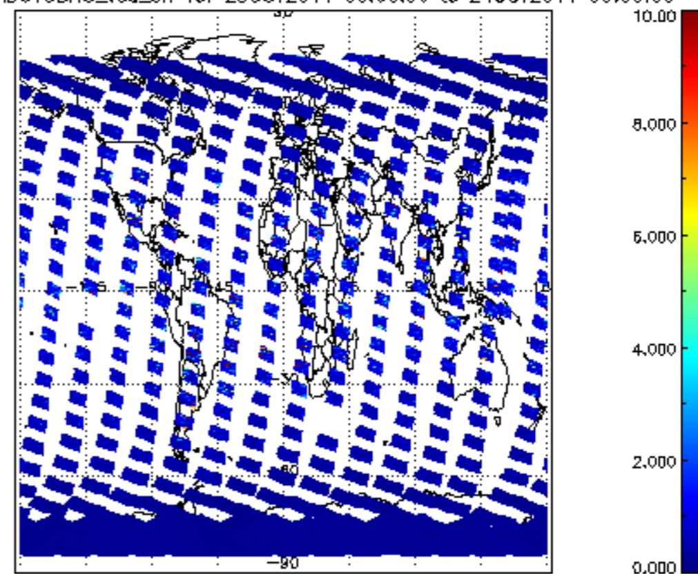
SCIOL2P_NADUV3BRO_vcd_err for 23OCT2011 00:00:00 to 24OCT2011 00:00:00
