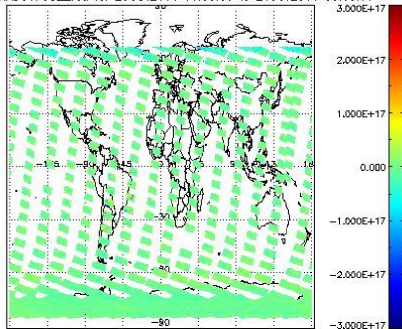
SCIOL2P_NADUV7S02_vcd for 23OCT2011 00:00:00 to 24OCT2011 00:00:00
