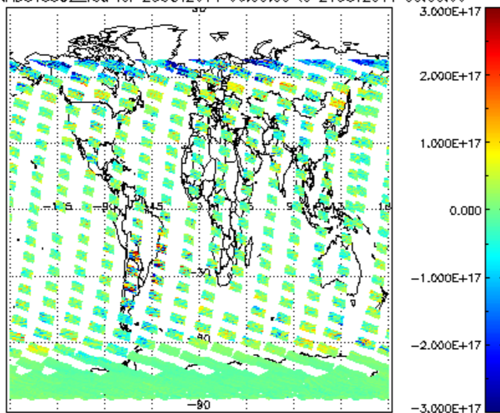
SCIOL2P_NADUV5S02_vcd for 23OCT2011 00:00:00 to 24OCT2011 00:00:00
