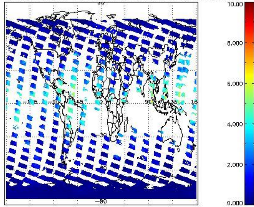
SCIOL2P_NADUV8H2O_vcd for 23OCT2011 00:00:00 to 24OCT2011 00:00:00
