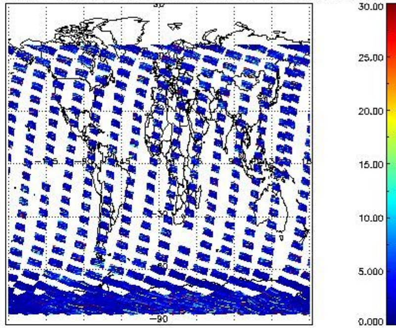
SCIOL2P_NADUV5S02_vcd_err for 23OCT2011 00:00:00 to 24OCT2011 00:00:00
