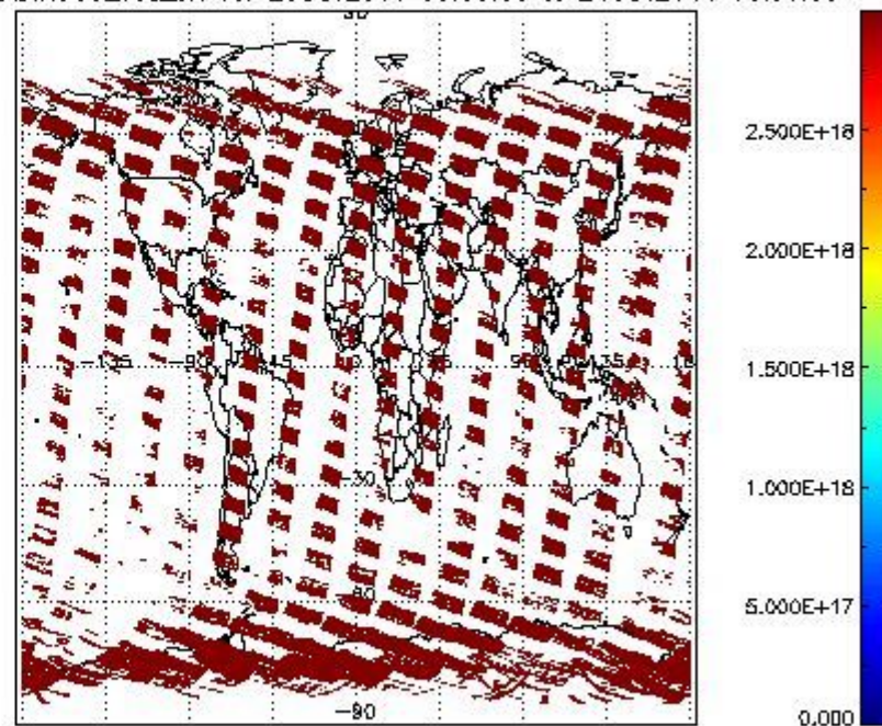
SCIO2P_NADIR3CO_vcd_err for 23OCT2011 00:00:00 to 24OCT2011 00:00:00
