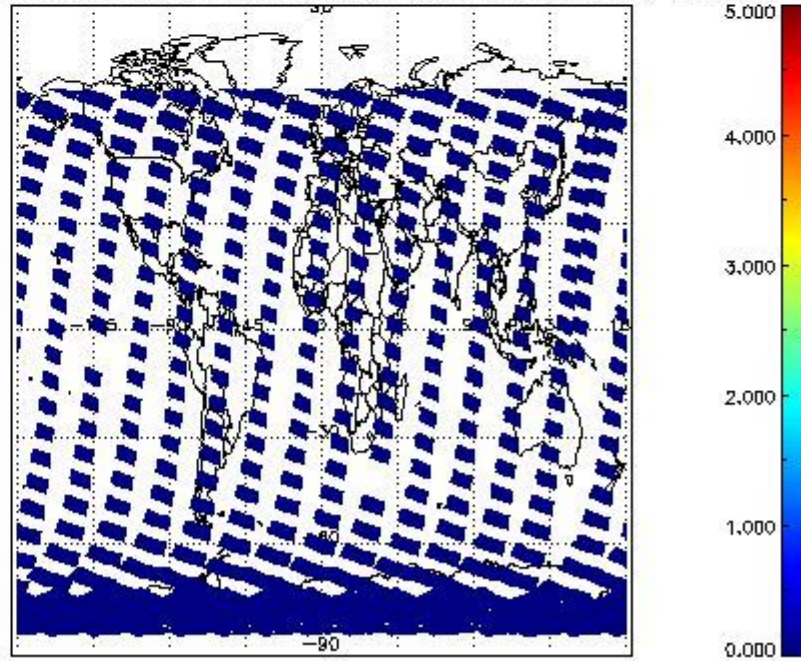
SCIOL2P_NADUV5S02_amf_cl for 23OCT2011 00:00:00 to 24OCT2011 00:00:00
