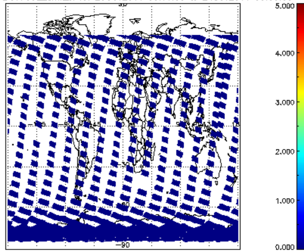
SCIOL2P_NADUV7S02_amf_sl for 23OCT2011 00:00:00 to 24OCT2011 00:00:00
