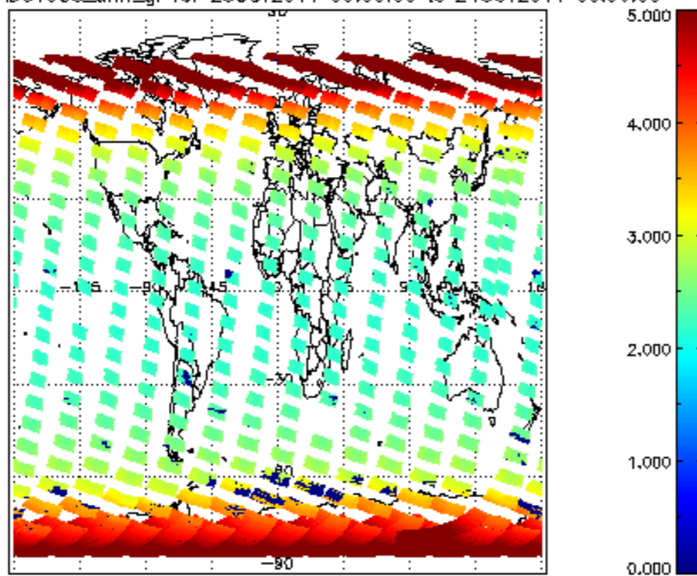
SCIOL2P_NADUV003_amf_gr for 23OCT2011 00:00:00 to 24OCT2011 00:00:00
