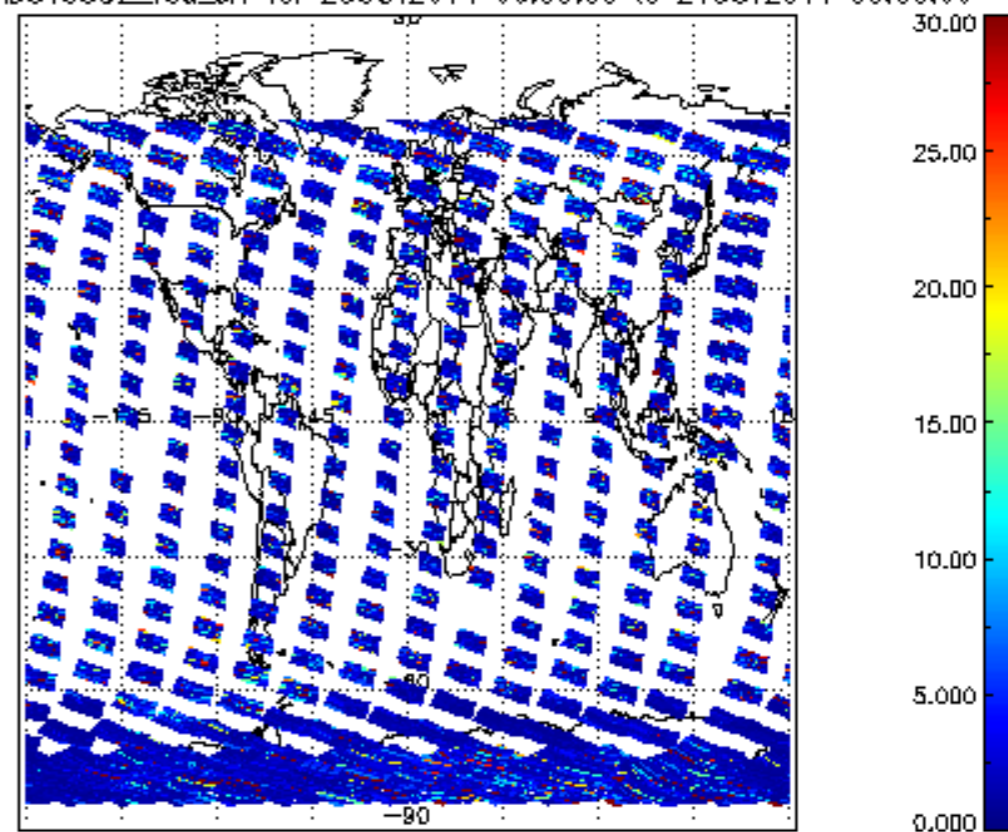
SCIOL2P_NADUV5S02_vcd_err for 23OCT2011 00:00:00 to 24OCT2011 00:00:00
