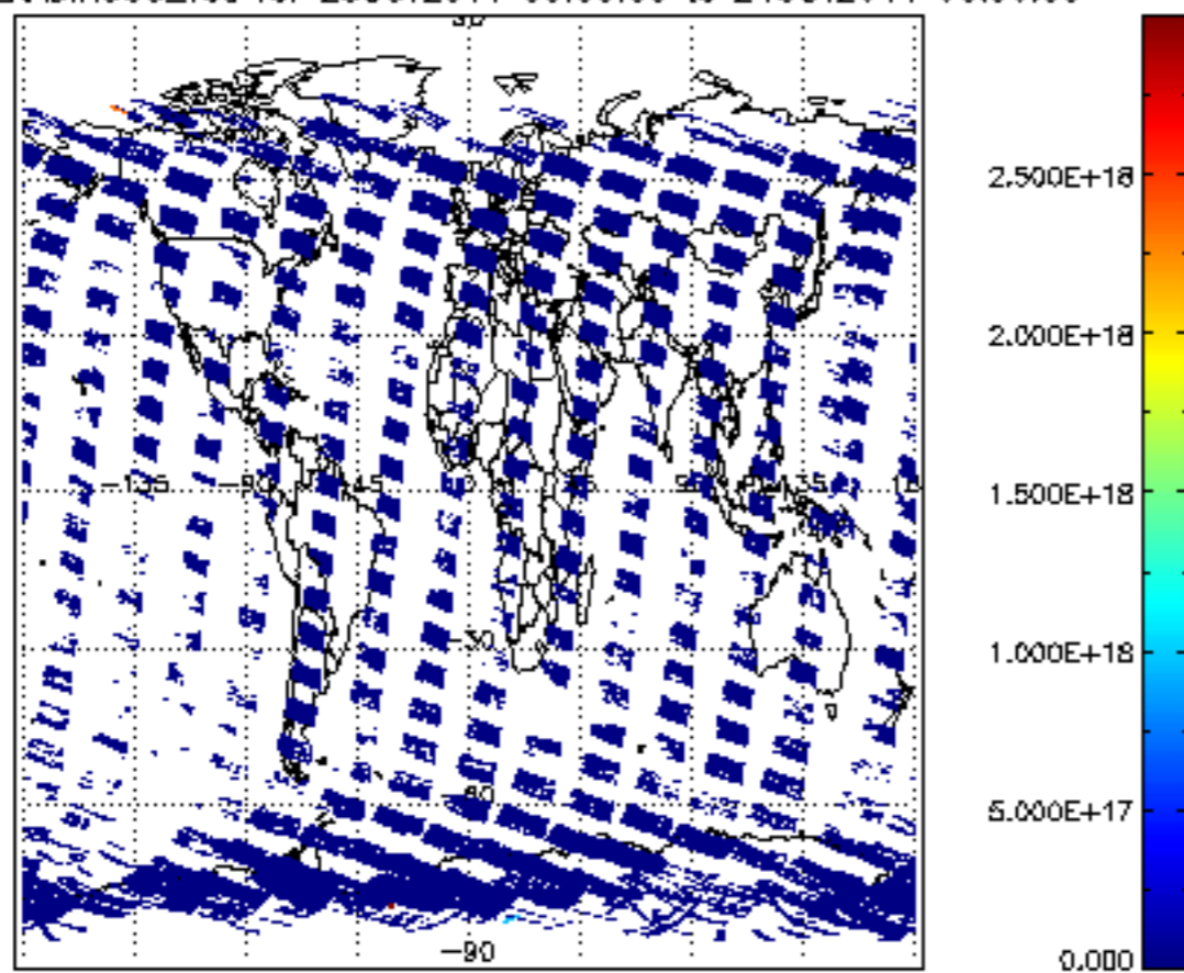
SCIOL2P_NADIR3CO_vcd for 23OCT2011 00:00:00 to 24OCT2011 00:00:00
