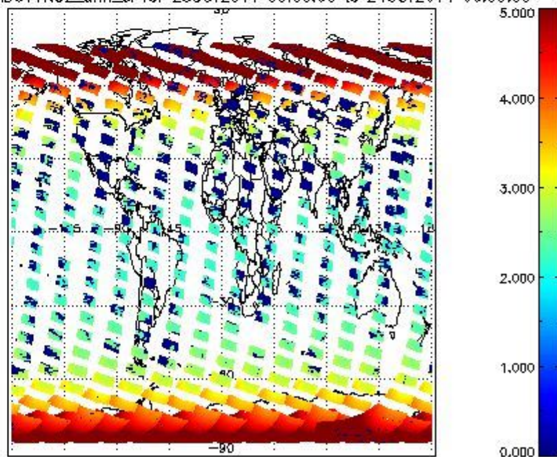
SCIOL2P_NADUV1NO2_amf_cl for 23OCT2011 00:00:00 to 24OCT2011 00:00:00
