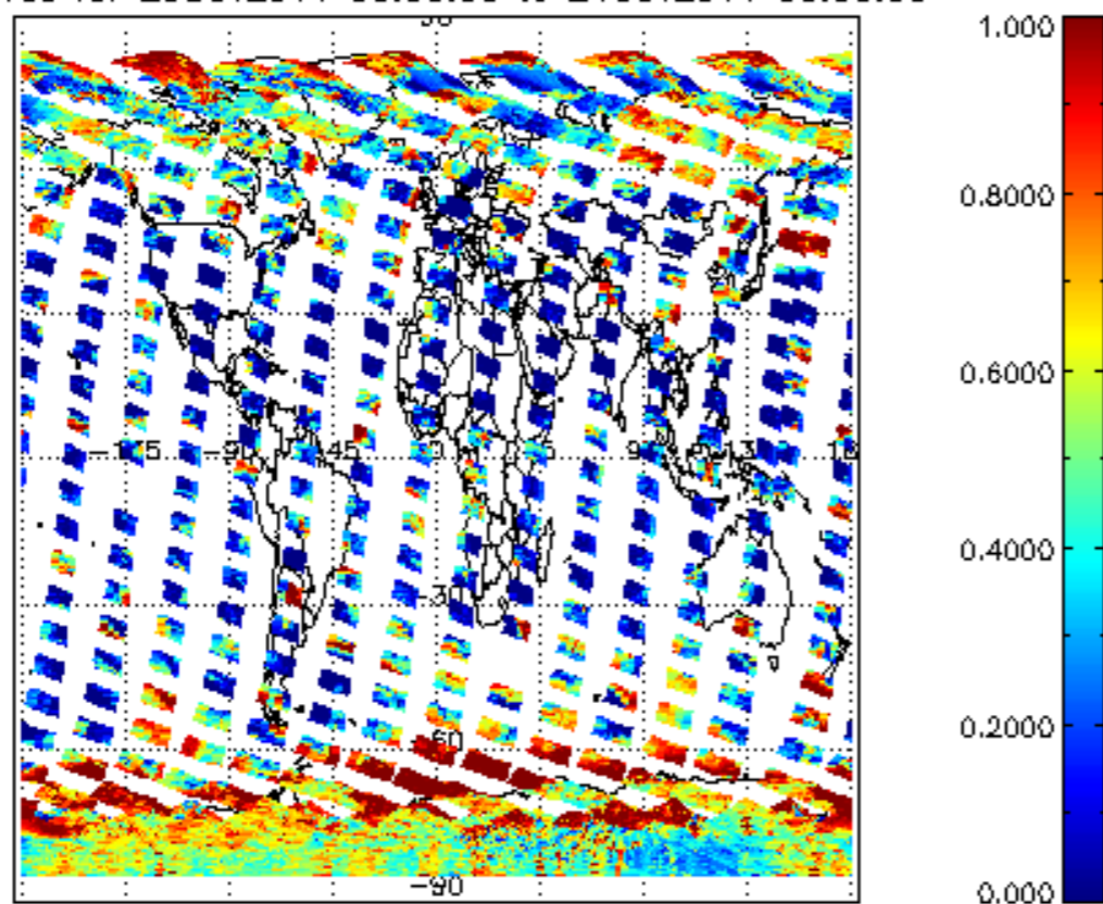
cl_frac for 23OCT2011 00:00:00 to 24OCT2011 00:00:00
