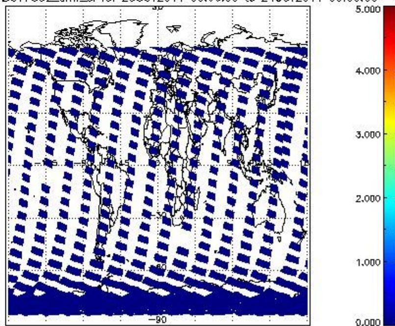
SCIOL2P_NADUV7S02_amf_cl for 23OCT2011 00:00:00 to 24OCT2011 00:00:00
