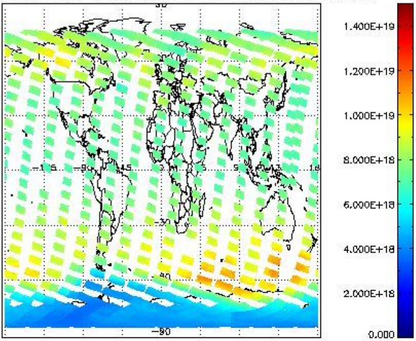
SCIOL2P_NADUV003_vcd for 23OCT2011 00:00:00 to 24OCT2011 00:00:00
