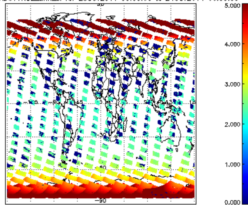
SCIOL2P_NADUV1NO2_amf_cl for 23OCT2011 00:00:00 to 24OCT2011 00:00:00
