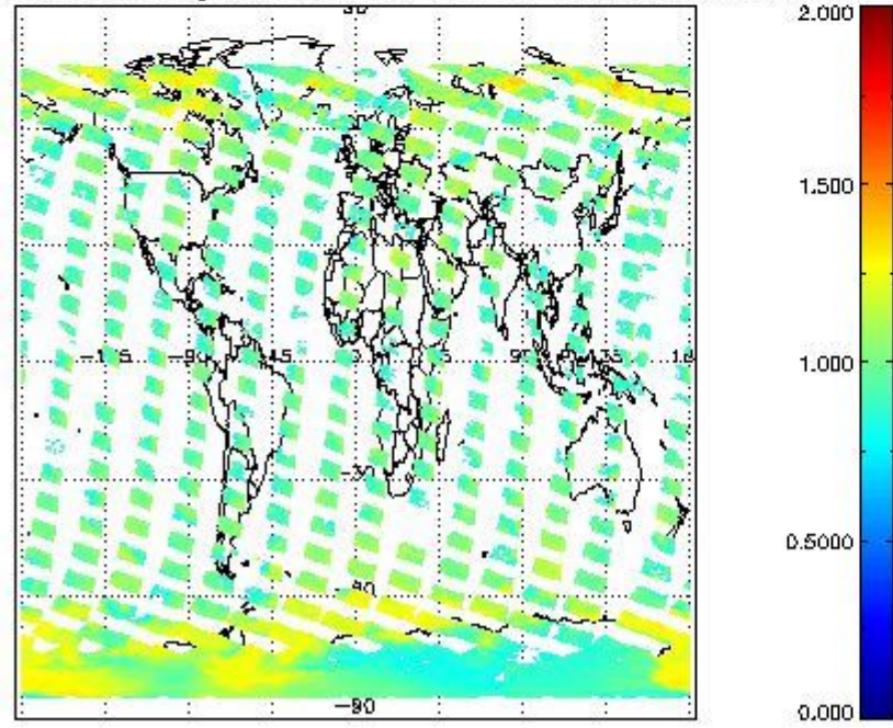
SCIOL2P_NADUV8H2O_amf_gr for 23OCT2011 00:00:00 to 24OCT2011 00:00:00
