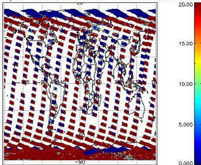
cL_opt_depth for 23OCT2011 00:00:00 to 24OCT2011 00:00:00
