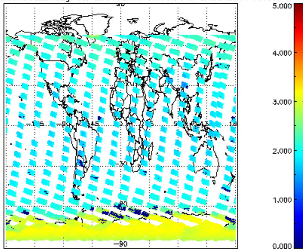
SCIOL2P_NADUV7S02_amf_gr for 23OCT2011 00:00:00 to 24OCT2011 00:00:00
