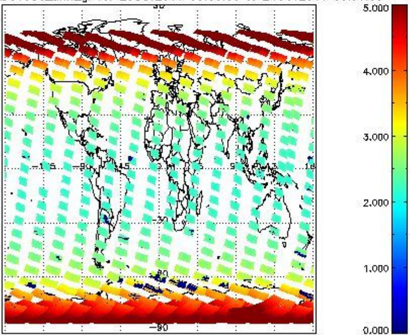
SCIOL2P_NADUV003_amf_gr for 23OCT2011 00:00:00 to 24OCT2011 00:00:00
