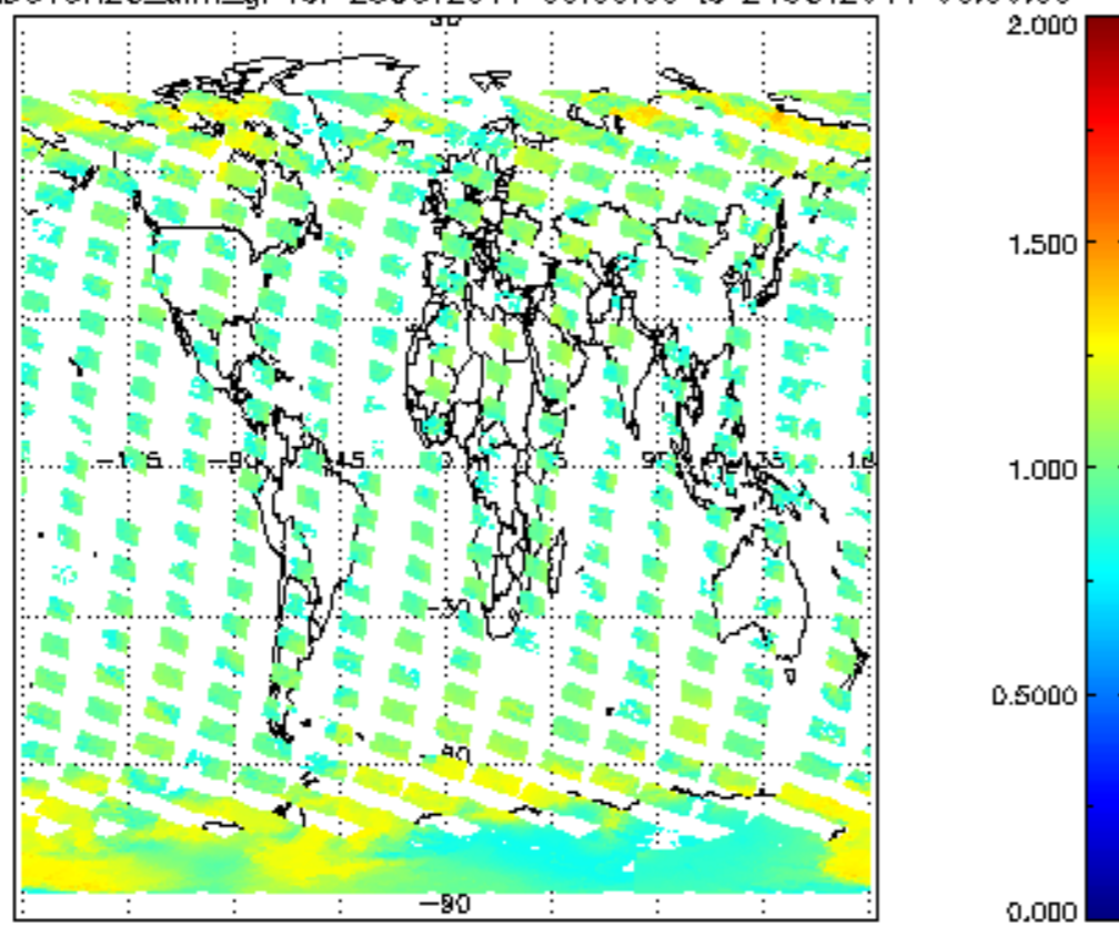
SCIOL2P_NADUV8H20_amf_gr for 23OCT2011 00:00:00 to 24OCT2011 00:00:00
