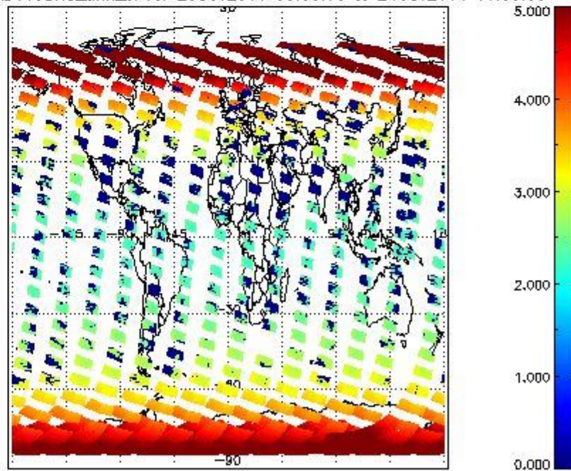
SCIOL2P_NADUV3BRO_amf_cl for 23OCT2011 00:00:00 to 24OCT2011 00:00:00
