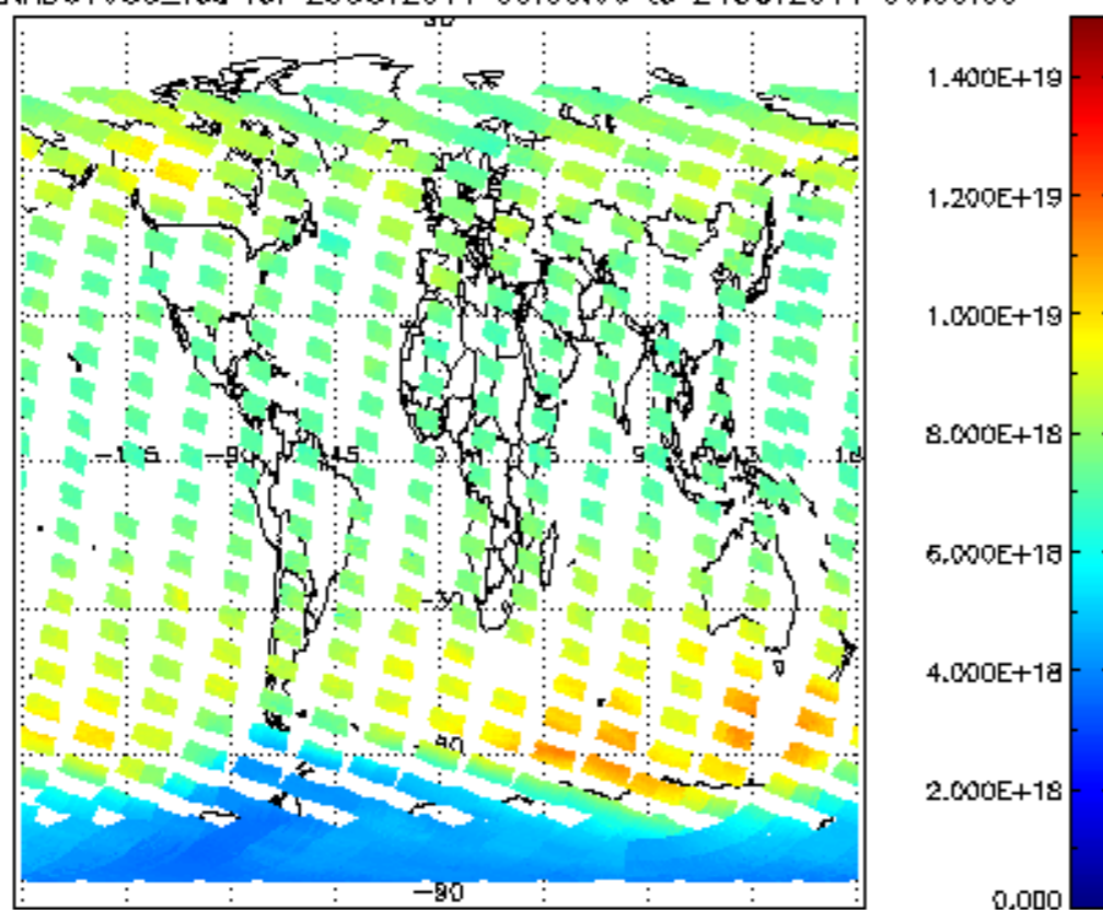
SCIOL2P_NADUV003_vcd for 23OCT2011 00:00:00 to 24OCT2011 00:00:00
