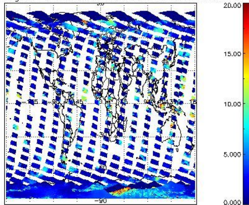
cL_top_height for 23OCT2011 00:00:00 to 24OCT2011 00:00:00
