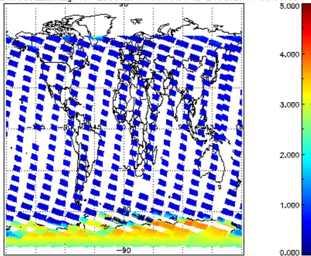
SCIOL2P_NADUV5S02_amf_gr for 23OCT2011 00:00:00 to 24OCT2011 00:00:00
