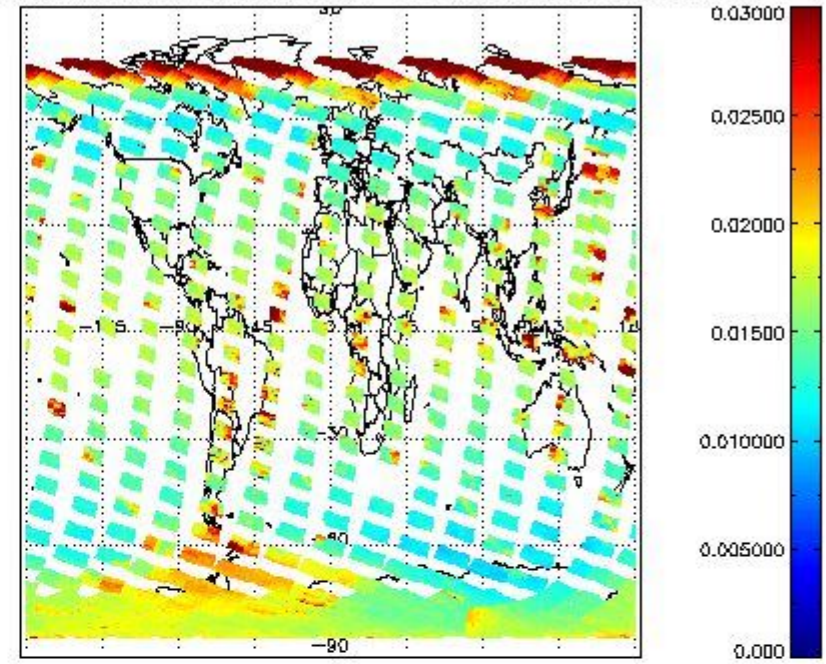
SCIOL2P_NADUV003_vcd_err for 23OCT2011 00:00:00 to 24OCT2011 00:00:00
