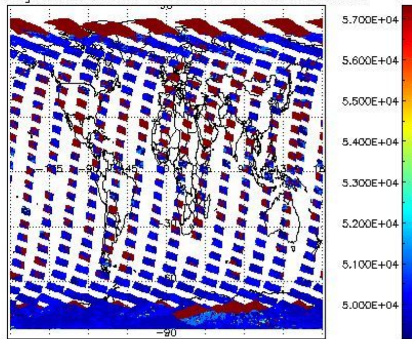
cloud_flags for 23OCT2011 00:00:00 to 24OCT2011 00:00:00
