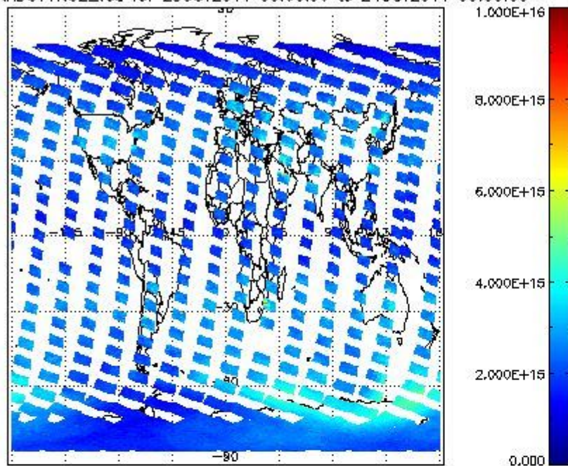
SCIOL2P_NADUV1NO2_vcd for 23OCT2011 00:00:00 to 24OCT2011 00:00:00
