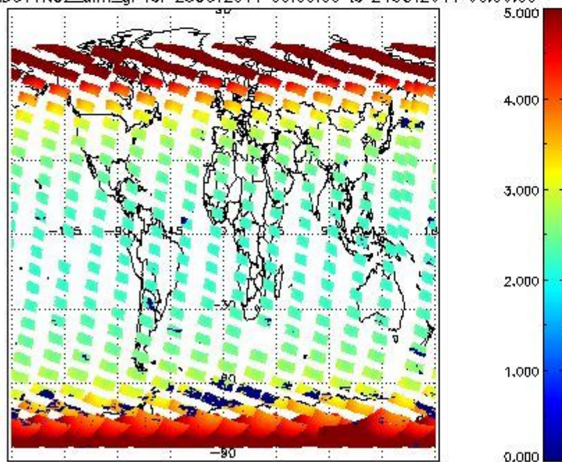
SCIOL2P_NADUV1NO2_amf_gr for 23OCT2011 00:00:00 to 24OCT2011 00:00:00
