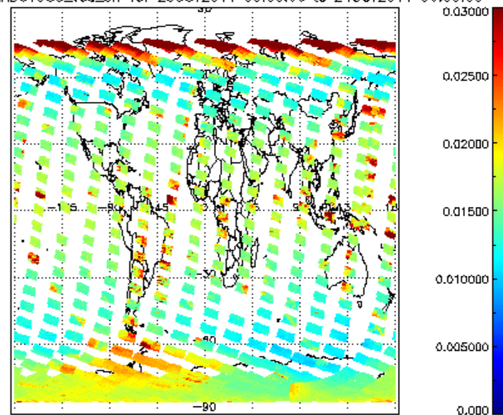
SCIOL2P_NADUV003_vcd_err for 23OCT2011 00:00:00 to 24OCT2011 00:00:00
