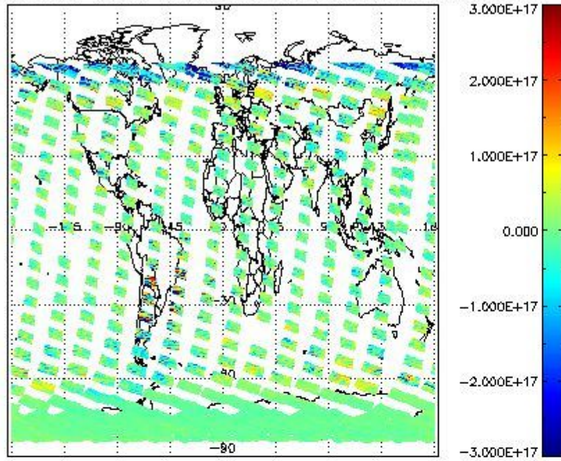
SCIOL2P_NADUV5S02_vcd for 23OCT2011 00:00:00 to 24OCT2011 00:00:00
