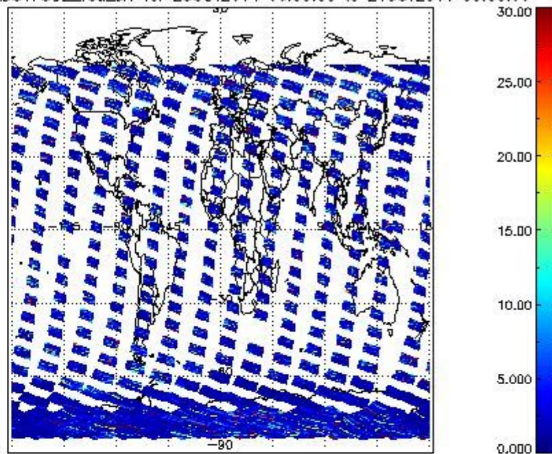
SCIOL2P_NADUV7S02_vcd_err for 23OCT2011 00:00:00 to 24OCT2011 00:00:00
