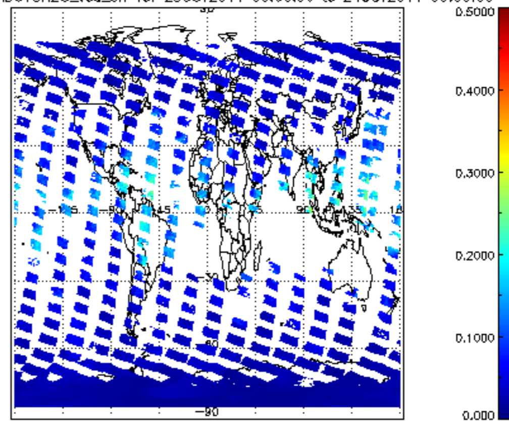
SCIOL2P_NADUV8H20_vcd_err for 23OCT2011 00:00:00 to 24OCT2011 00:00:00
