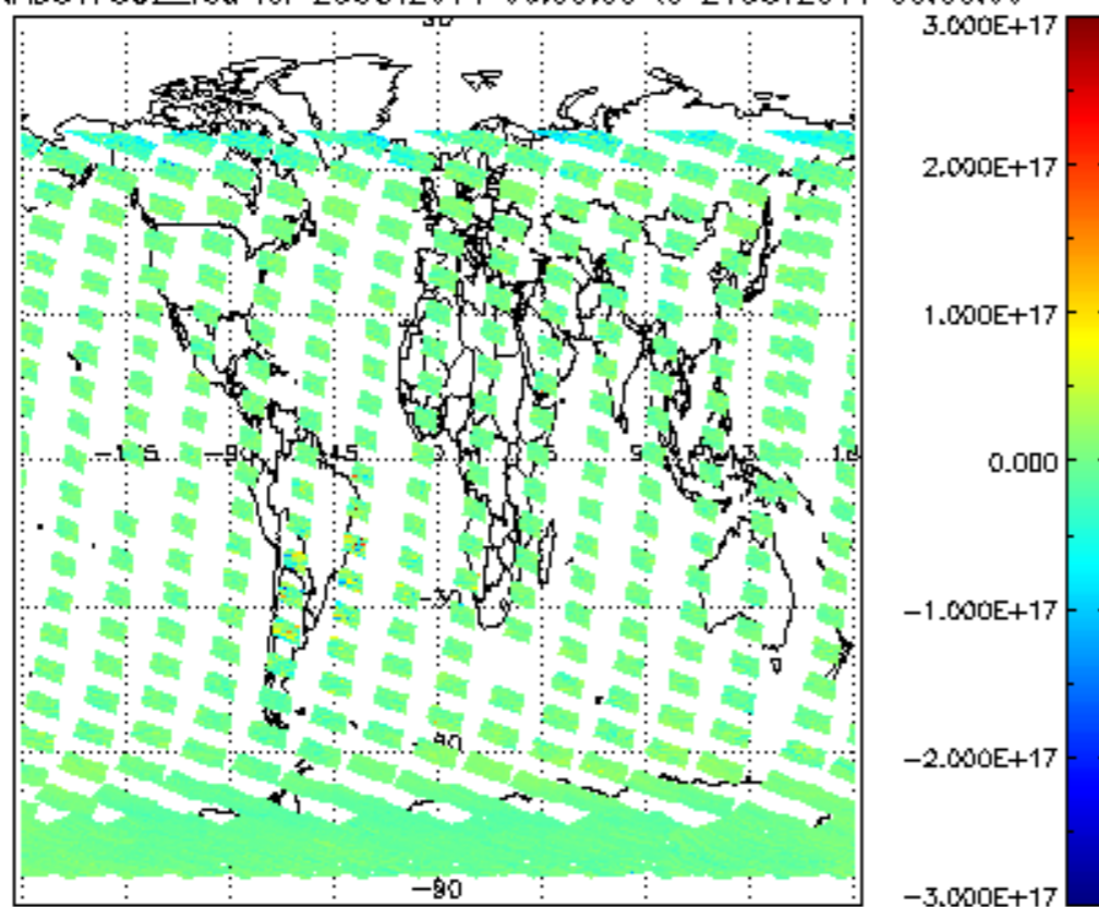
SCIOL2P_NADUV7S02_vcd for 23OCT2011 00:00:00 to 24OCT2011 00:00:00
