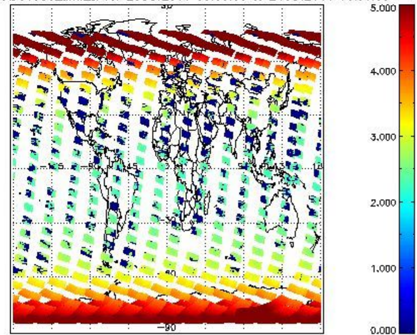
SCIOL2P_NADUV003_amf_cl for 23OCT2011 00:00:00 to 24OCT2011 00:00:00
