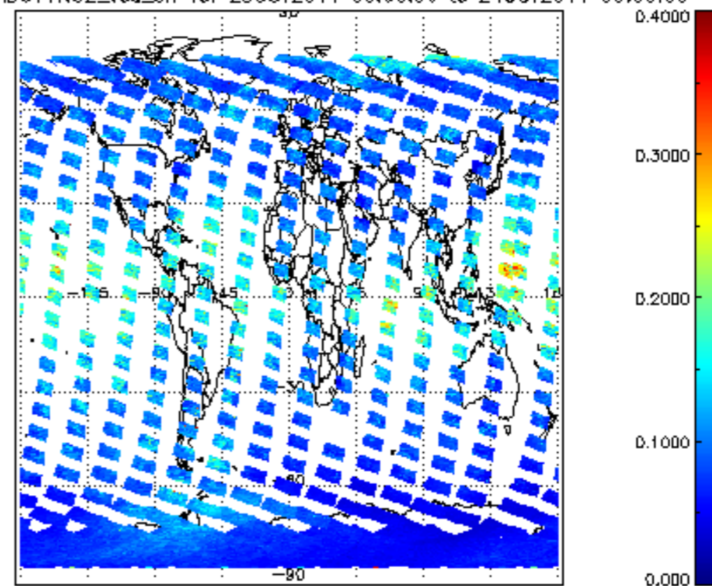
SCIOL2P_NADUV1NO2_vcd_err for 23OCT2011 00:00:00 to 24OCT2011 00:00:00
