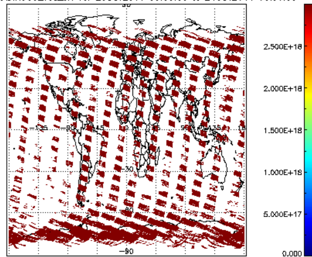
SCIOL2P_NADIR3CO_vcd_err for 23OCT2011 00:00:00 to 24OCT2011 00:00:00
