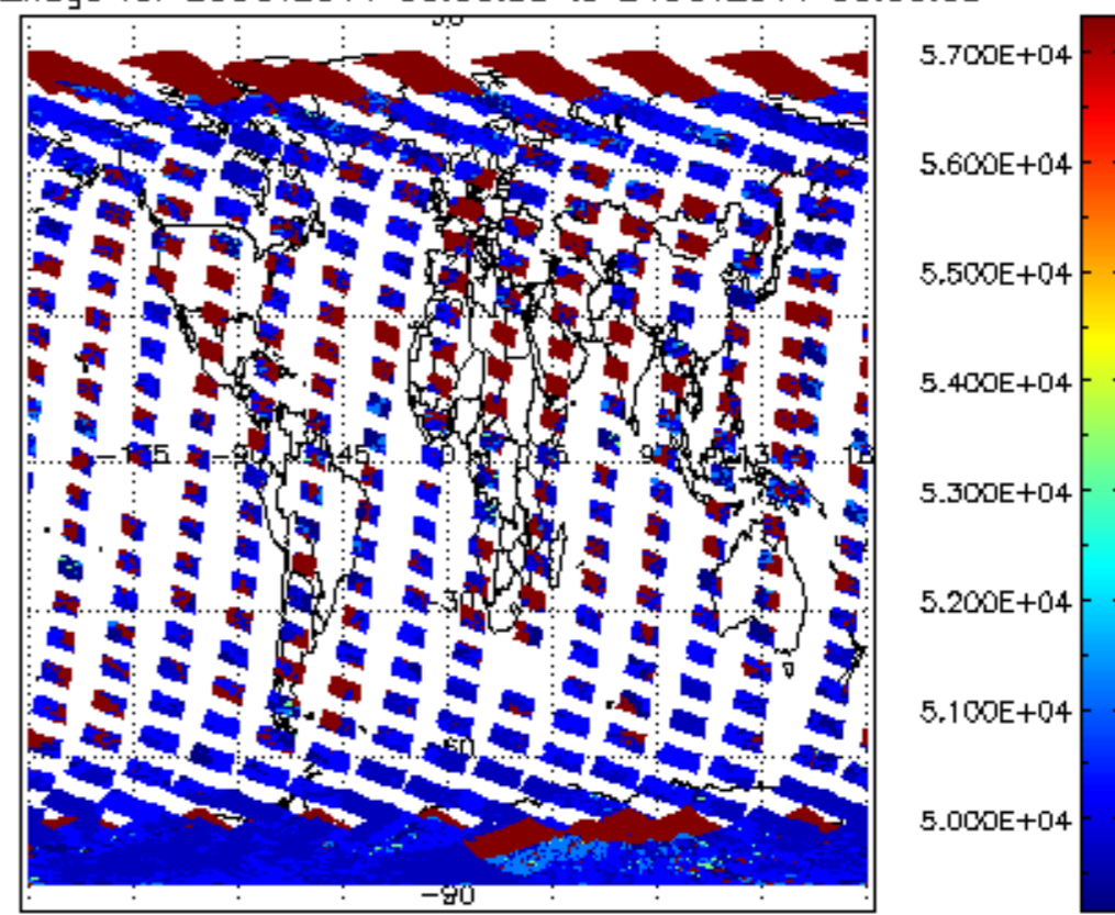
cloud_flags for 23OCT2011 00:00:00 to 24OCT2011 00:00:00
