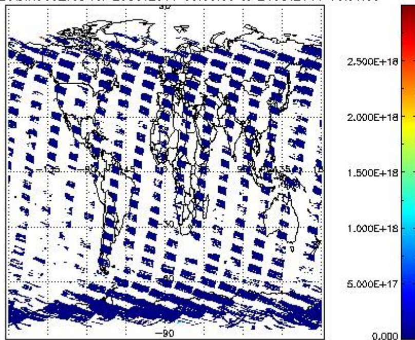
SCIO2P_NADIR3CO_vcd for 23OCT2011 00:00:00 to 24OCT2011 00:00:00
