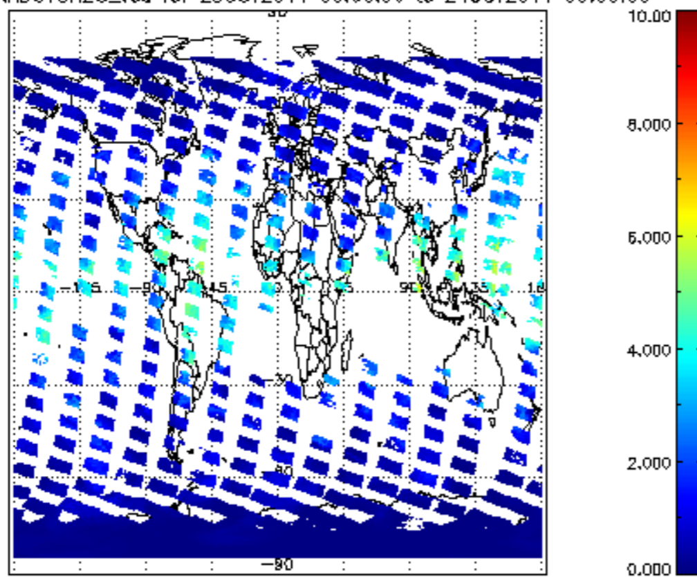
SCIOL2P_NADUV8H20_vcd for 23OCT2011 00:00:00 to 24OCT2011 00:00:00
