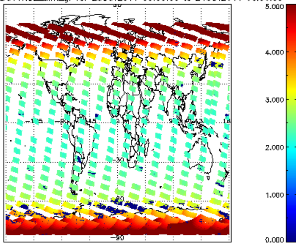
SCIOL2P_NADUV1NO2_amf_gr for 23OCT2011 00:00:00 to 24OCT2011 00:00:00
