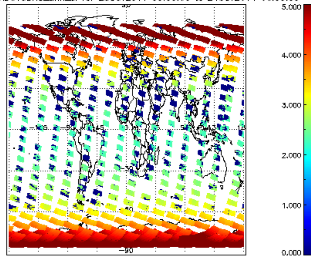
SCIOL2P_NADUV3BRO_amf_cl for 23OCT2011 00:00:00 to 24OCT2011 00:00:00
