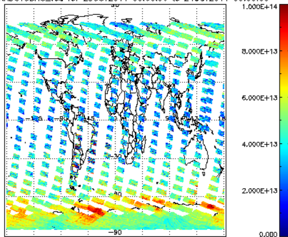
SCIOL2P_NADUV3BRO_vcd for 23OCT2011 00:00:00 to 24OCT2011 00:00:00
