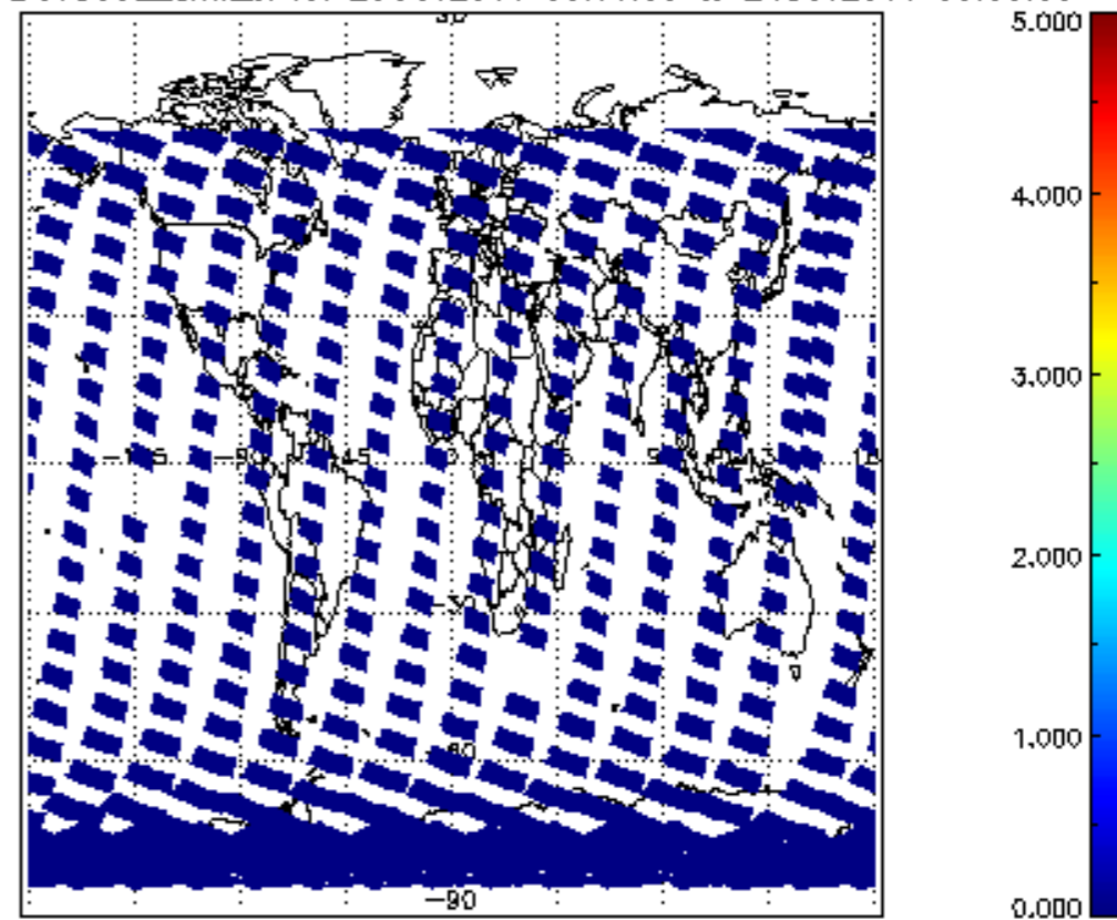
SCIOL2P_NADUV5S02_amf_sl for 23OCT2011 00:00:00 to 24OCT2011 00:00:00
