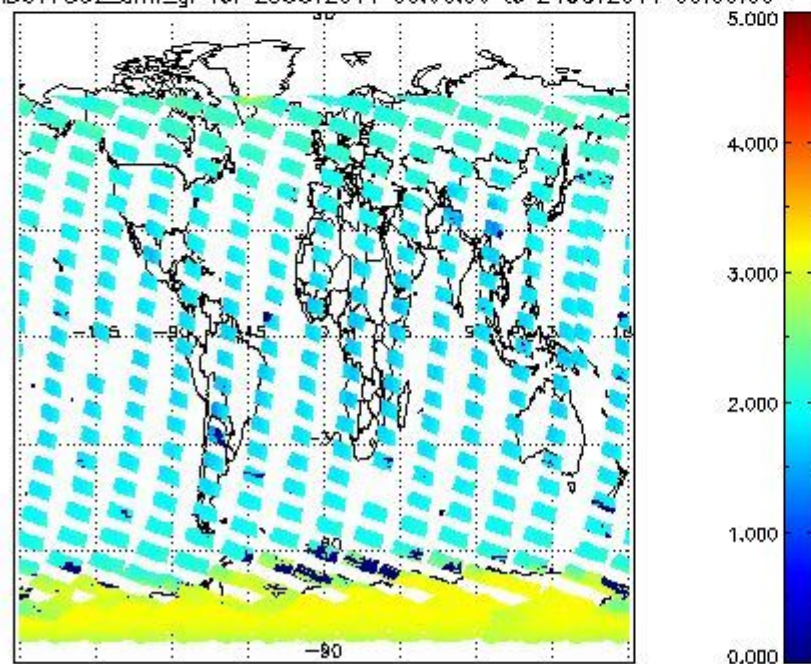
SCIOL2P_NADUV7S02_amf_gr for 23OCT2011 00:00:00 to 24OCT2011 00:00:00
