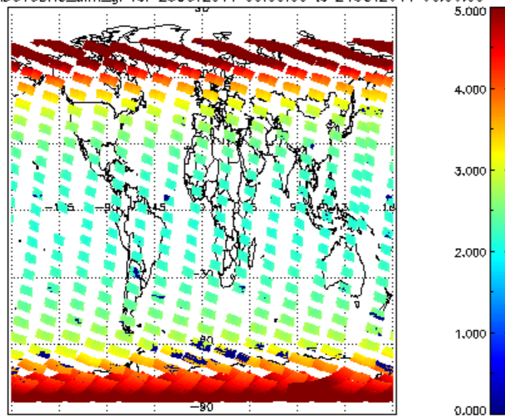
SCIOL2P_NADUV3BRO_amf_gr for 23OCT2011 00:00:00 to 24OCT2011 00:00:00
