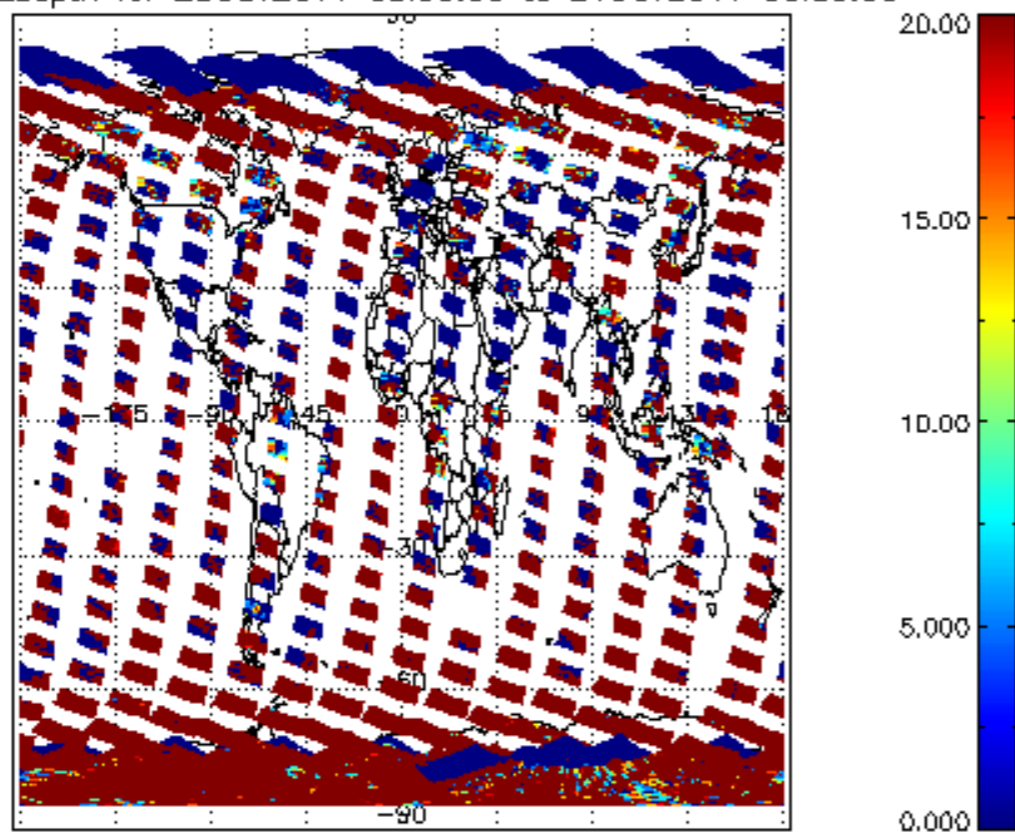
cl_opt_depth for 23OCT2011 00:00:00 to 24OCT2011 00:00:00
