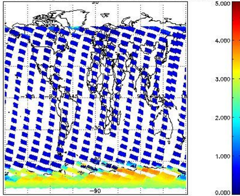
SCIOL2P_NADUV5S02_amf_gr for 23OCT2011 00:00:00 to 24OCT2011 00:00:00
