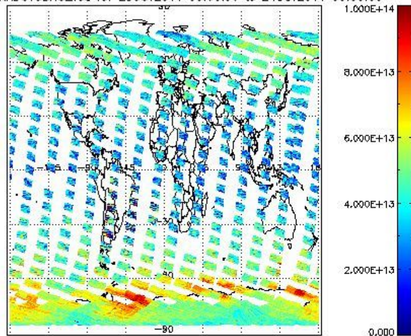
SCIOL2P_NADUV3BRO_vcd for 23OCT2011 00:00:00 to 24OCT2011 00:00:00
