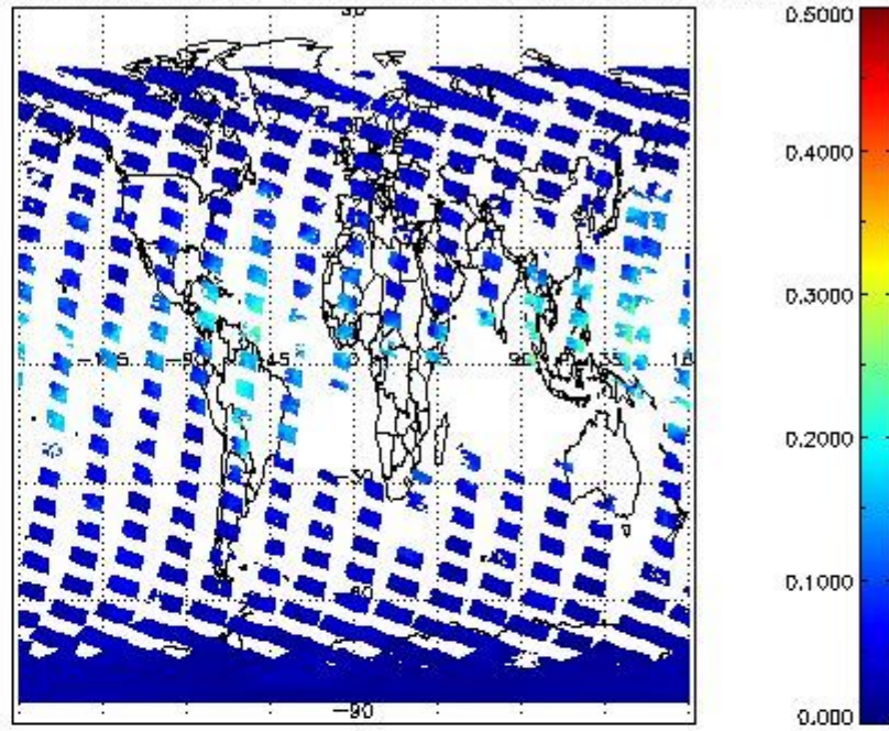
SCIOL2P_NADUV8H2O_vcd_err for 23OCT2011 00:00:00 to 24OCT2011 00:00:00
