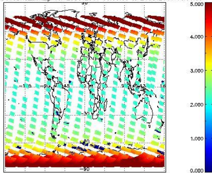
SCIOL2P_NADUV3BRO_amf_gr for 23OCT2011 00:00:00 to 24OCT2011 00:00:00
