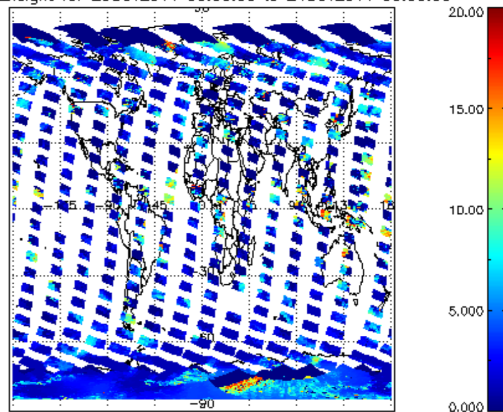
cl_top_height for 23OCT2011 00:00:00 to 24OCT2011 00:00:00
