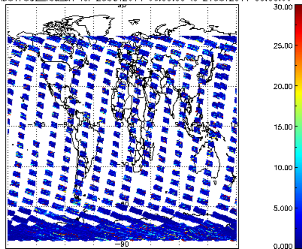
SCIOL2P_NADUV7S02_vcd_err for 23OCT2011 00:00:00 to 24OCT2011 00:00:00
