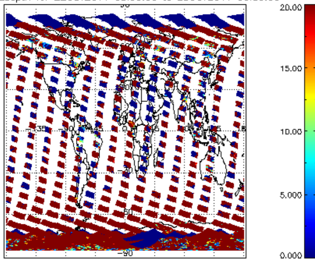
cl_opt_depth for 22OCT2011 00:00:00 to 23OCT2011 00:00:00
