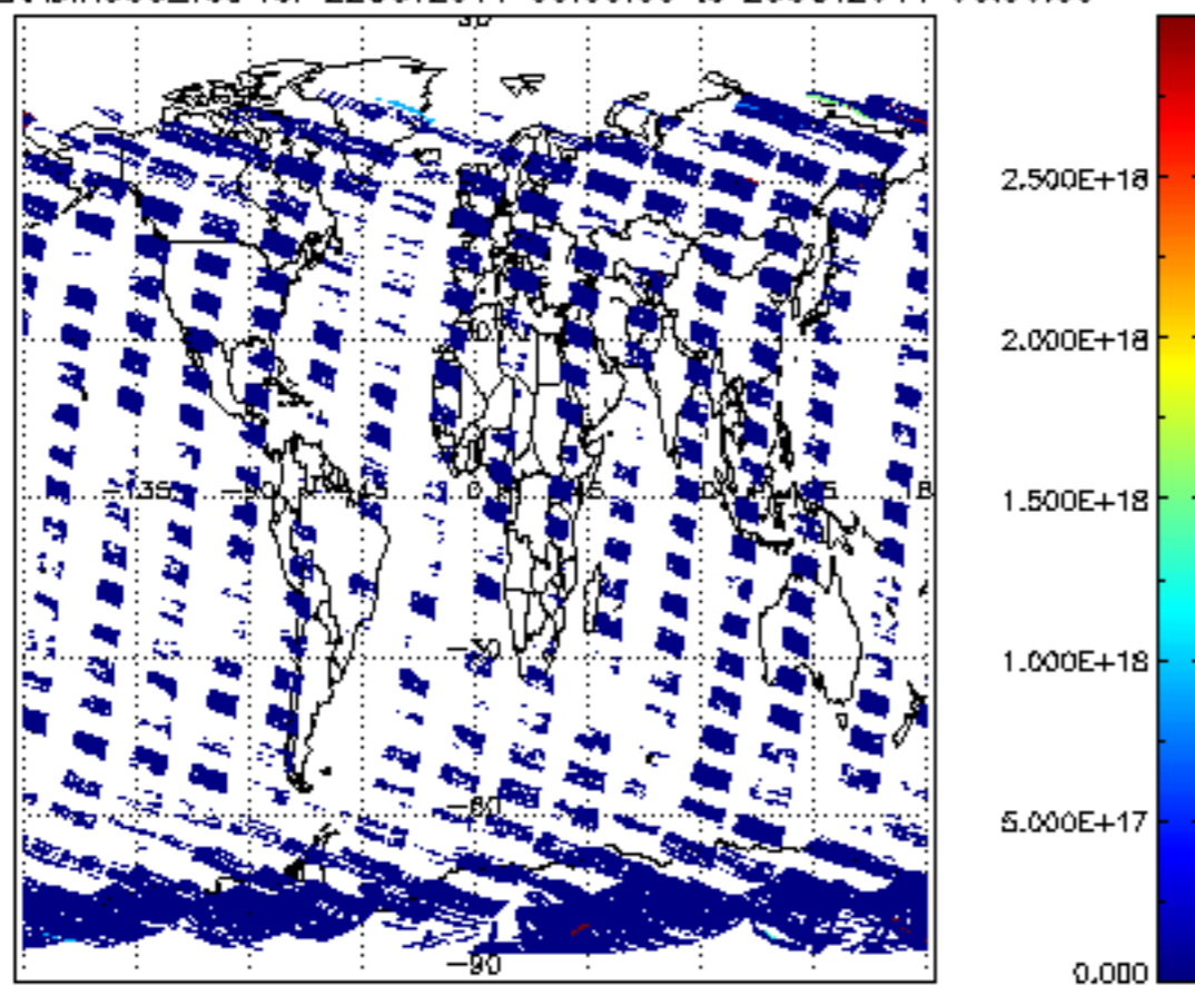
SCIOL2P_NADIR3CO_vcd for 22OCT2011 00:00:00 to 23OCT2011 00:00:00
