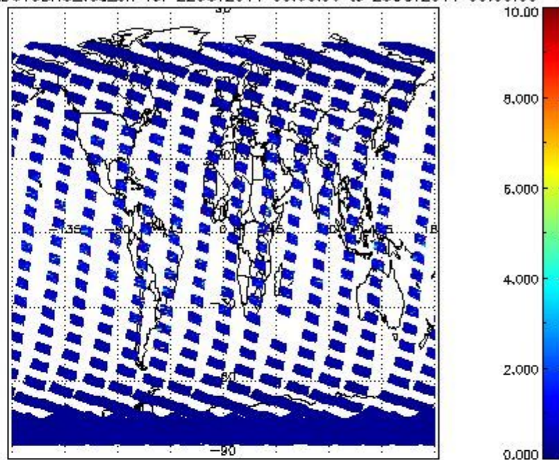
SCIOL2P_NADUV3BRO_vcd_err for 22OCT2011 00:00:00 to 23OCT2011 00:00:00
