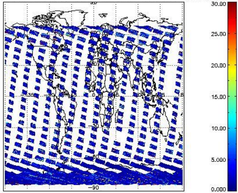
SCIOL2P_NADUV7S02_vcd_err for 22OCT2011 00:00:00 to 23OCT2011 00:00:00
