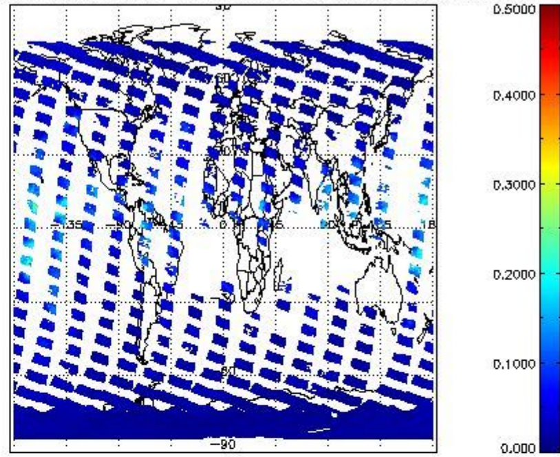
SCIOL2P_NADUV8H2O_vcd_err for 22OCT2011 00:00:00 to 23OCT2011 00:00:00
