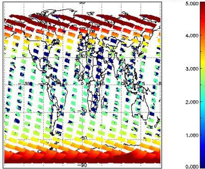
SCIOL2P_NADUV003_amf_cl for 22OCT2011 00:00:00 to 23OCT2011 00:00:00
