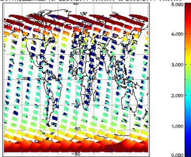
SCIOL2P_NADUV1NO2_amf_cl for 22OCT2011 00:00:00 to 23OCT2011 00:00:00
