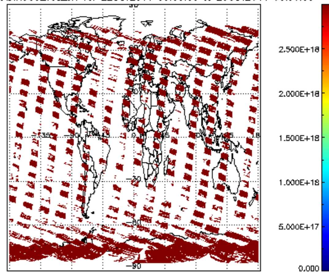
SCIOL2P_NADIR3CO_vcd_err for 22OCT2011 00:00:00 to 23OCT2011 00:00:00
