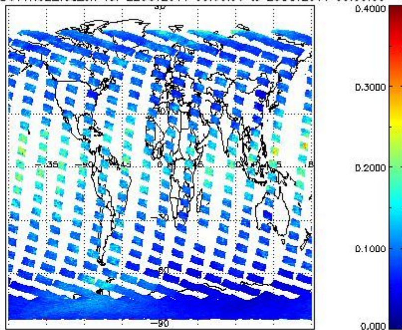
SCIOL2P_NADUV1NO2_vcd_err for 22OCT2011 00:00:00 to 23OCT2011 00:00:00
