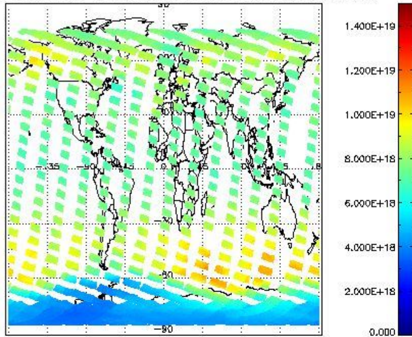
SCIOL2P_NADUV003_vcd for 22OCT2011 00:00:00 to 23OCT2011 00:00:00
