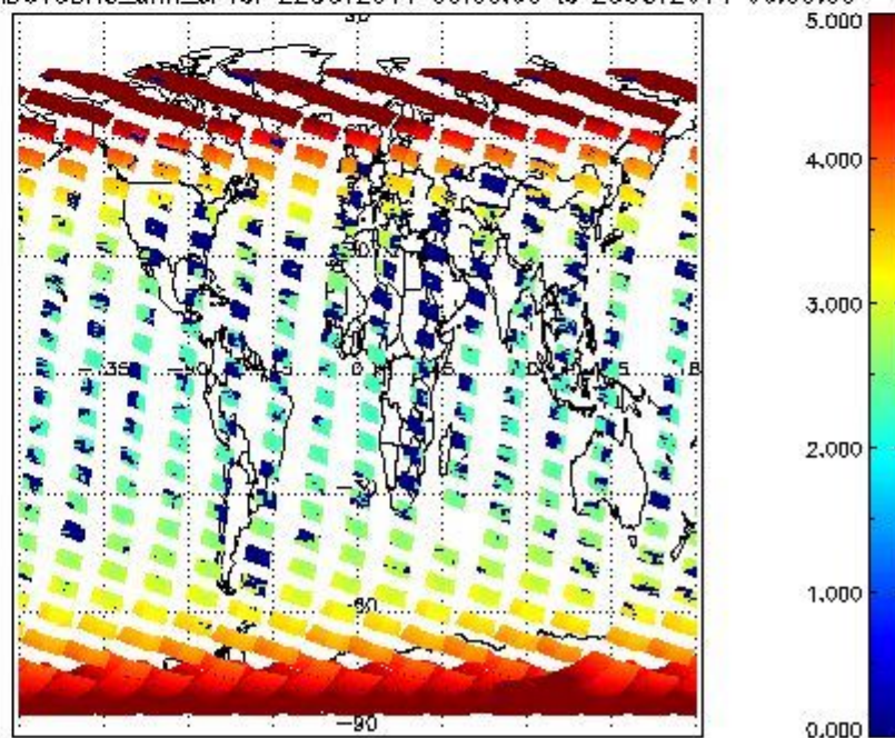
SCIOL2P_NADUV3BRO_amf_cl for 22OCT2011 00:00:00 to 23OCT2011 00:00:00
