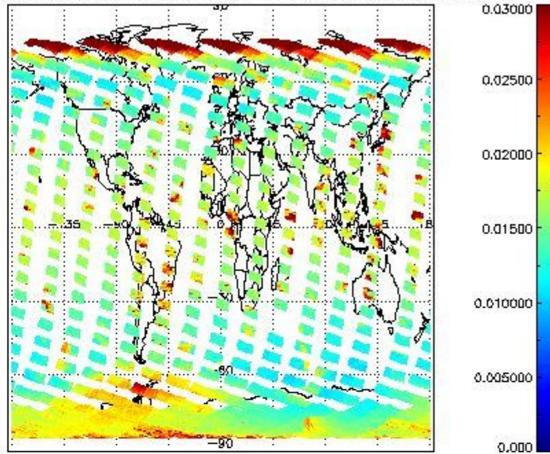
SCIOL2P_NADUV003_vcd_err for 22OCT2011 00:00:00 to 23OCT2011 00:00:00
