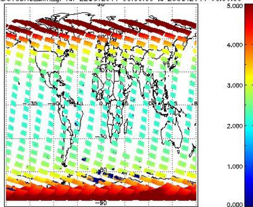
SCIOL2P_NADUV3BRO_amf_gr for 22OCT2011 00:00:00 to 23OCT2011 00:00:00
