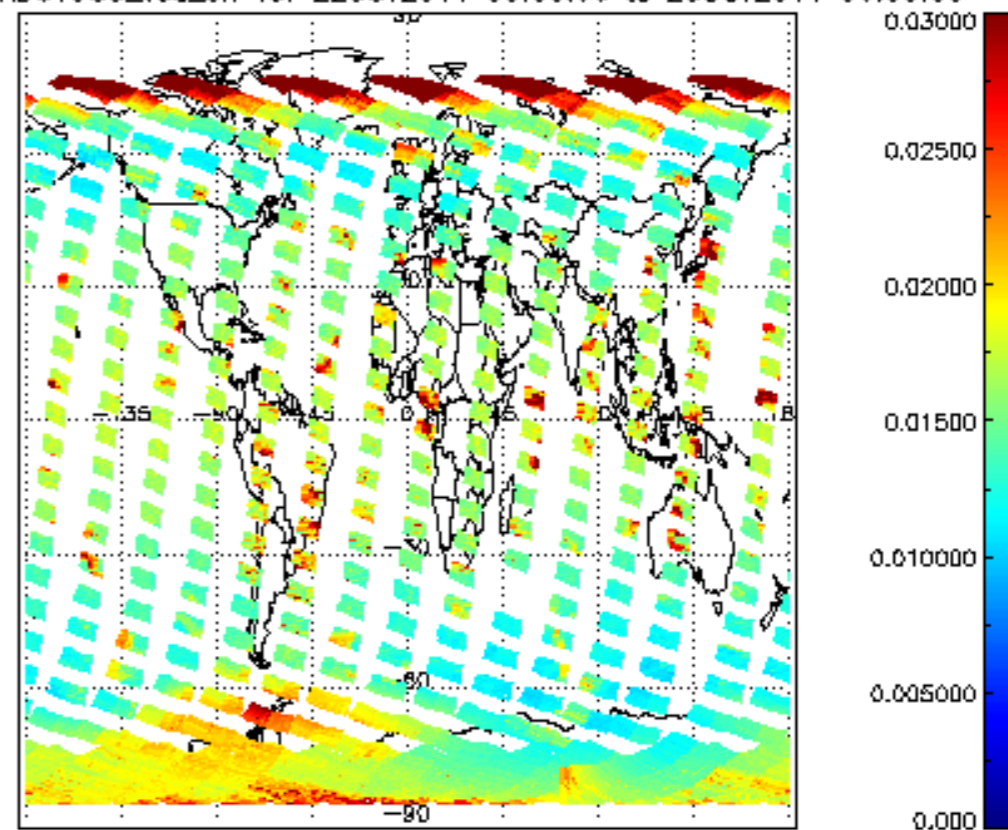
SCIOL2P_NADUV003_vcd_err for 22OCT2011 00:00:00 to 23OCT2011 00:00:00
