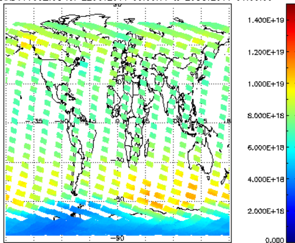
SCIOL2P_NADUV003_vcd for 22OCT2011 00:00:00 to 23OCT2011 00:00:00
