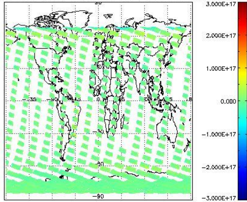
SCIOL2P_NADUV7S02_vcd for 22OCT2011 00:00:00 to 23OCT2011 00:00:00
