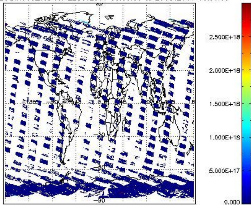
SCIDL2P_NADIR3CO_vcd for 22OCT2011 00:00:00 to 23OCT2011 00:00:00
