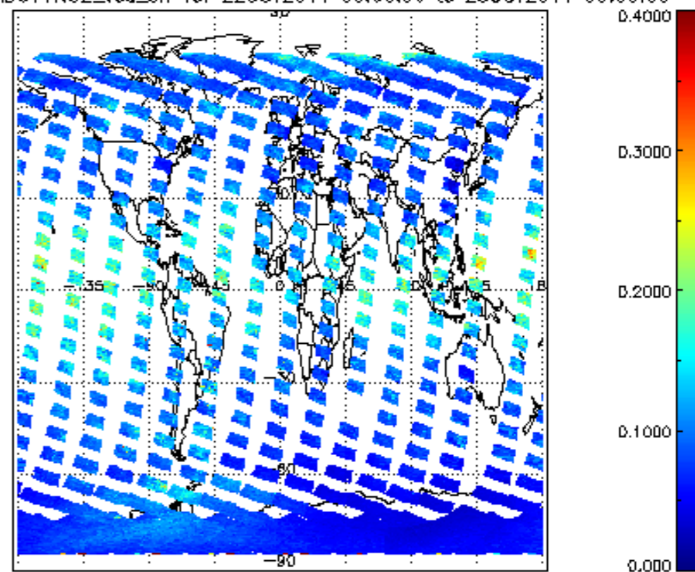
SCIOL2P_NADUV1NO2_vcd_err for 22OCT2011 00:00:00 to 23OCT2011 00:00:00
