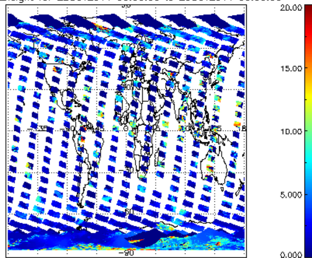
cl_top_height for 22OCT2011 00:00:00 to 23OCT2011 00:00:00
