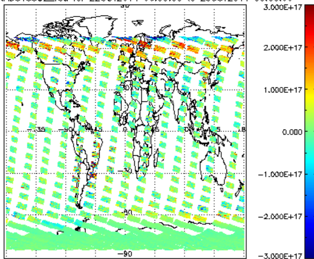
SCIOL2P_NADUV5S02_vcd for 22OCT2011 00:00:00 to 23OCT2011 00:00:00
