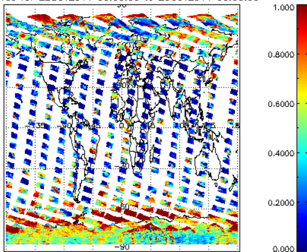
cl_frac for 22OCT2011 00:00:00 to 23OCT2011 00:00:00
