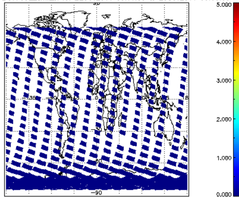
SCIOL2P_NADUV7S02_amf_sl for 22OCT2011 00:00:00 to 23OCT2011 00:00:00
