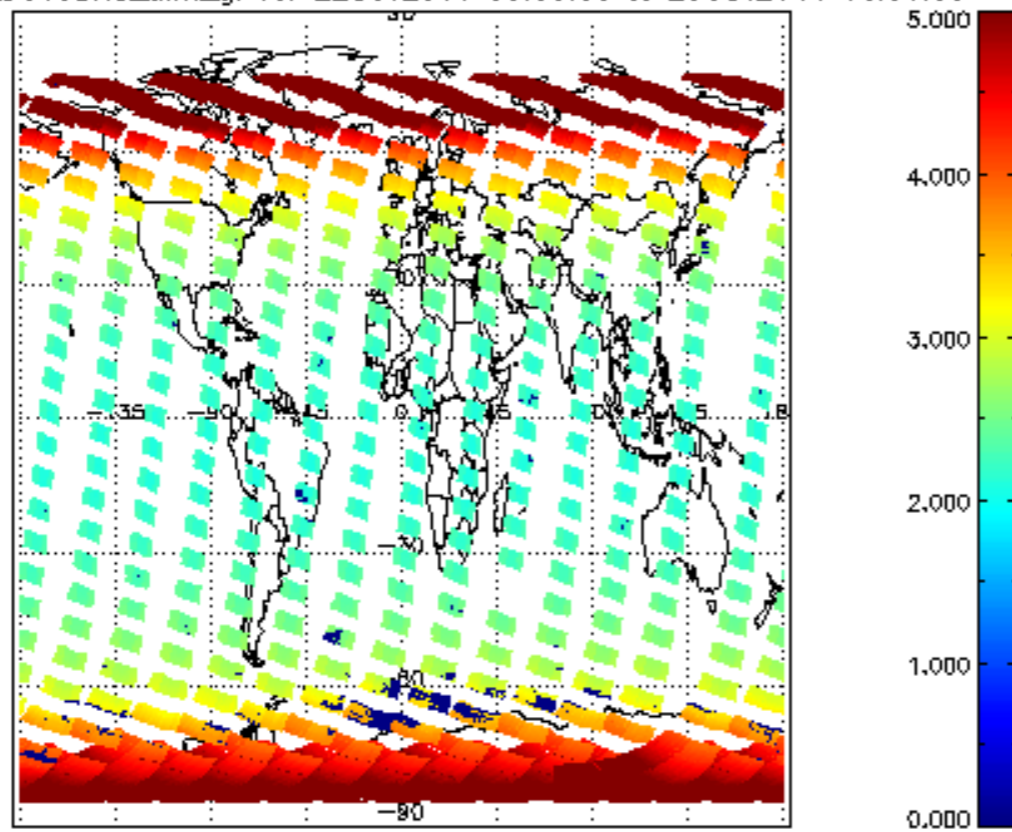
SCIOL2P_NADUV3BRO_amf_gr for 22OCT2011 00:00:00 to 23OCT2011 00:00:00
