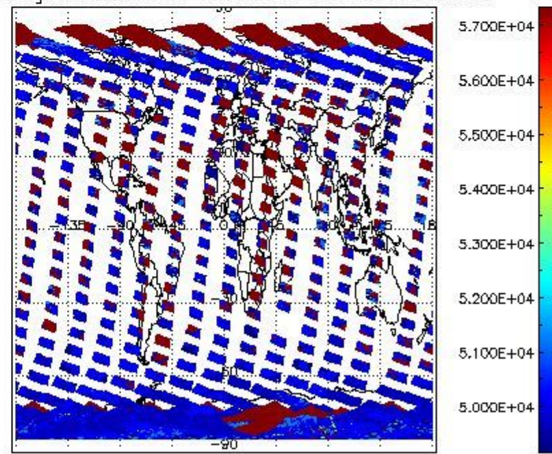
cloud_flags for 22OCT2011 00:00:00 to 23OCT2011 00:00:00
