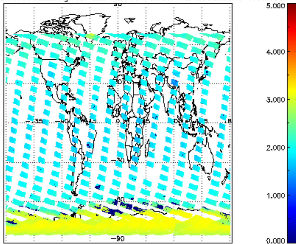
SCIOL2P_NADUV7S02_amf_gr for 22OCT2011 00:00:00 to 23OCT2011 00:00:00
