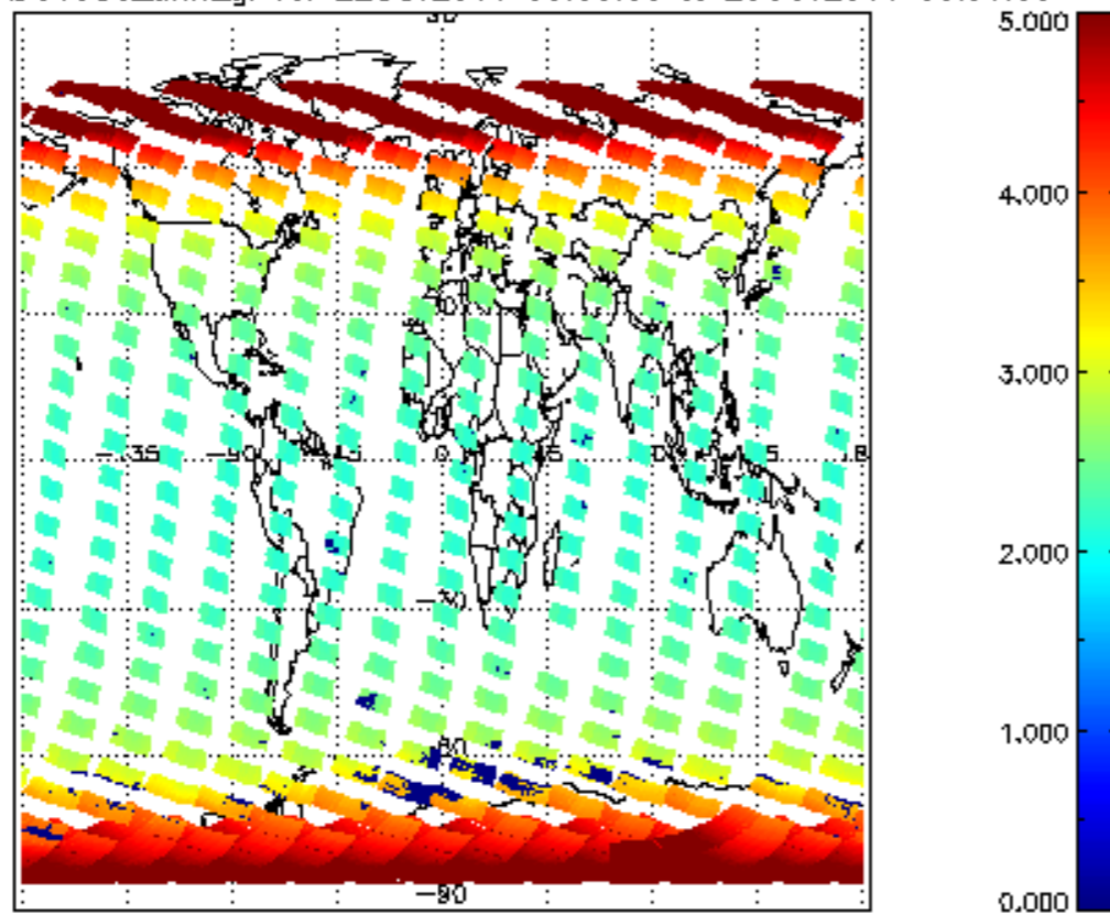
SCIOL2P_NADUV003_amf_gr for 22OCT2011 00:00:00 to 23OCT2011 00:00:00
