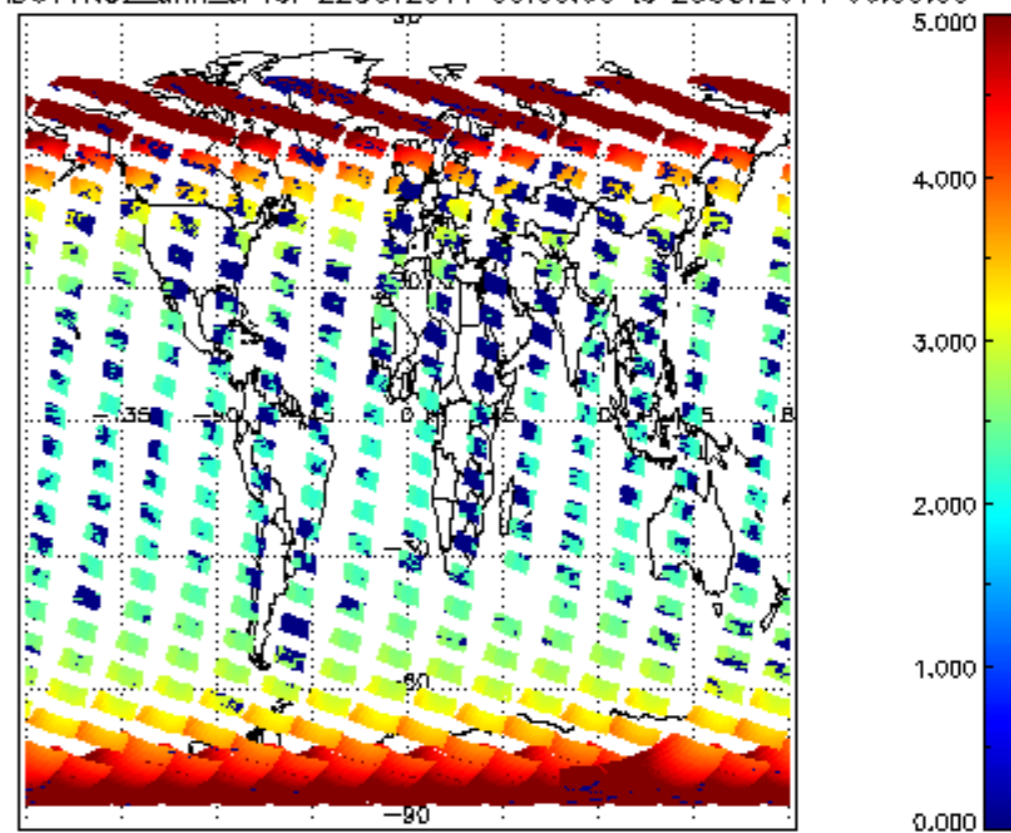
SCIOL2P_NADUV1NO2_amf_cl for 22OCT2011 00:00:00 to 23OCT2011 00:00:00
