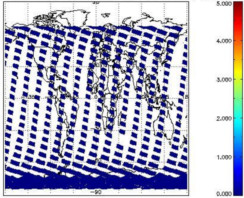
SCIOL2P_NADUV7S02_amf_cl for 22OCT2011 00:00:00 to 23OCT2011 00:00:00
