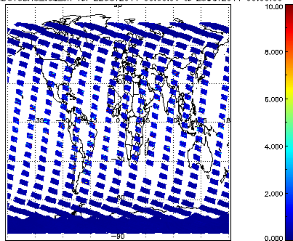
SCIOL2P_NADUV3BRO_vcd_err for 22OCT2011 00:00:00 to 23OCT2011 00:00:00
