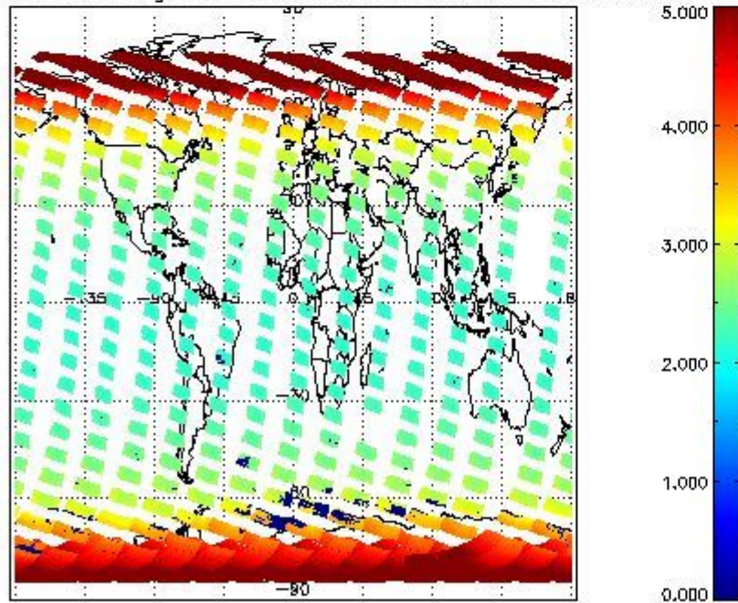
SCIOL2P_NADUV003_amf_gr for 22OCT2011 00:00:00 to 23OCT2011 00:00:00
