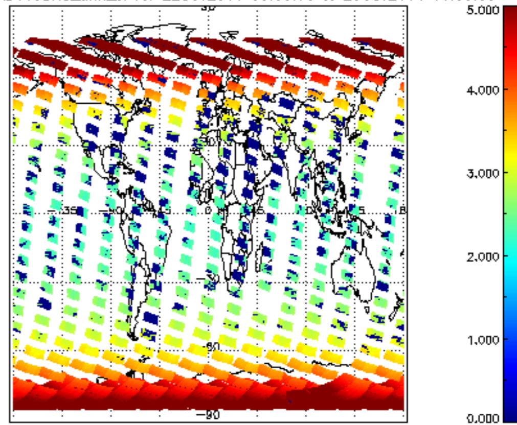
SCIOL2P_NADUV3BRO_amf_cl for 22OCT2011 00:00:00 to 23OCT2011 00:00:00
