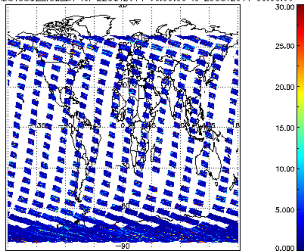
SCIOL2P_NADUV5S02_vcd_err for 22OCT2011 00:00:00 to 23OCT2011 00:00:00
