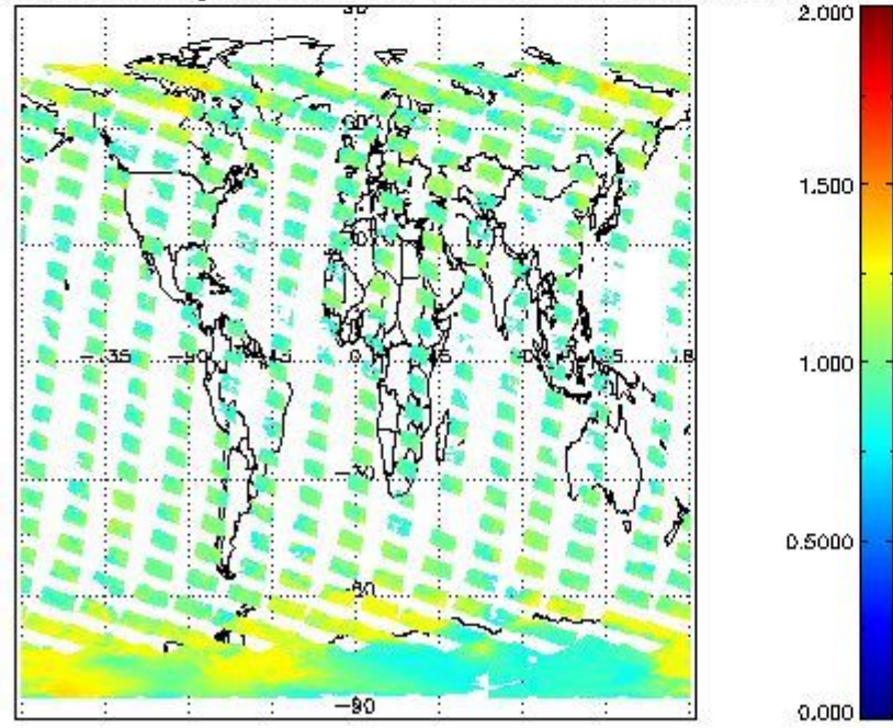
SCIOL2P_NADUV8H2O_amf_gr for 22OCT2011 00:00:00 to 23OCT2011 00:00:00
