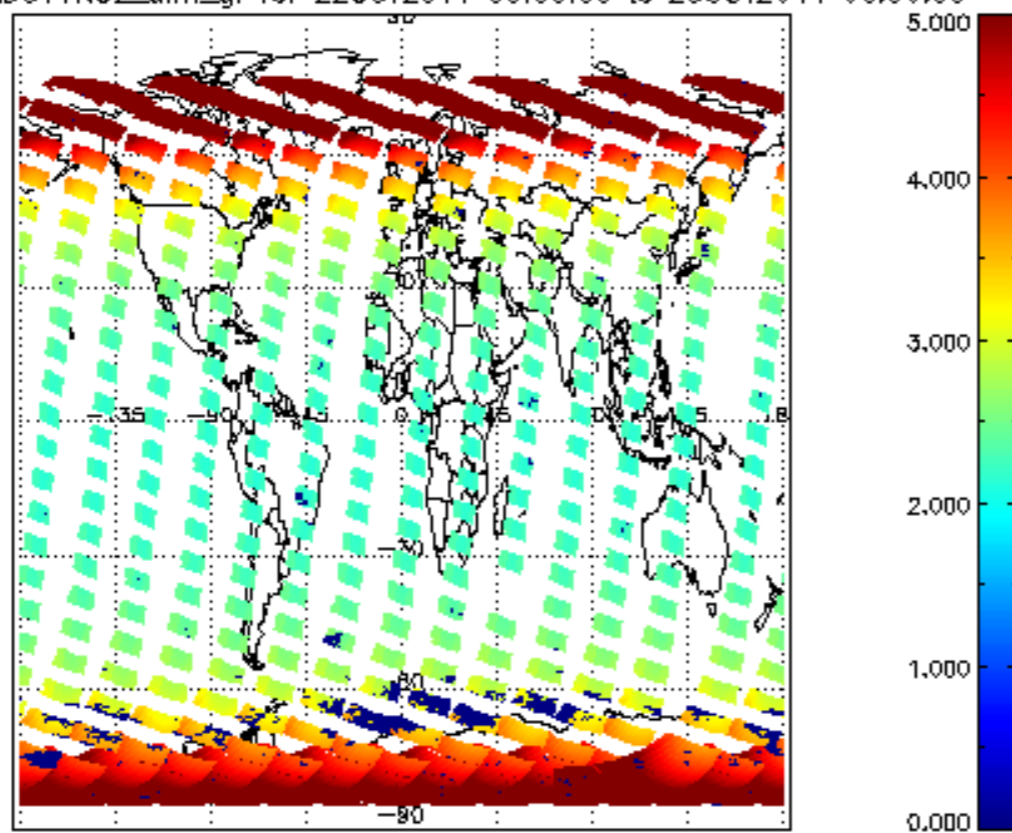
SCIOL2P_NADUV1NO2_amf_gr for 22OCT2011 00:00:00 to 23OCT2011 00:00:00
