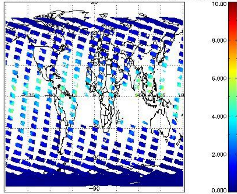
SCIOL2P_NADUV8H2O_vcd for 22OCT2011 00:00:00 to 23OCT2011 00:00:00
