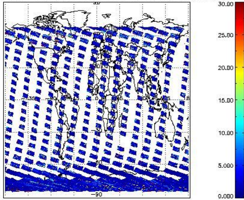
SCIOL2P_NADUV5SO2_vcd_err for 22OCT2011 00:00:00 to 23OCT2011 00:00:00
