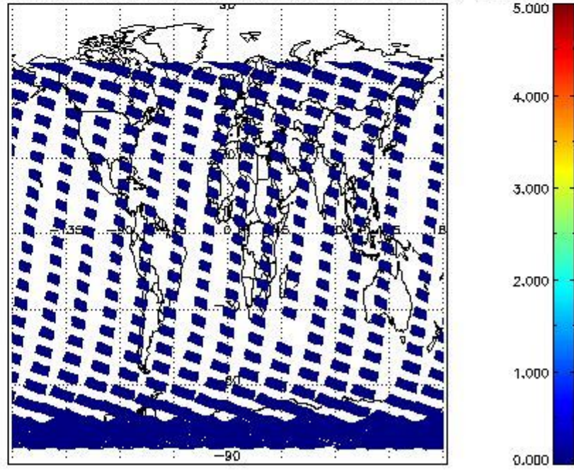
SCIOL2P_NADUV5SO2_amf_cl for 22OCT2011 00:00:00 to 23OCT2011 00:00:00
