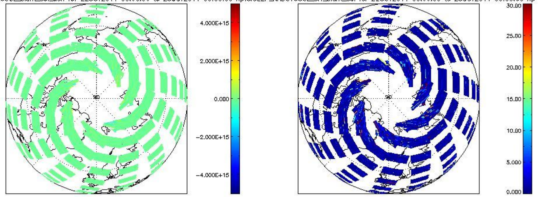
CIOL2P_NADUV60CL_slant_col_den for 22OCT2011 00:00:00 to 23OCT2011 00:00:00 np CIOL2P_NADUV60CL_err_slant_col for 22OCT2011 00:00:00 to 23OCT2011 00:00:00 np
