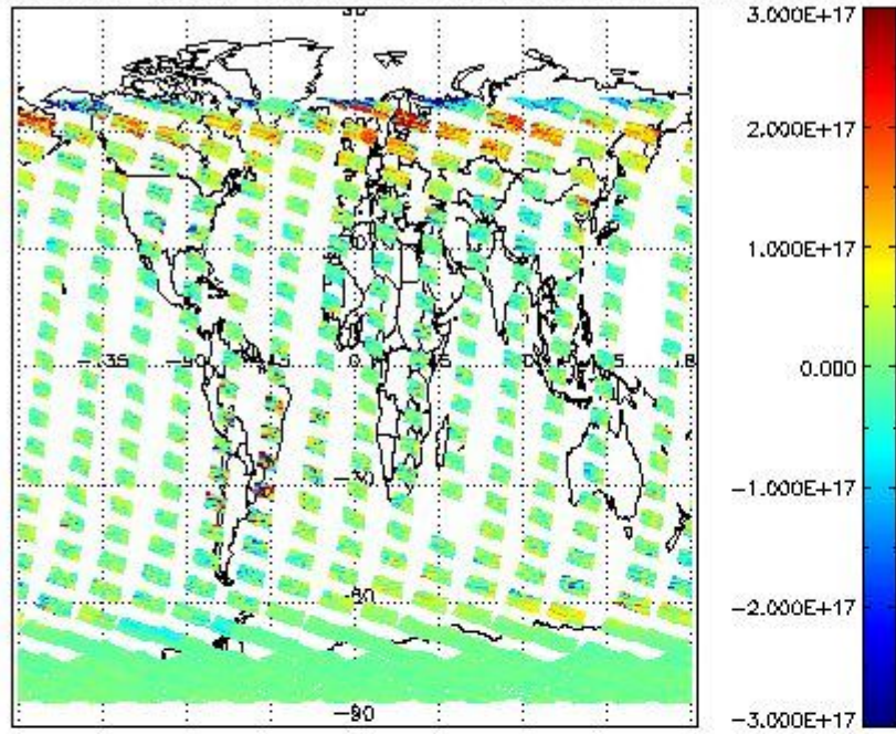
SCIOL2P_NADUV5SO2_vcd for 22OCT2011 00:00:00 to 23OCT2011 00:00:00
