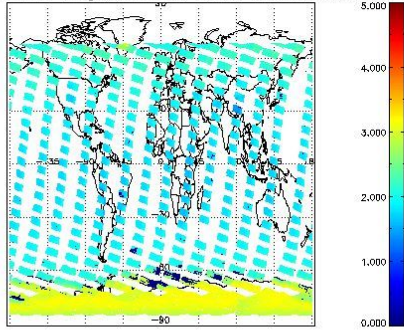
SCIOL2P_NADUV7S02_amf_gr for 22OCT2011 00:00:00 to 23OCT2011 00:00:00
