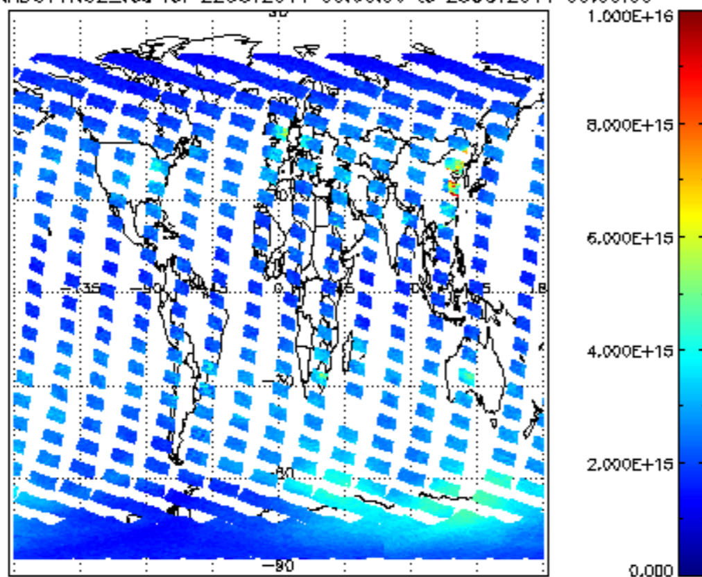
SCIOL2P_NADUV1NO2_vcd for 22OCT2011 00:00:00 to 23OCT2011 00:00:00
