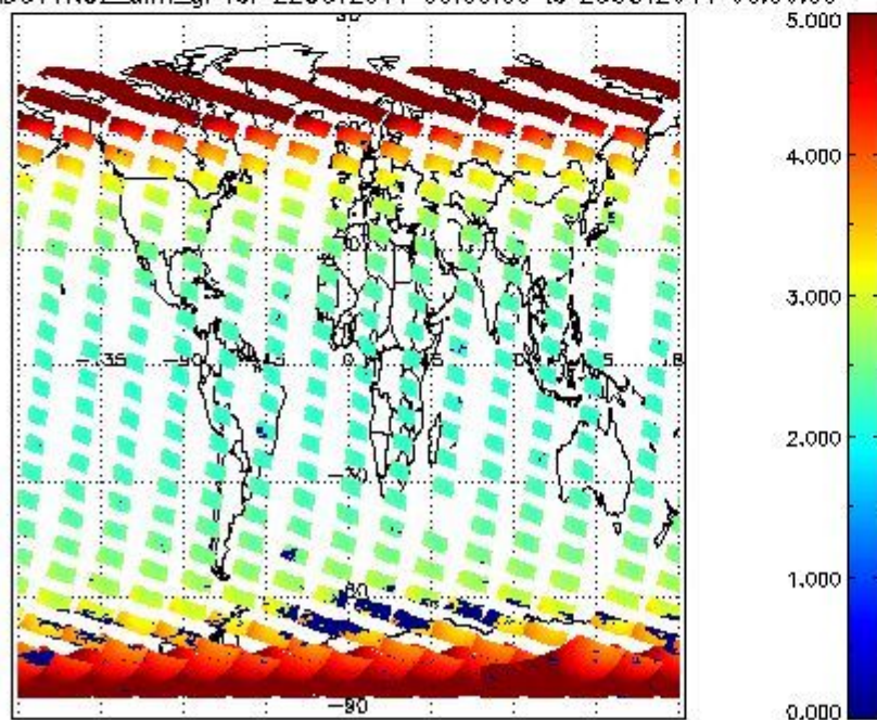
SCIOL2P_NADUV1NO2_amf_gr for 22OCT2011 00:00:00 to 23OCT2011 00:00:00
