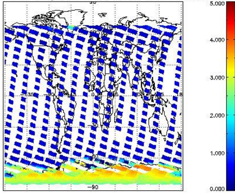
SCIOL2P_NADUV5SO2_amf_gr for 22OCT2011 00:00:00 to 23OCT2011 00:00:00
