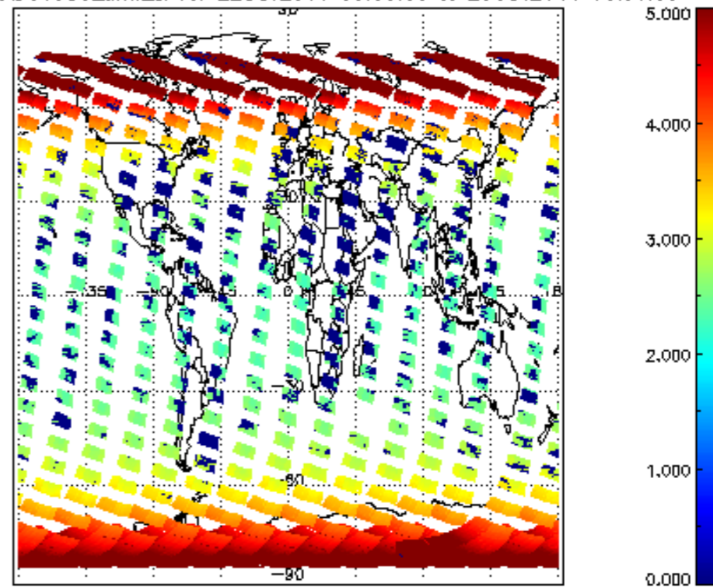
SCIOL2P_NADUV003_amf_cl for 22OCT2011 00:00:00 to 23OCT2011 00:00:00
