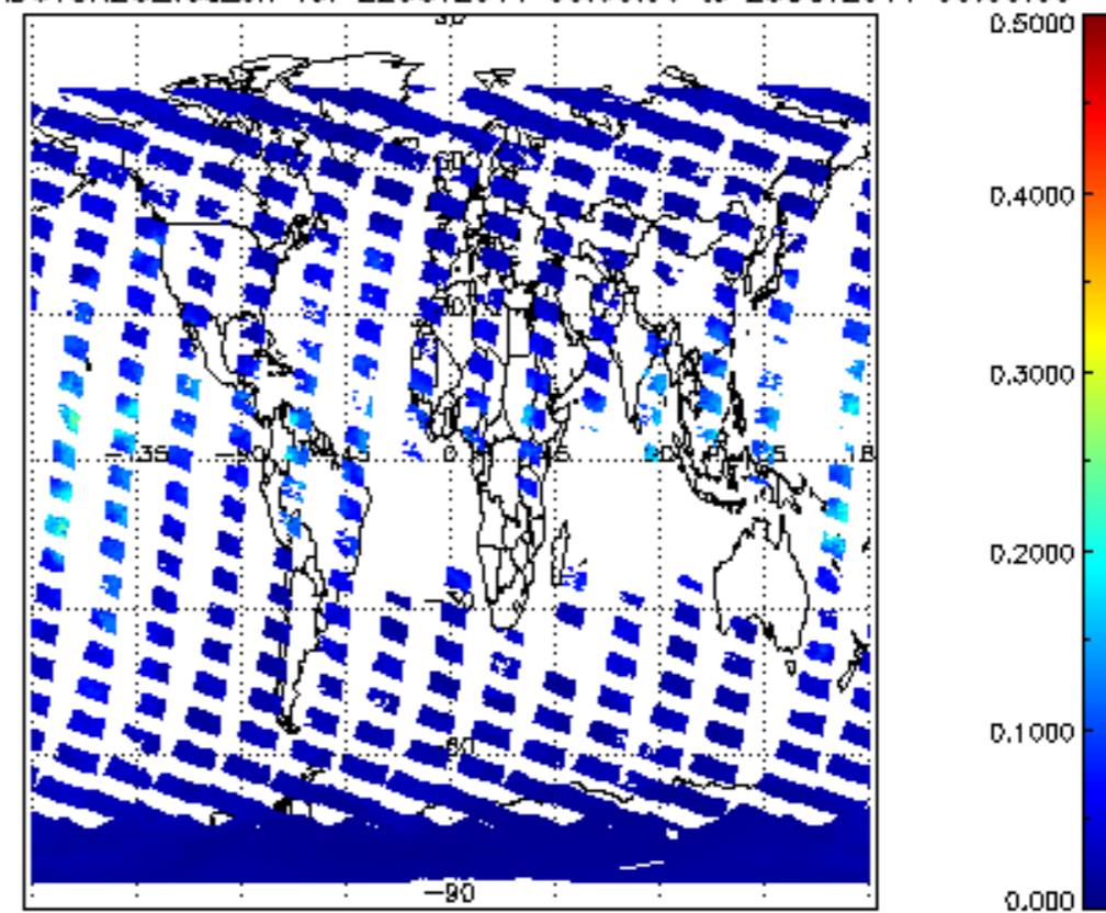
SCIOL2P_NADUV8H20_vcd_err for 22OCT2011 00:00:00 to 23OCT2011 00:00:00
