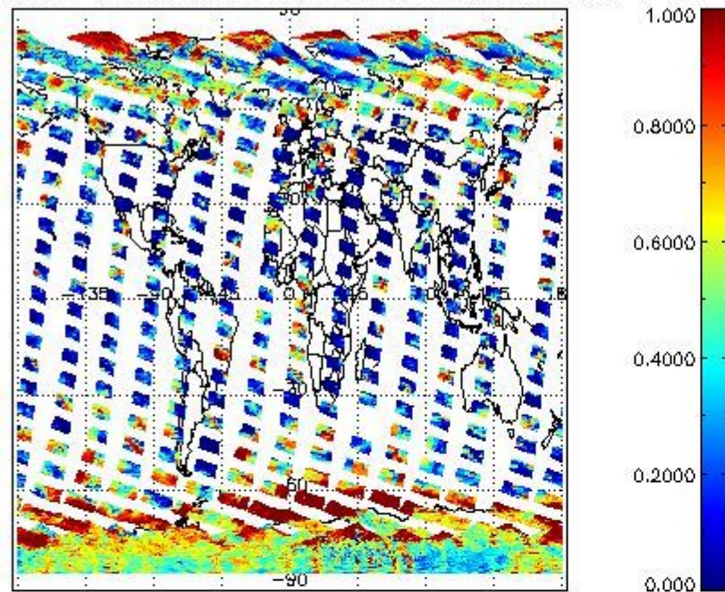
cLfrac for 22OCT2011 00:00:00 to 23OCT2011 00:00:00
