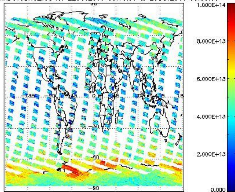
SCIOL2P_NADUV3BRO_vcd for 22OCT2011 00:00:00 to 23OCT2011 00:00:00
