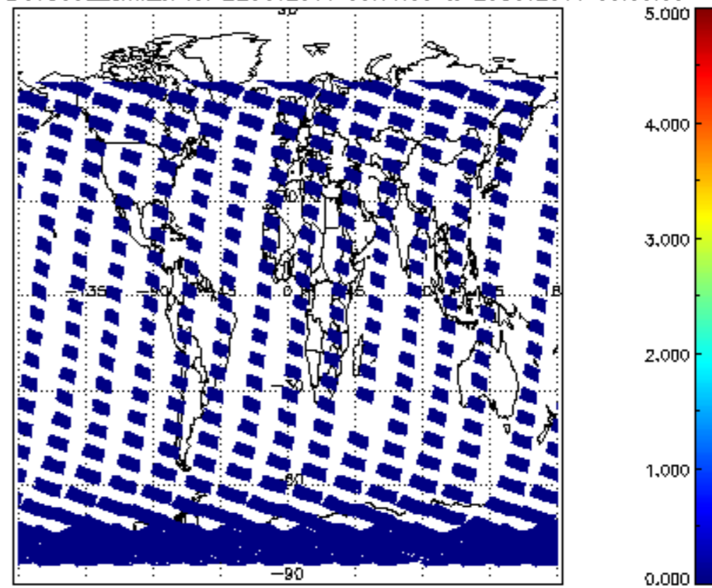
SCIOL2P_NADUV5S02_amf_sl for 22OCT2011 00:00:00 to 23OCT2011 00:00:00
