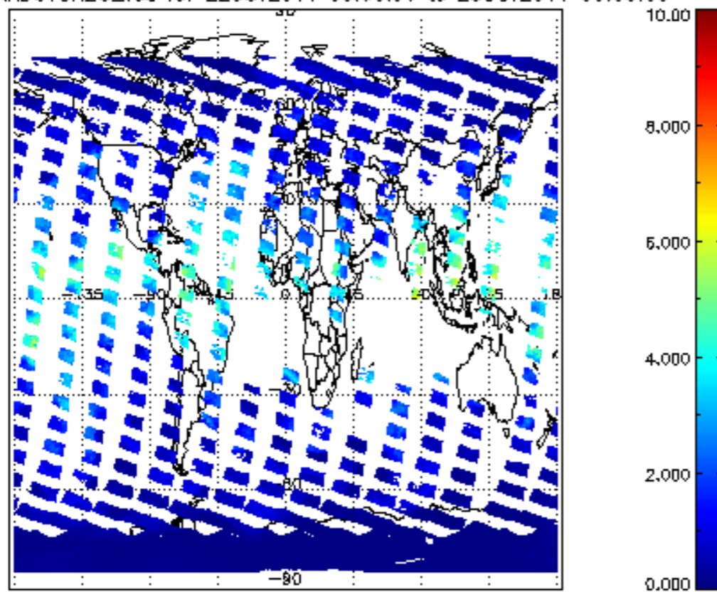
SCIOL2P_NADUV8H20_vcd for 22OCT2011 00:00:00 to 23OCT2011 00:00:00
