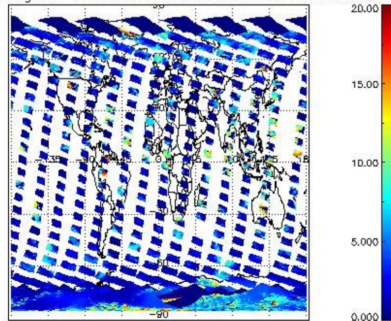
cL_top_height for 22OCT2011 00:00:00 to 23OCT2011 00:00:00
