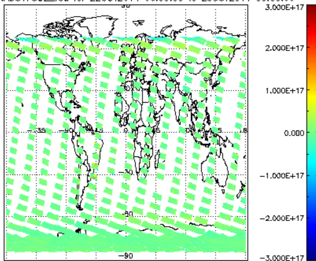
SCIOL2P_NADUV7S02_vcd for 22OCT2011 00:00:00 to 23OCT2011 00:00:00
