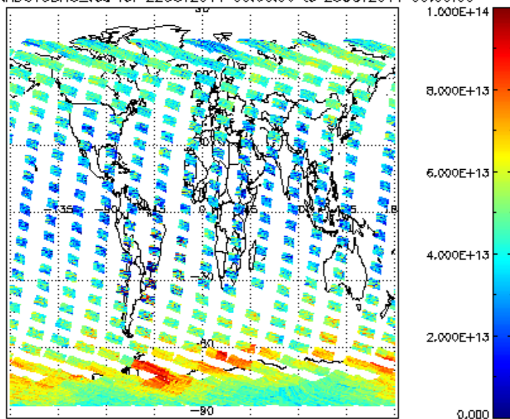
SCIOL2P_NADUV3BRO_vcd for 22OCT2011 00:00:00 to 23OCT2011 00:00:00
