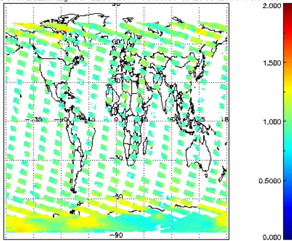
SCIOL2P_NADUV8H20_amf_gr for 22OCT2011 00:00:00 to 23OCT2011 00:00:00
