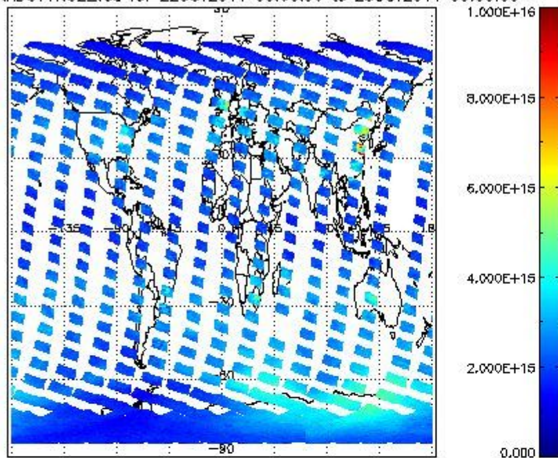
SCIOL2P_NADUV1NO2_vcd for 22OCT2011 00:00:00 to 23OCT2011 00:00:00
