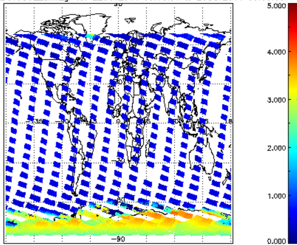
SCIOL2P_NADUV5S02_amf_gr for 22OCT2011 00:00:00 to 23OCT2011 00:00:00
