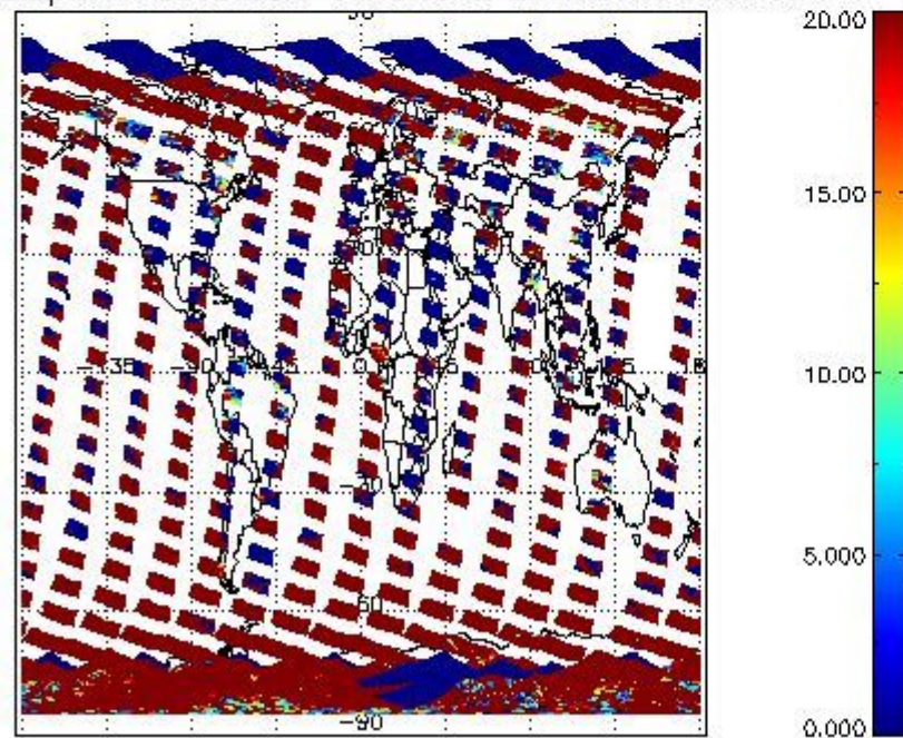
cL_opt_depth for 22OCT2011 00:00:00 to 23OCT2011 00:00:00
