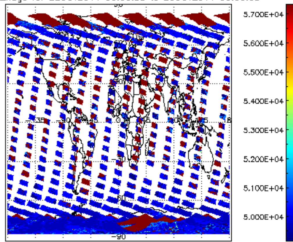
cloud_flags for 22OCT2011 00:00:00 to 23OCT2011 00:00:00
