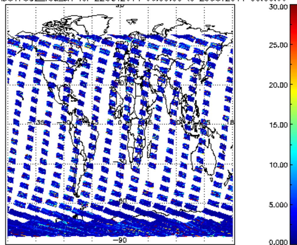
SCIOL2P_NADUV7S02_vcd_err for 22OCT2011 00:00:00 to 23OCT2011 00:00:00
