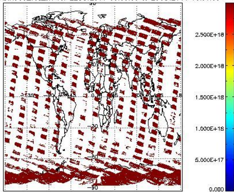
SCIDL2P_NADIR3CO_vcd_err for 22OCT2011 00:00:00 to 23OCT2011 00:00:00
