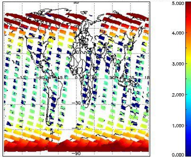
SCIOL2P_NADUV003_amf_cl for 21OCT2011 00:00:00 to 22OCT2011 00:00:00
