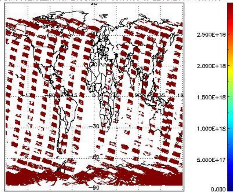
SCIOI2P_NADIR3CO_vcd_err for 21OCT2011 00:00:00 to 22OCT2011 00:00:00
