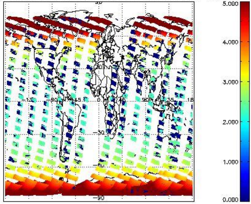
SCIOL2P_NADUV1NO2_amf_cl for 21OCT2011 00:00:00 to 22OCT2011 00:00:00
