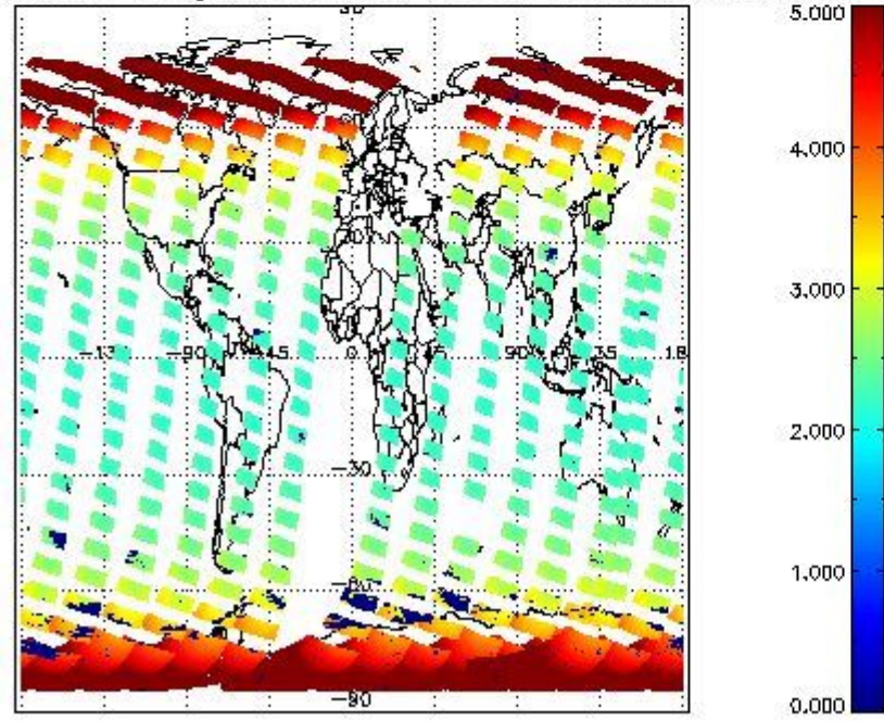
SCIOL2P_NADUV1NO2_amf_gr for 21OCT2011 00:00:00 to 22OCT2011 00:00:00
