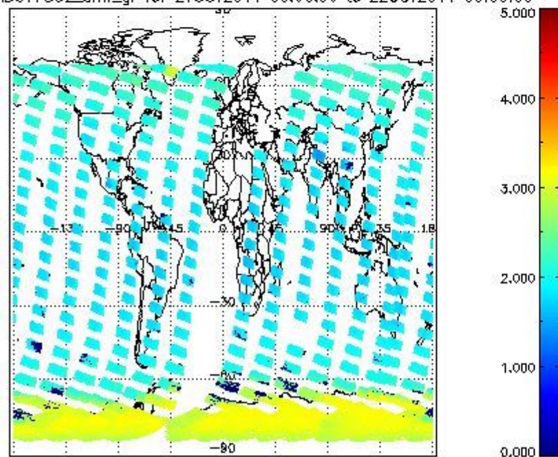
SCIOL2P_NADUV7S02_amf_gr for 21OCT2011 00:00:00 to 22OCT2011 00:00:00
