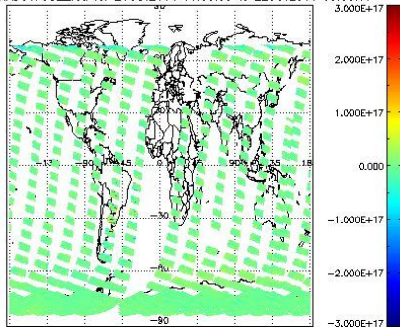
SCIOL2P_NADUV7S02_vcd for 21OCT2011 00:00:00 to 22OCT2011 00:00:00
