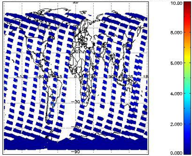
SCIOL2P_NADUV3BRO_vcd_err for 21OCT2011 00:00:00 to 22OCT2011 00:00:00
