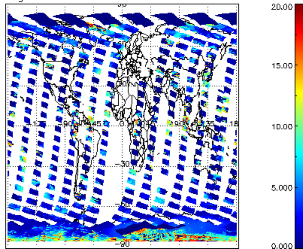
cl_top_height for 21OCT2011 00:00:00 to 22OCT2011 00:00:00
