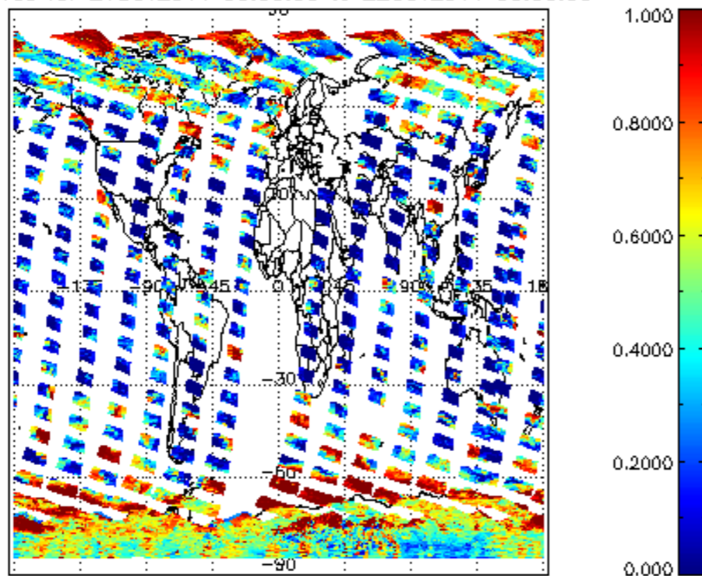
cl_frac for 21OCT2011 00:00:00 to 22OCT2011 00:00:00
