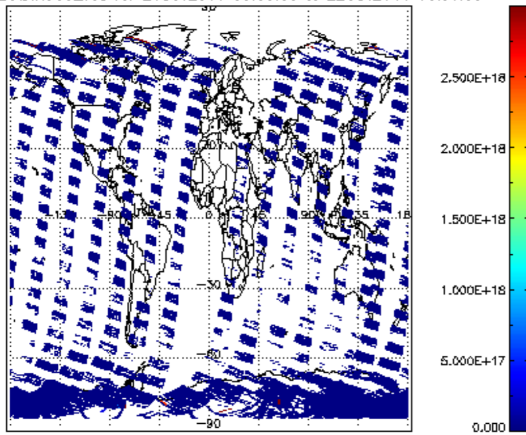
SCIOL2P_NADIR3CO_vcd for 21OCT2011 00:00:00 to 22OCT2011 00:00:00
