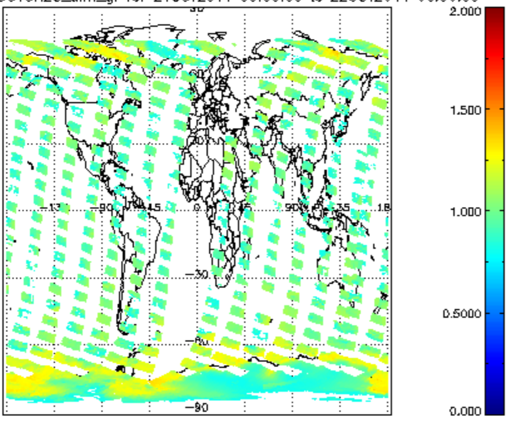
SCIOL2P_NADUV8H20_amf_gr for 21OCT2011 00:00:00 to 22OCT2011 00:00:00
