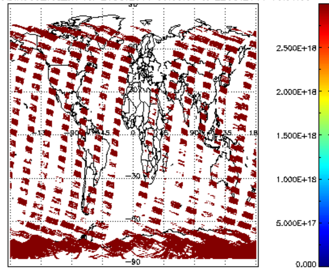
SCIOL2P_NADIR3CO_vcd_err for 21OCT2011 00:00:00 to 22OCT2011 00:00:00
