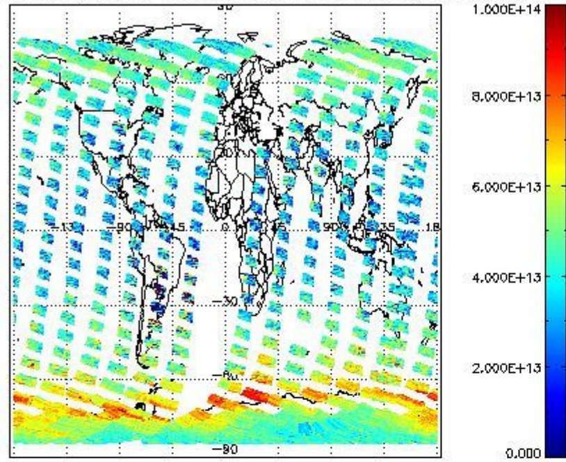
SCIOL2P_NADUV3BRO_vcd for 21OCT2011 00:00:00 to 22OCT2011 00:00:00
