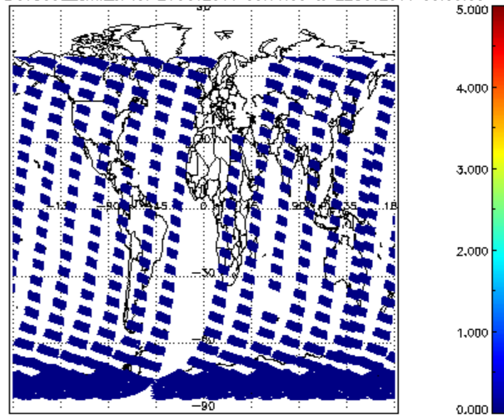
SCIOL2P_NADUV5S02_amf_cl for 21OCT2011 00:00:00 to 22OCT2011 00:00:00
