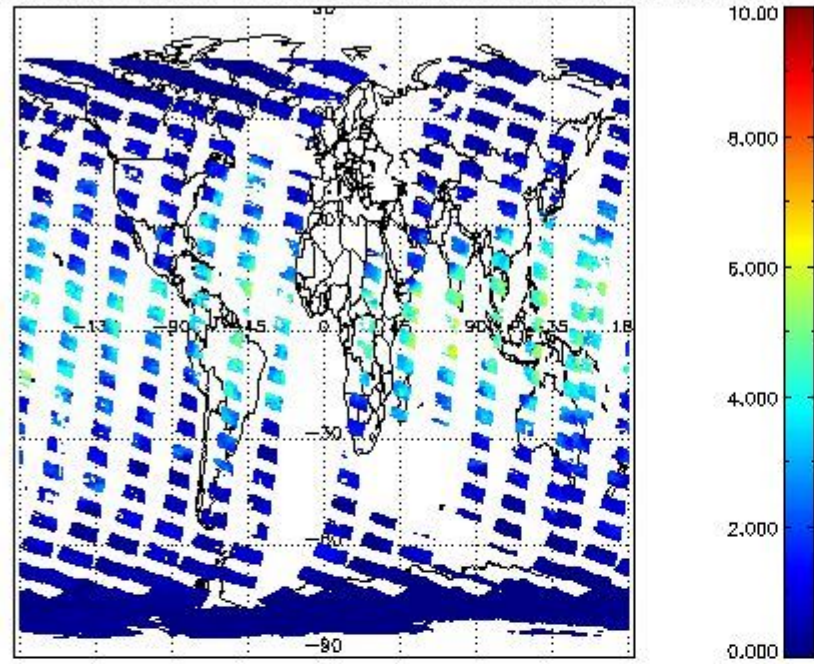
SCIOL2P_NADUV8H20_vcd for 21OCT2011 00:00:00 to 22OCT2011 00:00:00
