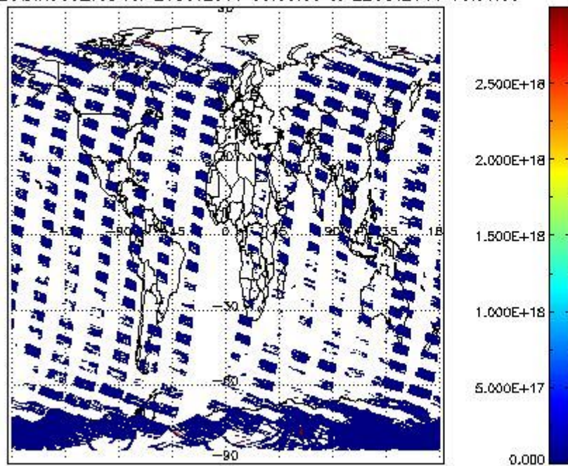
SCIOI2P_NADIR3CO_vcd for 21OCT2011 00:00:00 to 22OCT2011 00:00:00
