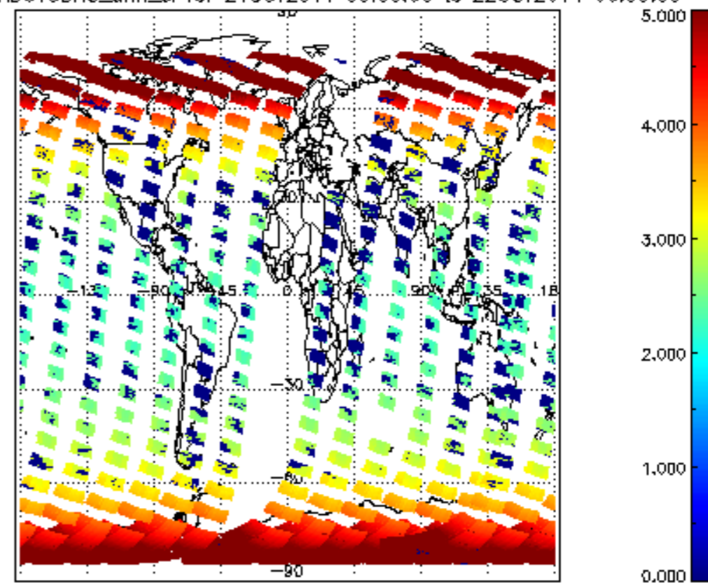
SCIOL2P_NADUV3BRO_amf_cl for 21OCT2011 00:00:00 to 22OCT2011 00:00:00
