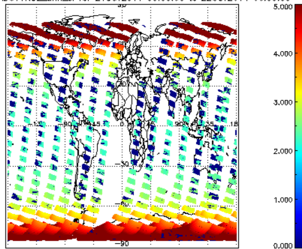
SCIOL2P_NADUV1NO2_amf_cl for 21OCT2011 00:00:00 to 22OCT2011 00:00:00
