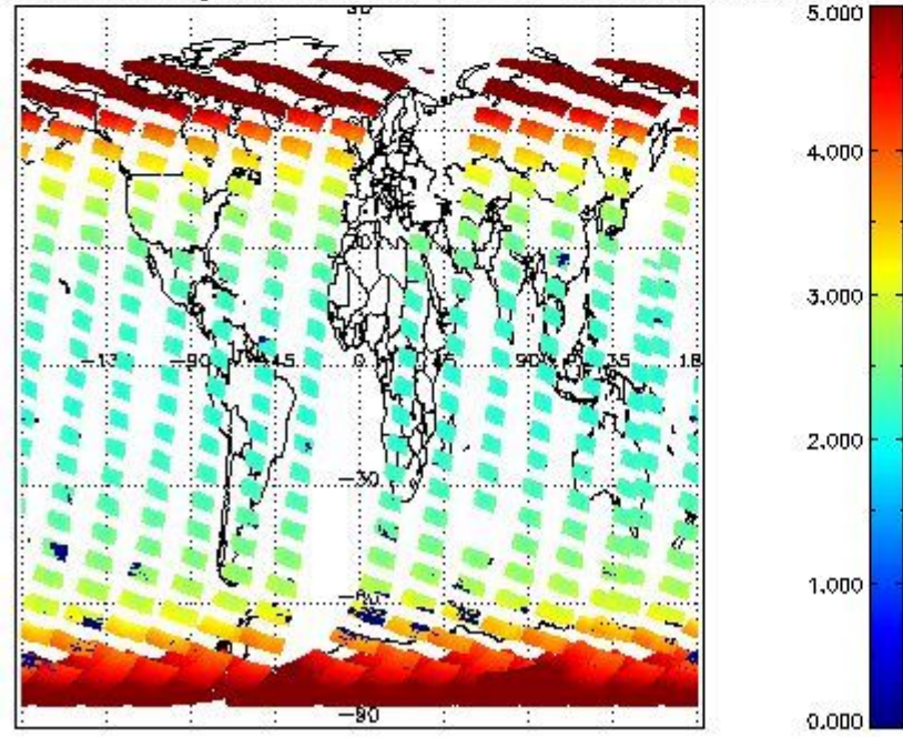
SCIOL2P_NADUV3BRO_amf_gr for 21OCT2011 00:00:00 to 22OCT2011 00:00:00
