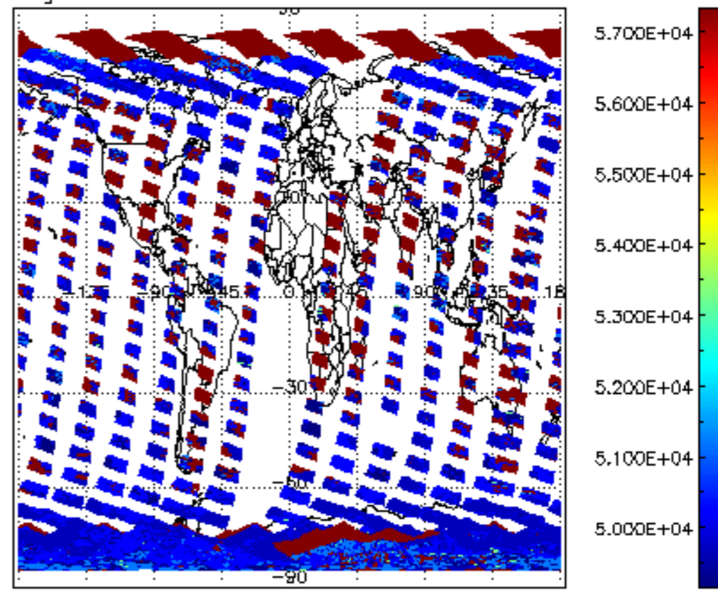
cloud_flags for 21OCT2011 00:00:00 to 22OCT2011 00:00:00
