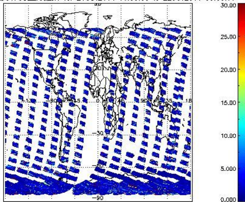
SCIOL2P_NADUV7S02_vcd_err for 21OCT2011 00:00:00 to 22OCT2011 00:00:00
