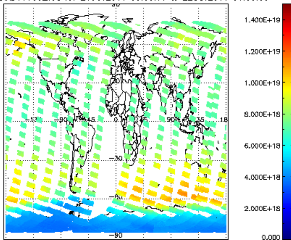
SCIOL2P_NADUV003_vcd for 21OCT2011 00:00:00 to 22OCT2011 00:00:00
