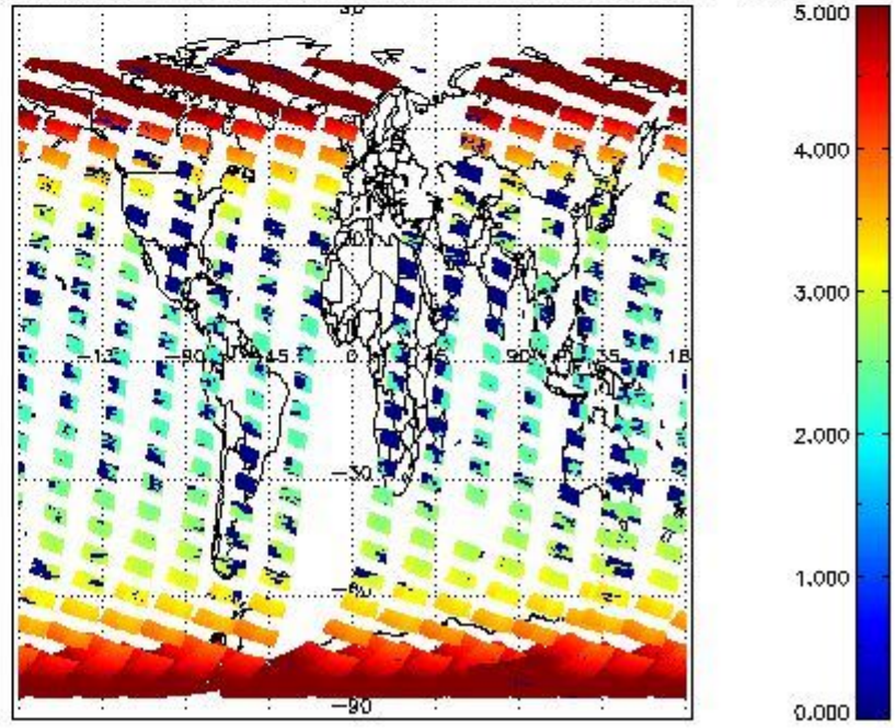
SCIOL2P_NADUV3BRO_amf_cl for 21OCT2011 00:00:00 to 22OCT2011 00:00:00
