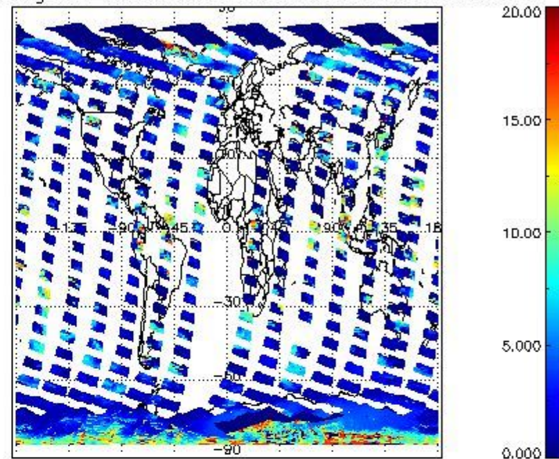
cL_top_height for 21OCT2011 00:00:00 to 22OCT2011 00:00:00
