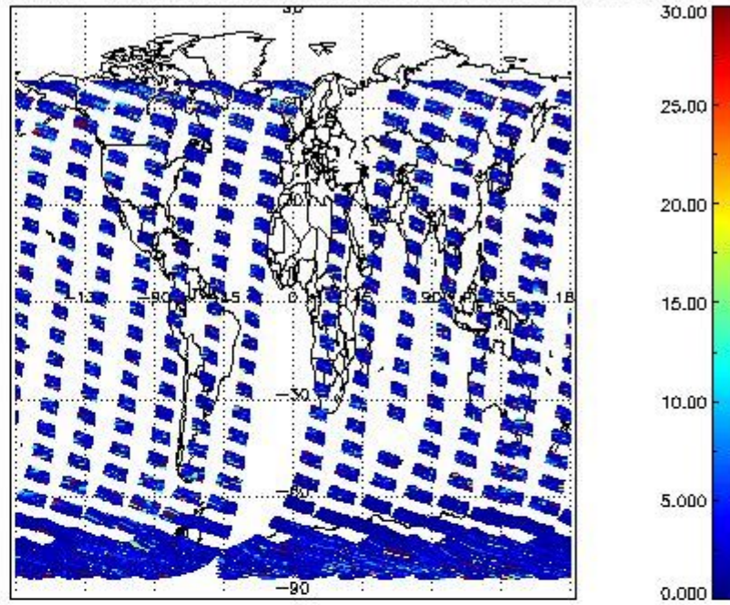
SCIOL2P_NADUV5S02_vcd_err for 21OCT2011 00:00:00 to 22OCT2011 00:00:00
