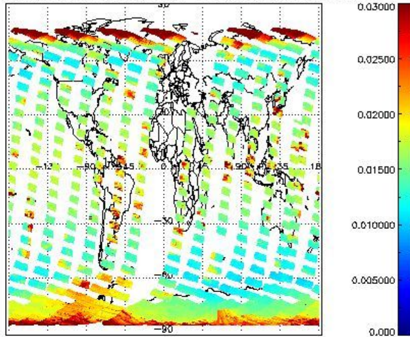
SCIOL2P_NADUV003_vcd_err for 21OCT2011 00:00:00 to 22OCT2011 00:00:00
