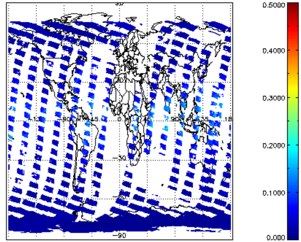
SCIOL2P_NADUV8H20_vcd_err for 21OCT2011 00:00:00 to 22OCT2011 00:00:00
