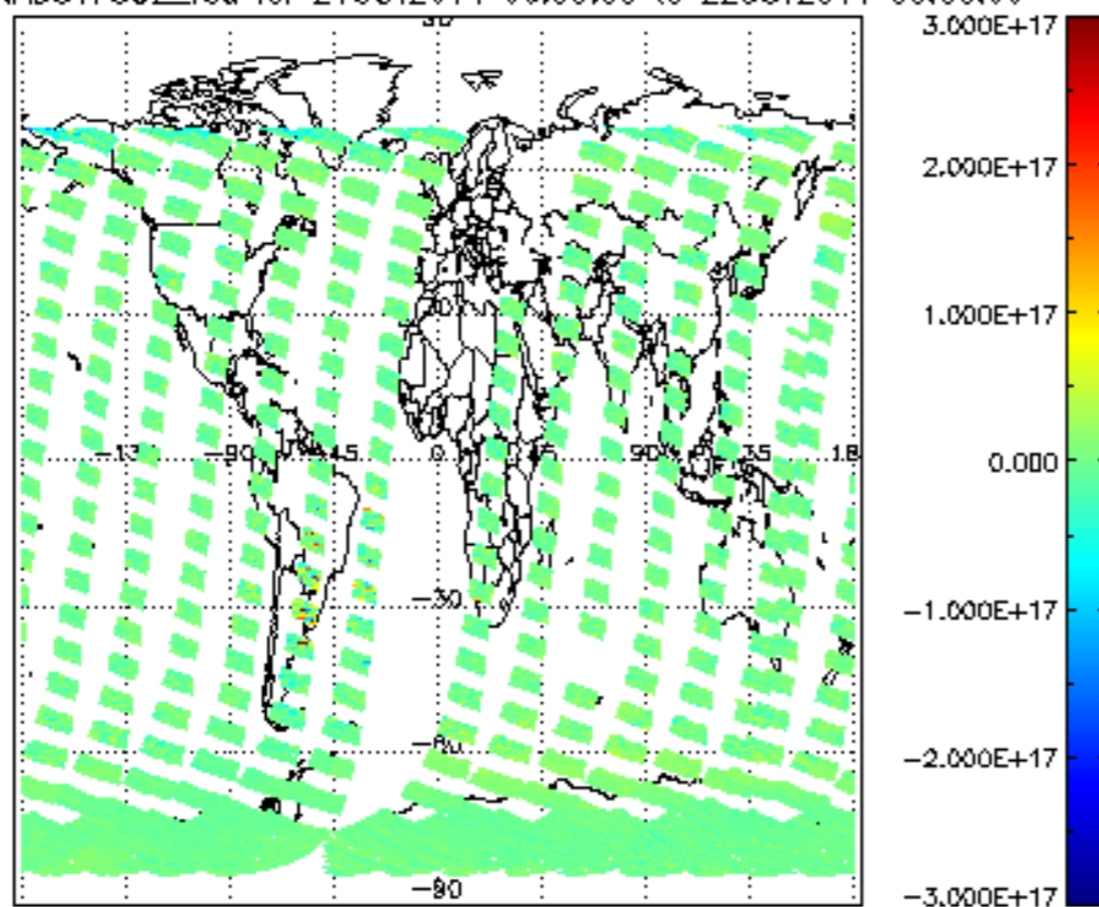
SCIOL2P_NADUV7S02_vcd for 21OCT2011 00:00:00 to 22OCT2011 00:00:00
