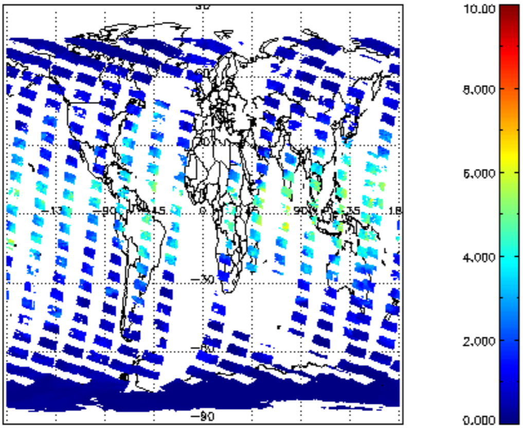
SCIOL2P_NADUV8H20_vcd for 21OCT2011 00:00:00 to 22OCT2011 00:00:00
