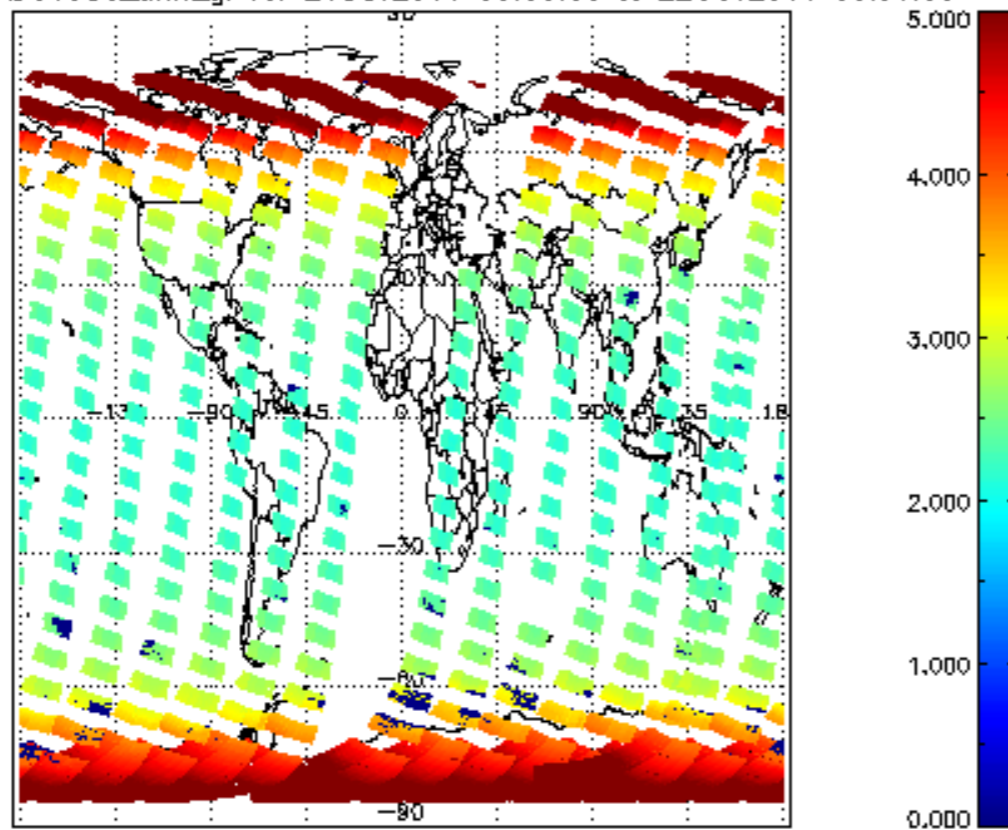
SCIOL2P_NADUV003_amf_gr for 21OCT2011 00:00:00 to 22OCT2011 00:00:00
