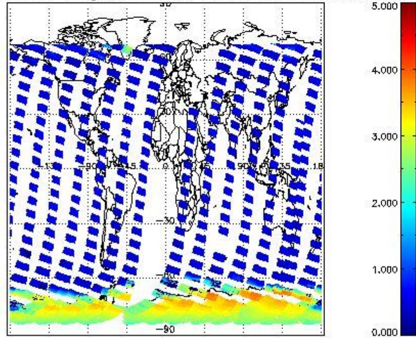
SCIOL2P_NADUV5S02_amf_gr for 21OCT2011 00:00:00 to 22OCT2011 00:00:00
