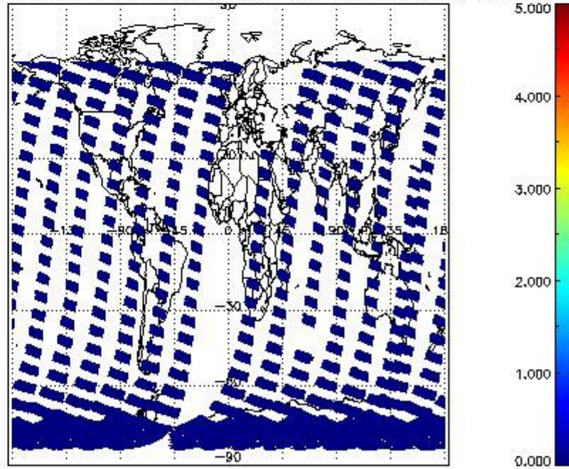
SCIOL2P_NADUV5S02_amf_cl for 21OCT2011 00:00:00 to 22OCT2011 00:00:00
