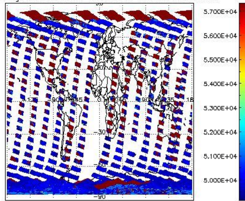
cloud_flags for 21OCT2011 00:00:00 to 22OCT2011 00:00:00
