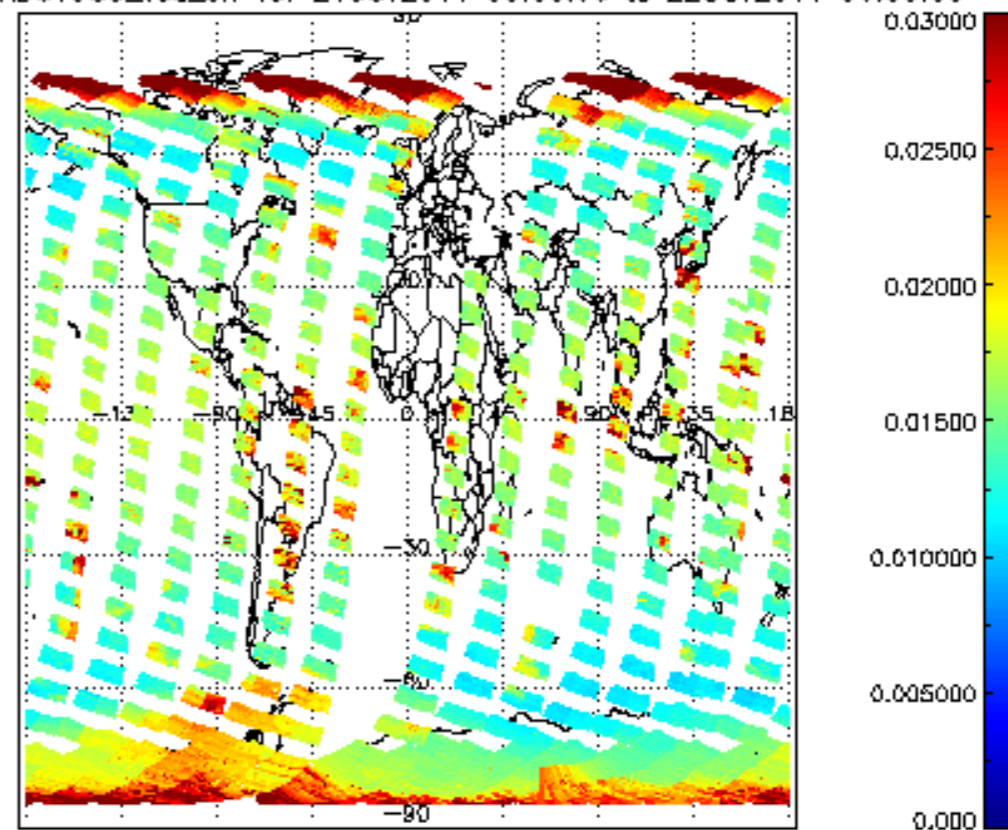
SCIOL2P_NADUV003_vcd_err for 21OCT2011 00:00:00 to 22OCT2011 00:00:00
