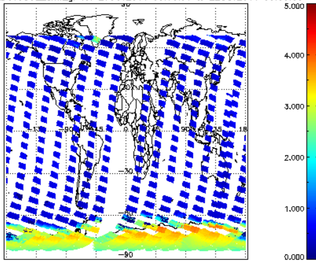
SCIOL2P_NADUV5S02_amf_gr for 21OCT2011 00:00:00 to 22OCT2011 00:00:00
