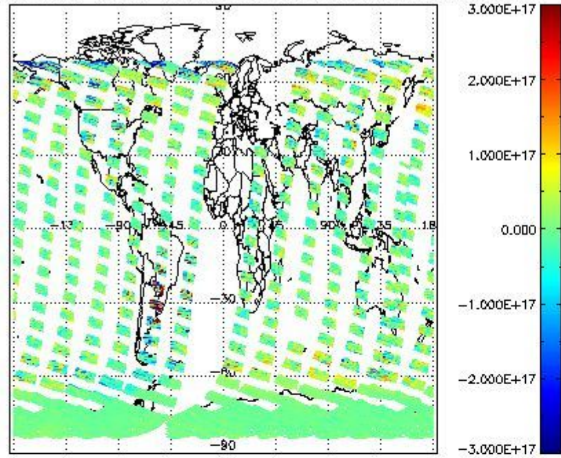
SCIOL2P_NADUV5S02_vcd for 21OCT2011 00:00:00 to 22OCT2011 00:00:00
