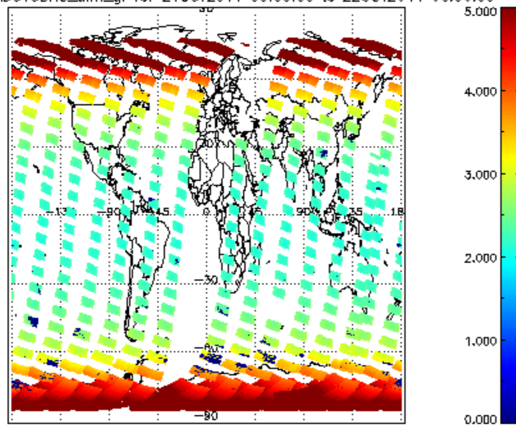
SCIOL2P_NADUV3BRO_amf_gr for 21OCT2011 00:00:00 to 22OCT2011 00:00:00
