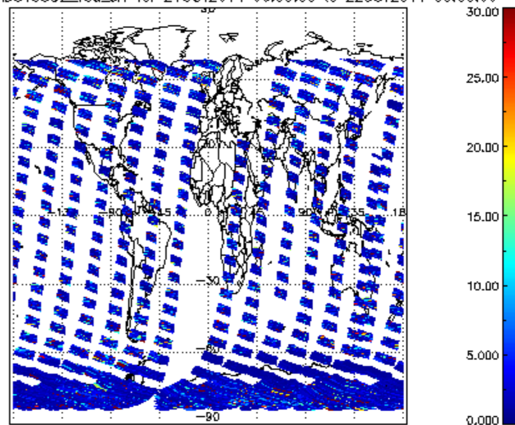
SCIOL2P_NADUV5S02_vcd_err for 21OCT2011 00:00:00 to 22OCT2011 00:00:00
