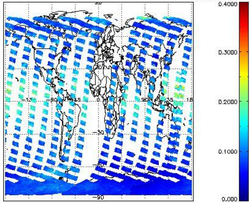
SCIOL2P_NADUV1NO2_vcd_err for 21OCT2011 00:00:00 to 22OCT2011 00:00:00
