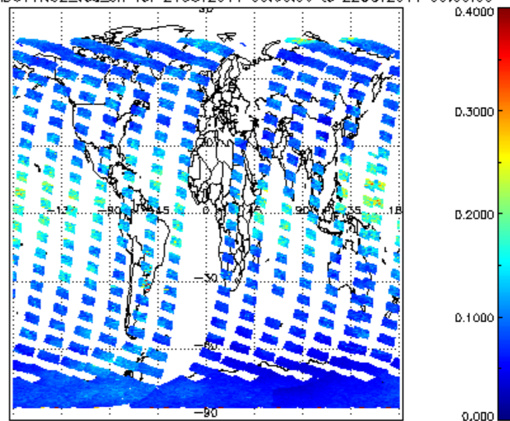
SCIOL2P_NADUV1NO2_vcd_err for 21OCT2011 00:00:00 to 22OCT2011 00:00:00
