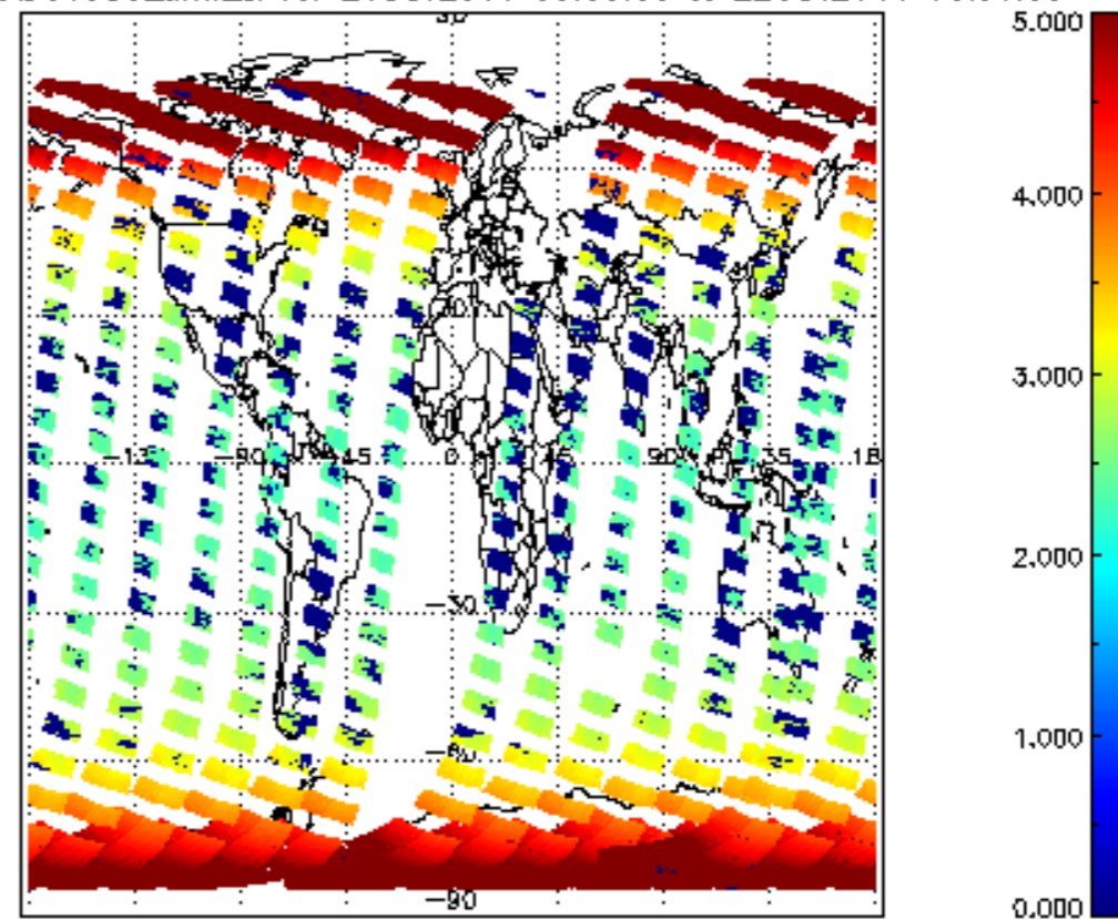
SCIOL2P_NADUV003_amf_cl for 21OCT2011 00:00:00 to 22OCT2011 00:00:00
