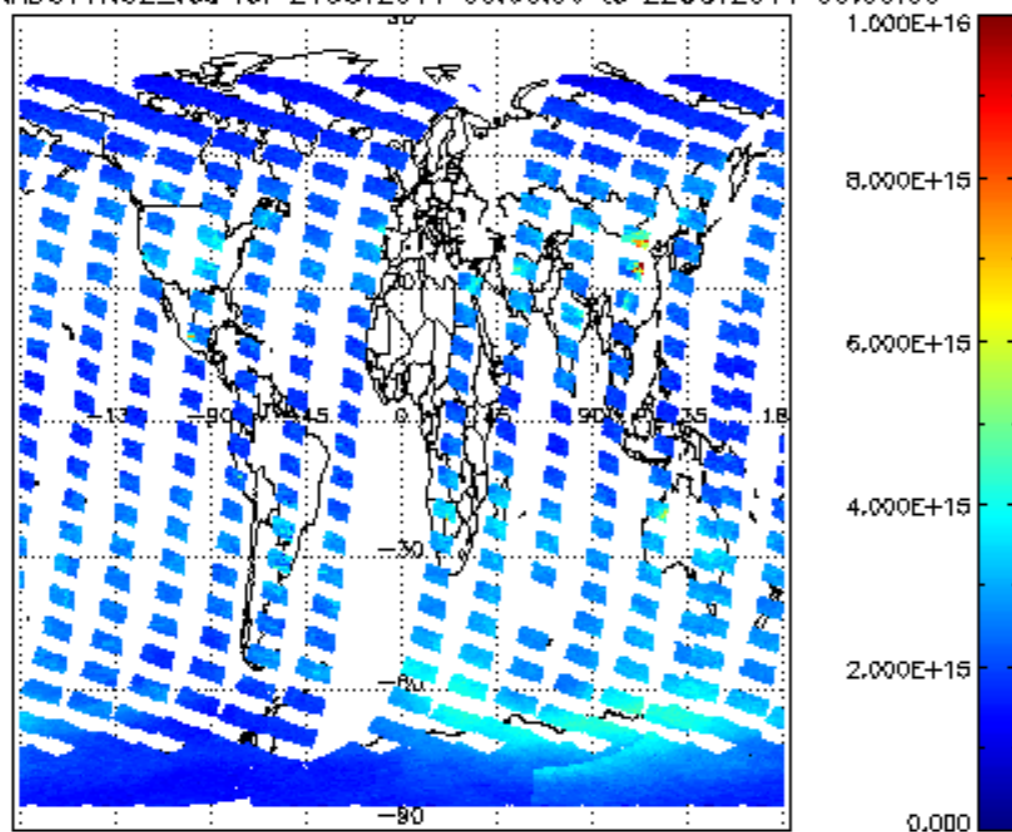
SCIOL2P_NADUV1NO2_vcd for 21OCT2011 00:00:00 to 22OCT2011 00:00:00
