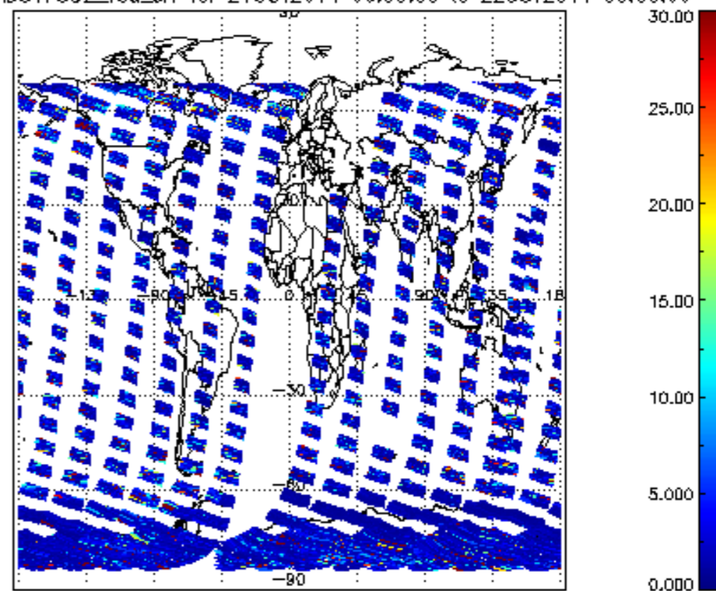
SCIOL2P_NADUV7S02_vcd_err for 21OCT2011 00:00:00 to 22OCT2011 00:00:00
