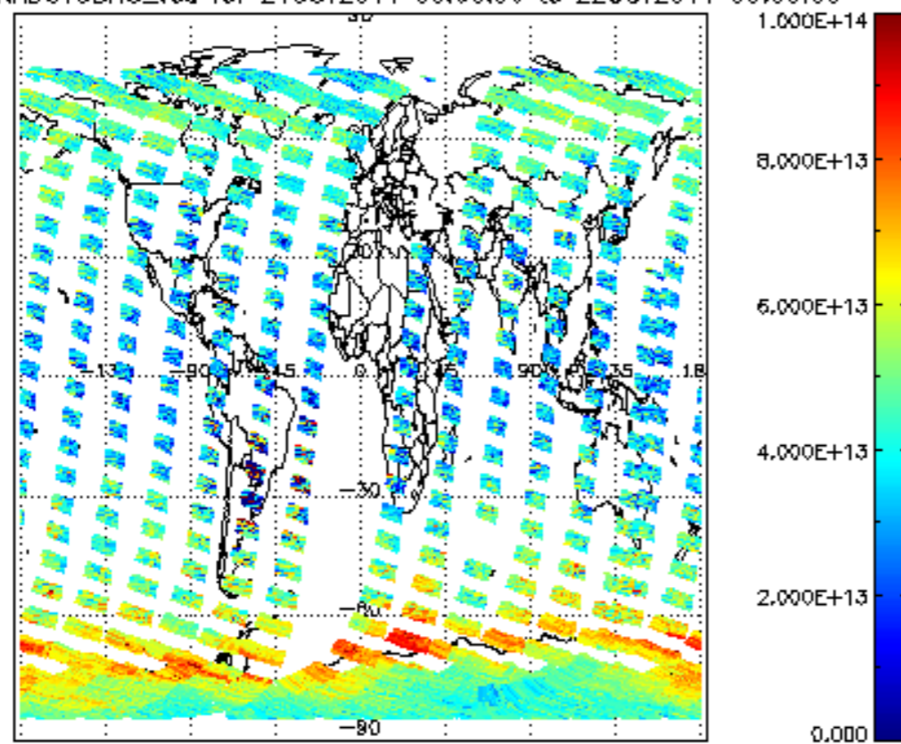
SCIOL2P_NADUV3BRO_vcd for 21OCT2011 00:00:00 to 22OCT2011 00:00:00
