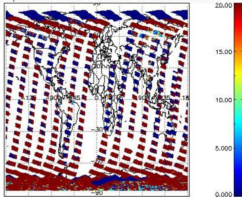
cL_opt_depth for 21OCT2011 00:00:00 to 22OCT2011 00:00:00
