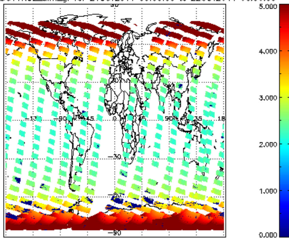
SCIOL2P_NADUV1NO2_amf_gr for 21OCT2011 00:00:00 to 22OCT2011 00:00:00
