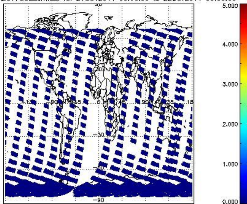
SCIOL2P_NADUV7S02_amf_cl for 21OCT2011 00:00:00 to 22OCT2011 00:00:00
