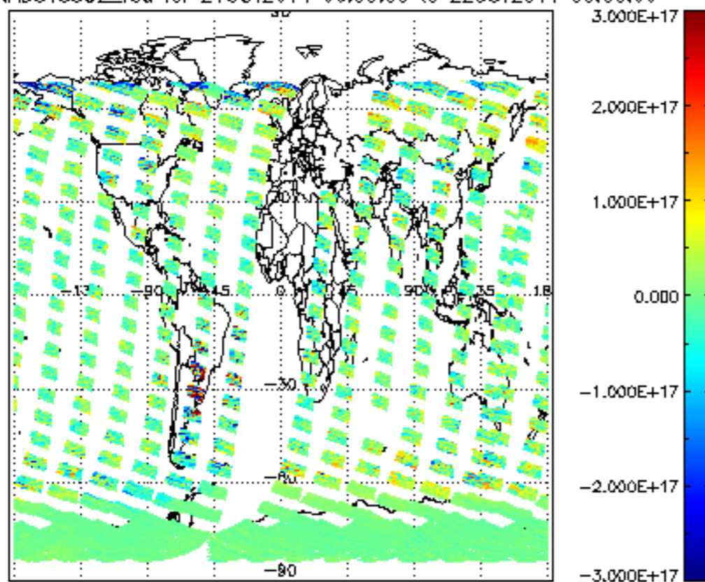
SCIOL2P_NADUV5S02_vcd for 21OCT2011 00:00:00 to 22OCT2011 00:00:00
