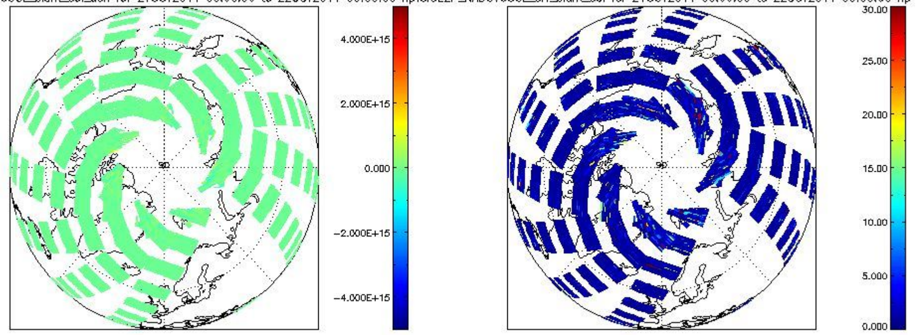
CIOL2P_NADUV60CL_slant_col_den for 21OCT2011 00:00:00 to 22OCT2011 00:00:00 np CIOL2P_NADUV60CL_err_slant_col for 21OCT2011 00:00:00 to 22OCT2011 00:00:00 np
