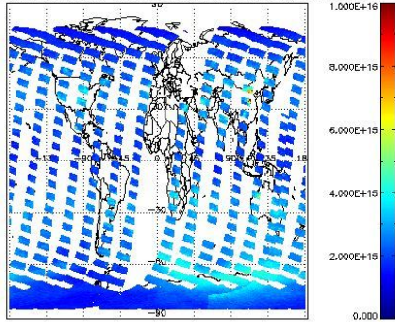
SCIOL2P_NADUV1NO2_vcd for 21OCT2011 00:00:00 to 22OCT2011 00:00:00
