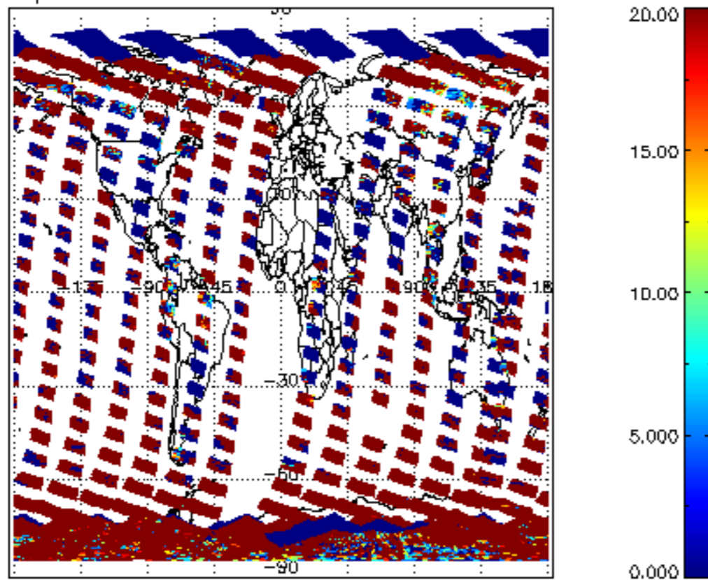
cl_opt_depth for 21OCT2011 00:00:00 to 22OCT2011 00:00:00
