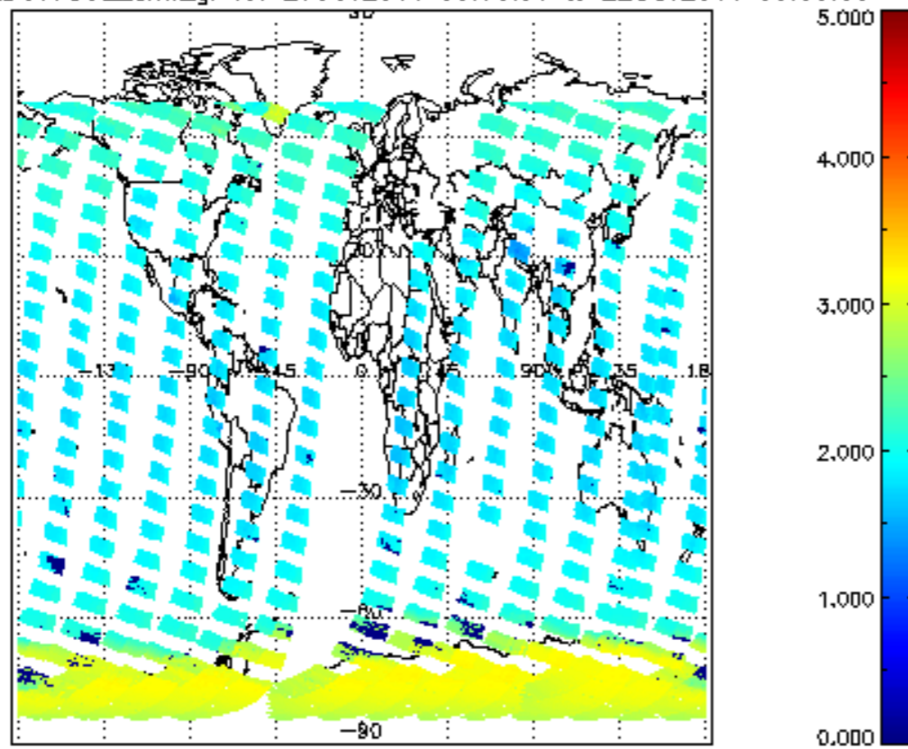
SCIOL2P_NADUV7S02_amf_gr for 21OCT2011 00:00:00 to 22OCT2011 00:00:00
