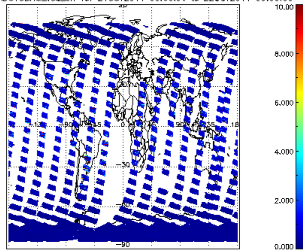
SCIOL2P_NADUV3BRO_vcd_err for 21OCT2011 00:00:00 to 22OCT2011 00:00:00
