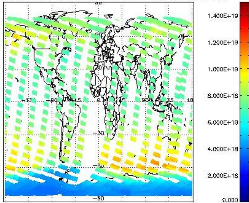
SCIOL2P_NADUV003_vcd for 21OCT2011 00:00:00 to 22OCT2011 00:00:00
