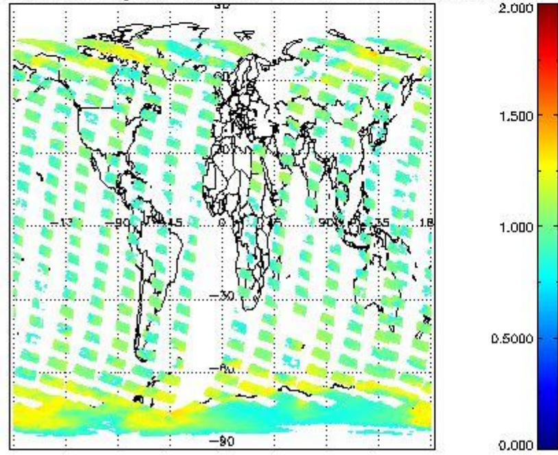
SCIOL2P_NADUV8H20_amf_gr for 21OCT2011 00:00:00 to 22OCT2011 00:00:00
