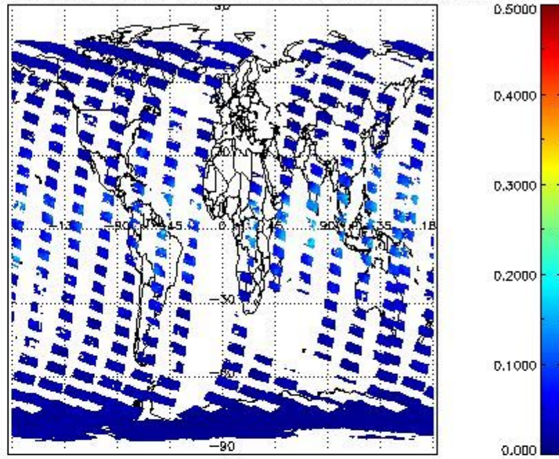
SCIOL2P_NADUV8H20_vcd_err for 21OCT2011 00:00:00 to 22OCT2011 00:00:00
