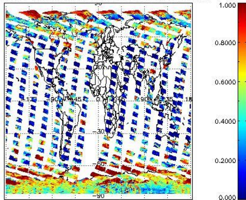
cLfrac for 21OCT2011 00:00:00 to 22OCT2011 00:00:00
