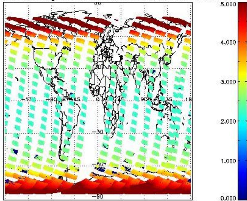
SCIOL2P_NADUV003_amf_gr for 21OCT2011 00:00:00 to 22OCT2011 00:00:00
