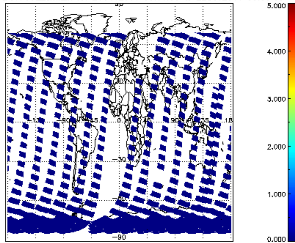
SCIOL2P_NADUV7S02_amf_sl for 21OCT2011 00:00:00 to 22OCT2011 00:00:00
