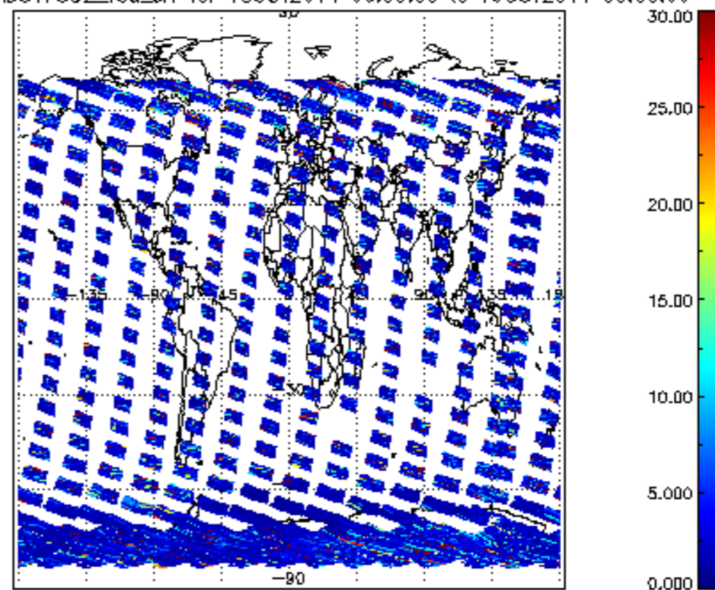
SCIOL2P_NADUV7S02_vcd_err for 18OCT2011 00:00:00 to 19OCT2011 00:00:00
