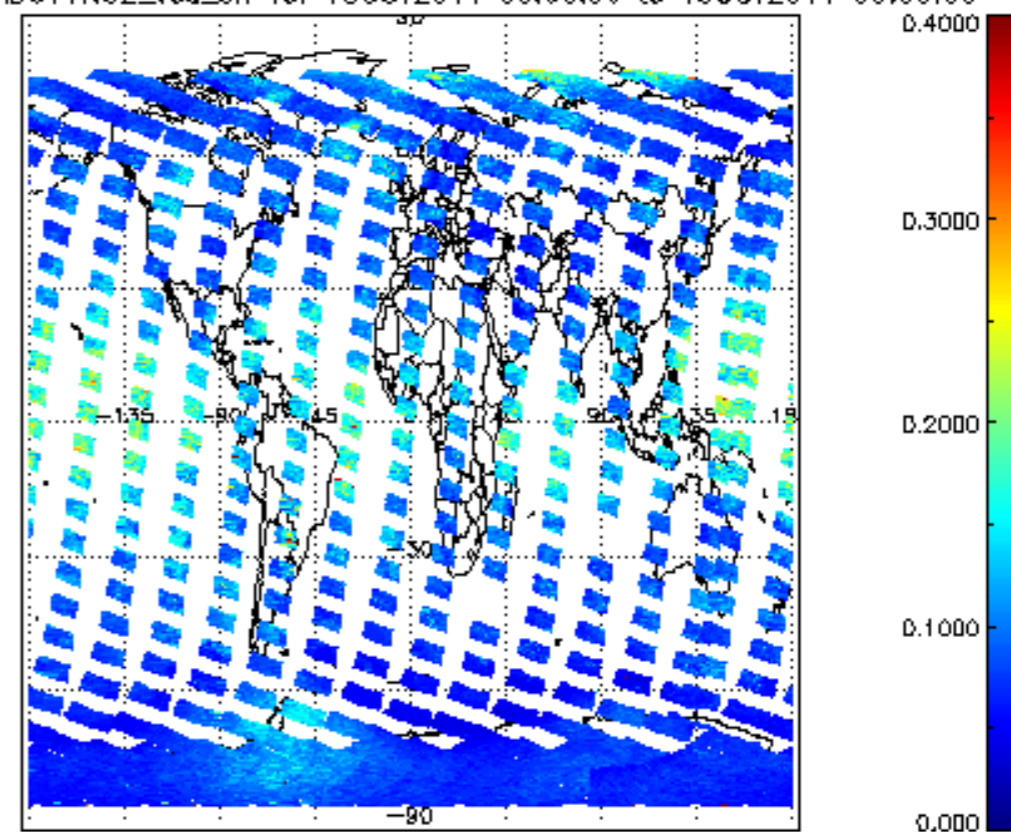
SCIOL2P_NADUV1NO2_vcd_err for 18OCT2011 00:00:00 to 19OCT2011 00:00:00
