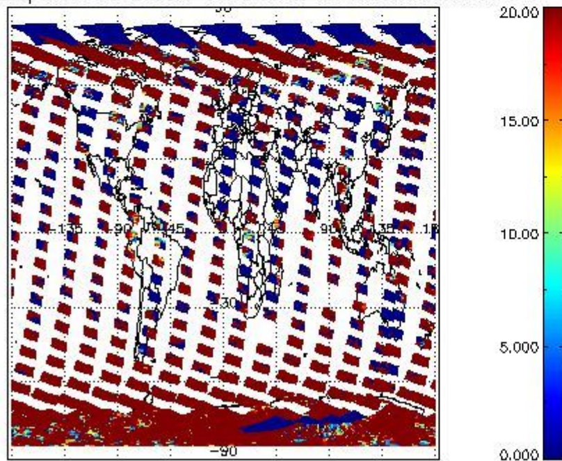
cL_opt_depth for 18OCT2011 00:00:00 to 19OCT2011 00:00:00
