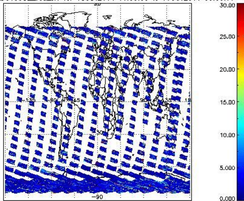
SCIOL2P_NADUV5S02_vcd_err for 18OCT2011 00:00:00 to 19OCT2011 00:00:00
