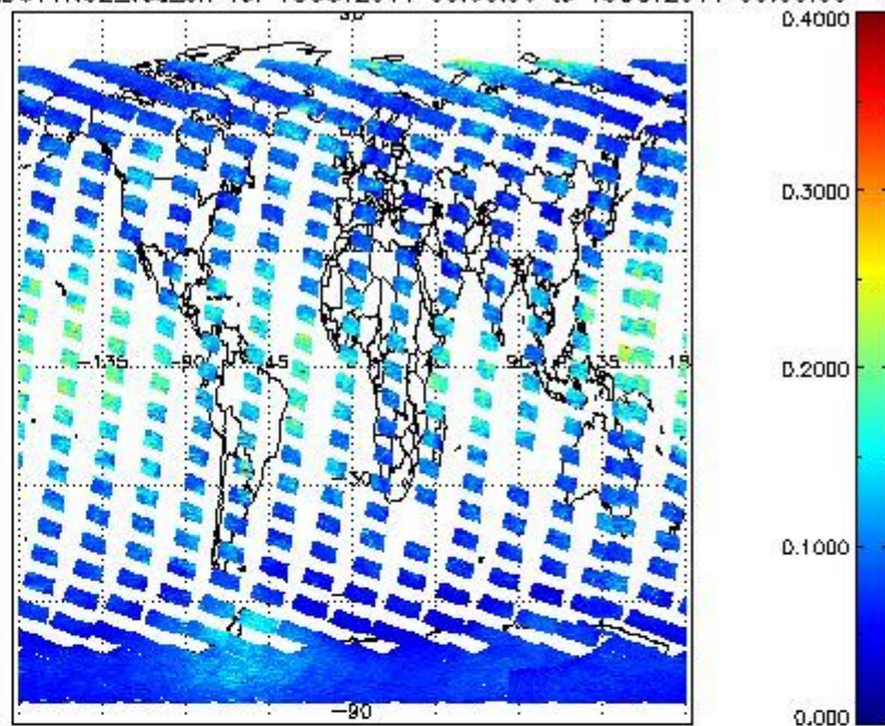
SCIOL2P_NADUV1NO2_vcd_err for 18OCT2011 00:00:00 to 19OCT2011 00:00:00
