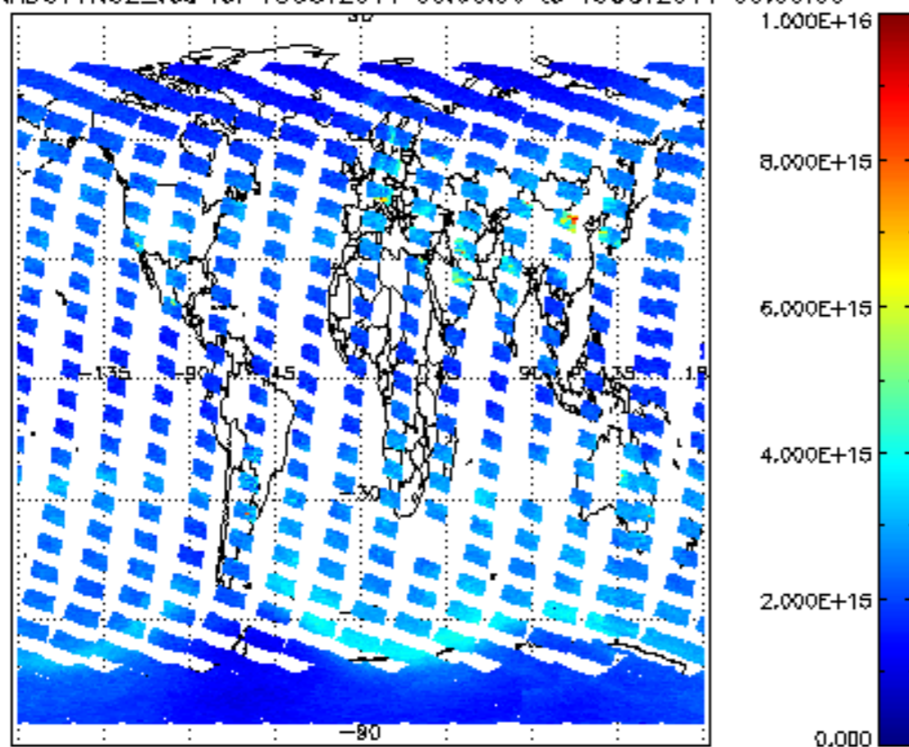
SCIOL2P_NADUV1NO2_vcd for 18OCT2011 00:00:00 to 19OCT2011 00:00:00
