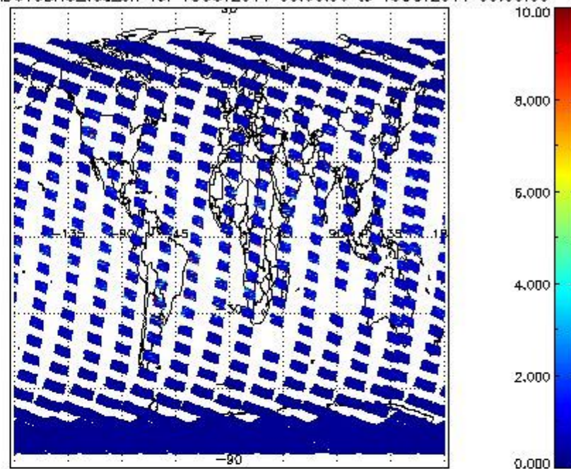
SCIOL2P_NADUV3BRO_vcd_err for 18OCT2011 00:00:00 to 19OCT2011 00:00:00
