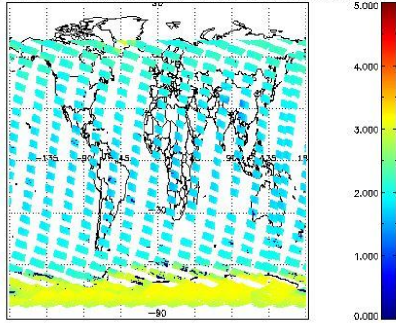
SCIOL2P_NADUV7S02_amf_gr for 18OCT2011 00:00:00 to 19OCT2011 00:00:00
