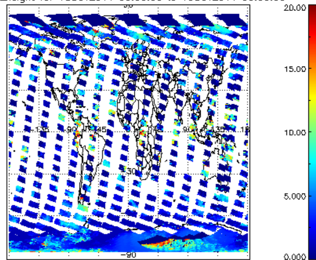
cl_top_height for 18OCT2011 00:00:00 to 19OCT2011 00:00:00
