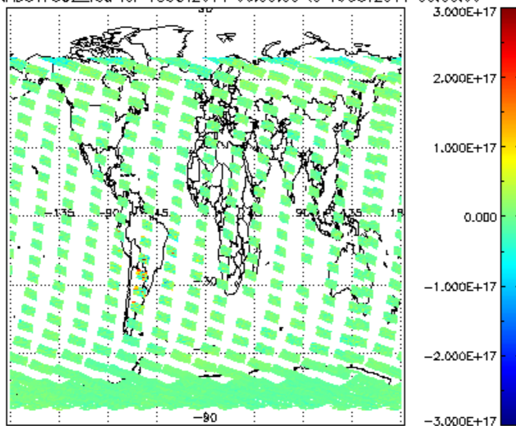
SCIOL2P_NADUV7S02_vcd for 18OCT2011 00:00:00 to 19OCT2011 00:00:00
