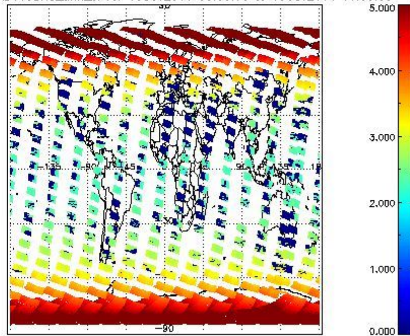
SCIOL2P_NADUV3BRO_amf_cl for 18OCT2011 00:00:00 to 19OCT2011 00:00:00
