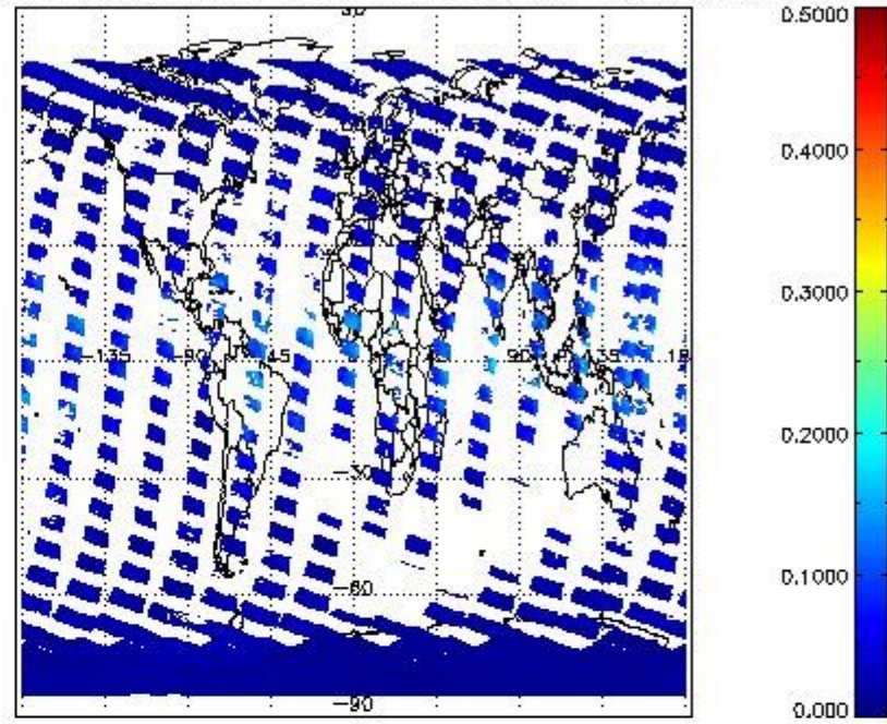
SCIOL2P_NADUV8H20_vcd_err for 18OCT2011 00:00:00 to 19OCT2011 00:00:00
