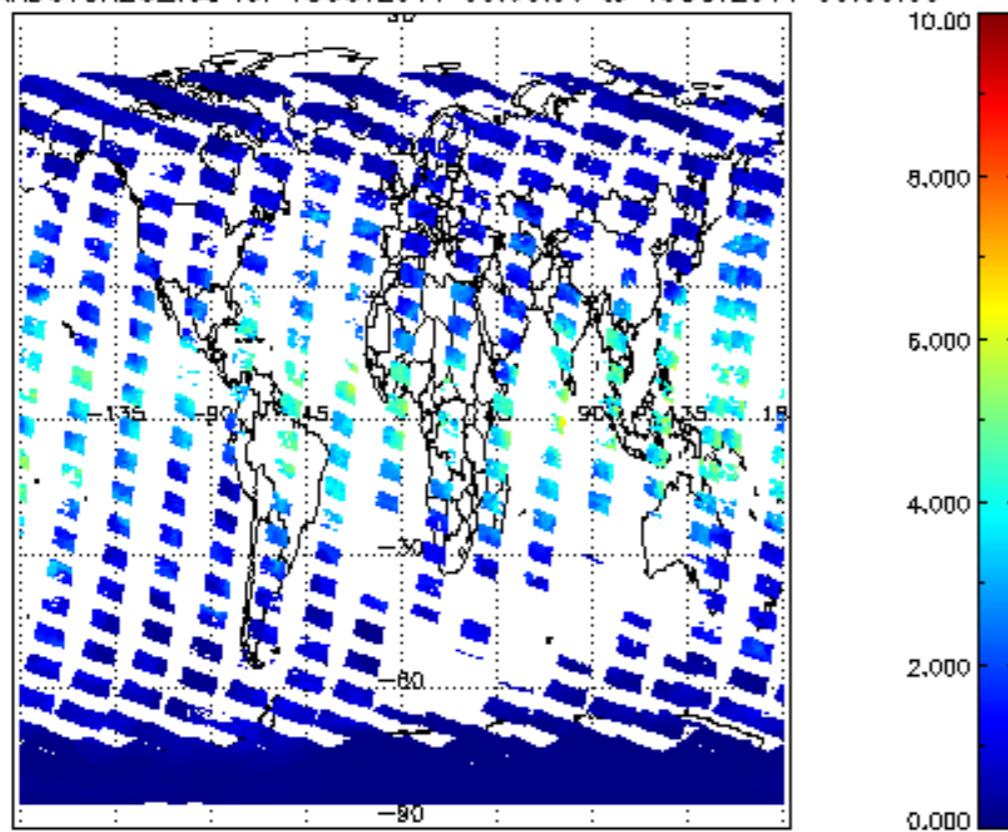
SCIOL2P_NADUV8H20_vcd for 18OCT2011 00:00:00 to 19OCT2011 00:00:00
