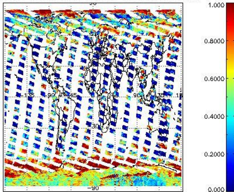
cLfrac for 18OCT2011 00:00:00 to 19OCT2011 00:00:00
