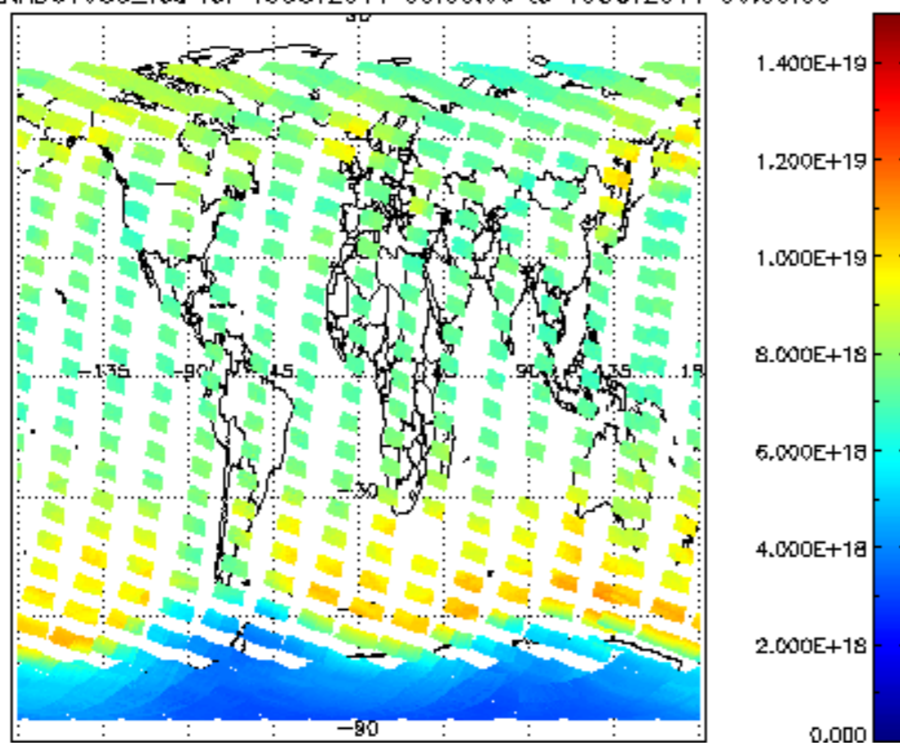
SCIOL2P_NADUV003_vcd for 18OCT2011 00:00:00 to 19OCT2011 00:00:00
