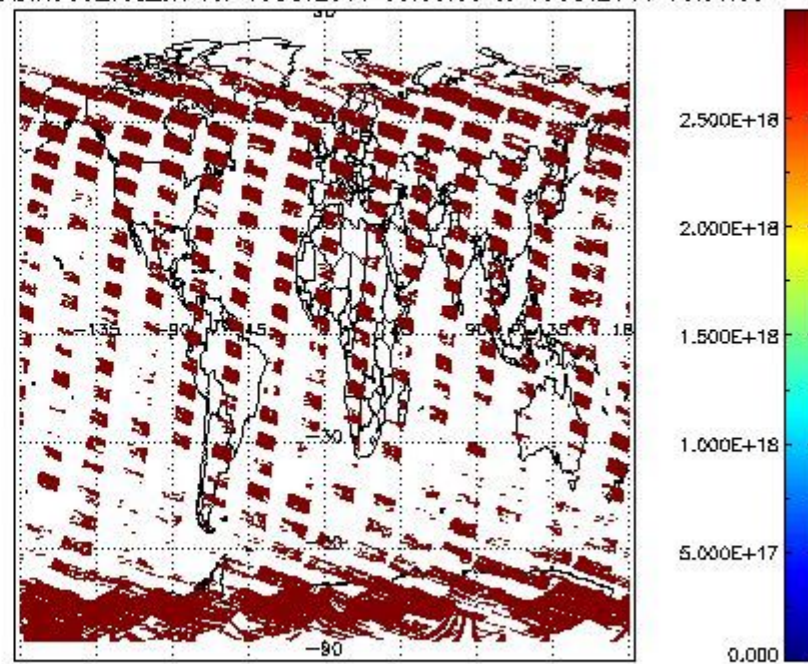
SCIOL2P_NADIR3CO_vcd_err for 18OCT2011 00:00:00 to 19OCT2011 00:00:00
