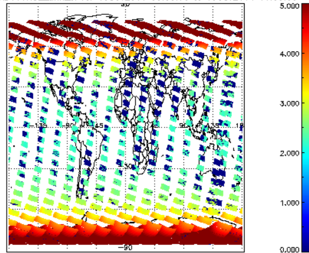
SCIOL2P_NADUV1NO2_amf_cl for 18OCT2011 00:00:00 to 19OCT2011 00:00:00
