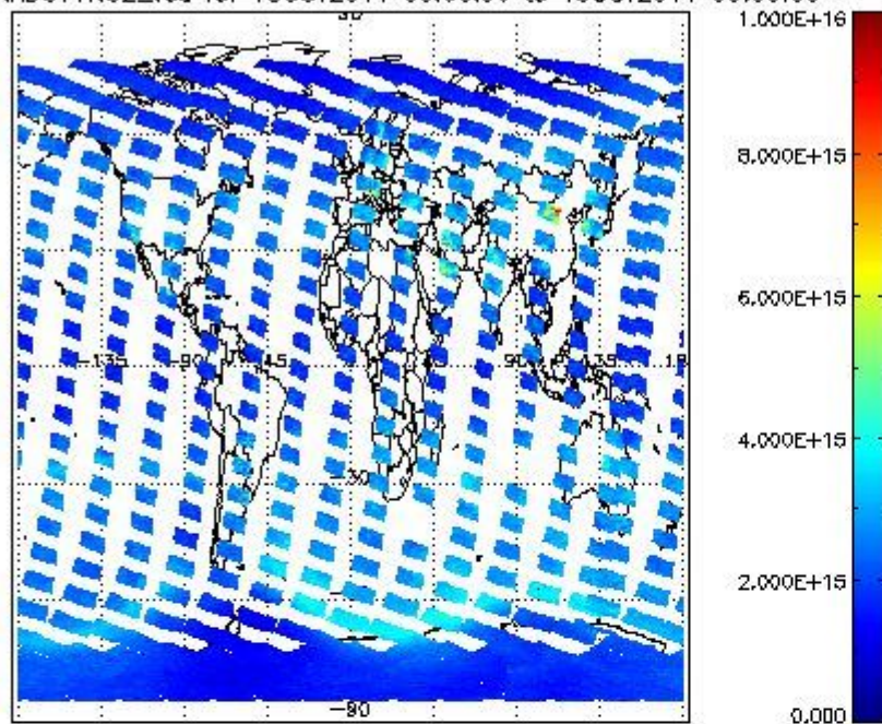
SCIOL2P_NADUV1NO2_vcd for 18OCT2011 00:00:00 to 19OCT2011 00:00:00
