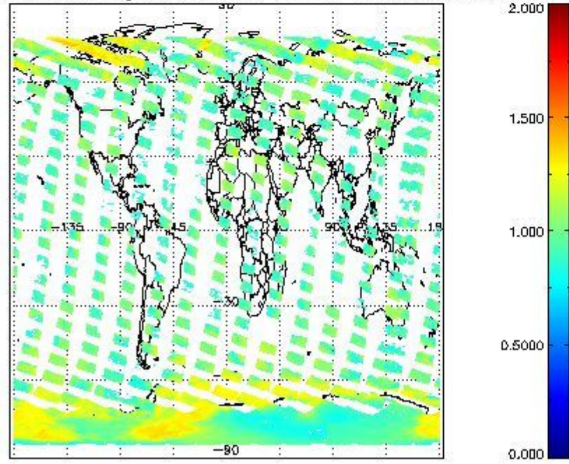
SCIOL2P_NADUV8H20_amf_gr for 18OCT2011 00:00:00 to 19OCT2011 00:00:00
