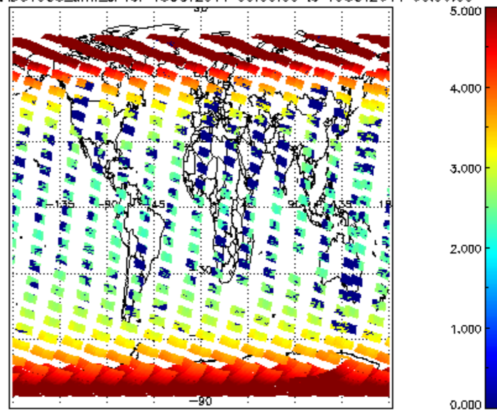
SCIOL2P_NADUV003_amf_cl for 18OCT2011 00:00:00 to 19OCT2011 00:00:00
