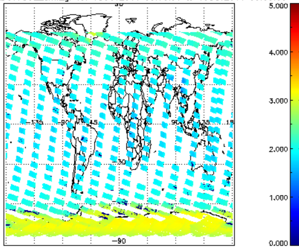
SCIOL2P_NADUV7S02_amf_gr for 18OCT2011 00:00:00 to 19OCT2011 00:00:00
