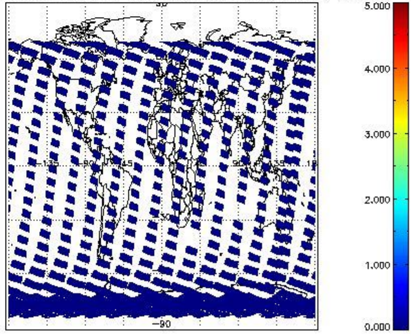
SCIOL2P_NADUV7S02_amf_cl for 18OCT2011 00:00:00 to 19OCT2011 00:00:00
