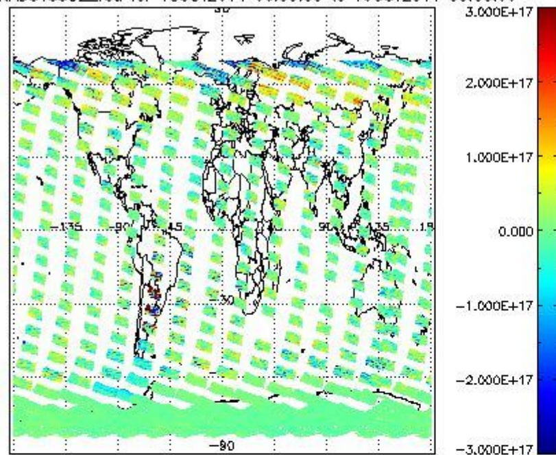
SCIOL2P_NADUV5S02_vcd for 18OCT2011 00:00:00 to 19OCT2011 00:00:00
