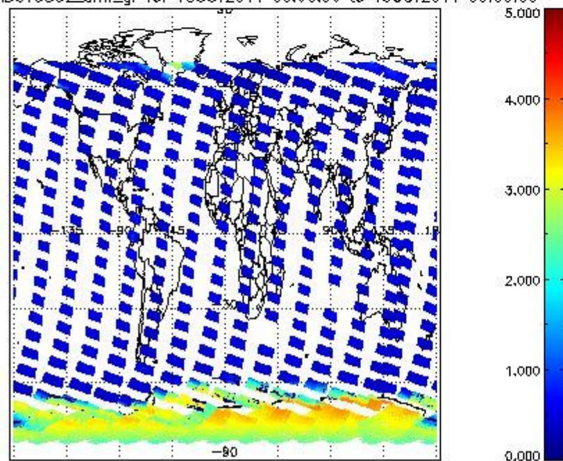
SCIOL2P_NADUV5S02_amf_gr for 18OCT2011 00:00:00 to 19OCT2011 00:00:00
