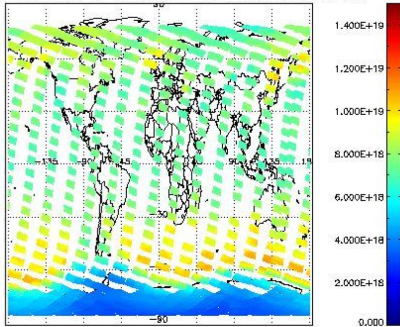
SCIOL2P_NADUV003_vcd for 18OCT2011 00:00:00 to 19OCT2011 00:00:00
