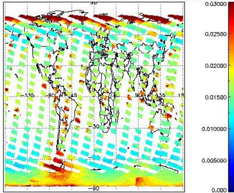
SCIOL2P_NADUV003_vcd_err for 18OCT2011 00:00:00 to 19OCT2011 00:00:00
