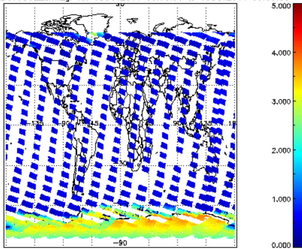
SCIOL2P_NADUV5S02_amf_gr for 18OCT2011 00:00:00 to 19OCT2011 00:00:00
