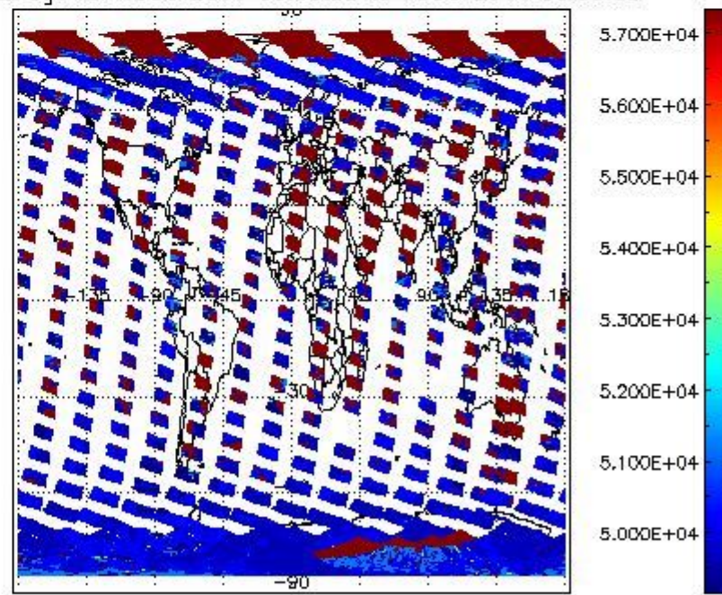
cloud_flags for 18OCT2011 00:00:00 to 19OCT2011 00:00:00
