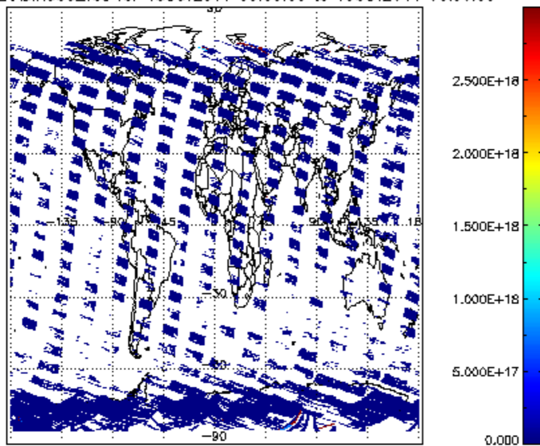
SCIOL2P_NADIR3CO_vcd for 18OCT2011 00:00:00 to 19OCT2011 00:00:00
