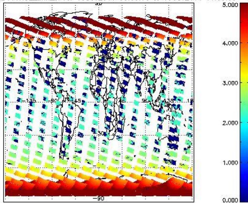
SCIOL2P_NADUV1NO2_amf_cl for 18OCT2011 00:00:00 to 19OCT2011 00:00:00
