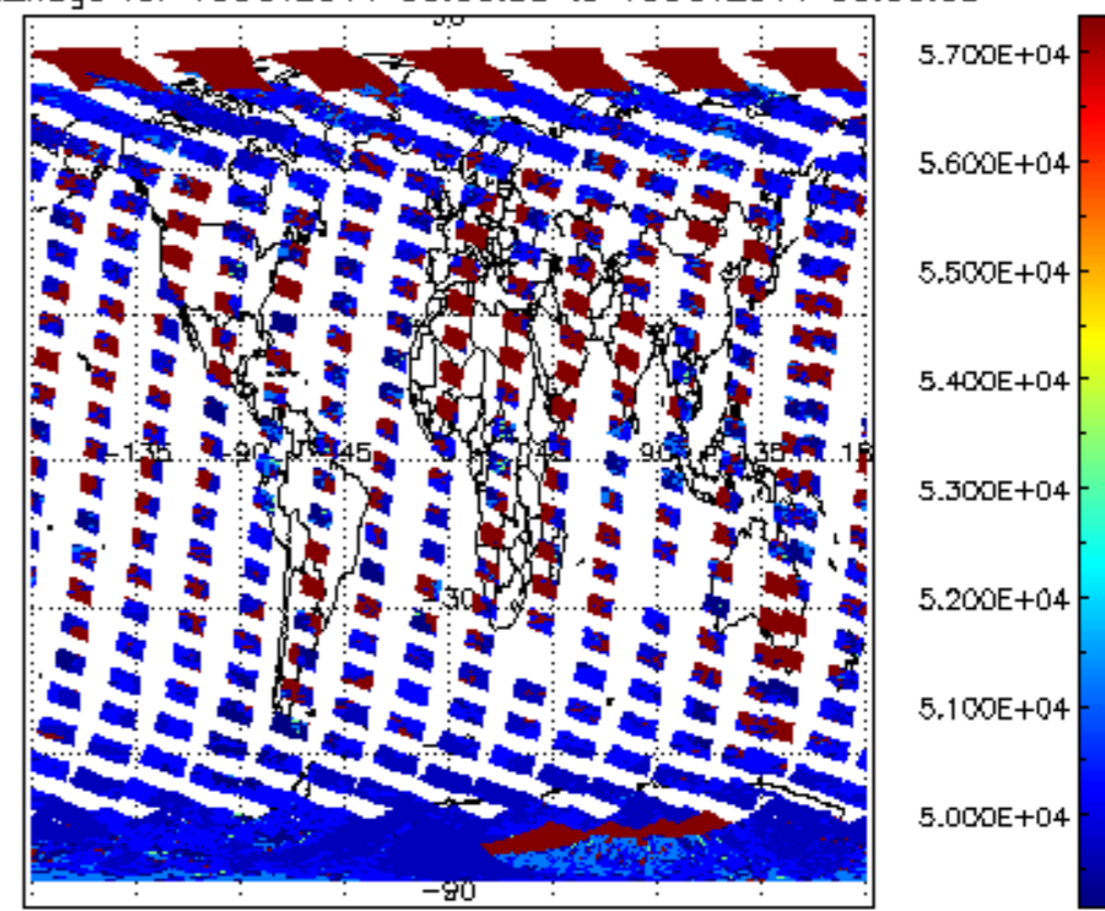
cloud_flags for 18OCT2011 00:00:00 to 19OCT2011 00:00:00
