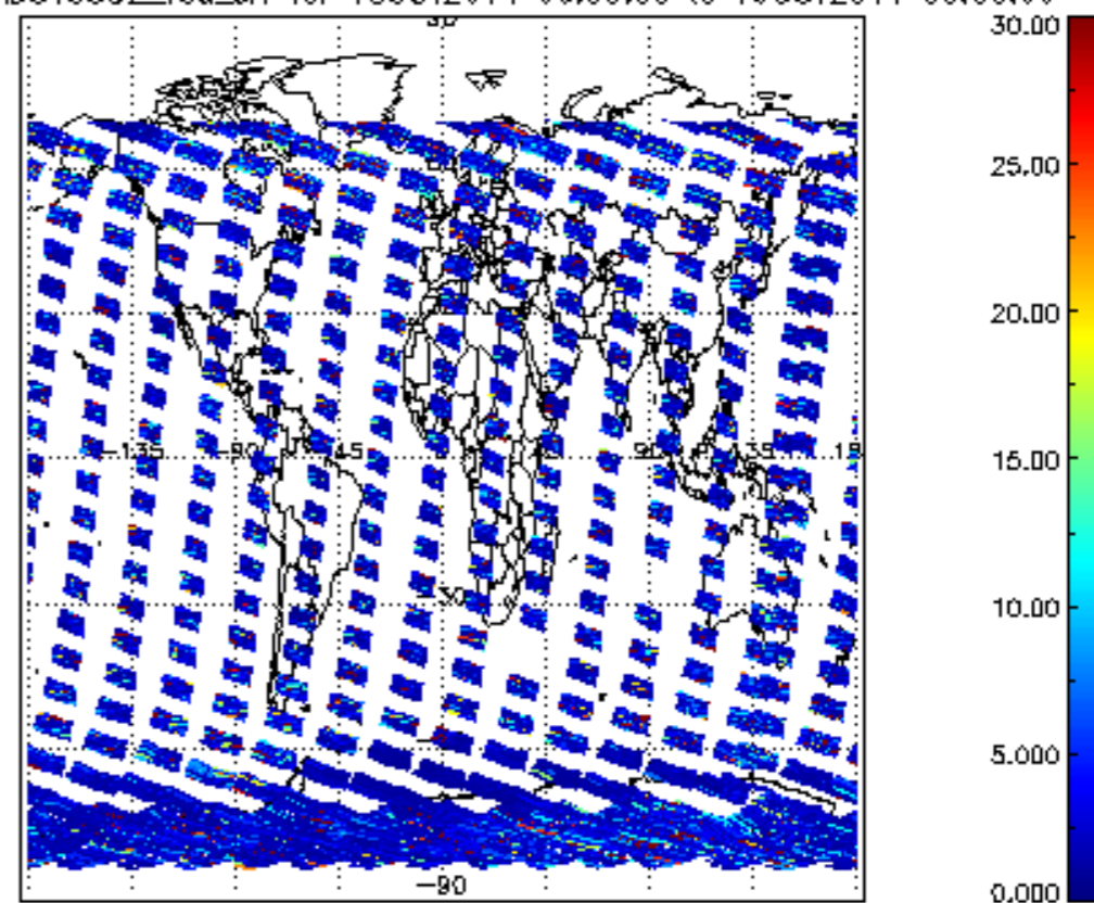
SCIOL2P_NADUV5S02_vcd_err for 18OCT2011 00:00:00 to 19OCT2011 00:00:00
