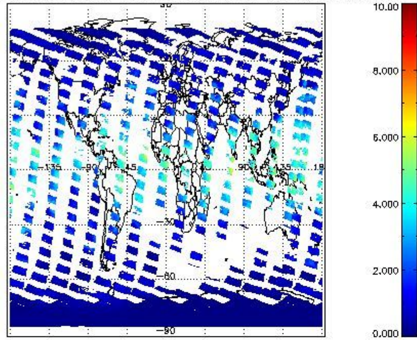
SCIOL2P_NADUV8H20_vcd for 18OCT2011 00:00:00 to 19OCT2011 00:00:00
