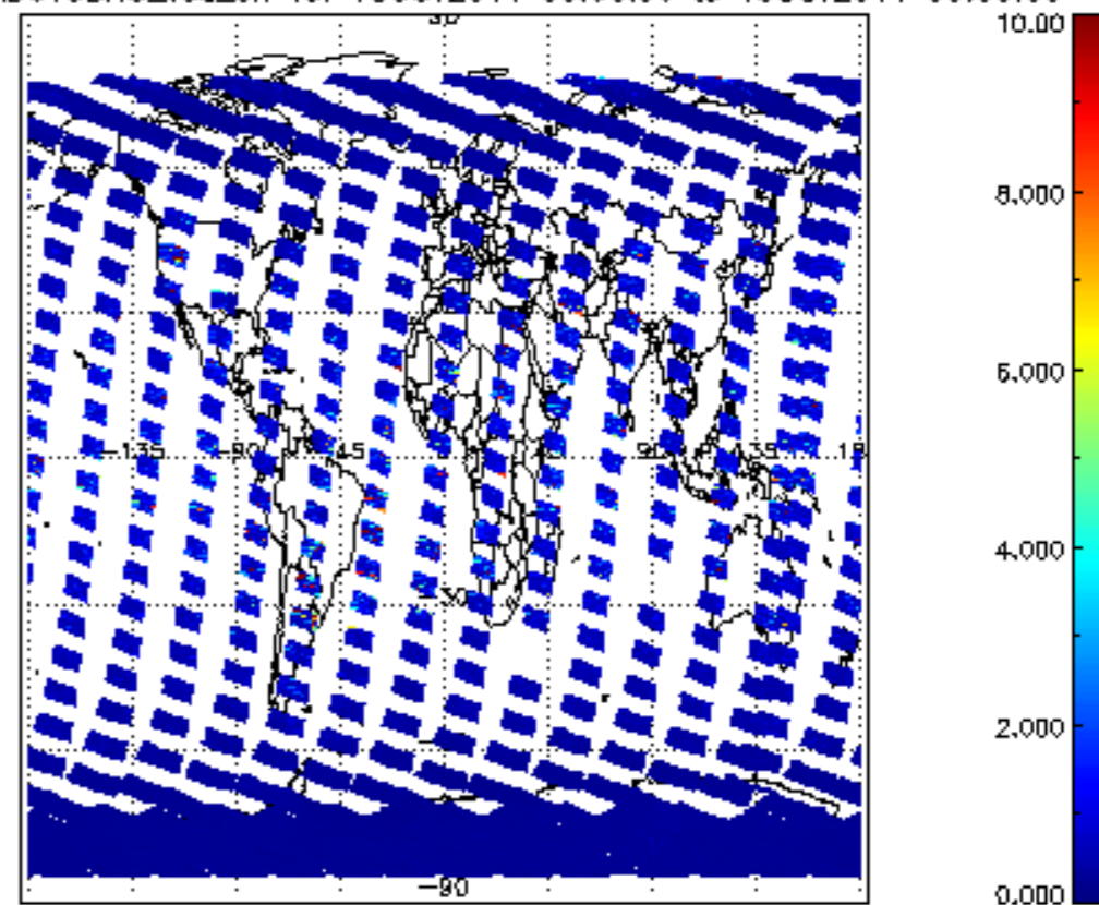
SCIOL2P_NADUV3BRO_vcd_err for 18OCT2011 00:00:00 to 19OCT2011 00:00:00
