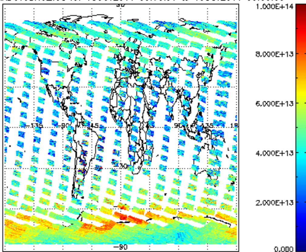
SCIOL2P_NADUV3BRO_vcd for 18OCT2011 00:00:00 to 19OCT2011 00:00:00
