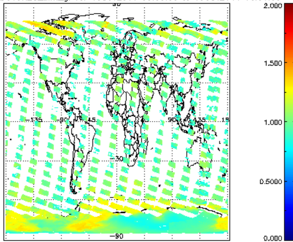
SCIOL2P_NADUV8H20_amf_gr for 18OCT2011 00:00:00 to 19OCT2011 00:00:00
