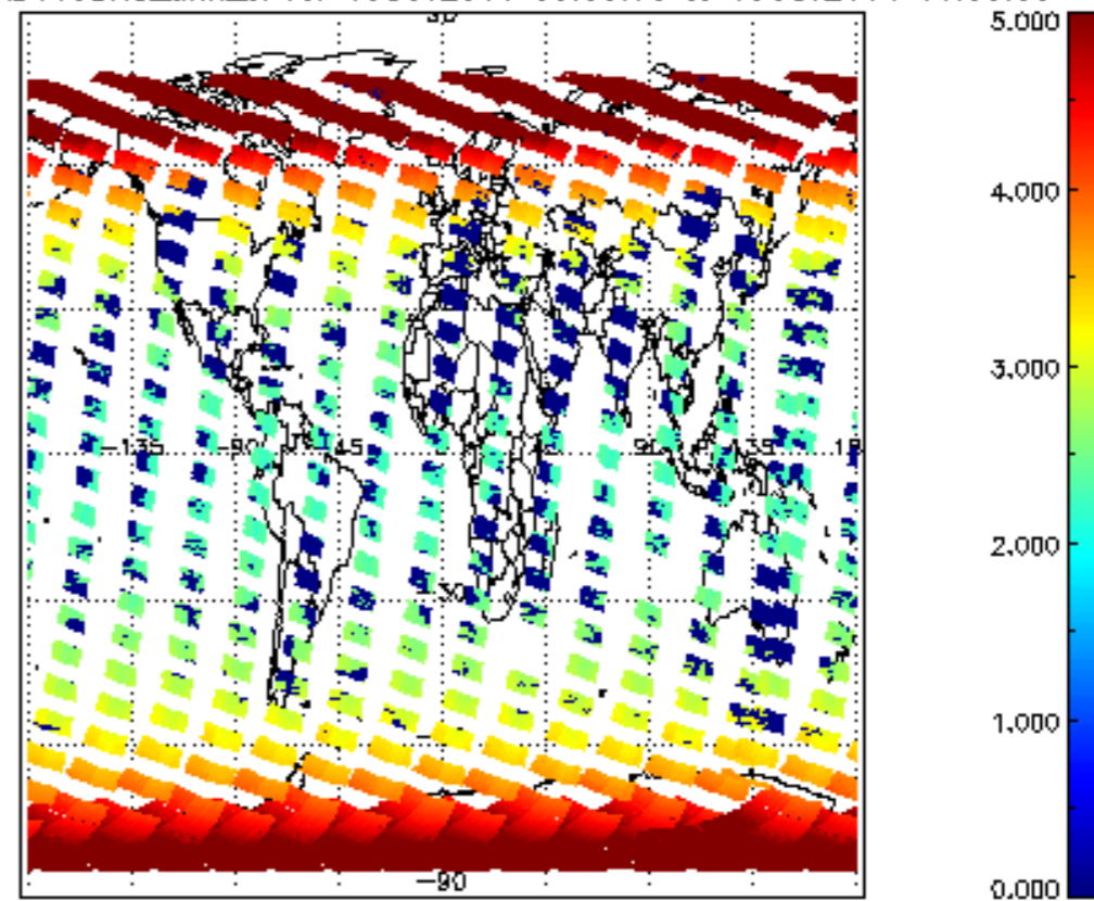
SCIOL2P_NADUV3BRO_amf_cl for 18OCT2011 00:00:00 to 19OCT2011 00:00:00
