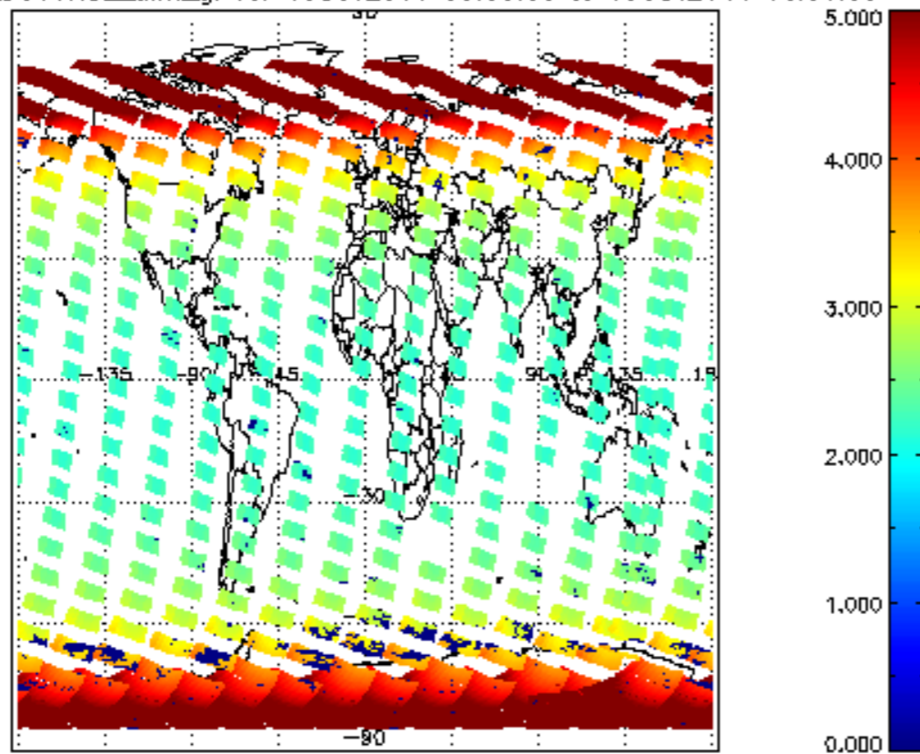
SCIOL2P_NADUV1NO2_amf_gr for 18OCT2011 00:00:00 to 19OCT2011 00:00:00
