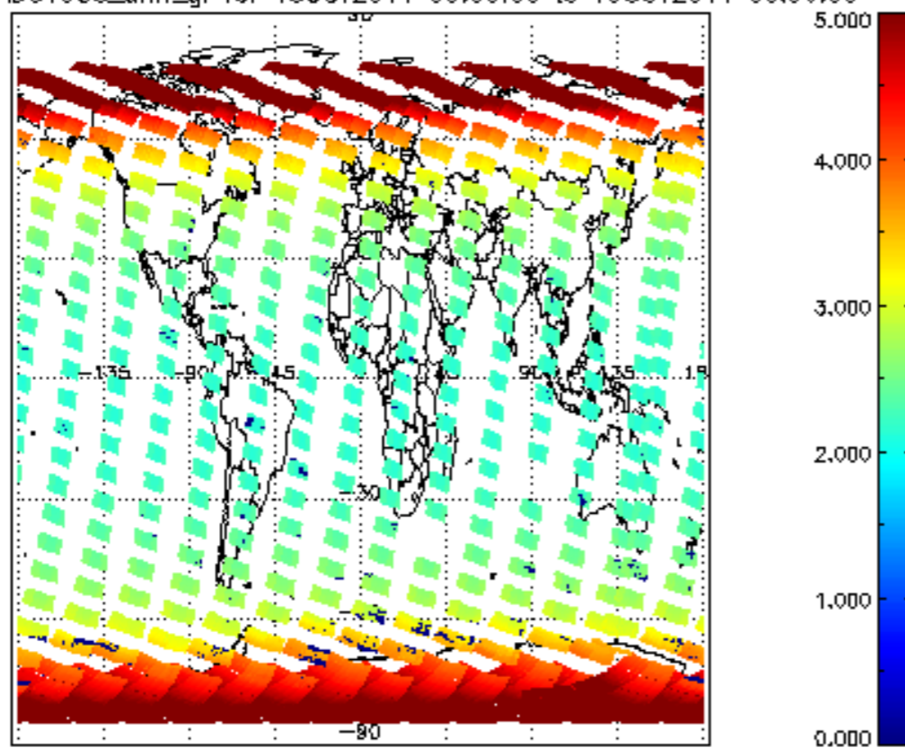
SCIOL2P_NADUV003_amf_gr for 18OCT2011 00:00:00 to 19OCT2011 00:00:00
