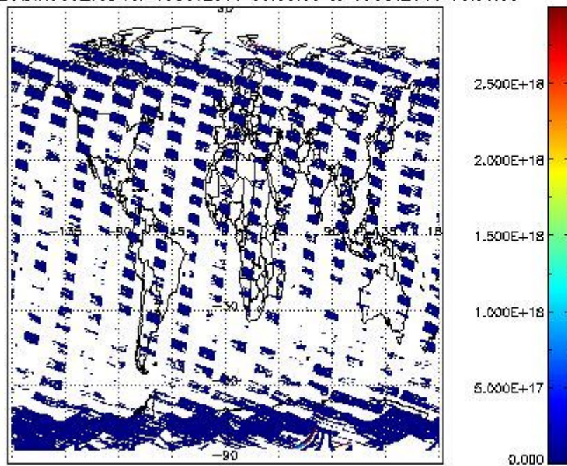
SCIOL2P_NADIR3CO_vcd for 18OCT2011 00:00:00 to 19OCT2011 00:00:00
