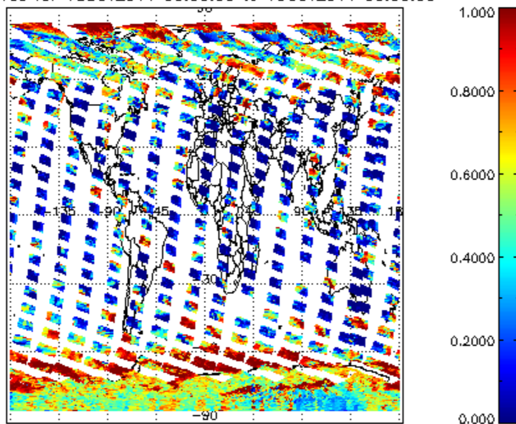
cl_frac for 18OCT2011 00:00:00 to 19OCT2011 00:00:00
