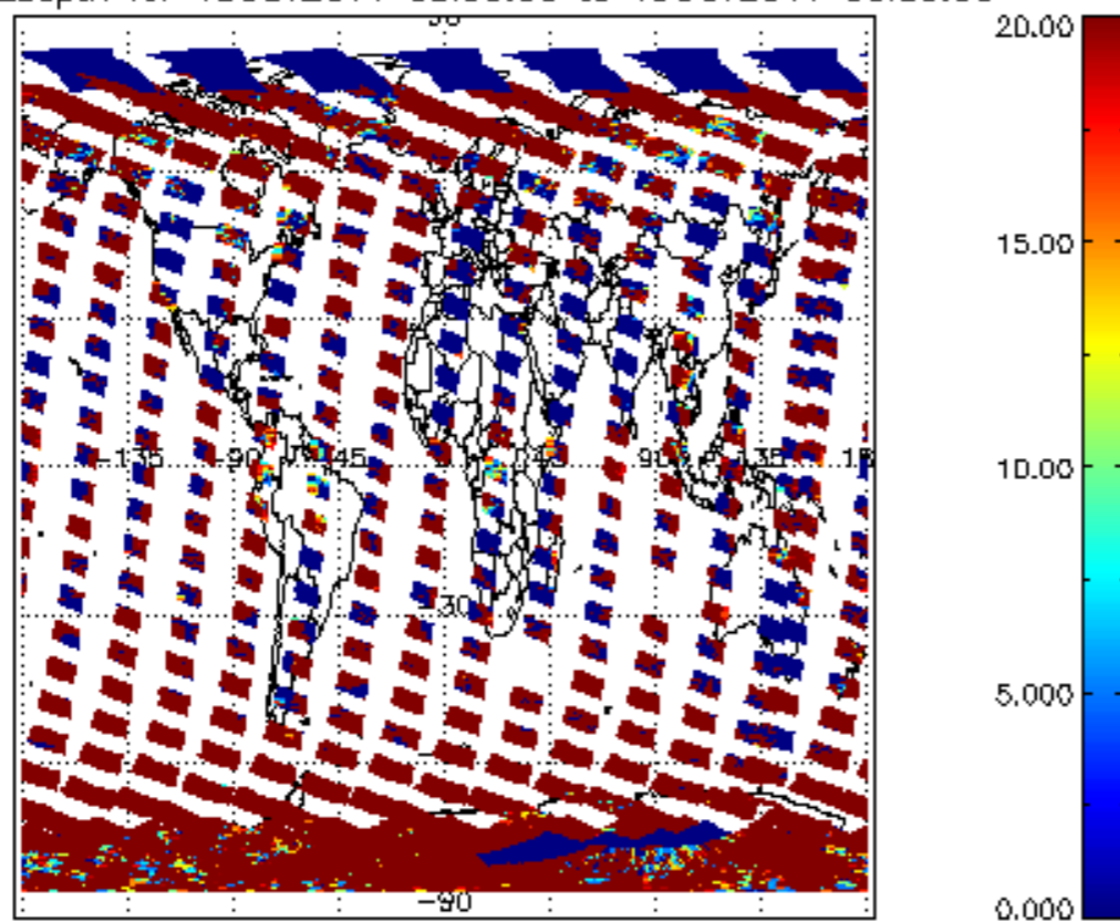
cl_opt_depth for 18OCT2011 00:00:00 to 19OCT2011 00:00:00
