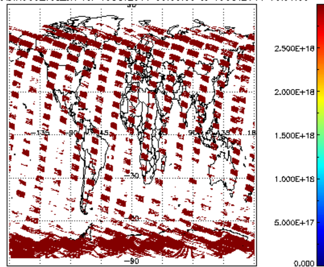
SCIOL2P_NADIR3CO_vcd_err for 18OCT2011 00:00:00 to 19OCT2011 00:00:00
