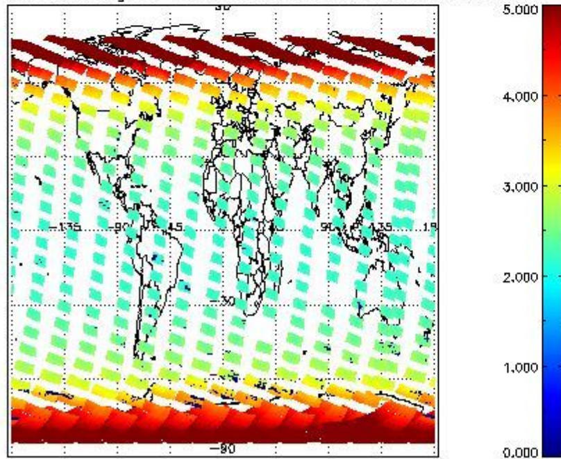
SCIOL2P_NADUV003_amf_gr for 18OCT2011 00:00:00 to 19OCT2011 00:00:00
