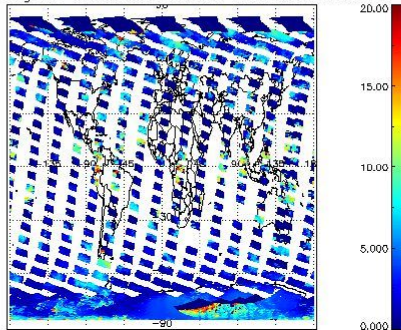
cL_top_height for 18OCT2011 00:00:00 to 19OCT2011 00:00:00
