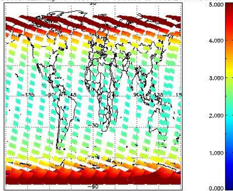
SCIOL2P_NADUV3BRO_amf_gr for 18OCT2011 00:00:00 to 19OCT2011 00:00:00
