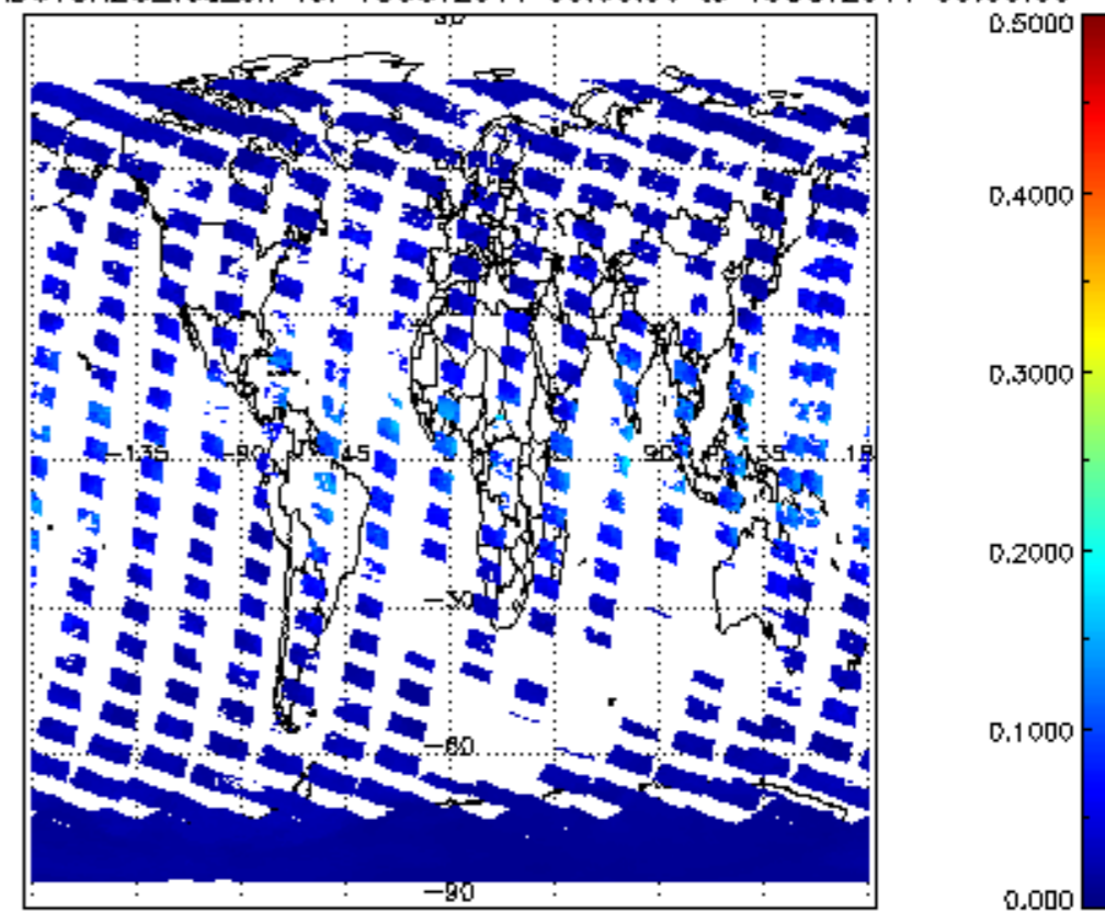
SCIOL2P_NADUV8H20_vcd_err for 18OCT2011 00:00:00 to 19OCT2011 00:00:00
