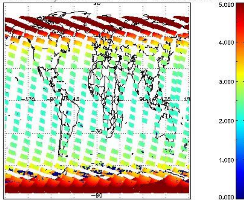
SCIOL2P_NADUV1NO2_amf_gr for 18OCT2011 00:00:00 to 19OCT2011 00:00:00
