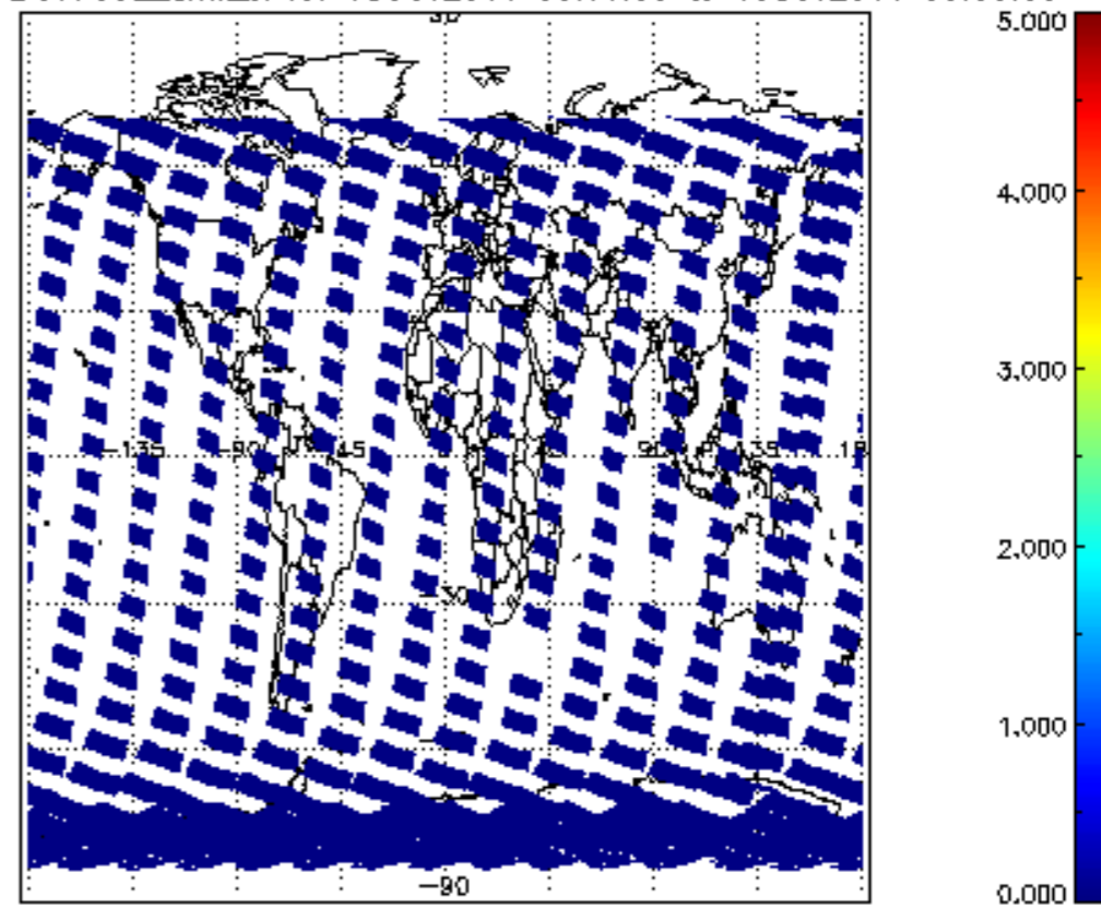
SCIOL2P_NADUV7S02_amf_cl for 18OCT2011 00:00:00 to 19OCT2011 00:00:00
