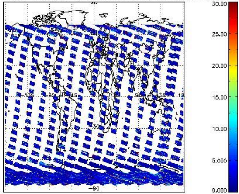
SCIOL2P_NADUV7S02_vcd_err for 18OCT2011 00:00:00 to 19OCT2011 00:00:00
