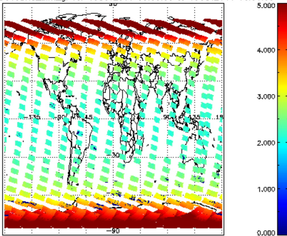
SCIOL2P_NADUV3BRO_amf_gr for 18OCT2011 00:00:00 to 19OCT2011 00:00:00
