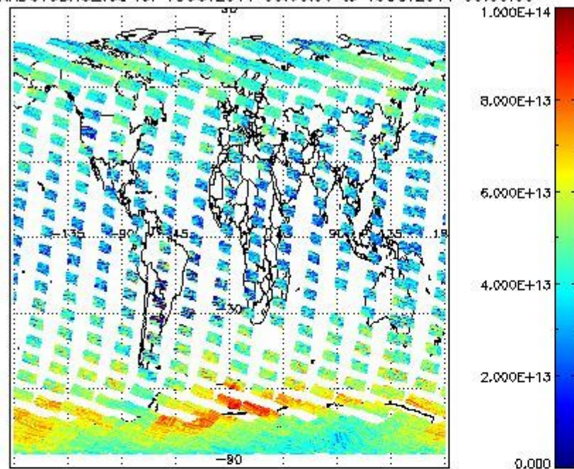
SCIOL2P_NADUV3BRO_vcd for 18OCT2011 00:00:00 to 19OCT2011 00:00:00
