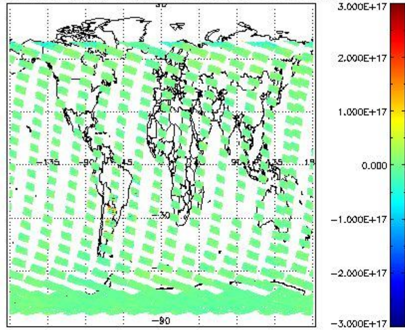
SCIOL2P_NADUV7S02_vcd for 18OCT2011 00:00:00 to 19OCT2011 00:00:00
