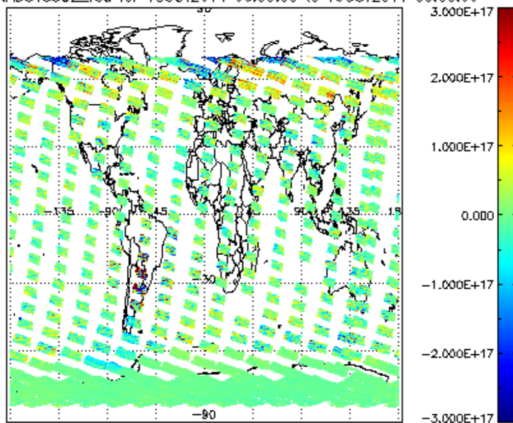
SCIOL2P_NADUV5S02_vcd for 18OCT2011 00:00:00 to 19OCT2011 00:00:00
