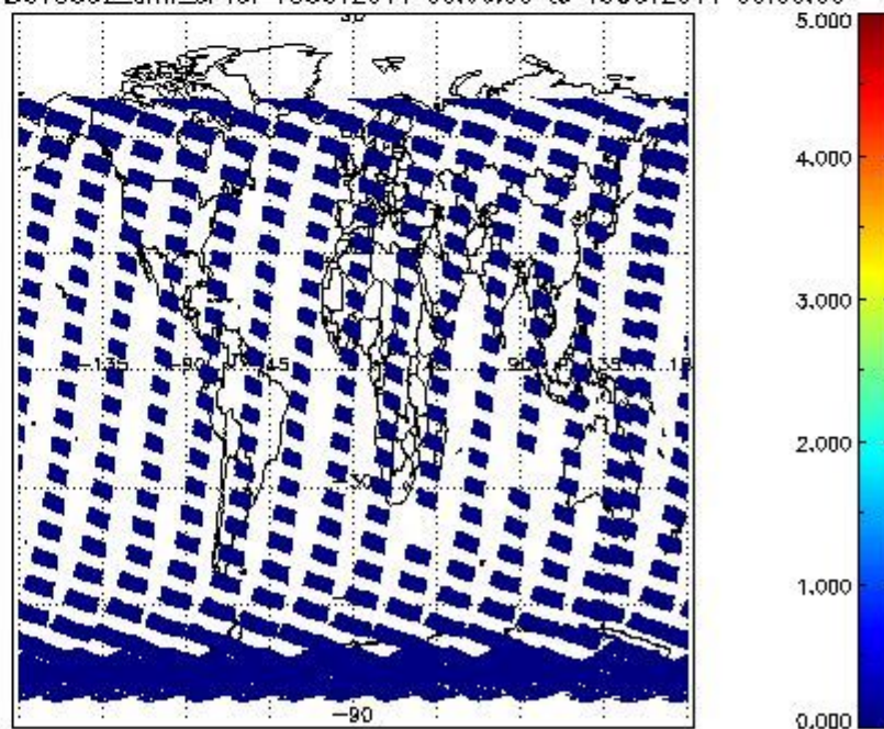
SCIOL2P_NADUV5S02_amf_cl for 18OCT2011 00:00:00 to 19OCT2011 00:00:00
