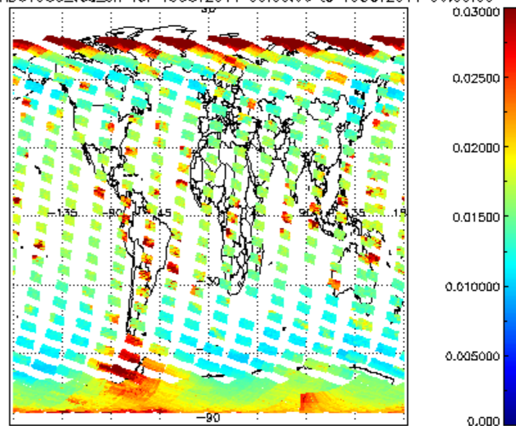
SCIOL2P_NADUV003_vcd_err for 18OCT2011 00:00:00 to 19OCT2011 00:00:00
