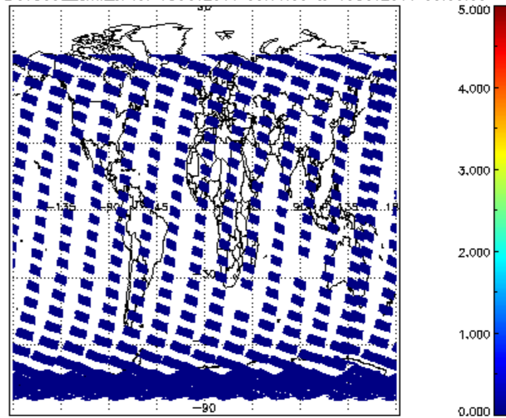
SCIOL2P_NADUV5S02_amf_cl for 18OCT2011 00:00:00 to 19OCT2011 00:00:00
