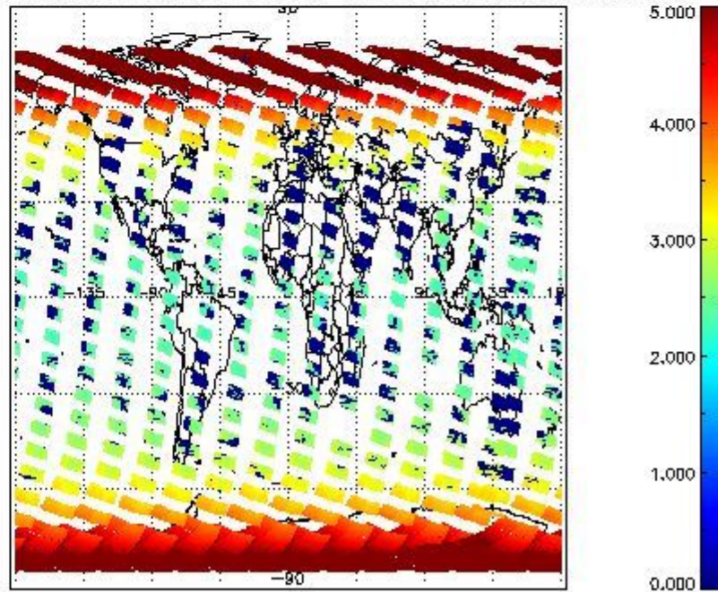
SCIOL2P_NADUV003_amf_cl for 18OCT2011 00:00:00 to 19OCT2011 00:00:00
