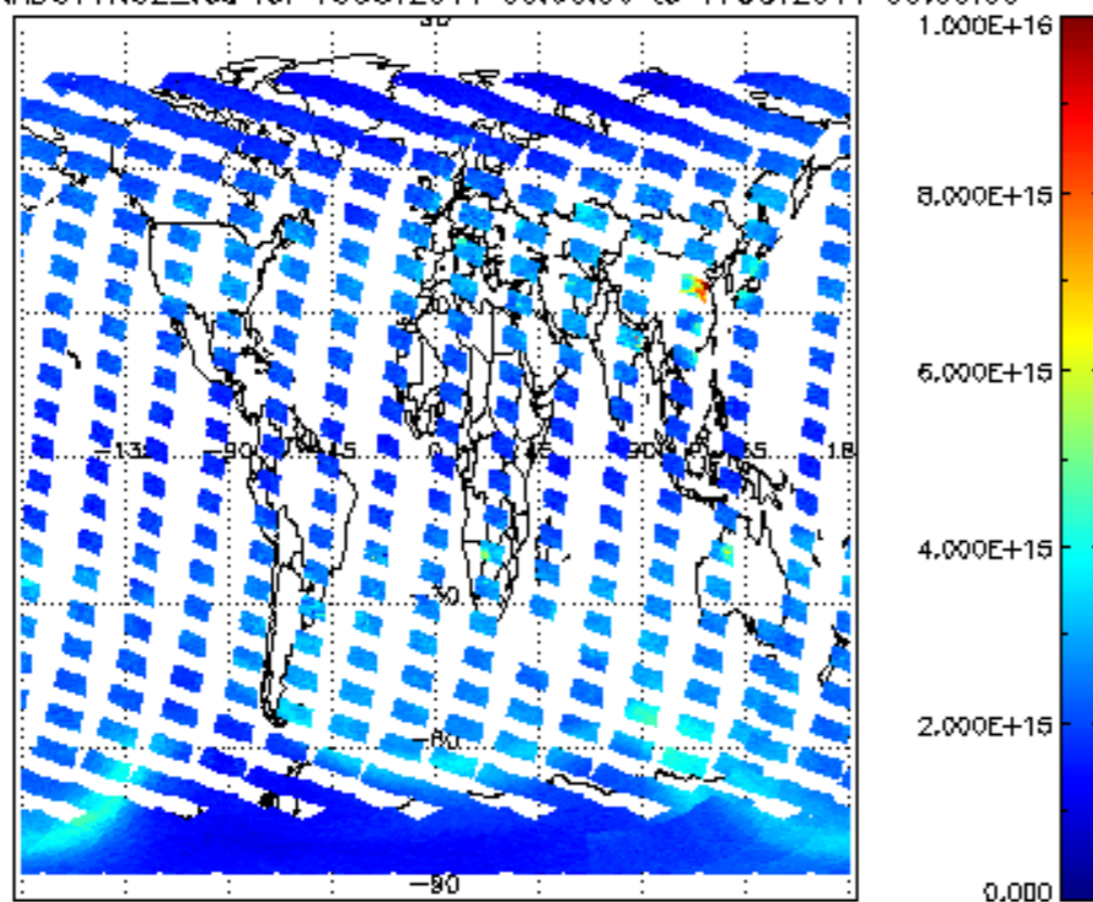
SCIOL2P_NADUV1NO2_vcd for 16OCT2011 00:00:00 to 17OCT2011 00:00:00
