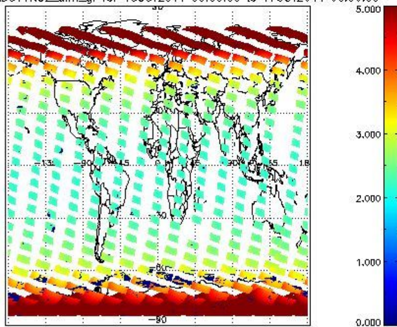
SCIOL2P_NADUV1NO2_amf_gr for 16OCT2011 00:00:00 to 17OCT2011 00:00:00
