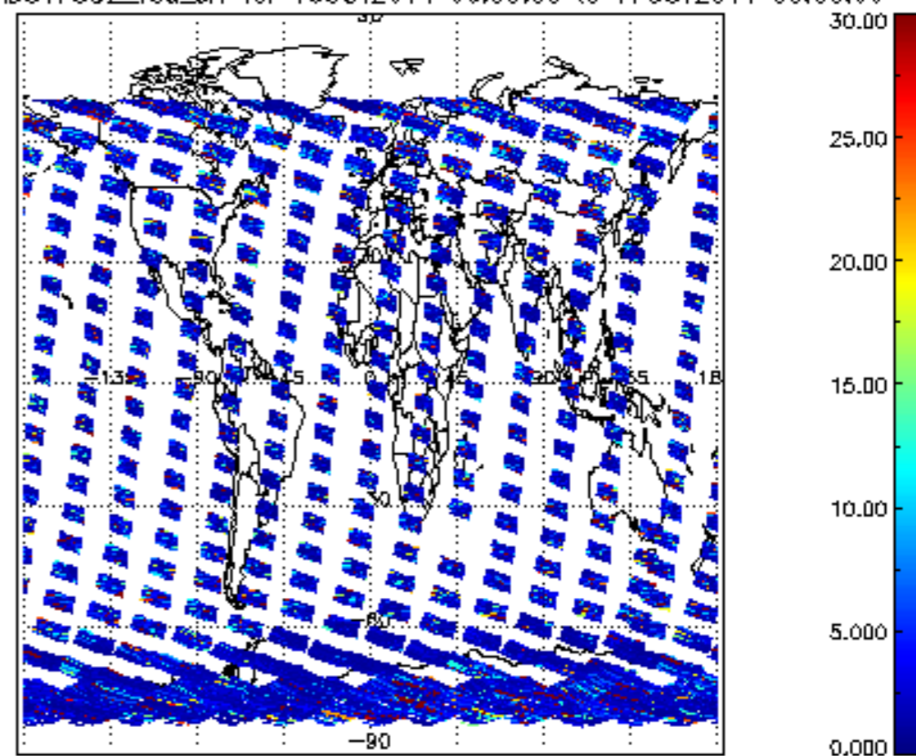
SCIOL2P_NADUV7S02_vcd_err for 16OCT2011 00:00:00 to 17OCT2011 00:00:00
