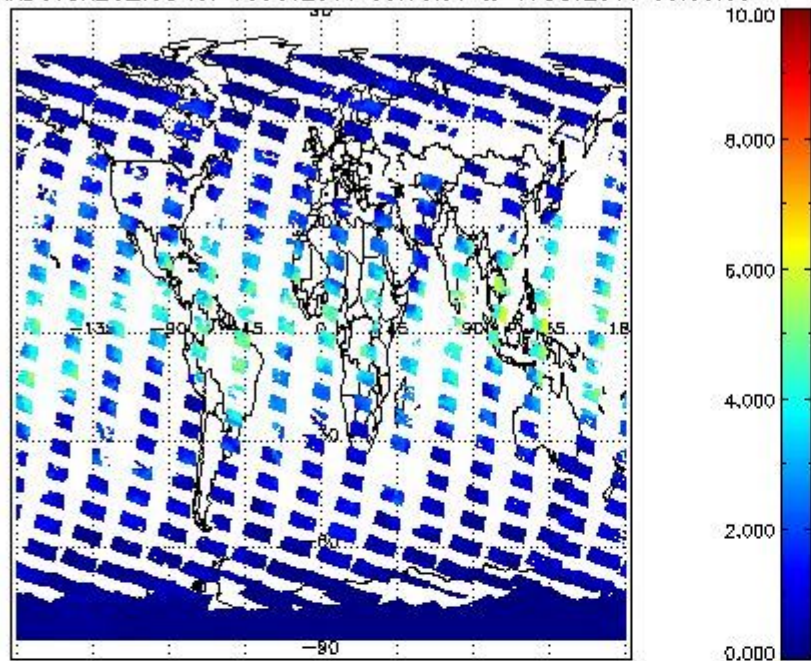
SCIOL2P_NADUV8H20_vcd for 16OCT2011 00:00:00 to 17OCT2011 00:00:00
