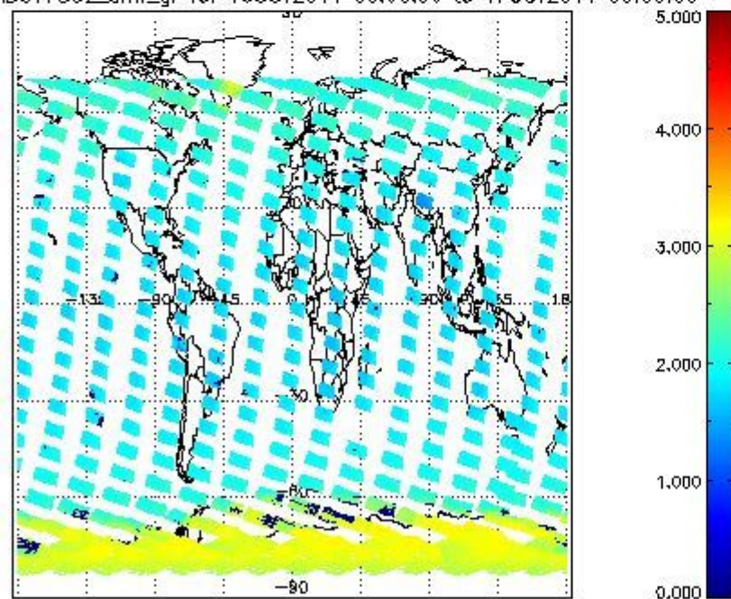
SCIOL2P_NADUV7S02_amf_gr for 16OCT2011 00:00:00 to 17OCT2011 00:00:00
