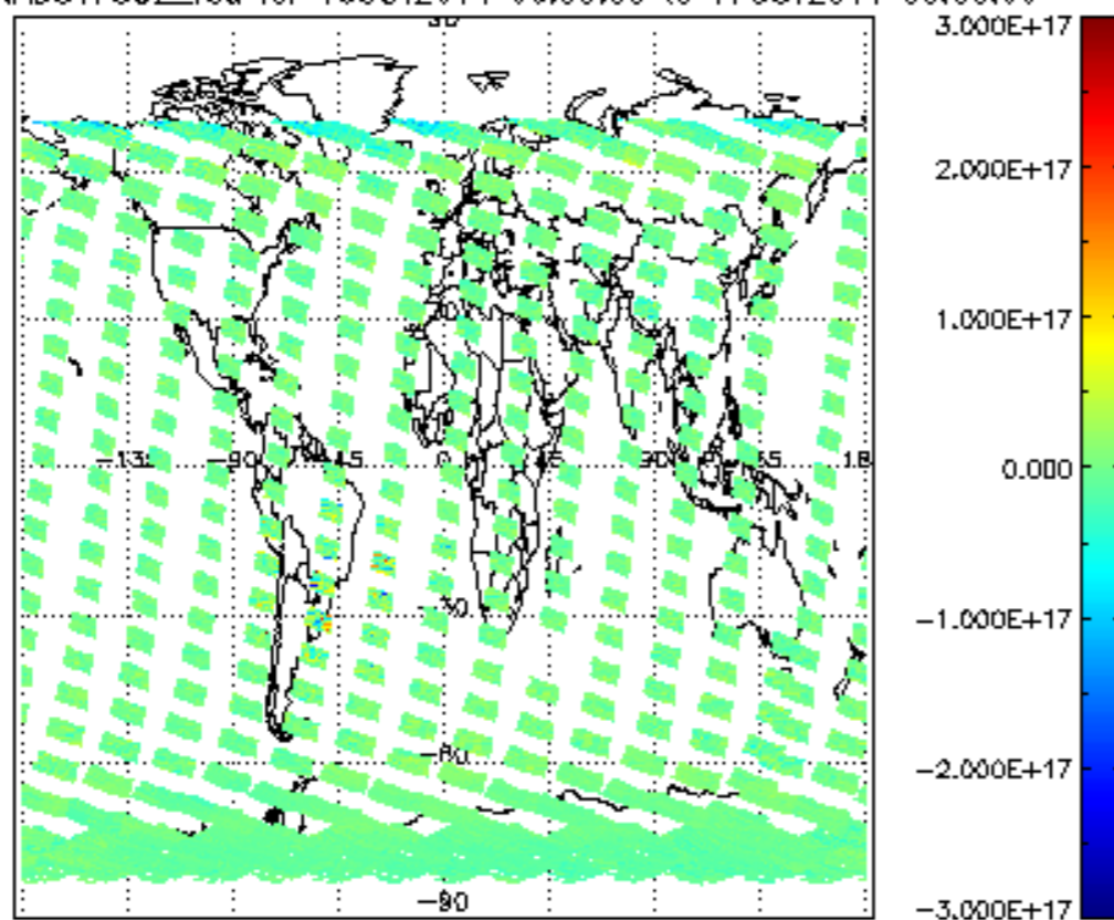
SCIOL2P_NADUV7S02_vcd for 16OCT2011 00:00:00 to 17OCT2011 00:00:00
