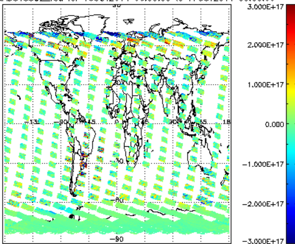
SCIOL2P_NADUV5S02_vcd for 16OCT2011 00:00:00 to 17OCT2011 00:00:00
