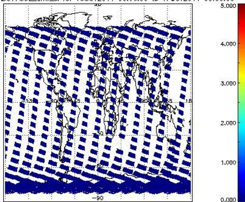
SCIOL2P_NADUV7S02_amf_cl for 16OCT2011 00:00:00 to 17OCT2011 00:00:00
