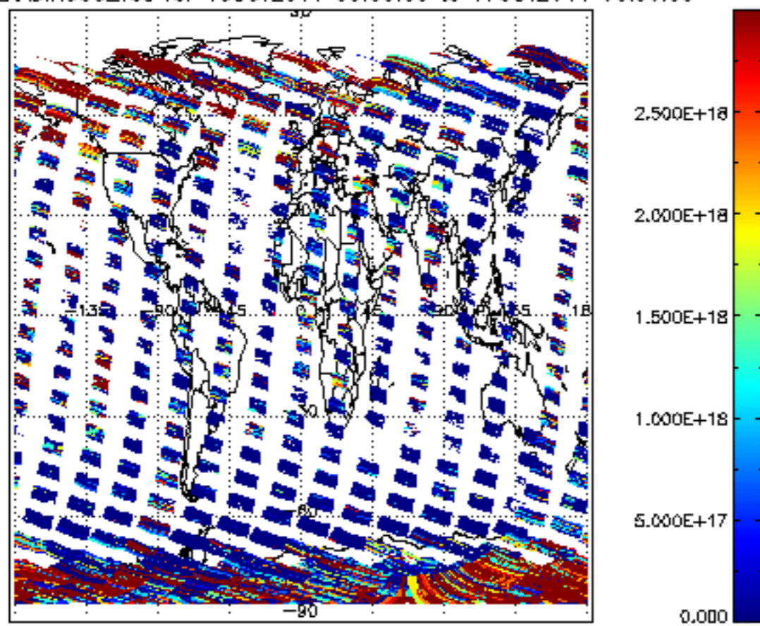
SCIOL2P_NADIR3CO_vcd for 16OCT2011 00:00:00 to 17OCT2011 00:00:00
