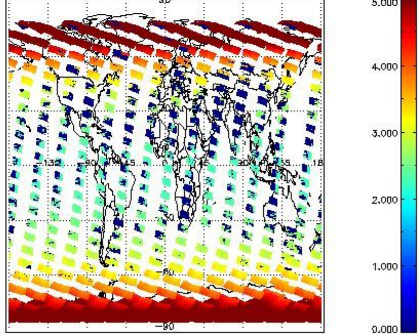
SCIOL2P_NADUV3BRO_amf_cl for 16OCT2011 00:00:00 to 17OCT2011 00:00:00
