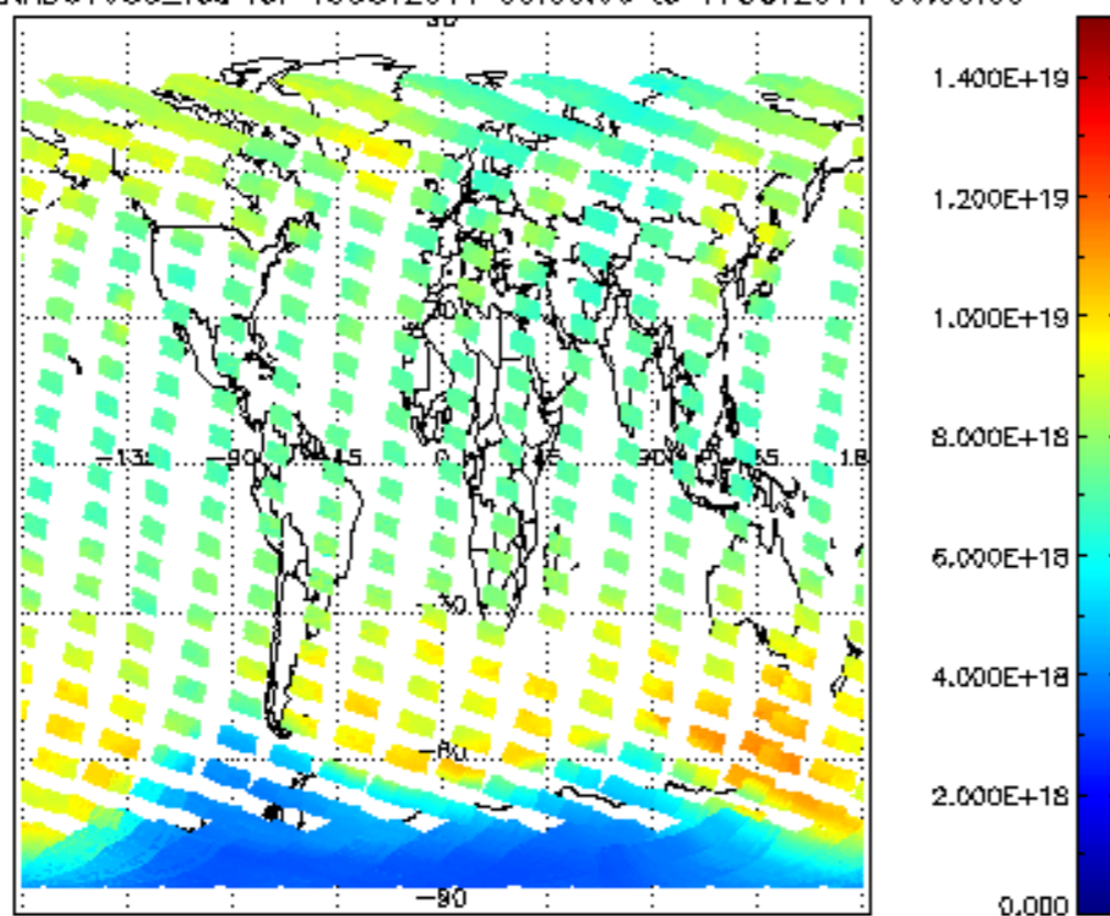
SCIOL2P_NADUV003_vcd for 16OCT2011 00:00:00 to 17OCT2011 00:00:00
