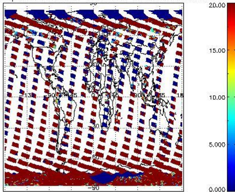
cL_opt_depth for 16OCT2011 00:00:00 to 17OCT2011 00:00:00
