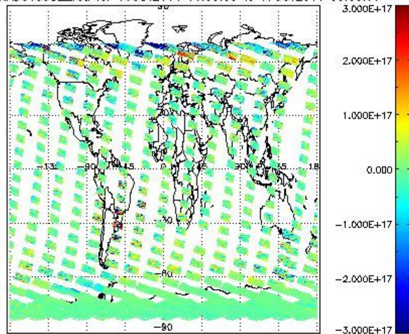
SCIOL2P_NADUV5S02_vcd for 16OCT2011 00:00:00 to 17OCT2011 00:00:00
