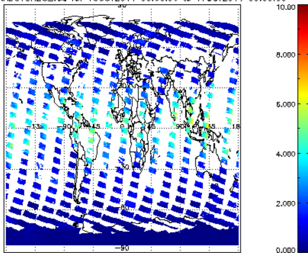
SCIOL2P_NADUV8H20_vcd for 16OCT2011 00:00:00 to 17OCT2011 00:00:00
