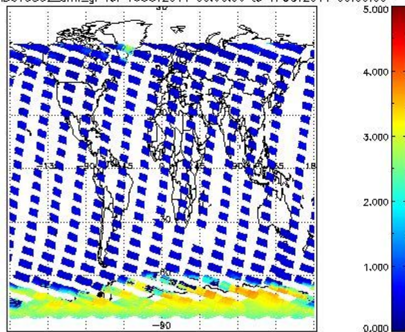
SCIOL2P_NADUV5S02_amf_gr for 16OCT2011 00:00:00 to 17OCT2011 00:00:00
