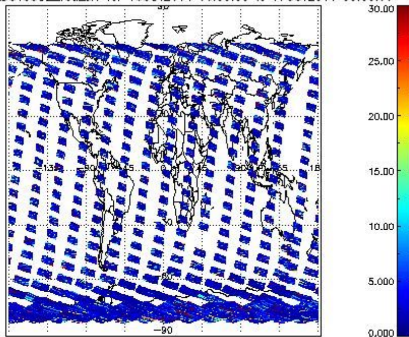
SCIOL2P_NADUV5S02_vcd_err for 16OCT2011 00:00:00 to 17OCT2011 00:00:00
