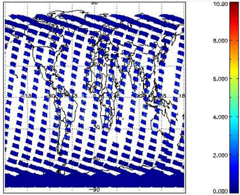
SCIOL2P_NADUV3BRO_vcd_err for 16OCT2011 00:00:00 to 17OCT2011 00:00:00
