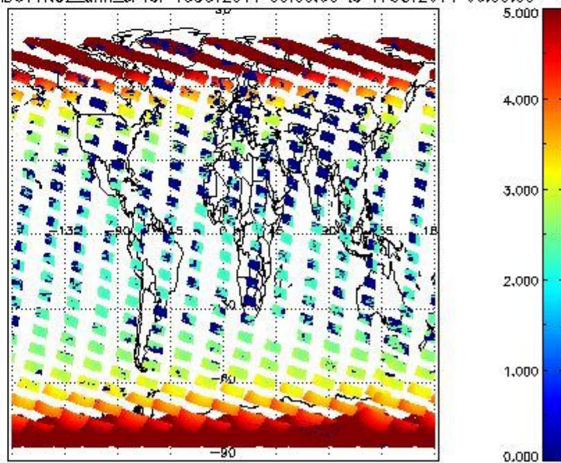
SCIOL2P_NADUV1NO2_amf_cl for 16OCT2011 00:00:00 to 17OCT2011 00:00:00
