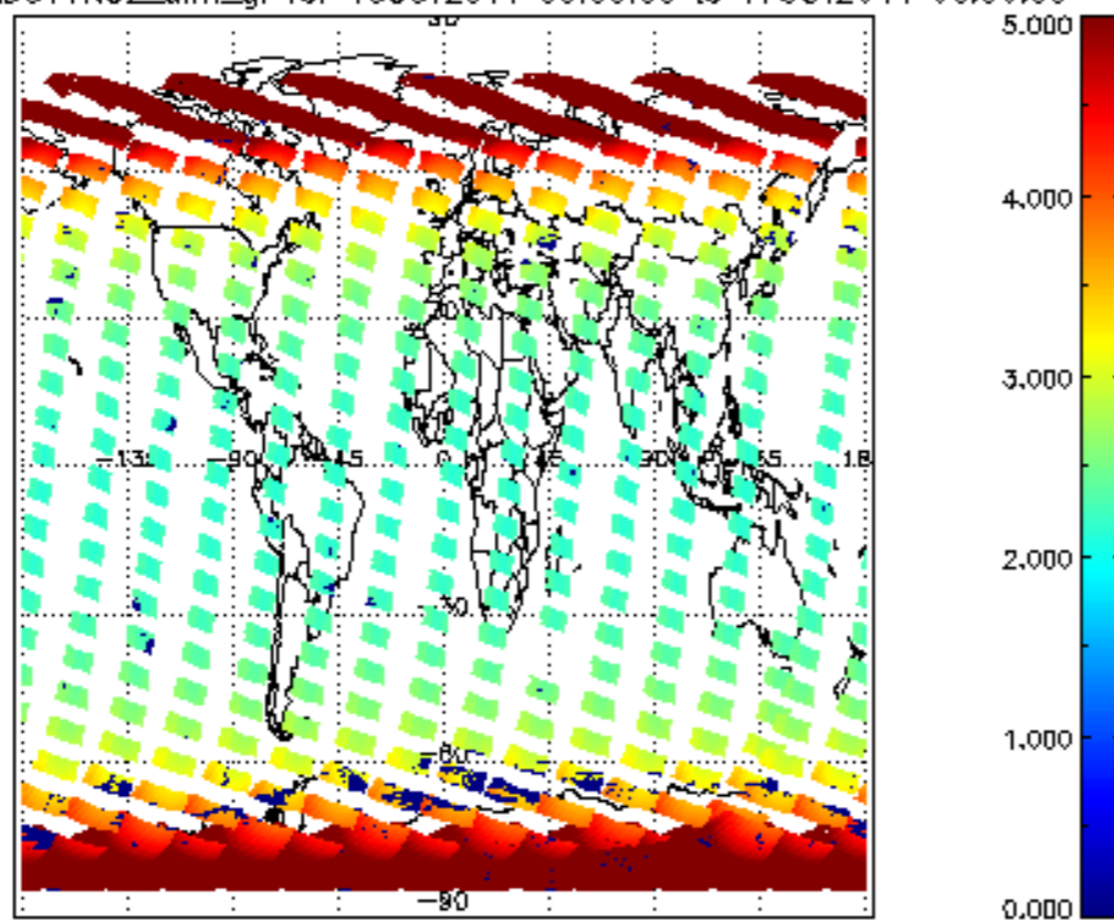
SCIOL2P_NADUV1NO2_amf_gr for 16OCT2011 00:00:00 to 17OCT2011 00:00:00
