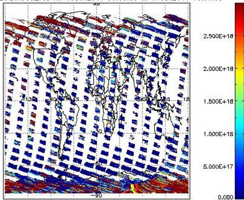
SCIDL2P_NADIR3CO_vcd for 16OCT2011 00:00:00 to 17OCT2011 00:00:00
