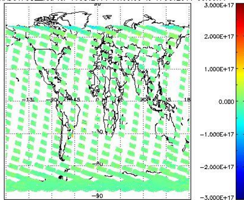
SCIOL2P_NADUV7S02_vcd for 16OCT2011 00:00:00 to 17OCT2011 00:00:00
