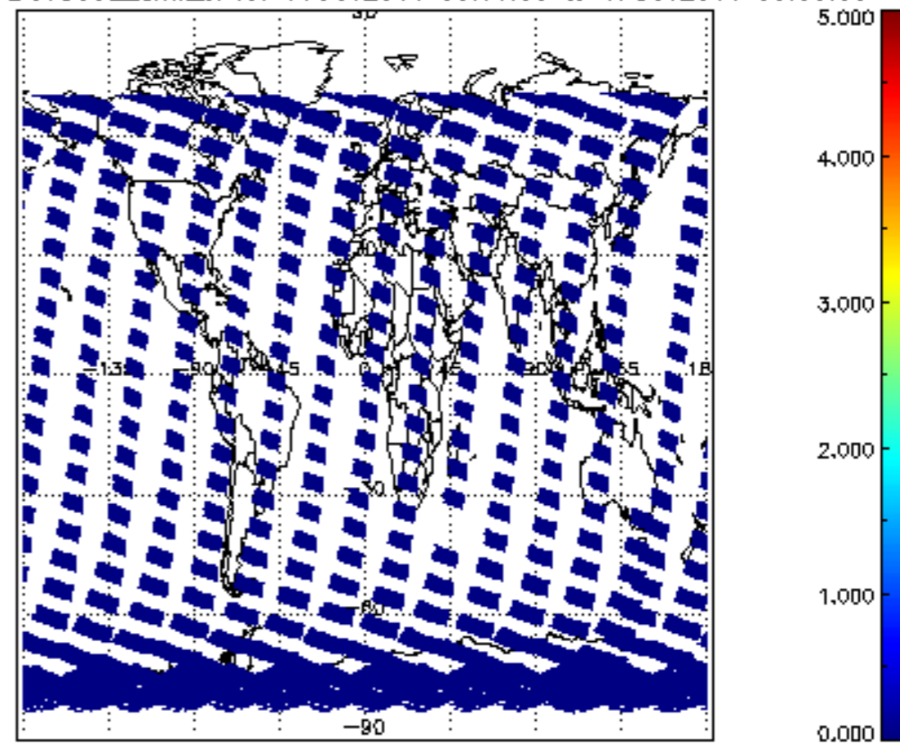
SCIOL2P_NADUV5S02_amf_cl for 16OCT2011 00:00:00 to 17OCT2011 00:00:00
