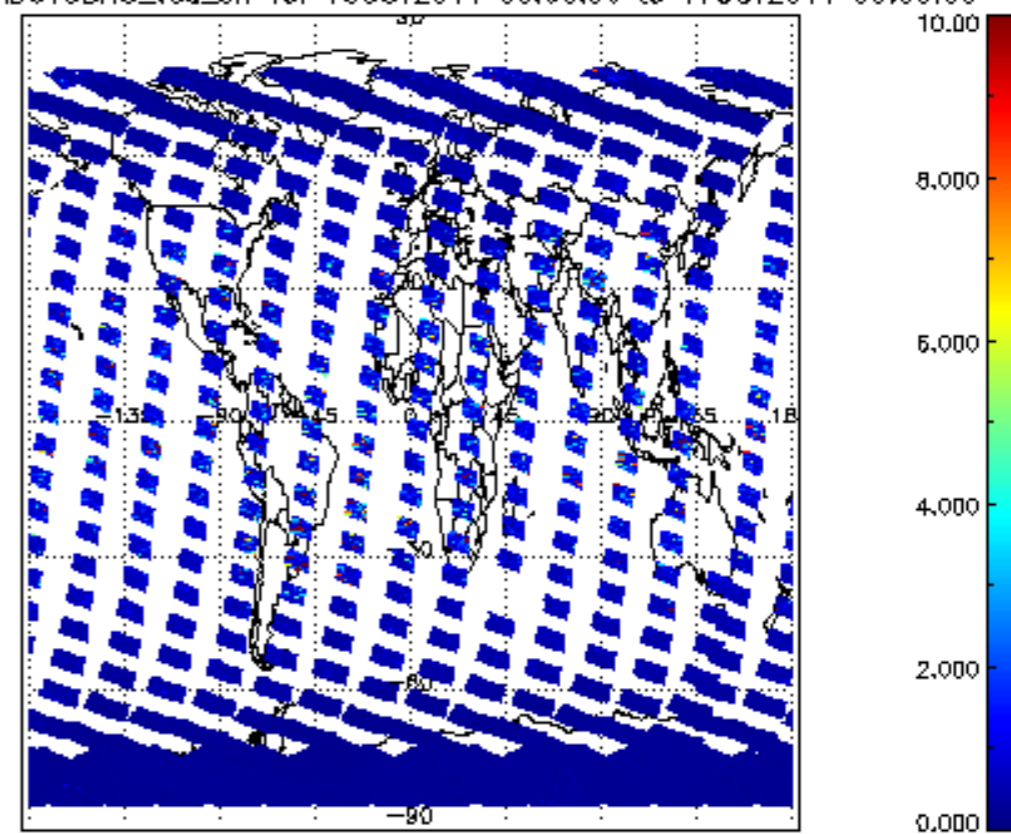
SCIOL2P_NADUV3BRO_vcd_err for 16OCT2011 00:00:00 to 17OCT2011 00:00:00
