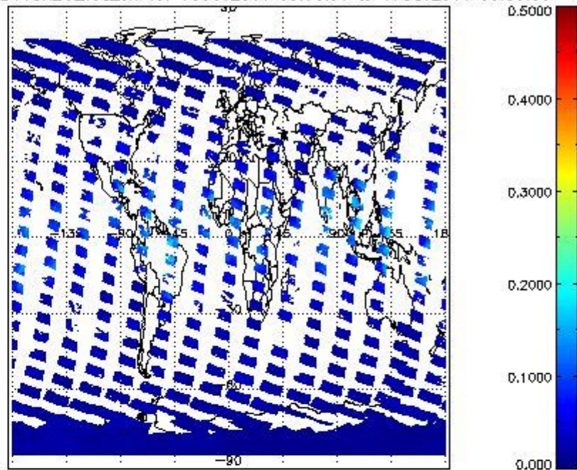
SCIOL2P_NADUV8H20_vcd_err for 16OCT2011 00:00:00 to 17OCT2011 00:00:00
