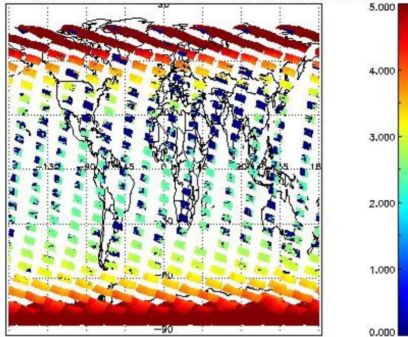
SCIOL2P_NADUV003_amf_cl for 16OCT2011 00:00:00 to 17OCT2011 00:00:00
