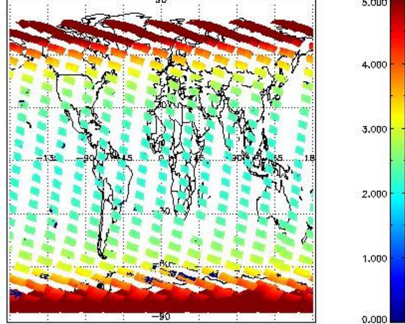
SCIOL2P_NADUV3BRO_amf_gr for 16OCT2011 00:00:00 to 17OCT2011 00:00:00
