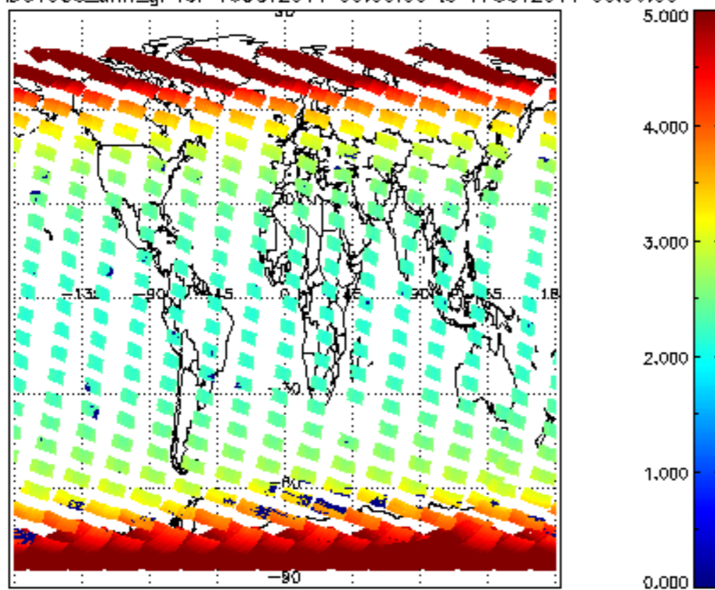
SCIOL2P_NADUV003_amf_gr for 16OCT2011 00:00:00 to 17OCT2011 00:00:00
