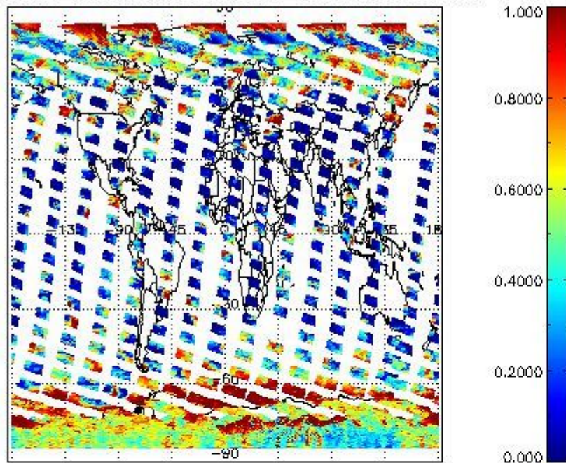
cLfrac for 16OCT2011 00:00:00 to 17OCT2011 00:00:00
