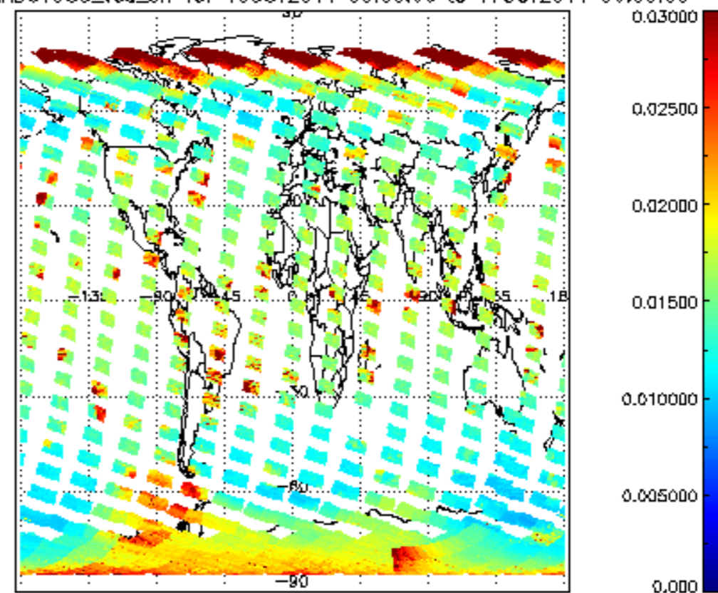
SCIOL2P_NADUV003_vcd_err for 16OCT2011 00:00:00 to 17OCT2011 00:00:00
