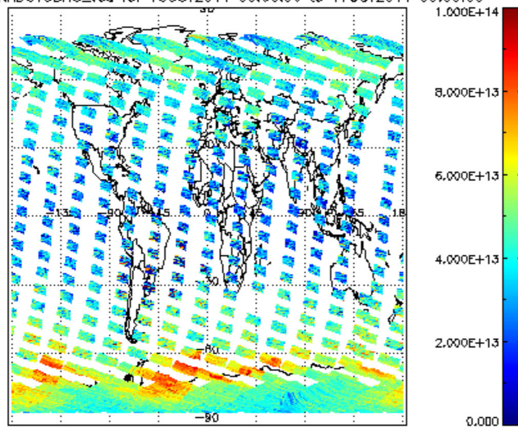
SCIOL2P_NADUV3BRO_vcd for 16OCT2011 00:00:00 to 17OCT2011 00:00:00
