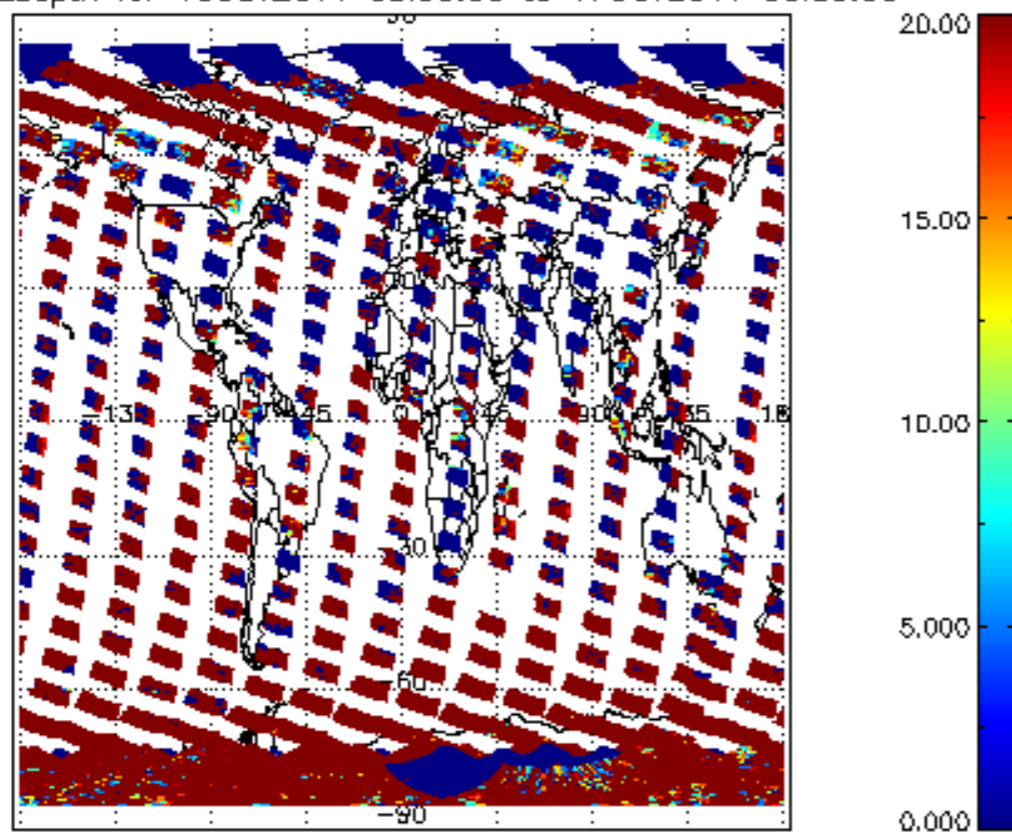
cl_opt_depth for 16OCT2011 00:00:00 to 17OCT2011 00:00:00
