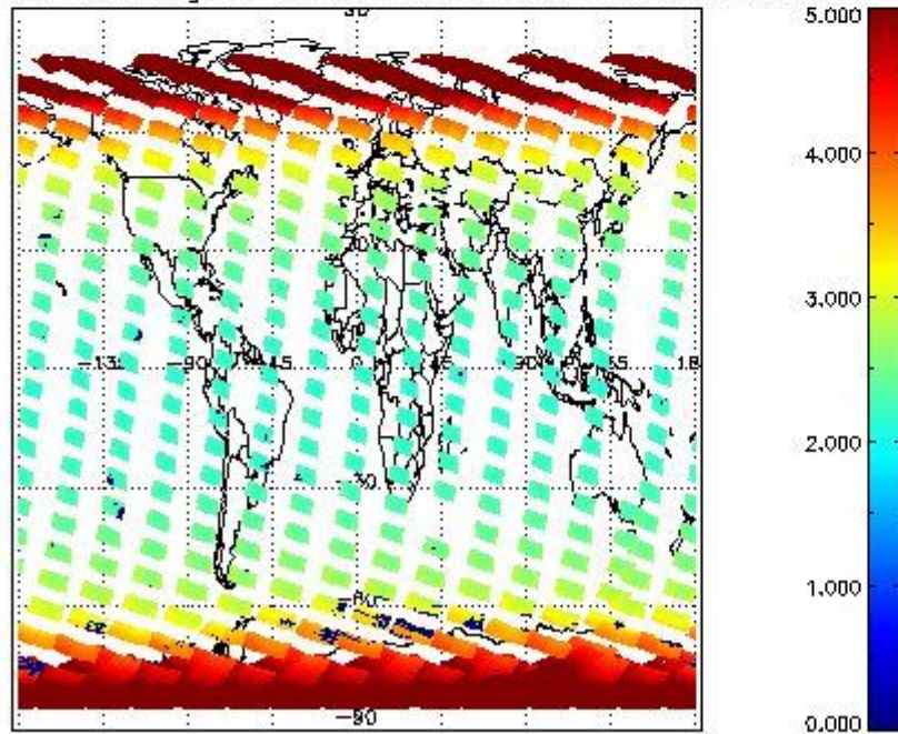
SCIOL2P_NADUV003_amf_gr for 16OCT2011 00:00:00 to 17OCT2011 00:00:00
