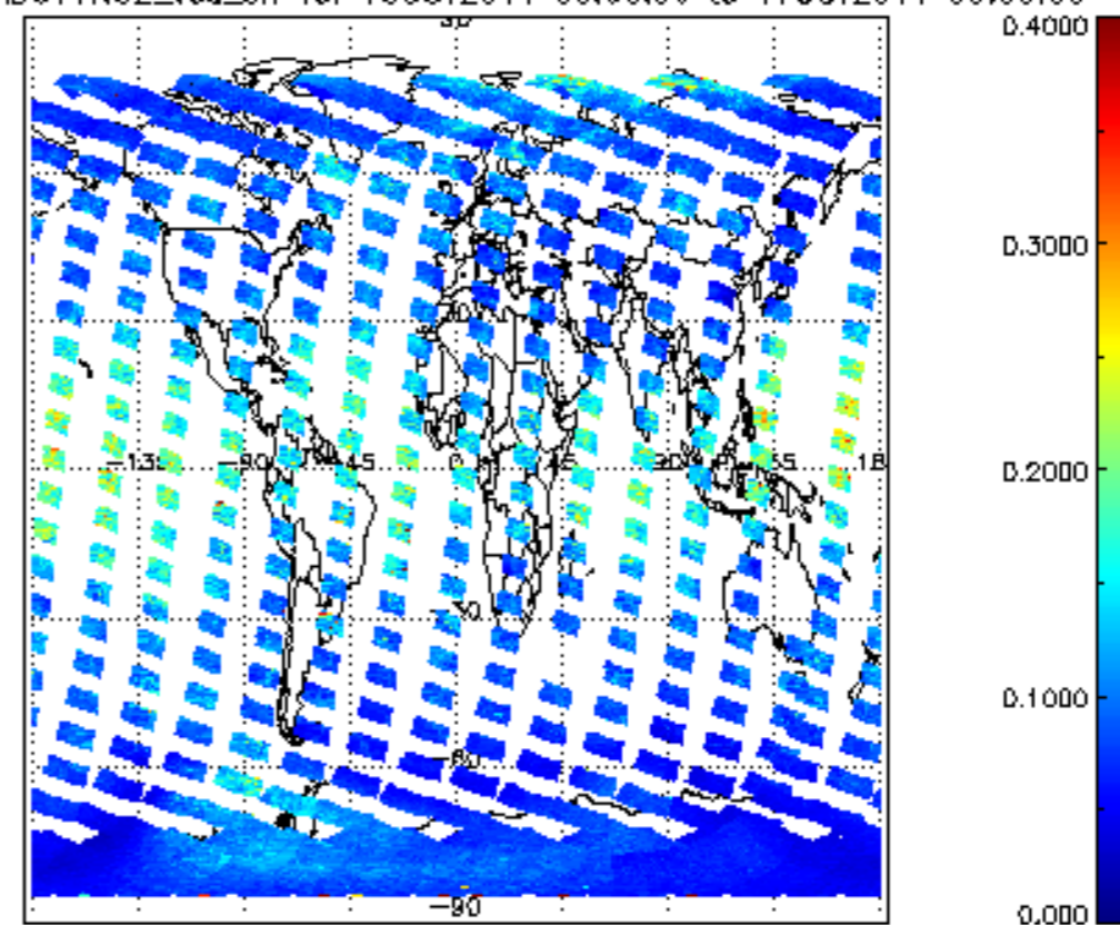
SCIOL2P_NADUV1NO2_vcd_err for 16OCT2011 00:00:00 to 17OCT2011 00:00:00
