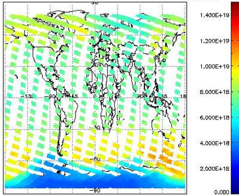
SCIOL2P_NADUV003_vcd for 16OCT2011 00:00:00 to 17OCT2011 00:00:00
