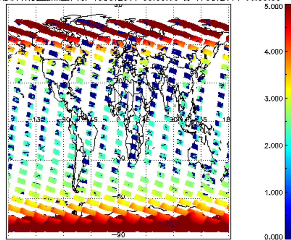
SCIOL2P_NADUV1NO2_amf_cl for 16OCT2011 00:00:00 to 17OCT2011 00:00:00
