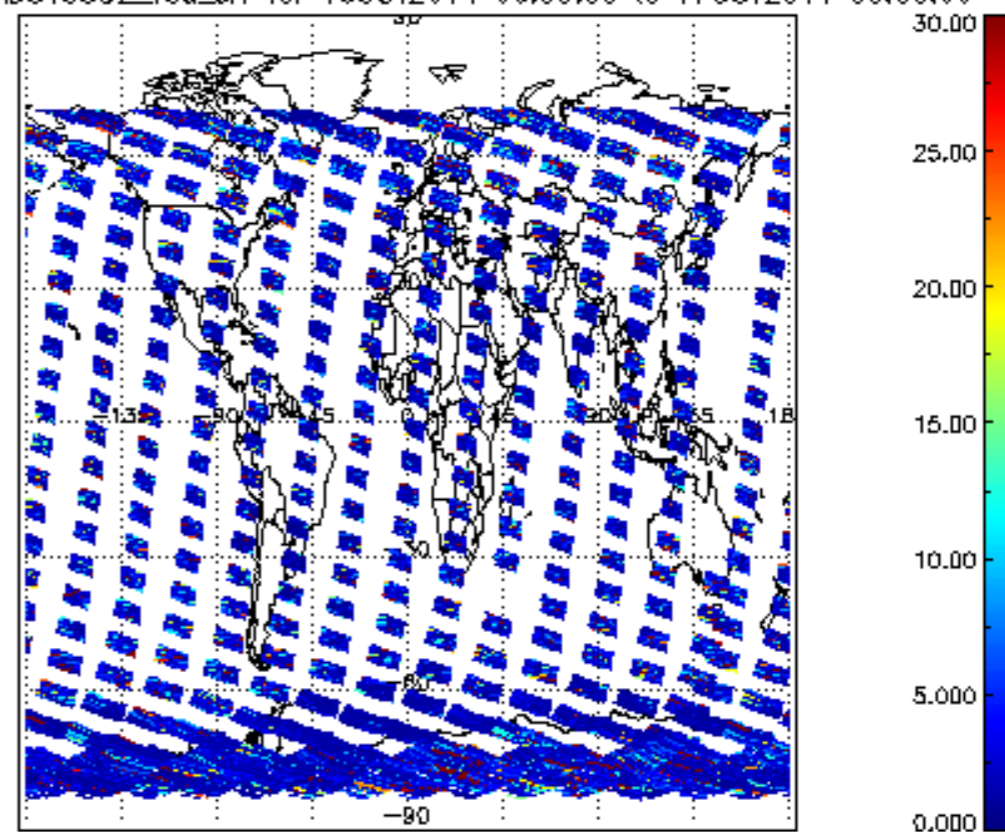
SCIOL2P_NADUV5S02_vcd_err for 16OCT2011 00:00:00 to 17OCT2011 00:00:00
