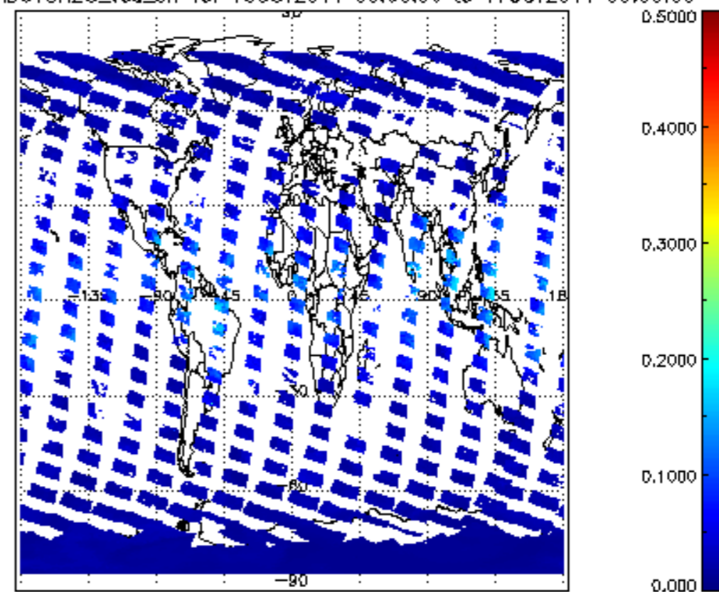
SCIOL2P_NADUV8H20_vcd_err for 16OCT2011 00:00:00 to 17OCT2011 00:00:00
