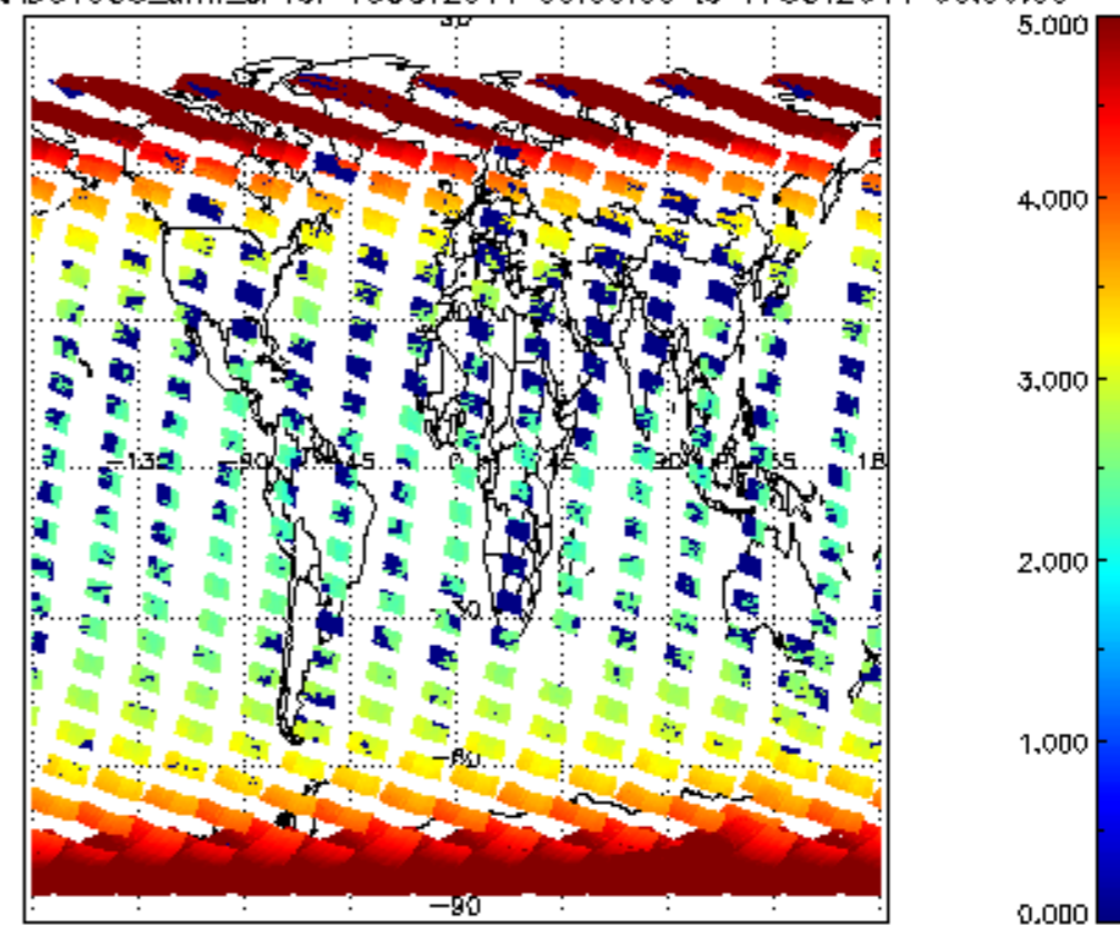
SCIOL2P_NADUV003_amf_cl for 16OCT2011 00:00:00 to 17OCT2011 00:00:00
