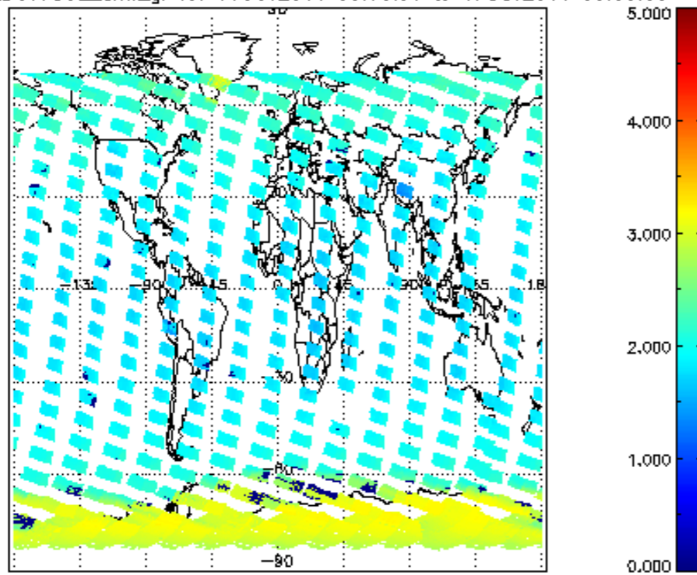
SCIOL2P_NADUV7S02_amf_gr for 16OCT2011 00:00:00 to 17OCT2011 00:00:00
