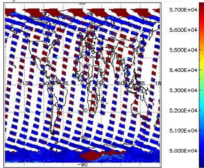
cloud_flags for 16OCT2011 00:00:00 to 17OCT2011 00:00:00
