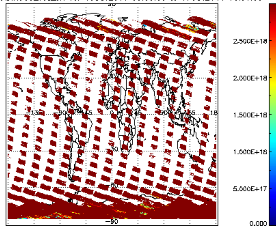
SCIOL2P_NADIR3CO_vcd_err for 16OCT2011 00:00:00 to 17OCT2011 00:00:00
