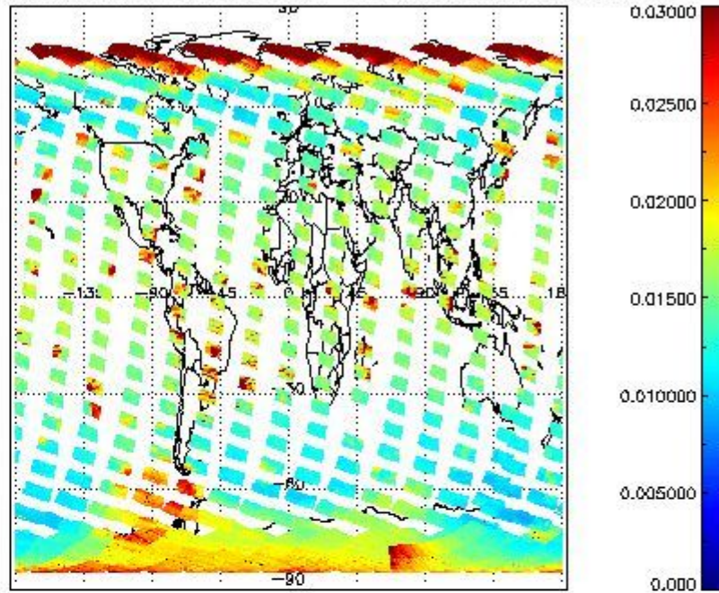
SCIOL2P_NADUV003_vcd_err for 16OCT2011 00:00:00 to 17OCT2011 00:00:00
