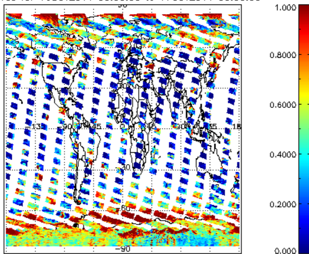
cl_frac for 16OCT2011 00:00:00 to 17OCT2011 00:00:00
