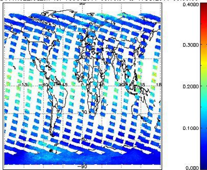
SCIOL2P_NADUV1NO2_vcd_err for 16OCT2011 00:00:00 to 17OCT2011 00:00:00
