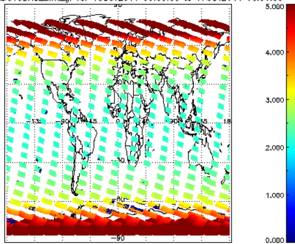
SCIOL2P_NADUV3BRO_amf_gr for 16OCT2011 00:00:00 to 17OCT2011 00:00:00
