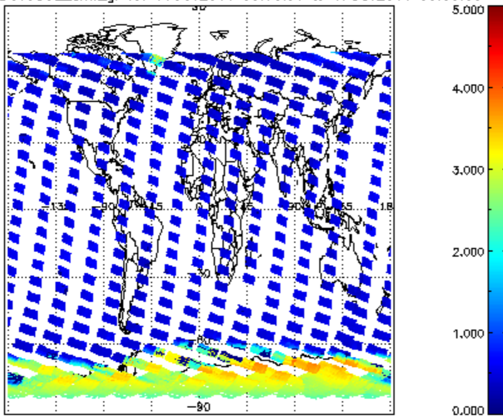
SCIOL2P_NADUV5S02_amf_gr for 16OCT2011 00:00:00 to 17OCT2011 00:00:00
