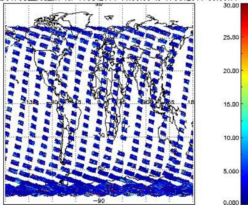
SCIOL2P_NADUV7S02_vcd_err for 16OCT2011 00:00:00 to 17OCT2011 00:00:00
