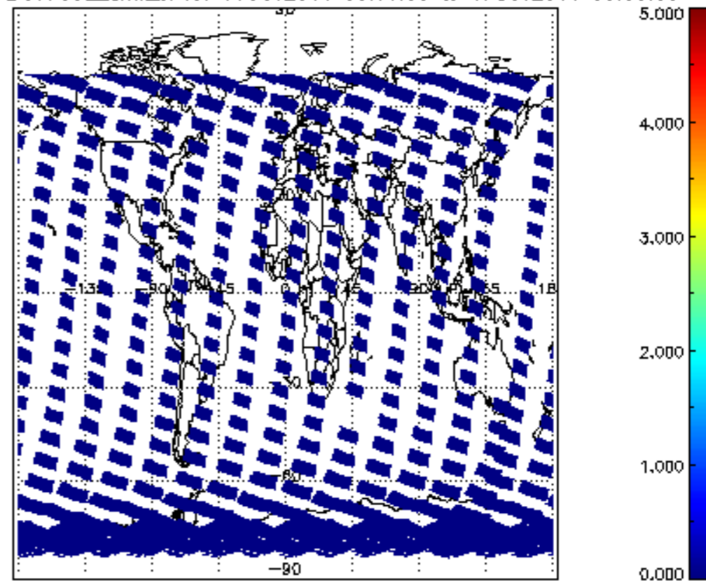
SCIOL2P_NADUV7S02_amf_cl for 16OCT2011 00:00:00 to 17OCT2011 00:00:00
