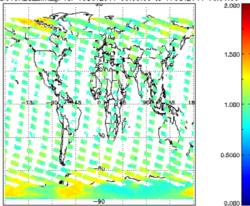
SCIOL2P_NADUV8H20_amf_gr for 16OCT2011 00:00:00 to 17OCT2011 00:00:00
