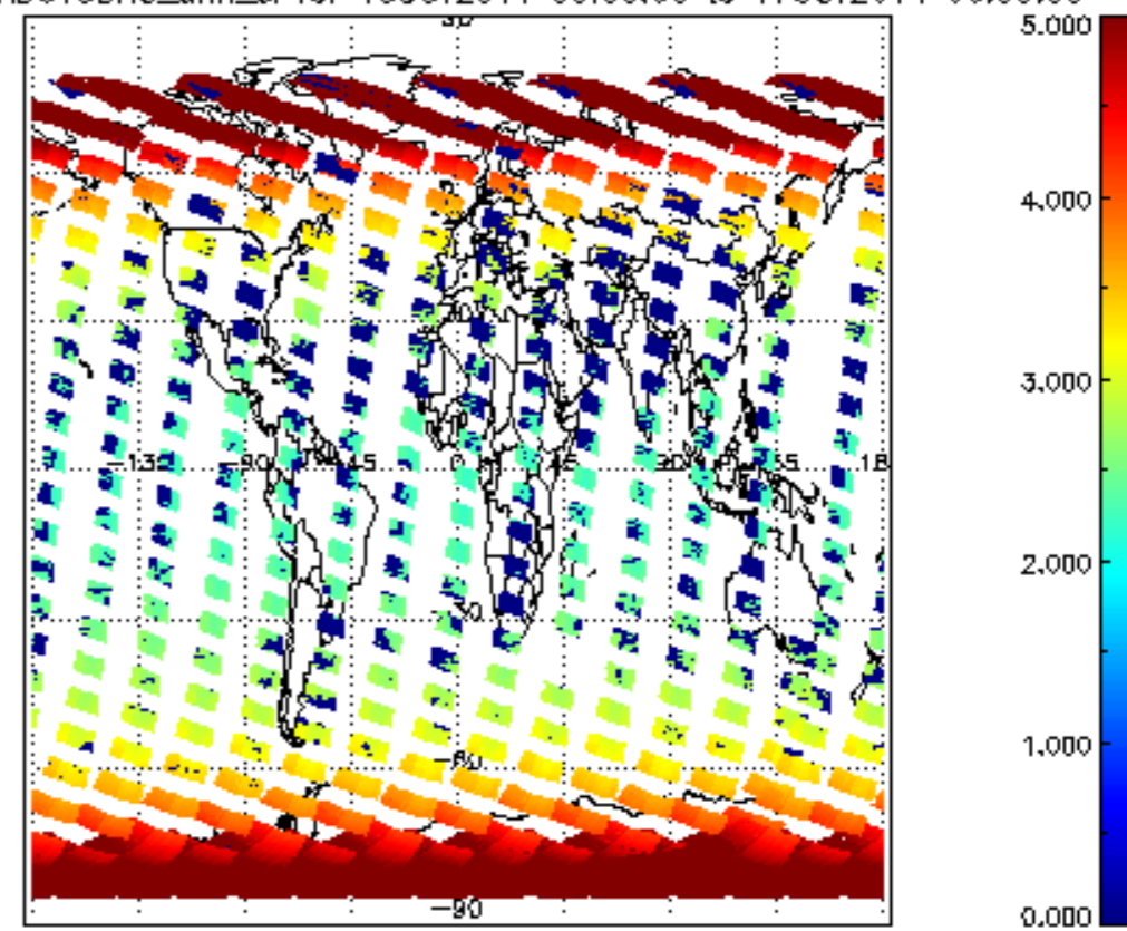
SCIOL2P_NADUV3BRO_amf_cl for 16OCT2011 00:00:00 to 17OCT2011 00:00:00
