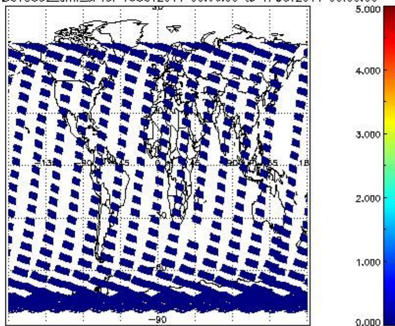
SCIOL2P_NADUV5S02_amf_cl for 16OCT2011 00:00:00 to 17OCT2011 00:00:00
