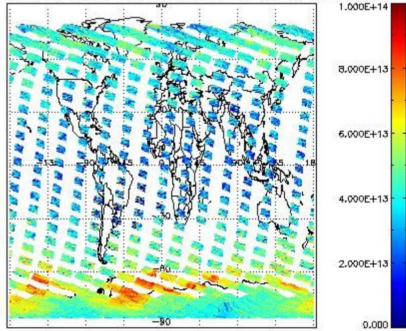
SCIOL2P_NADUV3BRO_vcd for 16OCT2011 00:00:00 to 17OCT2011 00:00:00
