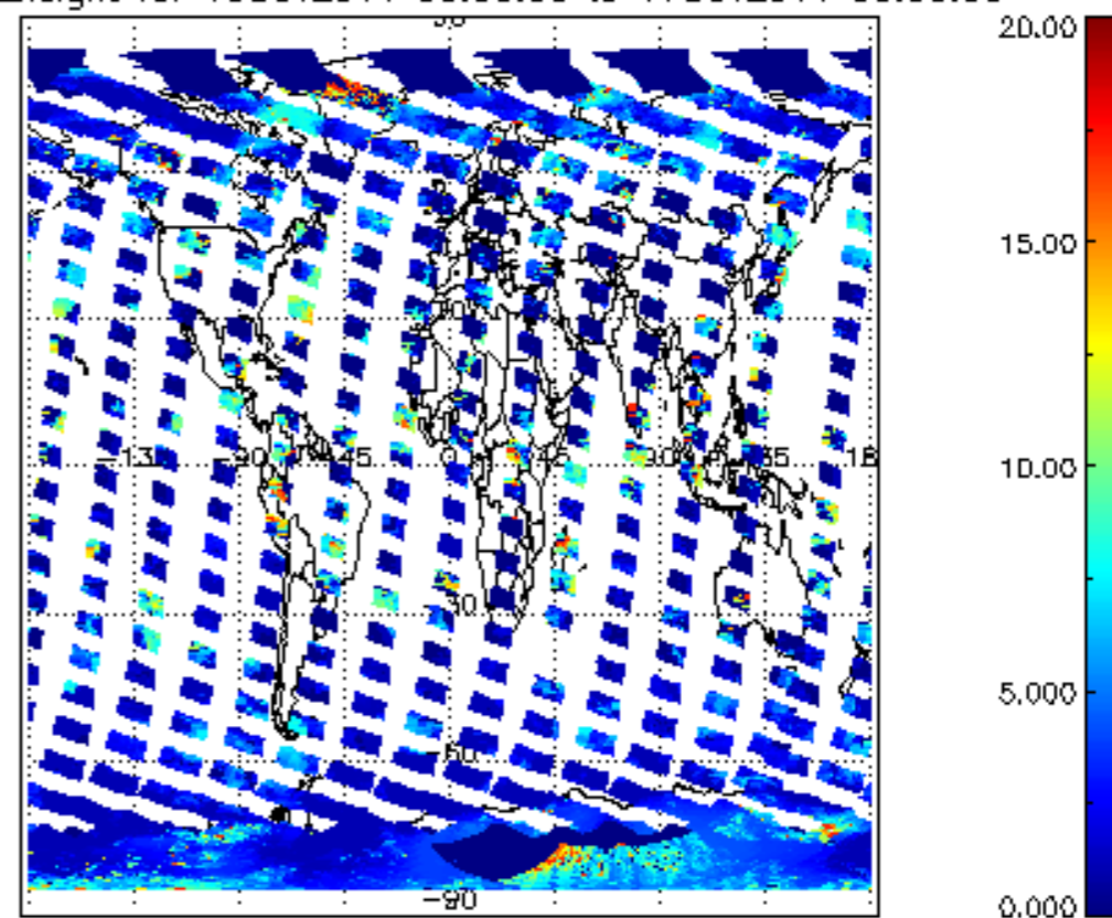
cl_top_height for 16OCT2011 00:00:00 to 17OCT2011 00:00:00
