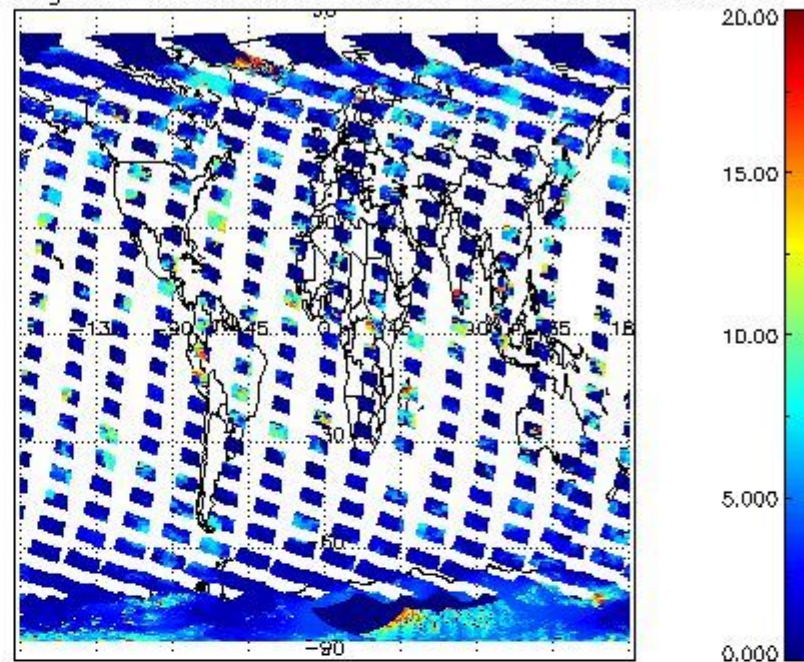
cL_top_height for 16OCT2011 00:00:00 to 17OCT2011 00:00:00
