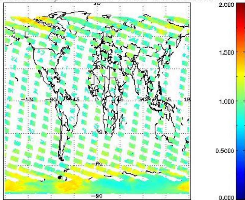
SCIOL2P_NADUV8H20_amf_gr for 16OCT2011 00:00:00 to 17OCT2011 00:00:00
