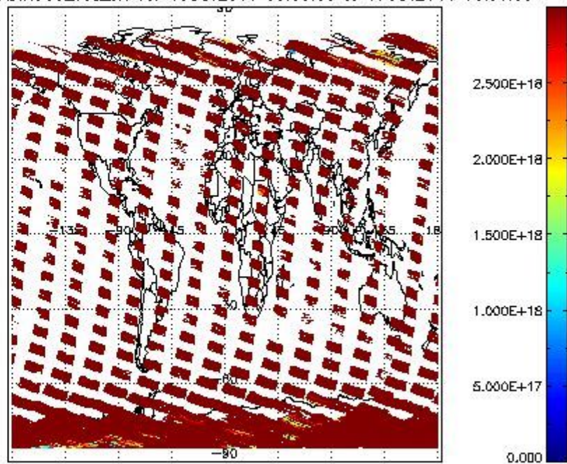
SCIDL2P_NADIR3CO_vcd_err for 16OCT2011 00:00:00 to 17OCT2011 00:00:00
