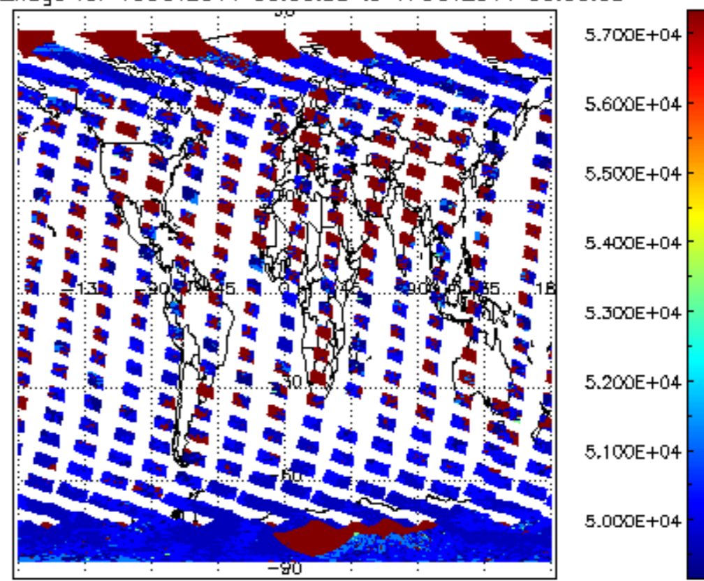
cloud_flags for 16OCT2011 00:00:00 to 17OCT2011 00:00:00
