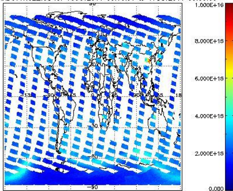
SCIOL2P_NADUV1NO2_vcd for 16OCT2011 00:00:00 to 17OCT2011 00:00:00
