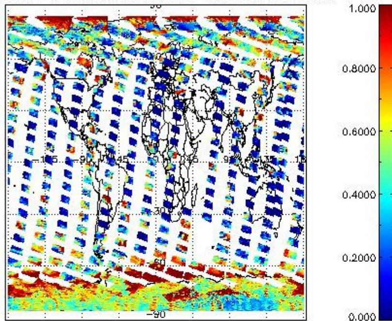
cLfrac for 15OCT2011 00:00:00 to 16OCT2011 00:00:00
