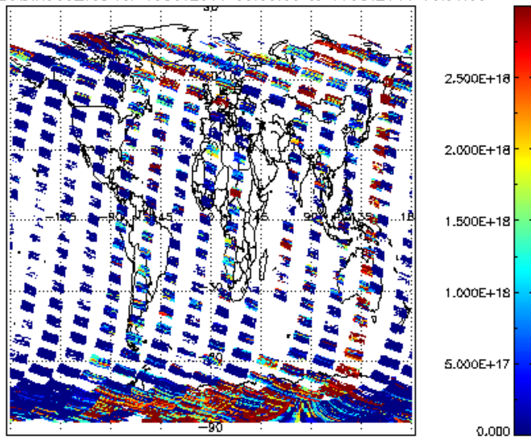
SCIOL2P_NADIR3CO_vcd for 15OCT2011 00:00:00 to 16OCT2011 00:00:00
