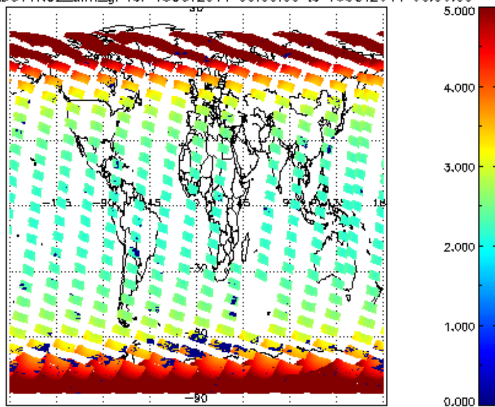
SCIOL2P_NADUV1NO2_amf_gr for 15OCT2011 00:00:00 to 16OCT2011 00:00:00
