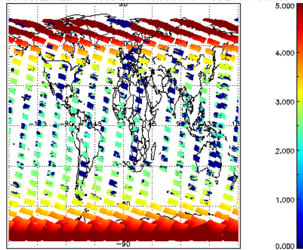
SCIOL2P_NADUV003_amf_cl for 15OCT2011 00:00:00 to 16OCT2011 00:00:00
