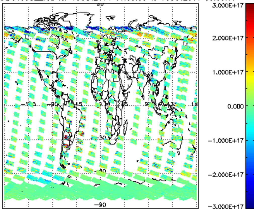
SCIOL2P_NADUV5S02_vcd for 15OCT2011 00:00:00 to 16OCT2011 00:00:00
