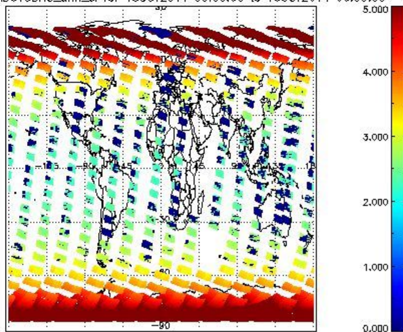
SCIOL2P_NADUV3BRO_amf_cl for 15OCT2011 00:00:00 to 16OCT2011 00:00:00
