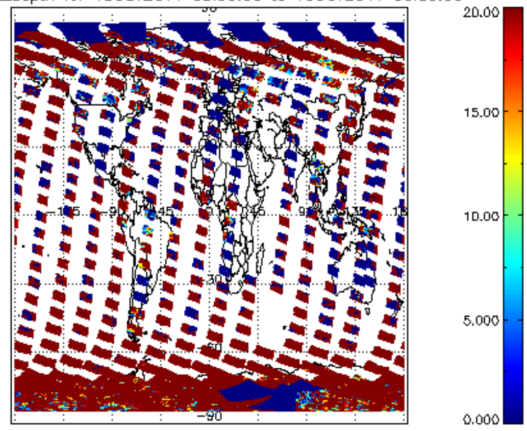
cl_opt_depth for 15OCT2011 00:00:00 to 16OCT2011 00:00:00
