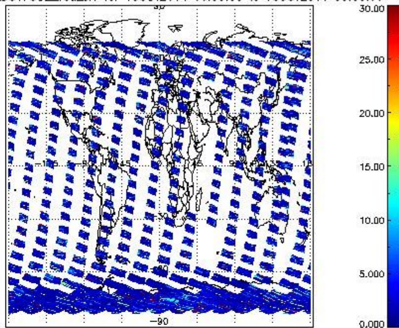
SCIOL2P_NADUV7S02_vcd_err for 15OCT2011 00:00:00 to 16OCT2011 00:00:00
