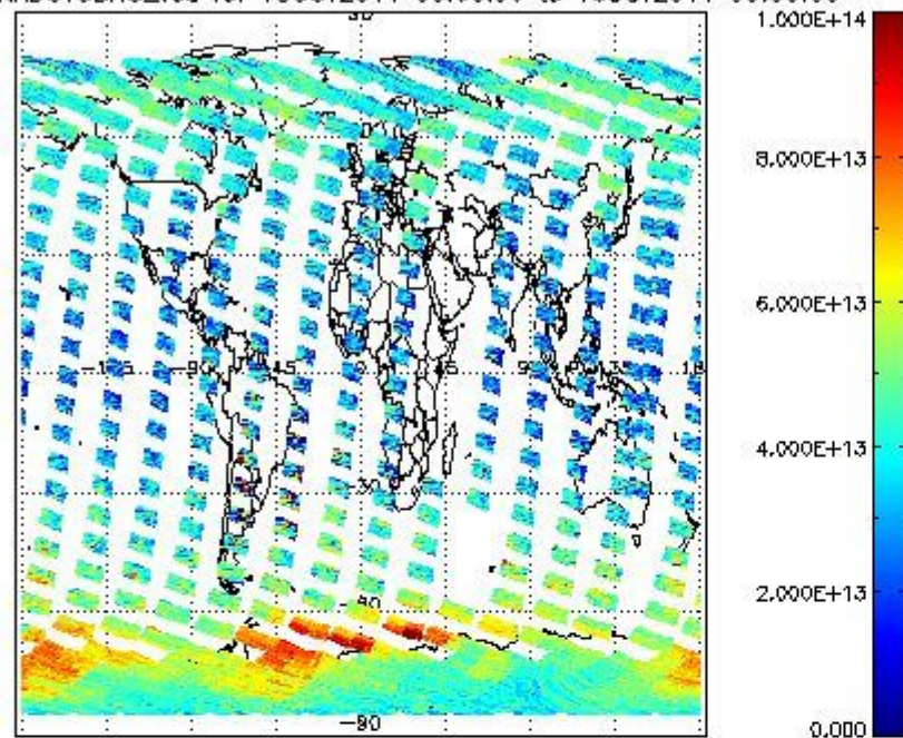
SCIOL2P_NADUV3BRO_vcd for 15OCT2011 00:00:00 to 16OCT2011 00:00:00
