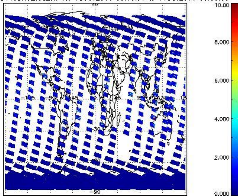
SCIOL2P_NADUV3BRO_vcd_err for 15OCT2011 00:00:00 to 16OCT2011 00:00:00
