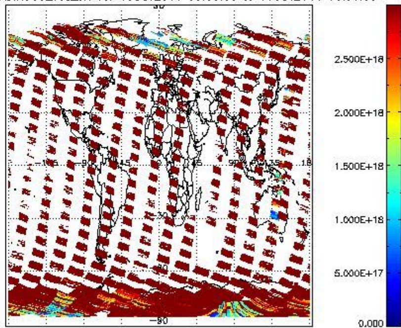
SCIOI2P_NADIR3CO_vcd_err for 15OCT2011 00:00:00 to 16OCT2011 00:00:00
