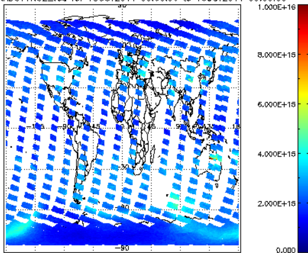
SCIOL2P_NADUV1NO2_vcd for 15OCT2011 00:00:00 to 16OCT2011 00:00:00
