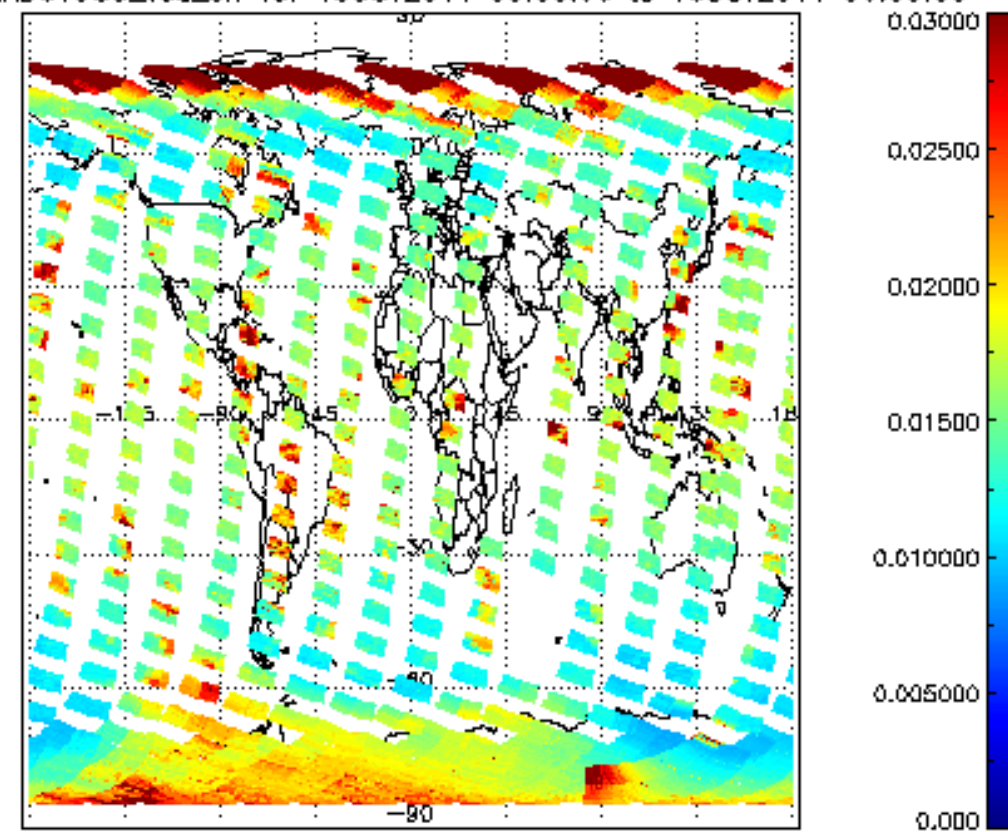
SCIOL2P_NADUV003_vcd_err for 15OCT2011 00:00:00 to 16OCT2011 00:00:00
