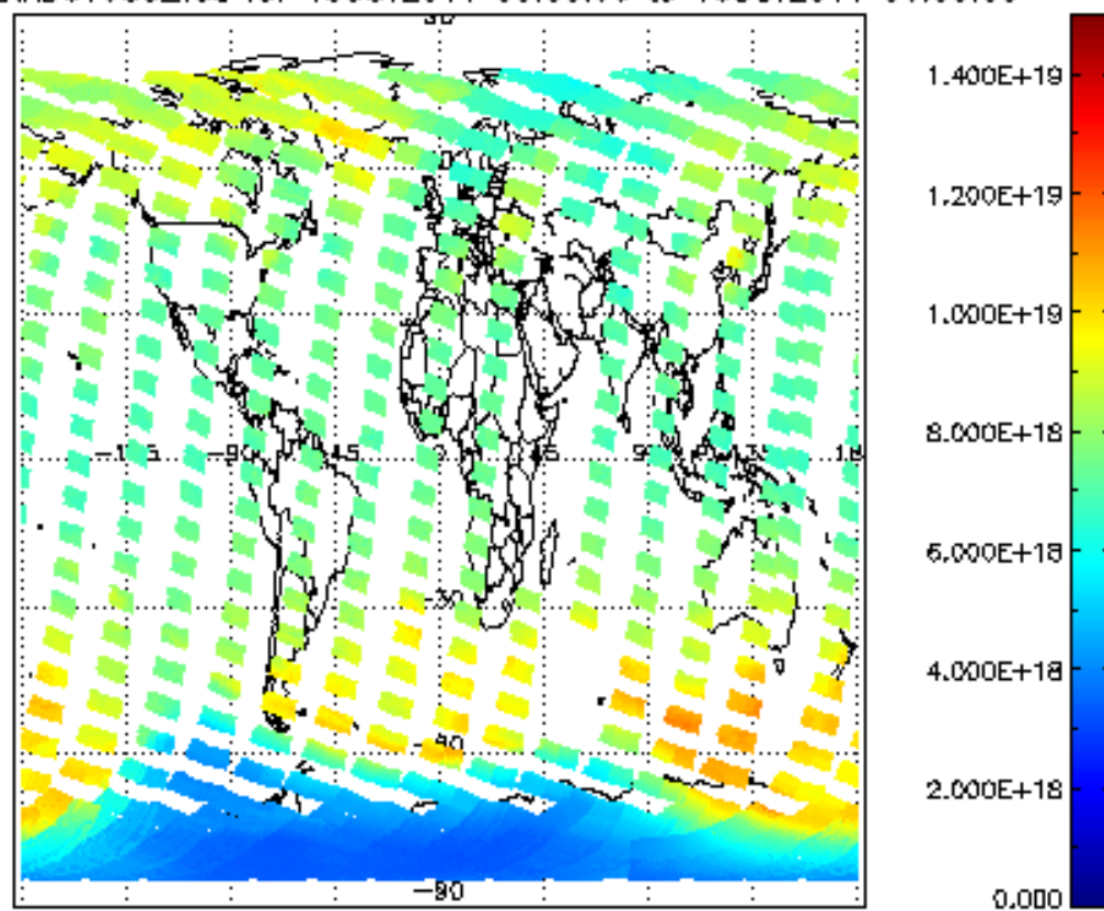
SCIOL2P_NADUV003_vcd for 15OCT2011 00:00:00 to 16OCT2011 00:00:00
