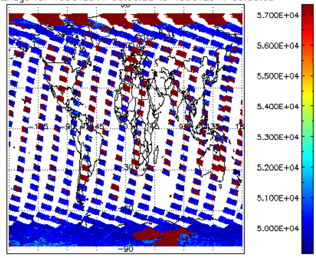
cloud_flags for 15OCT2011 00:00:00 to 16OCT2011 00:00:00
