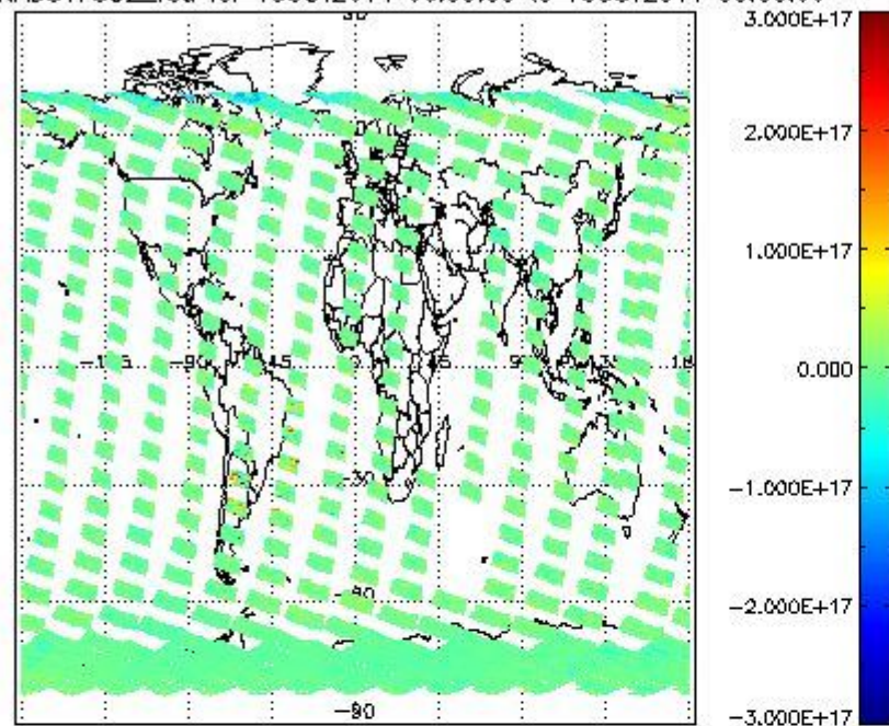
SCIOL2P_NADUV7S02_vcd for 15OCT2011 00:00:00 to 16OCT2011 00:00:00
