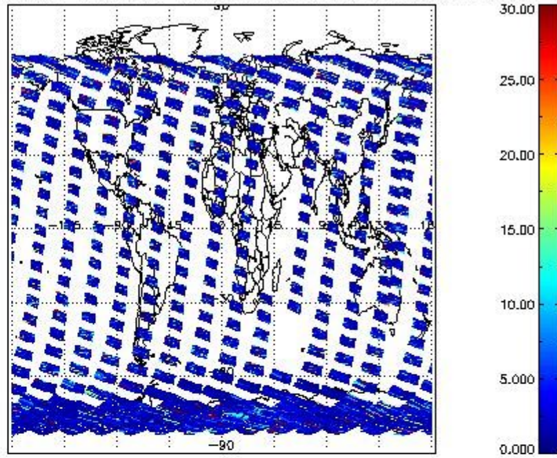
SCIOL2P_NADUV5S02_vcd_err for 15OCT2011 00:00:00 to 16OCT2011 00:00:00
