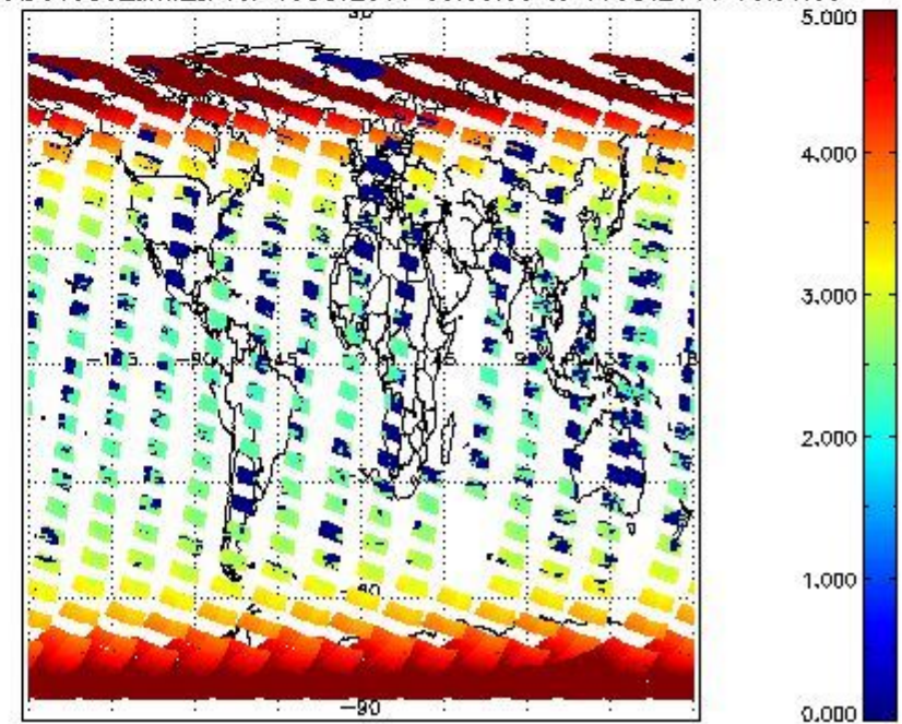
SCIOL2P_NADUV003_amf_cl for 15OCT2011 00:00:00 to 16OCT2011 00:00:00
