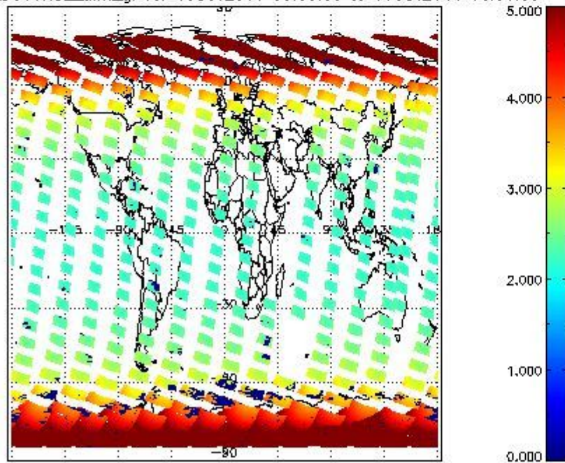
SCIOL2P_NADUV1NO2_amf_gr for 15OCT2011 00:00:00 to 16OCT2011 00:00:00
