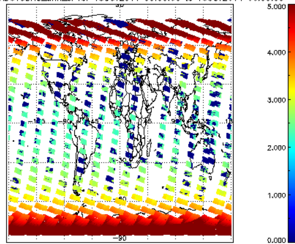
SCIOL2P_NADUV3BRO_amf_cl for 15OCT2011 00:00:00 to 16OCT2011 00:00:00
