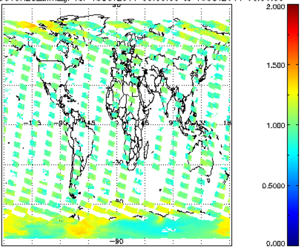
SCIOL2P_NADUV8H20_amf_gr for 15OCT2011 00:00:00 to 16OCT2011 00:00:00
