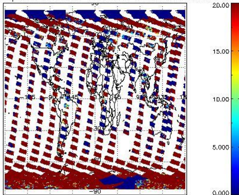
cL_opt_depth for 15OCT2011 00:00:00 to 16OCT2011 00:00:00
