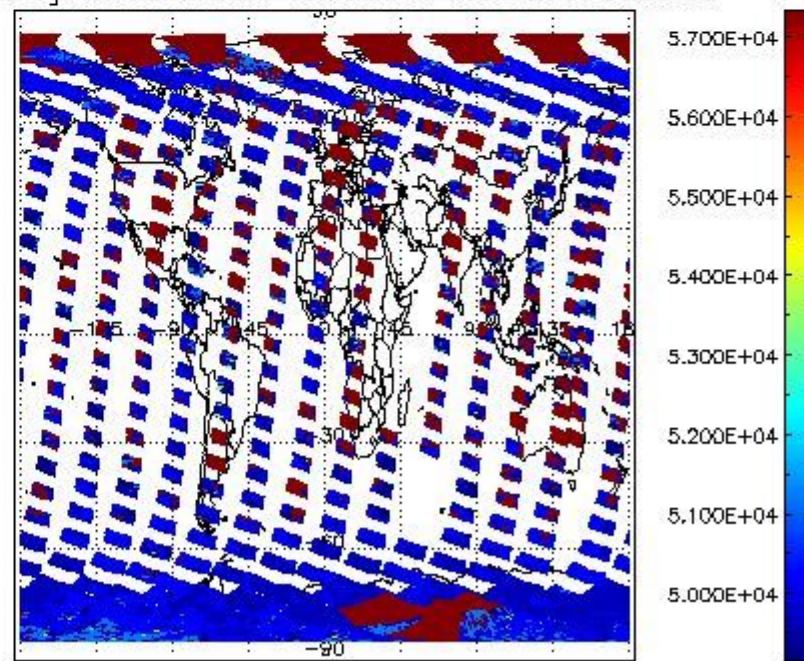
cloud_flags for 15OCT2011 00:00:00 to 16OCT2011 00:00:00
