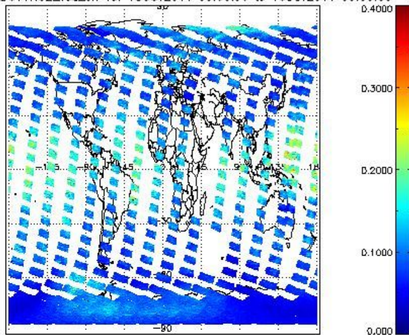
SCIOL2P_NADUV1NO2_vcd_err for 15OCT2011 00:00:00 to 16OCT2011 00:00:00
