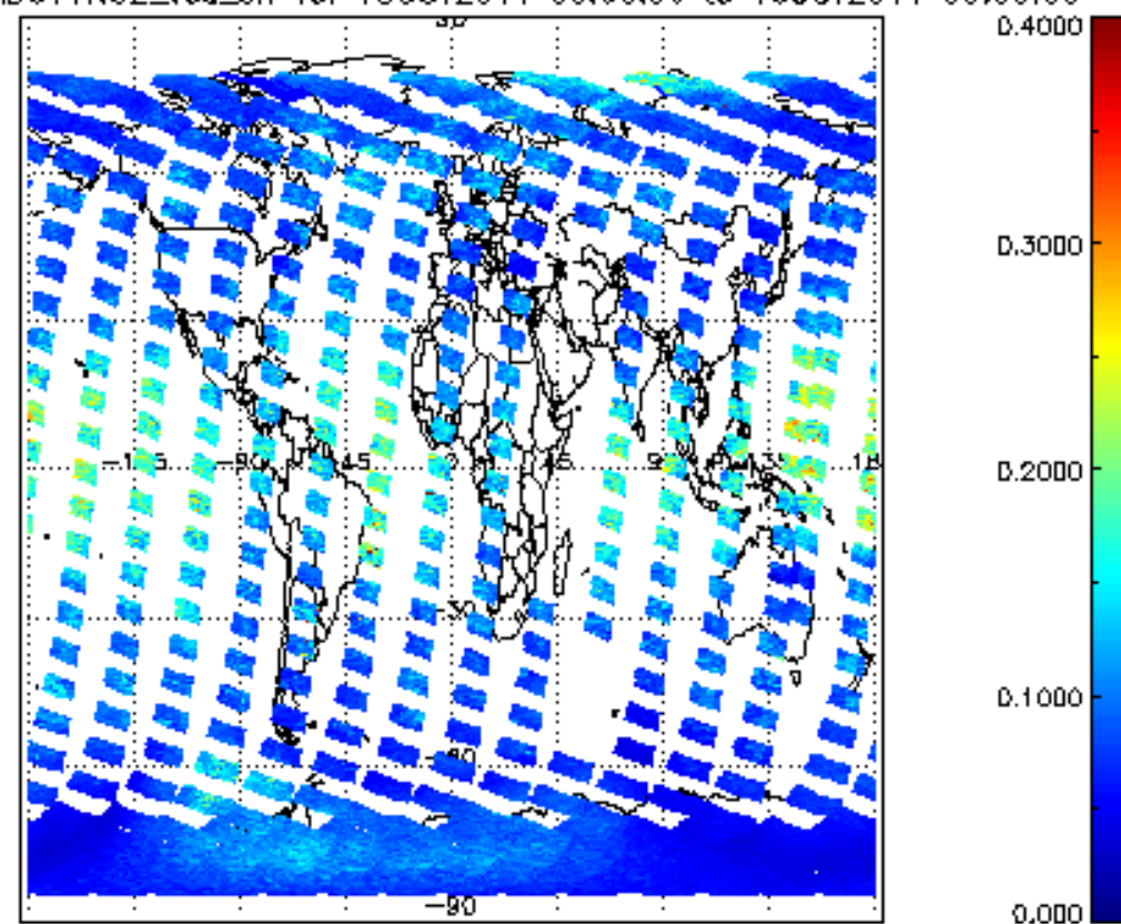
SCIOL2P_NADUV1NO2_vcd_err for 15OCT2011 00:00:00 to 16OCT2011 00:00:00
