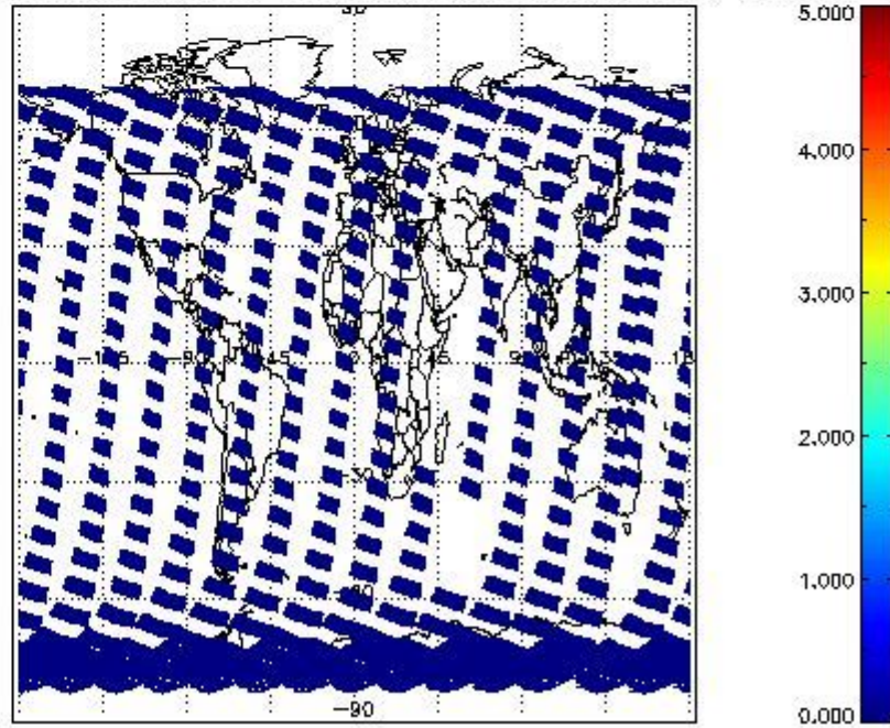
SCIOL2P_NADUV5S02_amf_cl for 15OCT2011 00:00:00 to 16OCT2011 00:00:00
