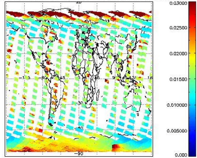
SCIOL2P_NADUV003_vcd_err for 15OCT2011 00:00:00 to 16OCT2011 00:00:00
