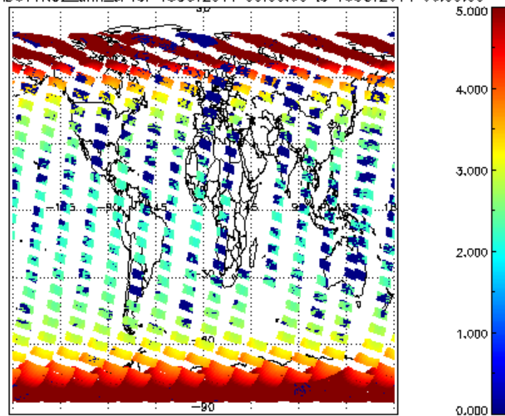
SCIOL2P_NADUV1NO2_amf_cl for 15OCT2011 00:00:00 to 16OCT2011 00:00:00
