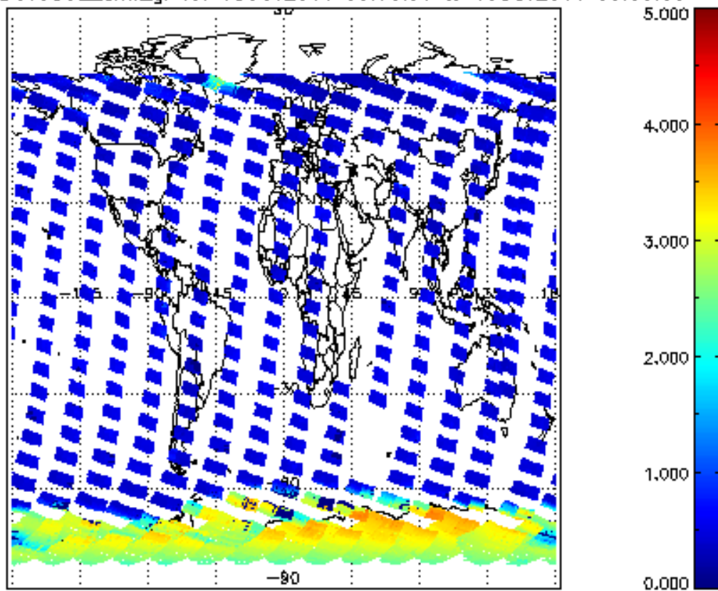
SCIOL2P_NADUV5S02_amf_gr for 15OCT2011 00:00:00 to 16OCT2011 00:00:00
