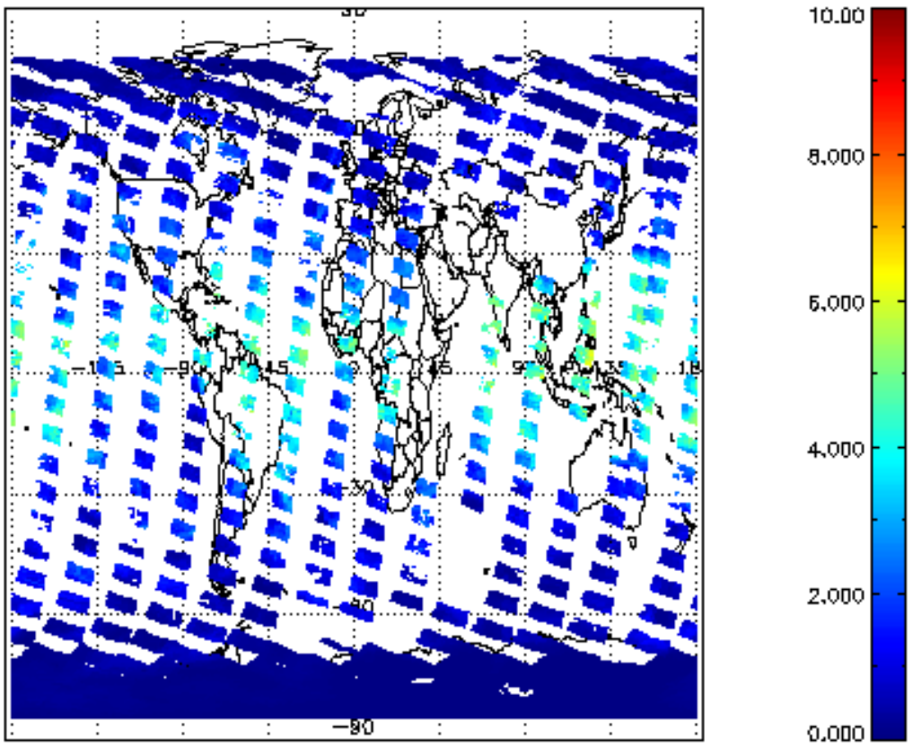
SCIOL2P_NADUV8H20_vcd for 15OCT2011 00:00:00 to 16OCT2011 00:00:00
