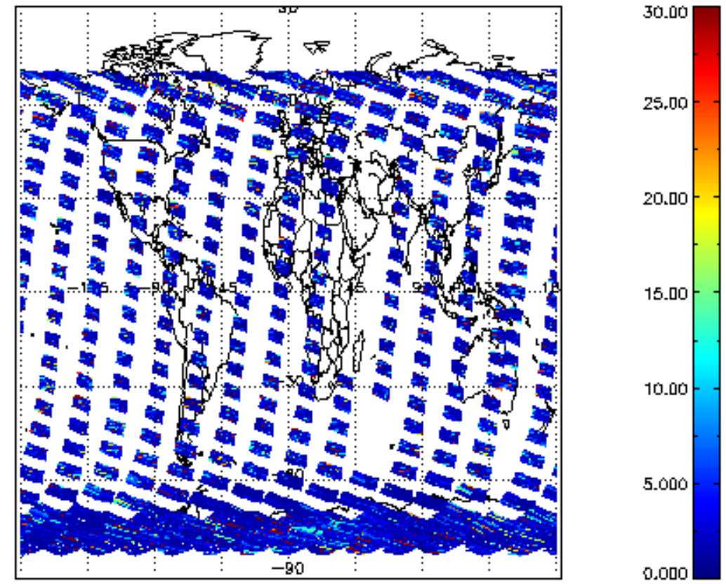
SCIOL2P_NADUV7S02_vcd_err for 15OCT2011 00:00:00 to 16OCT2011 00:00:00
