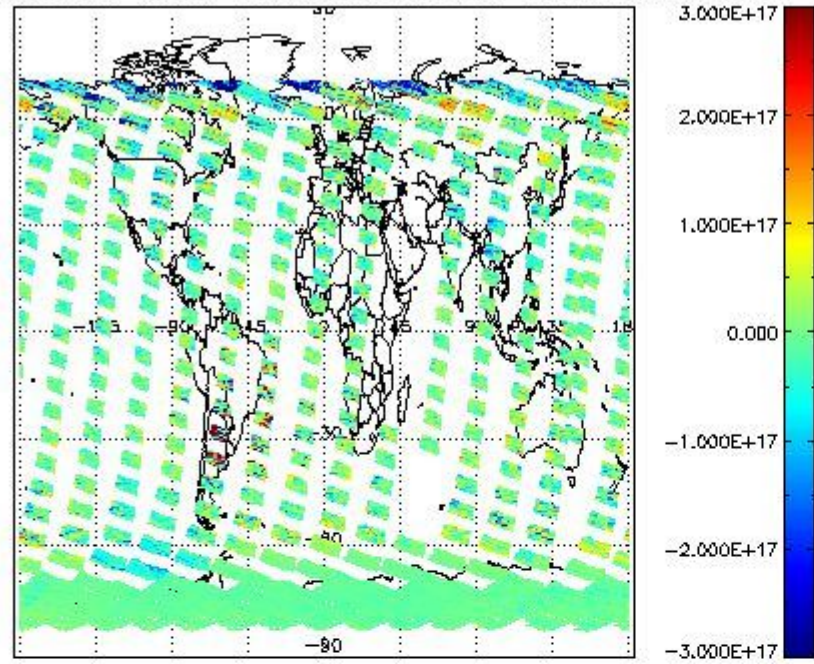
SCIOL2P_NADUV5S02_vcd for 15OCT2011 00:00:00 to 16OCT2011 00:00:00
