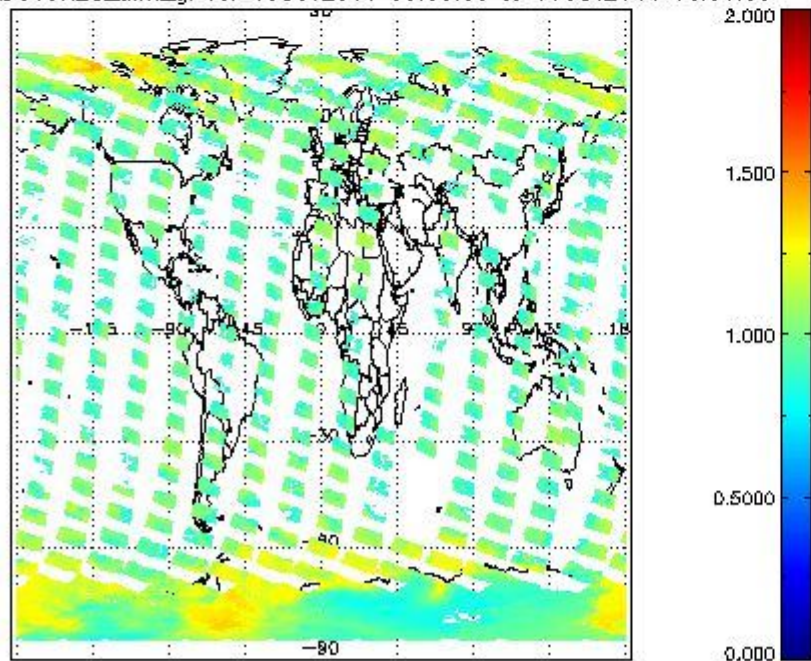
SCIOL2P_NADUV8H20_amf_gr for 15OCT2011 00:00:00 to 16OCT2011 00:00:00
