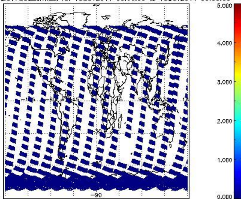
SCIOL2P_NADUV7S02_amf_cl for 15OCT2011 00:00:00 to 16OCT2011 00:00:00
