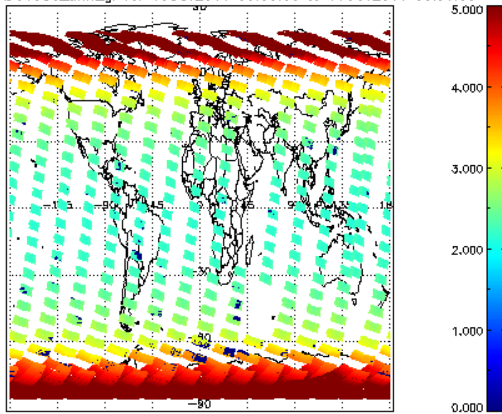
SCIOL2P_NADUV003_amf_gr for 15OCT2011 00:00:00 to 16OCT2011 00:00:00
