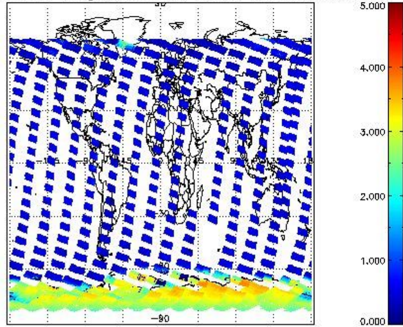
SCIOL2P_NADUV5S02_amf_gr for 15OCT2011 00:00:00 to 16OCT2011 00:00:00
