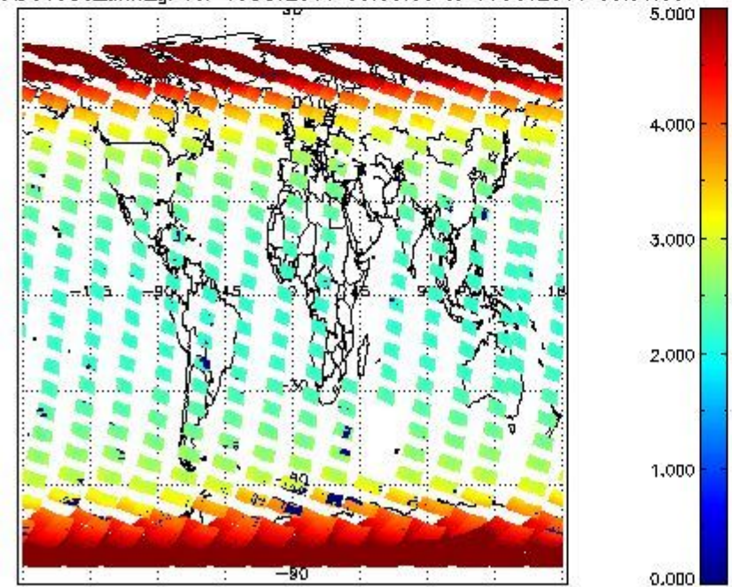
SCIOL2P_NADUV003_amf_gr for 15OCT2011 00:00:00 to 16OCT2011 00:00:00
