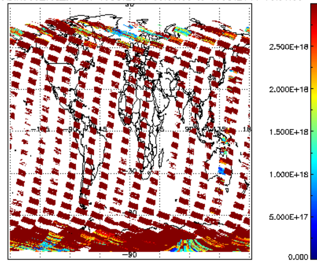
SCIOL2P_NADIR3CO_vcd_err for 15OCT2011 00:00:00 to 16OCT2011 00:00:00
