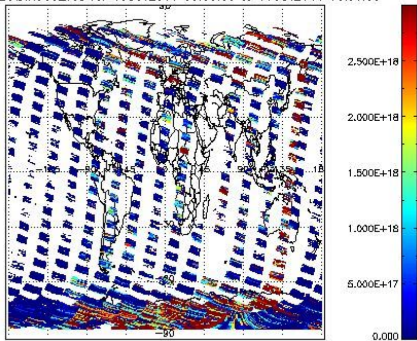
SCIOI2P_NADIR3CO_vcd for 15OCT2011 00:00:00 to 16OCT2011 00:00:00
