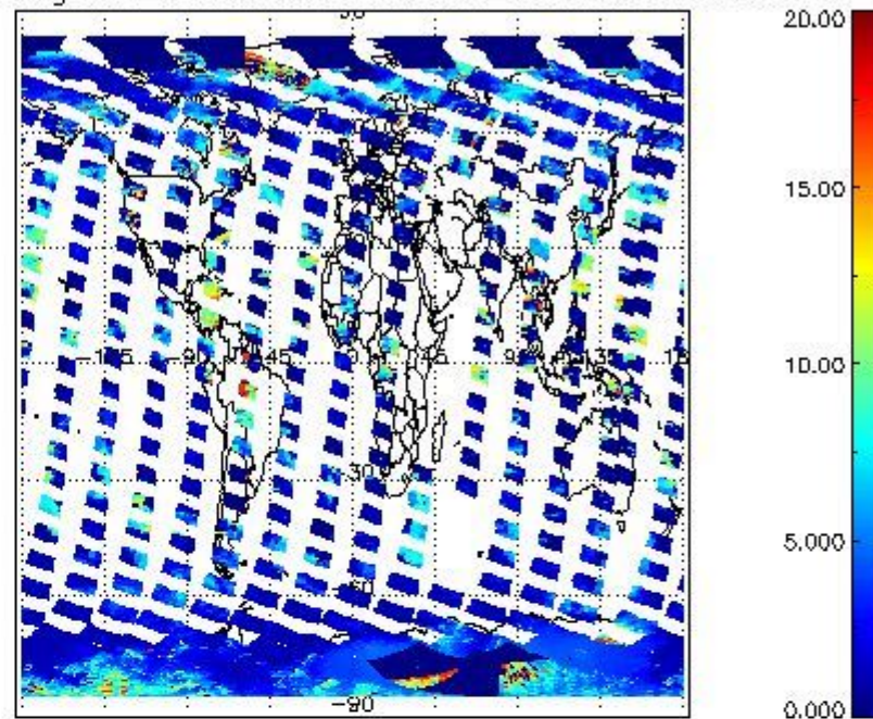
cL_top_height for 15OCT2011 00:00:00 to 16OCT2011 00:00:00
