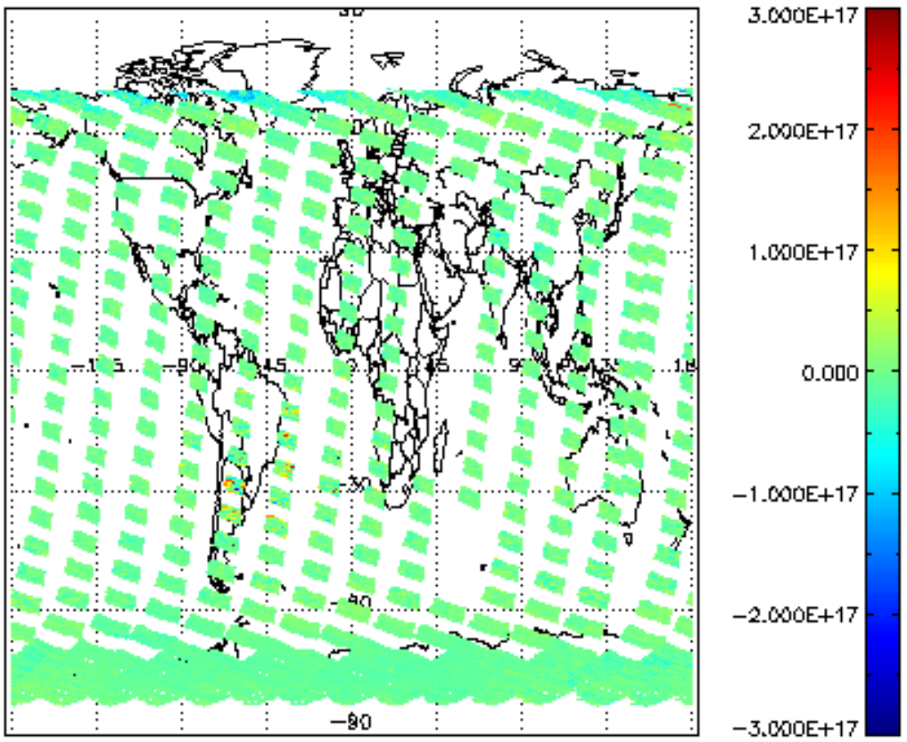
SCIOL2P_NADUV7S02_vcd for 15OCT2011 00:00:00 to 16OCT2011 00:00:00
