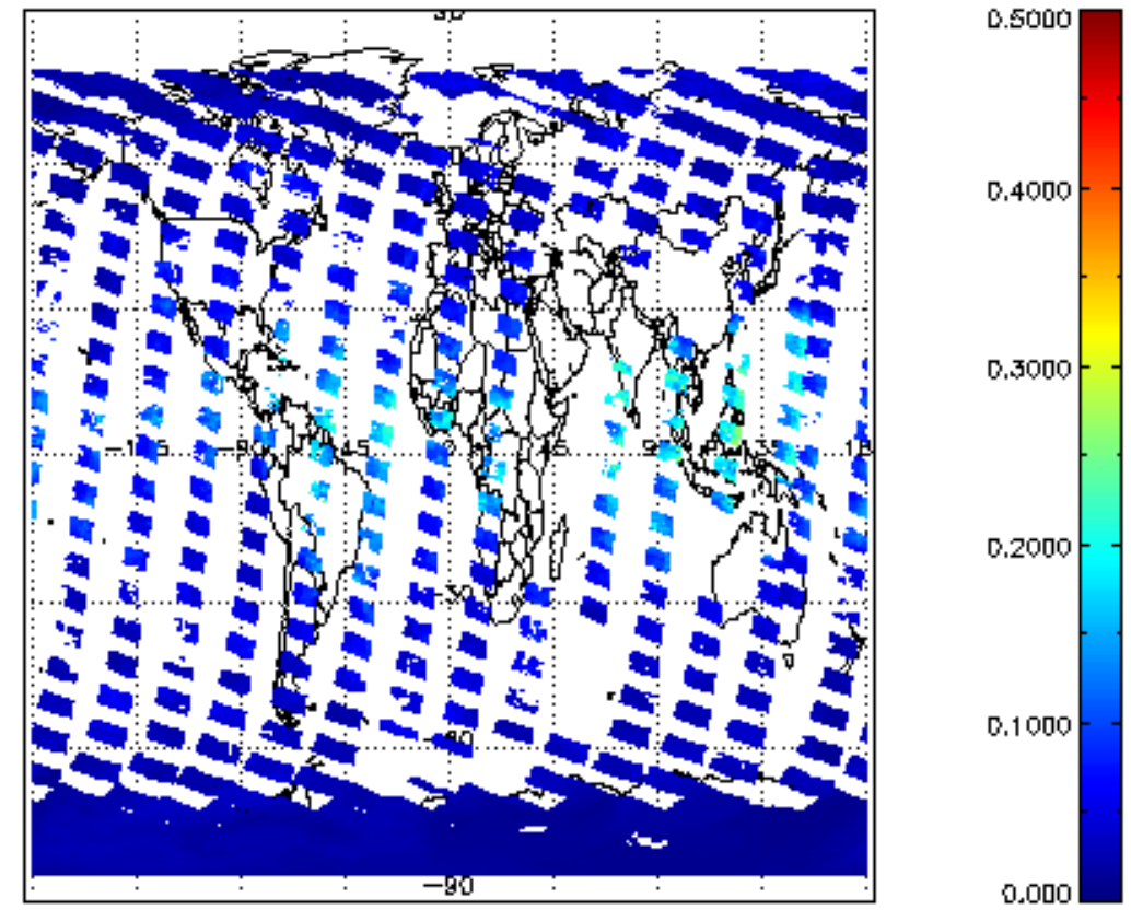
SCIOL2P_NADUV8H20_vcd_err for 15OCT2011 00:00:00 to 16OCT2011 00:00:00
