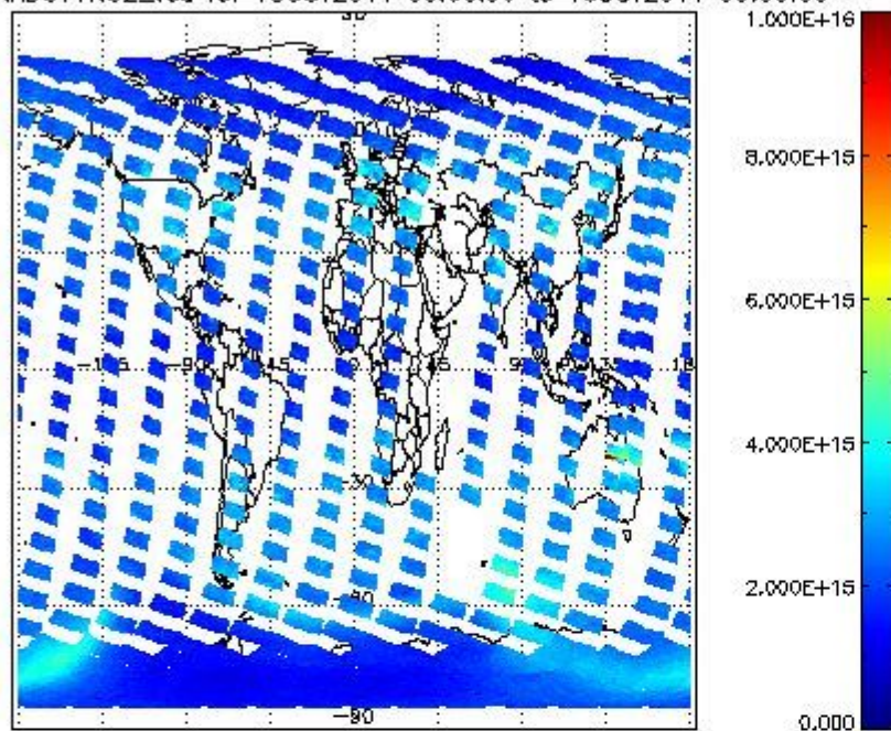
SCIOL2P_NADUV1NO2_vcd for 15OCT2011 00:00:00 to 16OCT2011 00:00:00
