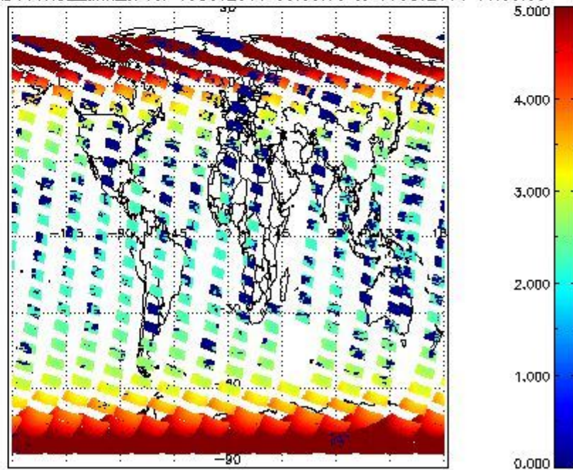
SCIOL2P_NADUV1NO2_amf_cl for 15OCT2011 00:00:00 to 16OCT2011 00:00:00
