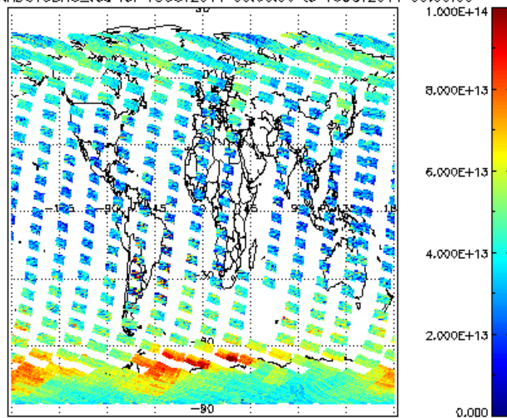
SCIOL2P_NADUV3BRO_vcd for 15OCT2011 00:00:00 to 16OCT2011 00:00:00
