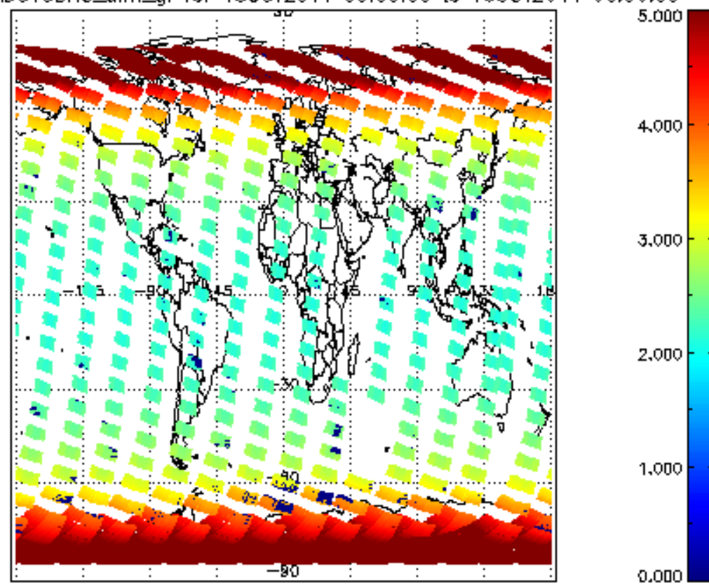
SCIOL2P_NADUV3BRO_amf_gr for 15OCT2011 00:00:00 to 16OCT2011 00:00:00
