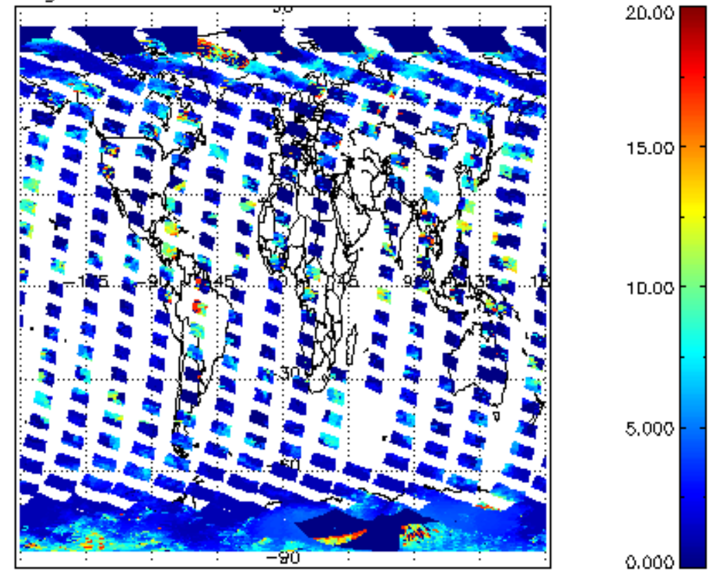
cl_top_height for 15OCT2011 00:00:00 to 16OCT2011 00:00:00
