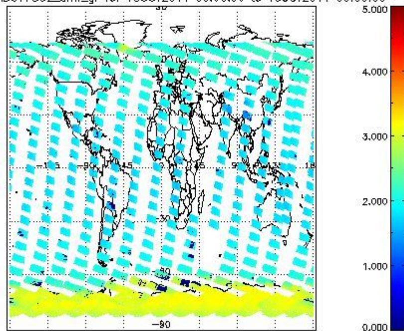
SCIOL2P_NADUV7S02_amf_gr for 15OCT2011 00:00:00 to 16OCT2011 00:00:00
