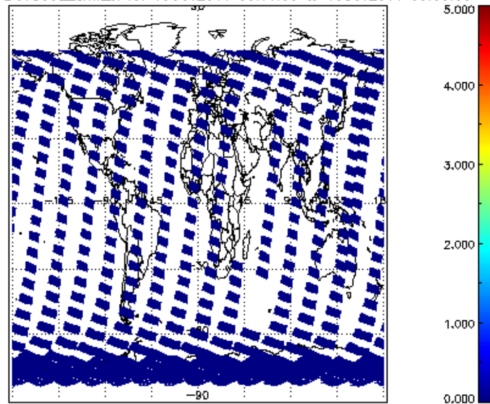
SCIOL2P_NADUV5S02_amf_cl for 15OCT2011 00:00:00 to 16OCT2011 00:00:00
