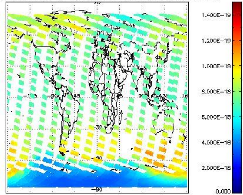
SCIOL2P_NADUV003_vcd for 15OCT2011 00:00:00 to 16OCT2011 00:00:00
