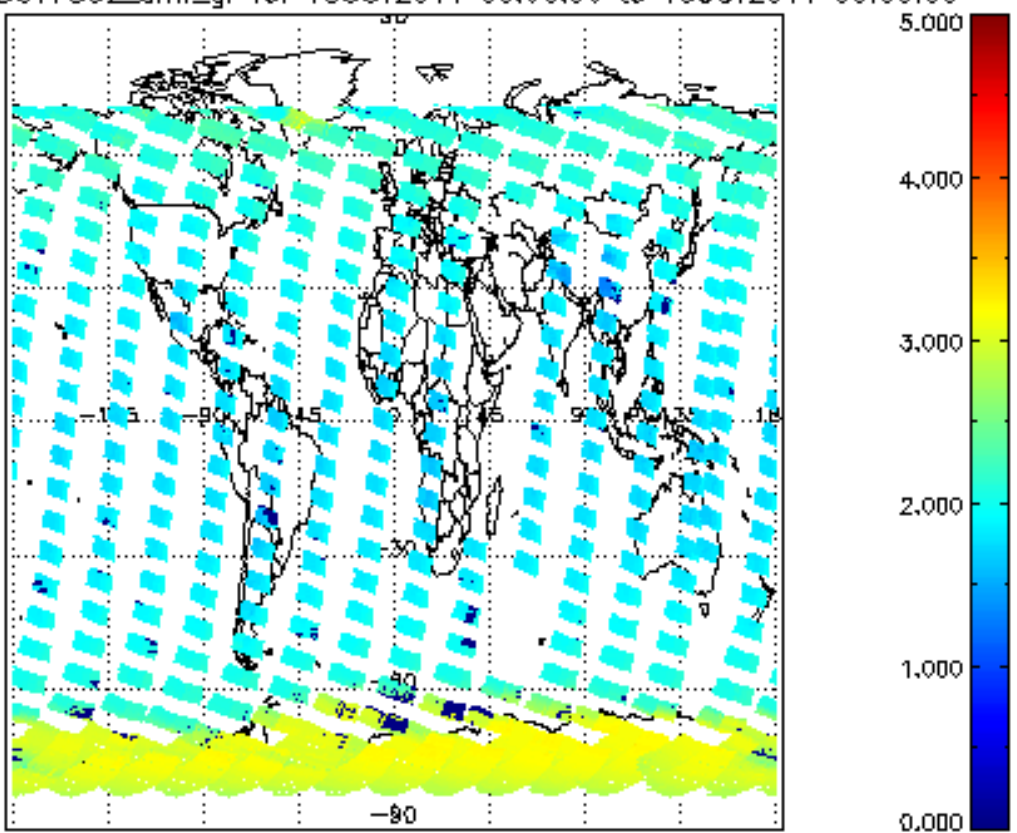
SCIOL2P_NADUV7S02_amf_gr for 15OCT2011 00:00:00 to 16OCT2011 00:00:00
