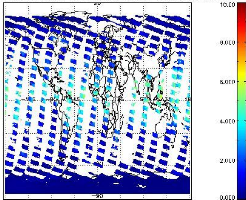
SCIOL2P_NADUV8H20_vcd for 15OCT2011 00:00:00 to 16OCT2011 00:00:00
