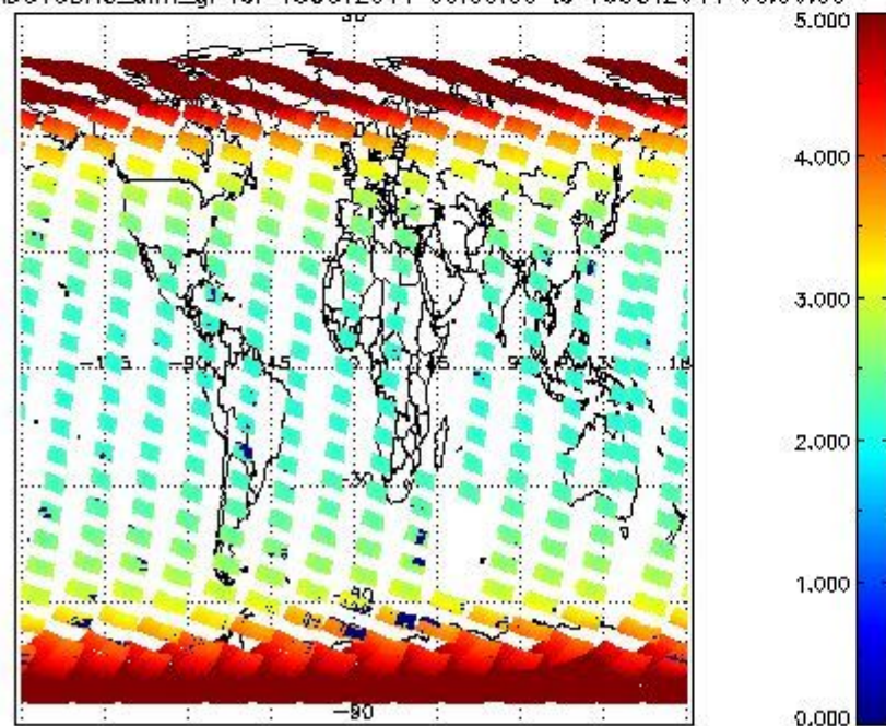
SCIOL2P_NADUV3BRO_amf_gr for 15OCT2011 00:00:00 to 16OCT2011 00:00:00
