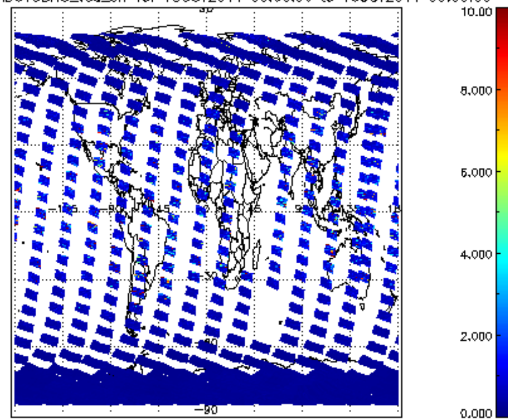
SCIOL2P_NADUV3BRO_vcd_err for 15OCT2011 00:00:00 to 16OCT2011 00:00:00
