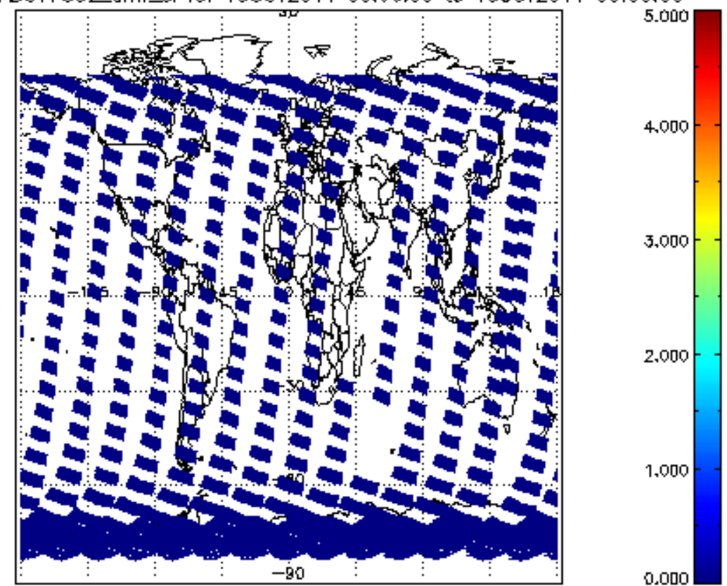
SCIOL2P_NADUV7S02_amf_sl for 15OCT2011 00:00:00 to 16OCT2011 00:00:00
