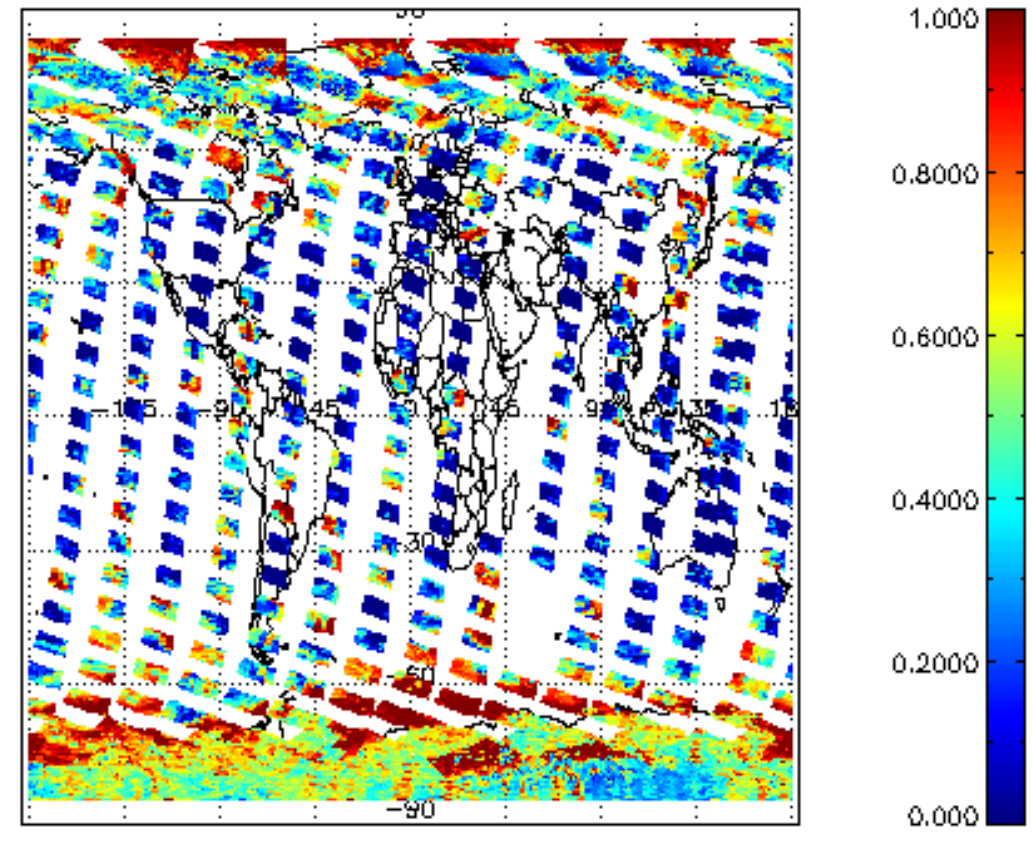
cl_frac for 15OCT2011 00:00:00 to 16OCT2011 00:00:00
