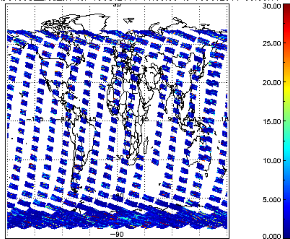
SCIOL2P_NADUV5S02_vcd_err for 15OCT2011 00:00:00 to 16OCT2011 00:00:00
