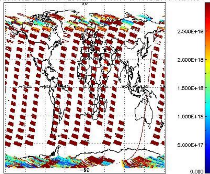
SCIO2P_NADIR3CO_vcd_err for 12OCT2011 00:00:00 to 13OCT2011 00:00:00
