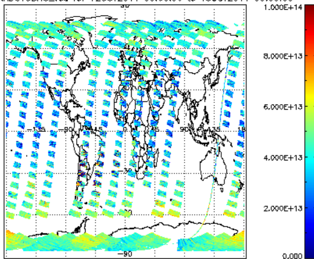
SCIOL2P_NADUV3BRO_vcd for 12OCT2011 00:00:00 to 13OCT2011 00:00:00
