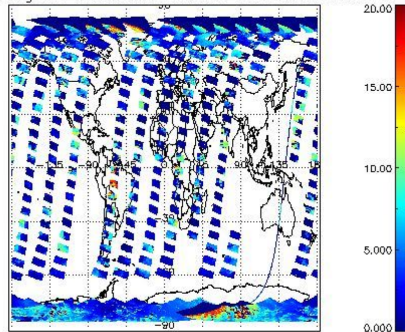
cL_top_height for 12OCT2011 00:00:00 to 13OCT2011 00:00:00
