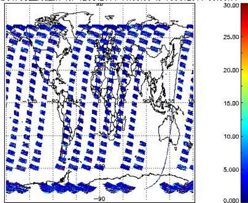
SCIOL2P_NADUV7S02_vcd_err for 12OCT2011 00:00:00 to 13OCT2011 00:00:00
