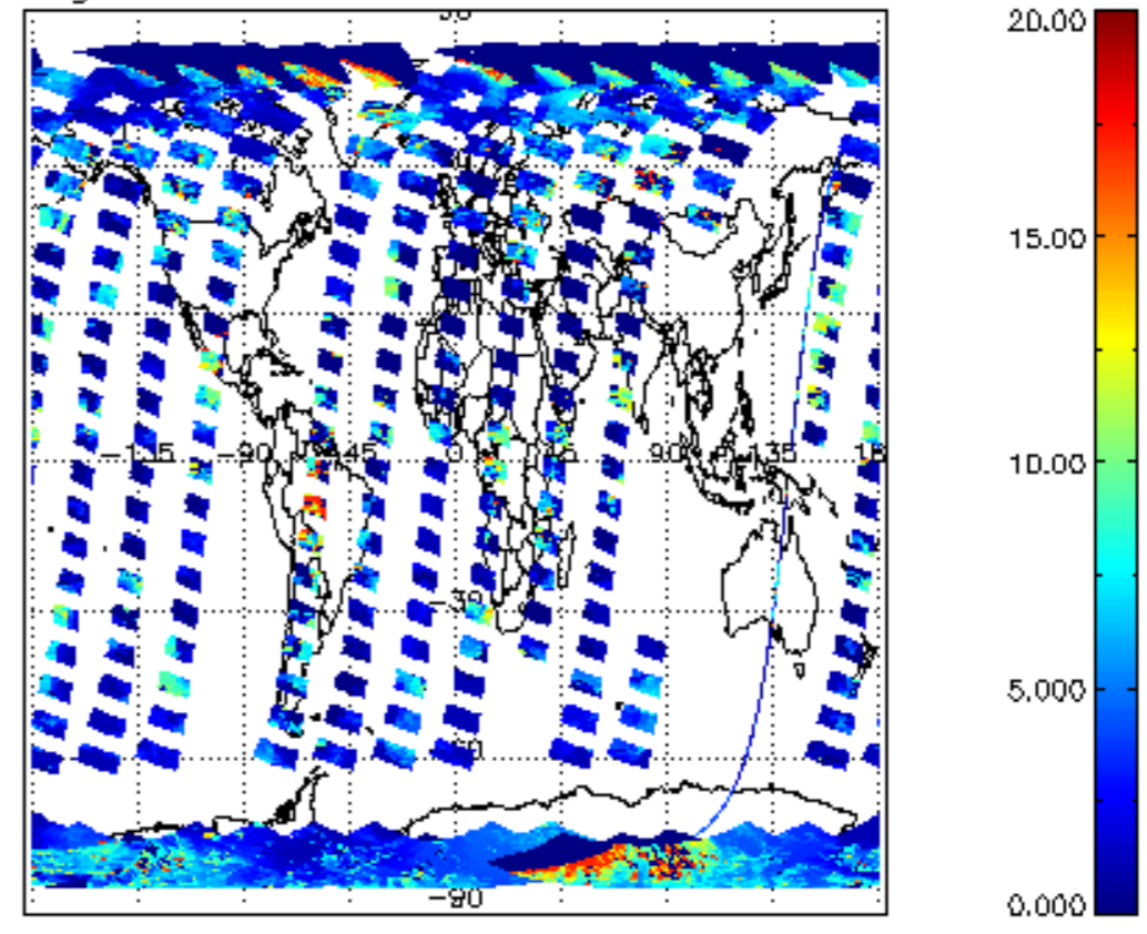
cl_top_height for 12OCT2011 00:00:00 to 13OCT2011 00:00:00
