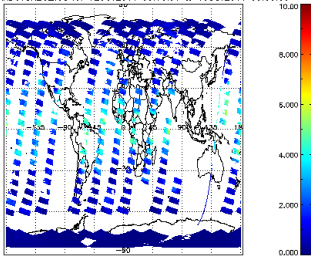
SCIOL2P_NADUV8H20_vcd for 12OCT2011 00:00:00 to 13OCT2011 00:00:00
