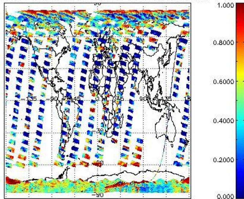
cLfrac for 12OCT2011 00:00:00 to 13OCT2011 00:00:00
