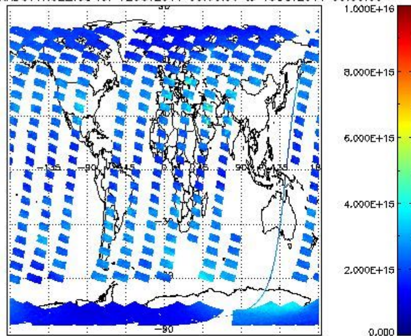
SCIOL2P_NADUV1NO2_vcd for 12OCT2011 00:00:00 to 13OCT2011 00:00:00
