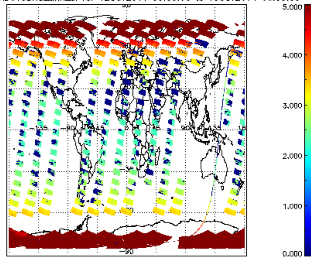
SCIOL2P_NADUV3BRO_amf_cl for 12OCT2011 00:00:00 to 13OCT2011 00:00:00
