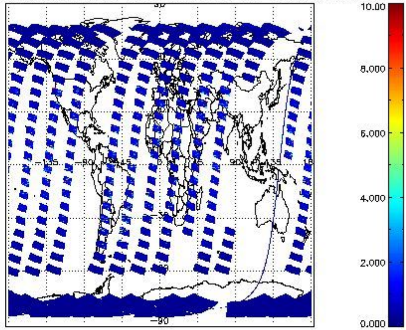
SCIOL2P_NADUV3BRO_vcd_err for 12OCT2011 00:00:00 to 13OCT2011 00:00:00
