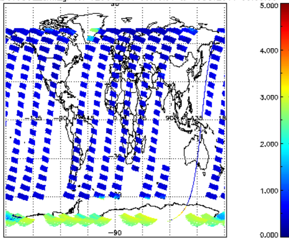
SCIOL2P_NADUV5S02_amf_gr for 12OCT2011 00:00:00 to 13OCT2011 00:00:00
