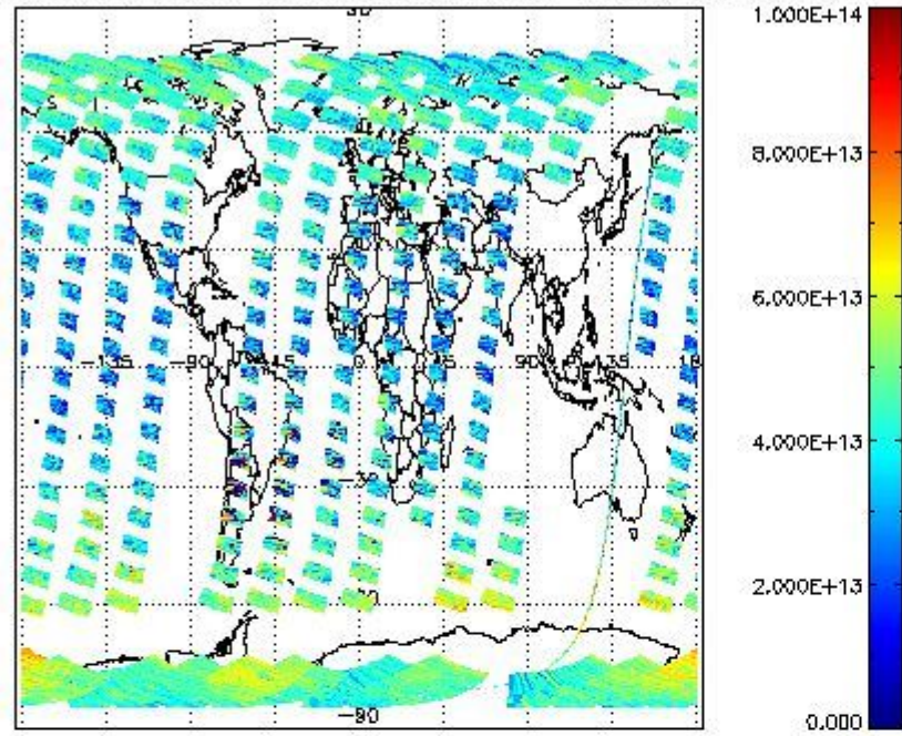
SCIOL2P_NADUV3BRO_vcd for 12OCT2011 00:00:00 to 13OCT2011 00:00:00
