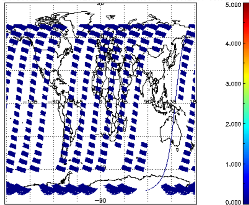
SCIOL2P_NADUV5S02_amf_cl for 12OCT2011 00:00:00 to 13OCT2011 00:00:00
