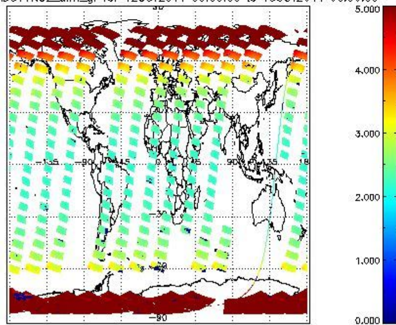
SCIOL2P_NADUV1NO2_amf_gr for 12OCT2011 00:00:00 to 13OCT2011 00:00:00
