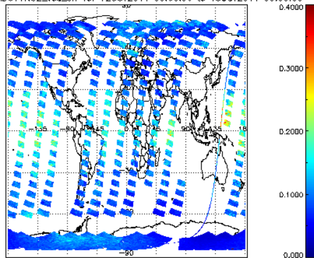
SCIOL2P_NADUV1NO2_vcd_err for 12OCT2011 00:00:00 to 13OCT2011 00:00:00
