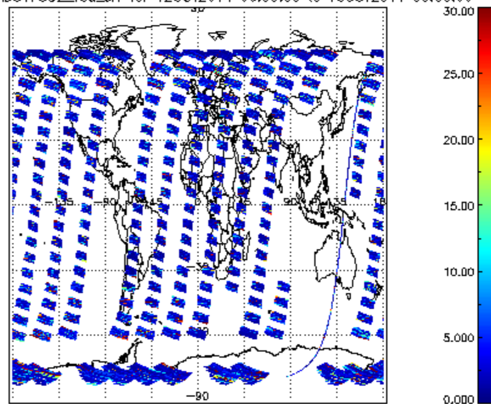
SCIOL2P_NADUV7S02_vcd_err for 12OCT2011 00:00:00 to 13OCT2011 00:00:00
