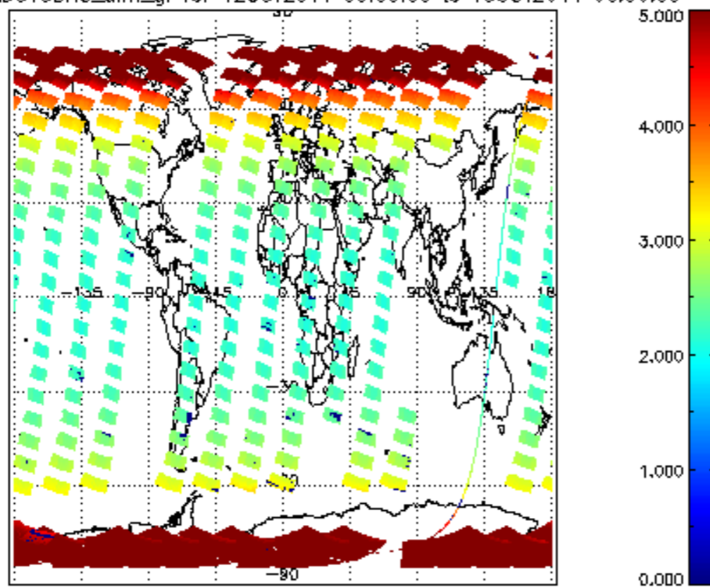
SCIOL2P_NADUV3BRO_amf_gr for 12OCT2011 00:00:00 to 13OCT2011 00:00:00
