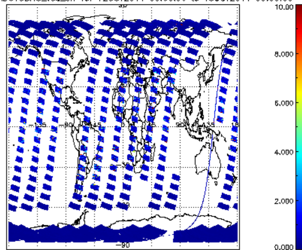
SCIOL2P_NADUV3BRO_vcd_err for 12OCT2011 00:00:00 to 13OCT2011 00:00:00
