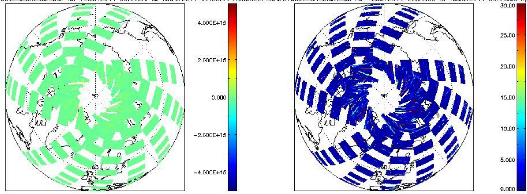
CIOL2P_NADUV60CL_slant_col_den for 12OCT2011 00:00:00 to 13OCT2011 00:00:00 np CIOL2P_NADUV60CL_err_slant_col for 12OCT2011 00:00:00 to 13OCT2011 00:00:00 np
