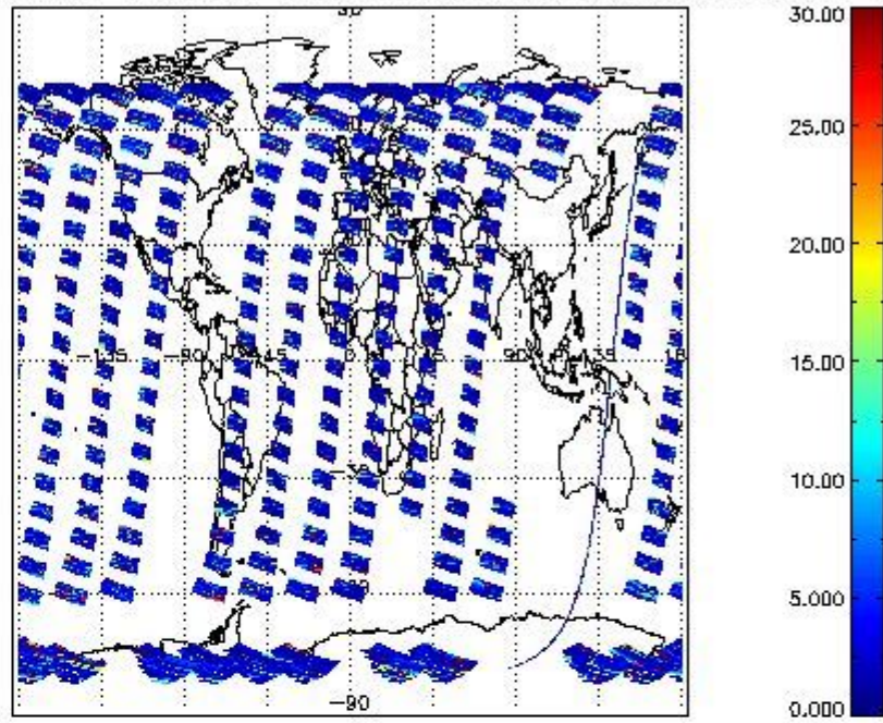
SCIOL2P_NADUV5S02_vcd_err for 12OCT2011 00:00:00 to 13OCT2011 00:00:00
