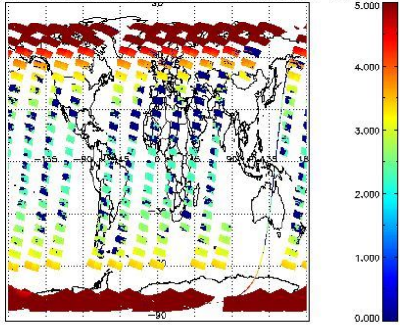
SCIOL2P_NADUV3BRO_amf_cl for 12OCT2011 00:00:00 to 13OCT2011 00:00:00
