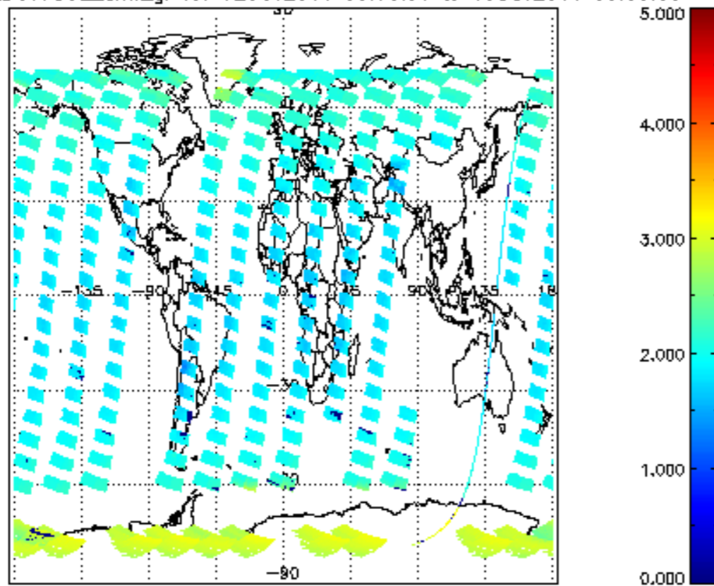
SCIOL2P_NADUV7S02_amf_gr for 12OCT2011 00:00:00 to 13OCT2011 00:00:00
