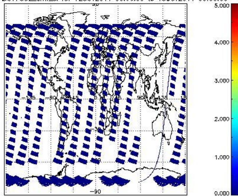
SCIOL2P_NADUV7S02_amf_cl for 12OCT2011 00:00:00 to 13OCT2011 00:00:00
