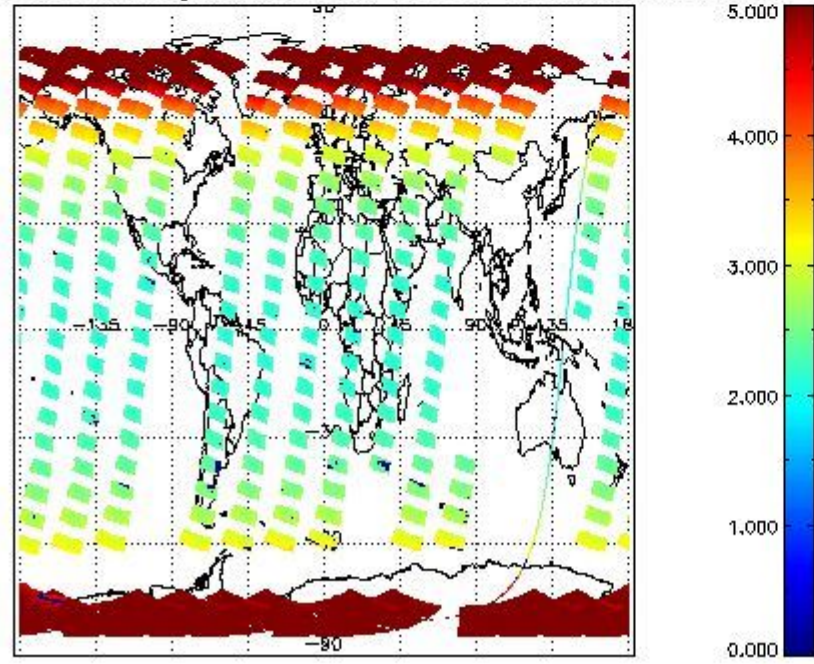
SCIOL2P_NADUV3BRO_amf_gr for 12OCT2011 00:00:00 to 13OCT2011 00:00:00
