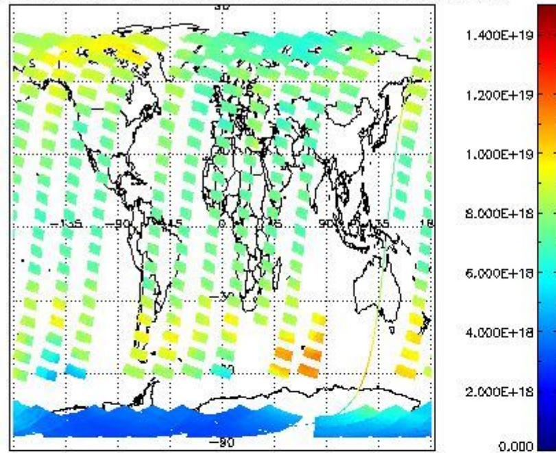
SCIOL2P_NADUV003_vcd for 12OCT2011 00:00:00 to 13OCT2011 00:00:00
