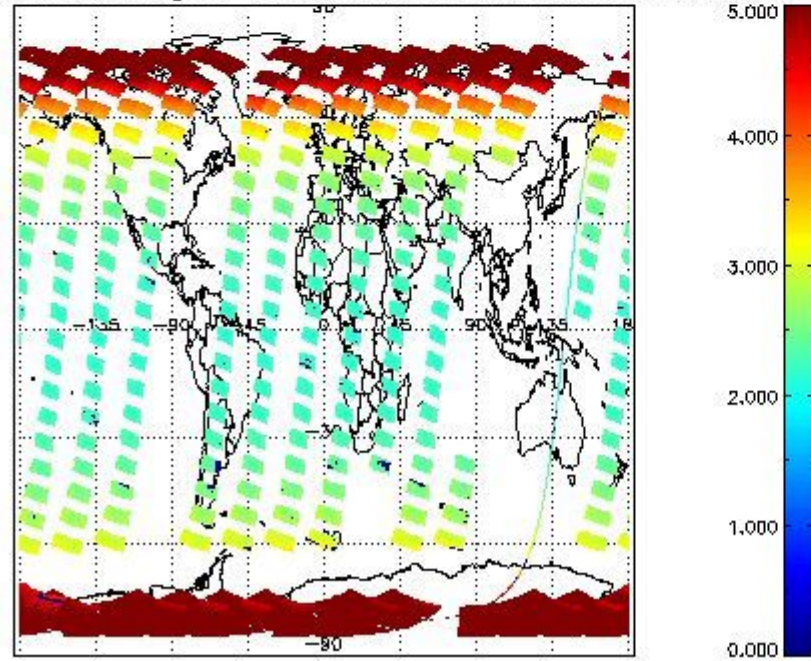
SCIOL2P_NADUV003_amf_gr for 12OCT2011 00:00:00 to 13OCT2011 00:00:00
