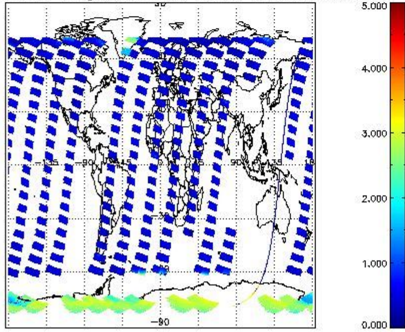
SCIOL2P_NADUV5S02_amf_gr for 12OCT2011 00:00:00 to 13OCT2011 00:00:00
