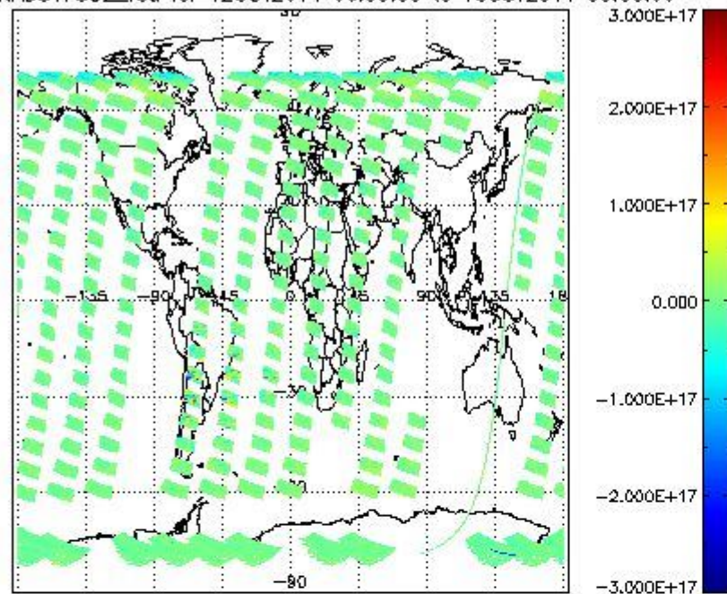
SCIOL2P_NADUV7S02_vcd for 12OCT2011 00:00:00 to 13OCT2011 00:00:00
