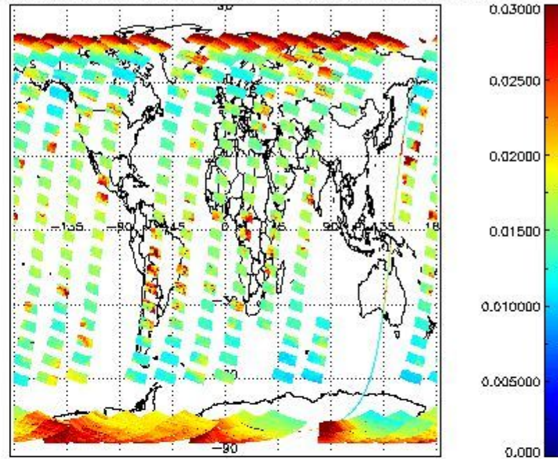
SCIOL2P_NADUV003_vcd_err for 12OCT2011 00:00:00 to 13OCT2011 00:00:00
