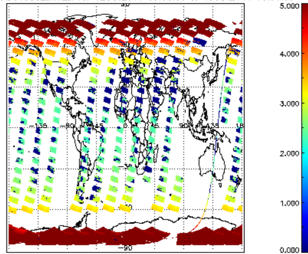
SCIOL2P_NADUV003_amf_cl for 12OCT2011 00:00:00 to 13OCT2011 00:00:00
