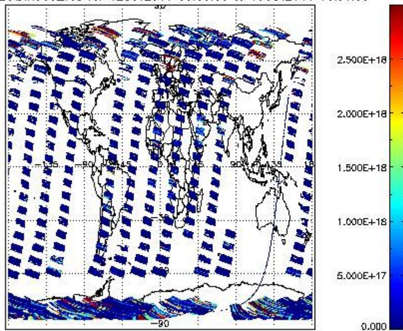
SCIO2P_NADIR3CO_vcd for 12OCT2011 00:00:00 to 13OCT2011 00:00:00
