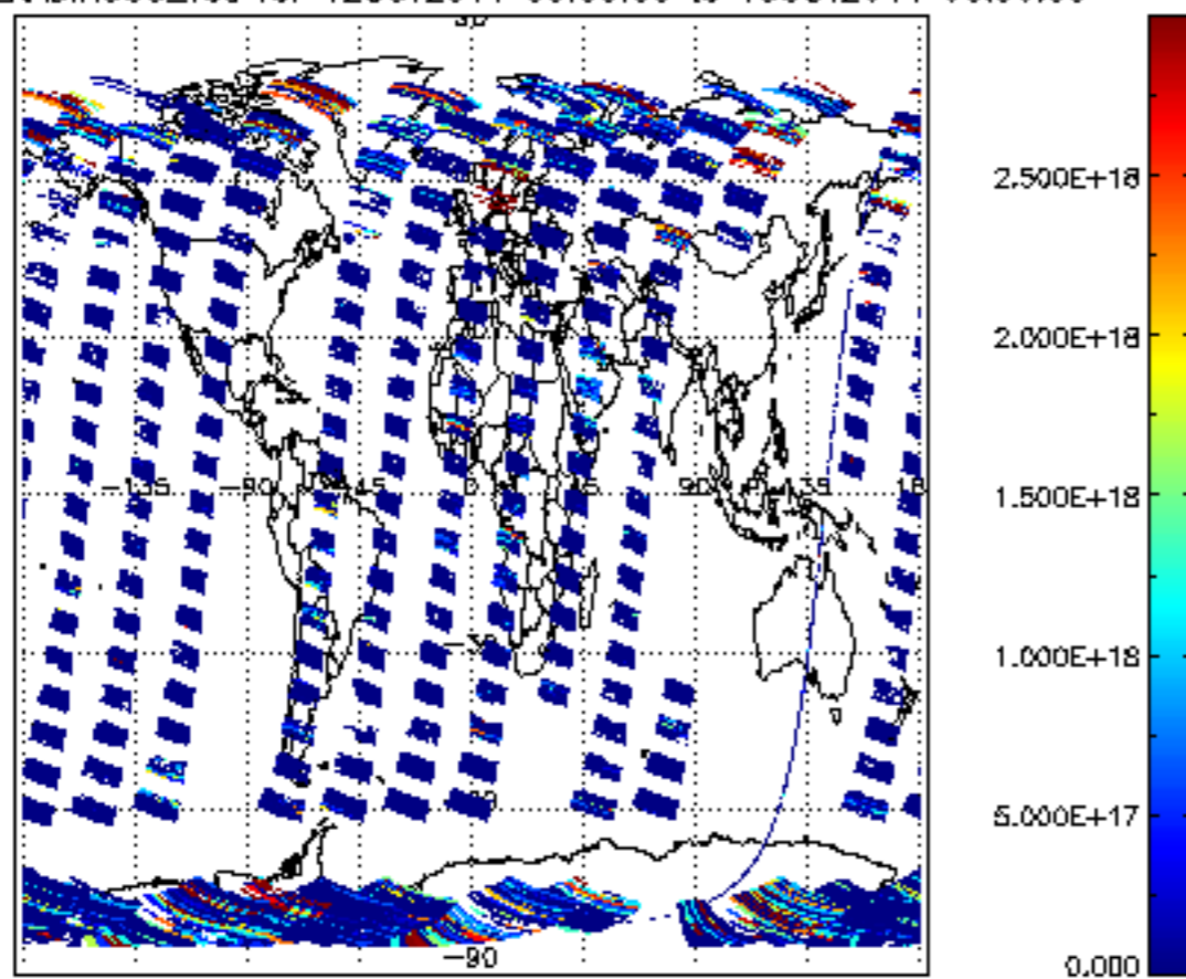
SCIOL2P_NADIR3CO_vcd for 12OCT2011 00:00:00 to 13OCT2011 00:00:00
