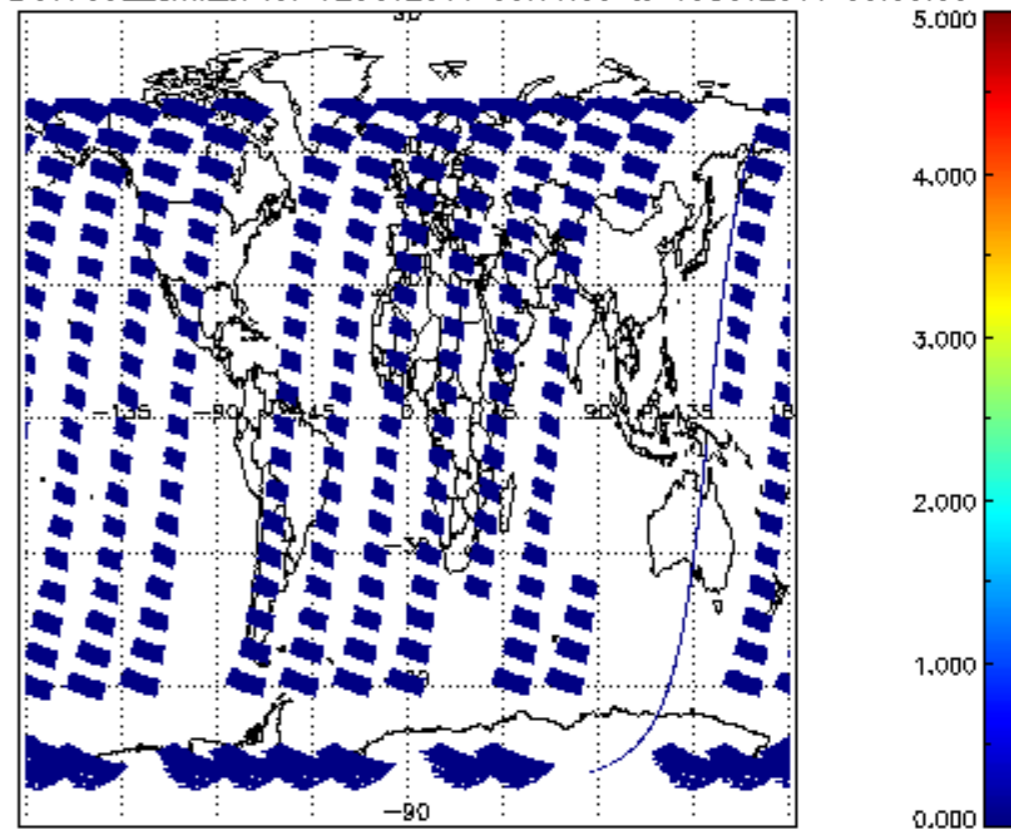
SCIOL2P_NADUV7S02_amf_cl for 12OCT2011 00:00:00 to 13OCT2011 00:00:00
