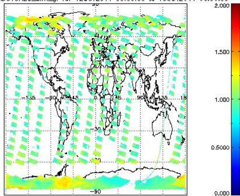
SCIOL2P_NADUV8H2O_amf_gr for 12OCT2011 00:00:00 to 13OCT2011 00:00:00
