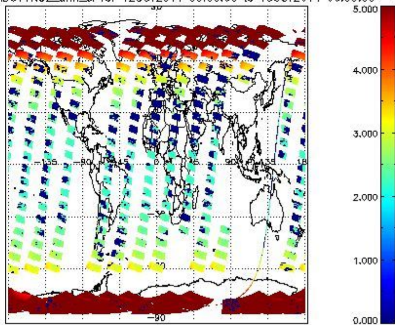
SCIOL2P_NADUV1NO2_amf_cl for 12OCT2011 00:00:00 to 13OCT2011 00:00:00
