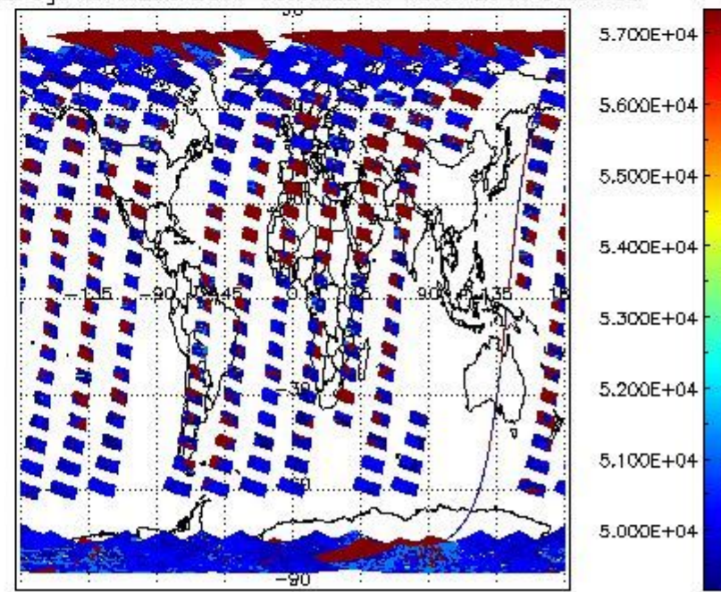
cloud_flags for 12OCT2011 00:00:00 to 13OCT2011 00:00:00
