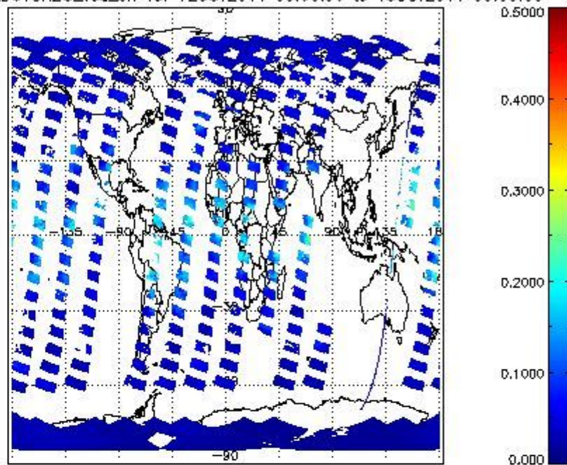
SCIOL2P_NADUV8H2O_vcd_err for 12OCT2011 00:00:00 to 13OCT2011 00:00:00
