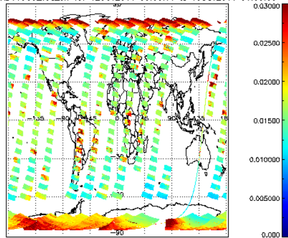
SCIOL2P_NADUV003_vcd_err for 12OCT2011 00:00:00 to 13OCT2011 00:00:00
