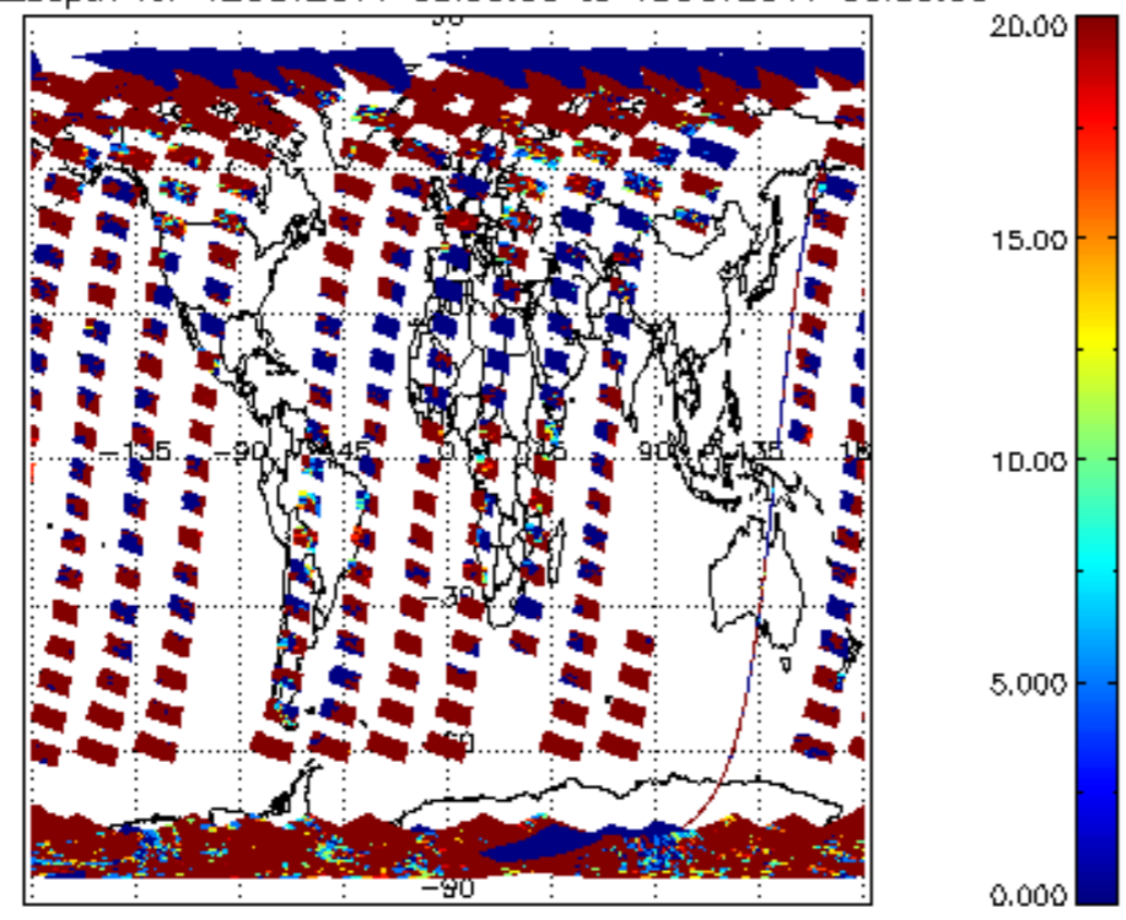
cl_opt_depth for 12OCT2011 00:00:00 to 13OCT2011 00:00:00
