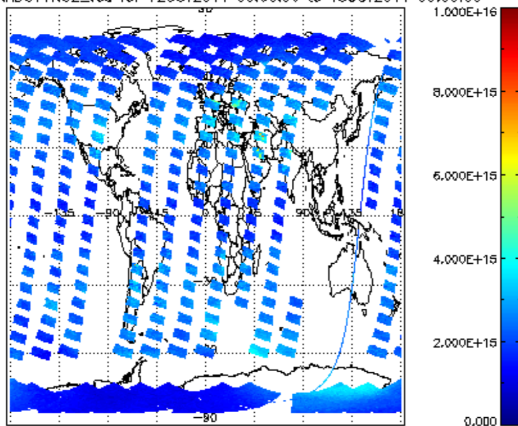
SCIOL2P_NADUV1NO2_vcd for 12OCT2011 00:00:00 to 13OCT2011 00:00:00
