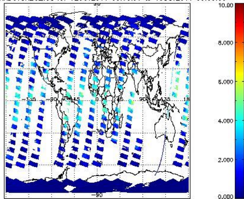
SCIOL2P_NADUV8H2O_vcd for 12OCT2011 00:00:00 to 13OCT2011 00:00:00
