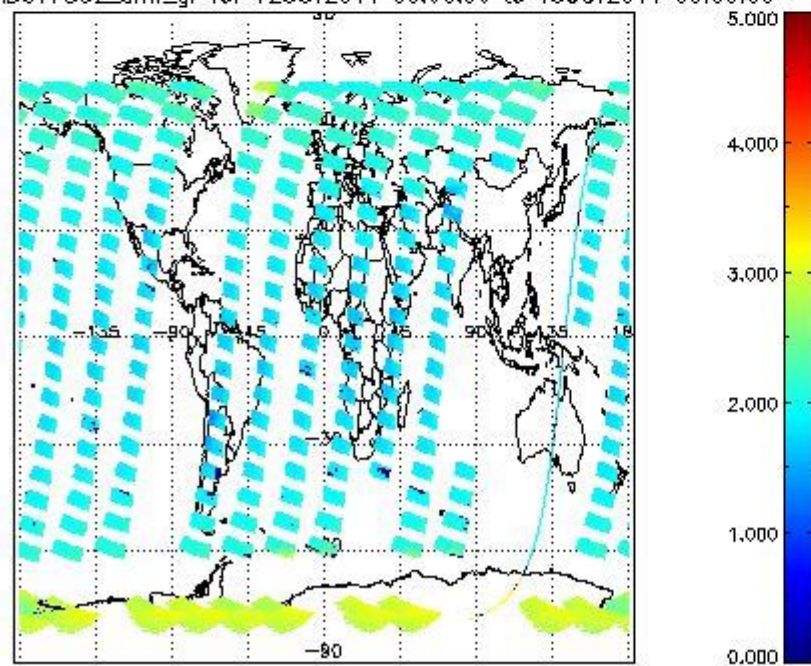
SCIOL2P_NADUV7S02_amf_gr for 12OCT2011 00:00:00 to 13OCT2011 00:00:00
