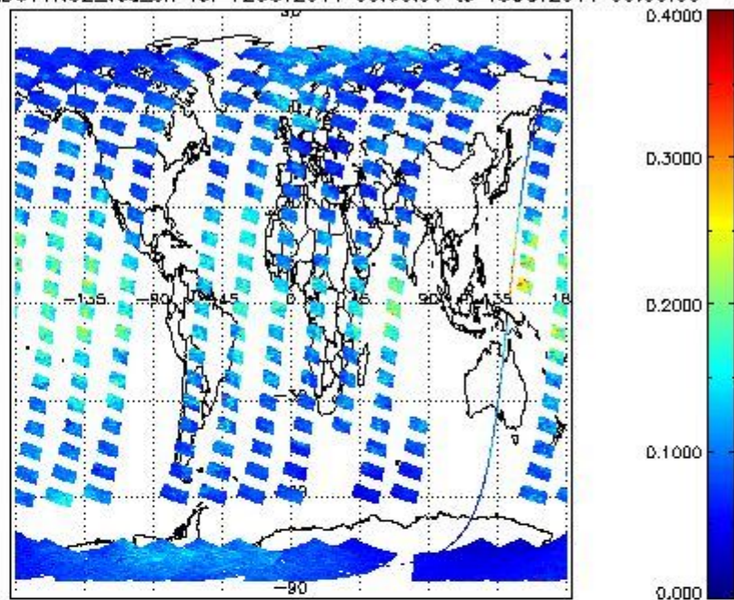
SCIOL2P_NADUV1NO2_vcd_err for 12OCT2011 00:00:00 to 13OCT2011 00:00:00
