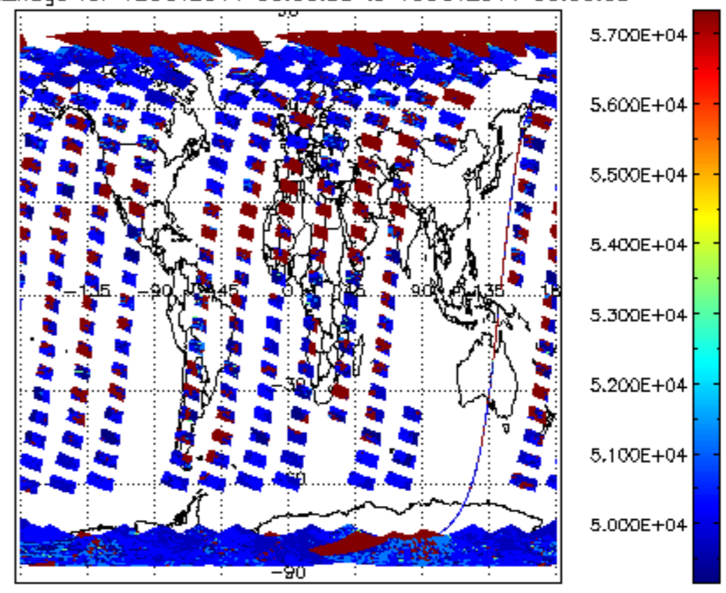
cloud_flags for 12OCT2011 00:00:00 to 13OCT2011 00:00:00
