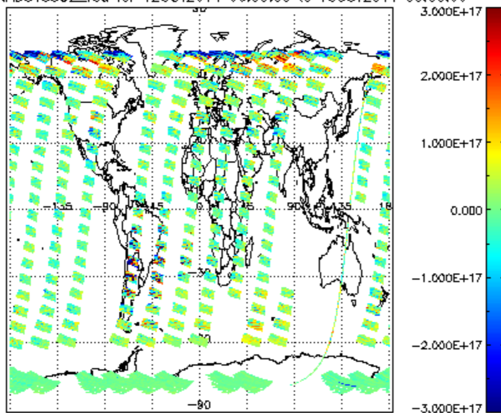
SCIOL2P_NADUV5S02_vcd for 12OCT2011 00:00:00 to 13OCT2011 00:00:00
