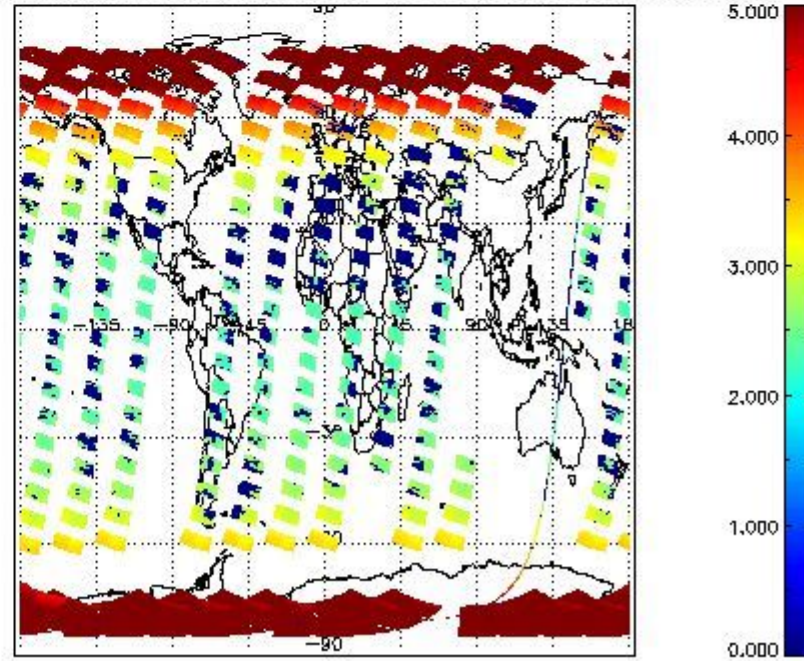
SCIOL2P_NADUV003_amf_cl for 12OCT2011 00:00:00 to 13OCT2011 00:00:00
