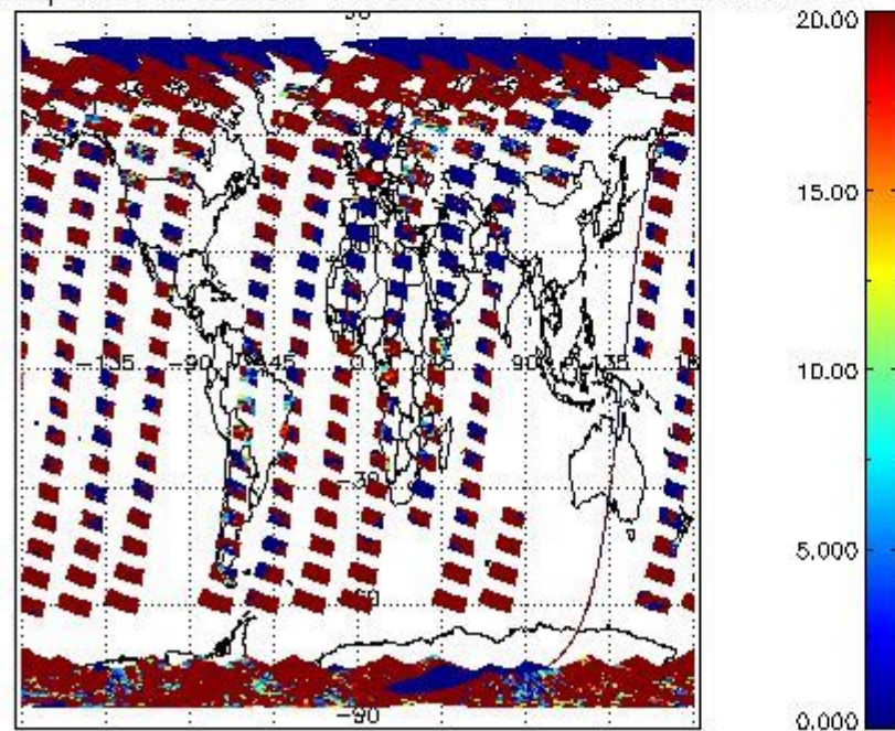
cL_opt_depth for 12OCT2011 00:00:00 to 13OCT2011 00:00:00
