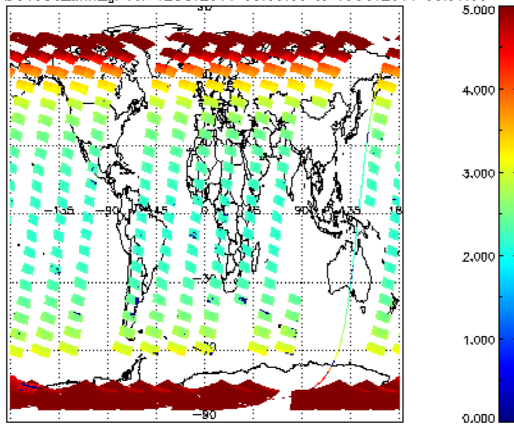
SCIOL2P_NADUV003_amf_gr for 12OCT2011 00:00:00 to 13OCT2011 00:00:00
