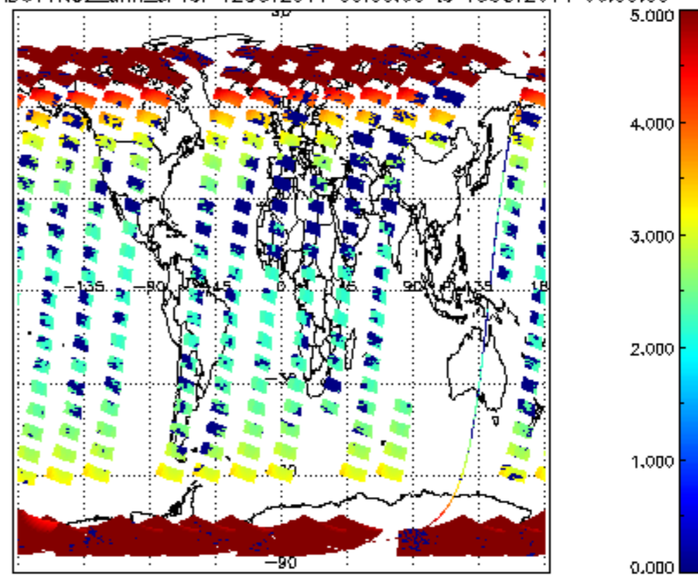
SCIOL2P_NADUV1NO2_amf_cl for 12OCT2011 00:00:00 to 13OCT2011 00:00:00
