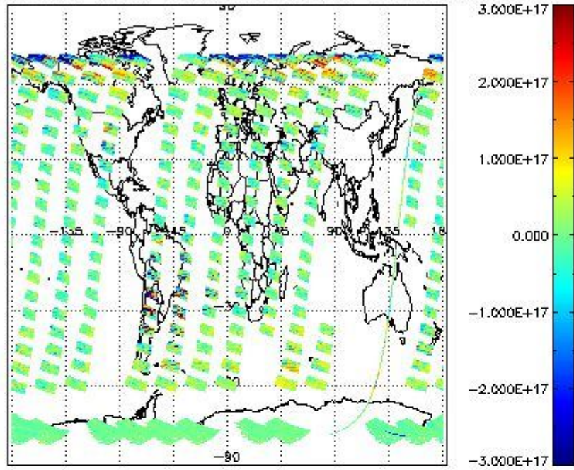
SCIOL2P_NADUV5S02_vcd for 12OCT2011 00:00:00 to 13OCT2011 00:00:00
