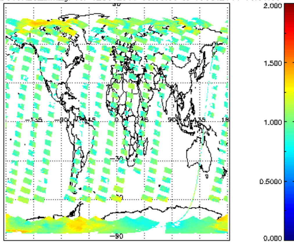
SCIOL2P_NADUV8H20_amf_gr for 12OCT2011 00:00:00 to 13OCT2011 00:00:00
