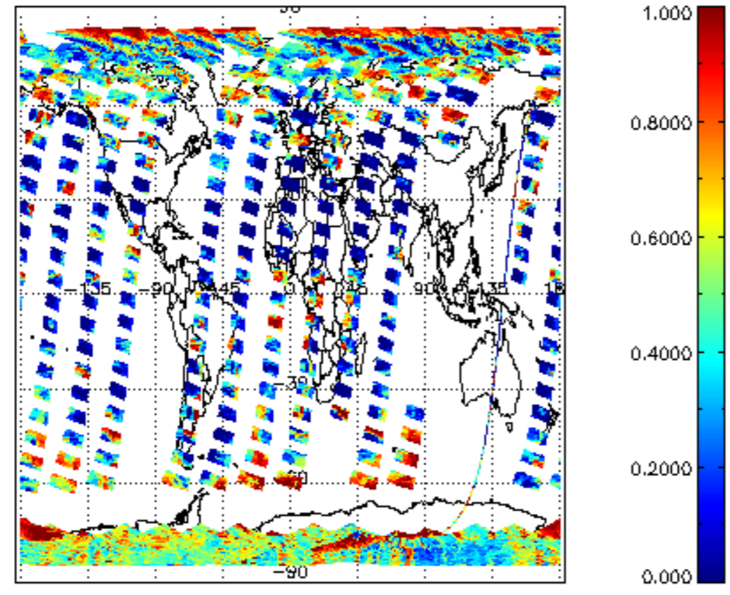
cl_frac for 12OCT2011 00:00:00 to 13OCT2011 00:00:00
