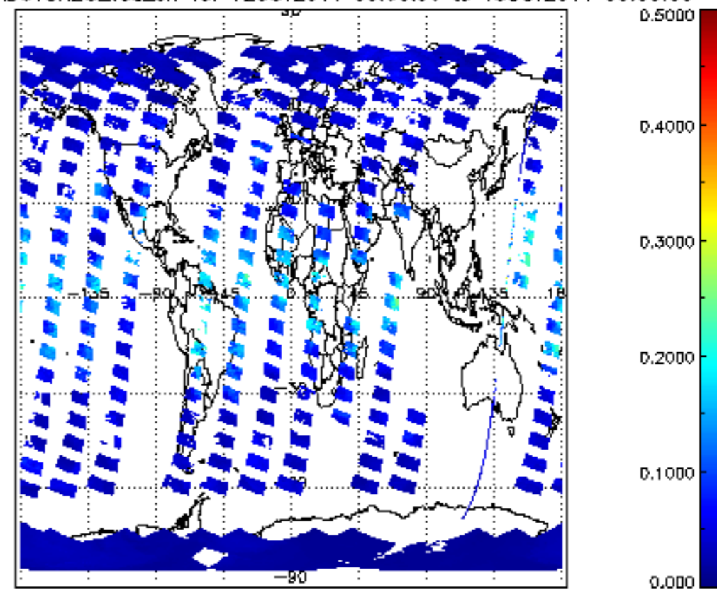
SCIOL2P_NADUV8H20_vcd_err for 12OCT2011 00:00:00 to 13OCT2011 00:00:00
