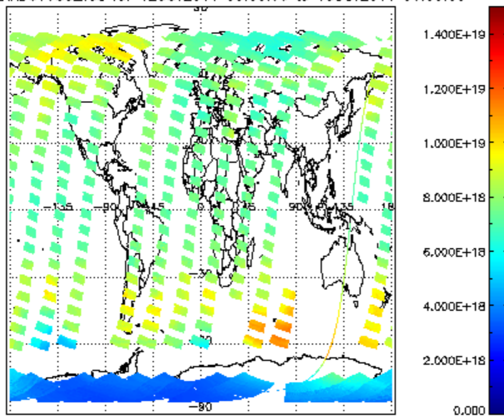
SCIOL2P_NADUV003_vcd for 12OCT2011 00:00:00 to 13OCT2011 00:00:00
