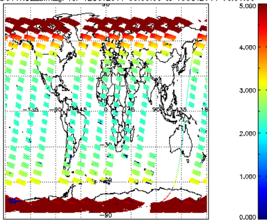
SCIOL2P_NADUV1NO2_amf_gr for 12OCT2011 00:00:00 to 13OCT2011 00:00:00
