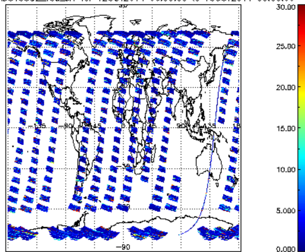
SCIOL2P_NADUV5S02_vcd_err for 12OCT2011 00:00:00 to 13OCT2011 00:00:00
