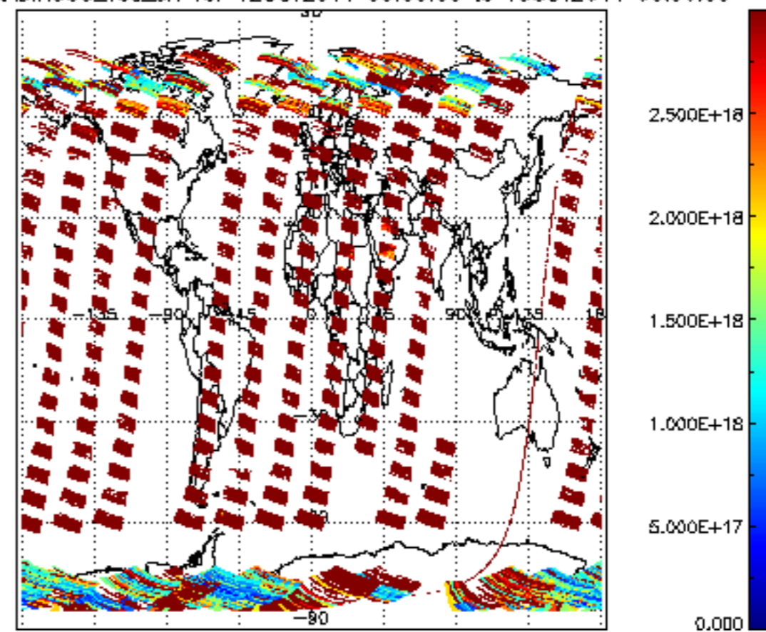
SCIOL2P_NADIR3CO_vcd_err for 12OCT2011 00:00:00 to 13OCT2011 00:00:00
