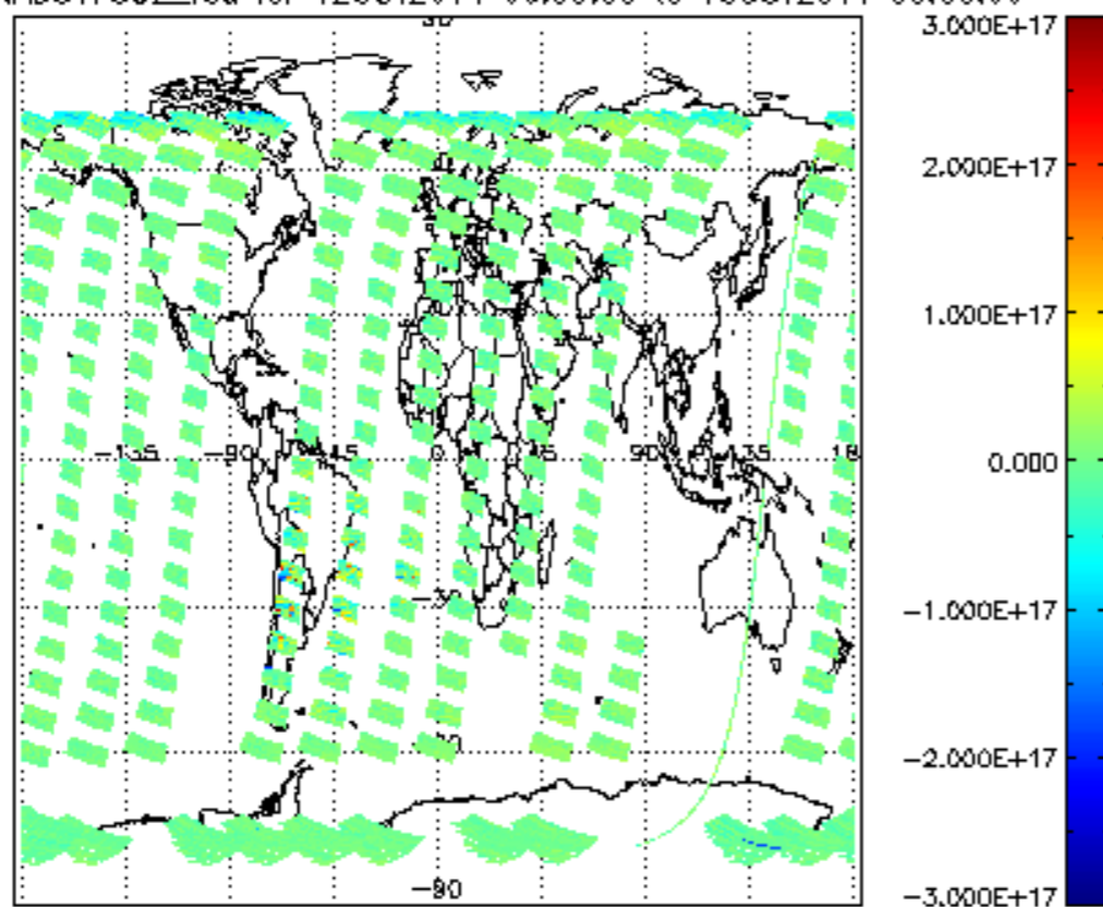
SCIOL2P_NADUV7S02_vcd for 12OCT2011 00:00:00 to 13OCT2011 00:00:00
