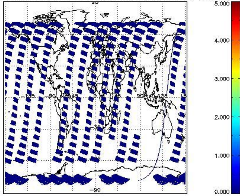
SCIOL2P_NADUV5S02_amf_cl for 12OCT2011 00:00:00 to 13OCT2011 00:00:00
