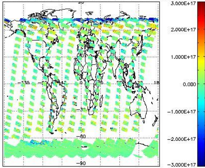
SCIOL2P_NADUV5SO2_vcd for 09OCT2011 00:00:00 to 10OCT2011 00:00:00
