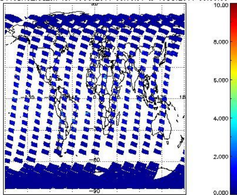
SCIOL2P_NADUV3BRO_vcd_err for 09OCT2011 00:00:00 to 10OCT2011 00:00:00
