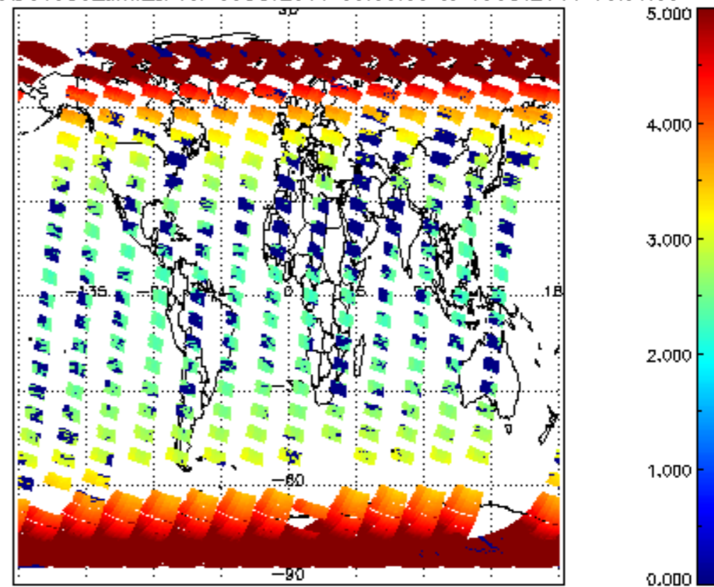
SCIOL2P_NADUV003_amf_cl for 09OCT2011 00:00:00 to 10OCT2011 00:00:00
