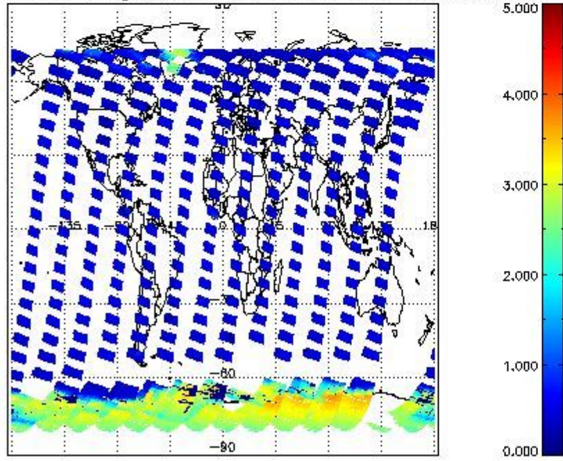
SCIOL2P_NADUV5SO2_amf_gr for 09OCT2011 00:00:00 to 10OCT2011 00:00:00
