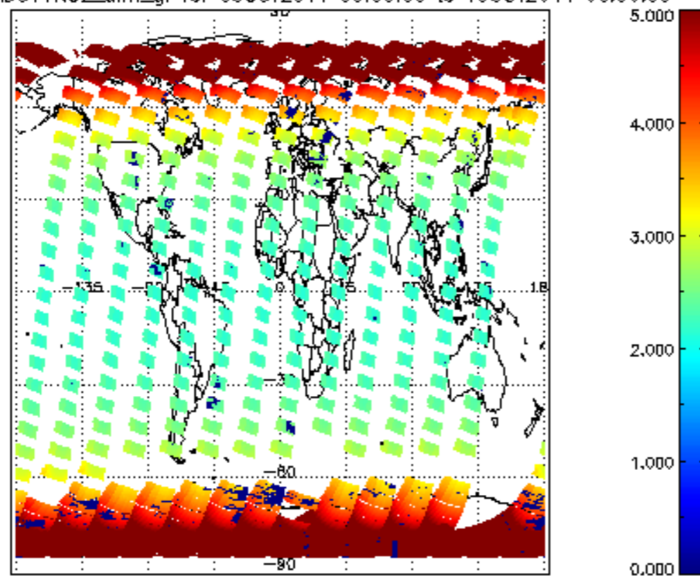
SCIOL2P_NADUV1NO2_amf_gr for 09OCT2011 00:00:00 to 10OCT2011 00:00:00
