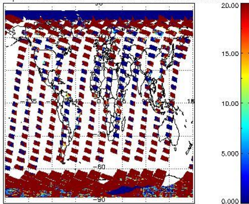
cL_opt_depth for 09OCT2011 00:00:00 to 10OCT2011 00:00:00
