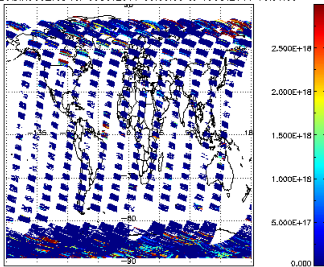
SCIOL2P_NADIR3CO_vcd for 09OCT2011 00:00:00 to 10OCT2011 00:00:00
