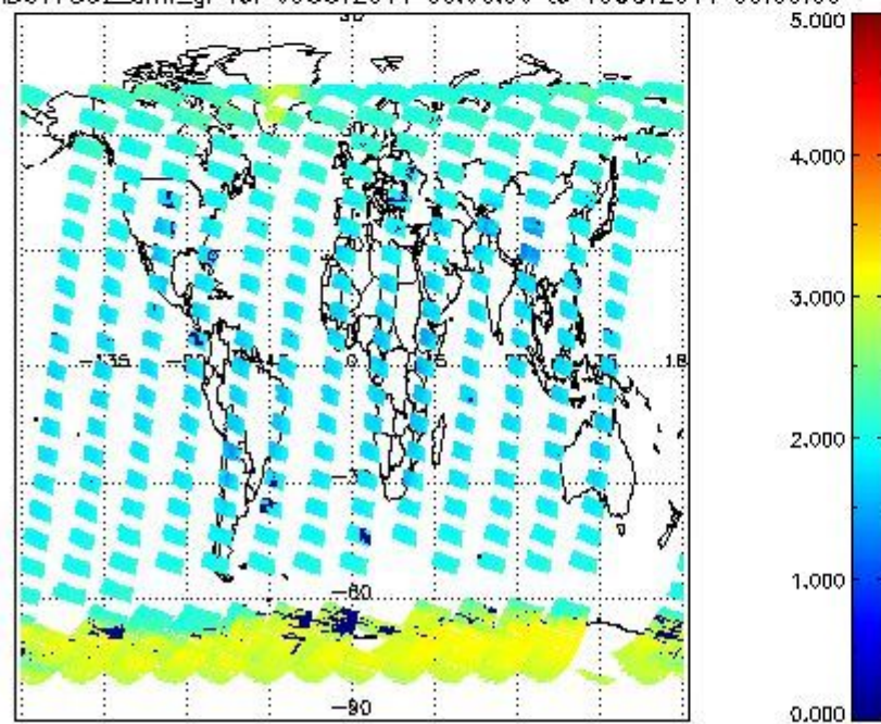
SCIOL2P_NADUV7S02_amf_gr for 09OCT2011 00:00:00 to 10OCT2011 00:00:00
