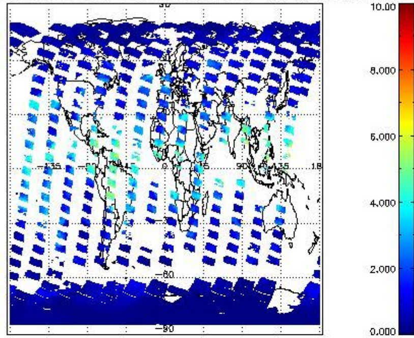
SCIOL2P_NADUV8H20_vcd for 09OCT2011 00:00:00 to 10OCT2011 00:00:00
