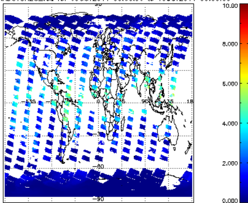
SCIOL2P_NADUV8H20_vcd for 09OCT2011 00:00:00 to 10OCT2011 00:00:00
