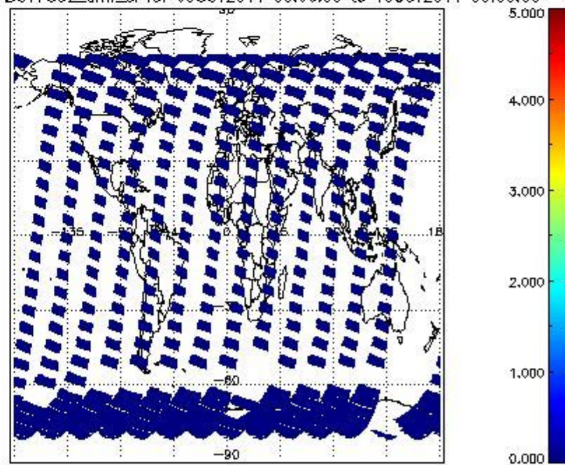
SCIOL2P_NADUV7S02_amf_cl for 09OCT2011 00:00:00 to 10OCT2011 00:00:00
