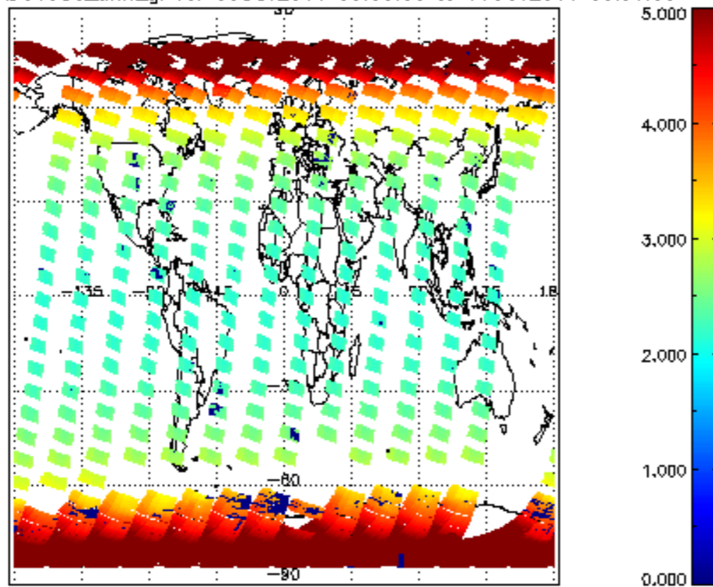
SCIOL2P_NADUV003_amf_gr for 09OCT2011 00:00:00 to 10OCT2011 00:00:00
