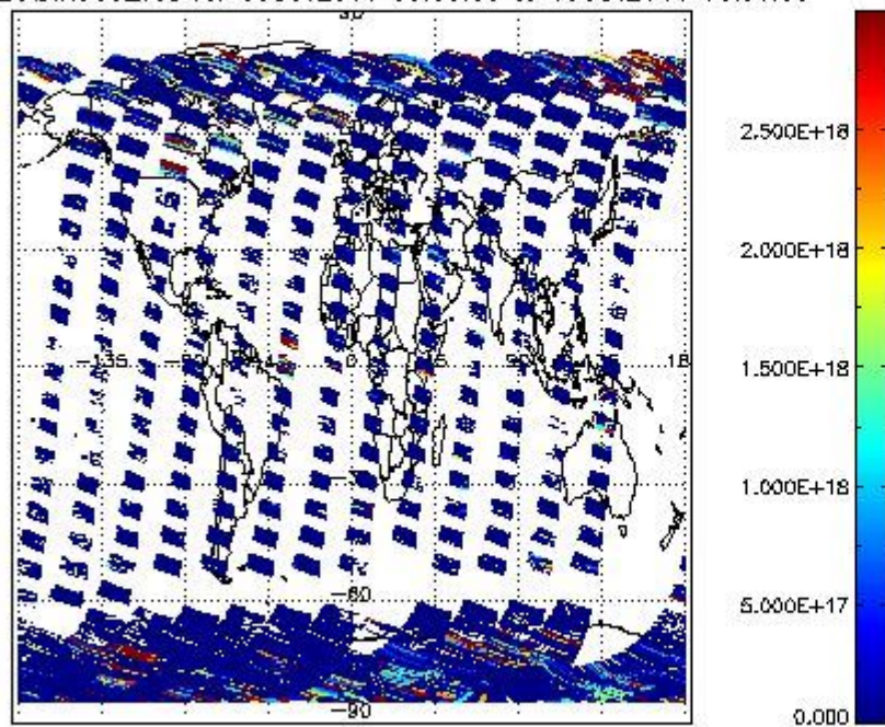
SCIDL2P_NADIR3CO_vcd for 09OCT2011 00:00:00 to 10OCT2011 00:00:00
