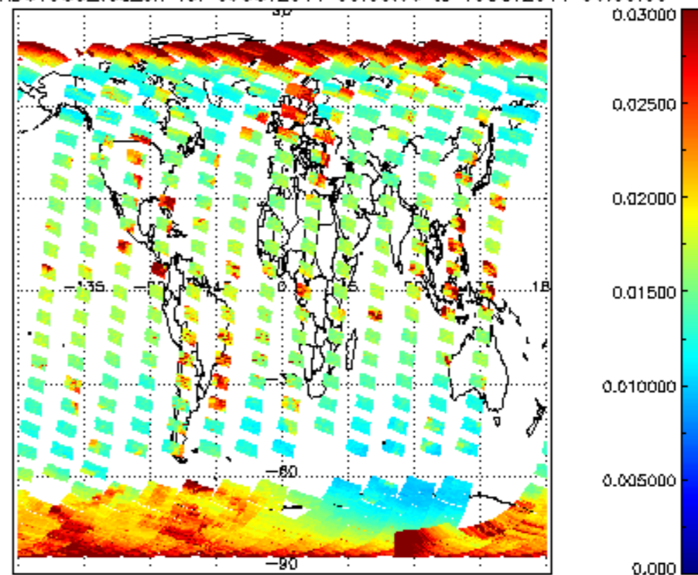
SCIOL2P_NADUV003_vcd_err for 09OCT2011 00:00:00 to 10OCT2011 00:00:00
