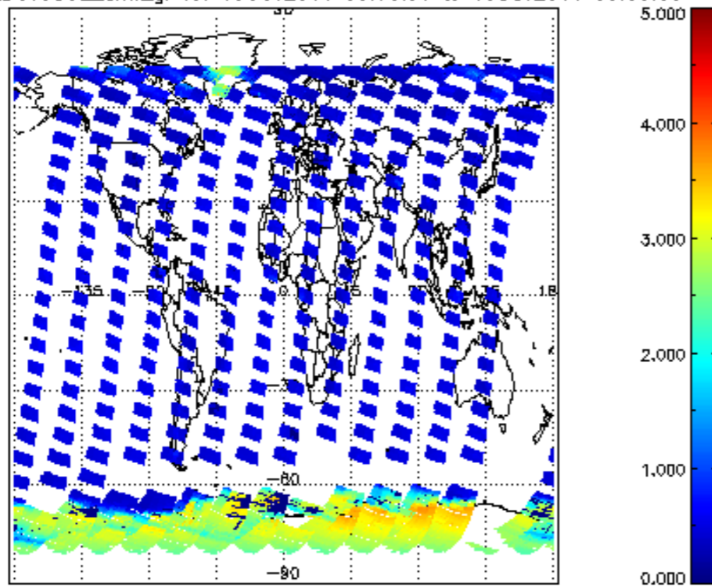
SCIOL2P_NADUV5S02_amf_gr for 09OCT2011 00:00:00 to 10OCT2011 00:00:00
