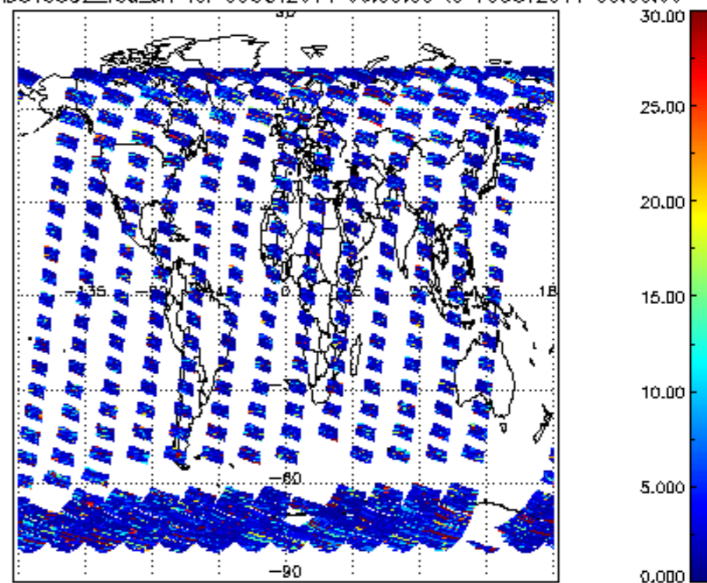
SCIOL2P_NADUV5S02_vcd_err for 09OCT2011 00:00:00 to 10OCT2011 00:00:00
