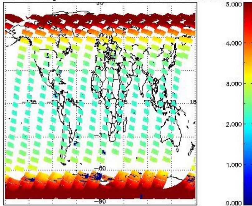
SCIOL2P_NADUV003_amf_gr for 09OCT2011 00:00:00 to 10OCT2011 00:00:00
