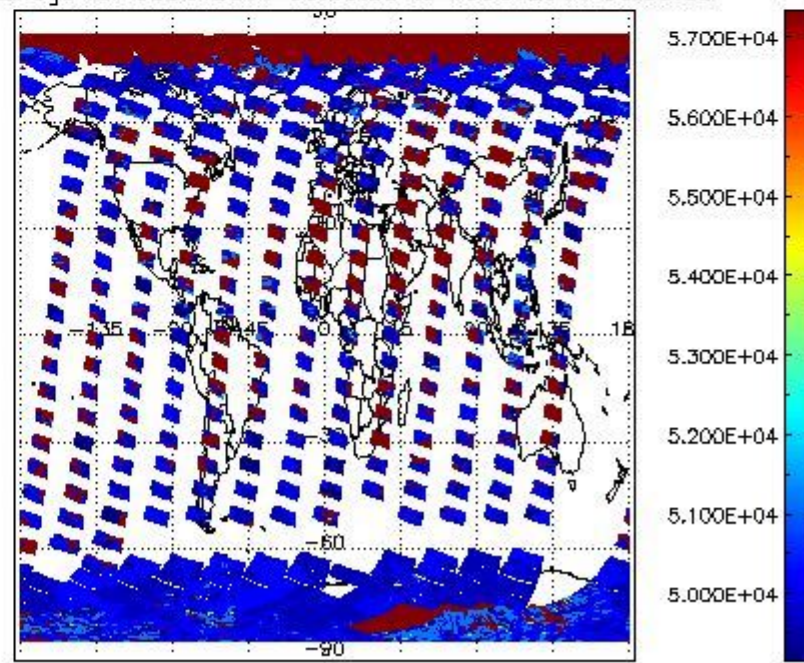
cloud_flags for 09OCT2011 00:00:00 to 10OCT2011 00:00:00
