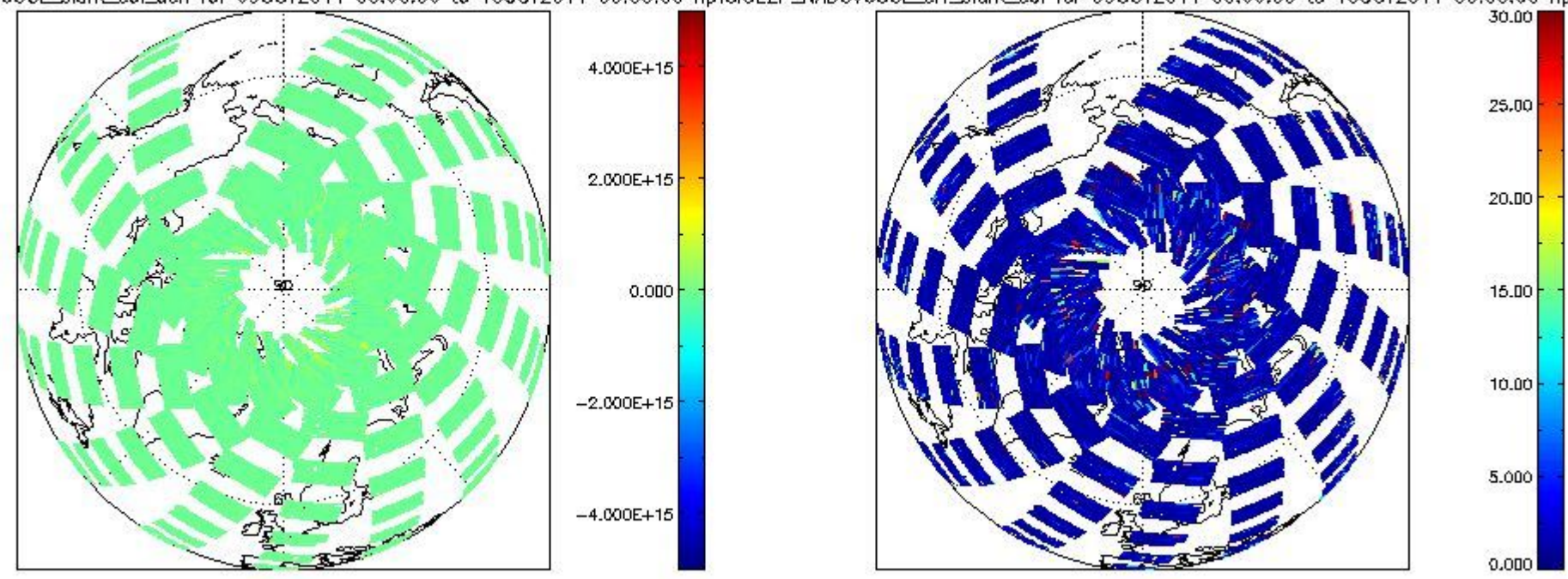
CIOL2P_NADUV60CL_slant_col_den for 09OCT2011 00:00:00 to 10OCT2011 00:00:00 np CIOL2P_NADUV60CL_err_slant_col for 09OCT2011 00:00:00 to 10OCT2011 00:00:00 np
