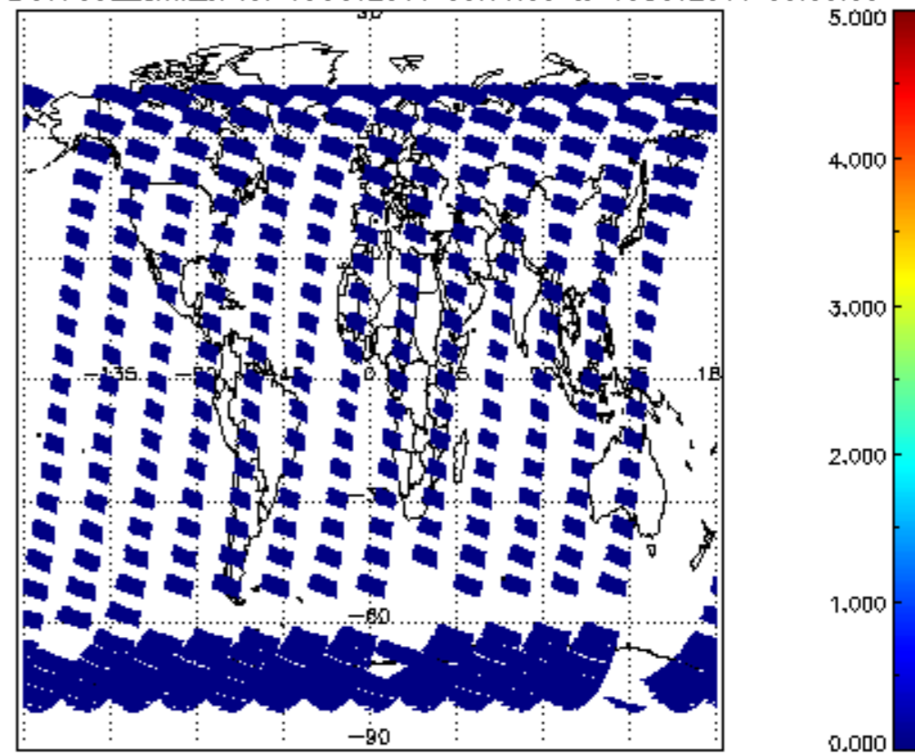
SCIOL2P_NADUV7S02_amf_cl for 09OCT2011 00:00:00 to 10OCT2011 00:00:00
