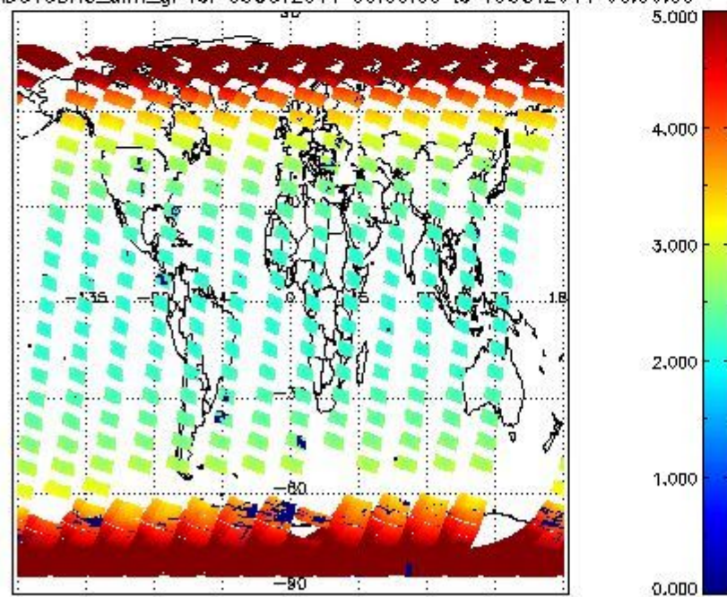
SCIOL2P_NADUV3BRO_amf_gr for 09OCT2011 00:00:00 to 10OCT2011 00:00:00
