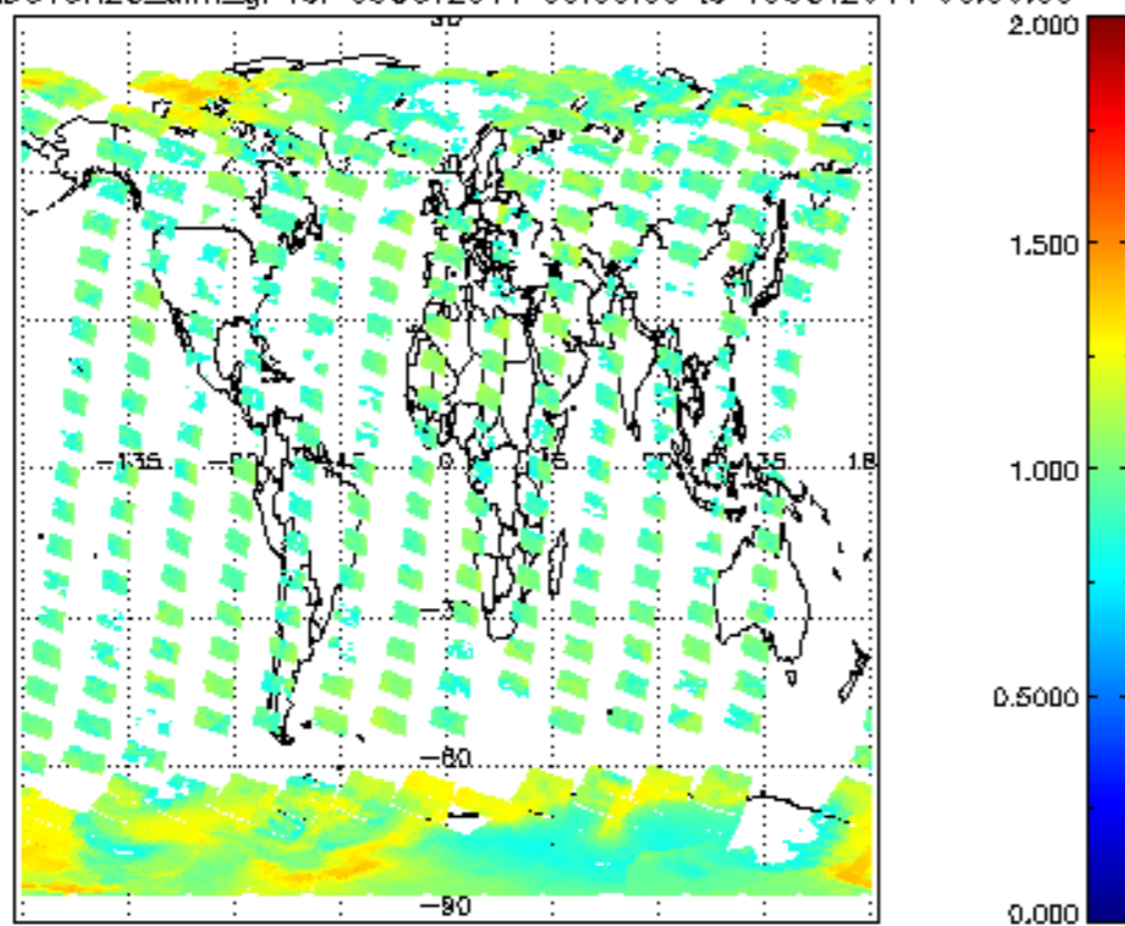
SCIOL2P_NADUV8H20_amf_gr for 09OCT2011 00:00:00 to 10OCT2011 00:00:00
