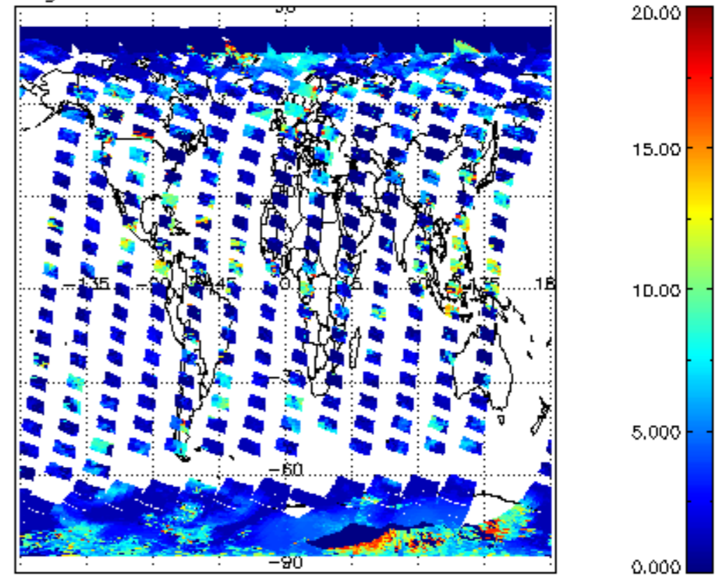
cl_top_height for 09OCT2011 00:00:00 to 10OCT2011 00:00:00
