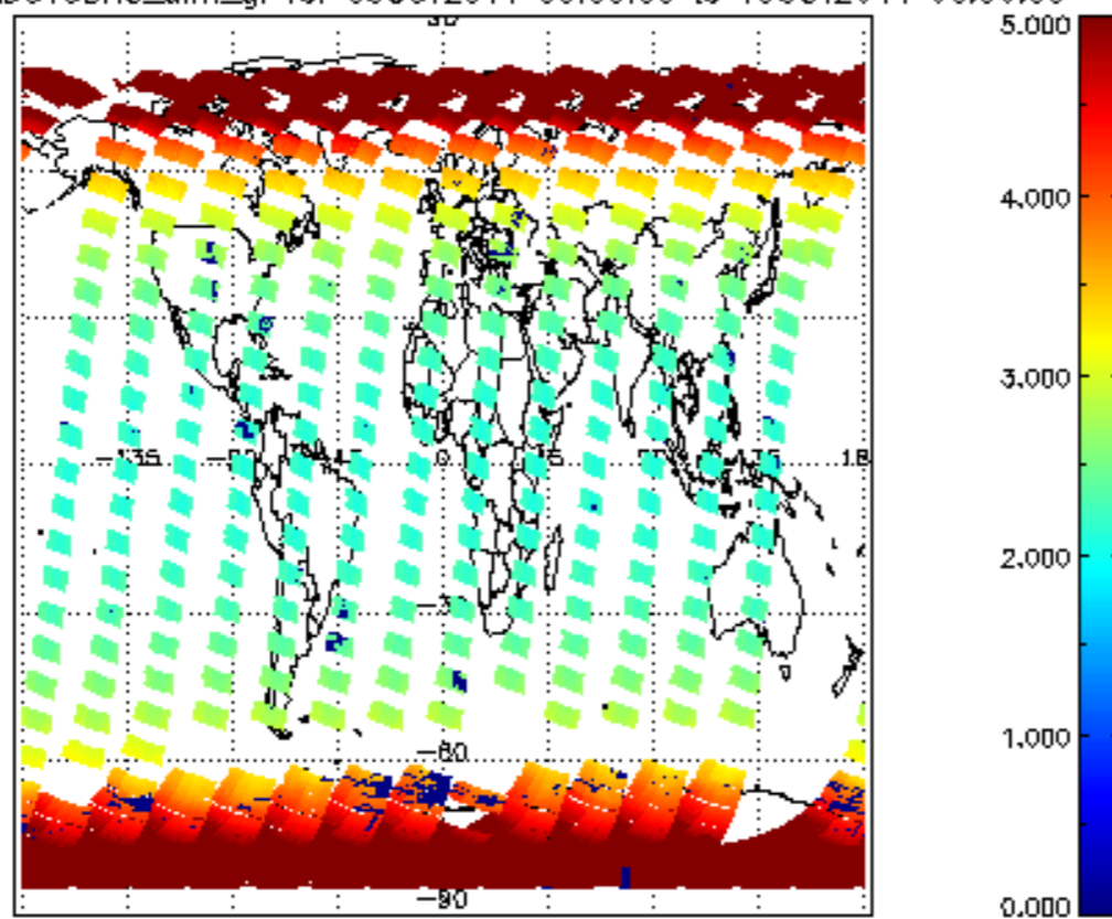
SCIOL2P_NADUV3BRO_amf_gr for 09OCT2011 00:00:00 to 10OCT2011 00:00:00
