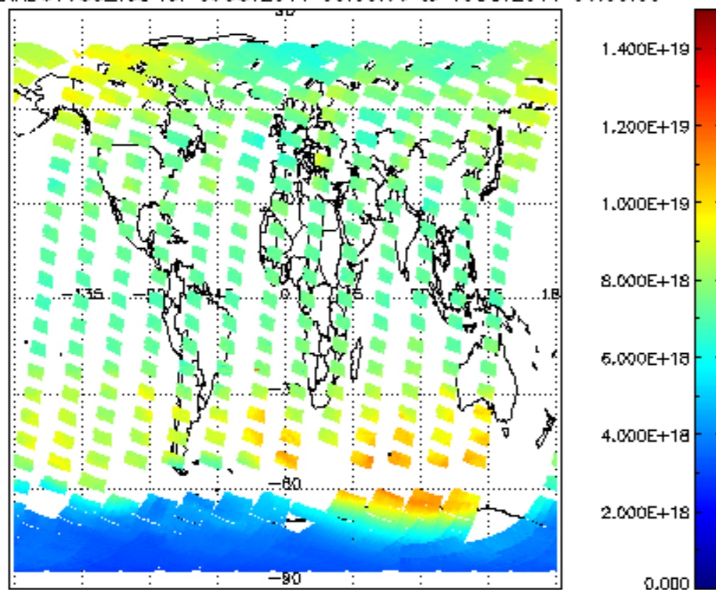
SCIOL2P_NADUV003_vcd for 09OCT2011 00:00:00 to 10OCT2011 00:00:00
