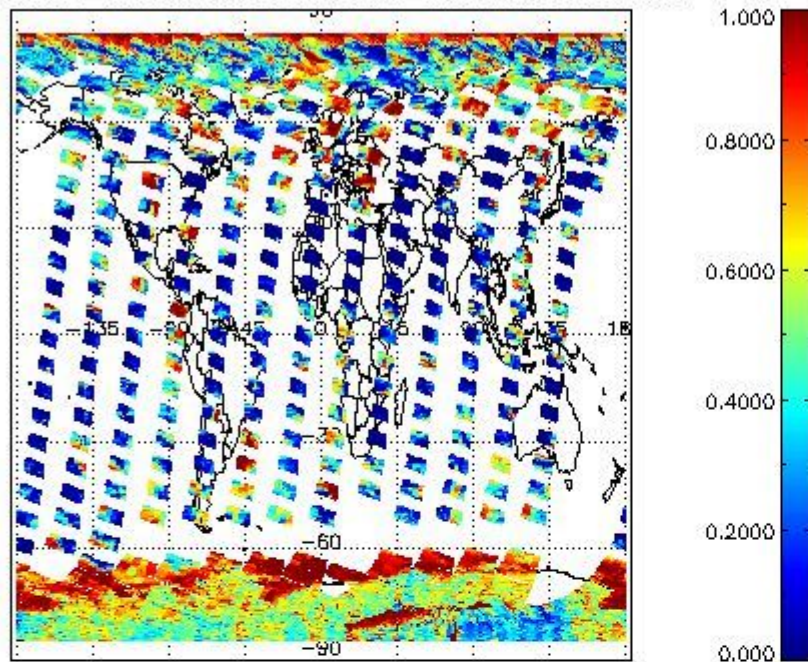
cLfrac for 09OCT2011 00:00:00 to 10OCT2011 00:00:00
