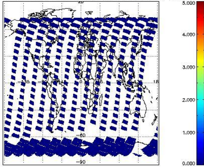
SCIOL2P_NADUV5SO2_amf_cl for 09OCT2011 00:00:00 to 10OCT2011 00:00:00
