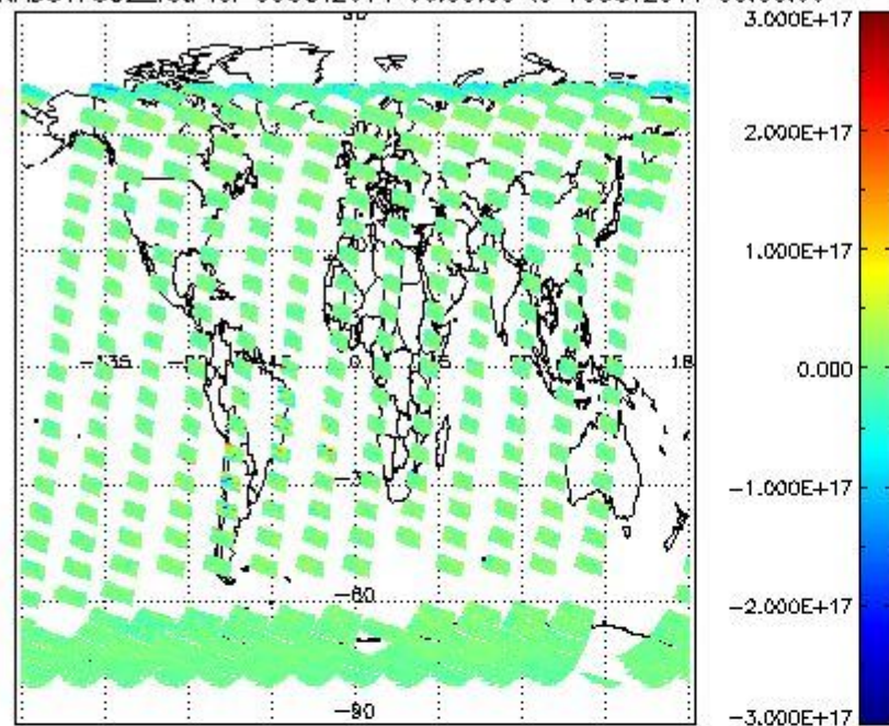
SCIOL2P_NADUV7S02_vcd for 09OCT2011 00:00:00 to 10OCT2011 00:00:00
