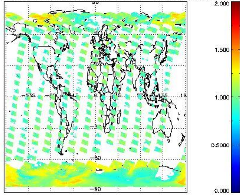
SCIOL2P_NADUV8H20_amf_gr for 09OCT2011 00:00:00 to 10OCT2011 00:00:00
