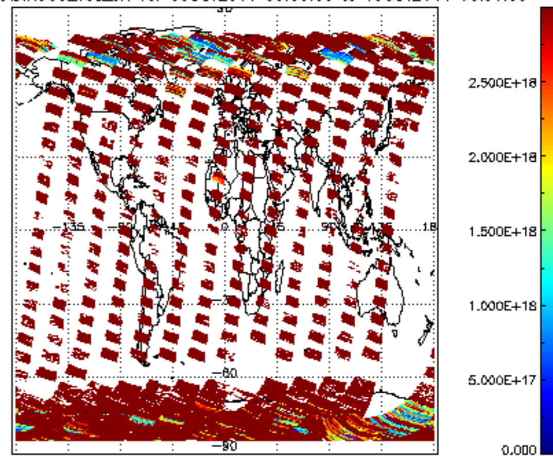
SCIOL2P_NADIR3CO_vcd_err for 09OCT2011 00:00:00 to 10OCT2011 00:00:00
