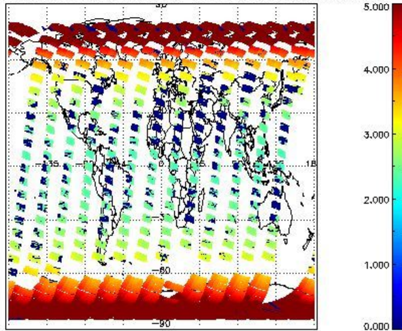
SCIOL2P_NADUV003_amf_cl for 09OCT2011 00:00:00 to 10OCT2011 00:00:00
