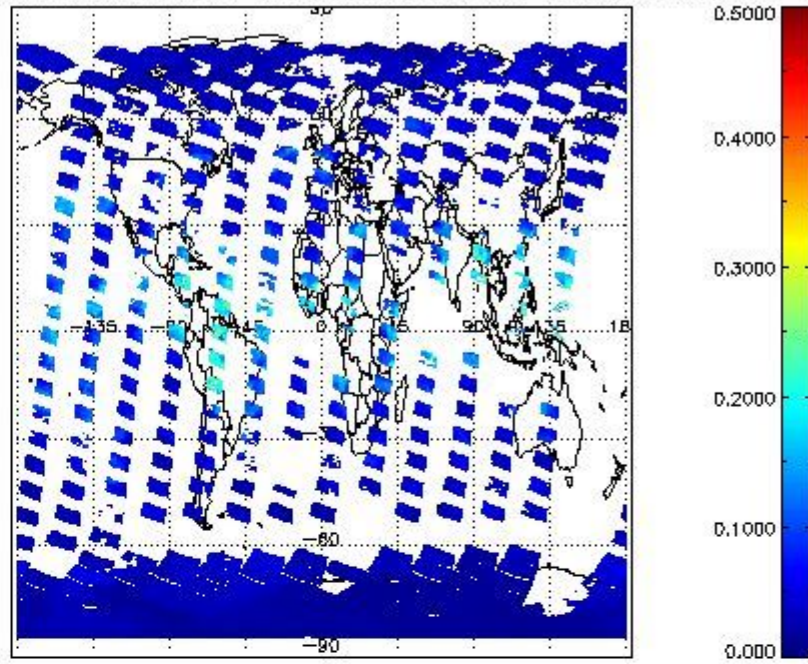
SCIOL2P_NADUV8H20_vcd_err for 09OCT2011 00:00:00 to 10OCT2011 00:00:00
