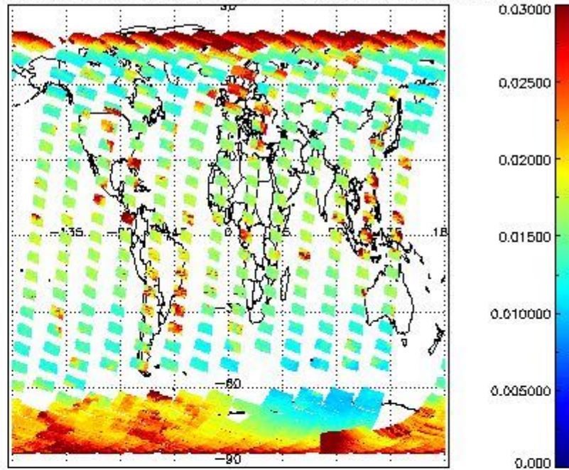
SCIOL2P_NADUV003_vcd_err for 09OCT2011 00:00:00 to 10OCT2011 00:00:00
