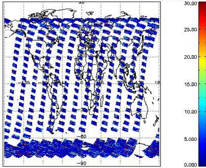
SCIOL2P_NADUV5SO2_vcd_err for 09OCT2011 00:00:00 to 10OCT2011 00:00:00
