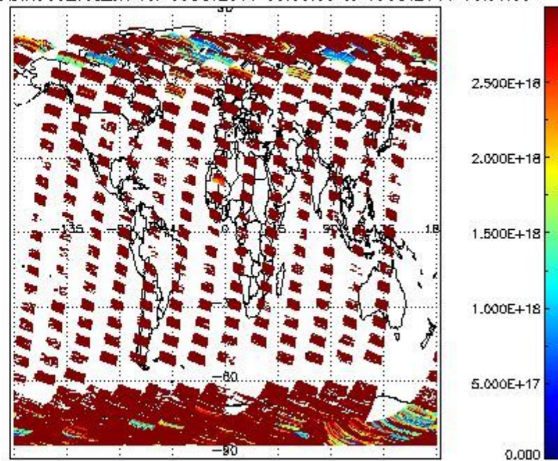
SCIDL2P_NADIR3CO_vcd_err for 09OCT2011 00:00:00 to 10OCT2011 00:00:00
