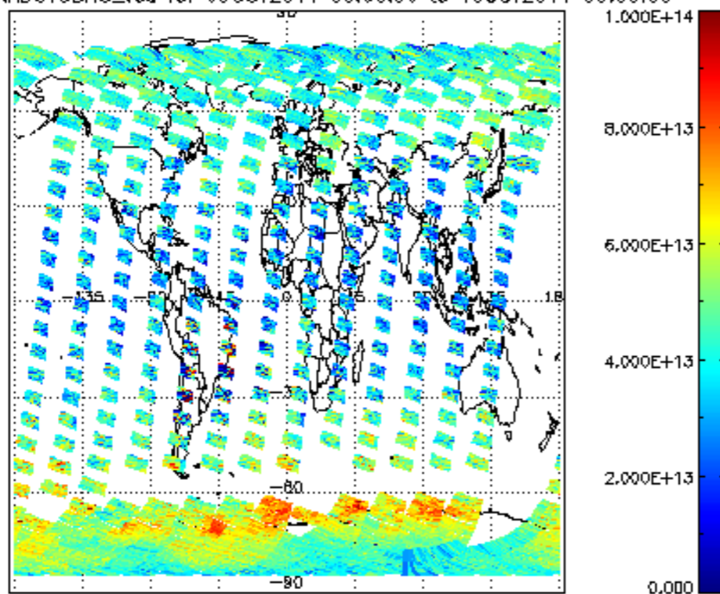
SCIOL2P_NADUV3BRO_vcd for 09OCT2011 00:00:00 to 10OCT2011 00:00:00
