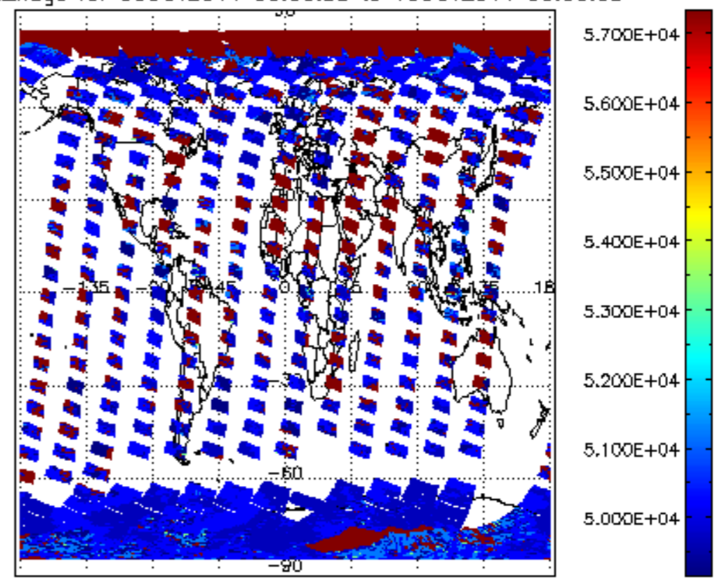
cloud_flags for 09OCT2011 00:00:00 to 10OCT2011 00:00:00
