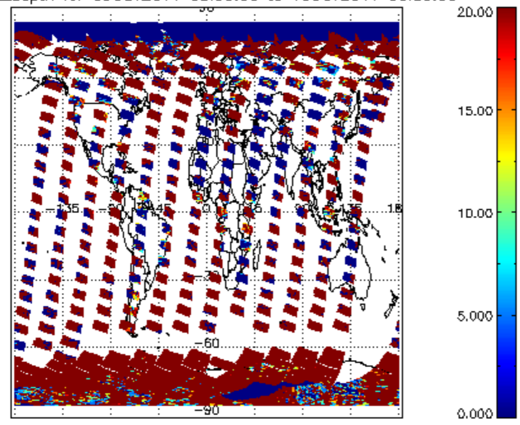
cl_opt_depth for 09OCT2011 00:00:00 to 10OCT2011 00:00:00
