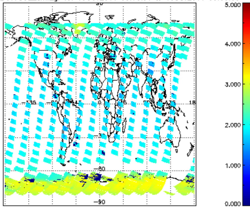
SCIOL2P_NADUV7S02_amf_gr for 09OCT2011 00:00:00 to 10OCT2011 00:00:00
