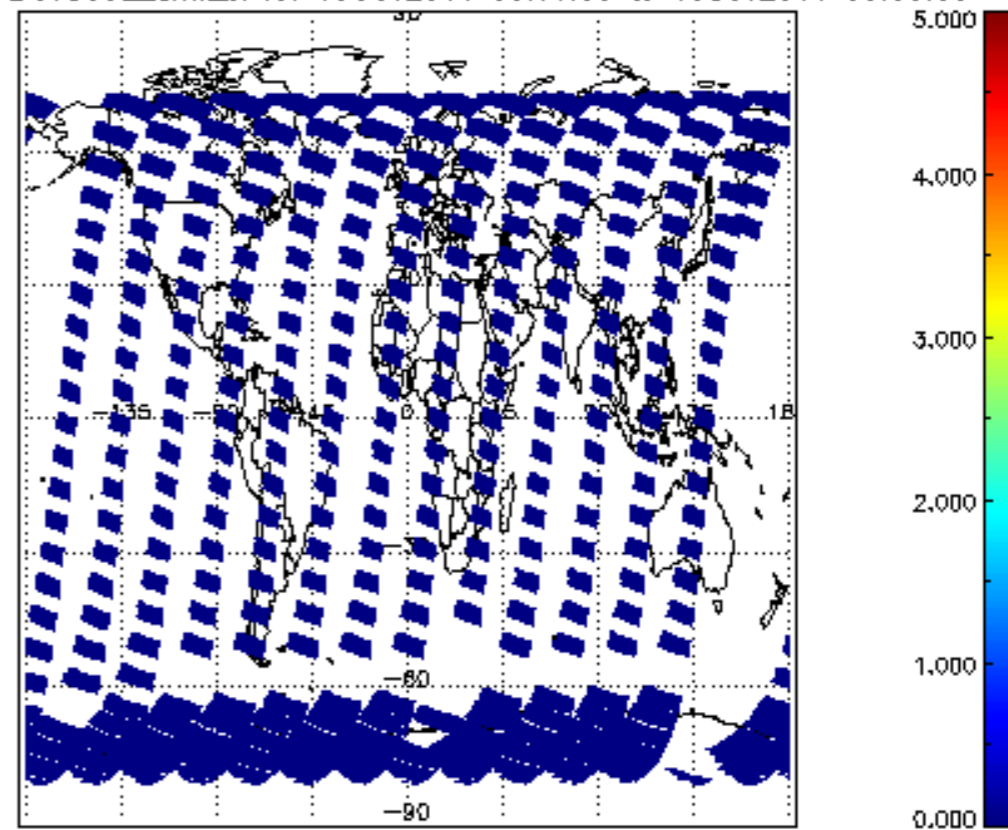
SCIOL2P_NADUV5S02_amf_cl for 09OCT2011 00:00:00 to 10OCT2011 00:00:00
