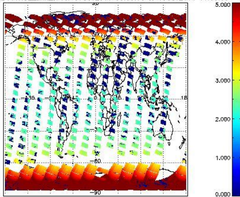
SCIOL2P_NADUV1N02_amf_cl for 09OCT2011 00:00:00 to 10OCT2011 00:00:00
