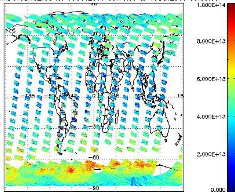
SCIOL2P_NADUV3BRO_vcd for 09OCT2011 00:00:00 to 10OCT2011 00:00:00
