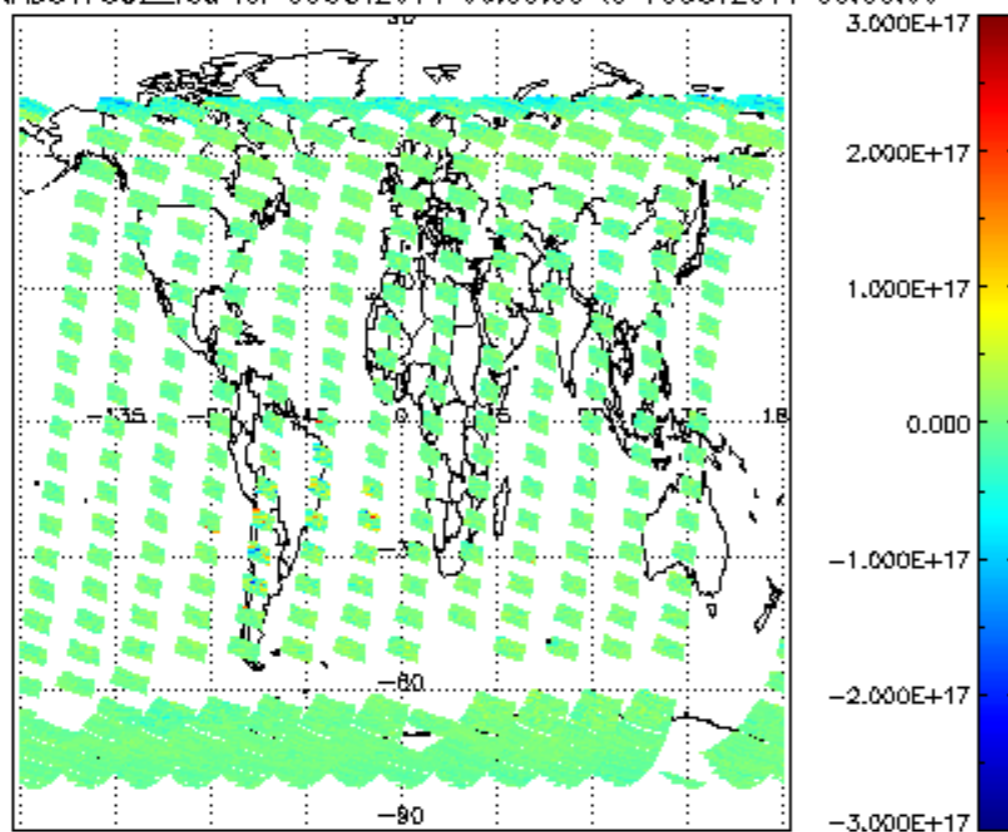
SCIOL2P_NADUV7S02_vcd for 09OCT2011 00:00:00 to 10OCT2011 00:00:00
