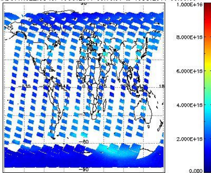
SCIOL2P_NADUV1N02_vcd for 09OCT2011 00:00:00 to 10OCT2011 00:00:00
