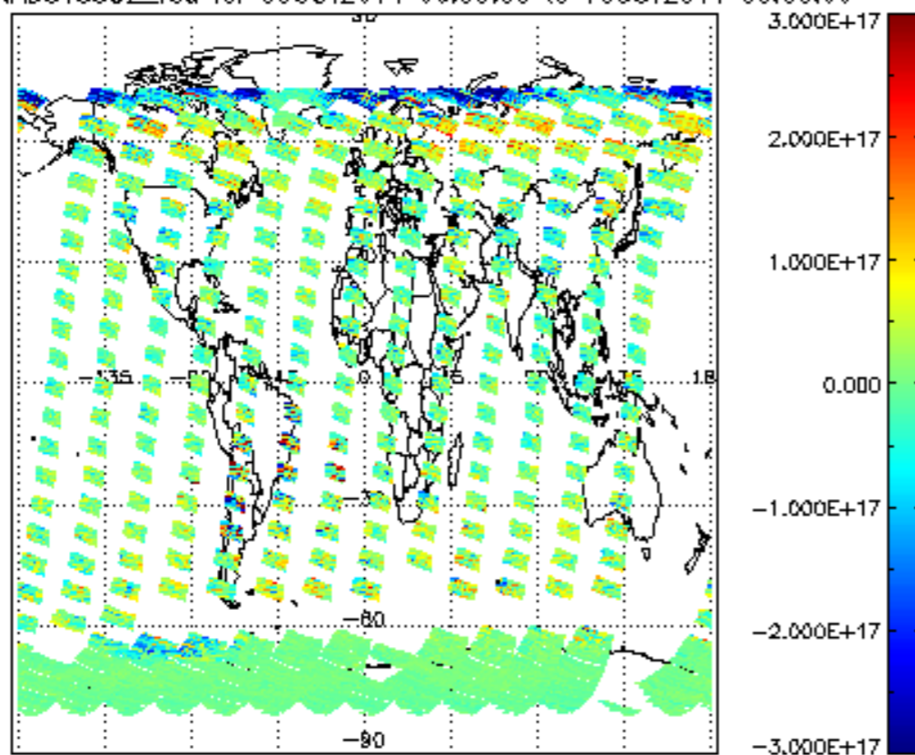
SCIOL2P_NADUV5S02_vcd for 09OCT2011 00:00:00 to 10OCT2011 00:00:00
