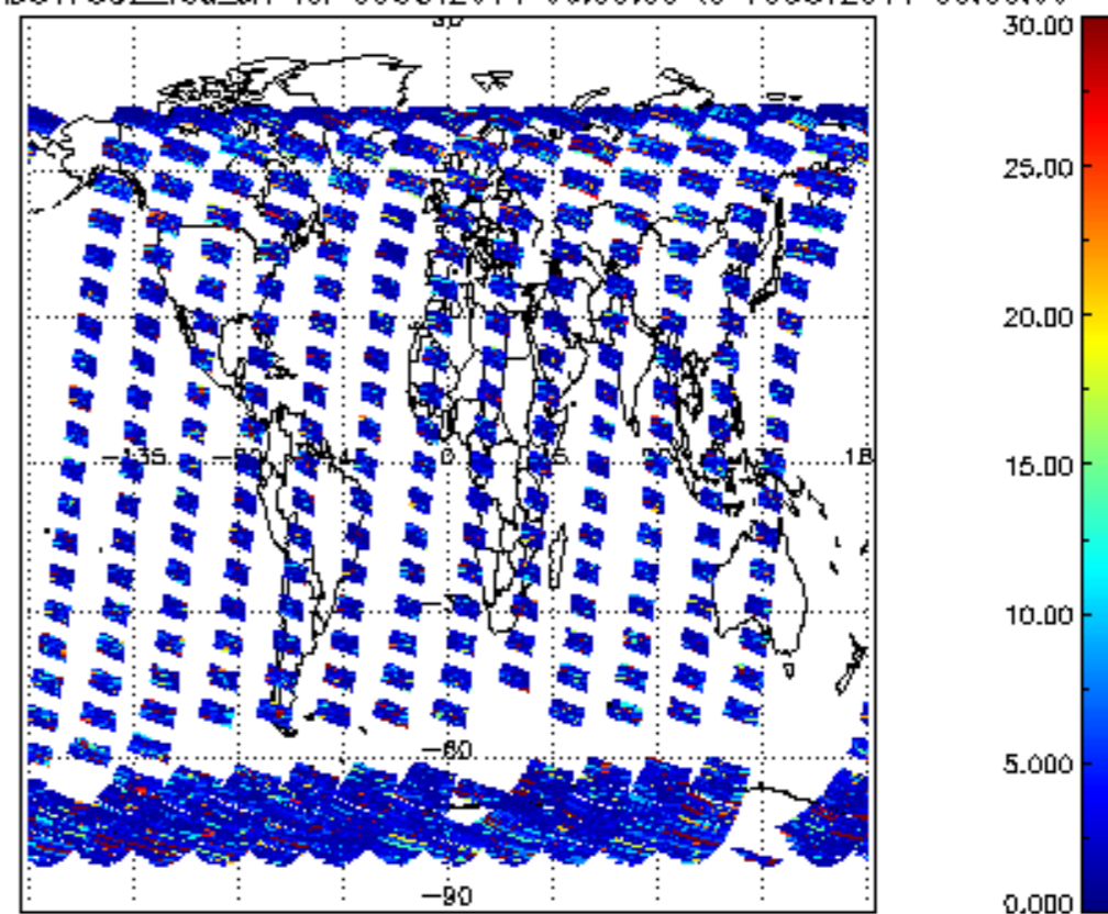
SCIOL2P_NADUV7S02_vcd_err for 09OCT2011 00:00:00 to 10OCT2011 00:00:00
