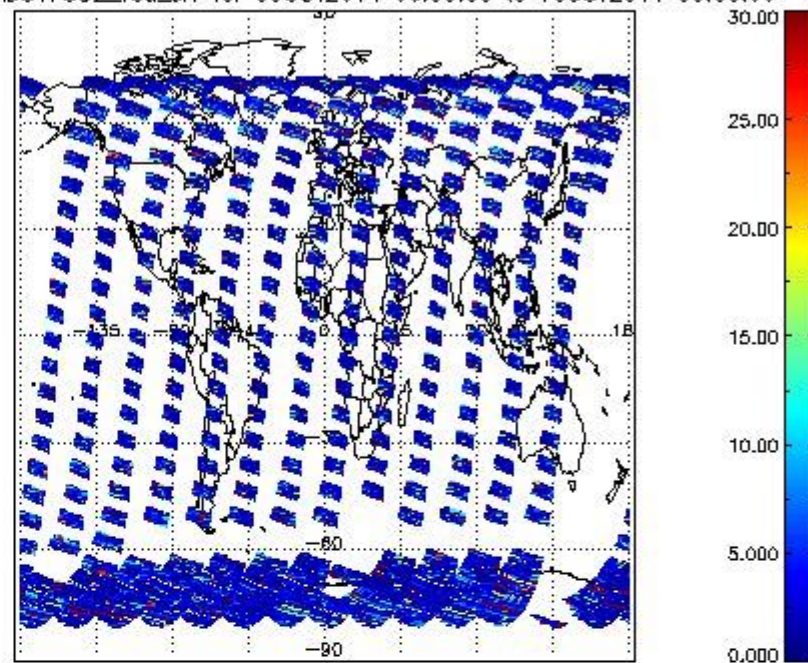
SCIOL2P_NADUV7S02_vcd_err for 09OCT2011 00:00:00 to 10OCT2011 00:00:00
