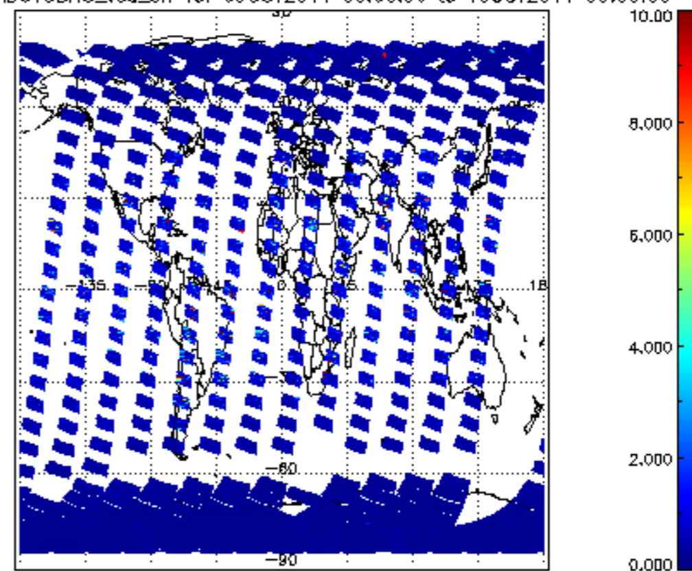
SCIOL2P_NADUV3BRO_vcd_err for 09OCT2011 00:00:00 to 10OCT2011 00:00:00
