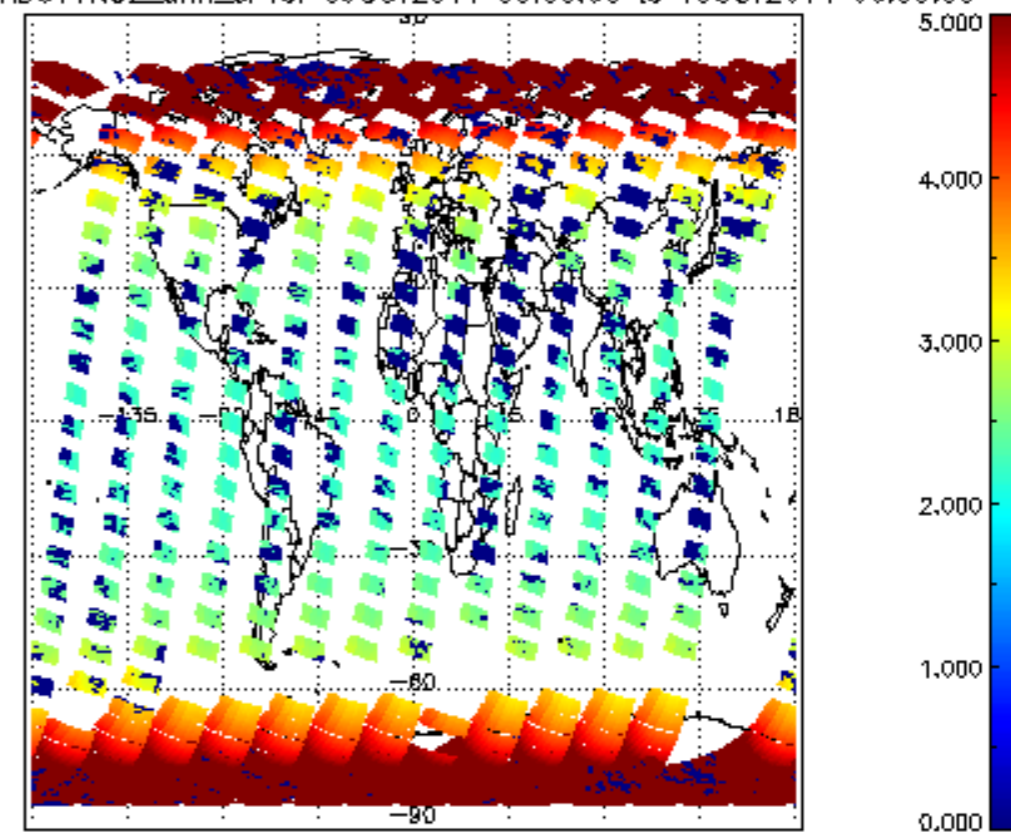
SCIOL2P_NADUV1NO2_amf_cl for 09OCT2011 00:00:00 to 10OCT2011 00:00:00
