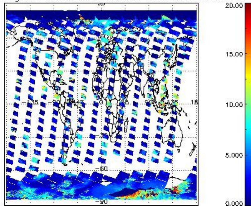
cL_top_height for 09OCT2011 00:00:00 to 10OCT2011 00:00:00
