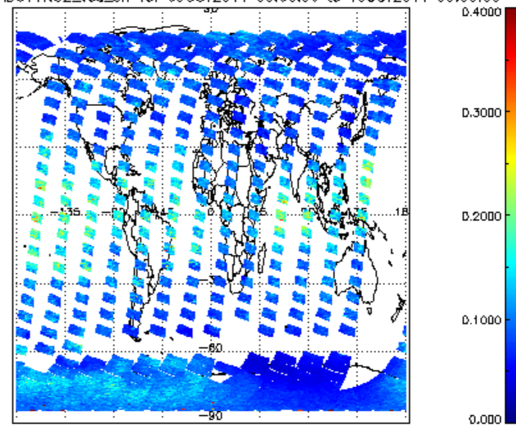
SCIOL2P_NADUV1NO2_vcd_err for 09OCT2011 00:00:00 to 10OCT2011 00:00:00
