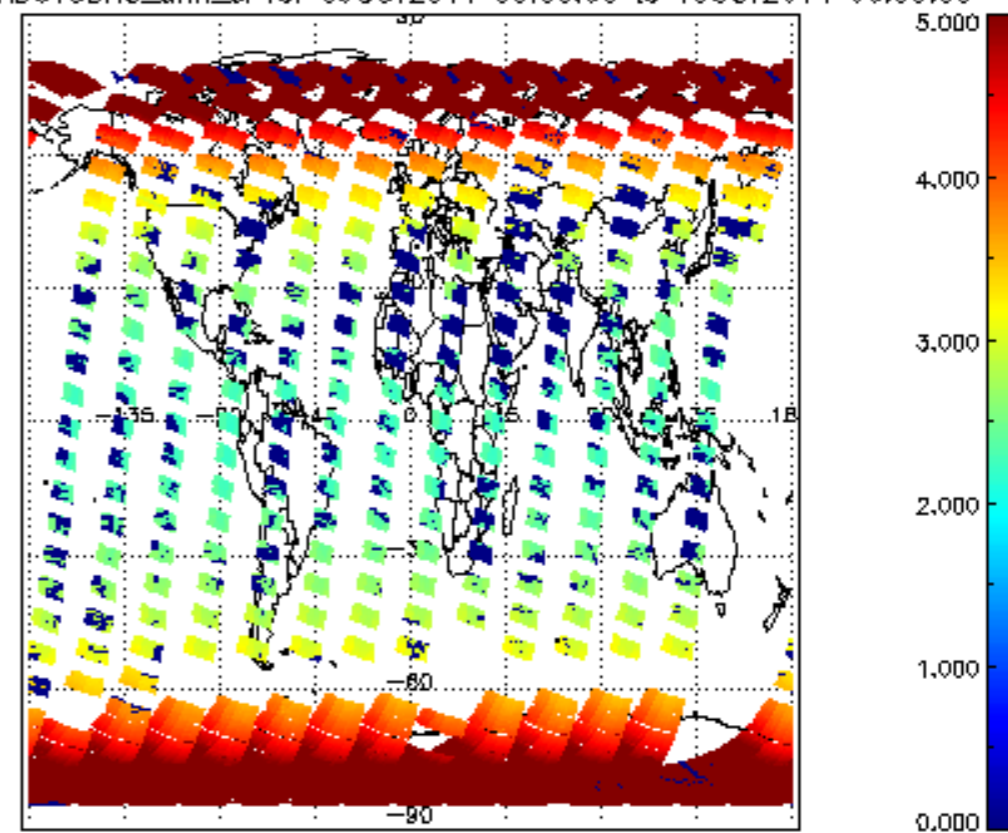
SCIOL2P_NADUV3BRO_amf_cl for 09OCT2011 00:00:00 to 10OCT2011 00:00:00
