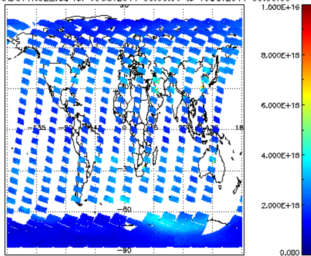
SCIOL2P_NADUV1NO2_vcd for 09OCT2011 00:00:00 to 10OCT2011 00:00:00
