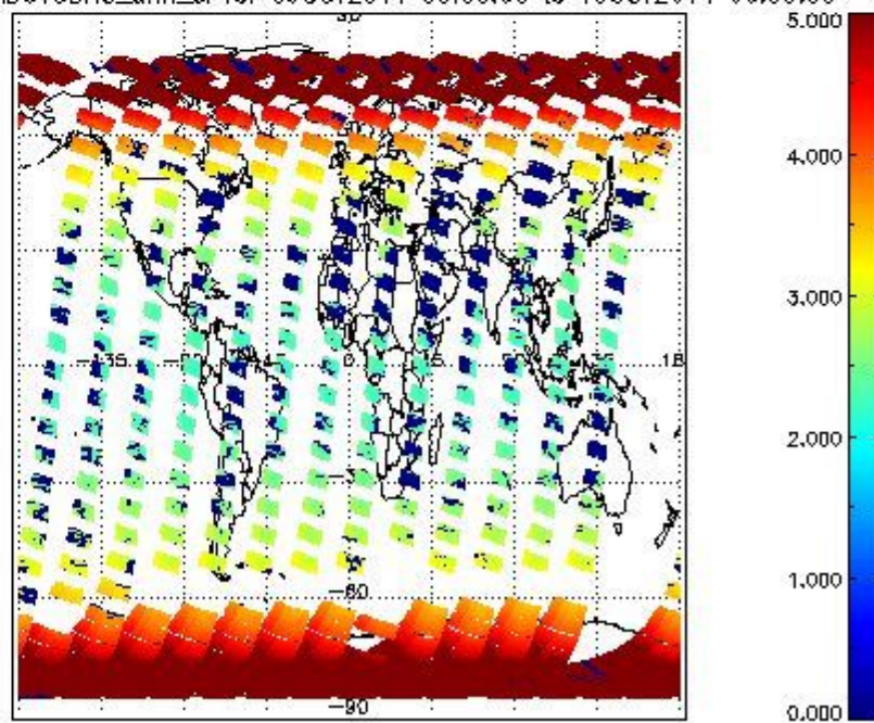
SCIOL2P_NADUV3BRO_amf_cl for 09OCT2011 00:00:00 to 10OCT2011 00:00:00
