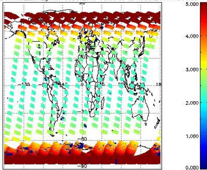
SCIOL2P_NADUV1N02_amf_gr for 09OCT2011 00:00:00 to 10OCT2011 00:00:00
