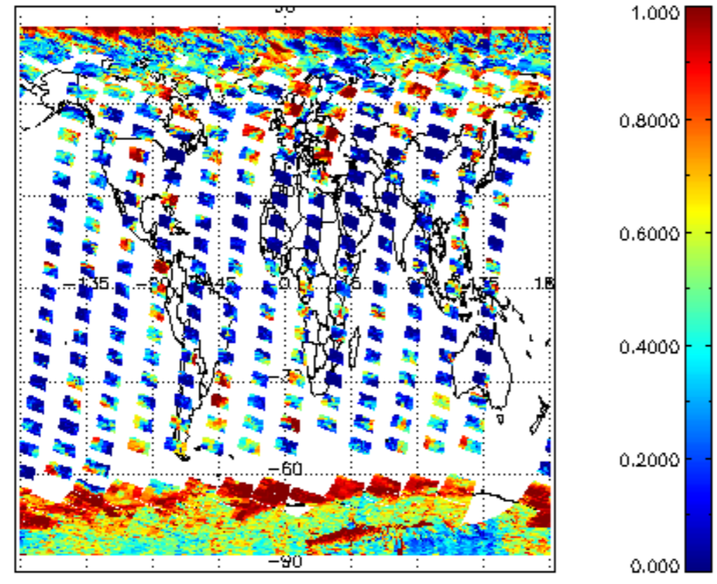
cl_frac for 09OCT2011 00:00:00 to 10OCT2011 00:00:00
