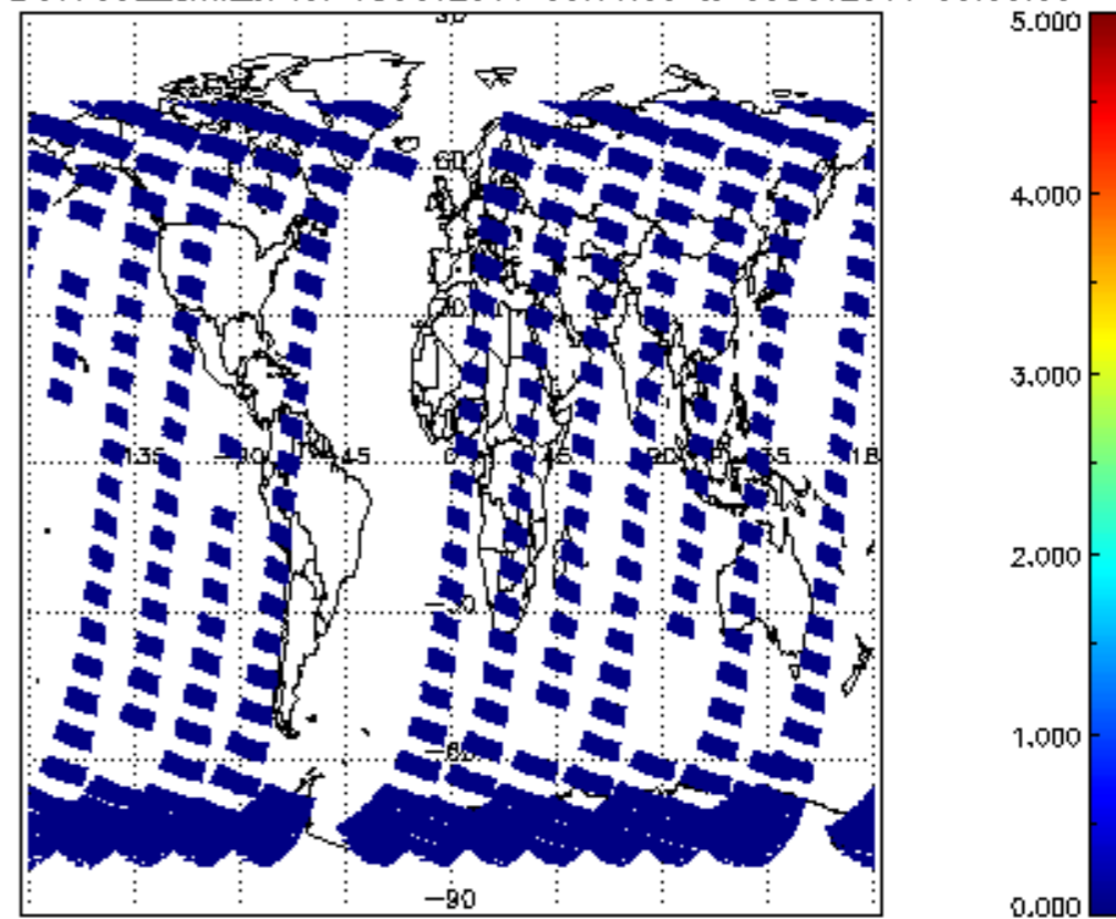
SCIOL2P_NADUV7S02_amf_cl for 08OCT2011 00:00:00 to 09OCT2011 00:00:00
