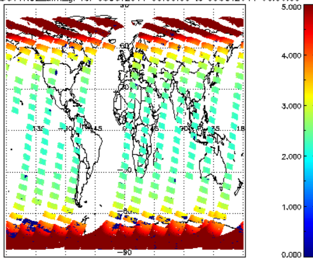
SCIOL2P_NADUV1NO2_amf_gr for 08OCT2011 00:00:00 to 09OCT2011 00:00:00
