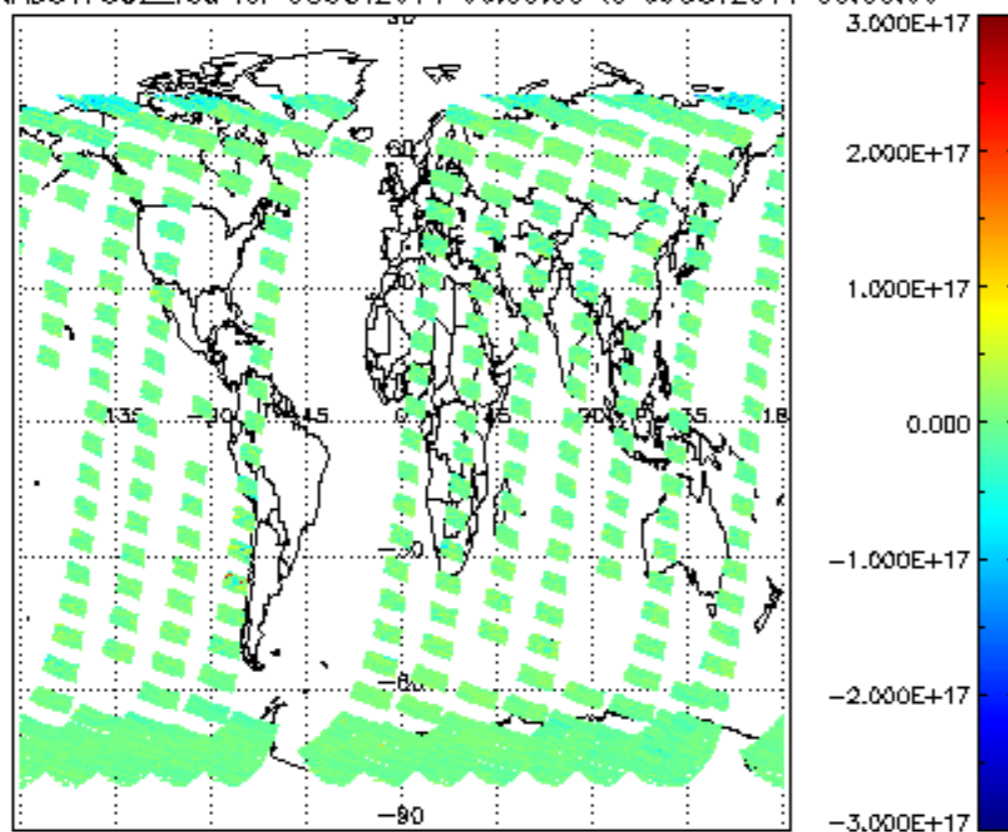
SCIOL2P_NADUV7S02_vcd for 08OCT2011 00:00:00 to 09OCT2011 00:00:00
