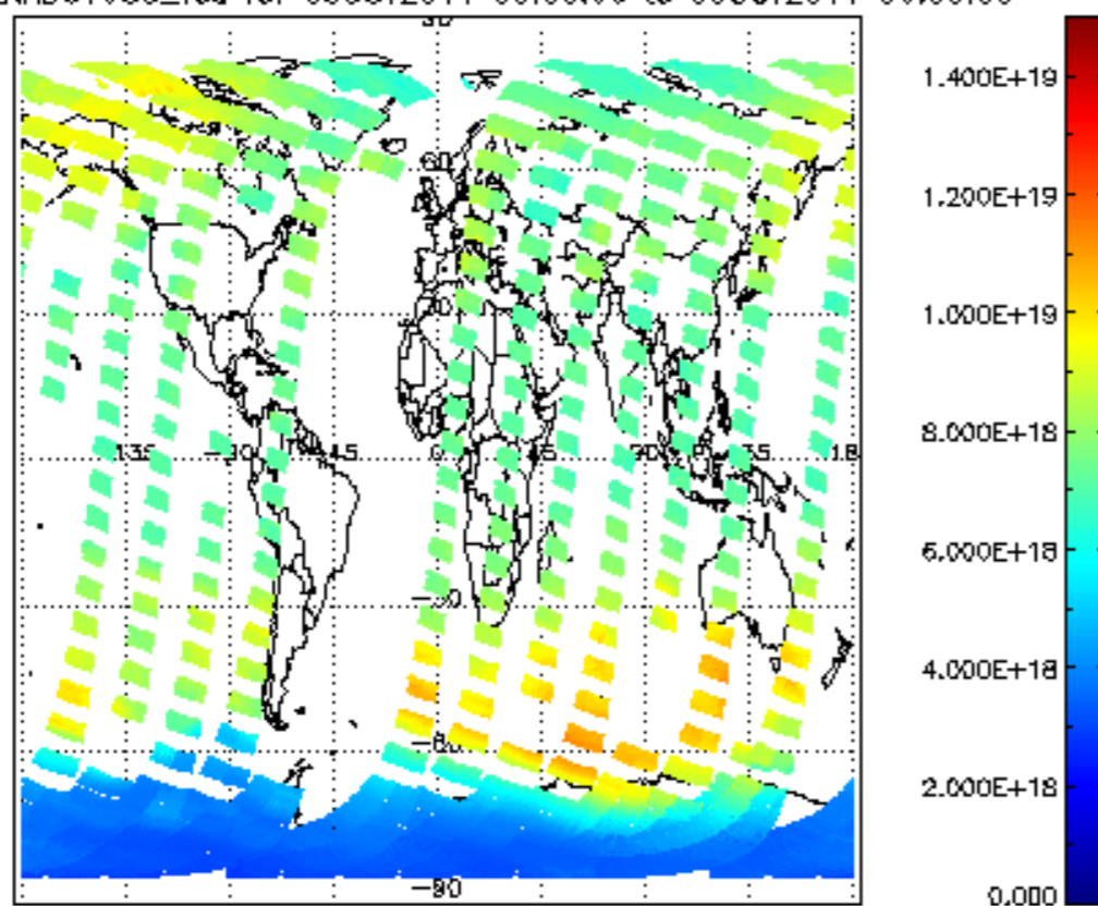
SCIOL2P_NADUV003_vcd for 08OCT2011 00:00:00 to 09OCT2011 00:00:00
