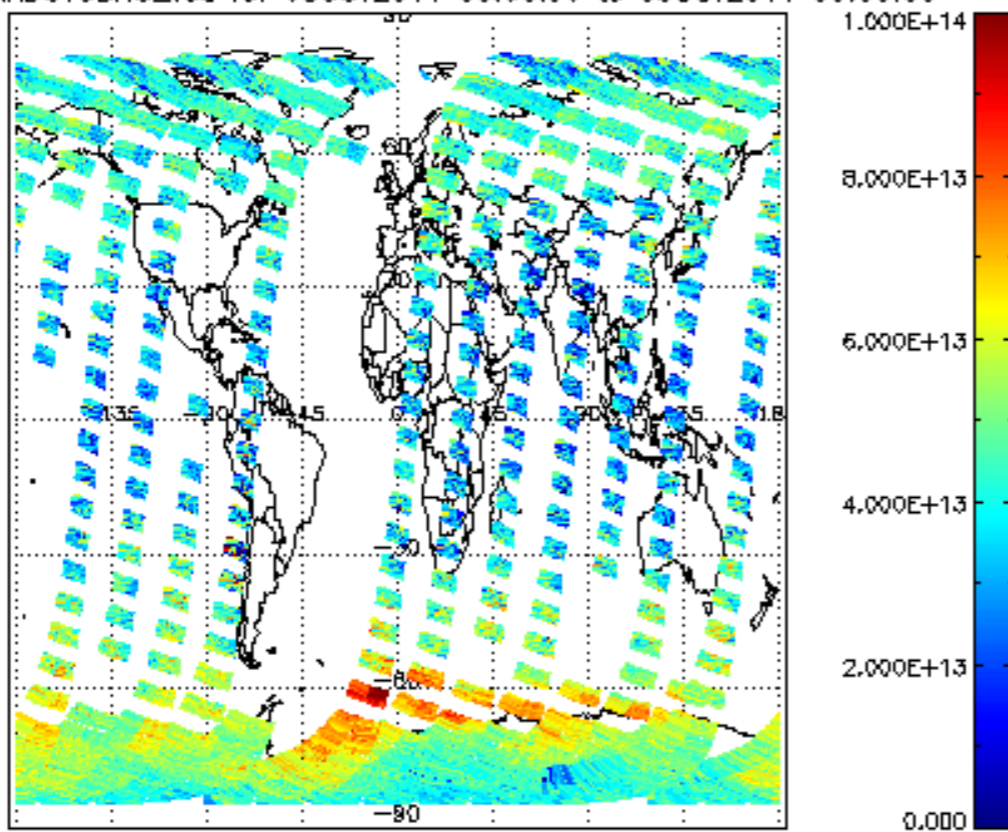
SCIOL2P_NADUV3BRO_vcd for 08OCT2011 00:00:00 to 09OCT2011 00:00:00
