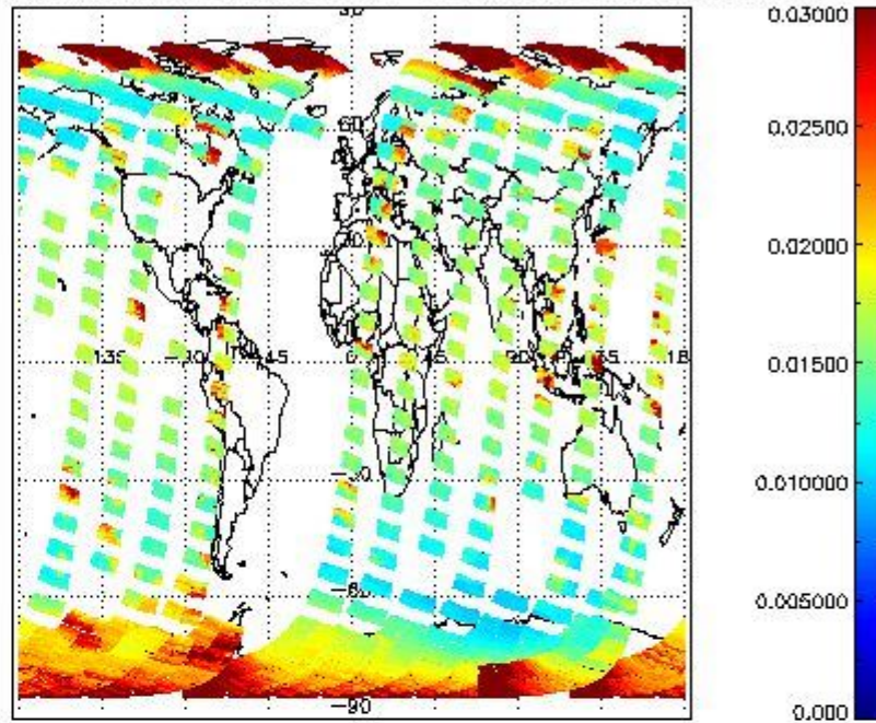
SCIOL2P_NADUV003_vcd_err for 08OCT2011 00:00:00 to 09OCT2011 00:00:00
