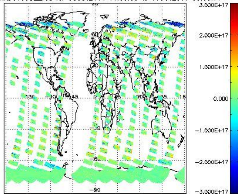
SCIOL2P_NADUV5S02_vcd for 08OCT2011 00:00:00 to 09OCT2011 00:00:00
