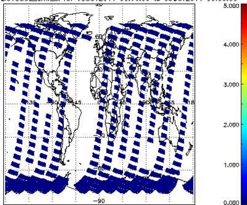
SCIOL2P_NADUV5S02_amf_cl for 08OCT2011 00:00:00 to 09OCT2011 00:00:00
