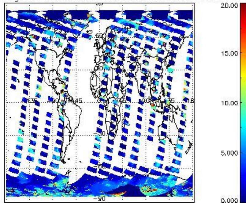
cL_top_height for 08OCT2011 00:00:00 to 09OCT2011 00:00:00
