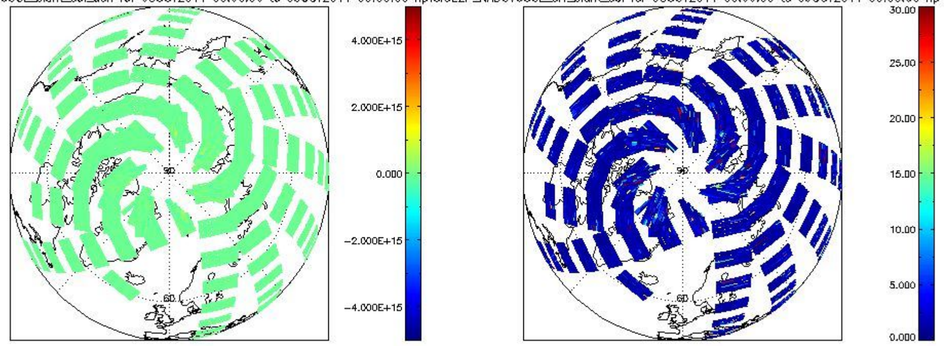
CIOL2P_NADUV60CL_slant_col_den for 08OCT2011 00:00:00 to 09OCT2011 00:00:00 np CIOL2P_NADUV60CL_err_slant_col for 08OCT2011 00:00:00 to 09OCT2011 00:00:00 np
