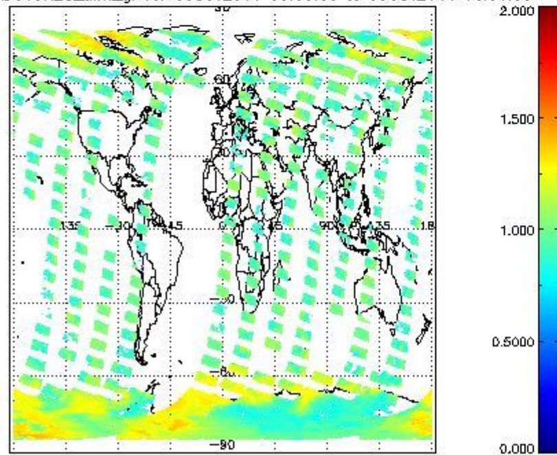
SCIOL2P_NADUV8H20_amf_gr for 08OCT2011 00:00:00 to 09OCT2011 00:00:00
