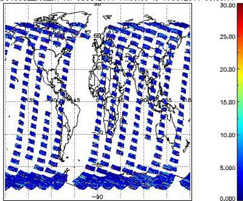
SCIOL2P_NADUV5S02_vcd_err for 08OCT2011 00:00:00 to 09OCT2011 00:00:00
