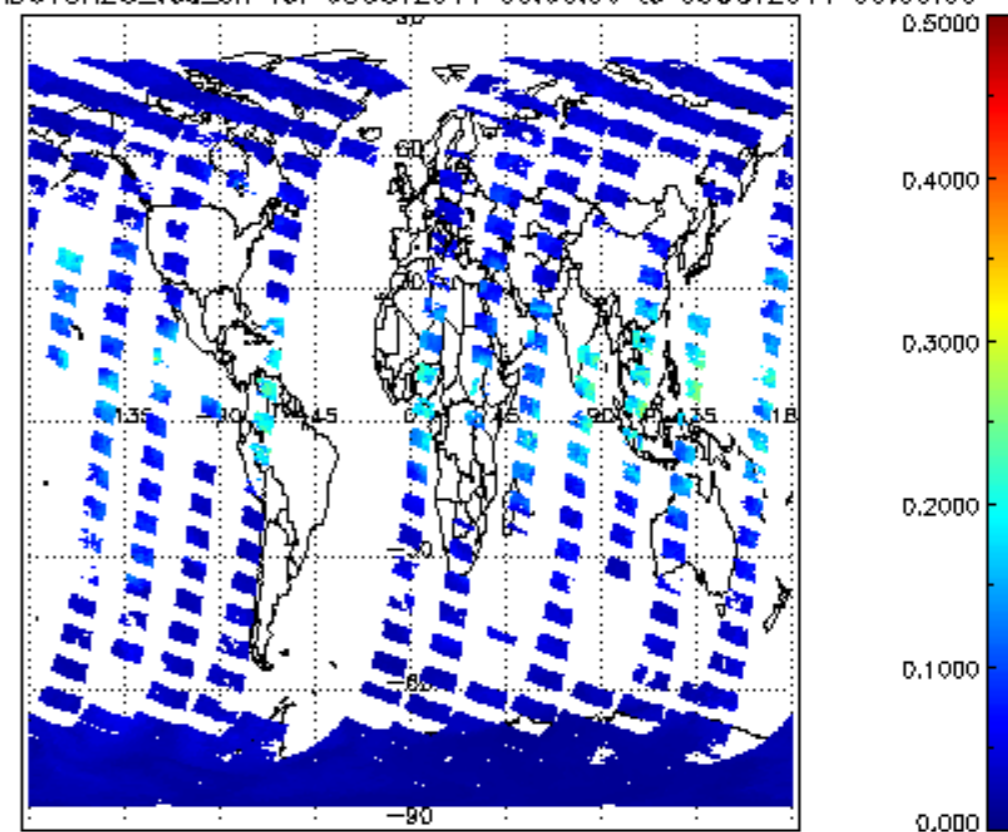
SCIOL2P_NADUV8H20_vcd_err for 08OCT2011 00:00:00 to 09OCT2011 00:00:00
