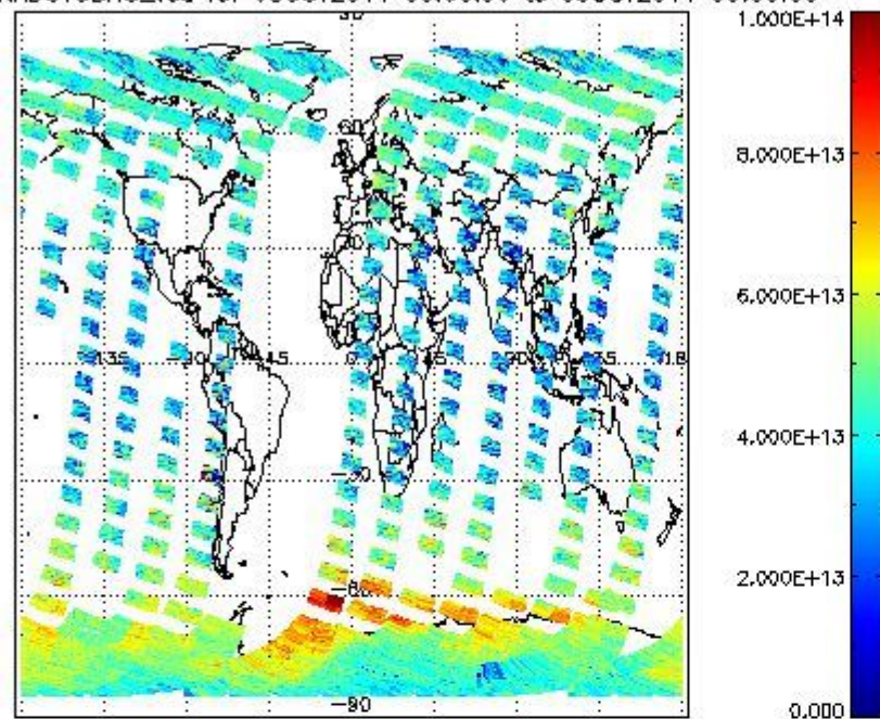
SCIOL2P_NADUV3BRO_vcd for 08OCT2011 00:00:00 to 09OCT2011 00:00:00
