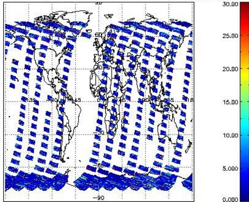
SCIOL2P_NADUV7S02_vcd_err for 08OCT2011 00:00:00 to 09OCT2011 00:00:00
