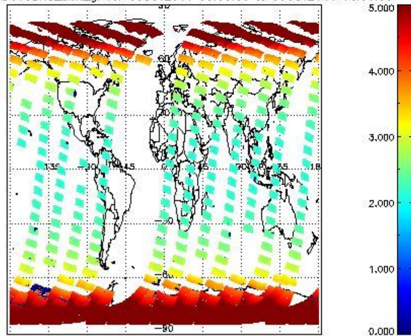
SCIOL2P_NADUV3BRO_amf_gr for 08OCT2011 00:00:00 to 09OCT2011 00:00:00
