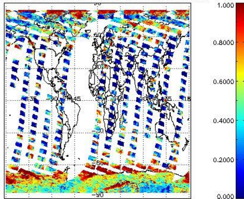
cLfrac for 08OCT2011 00:00:00 to 09OCT2011 00:00:00
