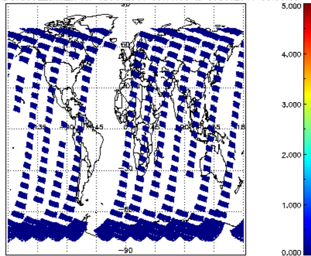
SCIOL2P_NADUV5S02_amf_cl for 08OCT2011 00:00:00 to 09OCT2011 00:00:00
