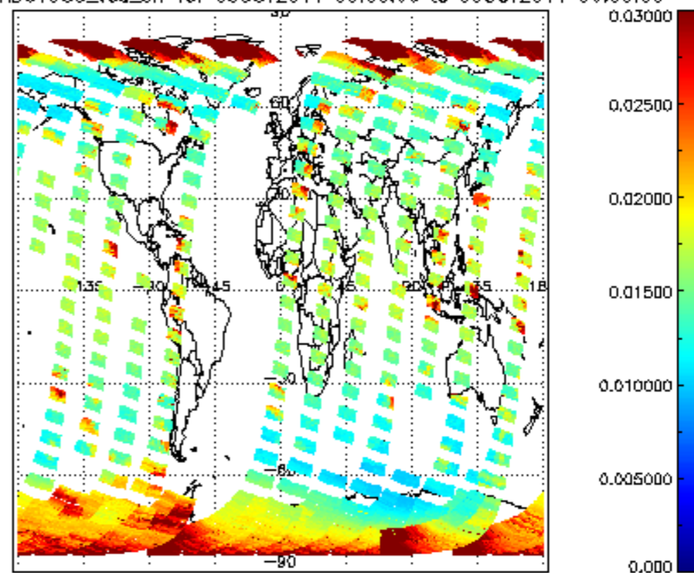
SCIOL2P_NADUV003_vcd_err for 08OCT2011 00:00:00 to 09OCT2011 00:00:00
