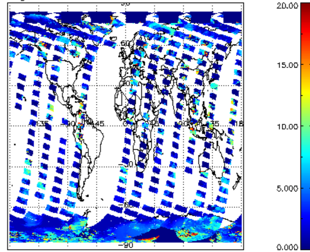
cl_top_height for 08OCT2011 00:00:00 to 09OCT2011 00:00:00
