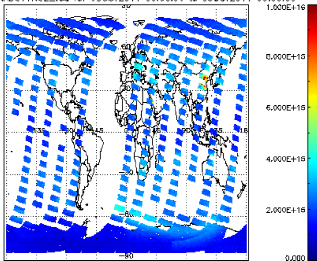
SCIOL2P_NADUV1NO2_vcd for 08OCT2011 00:00:00 to 09OCT2011 00:00:00
