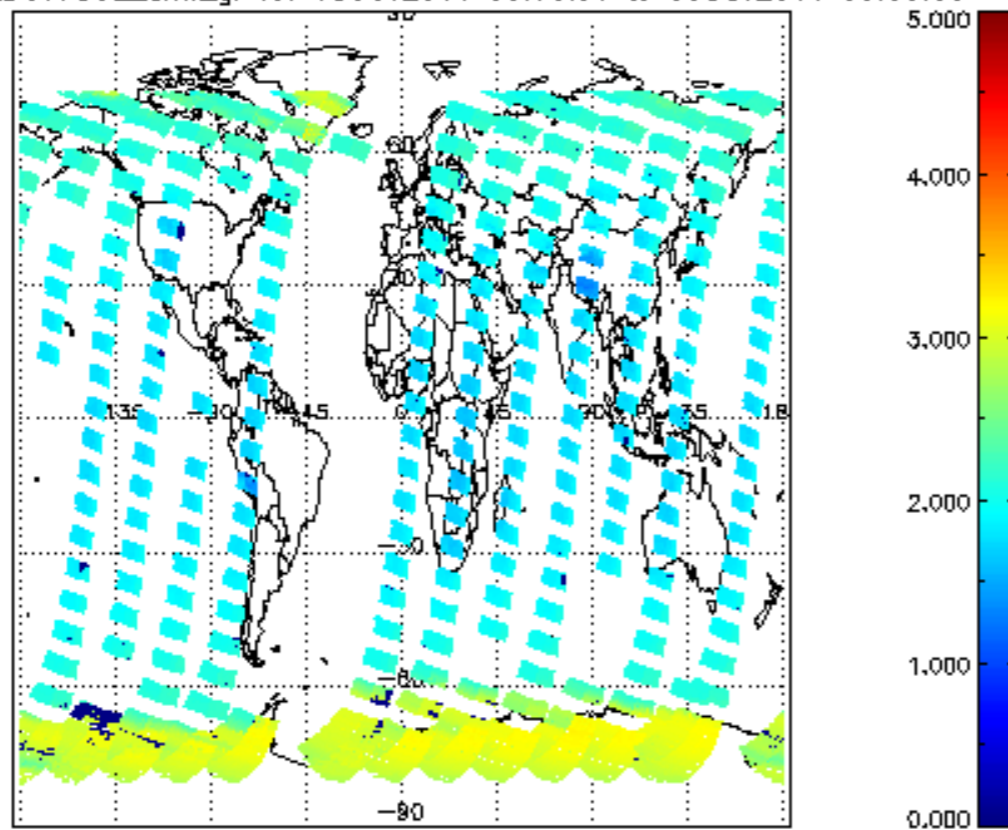
SCIOL2P_NADUV7S02_amf_gr for 08OCT2011 00:00:00 to 09OCT2011 00:00:00
