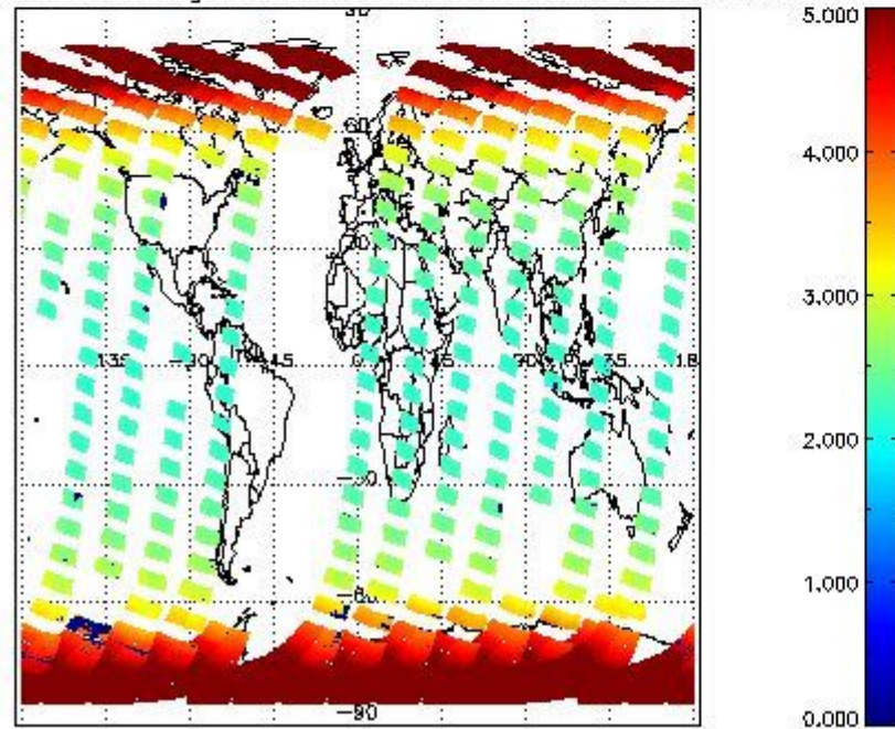
SCIOL2P_NADUV003_amf_gr for 08OCT2011 00:00:00 to 09OCT2011 00:00:00
