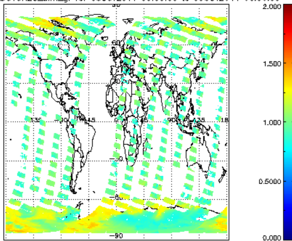
SCIOL2P_NADUV8H20_amf_gr for 08OCT2011 00:00:00 to 09OCT2011 00:00:00
