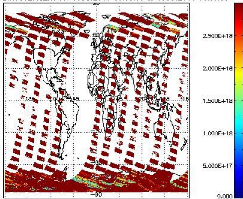
SCIO2P_NADIR3CO_vcd_err for 08OCT2011 00:00:00 to 09OCT2011 00:00:00
