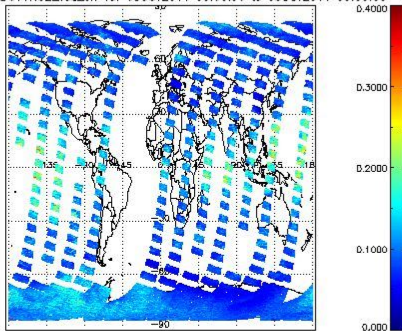
SCIOL2P_NADUV1N02_vcd_err for 08OCT2011 00:00:00 to 09OCT2011 00:00:00
