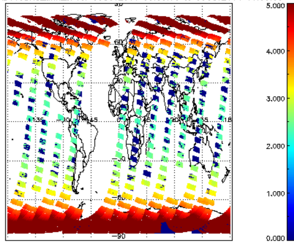
SCIOL2P_NADUV3BRO_amf_cl for 08OCT2011 00:00:00 to 09OCT2011 00:00:00
