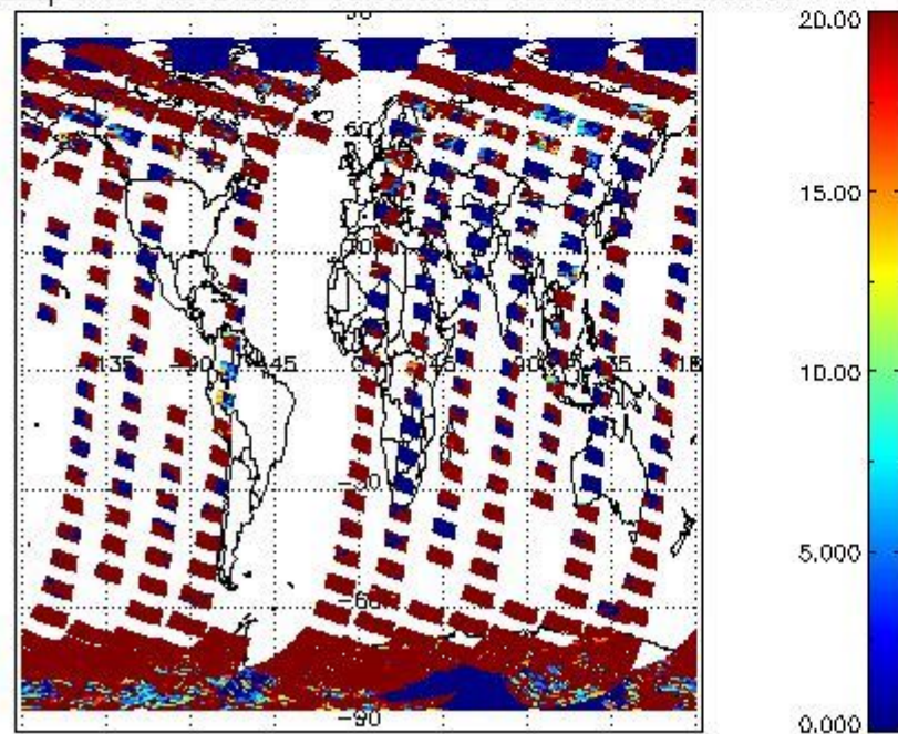
cL_opt_depth for 08OCT2011 00:00:00 to 09OCT2011 00:00:00
