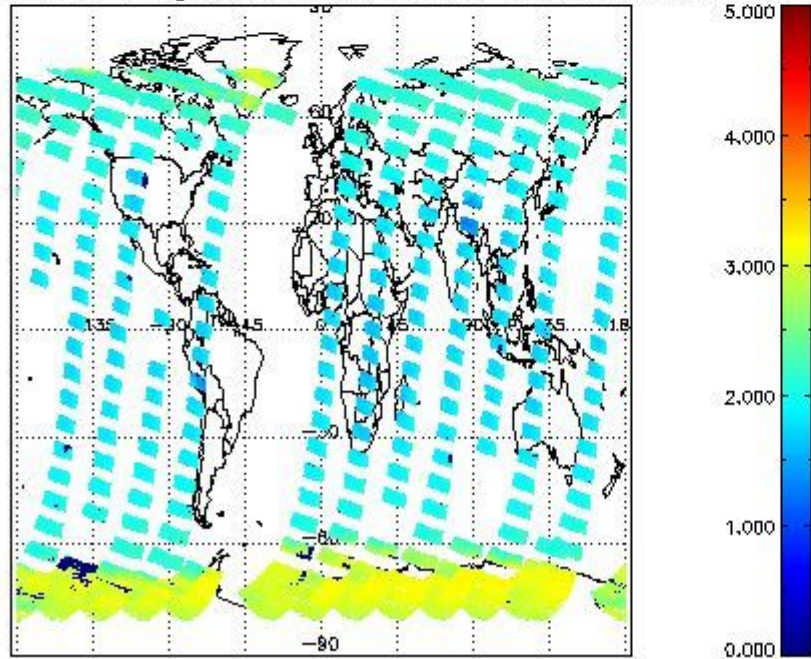
SCIOL2P_NADUV7S02_amf_gr for 08OCT2011 00:00:00 to 09OCT2011 00:00:00
