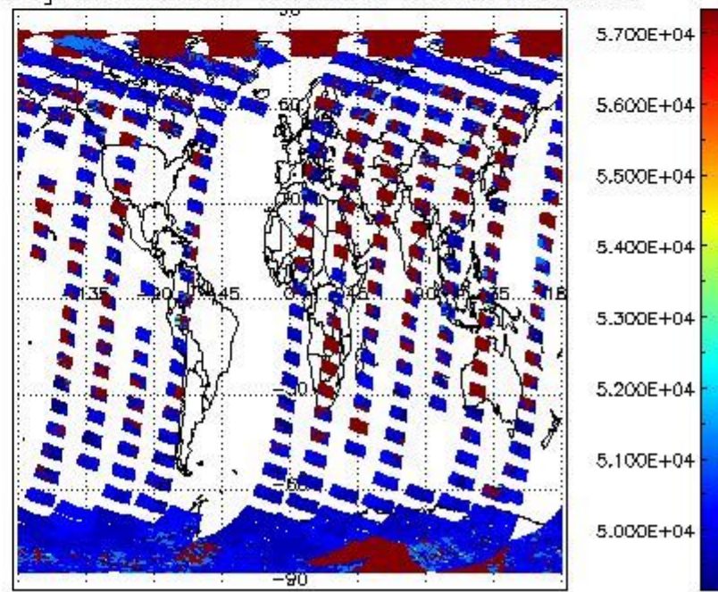
cloud_flags for 08OCT2011 00:00:00 to 09OCT2011 00:00:00
