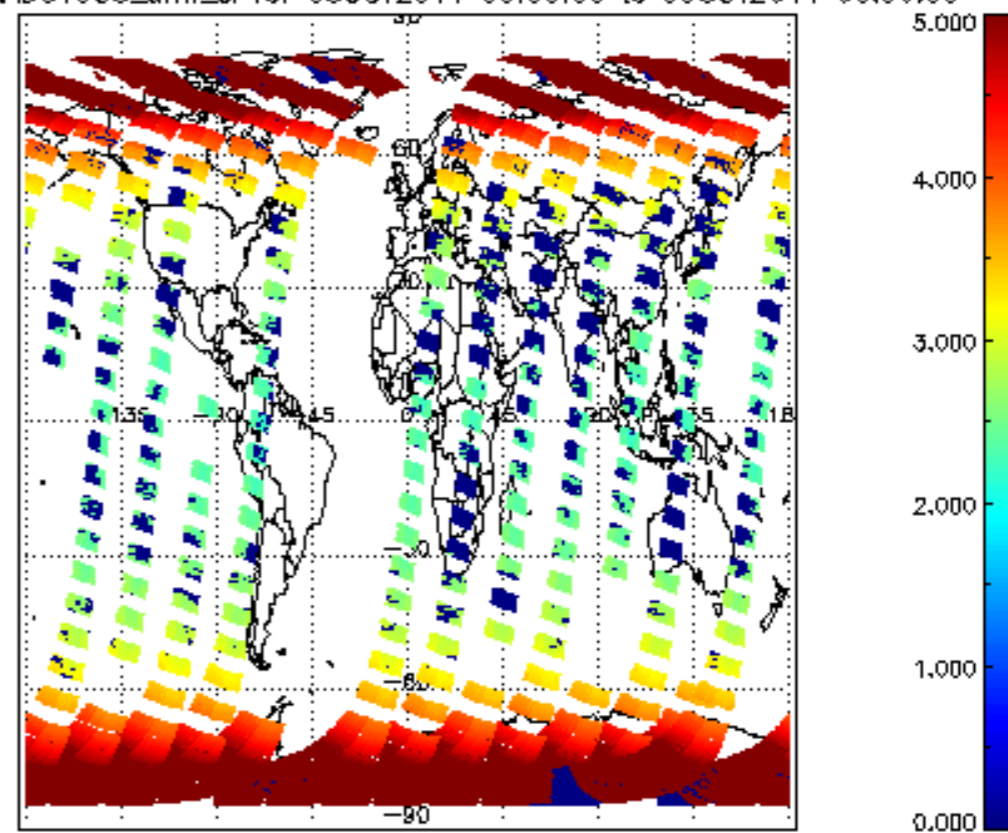
SCIOL2P_NADUV003_amf_cl for 08OCT2011 00:00:00 to 09OCT2011 00:00:00
