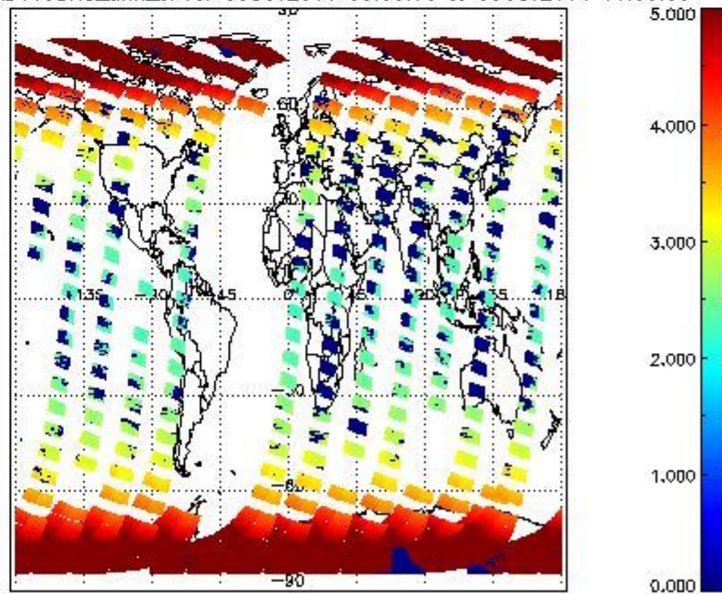
SCIOL2P_NADUV3BRO_amf_cl for 08OCT2011 00:00:00 to 09OCT2011 00:00:00
