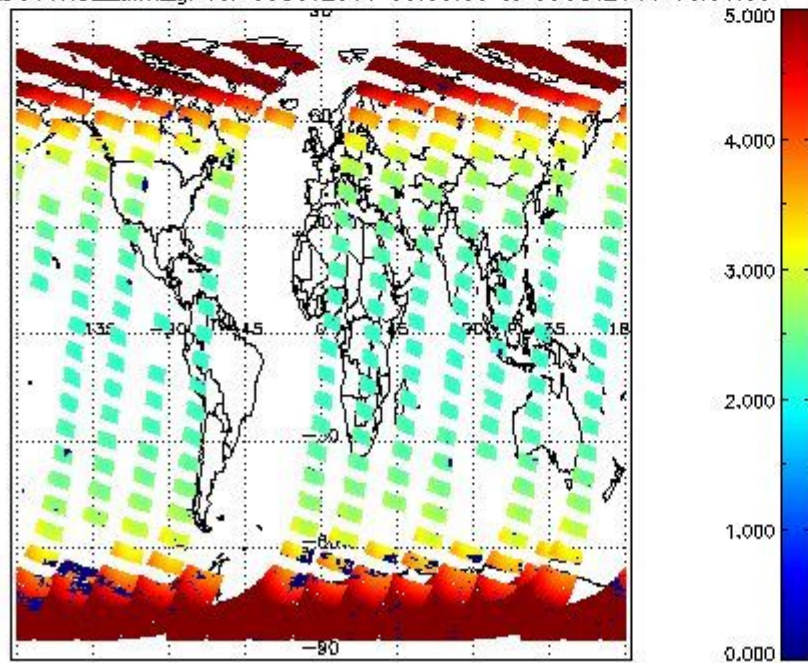
SCIOL2P_NADUV1N02_amf_gr for 08OCT2011 00:00:00 to 09OCT2011 00:00:00
