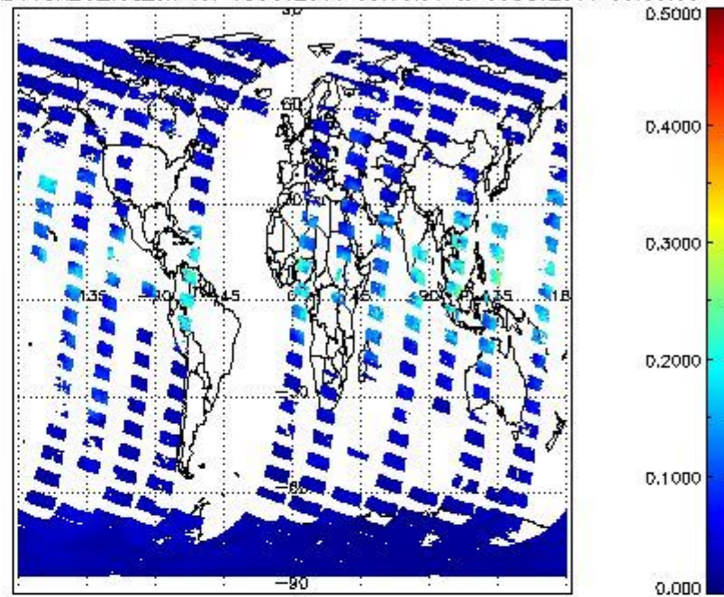
SCIOL2P_NADUV8H20_vcd_err for 08OCT2011 00:00:00 to 09OCT2011 00:00:00
