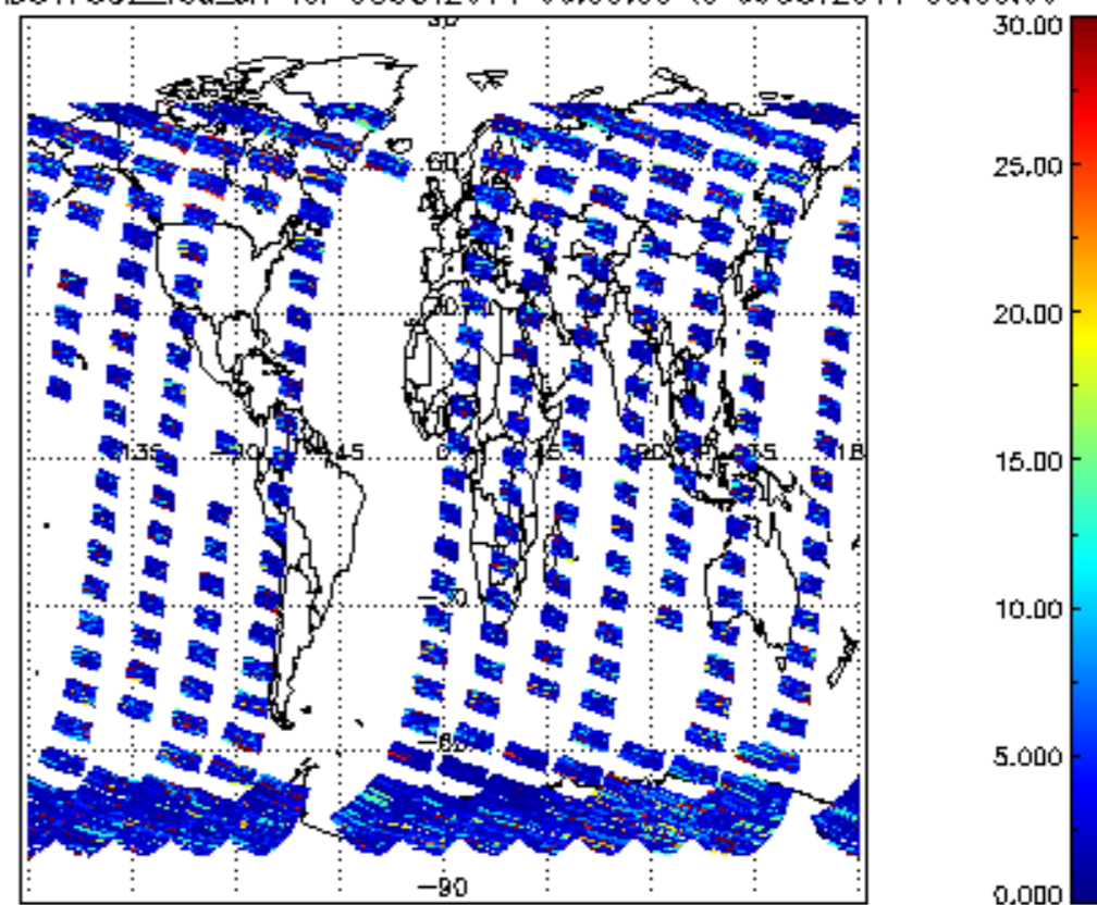
SCIOL2P_NADUV7S02_vcd_err for 08OCT2011 00:00:00 to 09OCT2011 00:00:00
