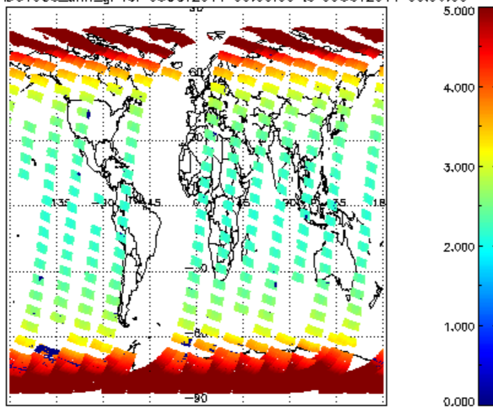
SCIOL2P_NADUV003_amf_gr for 08OCT2011 00:00:00 to 09OCT2011 00:00:00
