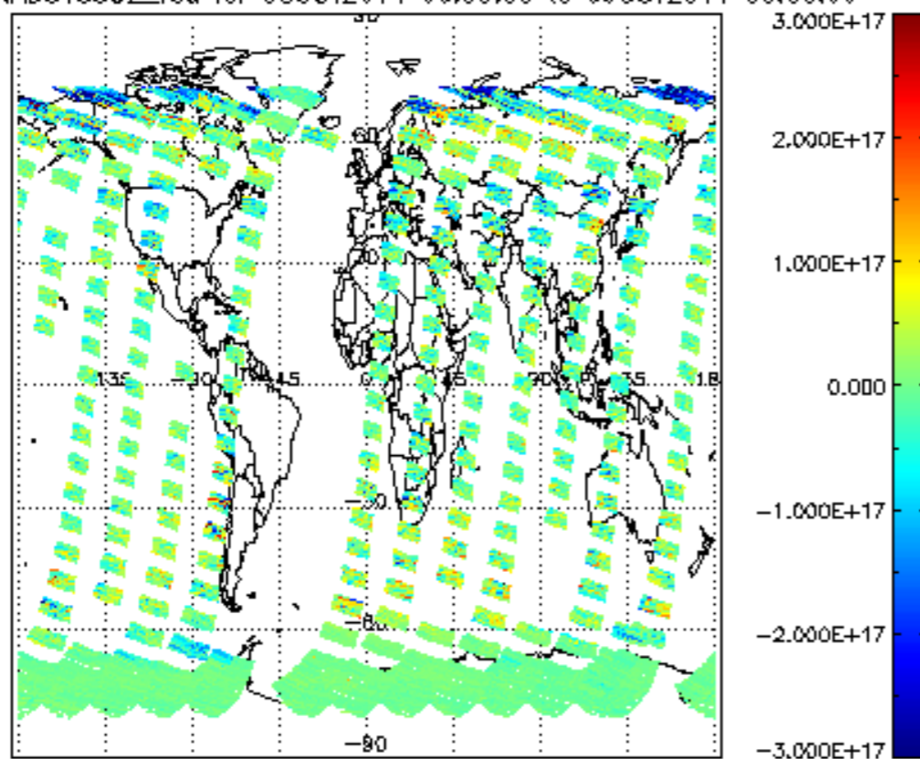
SCIOL2P_NADUV5S02_vcd for 08OCT2011 00:00:00 to 09OCT2011 00:00:00
