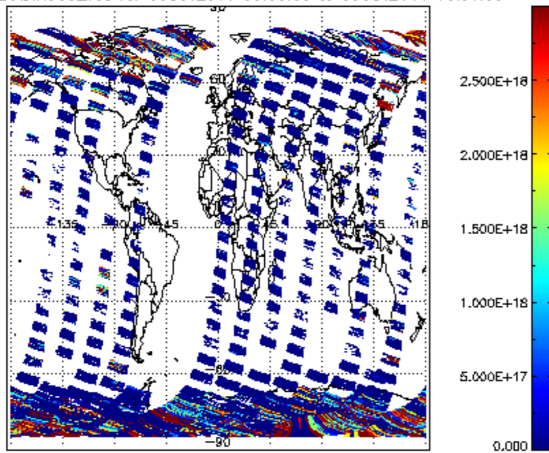
SCIOL2P_NADIR3CO_vcd for 08OCT2011 00:00:00 to 09OCT2011 00:00:00
