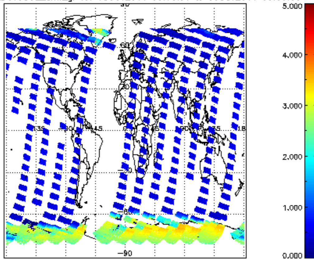
SCIOL2P_NADUV5S02_amf_gr for 08OCT2011 00:00:00 to 09OCT2011 00:00:00
