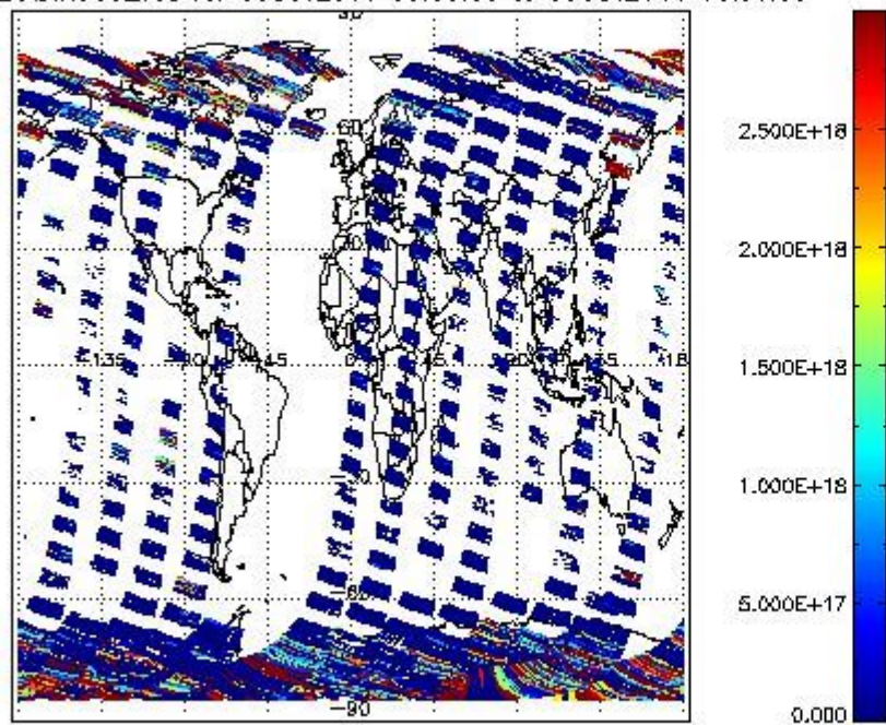
SCIO2P_NADIR3CO_vcd for 08OCT2011 00:00:00 to 09OCT2011 00:00:00
