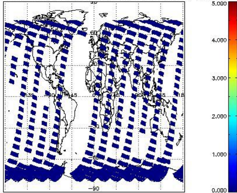
SCIOL2P_NADUV7S02_amf_cl for 08OCT2011 00:00:00 to 09OCT2011 00:00:00
