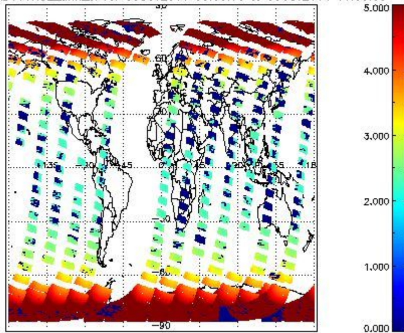
SCIOL2P_NADUV1N02_amf_cl for 08OCT2011 00:00:00 to 09OCT2011 00:00:00
