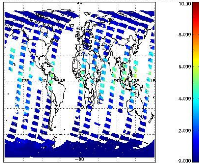
SCIOL2P_NADUV8H20_vcd for 08OCT2011 00:00:00 to 09OCT2011 00:00:00
