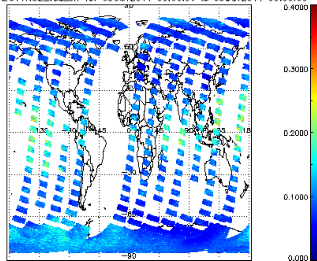
SCIOL2P_NADUV1NO2_vcd_err for 08OCT2011 00:00:00 to 09OCT2011 00:00:00
