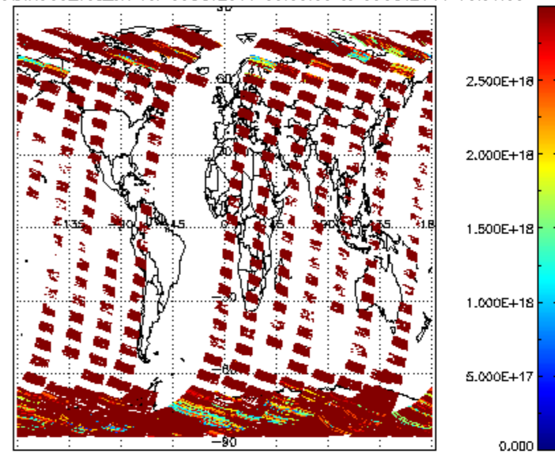
SCIOL2P_NADIR3CO_vcd_err for 08OCT2011 00:00:00 to 09OCT2011 00:00:00
