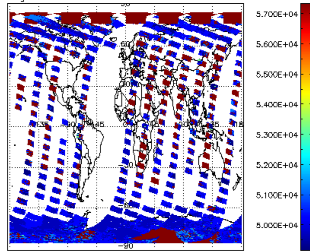
cloud_flags for 08OCT2011 00:00:00 to 09OCT2011 00:00:00
