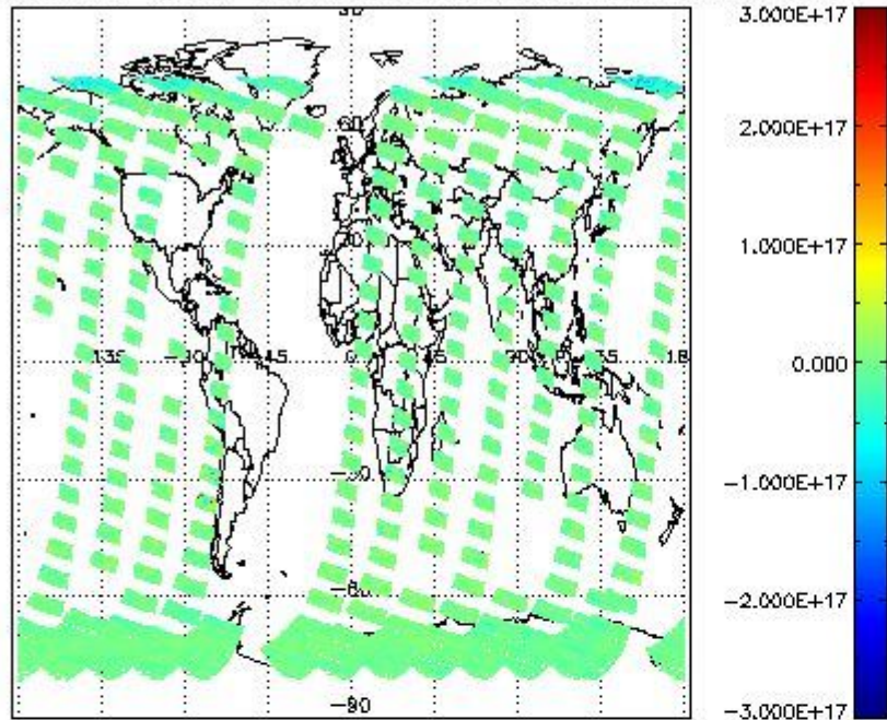
SCIOL2P_NADUV7S02_vcd for 08OCT2011 00:00:00 to 09OCT2011 00:00:00
