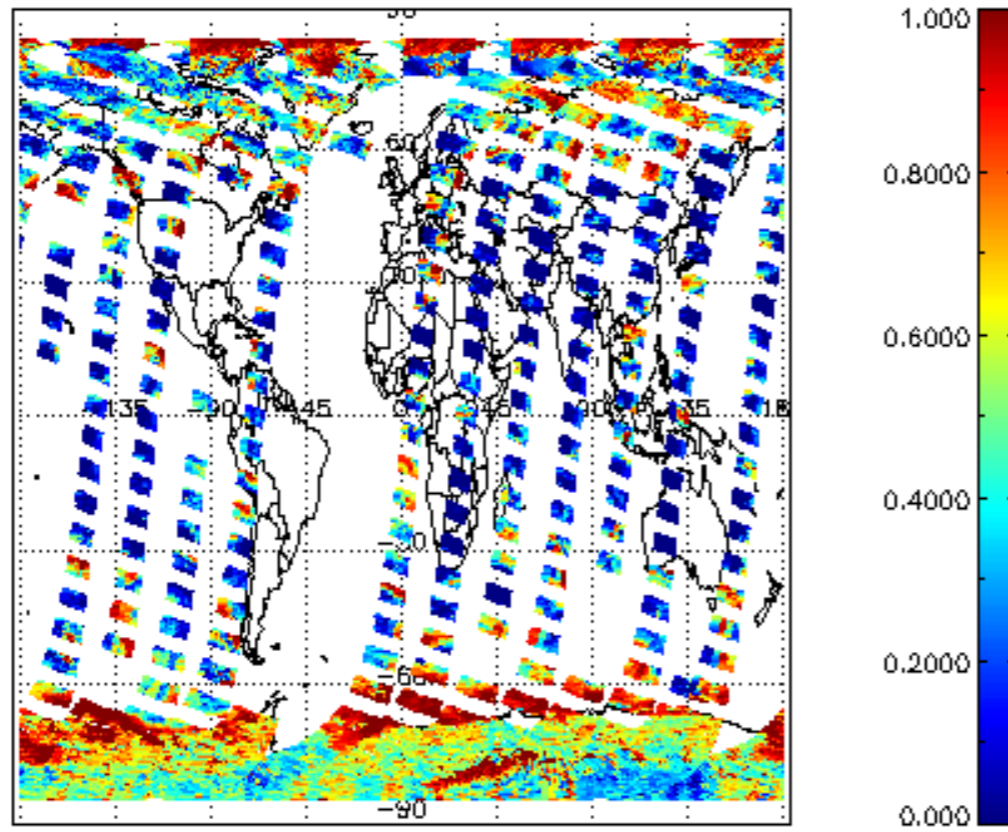
cl_frac for 08OCT2011 00:00:00 to 09OCT2011 00:00:00
