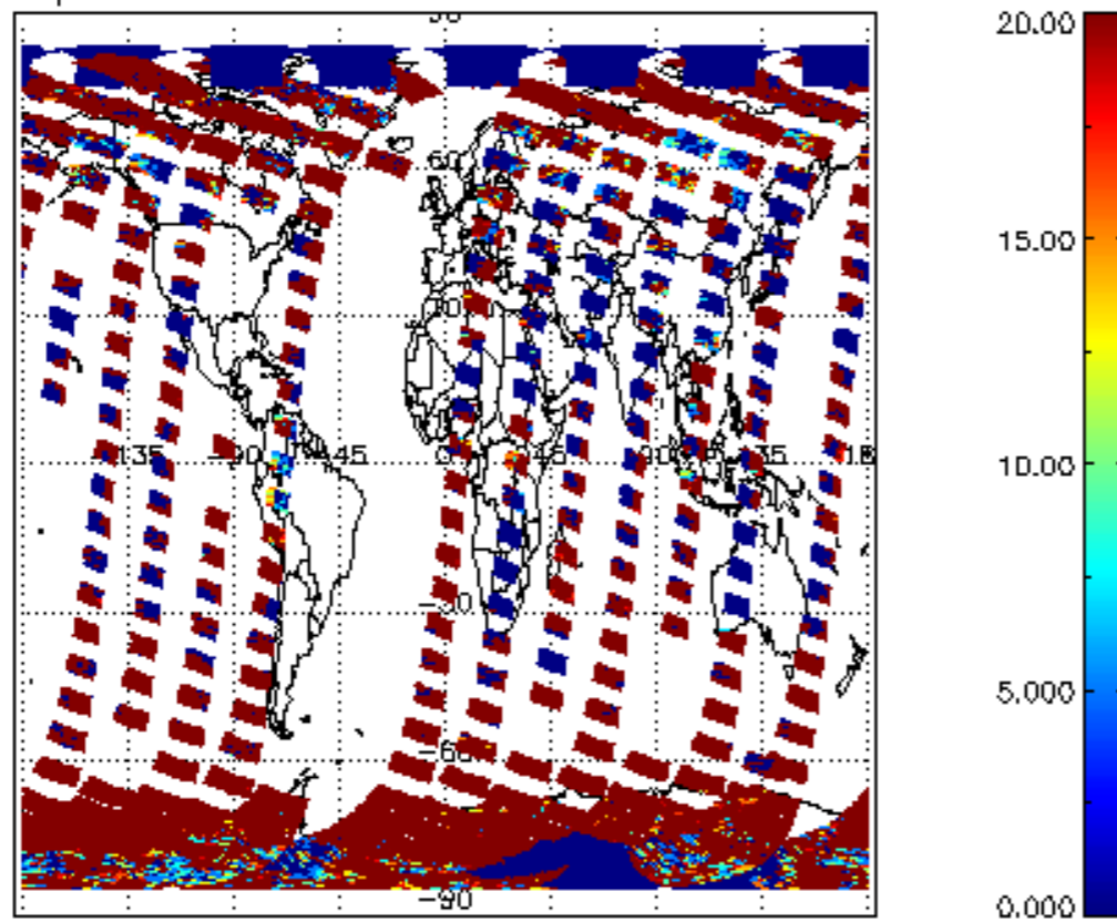
cl_opt_depth for 08OCT2011 00:00:00 to 09OCT2011 00:00:00
