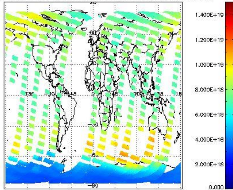
SCIOL2P_NADUV003_vcd for 08OCT2011 00:00:00 to 09OCT2011 00:00:00
