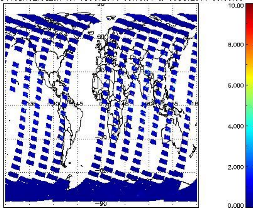
SCIOL2P_NADUV3BRO_vcd_err for 08OCT2011 00:00:00 to 09OCT2011 00:00:00
