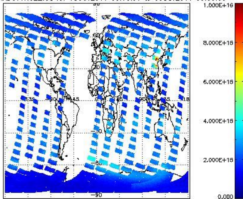
SCIOL2P_NADUV1N02_vcd for 08OCT2011 00:00:00 to 09OCT2011 00:00:00
