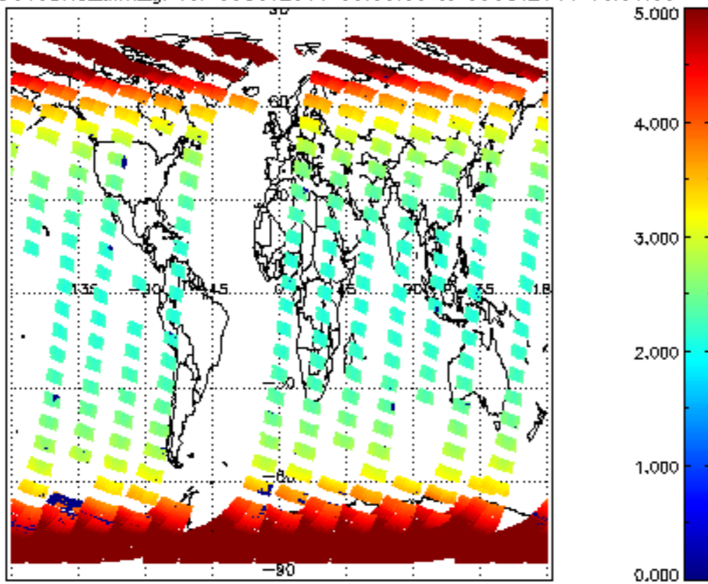
SCIOL2P_NADUV3BRO_amf_gr for 08OCT2011 00:00:00 to 09OCT2011 00:00:00
