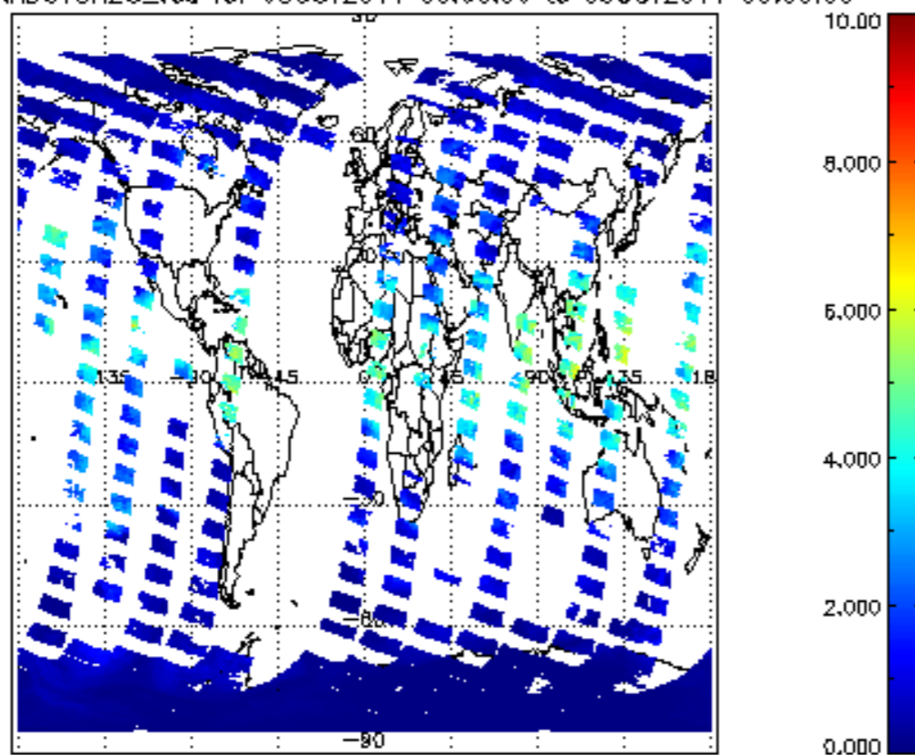
SCIOL2P_NADUV8H20_vcd for 08OCT2011 00:00:00 to 09OCT2011 00:00:00
