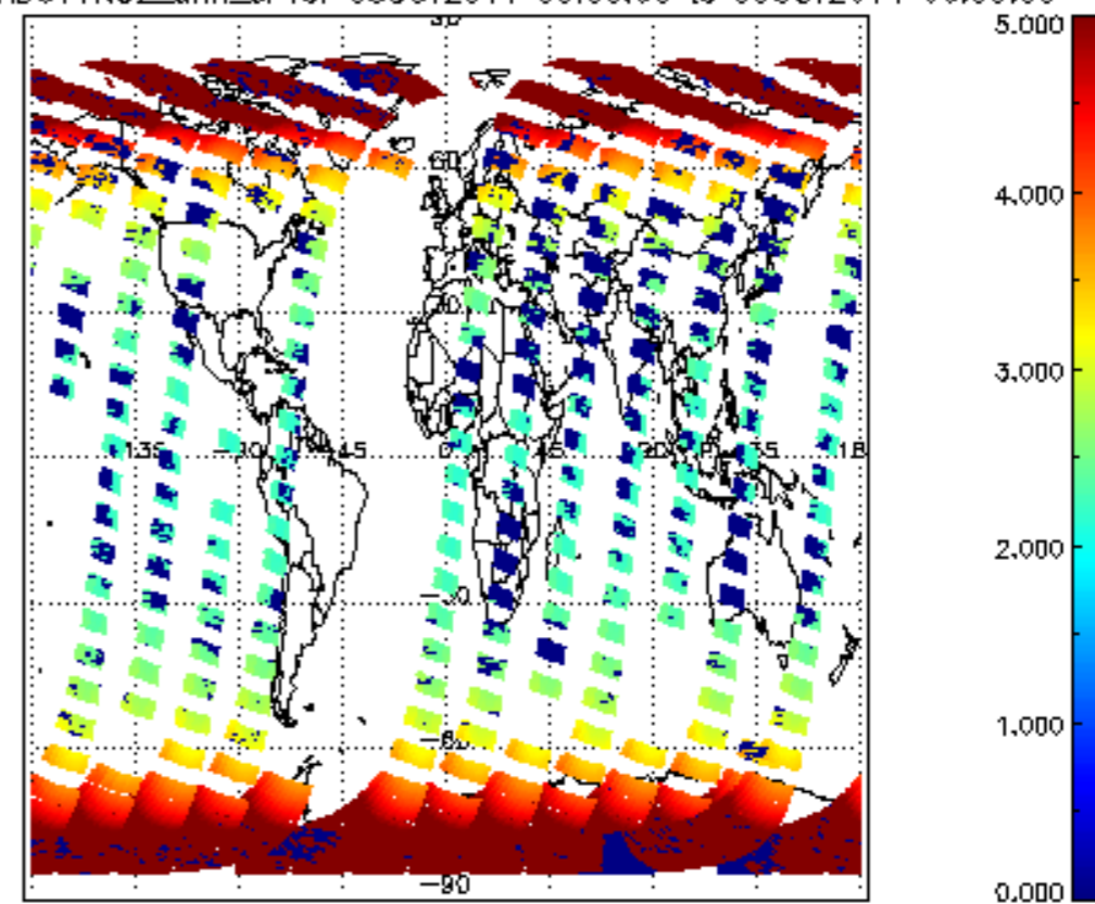
SCIOL2P_NADUV1NO2_amf_cl for 08OCT2011 00:00:00 to 09OCT2011 00:00:00
