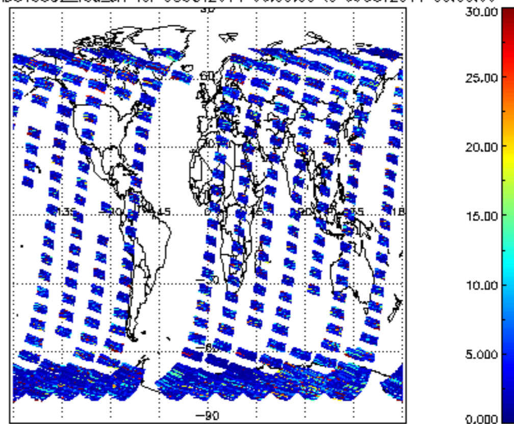
SCIOL2P_NADUV5S02_vcd_err for 08OCT2011 00:00:00 to 09OCT2011 00:00:00
