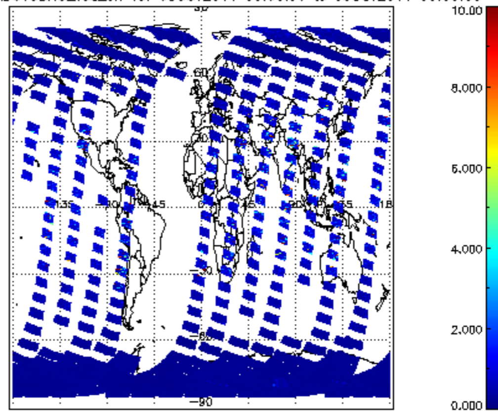
SCIOL2P_NADUV3BRO_vcd_err for 08OCT2011 00:00:00 to 09OCT2011 00:00:00
