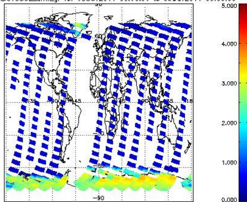
SCIOL2P_NADUV5S02_amf_gr for 08OCT2011 00:00:00 to 09OCT2011 00:00:00
