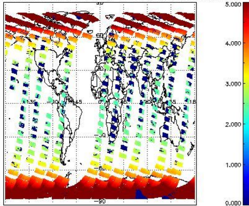
SCIOL2P_NADUV003_amf_cl for 08OCT2011 00:00:00 to 09OCT2011 00:00:00
