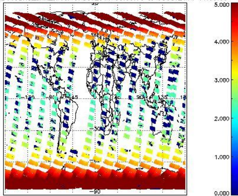
SCIOL2P_NADUV3BRO_amf_cl for 07OCT2011 00:00:00 to 08OCT2011 00:00:00
