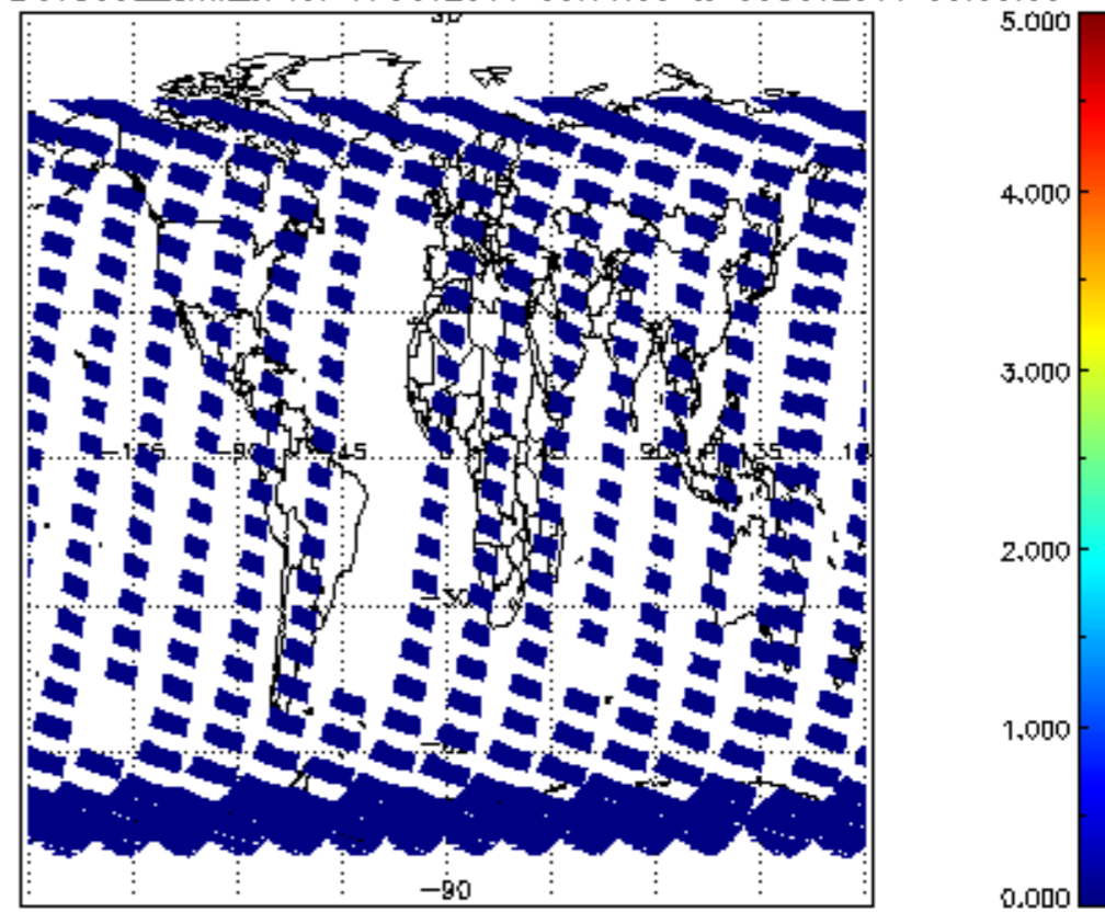
SCIOL2P_NADUV5S02_amf_cl for 07OCT2011 00:00:00 to 08OCT2011 00:00:00
