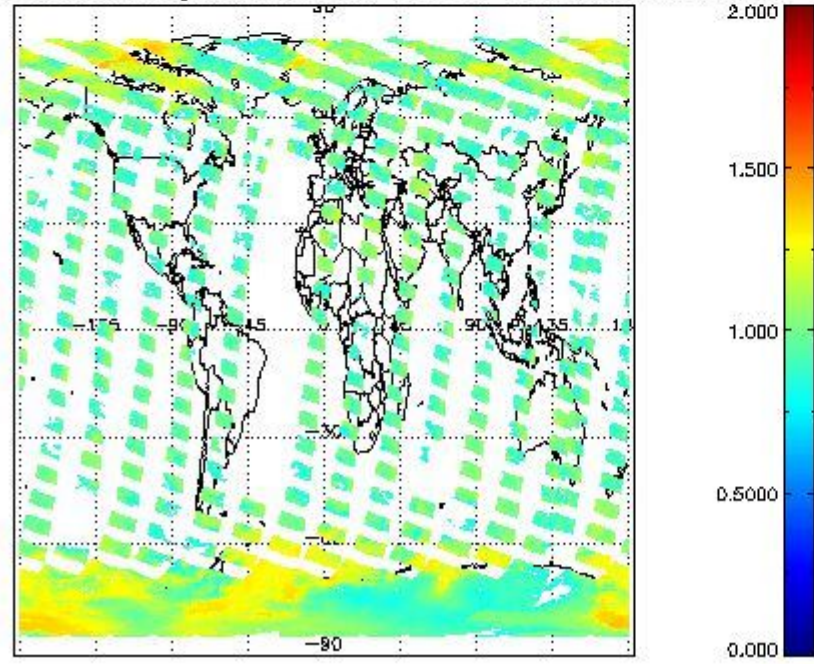
SCIOL2P_NADUV8H20_amf_gr for 07OCT2011 00:00:00 to 08OCT2011 00:00:00
