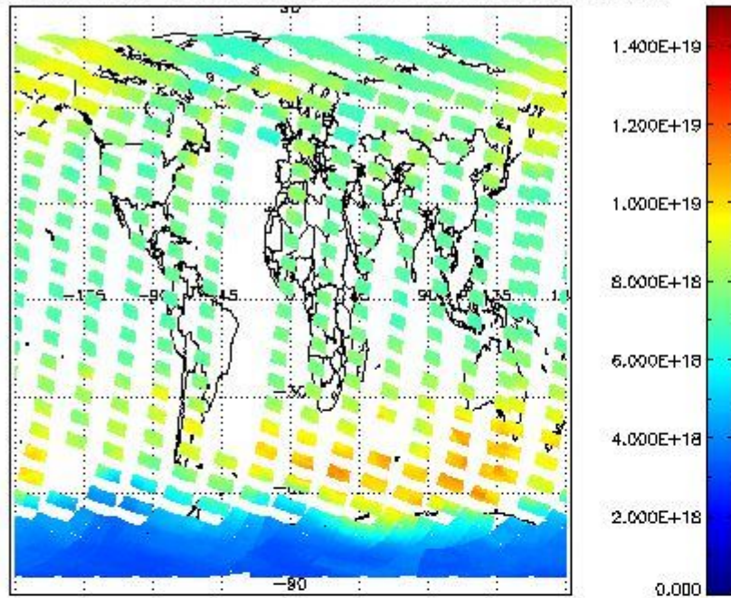
SCIOL2P_NADUV003_vcd for 07OCT2011 00:00:00 to 08OCT2011 00:00:00
