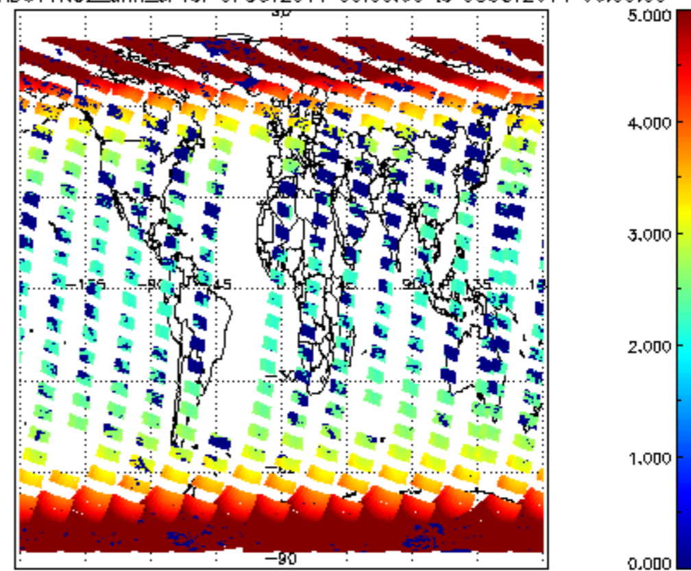
SCIOL2P_NADUV1NO2_amf_cl for 07OCT2011 00:00:00 to 08OCT2011 00:00:00
