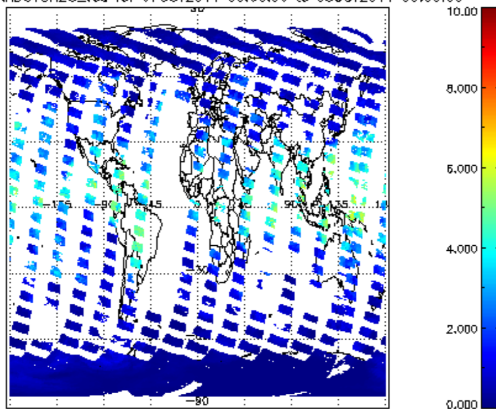
SCIOL2P_NADUV8H20_vcd for 07OCT2011 00:00:00 to 08OCT2011 00:00:00
