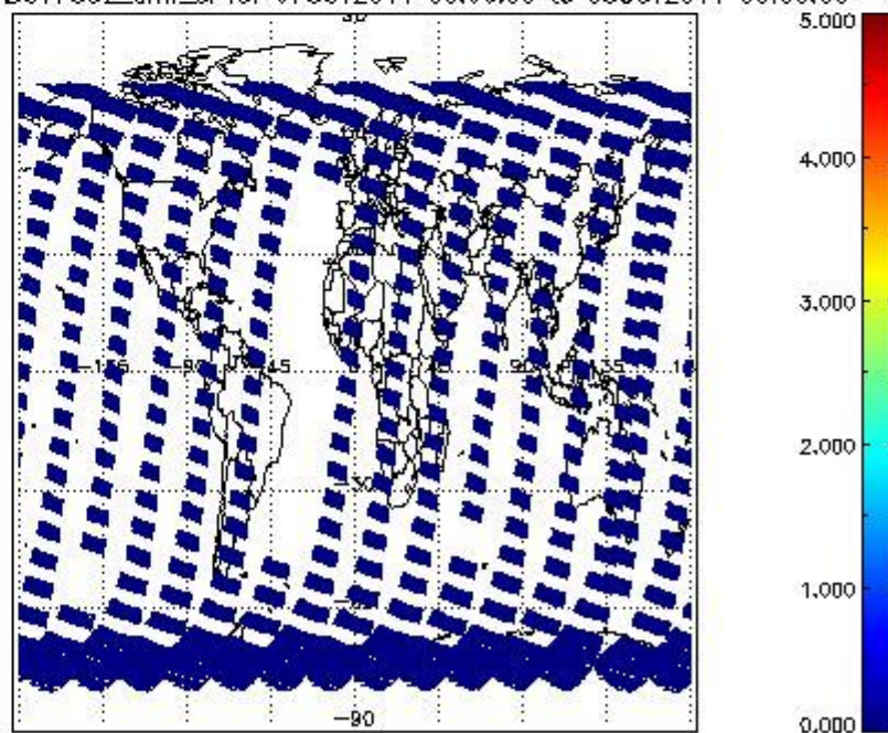
SCIOL2P_NADUV7S02_amf_cl for 07OCT2011 00:00:00 to 08OCT2011 00:00:00
