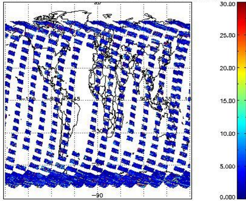
SCIOL2P_NADUV5SO2_vcd_err for 07OCT2011 00:00:00 to 08OCT2011 00:00:00
