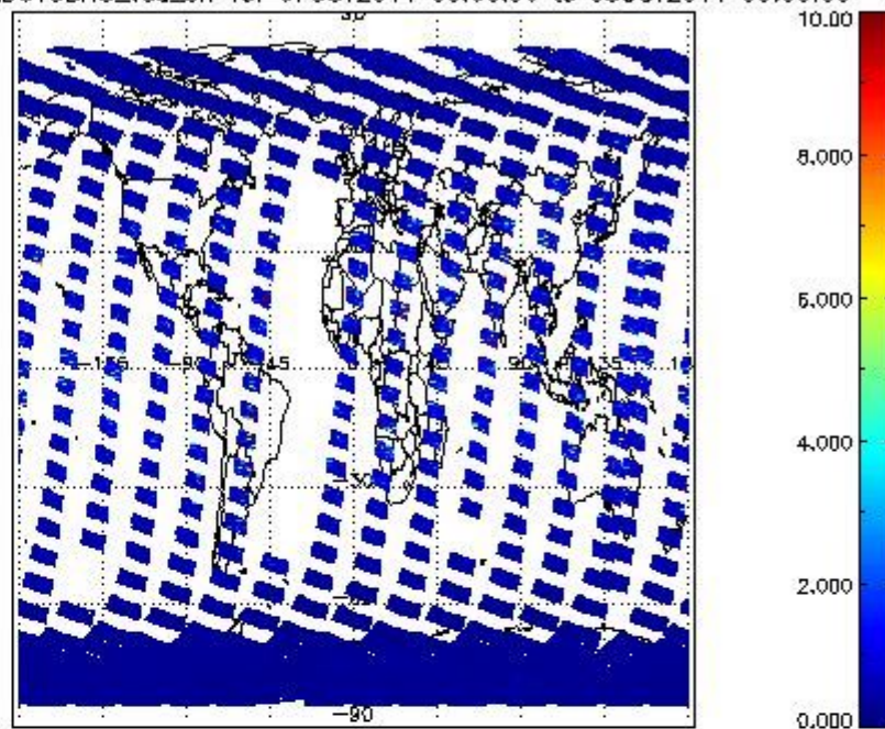
SCIOL2P_NADUV3BRO_vcd_err for 07OCT2011 00:00:00 to 08OCT2011 00:00:00
