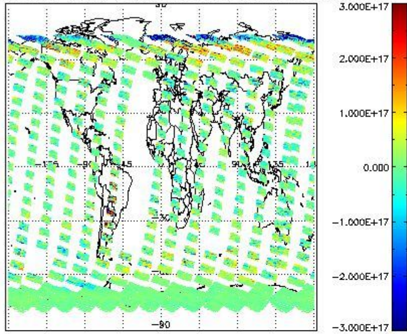
SCIOL2P_NADUV5SO2_vcd for 07OCT2011 00:00:00 to 08OCT2011 00:00:00
