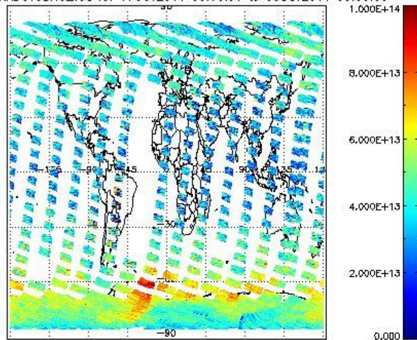
SCIOL2P_NADUV3BRO_vcd for 07OCT2011 00:00:00 to 08OCT2011 00:00:00
