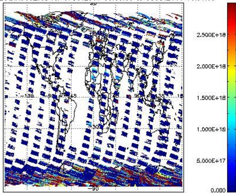
SCIDL2P_NADIR3CO_vcd for 07OCT2011 00:00:00 to 08OCT2011 00:00:00
