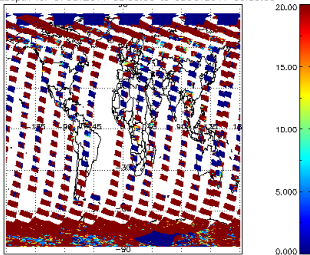
cl_opt_depth for 07OCT2011 00:00:00 to 08OCT2011 00:00:00
