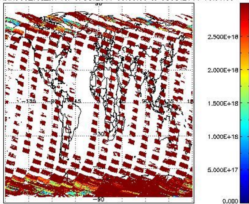
SCIDL2P_NADIR3CO_vcd_err for 07OCT2011 00:00:00 to 08OCT2011 00:00:00
