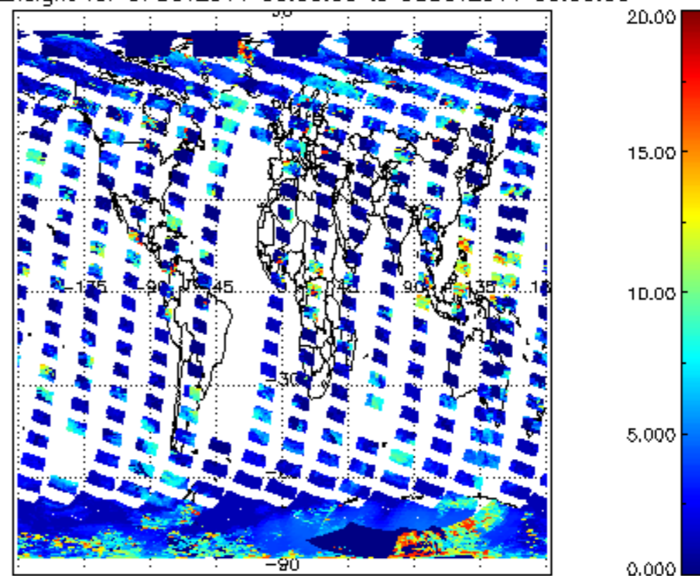
cl_top_height for 07OCT2011 00:00:00 to 08OCT2011 00:00:00
