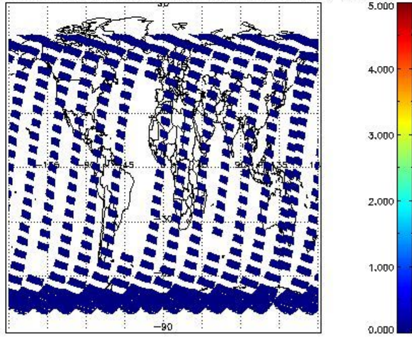
SCIOL2P_NADUV5SO2_amf_cl for 07OCT2011 00:00:00 to 08OCT2011 00:00:00
