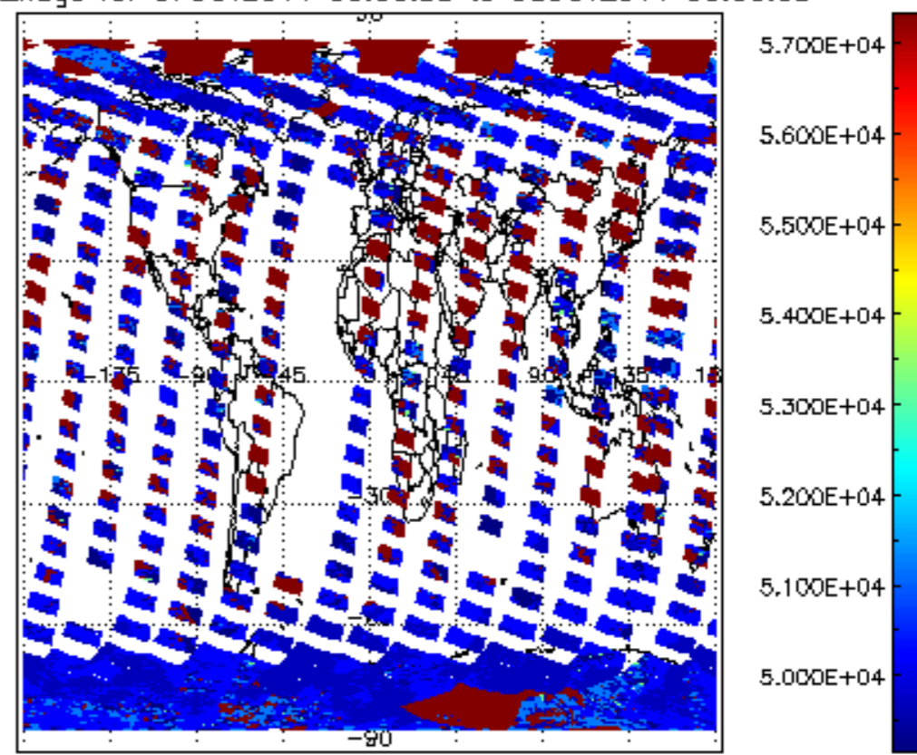
cloud_flags for 07OCT2011 00:00:00 to 08OCT2011 00:00:00
