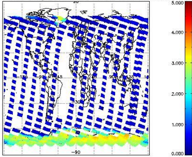
SCIOL2P_NADUV5SO2_amf_gr for 07OCT2011 00:00:00 to 08OCT2011 00:00:00
