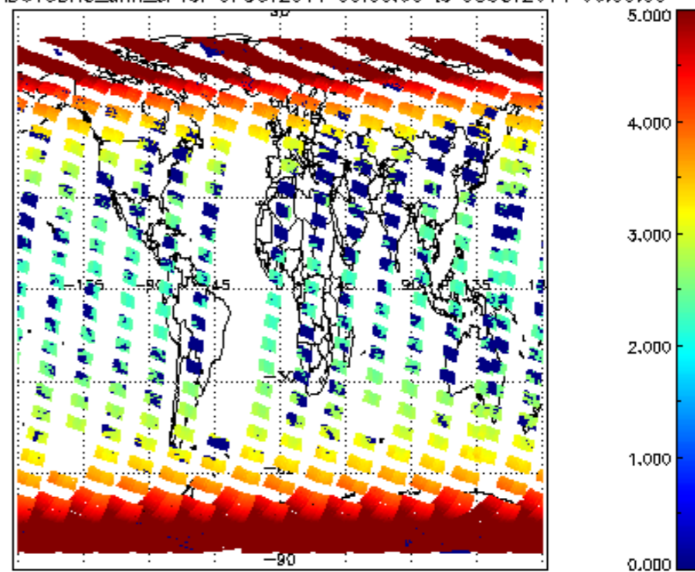
SCIOL2P_NADUV3BRO_amf_cl for 07OCT2011 00:00:00 to 08OCT2011 00:00:00
