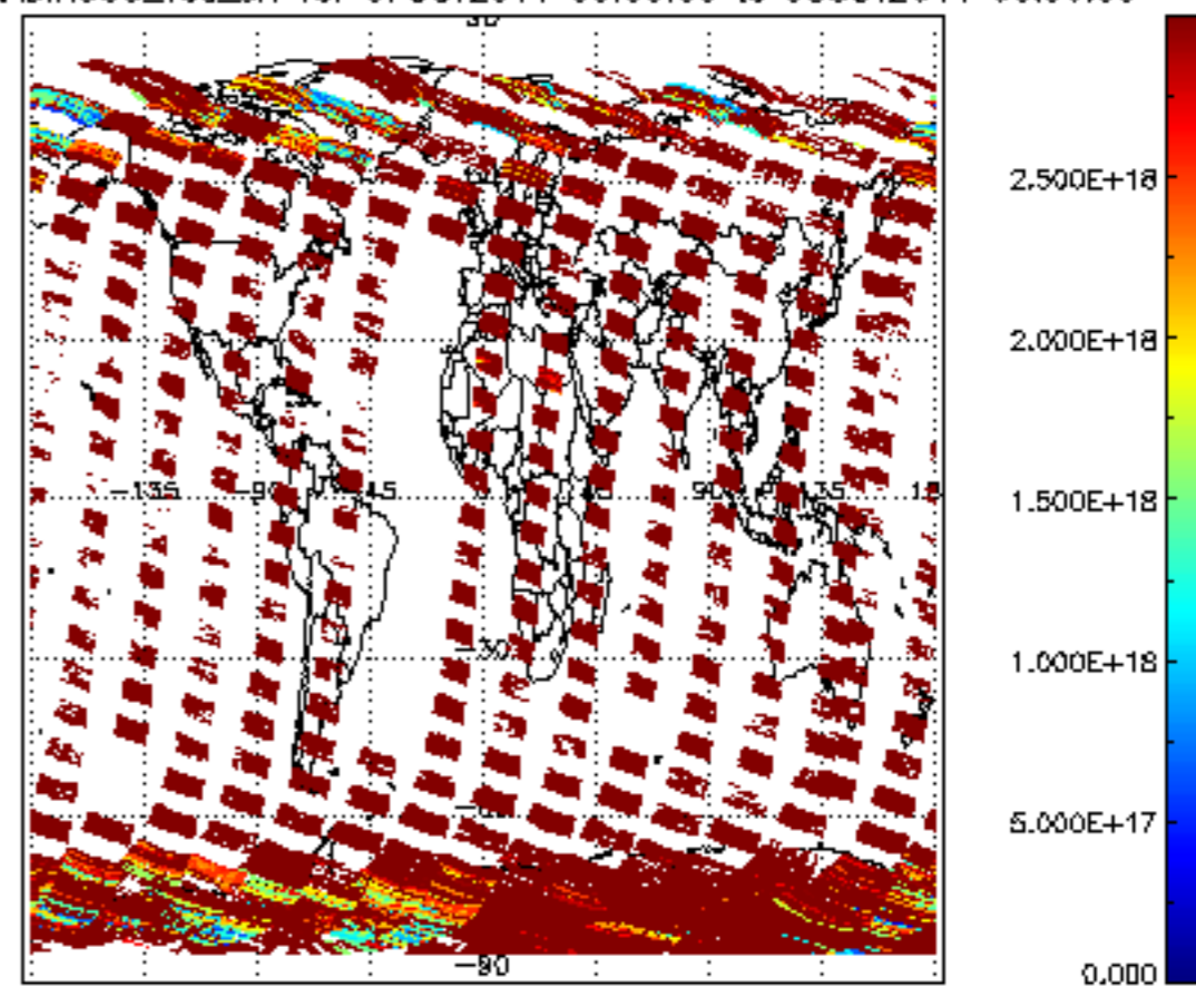
SCIOL2P_NADIR3CO_vcd_err for 07OCT2011 00:00:00 to 08OCT2011 00:00:00
