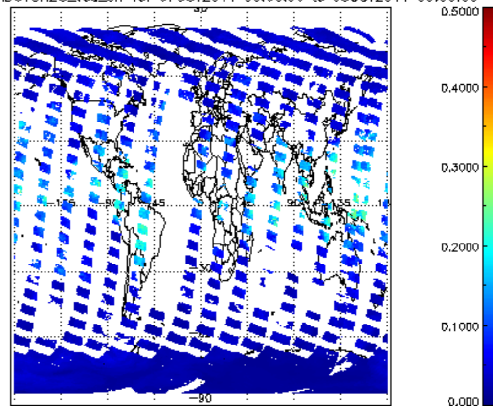
SCIOL2P_NADUV8H20_vcd_err for 07OCT2011 00:00:00 to 08OCT2011 00:00:00
