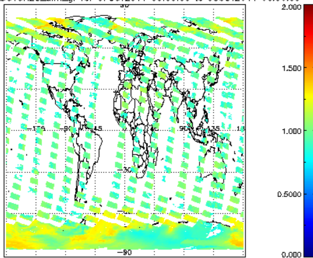
SCIOL2P_NADUV8H20_amf_gr for 07OCT2011 00:00:00 to 08OCT2011 00:00:00
