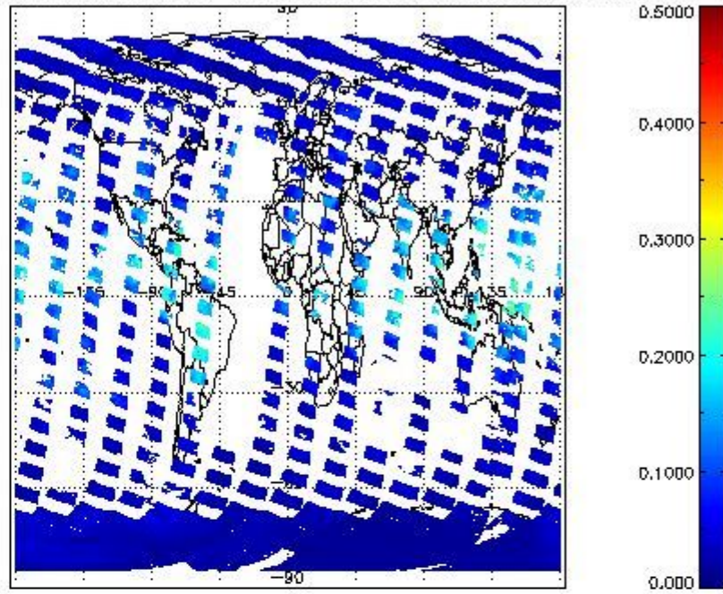
SCIOL2P_NADUV8H20_vcd_err for 07OCT2011 00:00:00 to 08OCT2011 00:00:00
