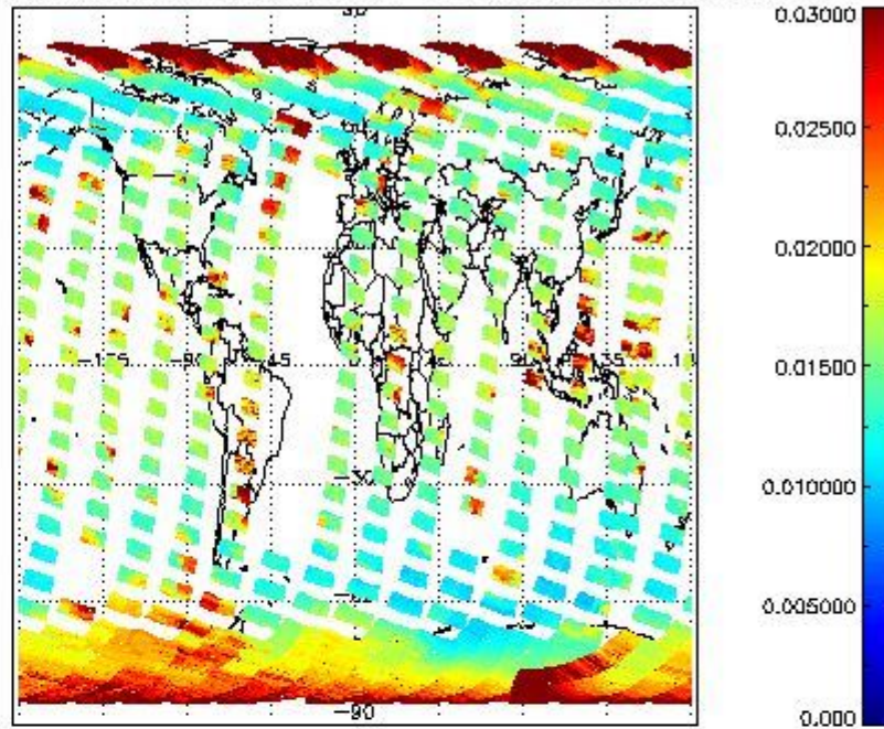
SCIOL2P_NADUV003_vcd_err for 07OCT2011 00:00:00 to 08OCT2011 00:00:00
