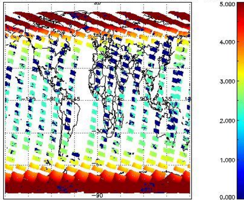
SCIOL2P_NADUV1NO2_amf_cl for 07OCT2011 00:00:00 to 08OCT2011 00:00:00
