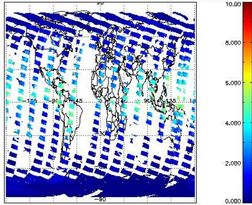
SCIOL2P_NADUV8H20_vcd for 07OCT2011 00:00:00 to 08OCT2011 00:00:00
