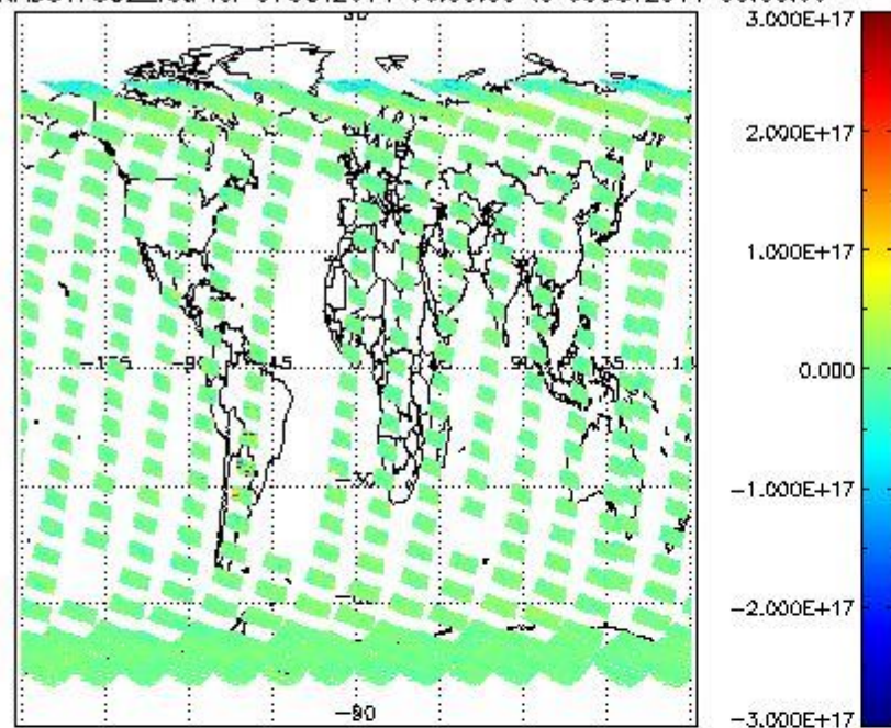
SCIOL2P_NADUV7S02_vcd for 07OCT2011 00:00:00 to 08OCT2011 00:00:00
