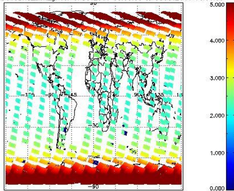
SCIOL2P_NADUV3BRO_amf_gr for 07OCT2011 00:00:00 to 08OCT2011 00:00:00
