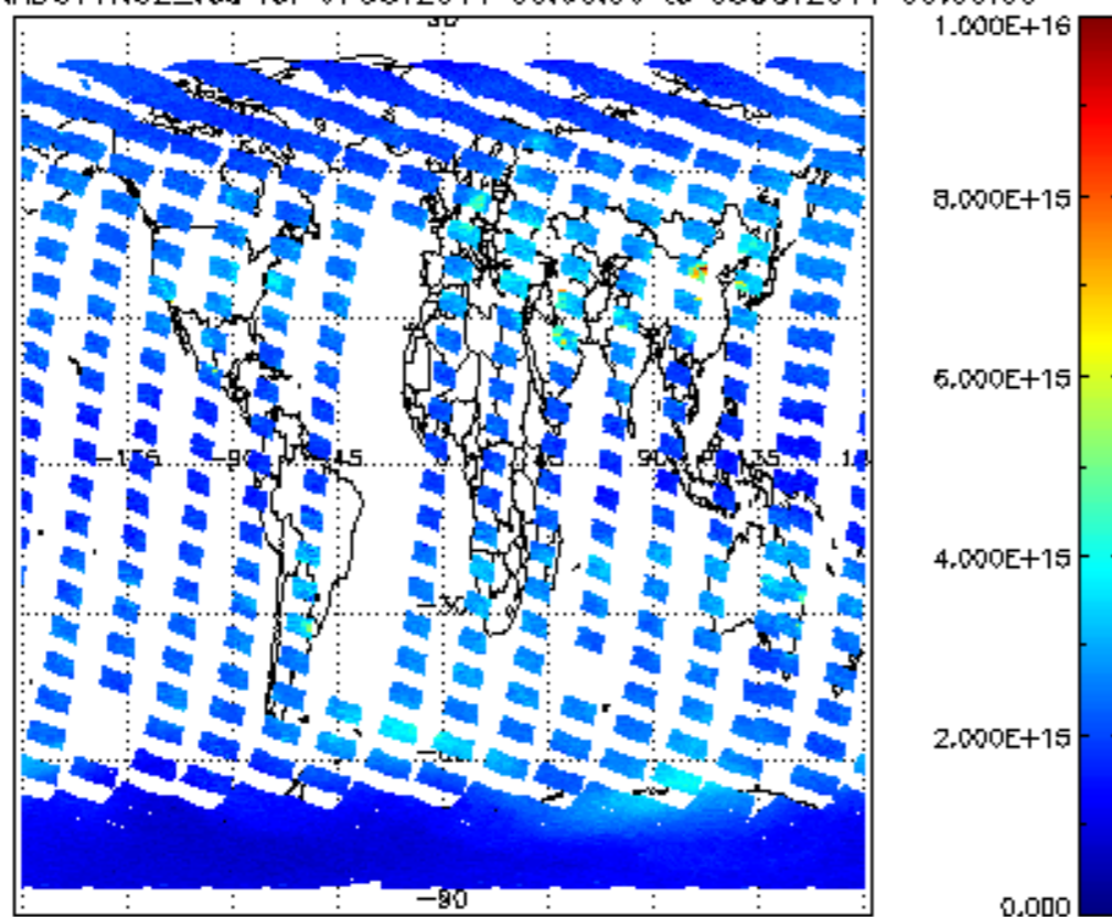
SCIOL2P_NADUV1NO2_vcd for 07OCT2011 00:00:00 to 08OCT2011 00:00:00
