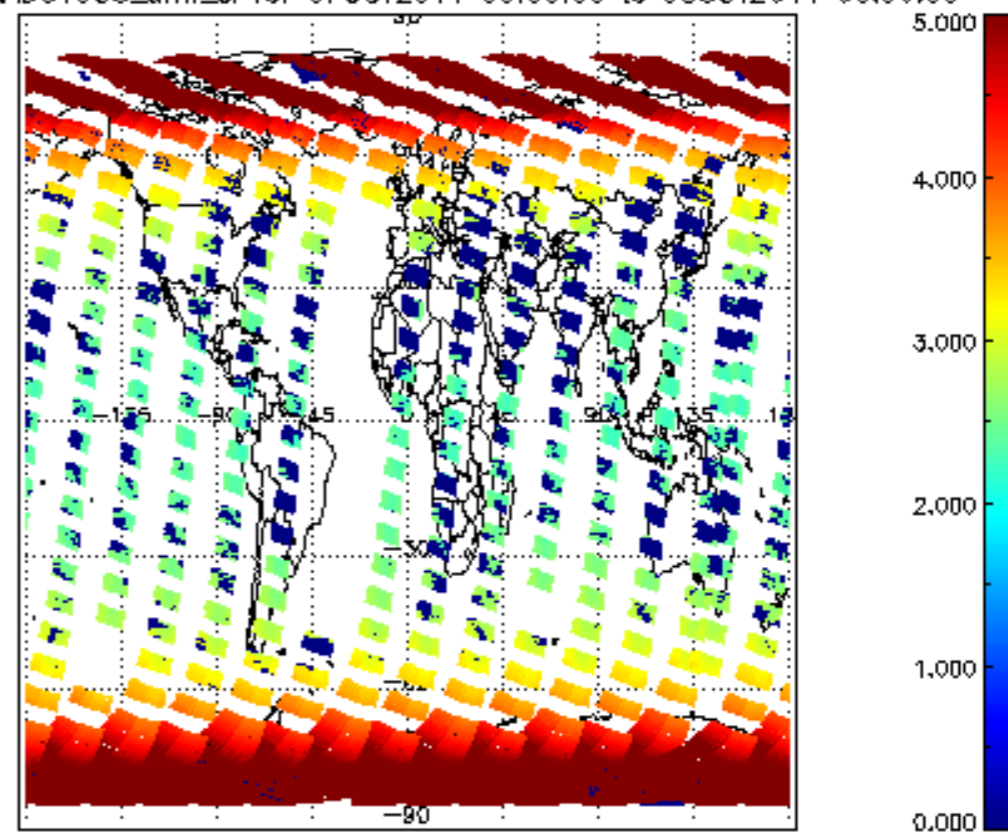
SCIOL2P_NADUV003_amf_cl for 07OCT2011 00:00:00 to 08OCT2011 00:00:00
