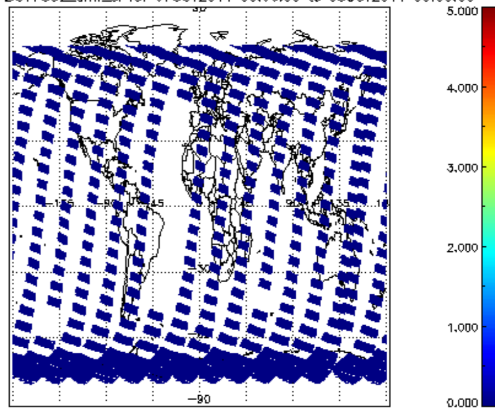
SCIOL2P_NADUV7S02_amf_sl for 07OCT2011 00:00:00 to 08OCT2011 00:00:00
