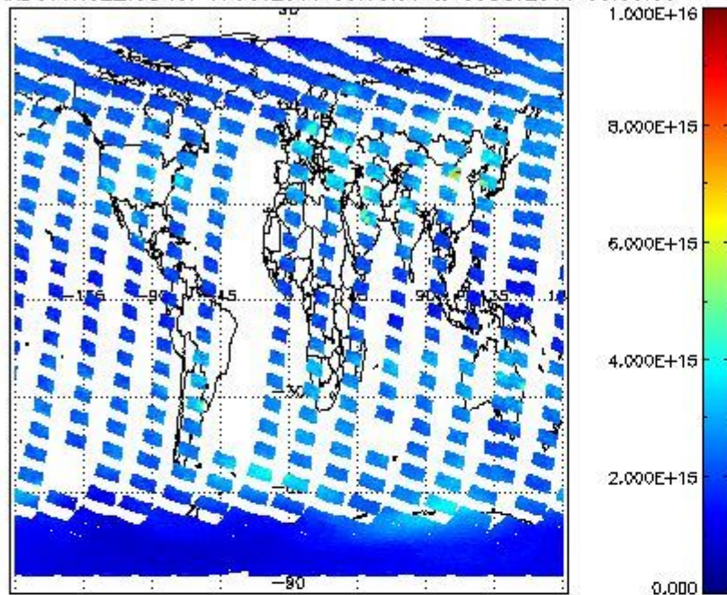
SCIOL2P_NADUV1NO2_vcd for 07OCT2011 00:00:00 to 08OCT2011 00:00:00
