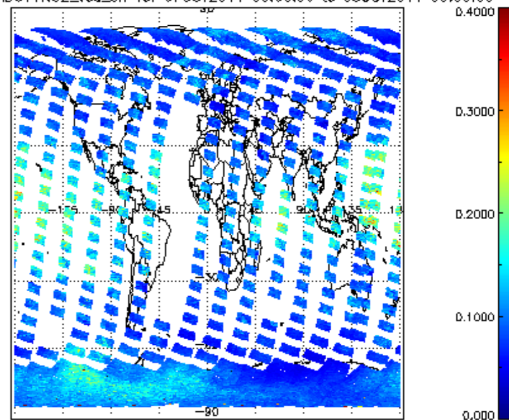
SCIOL2P_NADUV1NO2_vcd_err for 07OCT2011 00:00:00 to 08OCT2011 00:00:00
