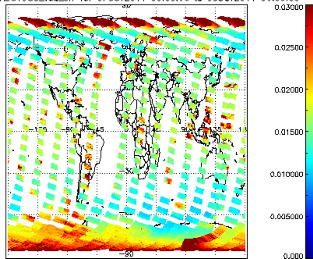
SCIOL2P_NADUV003_vcd_err for 07OCT2011 00:00:00 to 08OCT2011 00:00:00
