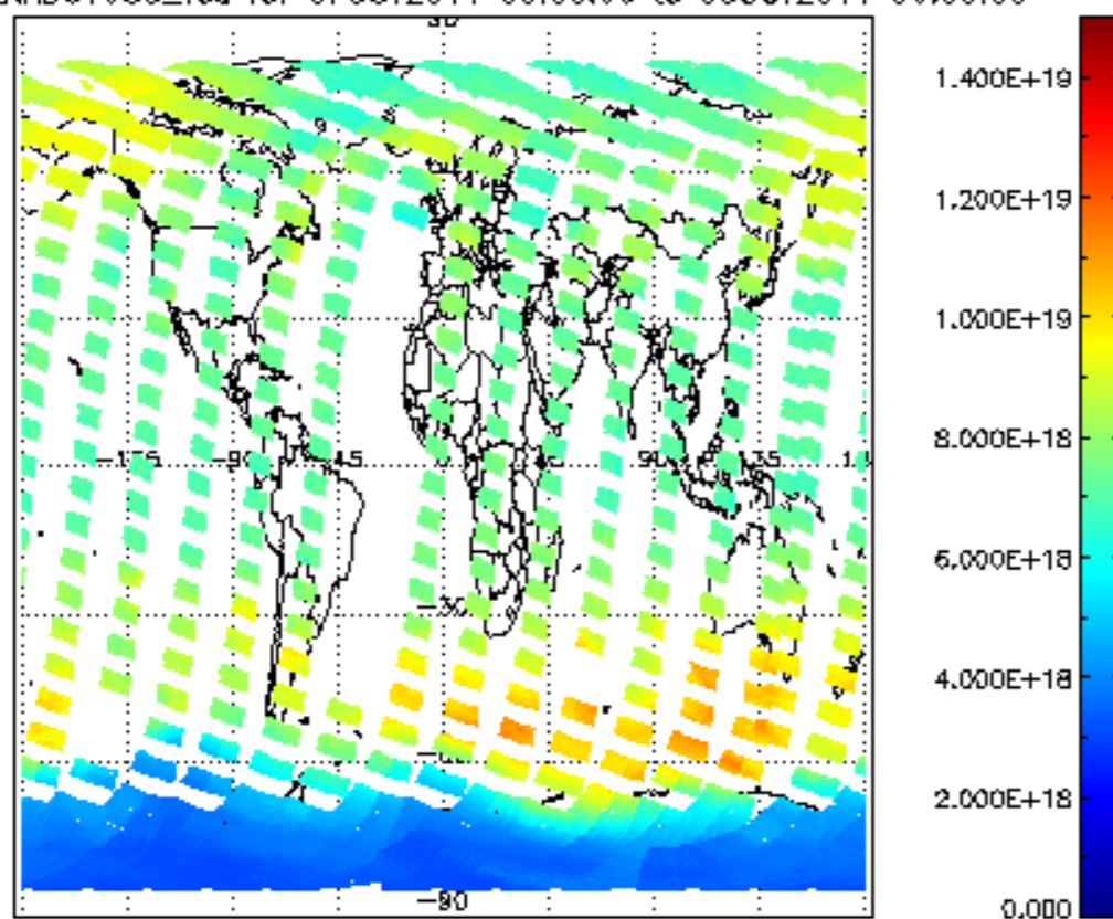
SCIOL2P_NADUV003_vcd for 07OCT2011 00:00:00 to 08OCT2011 00:00:00
