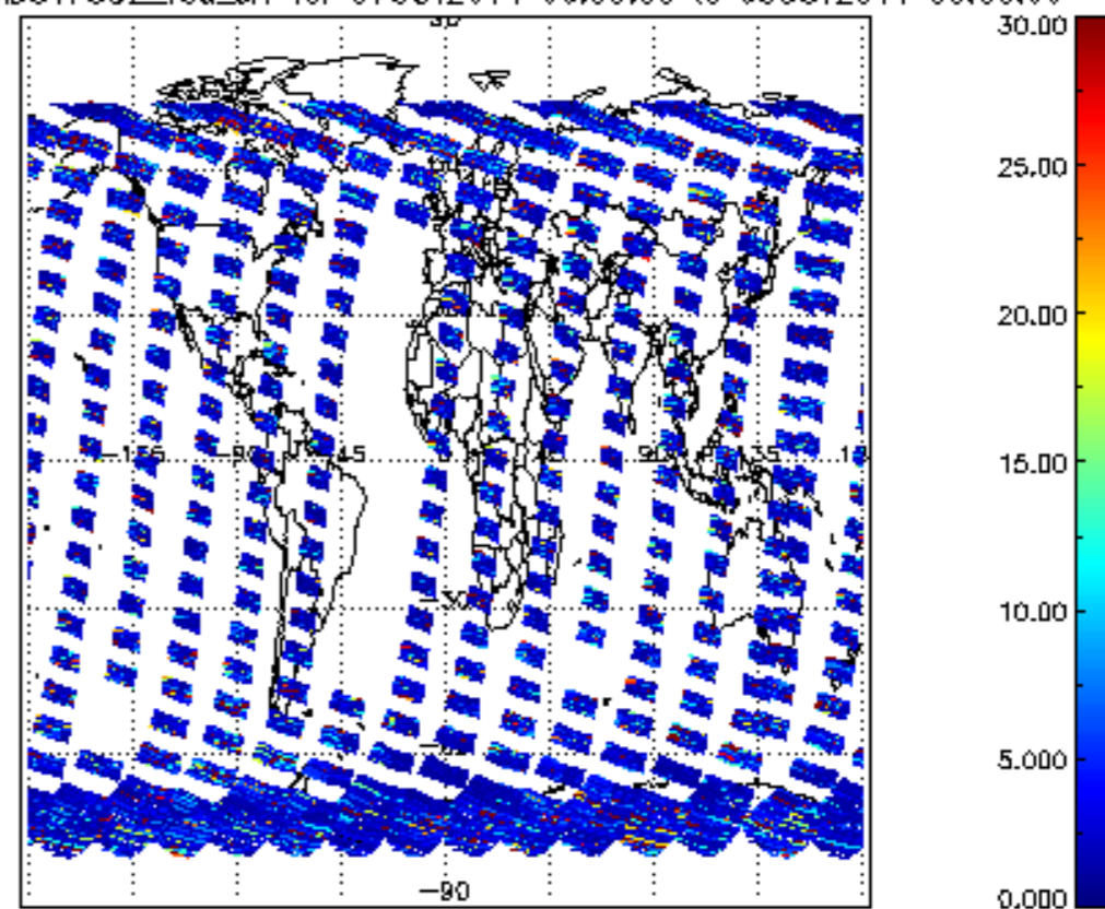
SCIOL2P_NADUV7S02_vcd_err for 07OCT2011 00:00:00 to 08OCT2011 00:00:00
