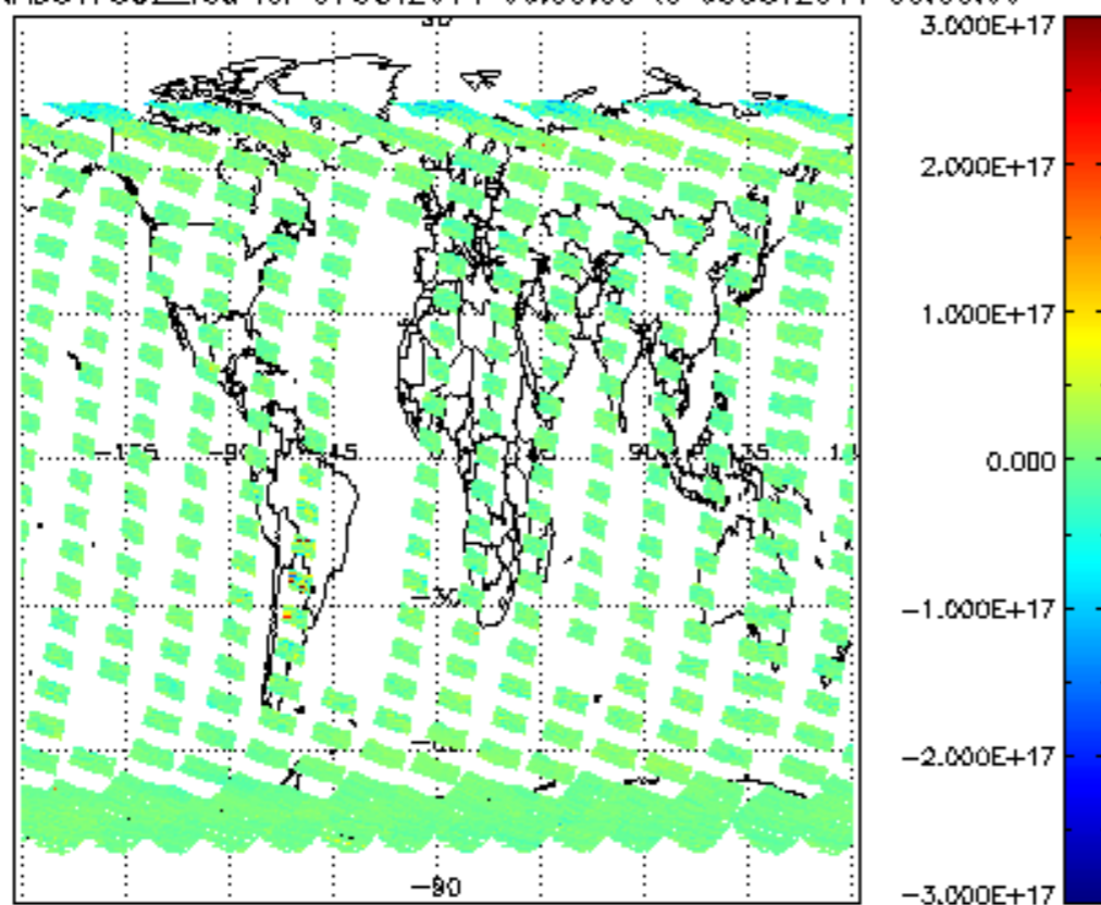
SCIOL2P_NADUV7S02_vcd for 07OCT2011 00:00:00 to 08OCT2011 00:00:00
