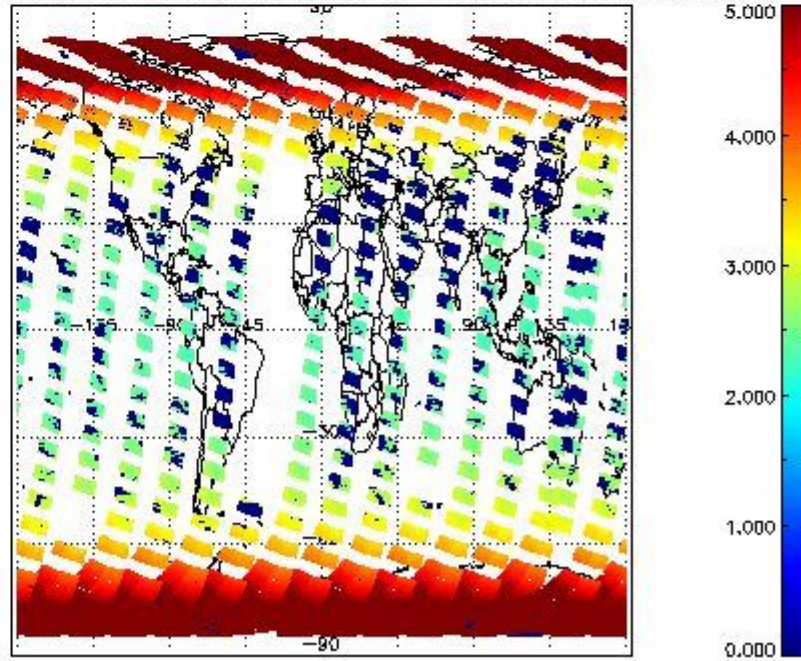
SCIOL2P_NADUV003_amf_cl for 07OCT2011 00:00:00 to 08OCT2011 00:00:00
