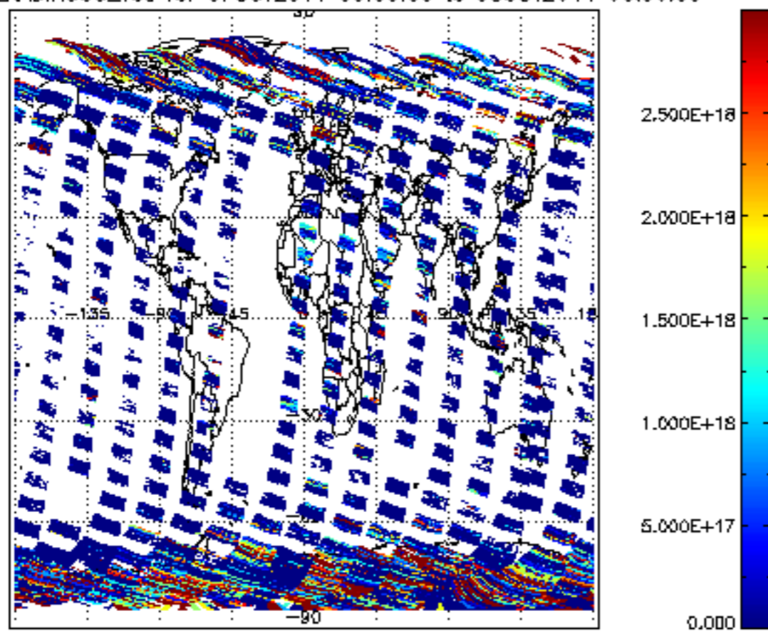
SCIOL2P_NADIR3CO_vcd for 07OCT2011 00:00:00 to 08OCT2011 00:00:00
