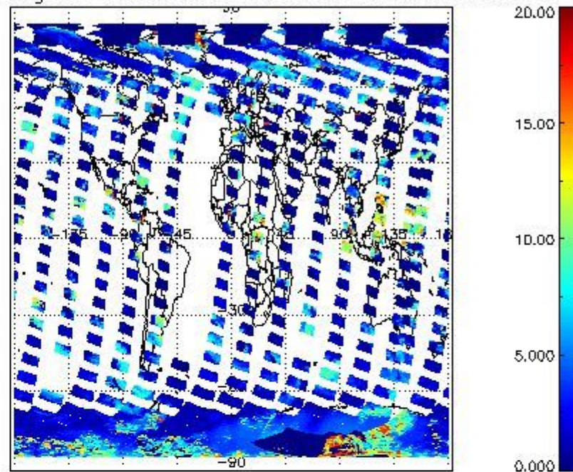
cL_top_height for 07OCT2011 00:00:00 to 08OCT2011 00:00:00
