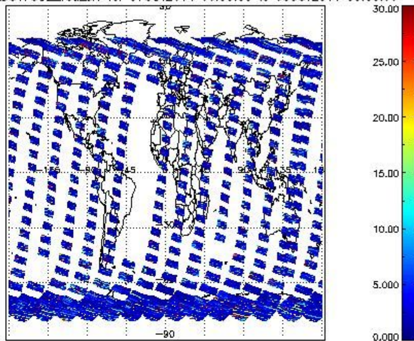
SCIOL2P_NADUV7S02_vcd_err for 07OCT2011 00:00:00 to 08OCT2011 00:00:00
