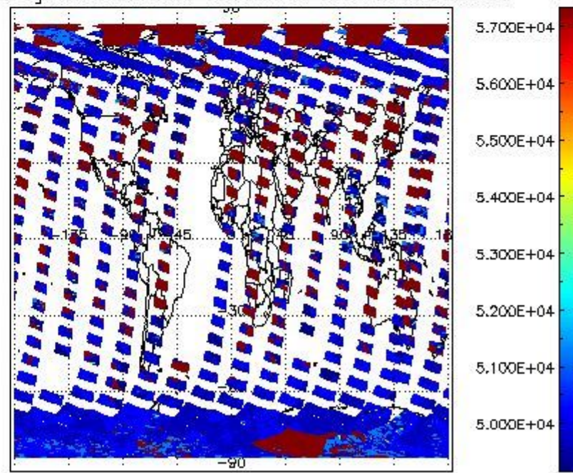
cloud_flags for 07OCT2011 00:00:00 to 08OCT2011 00:00:00
