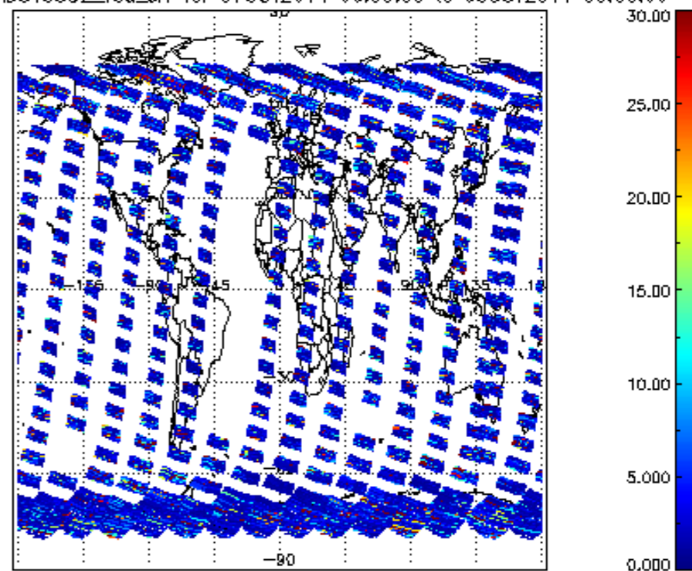
SCIOL2P_NADUV5S02_vcd_err for 07OCT2011 00:00:00 to 08OCT2011 00:00:00
