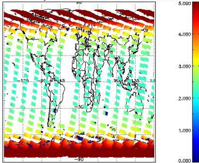
SCIOL2P_NADUV1NO2_amf_gr for 07OCT2011 00:00:00 to 08OCT2011 00:00:00
