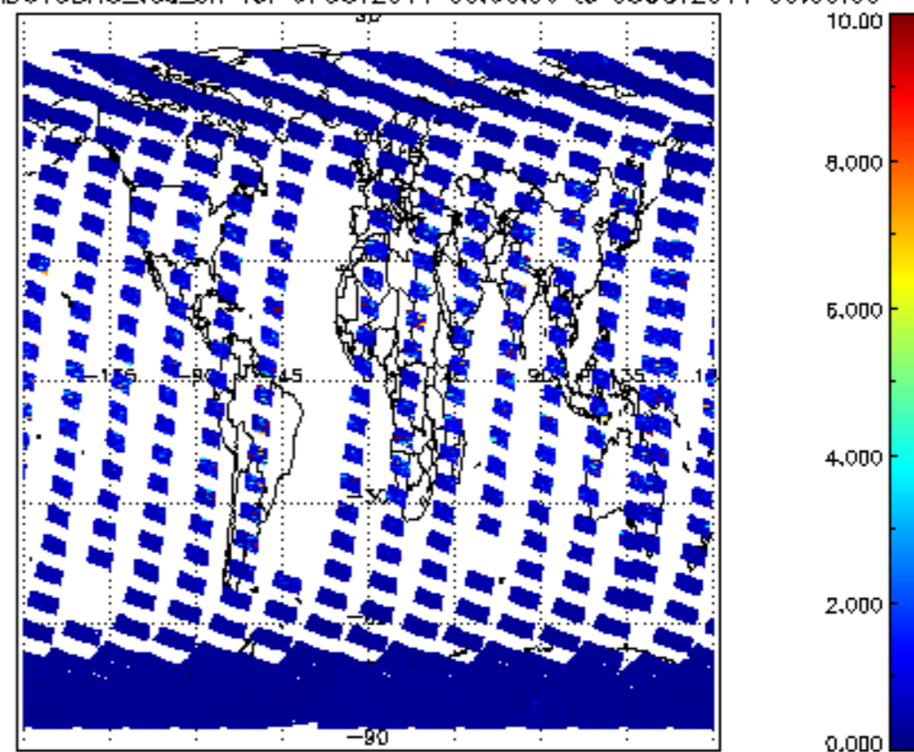
SCIOL2P_NADUV3BRO_vcd_err for 07OCT2011 00:00:00 to 08OCT2011 00:00:00
