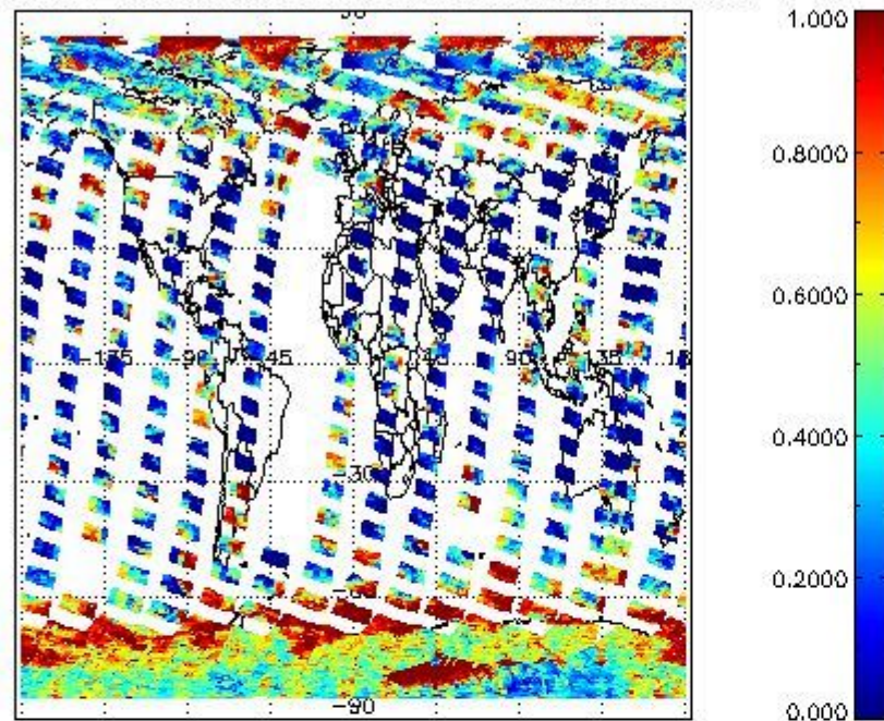
cLfrac for 07OCT2011 00:00:00 to 08OCT2011 00:00:00
