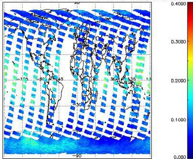
SCIOL2P_NADUV1NO2_vcd_err for 07OCT2011 00:00:00 to 08OCT2011 00:00:00
