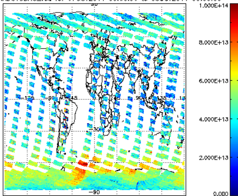
SCIOL2P_NADUV3BRO_vcd for 07OCT2011 00:00:00 to 08OCT2011 00:00:00
