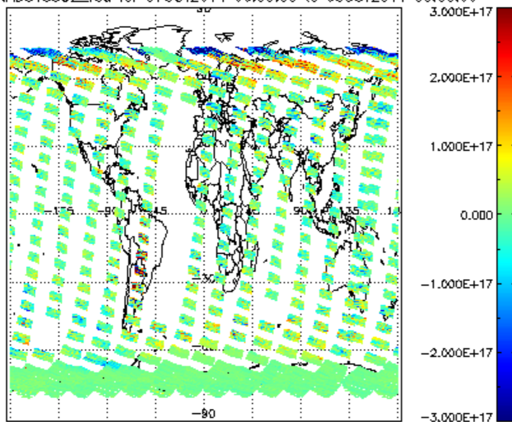
SCIOL2P_NADUV5S02_vcd for 07OCT2011 00:00:00 to 08OCT2011 00:00:00
