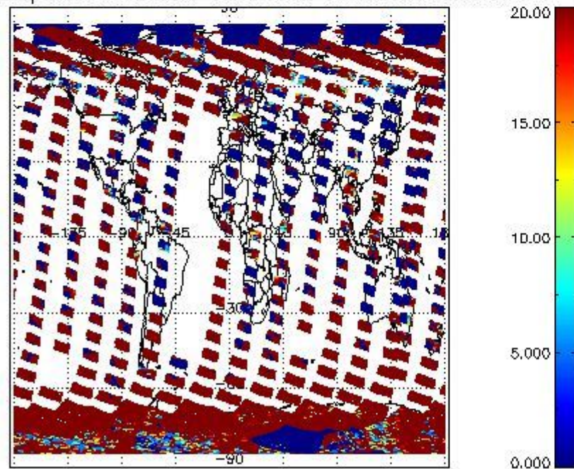
cL_opt_depth for 07OCT2011 00:00:00 to 08OCT2011 00:00:00
