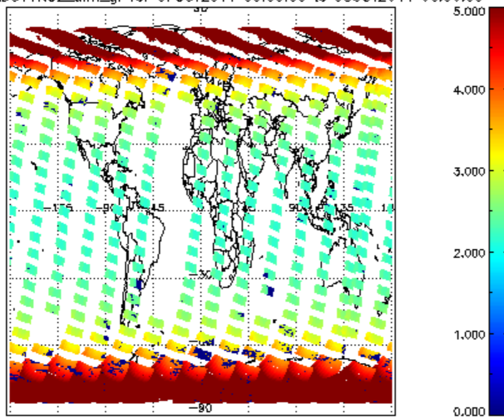
SCIOL2P_NADUV1NO2_amf_gr for 07OCT2011 00:00:00 to 08OCT2011 00:00:00
