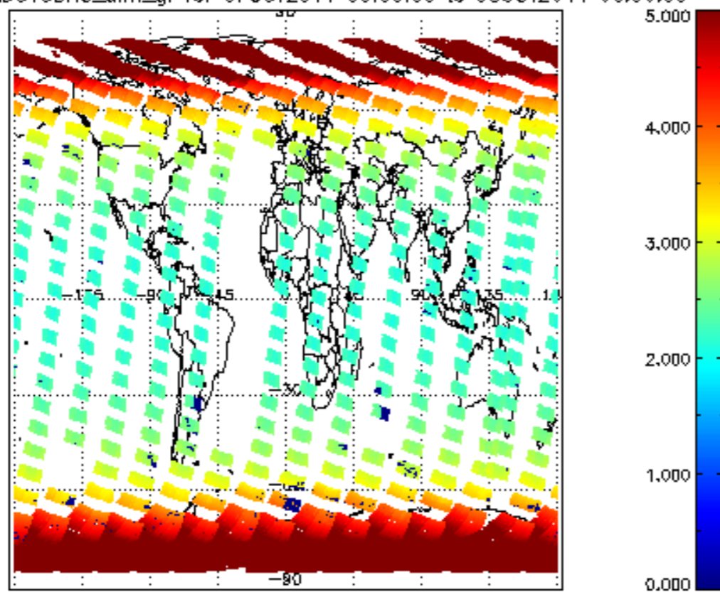
SCIOL2P_NADUV3BRO_amf_gr for 07OCT2011 00:00:00 to 08OCT2011 00:00:00
