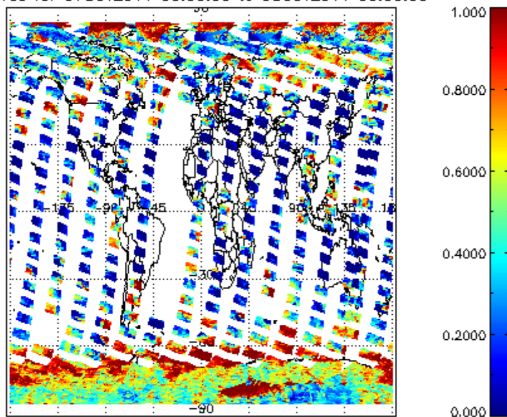
cl_frac for 07OCT2011 00:00:00 to 08OCT2011 00:00:00
