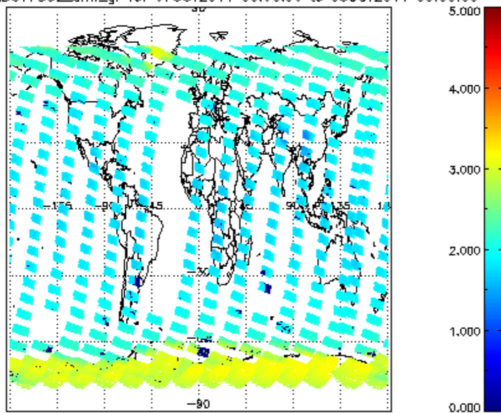
SCIOL2P_NADUV7S02_amf_gr for 07OCT2011 00:00:00 to 08OCT2011 00:00:00
