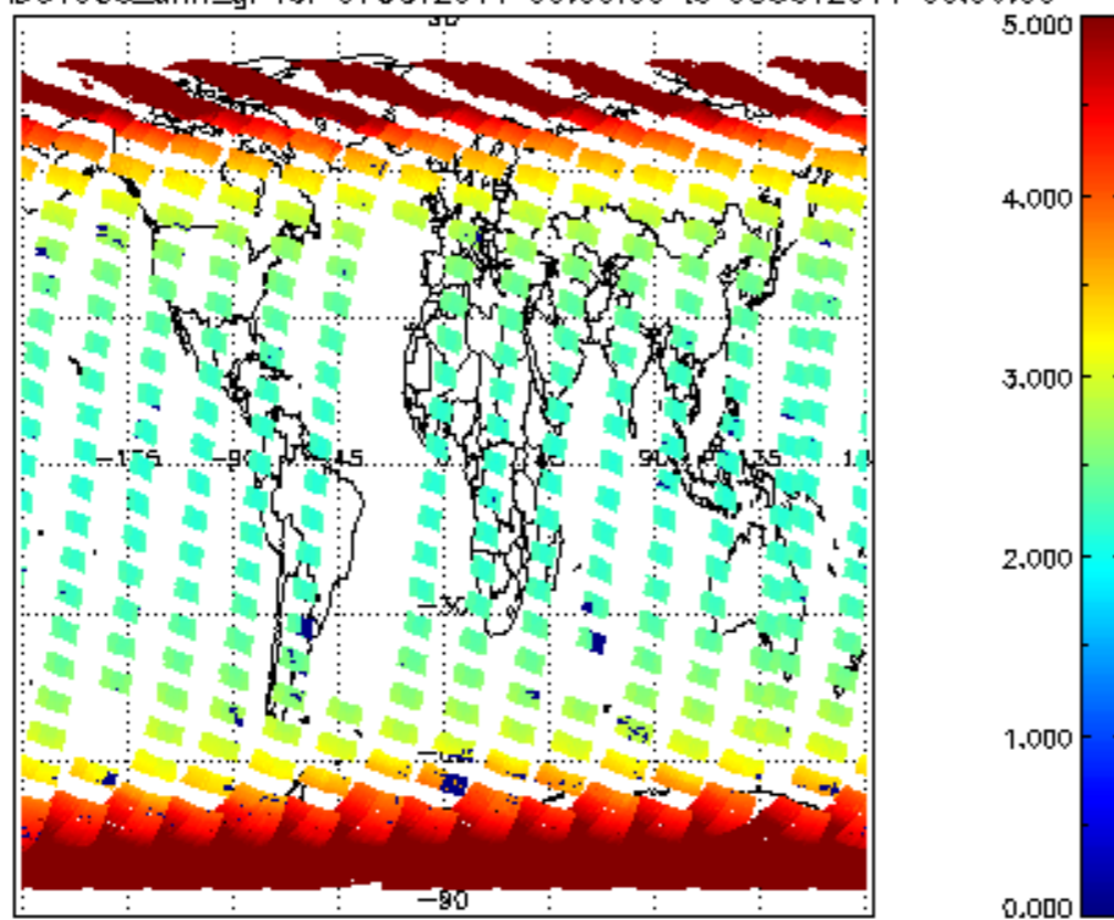
SCIOL2P_NADUV003_amf_gr for 07OCT2011 00:00:00 to 08OCT2011 00:00:00
