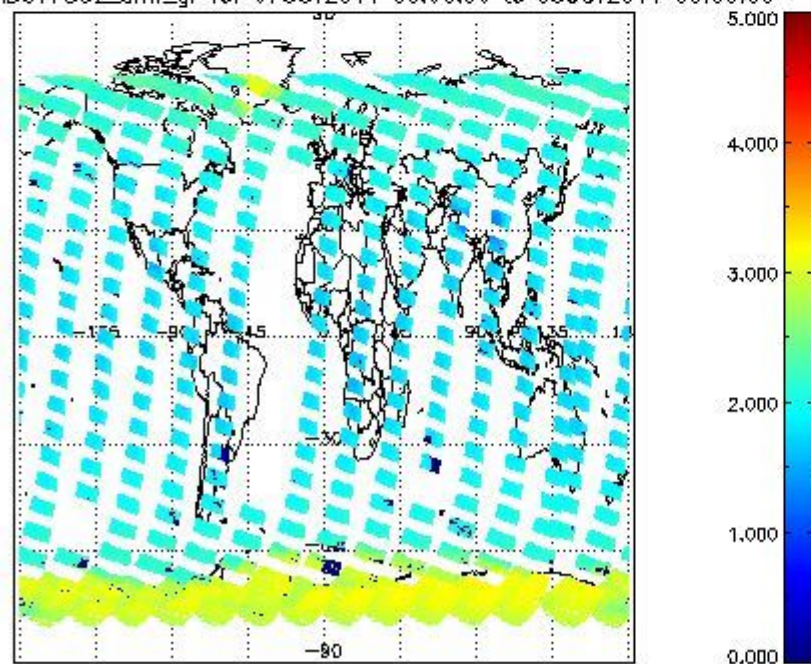
SCIOL2P_NADUV7S02_amf_gr for 07OCT2011 00:00:00 to 08OCT2011 00:00:00
