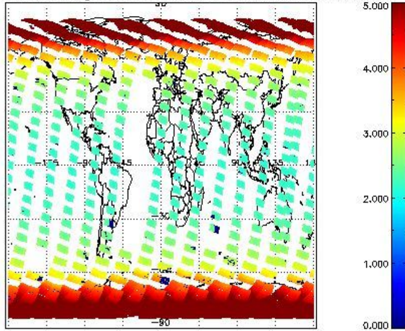
SCIOL2P_NADUV003_amf_gr for 07OCT2011 00:00:00 to 08OCT2011 00:00:00
