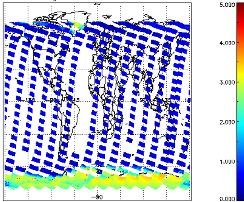
SCIOL2P_NADUV5S02_amf_gr for 07OCT2011 00:00:00 to 08OCT2011 00:00:00
