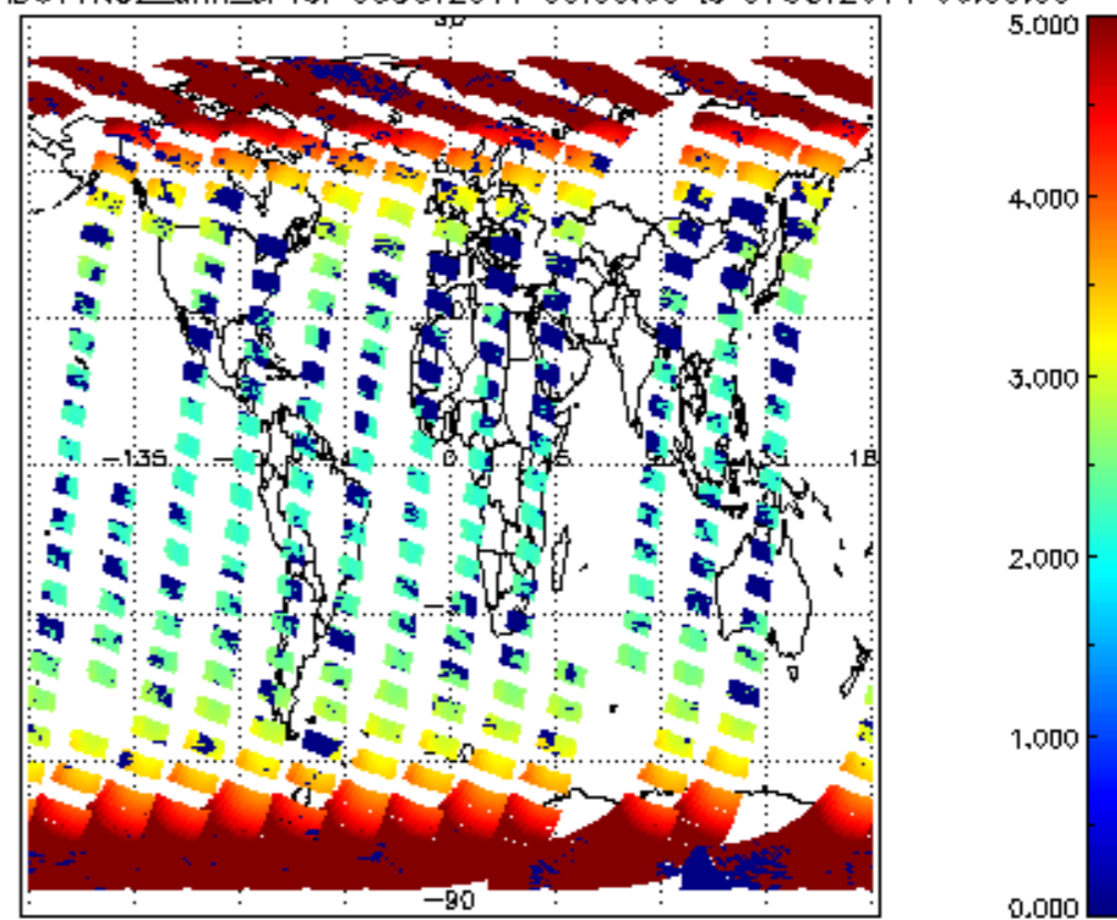
SCIOL2P_NADUV1NO2_amf_cl for 06OCT2011 00:00:00 to 07OCT2011 00:00:00
