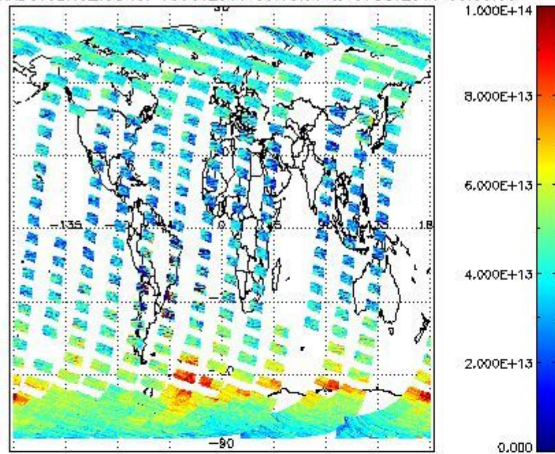
SCIOL2P_NADUV3BRO_vcd for 06OCT2011 00:00:00 to 07OCT2011 00:00:00
