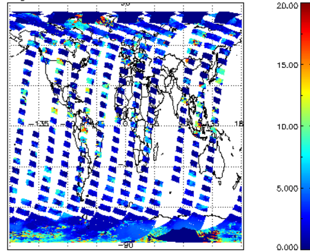
cl_top_height for 06OCT2011 00:00:00 to 07OCT2011 00:00:00
