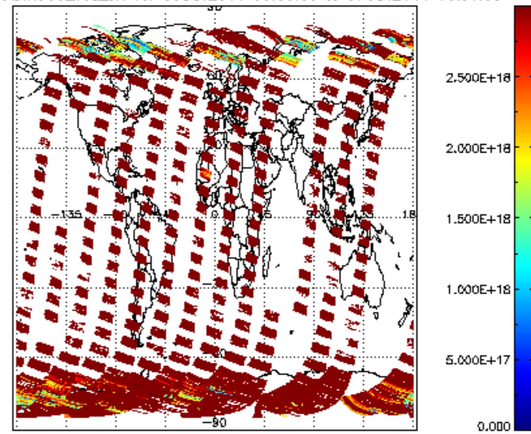
SCIOL2P_NADIR3CO_vcd_err for 06OCT2011 00:00:00 to 07OCT2011 00:00:00
