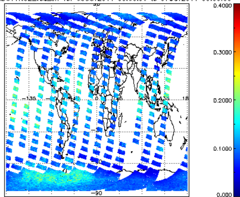
SCIOL2P_NADUV1NO2_vcd_err for 06OCT2011 00:00:00 to 07OCT2011 00:00:00
