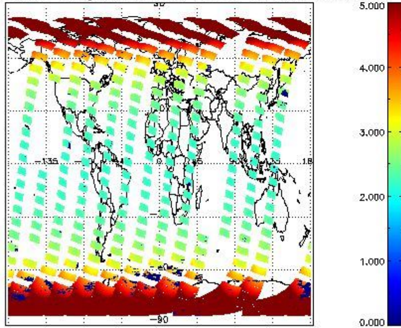
SCIOL2P_NADUV1NO2_amf_gr for 06OCT2011 00:00:00 to 07OCT2011 00:00:00
