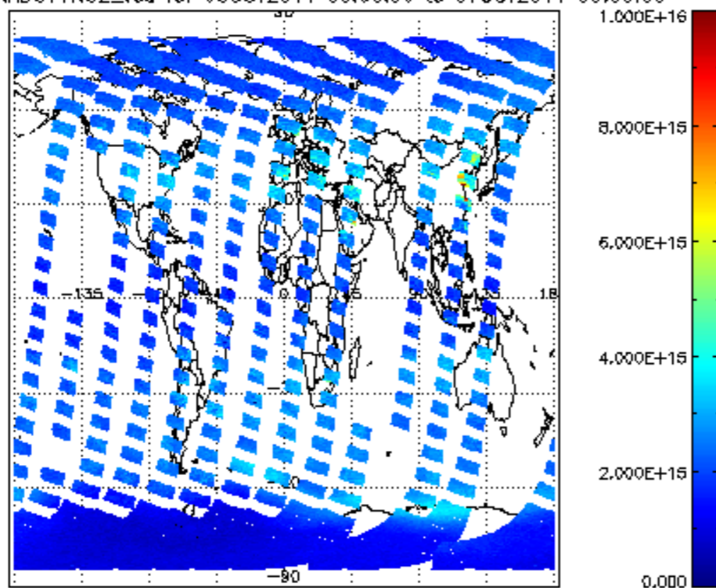
SCIOL2P_NADUV1NO2_vcd for 06OCT2011 00:00:00 to 07OCT2011 00:00:00
