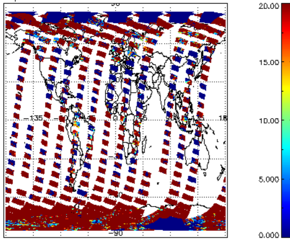
cl_opt_depth for 06OCT2011 00:00:00 to 07OCT2011 00:00:00
