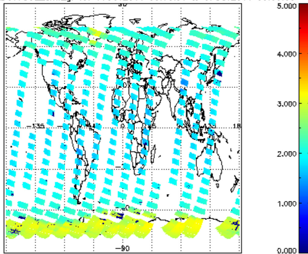
SCIOL2P_NADUV7S02_amf_gr for 06OCT2011 00:00:00 to 07OCT2011 00:00:00
