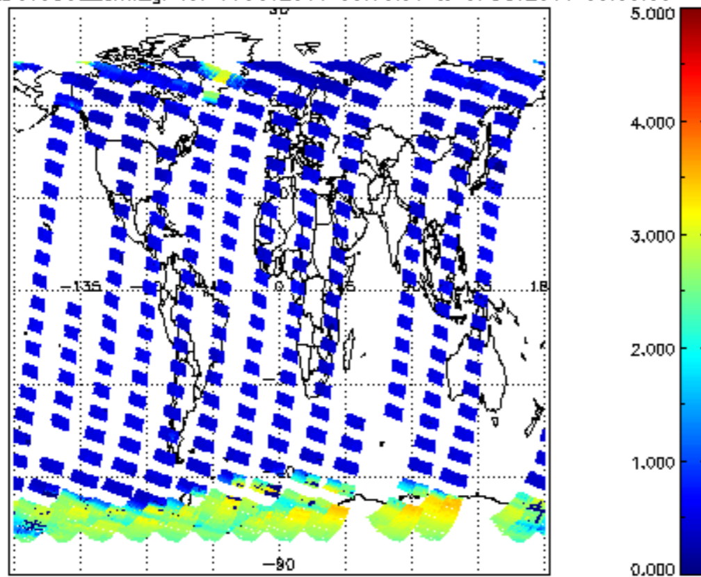
SCIOL2P_NADUV5S02_amf_gr for 06OCT2011 00:00:00 to 07OCT2011 00:00:00
