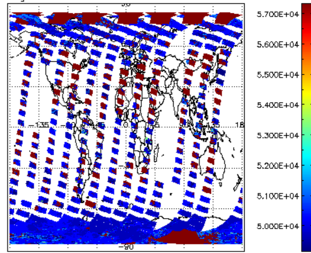
cloud_flags for 06OCT2011 00:00:00 to 07OCT2011 00:00:00
