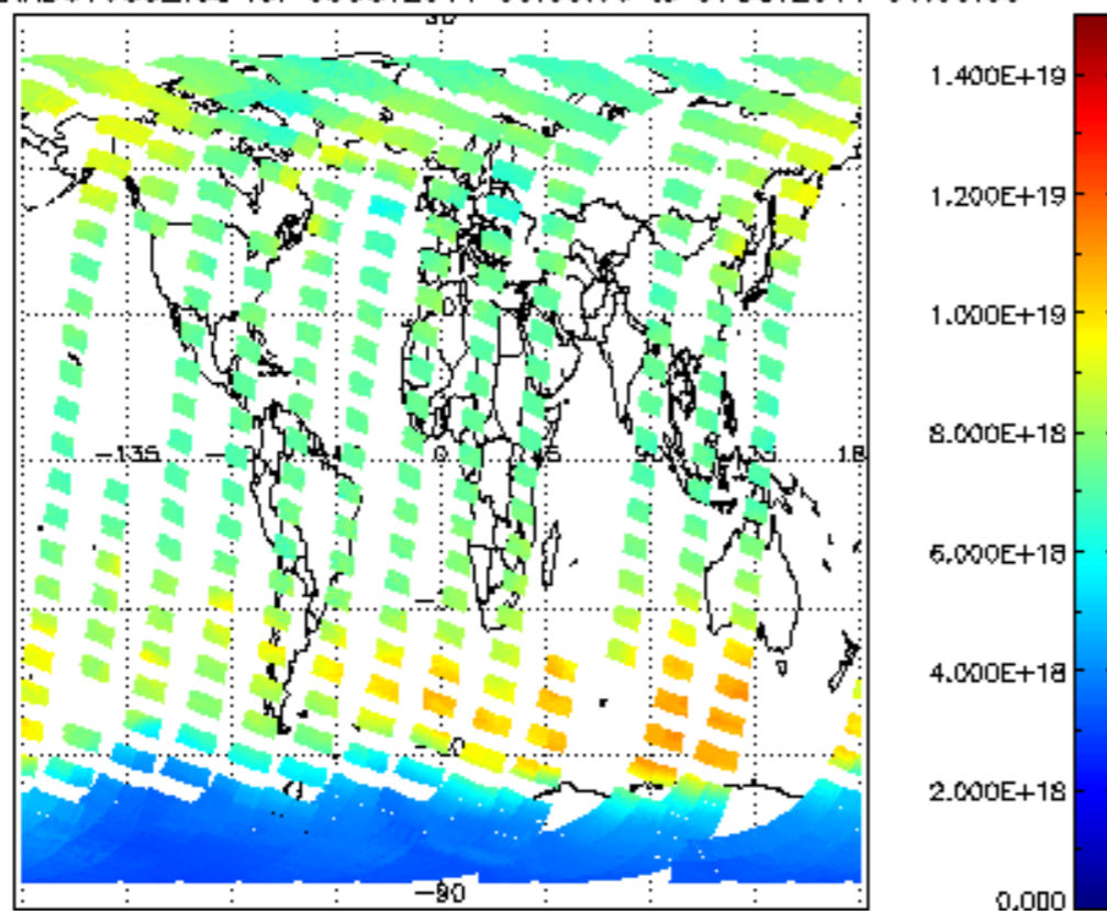
SCIOL2P_NADUV003_vcd for 06OCT2011 00:00:00 to 07OCT2011 00:00:00
