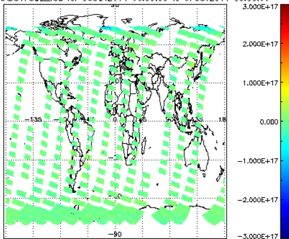
SCIOL2P_NADUV7S02_vcd for 06OCT2011 00:00:00 to 07OCT2011 00:00:00
