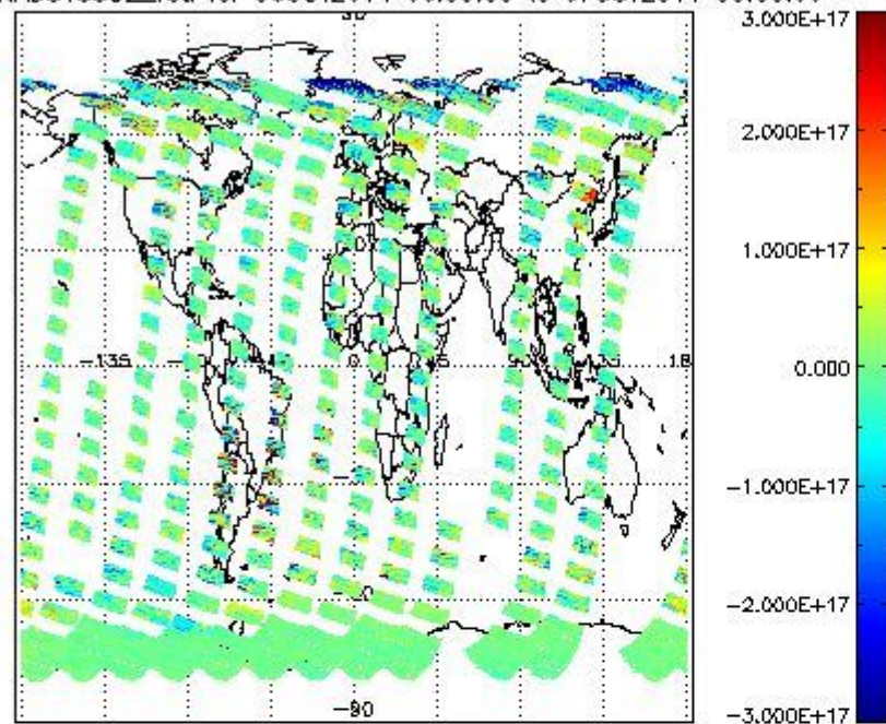
SCIOL2P_NADUV5S02_vcd for 06OCT2011 00:00:00 to 07OCT2011 00:00:00
