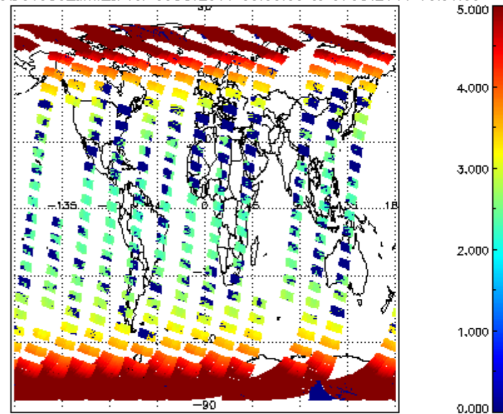
SCIOL2P_NADUV003_amf_cl for 06OCT2011 00:00:00 to 07OCT2011 00:00:00
