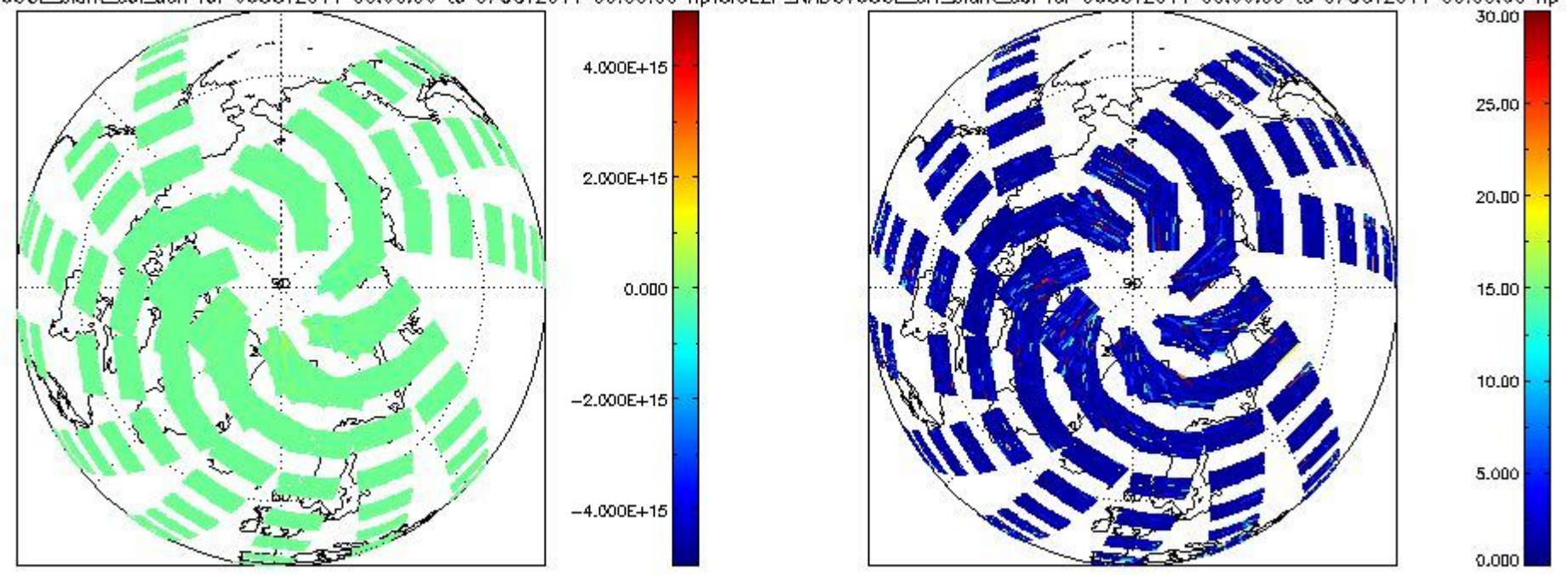
CIOL2P_NADUV60CL_slant_col_den for 06OCT2011 00:00:00 to 07OCT2011 00:00:00 np CIOL2P_NADUV60CL_err_slant_col for 06OCT2011 00:00:00 to 07OCT2011 00:00:00 np
