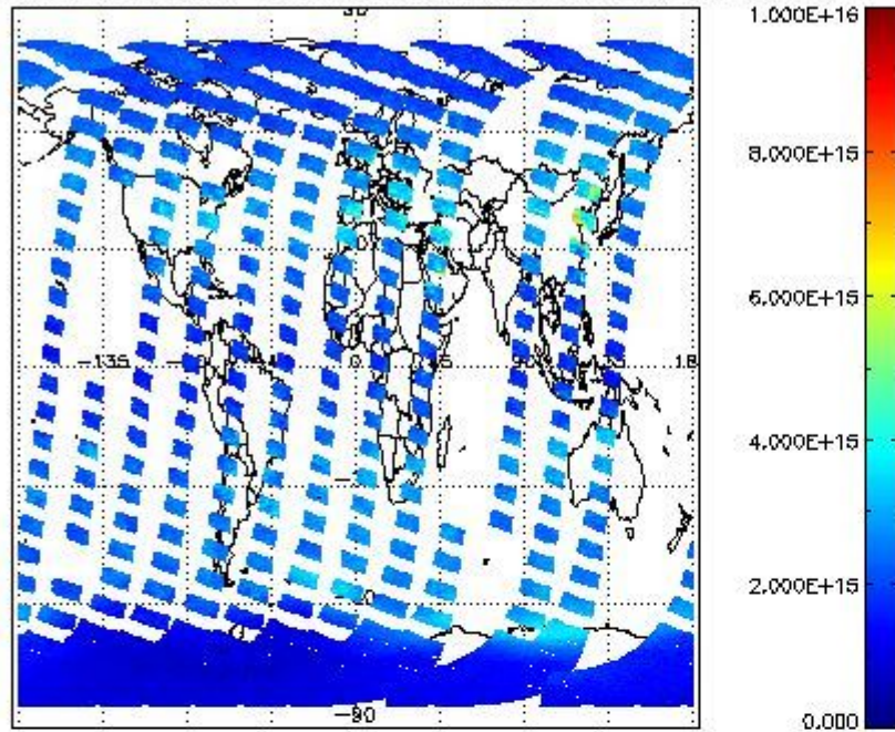
SCIOL2P_NADUV1NO2_vcd for 06OCT2011 00:00:00 to 07OCT2011 00:00:00
