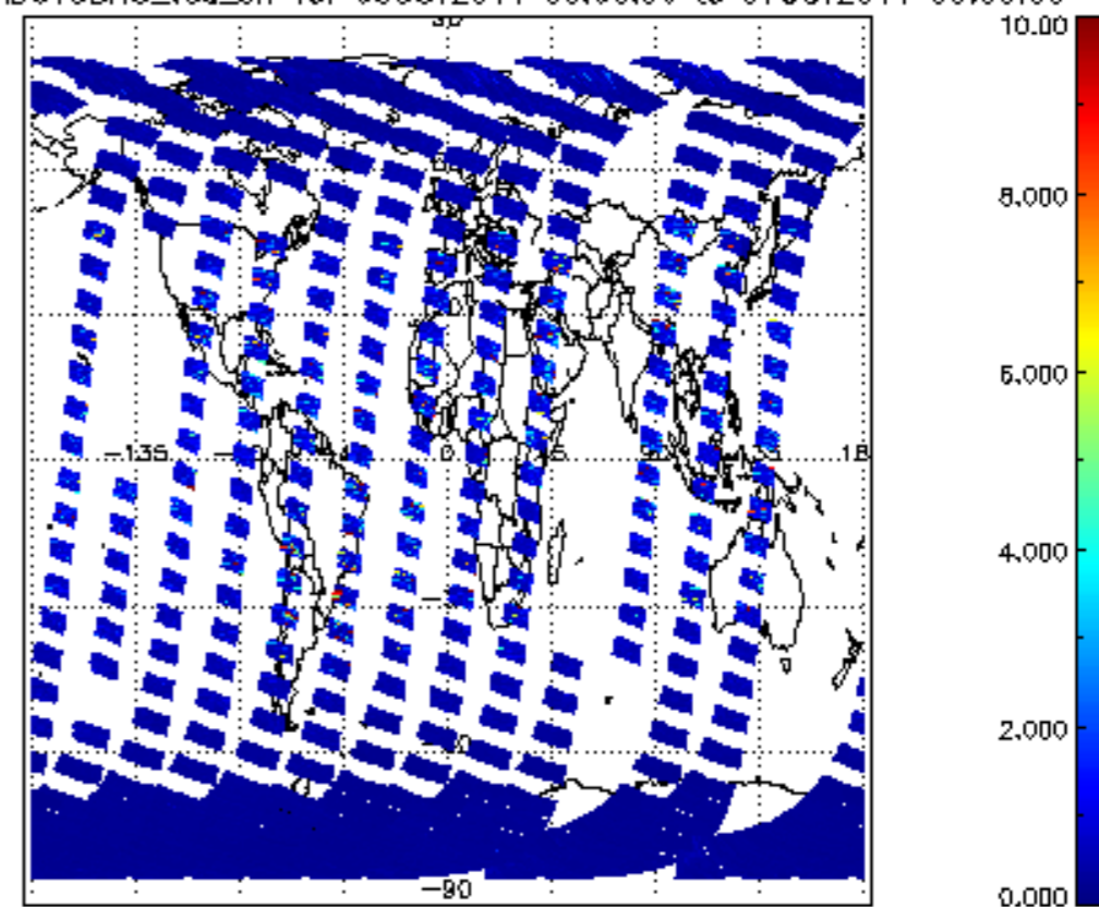
SCIOL2P_NADUV3BRO_vcd_err for 06OCT2011 00:00:00 to 07OCT2011 00:00:00
