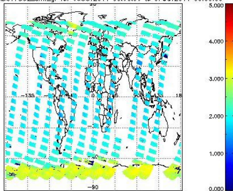
SCIOL2P_NADUV7S02_amf_gr for 06OCT2011 00:00:00 to 07OCT2011 00:00:00
