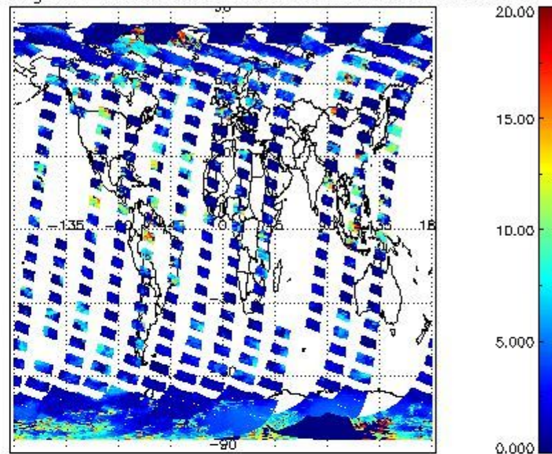
cL_top_height for 06OCT2011 00:00:00 to 07OCT2011 00:00:00
