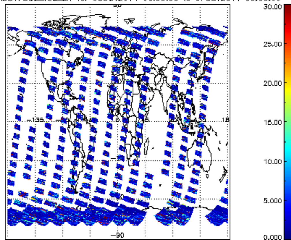
SCIOL2P_NADUV7S02_vcd_err for 06OCT2011 00:00:00 to 07OCT2011 00:00:00
