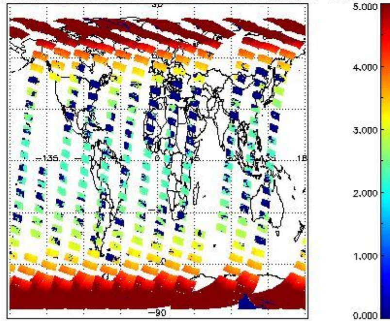
SCIOL2P_NADUV3BRO_amf_cl for 06OCT2011 00:00:00 to 07OCT2011 00:00:00
