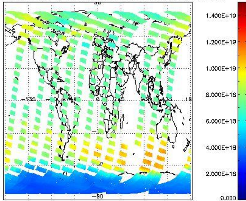
SCIOL2P_NADUV003_vcd for 06OCT2011 00:00:00 to 07OCT2011 00:00:00
