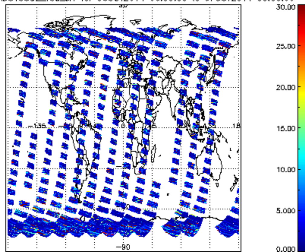
SCIOL2P_NADUV5S02_vcd_err for 06OCT2011 00:00:00 to 07OCT2011 00:00:00
