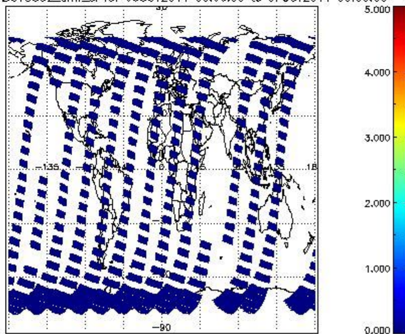
SCIOL2P_NADUV5S02_amf_cl for 06OCT2011 00:00:00 to 07OCT2011 00:00:00
