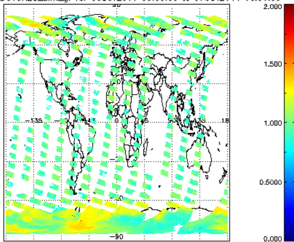
SCIOL2P_NADUV8H20_amf_gr for 06OCT2011 00:00:00 to 07OCT2011 00:00:00
