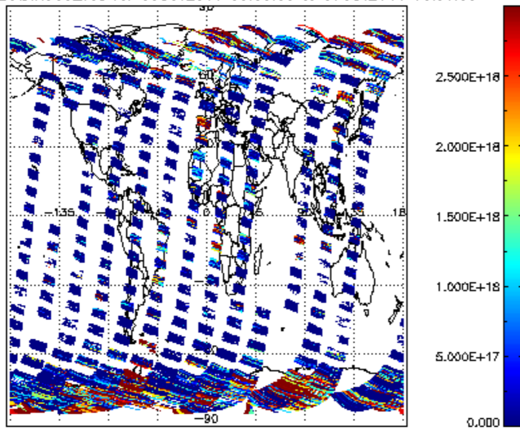
SCIOL2P_NADIR3CO_vcd for 06OCT2011 00:00:00 to 07OCT2011 00:00:00
