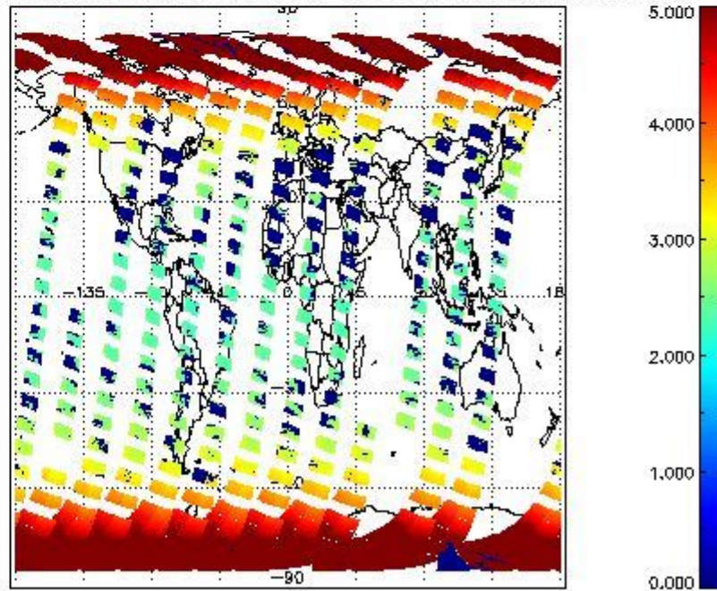
SCIOL2P_NADUV003_amf_cl for 06OCT2011 00:00:00 to 07OCT2011 00:00:00
