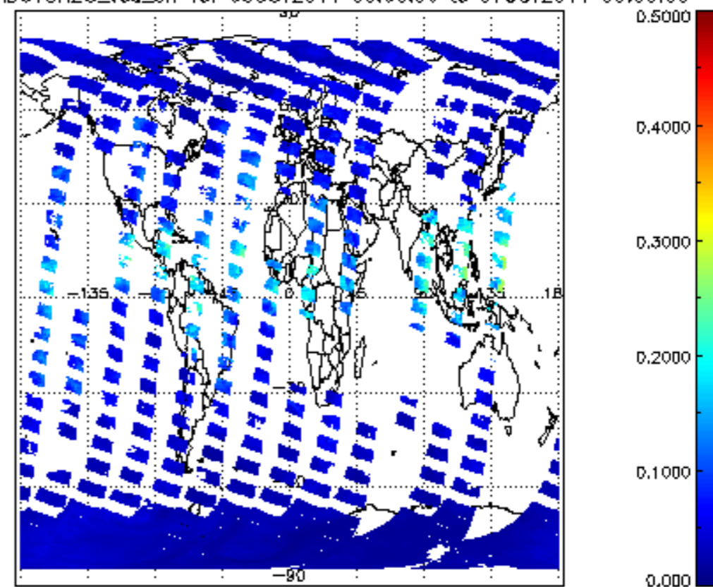
SCIOL2P_NADUV8H20_vcd_err for 06OCT2011 00:00:00 to 07OCT2011 00:00:00
