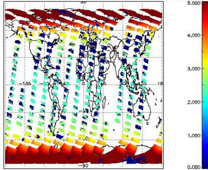
SCIOL2P_NADUV1NO2_amf_cl for 06OCT2011 00:00:00 to 07OCT2011 00:00:00
