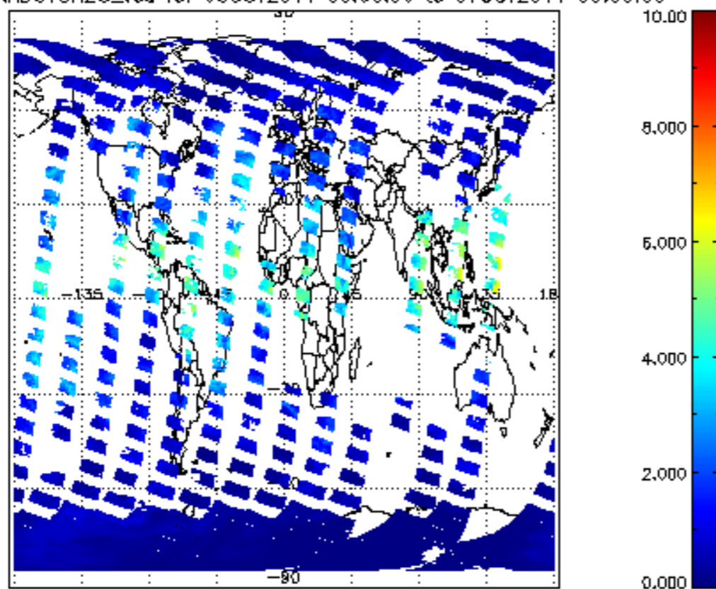
SCIOL2P_NADUV8H20_vcd for 06OCT2011 00:00:00 to 07OCT2011 00:00:00
