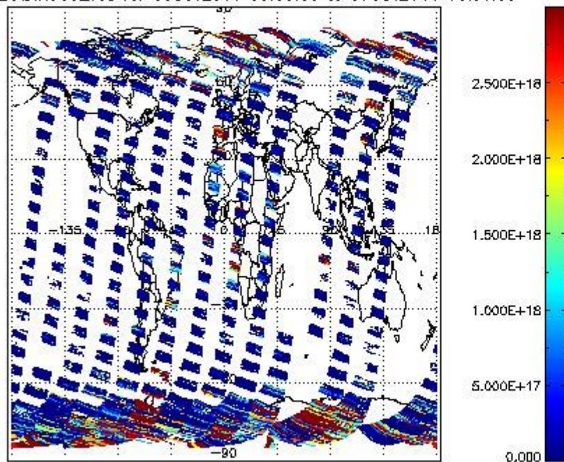
SCIDL2P_NADIR3CO_vcd for 06OCT2011 00:00:00 to 07OCT2011 00:00:00
