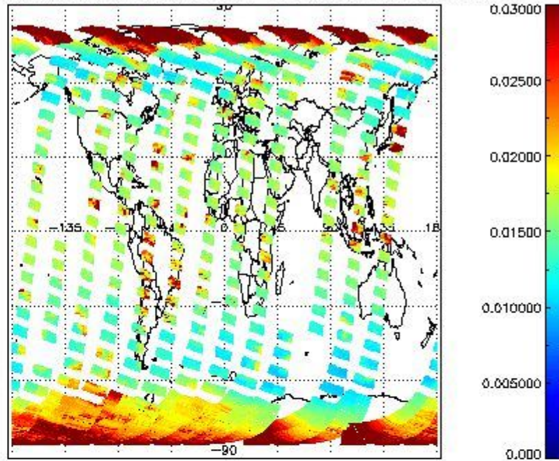
SCIOL2P_NADUV003_vcd_err for 06OCT2011 00:00:00 to 07OCT2011 00:00:00
