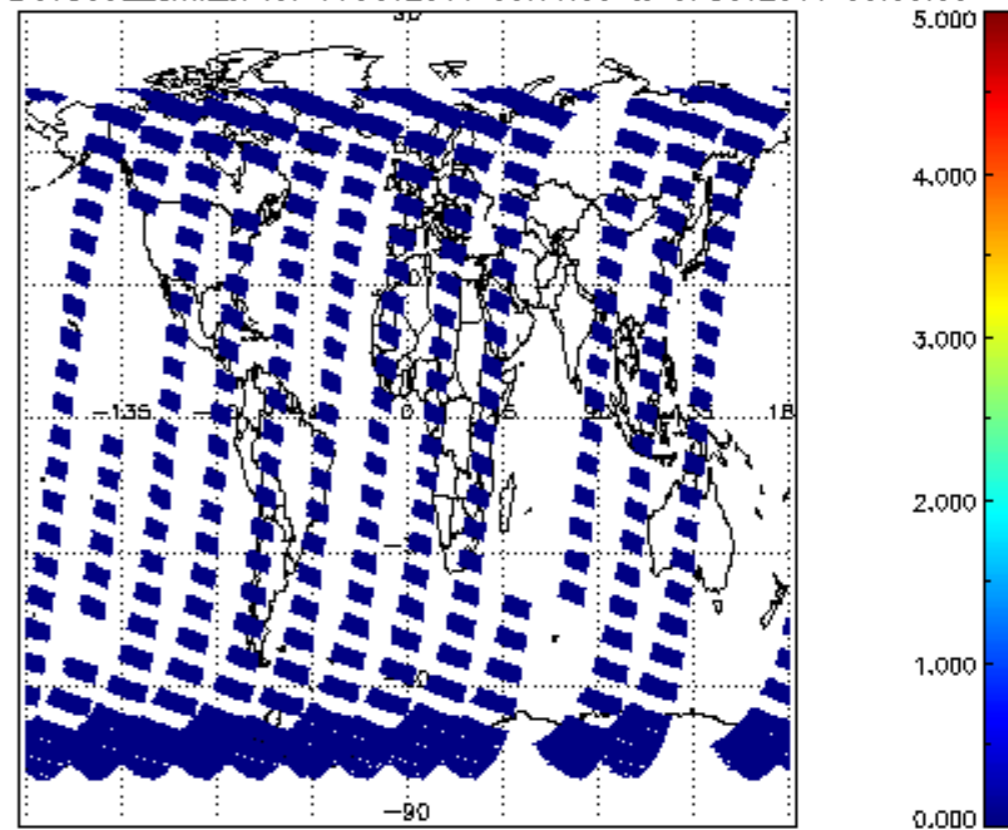
SCIOL2P_NADUV5S02_amf_cl for 06OCT2011 00:00:00 to 07OCT2011 00:00:00
