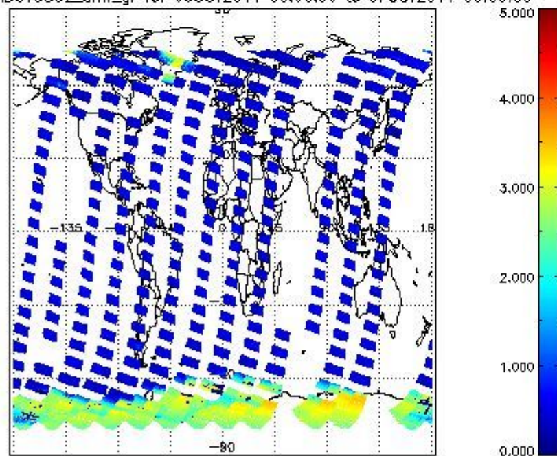
SCIOL2P_NADUV5S02_amf_gr for 06OCT2011 00:00:00 to 07OCT2011 00:00:00
