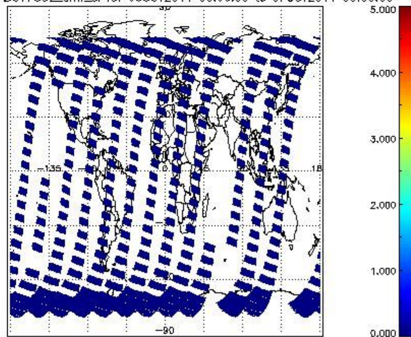
SCIOL2P_NADUV7S02_amf_cl for 06OCT2011 00:00:00 to 07OCT2011 00:00:00
