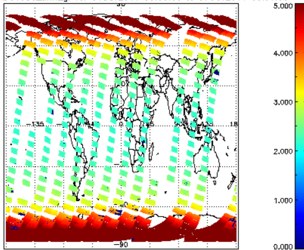
SCIOL2P_NADUV003_amf_gr for 06OCT2011 00:00:00 to 07OCT2011 00:00:00
