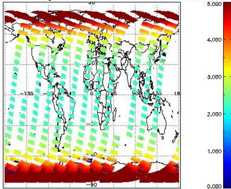
SCIOL2P_NADUV003_amf_gr for 06OCT2011 00:00:00 to 07OCT2011 00:00:00
