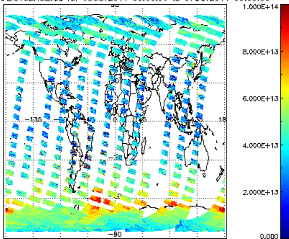
SCIOL2P_NADUV3BRO_vcd for 06OCT2011 00:00:00 to 07OCT2011 00:00:00
