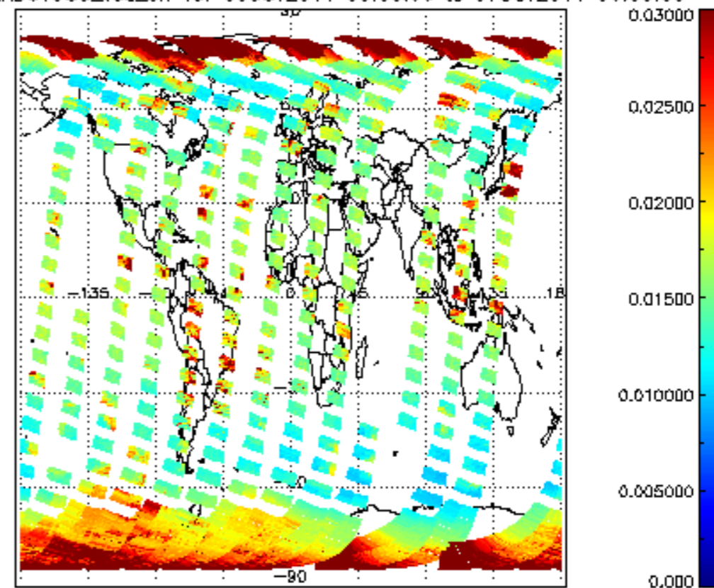
SCIOL2P_NADUV003_vcd_err for 06OCT2011 00:00:00 to 07OCT2011 00:00:00
