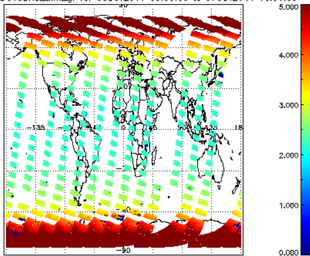
SCIOL2P_NADUV3BRO_amf_gr for 06OCT2011 00:00:00 to 07OCT2011 00:00:00
