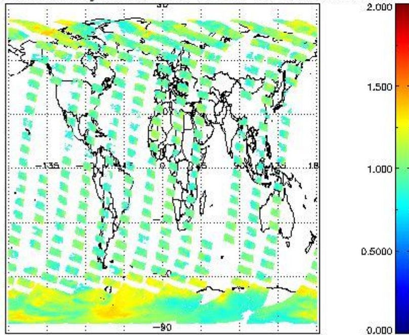
SCIOL2P_NADUV8H2O_amf_gr for 06OCT2011 00:00:00 to 07OCT2011 00:00:00
