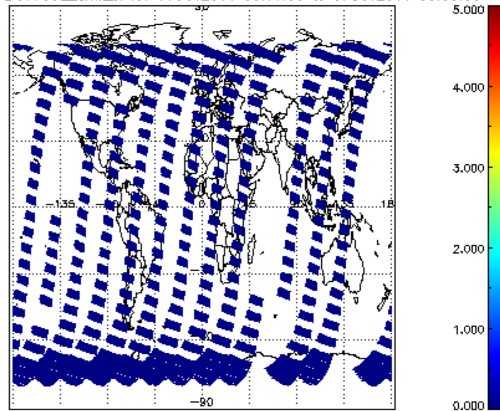
SCIOL2P_NADUV7S02_amf_cl for 06OCT2011 00:00:00 to 07OCT2011 00:00:00
