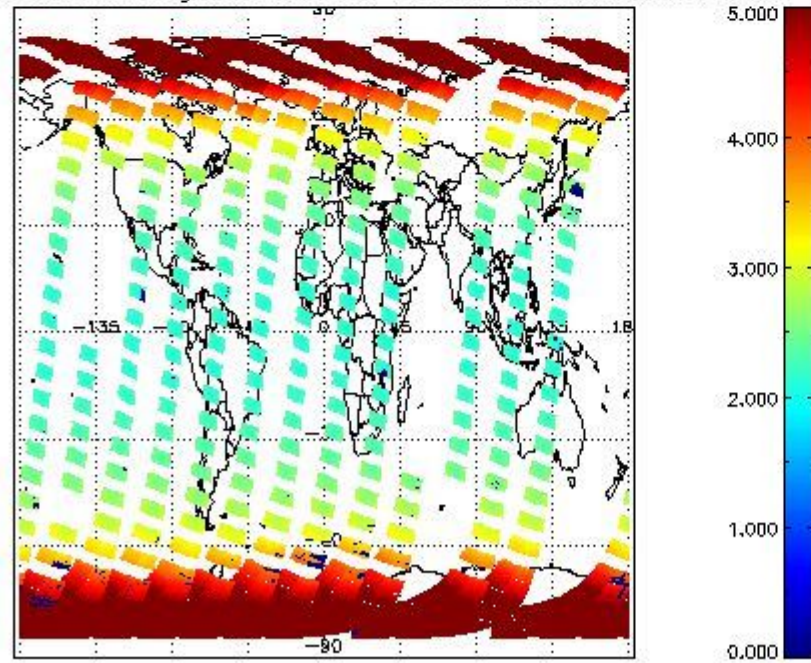
SCIOL2P_NADUV3BRO_amf_gr for 06OCT2011 00:00:00 to 07OCT2011 00:00:00
