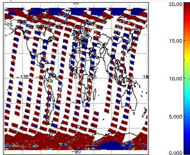
cL_opt_depth for 06OCT2011 00:00:00 to 07OCT2011 00:00:00
