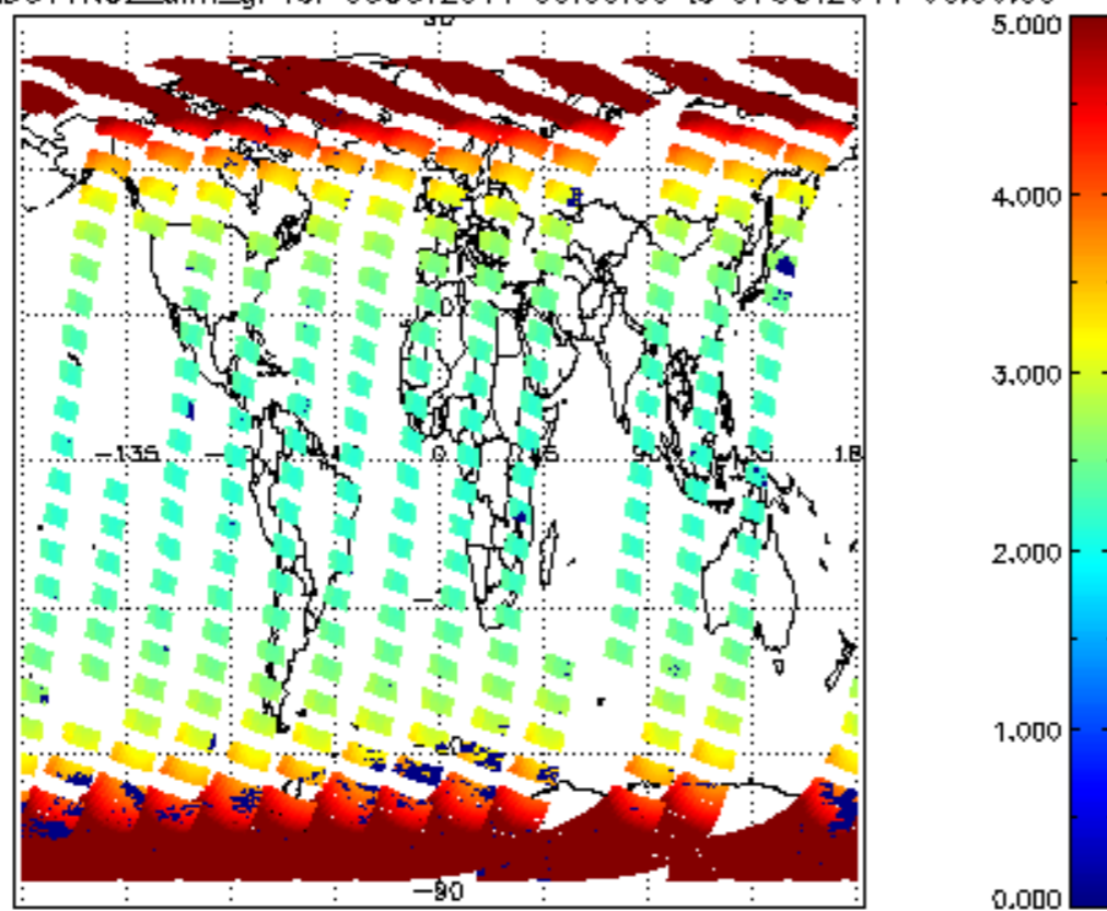
SCIOL2P_NADUV1NO2_amf_gr for 06OCT2011 00:00:00 to 07OCT2011 00:00:00
