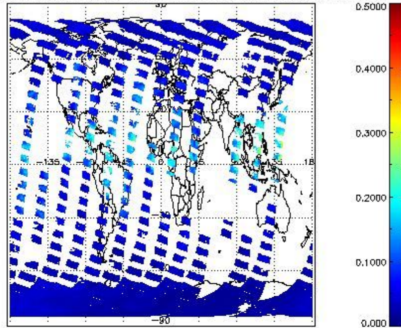
SCIOL2P_NADUV8H2O_vcd_err for 06OCT2011 00:00:00 to 07OCT2011 00:00:00
