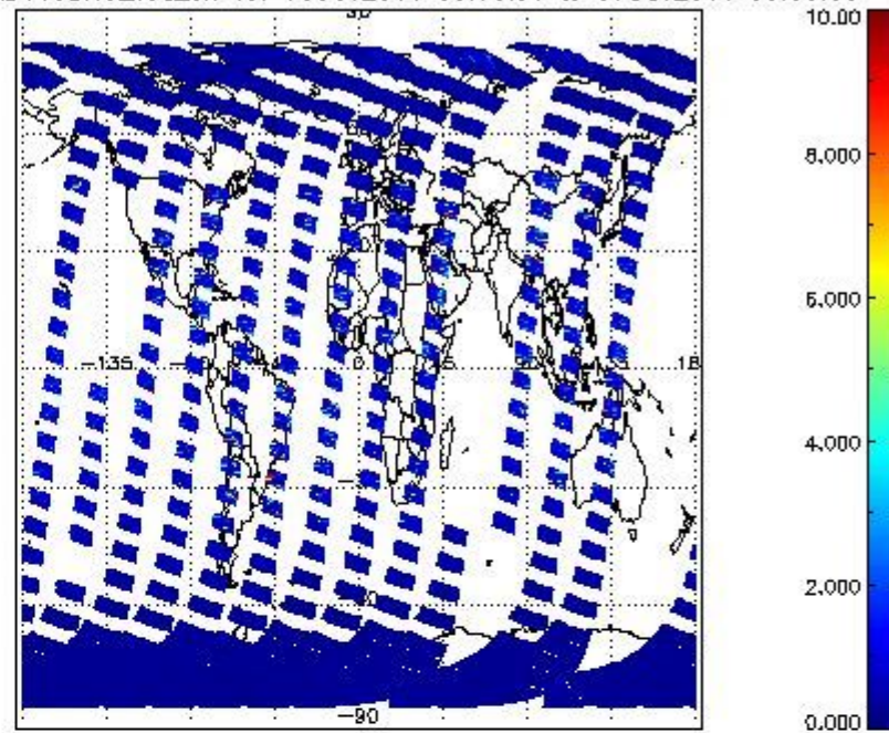
SCIOL2P_NADUV3BRO_vcd_err for 06OCT2011 00:00:00 to 07OCT2011 00:00:00
