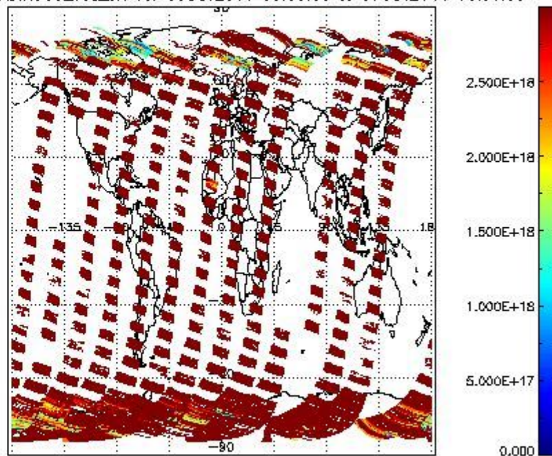
SCIDL2P_NADIR3CO_vcd_err for 06OCT2011 00:00:00 to 07OCT2011 00:00:00
