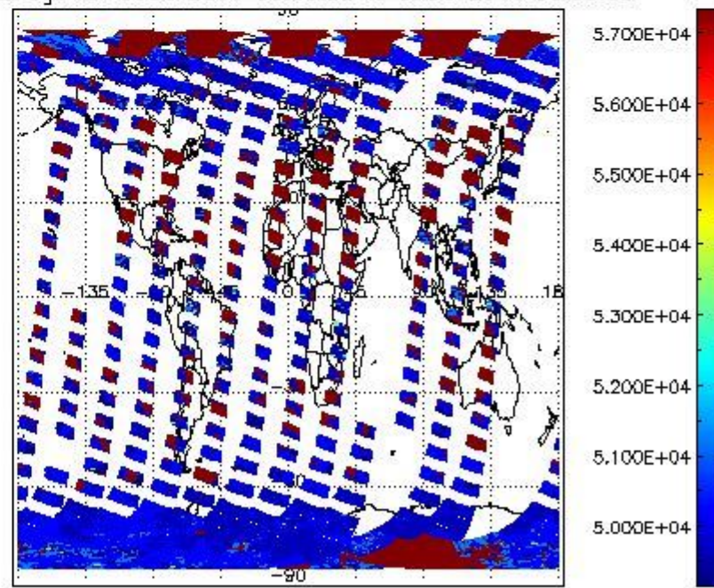
cloud_flags for 06OCT2011 00:00:00 to 07OCT2011 00:00:00
