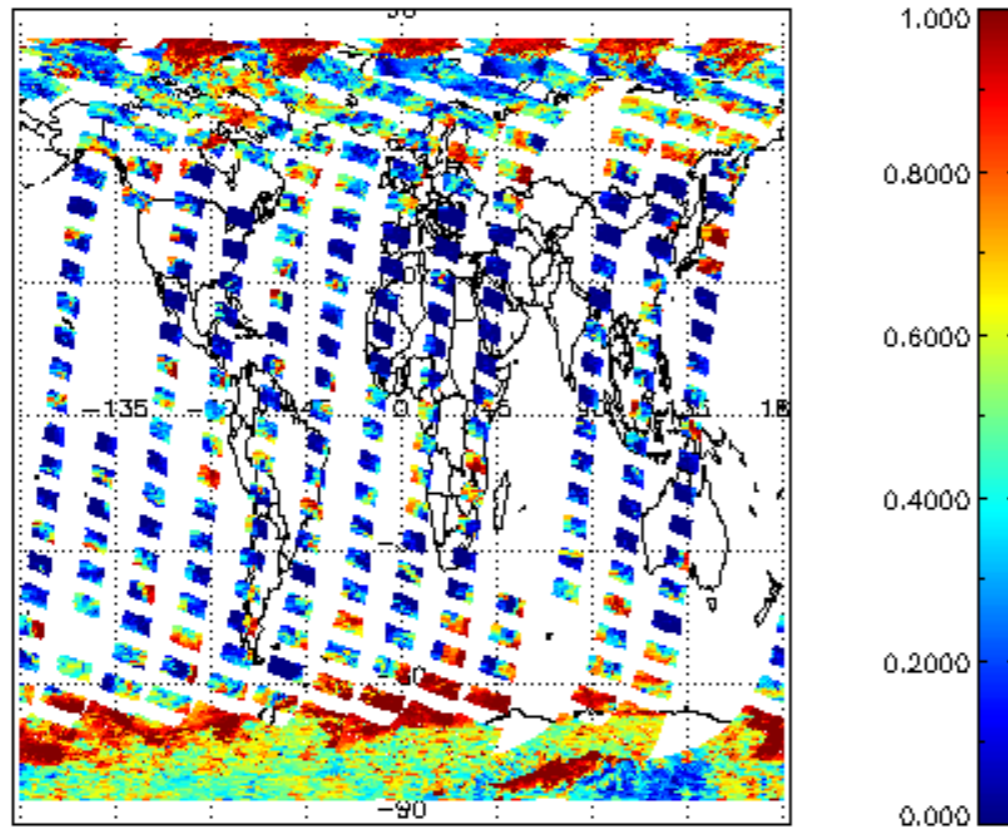
cl_frac for 06OCT2011 00:00:00 to 07OCT2011 00:00:00
