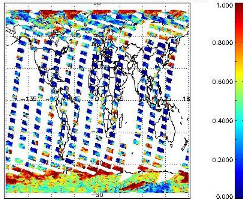
cLfrac for 06OCT2011 00:00:00 to 07OCT2011 00:00:00
