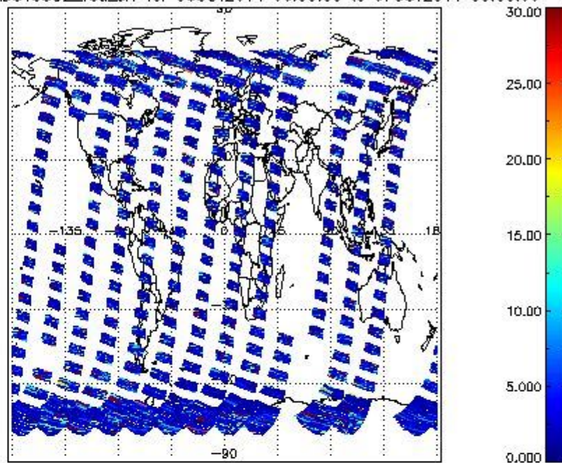
SCIOL2P_NADUV5S02_vcd_err for 06OCT2011 00:00:00 to 07OCT2011 00:00:00
