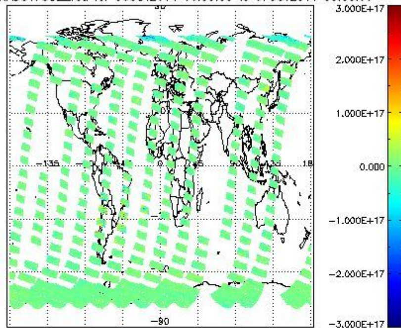
SCIOL2P_NADUV7S02_vcd for 06OCT2011 00:00:00 to 07OCT2011 00:00:00
