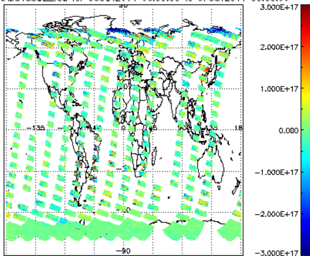
SCIOL2P_NADUV5S02_vcd for 06OCT2011 00:00:00 to 07OCT2011 00:00:00
