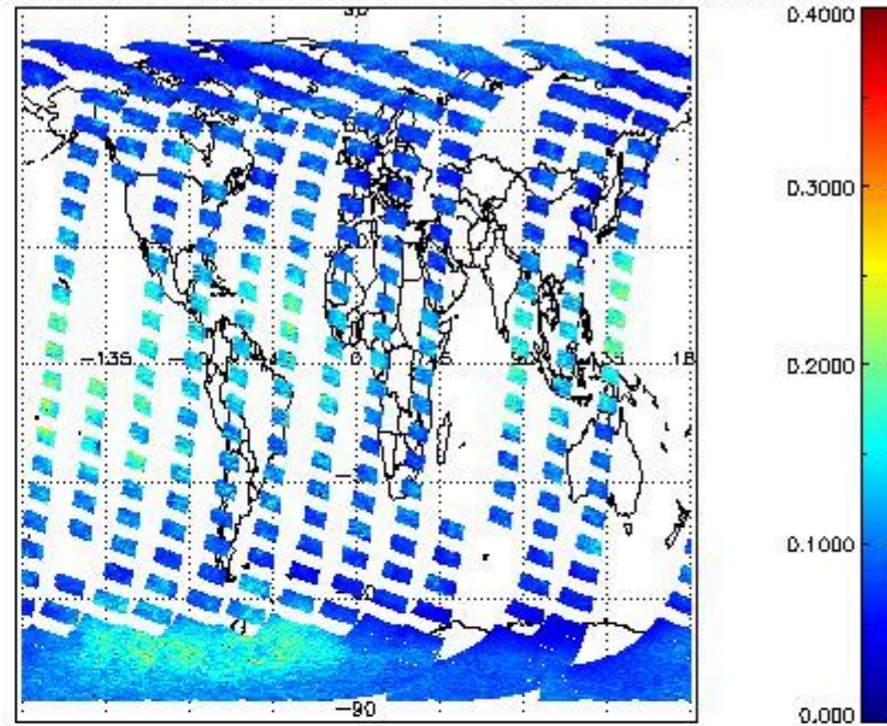
SCIOL2P_NADUV1NO2_vcd_err for 06OCT2011 00:00:00 to 07OCT2011 00:00:00
