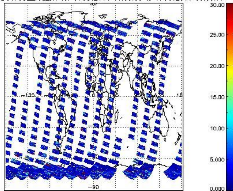
SCIOL2P_NADUV7S02_vcd_err for 06OCT2011 00:00:00 to 07OCT2011 00:00:00
