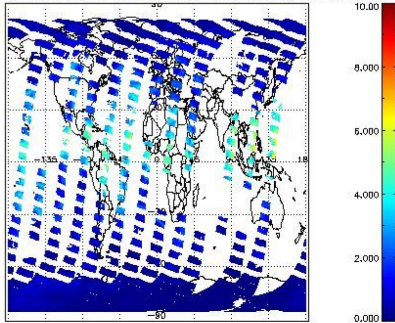
SCIOL2P_NADUV8H2O_vcd for 06OCT2011 00:00:00 to 07OCT2011 00:00:00
