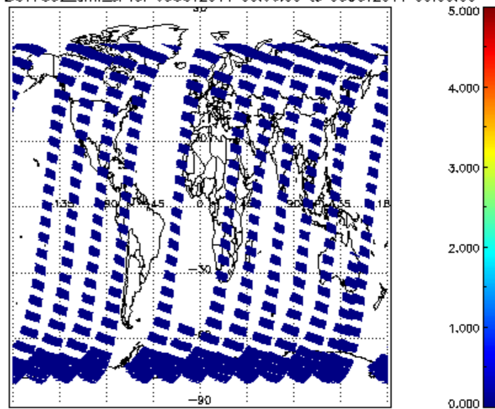
SCIOL2P_NADUV7S02_amf_cl for 05OCT2011 00:00:00 to 06OCT2011 00:00:00
