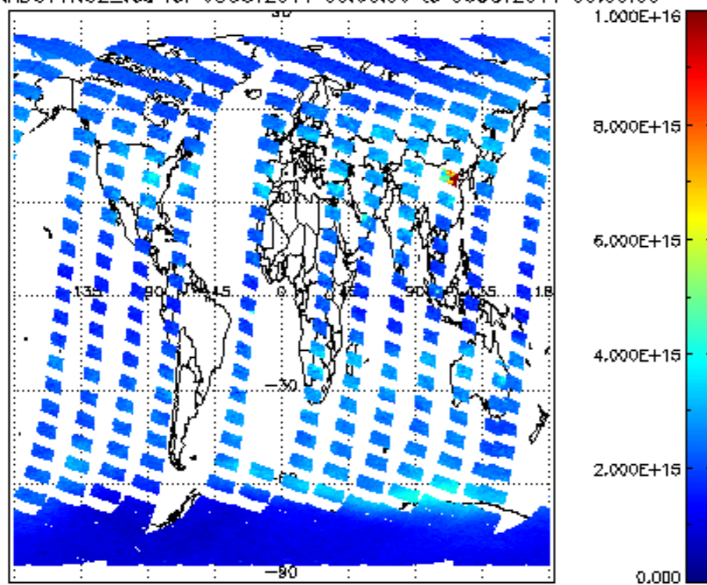
SCIOL2P_NADUV1NO2_vcd for 05OCT2011 00:00:00 to 06OCT2011 00:00:00
