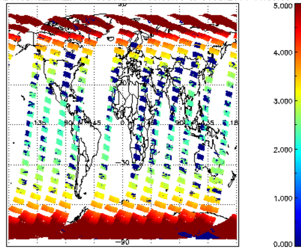
SCIOL2P_NADUV3BRO_amf_cl for 05OCT2011 00:00:00 to 06OCT2011 00:00:00
