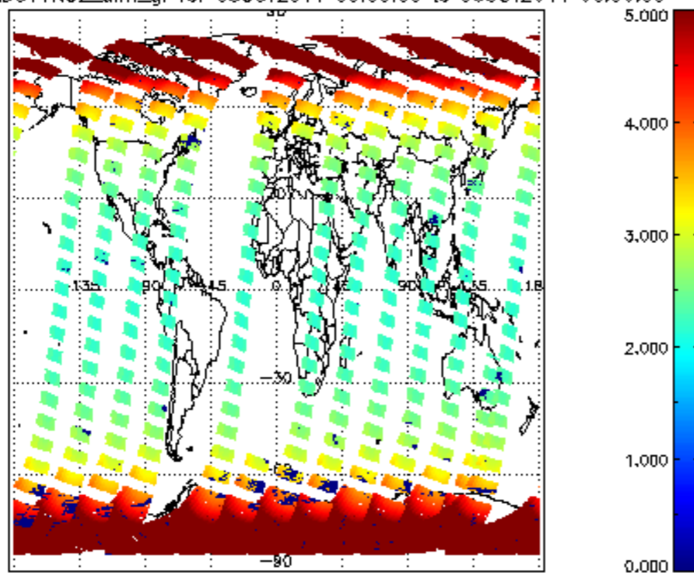
SCIOL2P_NADUV1NO2_amf_gr for 05OCT2011 00:00:00 to 06OCT2011 00:00:00
