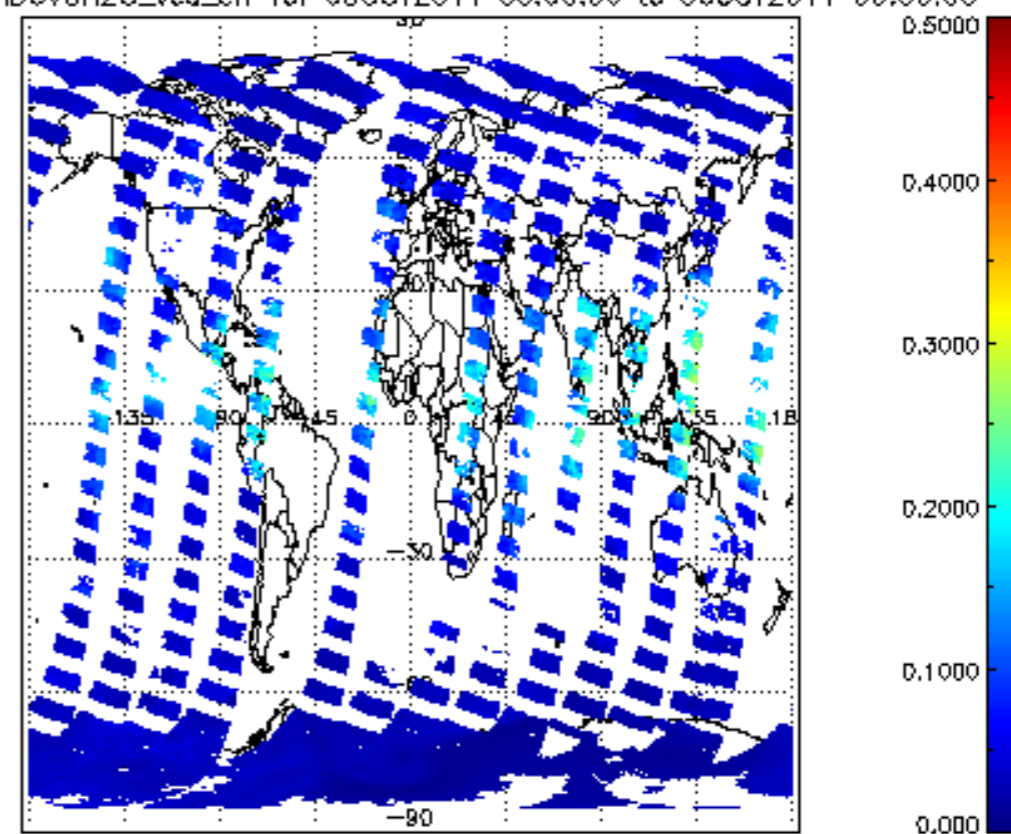
SCIOL2P_NADUV8H20_vcd_err for 05OCT2011 00:00:00 to 06OCT2011 00:00:00
