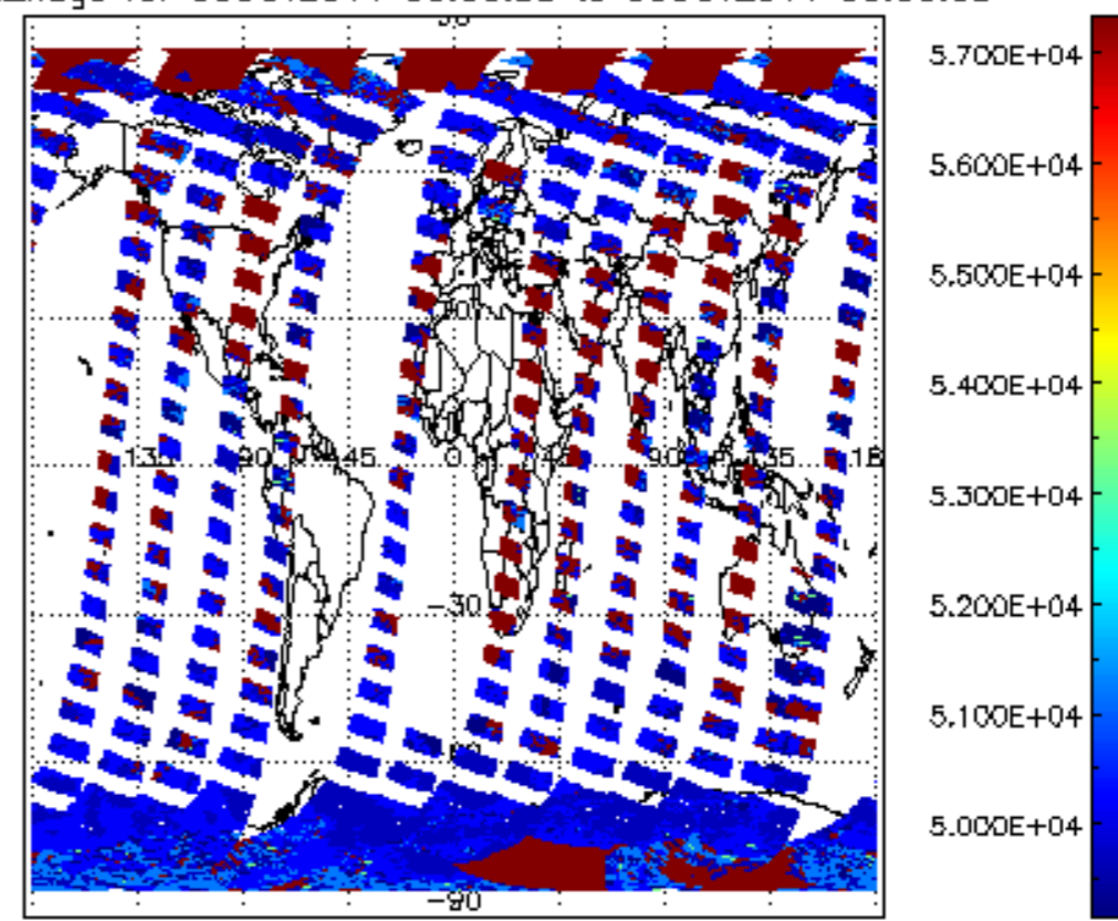
cloud_flags for 05OCT2011 00:00:00 to 06OCT2011 00:00:00
