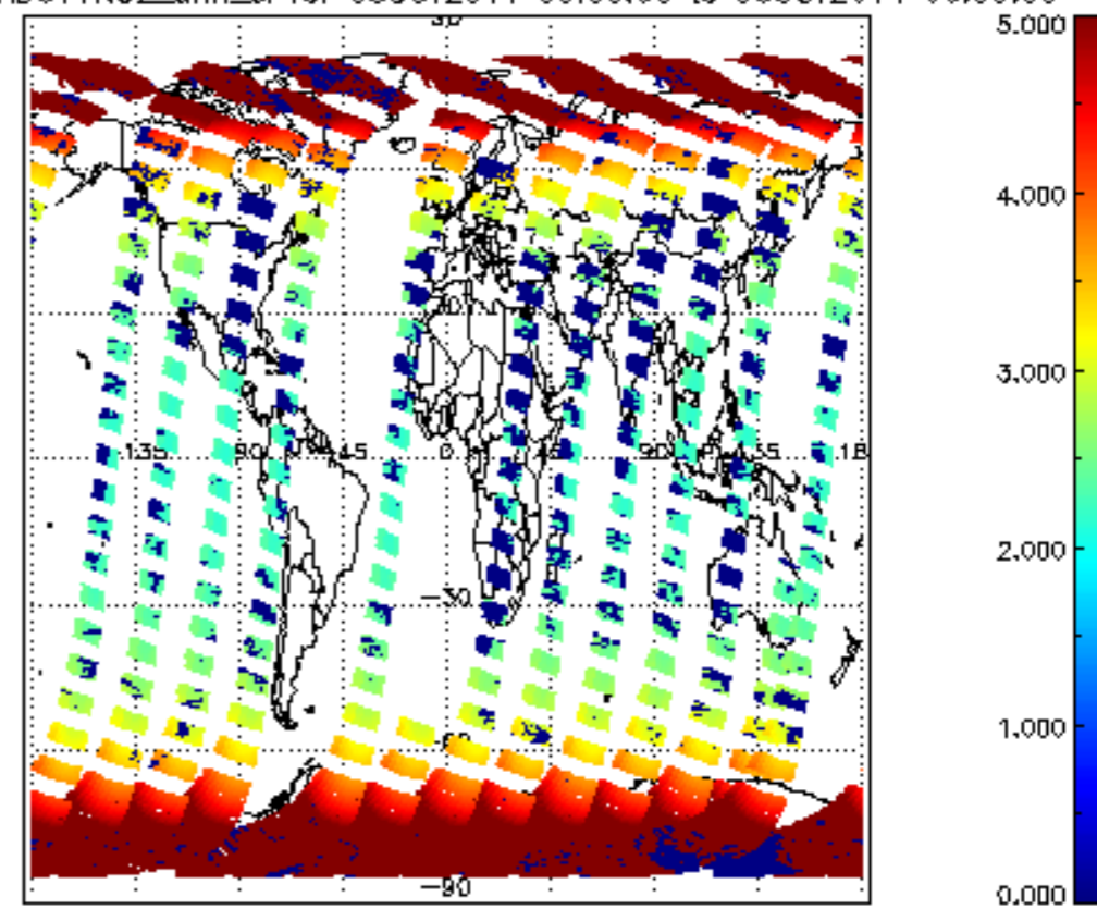
SCIOL2P_NADUV1NO2_amf_cl for 05OCT2011 00:00:00 to 06OCT2011 00:00:00
