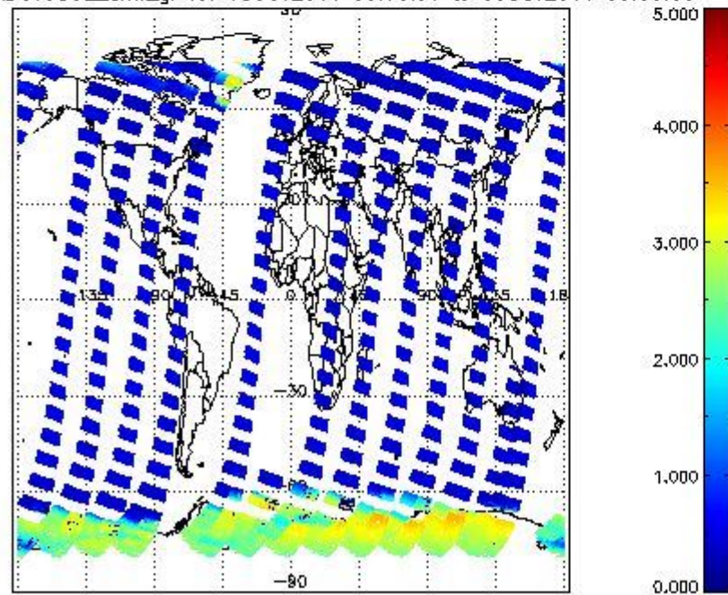
SCIOL2P_NADUV5S02_amf_gr for 05OCT2011 00:00:00 to 06OCT2011 00:00:00
