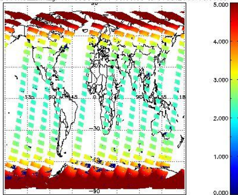
SCIOL2P_NADUV1N02_amf_gr for 05OCT2011 00:00:00 to 06OCT2011 00:00:00
