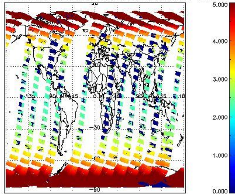
SCIOL2P_NADUV3BRO_amf_cl for 05OCT2011 00:00:00 to 06OCT2011 00:00:00
