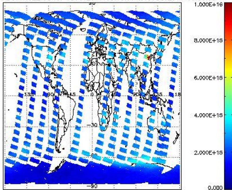
SCIOL2P_NADUV1N02_vcd for 05OCT2011 00:00:00 to 06OCT2011 00:00:00
