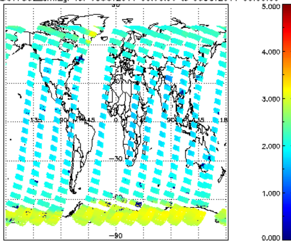
SCIOL2P_NADUV7S02_amf_gr for 05OCT2011 00:00:00 to 06OCT2011 00:00:00
