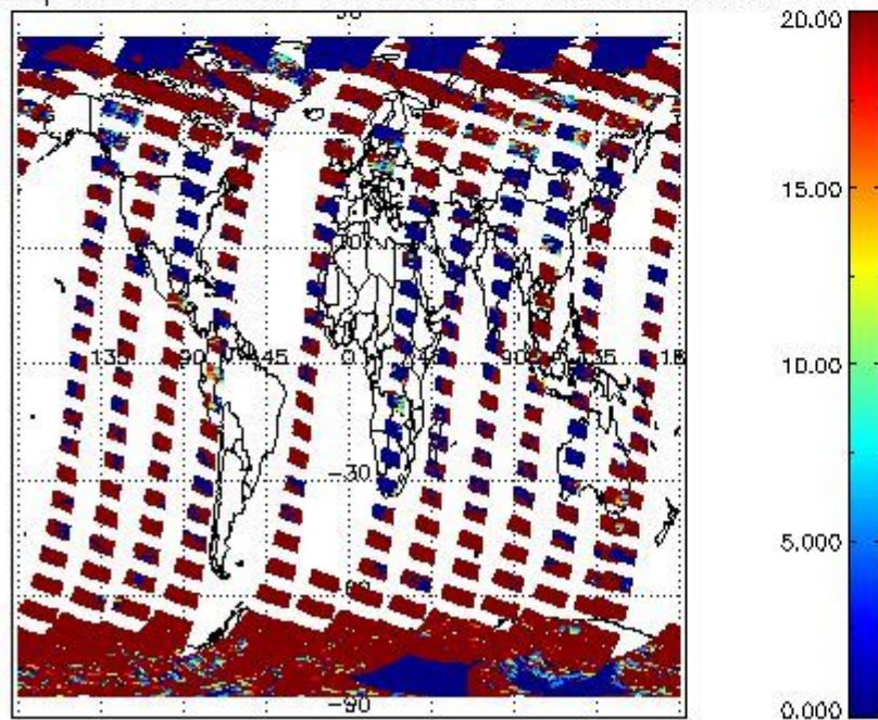
cL_opt_depth for 05OCT2011 00:00:00 to 06OCT2011 00:00:00
