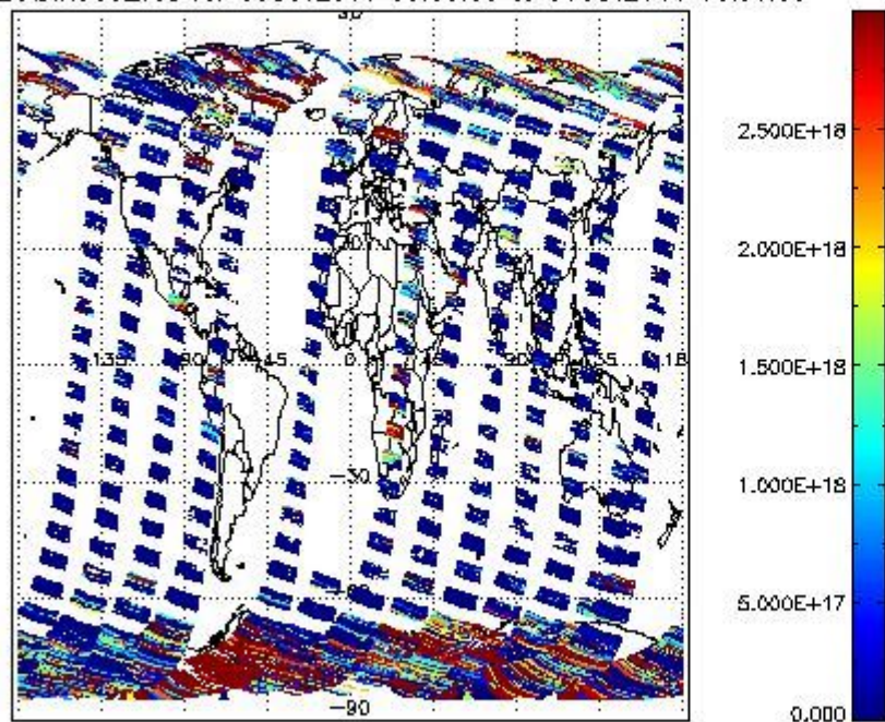
SCIDL2P_NADIR3CO_vcd for 05OCT2011 00:00:00 to 06OCT2011 00:00:00
