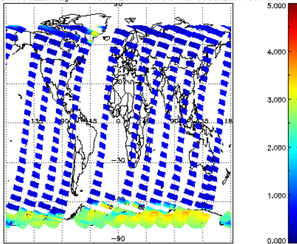
SCIOL2P_NADUV5S02_amf_gr for 05OCT2011 00:00:00 to 06OCT2011 00:00:00
