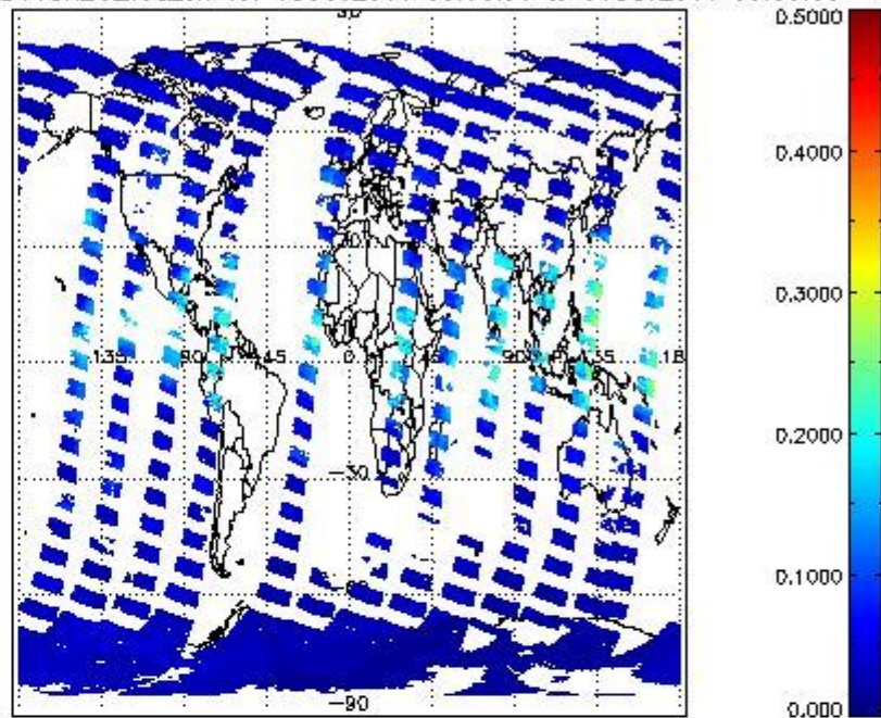
SCIOL2P_NADUV8H20_vcd_err for 05OCT2011 00:00:00 to 06OCT2011 00:00:00
