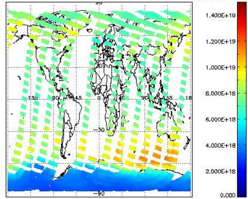
SCIOL2P_NADUV003_vcd for 05OCT2011 00:00:00 to 06OCT2011 00:00:00
