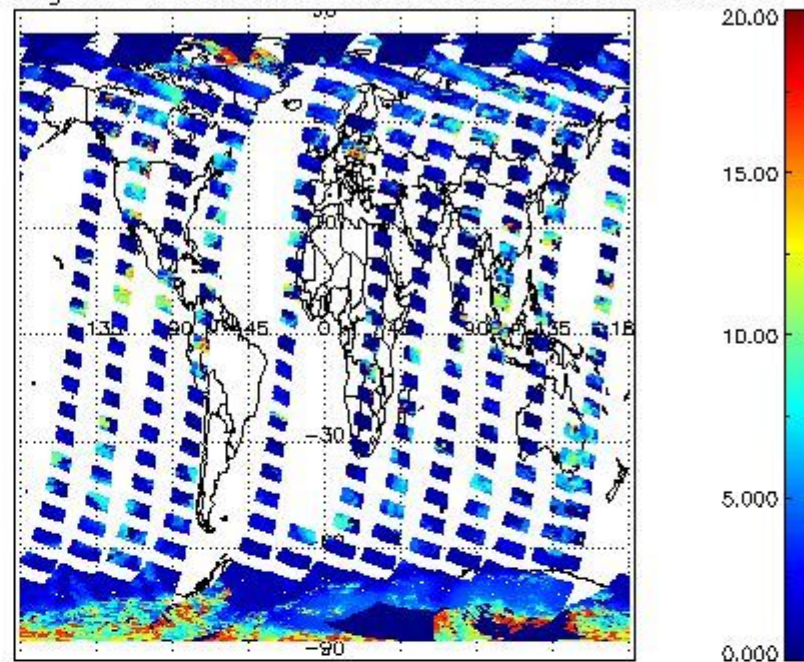
cL_top_height for 05OCT2011 00:00:00 to 06OCT2011 00:00:00
