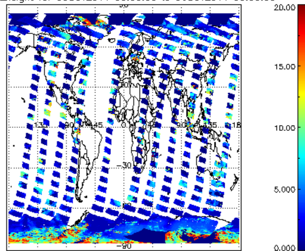
cl_top_height for 05OCT2011 00:00:00 to 06OCT2011 00:00:00
