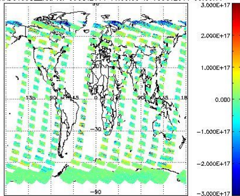
SCIOL2P_NADUV5S02_vcd for 05OCT2011 00:00:00 to 06OCT2011 00:00:00
