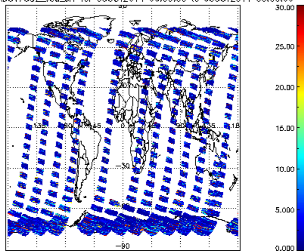
SCIOL2P_NADUV7S02_vcd_err for 05OCT2011 00:00:00 to 06OCT2011 00:00:00
