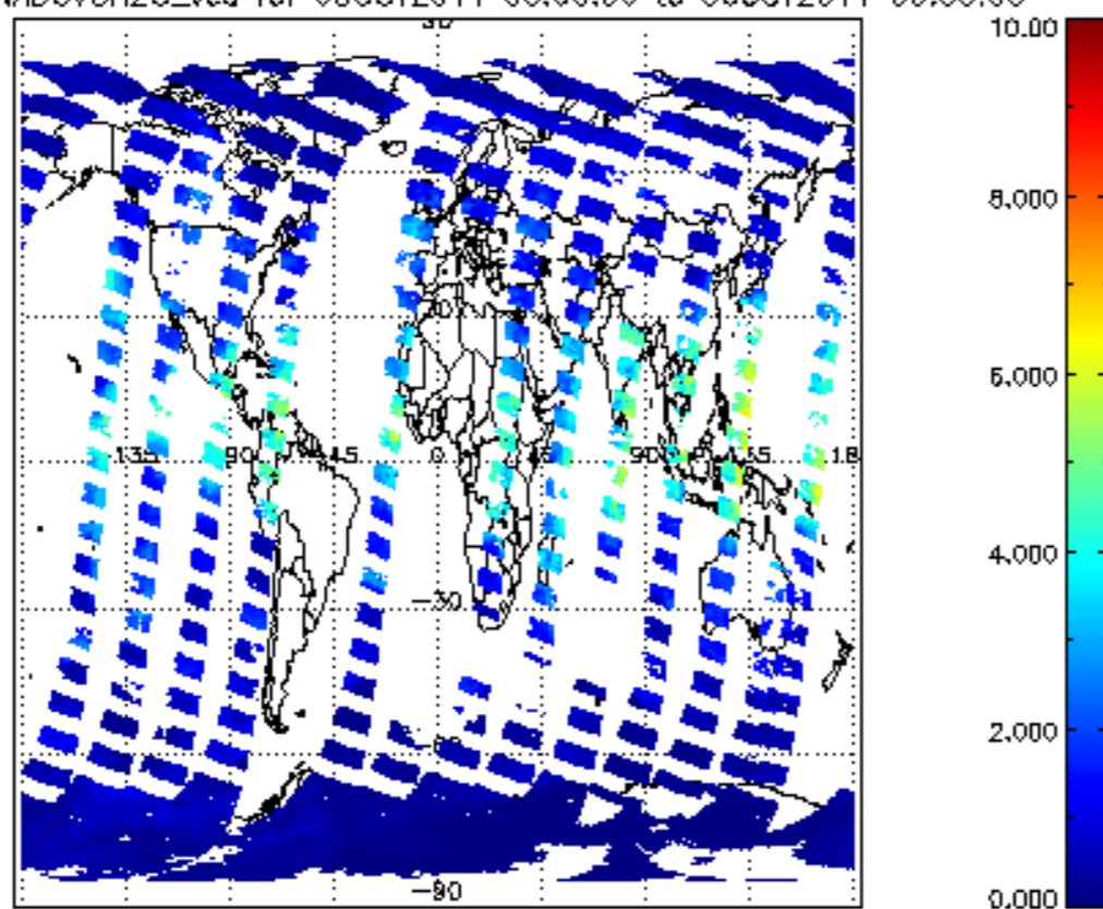
SCIOL2P_NADUV8H20_vcd for 05OCT2011 00:00:00 to 06OCT2011 00:00:00
