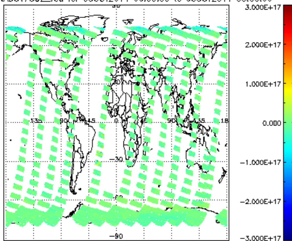
SCIOL2P_NADUV7S02_vcd for 05OCT2011 00:00:00 to 06OCT2011 00:00:00
