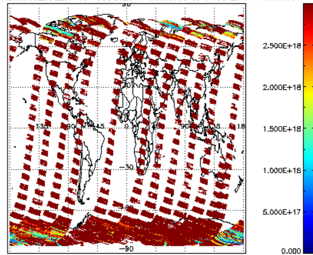
SCIOL2P_NADIR3CO_vcd_err for 05OCT2011 00:00:00 to 06OCT2011 00:00:00
