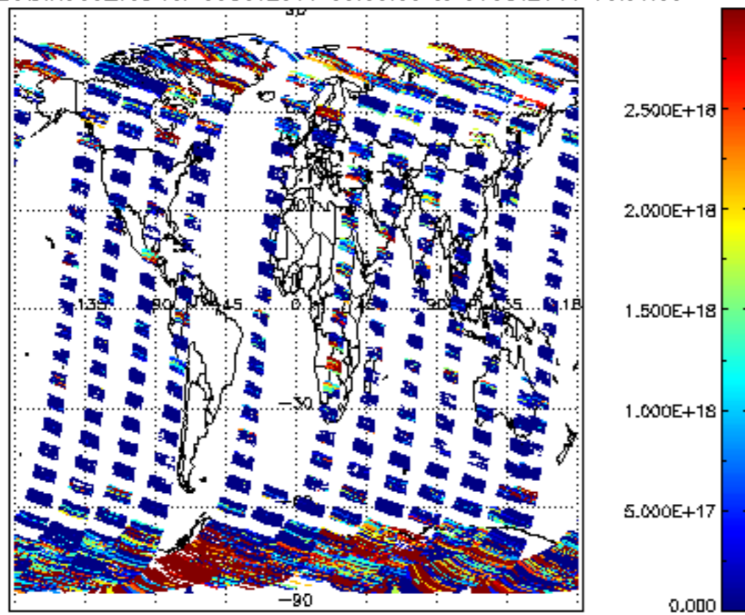
SCIOL2P_NADIR3CO_vcd for 05OCT2011 00:00:00 to 06OCT2011 00:00:00
