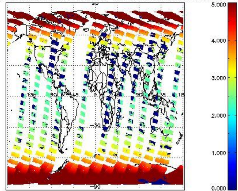
SCIOL2P_NADUV003_amf_cl for 05OCT2011 00:00:00 to 06OCT2011 00:00:00
