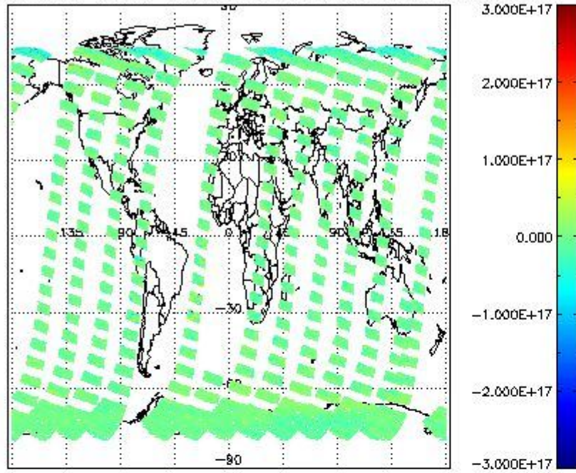
SCIOL2P_NADUV7S02_vcd for 05OCT2011 00:00:00 to 06OCT2011 00:00:00
