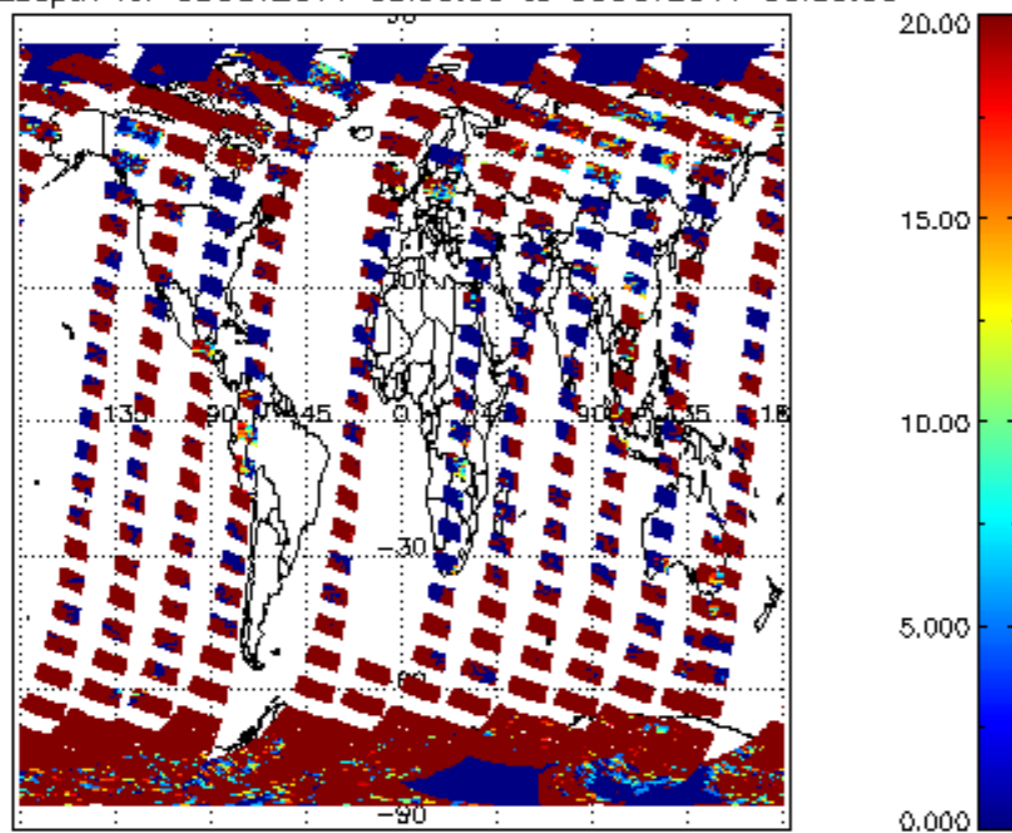
cl_opt_depth for 05OCT2011 00:00:00 to 06OCT2011 00:00:00
