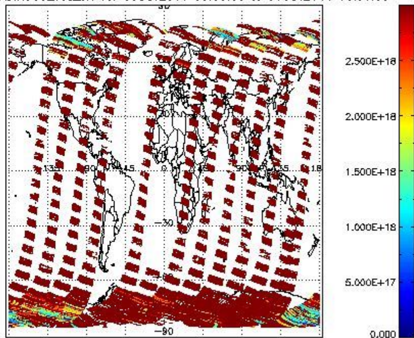
SCIDL2P_NADIR3CO_vcd_err for 05OCT2011 00:00:00 to 06OCT2011 00:00:00
