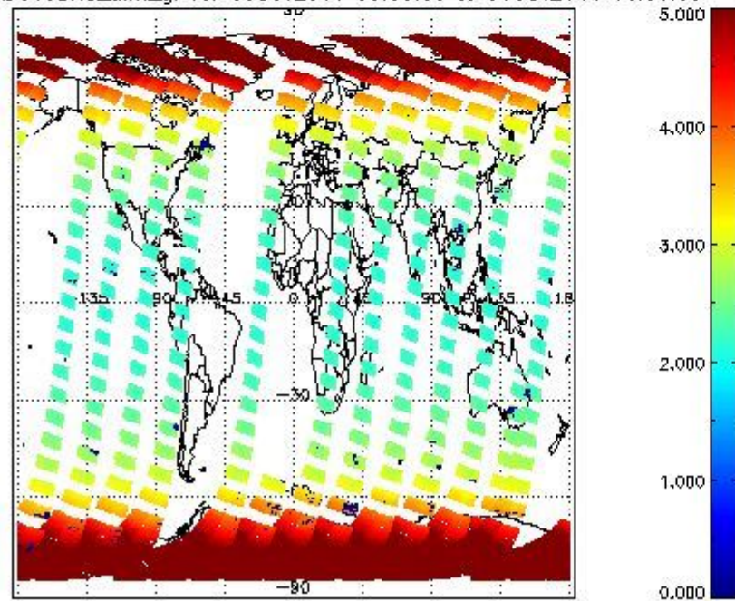
SCIOL2P_NADUV3BRO_amf_gr for 05OCT2011 00:00:00 to 06OCT2011 00:00:00
