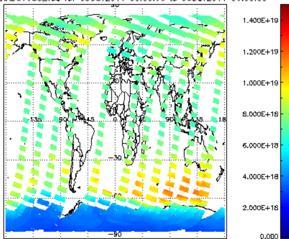
SCIOL2P_NADUV003_vcd for 05OCT2011 00:00:00 to 06OCT2011 00:00:00
