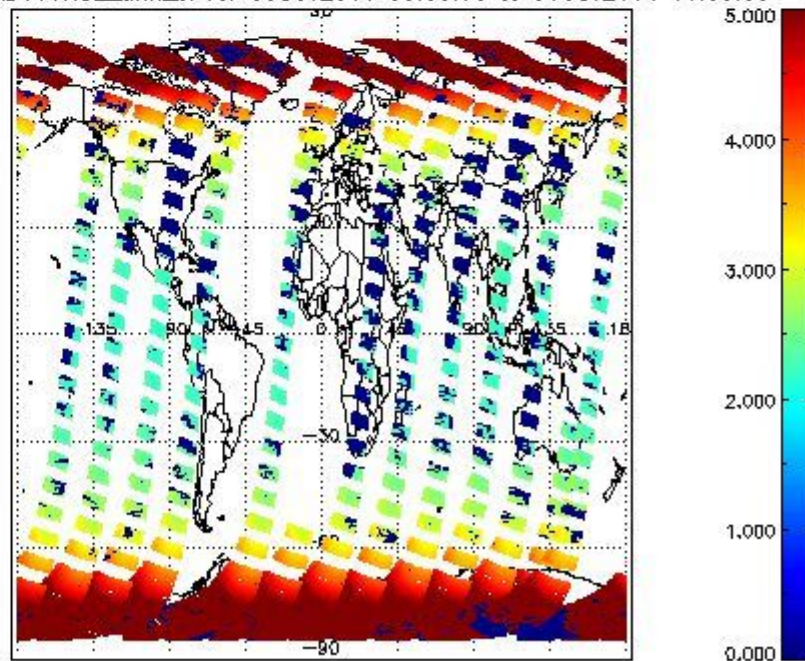
SCIOL2P_NADUV1N02_amf_cl for 05OCT2011 00:00:00 to 06OCT2011 00:00:00
