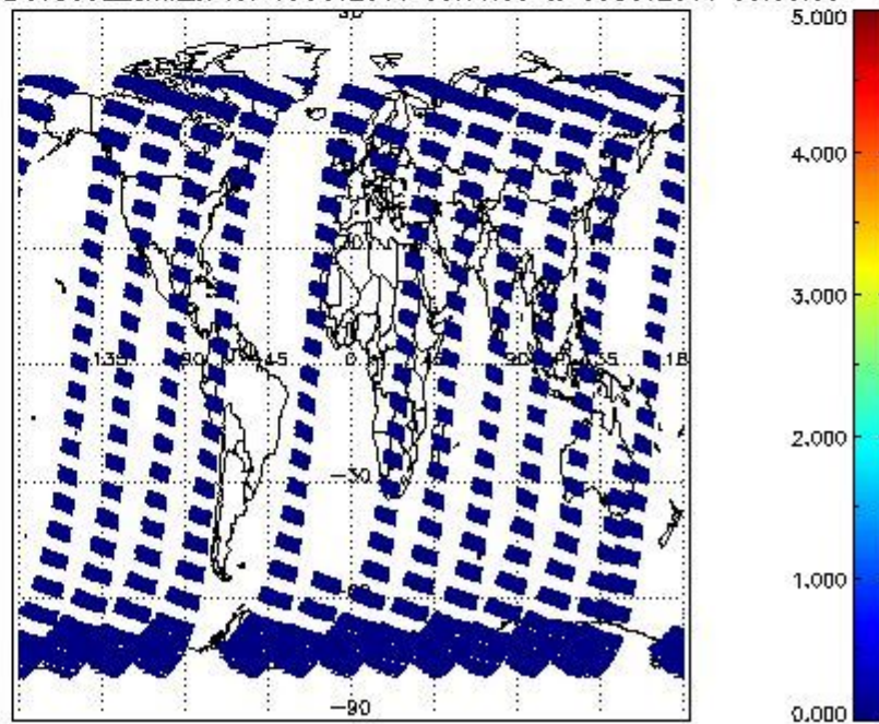
SCIOL2P_NADUV5S02_amf_cl for 05OCT2011 00:00:00 to 06OCT2011 00:00:00
