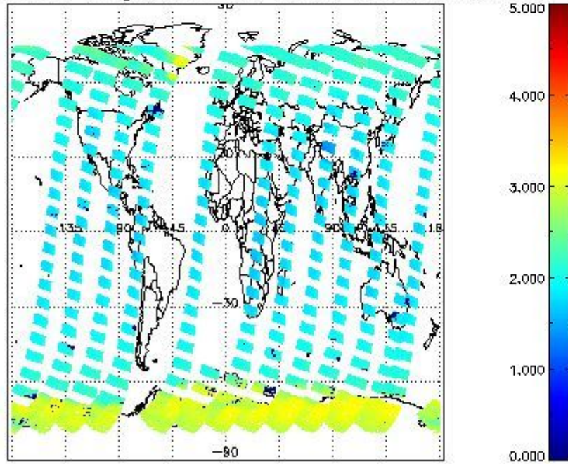
SCIOL2P_NADUV7S02_amf_gr for 05OCT2011 00:00:00 to 06OCT2011 00:00:00
