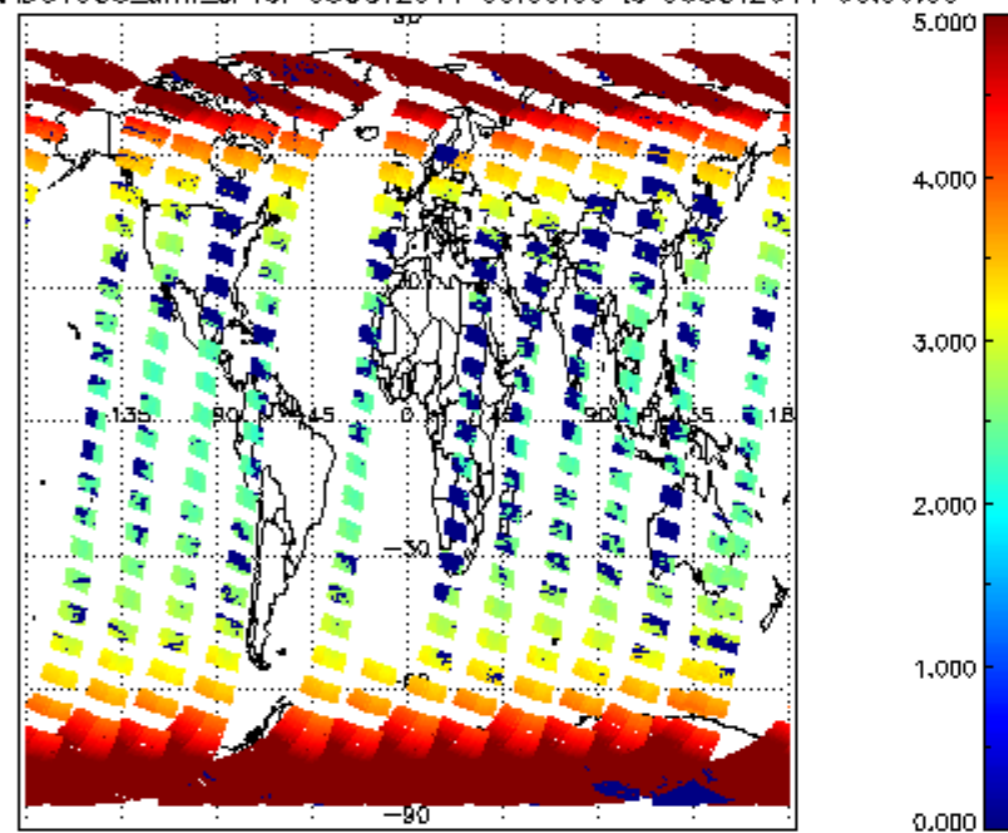
SCIOL2P_NADUV003_amf_cl for 05OCT2011 00:00:00 to 06OCT2011 00:00:00
