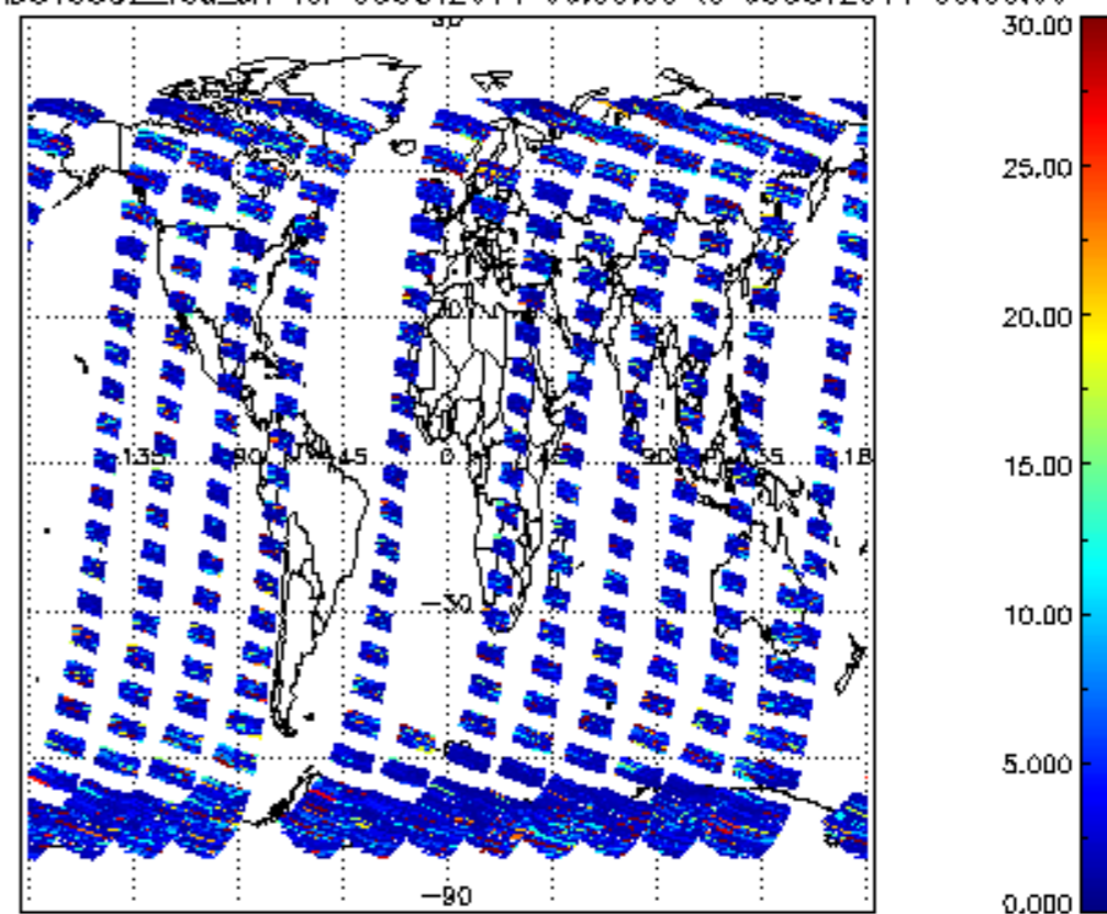
SCIOL2P_NADUV5S02_vcd_err for 05OCT2011 00:00:00 to 06OCT2011 00:00:00
