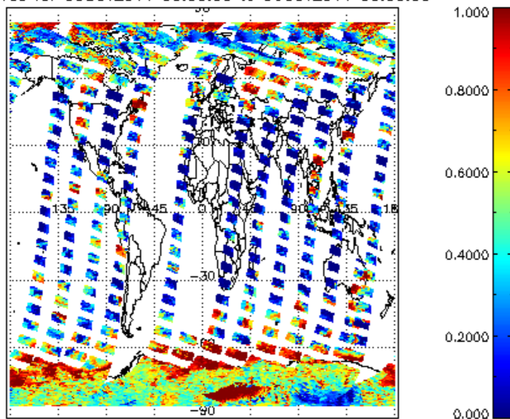
cl_frac for 05OCT2011 00:00:00 to 06OCT2011 00:00:00
