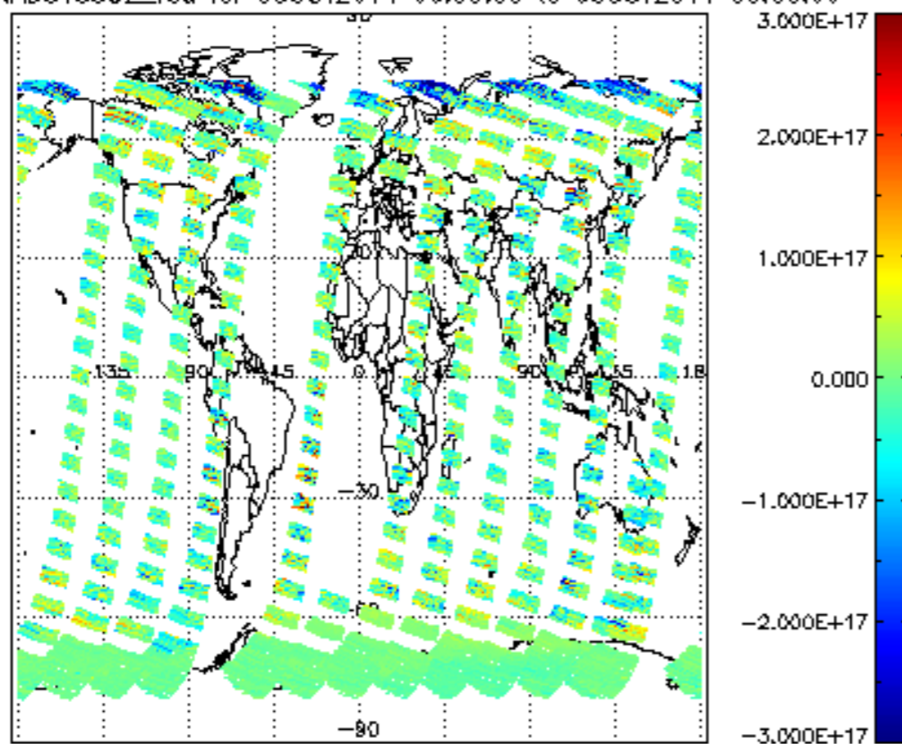
SCIOL2P_NADUV5S02_vcd for 05OCT2011 00:00:00 to 06OCT2011 00:00:00
