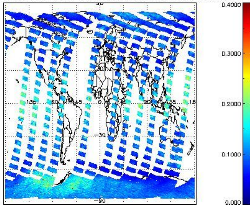
SCIOL2P_NADUV1N02_vcd_err for 05OCT2011 00:00:00 to 06OCT2011 00:00:00
