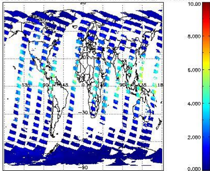
SCIOL2P_NADUV8H20_vcd for 05OCT2011 00:00:00 to 06OCT2011 00:00:00
