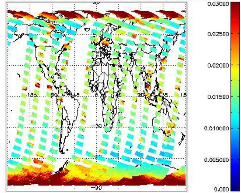
SCIOL2P_NADUV003_vcd_err for 05OCT2011 00:00:00 to 06OCT2011 00:00:00
