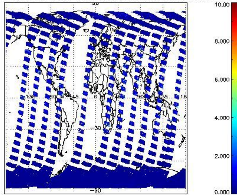
SCIOL2P_NADUV3BRO_vcd_err for 05OCT2011 00:00:00 to 06OCT2011 00:00:00
