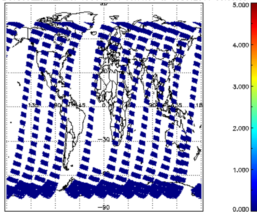
SCIOL2P_NADUV5S02_amf_cl for 05OCT2011 00:00:00 to 06OCT2011 00:00:00
