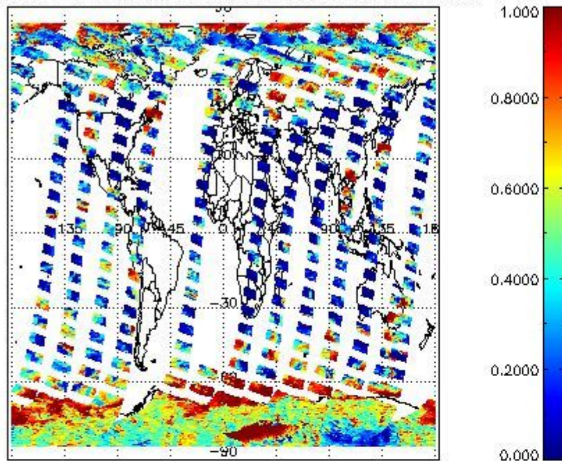
cLfrac for 05OCT2011 00:00:00 to 06OCT2011 00:00:00
