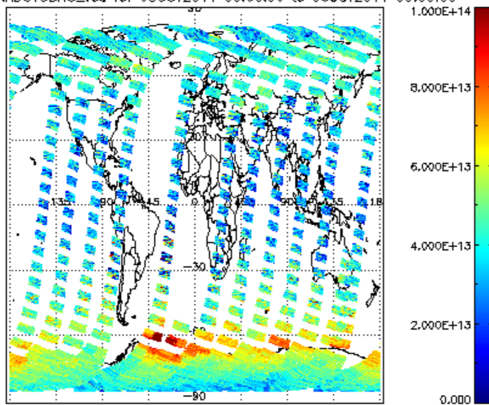
SCIOL2P_NADUV3BRO_vcd for 05OCT2011 00:00:00 to 06OCT2011 00:00:00
