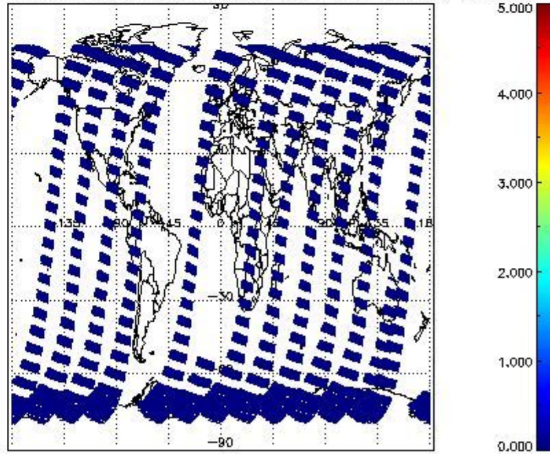
SCIOL2P_NADUV7S02_amf_cl for 05OCT2011 00:00:00 to 06OCT2011 00:00:00
