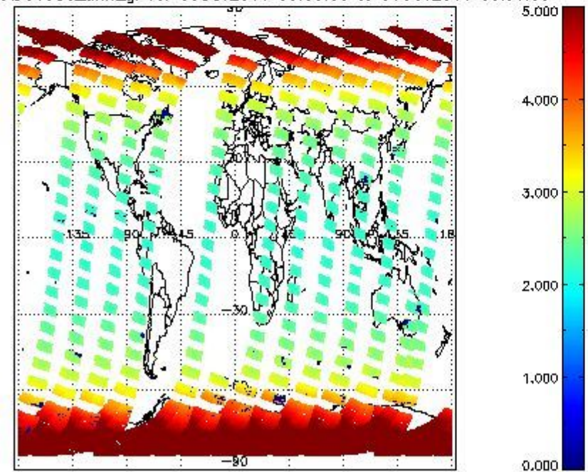
SCIOL2P_NADUV003_amf_gr for 05OCT2011 00:00:00 to 06OCT2011 00:00:00
