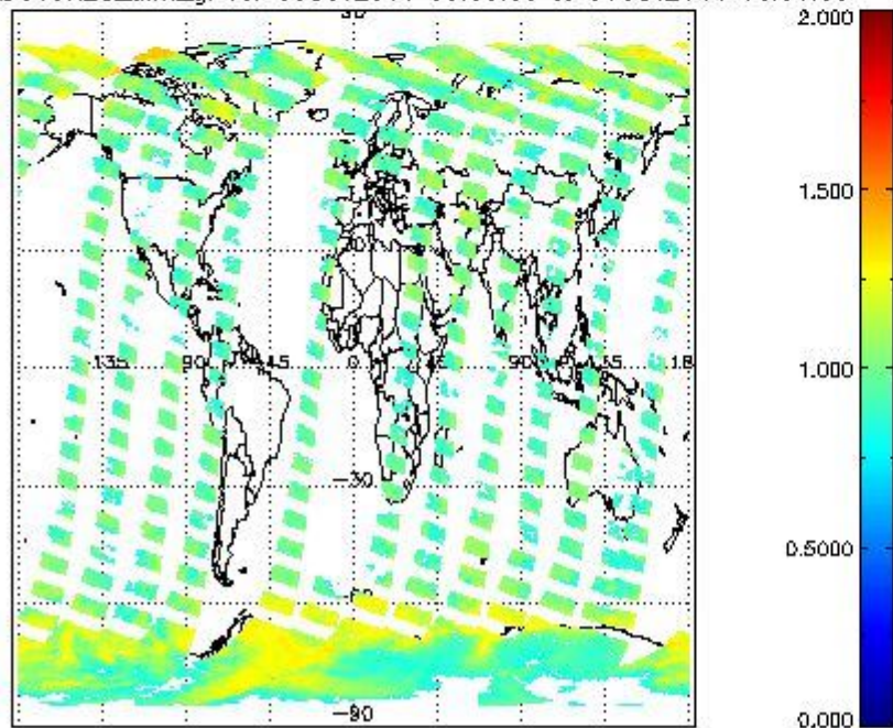
SCIOL2P_NADUV8H20_amf_gr for 05OCT2011 00:00:00 to 06OCT2011 00:00:00
