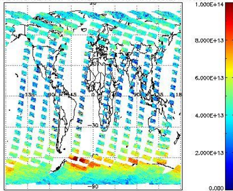
SCIOL2P_NADUV3BRO_vcd for 05OCT2011 00:00:00 to 06OCT2011 00:00:00
