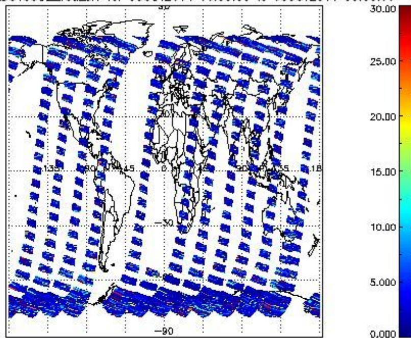
SCIOL2P_NADUV5S02_vcd_err for 05OCT2011 00:00:00 to 06OCT2011 00:00:00
