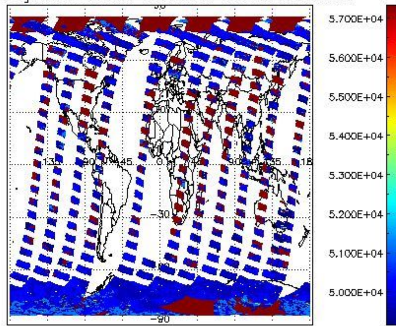
cloud_flags for 05OCT2011 00:00:00 to 06OCT2011 00:00:00
