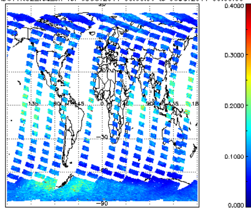
SCIOL2P_NADUV1NO2_vcd_err for 05OCT2011 00:00:00 to 06OCT2011 00:00:00
