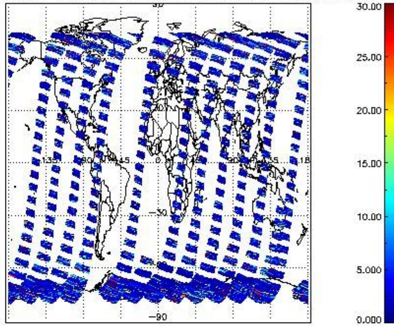
SCIOL2P_NADUV7S02_vcd_err for 05OCT2011 00:00:00 to 06OCT2011 00:00:00
