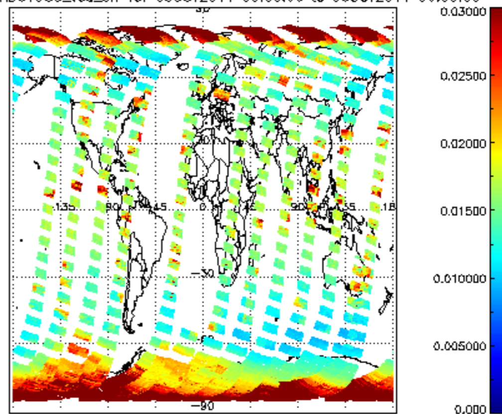
SCIOL2P_NADUV003_vcd_err for 05OCT2011 00:00:00 to 06OCT2011 00:00:00
