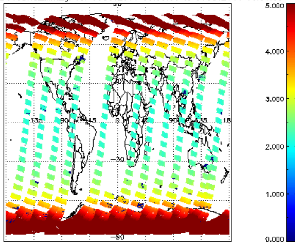
SCIOL2P_NADUV3BRO_amf_gr for 05OCT2011 00:00:00 to 06OCT2011 00:00:00
