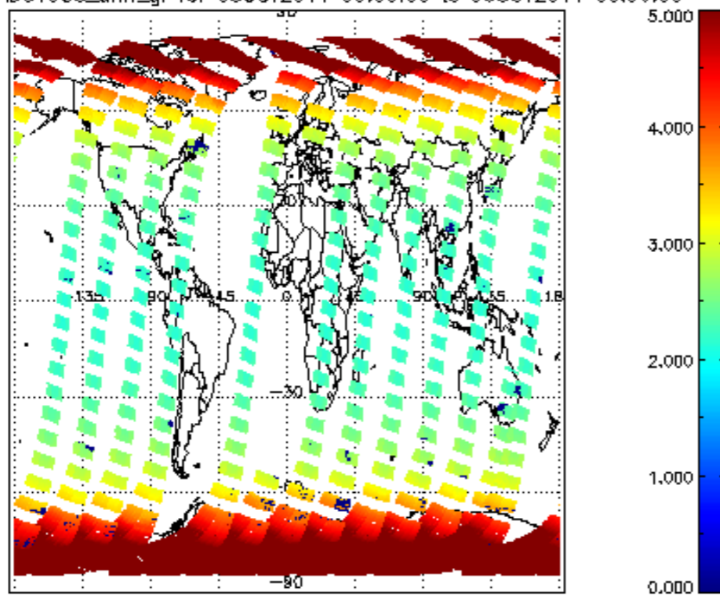
SCIOL2P_NADUV003_amf_gr for 05OCT2011 00:00:00 to 06OCT2011 00:00:00
