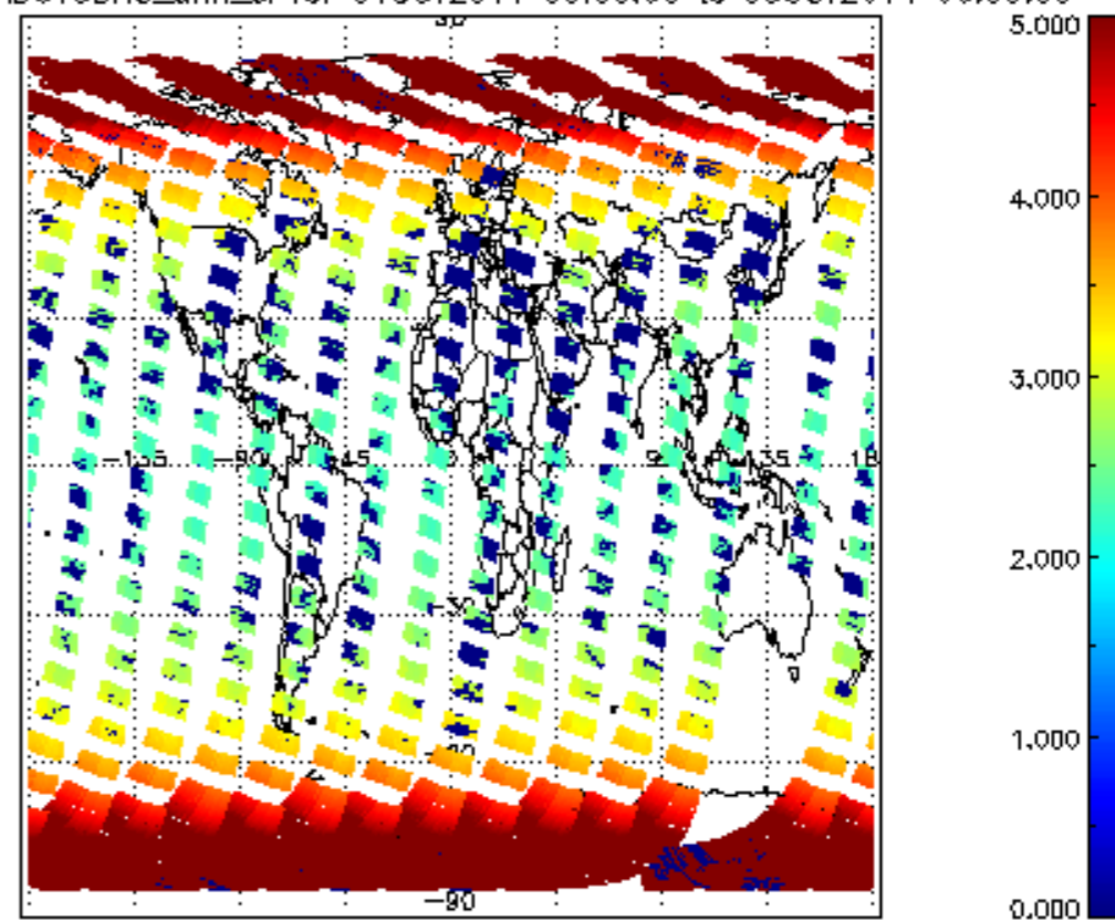
SCIOL2P_NADUV3BRO_amf_cl for 04OCT2011 00:00:00 to 05OCT2011 00:00:00
