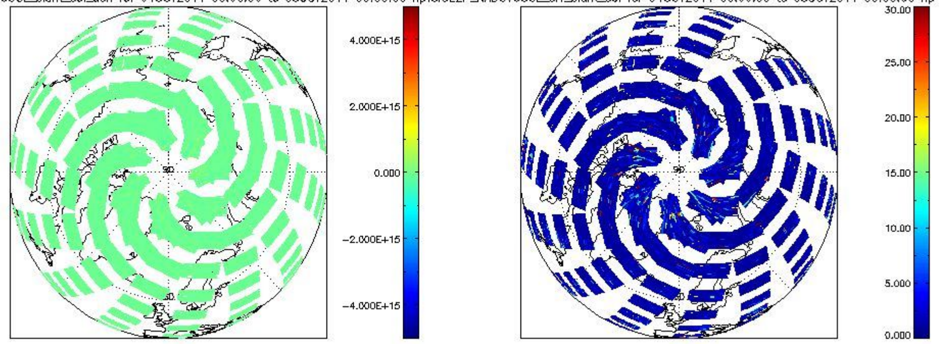
CIOL2P_NADUV60CL_slant_col_den for 04OCT2011 00:00:00 to 05OCT2011 00:00:00 npCIOL2P_NADUV60CL_err_slant_col for 04OCT2011 00:00:00 to 05OCT2011 00:00:00 np
