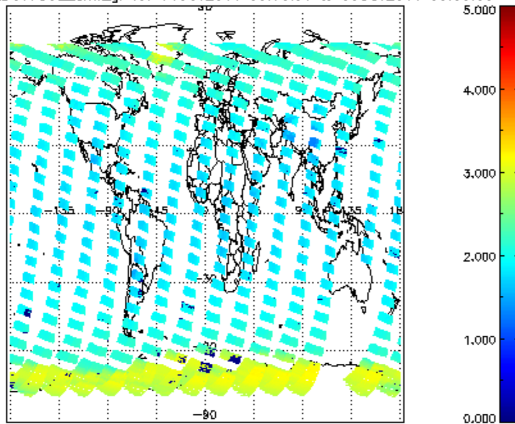
SCIOL2P_NADUV7S02_amf_gr for 04OCT2011 00:00:00 to 05OCT2011 00:00:00
