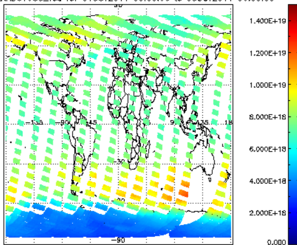
SCIOL2P_NADUV003_vcd for 04OCT2011 00:00:00 to 05OCT2011 00:00:00
