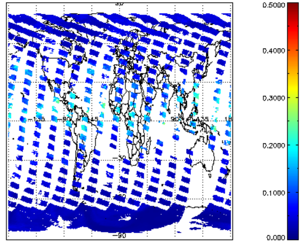
SCIOL2P_NADUV8H20_vcd_err for 04OCT2011 00:00:00 to 05OCT2011 00:00:00
