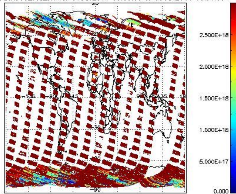
SCIOL2P_NADIR3CO_vcd_err for 04OCT2011 00:00:00 to 05OCT2011 00:00:00
