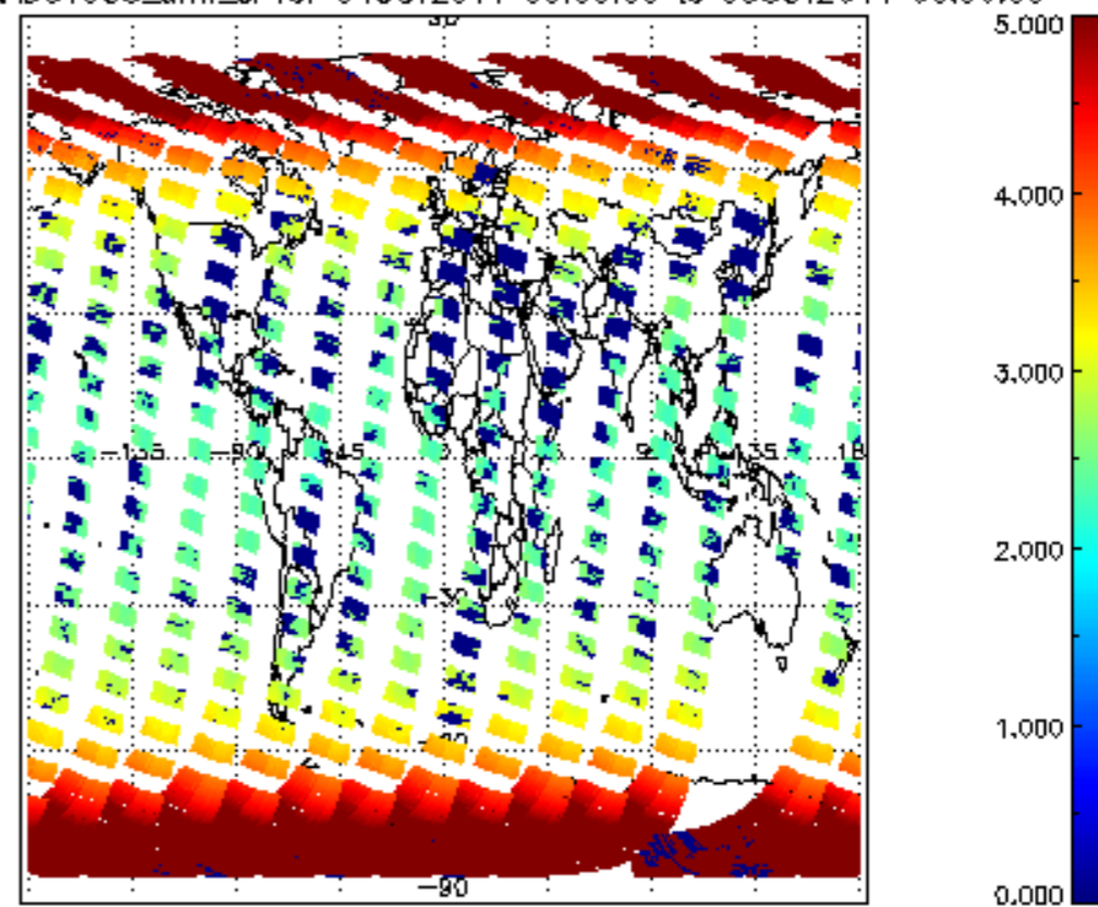
SCIOL2P_NADUV003_amf_cl for 04OCT2011 00:00:00 to 05OCT2011 00:00:00
