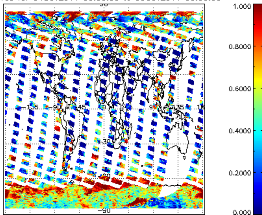
cl_frac for 04OCT2011 00:00:00 to 05OCT2011 00:00:00
