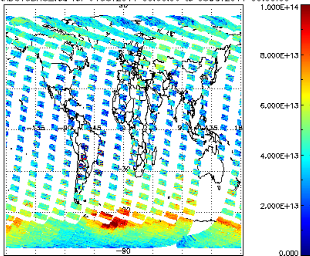
SCIOL2P_NADUV3BRO_vcd for 04OCT2011 00:00:00 to 05OCT2011 00:00:00
