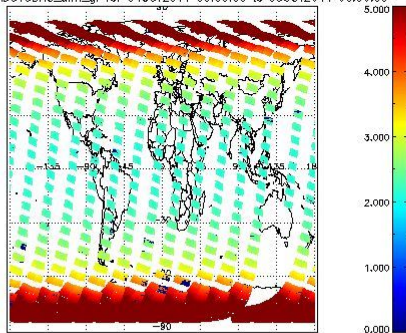
SCIOL2P_NADUV3BRO_amf_gr for 04OCT2011 00:00:00 to 05OCT2011 00:00:00
