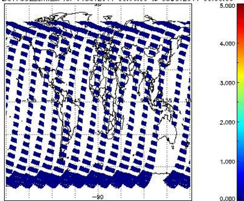
SCIOL2P_NADUV7S02_amf_cl for 04OCT2011 00:00:00 to 05OCT2011 00:00:00
