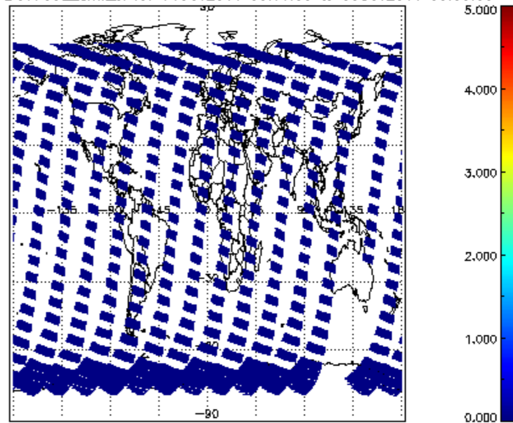
SCIOL2P_NADUV7S02_amf_cl for 04OCT2011 00:00:00 to 05OCT2011 00:00:00
