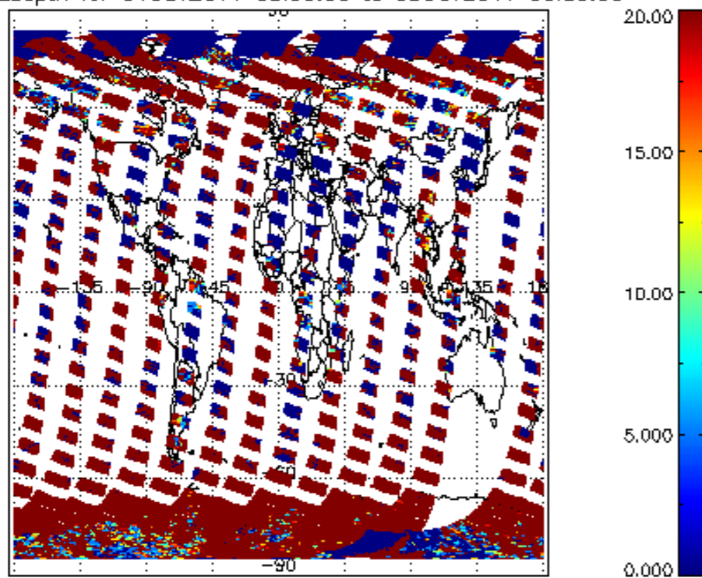
cl_opt_depth for 04OCT2011 00:00:00 to 05OCT2011 00:00:00
