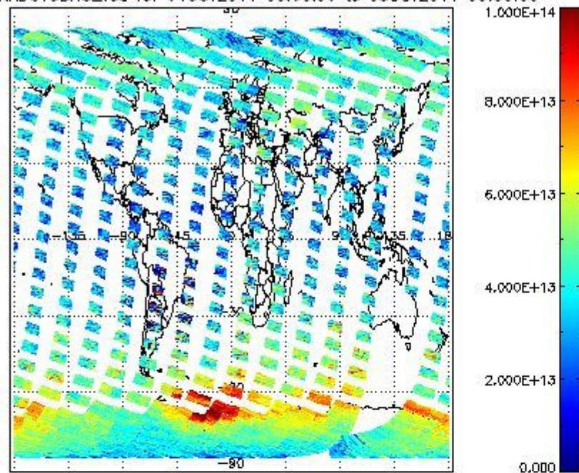
SCIOL2P_NADUV3BRO_vcd for 04OCT2011 00:00:00 to 05OCT2011 00:00:00
