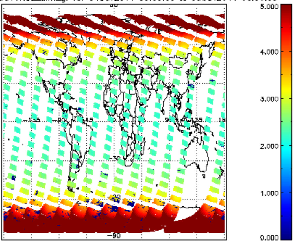
SCIOL2P_NADUV1NO2_amf_gr for 04OCT2011 00:00:00 to 05OCT2011 00:00:00
