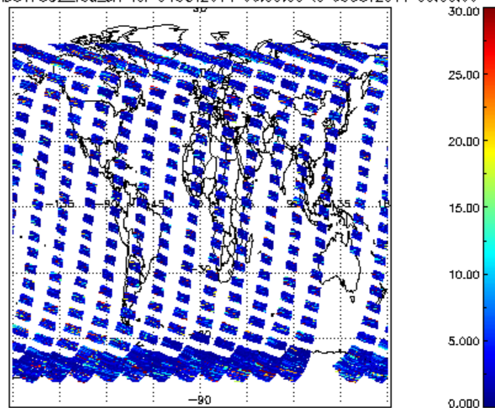
SCIOL2P_NADUV7S02_vcd_err for 04OCT2011 00:00:00 to 05OCT2011 00:00:00
