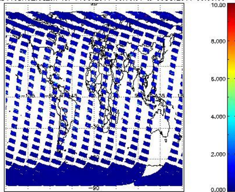
SCIOL2P_NADUV3BRO_vcd_err for 04OCT2011 00:00:00 to 05OCT2011 00:00:00
