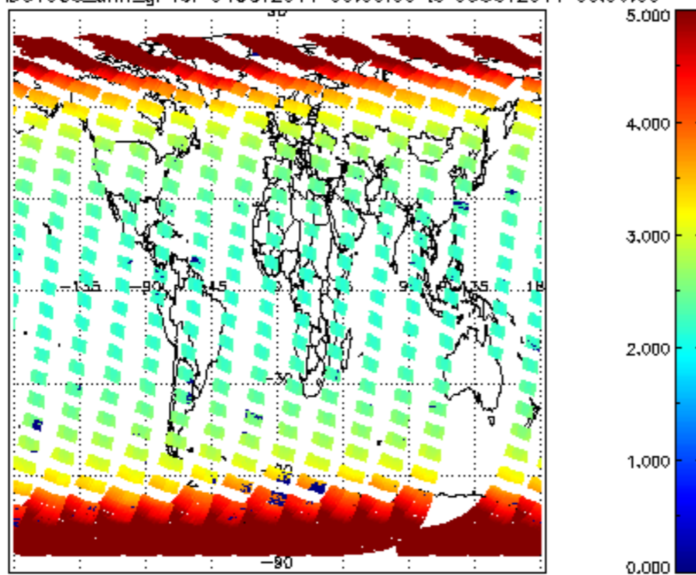
SCIOL2P_NADUV003_amf_gr for 04OCT2011 00:00:00 to 05OCT2011 00:00:00
