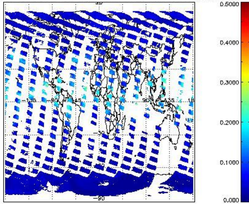
SCIOL2P_NADUV8H20_vcd_err for 04OCT2011 00:00:00 to 05OCT2011 00:00:00
