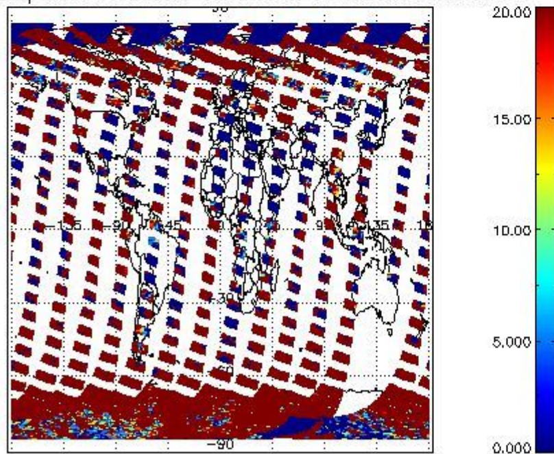
cL_opt_depth for 04OCT2011 00:00:00 to 05OCT2011 00:00:00
