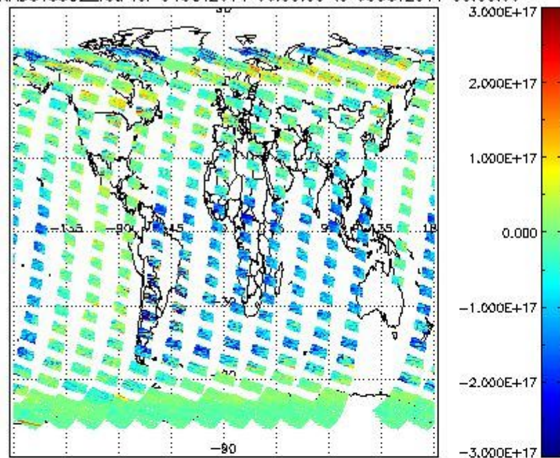
SCIOL2P_NADUV5SO2_vcd for 04OCT2011 00:00:00 to 05OCT2011 00:00:00
