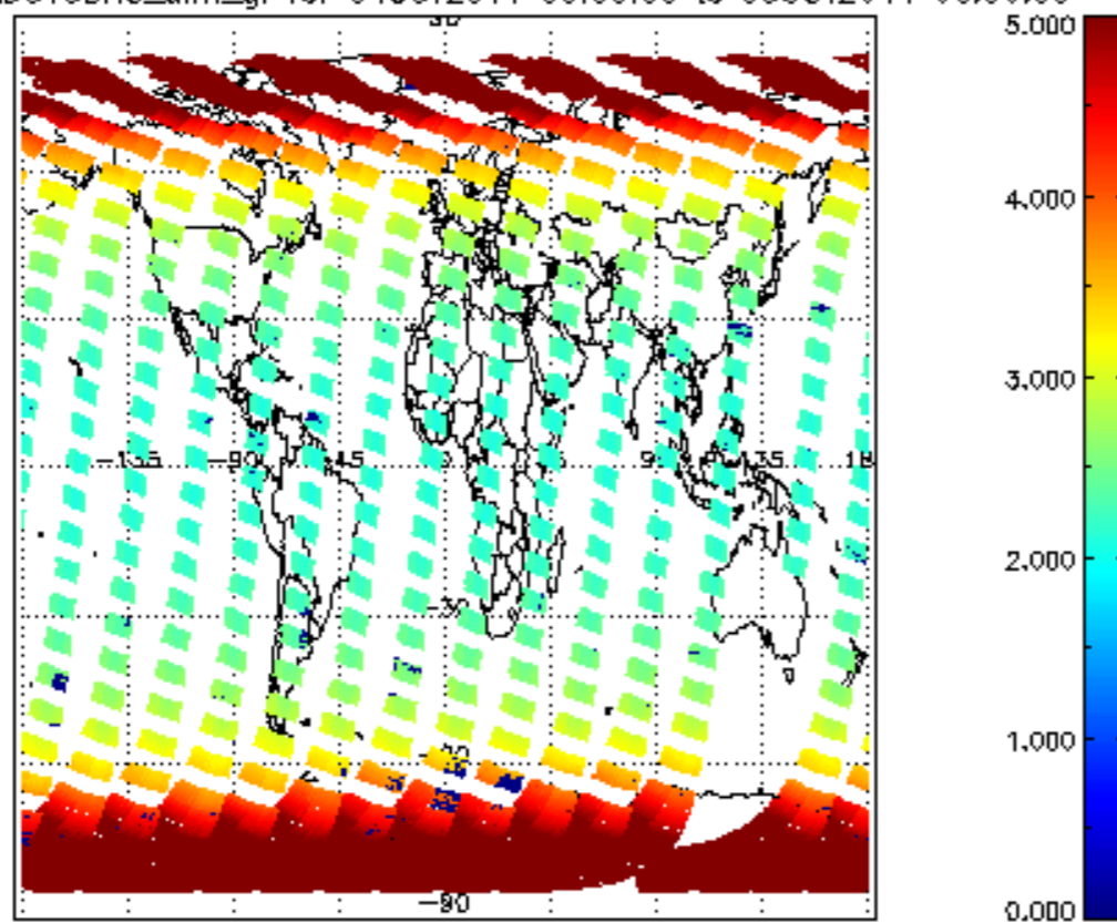
SCIOL2P_NADUV3BRO_amf_gr for 04OCT2011 00:00:00 to 05OCT2011 00:00:00
