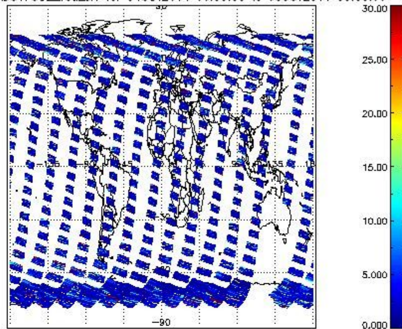
SCIOL2P_NADUV7S02_vcd_err for 04OCT2011 00:00:00 to 05OCT2011 00:00:00
