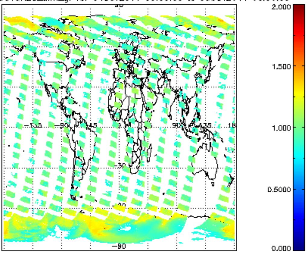
SCIOL2P_NADUV8H20_amf_gr for 04OCT2011 00:00:00 to 05OCT2011 00:00:00
