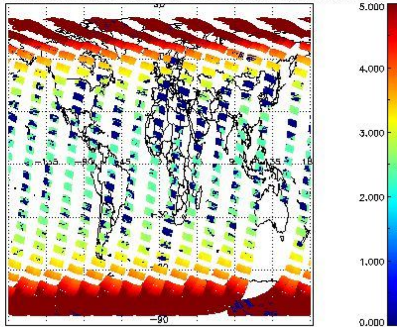
SCIOL2P_NADUV003_amf_cl for 04OCT2011 00:00:00 to 05OCT2011 00:00:00
