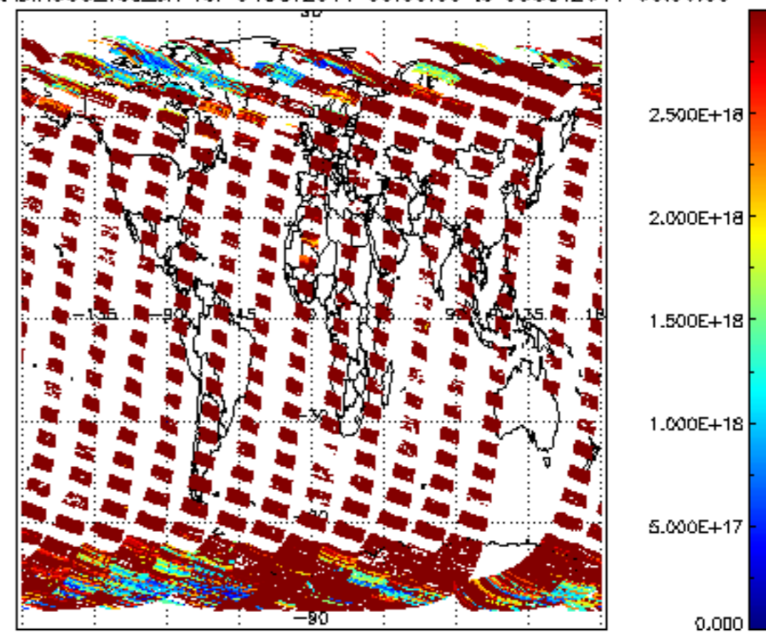
SCIOL2P_NADIR3CO_vcd_err for 04OCT2011 00:00:00 to 05OCT2011 00:00:00
