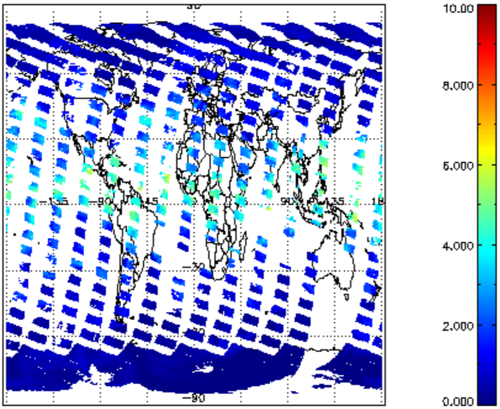
SCIOL2P_NADUV8H20_vcd for 04OCT2011 00:00:00 to 05OCT2011 00:00:00
