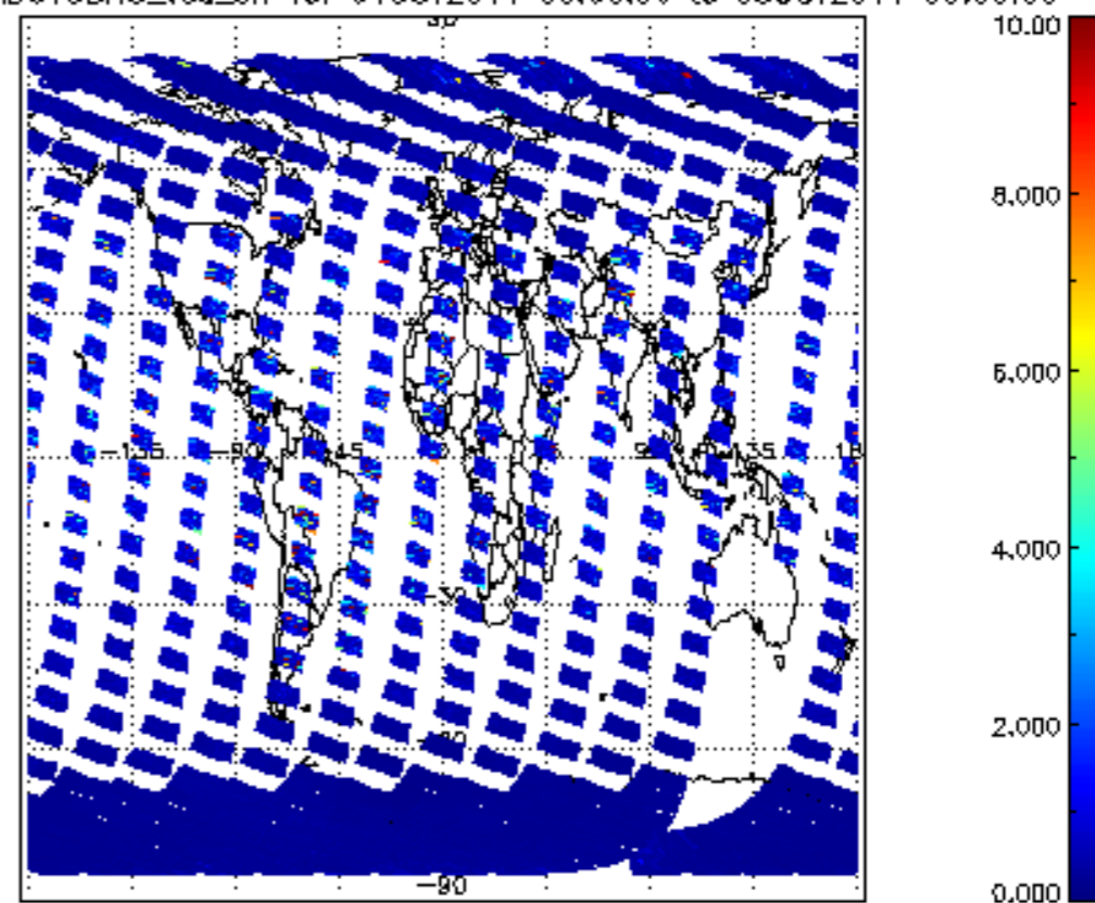
SCIOL2P_NADUV3BRO_vcd_err for 04OCT2011 00:00:00 to 05OCT2011 00:00:00
