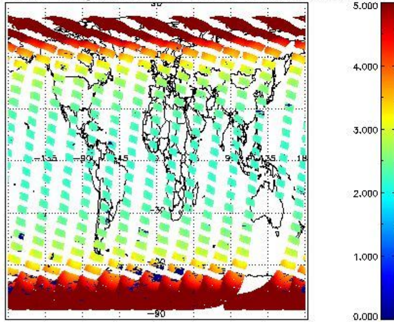
SCIOL2P_NADUV1NO2_amf_gr for 04OCT2011 00:00:00 to 05OCT2011 00:00:00
