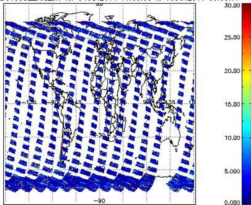
SCIOL2P_NADUV5SO2_vcd_err for 04OCT2011 00:00:00 to 05OCT2011 00:00:00
