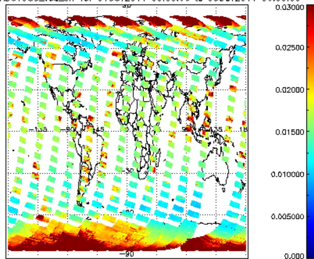
SCIOL2P_NADUV003_vcd_err for 04OCT2011 00:00:00 to 05OCT2011 00:00:00
