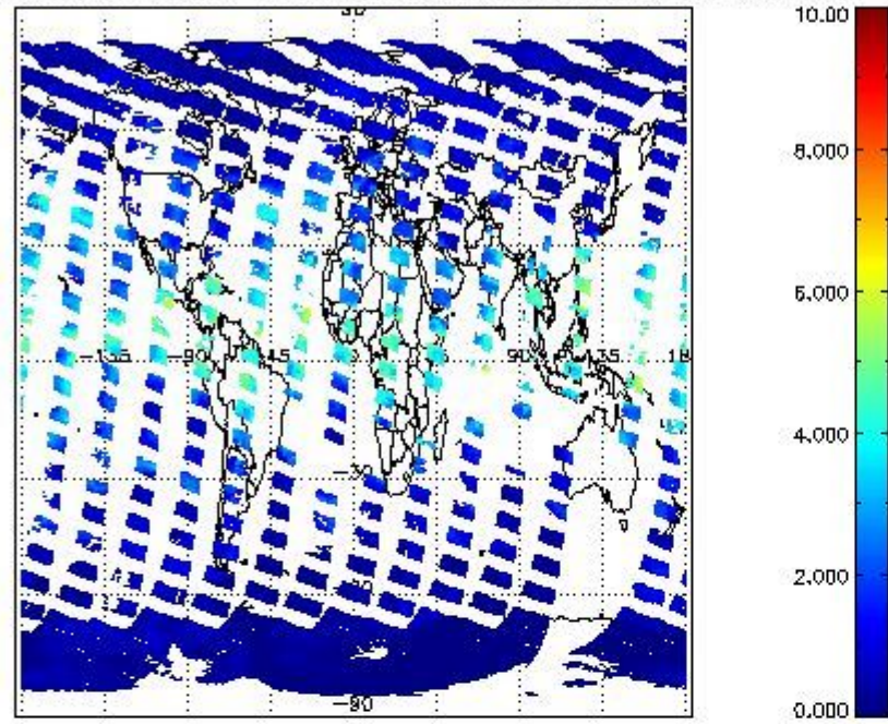
SCIOL2P_NADUV8H20_vcd for 04OCT2011 00:00:00 to 05OCT2011 00:00:00
