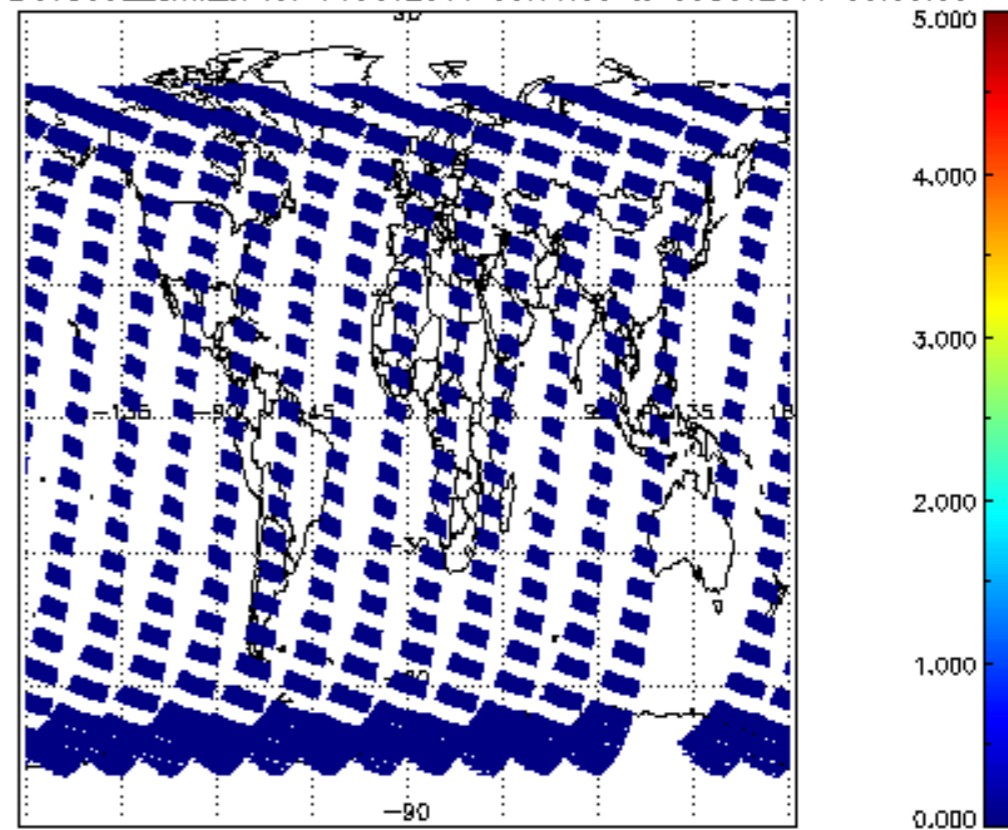
SCIOL2P_NADUV5S02_amf_cl for 04OCT2011 00:00:00 to 05OCT2011 00:00:00
