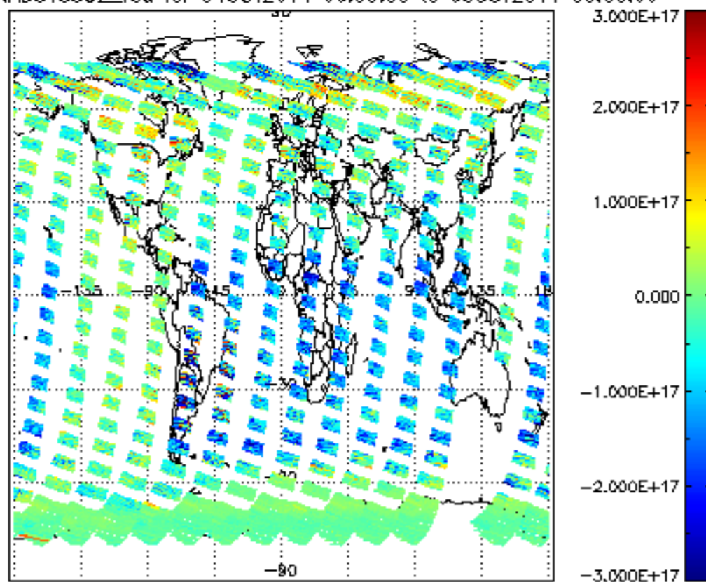
SCIOL2P_NADUV5S02_vcd for 04OCT2011 00:00:00 to 05OCT2011 00:00:00
