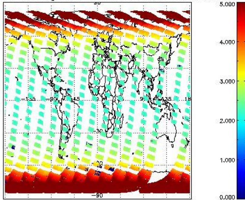
SCIOL2P_NADUV003_amf_gr for 04OCT2011 00:00:00 to 05OCT2011 00:00:00
