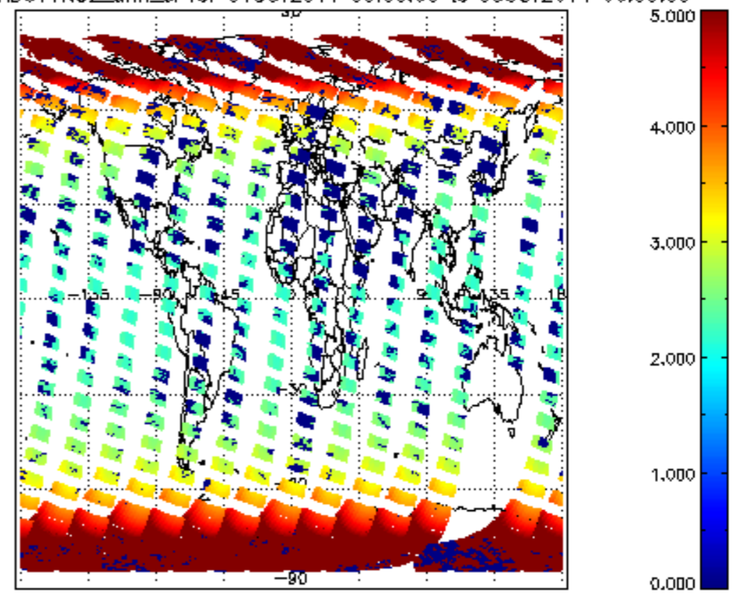
SCIOL2P_NADUV1NO2_amf_cl for 04OCT2011 00:00:00 to 05OCT2011 00:00:00
