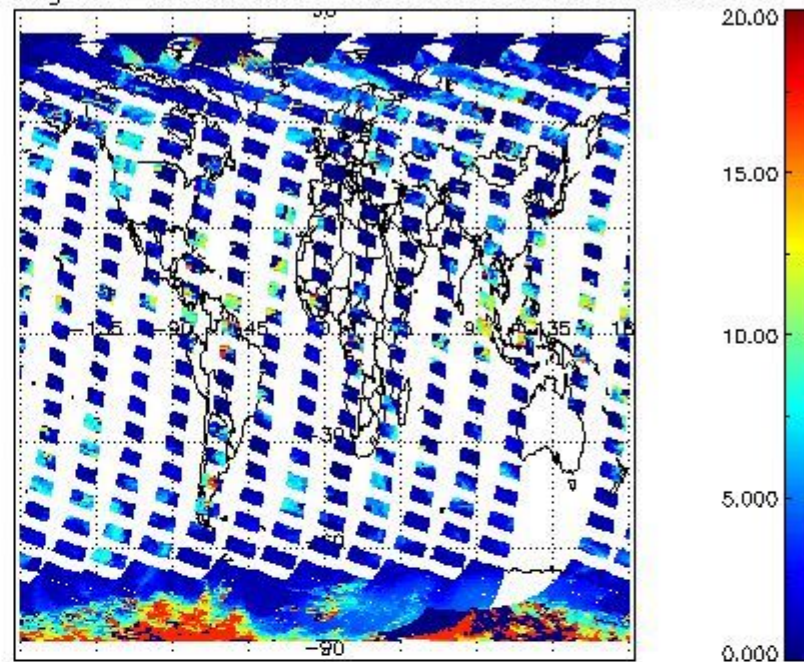
cL_top_height for 04OCT2011 00:00:00 to 05OCT2011 00:00:00
