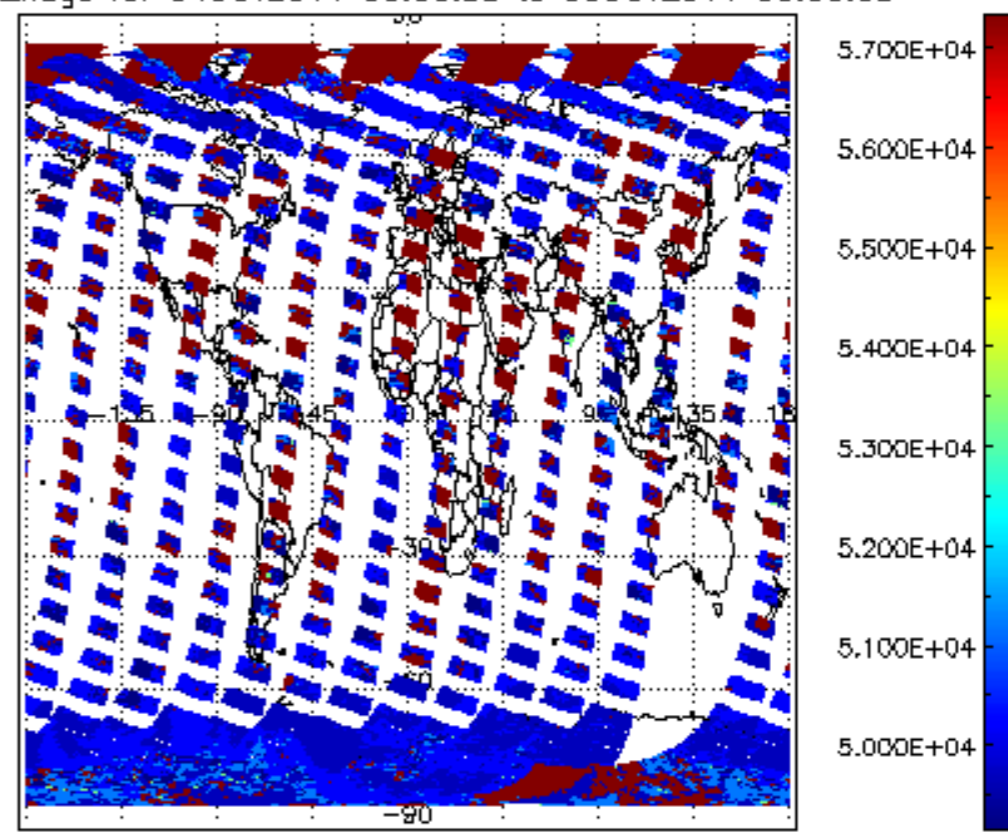
cloud_flags for 04OCT2011 00:00:00 to 05OCT2011 00:00:00
