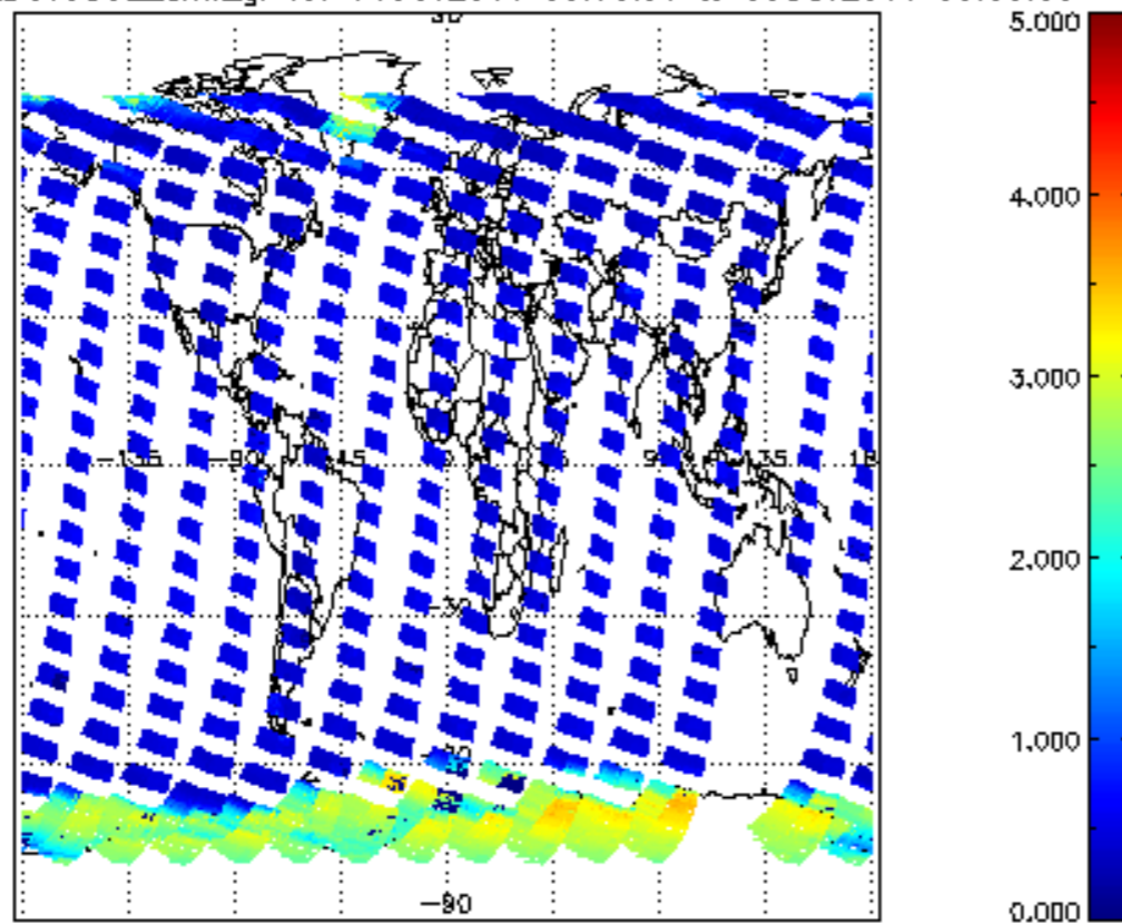
SCIOL2P_NADUV5S02_amf_gr for 04OCT2011 00:00:00 to 05OCT2011 00:00:00
