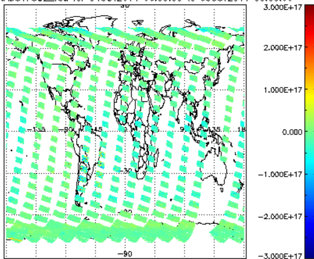
SCIOL2P_NADUV7S02_vcd for 04OCT2011 00:00:00 to 05OCT2011 00:00:00
