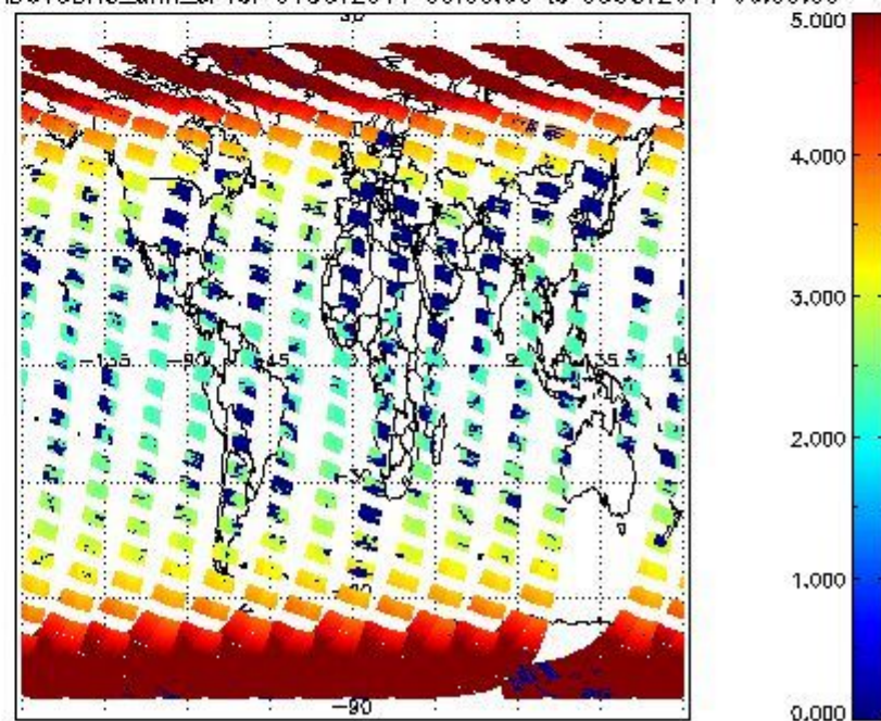
SCIOL2P_NADUV3BRO_amf_cl for 04OCT2011 00:00:00 to 05OCT2011 00:00:00
