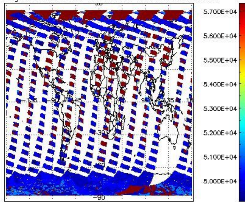
cloud_flags for 04OCT2011 00:00:00 to 05OCT2011 00:00:00
