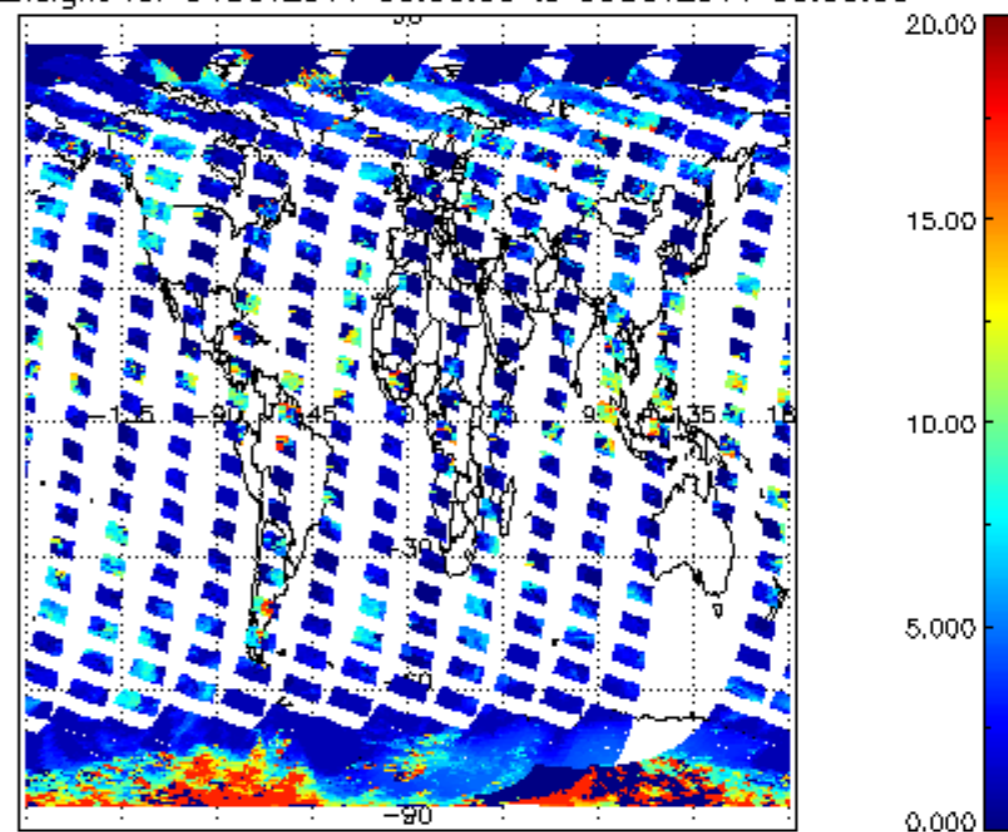
cl_top_height for 04OCT2011 00:00:00 to 05OCT2011 00:00:00
