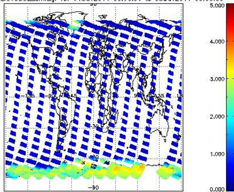
SCIOL2P_NADUV5SO2_amf_gr for 04OCT2011 00:00:00 to 05OCT2011 00:00:00
