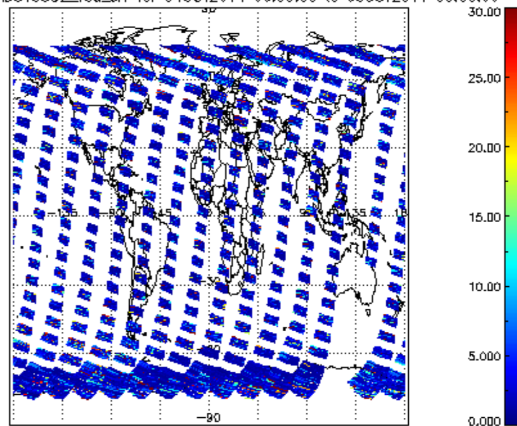
SCIOL2P_NADUV5S02_vcd_err for 04OCT2011 00:00:00 to 05OCT2011 00:00:00
