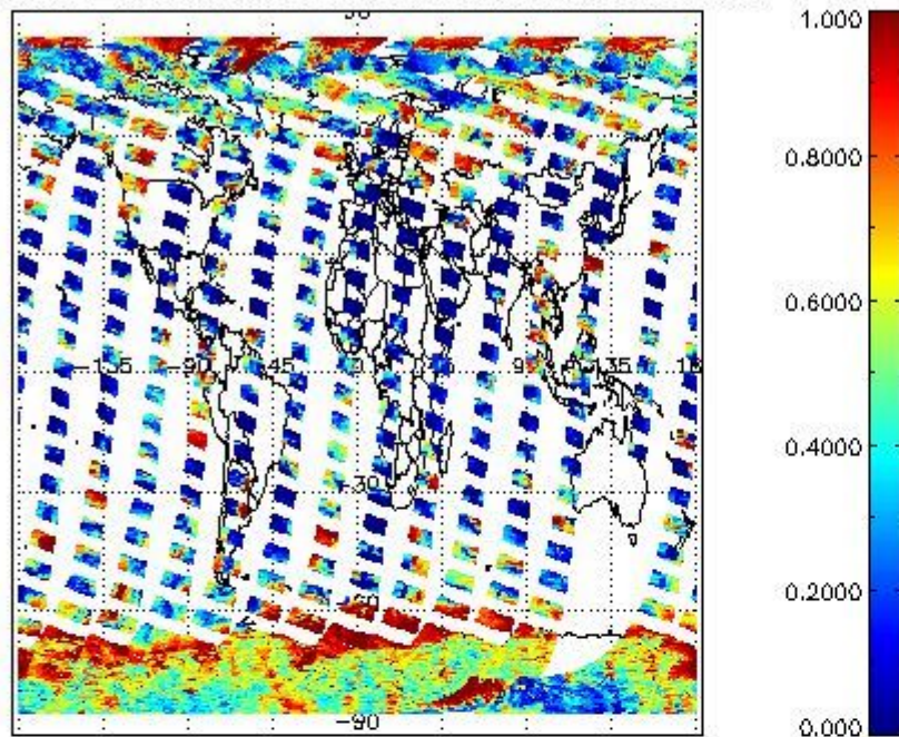
cLfrac for 04OCT2011 00:00:00 to 05OCT2011 00:00:00
