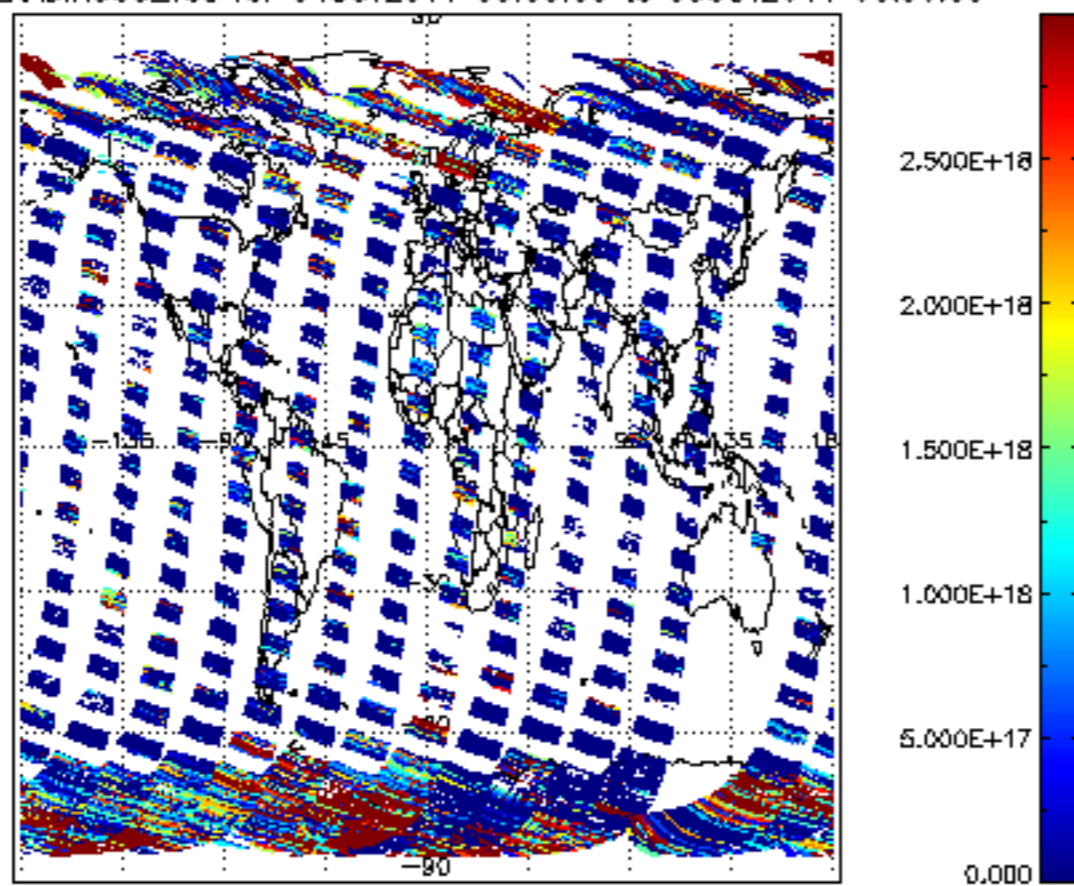
SCIOL2P_NADIR3CO_vcd for 04OCT2011 00:00:00 to 05OCT2011 00:00:00
