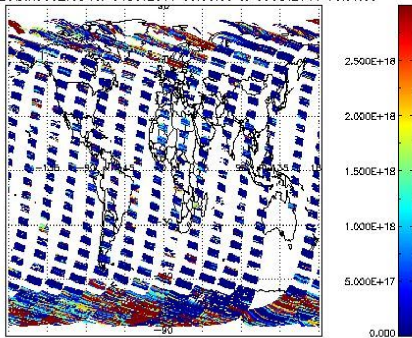
SCIOL2P_NADIR3CO_vcd for 04OCT2011 00:00:00 to 05OCT2011 00:00:00
