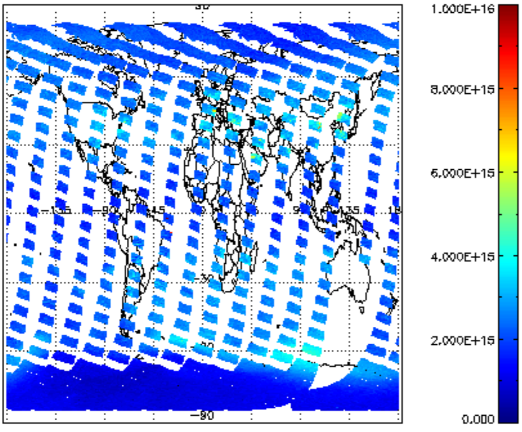
SCIOL2P_NADUV1NO2_vcd for 04OCT2011 00:00:00 to 05OCT2011 00:00:00
