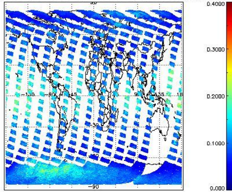
SCIOL2P_NADUV1NO2_vcd_err for 04OCT2011 00:00:00 to 05OCT2011 00:00:00
