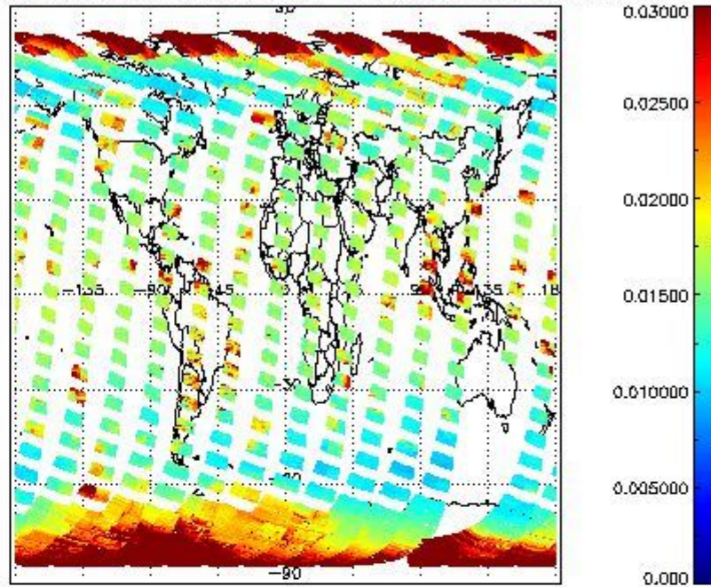
SCIOL2P_NADUV003_vcd_err for 04OCT2011 00:00:00 to 05OCT2011 00:00:00
