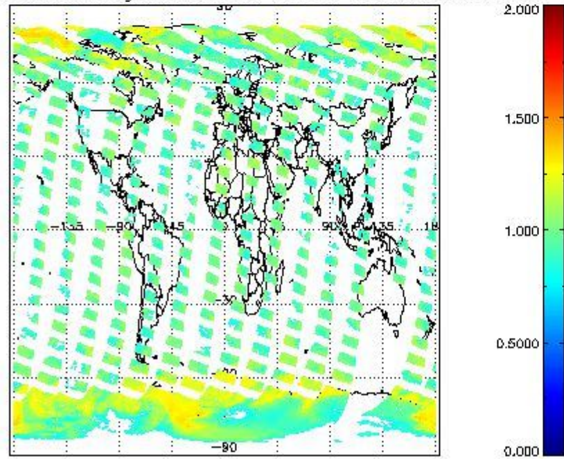
SCIOL2P_NADUV8H20_amf_gr for 04OCT2011 00:00:00 to 05OCT2011 00:00:00
