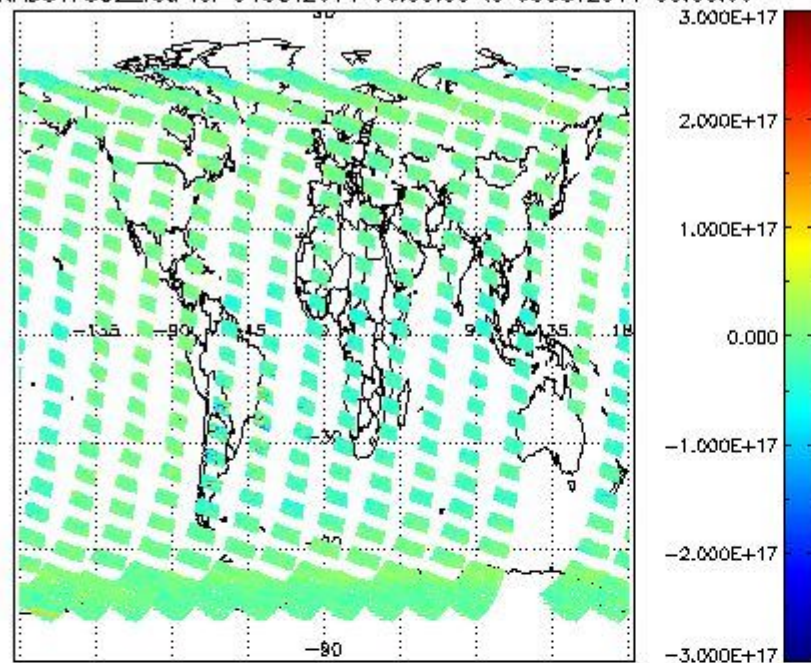
SCIOL2P_NADUV7S02_vcd for 04OCT2011 00:00:00 to 05OCT2011 00:00:00
