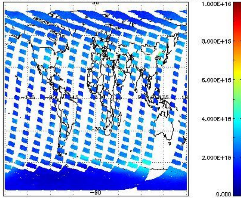
SCIOL2P_NADUV1NO2_vcd for 04OCT2011 00:00:00 to 05OCT2011 00:00:00
