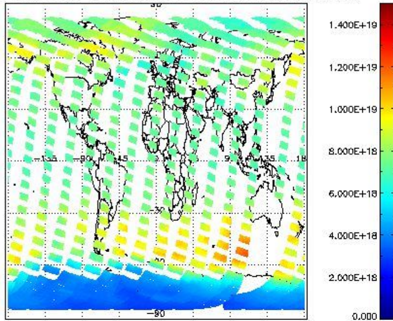
SCIOL2P_NADUV003_vcd for 04OCT2011 00:00:00 to 05OCT2011 00:00:00
