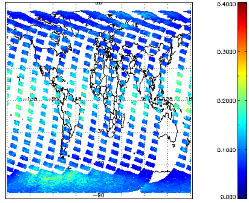
SCIOL2P_NADUV1NO2_vcd_err for 04OCT2011 00:00:00 to 05OCT2011 00:00:00
