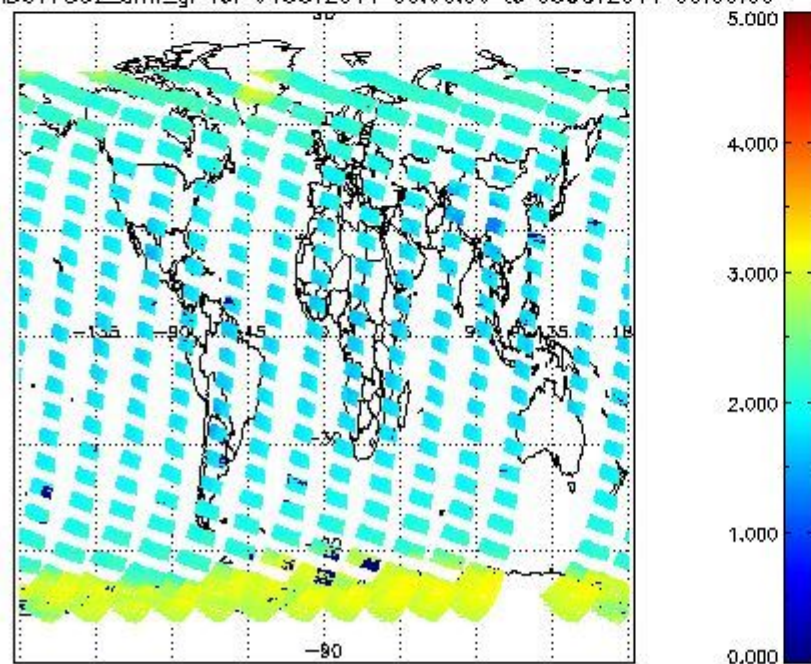
SCIOL2P_NADUV7S02_amf_gr for 04OCT2011 00:00:00 to 05OCT2011 00:00:00
