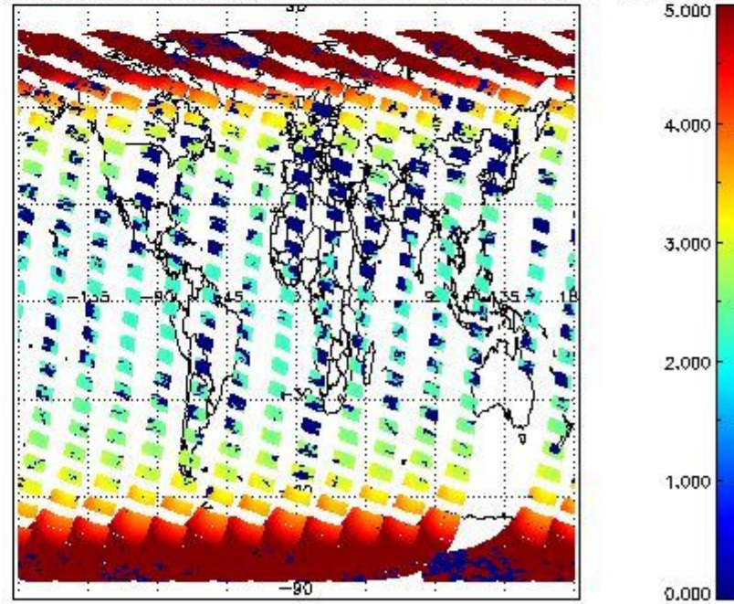
SCIOL2P_NADUV1NO2_amf_cl for 04OCT2011 00:00:00 to 05OCT2011 00:00:00
