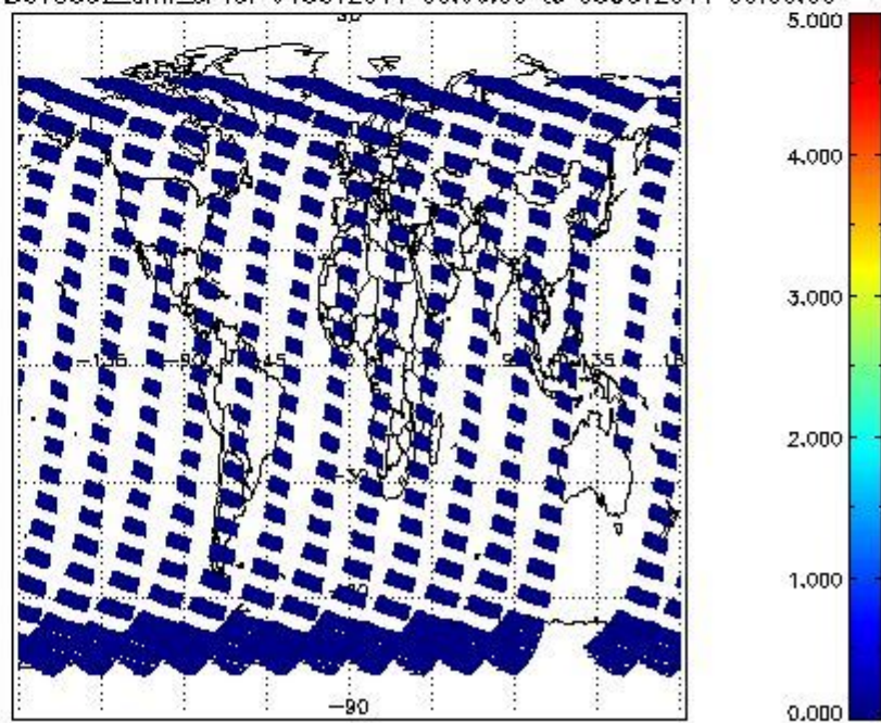
SCIOL2P_NADUV5SO2_amf_cl for 04OCT2011 00:00:00 to 05OCT2011 00:00:00
