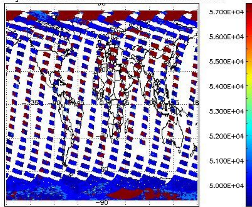
cloud_flags for 03OCT2011 00:00:00 to 04OCT2011 00:00:00
