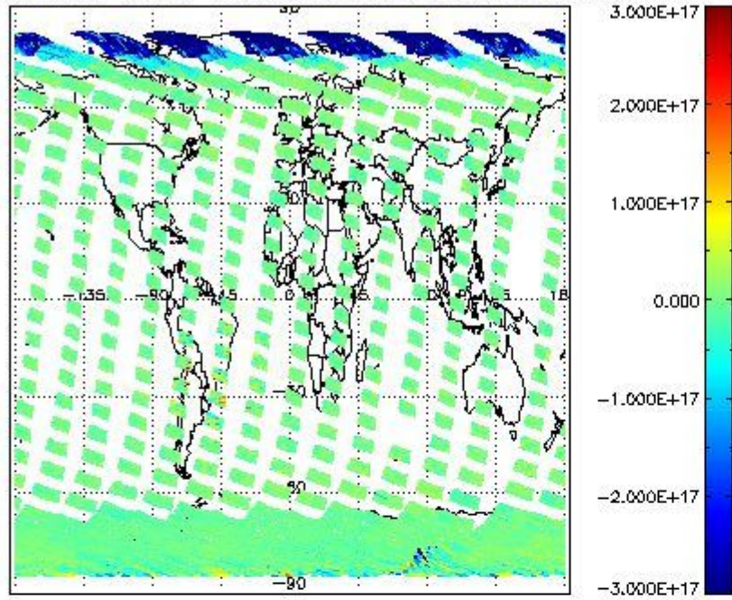
SCIOL2P_NADUV7S02_vcd for 03OCT2011 00:00:00 to 04OCT2011 00:00:00
