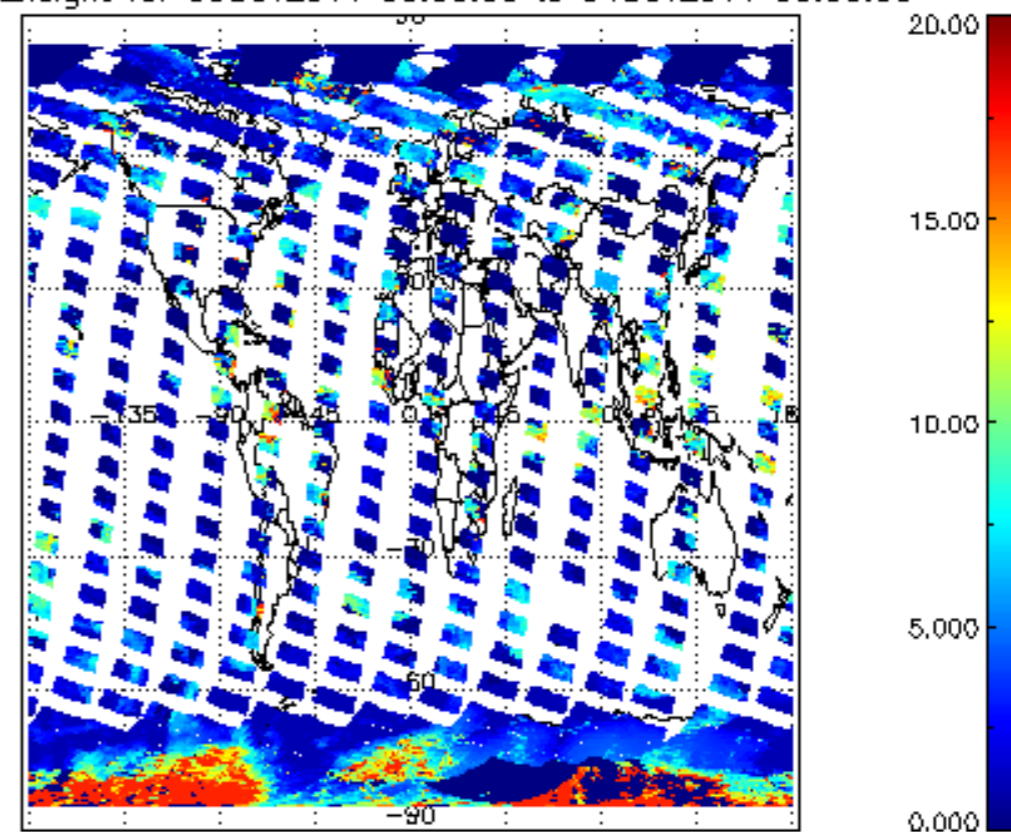
cl_top_height for 03OCT2011 00:00:00 to 04OCT2011 00:00:00
