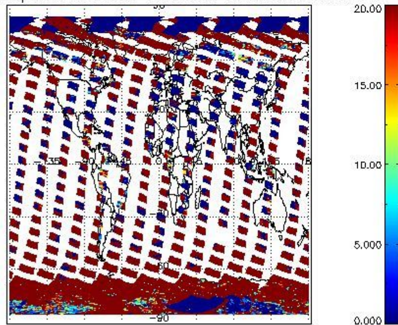
cL_opt_depth for 03OCT2011 00:00:00 to 04OCT2011 00:00:00
