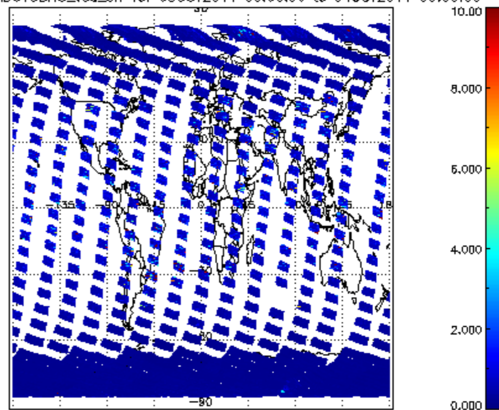
SCIOL2P_NADUV3BRO_vcd_err for 03OCT2011 00:00:00 to 04OCT2011 00:00:00
