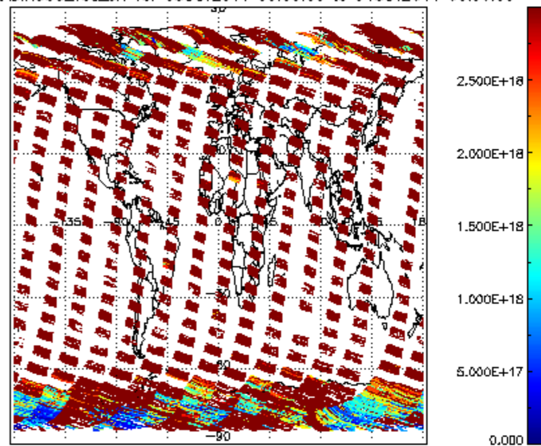
SCIOL2P_NADIR3CO_vcd_err for 03OCT2011 00:00:00 to 04OCT2011 00:00:00
