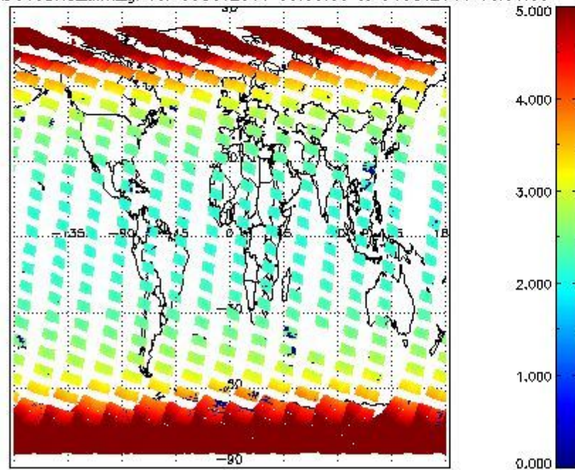
SCIOL2P_NADUV3BRO_amf_gr for 03OCT2011 00:00:00 to 04OCT2011 00:00:00
