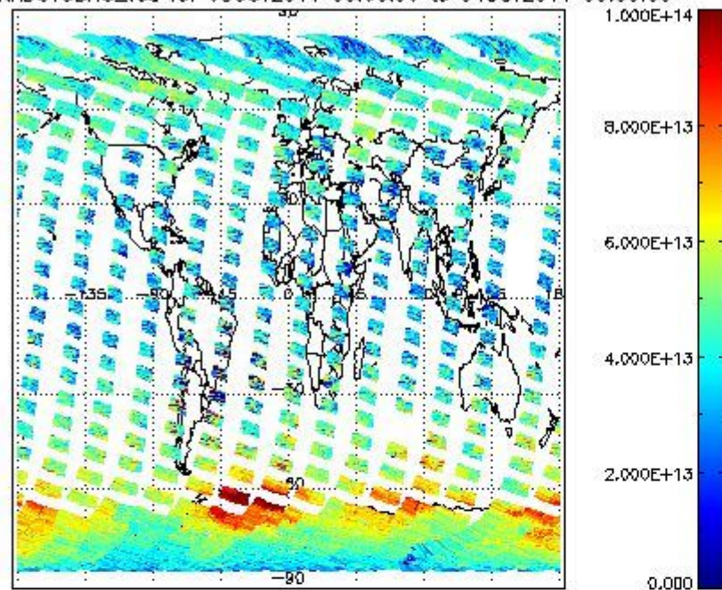
SCIOL2P_NADUV3BRO_vcd for 03OCT2011 00:00:00 to 04OCT2011 00:00:00
