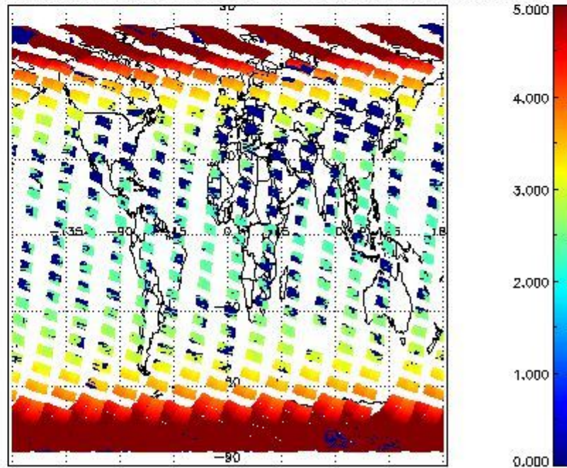
SCIOL2P_NADUV003_amf_cl for 03OCT2011 00:00:00 to 04OCT2011 00:00:00
