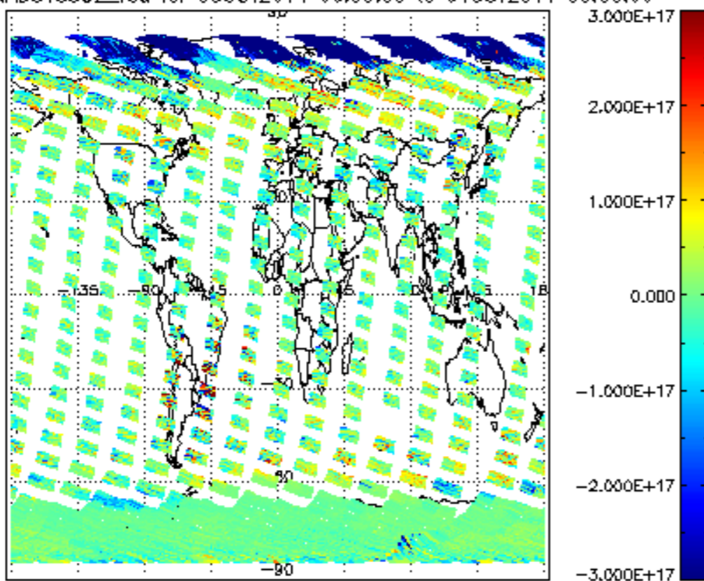
SCIOL2P_NADUV5S02_vcd for 03OCT2011 00:00:00 to 04OCT2011 00:00:00
