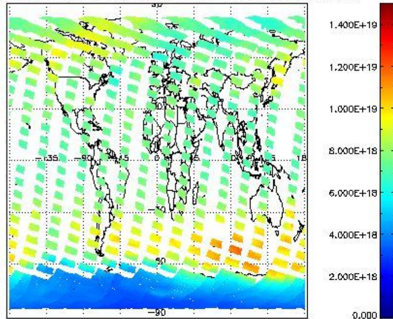
SCIOL2P_NADUV003_vcd for 03OCT2011 00:00:00 to 04OCT2011 00:00:00
