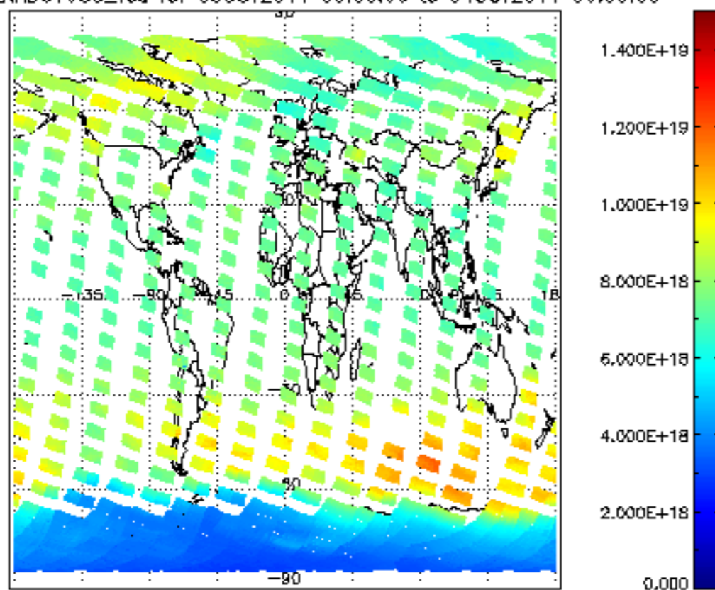
SCIOL2P_NADUV003_vcd for 03OCT2011 00:00:00 to 04OCT2011 00:00:00
