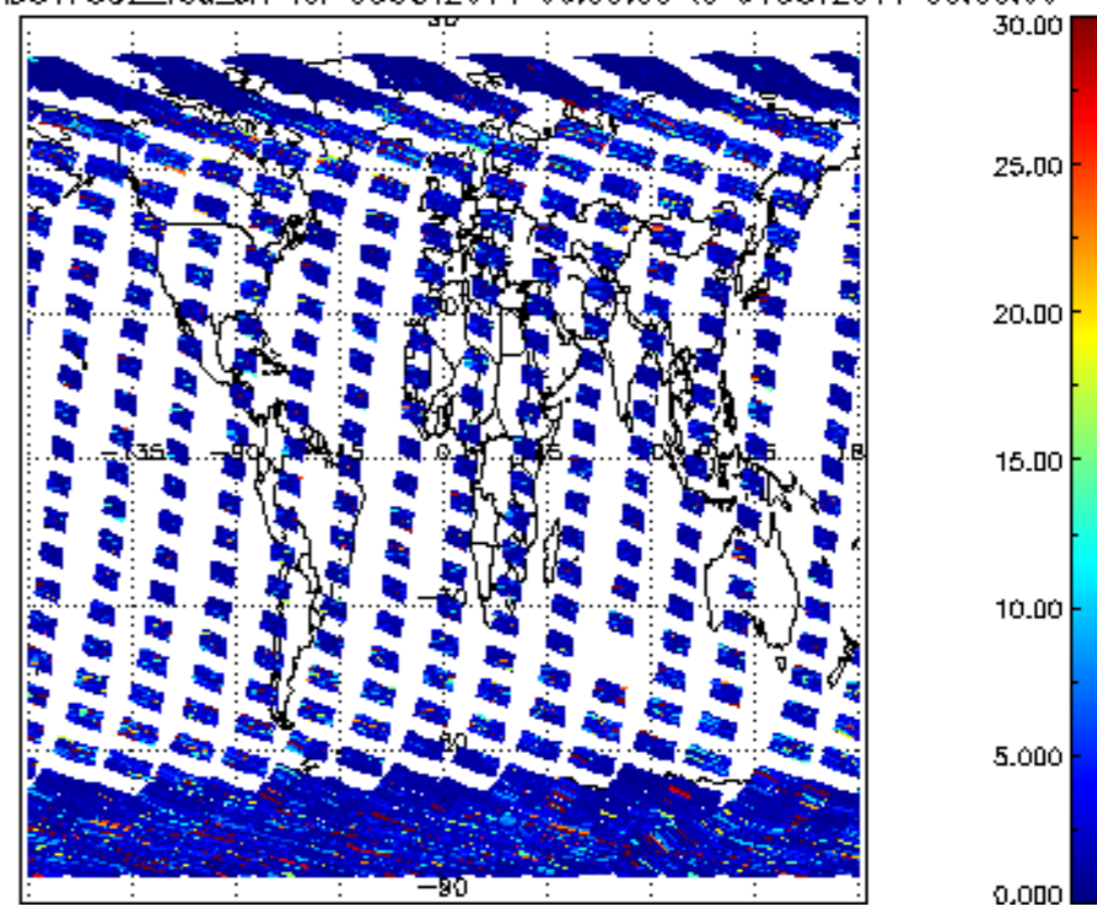
SCIOL2P_NADUV7S02_vcd_err for 03OCT2011 00:00:00 to 04OCT2011 00:00:00
