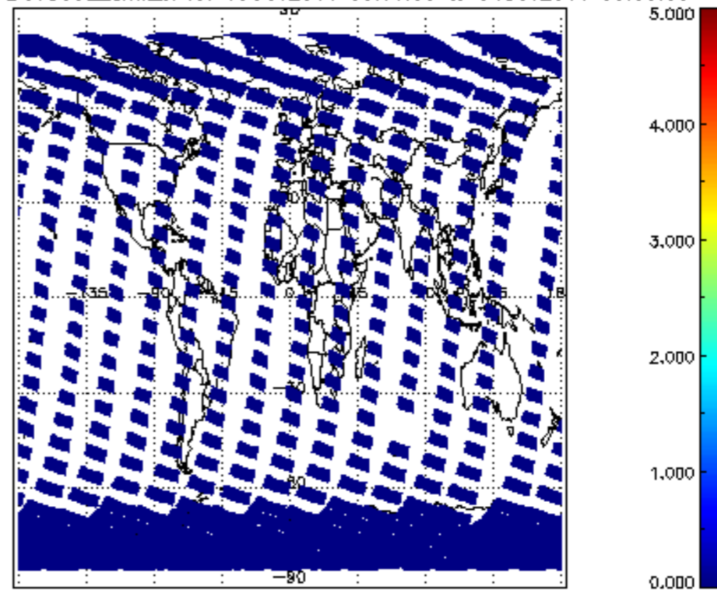
SCIOL2P_NADUV5S02_amf_cl for 03OCT2011 00:00:00 to 04OCT2011 00:00:00
