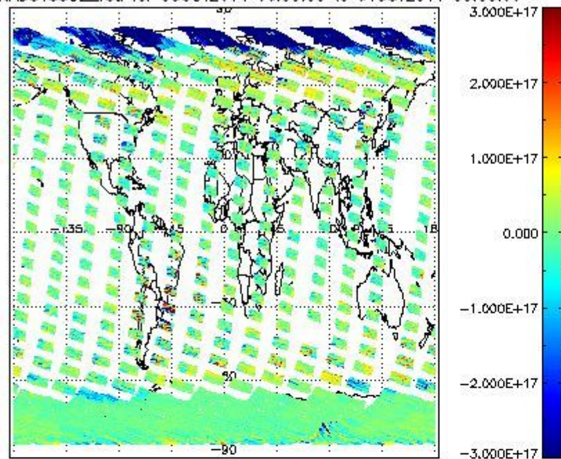
SCIOL2P_NADUV5SO2_vcd for 03OCT2011 00:00:00 to 04OCT2011 00:00:00
