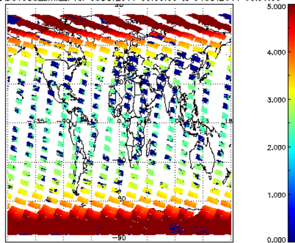
SCIOL2P_NADUV003_amf_cl for 03OCT2011 00:00:00 to 04OCT2011 00:00:00
