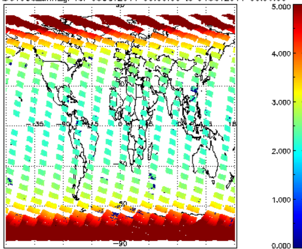
SCIOL2P_NADUV003_amf_gr for 03OCT2011 00:00:00 to 04OCT2011 00:00:00
