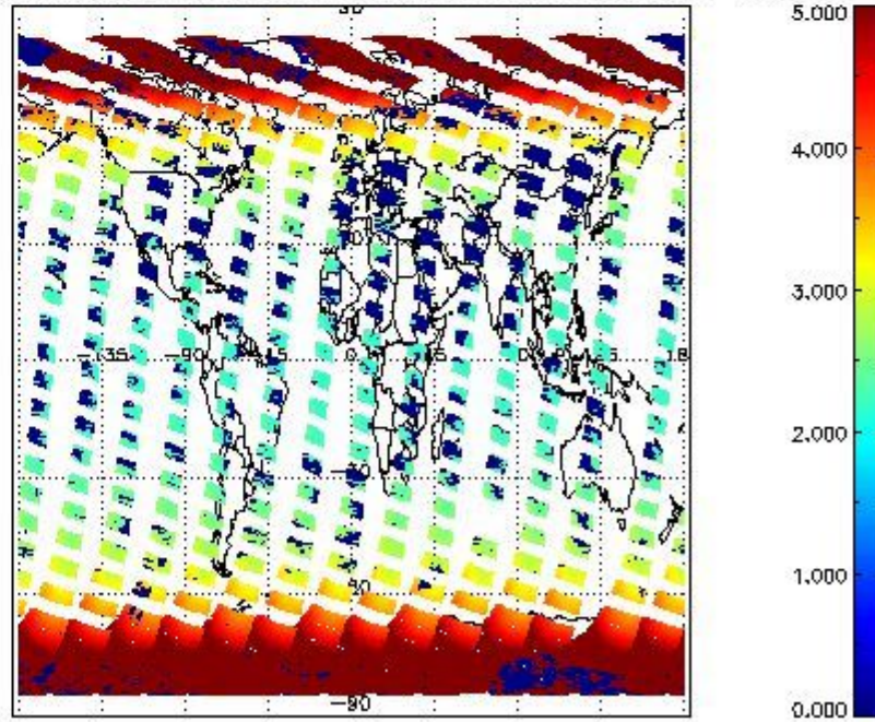
SCIOL2P_NADUV1NO2_amf_cl for 03OCT2011 00:00:00 to 04OCT2011 00:00:00
