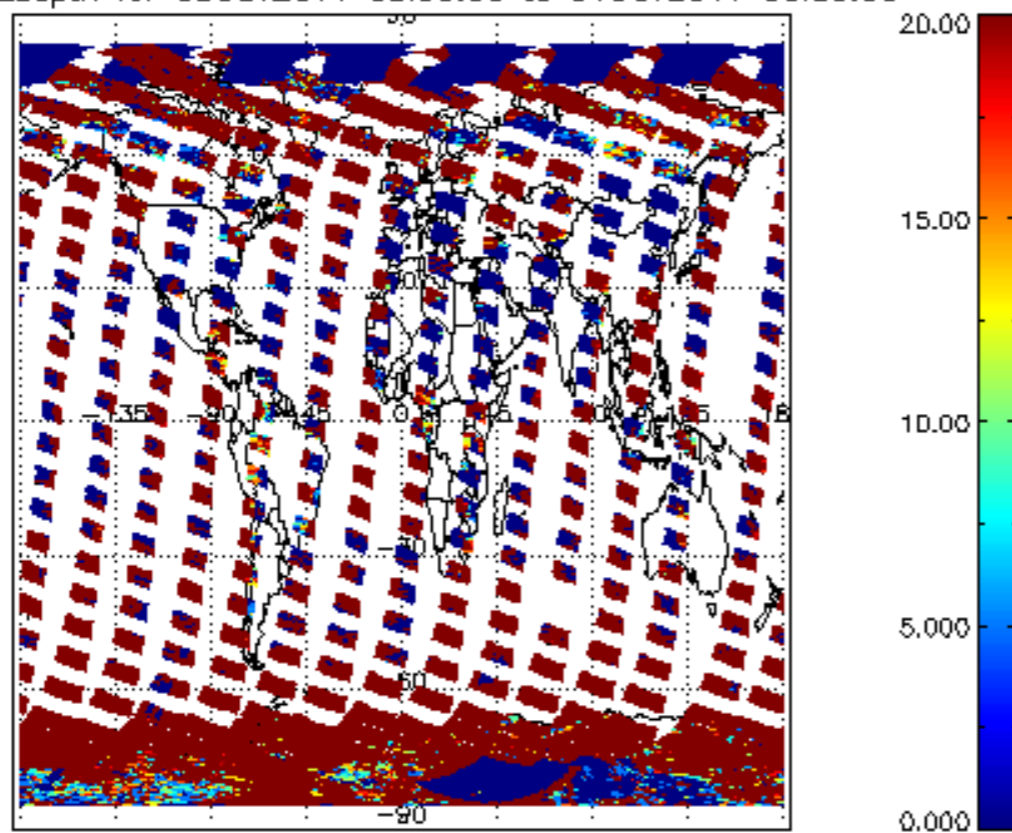
cl_opt_depth for 03OCT2011 00:00:00 to 04OCT2011 00:00:00
