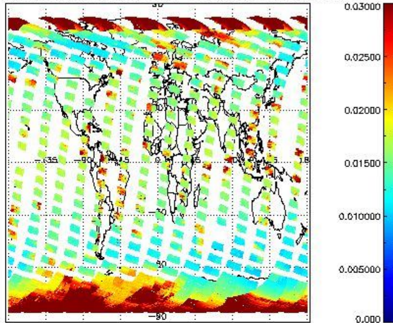
SCIOL2P_NADUV003_vcd_err for 03OCT2011 00:00:00 to 04OCT2011 00:00:00
