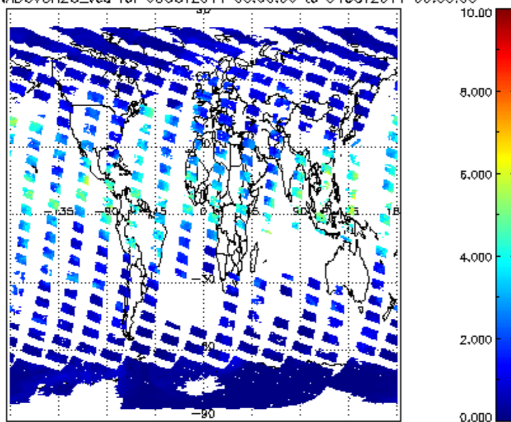
SCIOL2P_NADUV8H20_vcd for 03OCT2011 00:00:00 to 04OCT2011 00:00:00
