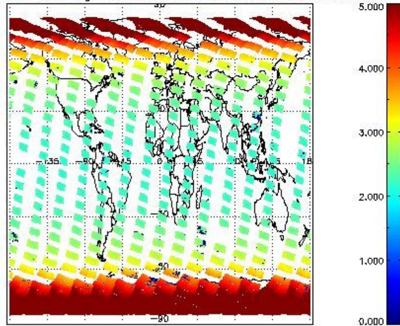
SCIOL2P_NADUV003_amf_gr for 03OCT2011 00:00:00 to 04OCT2011 00:00:00
