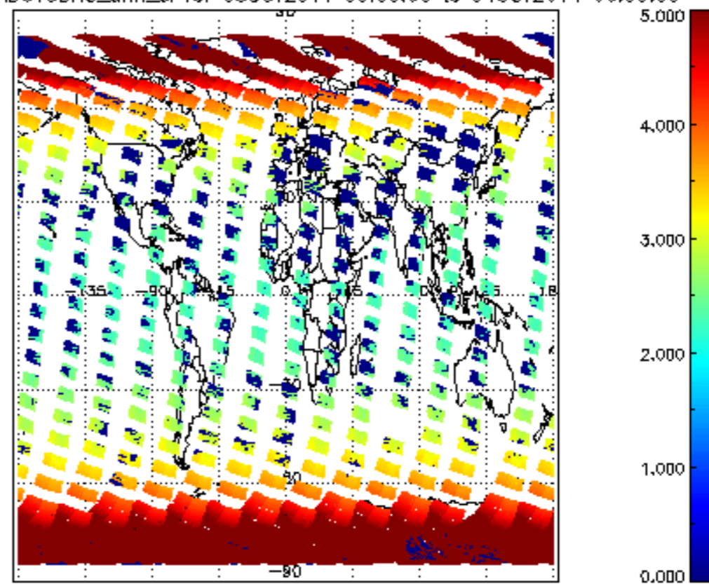
SCIOL2P_NADUV3BRO_amf_cl for 03OCT2011 00:00:00 to 04OCT2011 00:00:00
