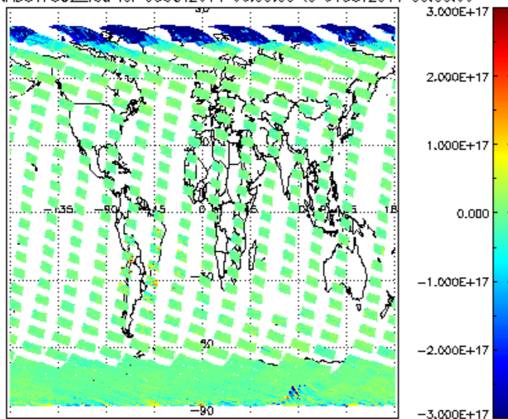
SCIOL2P_NADUV7S02_vcd for 03OCT2011 00:00:00 to 04OCT2011 00:00:00
