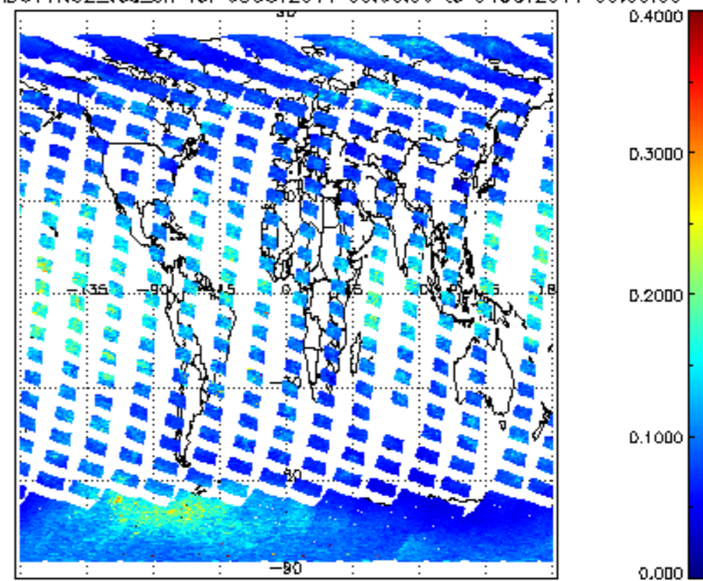
SCIOL2P_NADUV1NO2_vcd_err for 03OCT2011 00:00:00 to 04OCT2011 00:00:00
