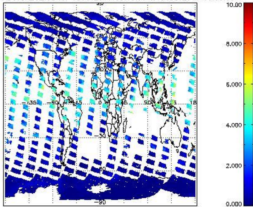
SCIOL2P_NADUV8H20_vcd for 03OCT2011 00:00:00 to 04OCT2011 00:00:00
