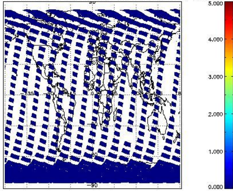
SCIOL2P_NADUV7S02_amf_cl for 03OCT2011 00:00:00 to 04OCT2011 00:00:00
