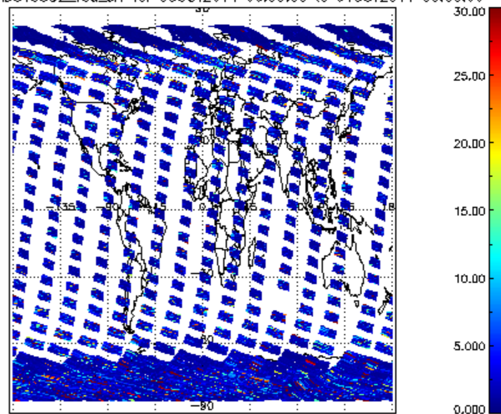
SCIOL2P_NADUV5S02_vcd_err for 03OCT2011 00:00:00 to 04OCT2011 00:00:00
