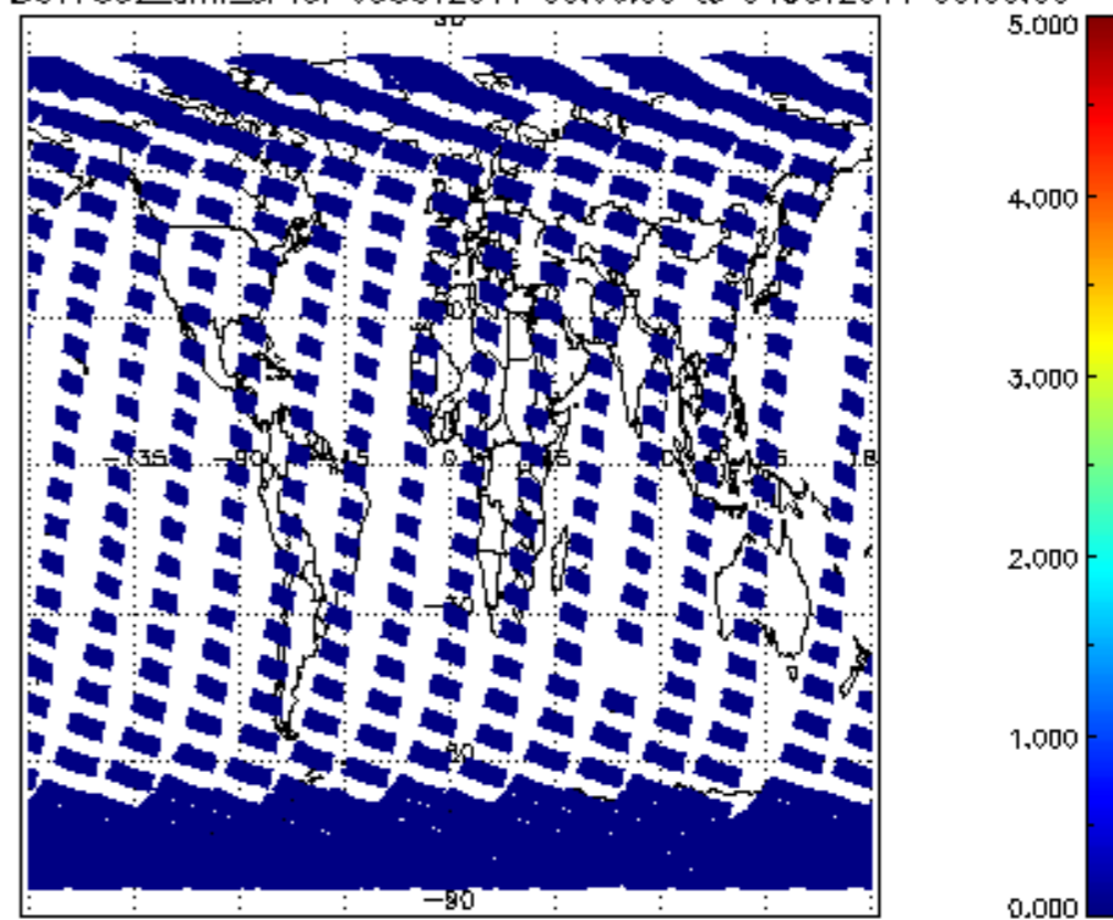
SCIOL2P_NADUV7S02_amf_cl for 03OCT2011 00:00:00 to 04OCT2011 00:00:00
