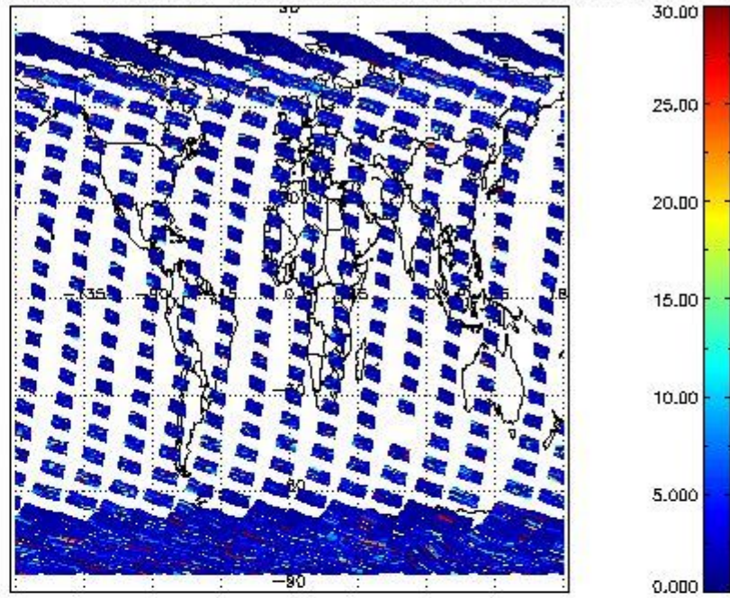
SCIOL2P_NADUV7S02_vcd_err for 03OCT2011 00:00:00 to 04OCT2011 00:00:00
