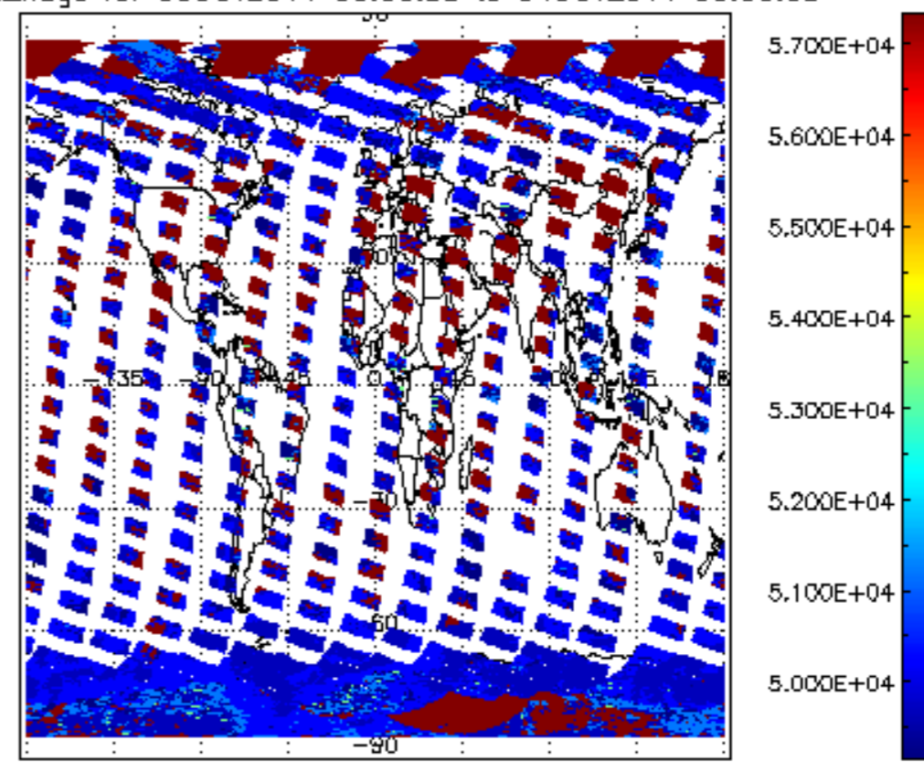
cloud_flags for 03OCT2011 00:00:00 to 04OCT2011 00:00:00
