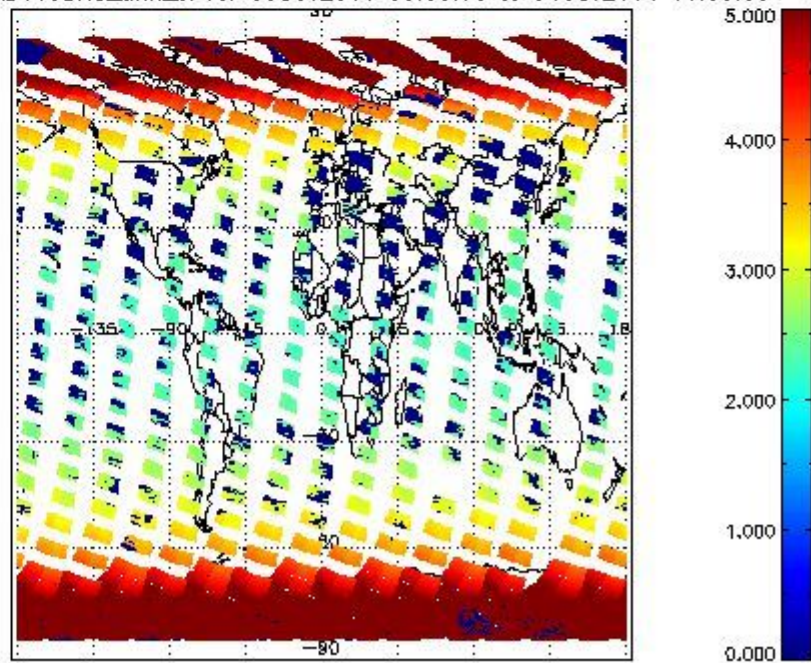
SCIOL2P_NADUV3BRO_amf_cl for 03OCT2011 00:00:00 to 04OCT2011 00:00:00
