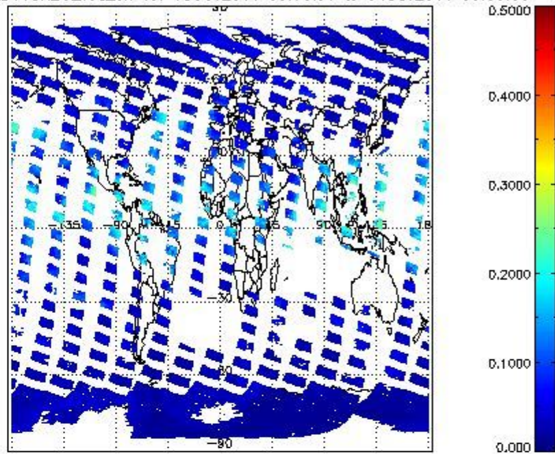
SCIOL2P_NADUV8H20_vcd_err for 03OCT2011 00:00:00 to 04OCT2011 00:00:00
