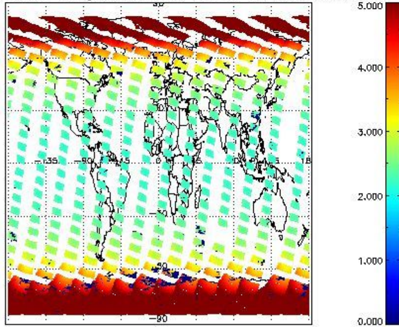
SCIOL2P_NADUV1NO2_amf_gr for 03OCT2011 00:00:00 to 04OCT2011 00:00:00
