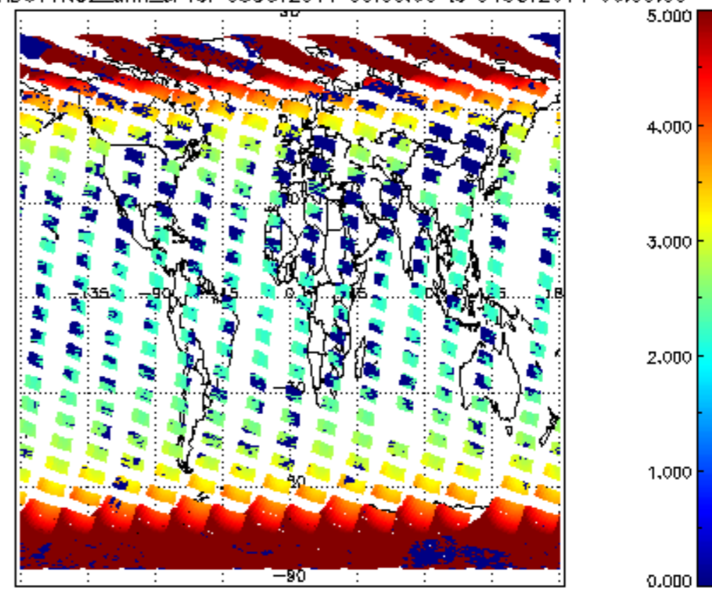
SCIOL2P_NADUV1NO2_amf_cl for 03OCT2011 00:00:00 to 04OCT2011 00:00:00
