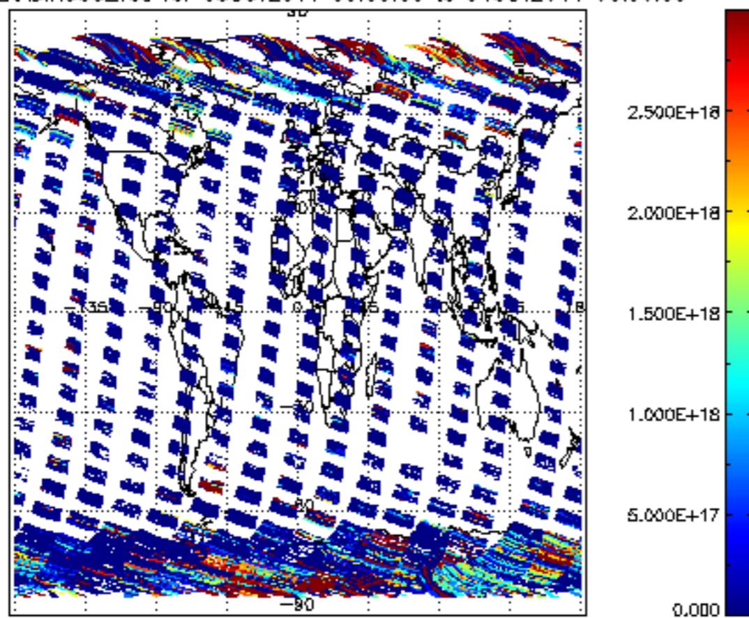
SCIOL2P_NADIR3CO_vcd for 03OCT2011 00:00:00 to 04OCT2011 00:00:00
