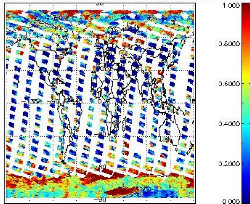
cLfrac for 03OCT2011 00:00:00 to 04OCT2011 00:00:00
