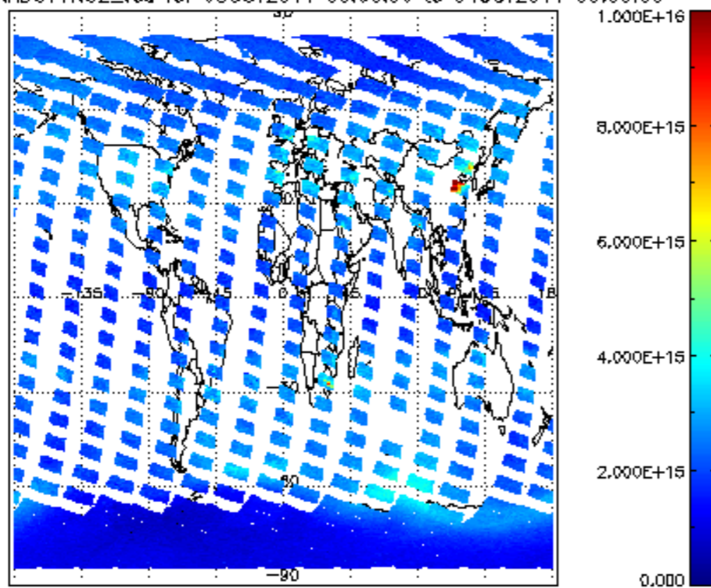
SCIOL2P_NADUV1NO2_vcd for 03OCT2011 00:00:00 to 04OCT2011 00:00:00
