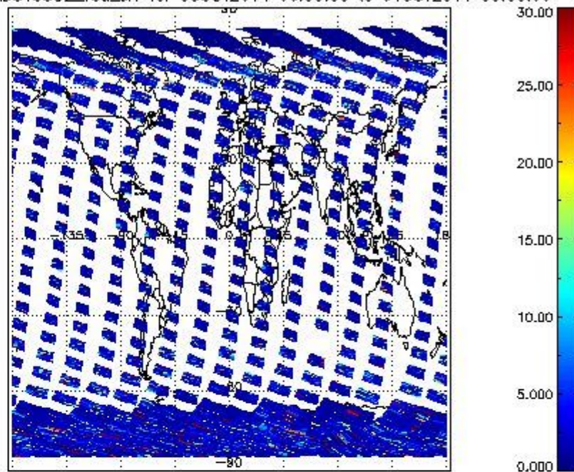
SCIOL2P_NADUV5SO2_vcd_err for 03OCT2011 00:00:00 to 04OCT2011 00:00:00
