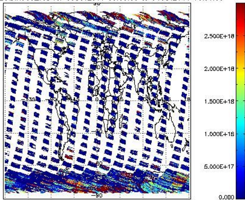
SCIOL2P_NADIR3CO_vcd for 03OCT2011 00:00:00 to 04OCT2011 00:00:00
