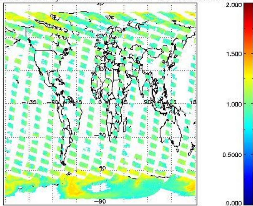
SCIOL2P_NADUV8H20_amf_gr for 03OCT2011 00:00:00 to 04OCT2011 00:00:00
