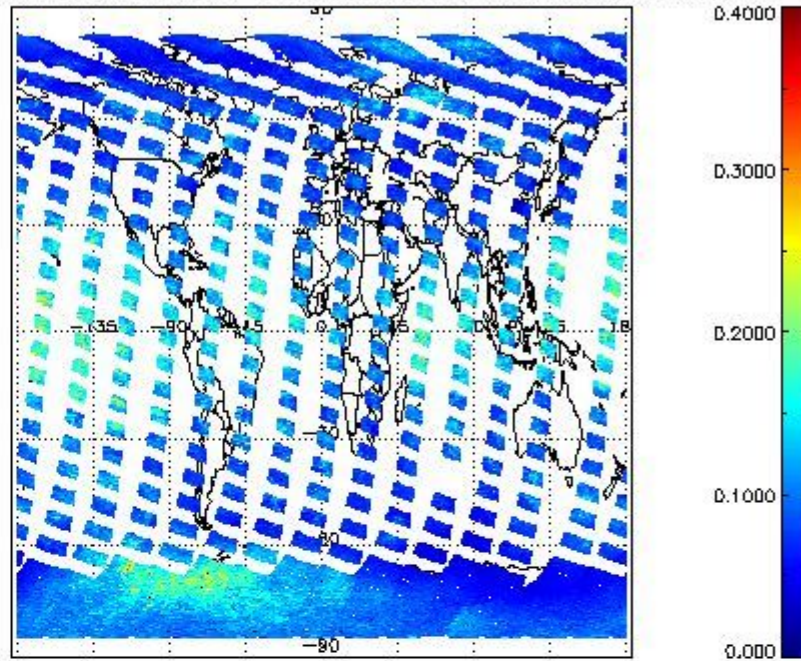
SCIOL2P_NADUV1NO2_vcd_err for 03OCT2011 00:00:00 to 04OCT2011 00:00:00
