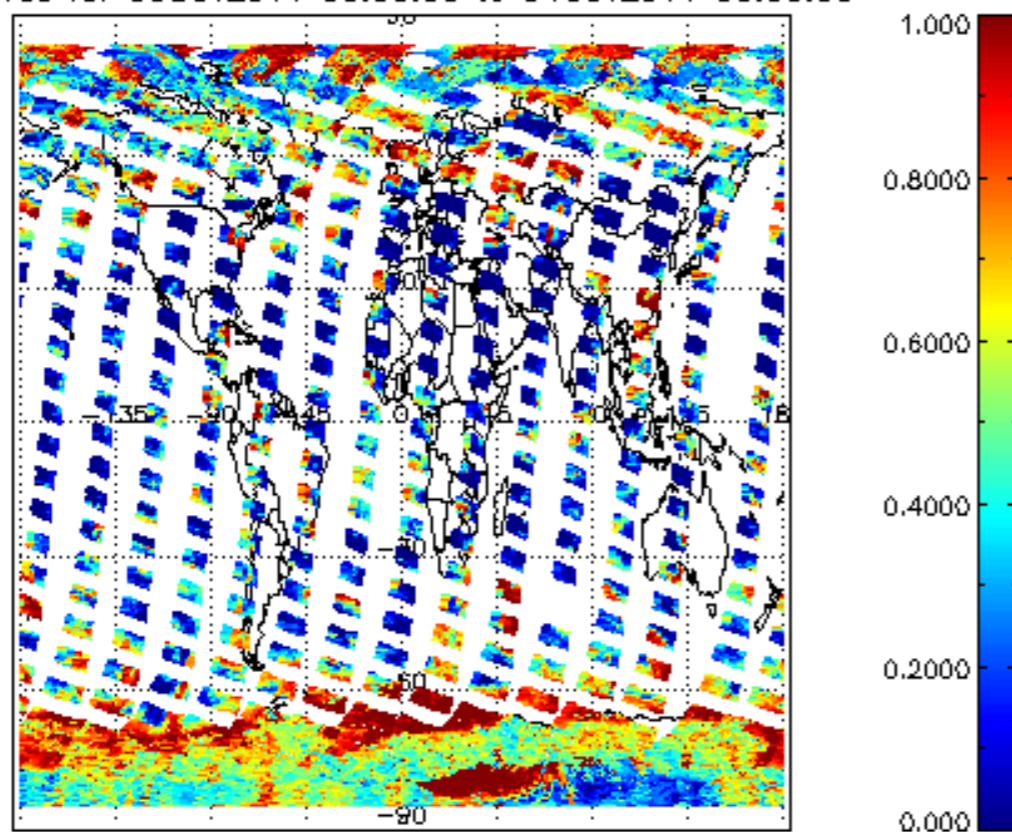
cl_frac for 03OCT2011 00:00:00 to 04OCT2011 00:00:00
