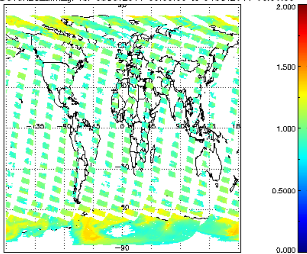
SCIOL2P_NADUV8H20_amf_gr for 03OCT2011 00:00:00 to 04OCT2011 00:00:00
