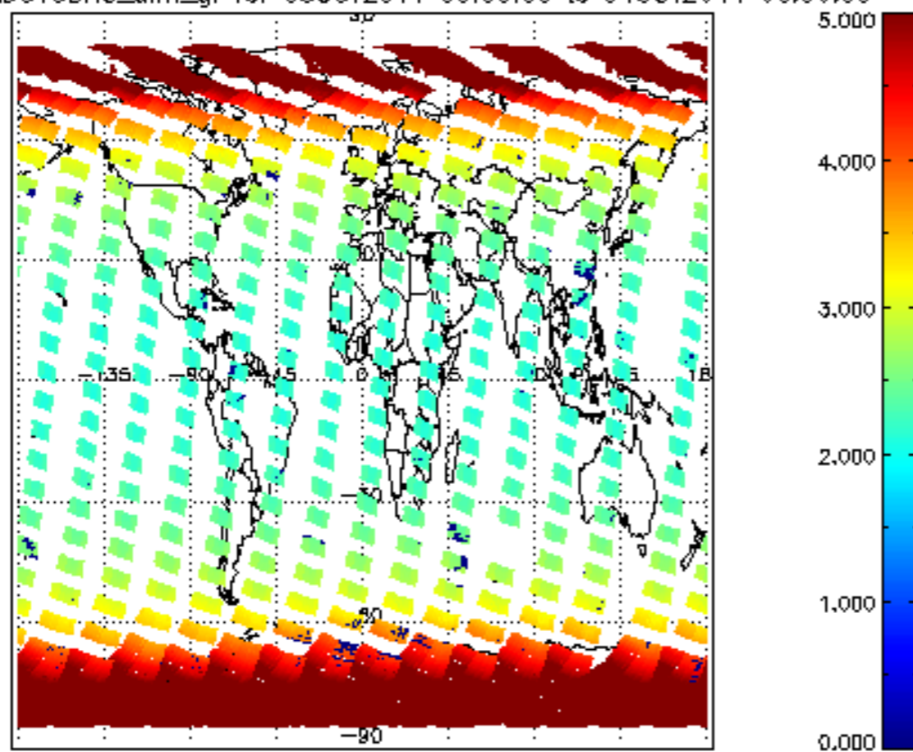
SCIOL2P_NADUV3BRO_amf_gr for 03OCT2011 00:00:00 to 04OCT2011 00:00:00
