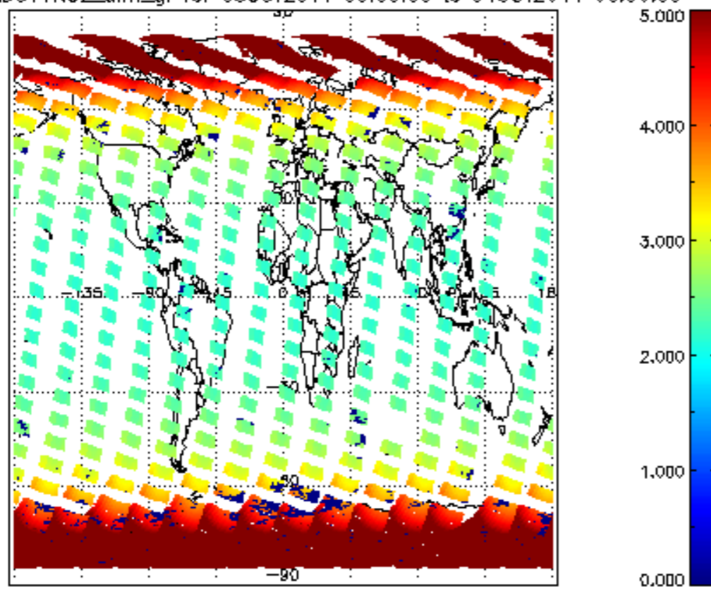
SCIOL2P_NADUV1NO2_amf_gr for 03OCT2011 00:00:00 to 04OCT2011 00:00:00
