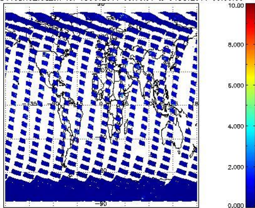
SCIOL2P_NADUV3BRO_vcd_err for 03OCT2011 00:00:00 to 04OCT2011 00:00:00
