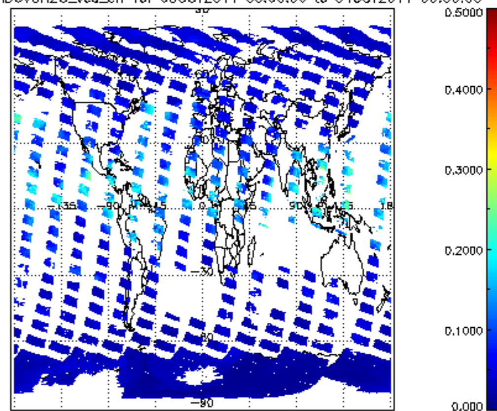
SCIOL2P_NADUV8H20_vcd_err for 03OCT2011 00:00:00 to 04OCT2011 00:00:00
