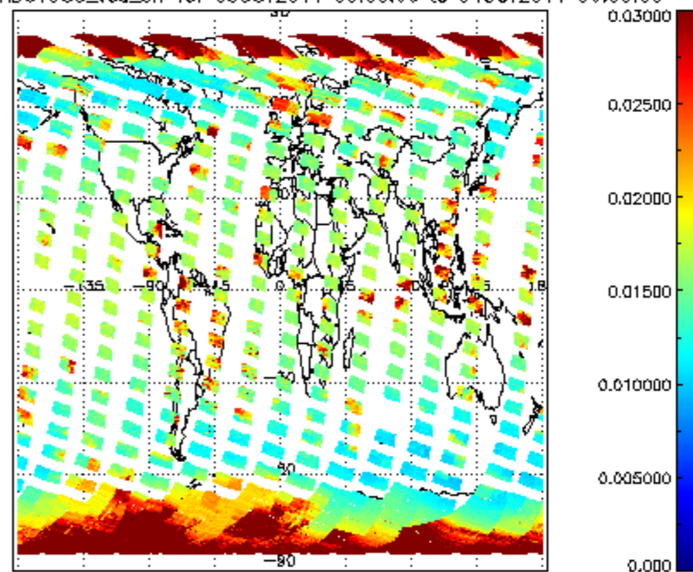
SCIOL2P_NADUV003_vcd_err for 03OCT2011 00:00:00 to 04OCT2011 00:00:00
