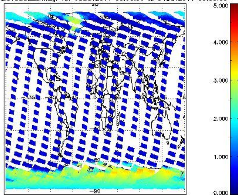
SCIOL2P_NADUV5SO2_amf_gr for 03OCT2011 00:00:00 to 04OCT2011 00:00:00
