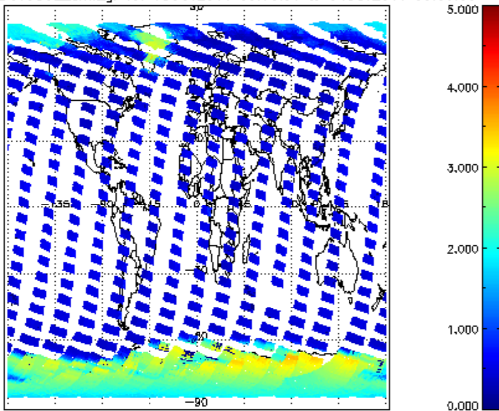
SCIOL2P_NADUV5S02_amf_gr for 03OCT2011 00:00:00 to 04OCT2011 00:00:00
