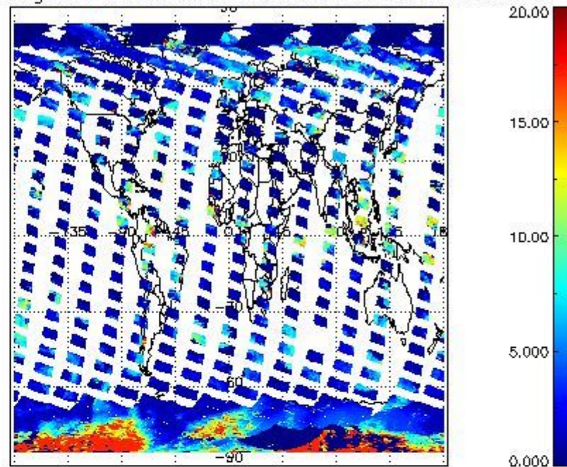
cL_top_height for 03OCT2011 00:00:00 to 04OCT2011 00:00:00
