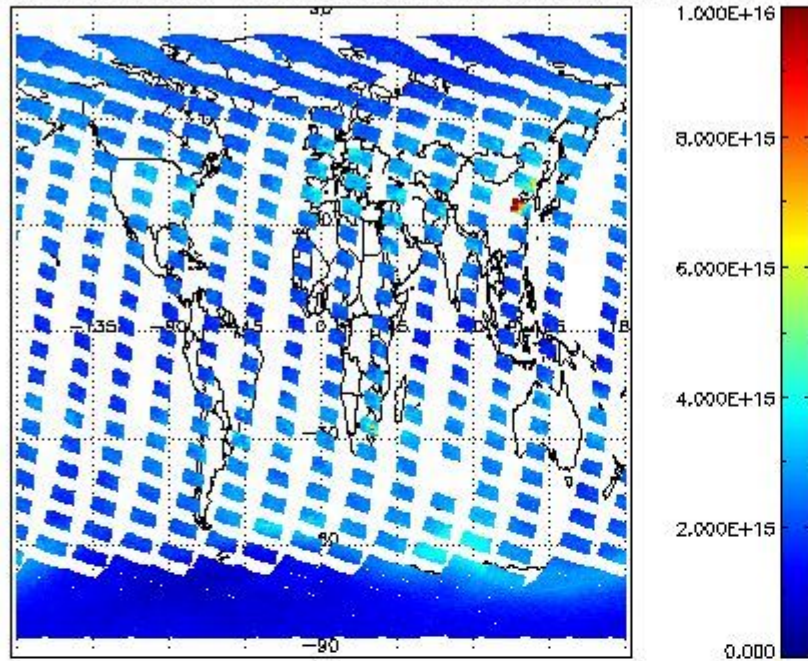
SCIOL2P_NADUV1NO2_vcd for 03OCT2011 00:00:00 to 04OCT2011 00:00:00
