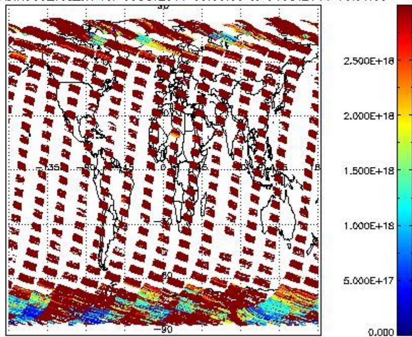
SCIOL2P_NADIR3CO_vcd_err for 03OCT2011 00:00:00 to 04OCT2011 00:00:00
