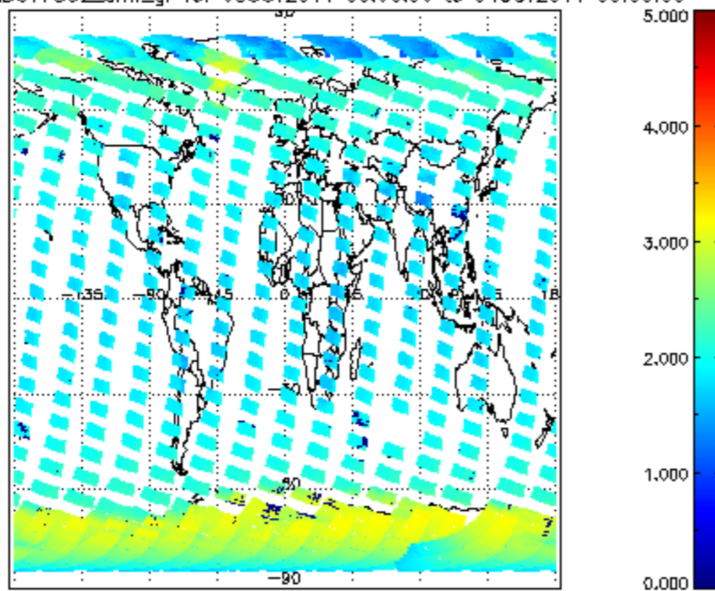
SCIOL2P_NADUV7S02_amf_gr for 03OCT2011 00:00:00 to 04OCT2011 00:00:00
