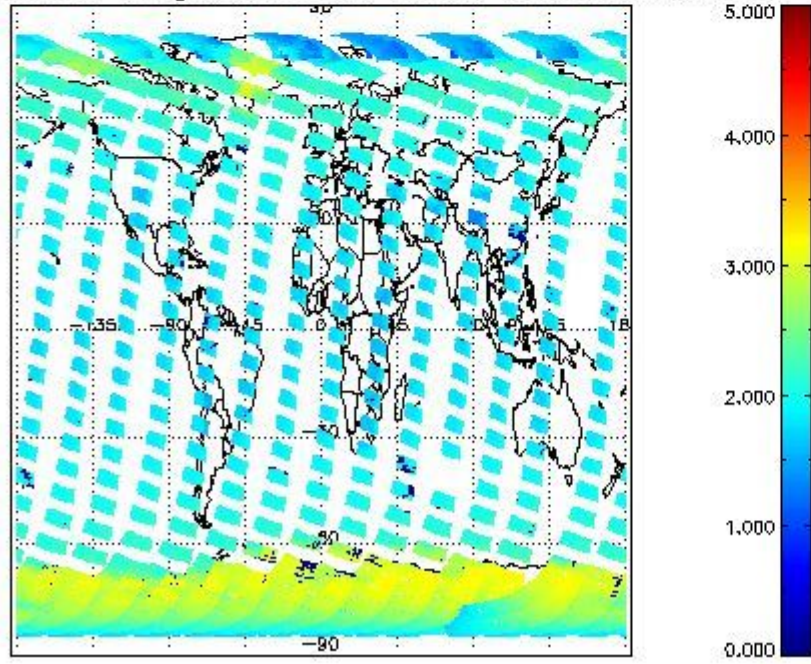
SCIOL2P_NADUV7S02_amf_gr for 03OCT2011 00:00:00 to 04OCT2011 00:00:00
