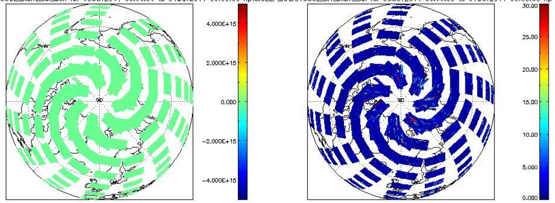
CIOL2P_NADUV60CL_slant_col_den for 03OCT2011 00:00:00 to 04OCT2011 00:00:00 np CIOL2P_NADUV60CL_err_slant_col for 03OCT2011 00:00:00 to 04OCT2011 00:00:00 np
