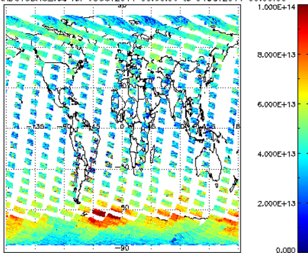
SCIOL2P_NADUV3BRO_vcd for 03OCT2011 00:00:00 to 04OCT2011 00:00:00
