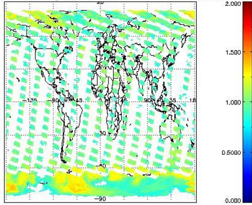
SCIOL2P_NADUV8H2O_amf_gr for 02OCT2011 00:00:00 to 03OCT2011 00:00:00
