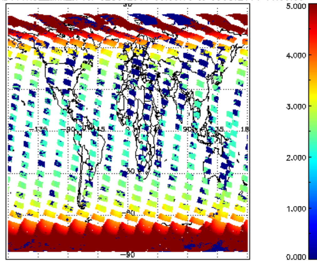
SCIOL2P_NADUV1N02_amf_cl for 02OCT2011 00:00:00 to 03OCT2011 00:00:00
