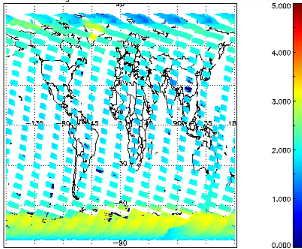
SCIOL2P_NADUV7S02_amf_gr for 02OCT2011 00:00:00 to 03OCT2011 00:00:00
