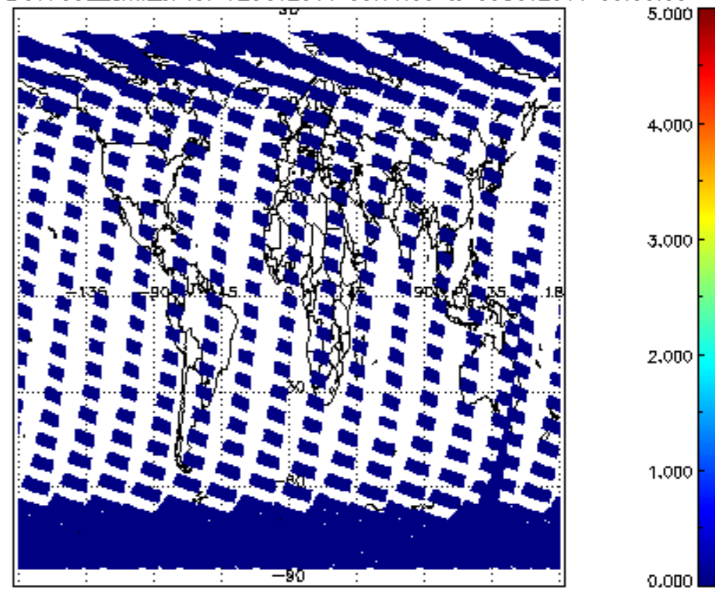
SCIOL2P_NADUV7S02_amf_sl for 02OCT2011 00:00:00 to 03OCT2011 00:00:00
