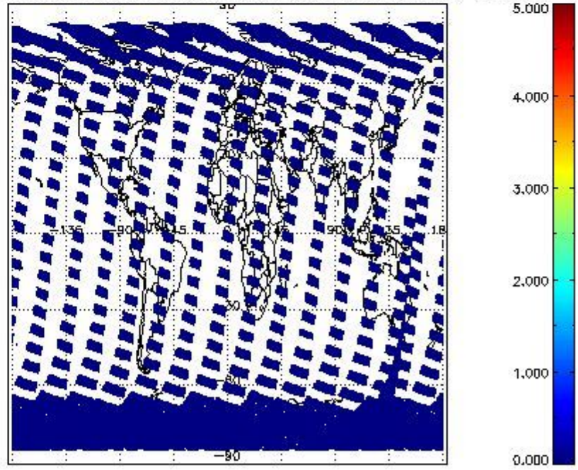
SCIOL2P_NADUV7S02_amf_cl for 02OCT2011 00:00:00 to 03OCT2011 00:00:00
