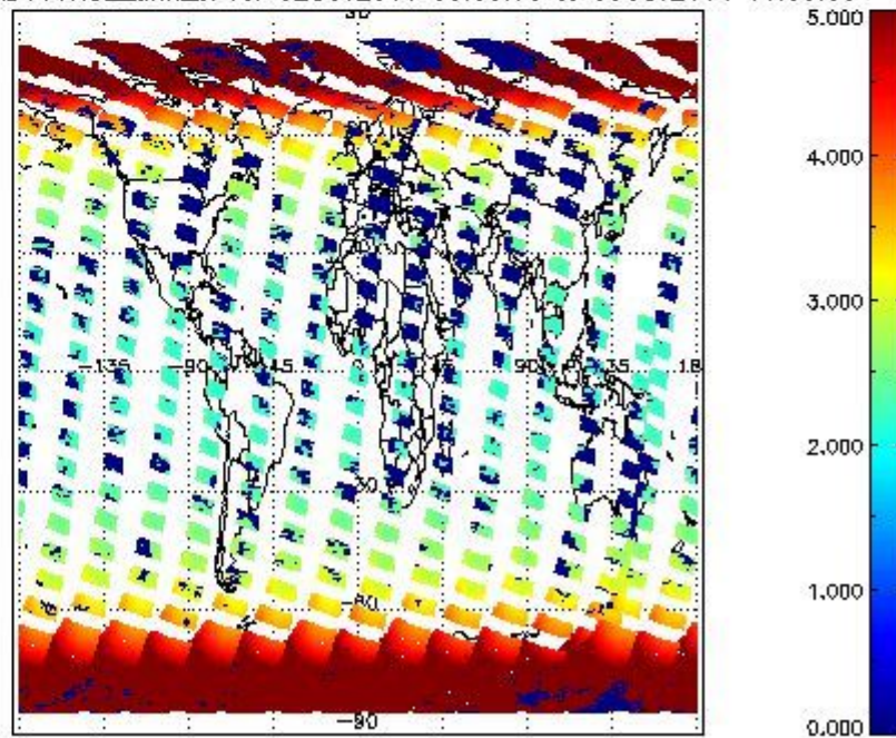
SCIOL2P_NADUV1NO2_amf_cl for 02OCT2011 00:00:00 to 03OCT2011 00:00:00
