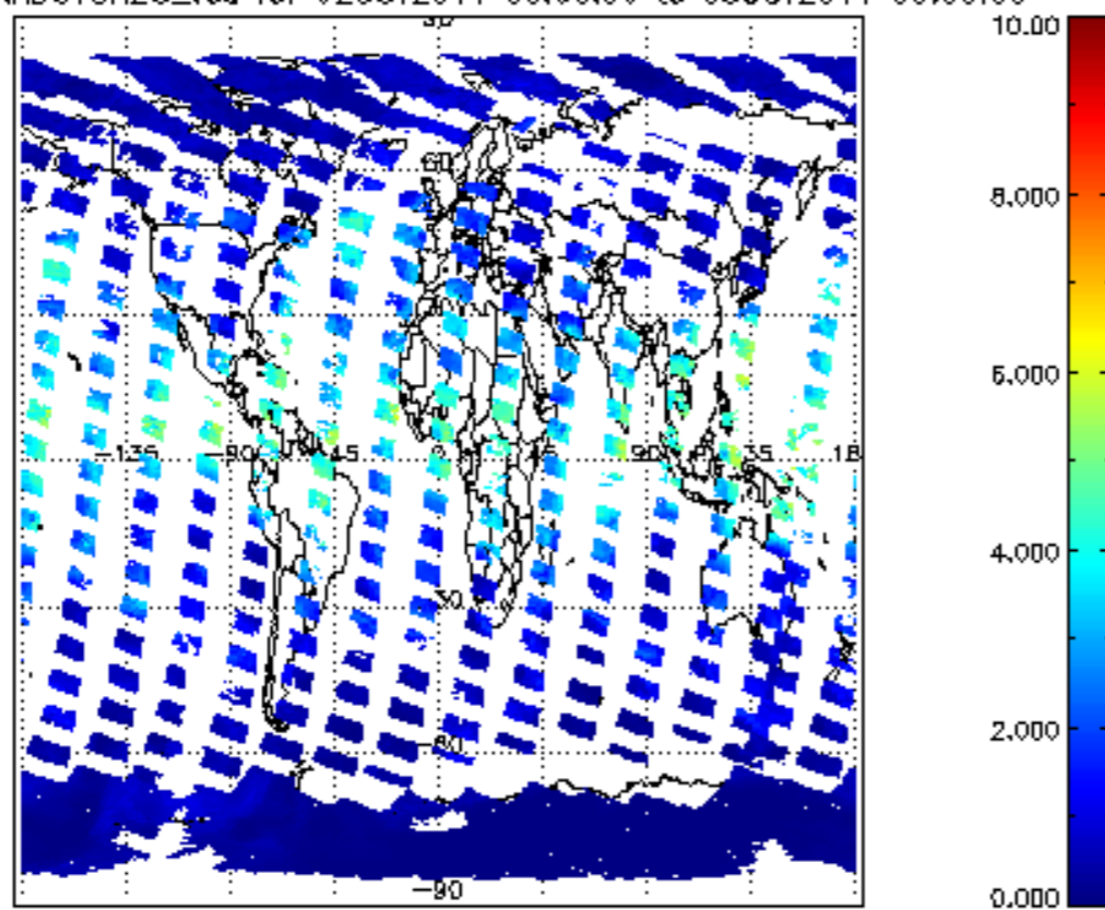
SCIOL2P_NADUV8H20_vcd for 02OCT2011 00:00:00 to 03OCT2011 00:00:00
