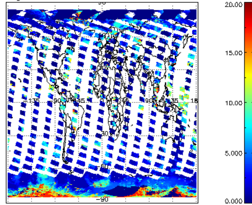
cl_top_height for 02OCT2011 00:00:00 to 03OCT2011 00:00:00
