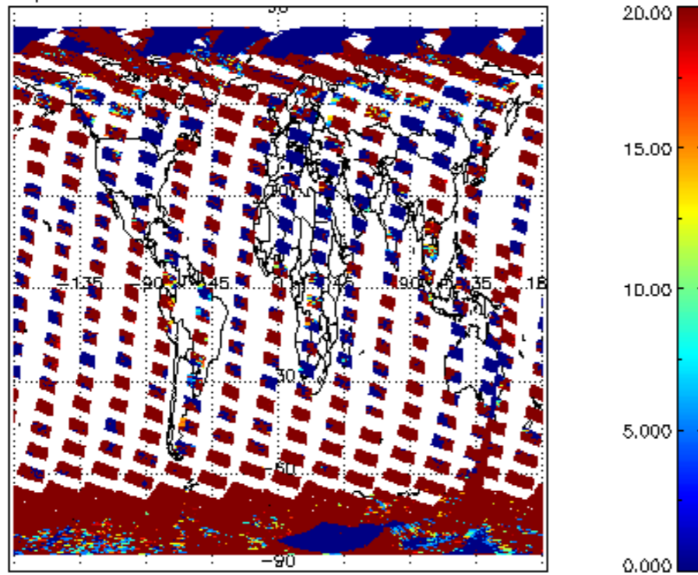
cl_opt_depth for 02OCT2011 00:00:00 to 03OCT2011 00:00:00
