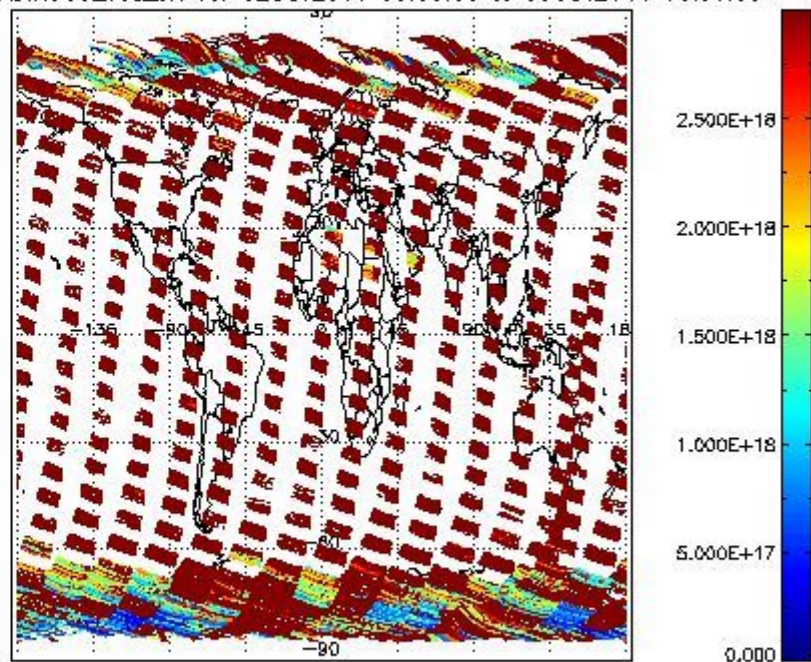
SCIOL2P_NADIR3CO_vcd_err for 02OCT2011 00:00:00 to 03OCT2011 00:00:00
