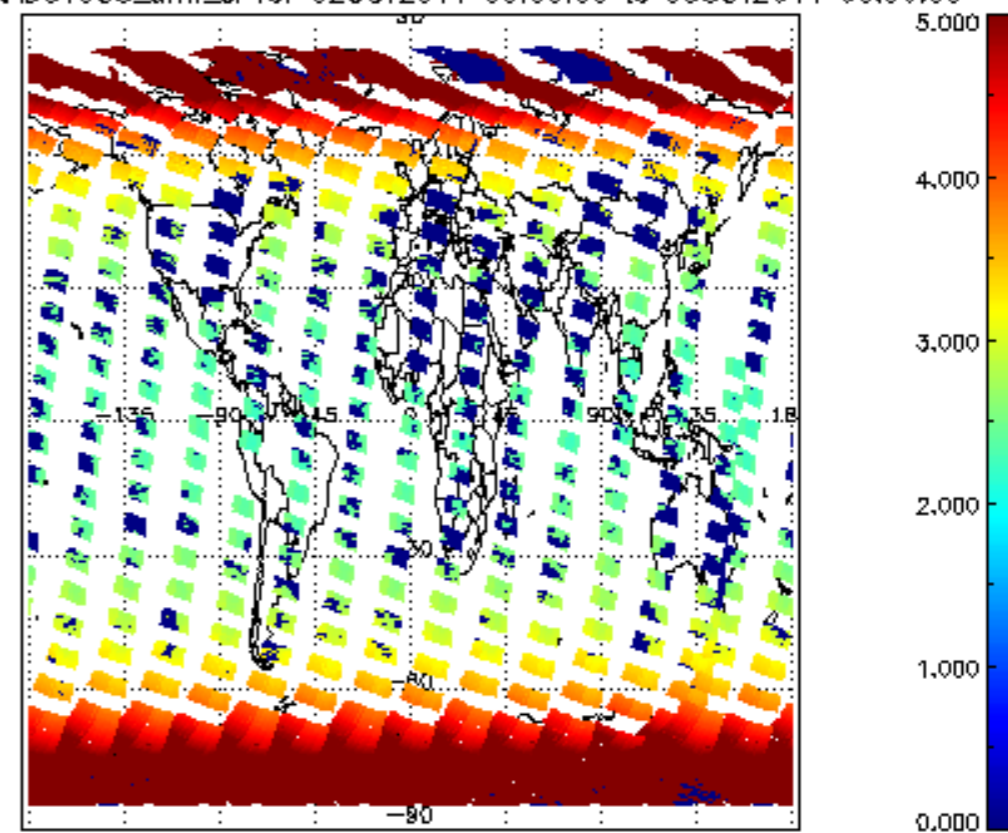
SCIOL2P_NADUV003_amf_cl for 02OCT2011 00:00:00 to 03OCT2011 00:00:00
