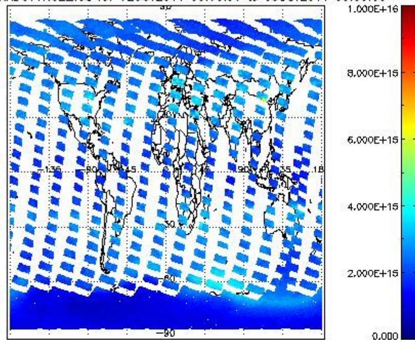
SCIOL2P_NADUV1NO2_vcd for 02OCT2011 00:00:00 to 03OCT2011 00:00:00
