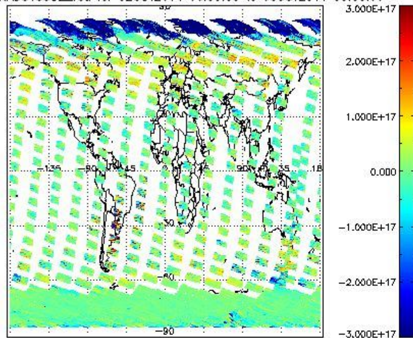
SCIOL2P_NADUV5SO2_vcd for 02OCT2011 00:00:00 to 03OCT2011 00:00:00
