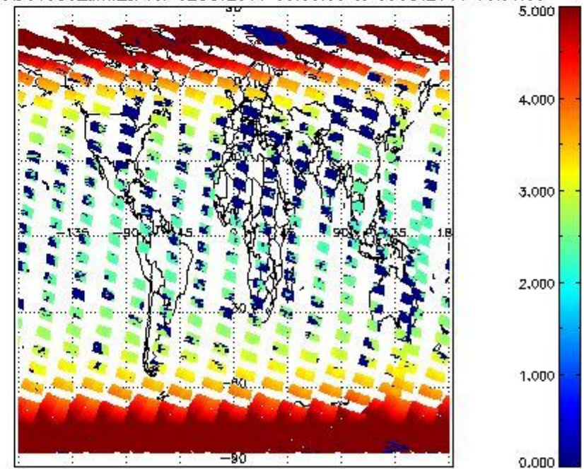
SCIOL2P_NADUV003_amf_cl for 02OCT2011 00:00:00 to 03OCT2011 00:00:00
