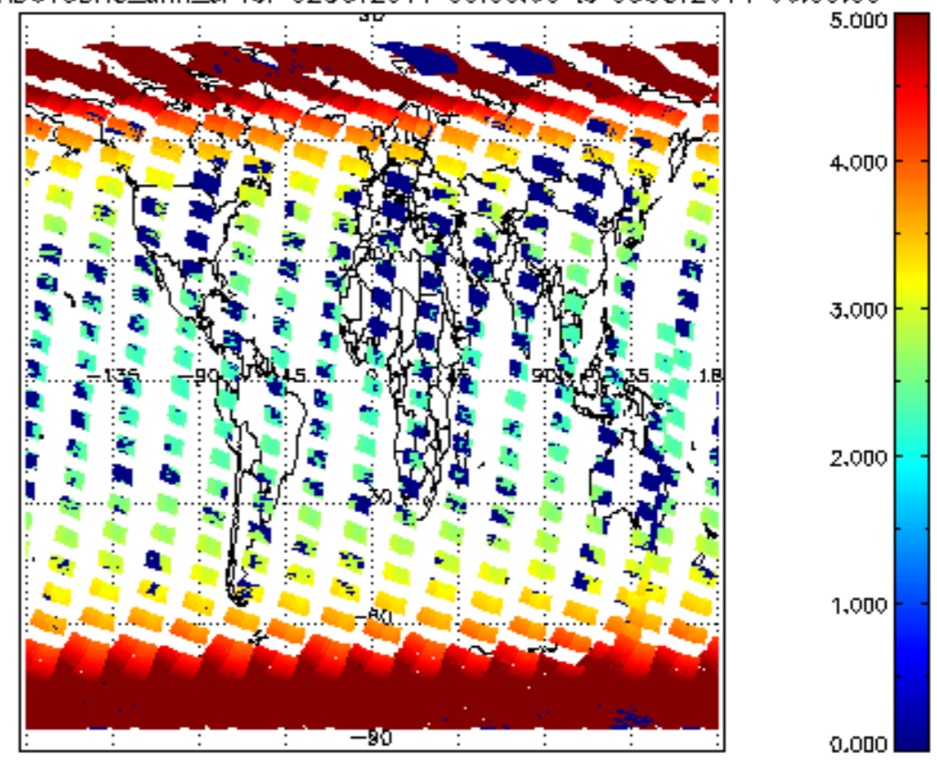
SCIOL2P_NADUV3BRO_amf_cl for 02OCT2011 00:00:00 to 03OCT2011 00:00:00
