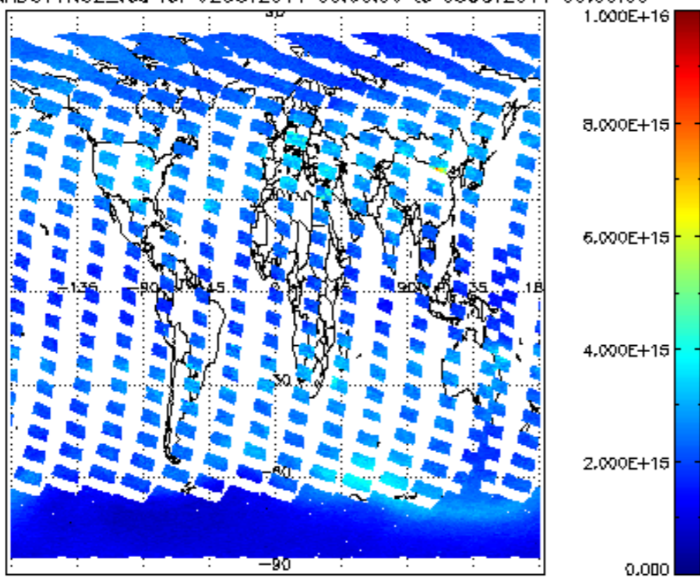
SCIOL2P_NADUV1N02_vcd for 02OCT2011 00:00:00 to 03OCT2011 00:00:00
