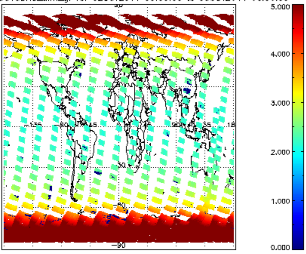
SCIOL2P_NADUV3BRO_amf_gr for 02OCT2011 00:00:00 to 03OCT2011 00:00:00
