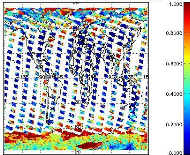
cLfrac for 02OCT2011 00:00:00 to 03OCT2011 00:00:00
