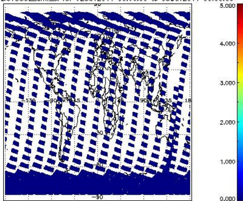
SCIOL2P_NADUV5SO2_amf_cl for 02OCT2011 00:00:00 to 03OCT2011 00:00:00
