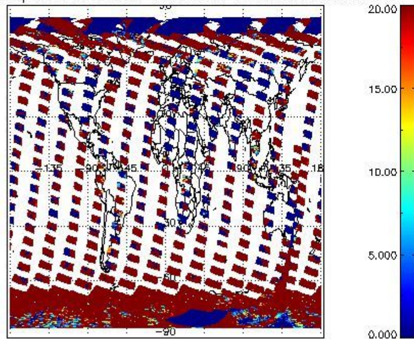
cL_opt_depth for 02OCT2011 00:00:00 to 03OCT2011 00:00:00
