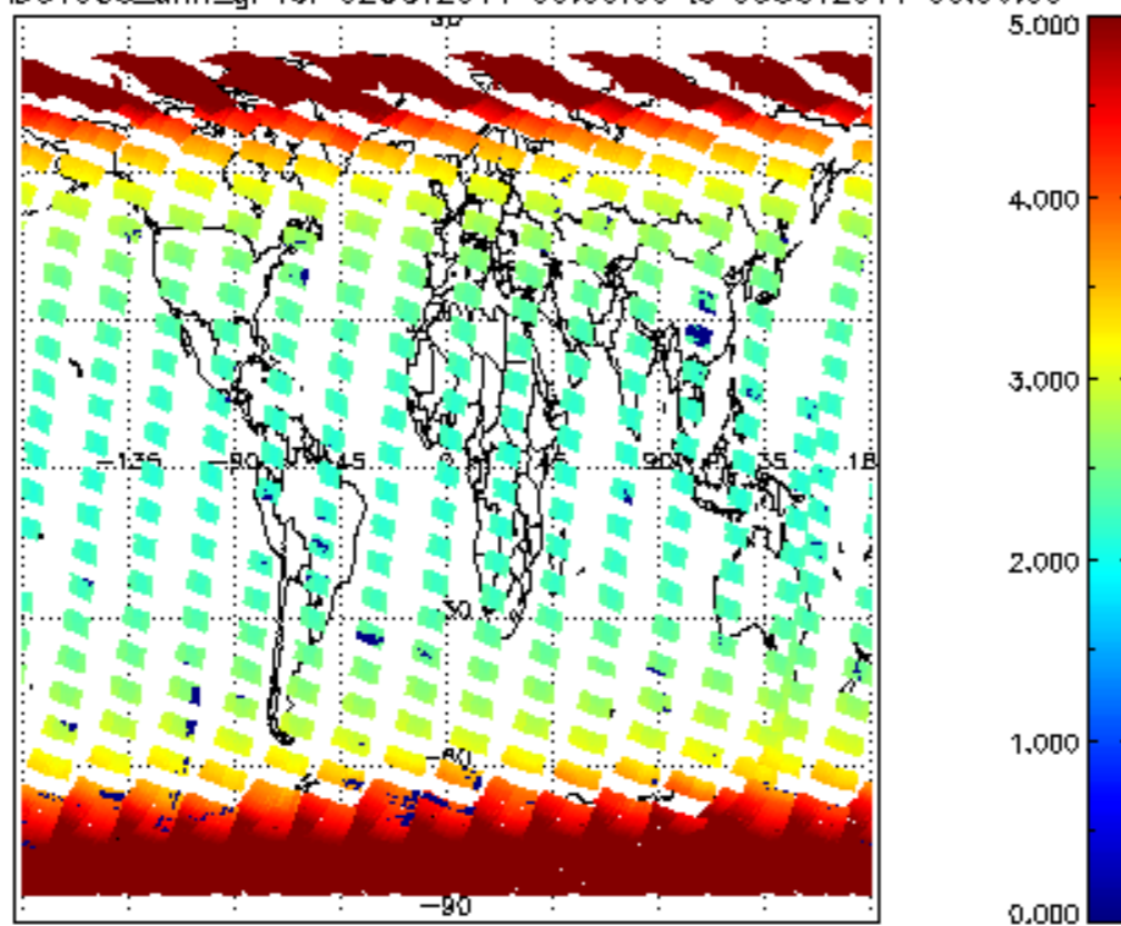
SCIOL2P_NADUV003_amf_gr for 02OCT2011 00:00:00 to 03OCT2011 00:00:00
