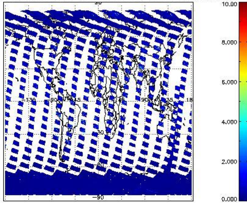
SCIOL2P_NADUV3BRO_vcd_err for 02OCT2011 00:00:00 to 03OCT2011 00:00:00
