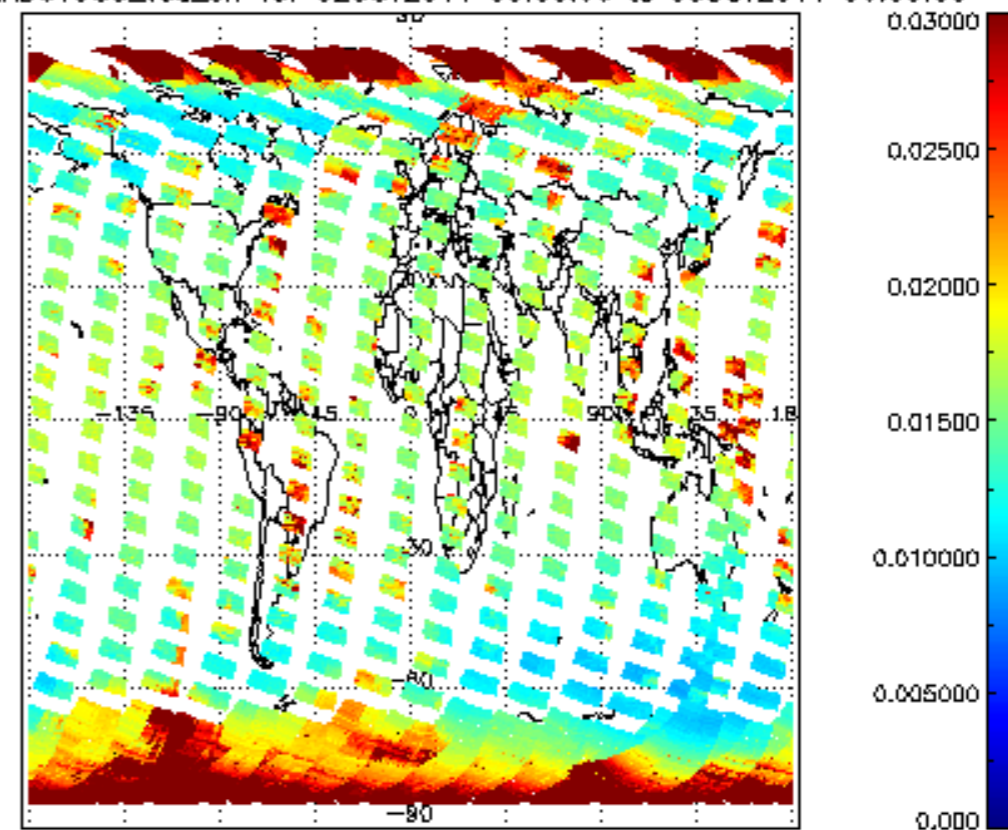
SCIOL2P_NADUV003_vcd_err for 02OCT2011 00:00:00 to 03OCT2011 00:00:00
