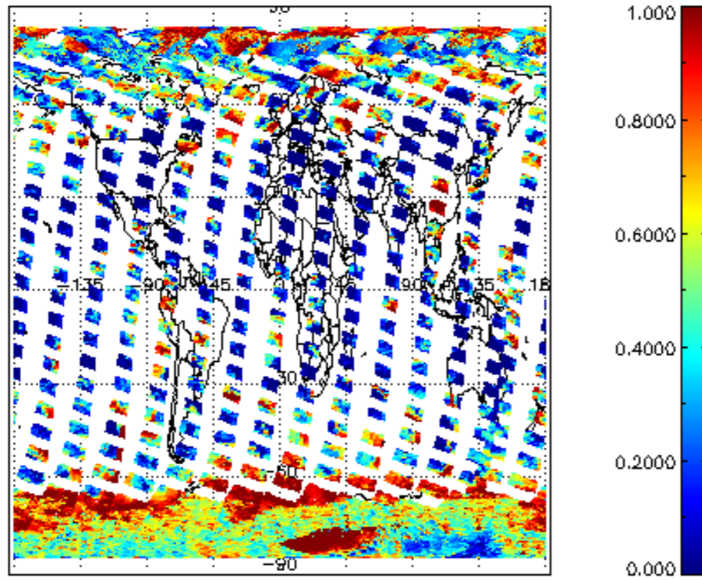
cl_frac for 02OCT2011 00:00:00 to 03OCT2011 00:00:00
