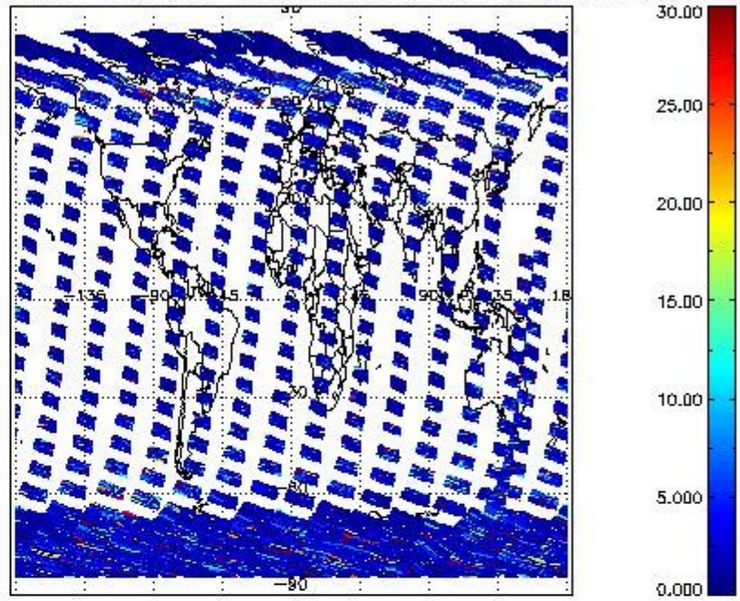
SCIOL2P_NADUV7S02_vcd_err for 02OCT2011 00:00:00 to 03OCT2011 00:00:00
