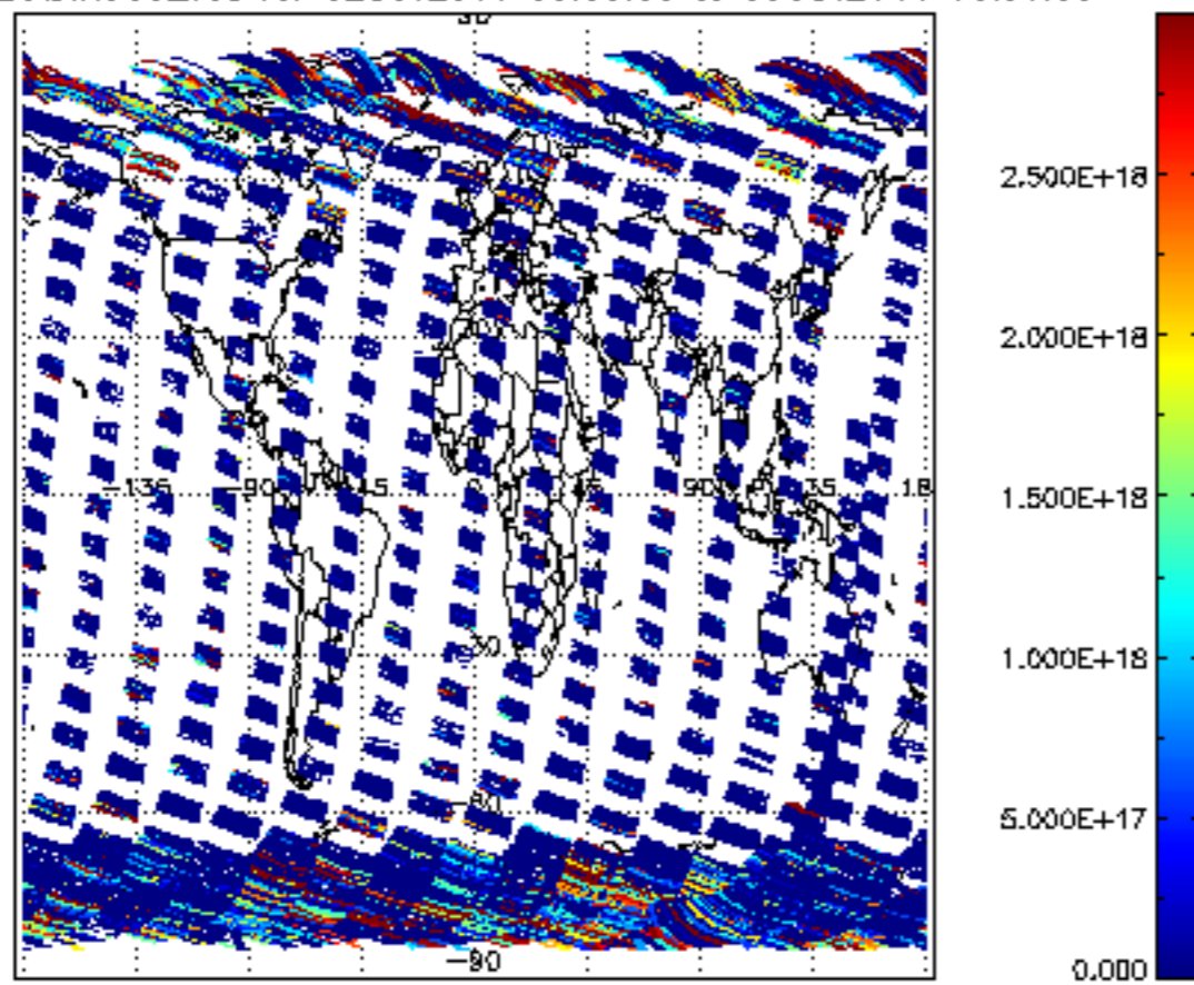
SCIOL2P_NADIR3CO_vcd for 02OCT2011 00:00:00 to 03OCT2011 00:00:00
