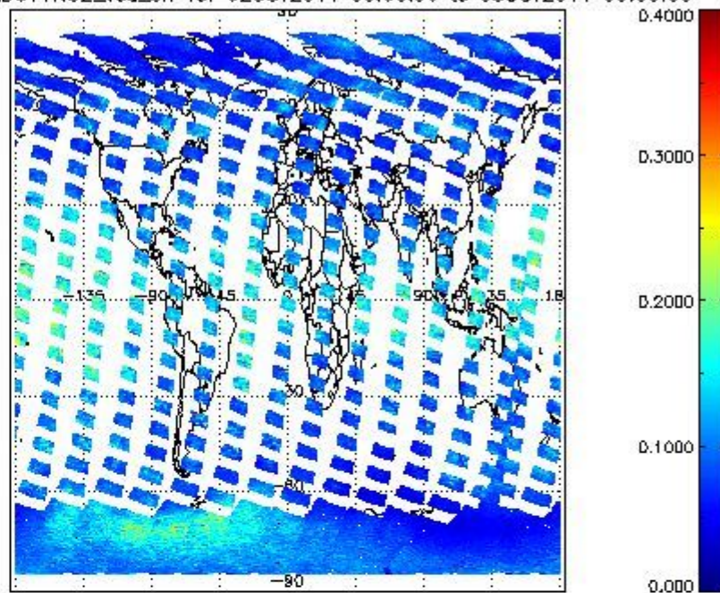
SCIOL2P_NADUV1NO2_vcd_err for 02OCT2011 00:00:00 to 03OCT2011 00:00:00
