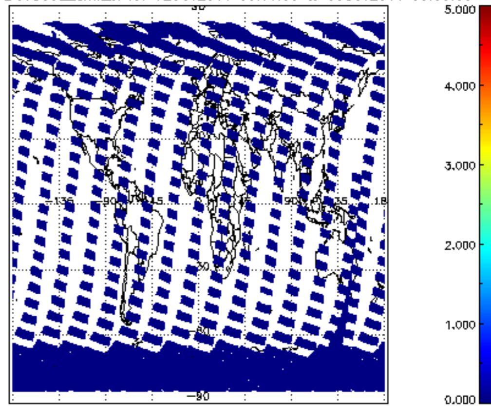
SCIOL2P_NADUV5S02_amf_cl for 02OCT2011 00:00:00 to 03OCT2011 00:00:00
