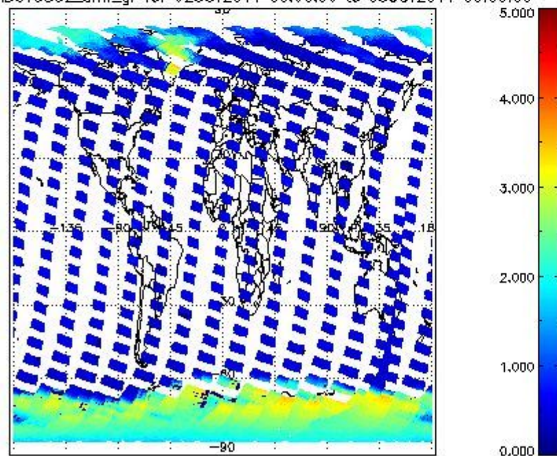
SCIOL2P_NADUV5SO2_amf_gr for 02OCT2011 00:00:00 to 03OCT2011 00:00:00
