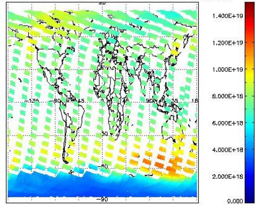
SCIOL2P_NADUV003_vcd for 02OCT2011 00:00:00 to 03OCT2011 00:00:00
