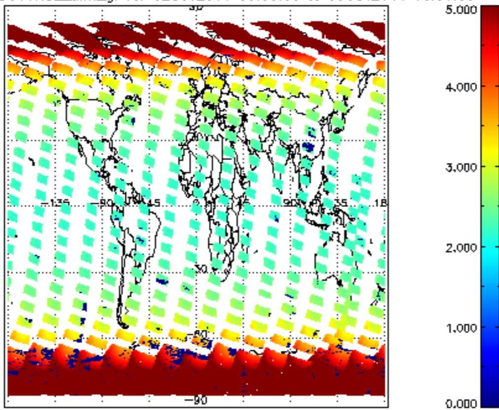
SCIOL2P_NADUV1N02_amf_gr for 02OCT2011 00:00:00 to 03OCT2011 00:00:00
