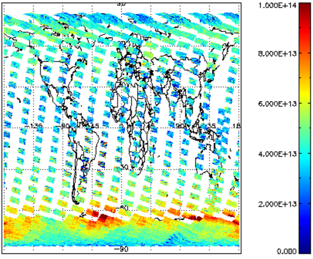
SCIOL2P_NADUV3BRO_vcd for 02OCT2011 00:00:00 to 03OCT2011 00:00:00
