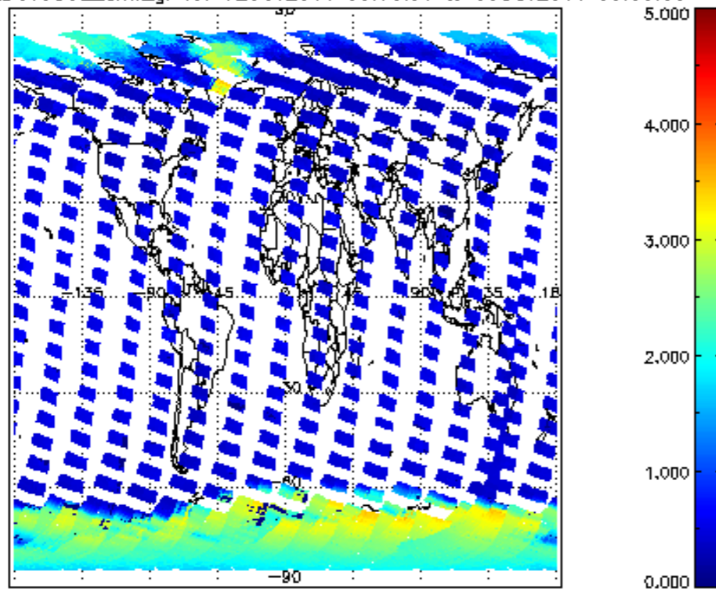
SCIOL2P_NADUV5S02_amf_gr for 02OCT2011 00:00:00 to 03OCT2011 00:00:00
