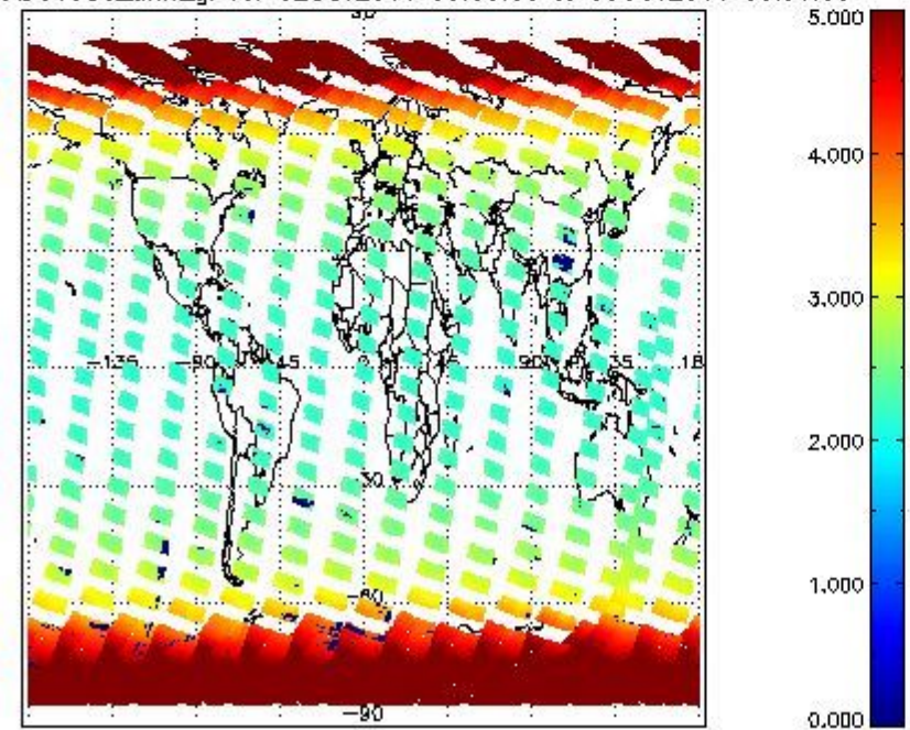
SCIOL2P_NADUV003_amf_gr for 02OCT2011 00:00:00 to 03OCT2011 00:00:00
