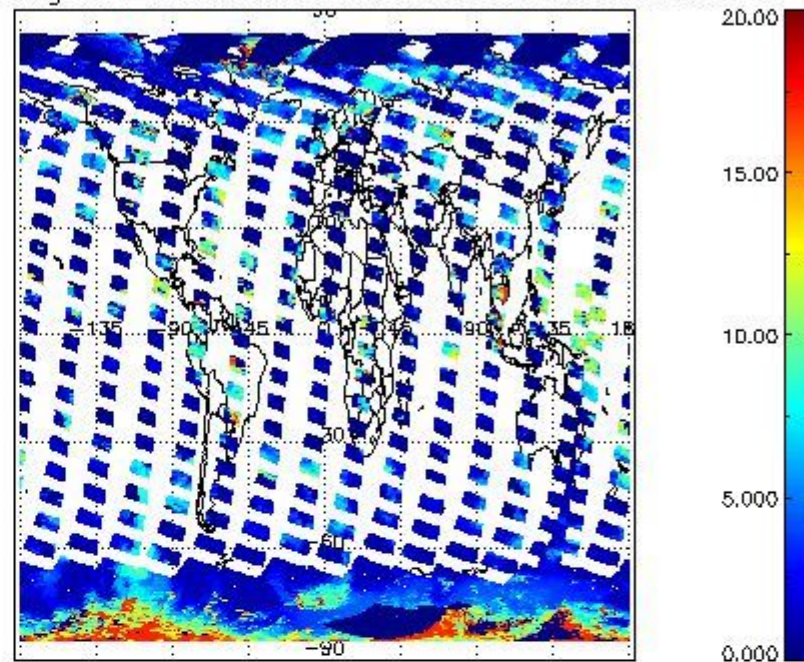
cL_top_height for 02OCT2011 00:00:00 to 03OCT2011 00:00:00
