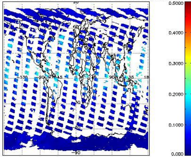
SCIOL2P_NADUV8H2O_vcd_err for 02OCT2011 00:00:00 to 03OCT2011 00:00:00
