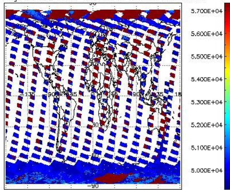
cloud_flags for 02OCT2011 00:00:00 to 03OCT2011 00:00:00
