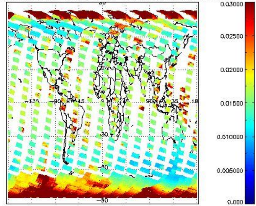
SCIOL2P_NADUV003_vcd_err for 02OCT2011 00:00:00 to 03OCT2011 00:00:00
