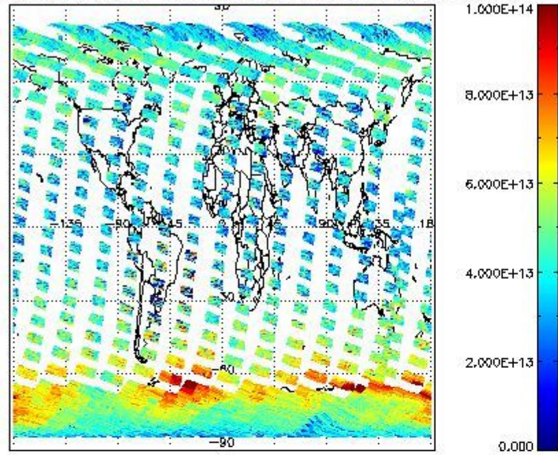
SCIOL2P_NADUV3BRO_vcd for 02OCT2011 00:00:00 to 03OCT2011 00:00:00
