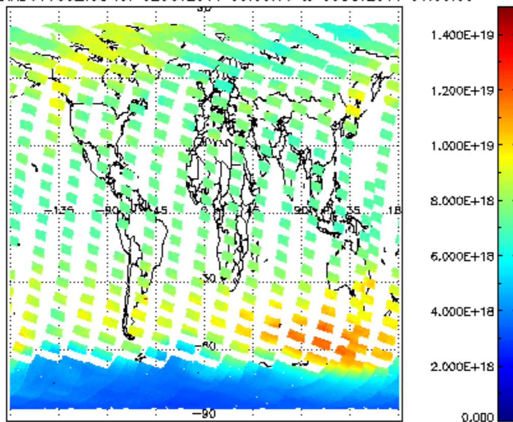
SCIOL2P_NADUV003_vcd for 02OCT2011 00:00:00 to 03OCT2011 00:00:00
