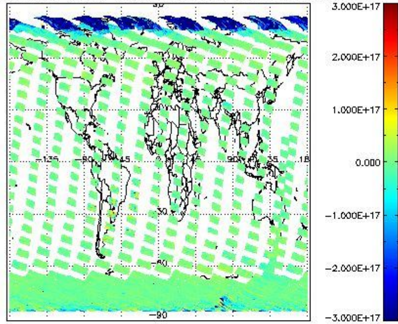
SCIOL2P_NADUV7S02_vcd for 02OCT2011 00:00:00 to 03OCT2011 00:00:00
