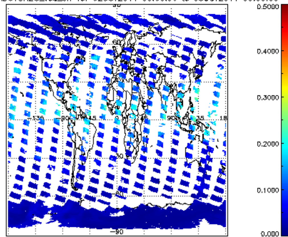
SCIOL2P_NADUV8H20_vcd_err for 02OCT2011 00:00:00 to 03OCT2011 00:00:00
