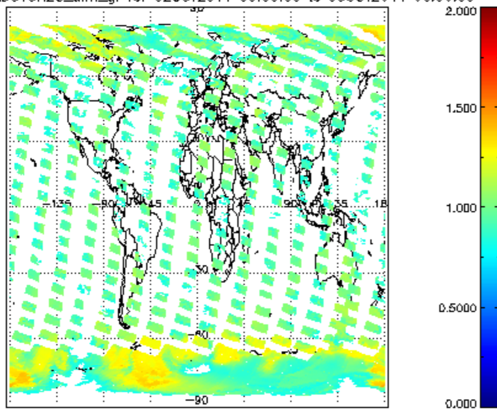
SCIOL2P_NADUV8H20_amf_gr for 02OCT2011 00:00:00 to 03OCT2011 00:00:00
