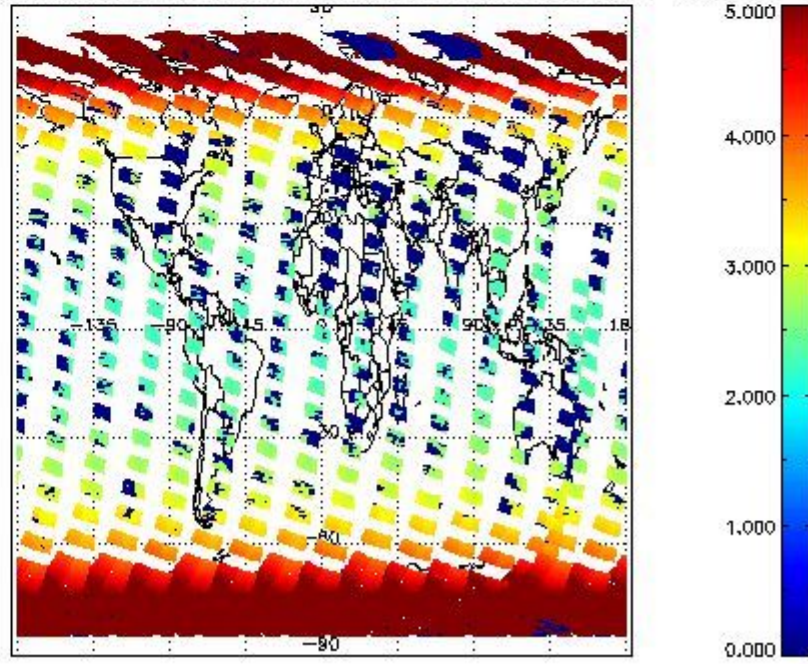
SCIOL2P_NADUV3BRO_amf_cl for 02OCT2011 00:00:00 to 03OCT2011 00:00:00
