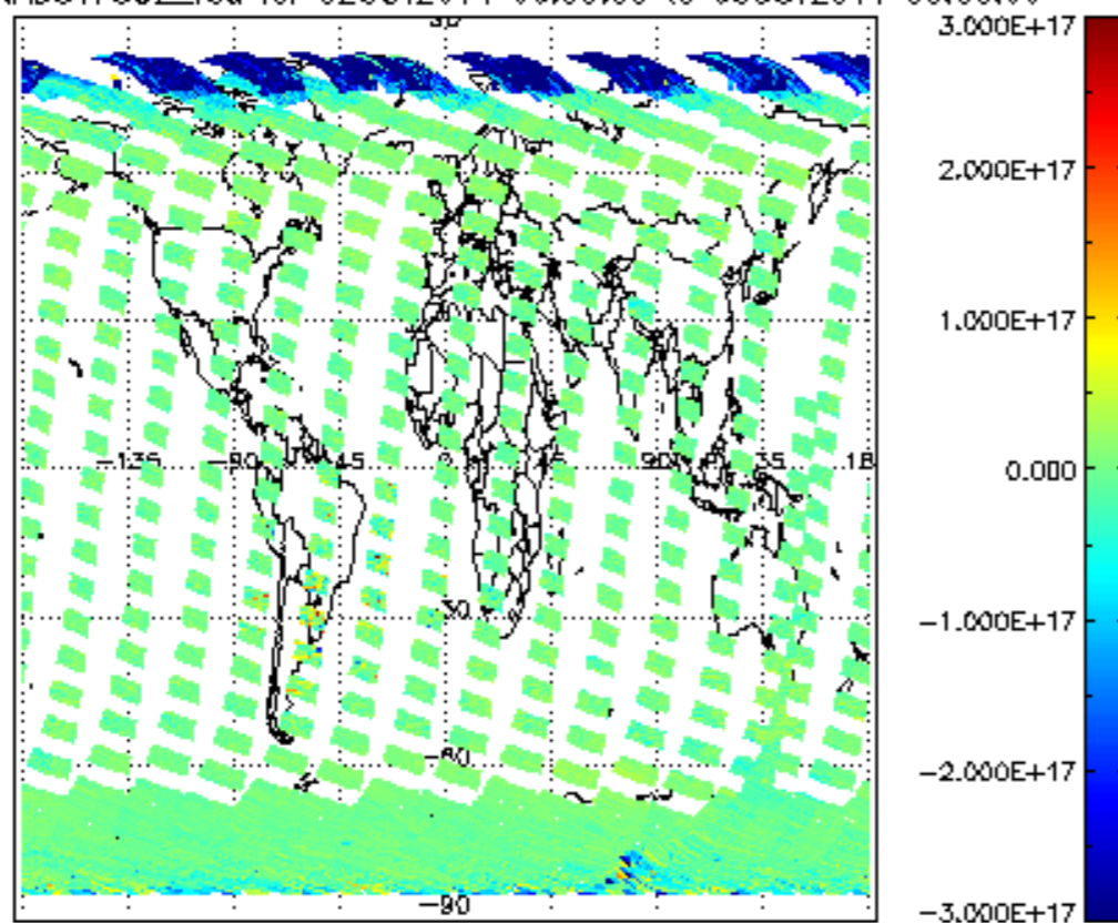
SCIOL2P_NADUV7S02_vcd for 02OCT2011 00:00:00 to 03OCT2011 00:00:00
