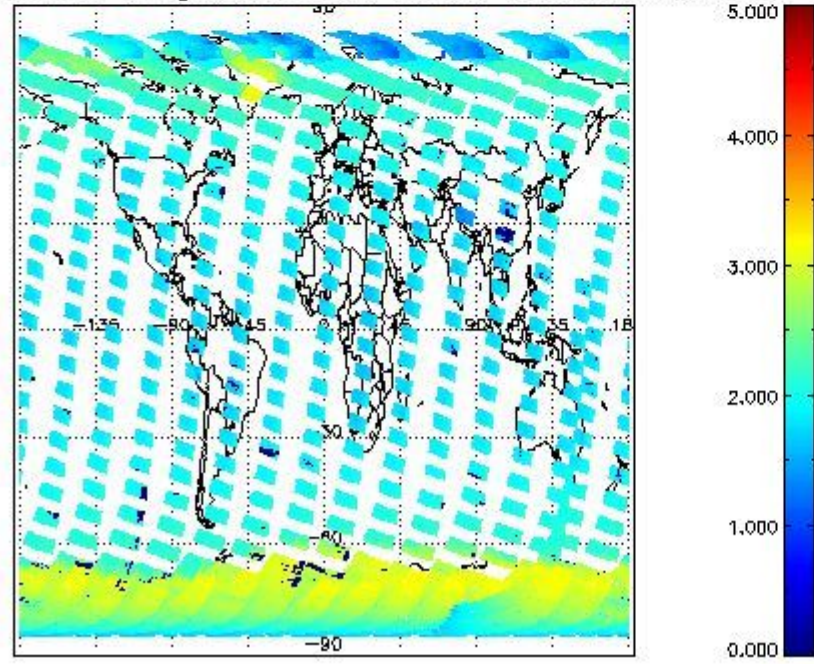
SCIOL2P_NADUV7S02_amf_gr for 02OCT2011 00:00:00 to 03OCT2011 00:00:00
