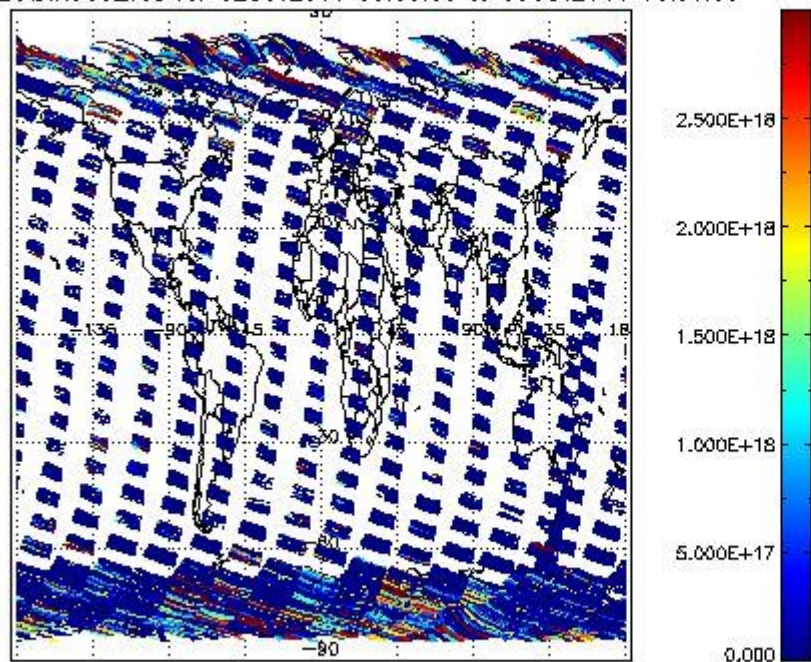
SCIOL2P_NADIR3CO_vcd for 02OCT2011 00:00:00 to 03OCT2011 00:00:00
