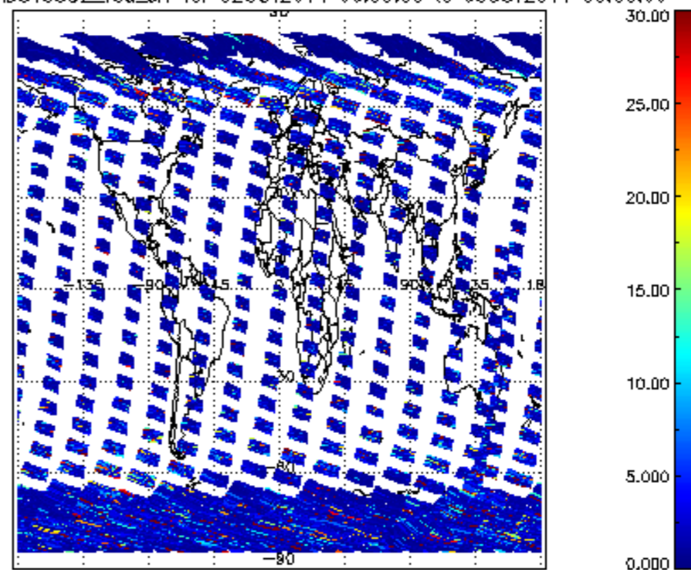
SCIOL2P_NADUV5S02_vcd_err for 02OCT2011 00:00:00 to 03OCT2011 00:00:00
