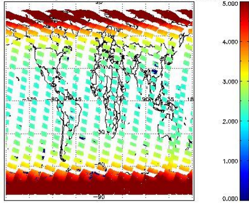
SCIOL2P_NADUV3BRO_amf_gr for 02OCT2011 00:00:00 to 03OCT2011 00:00:00
