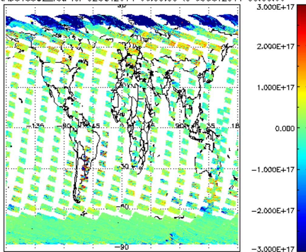
SCIOL2P_NADUV5S02_vcd for 02OCT2011 00:00:00 to 03OCT2011 00:00:00
