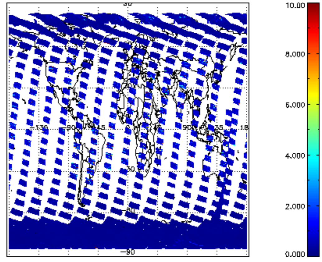
SCIOL2P_NADUV3BRO_vcd_err for 02OCT2011 00:00:00 to 03OCT2011 00:00:00
