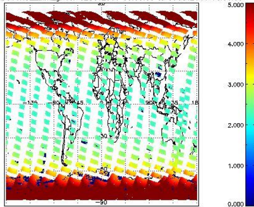
SCIOL2P_NADUV1NO2_amf_gr for 02OCT2011 00:00:00 to 03OCT2011 00:00:00
