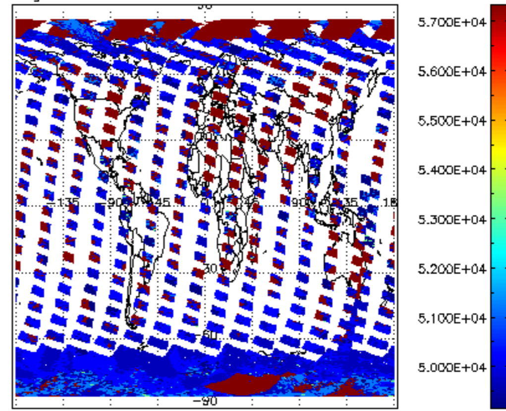
cloud_flags for 02OCT2011 00:00:00 to 03OCT2011 00:00:00
