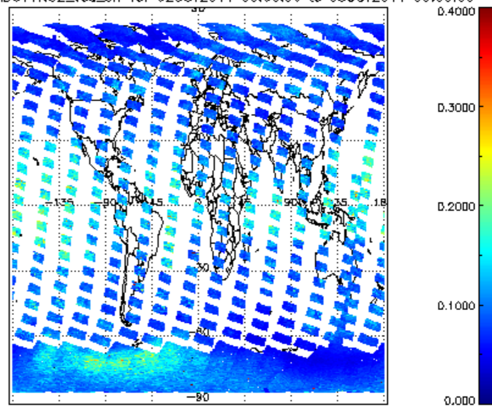
SCIOL2P_NADUV1N02_vcd_err for 02OCT2011 00:00:00 to 03OCT2011 00:00:00
