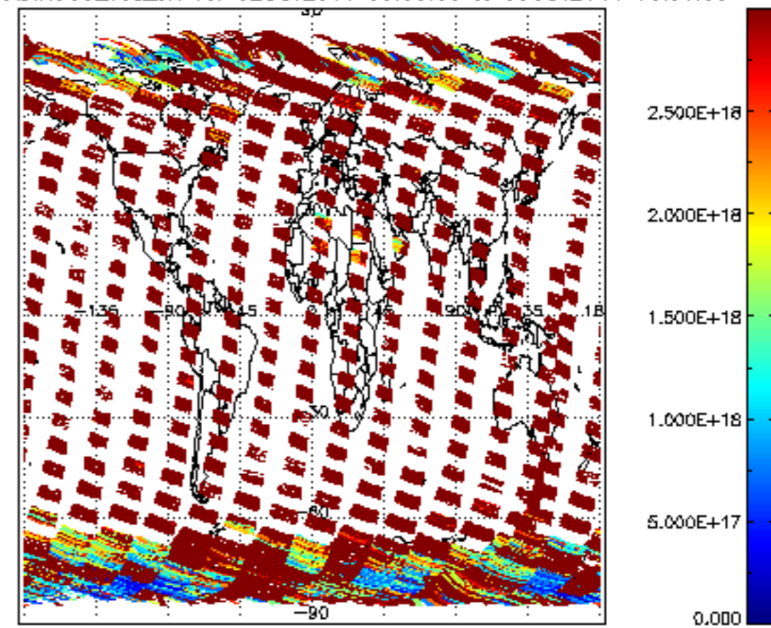
SCIOL2P_NADIR3CO_vcd_err for 02OCT2011 00:00:00 to 03OCT2011 00:00:00
