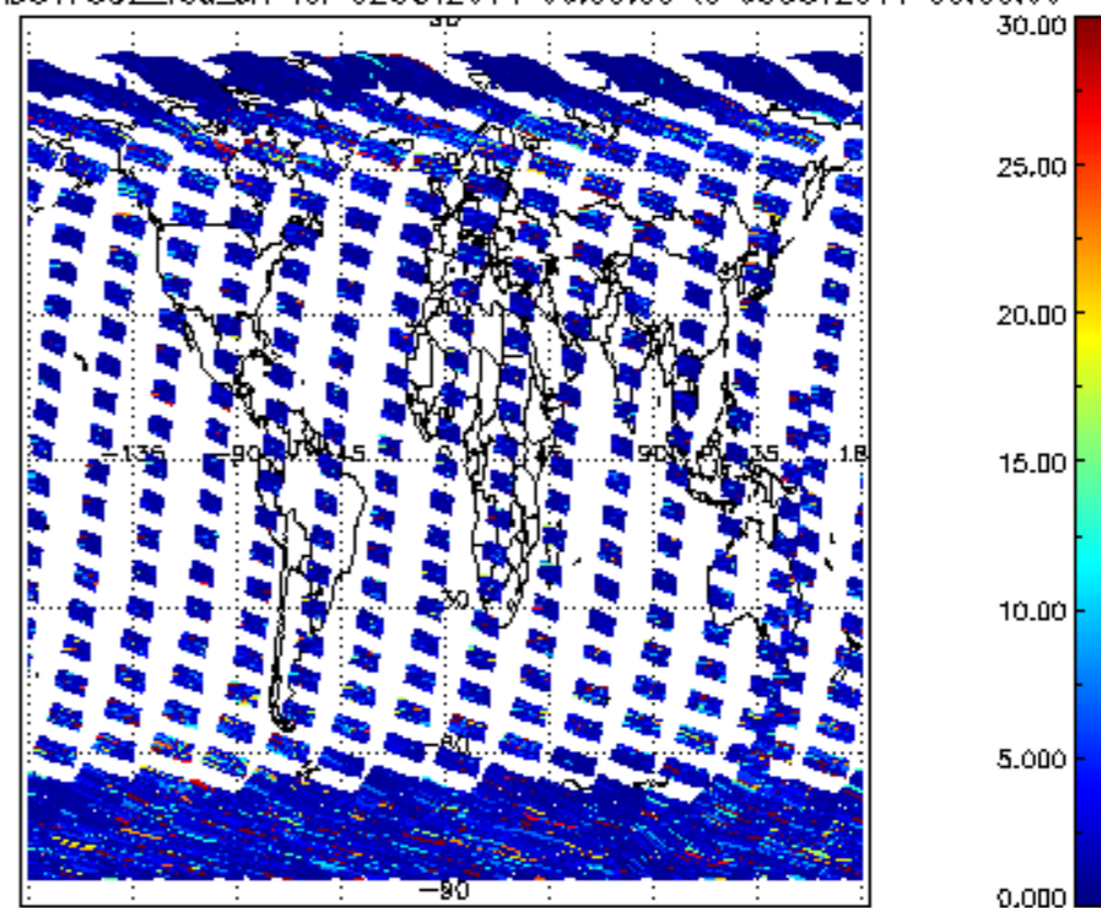
SCIOL2P_NADUV7S02_vcd_err for 02OCT2011 00:00:00 to 03OCT2011 00:00:00
