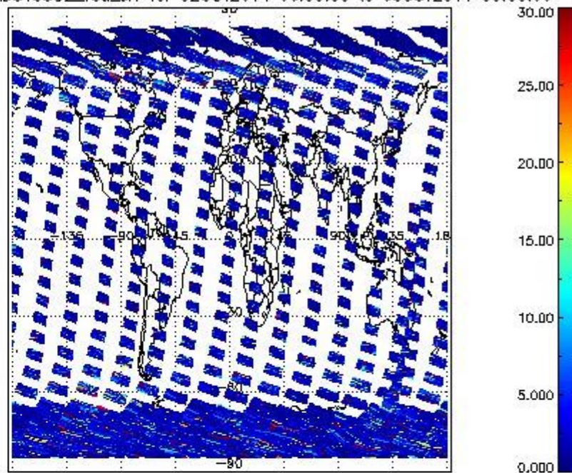
SCIOL2P_NADUV5SO2_vcd_err for 02OCT2011 00:00:00 to 03OCT2011 00:00:00
