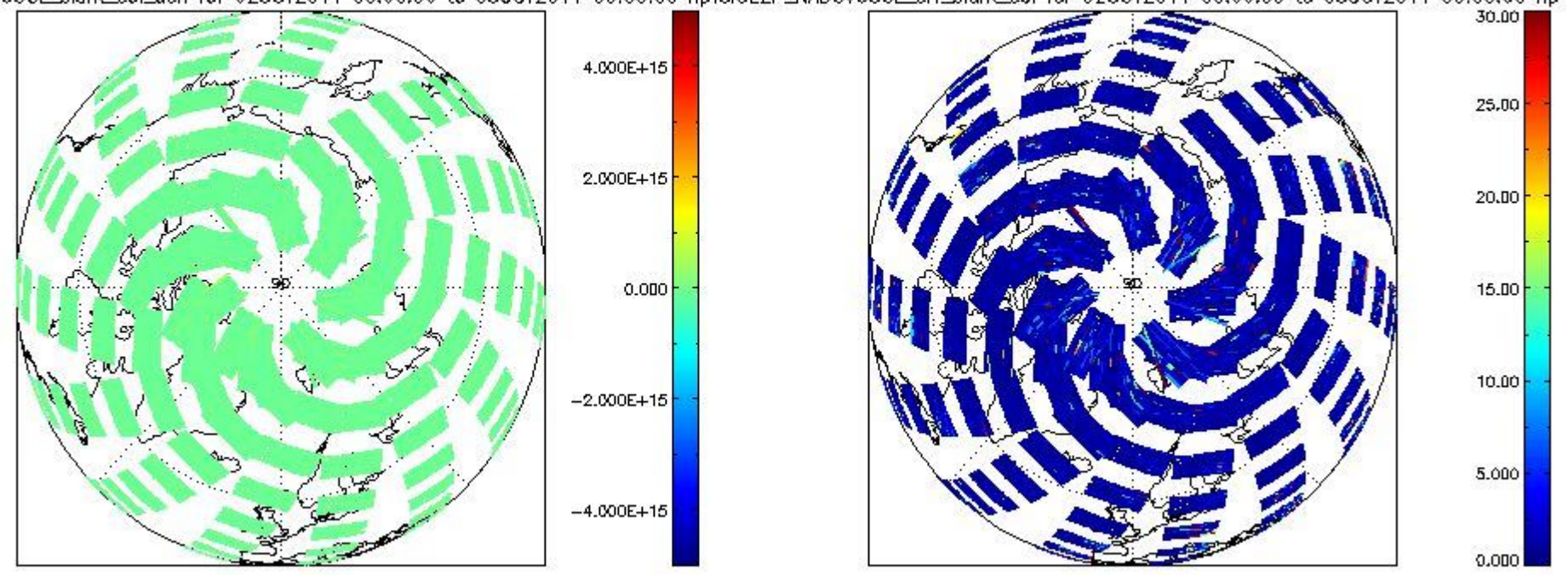
CIOL2P_NADUV60CL_slant_col_den for 02OCT2011 00:00:00 to 03OCT2011 00:00:00 np CIOL2P_NADUV60CL_err_slant_col for 02OCT2011 00:00:00 to 03OCT2011 00:00:00 np
