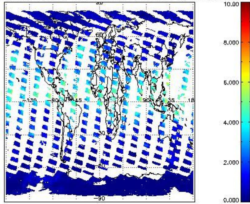
SCIOL2P_NADUV8H2O_vcd for 02OCT2011 00:00:00 to 03OCT2011 00:00:00
