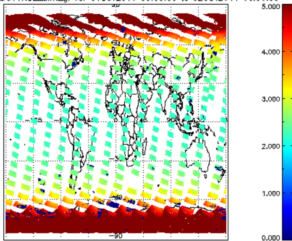
SCIOL2P_NADUV1NO2_amf_gr for 01OCT2011 00:00:00 to 02OCT2011 00:00:00
