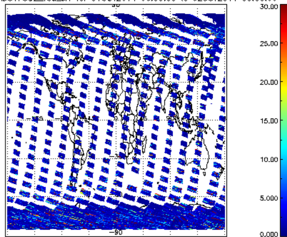
SCIOL2P_NADUV7S02_vcd_err for 01OCT2011 00:00:00 to 02OCT2011 00:00:00
