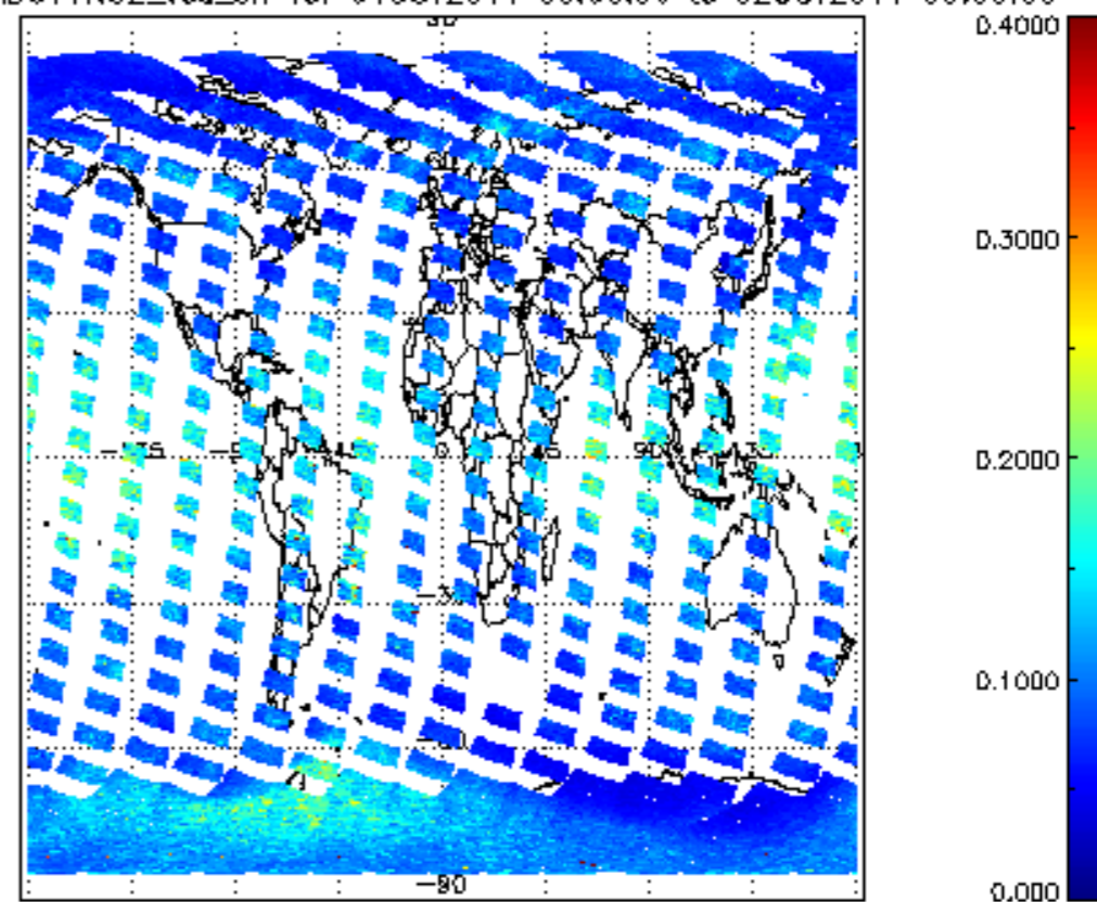
SCIOL2P_NADUV1NO2_vcd_err for 01OCT2011 00:00:00 to 02OCT2011 00:00:00
