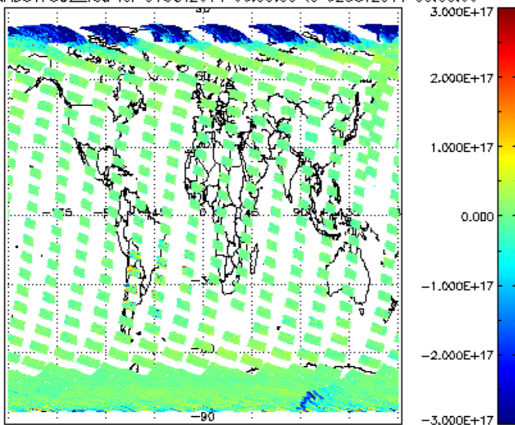
SCIOL2P_NADUV7S02_vcd for 01OCT2011 00:00:00 to 02OCT2011 00:00:00
