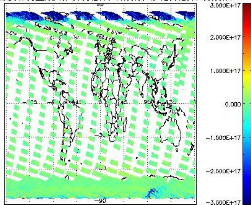
SCIOL2P_NADUV7S02_vcd for 01OCT2011 00:00:00 to 02OCT2011 00:00:00
