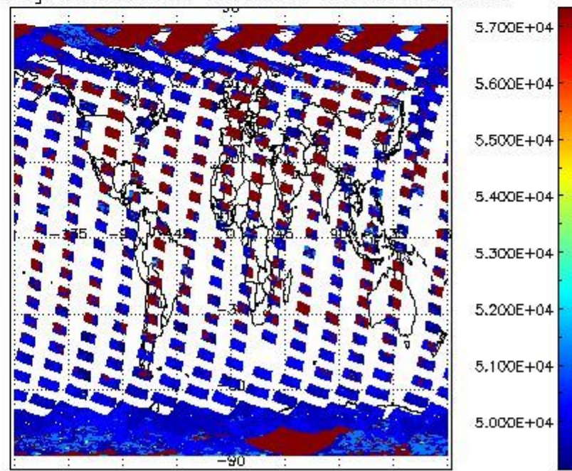
cloud_flags for 01OCT2011 00:00:00 to 02OCT2011 00:00:00
