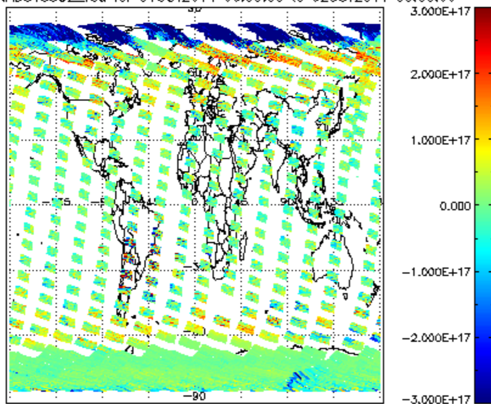
SCIOL2P_NADUV5S02_vcd for 01OCT2011 00:00:00 to 02OCT2011 00:00:00
