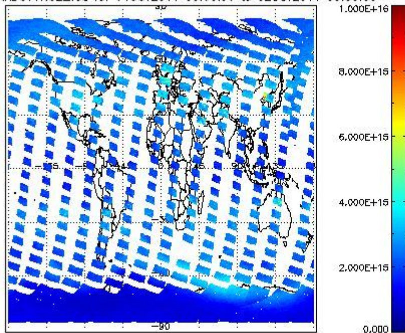
SCIOL2P_NADUV1NO2_vcd for 01OCT2011 00:00:00 to 02OCT2011 00:00:00
