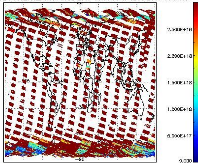
SCIDL2P_NADIR3CO_vcd_err for 01OCT2011 00:00:00 to 02OCT2011 00:00:00
