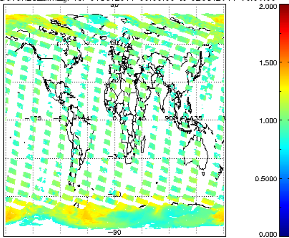
SCIOL2P_NADUV8H20_amf_gr for 01OCT2011 00:00:00 to 02OCT2011 00:00:00
