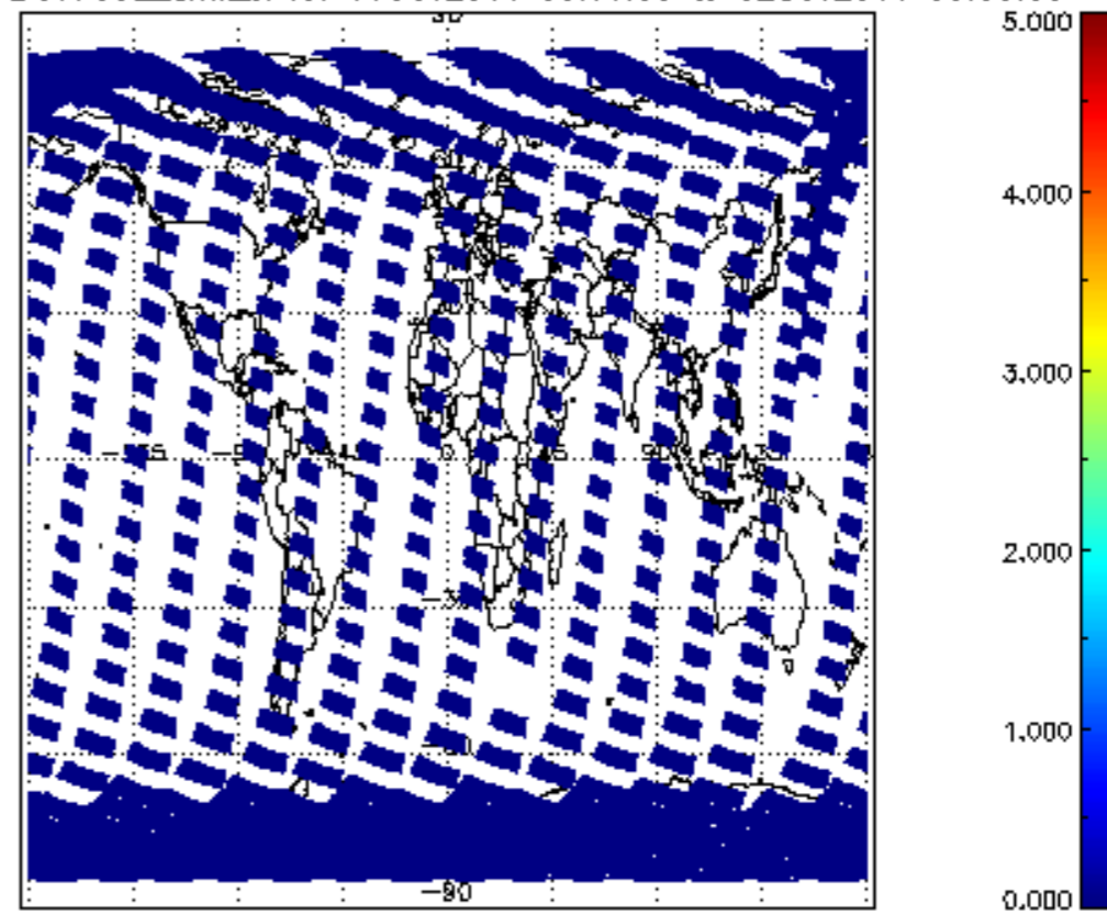
SCIOL2P_NADUV7S02_amf_sl for 01OCT2011 00:00:00 to 02OCT2011 00:00:00
