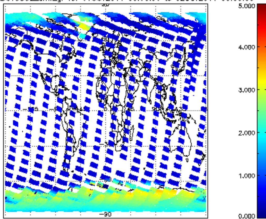
SCIOL2P_NADUV5S02_amf_gr for 01OCT2011 00:00:00 to 02OCT2011 00:00:00
