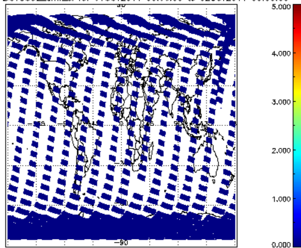
SCIOL2P_NADUV5S02_amf_sl for 01OCT2011 00:00:00 to 02OCT2011 00:00:00
