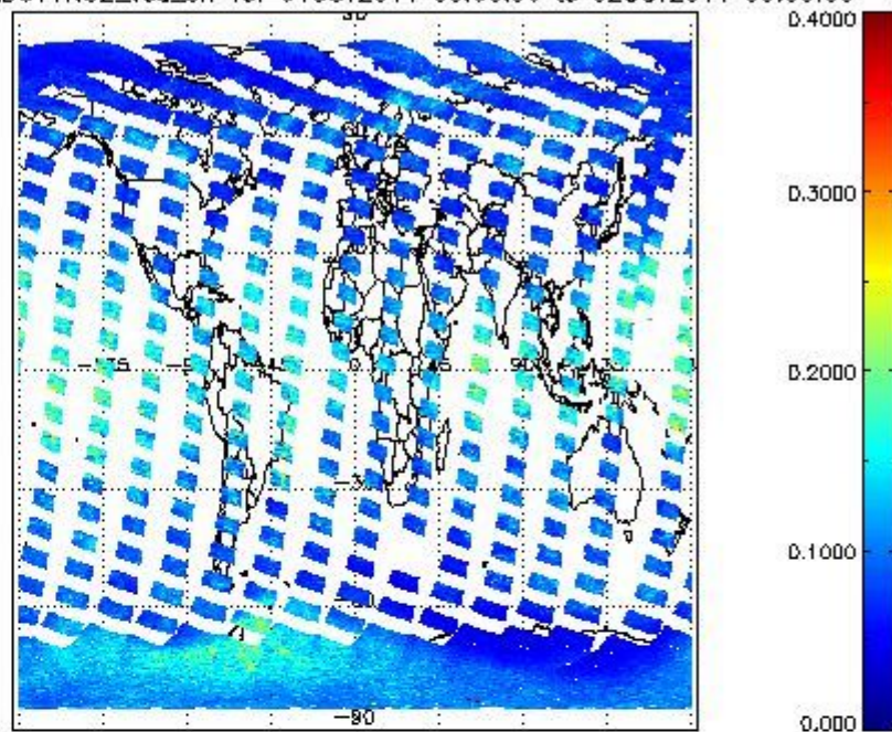
SCIOL2P_NADUV1NO2_vcd_err for 01OCT2011 00:00:00 to 02OCT2011 00:00:00
