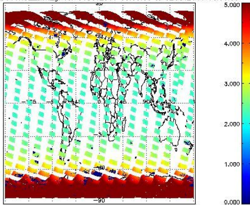
SCIOL2P_NADUV1NO2_amf_gr for 01OCT2011 00:00:00 to 02OCT2011 00:00:00
