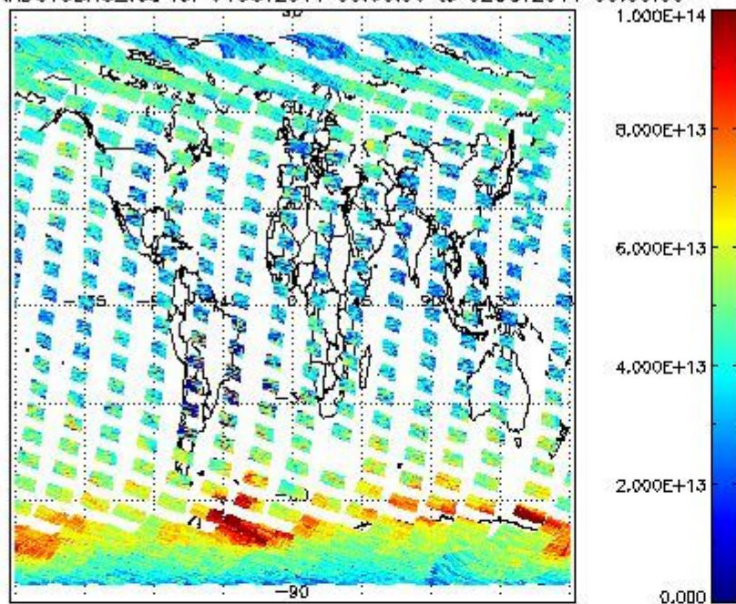
SCIOL2P_NADUV3BRO_vcd for 01OCT2011 00:00:00 to 02OCT2011 00:00:00
