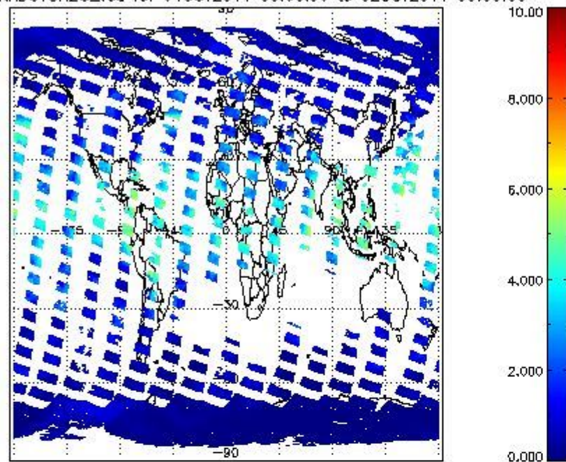
SCIOL2P_NADUV8H20_vcd for 01OCT2011 00:00:00 to 02OCT2011 00:00:00
