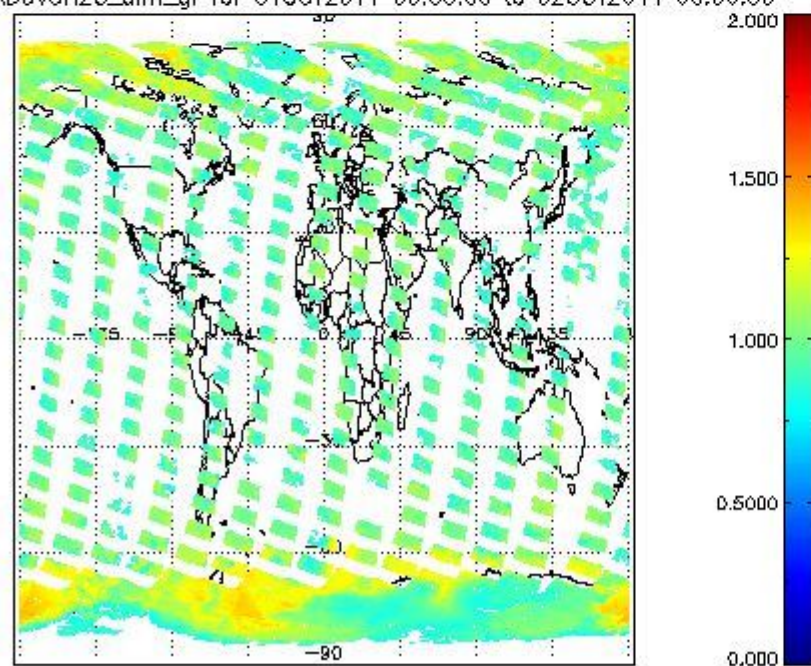
SCIOL2P_NADUV8H20_amf_gr for 01OCT2011 00:00:00 to 02OCT2011 00:00:00
