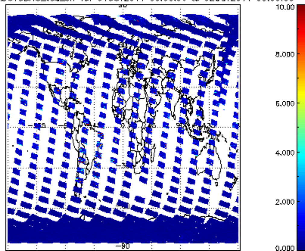
SCIOL2P_NADUV3BRO_vcd_err for 01OCT2011 00:00:00 to 02OCT2011 00:00:00
