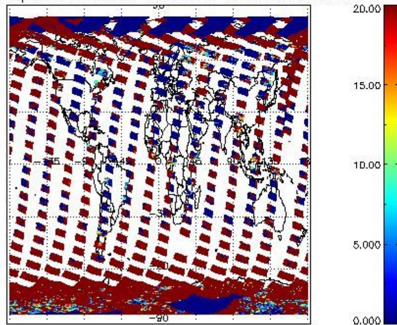
cL_opt_depth for 01OCT2011 00:00:00 to 02OCT2011 00:00:00
