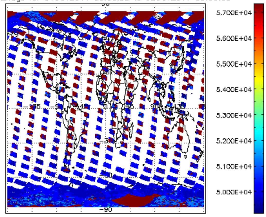
cloud_flags for 01OCT2011 00:00:00 to 02OCT2011 00:00:00
