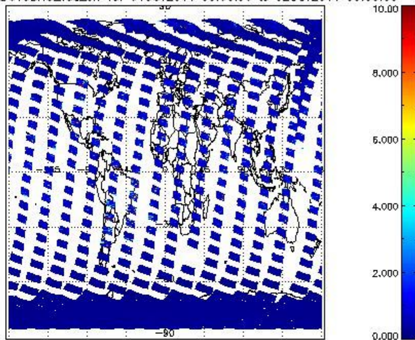
SCIOL2P_NADUV3BRO_vcd_err for 01OCT2011 00:00:00 to 02OCT2011 00:00:00
