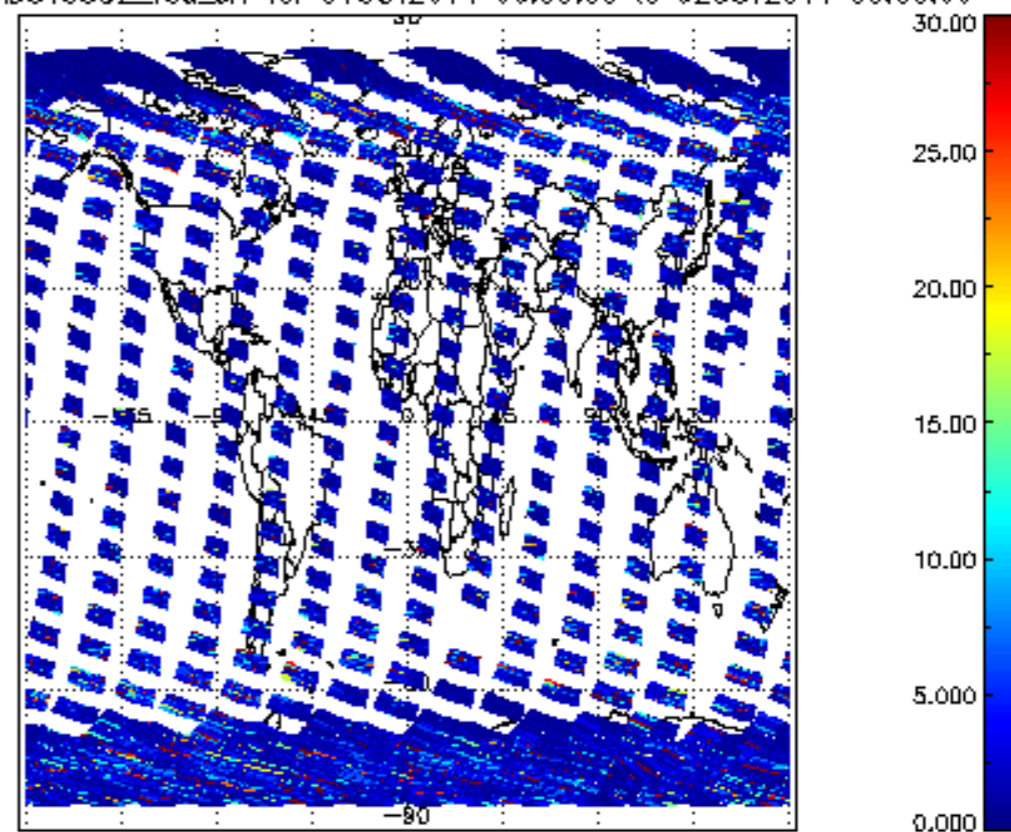
SCIOL2P_NADUV5S02_vcd_err for 01OCT2011 00:00:00 to 02OCT2011 00:00:00
