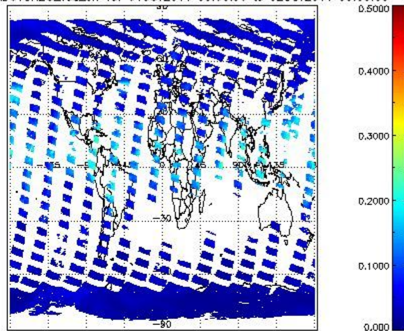
SCIOL2P_NADUV8H20_vcd_err for 01OCT2011 00:00:00 to 02OCT2011 00:00:00
