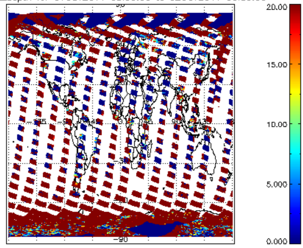
cl_opt_depth for 01OCT2011 00:00:00 to 02OCT2011 00:00:00
