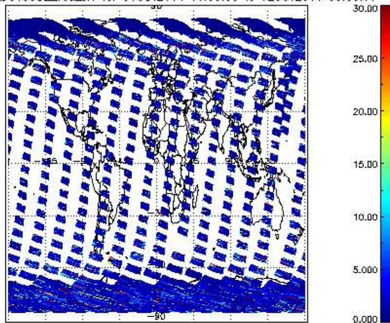
SCIOL2P_NADUV5SO2_vcd_err for 01OCT2011 00:00:00 to 02OCT2011 00:00:00
