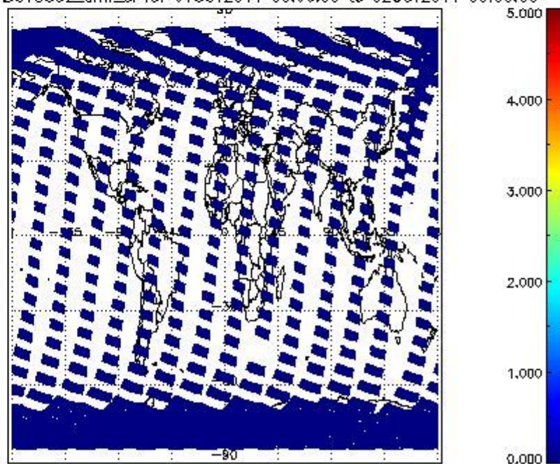
SCIOL2P_NADUV5SO2_amf_cl for 01OCT2011 00:00:00 to 02OCT2011 00:00:00
