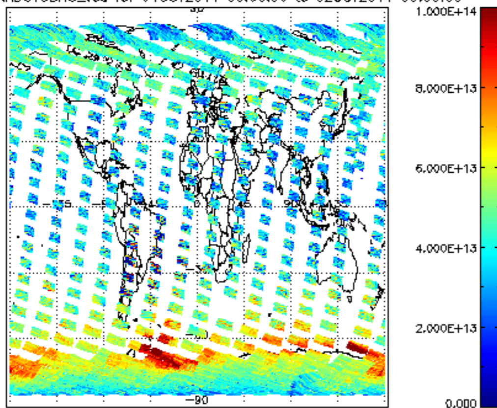
SCIOL2P_NADUV3BRO_vcd for 01OCT2011 00:00:00 to 02OCT2011 00:00:00
