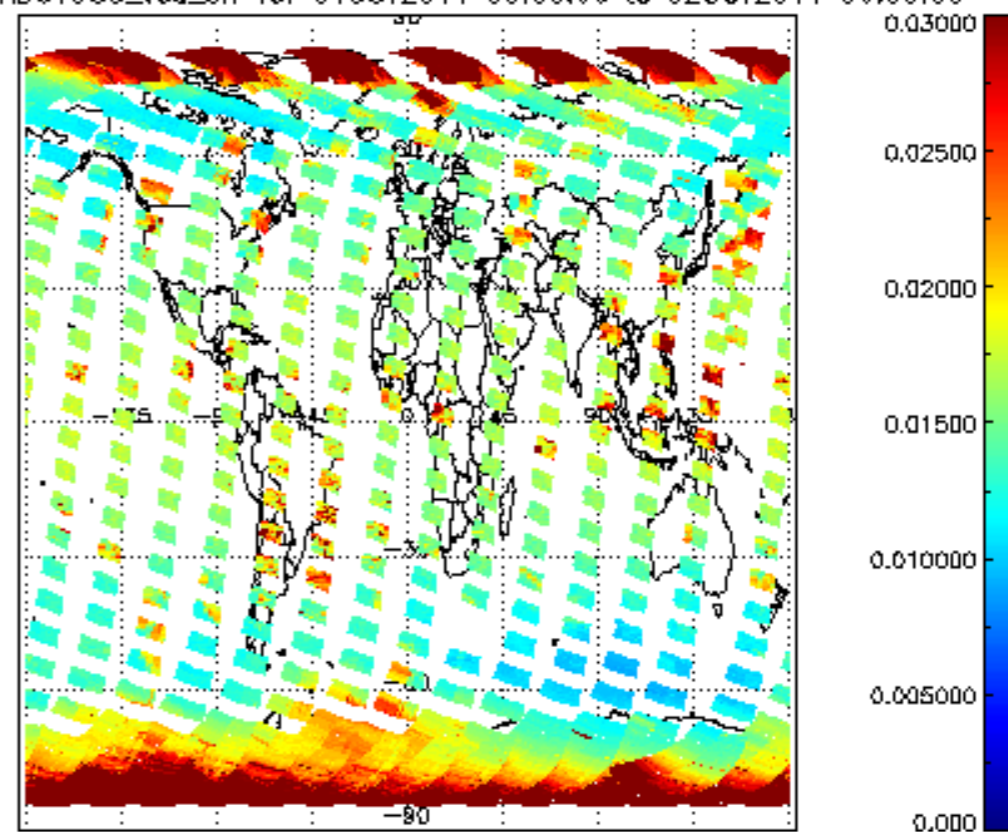
SCIOL2P_NADUV003_vcd_err for 01OCT2011 00:00:00 to 02OCT2011 00:00:00
