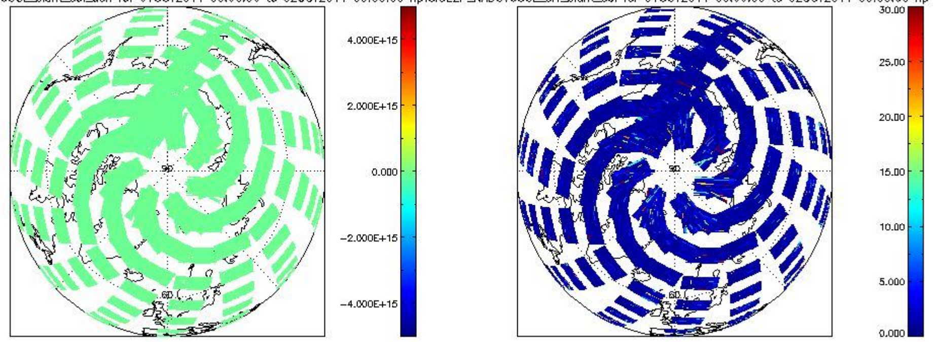
CIOL2P_NADUV60CL_slant_col_den for 01OCT2011 00:00:00 to 02OCT2011 00:00:00 np CIOL2P_NADUV60CL_err_slant_col for 01OCT2011 00:00:00 to 02OCT2011 00:00:00 np
