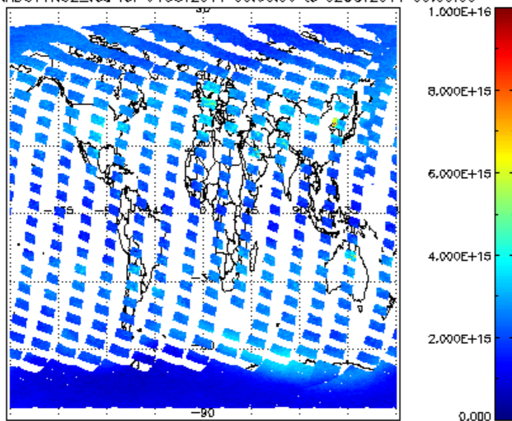
SCIOL2P_NADUV1NO2_vcd for 01OCT2011 00:00:00 to 02OCT2011 00:00:00
