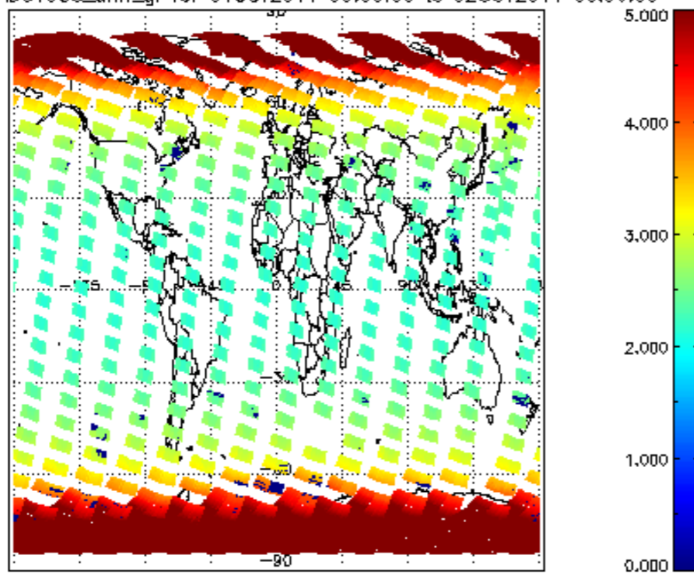
SCIOL2P_NADUV003_amf_gr for 01OCT2011 00:00:00 to 02OCT2011 00:00:00
