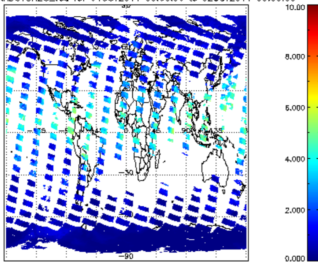
SCIOL2P_NADUV8H20_vcd for 01OCT2011 00:00:00 to 02OCT2011 00:00:00
