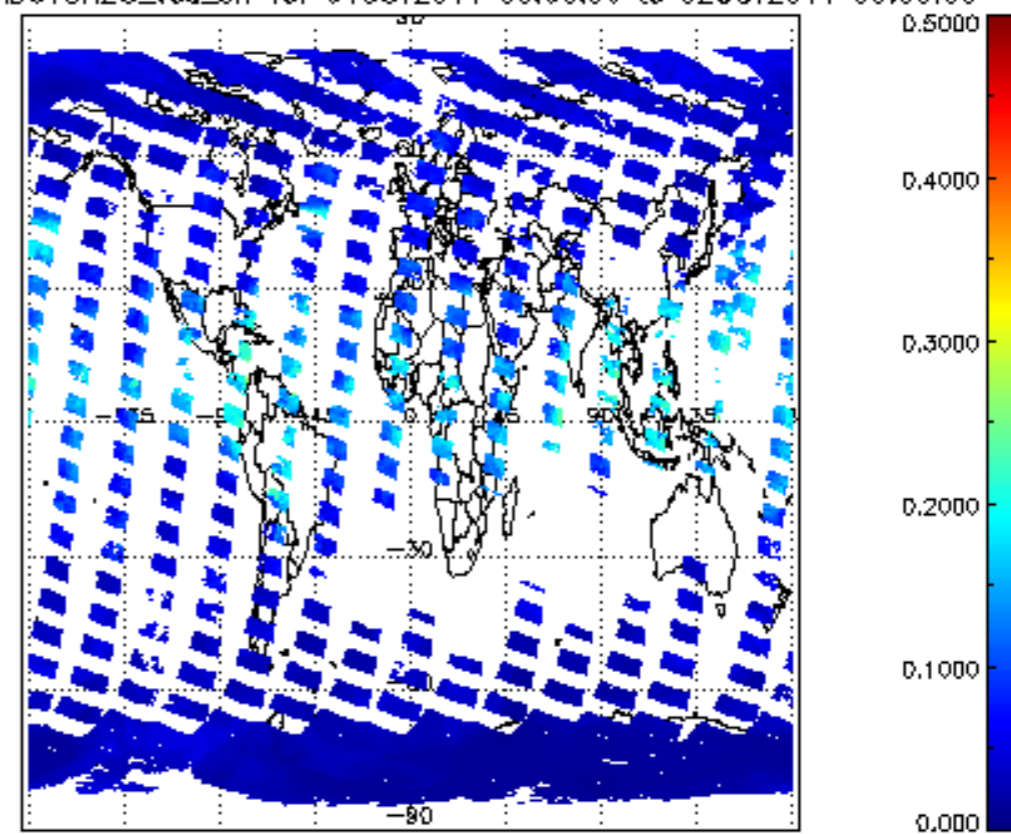
SCIOL2P_NADUV8H20_vcd_err for 01OCT2011 00:00:00 to 02OCT2011 00:00:00
