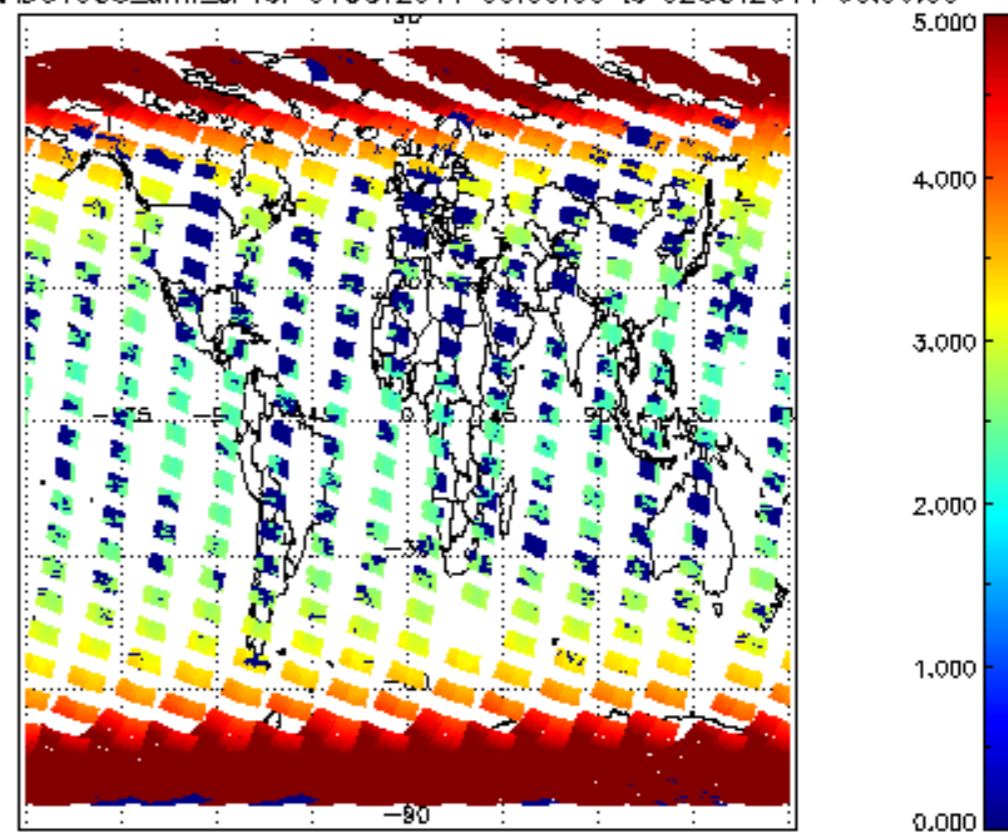
SCIOL2P_NADUV003_amf_cl for 01OCT2011 00:00:00 to 02OCT2011 00:00:00
