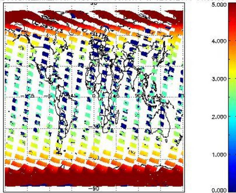
SCIOL2P_NADUV3BRO_amf_cl for 01OCT2011 00:00:00 to 02OCT2011 00:00:00
