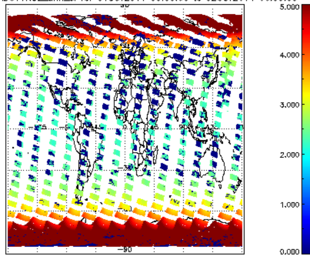
SCIOL2P_NADUV1NO2_amf_cl for 01OCT2011 00:00:00 to 02OCT2011 00:00:00
