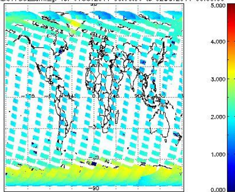
SCIOL2P_NADUV7S02_amf_gr for 01OCT2011 00:00:00 to 02OCT2011 00:00:00
