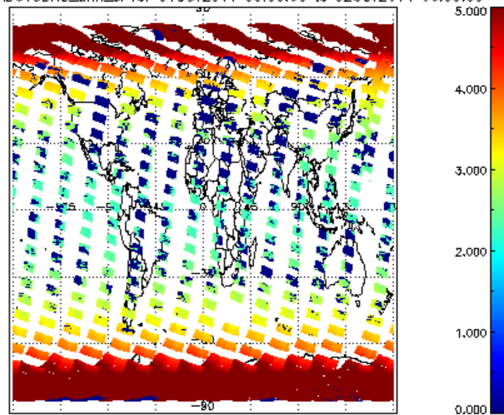
SCIOL2P_NADUV3BRO_amf_cl for 01OCT2011 00:00:00 to 02OCT2011 00:00:00
