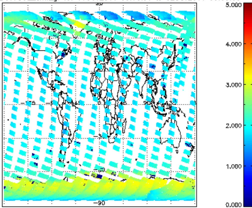
SCIOL2P_NADUV7S02_amf_gr for 01OCT2011 00:00:00 to 02OCT2011 00:00:00
