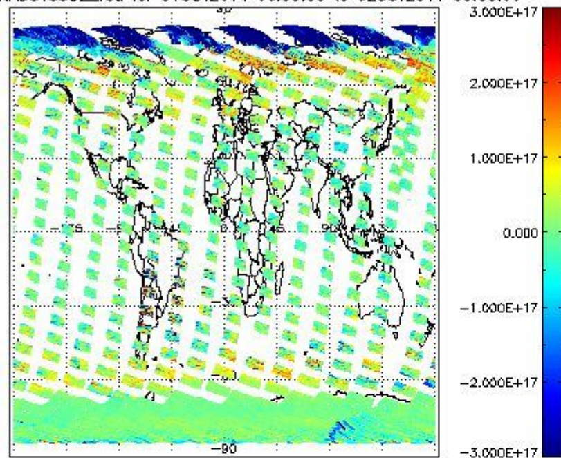
SCIOL2P_NADUV5SO2_vcd for 01OCT2011 00:00:00 to 02OCT2011 00:00:00
