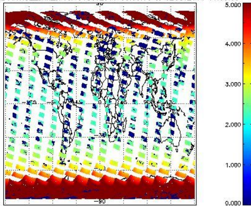
SCIOL2P_NADUV1NO2_amf_cl for 01OCT2011 00:00:00 to 02OCT2011 00:00:00
