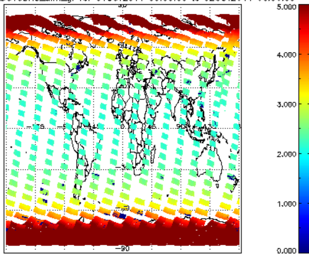
SCIOL2P_NADUV3BRO_amf_gr for 01OCT2011 00:00:00 to 02OCT2011 00:00:00
