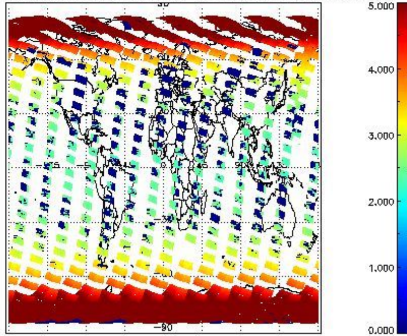
SCIOL2P_NADUV003_amf_cl for 01OCT2011 00:00:00 to 02OCT2011 00:00:00
