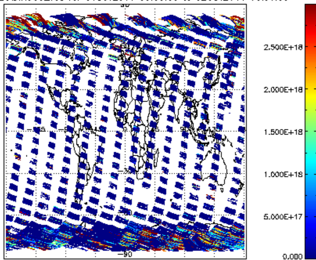
SCIOL2P_NADIR3CO_vcd for 01OCT2011 00:00:00 to 02OCT2011 00:00:00
