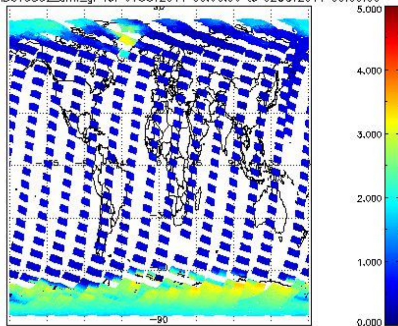
SCIOL2P_NADUV5SO2_amf_gr for 01OCT2011 00:00:00 to 02OCT2011 00:00:00
