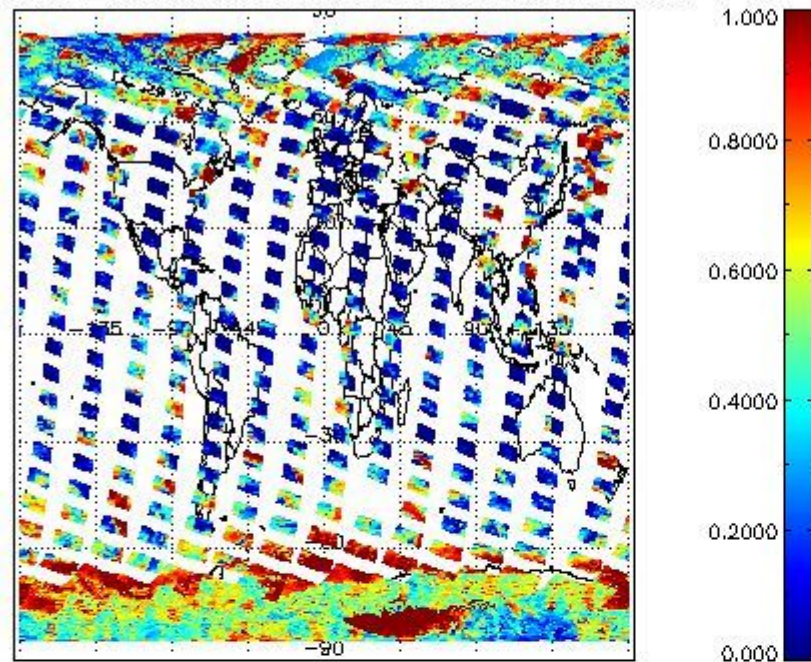
cLfrac for 01OCT2011 00:00:00 to 02OCT2011 00:00:00
