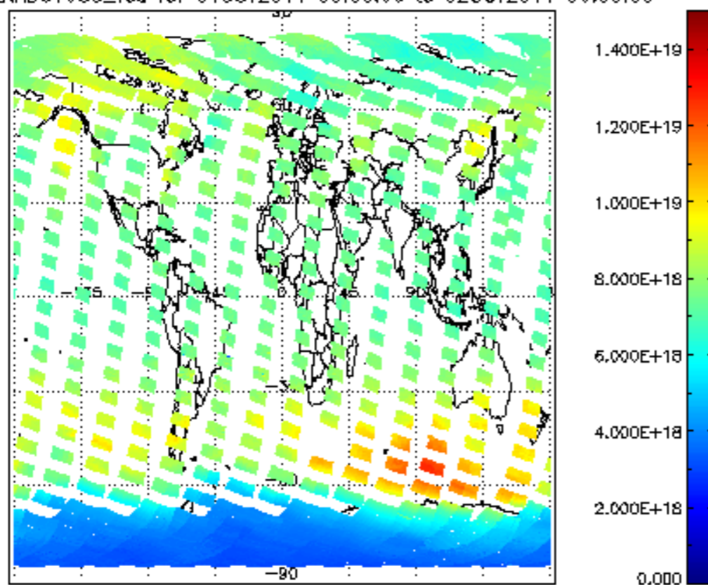
SCIOL2P_NADUV003_vcd for 01OCT2011 00:00:00 to 02OCT2011 00:00:00
