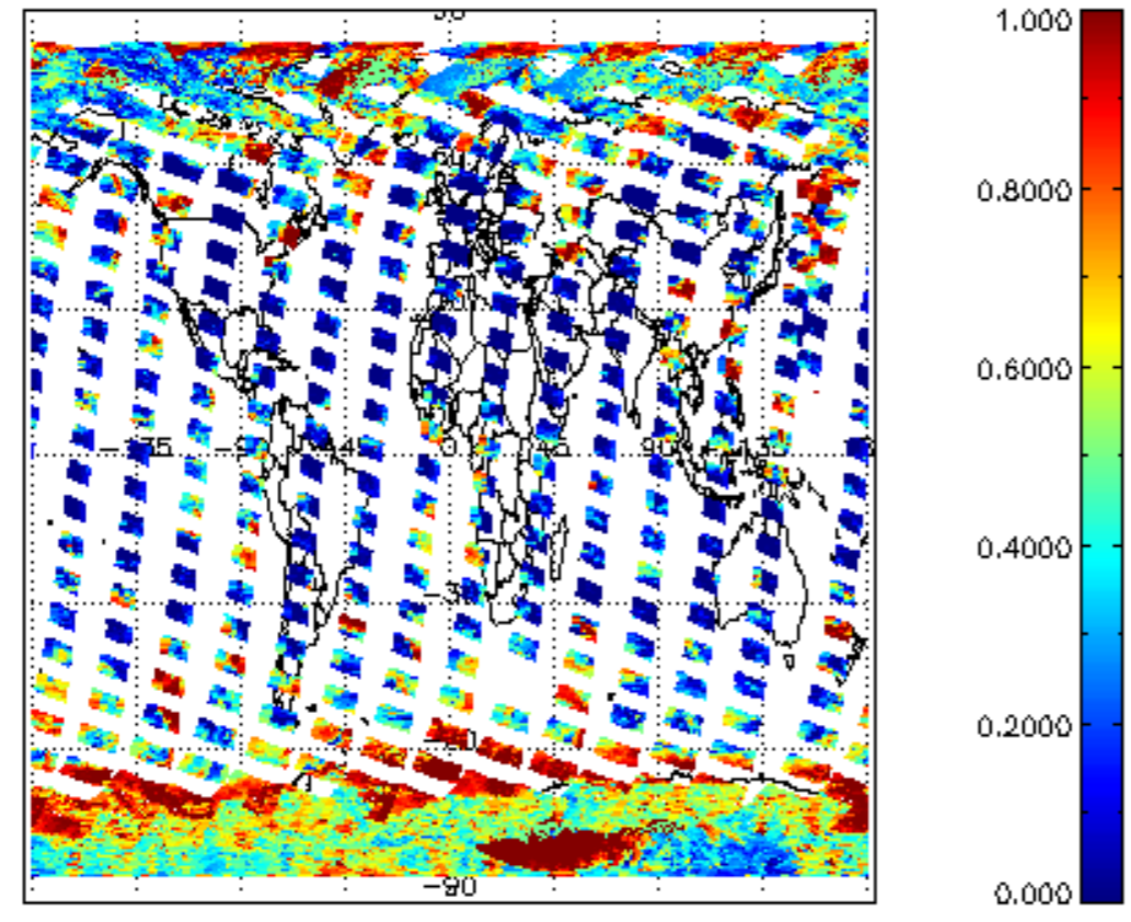
cl_frac for 01OCT2011 00:00:00 to 02OCT2011 00:00:00
