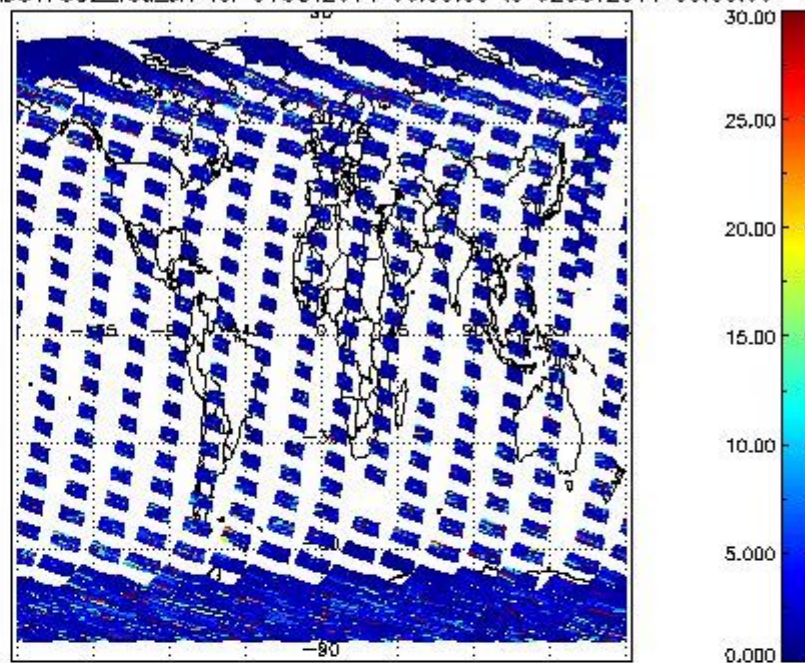
SCIOL2P_NADUV7S02_vcd_err for 01OCT2011 00:00:00 to 02OCT2011 00:00:00
