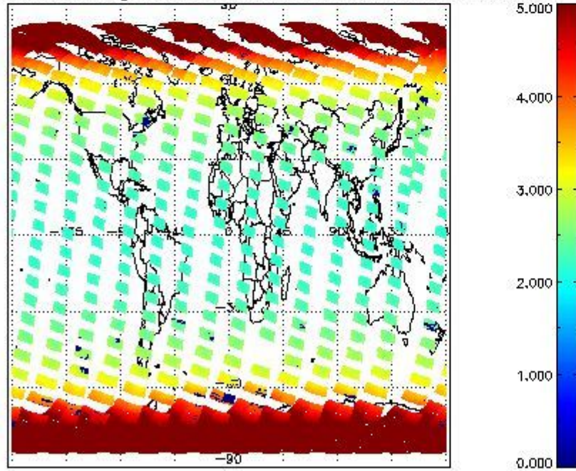
SCIOL2P_NADUV003_amf_gr for 01OCT2011 00:00:00 to 02OCT2011 00:00:00
