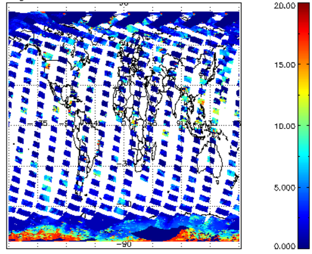
cl_top_height for 01OCT2011 00:00:00 to 02OCT2011 00:00:00
