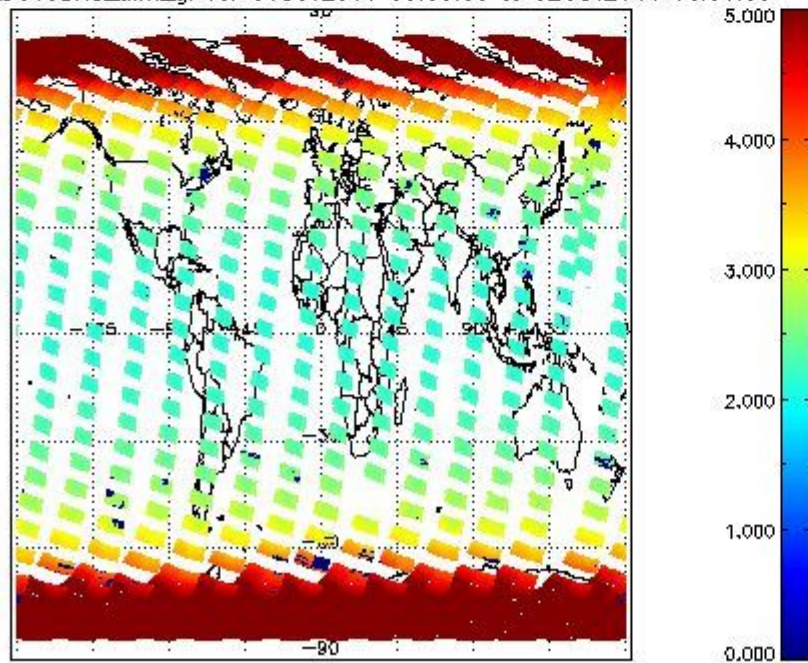
SCIOL2P_NADUV3BRO_amf_gr for 01OCT2011 00:00:00 to 02OCT2011 00:00:00
