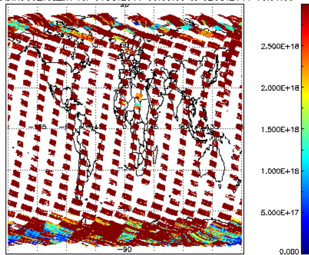
SCIOL2P_NADIR3CO_vcd_err for 01OCT2011 00:00:00 to 02OCT2011 00:00:00
