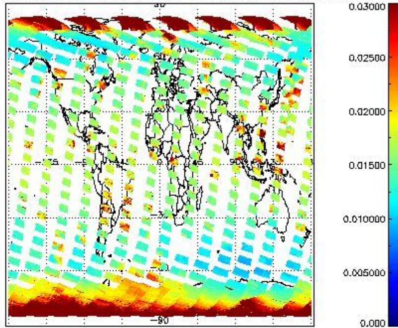
SCIOL2P_NADUV003_vcd_err for 01OCT2011 00:00:00 to 02OCT2011 00:00:00
