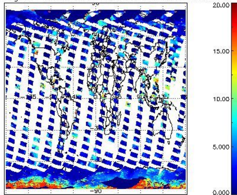
cL_top_height for 01OCT2011 00:00:00 to 02OCT2011 00:00:00
