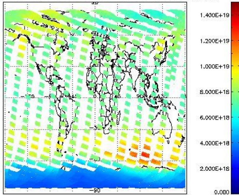
SCIOL2P_NADUV003_vcd for 01OCT2011 00:00:00 to 02OCT2011 00:00:00
