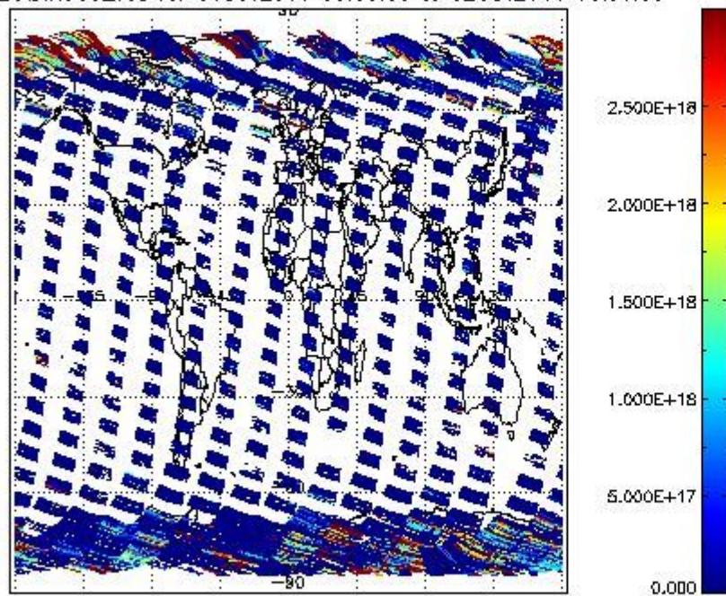
SCIDL2P_NADIR3CO_vcd for 01OCT2011 00:00:00 to 02OCT2011 00:00:00
