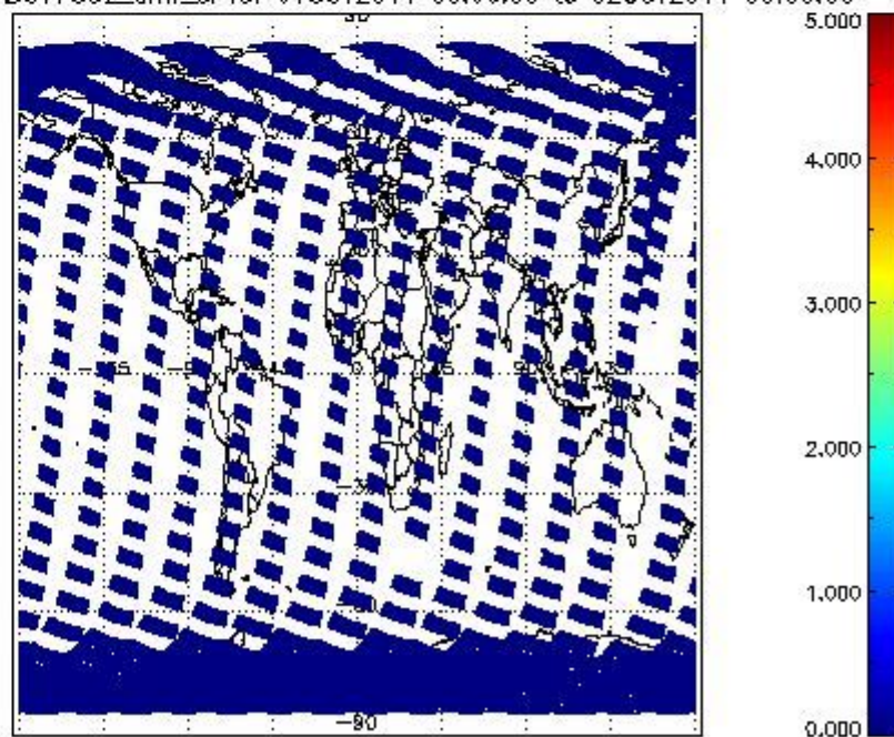
SCIOL2P_NADUV7S02_amf_cl for 01OCT2011 00:00:00 to 02OCT2011 00:00:00
