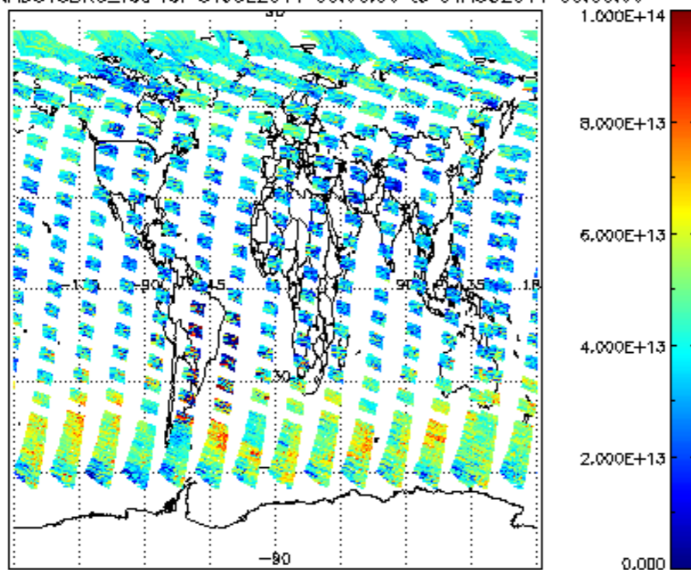
SCIOL2P_NADUV3BRO_vcd for 31JUL2011 00:00:00 to 01AUG2011 00:00:00
