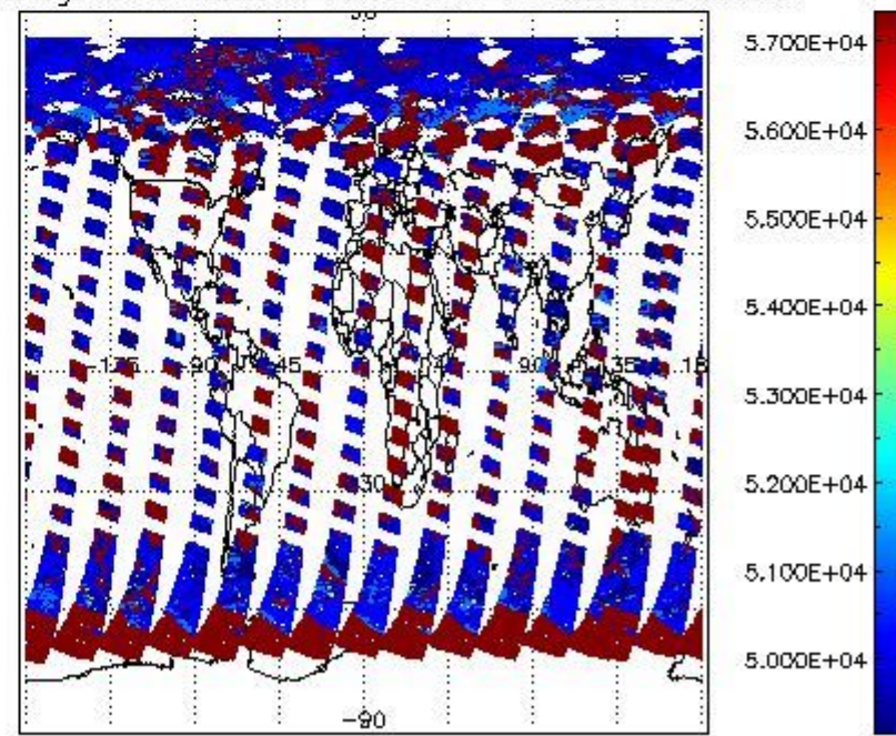
cloud_flags for 31JUL2011 00:00:00 to 01AUG2011 00:00:00
