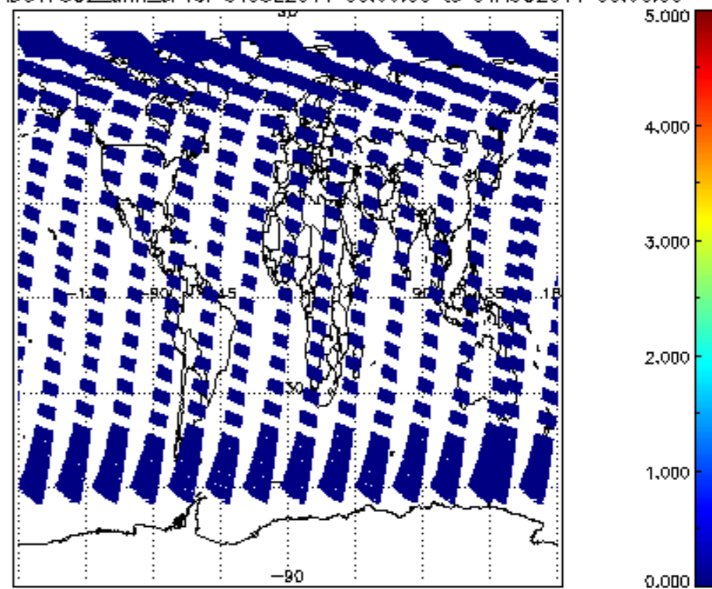
SCIOL2P_NADUV7S02_amf_cl for 31JUL2011 00:00:00 to 01AUG2011 00:00:00
