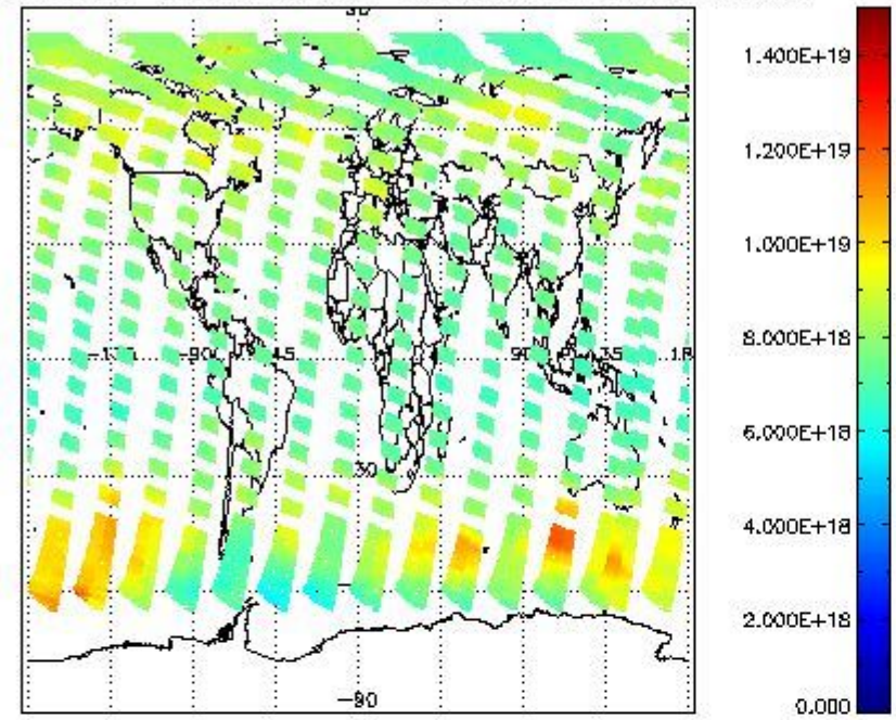
SCIOL2P_NADUV003_vcd for 31JUL2011 00:00:00 to 01AUG2011 00:00:00
