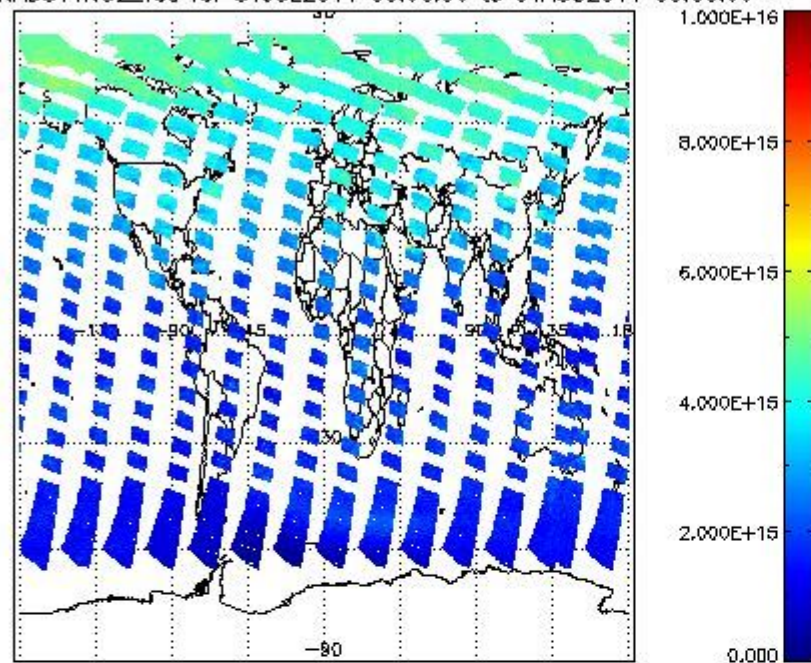
SCIOL2P_NADUV1N02_vcd for 31JUL2011 00:00:00 to 01AUG2011 00:00:00
