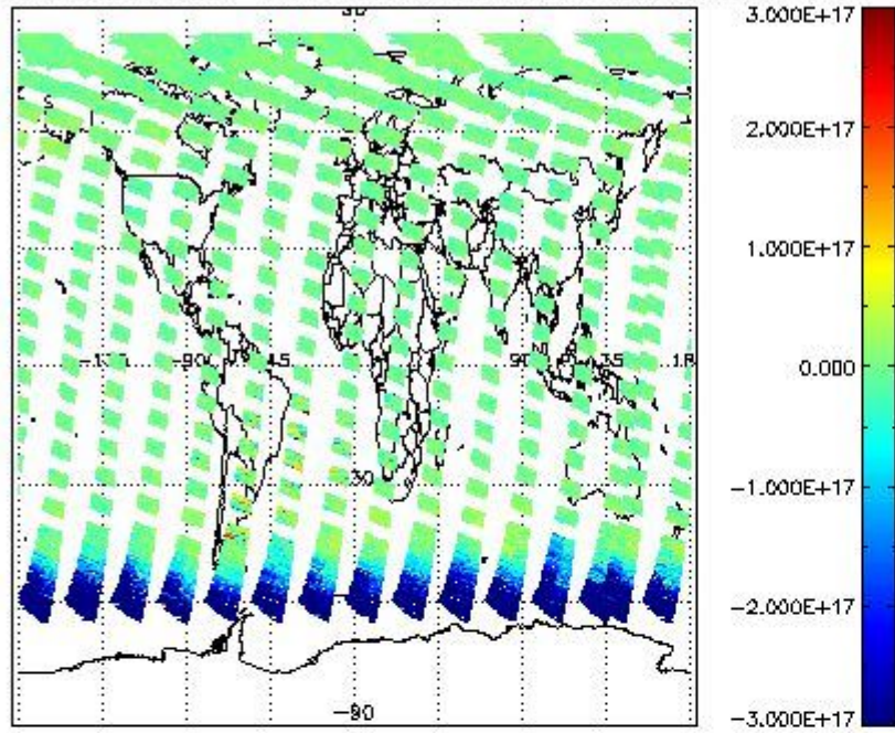
SCIOL2P_NADUV7S02_vcd for 31JUL2011 00:00:00 to 01AUG2011 00:00:00
