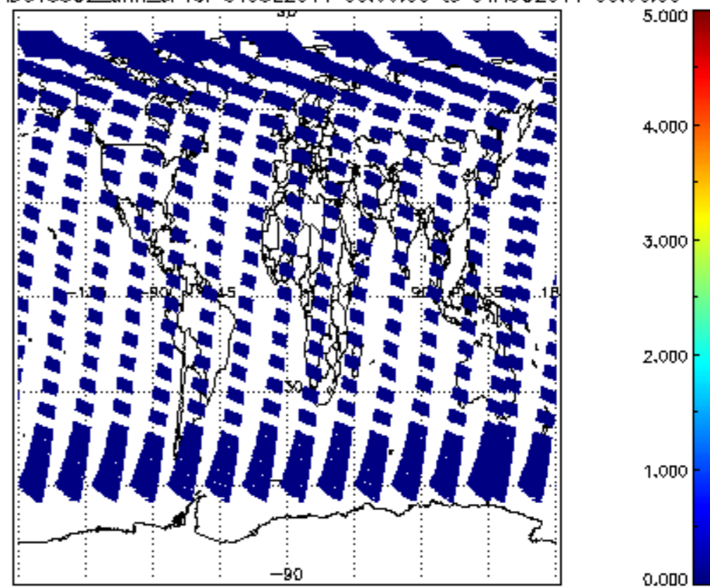
SCIOL2P_NADUV5S02_amf_cl for 31JUL2011 00:00:00 to 01AUG2011 00:00:00
