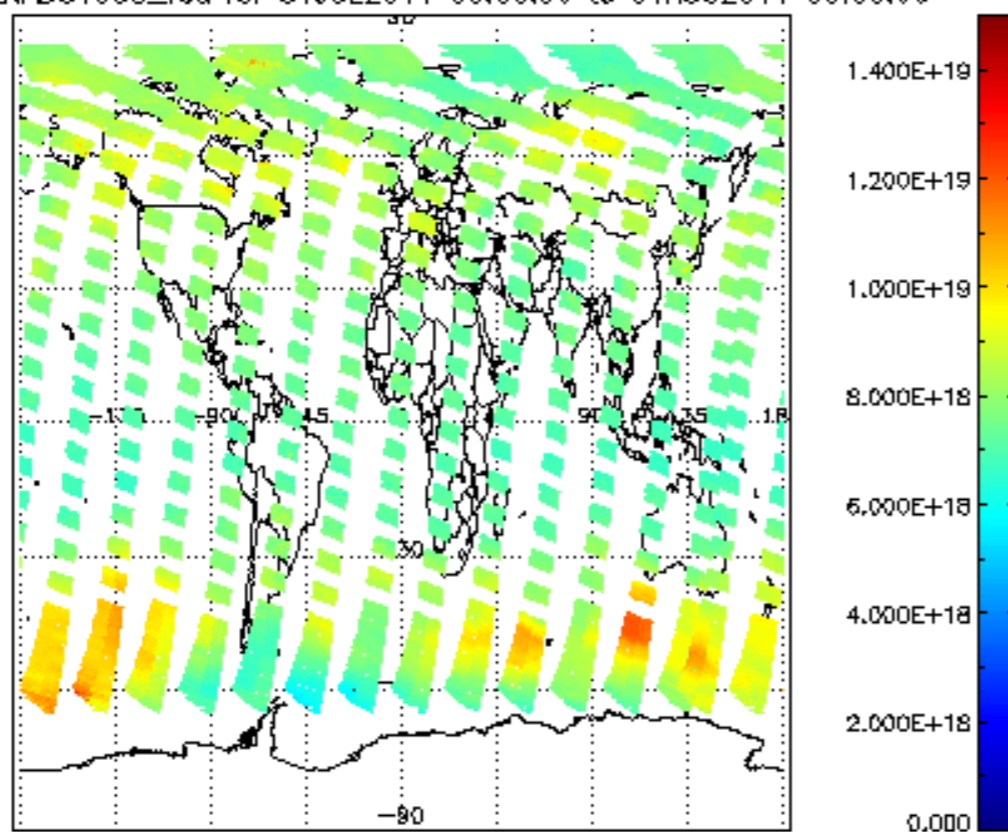
SCIOL2P_NADUV003_vcd for 31JUL2011 00:00:00 to 01AUG2011 00:00:00
