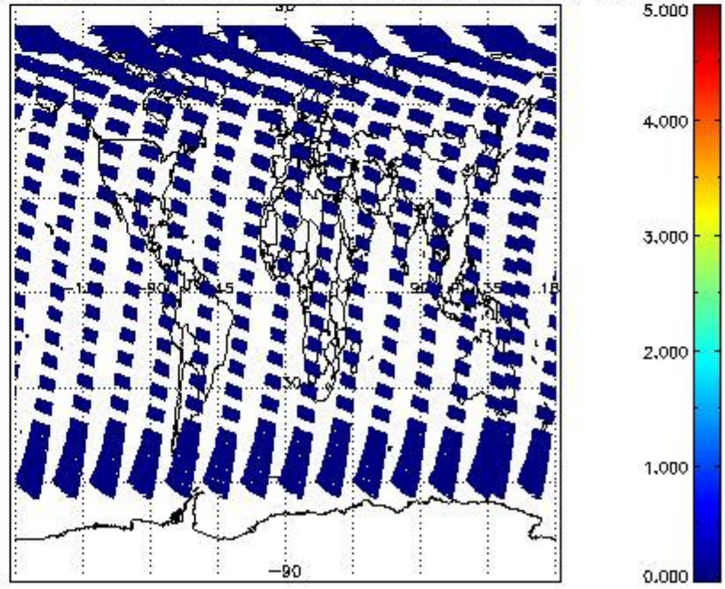
SCIOL2P_NADUV5S02_amf_cl for 31JUL2011 00:00:00 to 01AUG2011 00:00:00
