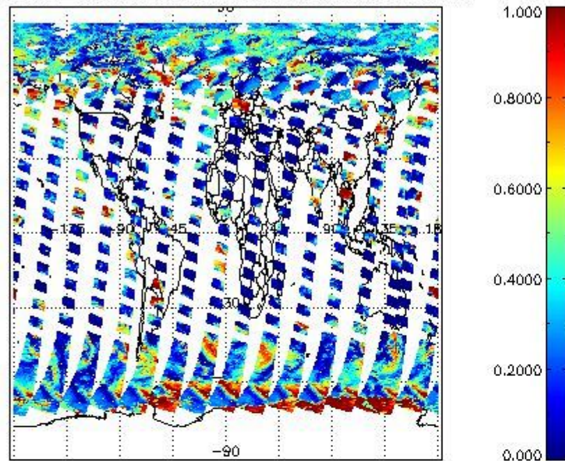
cL_frae for 31JUL2011 00:00:00 to 01AUG2011 00:00:00
