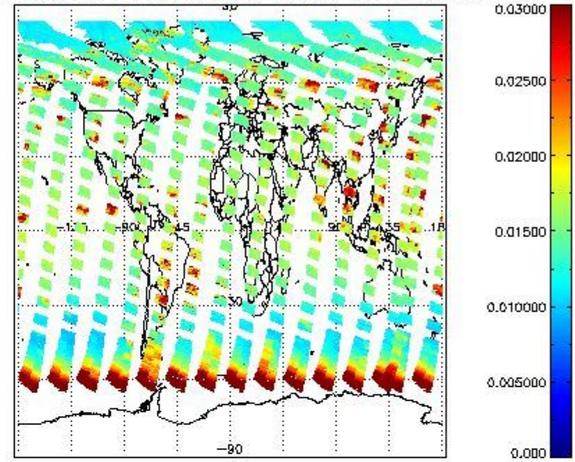
SCIOL2P_NADUV003_vcd_err for 31JUL2011 00:00:00 to 01AUG2011 00:00:00
