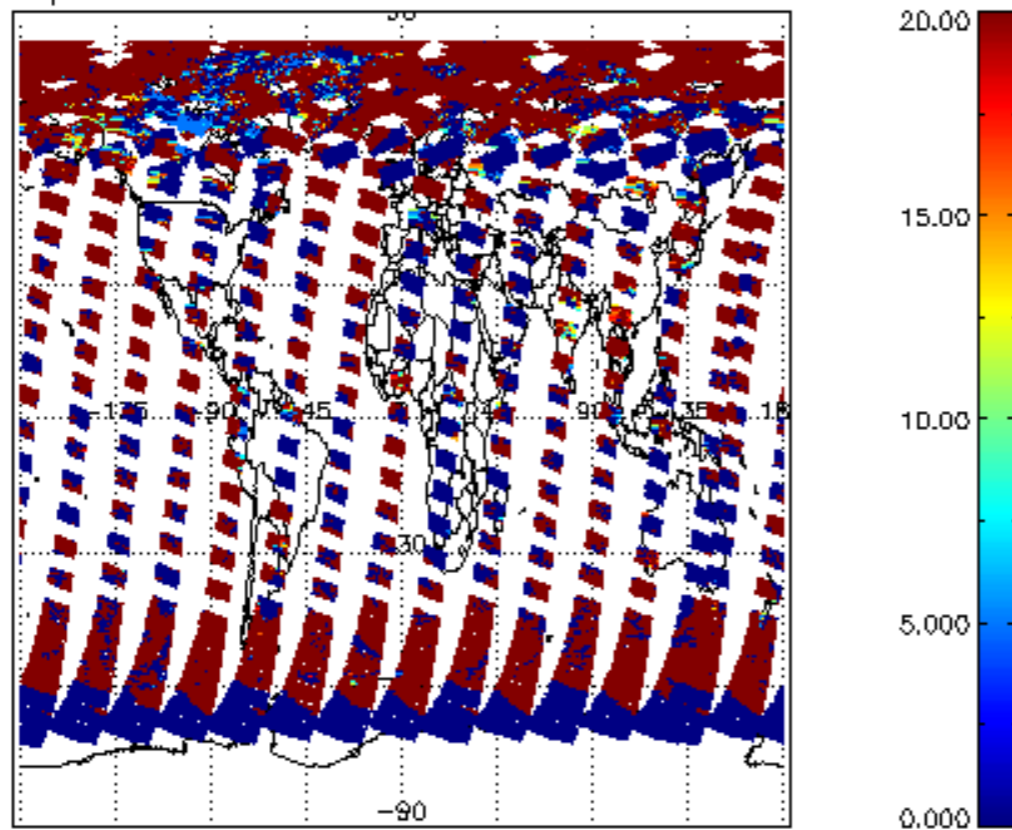
cl_opt_depth for 31JUL2011 00:00:00 to 01AUG2011 00:00:00
