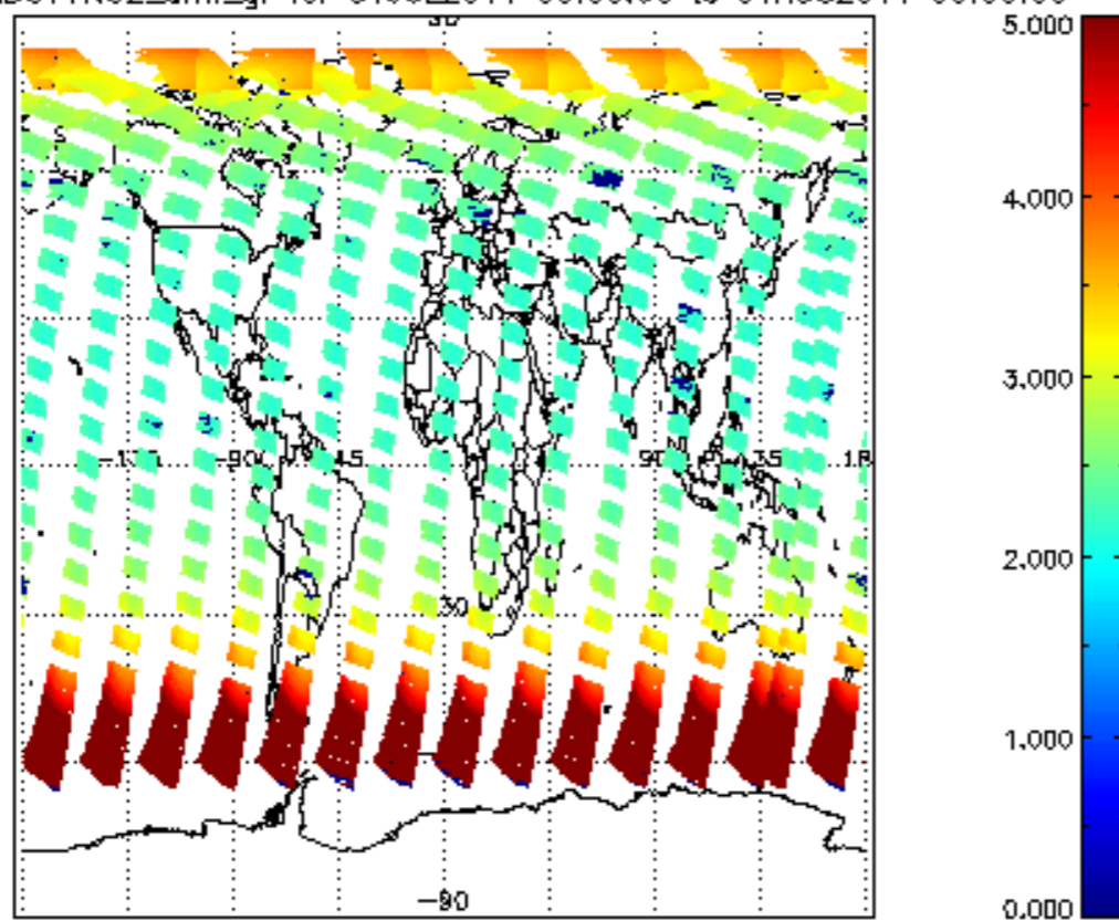
SCIOL2P_NADUV1N02_amf_gr for 31JUL2011 00:00:00 to 01AUG2011 00:00:00
