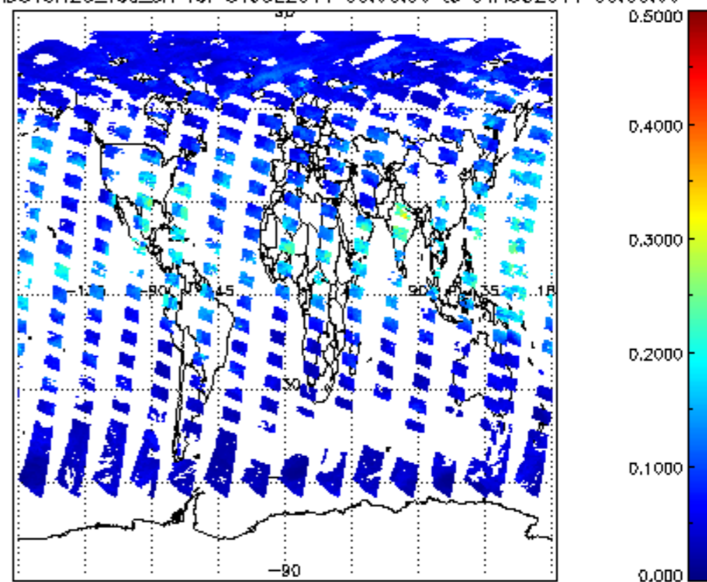
SCIOL2P_NADUV8H20_vcd_err for 31JUL2011 00:00:00 to 01AUG2011 00:00:00
