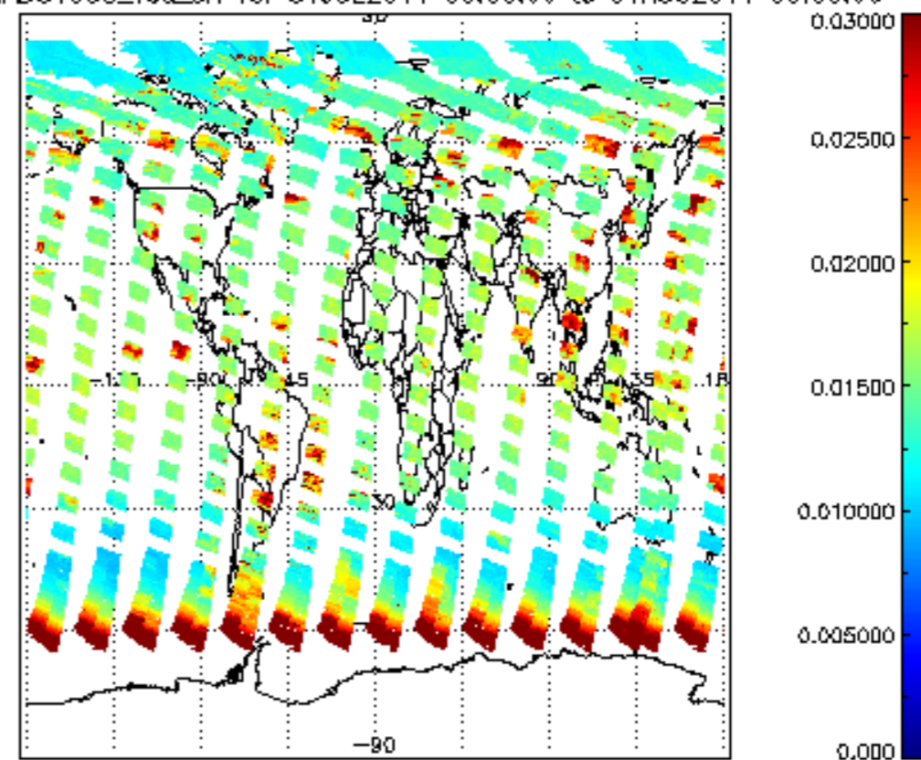
SCIOL2P_NADUV003_vcdLerr for 31JUL2011 00:00:00 to 01AUG2011 00:00:00
