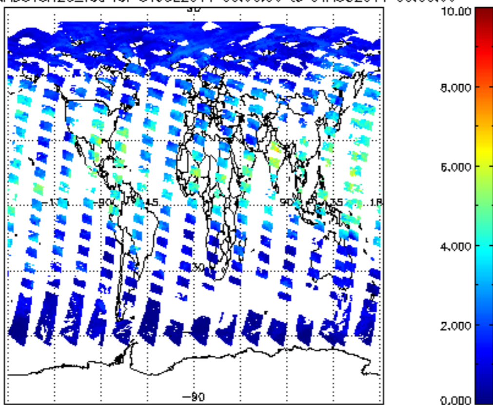
SCIOL2P_NADUV8H20_vcd for 31JUL2011 00:00:00 to 01AUG2011 00:00:00
