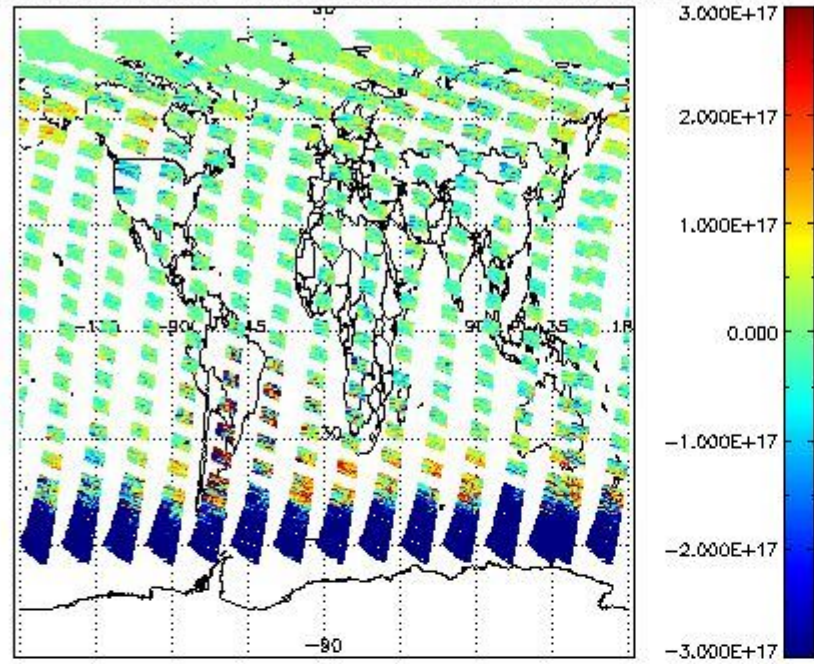
SCIOL2P_NADUV5S02_vcd for 31JUL2011 00:00:00 to 01AUG2011 00:00:00
