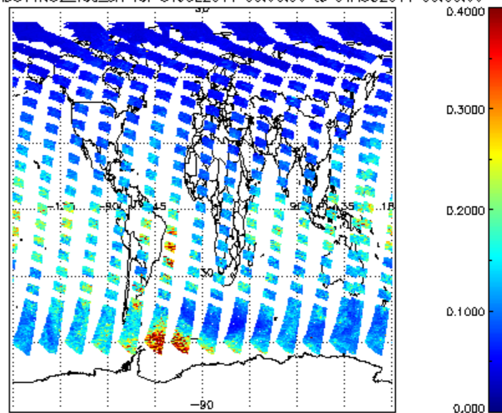
SCIOL2P_NADUV1N02_vcd_err for 31JUL2011 00:00:00 to 01AUG2011 00:00:00
