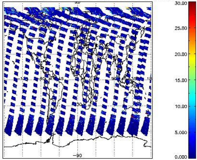
SCIOL2P_NADUV5S02_vcd_err for 31JUL2011 00:00:00 to 01AUG2011 00:00:00
