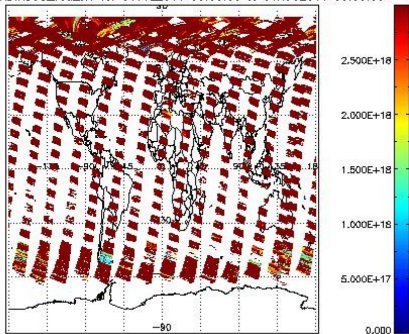
SCIDL2P_NADIR3CO_vcd_err for 31JUL2011 00:00:00 to 01AUG2011 00:00:00
