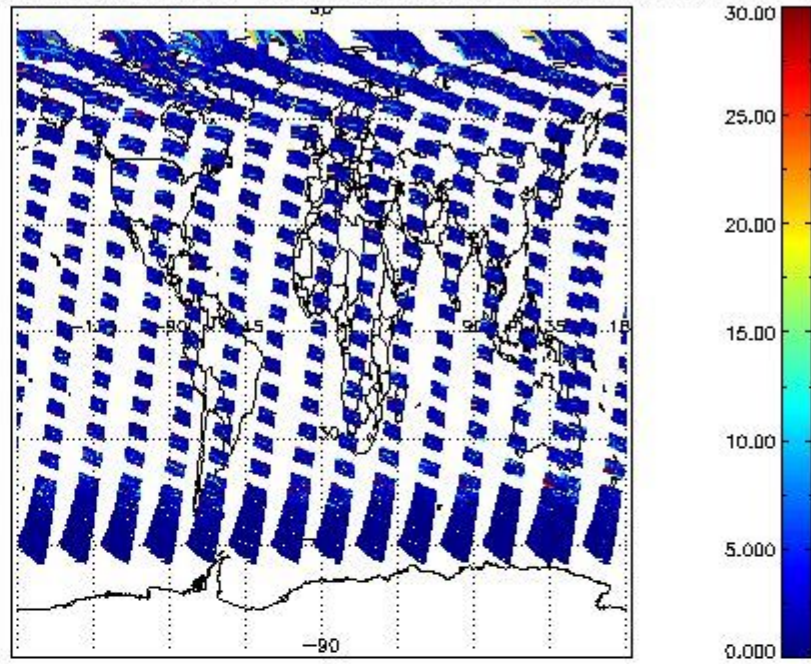
SCIOL2P_NADUV7S02_vcd_err for 31JUL2011 00:00:00 to 01AUG2011 00:00:00
