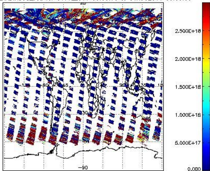
SCIDL2P_NADIR3CO_vcd for 31JUL2011 00:00:00 to 01AUG2011 00:00:00
