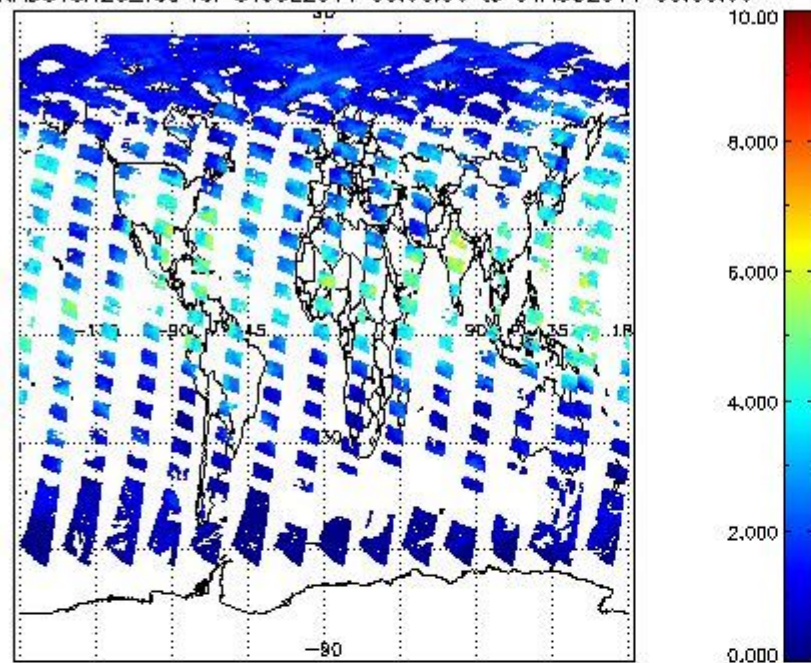
SCIOL2P_NADUV8H2O_vcd for 31JUL2011 00:00:00 to 01AUG2011 00:00:00
