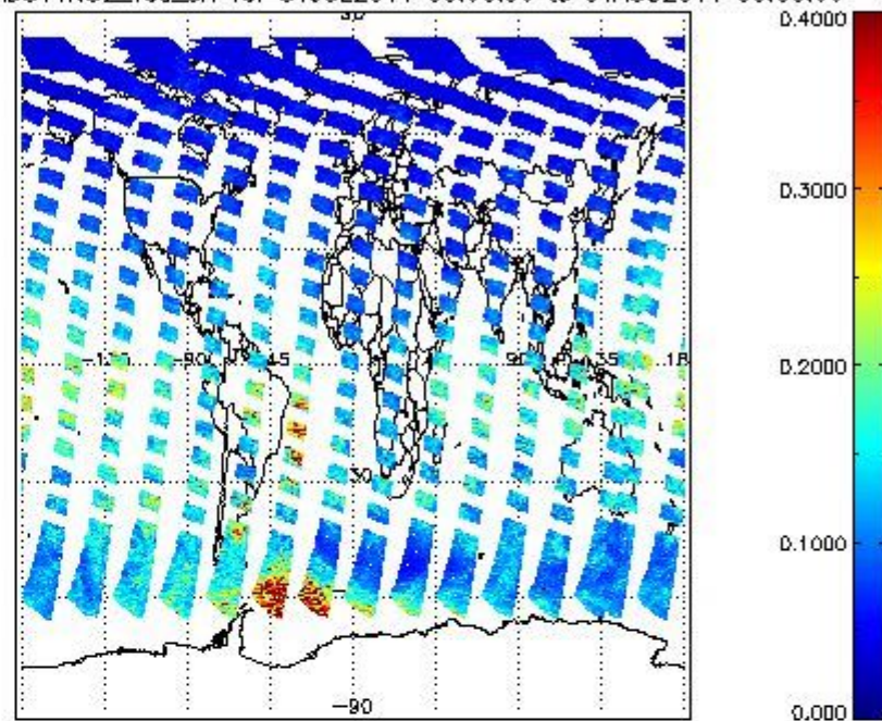
SCIOL2P_NADUV1N02_vcd_err for 31JUL2011 00:00:00 to 01AUG2011 00:00:00
