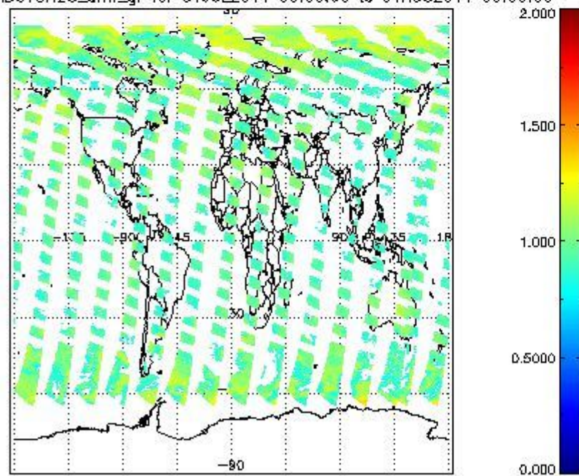
SCIOL2P_NADUV8H2O_amf_gr for 31JUL2011 00:00:00 to 01AUG2011 00:00:00
