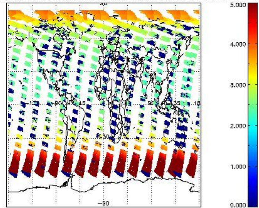
SCIOL2P_NADUV003_amf_cl for 31JUL2011 00:00:00 to 01AUG2011 00:00:00
