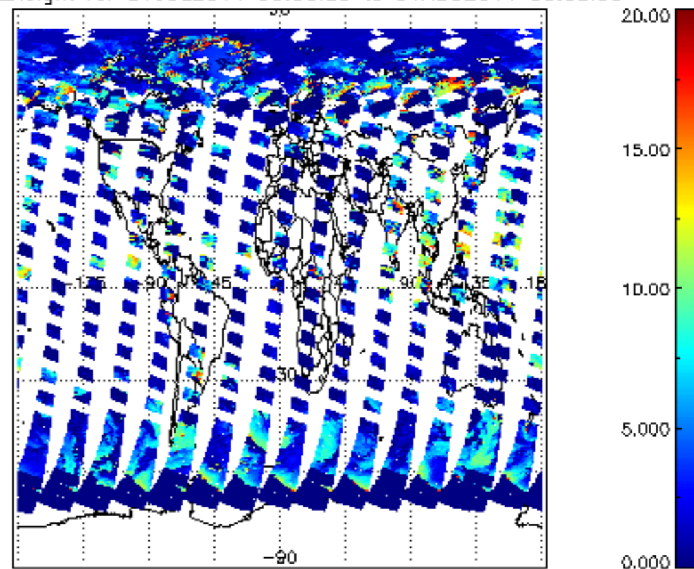
cl_top_height for 31JUL2011 00:00:00 to 01AUG2011 00:00:00
