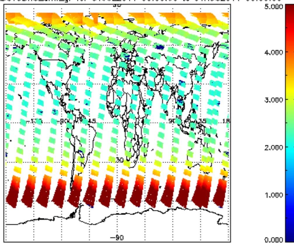
SCIOL2P_NADUV3BRO_amf_gr for 31JUL2011 00:00:00 to 01AUG2011 00:00:00
