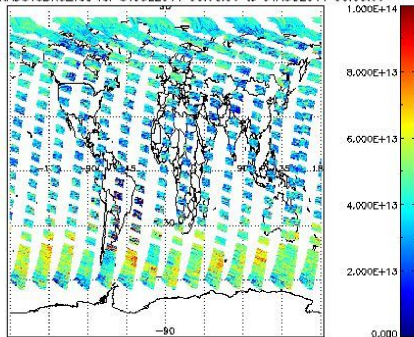
SCIOL2P_NADUV3BRO_vcd for 31JUL2011 00:00:00 to 01AUG2011 00:00:00
