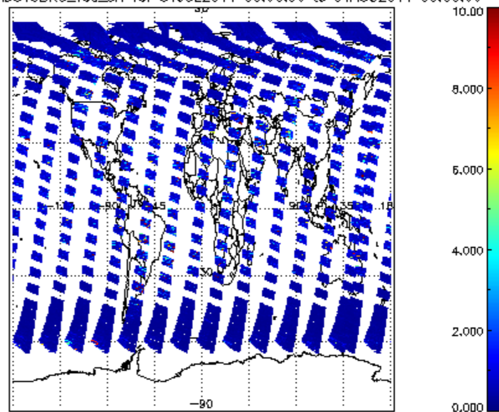
SCIOL2P_NADUV3BRO_vcd_err for 31JUL2011 00:00:00 to 01AUG2011 00:00:00
