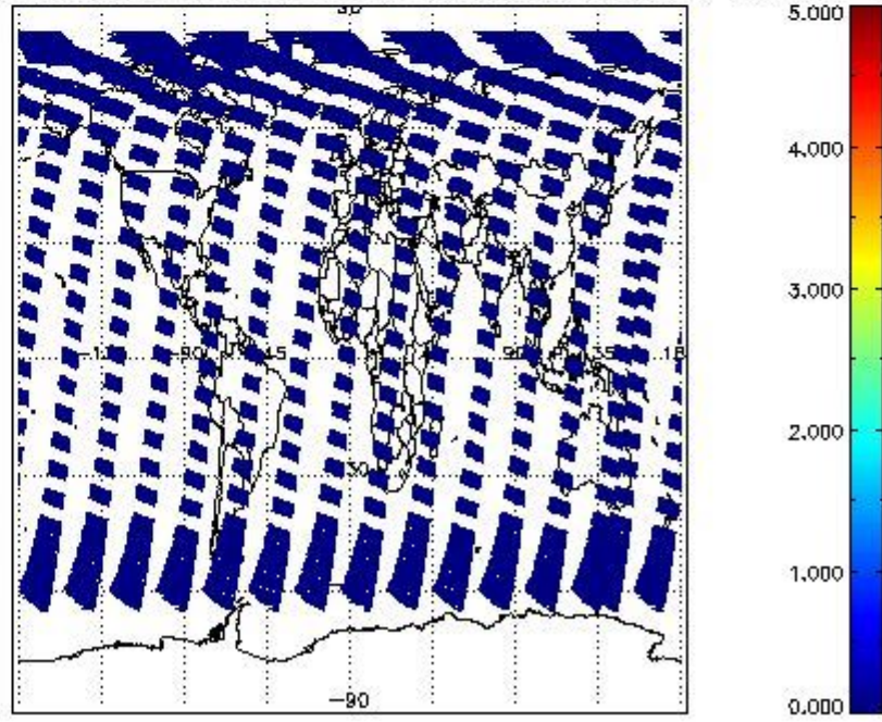
SCIOL2P_NADUV7S02_amf_cl for 31JUL2011 00:00:00 to 01AUG2011 00:00:00
