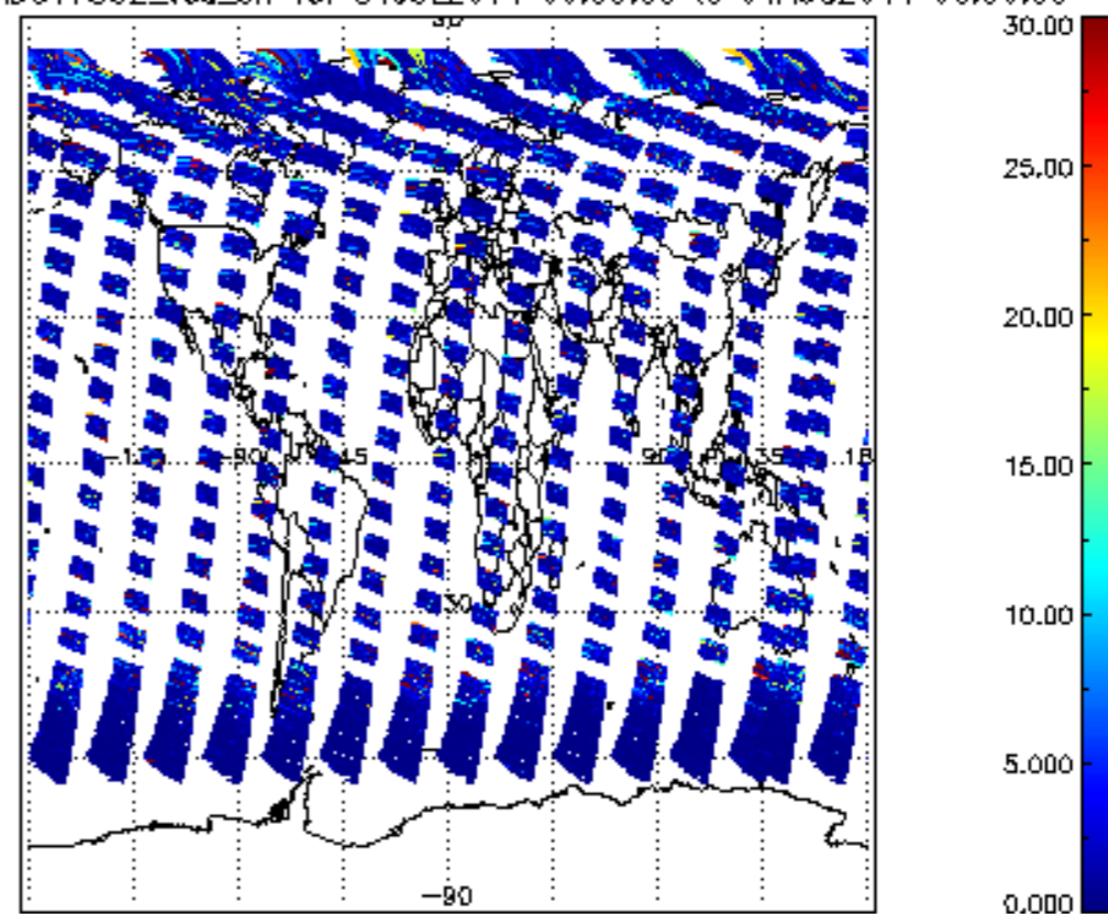
SCIOL2P_NADUV7S02_vcd_err for 31JUL2011 00:00:00 to 01AUG2011 00:00:00
