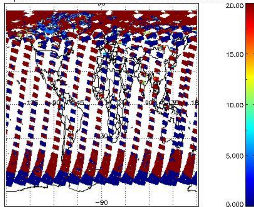
cL_opt_depth for 31JUL2011 00:00:00 to 01AUG2011 00:00:00
