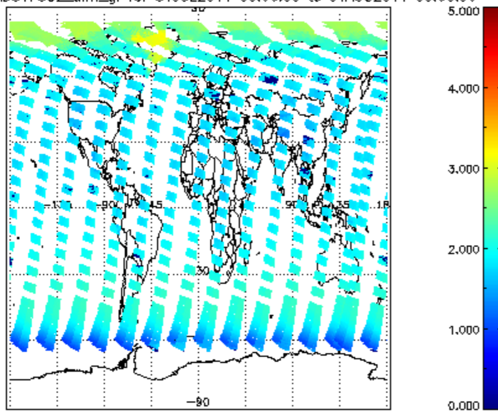
SCIOL2P_NADUV7S02_amf_gr for 31JUL2011 00:00:00 to 01AUG2011 00:00:00
