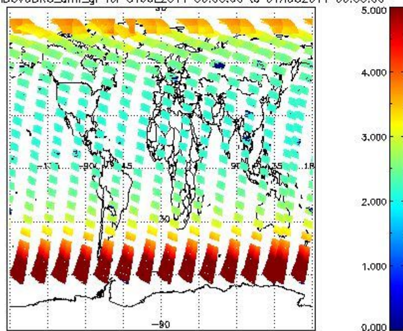
SCIOL2P_NADUV3BRO_amf_gr for 31JUL2011 00:00:00 to 01AUG2011 00:00:00
