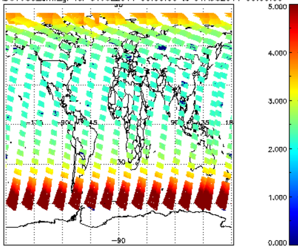
SCIOL2P_NADUV003_amf_gr for 31JUL2011 00:00:00 to 01AUG2011 00:00:00
