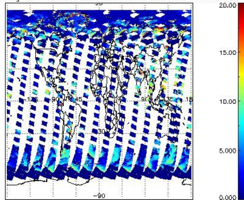
cL_top_height for 31JUL2011 00:00:00 to 01AUG2011 00:00:00
