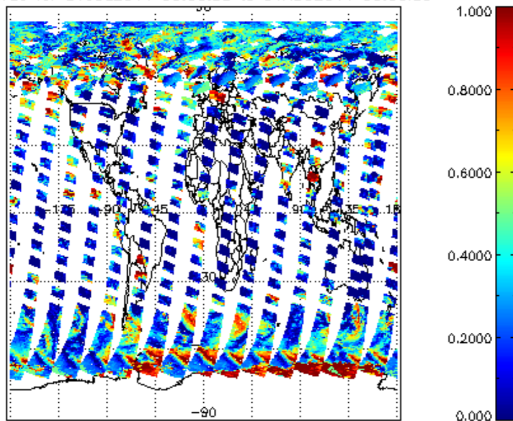
cl_frac for 31JUL2011 00:00:00 to 01AUG2011 00:00:00
