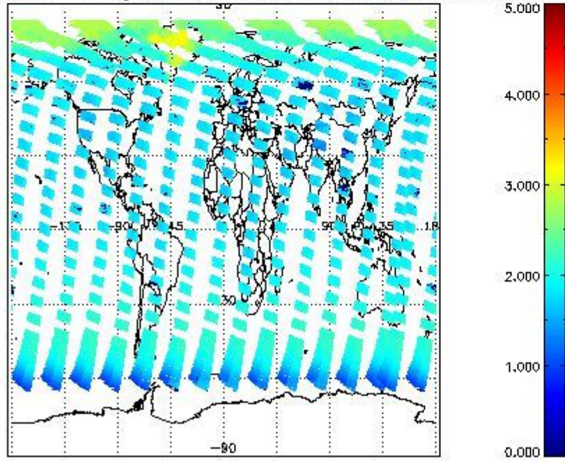
SCIOL2P_NADUV7S02_amf_gr for 31JUL2011 00:00:00 to 01AUG2011 00:00:00
