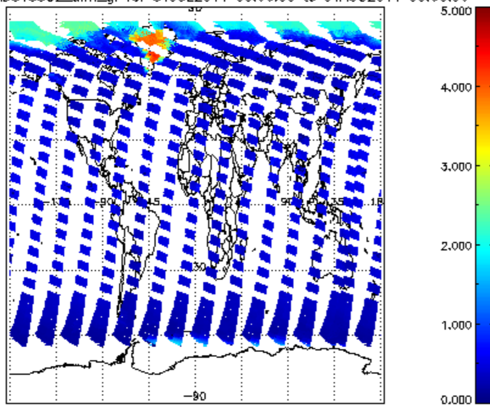
SCIOL2P_NADUV5S02_amf_gr for 31JUL2011 00:00:00 to 01AUG2011 00:00:00
