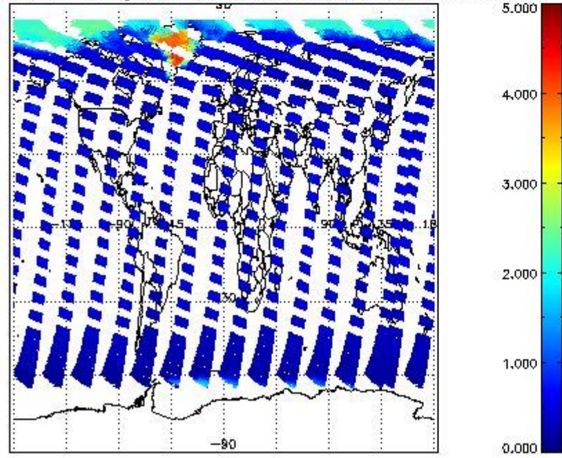
SCIOL2P_NADUV5S02_amf_gr for 31JUL2011 00:00:00 to 01AUG2011 00:00:00
