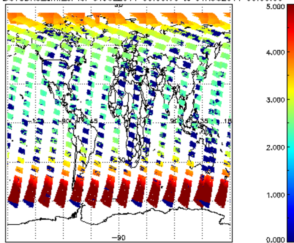
SCIOL2P_NADUV3BRO_amf_cl for 31JUL2011 00:00:00 to 01AUG2011 00:00:00
