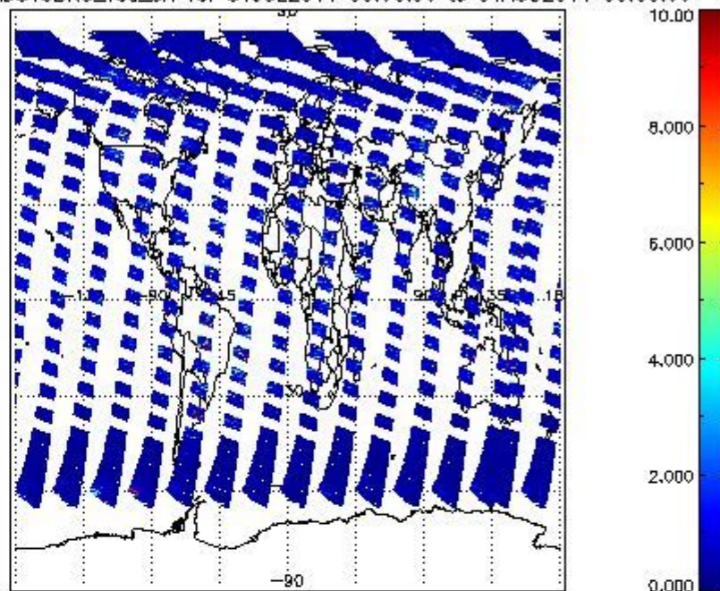
SCIOL2P_NADUV3BRO_vcd_err for 31JUL2011 00:00:00 to 01AUG2011 00:00:00
