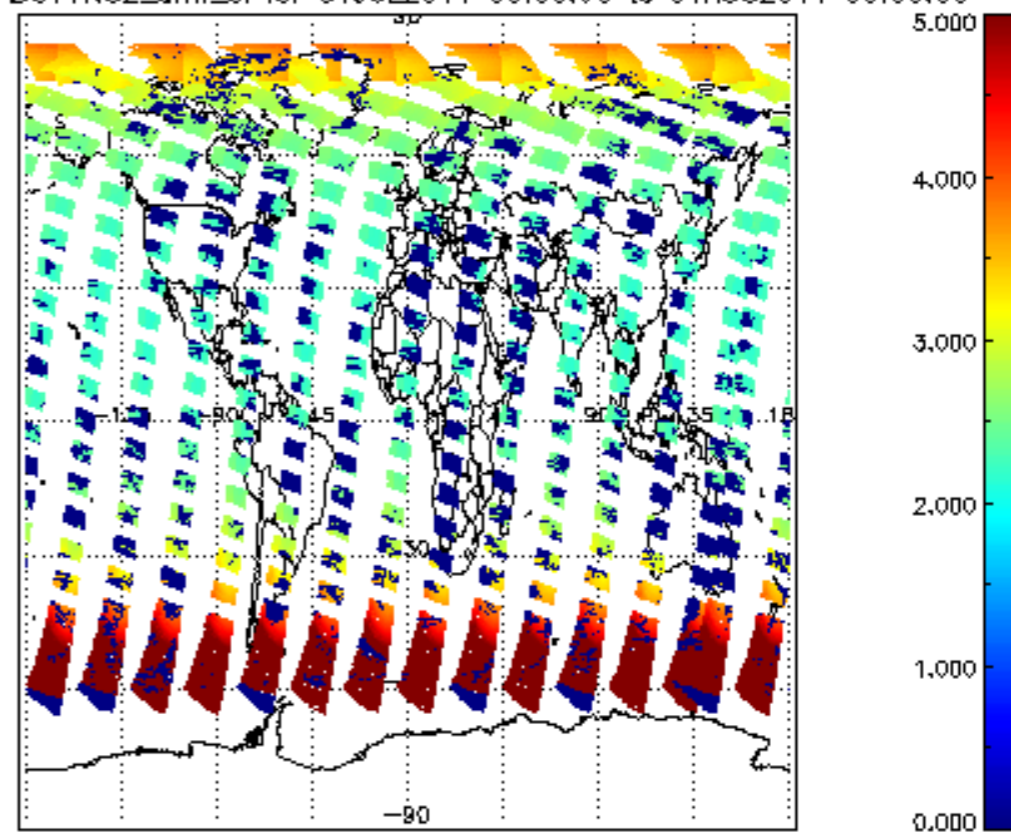
SCIOL2P_NADUV1N02_amf_cl for 31JUL2011 00:00:00 to 01AUG2011 00:00:00
