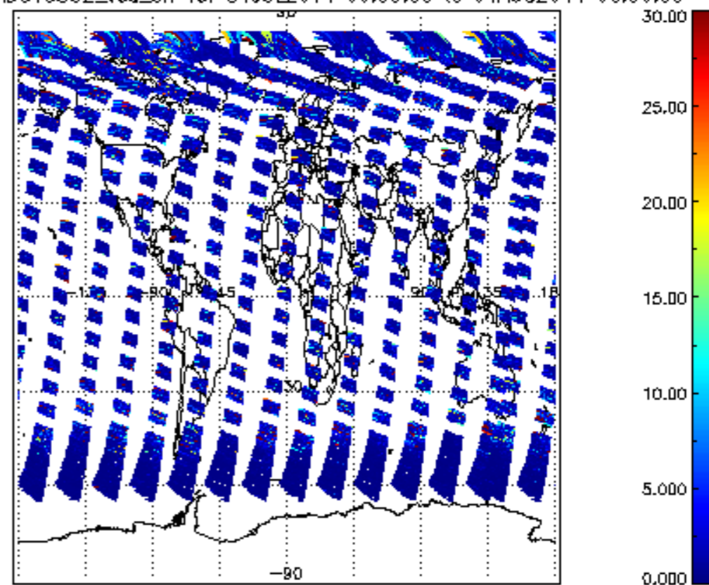
SCIOL2P_NADUV5S02_vcd_err for 31JUL2011 00:00:00 to 01AUG2011 00:00:00
