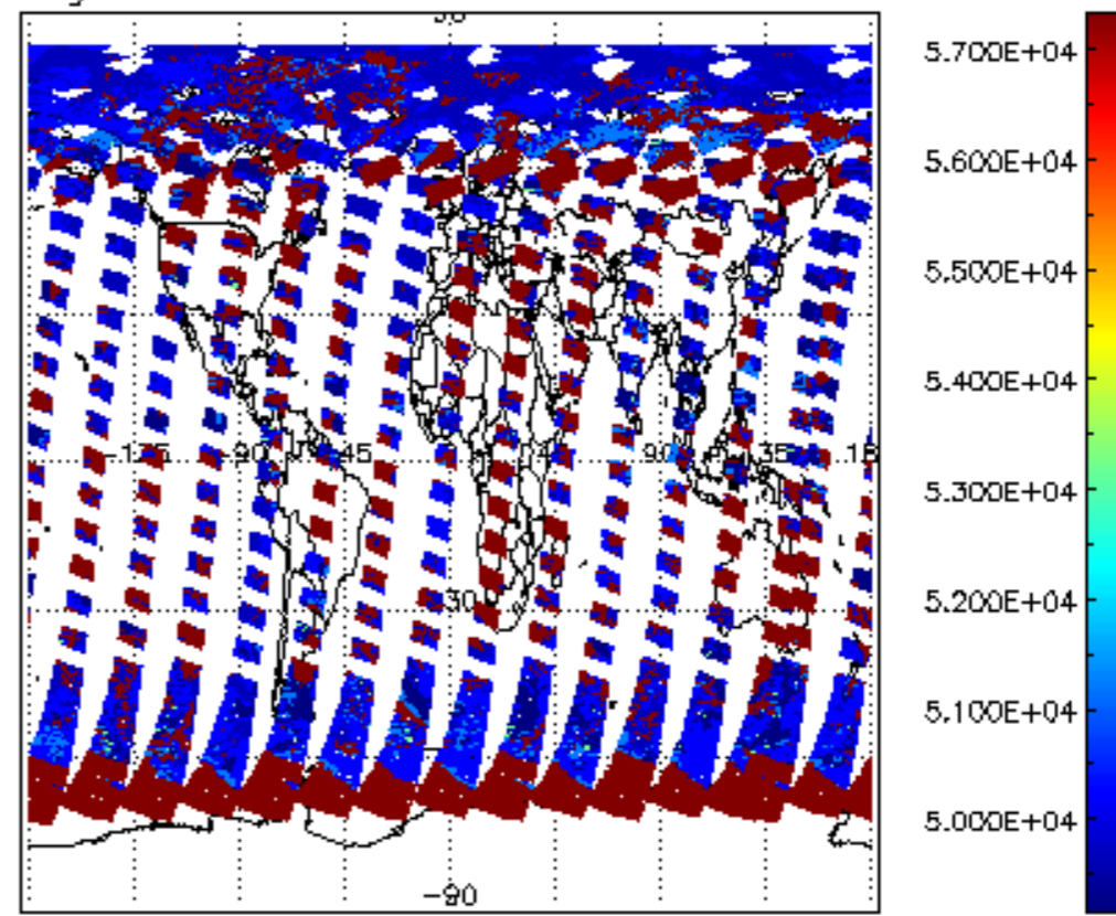
cloud_flags for 31JUL2011 00:00:00 to 01AUG2011 00:00:00
