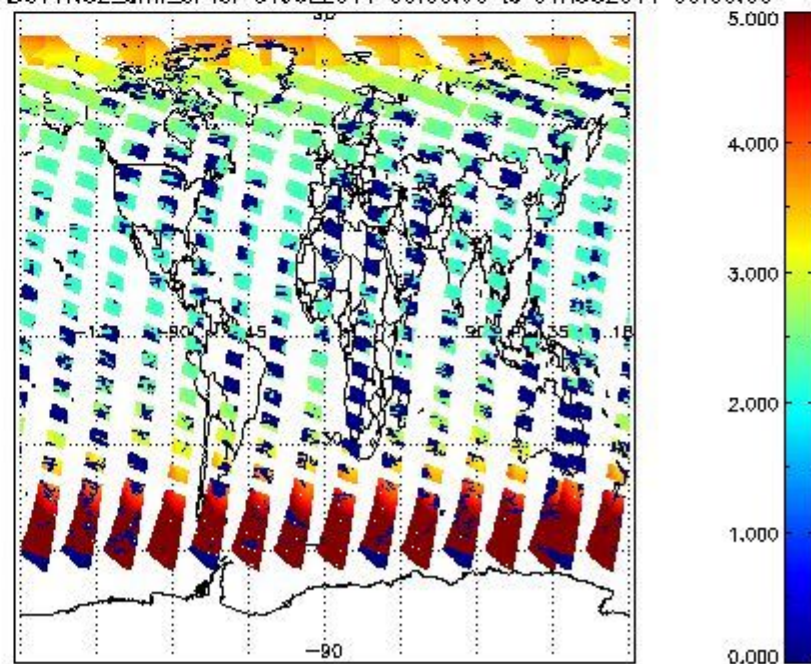
SCIOL2P_NADUV1N02_amf_cl for 31JUL2011 00:00:00 to 01AUG2011 00:00:00
