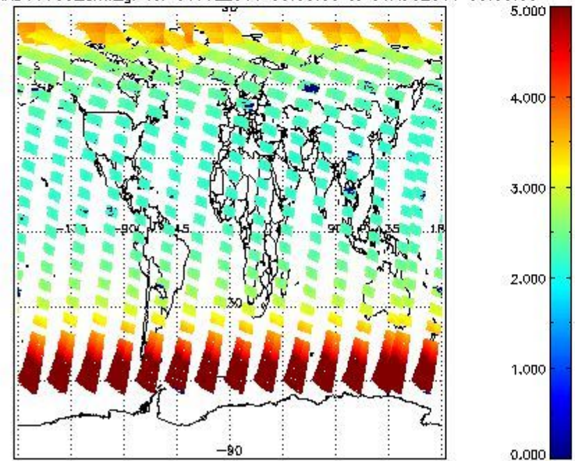
SCIOL2P_NADUV003_amf_gr for 31JUL2011 00:00:00 to 01AUG2011 00:00:00
