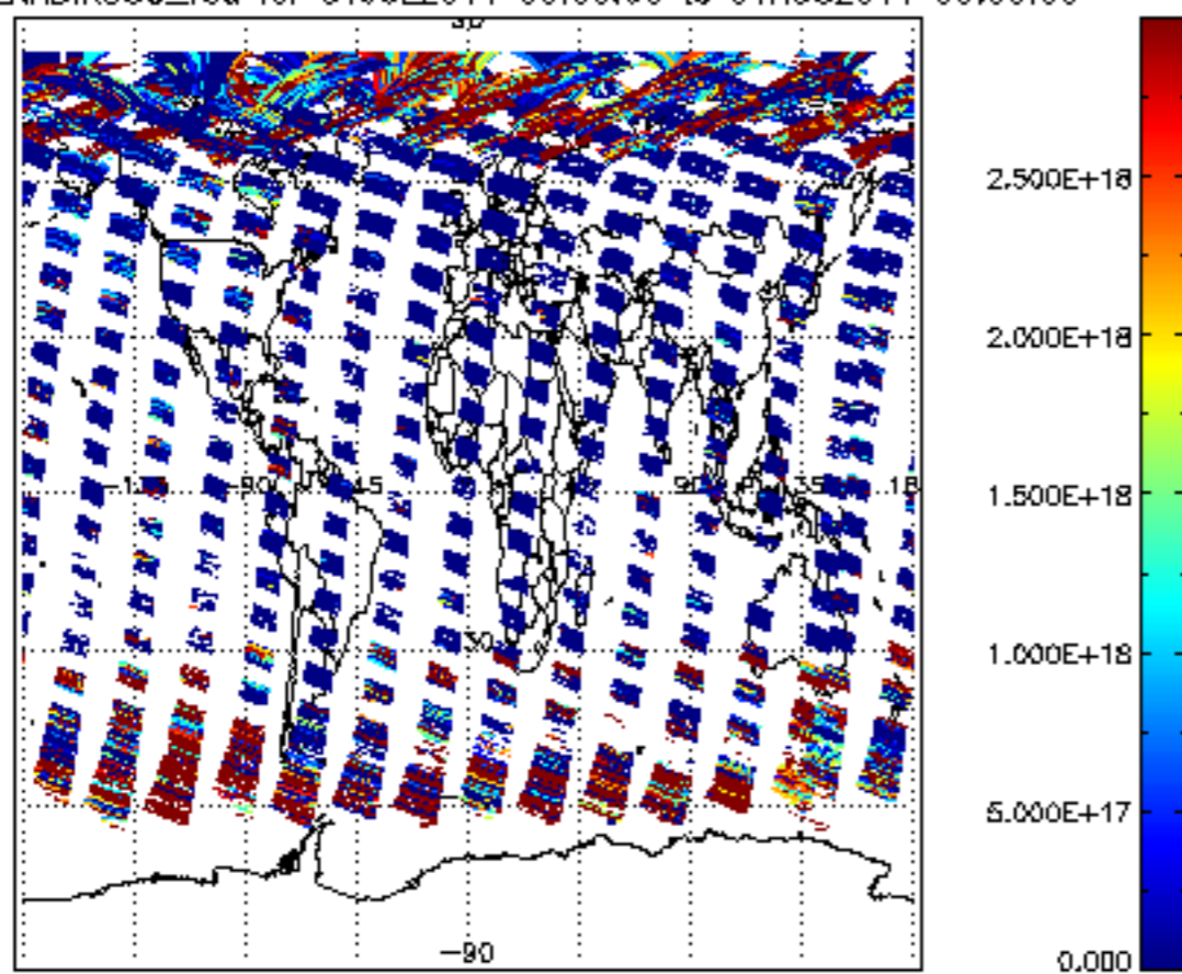
SCIOL2P_NADIR3CO_vcd for 31JUL2011 00:00:00 to 01AUG2011 00:00:00
