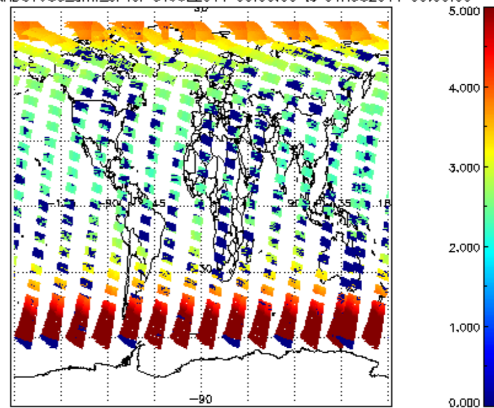
SCIOL2P_NADUV003_amf_cl for 31JUL2011 00:00:00 to 01AUG2011 00:00:00
