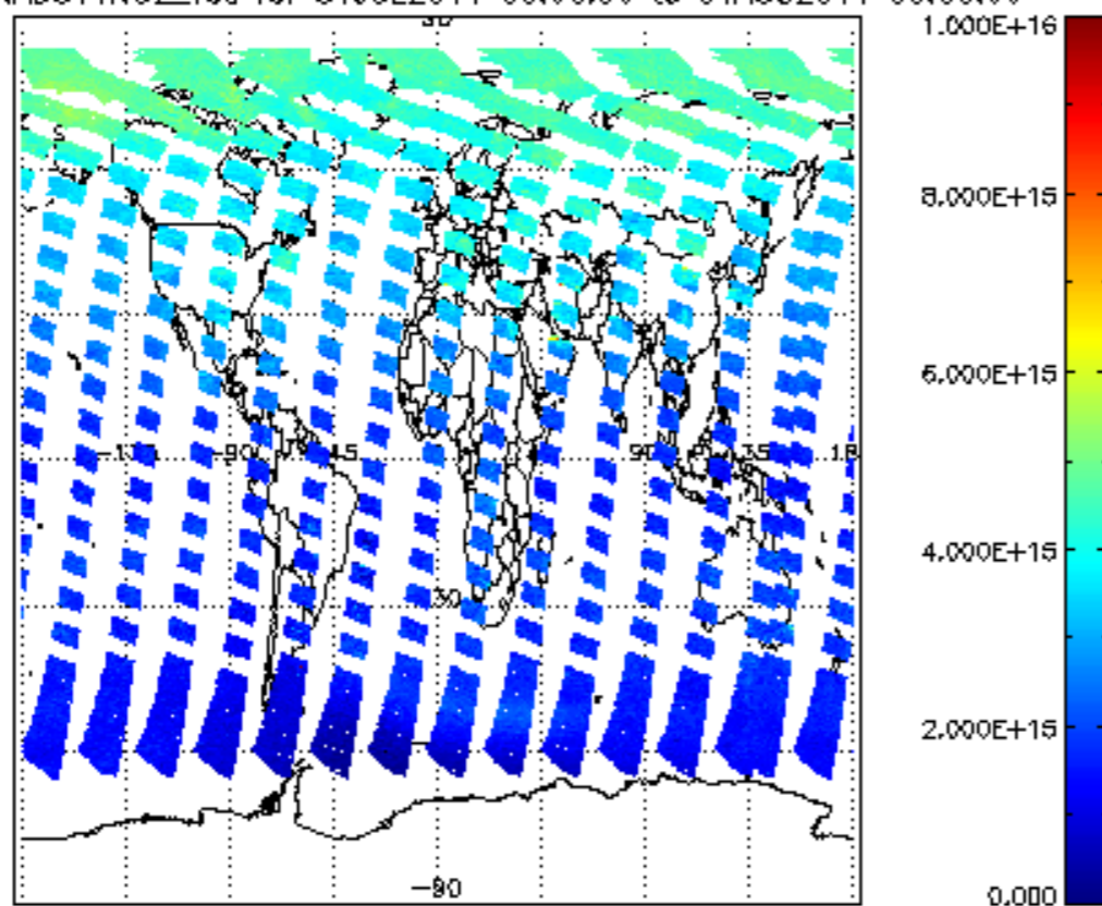
SCIOL2P_NADUV1N02_vcd for 31JUL2011 00:00:00 to 01AUG2011 00:00:00
