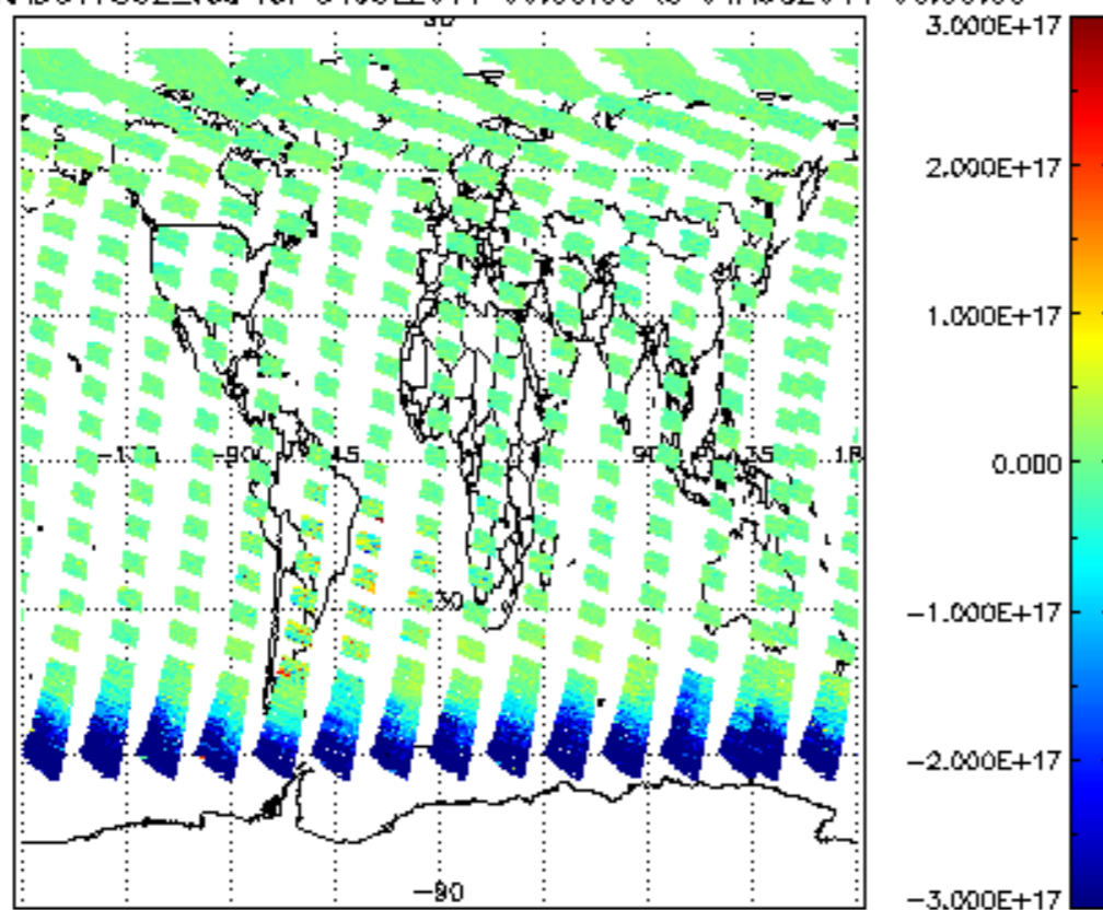
SCIOL2P_NADUV7S02_vcd for 31JUL2011 00:00:00 to 01AUG2011 00:00:00
