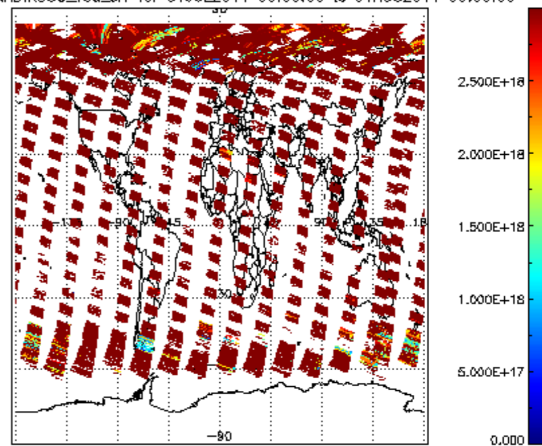
SCIOL2P_NADIR3CO_vcd_err for 31JUL2011 00:00:00 to 01AUG2011 00:00:00
