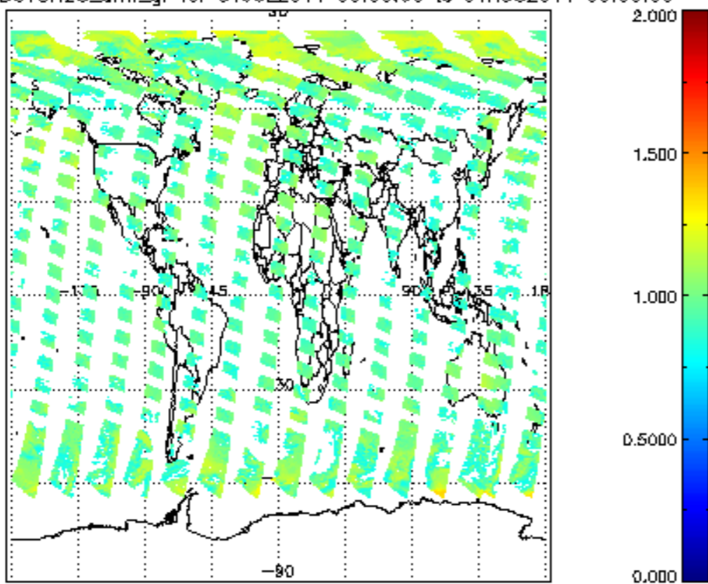
SCIOL2P_NADUV8H20_amf_gr for 31JUL2011 00:00:00 to 01AUG2011 00:00:00
