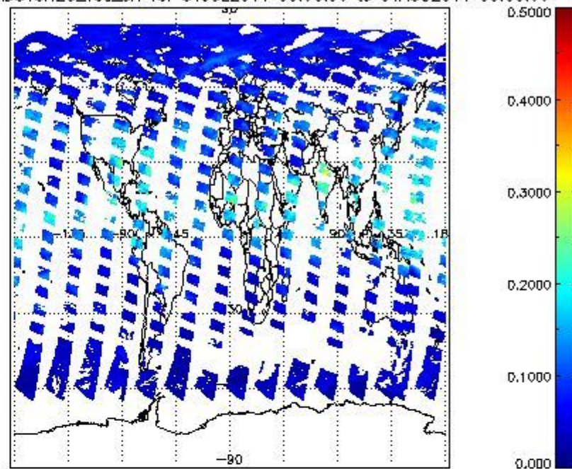
SCIOL2P_NADUV8H2O_vcd_err for 31JUL2011 00:00:00 to 01AUG2011 00:00:00
