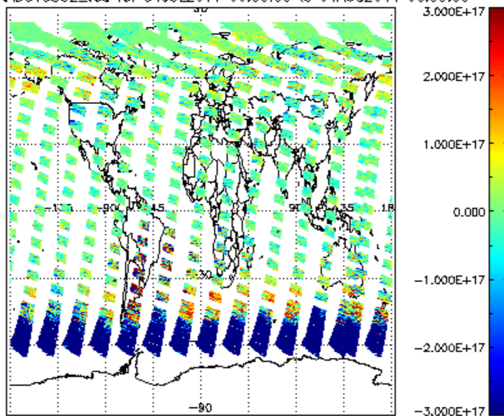
SCIOL2P_NADUV5S02_vcd for 31JUL2011 00:00:00 to 01AUG2011 00:00:00
