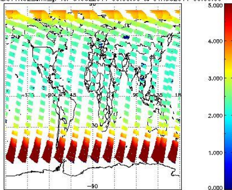
SCIOL2P_NADUV1N02_amf_gr for 31JUL2011 00:00:00 to 01AUG2011 00:00:00
