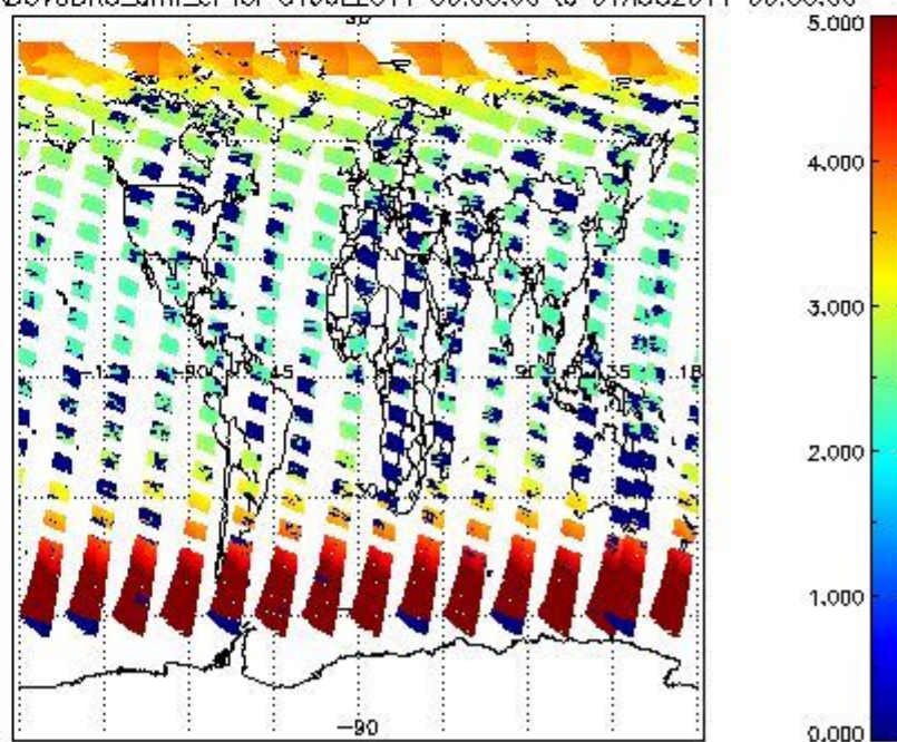
SCIOL2P_NADUV3BRO_amf_cl for 31JUL2011 00:00:00 to 01AUG2011 00:00:00
