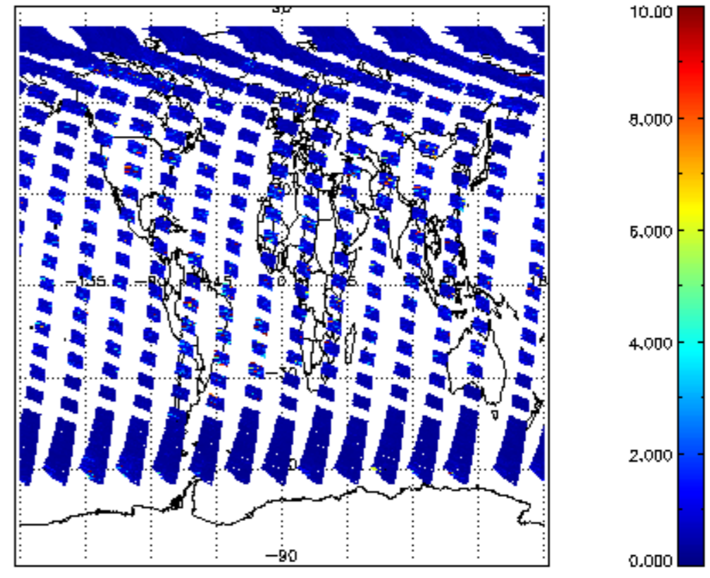
SCIOL2P_NADUV3BRO_vcd_err for 30JUL2011 00:00:00 to 31JUL2011 00:00:00
