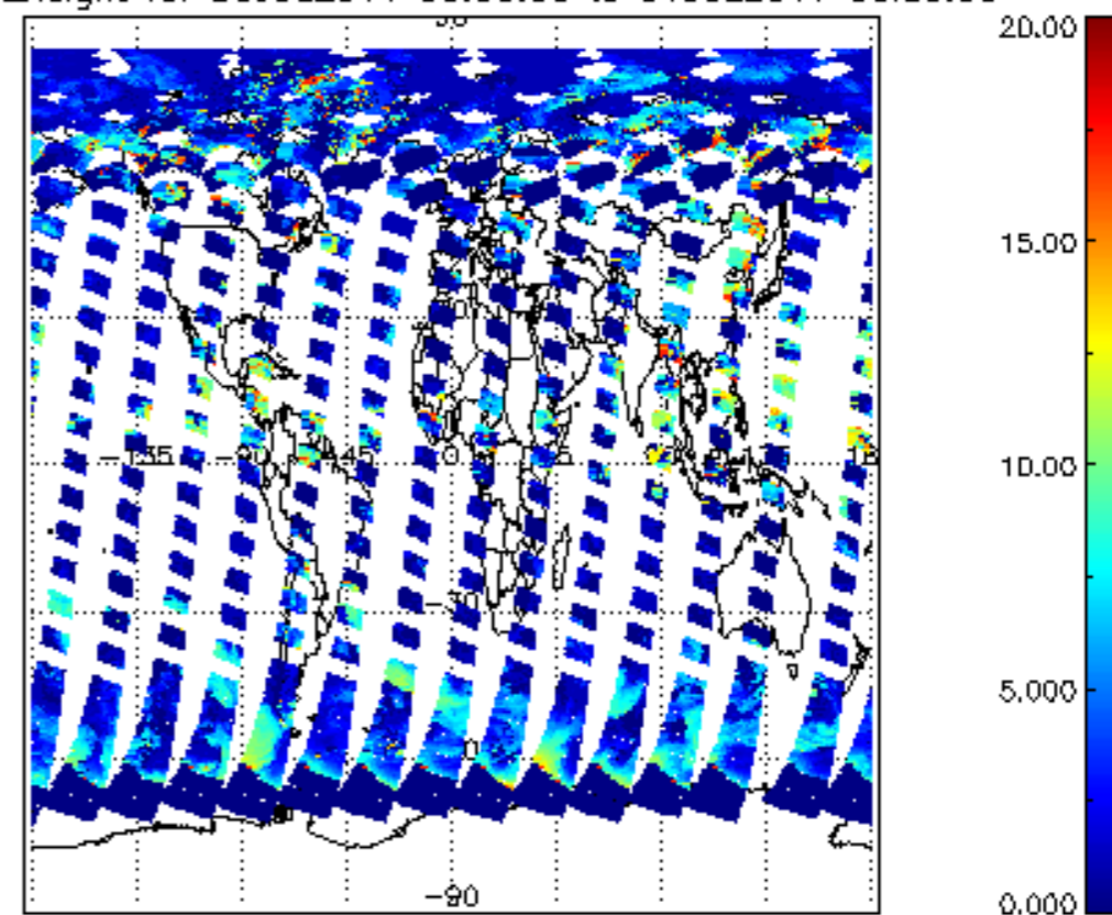
cl_top_height for 30JUL2011 00:00:00 to 31JUL2011 00:00:00
