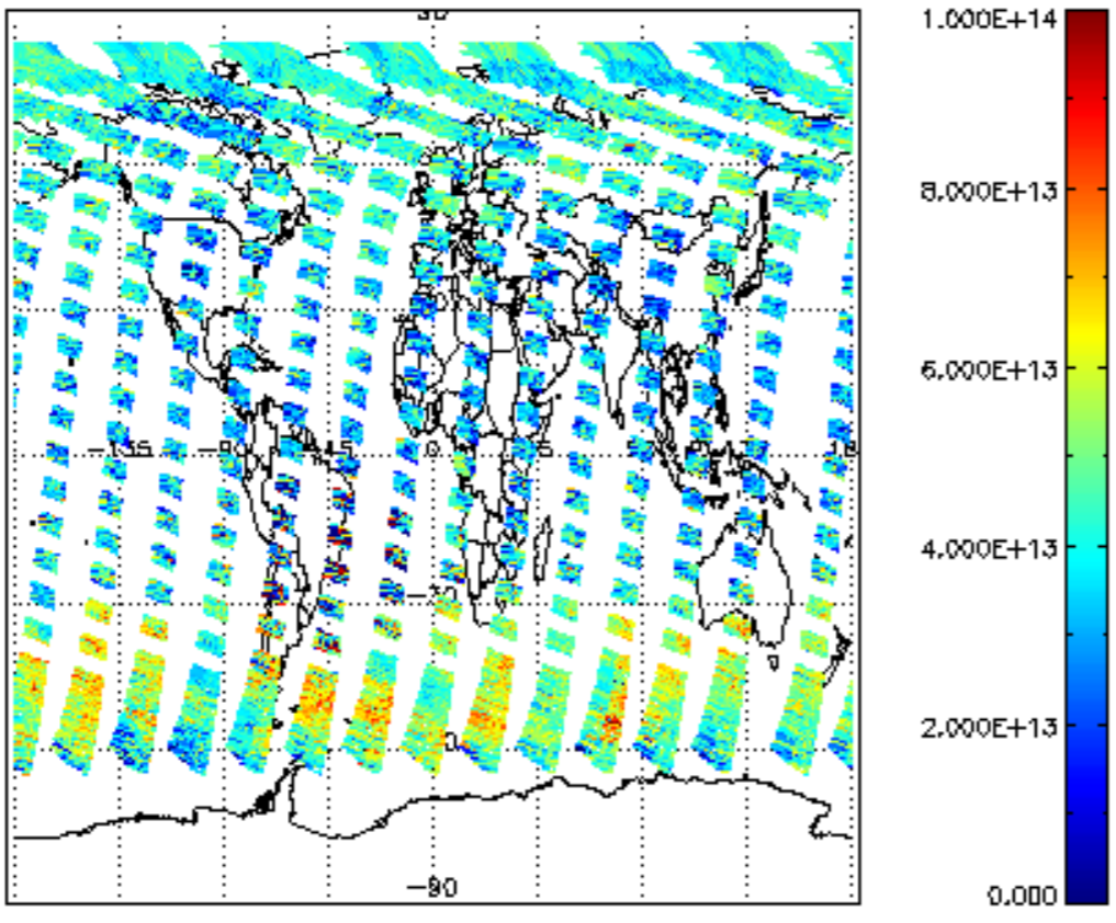
SCIOL2P_NADUV3BRO_vcd for 30JUL2011 00:00:00 to 31JUL2011 00:00:00
