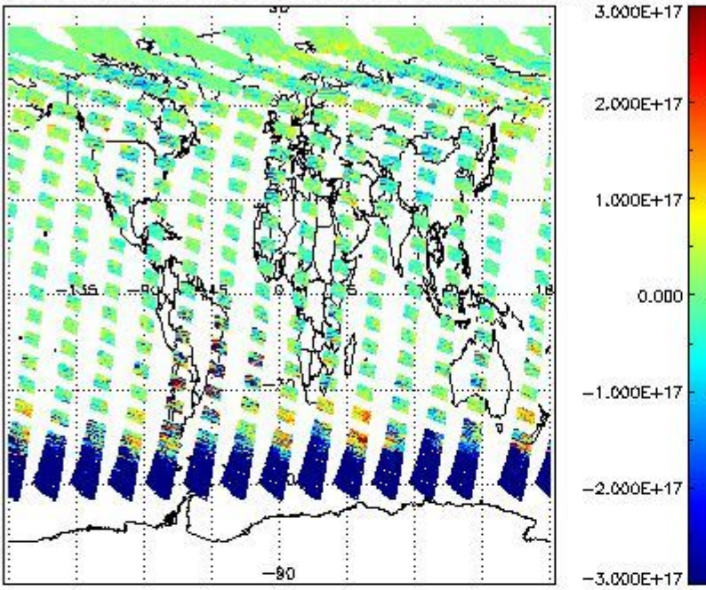
SCIOL2P_NADUV5S02_vcd for 30JUL2011 00:00:00 to 31JUL2011 00:00:00
