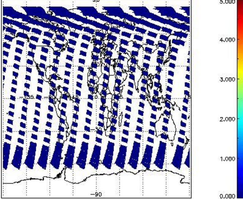
SCIOL2P_NADUV5S02_amf_cl for 30JUL2011 00:00:00 to 31JUL2011 00:00:00
