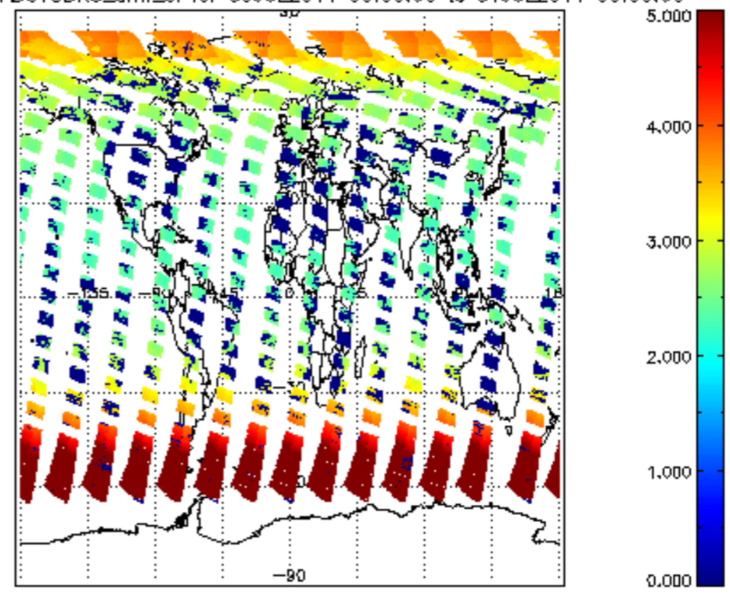
SCIOL2P_NADUV3BRO_arnf_cl for 30JUL2011 00:00:00 to 31JUL2011 00:00:00
