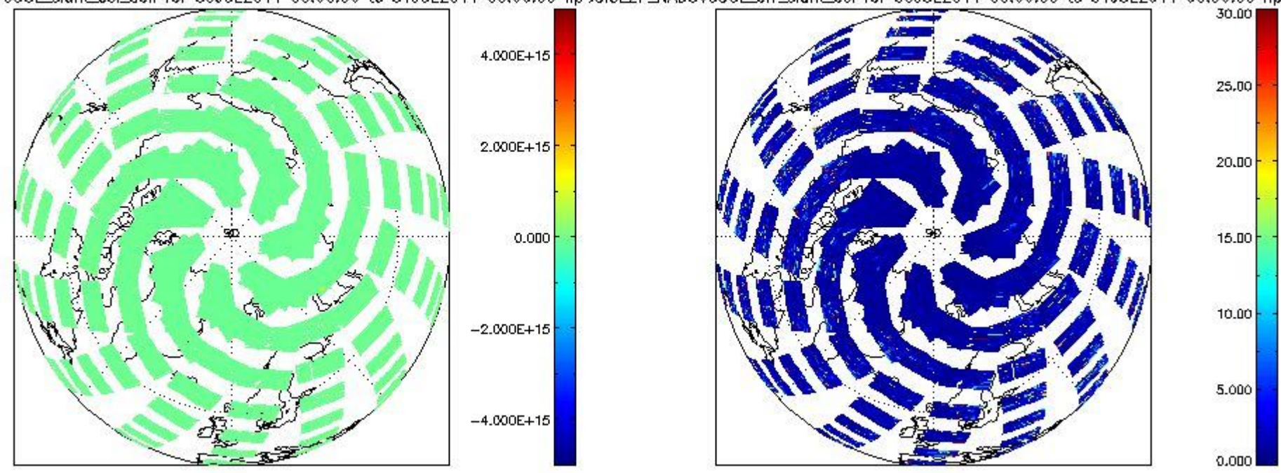
SCIOI2P_NADUV6OCLslant_col_den for 30JUL2011 00:00:00 to 31JUL2011 00:00:00 np SCIOI2P_NADUV6OCLarr_slant_col for 30JUL2011 00:00:00 to 31JUL2011 00:00:00 np
