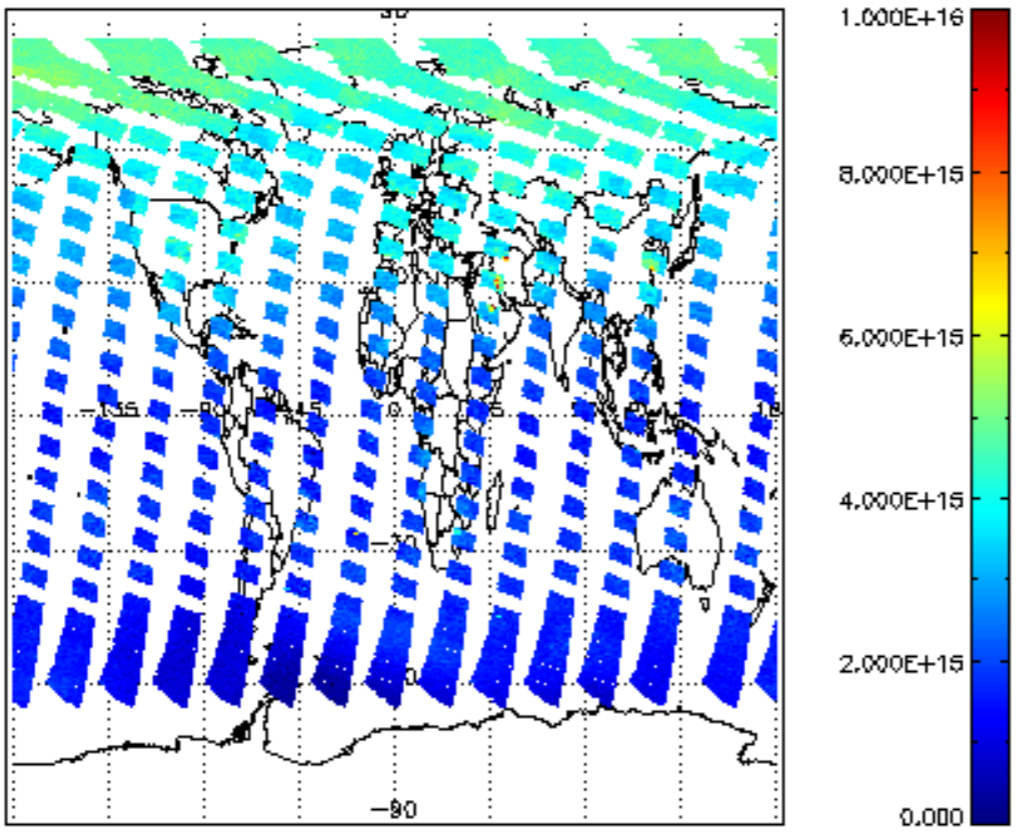
SCIOL2P_NADUV1N02_vcd for 30JUL2011 00:00:00 to 31JUL2011 00:00:00
