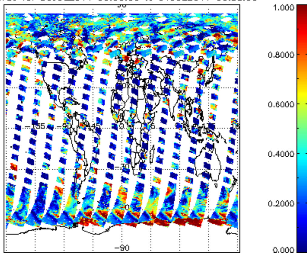
cl_frac for 30JUL2011 00:00:00 to 31JUL2011 00:00:00
