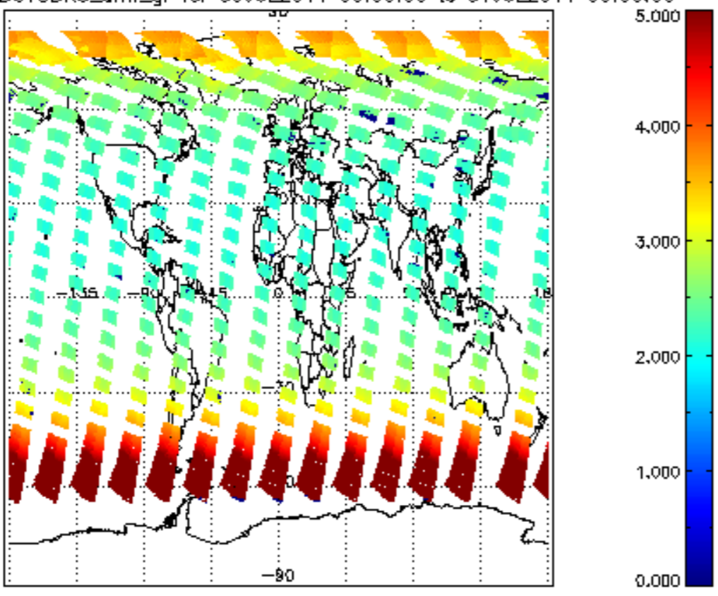
SCIOL2P_NADUV3BRO_arnf_gr for 30JUL2011 00:00:00 to 31JUL2011 00:00:00
