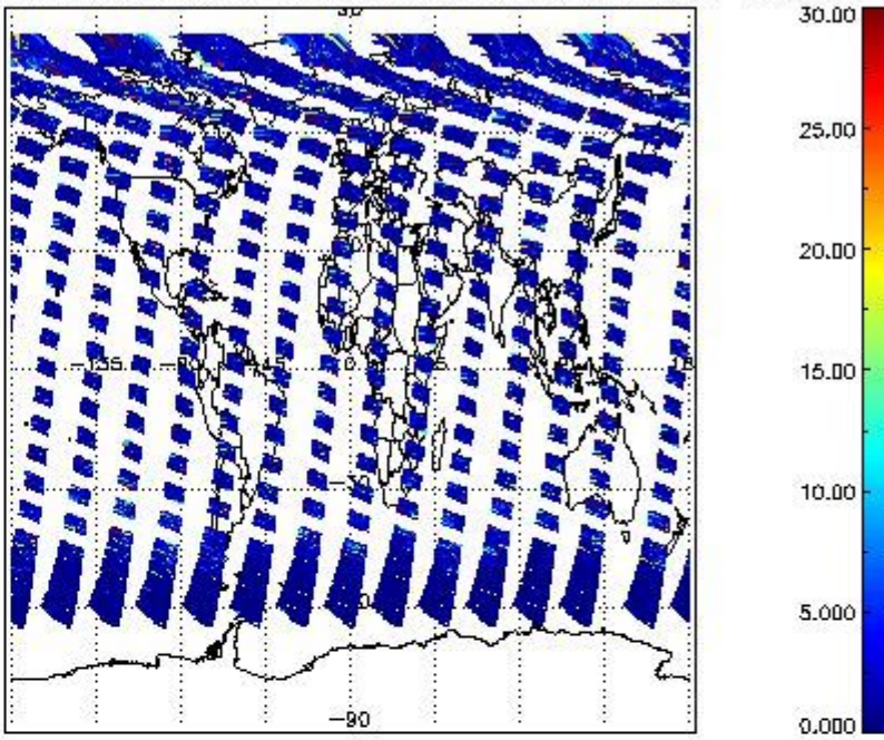
SCIOL2P_NADUV5S02_vcd_err for 30JUL2011 00:00:00 to 31JUL2011 00:00:00
