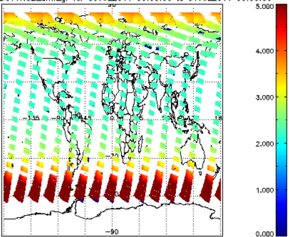
SCIOL2P_NADUV1N02_amf_gr for 30JUL2011 00:00:00 to 31JUL2011 00:00:00
