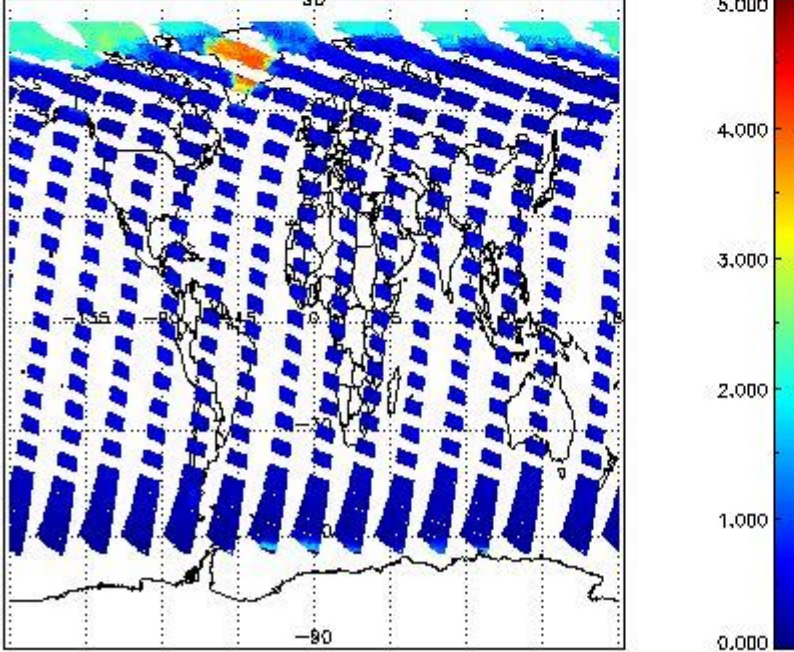
SCIOL2P_NADUV5S02_amf_gr for 30JUL2011 00:00:00 to 31JUL2011 00:00:00
