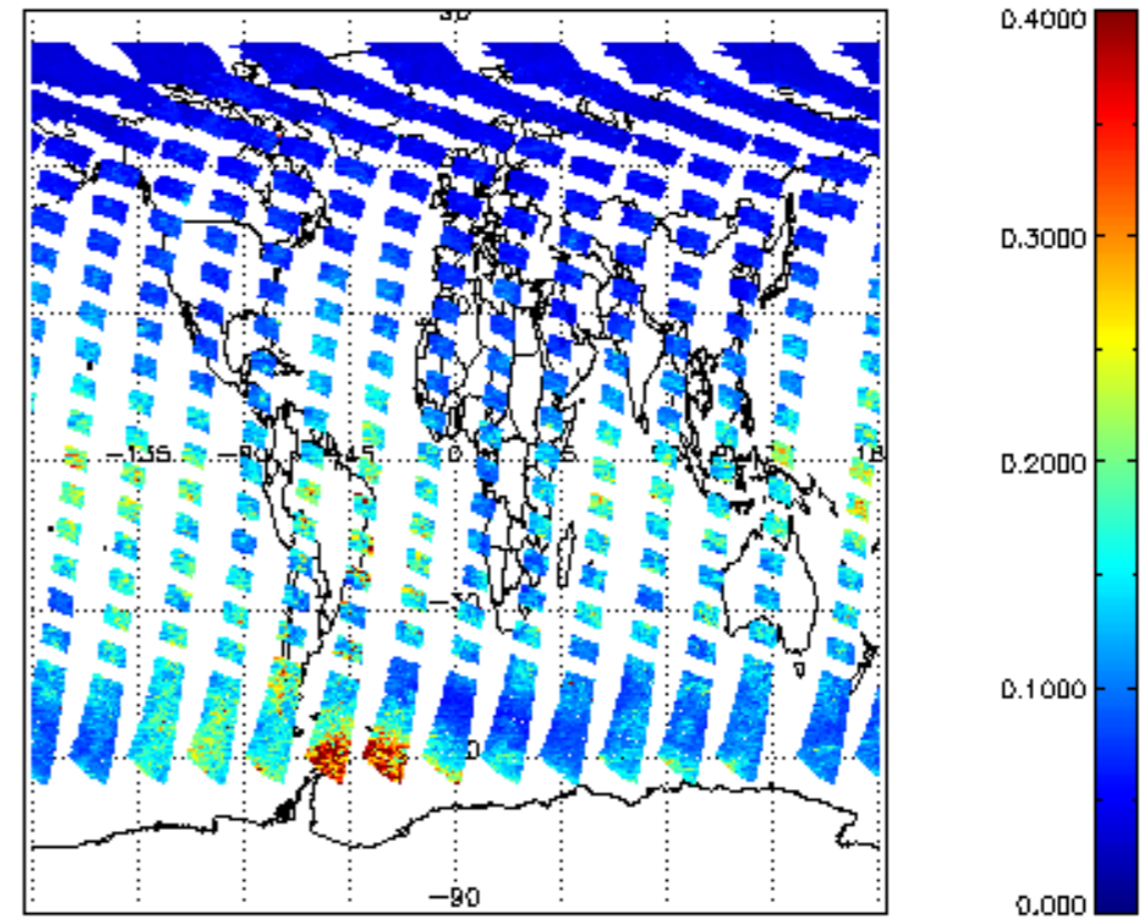
SCIOL2P_NADUV1N02_vcd_err for 30JUL2011 00:00:00 to 31JUL2011 00:00:00
