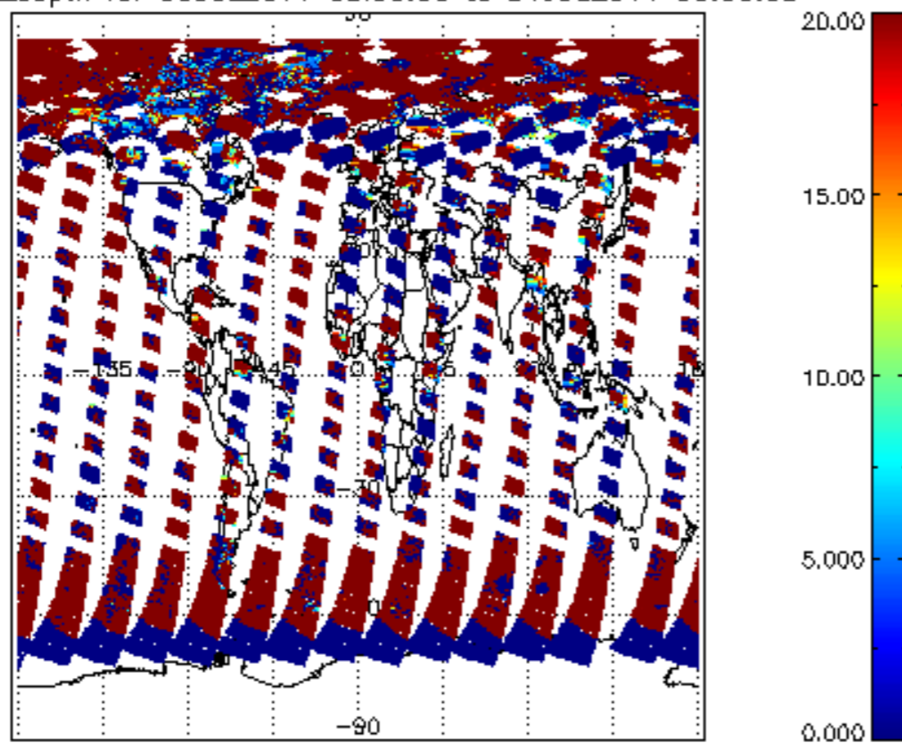
cl_lopt_depth for 30JUL2011 00:00:00 to 31JUL2011 00:00:00
