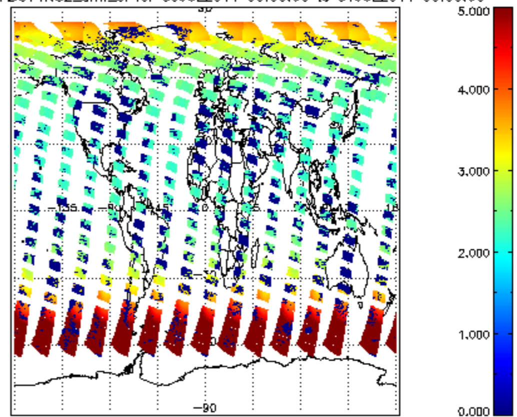
SCIOL2P_NADUV1N02_amf_cl for 30JUL2011 00:00:00 to 31JUL2011 00:00:00
