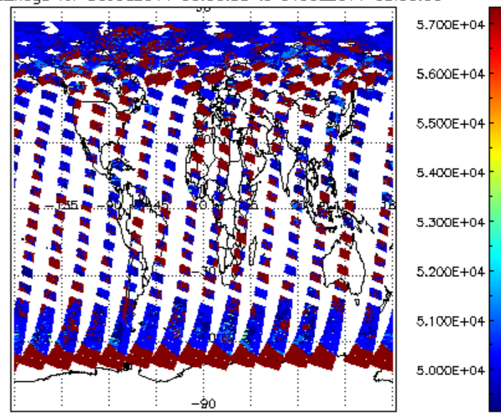
cloud_flags for 30JUL2011 00:00:00 to 31JUL2011 00:00:00
