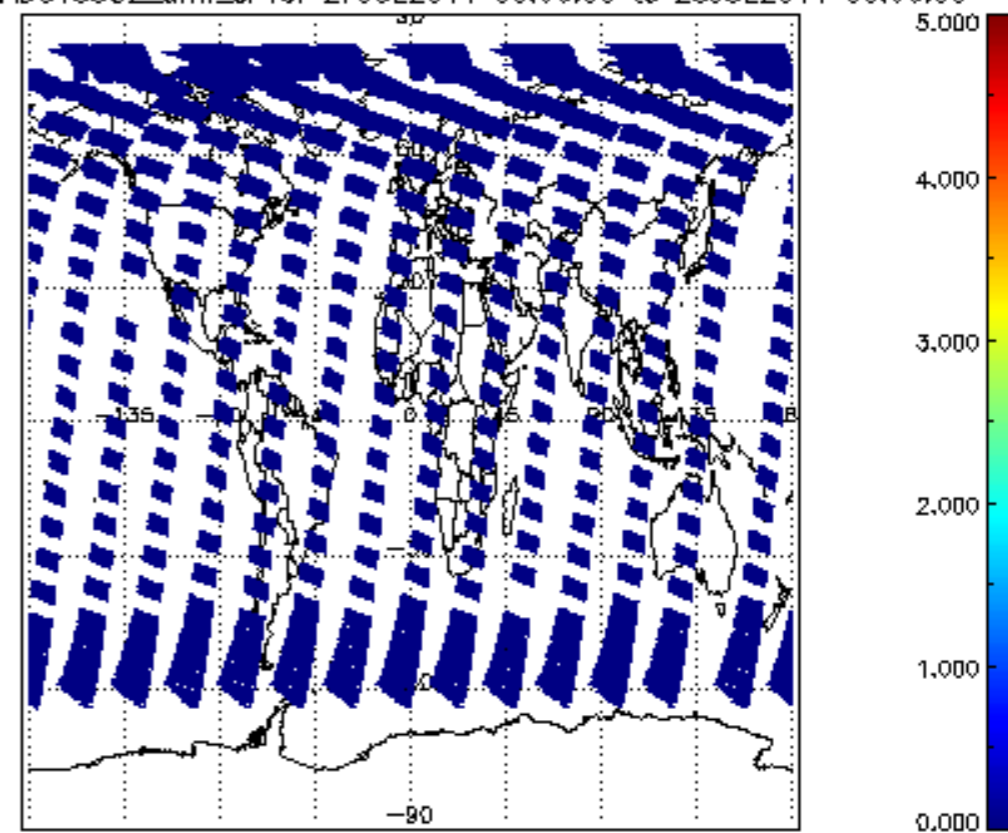
SCIOL2P_NADUV5S02_amf_cl for 27JUL2011 00:00:00 to 28JUL2011 00:00:00
