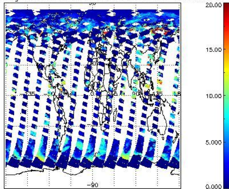
cL_top_height for 27JUL2011 00:00:00 to 28JUL2011 00:00:00
