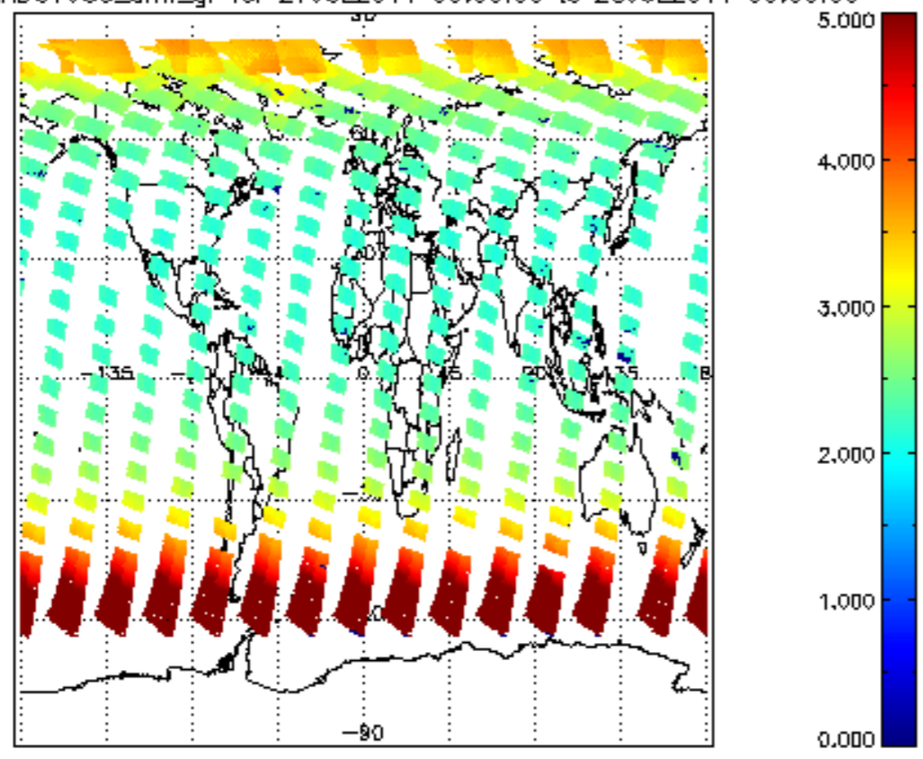
SCIOL2P_NADUV003_amf_gr for 27JUL2011 00:00:00 to 28JUL2011 00:00:00
