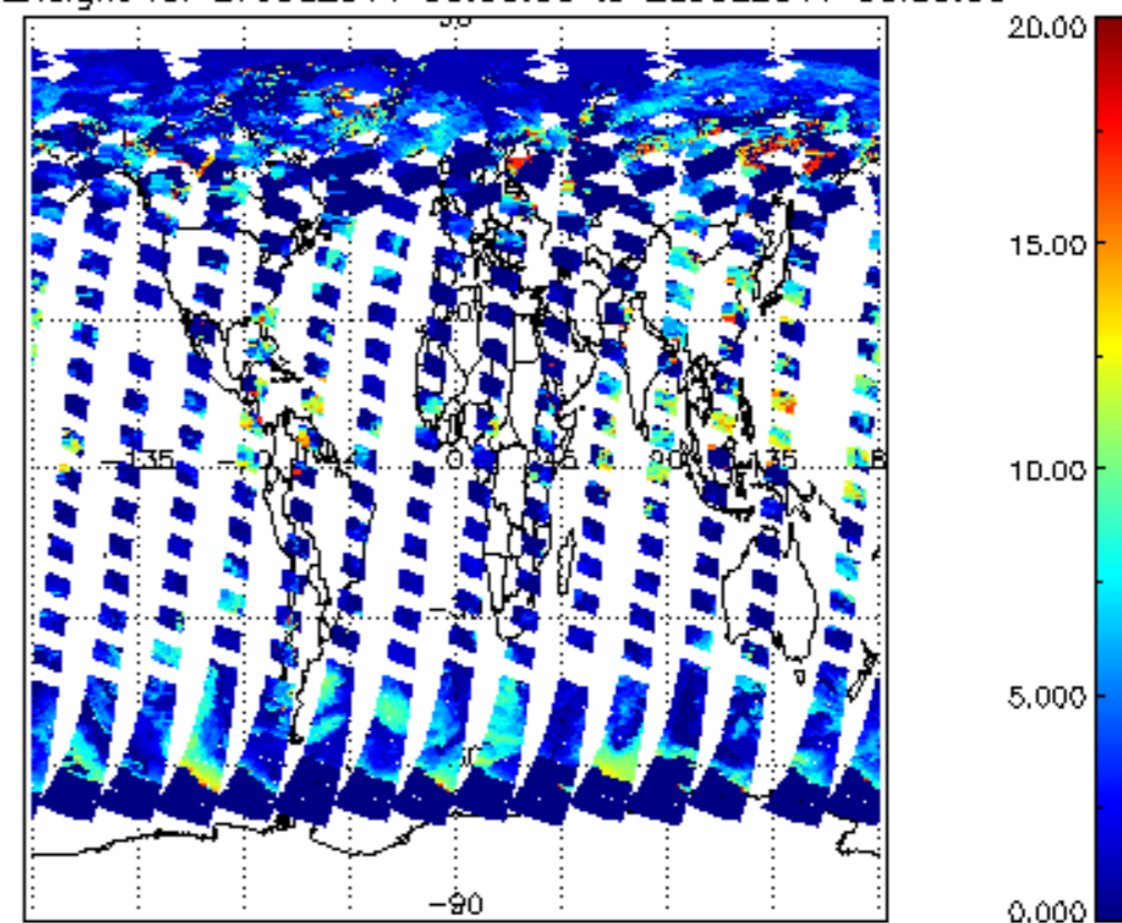
cl_top_height for 27JUL2011 00:00:00 to 28JUL2011 00:00:00
