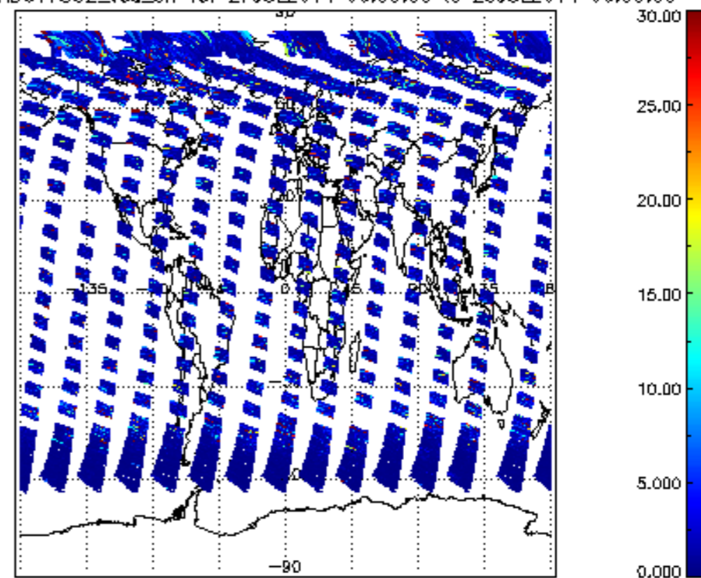
SCIOL2P_NADUV7S02_vcd_err for 27JUL2011 00:00:00 to 28JUL2011 00:00:00
