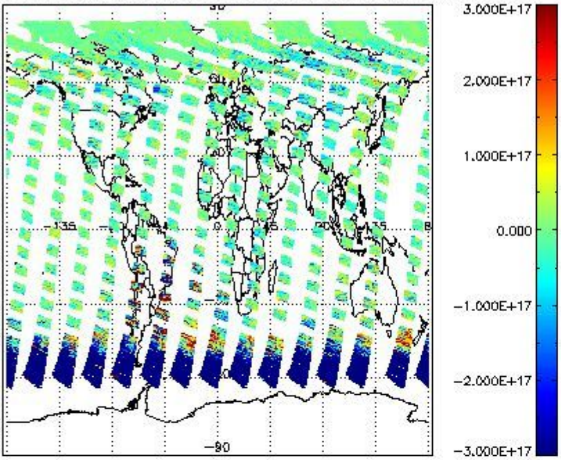
SCIOL2P_NADUV5S02_vcd for 27JUL2011 00:00:00 to 28JUL2011 00:00:00
