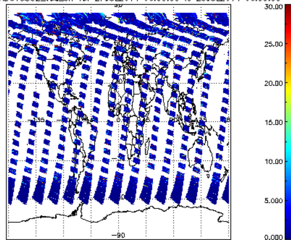
SCIOL2P_NADUV5S02_vcd_err for 27JUL2011 00:00:00 to 28JUL2011 00:00:00
