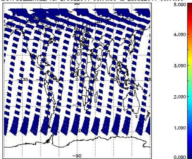
SCIOL2P_NADUV7S02_amf_cl for 27JUL2011 00:00:00 to 28JUL2011 00:00:00
