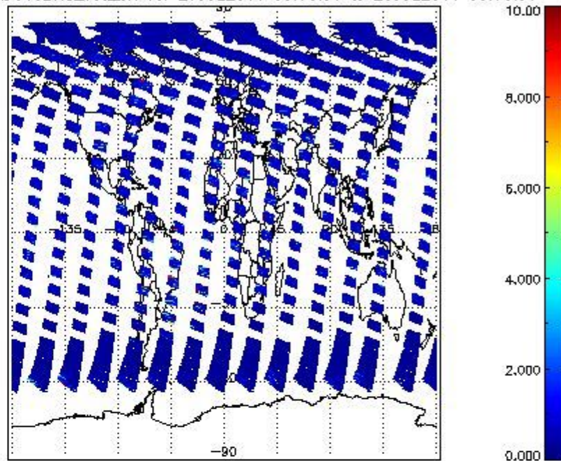
SCIOL2P_NADUV3BRO_vcd_err for 27JUL2011 00:00:00 to 28JUL2011 00:00:00
