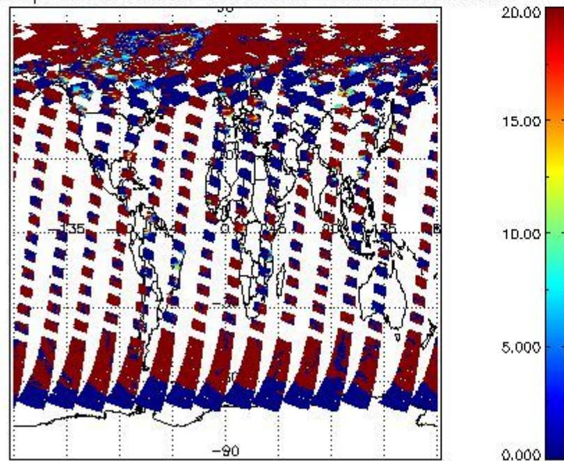
cL_opt_depth for 27JUL2011 00:00:00 to 28JUL2011 00:00:00
