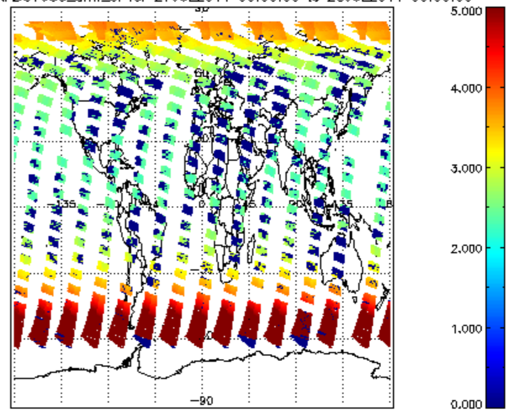
SCIOL2P_NADUV003_amf_cl for 27JUL2011 00:00:00 to 28JUL2011 00:00:00
