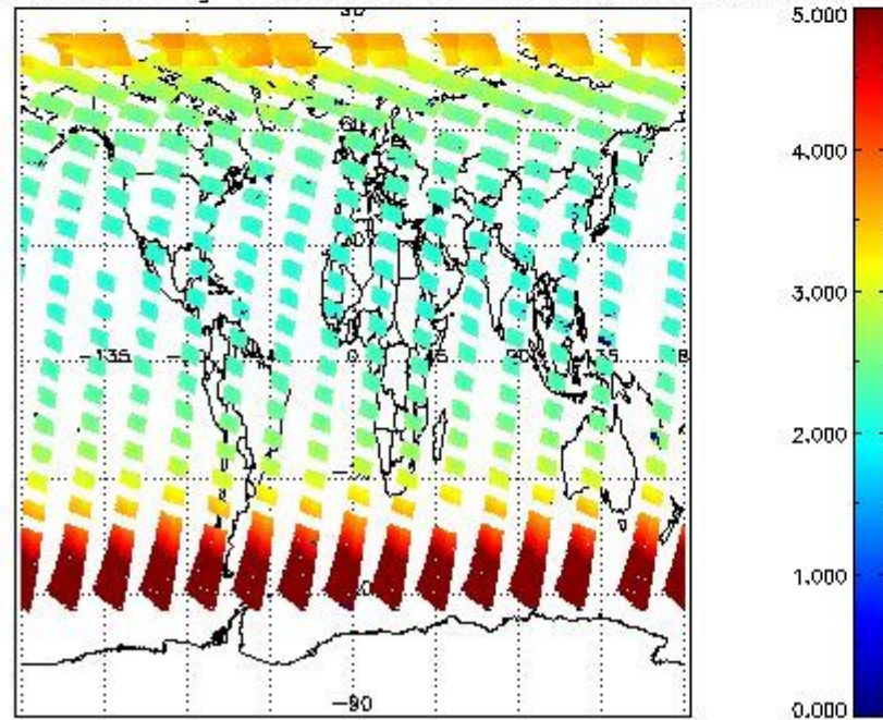
SCIOL2P_NADUV3BRO_amf_gr for 27JUL2011 00:00:00 to 28JUL2011 00:00:00
