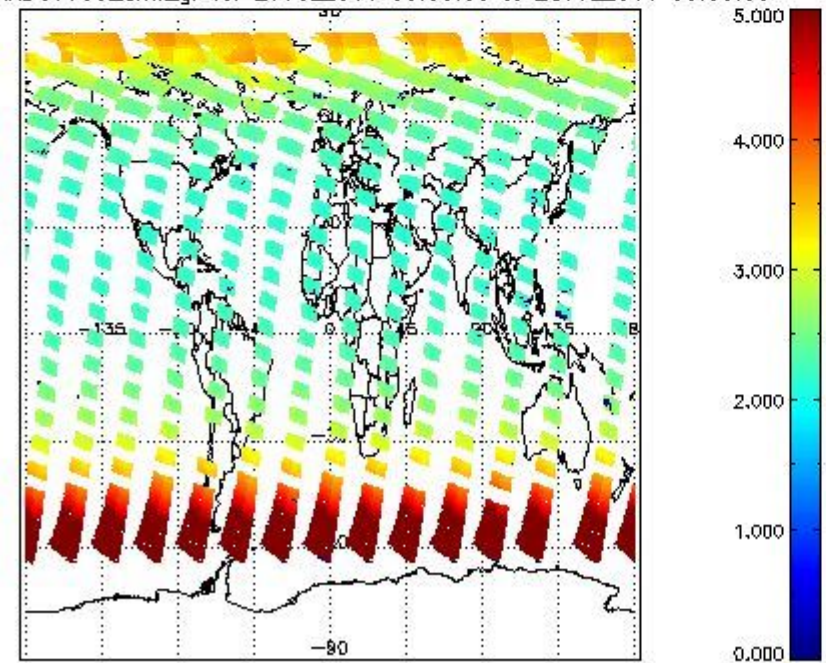
SCIOL2P_NADUV003_amf_gr for 27JUL2011 00:00:00 to 28JUL2011 00:00:00
