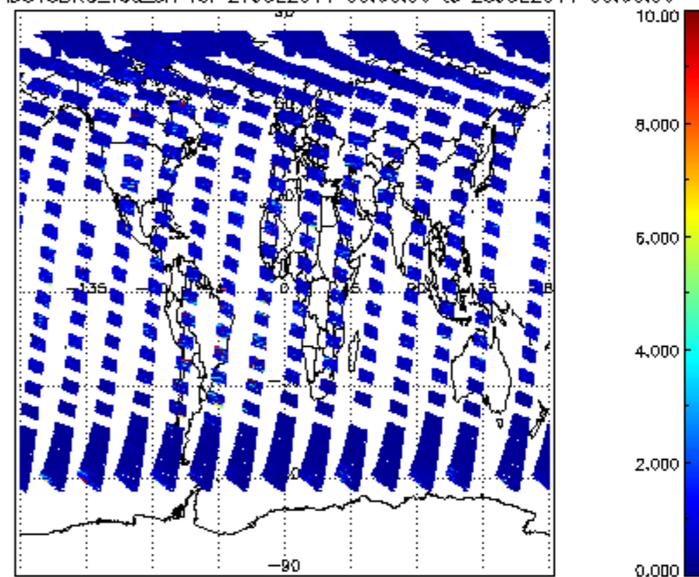
SCIOL2P_NADUV3BRO_vcd_err for 27JUL2011 00:00:00 to 28JUL2011 00:00:00
