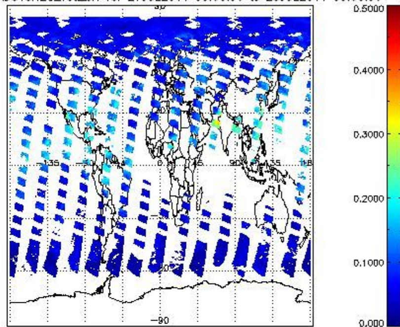
SCIOL2P_NADUV8H2O_vcd_err for 27JUL2011 00:00:00 to 28JUL2011 00:00:00
