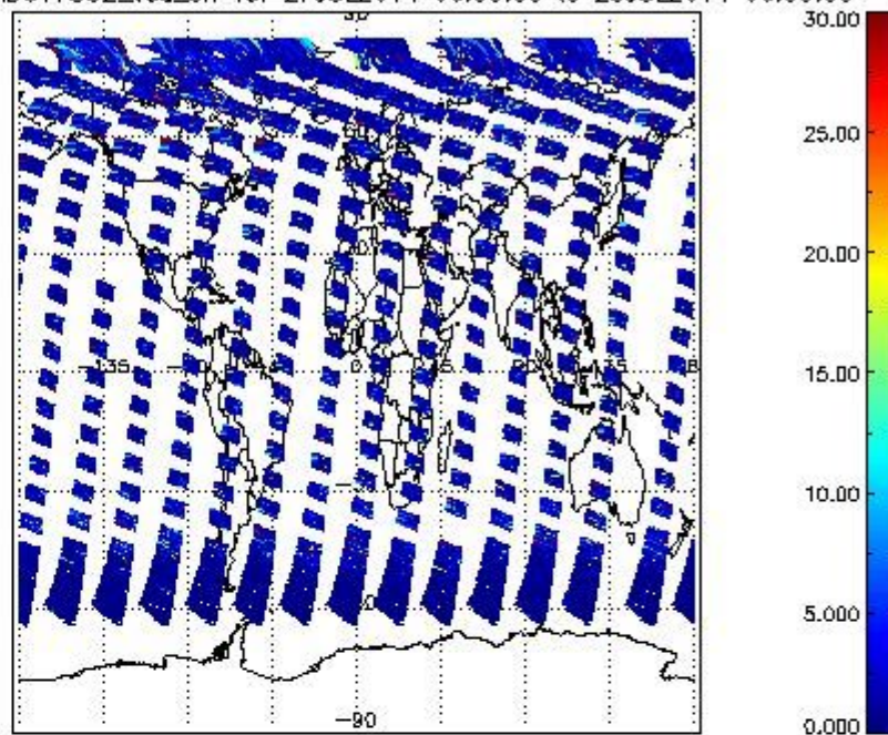
SCIOL2P_NADUV7S02_vcd_err for 27JUL2011 00:00:00 to 28JUL2011 00:00:00
