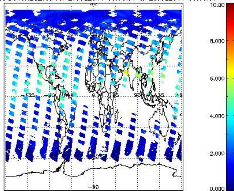
SCIOL2P_NADUV8H2O_vcd for 27JUL2011 00:00:00 to 28JUL2011 00:00:00
