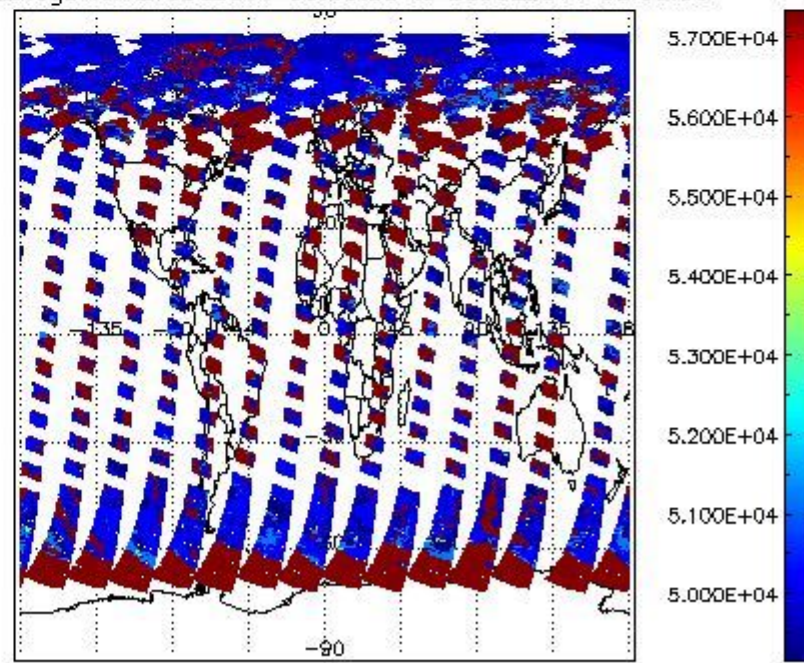
cloud_flags for 27JUL2011 00:00:00 to 28JUL2011 00:00:00
