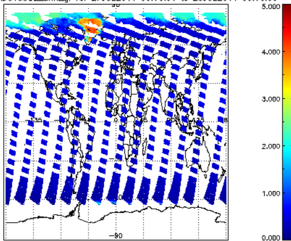
SCIOL2P_NADUV5S02_amf_gr for 27JUL2011 00:00:00 to 28JUL2011 00:00:00
