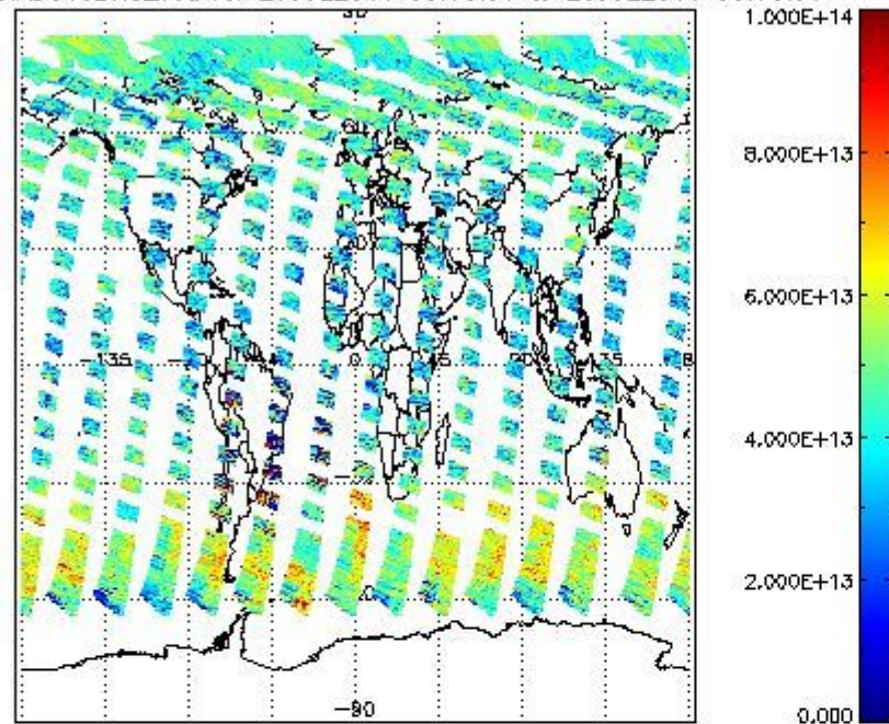
SCIOL2P_NADUV3BRO_vcd for 27JUL2011 00:00:00 to 28JUL2011 00:00:00
