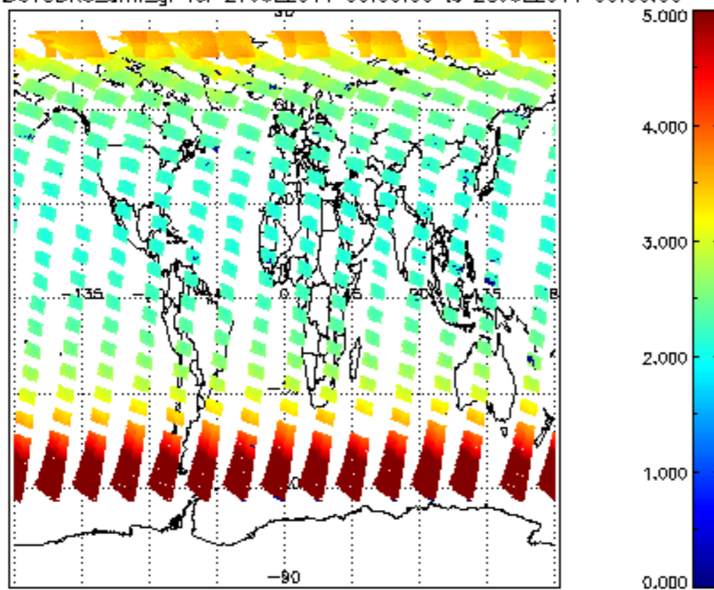
SCIOL2P_NADUV3BRO_amf_gr for 27JUL2011 00:00:00 to 28JUL2011 00:00:00
