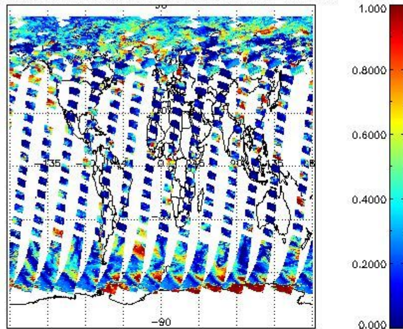
cL_frac for 27JUL2011 00:00:00 to 28JUL2011 00:00:00
