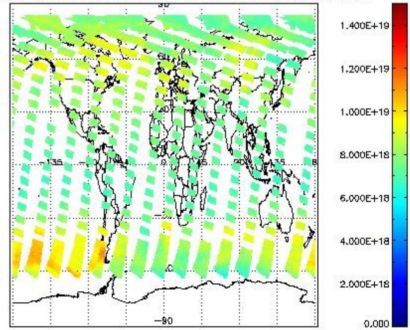
SCIOL2P_NADUV003_vcd for 27JUL2011 00:00:00 to 28JUL2011 00:00:00
