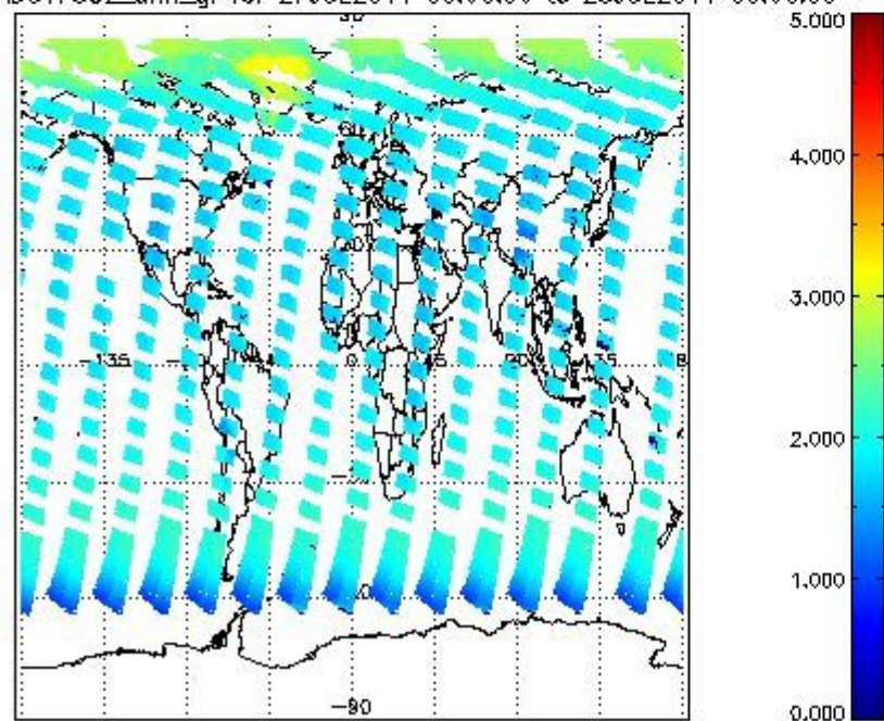
SCIOL2P_NADUV7S02_amf_gr for 27JUL2011 00:00:00 to 28JUL2011 00:00:00
