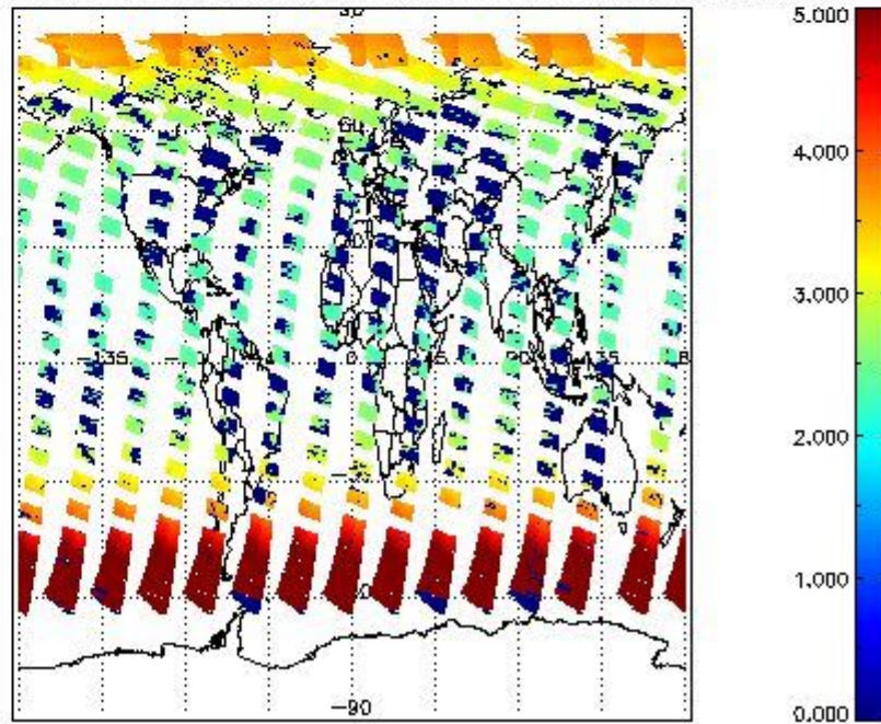
SCIOL2P_NADUV3BRO_amf_cl for 27JUL2011 00:00:00 to 28JUL2011 00:00:00
