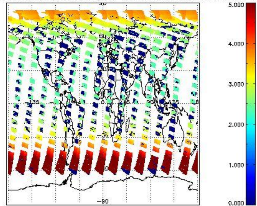
SCIOL2P_NADUV003_amf_cl for 27JUL2011 00:00:00 to 28JUL2011 00:00:00
