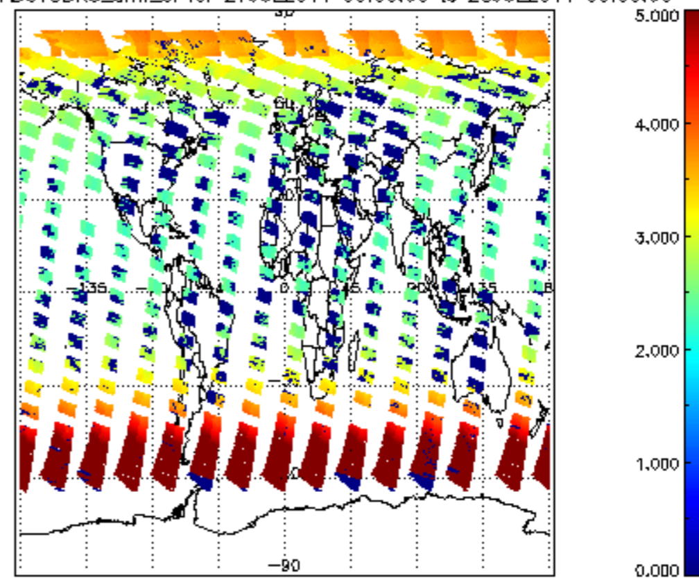
SCIOL2P_NADUV3BRO_amf_cl for 27JUL2011 00:00:00 to 28JUL2011 00:00:00
