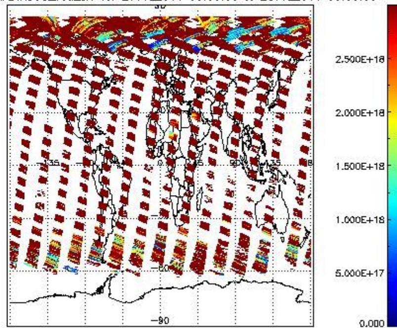
SCIDL2P_NADIR3CO_vcd_err for 27JUL2011 00:00:00 to 28JUL2011 00:00:00
