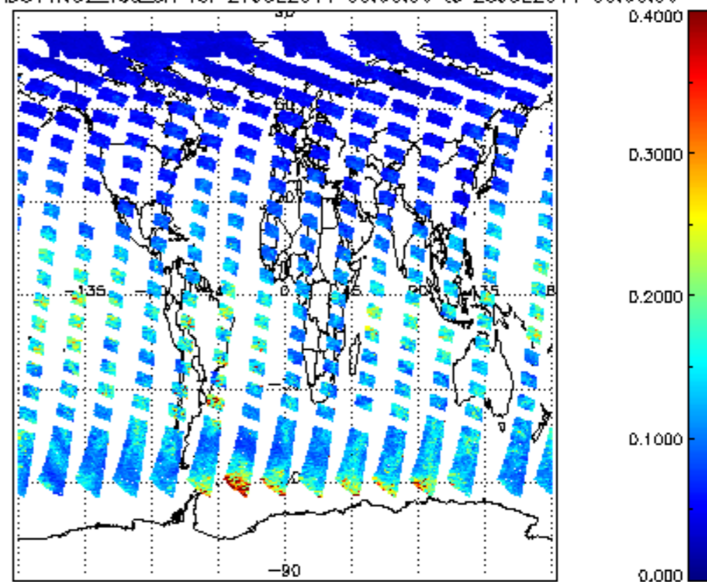
SCIOL2P_NADUV1N02_vcd_err for 27JUL2011 00:00:00 to 28JUL2011 00:00:00
