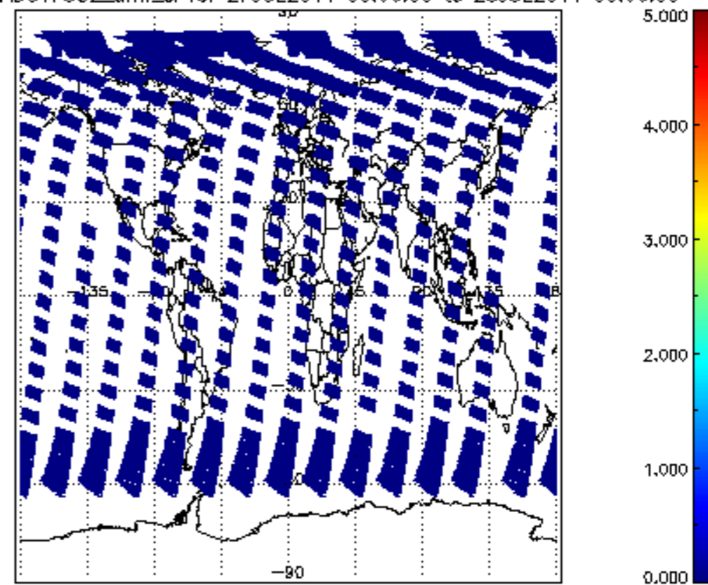
SCIOL2P_NADUV7S02_amf_cl for 27JUL2011 00:00:00 to 28JUL2011 00:00:00
