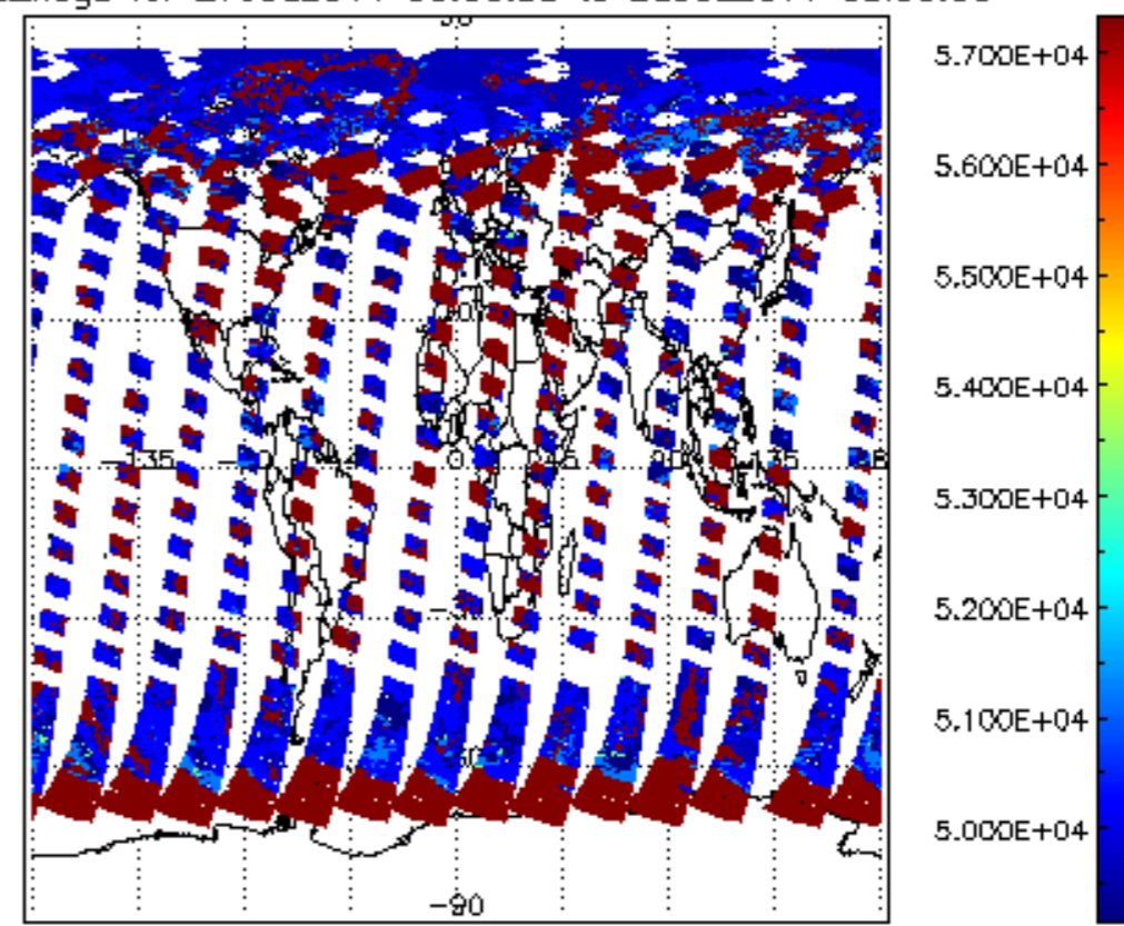
cloud_flags for 27JUL2011 00:00:00 to 28JUL2011 00:00:00
