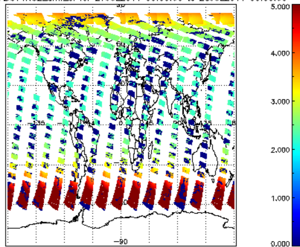
SCIOL2P_NADUV1N02_amf_cl for 27JUL2011 00:00:00 to 28JUL2011 00:00:00
