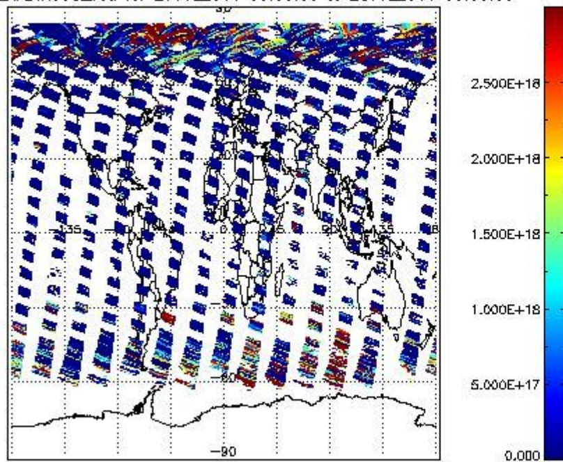
SCIDL2P_NADIR3CO_vcd for 27JUL2011 00:00:00 to 28JUL2011 00:00:00
