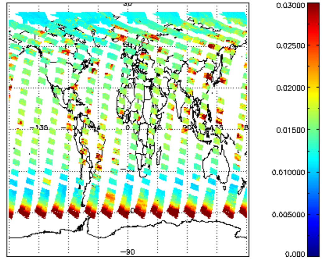
SCIOL2P_NADUV003_vcd_err for 27JUL2011 00:00:00 to 28JUL2011 00:00:00
