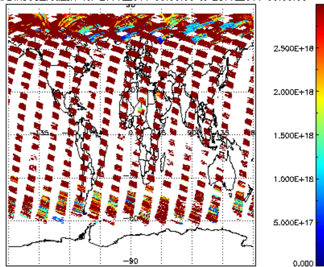
SCIOL2P_NADIR3CO_vcd_err for 27JUL2011 00:00:00 to 28JUL2011 00:00:00
