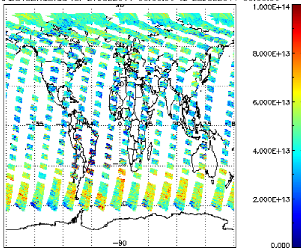
SCIOL2P_NADUV3BRO_vcd for 27JUL2011 00:00:00 to 28JUL2011 00:00:00
