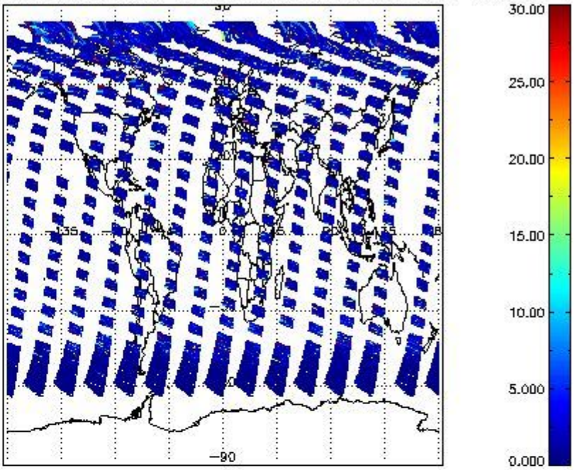
SCIOL2P_NADUV5S02_vcd_err for 27JUL2011 00:00:00 to 28JUL2011 00:00:00
