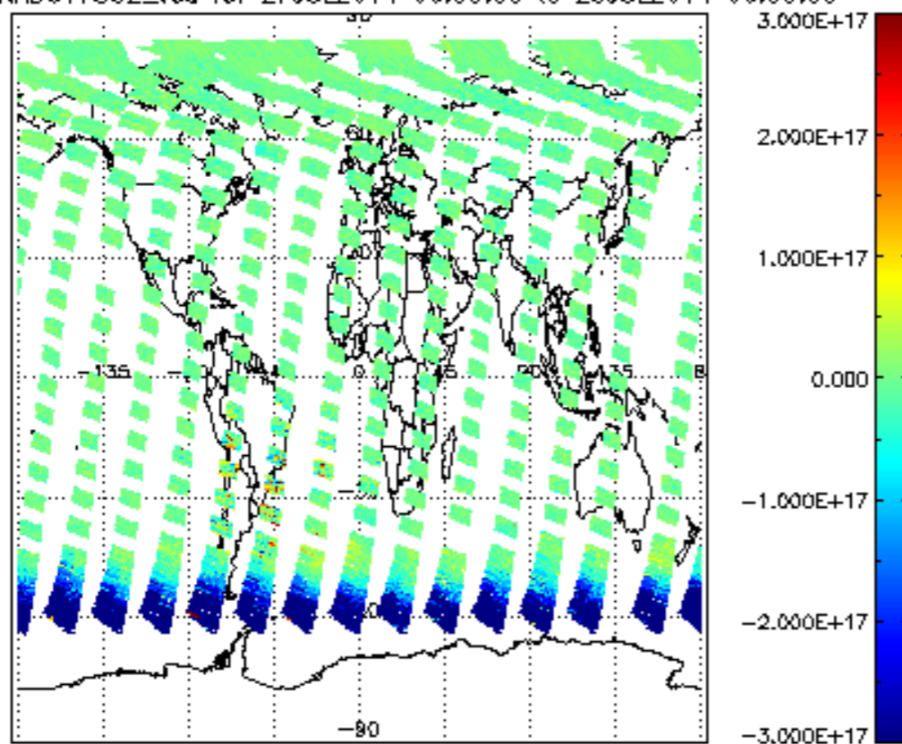
SCIOL2P_NADUV7S02_vcd for 27JUL2011 00:00:00 to 28JUL2011 00:00:00
