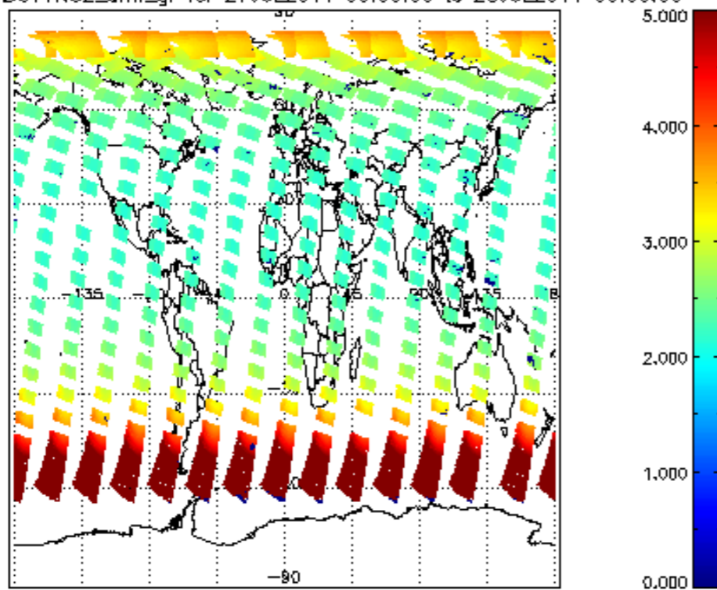
SCIOL2P_NADUV1N02_amf_gr for 27JUL2011 00:00:00 to 28JUL2011 00:00:00
