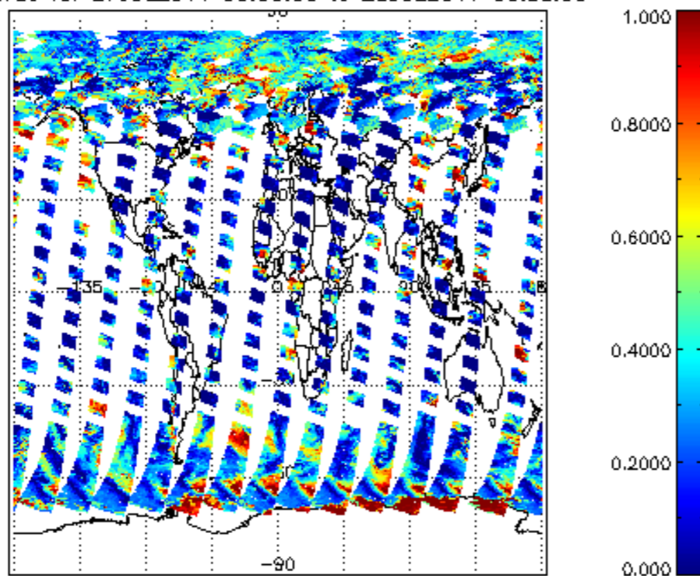
cl_frac for 27JUL2011 00:00:00 to 28JUL2011 00:00:00
