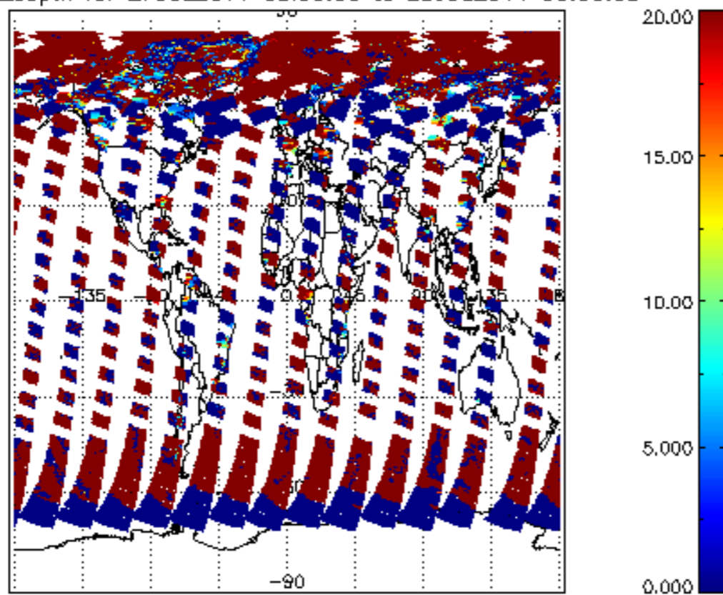
cl_opt_depth for 27JUL2011 00:00:00 to 28JUL2011 00:00:00
