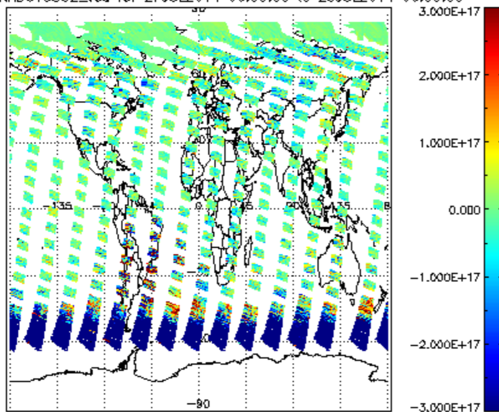
SCIOL2P_NADUV5S02_vcd for 27JUL2011 00:00:00 to 28JUL2011 00:00:00
