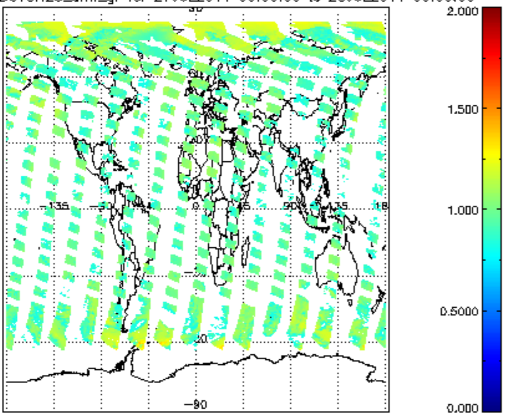
SCIOL2P_NADUV8H20_amf_gr for 27JUL2011 00:00:00 to 28JUL2011 00:00:00
