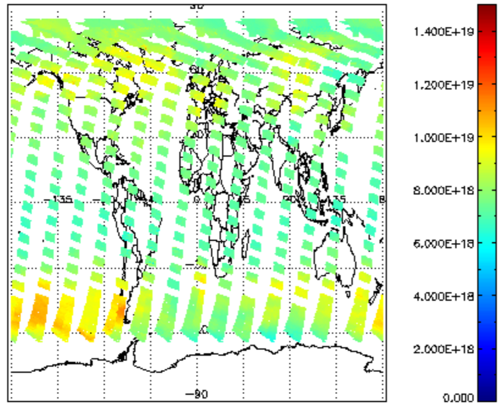
SCIOL2P_NADUV003_vcd for 27JUL2011 00:00:00 to 28JUL2011 00:00:00
