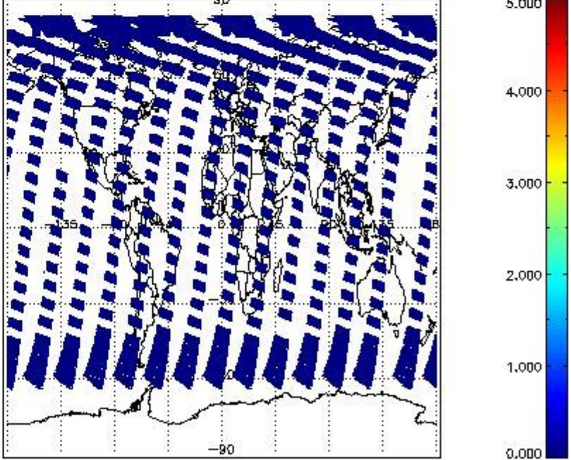
SCIOL2P_NADUV5S02_amf_cl for 27JUL2011 00:00:00 to 28JUL2011 00:00:00
