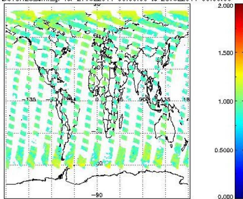
SCIOL2P_NADUV8H2O_amf_gr for 27JUL2011 00:00:00 to 28JUL2011 00:00:00
