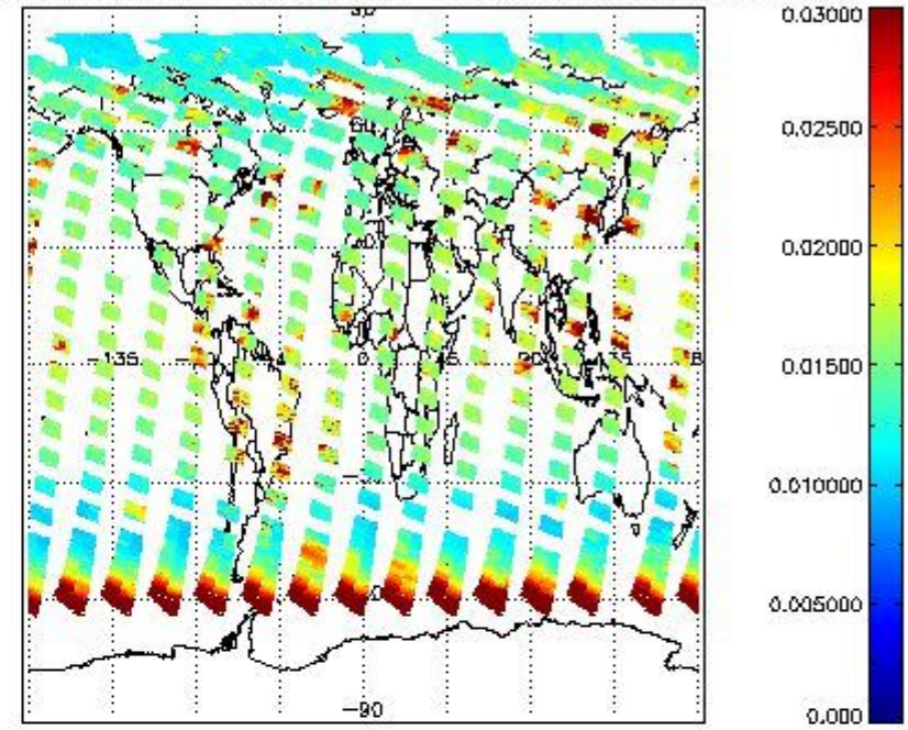
SCIOL2P_NADUV003_vcd_err for 27JUL2011 00:00:00 to 28JUL2011 00:00:00
