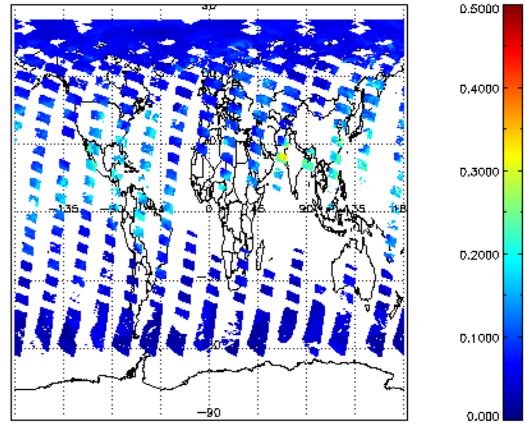
SCIOL2P_NADUV8H20_vcd_err for 27JUL2011 00:00:00 to 28JUL2011 00:00:00
