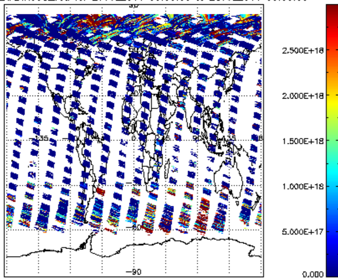
SCIOL2P_NADIR3CO_vcd for 27JUL2011 00:00:00 to 28JUL2011 00:00:00
