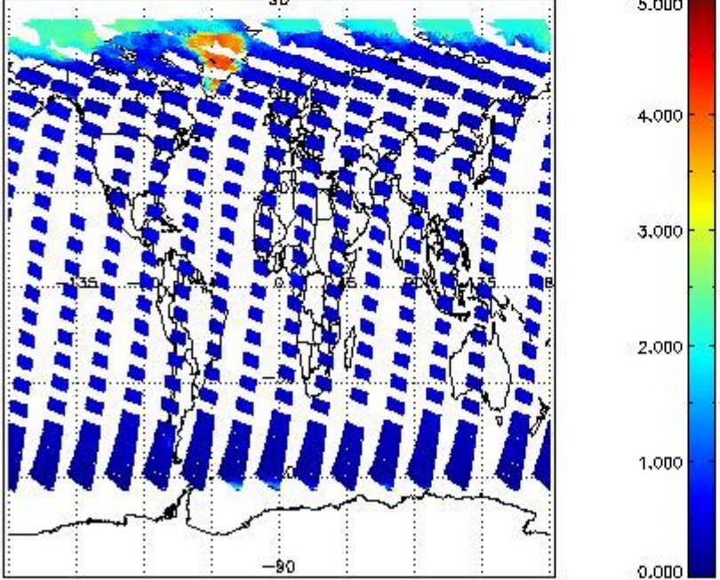
SCIOL2P_NADUV5S02_amf_gr for 27JUL2011 00:00:00 to 28JUL2011 00:00:00
