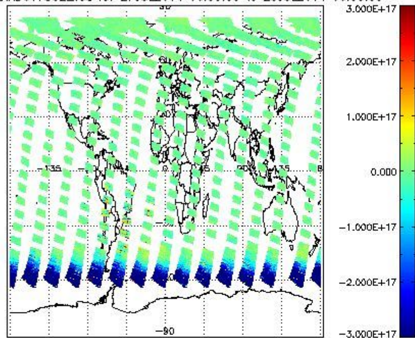
SCIOL2P_NADUV7S02_vcd for 27JUL2011 00:00:00 to 28JUL2011 00:00:00
