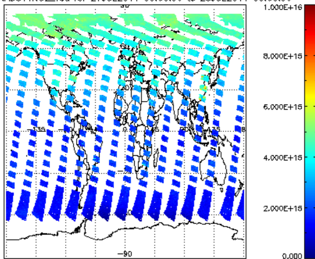
SCIOL2P_NADUV1N02_vcd for 27JUL2011 00:00:00 to 28JUL2011 00:00:00
