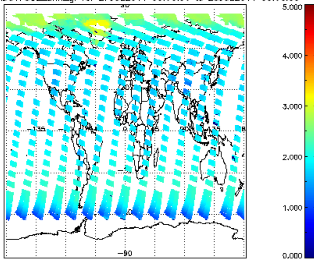
SCIOL2P_NADUV7S02_amf_gr for 27JUL2011 00:00:00 to 28JUL2011 00:00:00
