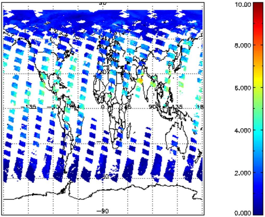
SCIOL2P_NADUV8H20_vcd for 27JUL2011 00:00:00 to 28JUL2011 00:00:00
