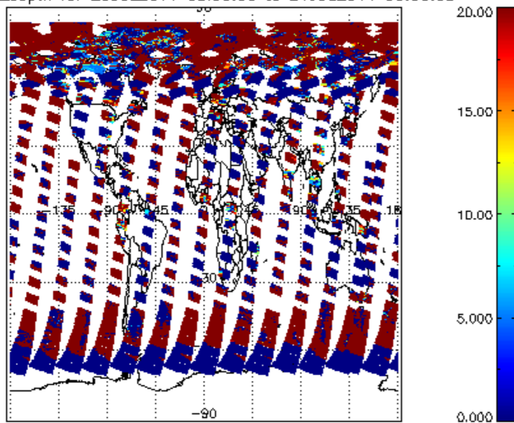
cl_opt_depth for 23JUL2011 00:00:00 to 24JUL2011 00:00:00
