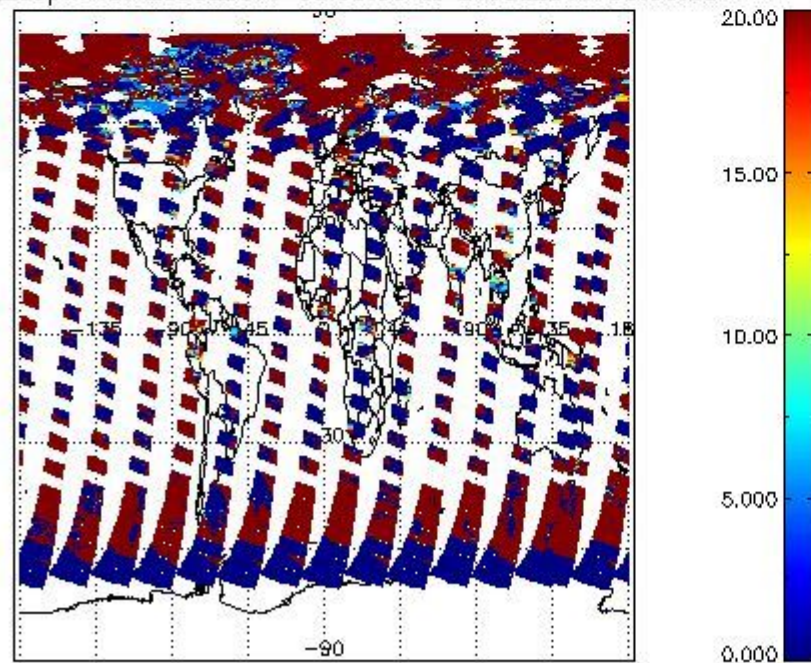
cL_opt_depth for 23JUL2011 00:00:00 to 24JUL2011 00:00:00
