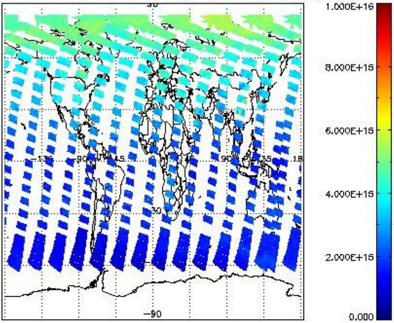
SCIOL2P_NADUV1NO2_vcd for 23JUL2011 00:00:00 to 24JUL2011 00:00:00
