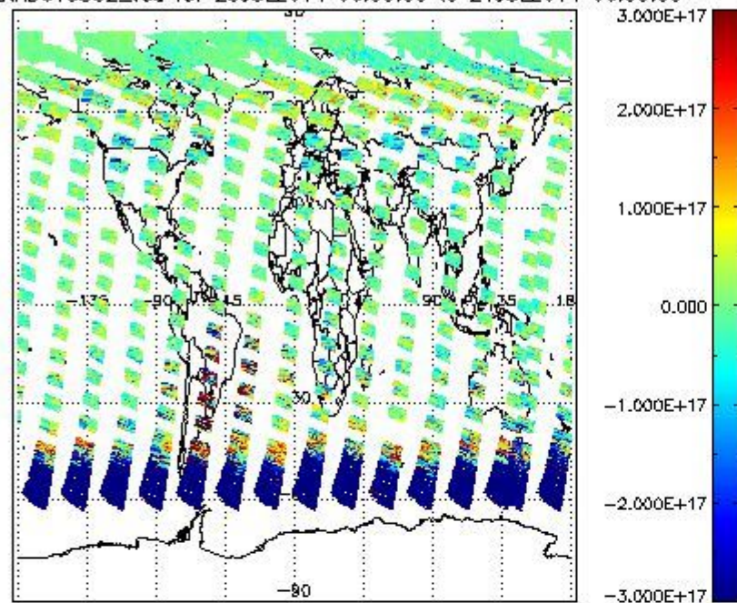
SCIOL2P_NADUV5S02_vcd for 23JUL2011 00:00:00 to 24JUL2011 00:00:00
