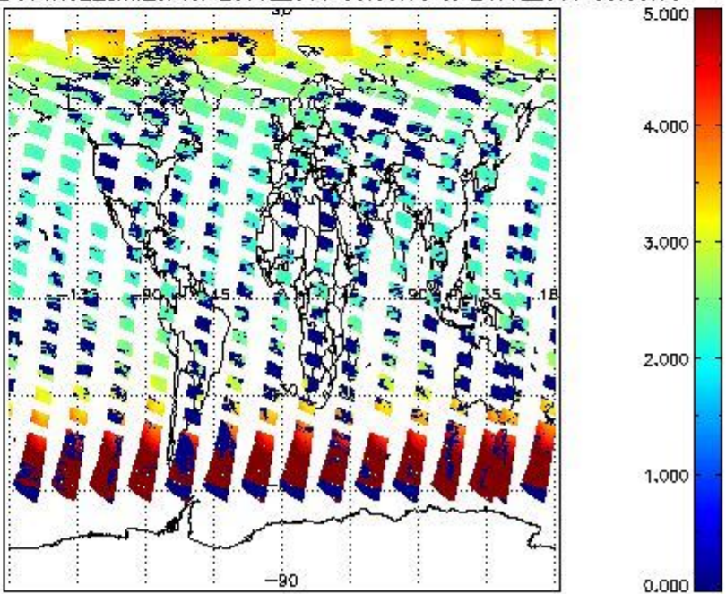
SCIOL2P_NADUV1NO2_amf_cl for 23JUL2011 00:00:00 to 24JUL2011 00:00:00
