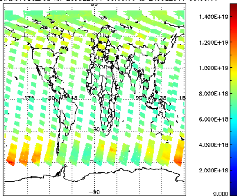
SCIOL2P_NADUV003_vcd for 23JUL2011 00:00:00 to 24JUL2011 00:00:00
