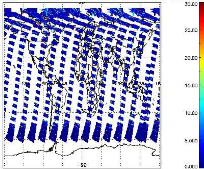
SCIOL2P_NADUV7S02_vcd_err for 23JUL2011 00:00:00 to 24JUL2011 00:00:00
