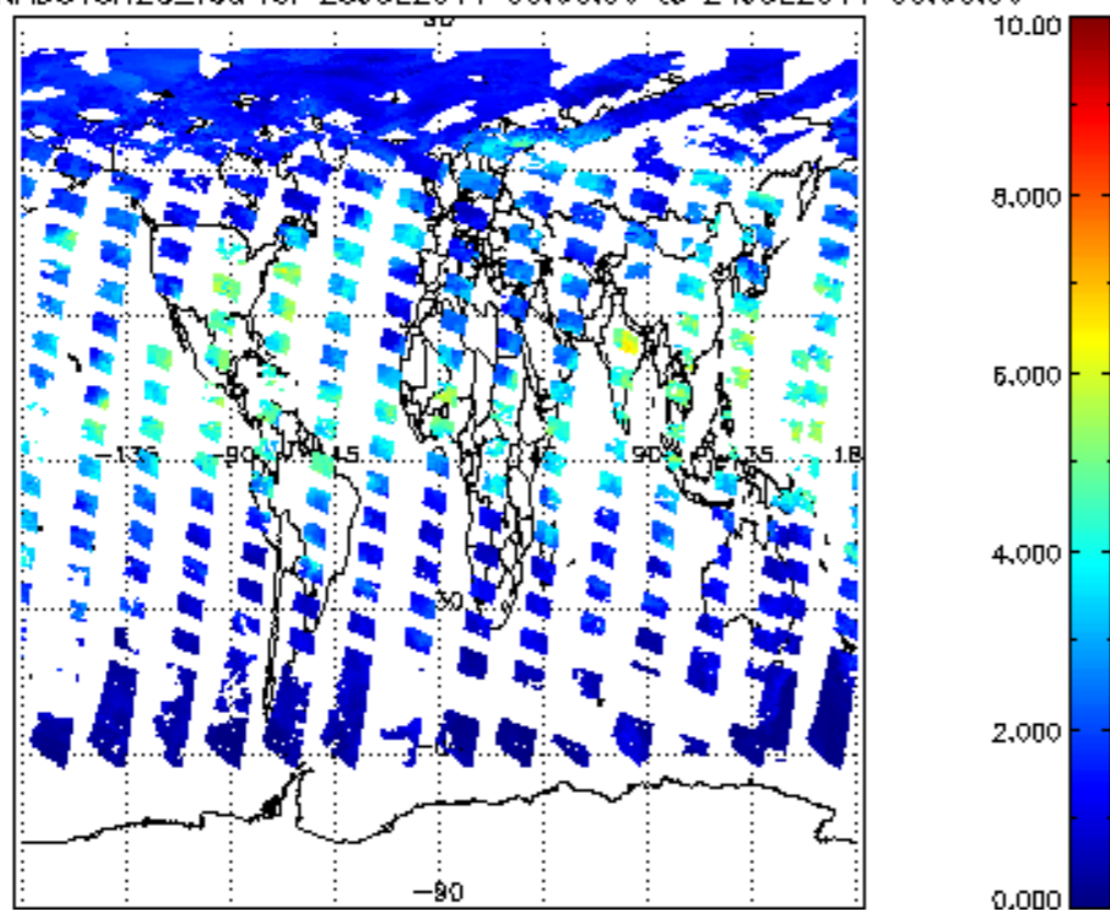
SCIOL2P_NADUV8H20_vcd for 23JUL2011 00:00:00 to 24JUL2011 00:00:00
