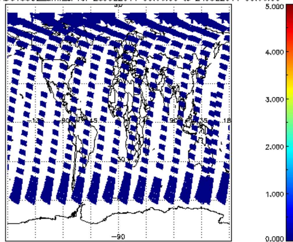
SCIOL2P_NADUV5S02_amf_cl for 23JUL2011 00:00:00 to 24JUL2011 00:00:00
