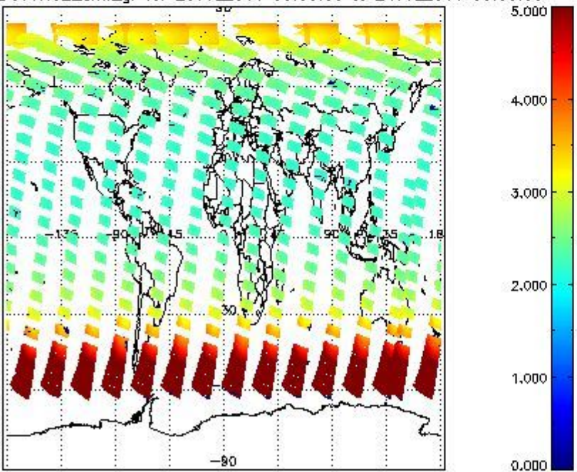
SCIOL2P_NADUV1NO2_amf_gr for 23JUL2011 00:00:00 to 24JUL2011 00:00:00
