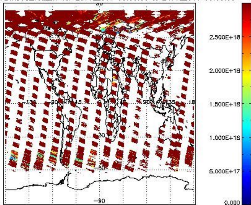
SCIO2P_NADIR3CO_vcd_err for 23JUL2011 00:00:00 to 24JUL2011 00:00:00
