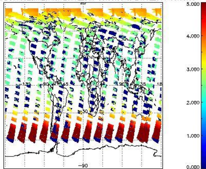
SCIOL2P_NADUV003_amf_cl for 23JUL2011 00:00:00 to 24JUL2011 00:00:00
