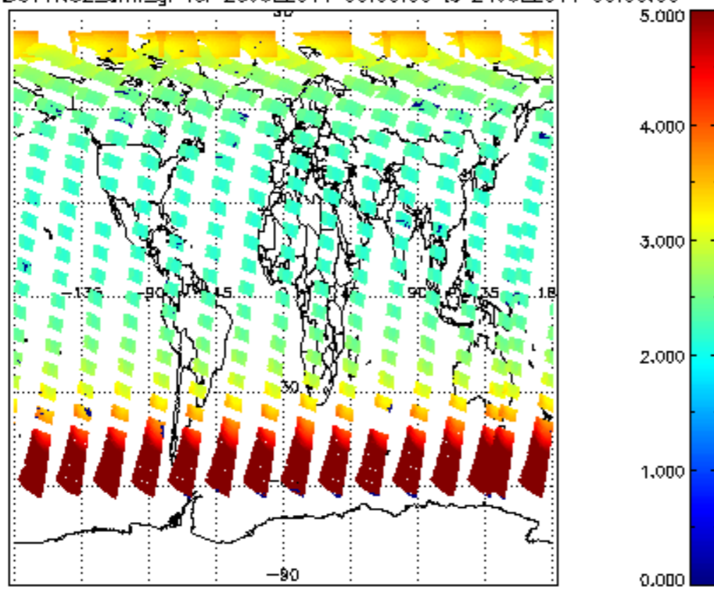
SCIOL2P_NADUV1NO2_amf_gr for 23JUL2011 00:00:00 to 24JUL2011 00:00:00
