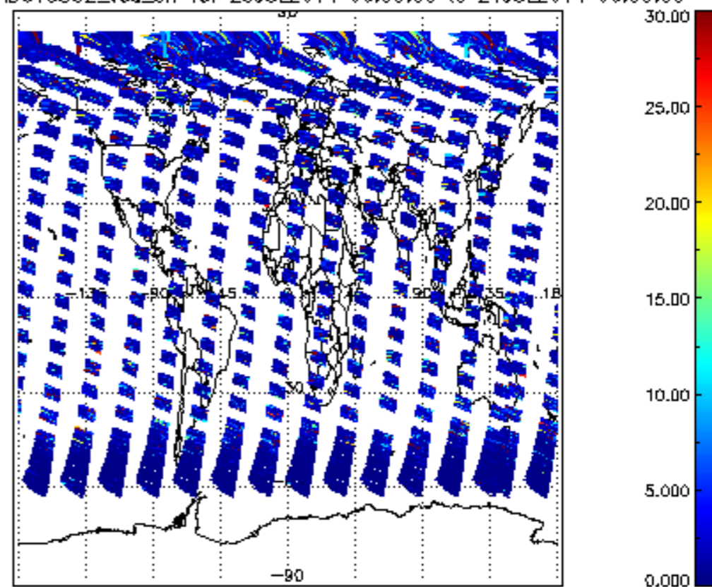
SCIOL2P_NADUV5S02_vcd_err for 23JUL2011 00:00:00 to 24JUL2011 00:00:00
