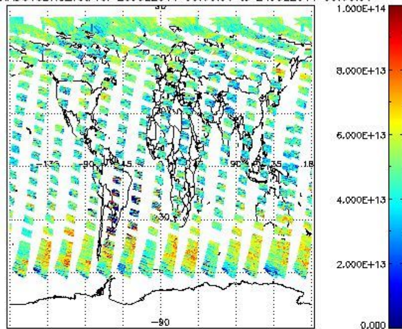
SCIOL2P_NADUV3BRO_vcd for 23JUL2011 00:00:00 to 24JUL2011 00:00:00
