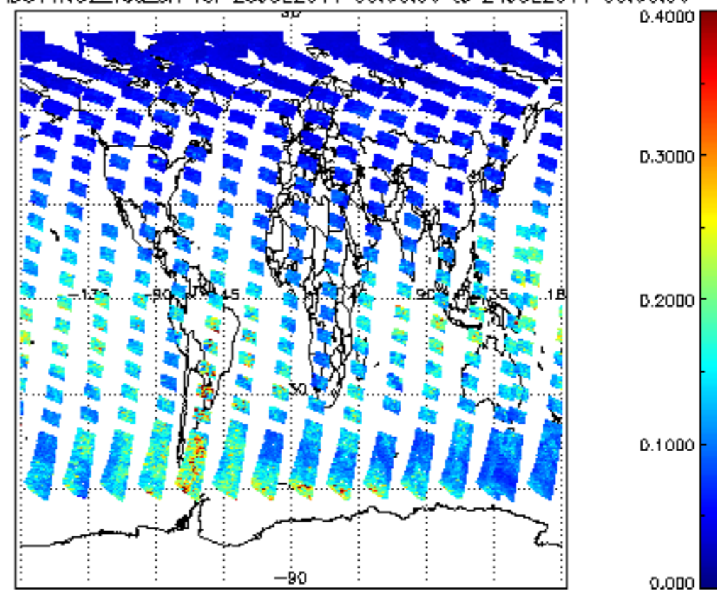
SCIOL2P_NADUV1NO2_vcd_err for 23JUL2011 00:00:00 to 24JUL2011 00:00:00
