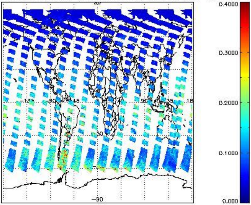
SCIOL2P_NADUV1NO2_vcd_err for 23JUL2011 00:00:00 to 24JUL2011 00:00:00
