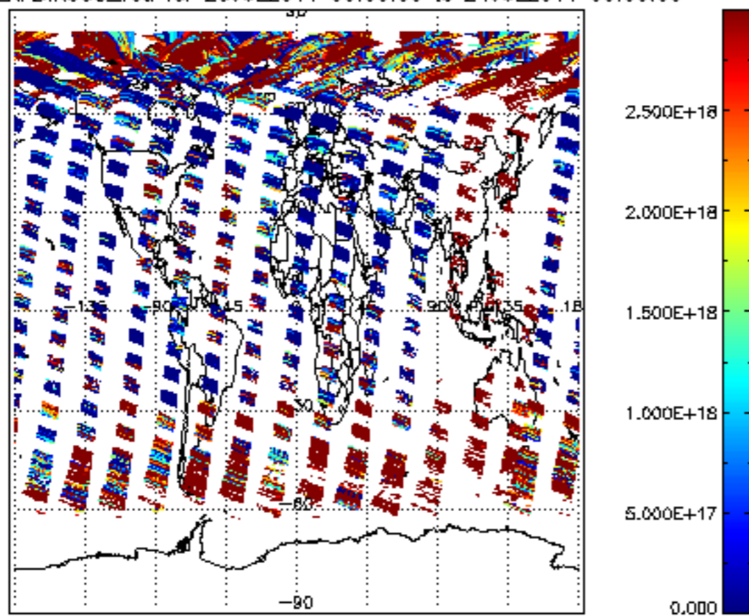
SCIOL2P_NADIR3CO_vcd for 23JUL2011 00:00:00 to 24JUL2011 00:00:00
