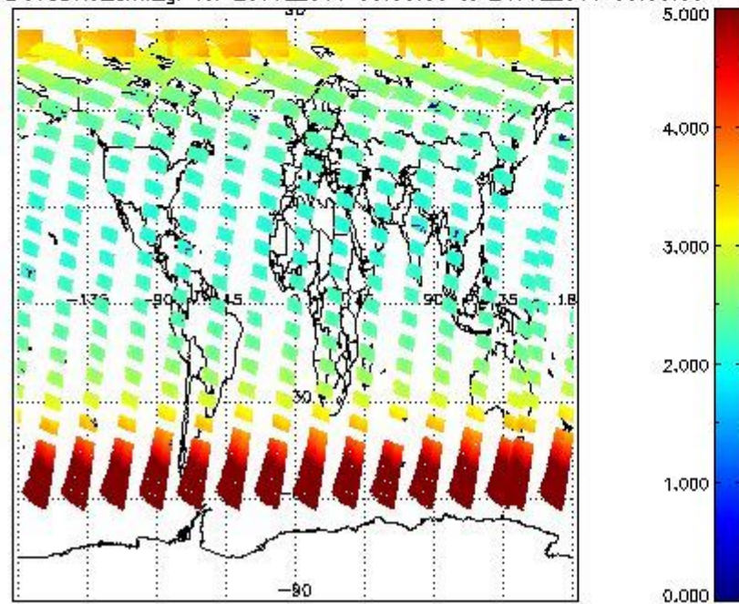
SCIOL2P_NADUV3BRO_amf_gr for 23JUL2011 00:00:00 to 24JUL2011 00:00:00
