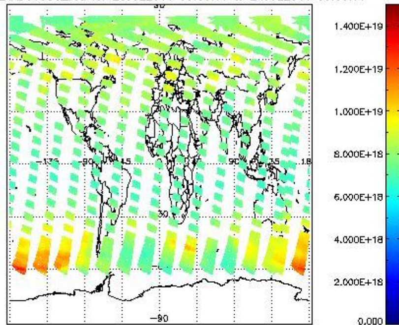
SCIOL2P_NADUV003_vcd for 23JUL2011 00:00:00 to 24JUL2011 00:00:00
