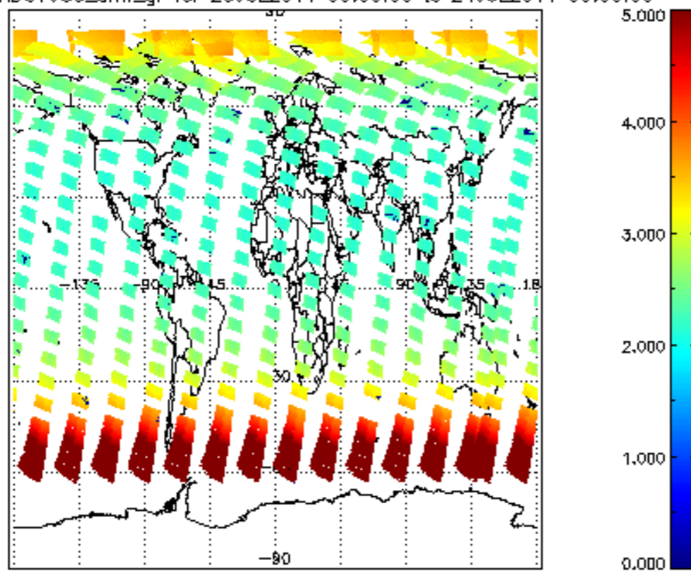
SCIOL2P_NADUV003_amf_gr for 23JUL2011 00:00:00 to 24JUL2011 00:00:00
