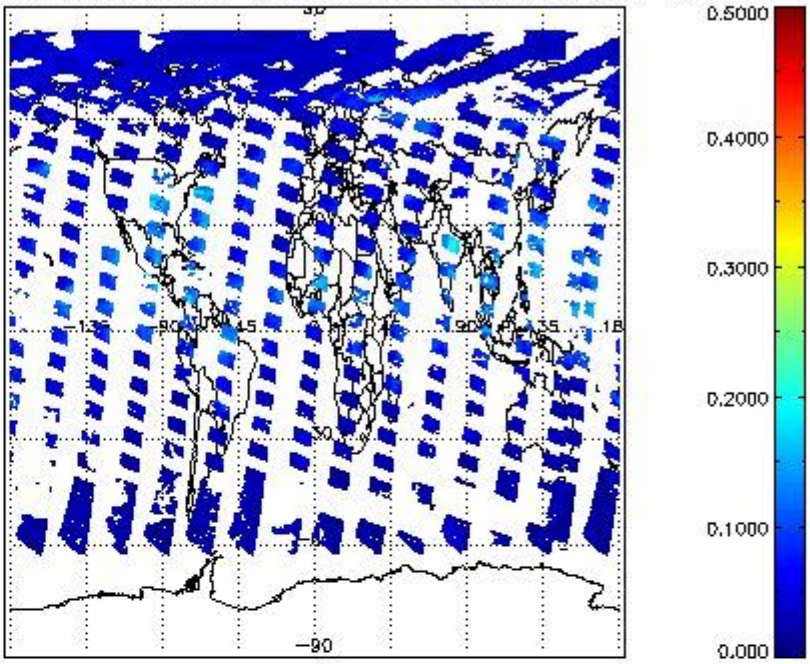
SCIOL2P_NADUV8H2O_vcd_err for 23JUL2011 00:00:00 to 24JUL2011 00:00:00
