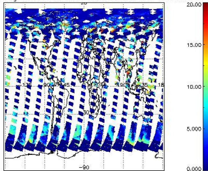
cL_top_height for 23JUL2011 00:00:00 to 24JUL2011 00:00:00
