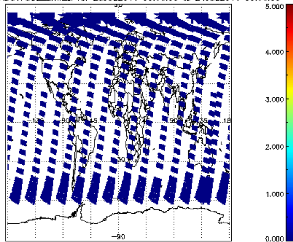
SCIOL2P_NADUV7S02_amf_cl for 23JUL2011 00:00:00 to 24JUL2011 00:00:00
