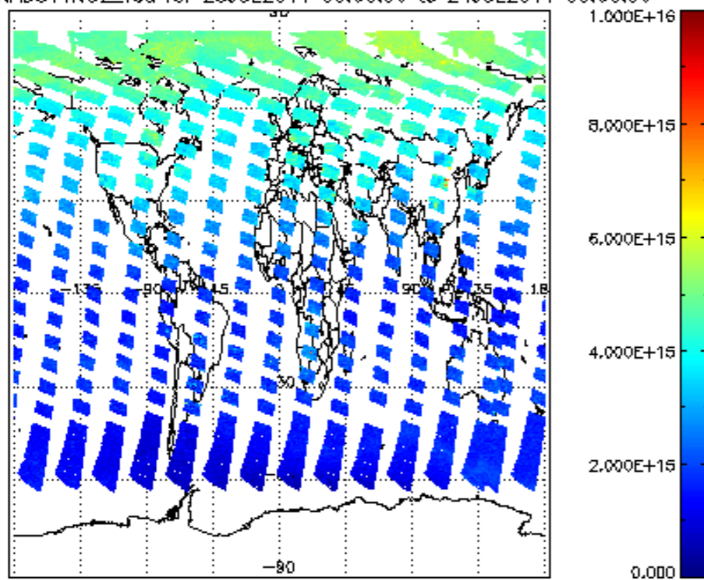
SCIOL2P_NADUV1NO2_vcd for 23JUL2011 00:00:00 to 24JUL2011 00:00:00
