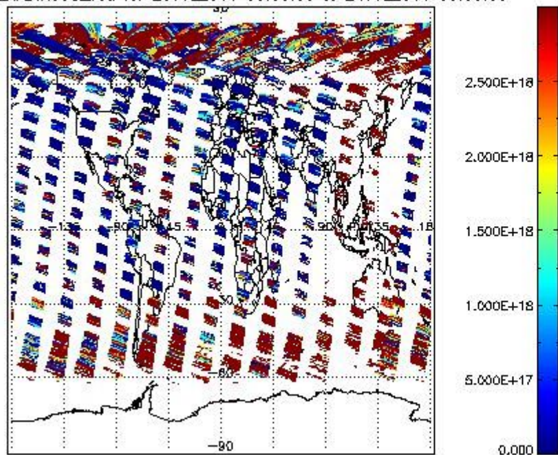
SCIO2P_NADIR3CO_vcd for 23JUL2011 00:00:00 to 24JUL2011 00:00:00
