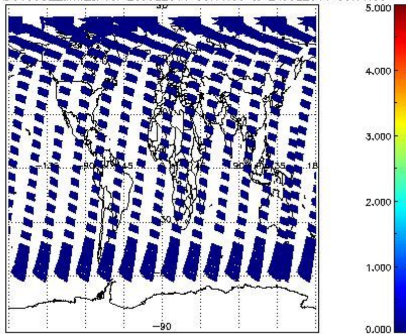
SCIOL2P_NADUV5S02_amf_cl for 23JUL2011 00:00:00 to 24JUL2011 00:00:00
