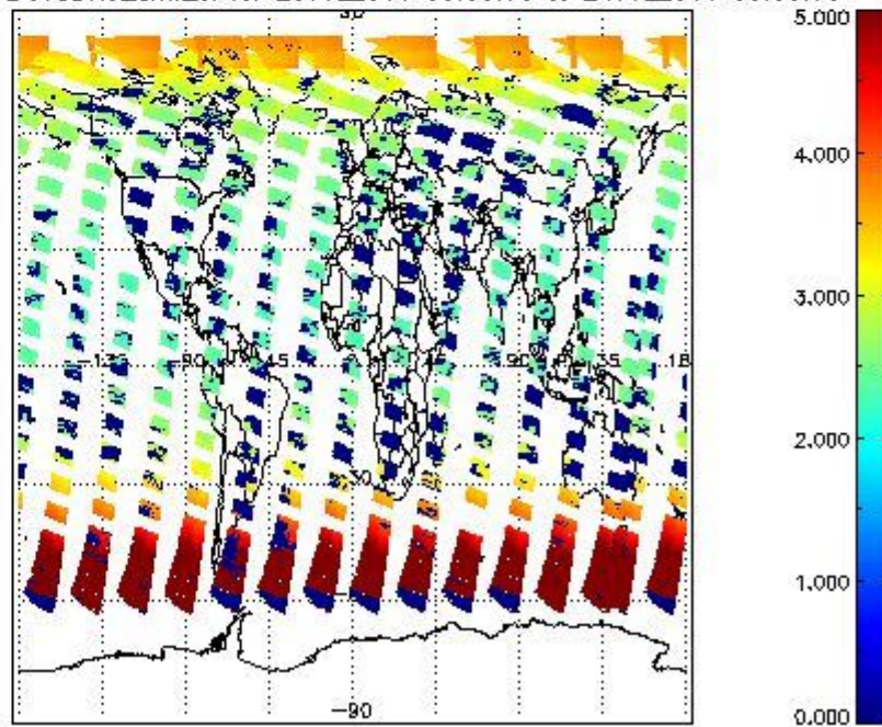
SCIOL2P_NADUV3BRO_amf_cl for 23JUL2011 00:00:00 to 24JUL2011 00:00:00
