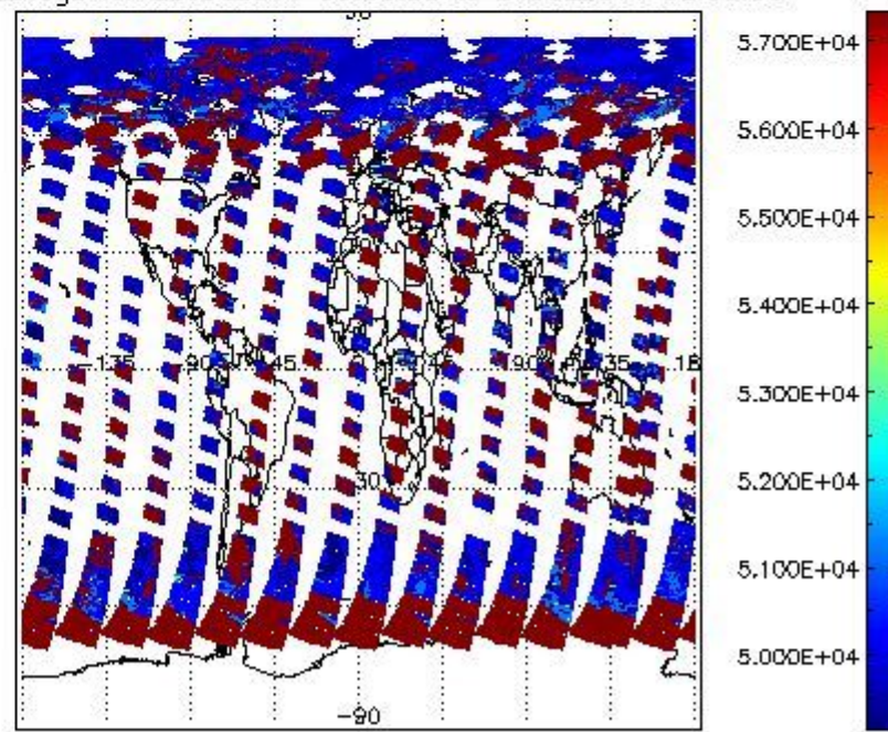
cloud_flags for 23JUL2011 00:00:00 to 24JUL2011 00:00:00
