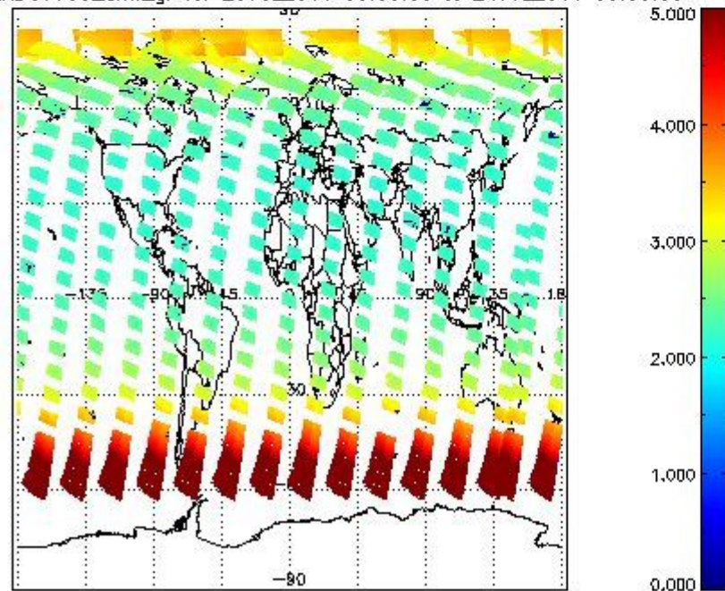
SCIOL2P_NADUV003_amf_gr for 23JUL2011 00:00:00 to 24JUL2011 00:00:00
