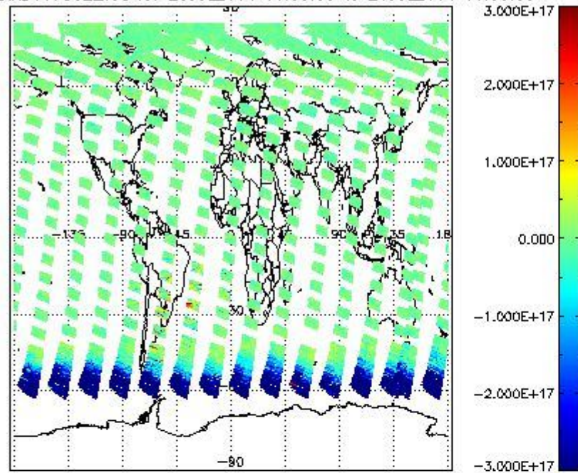
SCIOL2P_NADUV7S02_vcd for 23JUL2011 00:00:00 to 24JUL2011 00:00:00
