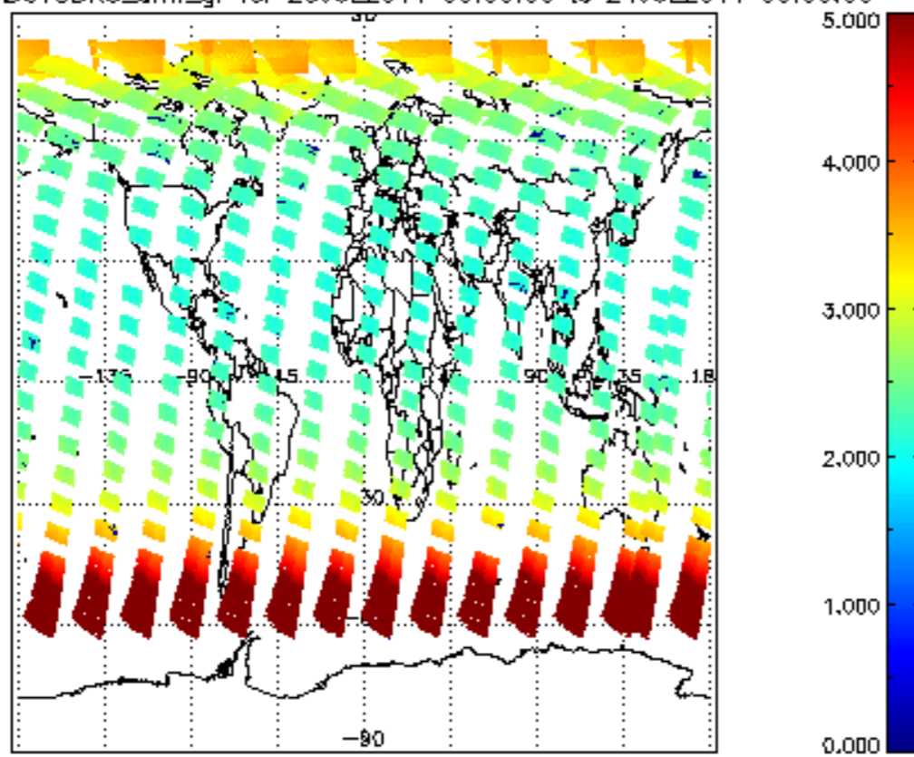
SCIOL2P_NADUV3BRO_arnf_gr for 23JUL2011 00:00:00 to 24JUL2011 00:00:00
