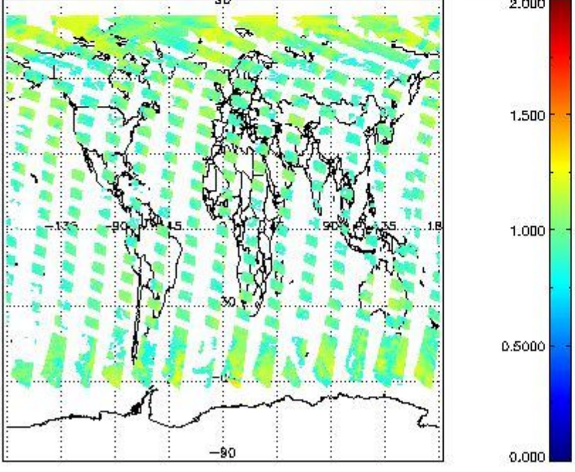
SCIOL2P_NADUV8H2O_amf_gr for 23JUL2011 00:00:00 to 24JUL2011 00:00:00
