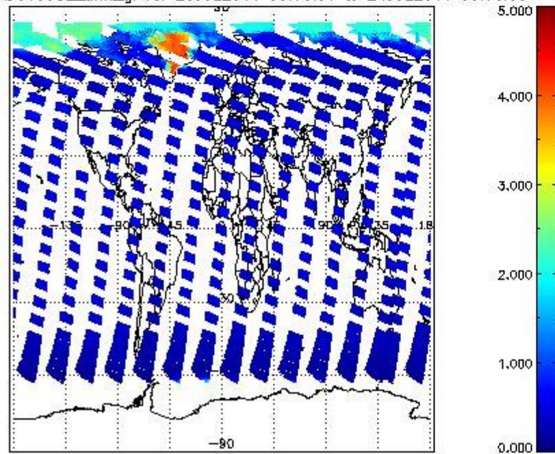
SCIOL2P_NADUV5S02_amf_gr for 23JUL2011 00:00:00 to 24JUL2011 00:00:00
