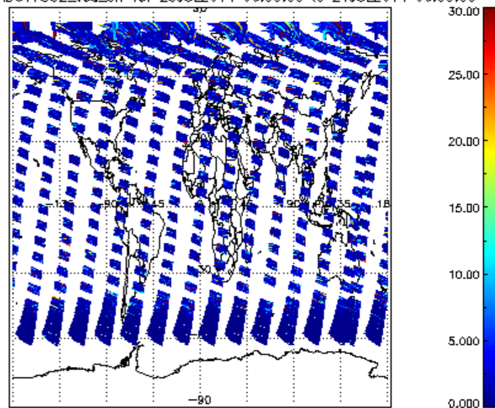
SCIOL2P_NADUV7S02_vcd_err for 23JUL2011 00:00:00 to 24JUL2011 00:00:00
