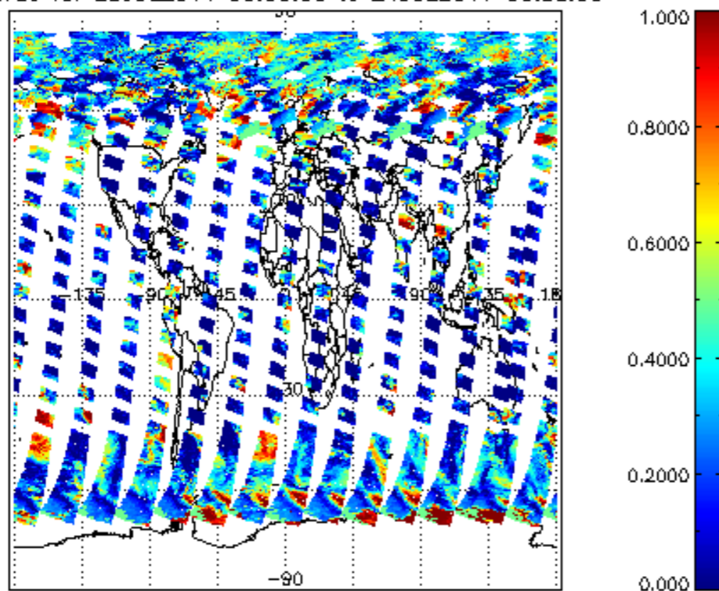
cl_frac for 23JUL2011 00:00:00 to 24JUL2011 00:00:00
