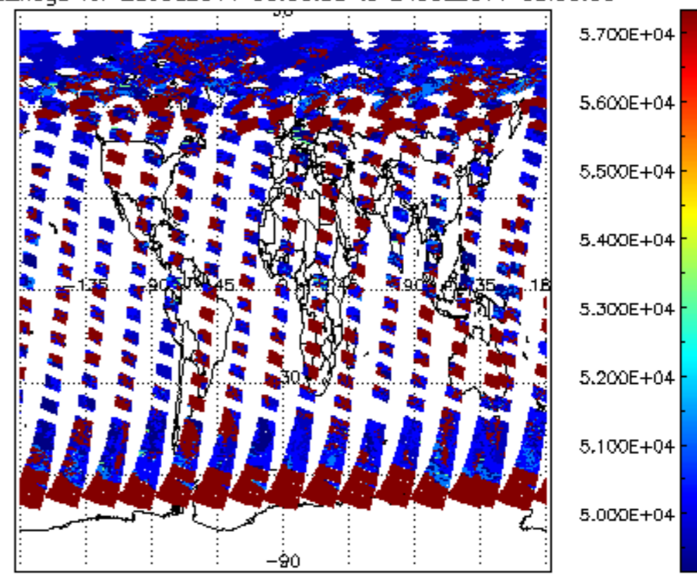
cloud_flags for 23JUL2011 00:00:00 to 24JUL2011 00:00:00
