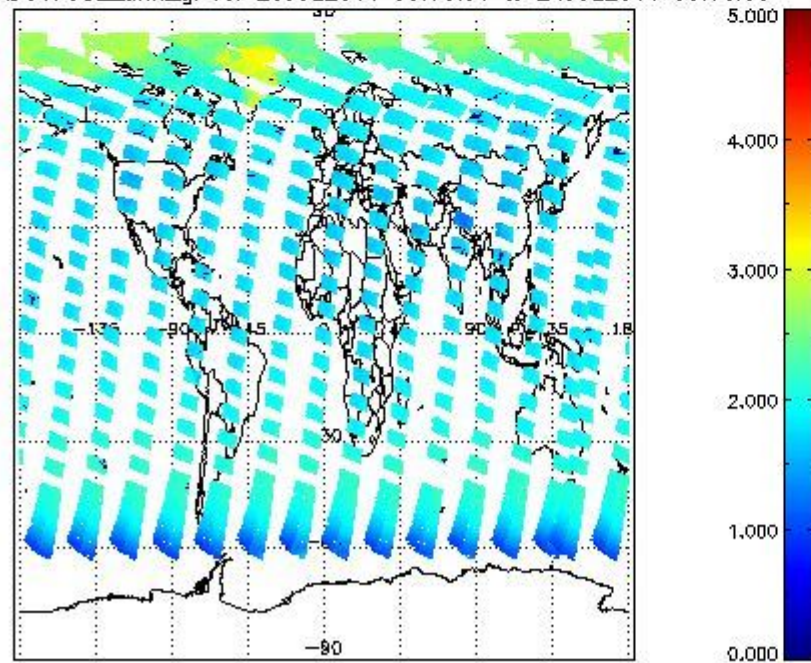
SCIOL2P_NADUV7S02_amf_gr for 23JUL2011 00:00:00 to 24JUL2011 00:00:00
