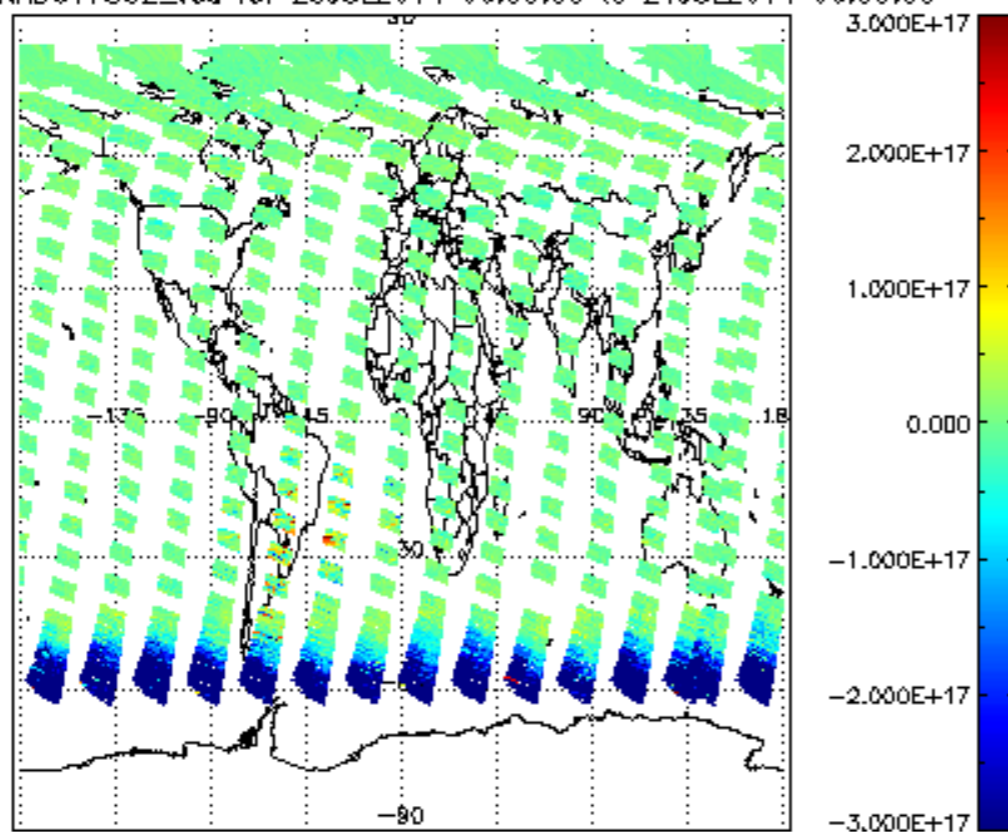
SCIOL2P_NADUV7S02_vcd for 23JUL2011 00:00:00 to 24JUL2011 00:00:00
