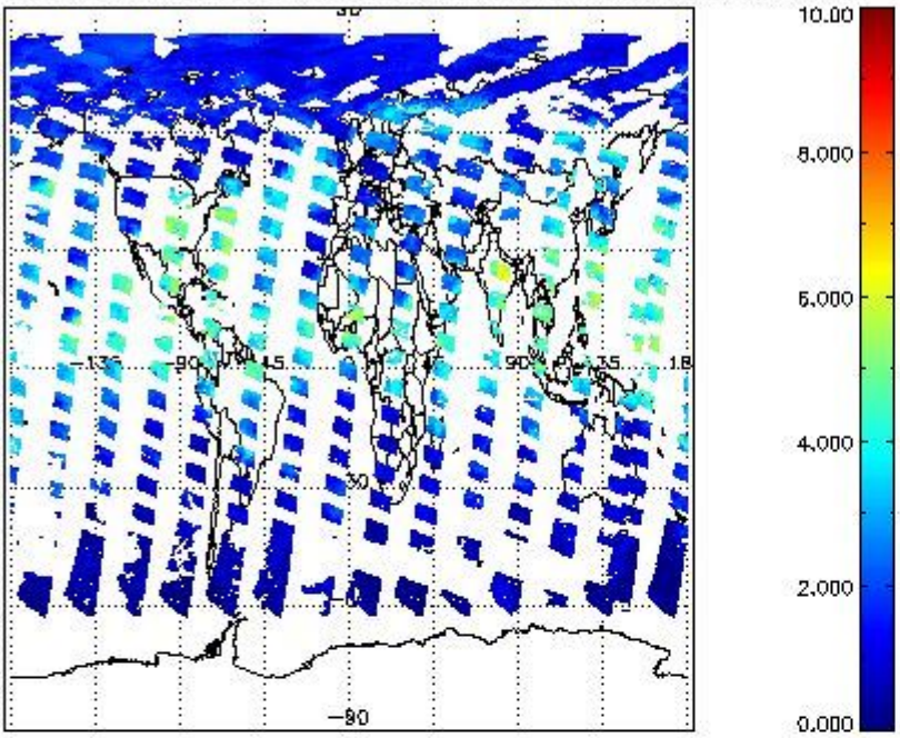
SCIOL2P_NADUV8H2O_vcd for 23JUL2011 00:00:00 to 24JUL2011 00:00:00
