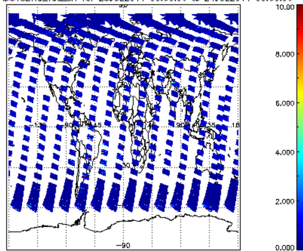
SCIOL2P_NADUV3BRO_vcd_err for 23JUL2011 00:00:00 to 24JUL2011 00:00:00
