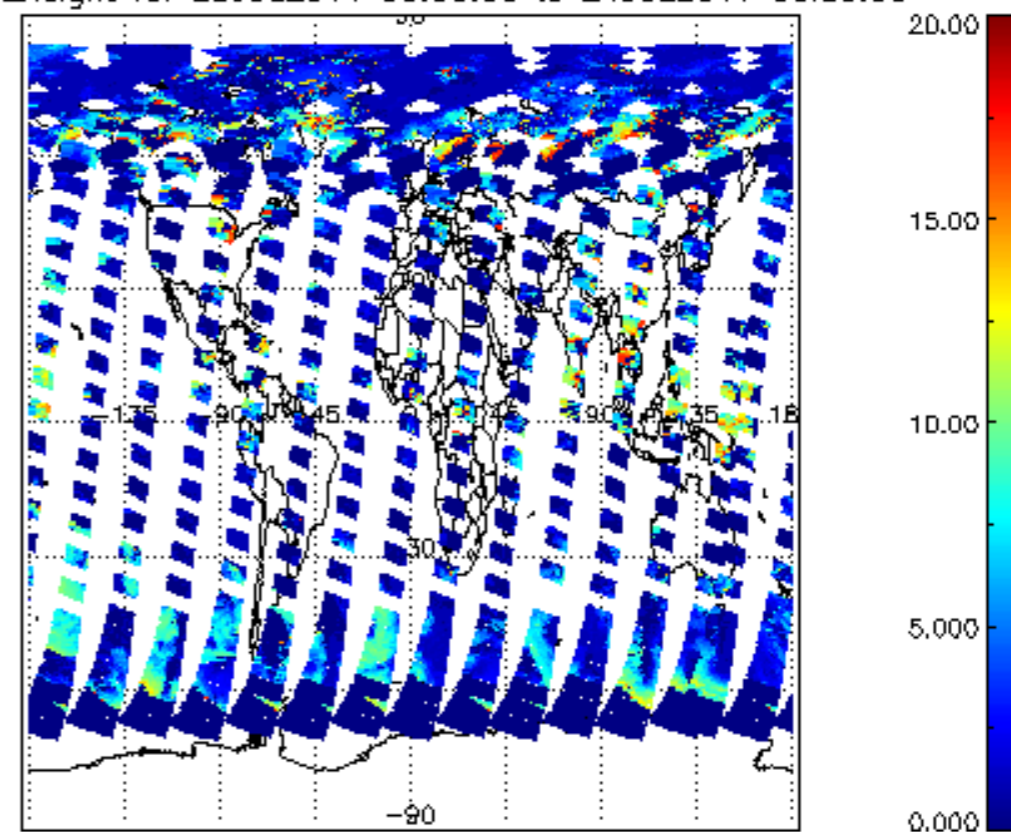
cl_top_height for 23JUL2011 00:00:00 to 24JUL2011 00:00:00
