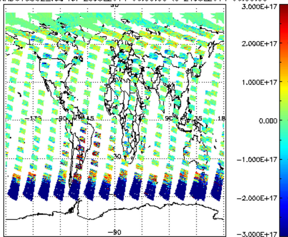
SCIOL2P_NADUV5S02_vcd for 23JUL2011 00:00:00 to 24JUL2011 00:00:00
