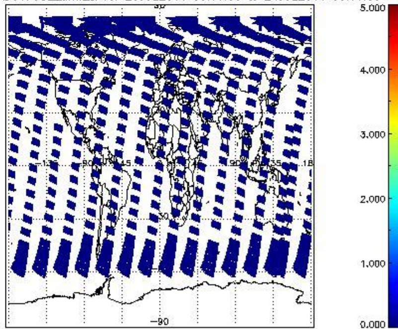
SCIOL2P_NADUV7S02_amf_cl for 23JUL2011 00:00:00 to 24JUL2011 00:00:00
