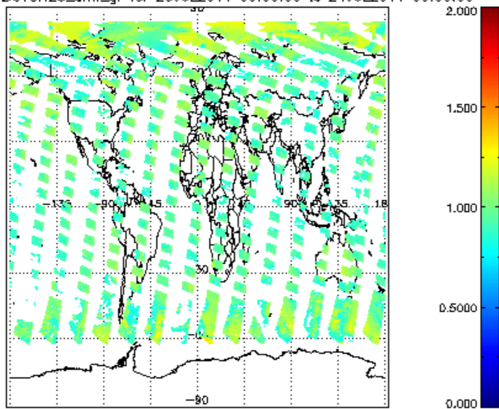
SCIOL2P_NADUV8H20_amf_gr for 23JUL2011 00:00:00 to 24JUL2011 00:00:00
