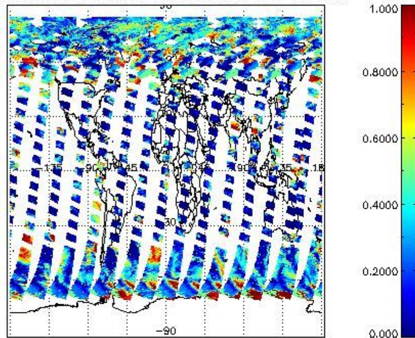
cL_frac for 23JUL2011 00:00:00 to 24JUL2011 00:00:00
