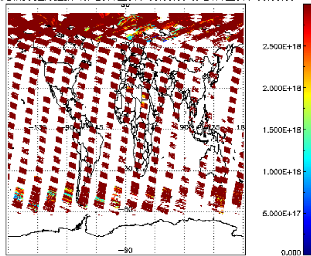
SCIOL2P_NADIR3CO_vcd_err for 23JUL2011 00:00:00 to 24JUL2011 00:00:00
