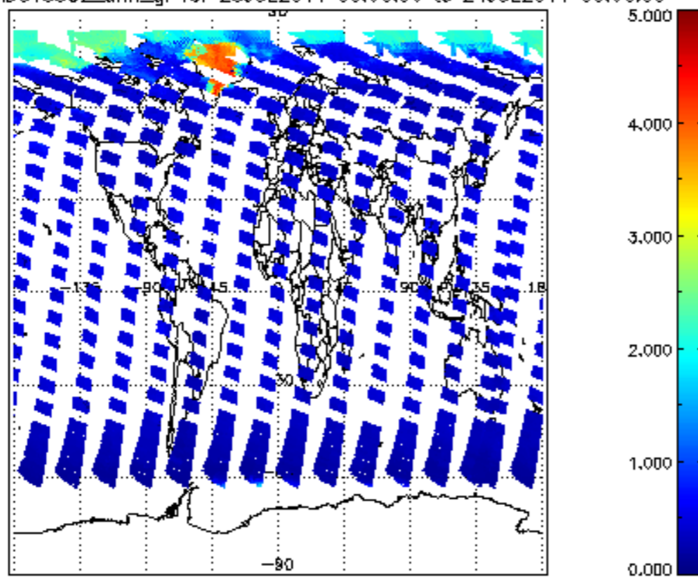
SCIOL2P_NADUV5S02_amf_gr for 23JUL2011 00:00:00 to 24JUL2011 00:00:00
