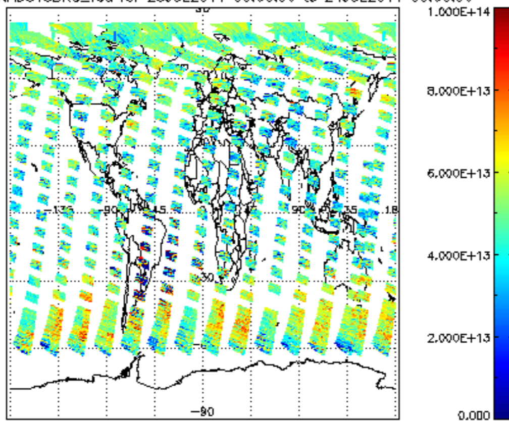
SCIOL2P_NADUV3BRO_vcd for 23JUL2011 00:00:00 to 24JUL2011 00:00:00
