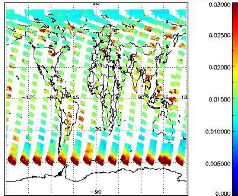
SCIOL2P_NADUV003_vcd_err for 23JUL2011 00:00:00 to 24JUL2011 00:00:00
