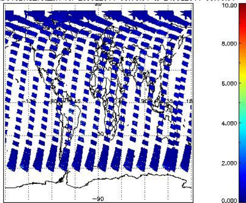
SCIOL2P_NADUV3BRO_vcd_err for 23JUL2011 00:00:00 to 24JUL2011 00:00:00
