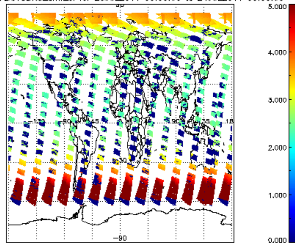
SCIOL2P_NADUV3BRO_arnf_cl for 23JUL2011 00:00:00 to 24JUL2011 00:00:00
