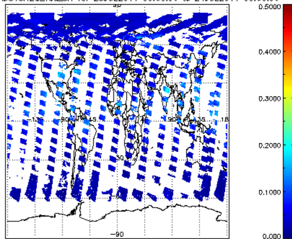
SCIOL2P_NADUV8H20_vcd_err for 23JUL2011 00:00:00 to 24JUL2011 00:00:00
