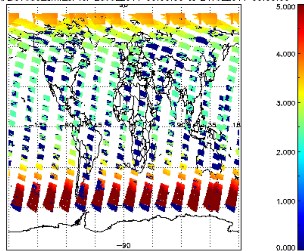
SCIOL2P_NADUV003_amf_cl for 23JUL2011 00:00:00 to 24JUL2011 00:00:00
