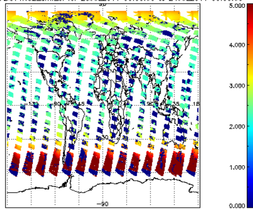
SCIOL2P_NADUV1NO2_amf_cl for 23JUL2011 00:00:00 to 24JUL2011 00:00:00
