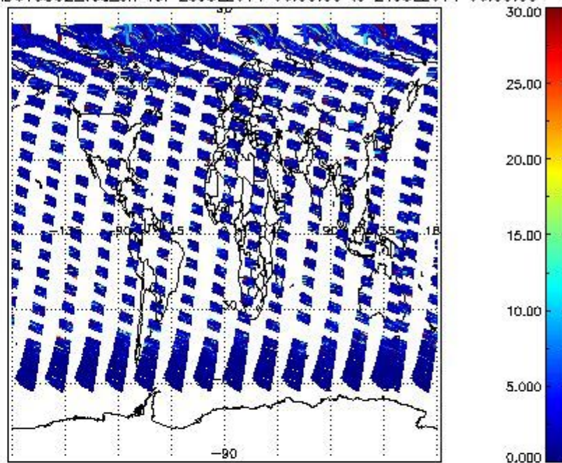
SCIOL2P_NADUV5S02_vcd_err for 23JUL2011 00:00:00 to 24JUL2011 00:00:00
