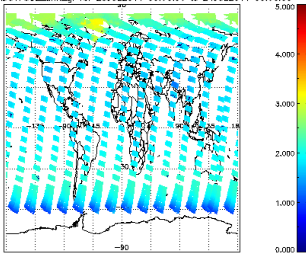
SCIOL2P_NADUV7S02_amf_gr for 23JUL2011 00:00:00 to 24JUL2011 00:00:00
