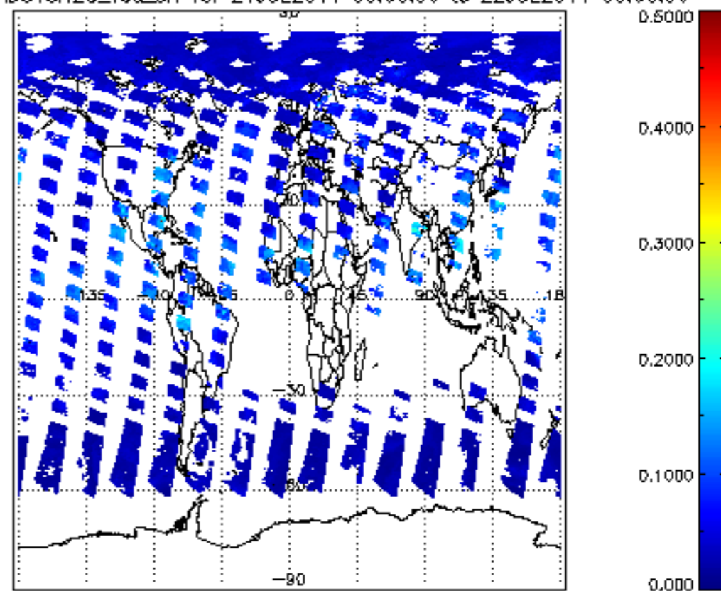
SCIOL2P_NADUV8H20_vcd_err for 21JUL2011 00:00:00 to 22JUL2011 00:00:00
