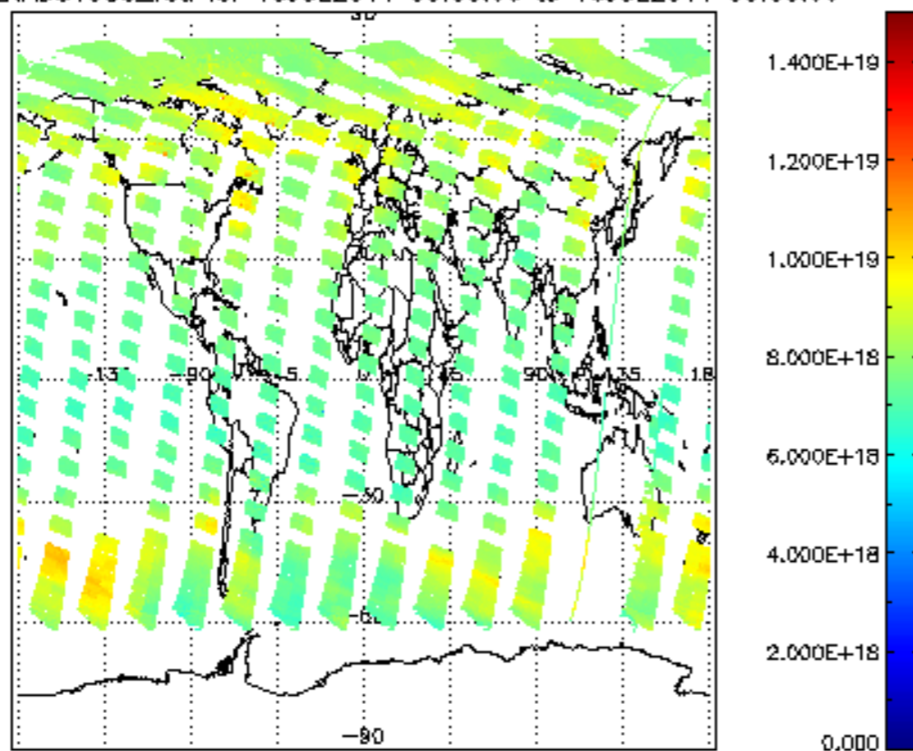
SCIOL2P_NADUV003_vcd for 15JUL2011 00:00:00 to 16JUL2011 00:00:00
