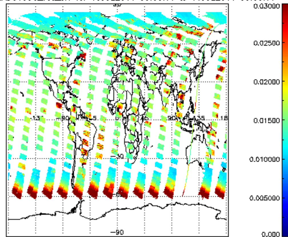
SCIOL2P_NADUV003_vcd_err for 15JUL2011 00:00:00 to 16JUL2011 00:00:00
