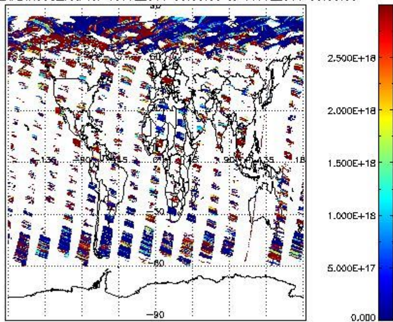
SCIDL2P_NADIR3CO_vcd for 15JUL2011 00:00:00 to 16JUL2011 00:00:00
