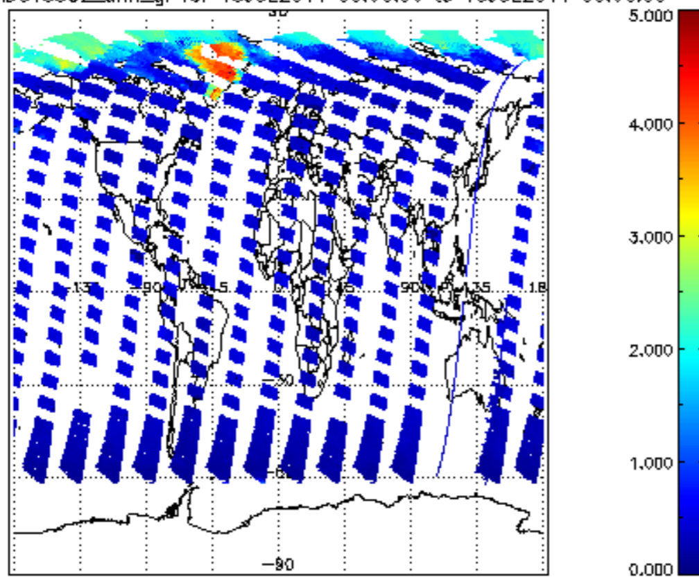
SCIOL2P_NADUV5S02_amf_gr for 15JUL2011 00:00:00 to 16JUL2011 00:00:00
