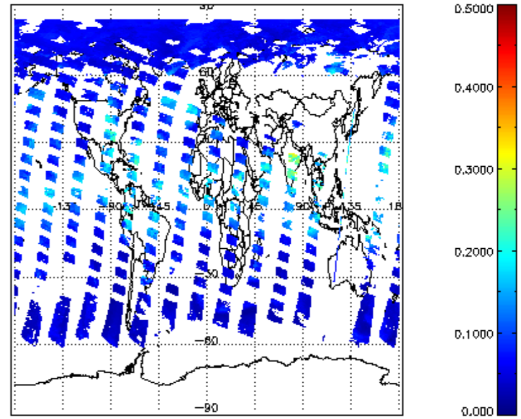
SCIOL2P_NADUV8H20_vcd_err for 15JUL2011 00:00:00 to 16JUL2011 00:00:00
