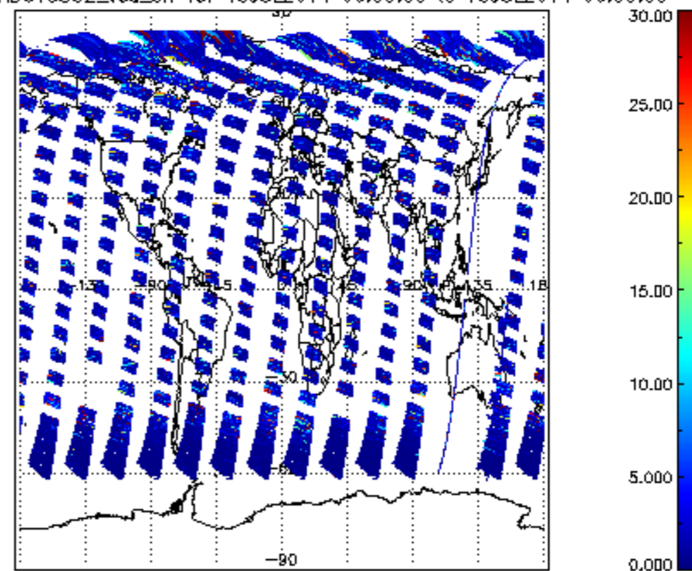
SCIOL2P_NADUV5S02_vcd_err for 15JUL2011 00:00:00 to 16JUL2011 00:00:00
