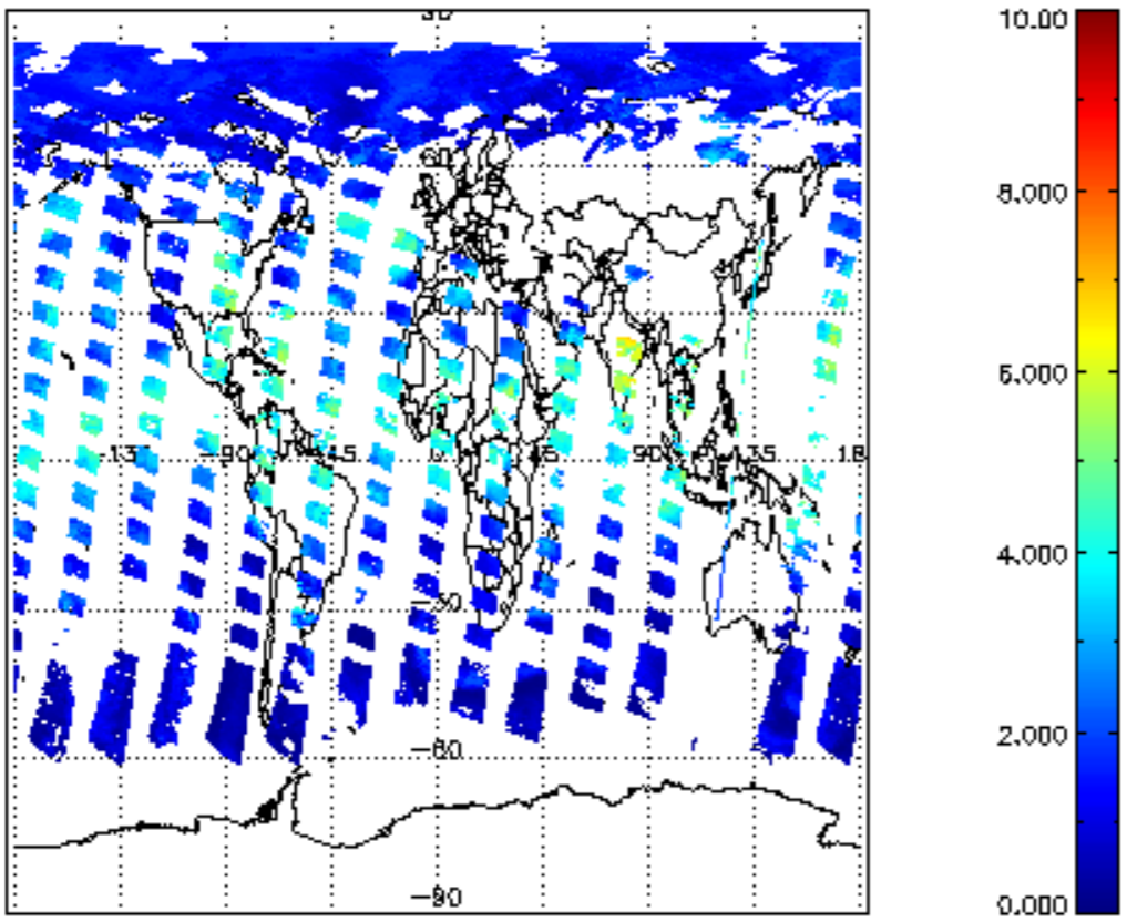
SCIOL2P_NADUV8H20_vcd for 15JUL2011 00:00:00 to 16JUL2011 00:00:00
