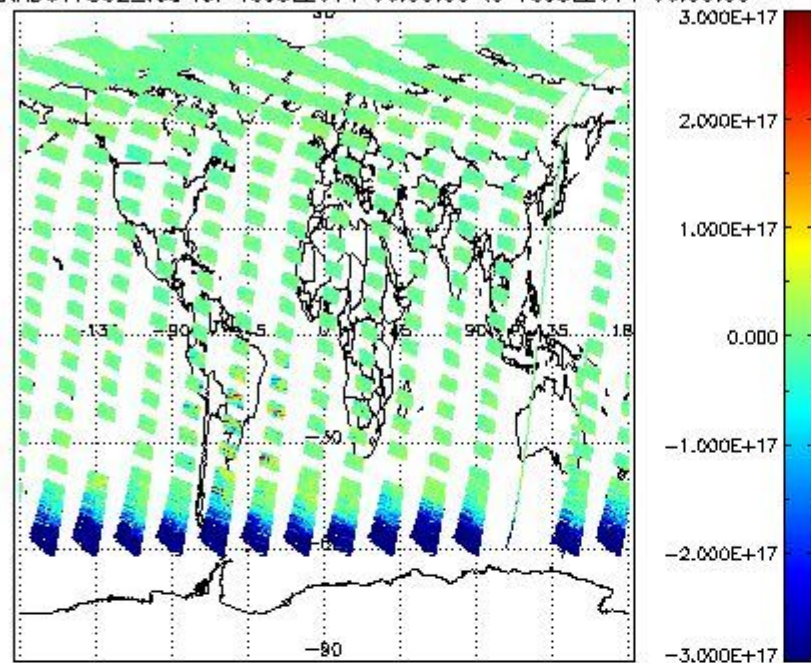
SCIOL2P_NADUV7S02_vcd for 15JUL2011 00:00:00 to 16JUL2011 00:00:00
