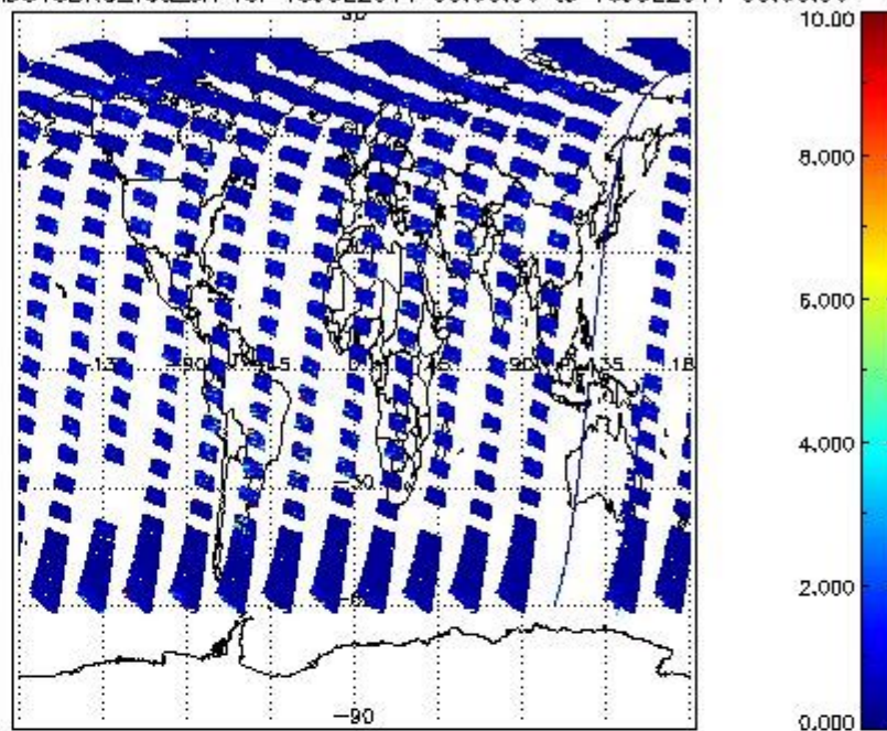
SCIOL2P_NADUV3BRO_vcd_err for 15JUL2011 00:00:00 to 16JUL2011 00:00:00
