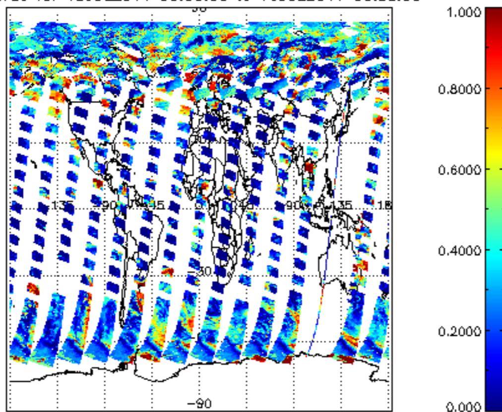
cl_frac for 15JUL2011 00:00:00 to 16JUL2011 00:00:00
