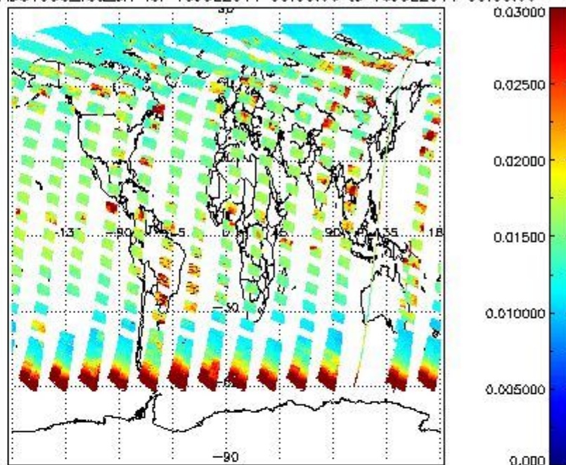
SCIOL2P_NADUV003_vcd_err for 15JUL2011 00:00:00 to 16JUL2011 00:00:00
