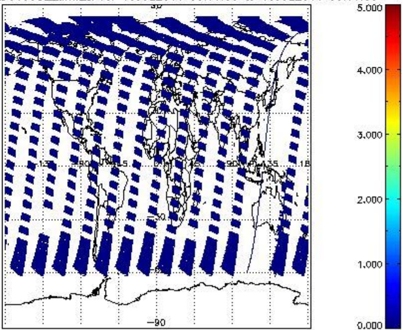
SCIOL2P_NADUV5S02_amf_cl for 15JUL2011 00:00:00 to 16JUL2011 00:00:00
