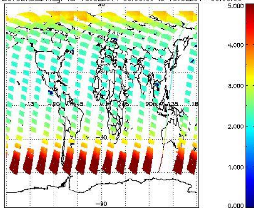
SCIOL2P_NADUV3BRO_amf_gr for 15JUL2011 00:00:00 to 16JUL2011 00:00:00
