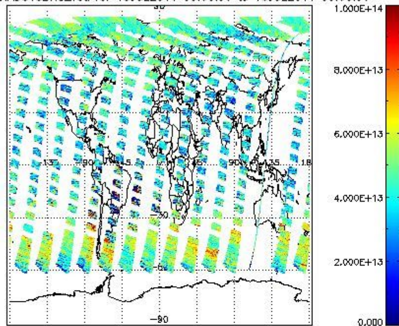
SCIOL2P_NADUV3BRO_vcd for 15JUL2011 00:00:00 to 16JUL2011 00:00:00
