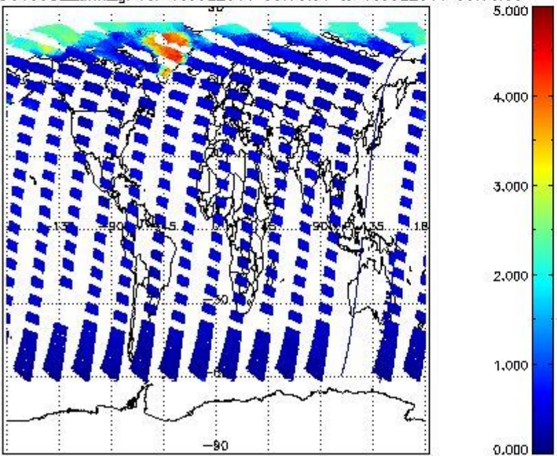
SCIOL2P_NADUV5S02_amf_gr for 15JUL2011 00:00:00 to 16JUL2011 00:00:00
