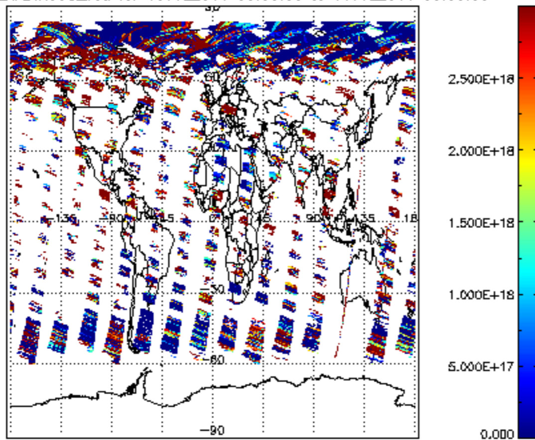
SCIOL2P_NADIR3CO_vcd for 15JUL2011 00:00:00 to 16JUL2011 00:00:00
