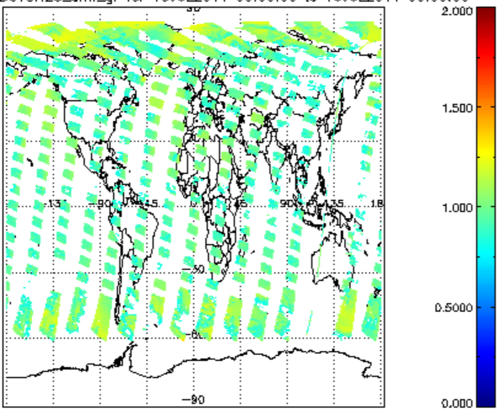
SCIOL2P_NADUV8H20_amf_gr for 15JUL2011 00:00:00 to 16JUL2011 00:00:00
