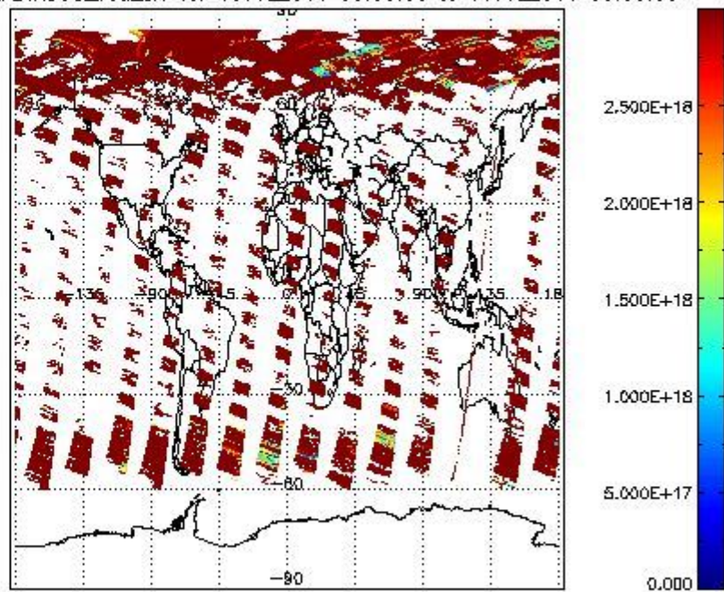
SCIDL2P_NADIR3CO_vcd_err for 15JUL2011 00:00:00 to 16JUL2011 00:00:00
