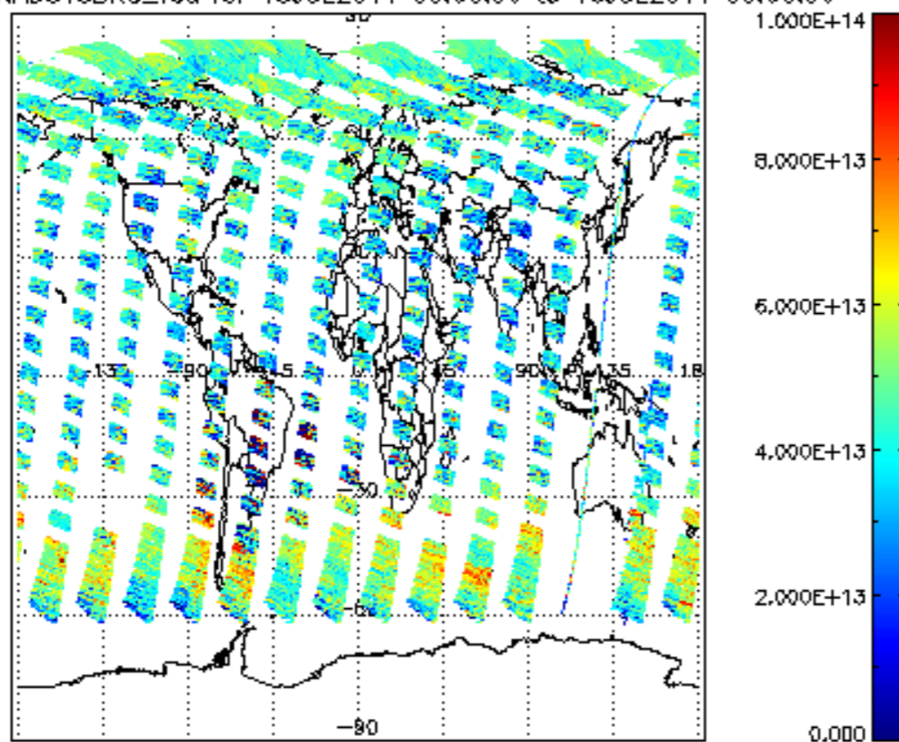
SCIOL2P_NADUV3BRO_vcd for 15JUL2011 00:00:00 to 16JUL2011 00:00:00
