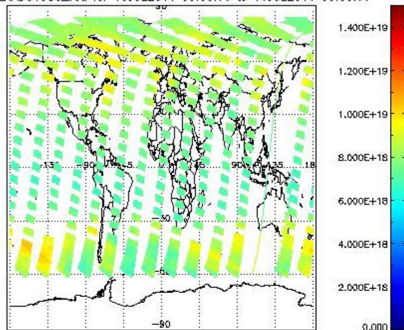
SCIOL2P_NADUV003_vcd for 15JUL2011 00:00:00 to 16JUL2011 00:00:00
