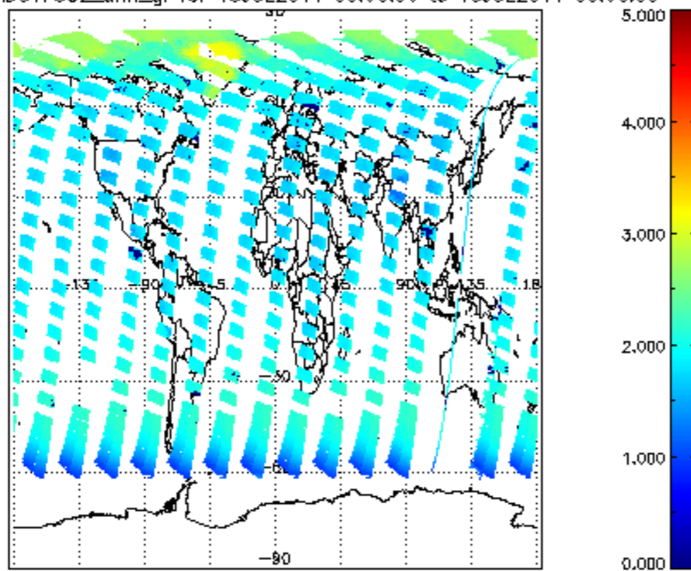
SCIOL2P_NADUV7S02_amf_gr for 15JUL2011 00:00:00 to 16JUL2011 00:00:00
