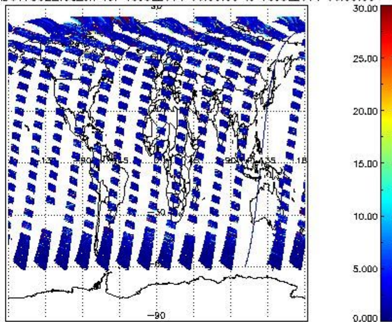
SCIOL2P_NADUV7S02_vcd_err for 15JUL2011 00:00:00 to 16JUL2011 00:00:00
