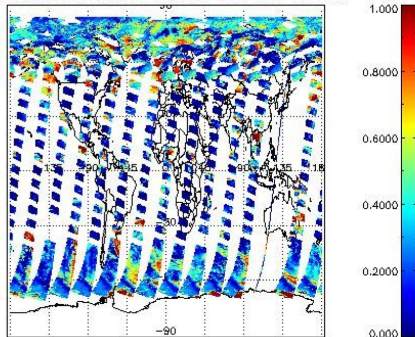
cL_frac for 15JUL2011 00:00:00 to 16JUL2011 00:00:00
