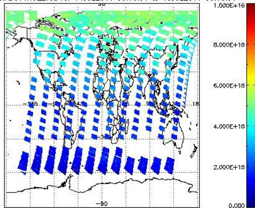
SCIOL2P_NADUV1NO2_vcd for 14JUL2011 00:00:00 to 15JUL2011 00:00:00
