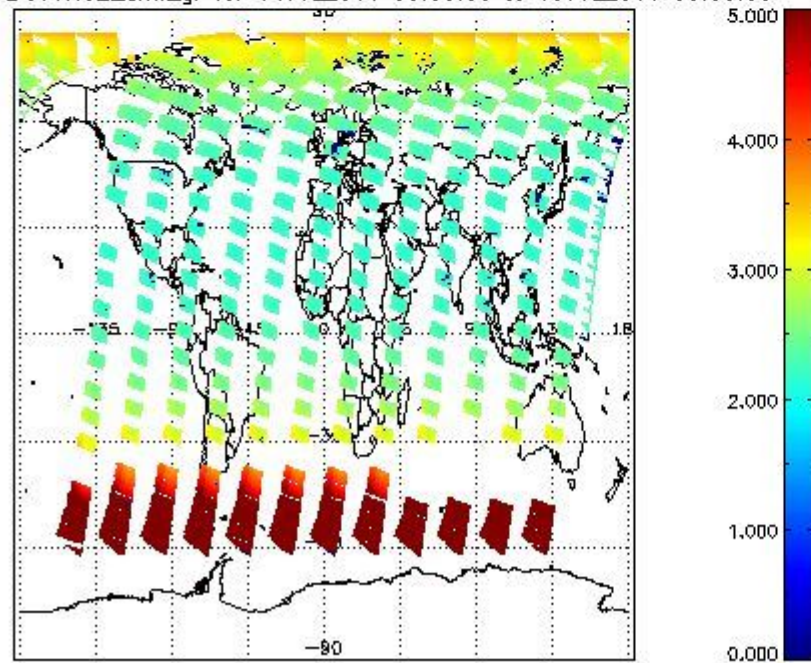
SCIOL2P_NADUV1NO2_amf_gr for 14JUL2011 00:00:00 to 15JUL2011 00:00:00
