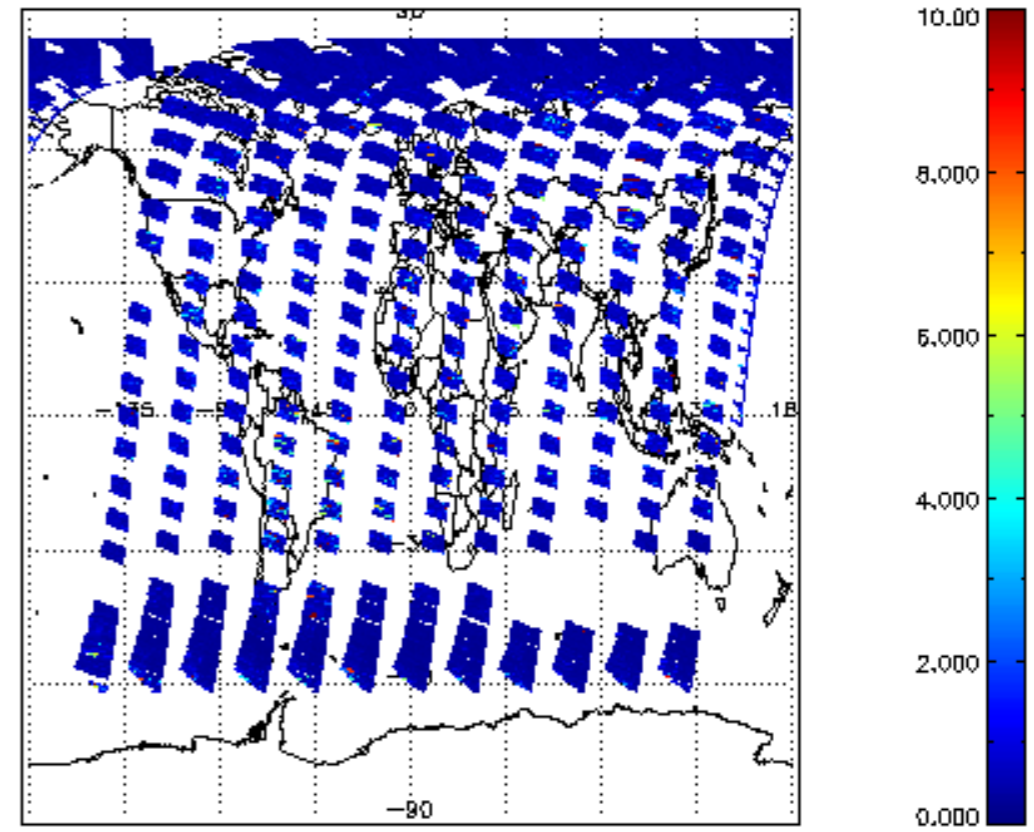
SCIOL2P_NADUV3BRO_vcd_err for 14JUL2011 00:00:00 to 15JUL2011 00:00:00
