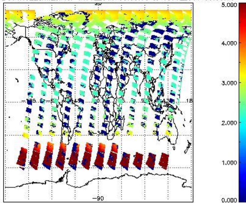
SCIOL2P_NADUV1NO2_amf_cl for 14JUL2011 00:00:00 to 15JUL2011 00:00:00
