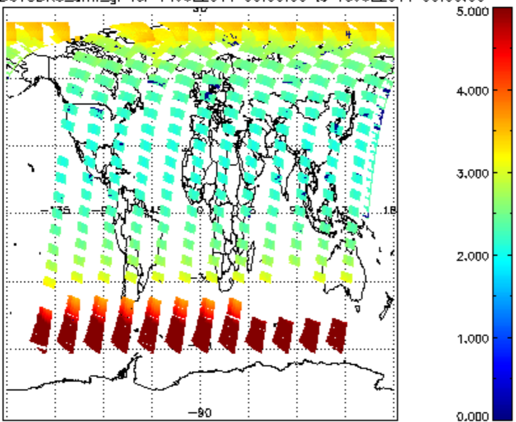
SCIOL2P_NADUV3BRO_amf_gr for 14JUL2011 00:00:00 to 15JUL2011 00:00:00
