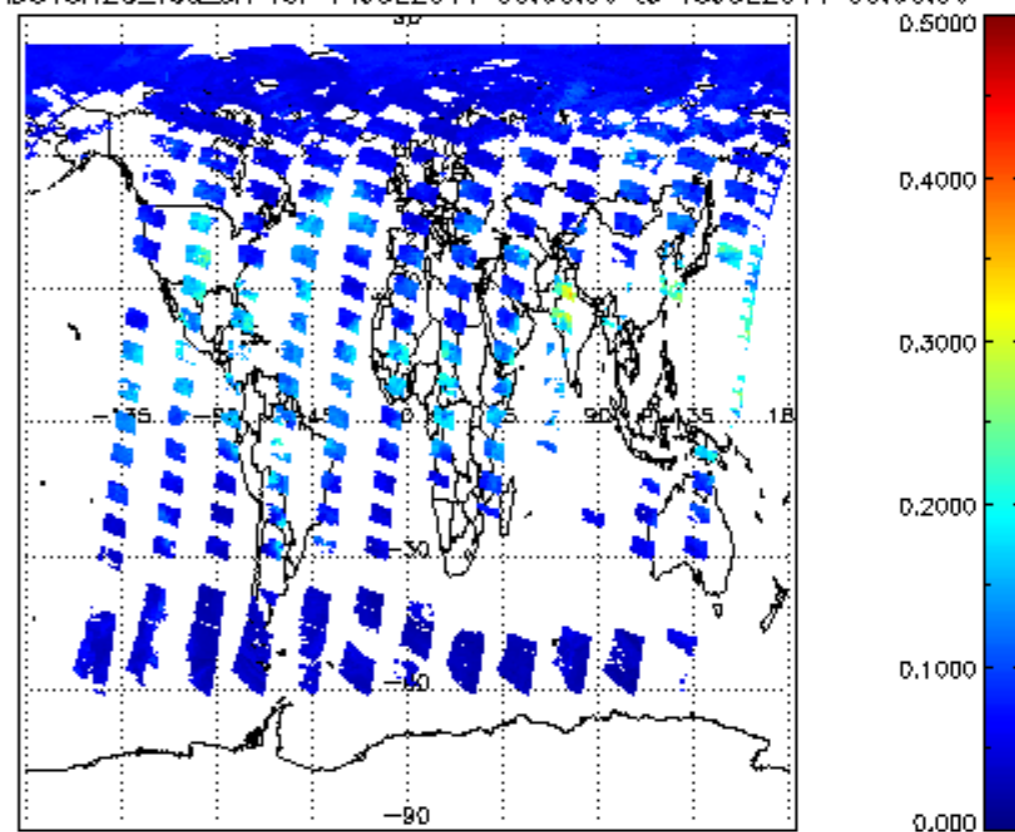
SCIOL2P_NADUV8H20_vcd_err for 14JUL2011 00:00:00 to 15JUL2011 00:00:00
