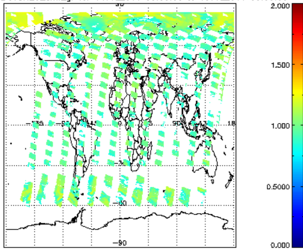
SCIOL2P_NADUV8H20_amf_gr for 14JUL2011 00:00:00 to 15JUL2011 00:00:00
