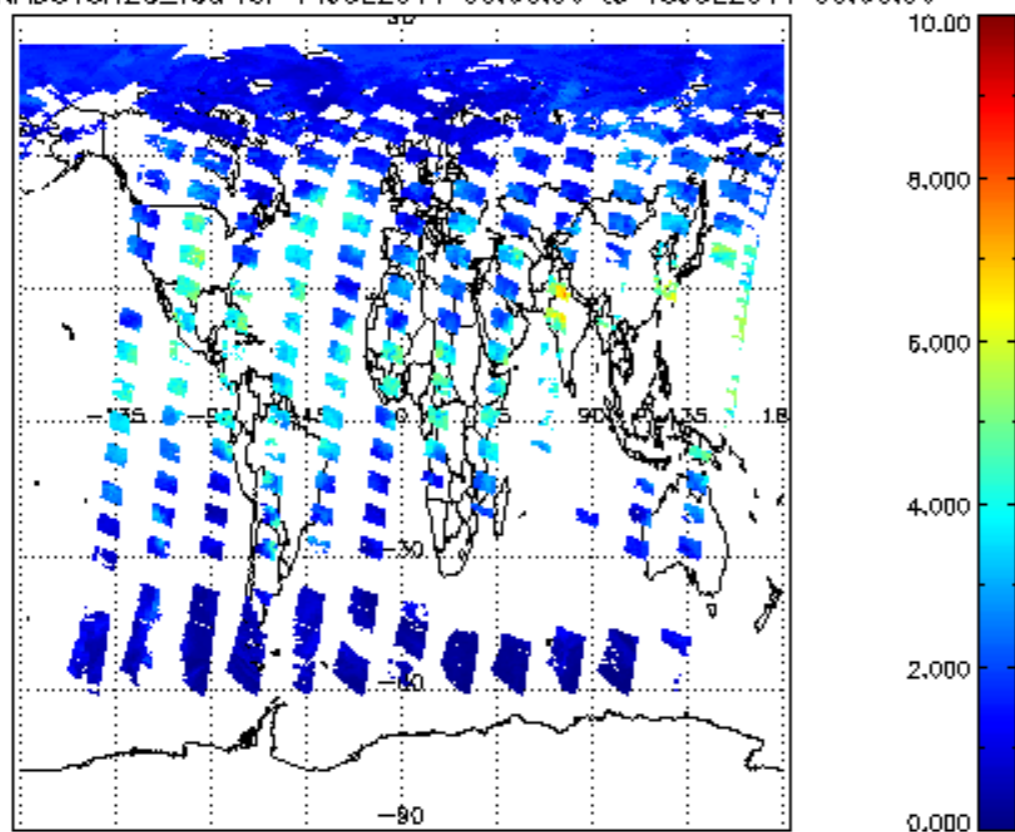
SCIOL2P_NADUV8H20_vcd for 14JUL2011 00:00:00 to 15JUL2011 00:00:00
