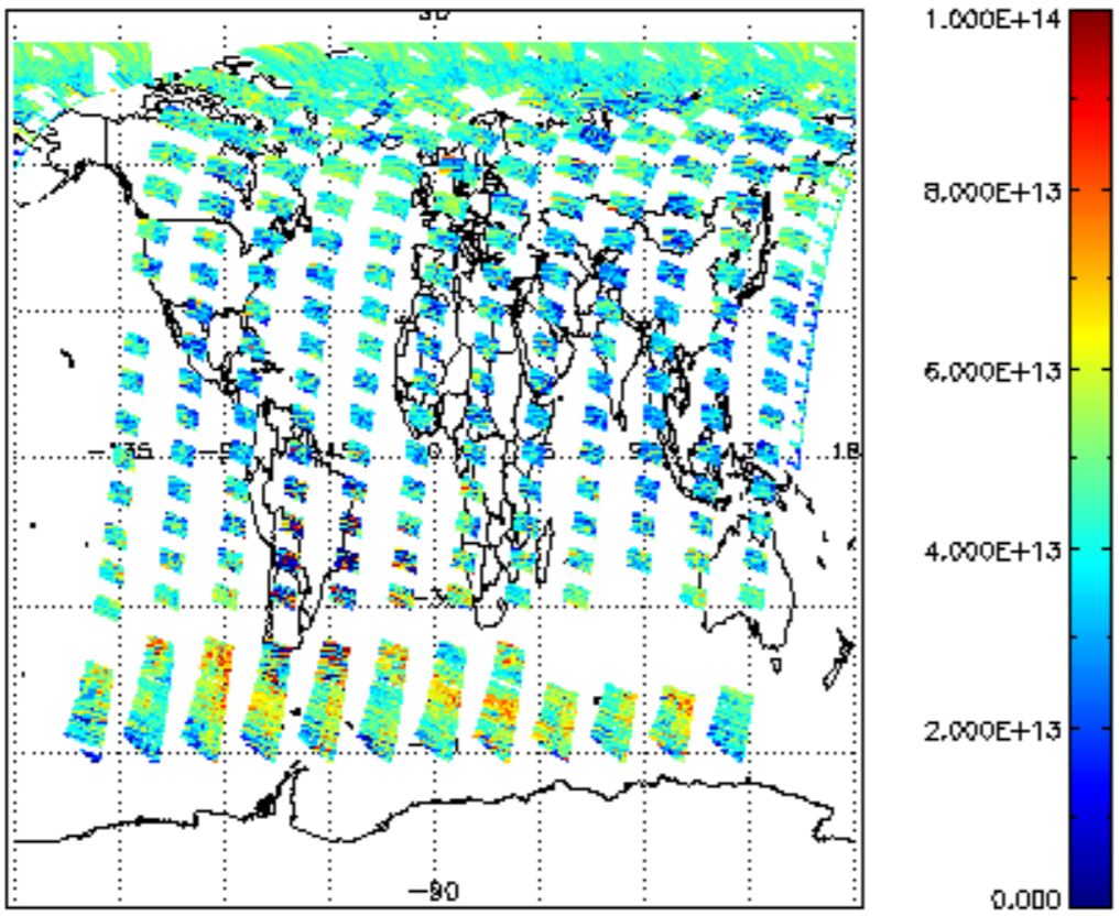
SCIOL2P_NADUV3BRO_vcd for 14JUL2011 00:00:00 to 15JUL2011 00:00:00
