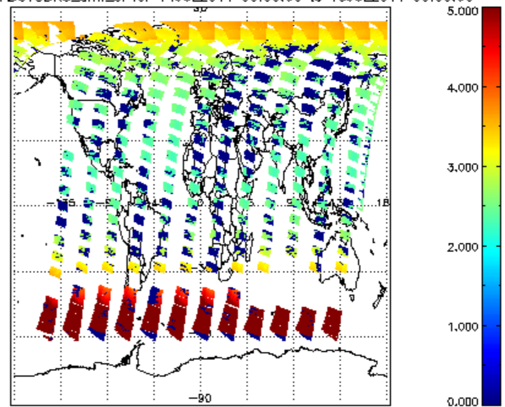
SCIOL2P_NADUV3BRO_amf_cl for 14JUL2011 00:00:00 to 15JUL2011 00:00:00
