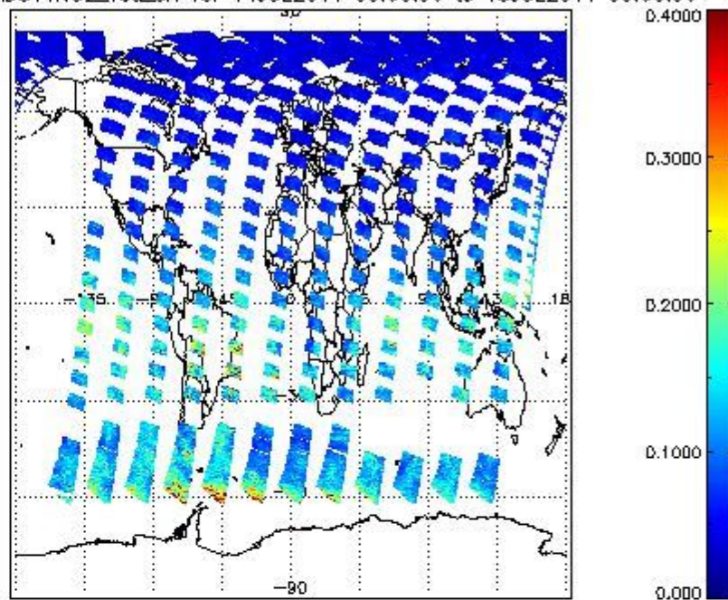
SCIOL2P_NADUV1NO2_vcd_err for 14JUL2011 00:00:00 to 15JUL2011 00:00:00
