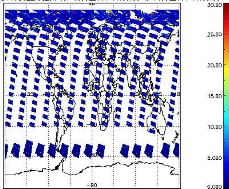
SCIOL2P_NADUV7S02_vcd_err for 13JUL2011 00:00:00 to 14JUL2011 00:00:00
