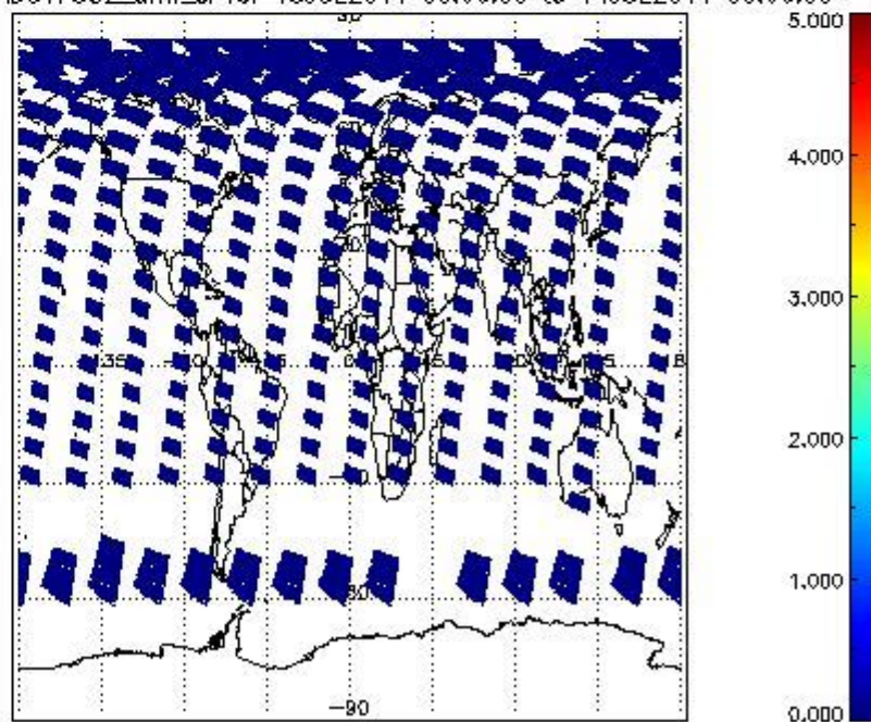
SCIOL2P_NADUV7S02_amf_cl for 13JUL2011 00:00:00 to 14JUL2011 00:00:00
