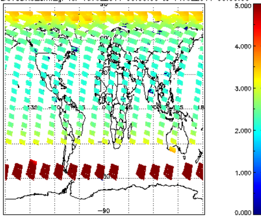
SCIOL2P_NADUV3BRO_arnf_gr for 13JUL2011 00:00:00 to 14JUL2011 00:00:00
