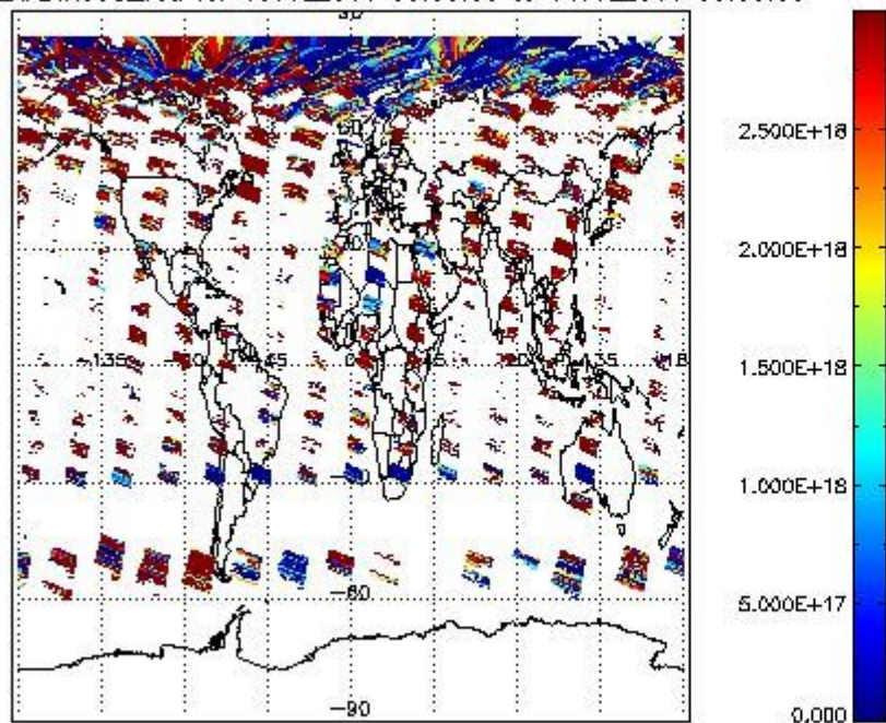
SCIDL2P_NADIR3CO_vcd for 13JUL2011 00:00:00 to 14JUL2011 00:00:00
