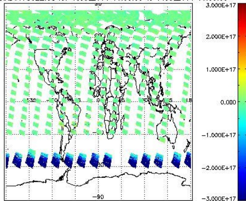
SCIOL2P_NADUV7S02_vcd for 13JUL2011 00:00:00 to 14JUL2011 00:00:00
