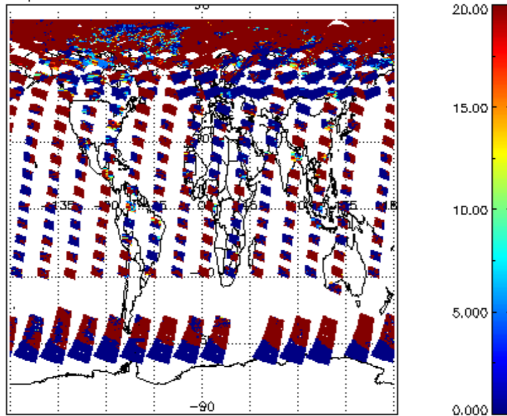
cl_lopt_depth for 13JUL2011 00:00:00 to 14JUL2011 00:00:00
