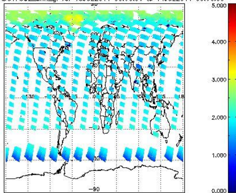
SCIOL2P_NADUV7S02_amf_gr for 13JUL2011 00:00:00 to 14JUL2011 00:00:00
