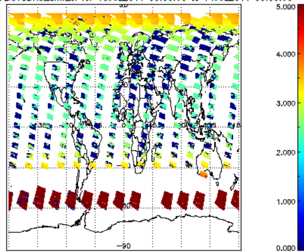
SCIOL2P_NADUV3BRO_arnf_cl for 13JUL2011 00:00:00 to 14JUL2011 00:00:00
