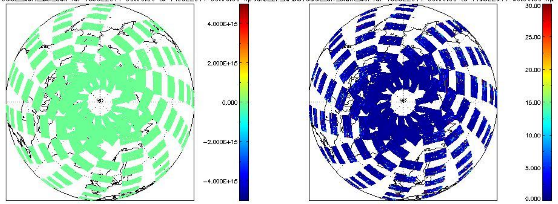
SCIOI2P_NADUV6OCLslant_col_den for 13JUL2011 00:00:00 to 14JUL2011 00:00:00 np SCIOI2P_NADUV6OCLlarr_slant_col for 13JUL2011 00:00:00 to 14JUL2011 00:00:00 np
