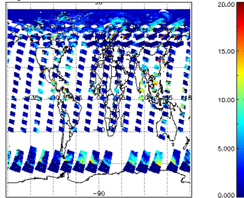
cl_top_height for 13JUL2011 00:00:00 to 14JUL2011 00:00:00
