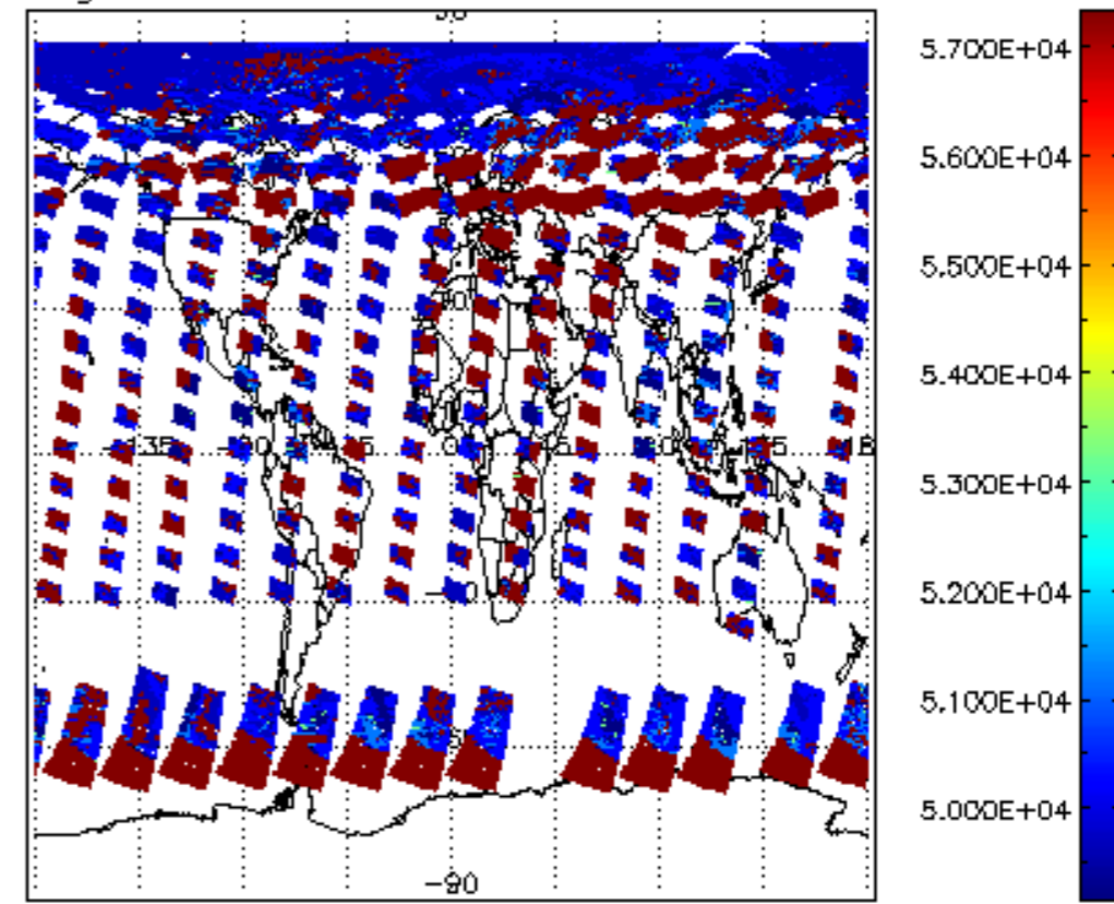
cloud_flags for 13JUL2011 00:00:00 to 14JUL2011 00:00:00
