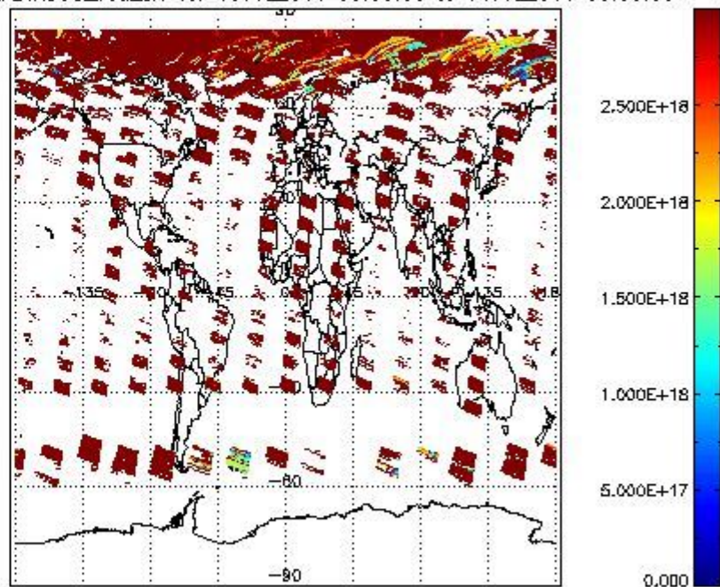
SCIDL2P_NADIR3CO_vcd_err for 13JUL2011 00:00:00 to 14JUL2011 00:00:00
