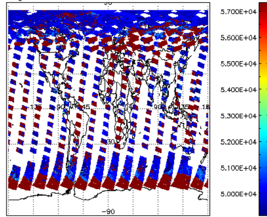
cloud_flags for 12JUL2011 00:00:00 to 13JUL2011 00:00:00
