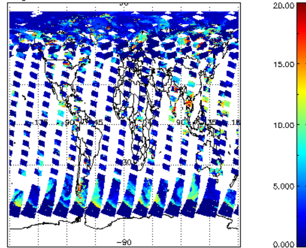
cl_top_height for 12JUL2011 00:00:00 to 13JUL2011 00:00:00
