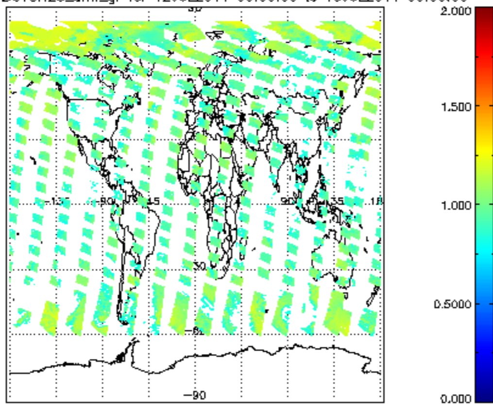
SCIOL2P_NADUV8H2O_amf_gr for 12JUL2011 00:00:00 to 13JUL2011 00:00:00
