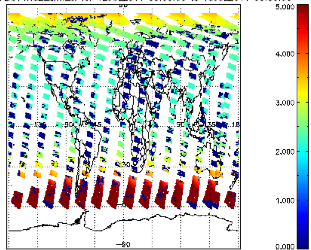
SCIOL2P_NADUV1NO2_amf_cl for 12JUL2011 00:00:00 to 13JUL2011 00:00:00
