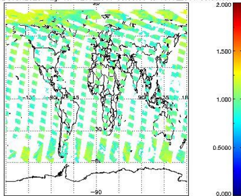
SCIOL2P_NADUV8H2O_amf_gr for 12JUL2011 00:00:00 to 13JUL2011 00:00:00
