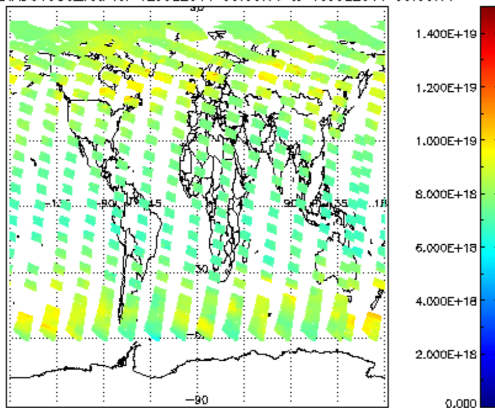
SCIOL2P_NADUV003_vcd for 12JUL2011 00:00:00 to 13JUL2011 00:00:00
