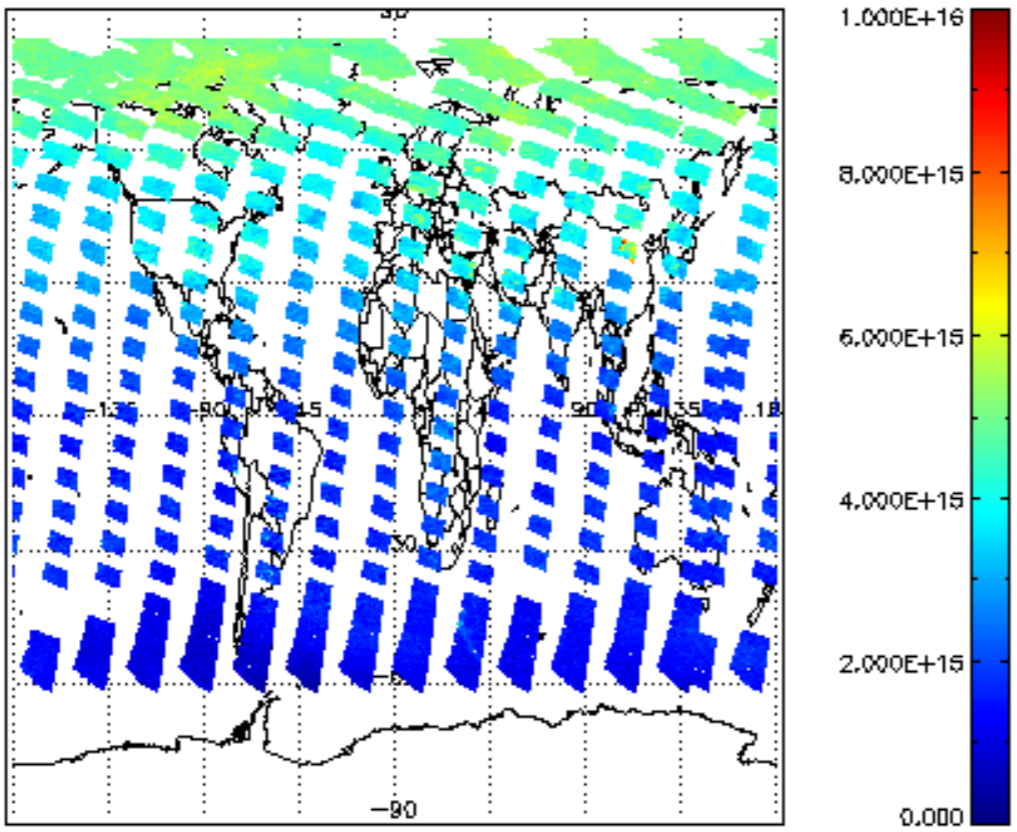
SCIOL2P_NADUV1NO2_vcd for 12JUL2011 00:00:00 to 13JUL2011 00:00:00
