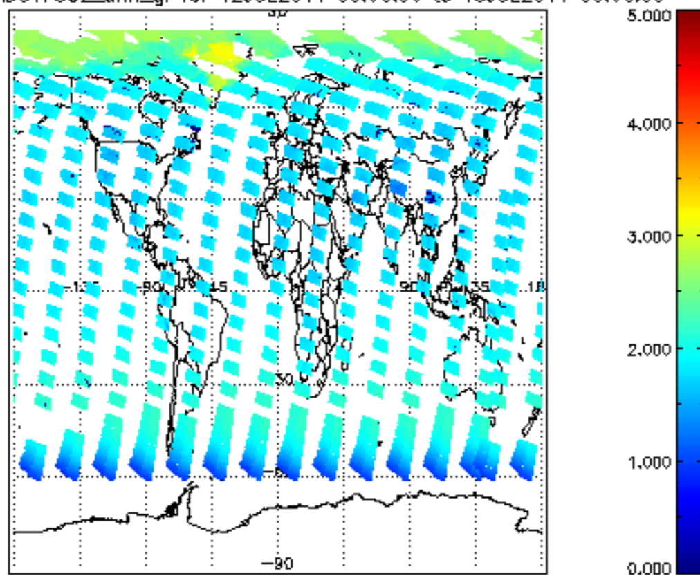
SCIOL2P_NADUV7S02_amf_gr for 12JUL2011 00:00:00 to 13JUL2011 00:00:00
