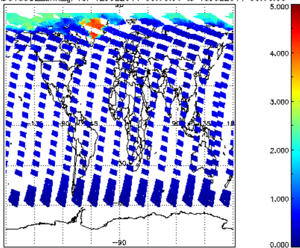
SCIOL2P_NADUV5S02_amf_gr for 12JUL2011 00:00:00 to 13JUL2011 00:00:00
