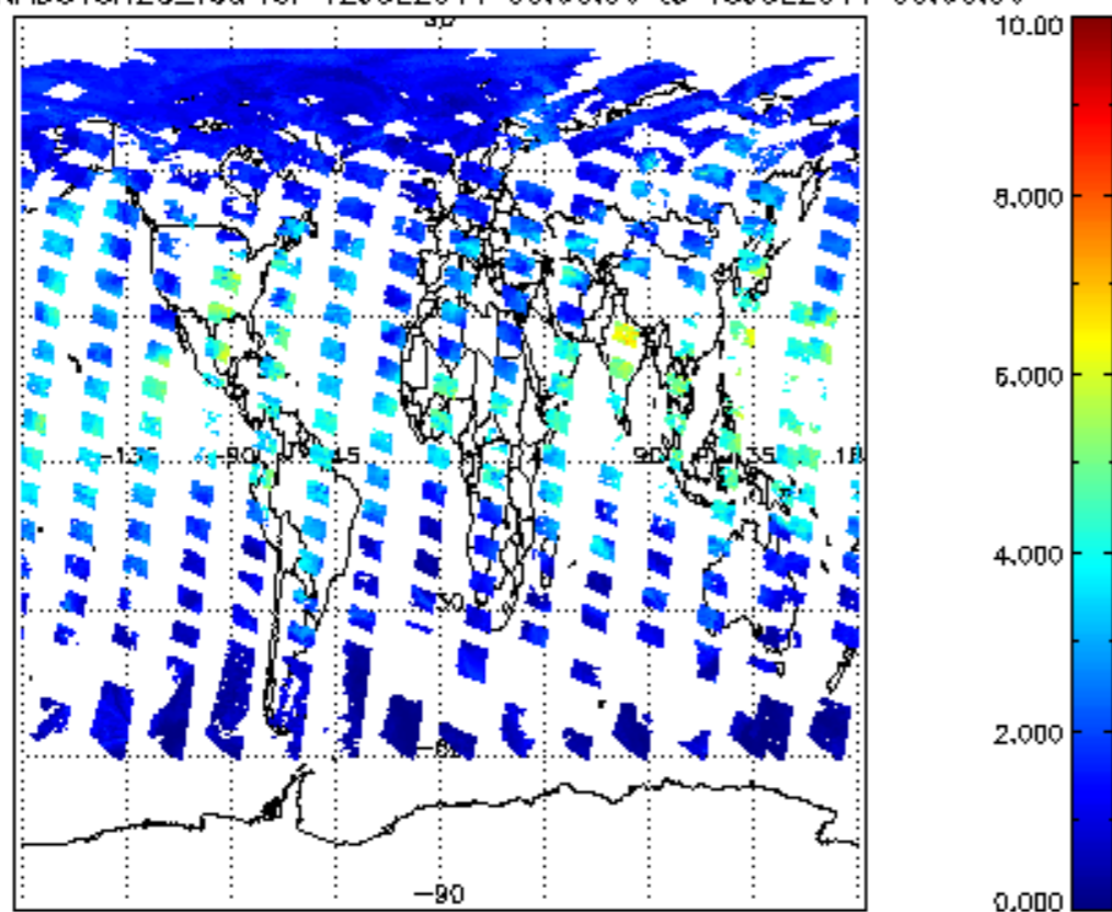
SCIOL2P_NADUV8H2O_vcd for 12JUL2011 00:00:00 to 13JUL2011 00:00:00
