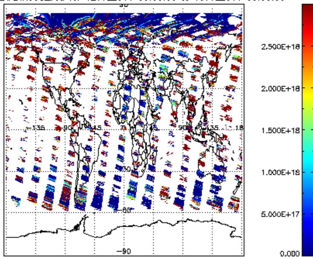
SCIOL2P_NADIR3CO_vcd for 12JUL2011 00:00:00 to 13JUL2011 00:00:00
