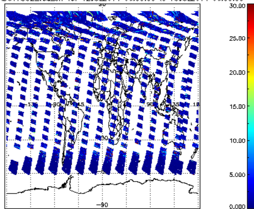
SCIOL2P_NADUV7S02_vcd_err for 12JUL2011 00:00:00 to 13JUL2011 00:00:00
