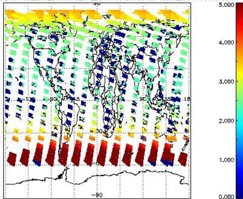
SCIOL2P_NADUV003_amf_cl for 12JUL2011 00:00:00 to 13JUL2011 00:00:00
