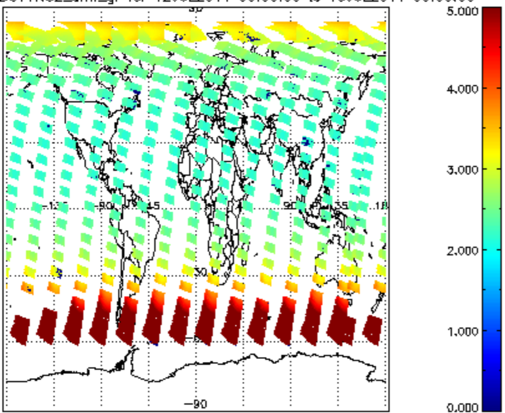
SCIOL2P_NADUV1NO2_amf_gr for 12JUL2011 00:00:00 to 13JUL2011 00:00:00
