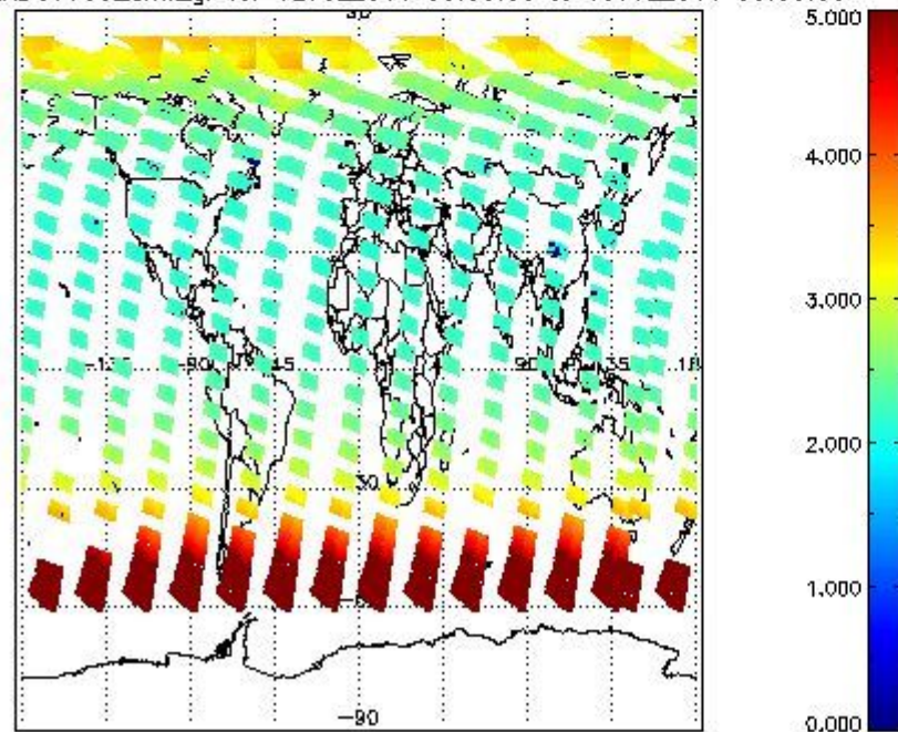
SCIOL2P_NADUV003_amf_gr for 12JUL2011 00:00:00 to 13JUL2011 00:00:00
