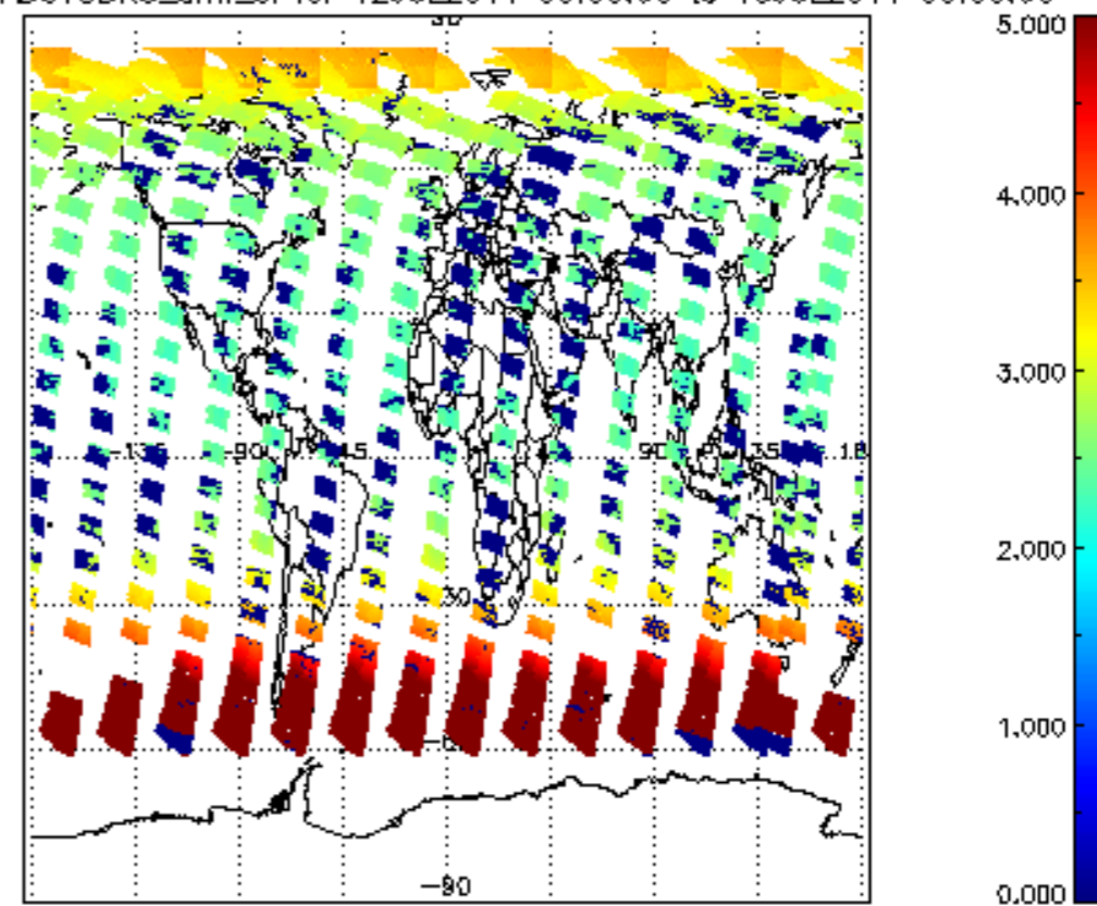
SCIOL2P_NADUV3BRO_amf_cl for 12JUL2011 00:00:00 to 13JUL2011 00:00:00
