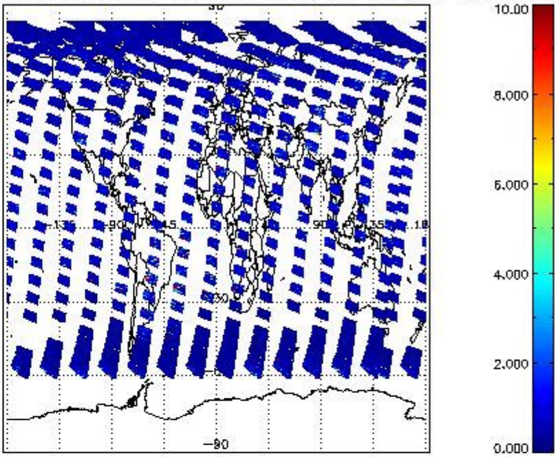
SCIOL2P_NADUV3BRO_vcd_err for 12JUL2011 00:00:00 to 13JUL2011 00:00:00
