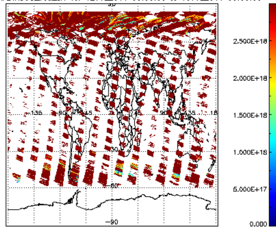
SCIOL2P_NADIR3CO_vcd_err for 12JUL2011 00:00:00 to 13JUL2011 00:00:00
