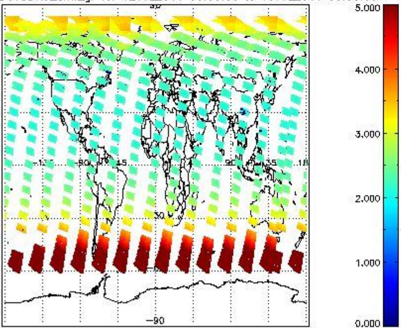
SCIOL2P_NADUV3BRO_amf_gr for 12JUL2011 00:00:00 to 13JUL2011 00:00:00
