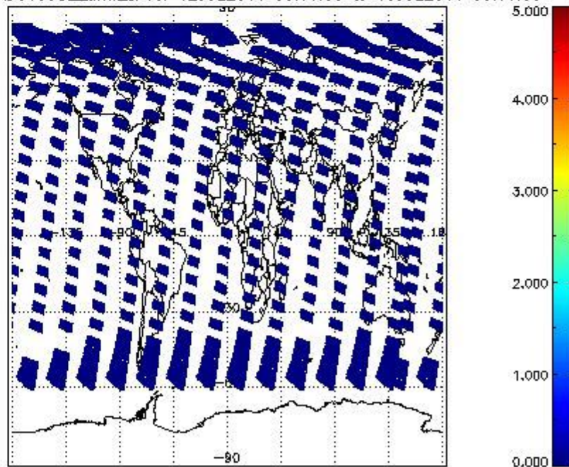
SCIOL2P_NADUV5S02_amf_cl for 12JUL2011 00:00:00 to 13JUL2011 00:00:00
