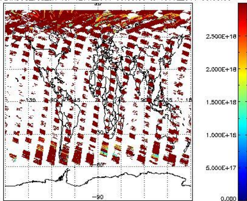
SCIDL2P_NADIR3CO_vcd_err for 12JUL2011 00:00:00 to 13JUL2011 00:00:00
