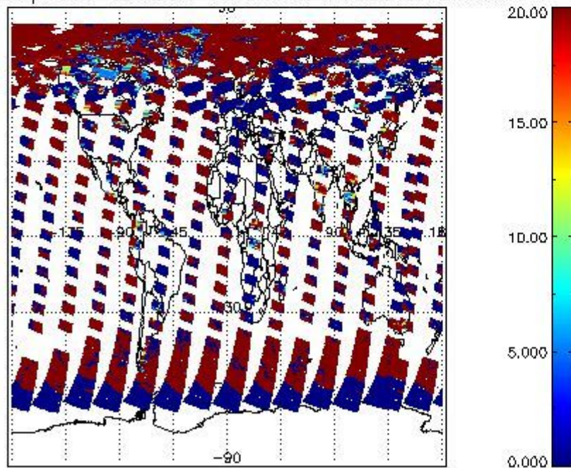
cL_opt_depth for 12JUL2011 00:00:00 to 13JUL2011 00:00:00
