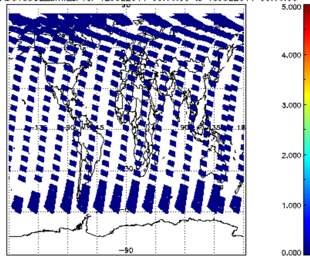
SCIOL2P_NADUV5S02_amf_cl for 12JUL2011 00:00:00 to 13JUL2011 00:00:00
