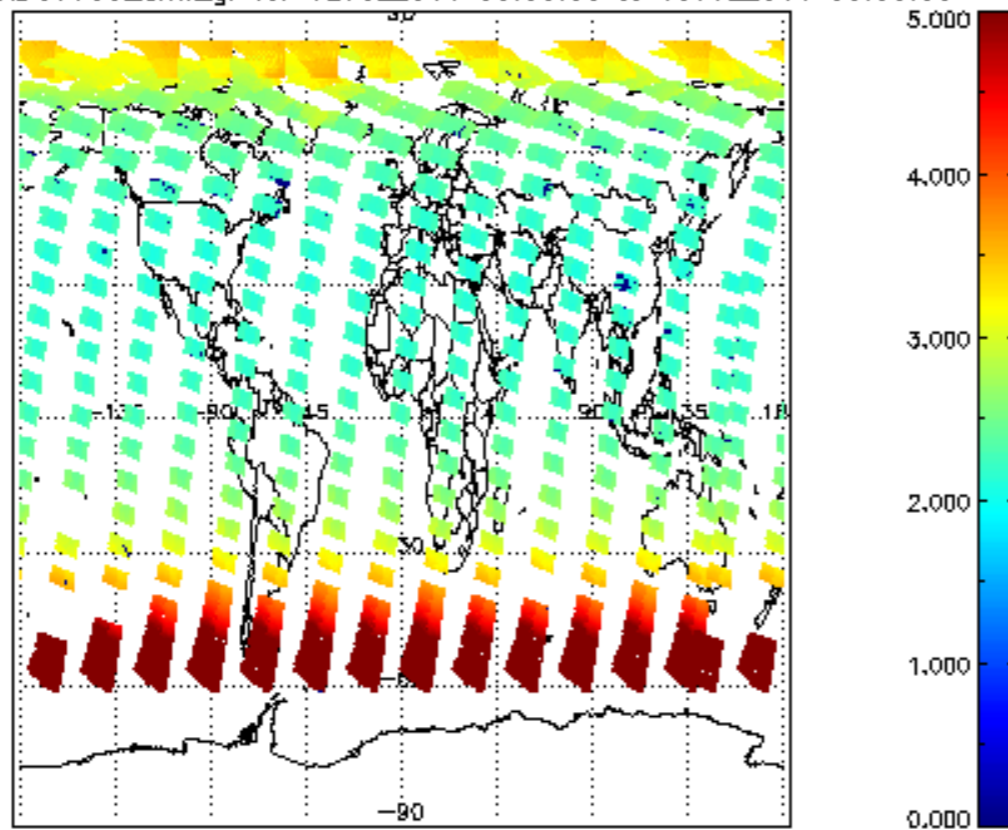
SCIOL2P_NADUV003_amf_gr for 12JUL2011 00:00:00 to 13JUL2011 00:00:00
