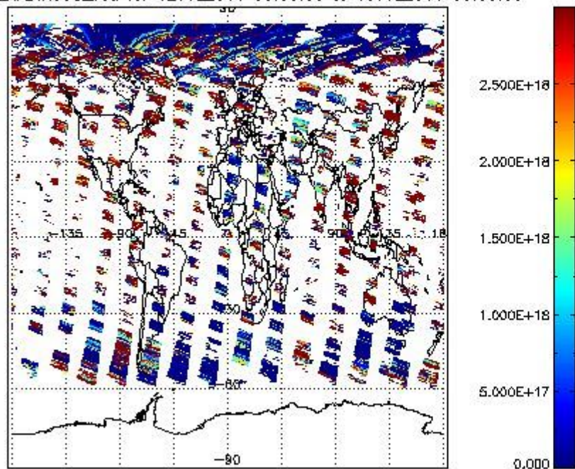
SCIDL2P_NADIR3CO_vcd for 12JUL2011 00:00:00 to 13JUL2011 00:00:00
