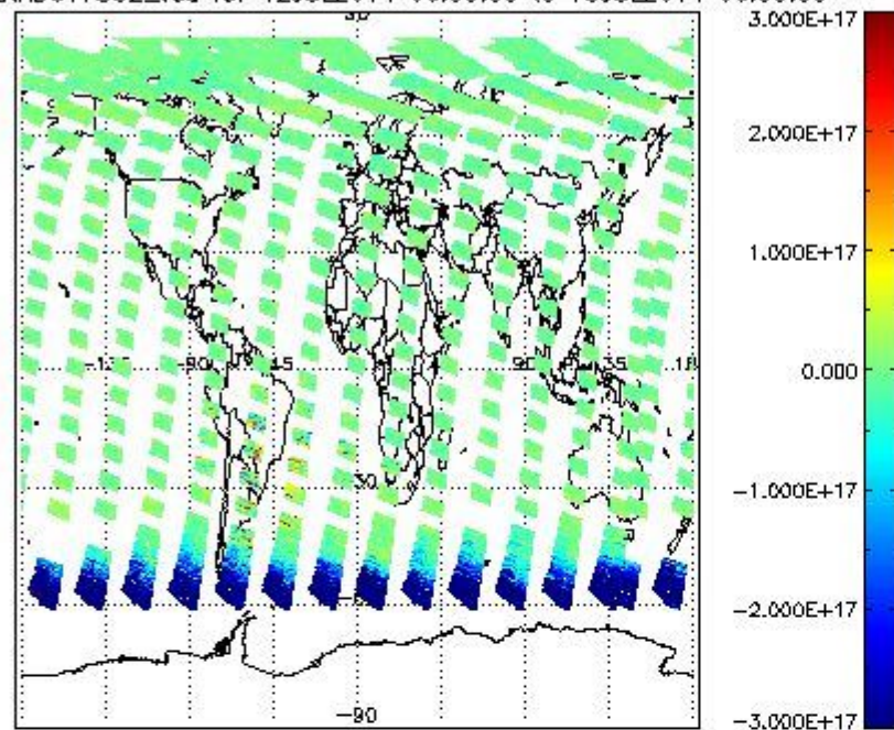
SCIOL2P_NADUV7S02_vcd for 12JUL2011 00:00:00 to 13JUL2011 00:00:00
