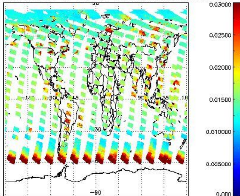
SCIOL2P_NADUV003_vcd_err for 12JUL2011 00:00:00 to 13JUL2011 00:00:00
