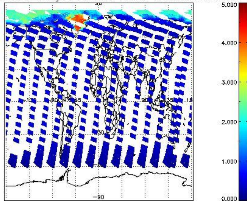
SCIOL2P_NADUV5S02_amf_gr for 12JUL2011 00:00:00 to 13JUL2011 00:00:00
