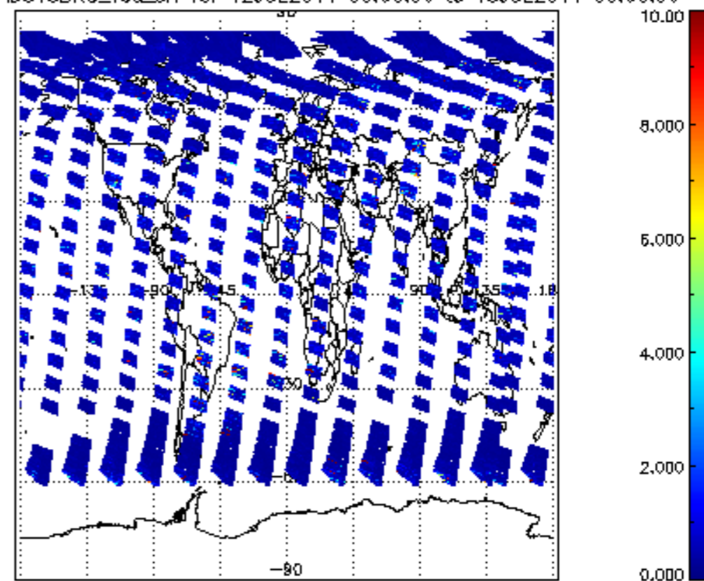
SCIOL2P_NADUV3BRO_vcd_err for 12JUL2011 00:00:00 to 13JUL2011 00:00:00
