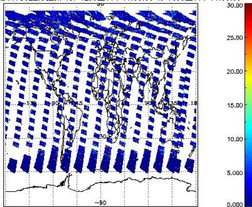
SCIOL2P_NADUV7S02_vcd_err for 12JUL2011 00:00:00 to 13JUL2011 00:00:00
