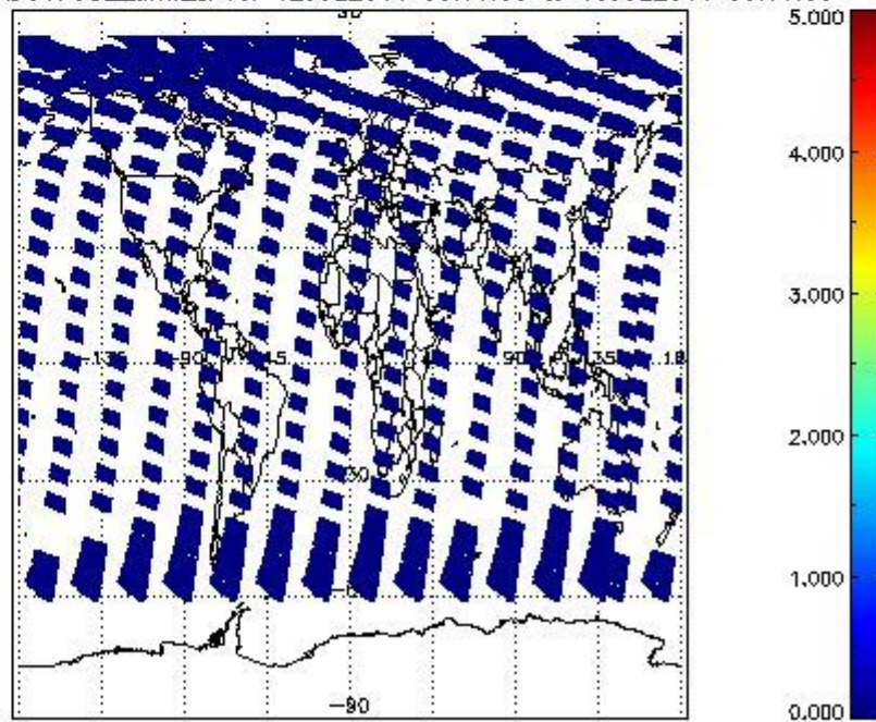
SCIOL2P_NADUV7S02_amf_cl for 12JUL2011 00:00:00 to 13JUL2011 00:00:00
