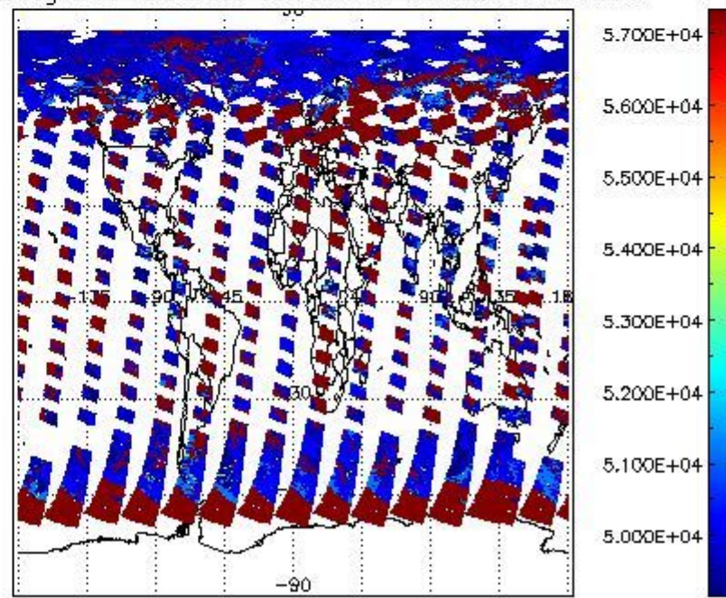
cloud_flags for 12JUL2011 00:00:00 to 13JUL2011 00:00:00
