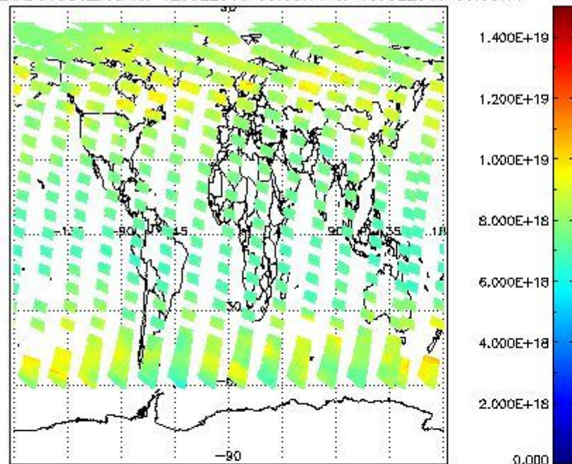
SCIOL2P_NADUV003_vcd for 12JUL2011 00:00:00 to 13JUL2011 00:00:00
