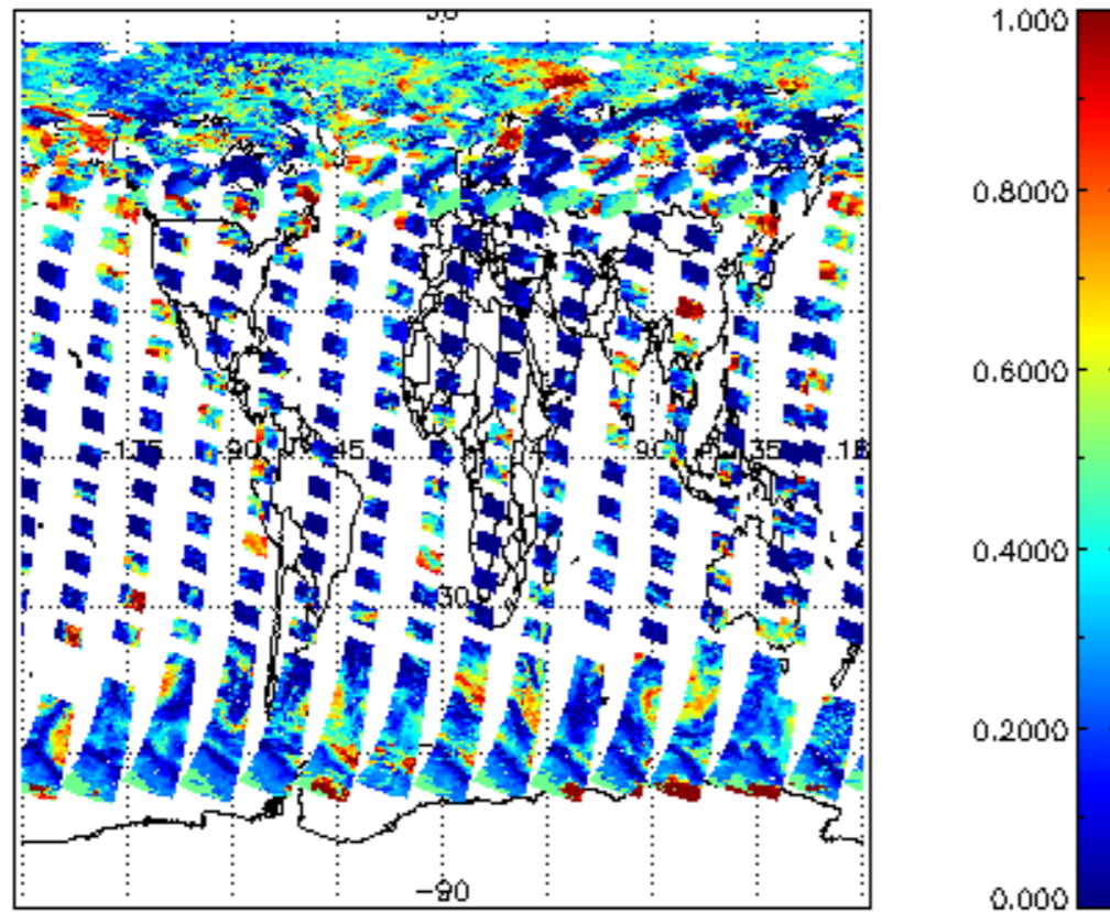
cl_frac for 12JUL2011 00:00:00 to 13JUL2011 00:00:00
