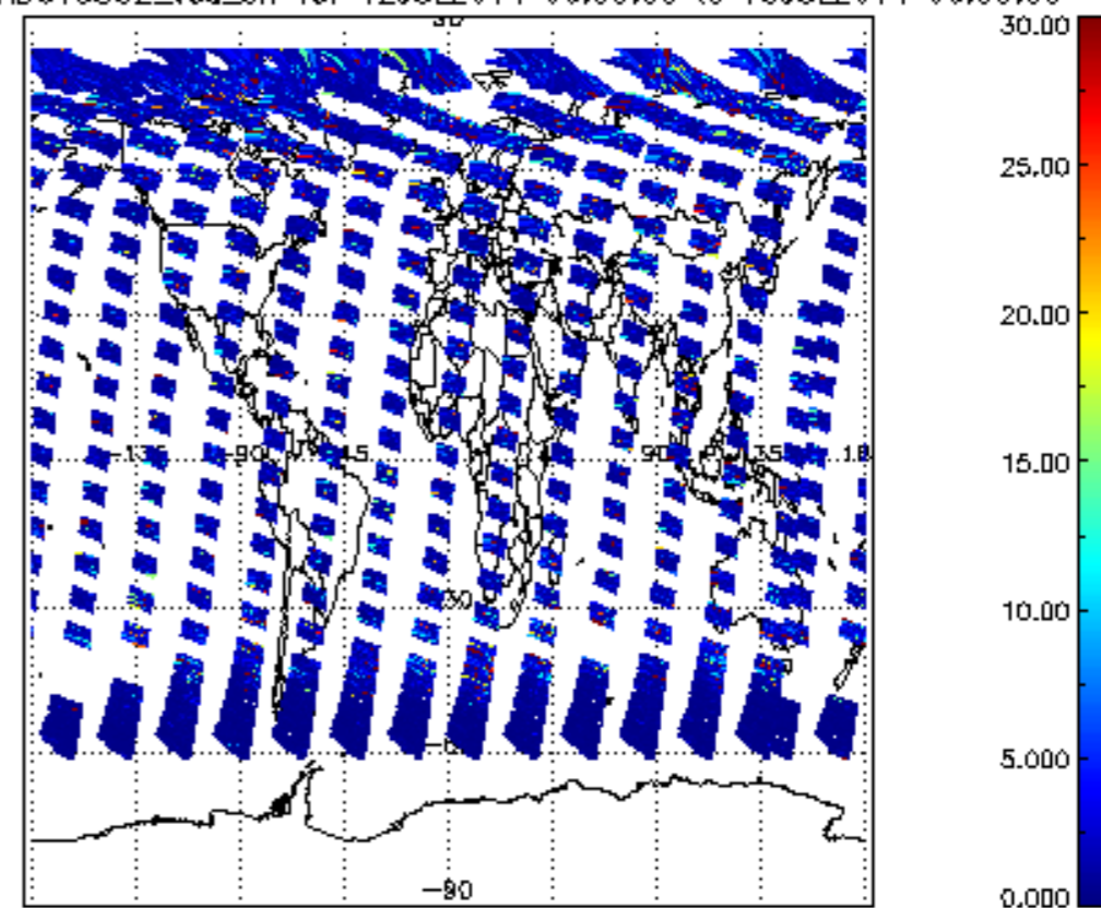
SCIOL2P_NADUV5S02_vcd_err for 12JUL2011 00:00:00 to 13JUL2011 00:00:00
