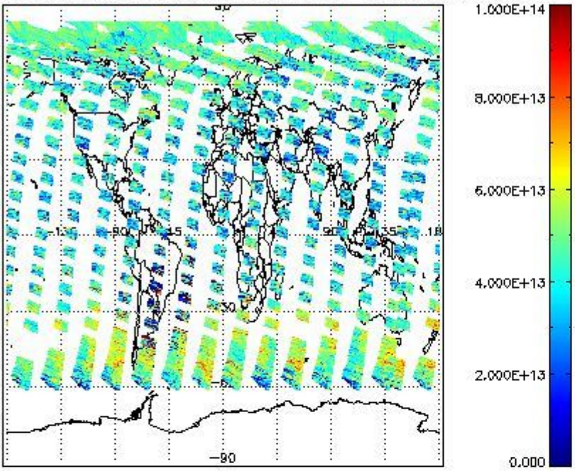
SCIOL2P_NADUV3BRO_vcd for 12JUL2011 00:00:00 to 13JUL2011 00:00:00
