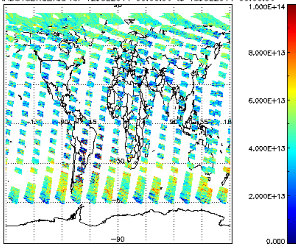
SCIOL2P_NADUV3BRO_vcd for 12JUL2011 00:00:00 to 13JUL2011 00:00:00
