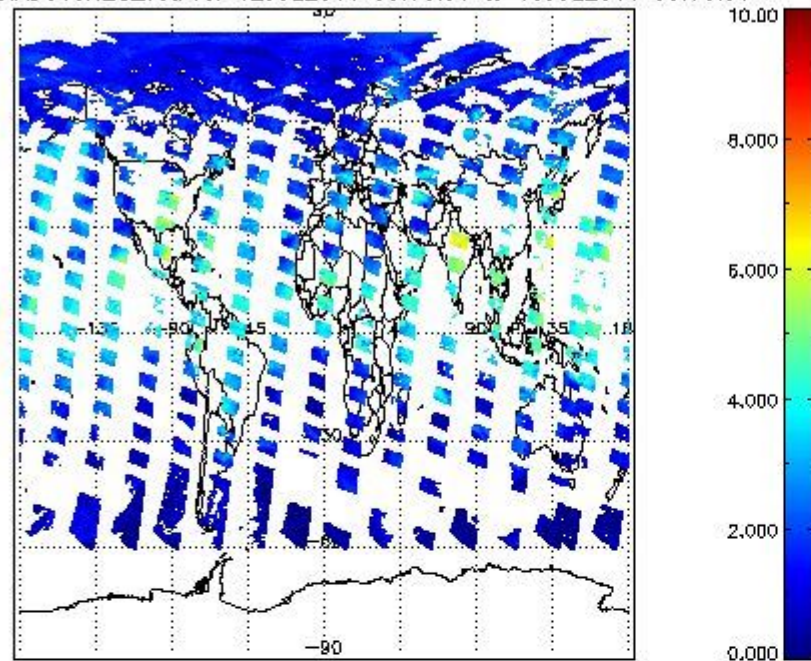
SCIOL2P_NADUV8H2O_vcd for 12JUL2011 00:00:00 to 13JUL2011 00:00:00
