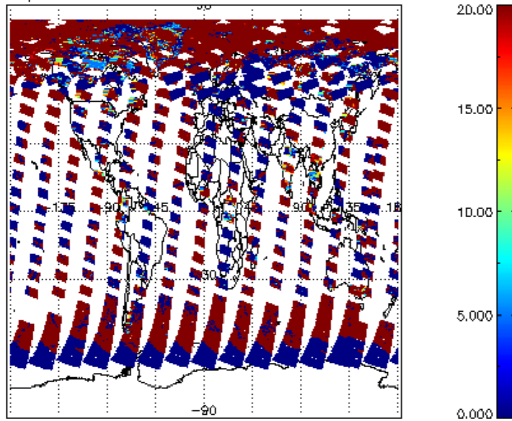
cl_opt_depth for 12JUL2011 00:00:00 to 13JUL2011 00:00:00
