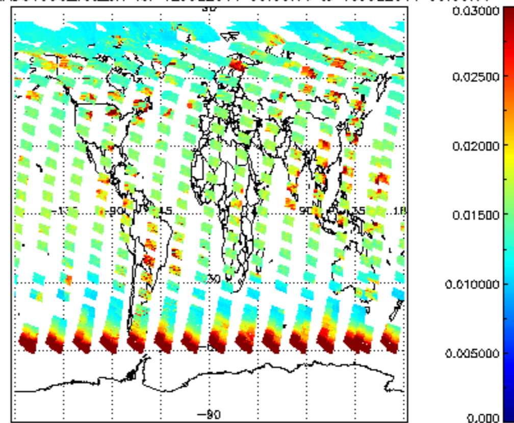
SCIOL2P_NADUV003_vcd_err for 12JUL2011 00:00:00 to 13JUL2011 00:00:00
