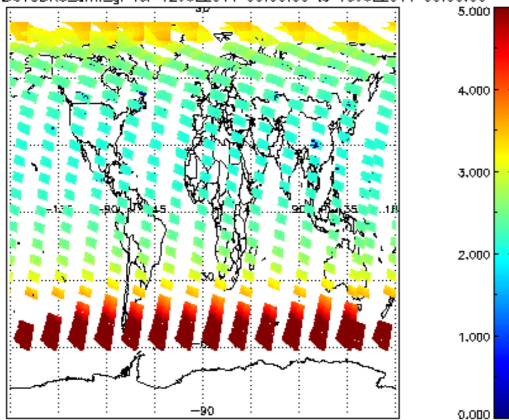
SCIOL2P_NADUV3BRO_amf_gr for 12JUL2011 00:00:00 to 13JUL2011 00:00:00
