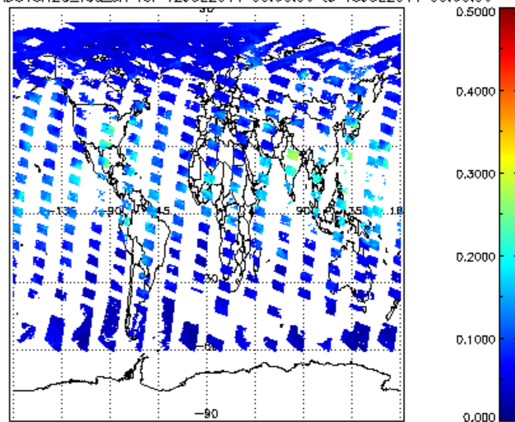
SCIOL2P_NADUV8H2O_vcd_err for 12JUL2011 00:00:00 to 13JUL2011 00:00:00
