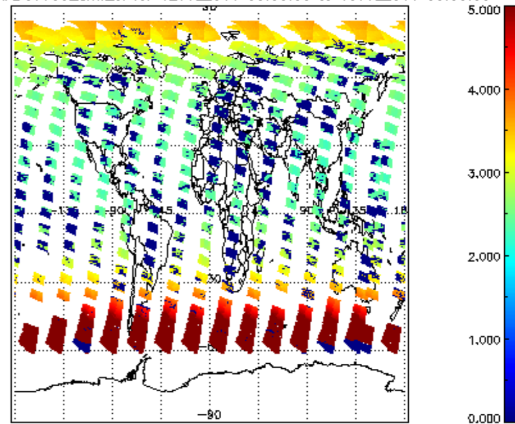
SCIOL2P_NADUV003_amf_cl for 12JUL2011 00:00:00 to 13JUL2011 00:00:00
