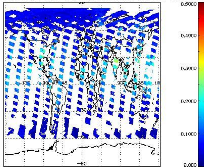
SCIOL2P_NADUV8H2O_vcd_err for 12JUL2011 00:00:00 to 13JUL2011 00:00:00
