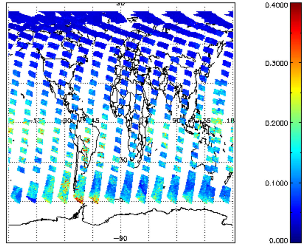
SCIOL2P_NADUV1NO2_vcd_err for 12JUL2011 00:00:00 to 13JUL2011 00:00:00
