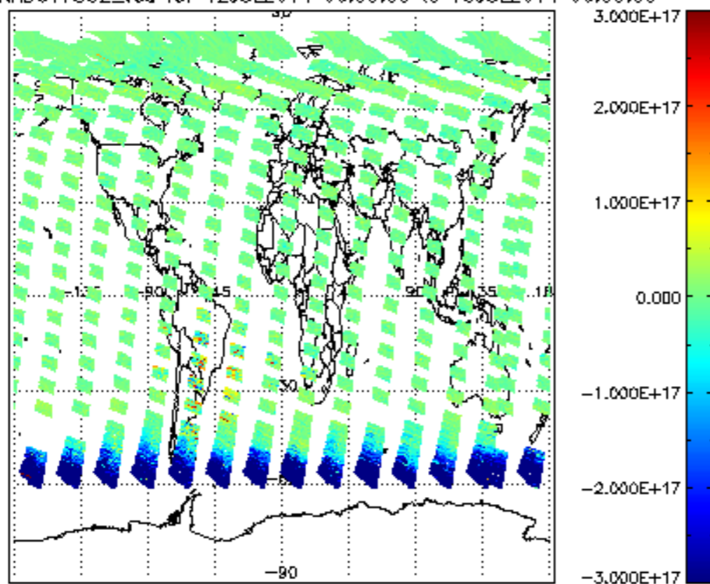
SCIOL2P_NADUV7S02_vcd for 12JUL2011 00:00:00 to 13JUL2011 00:00:00
