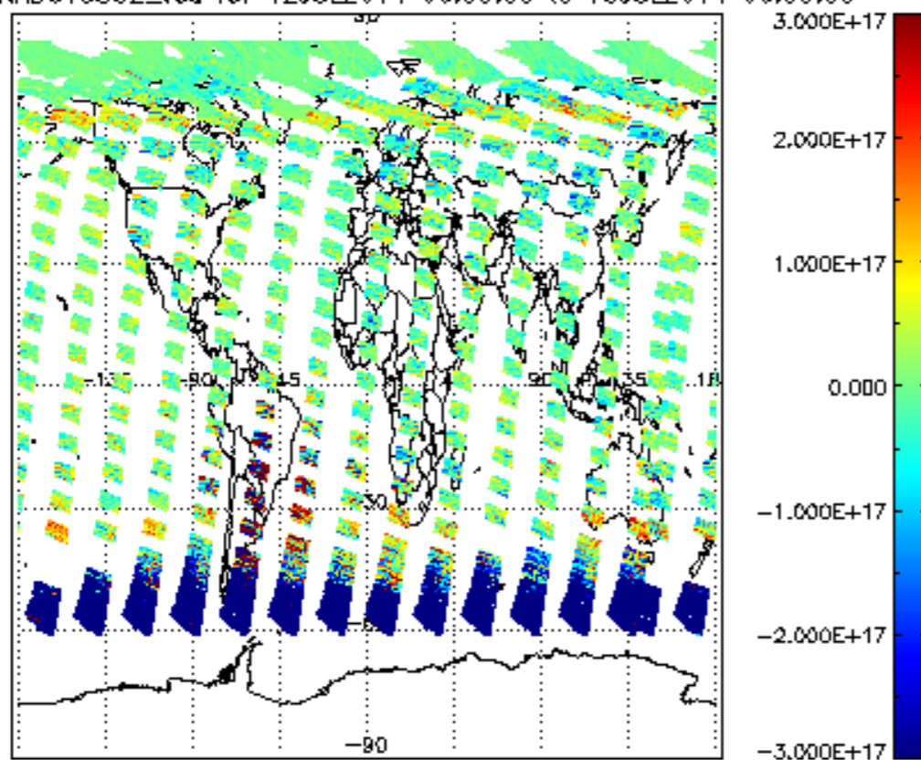
SCIOL2P_NADUV5S02_vcd for 12JUL2011 00:00:00 to 13JUL2011 00:00:00
