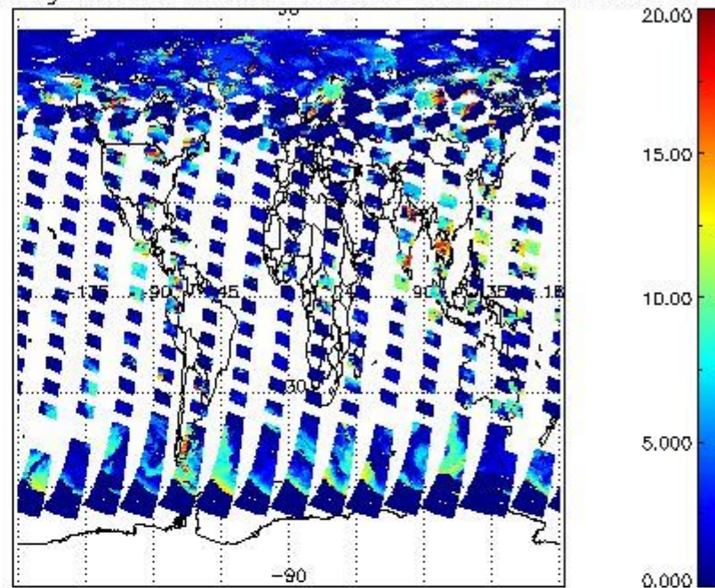
cL_top_height for 12JUL2011 00:00:00 to 13JUL2011 00:00:00
