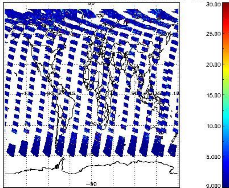
SCIOL2P_NADUV5S02_vcd_err for 12JUL2011 00:00:00 to 13JUL2011 00:00:00
