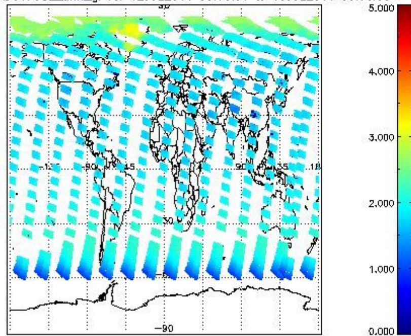
SCIOL2P_NADUV7S02_amf_gr for 12JUL2011 00:00:00 to 13JUL2011 00:00:00
