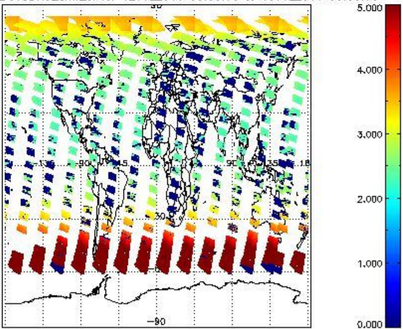
SCIOL2P_NADUV3BRO_amf_cl for 12JUL2011 00:00:00 to 13JUL2011 00:00:00
