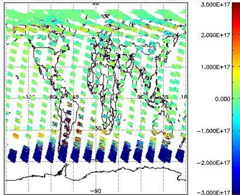
SCIOL2P_NADUV5S02_vcd for 12JUL2011 00:00:00 to 13JUL2011 00:00:00
