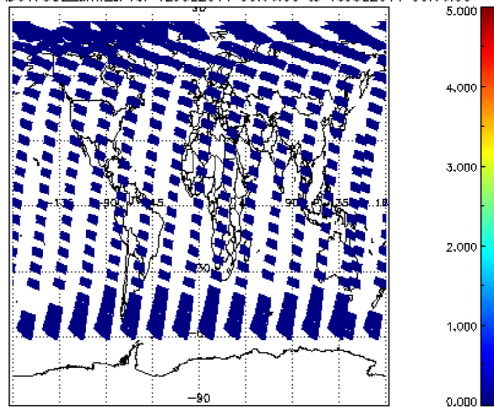
SCIOL2P_NADUV7S02_amf_cl for 12JUL2011 00:00:00 to 13JUL2011 00:00:00
