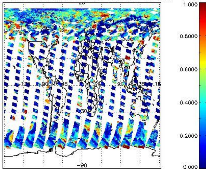
cL_frac for 12JUL2011 00:00:00 to 13JUL2011 00:00:00
